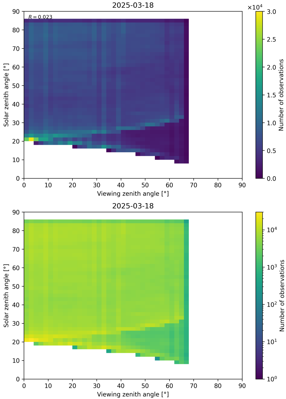
Figure 77: Scatter density plot of “Viewing zenith angle” against “Solar zenith angle” for 2025-03-17 to 2025-03-19.
