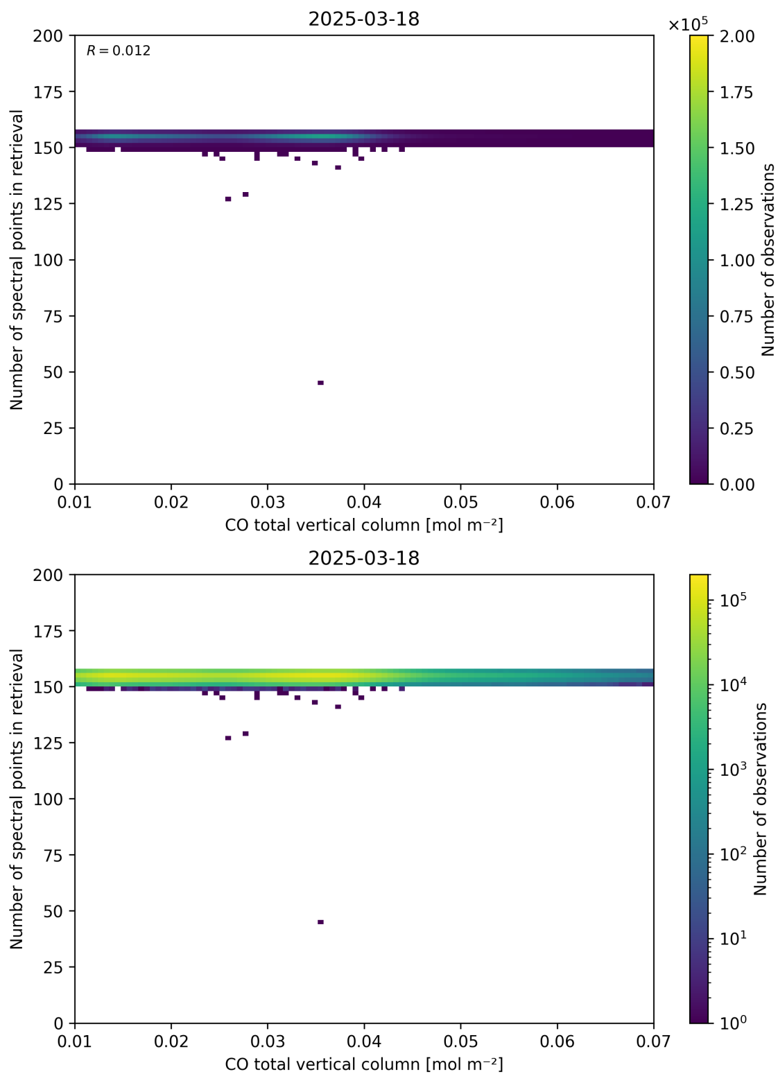
Figure 43: Scatter density plot of “CO total vertical column” against “Number of spectral points in retrieval” for 2025-03-17 to 2025-03-19.
