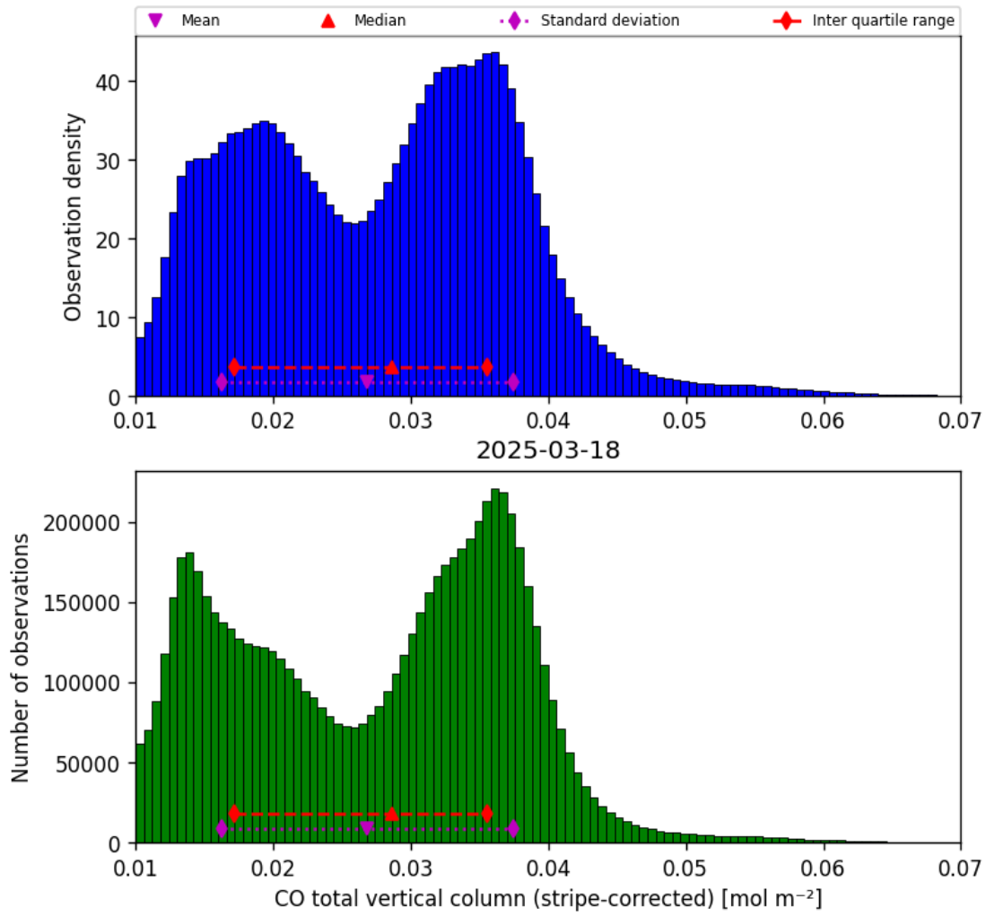
Figure 19: Histogram of “CO total vertical column (stripe-corrected)” for 2025-03-17 to 2025-03-19
