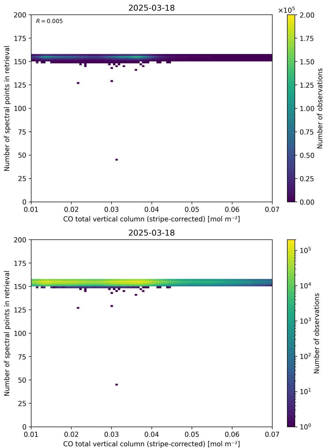
Figure 40: Scatter density plot of “CO total vertical column (stripe-corrected)” against “Number of spectral points in retrieval” for 2025-03-17 to 2025-03-19.
