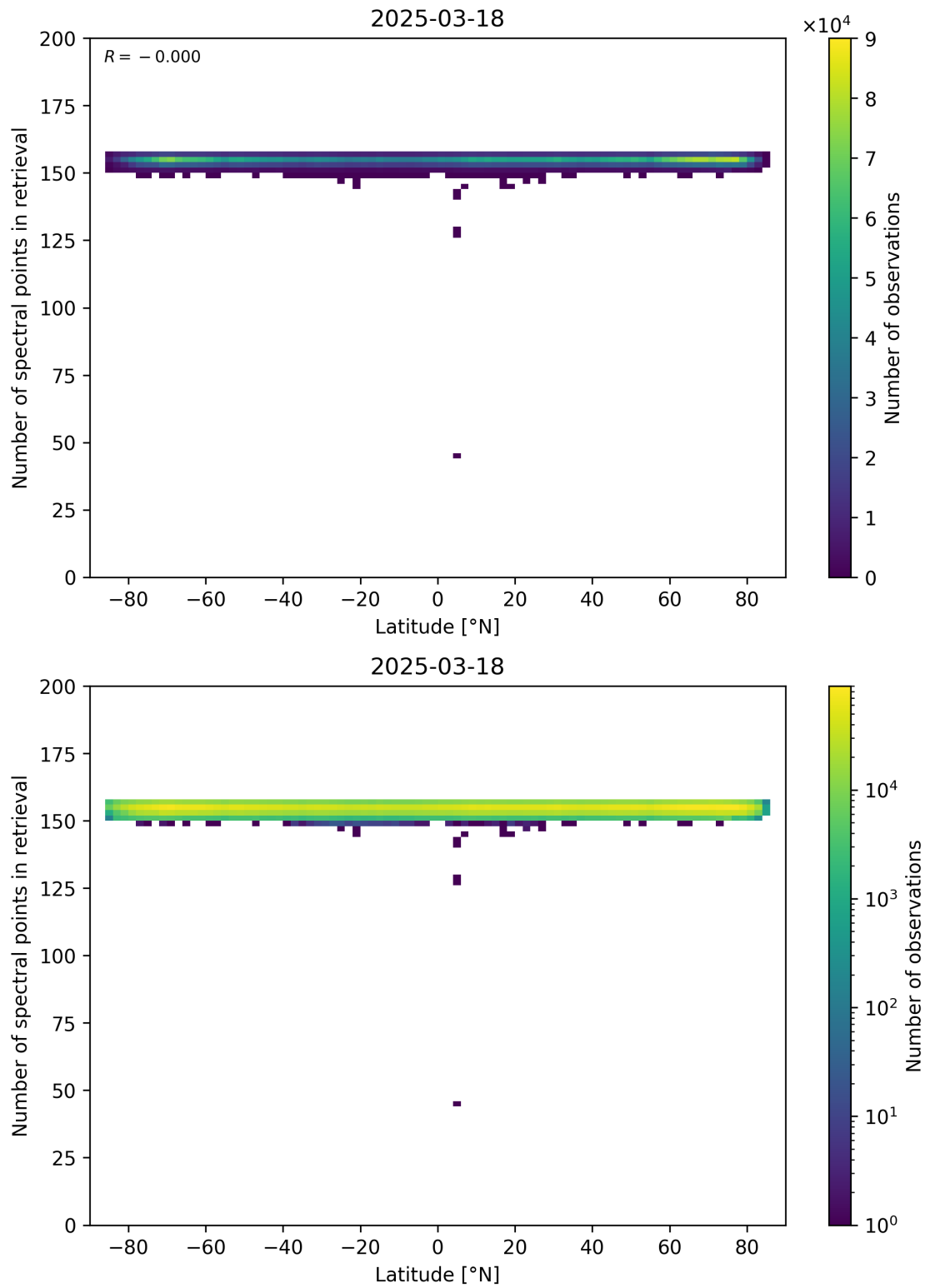
Figure 57: Scatter density plot of “Latitude” against “Number of spectral points in retrieval” for 2025-03-17 to 2025-03-19.
