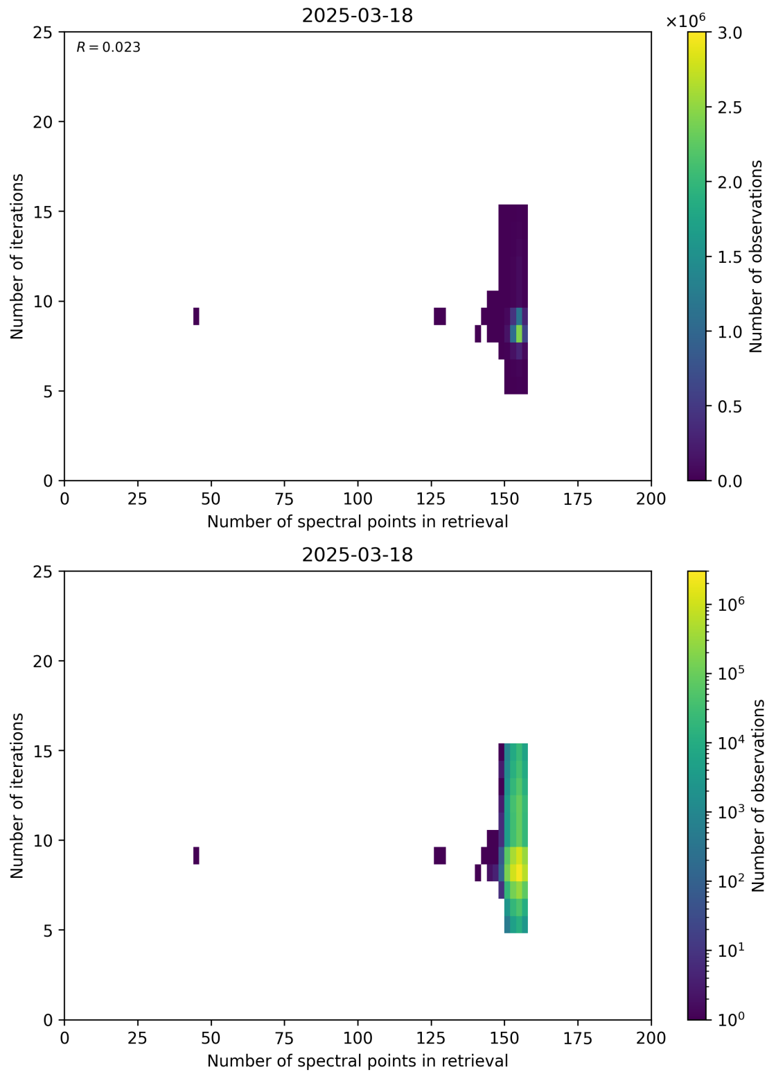
Figure 60: Scatter density plot of “Number of spectral points in retrieval” against “Number of iterations” for 2025-03-17 to 2025-03-19.
