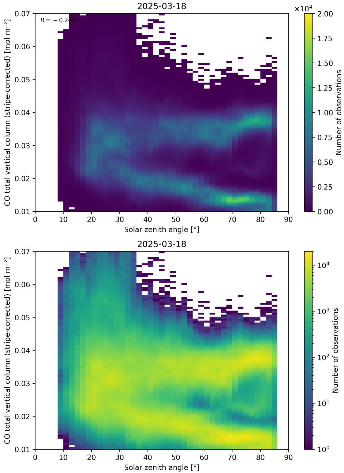
Figure 62: Scatter density plot of “Solar zenith angle” against “CO total vertical column (stripe-corrected)” for 2025-03-17 to 2025-03-19.
