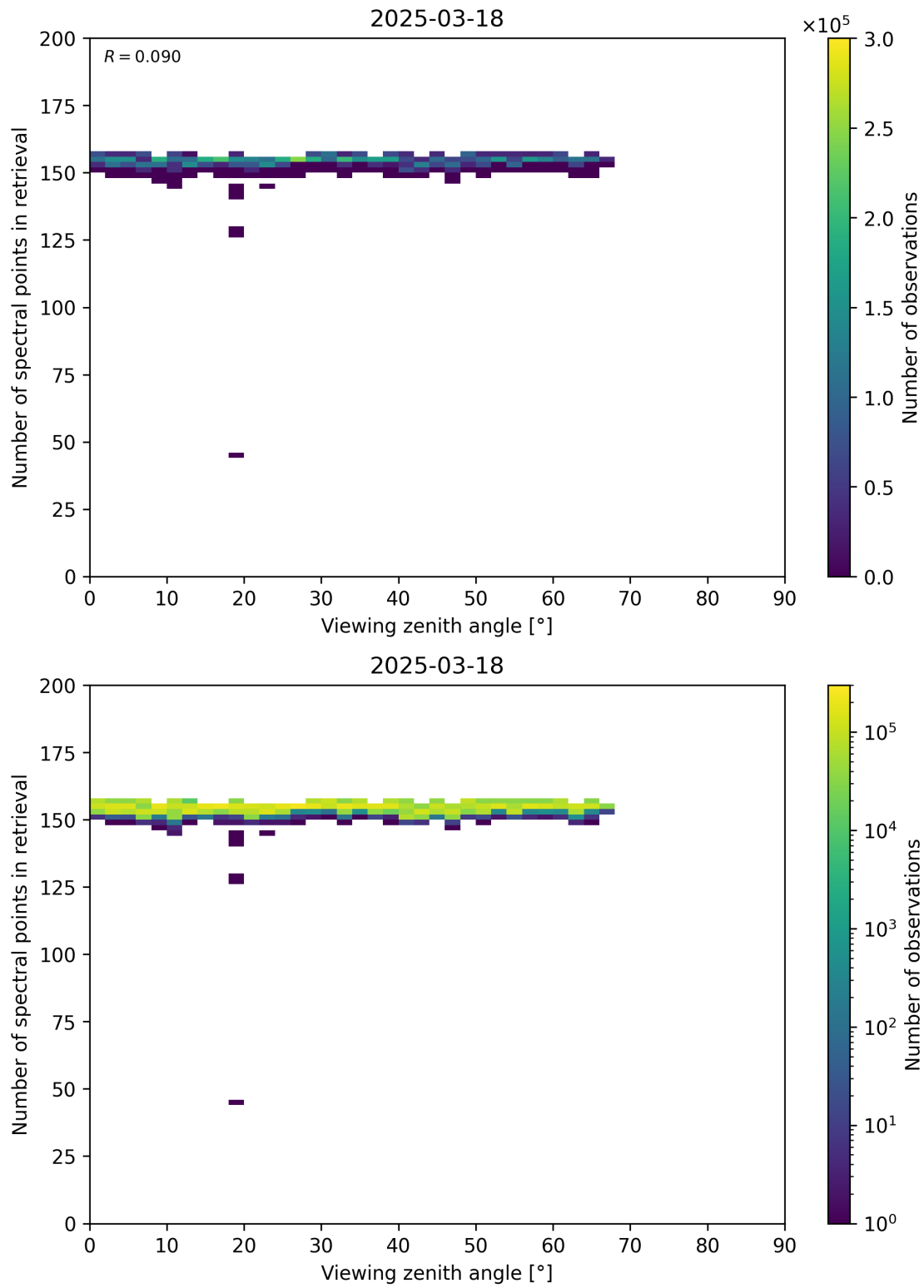
Figure 76: Scatter density plot of “Viewing zenith angle” against “Number of spectral points in retrieval” for 2025-03-17 to 2025-03-19.
