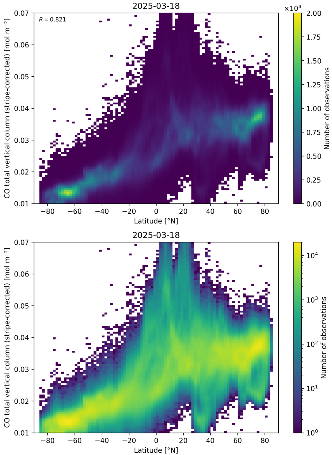
Figure 52: Scatter density plot of “Latitude” against “CO total vertical column (stripe-corrected)” for 2025-03-17 to 2025-03-19.
