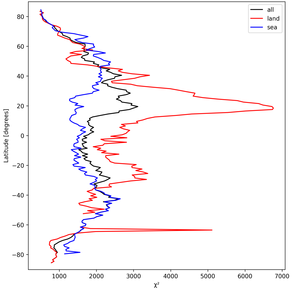
Figure 14: Zonal average of “ \chi^2 ” for 2025-03-17 to 2025-03-19.
