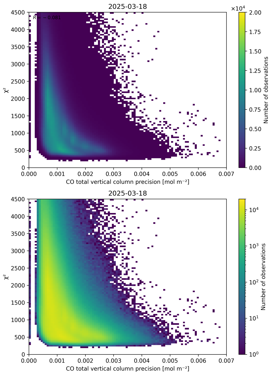
Figure 44: Scatter density plot of “CO total vertical column precision” against “ \chi^2 ” for 2025-03-17 to 2025-03-19.
