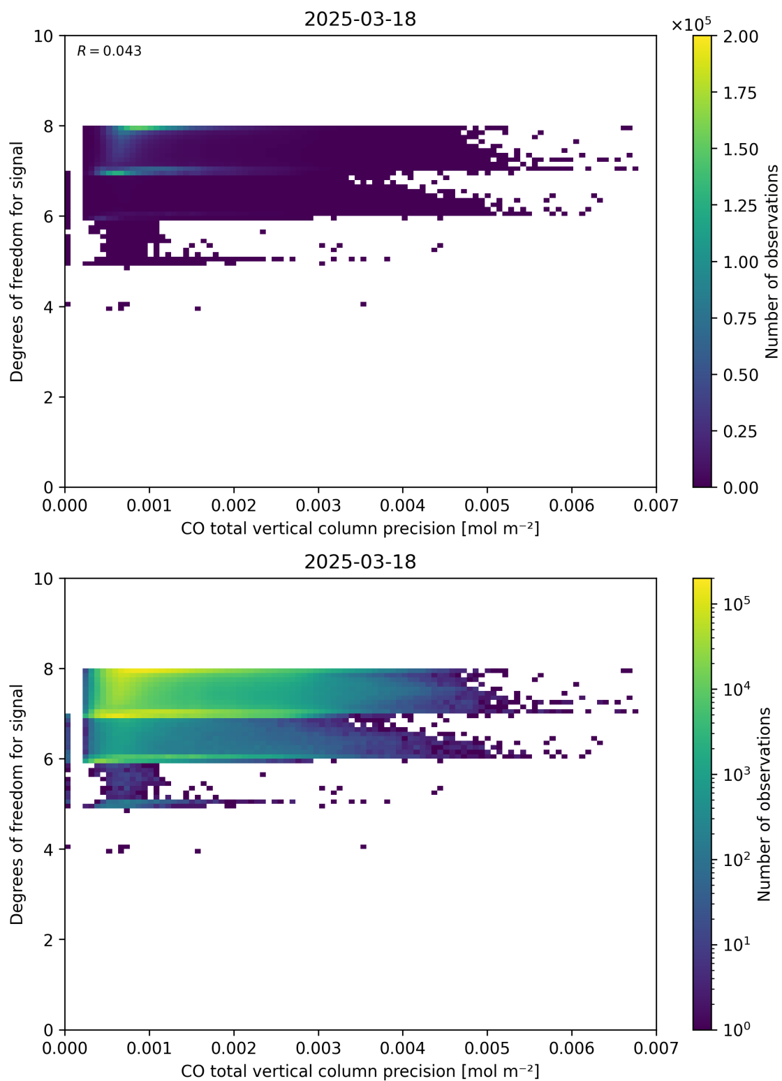
Figure 45: Scatter density plot of “CO total vertical column precision” against “Degrees of freedom for signal” for 2025-03-17 to 2025-03-19.
