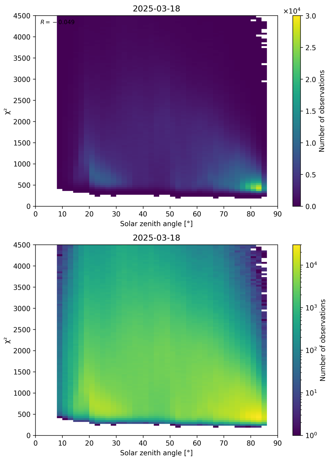
Figure 64: Scatter density plot of “Solar zenith angle” against “ \chi^2 ” for 2025-03-17 to 2025-03-19.
