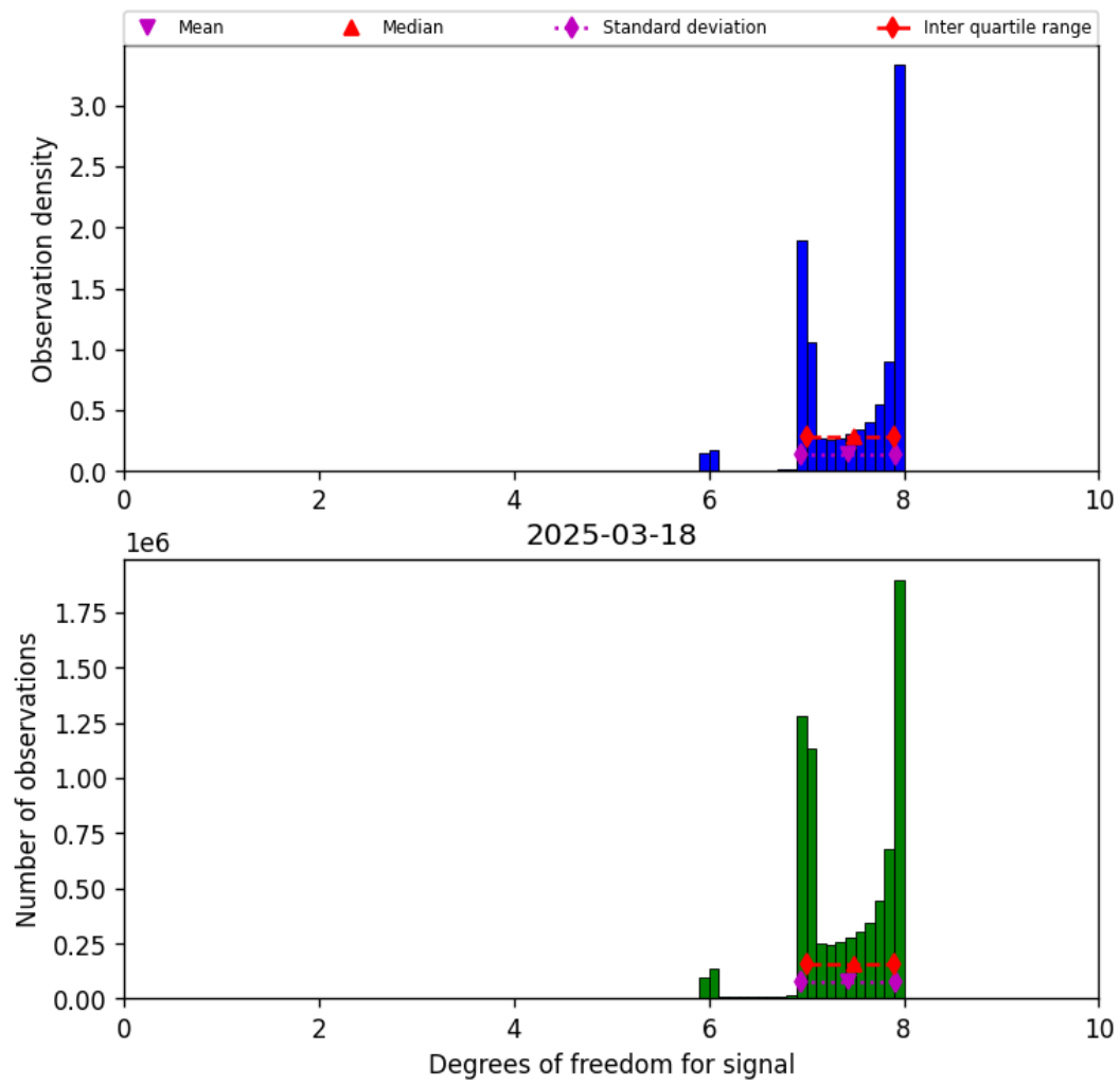
Figure 23: Histogram of “Degrees of freedom for signal” for 2025-03-17 to 2025-03-19
