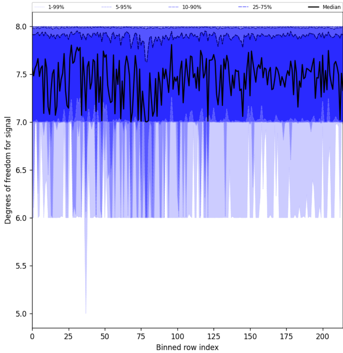
Figure 31: Along track statistics of “Degrees of freedom for signal” for 2025-03-17 to 2025-03-19
