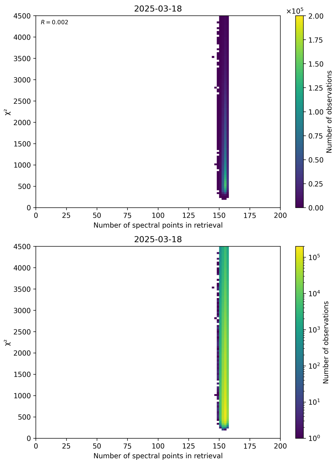
Figure 58: Scatter density plot of “Number of spectral points in retrieval” against “ \chi^2 ” for 2025-03-17 to 2025-03-19.
