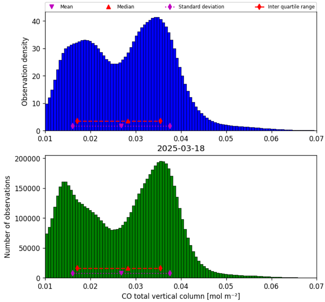
Figure 18: Histogram of “CO total vertical column” for 2025-03-17 to 2025-03-19
