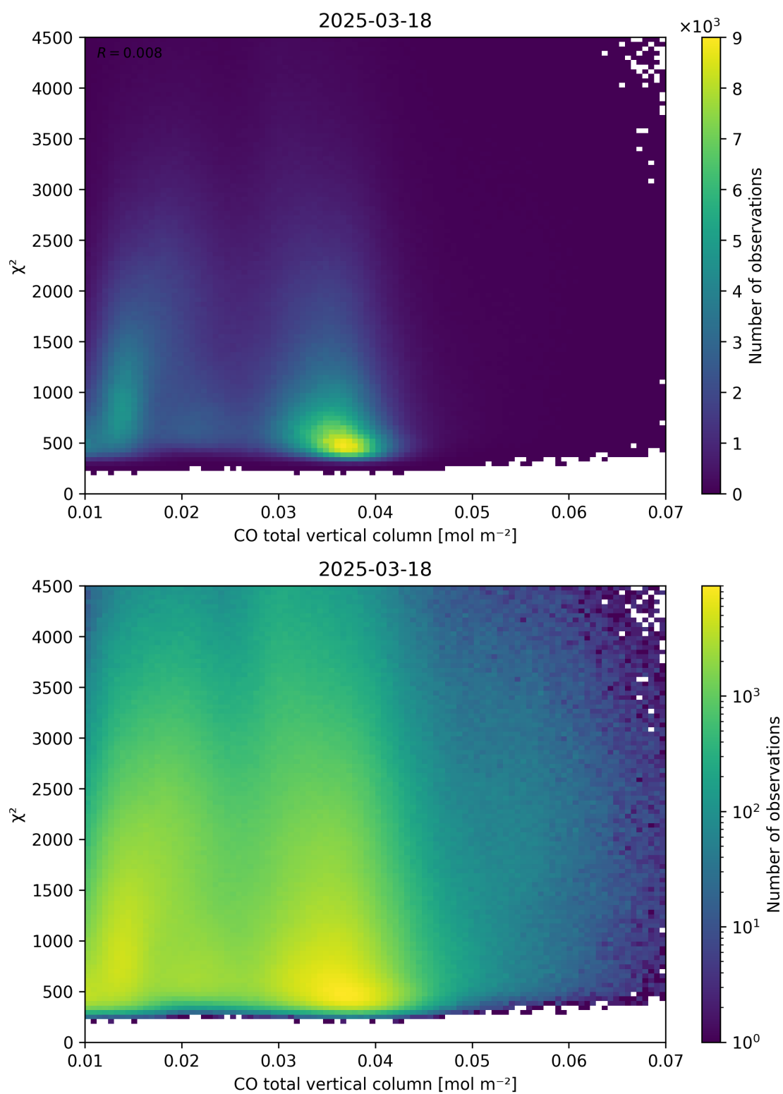
Figure 35: Scatter density plot of “CO total vertical column” against “ \chi^2 ” for 2025-03-17 to 2025-03-19.
