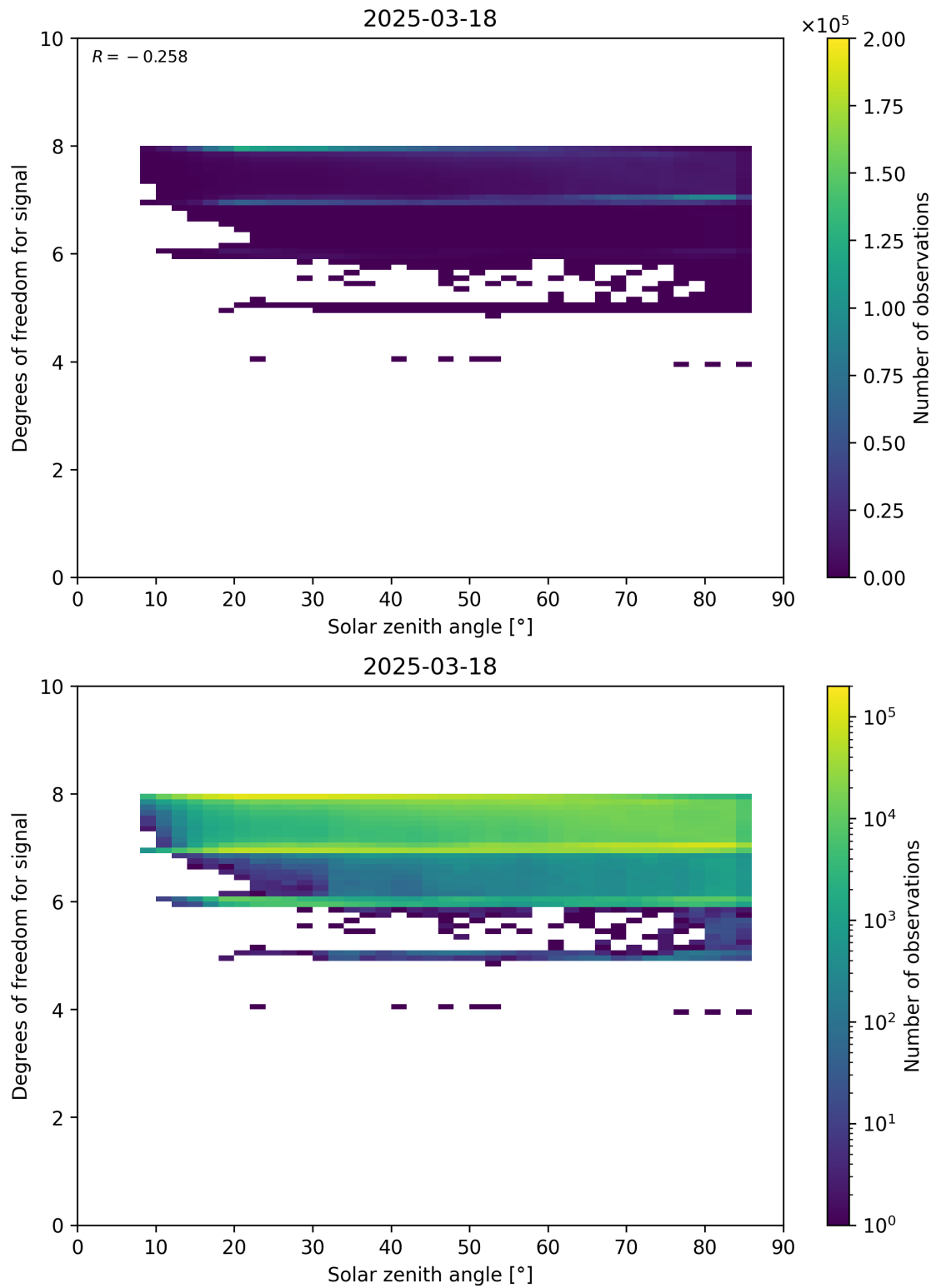
Figure 65: Scatter density plot of “Solar zenith angle” against “Degrees of freedom for signal” for 2025-03-17 to 2025-03-19.
