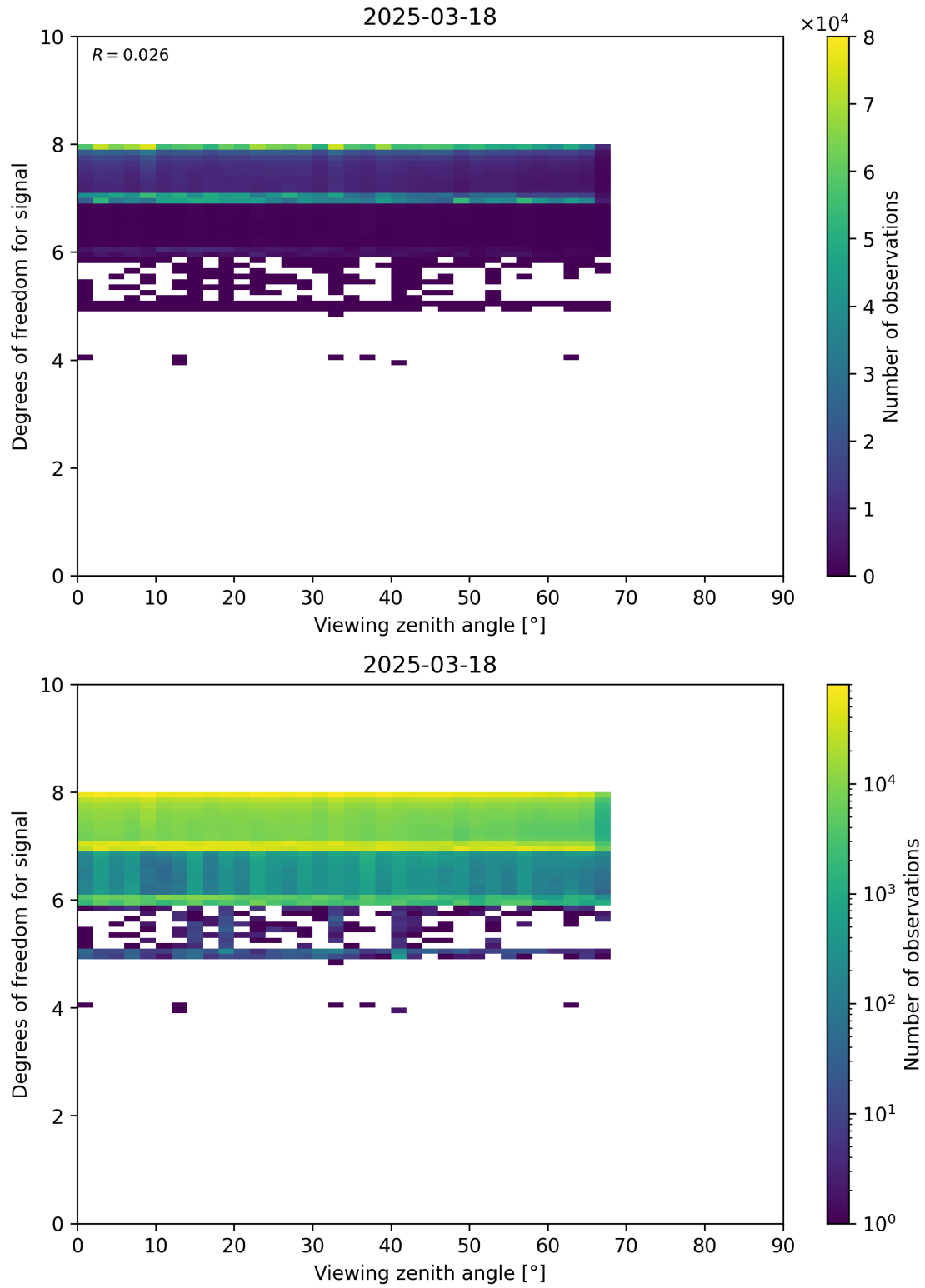
Figure 73: Scatter density plot of “Viewing zenith angle” against “Degrees of freedom for signal” for 2025-03-17 to 2025-03-19.
