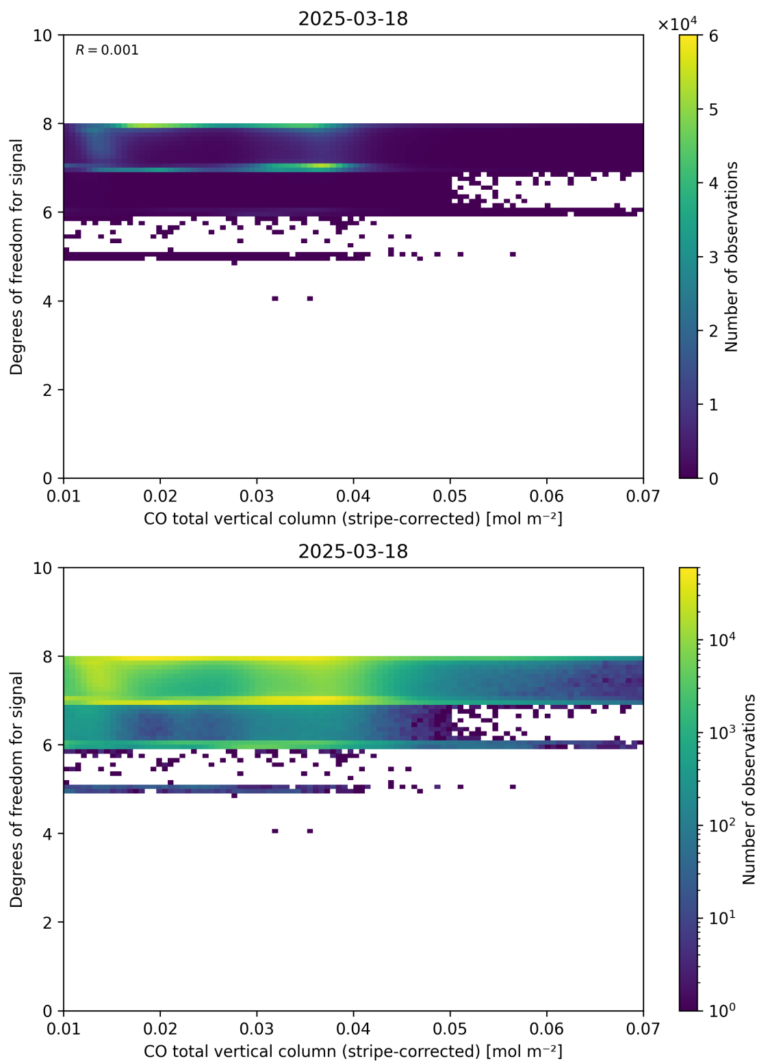
Figure 38: Scatter density plot of “CO total vertical column (stripe-corrected)” against “Degrees of freedom for signal” for 2025-03-17 to 2025-03-19.
