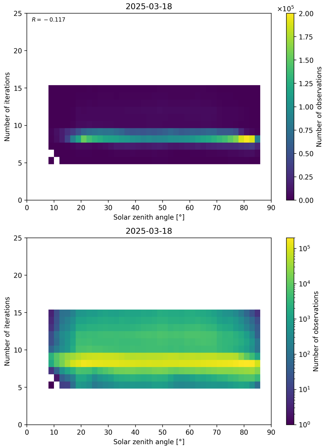
Figure 67: Scatter density plot of “Solar zenith angle” against “Number of iterations” for 2025-03-17 to 2025-03-19.
