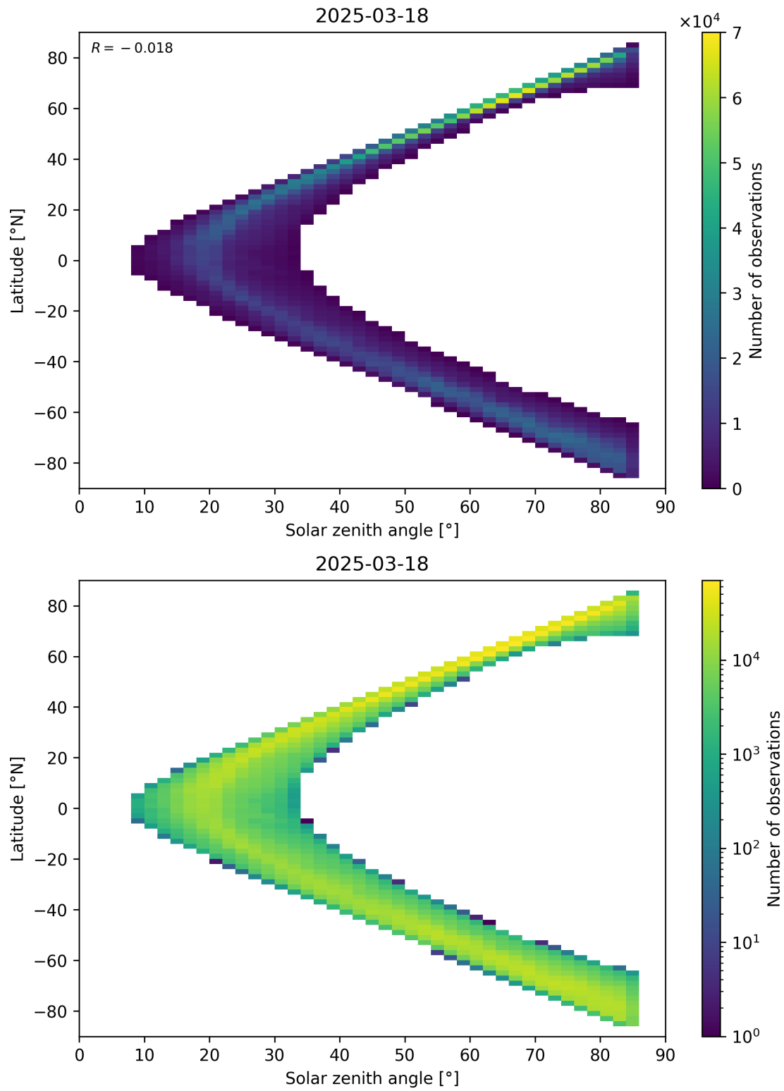
Figure 66: Scatter density plot of “Solar zenith angle” against “Latitude” for 2025-03-17 to 2025-03-19.
