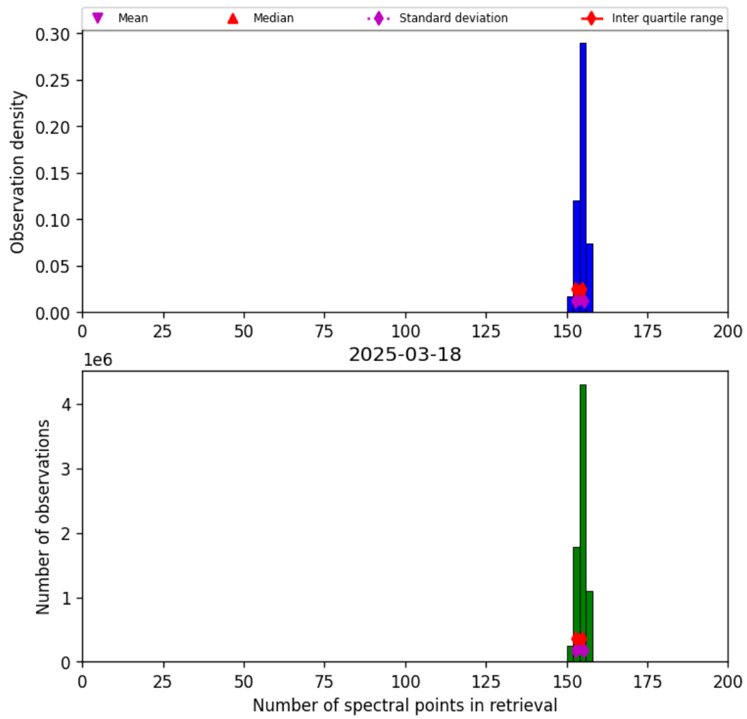
Figure 21: Histogram of “Number of spectral points in retrieval” for 2025-03-17 to 2025-03-19
