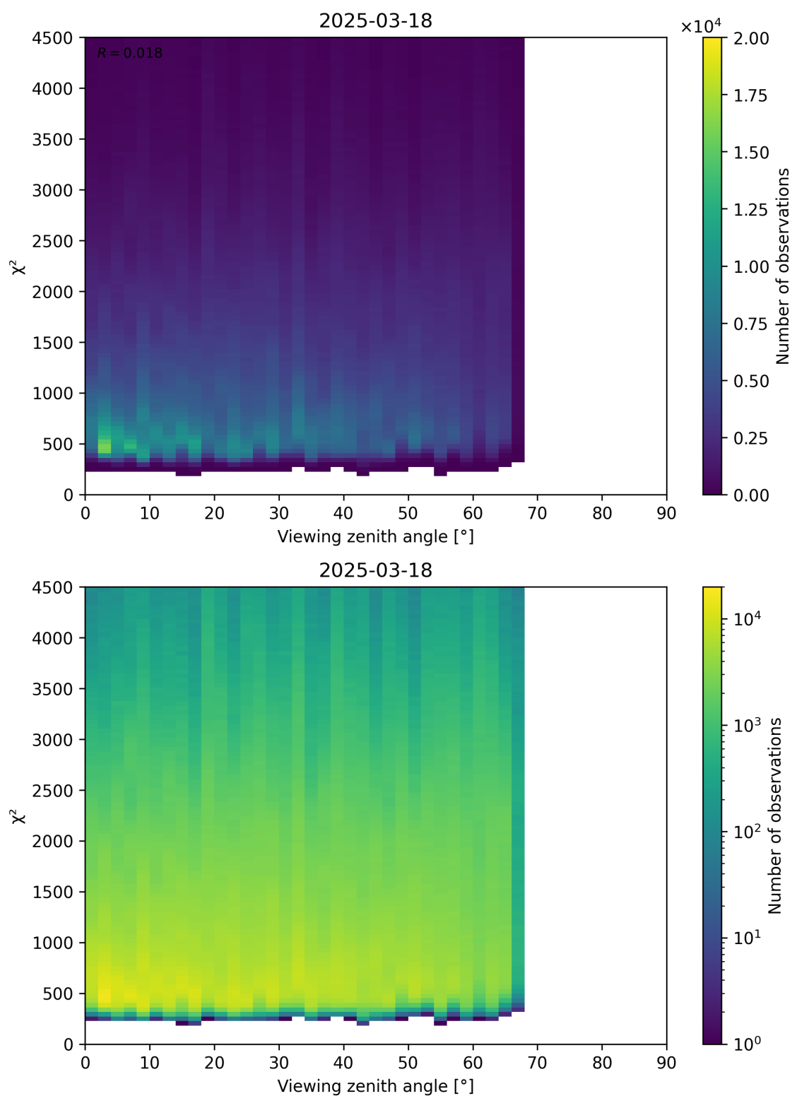
Figure 72: Scatter density plot of “Viewing zenith angle” against “ \chi^2 ” for 2025-03-17 to 2025-03-19.
