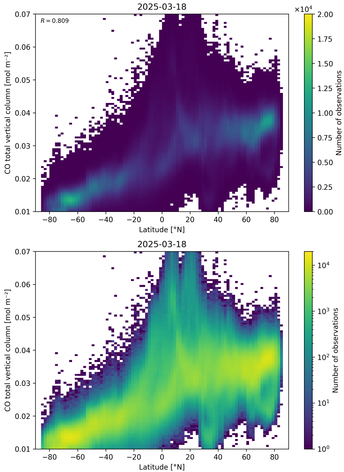
Figure 51: Scatter density plot of “Latitude” against “CO total vertical column” for 2025-03-17 to 2025-03-19.
