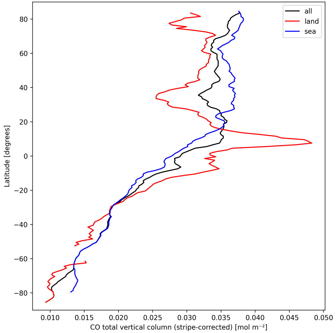
Figure 11: Zonal average of “CO total vertical column (stripe-corrected)” for 2025-03-17 to 2025-03-19.
