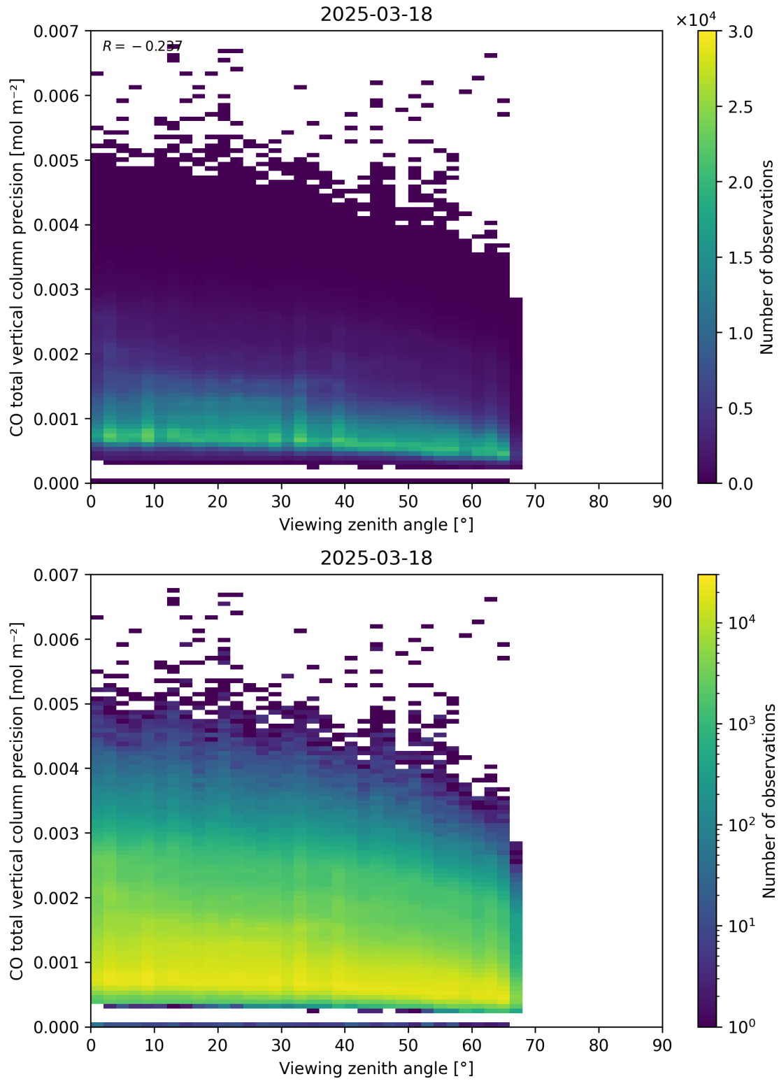
Figure 71: Scatter density plot of “Viewing zenith angle” against “CO total vertical column precision” for 2025-03-17 to 2025-03-19.
