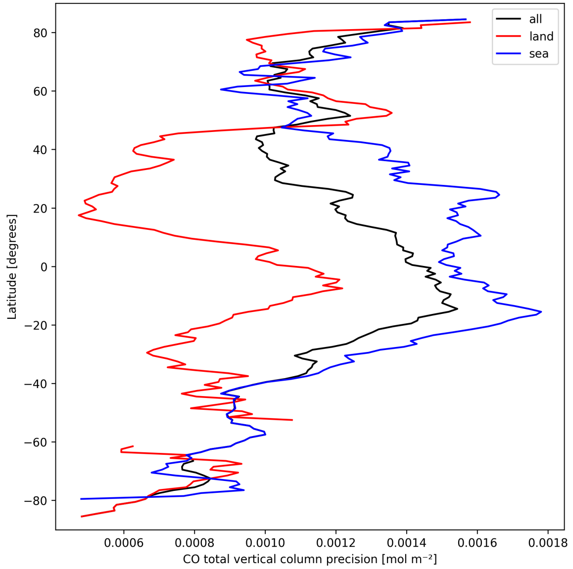
Figure 12: Zonal average of “CO total vertical column precision” for 2025-03-17 to 2025-03-19.
