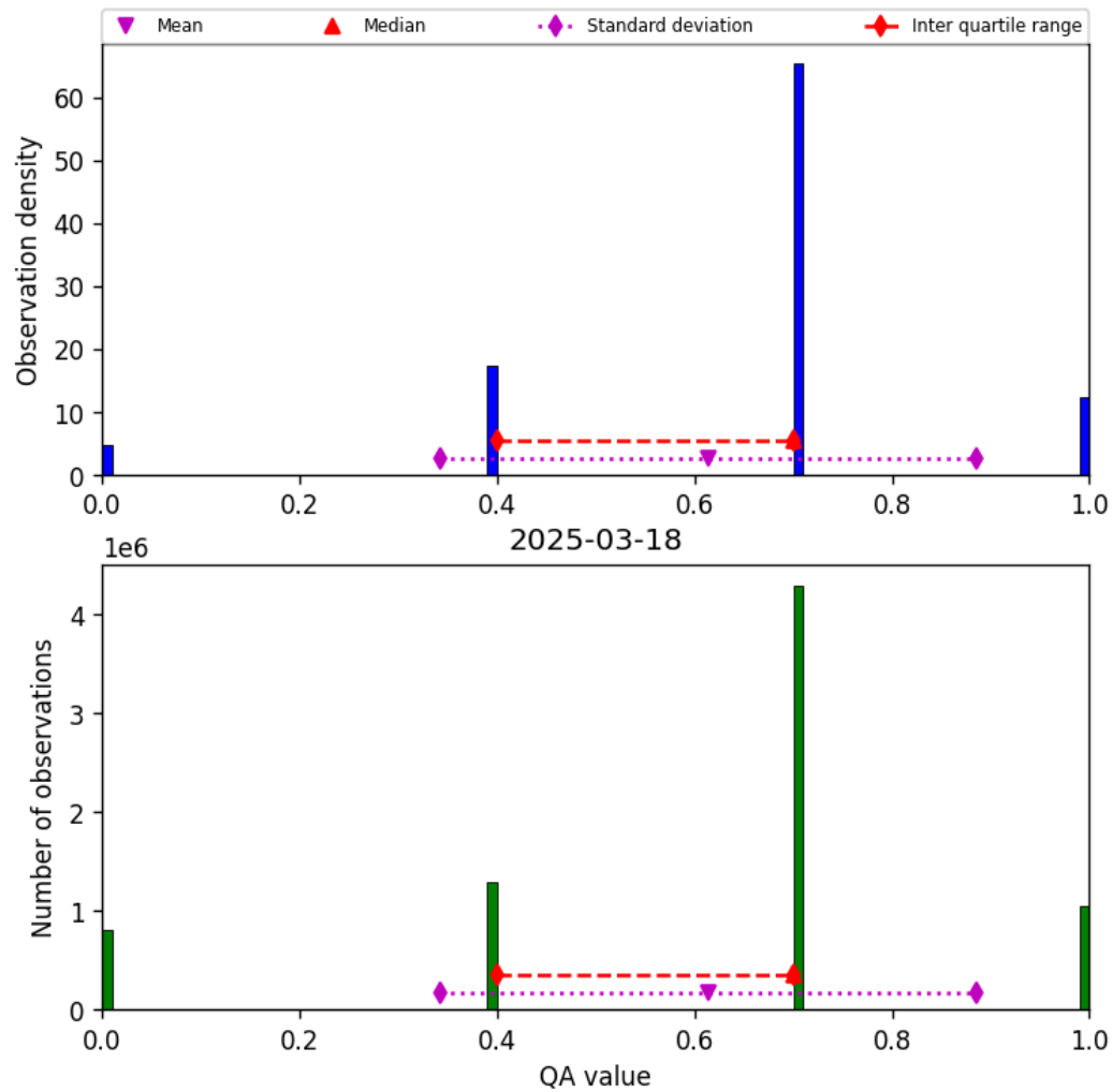
Figure 17: Histogram of “QA value” for 2025-03-17 to 2025-03-19
