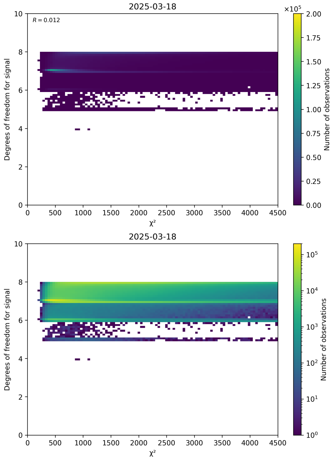
Figure 48: Scatter density plot of " \chi^2 " against "Degrees of freedom for signal" for 2025-03-17 to 2025-03-19.
