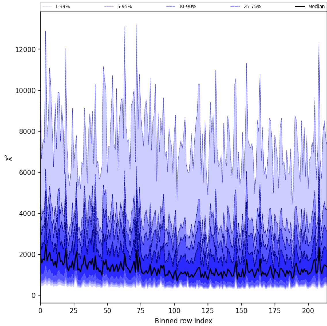
Figure 30: Along track statistics of “ \chi^2 ” for 2025-03-17 to 2025-03-19
