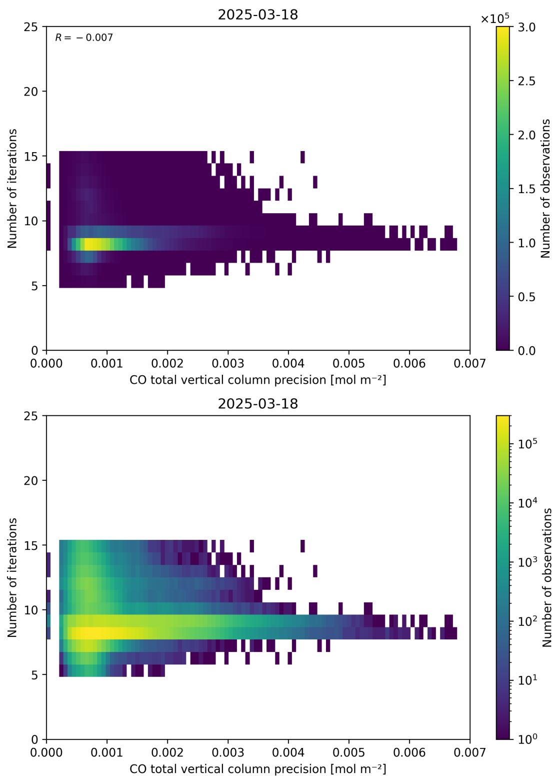
Figure 46: Scatter density plot of “CO total vertical column precision” against “Number of iterations” for 2025-03-17 to 2025-03-19.
