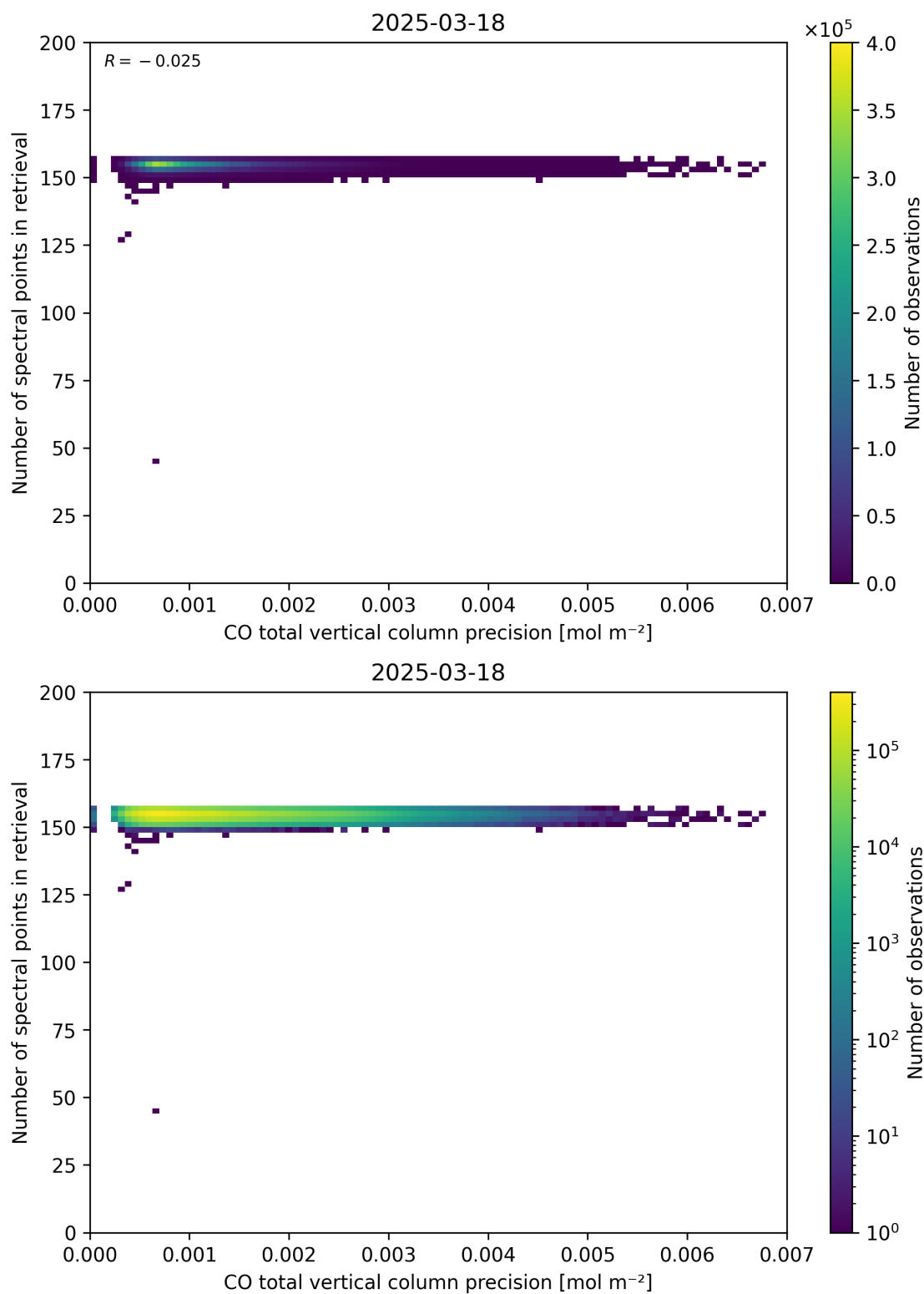
Figure 47: Scatter density plot of “CO total vertical column precision” against “Number of spectral points in retrieval” for 2025-03-17 to 2025-03-19.
