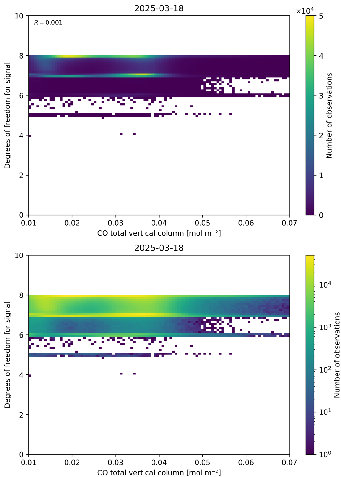
Figure 41: Scatter density plot of “CO total vertical column” against “Degrees of freedom for signal” for 2025-03-17 to 2025-03-19.
