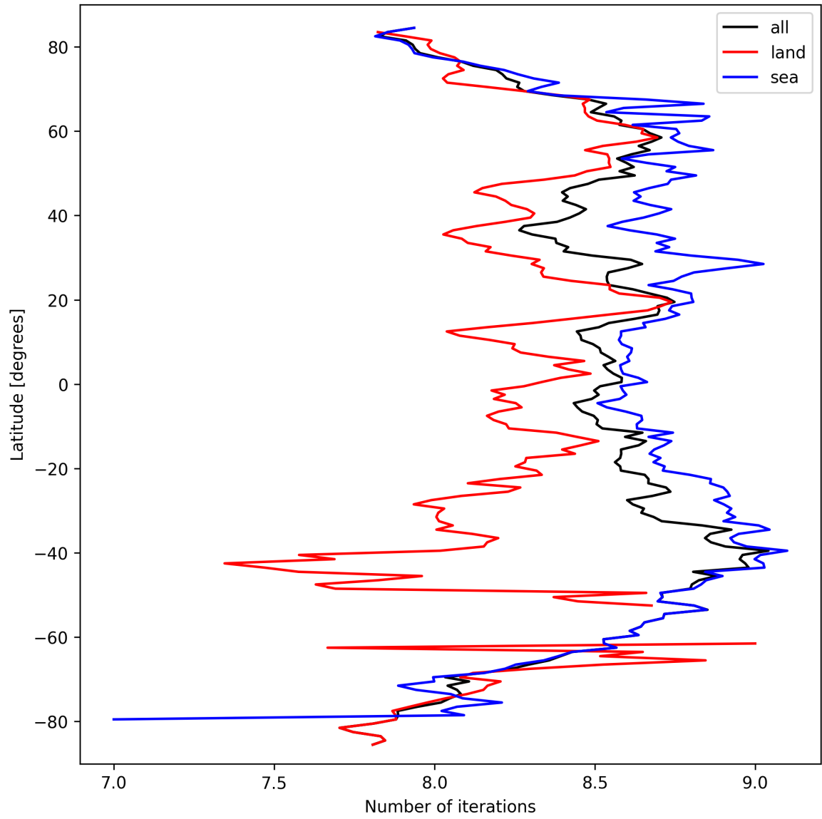
Figure 16: Zonal average of “Number of iterations” for 2025-03-17 to 2025-03-19.
