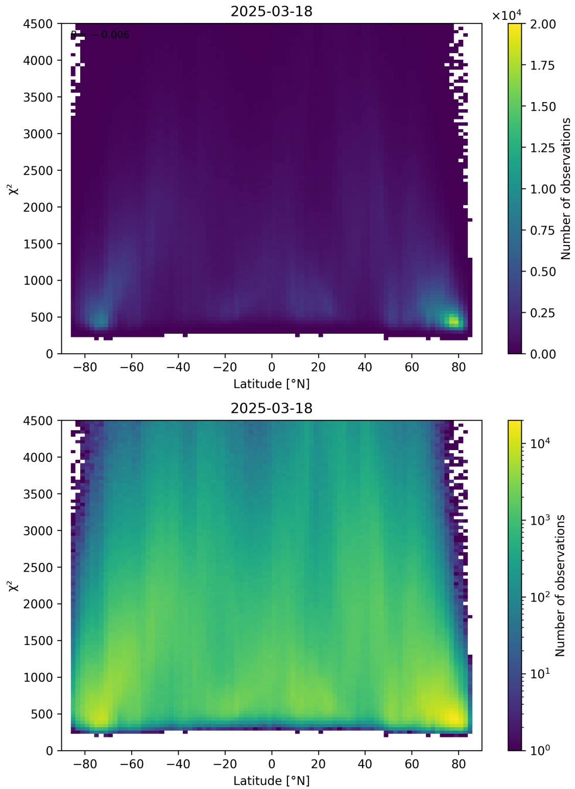
Figure 54: Scatter density plot of “Latitude” against “ \chi^2 ” for 2025-03-17 to 2025-03-19.
