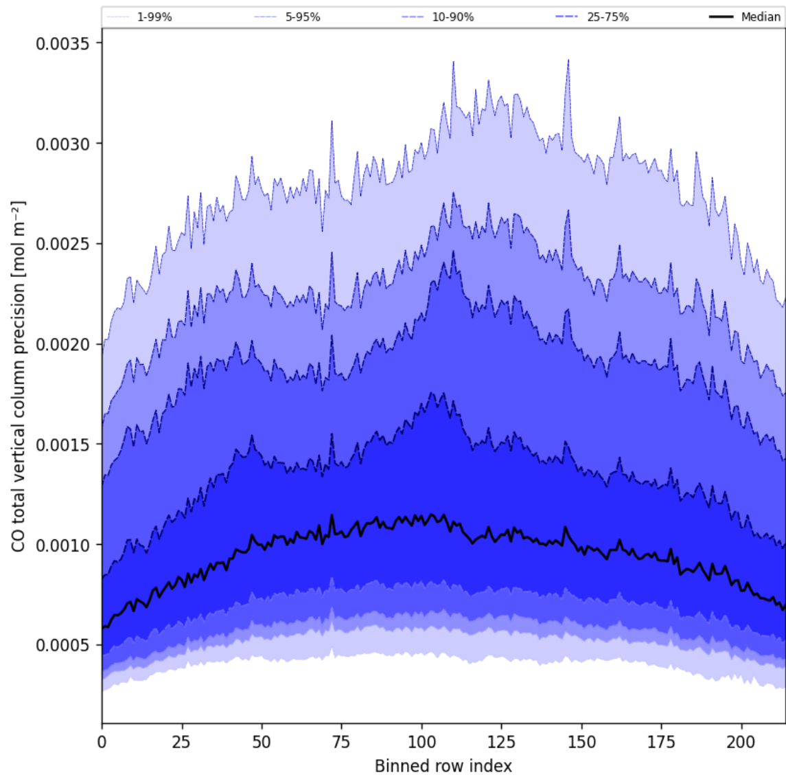
Figure 28: Along track statistics of “CO total vertical column precision” for 2025-03-17 to 2025-03-19
