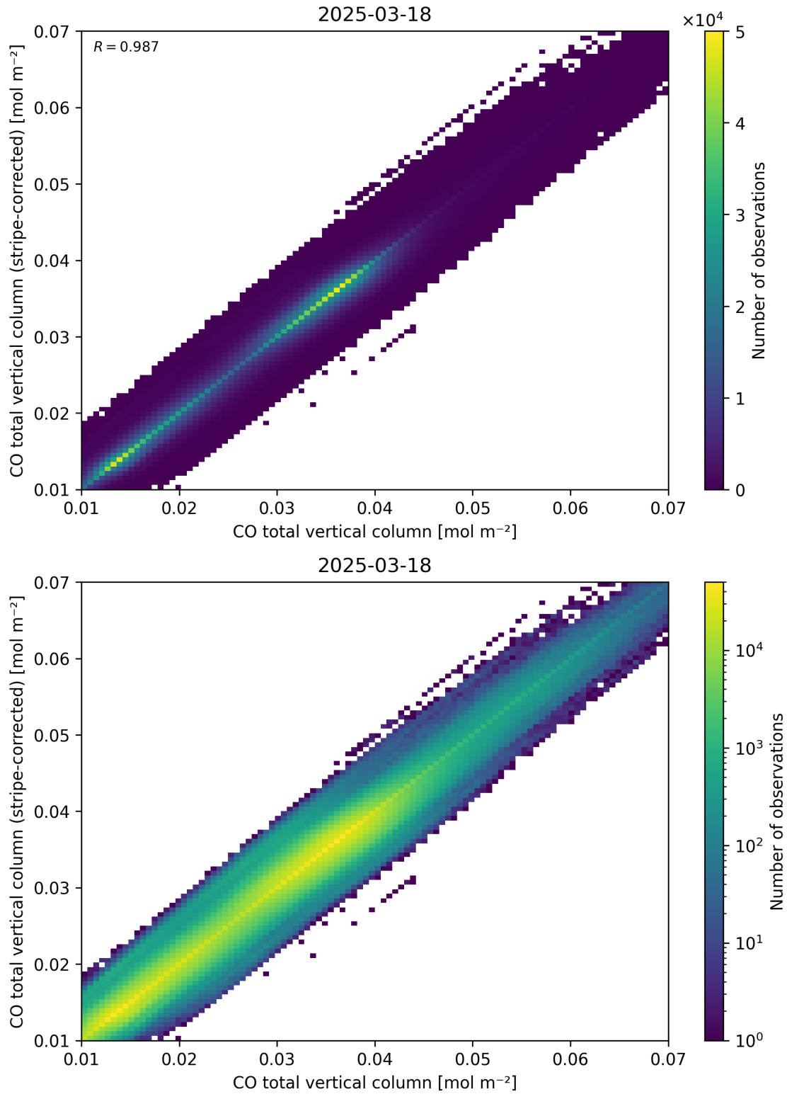
Figure 33: Scatter density plot of “CO total vertical column” against “CO total vertical column (stripe-corrected)” for 2025-03-17 to 2025-03-19.
