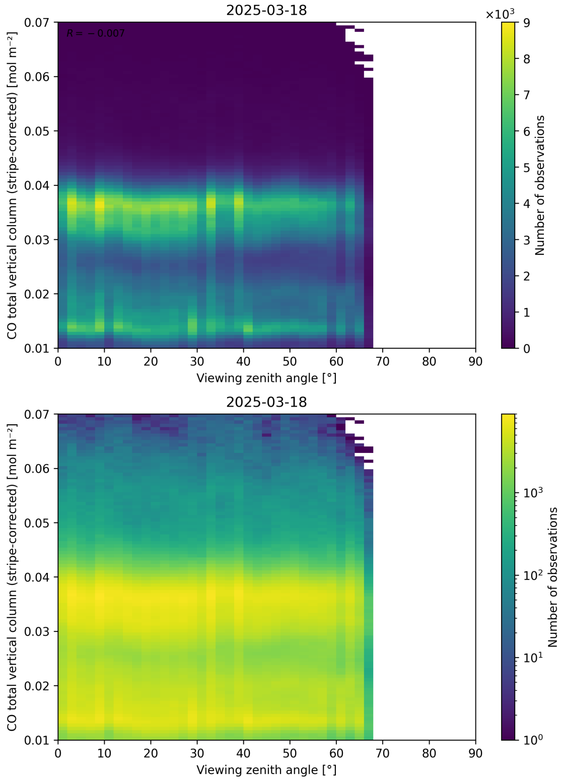
Figure 70: Scatter density plot of “Viewing zenith angle” against “CO total vertical column (stripe-corrected)” for 2025-03-17 to 2025-03-19.
