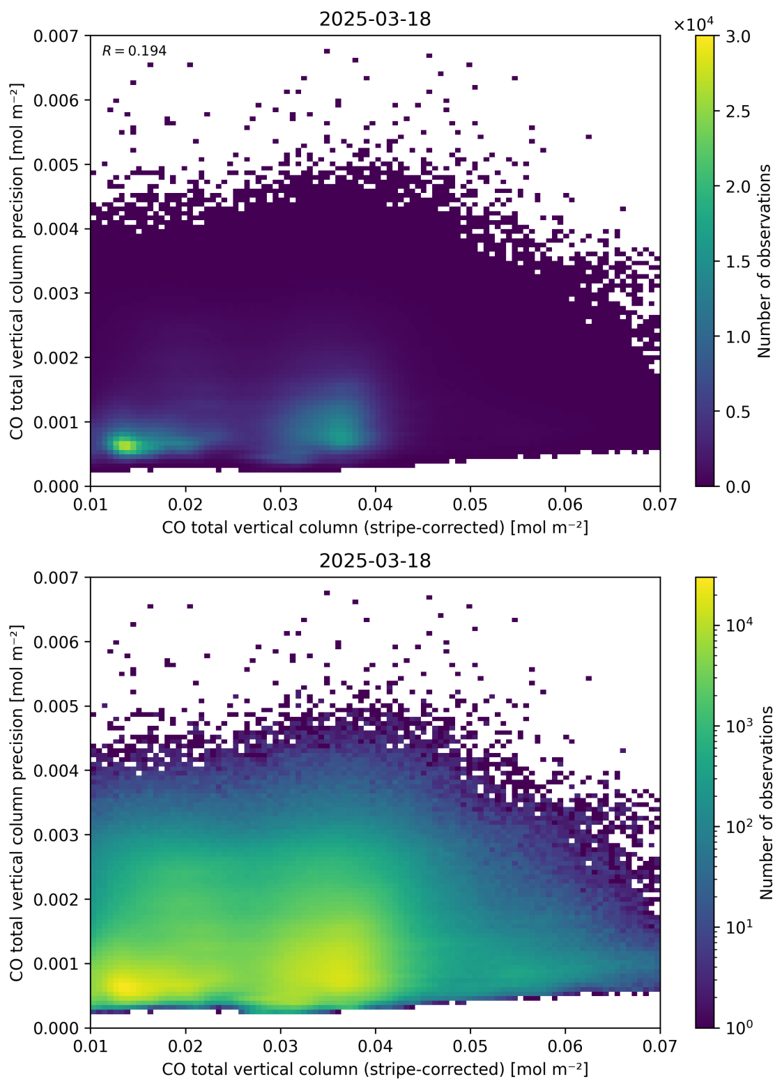
Figure 36: Scatter density plot of “CO total vertical column (stripe-corrected)” against “CO total vertical column precision” for 2025-03-17 to 2025-03-19.
