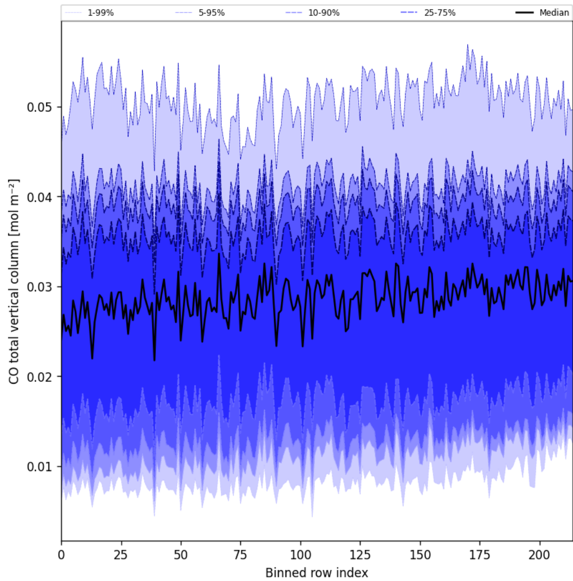
Figure 26: Along track statistics of “CO total vertical column” for 2025-03-17 to 2025-03-19
