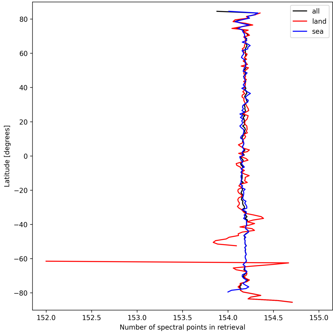
Figure 13: Zonal average of “Number of spectral points in retrieval” for 2025-03-17 to 2025-03-19.
