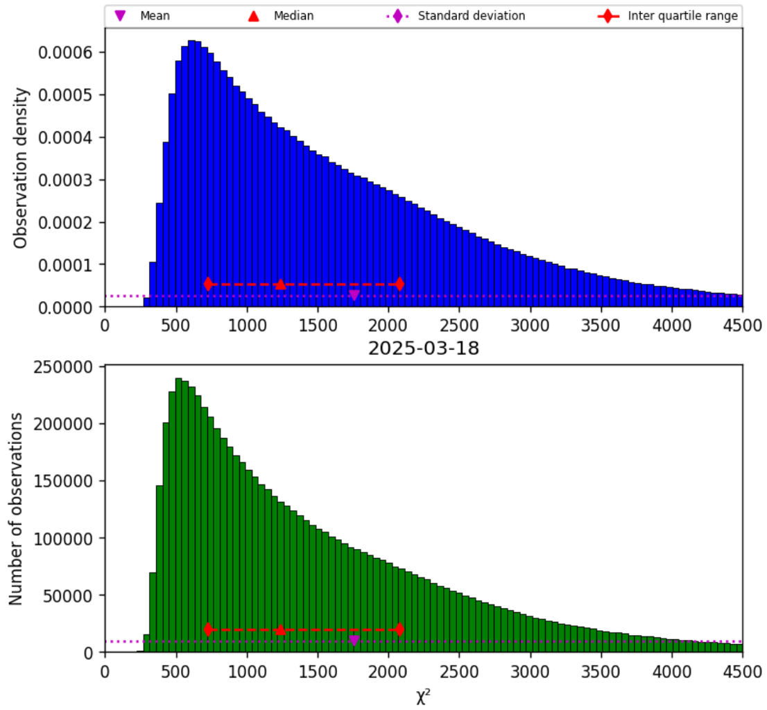
Figure 22: Histogram of “ \chi^2 ” for 2025-03-17 to 2025-03-19
