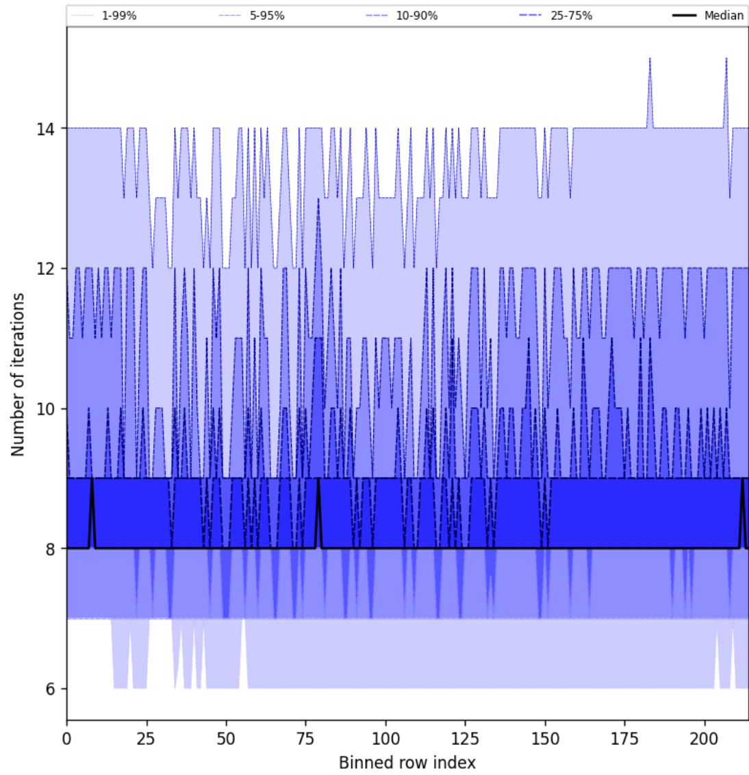
Figure 32: Along track statistics of “Number of iterations” for 2025-03-17 to 2025-03-19
