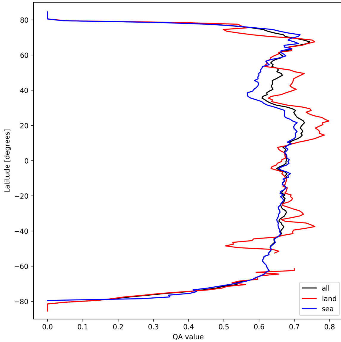
Figure 9: Zonal average of “QA value” for 2025-03-17 to 2025-03-19.
