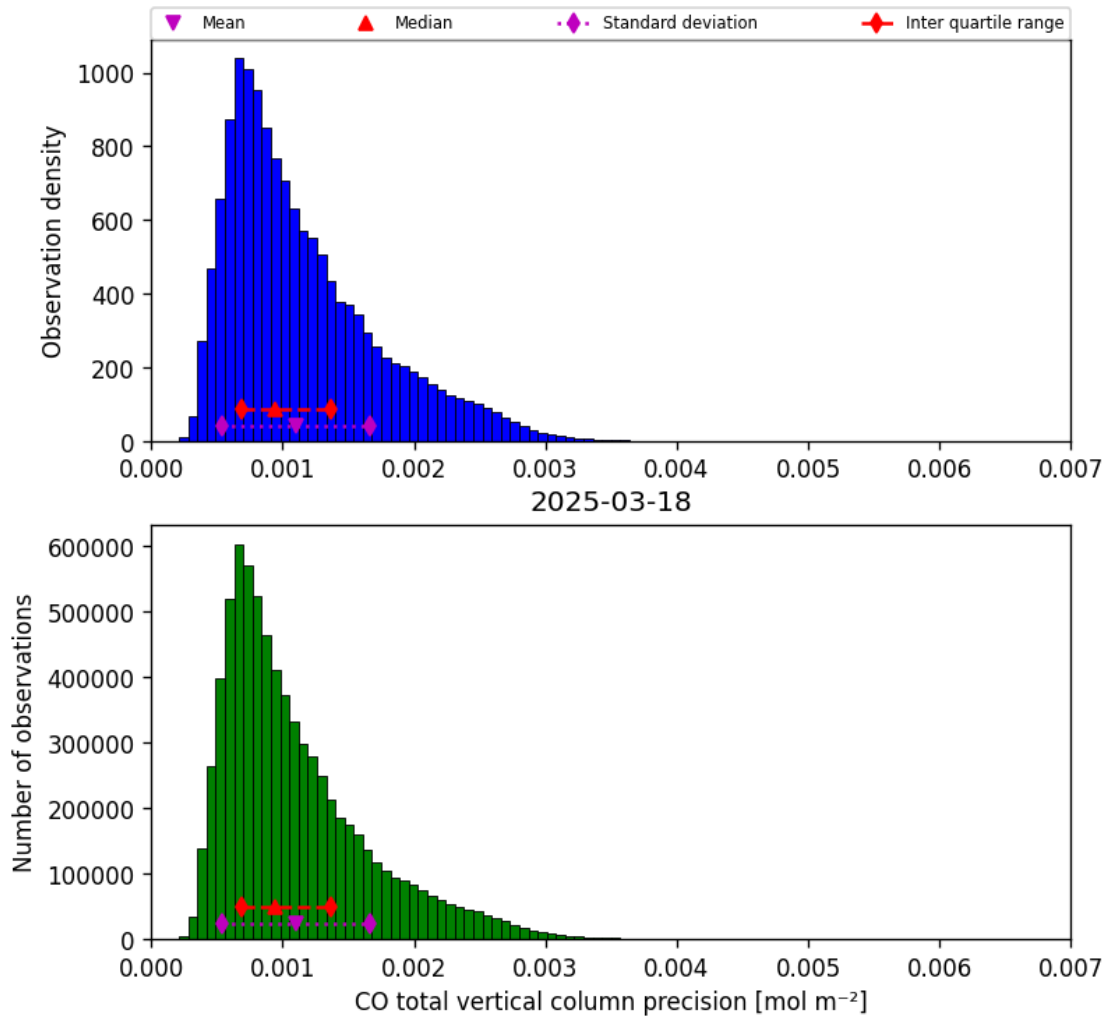
Figure 20: Histogram of “CO total vertical column precision” for 2025-03-17 to 2025-03-19
