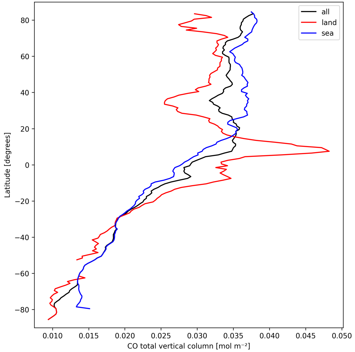
Figure 10: Zonal average of “CO total vertical column” for 2025-03-17 to 2025-03-19.
