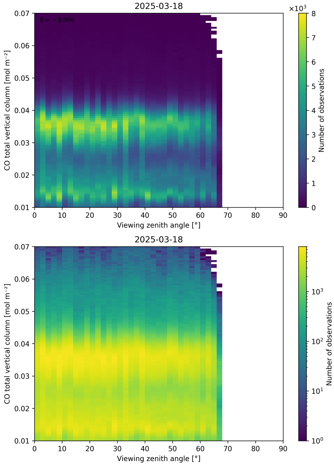
Figure 69: Scatter density plot of “Viewing zenith angle” against “CO total vertical column” for 2025-03-17 to 2025-03-19.
