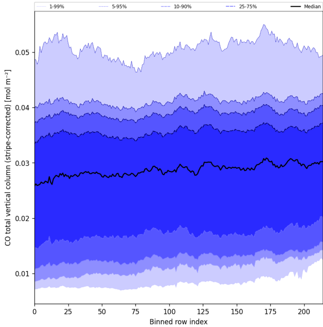
Figure 27: Along track statistics of “CO total vertical column (stripe-corrected)” for 2025-03-17 to 2025-03-19
