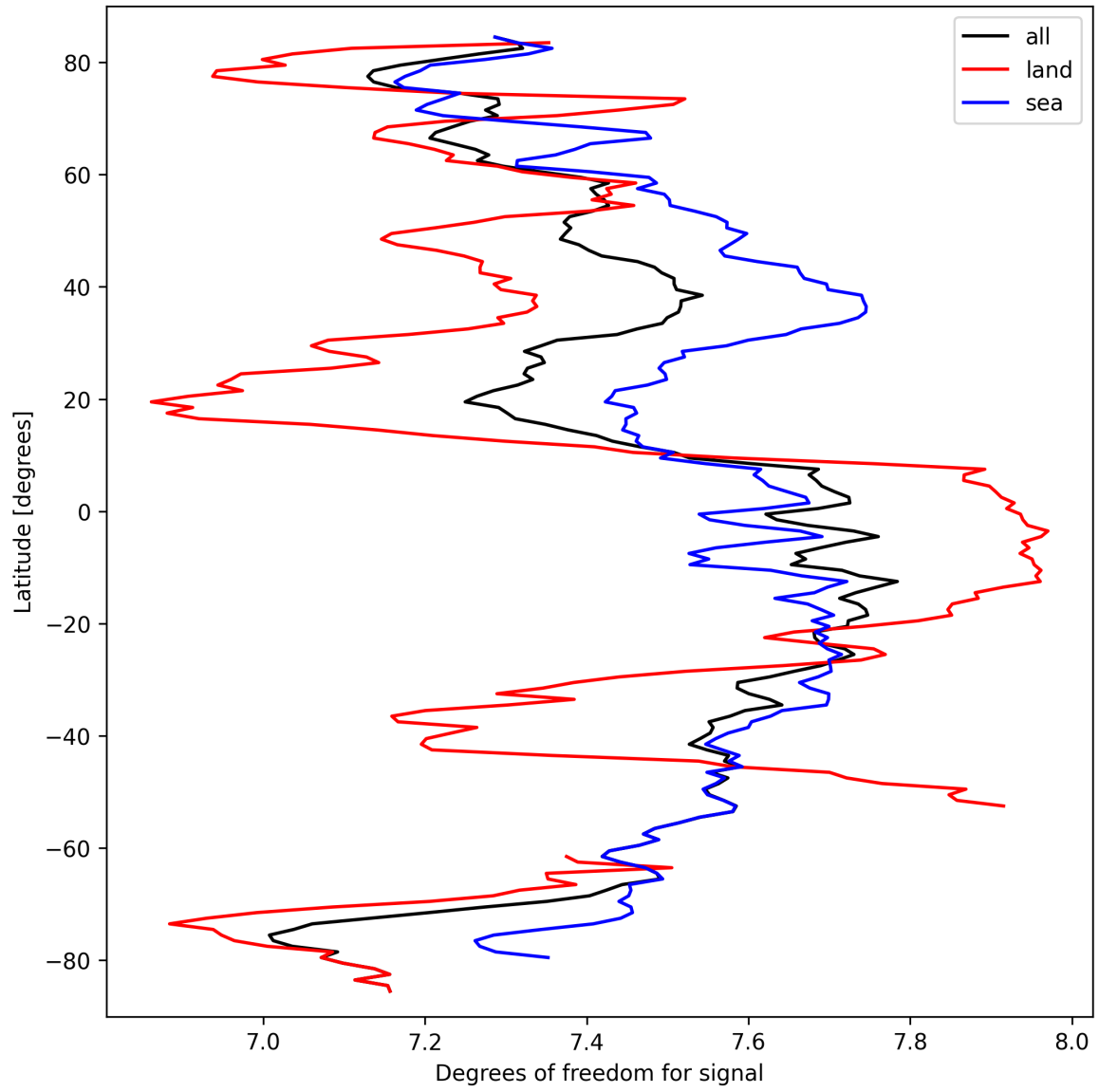
Figure 15: Zonal average of “Degrees of freedom for signal” for 2025-03-17 to 2025-03-19.
