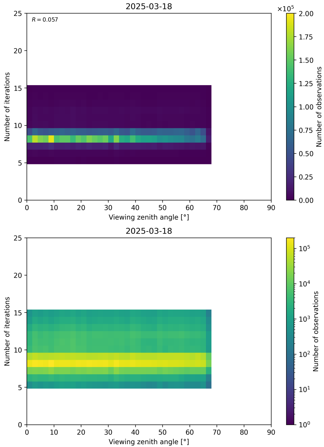
Figure 75: Scatter density plot of “Viewing zenith angle” against “Number of iterations” for 2025-03-17 to 2025-03-19.
