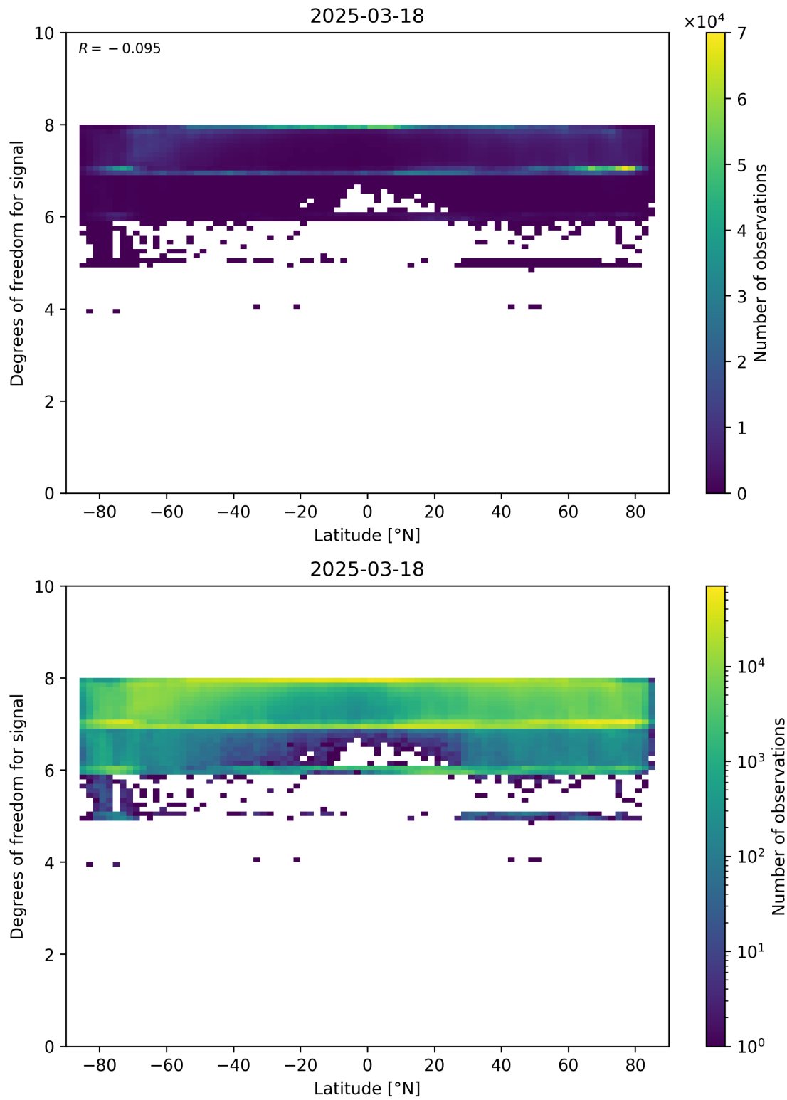
Figure 55: Scatter density plot of “Latitude” against “Degrees of freedom for signal” for 2025-03-17 to 2025-03-19.
