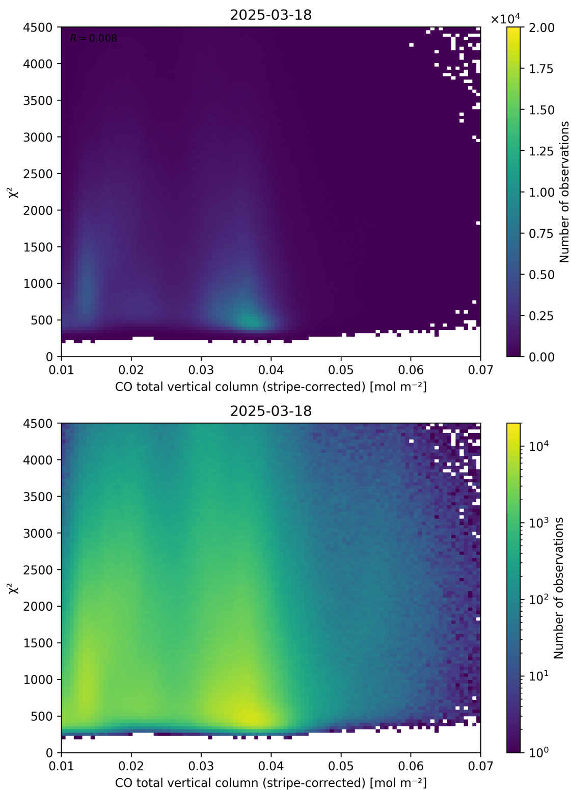
Figure 37: Scatter density plot of “CO total vertical column (stripe-corrected)” against “ \chi^2 ” for 2025-03-17 to 2025-03-19.
