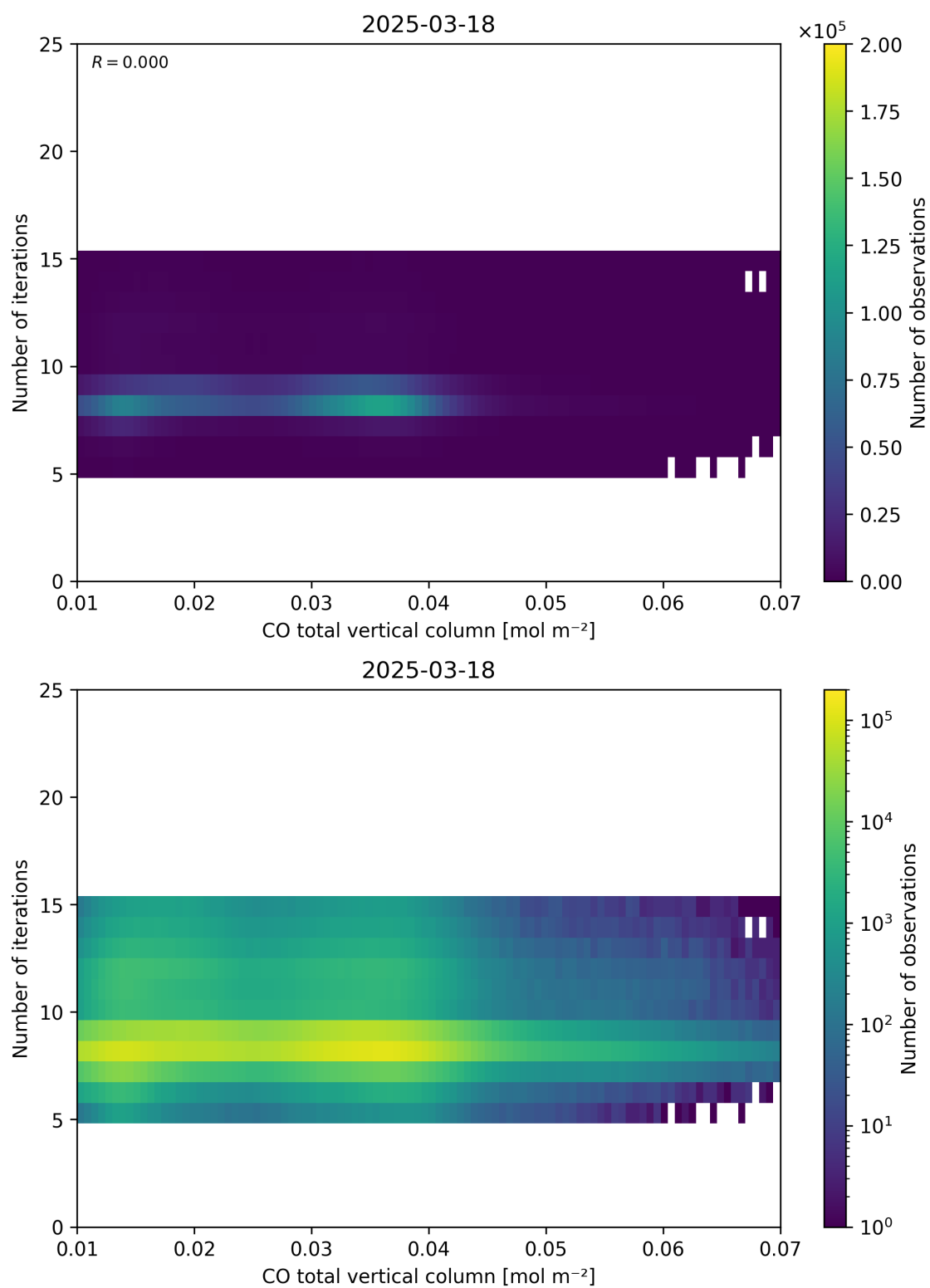
Figure 42: Scatter density plot of “CO total vertical column” against “Number of iterations” for 2025-03-17 to 2025-03-19.
