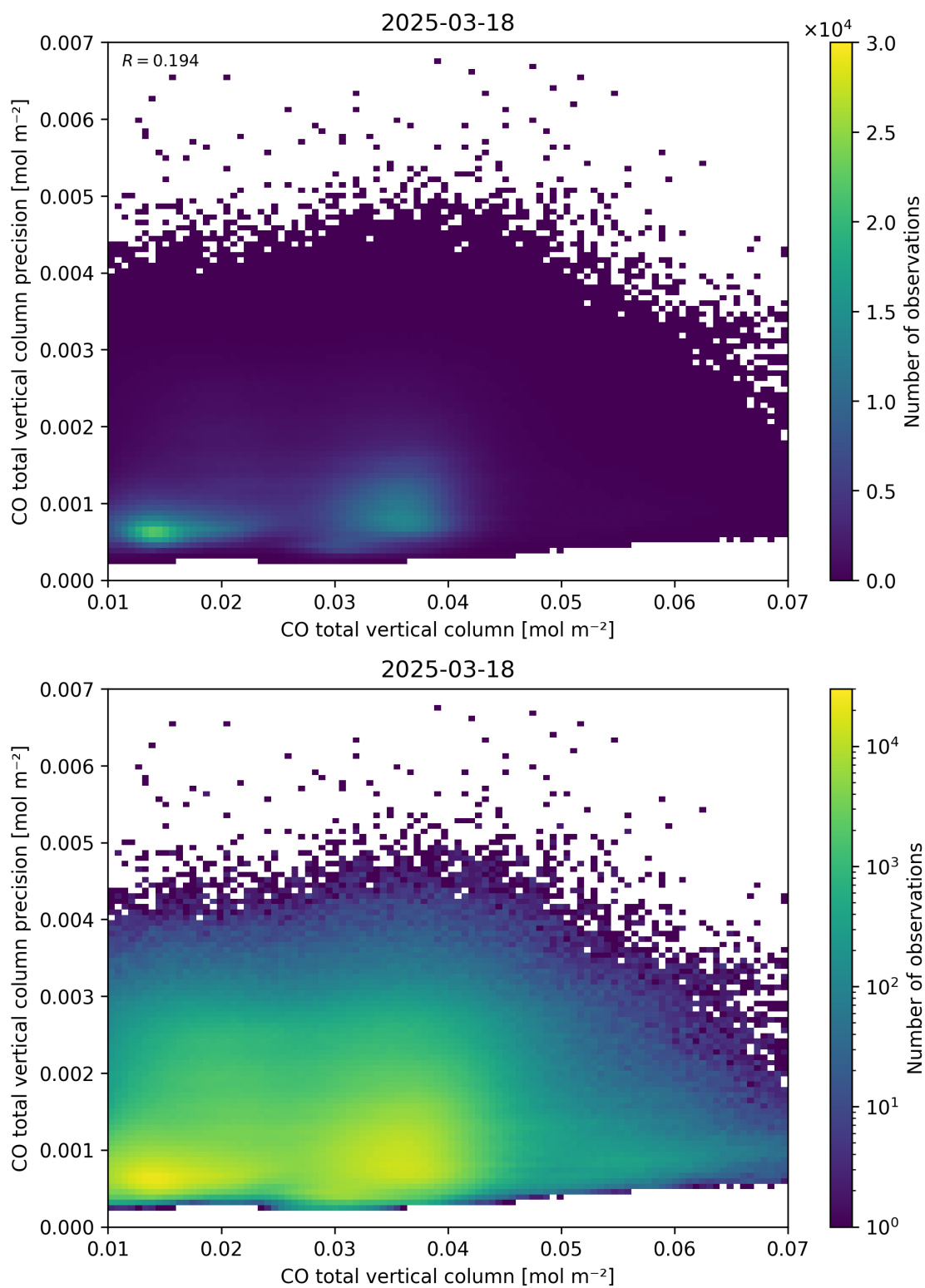
Figure 34: Scatter density plot of “CO total vertical column” against “CO total vertical column precision” for 2025-03-17 to 2025-03-19.
