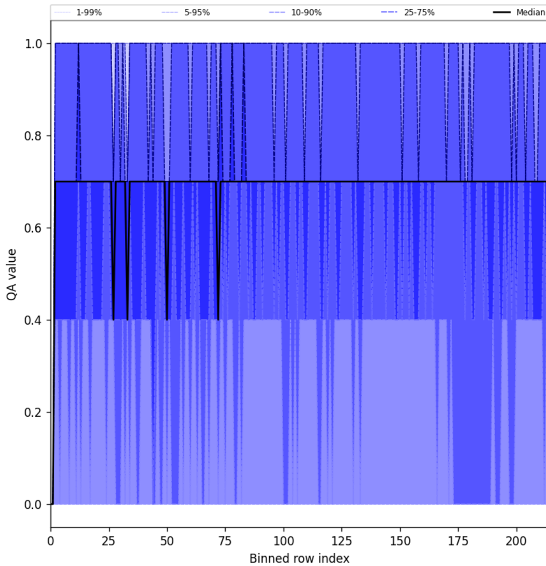
Figure 25: Along track statistics of “QA value” for 2025-03-17 to 2025-03-19
