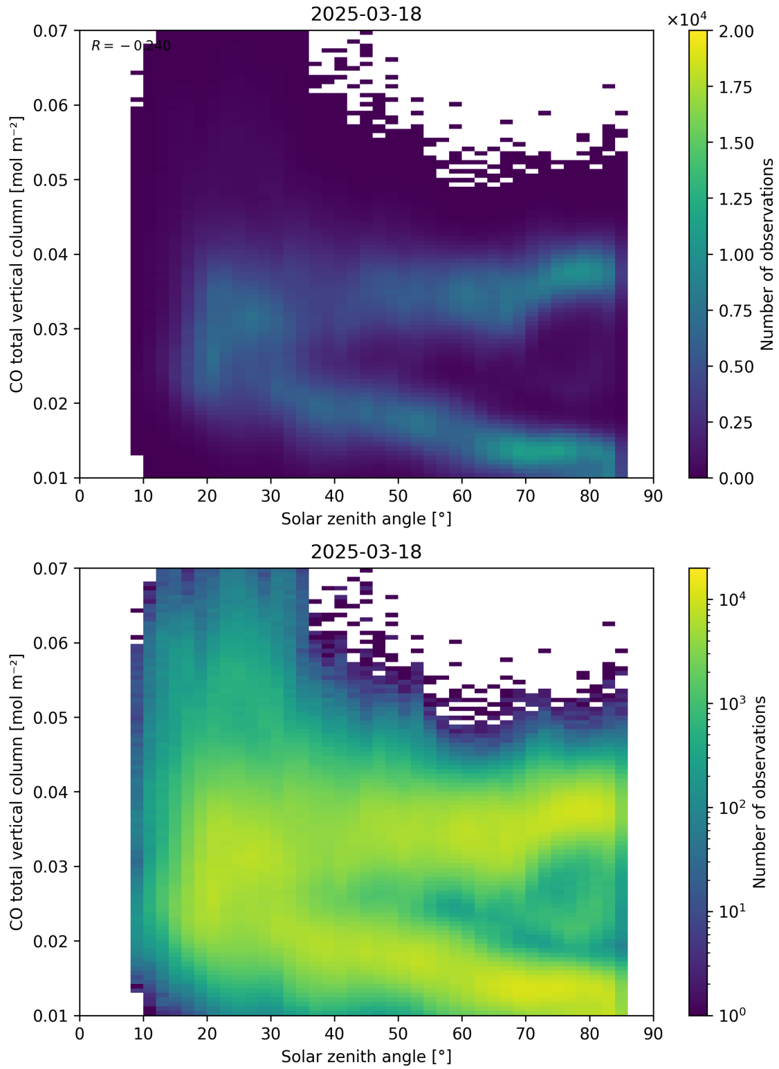
Figure 61: Scatter density plot of “Solar zenith angle” against “CO total vertical column” for 2025-03-17 to 2025-03-19.
