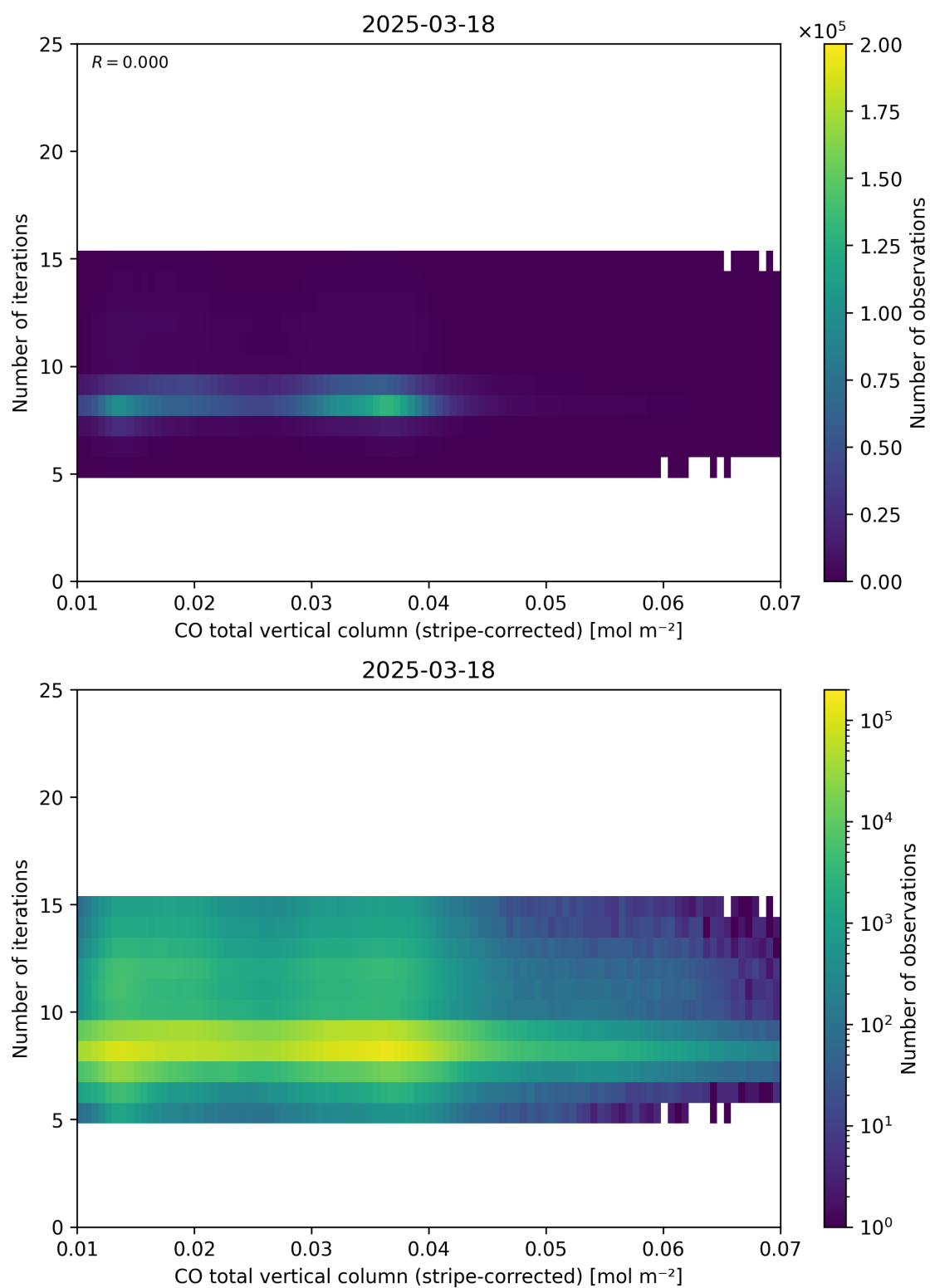
Figure 39: Scatter density plot of “CO total vertical column (stripe-corrected)” against “Number of iterations” for 2025-03-17 to 2025-03-19.
