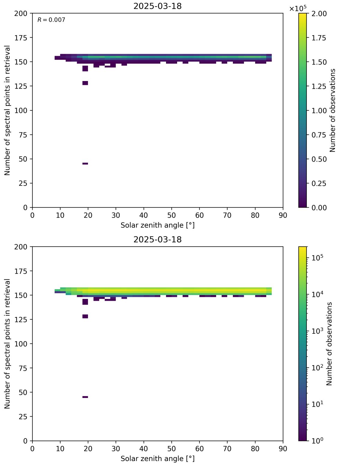
Figure 68: Scatter density plot of “Solar zenith angle” against “Number of spectral points in retrieval” for 2025-03-17 to 2025-03-19.
