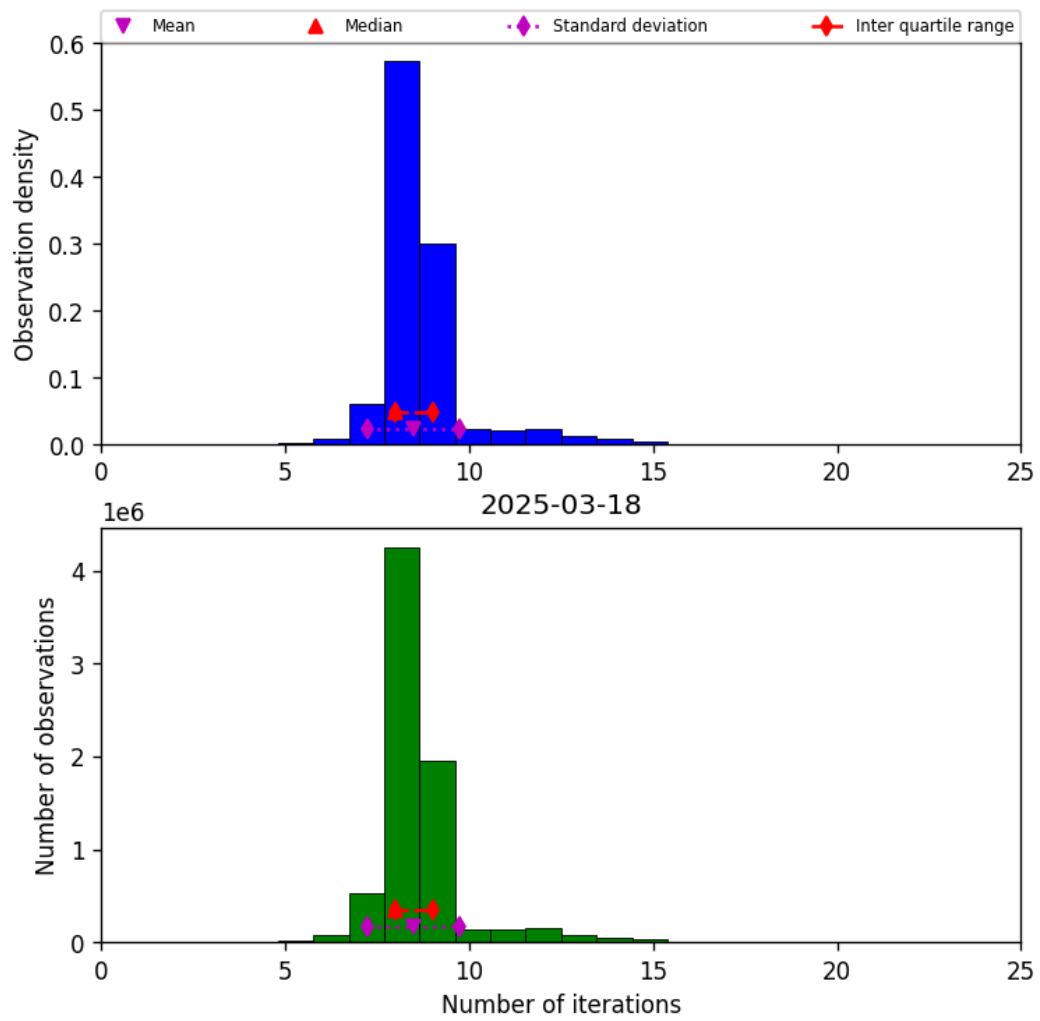
Figure 24: Histogram of “Number of iterations” for 2025-03-17 to 2025-03-19
