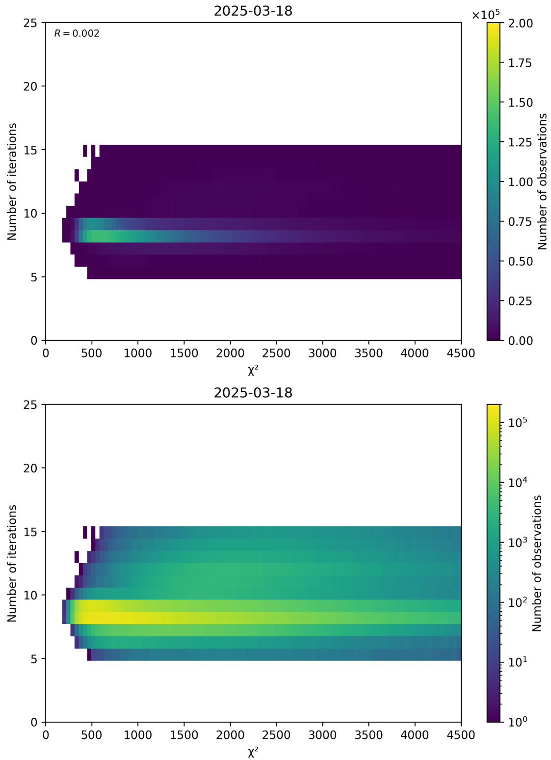
Figure 49: Scatter density plot of “ \chi^2 ” against “Number of iterations” for 2025-03-17 to 2025-03-19.
