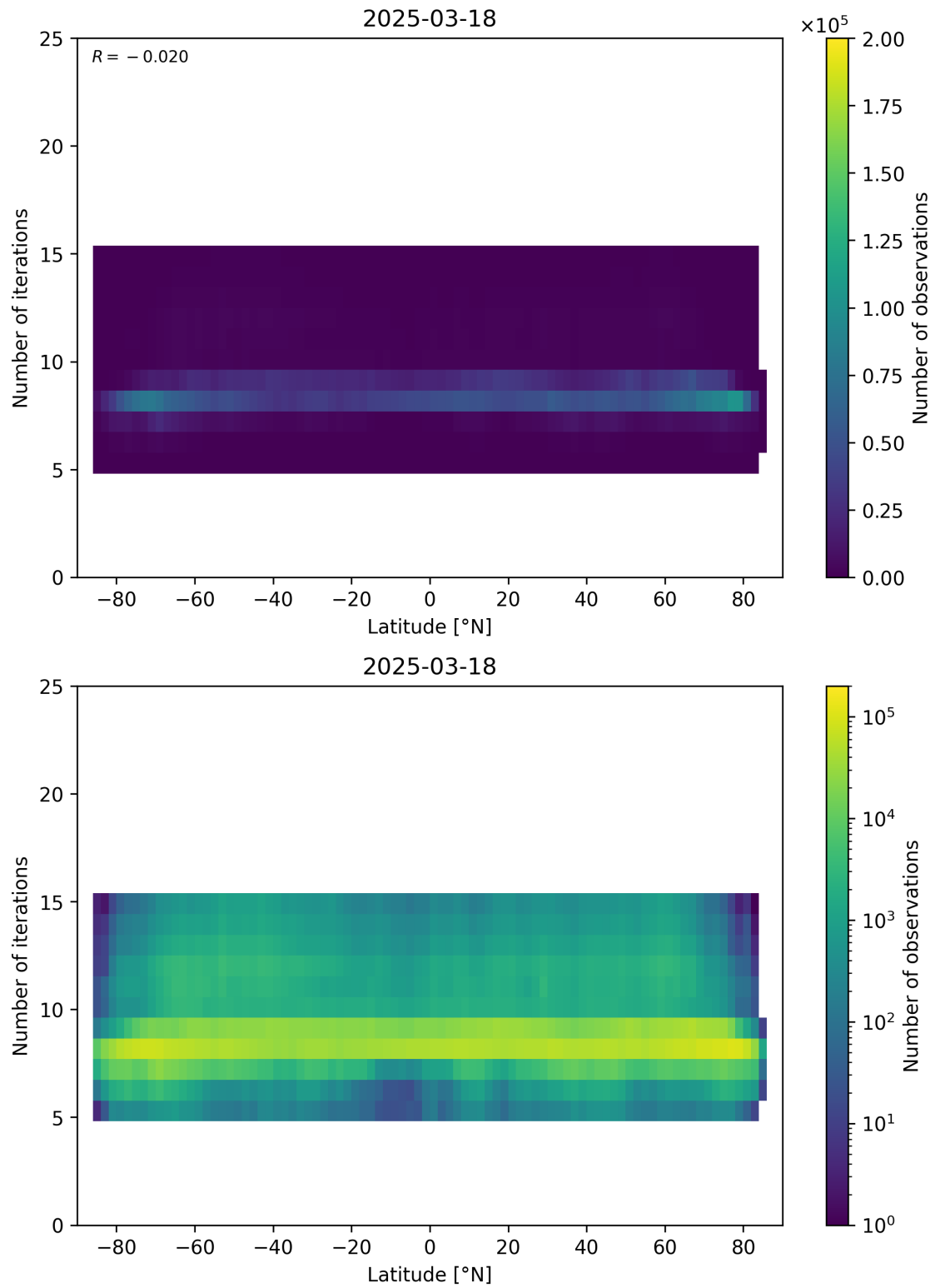
Figure 56: Scatter density plot of “Latitude” against “Number of iterations” for 2025-03-17 to 2025-03-19.
