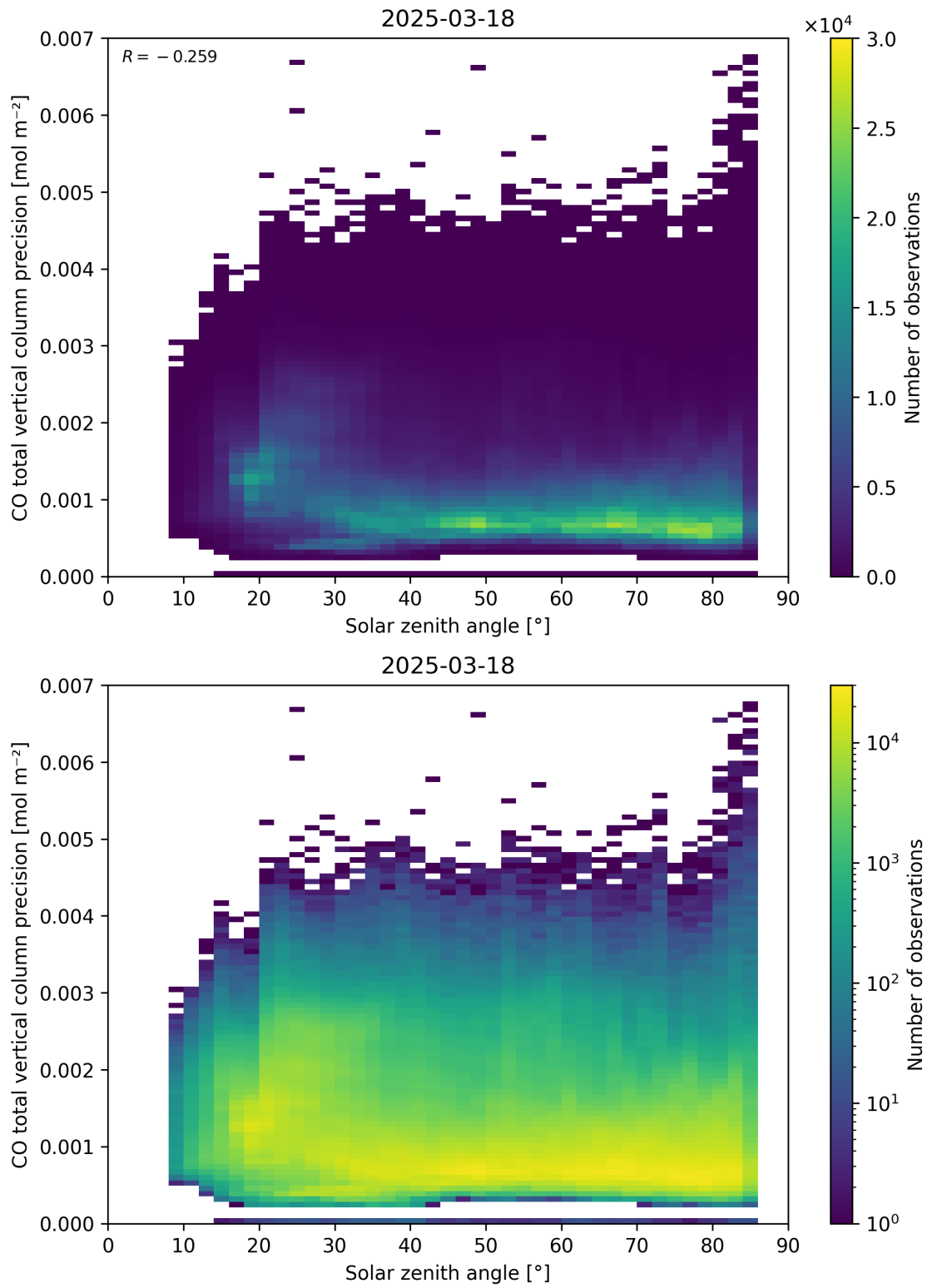
Figure 63: Scatter density plot of “Solar zenith angle” against “CO total vertical column precision” for 2025-03-17 to 2025-03-19.
