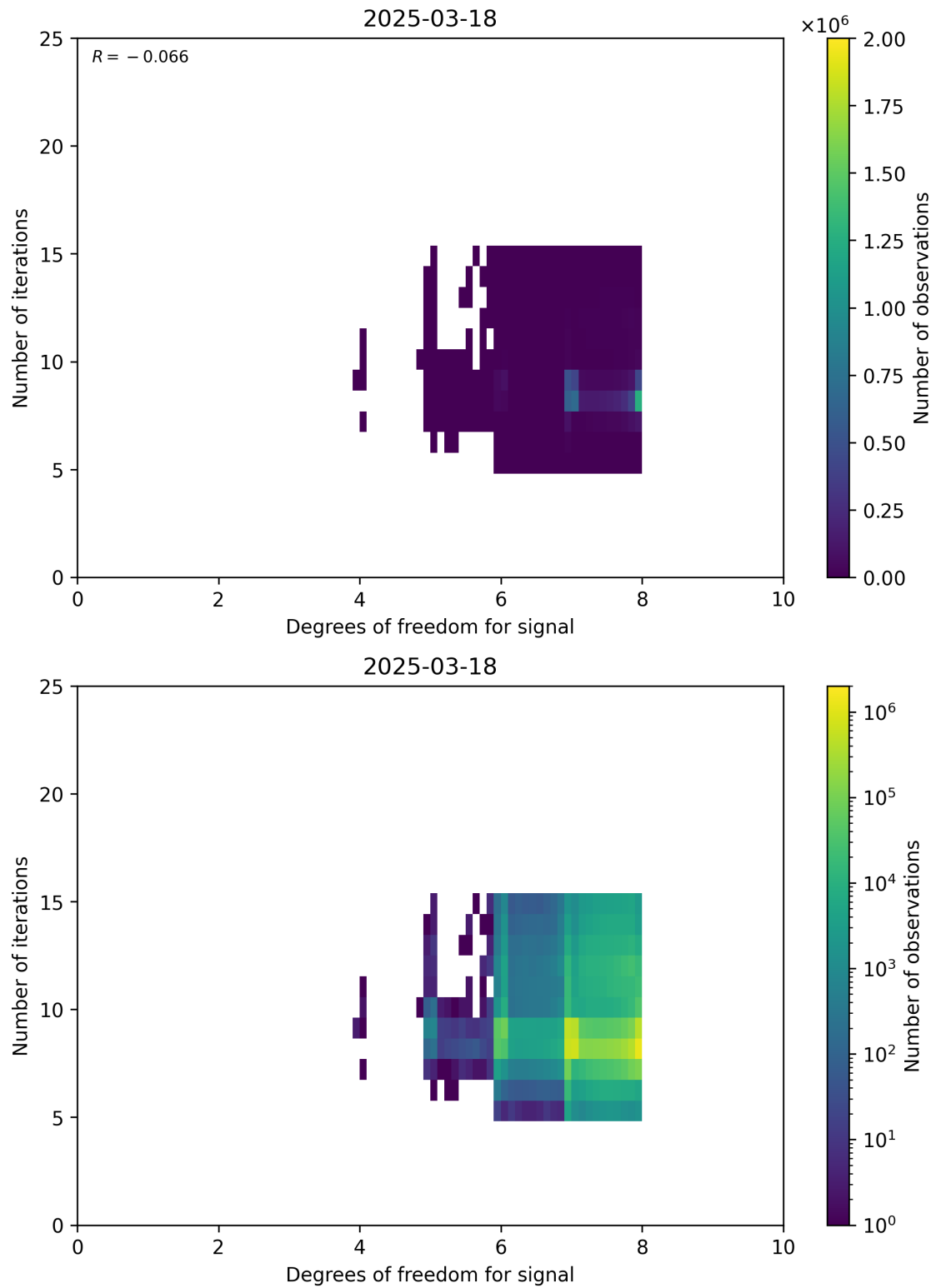
Figure 50: Scatter density plot of “Degrees of freedom for signal” against “Number of iterations” for 2025-03-17 to 2025-03-19.
