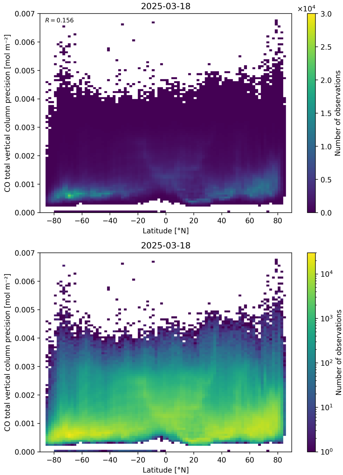
Figure 53: Scatter density plot of “Latitude” against “CO total vertical column precision” for 2025-03-17 to 2025-03-19.
