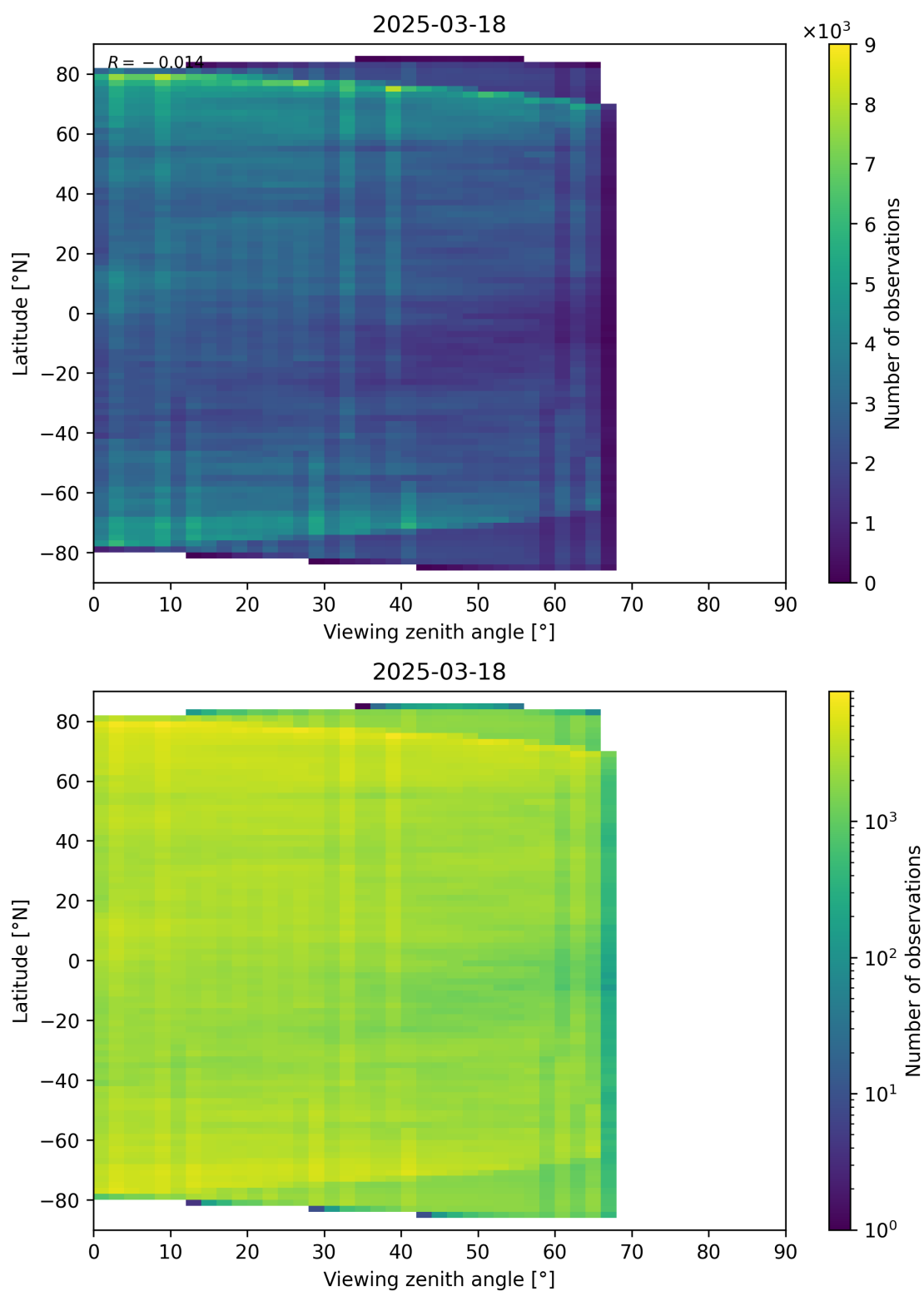
Figure 74: Scatter density plot of “Viewing zenith angle” against “Latitude” for 2025-03-17 to 2025-03-19.
