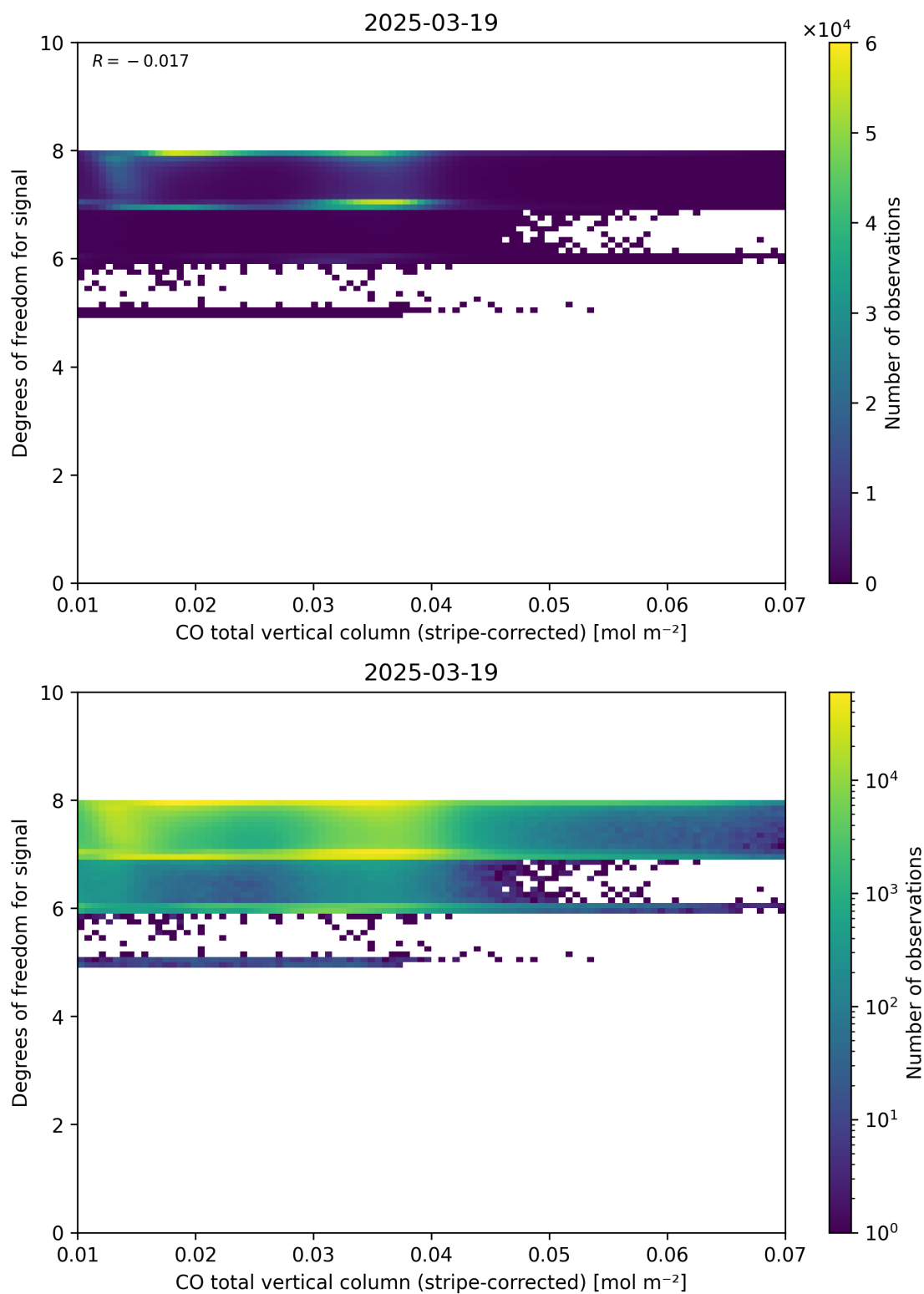
Figure 38: Scatter density plot of “CO total vertical column (stripe-corrected)” against “Degrees of freedom for signal” for 2025-03-18 to 2025-03-20.
