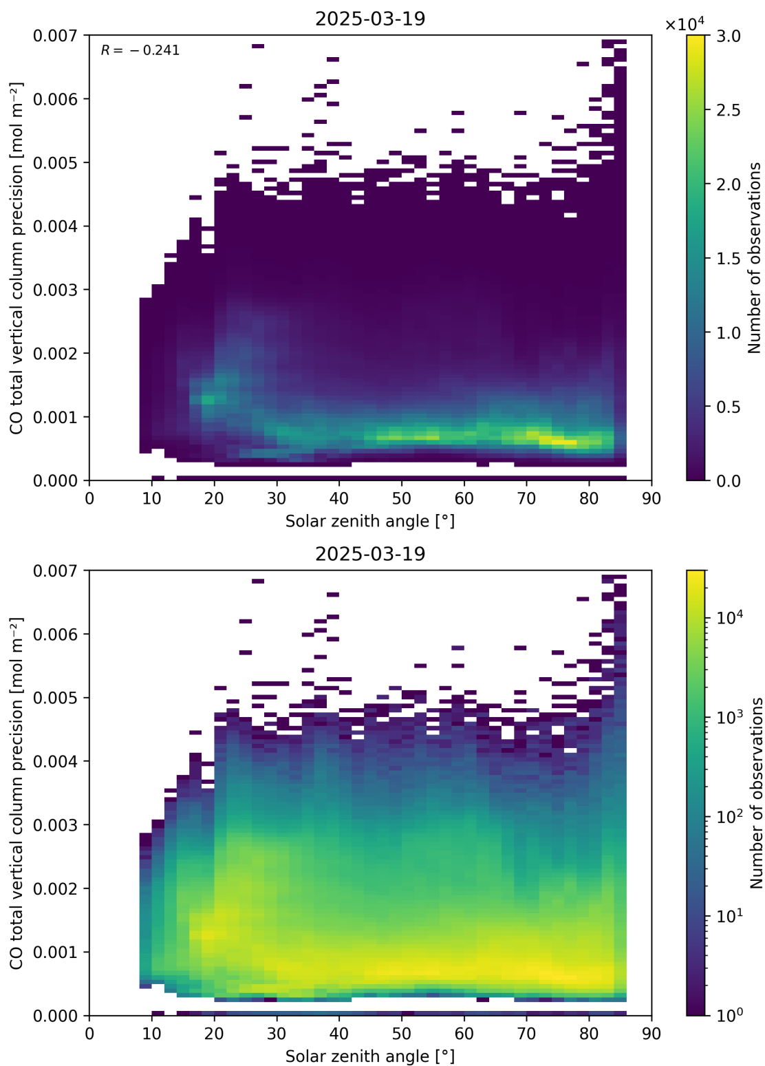
Figure 63: Scatter density plot of “Solar zenith angle” against “CO total vertical column precision” for 2025-03-18 to 2025-03-20.
