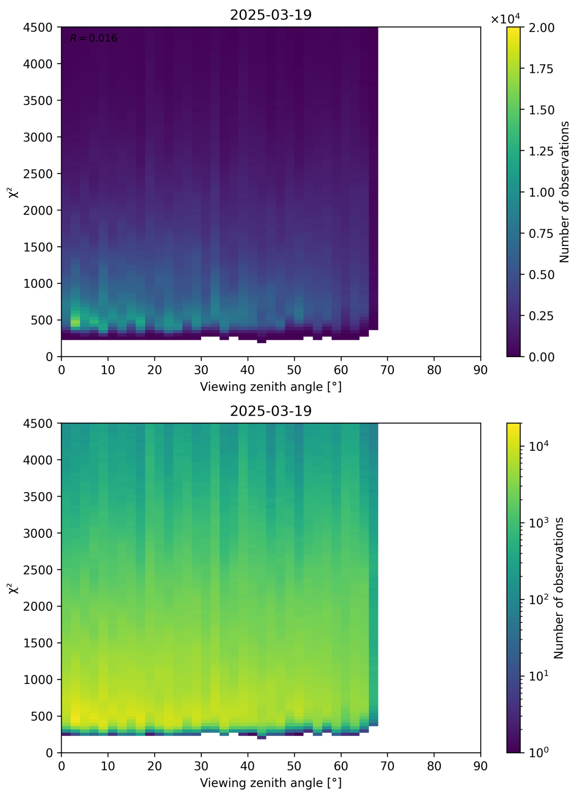
Figure 72: Scatter density plot of “Viewing zenith angle” against “ \chi^2 ” for 2025-03-18 to 2025-03-20.
