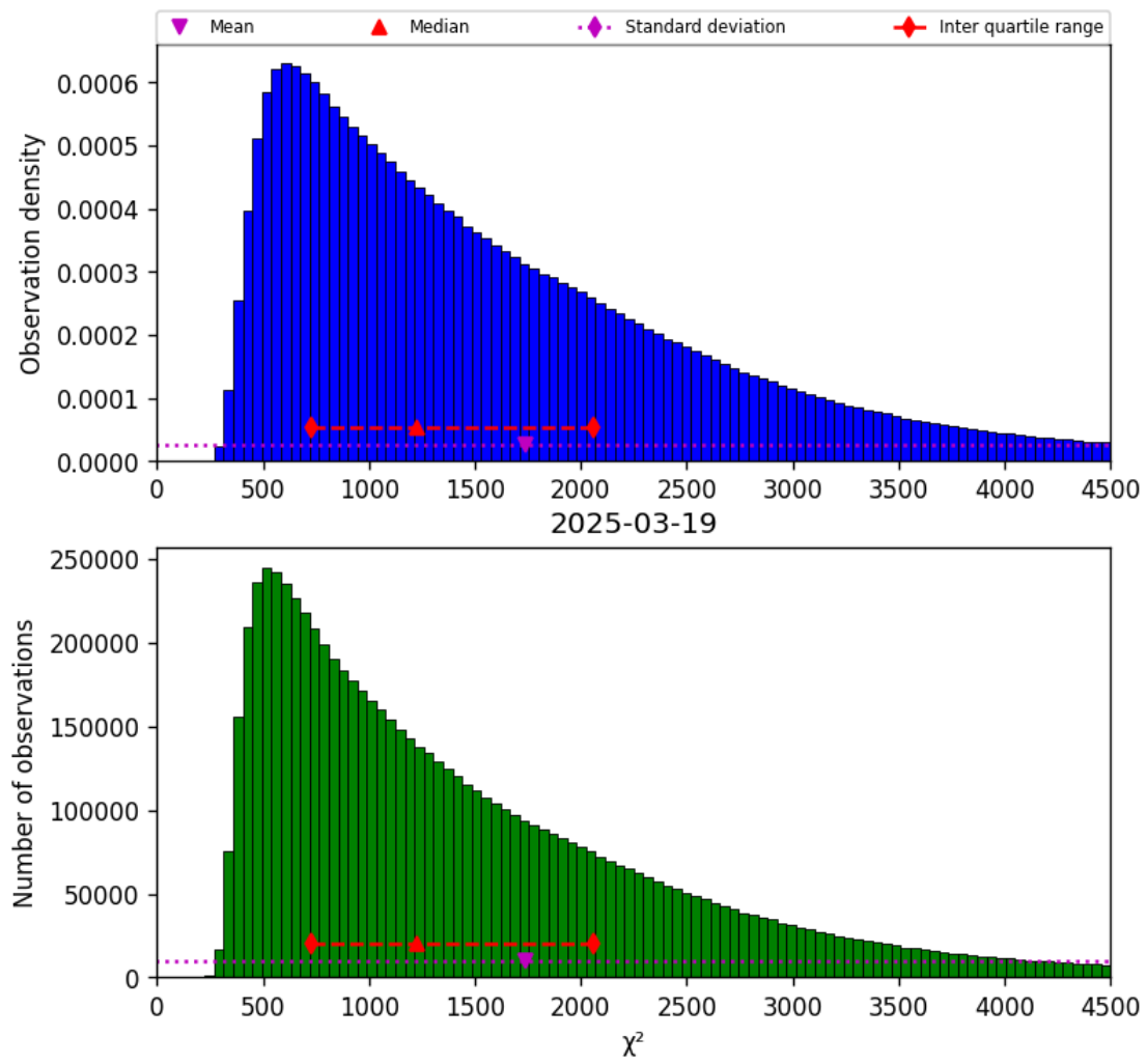
Figure 22: Histogram of “ \chi^2 ” for 2025-03-18 to 2025-03-20
