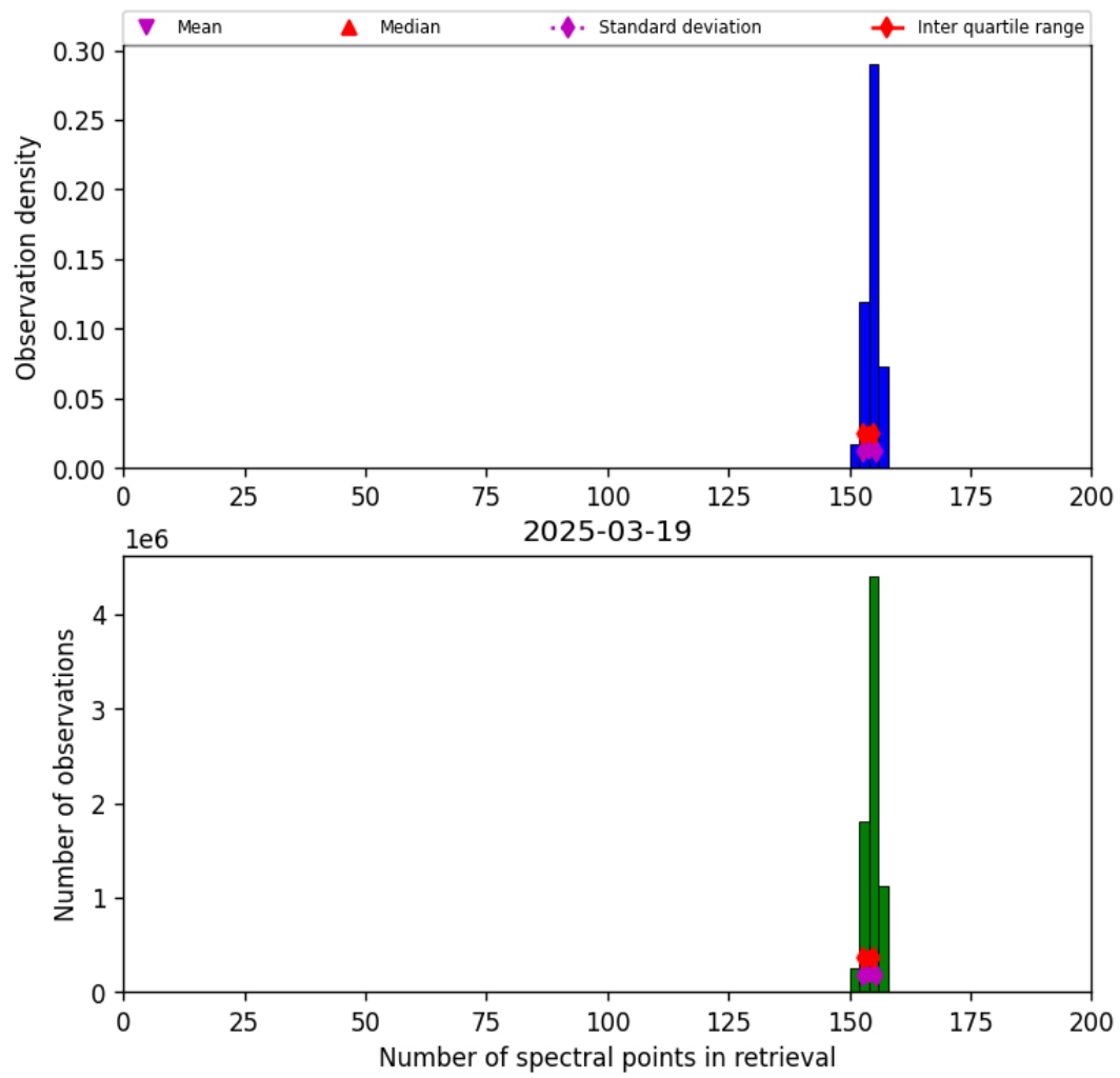
Figure 21: Histogram of “Number of spectral points in retrieval” for 2025-03-18 to 2025-03-20
