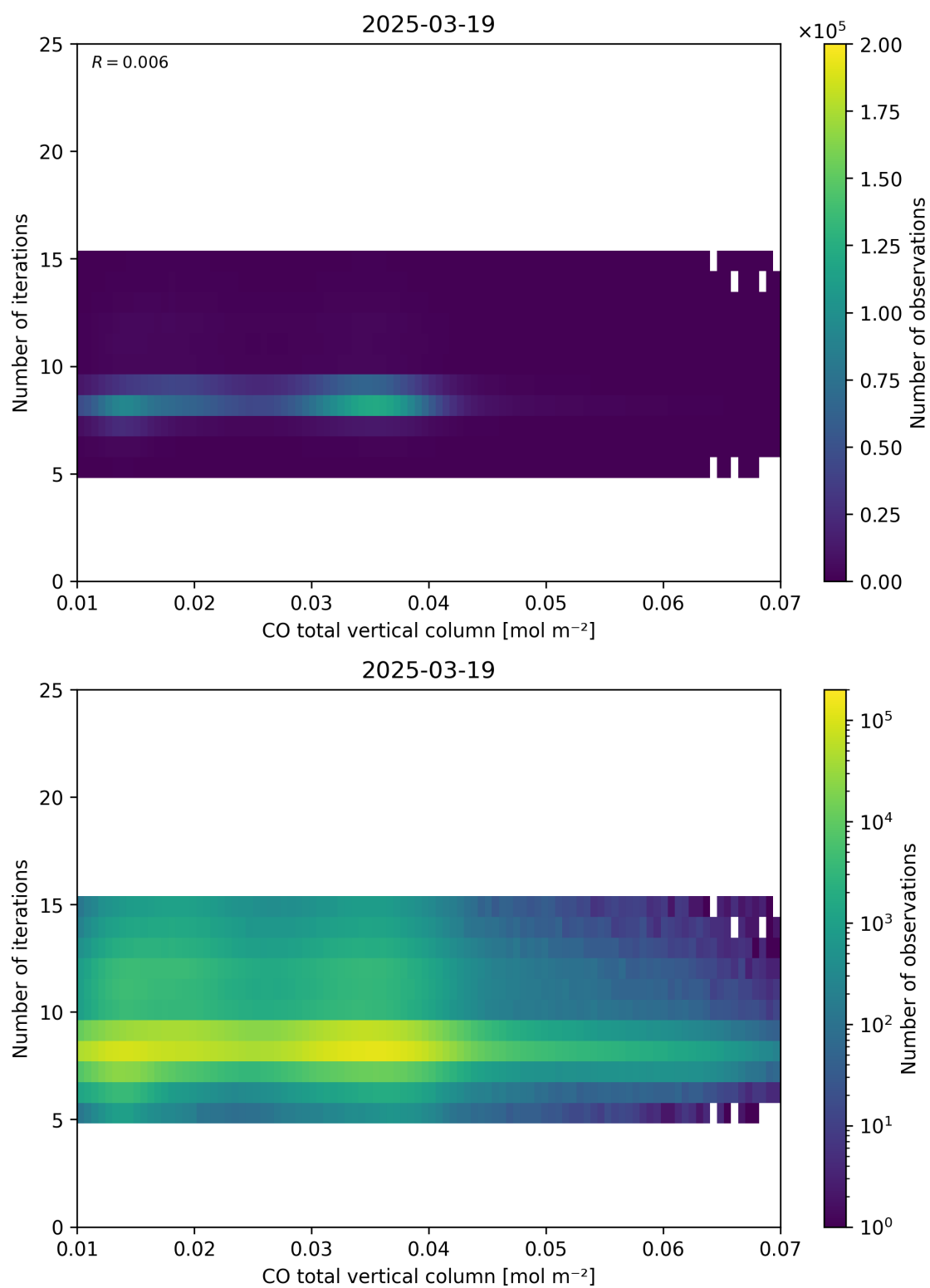
Figure 42: Scatter density plot of “CO total vertical column” against “Number of iterations” for 2025-03-18 to 2025-03-20.
