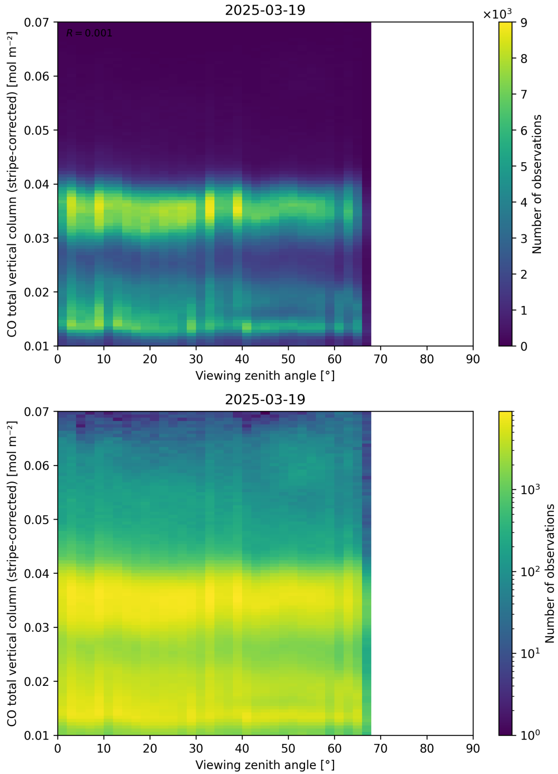
Figure 70: Scatter density plot of “Viewing zenith angle” against “CO total vertical column (stripe-corrected)” for 2025-03-18 to 2025-03-20.
