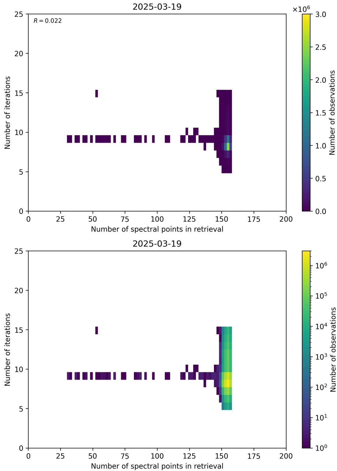
Figure 60: Scatter density plot of “Number of spectral points in retrieval” against “Number of iterations” for 2025-03-18 to 2025-03-20.
