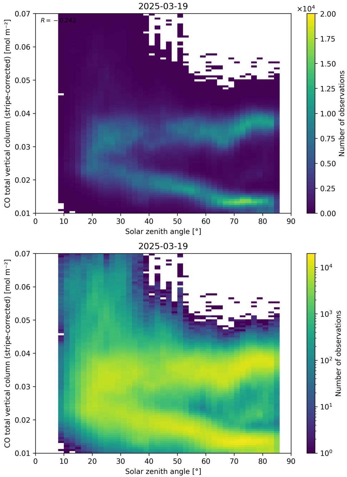
Figure 62: Scatter density plot of “Solar zenith angle” against “CO total vertical column (stripe-corrected)” for 2025-03-18 to 2025-03-20.
