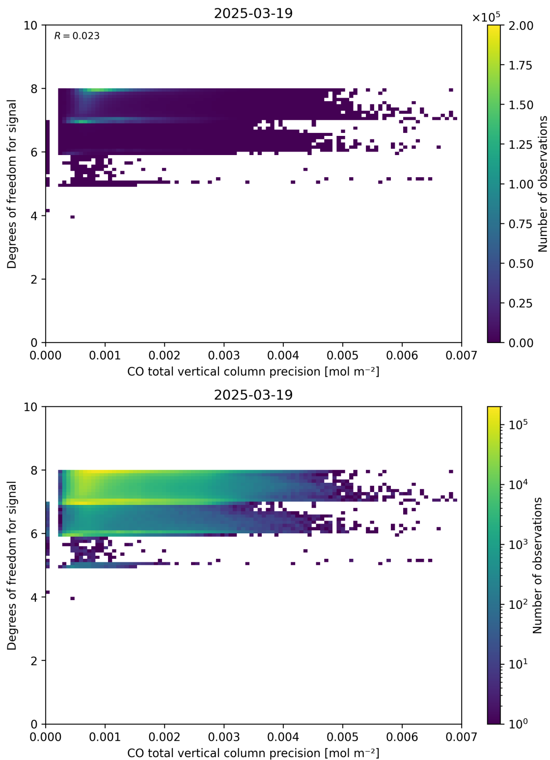
Figure 45: Scatter density plot of “CO total vertical column precision” against “Degrees of freedom for signal” for 2025-03-18 to 2025-03-20.
