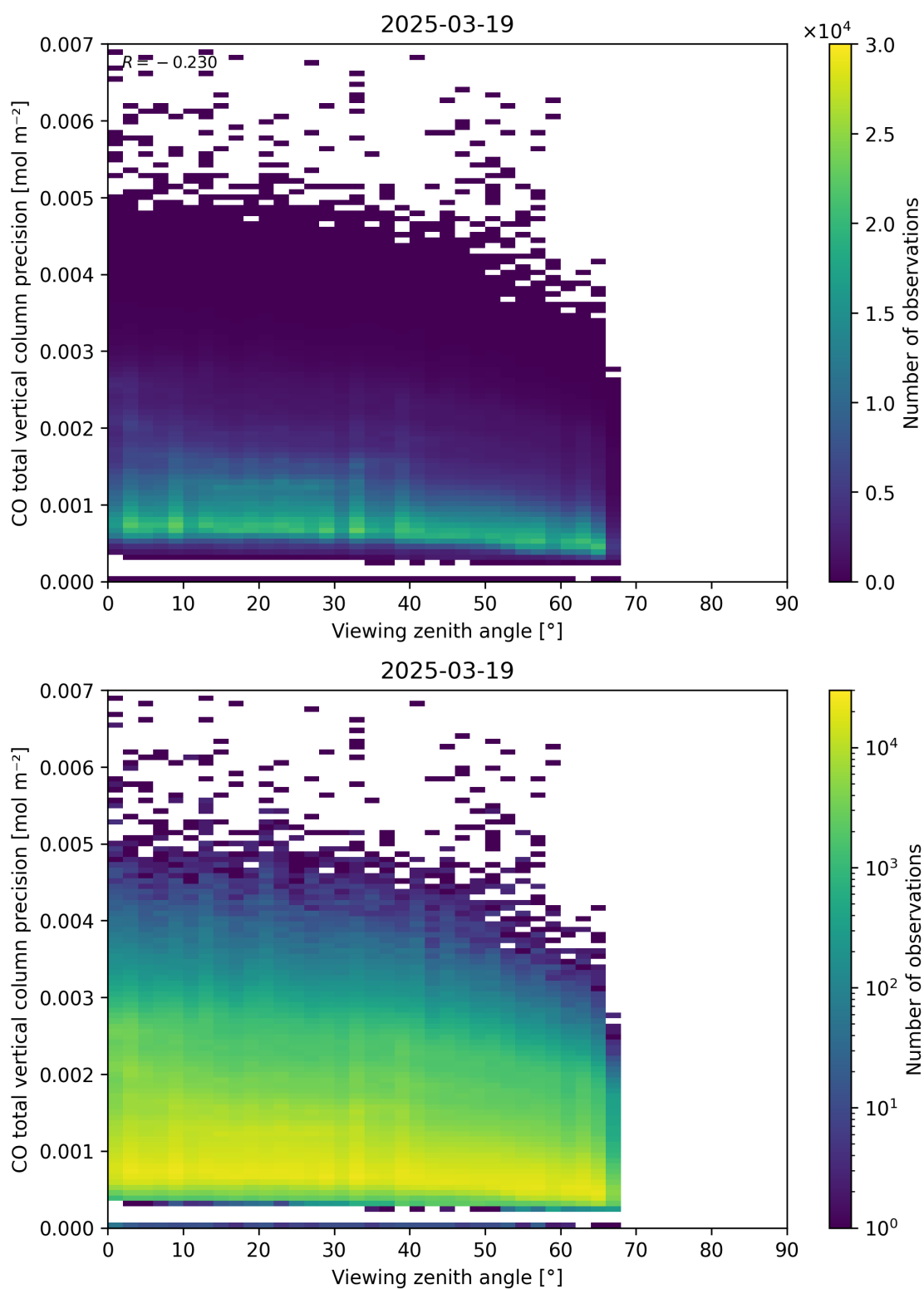
Figure 71: Scatter density plot of “Viewing zenith angle” against “CO total vertical column precision” for 2025-03-18 to 2025-03-20.
