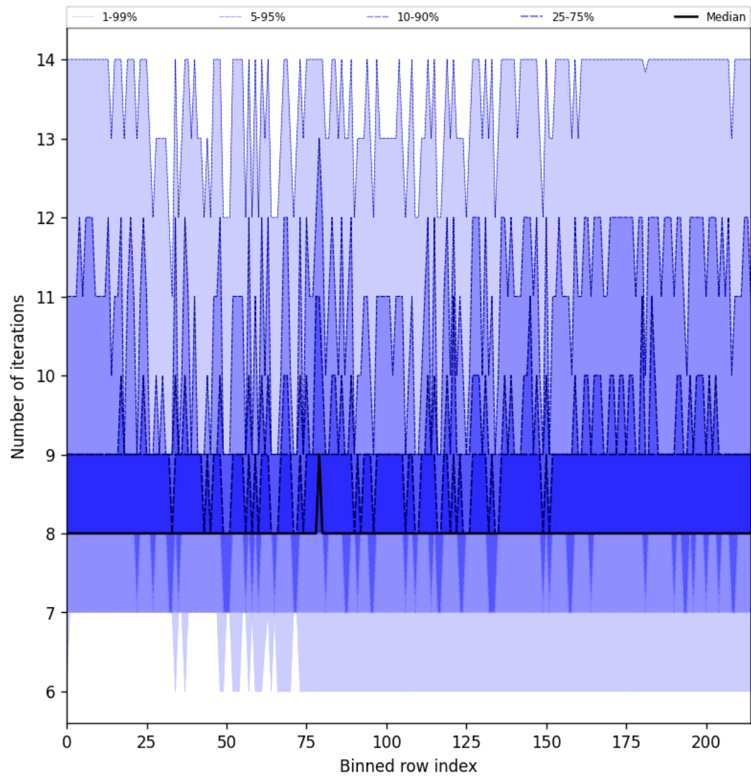
Figure 32: Along track statistics of “Number of iterations” for 2025-03-18 to 2025-03-20
