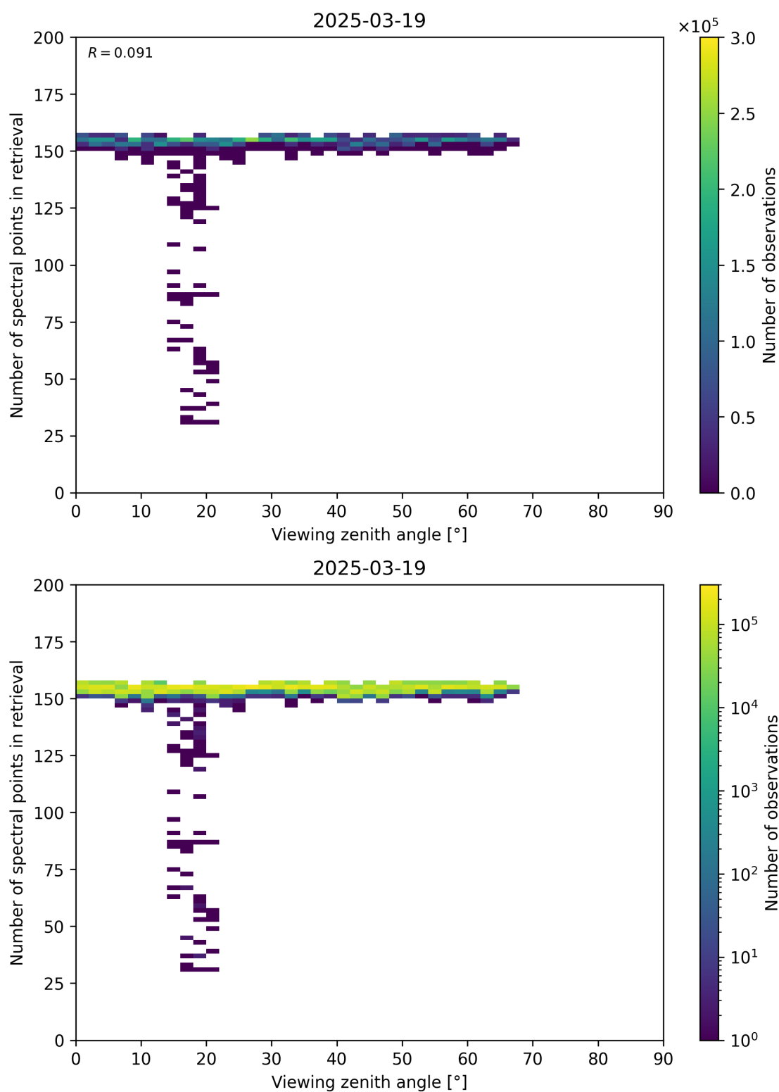
Figure 76: Scatter density plot of “Viewing zenith angle” against “Number of spectral points in retrieval” for 2025-03-18 to 2025-03-20.
