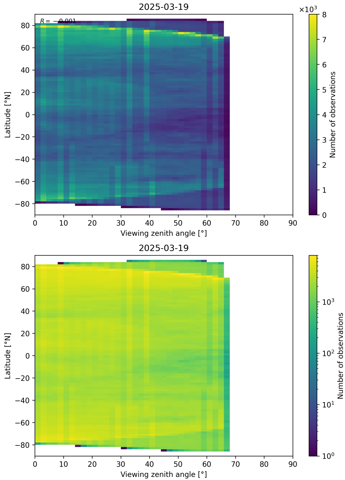
Figure 74: Scatter density plot of “Viewing zenith angle” against “Latitude” for 2025-03-18 to 2025-03-20.
