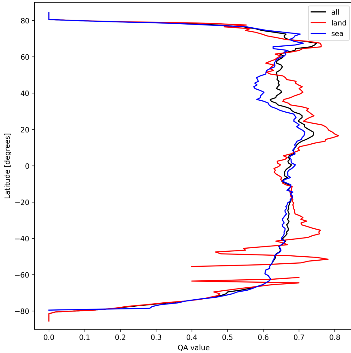
Figure 9: Zonal average of “QA value” for 2025-03-18 to 2025-03-20.
