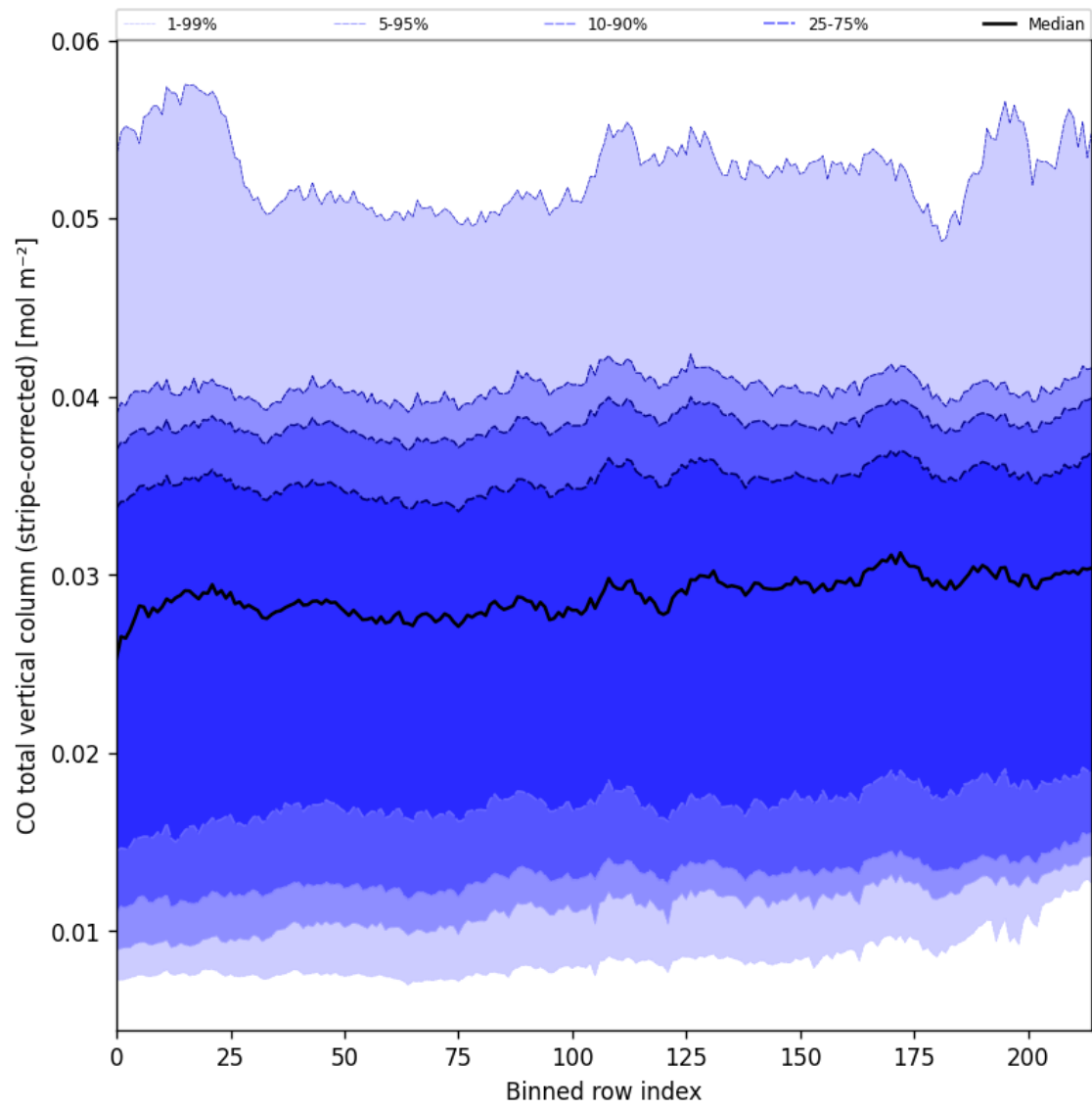
Figure 27: Along track statistics of “CO total vertical column (stripe-corrected)” for 2025-03-18 to 2025-03-20
