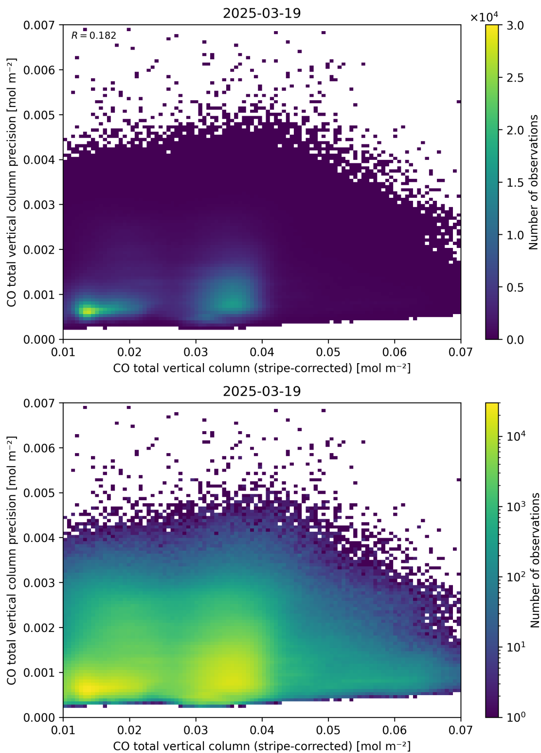
Figure 36: Scatter density plot of “CO total vertical column (stripe-corrected)” against “CO total vertical column precision” for 2025-03-18 to 2025-03-20.
