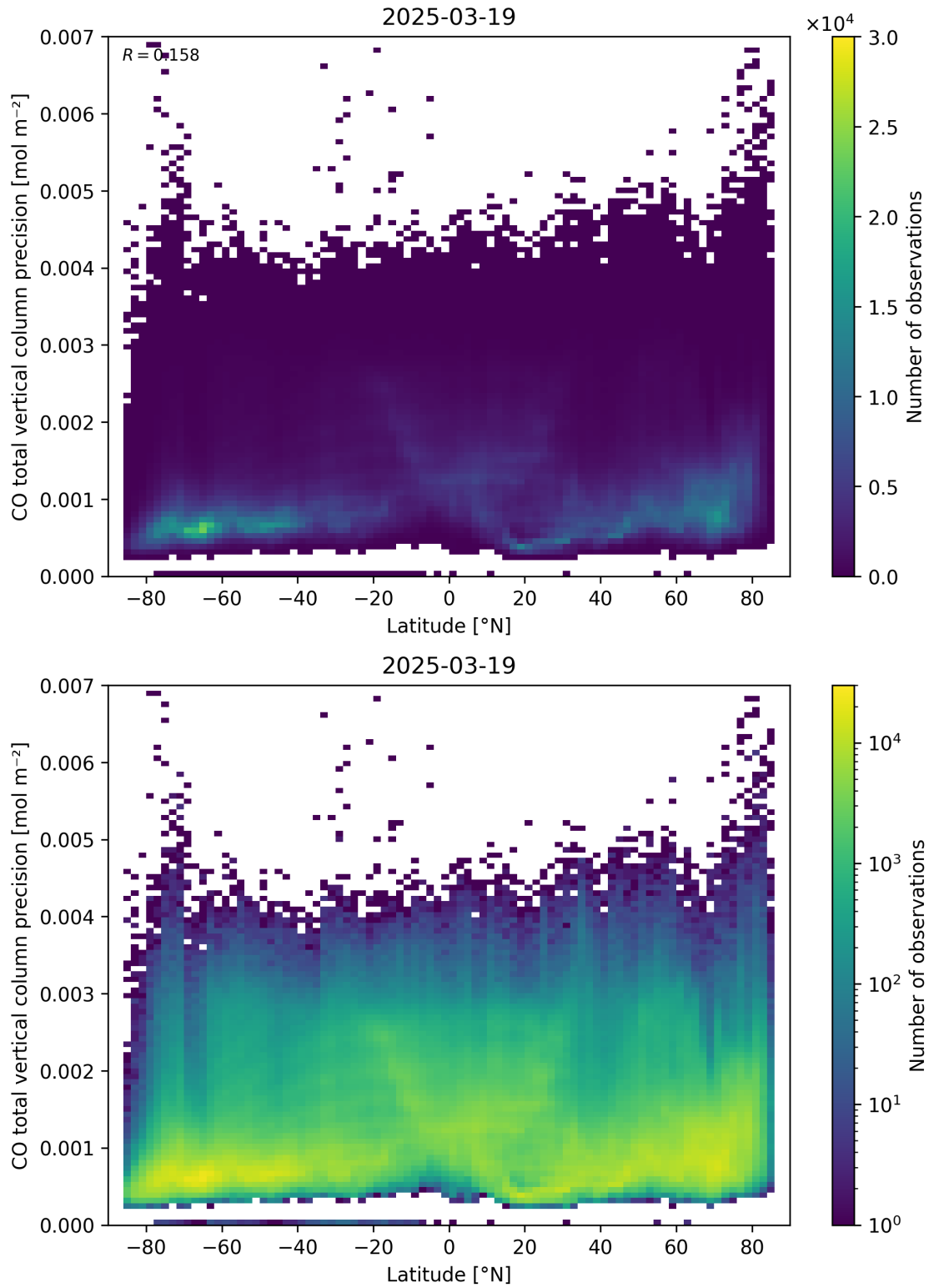
Figure 53: Scatter density plot of “Latitude” against “CO total vertical column precision” for 2025-03-18 to 2025-03-20.
