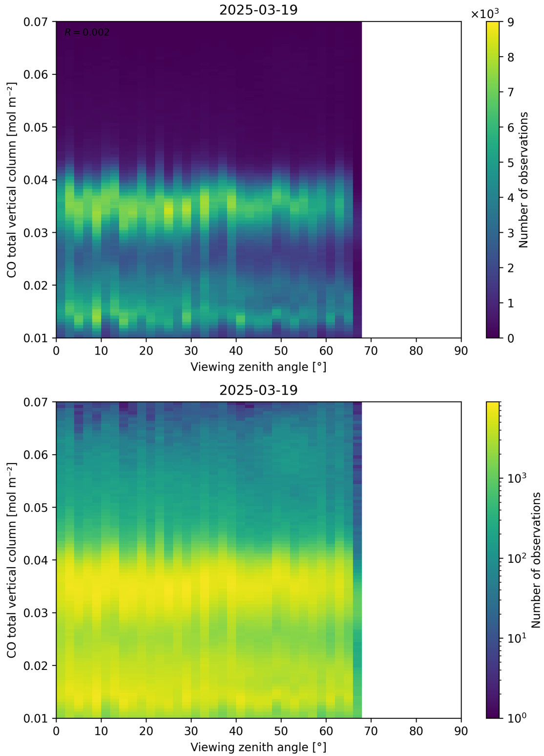
Figure 69: Scatter density plot of “Viewing zenith angle” against “CO total vertical column” for 2025-03-18 to 2025-03-20.
