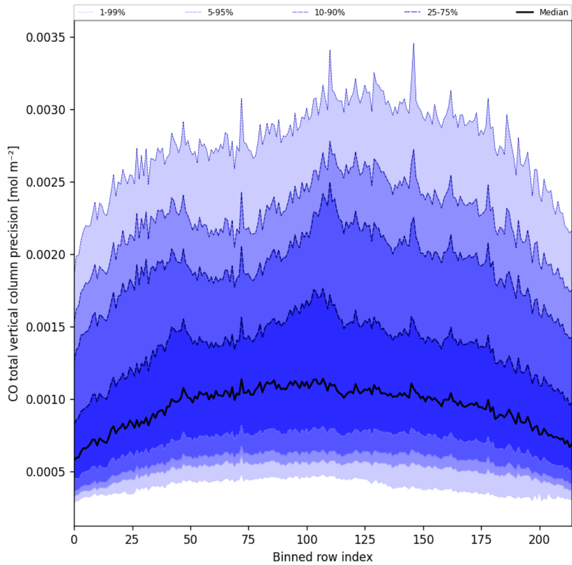
Figure 28: Along track statistics of “CO total vertical column precision” for 2025-03-18 to 2025-03-20
