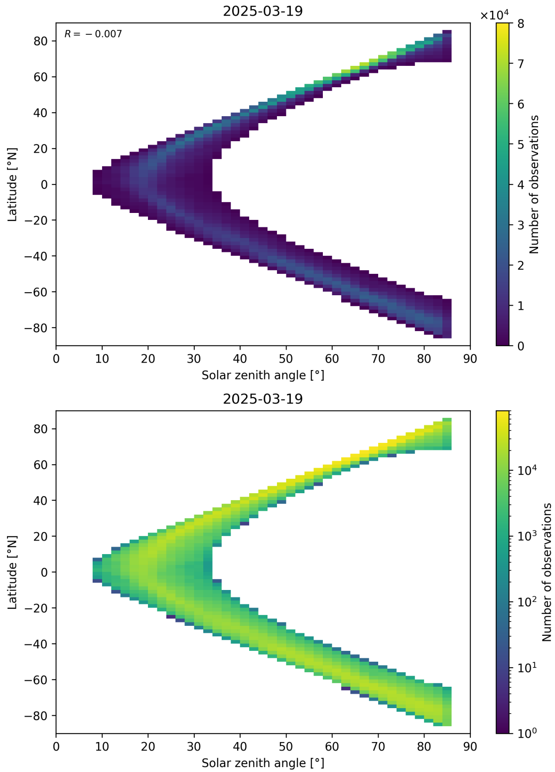
Figure 66: Scatter density plot of “Solar zenith angle” against “Latitude” for 2025-03-18 to 2025-03-20.
