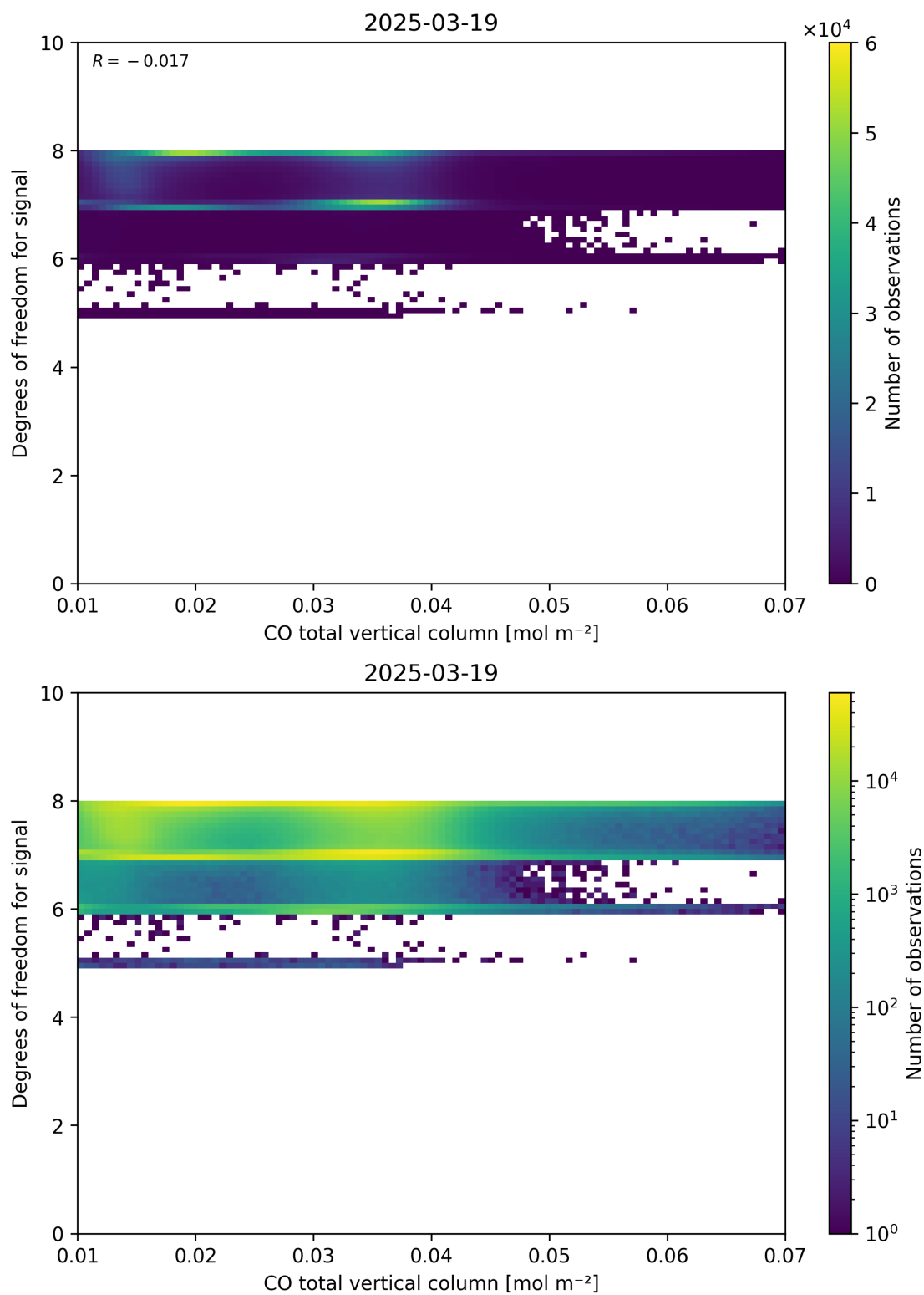
Figure 41: Scatter density plot of “CO total vertical column” against “Degrees of freedom for signal” for 2025-03-18 to 2025-03-20.
