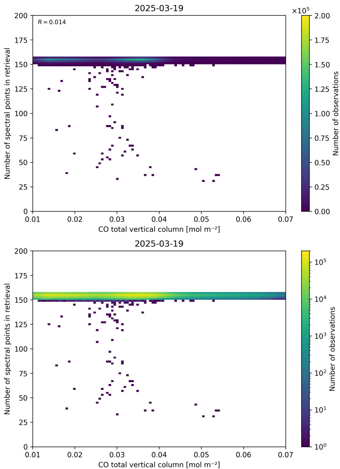
Figure 43: Scatter density plot of “CO total vertical column” against “Number of spectral points in retrieval” for 2025-03-18 to 2025-03-20.
