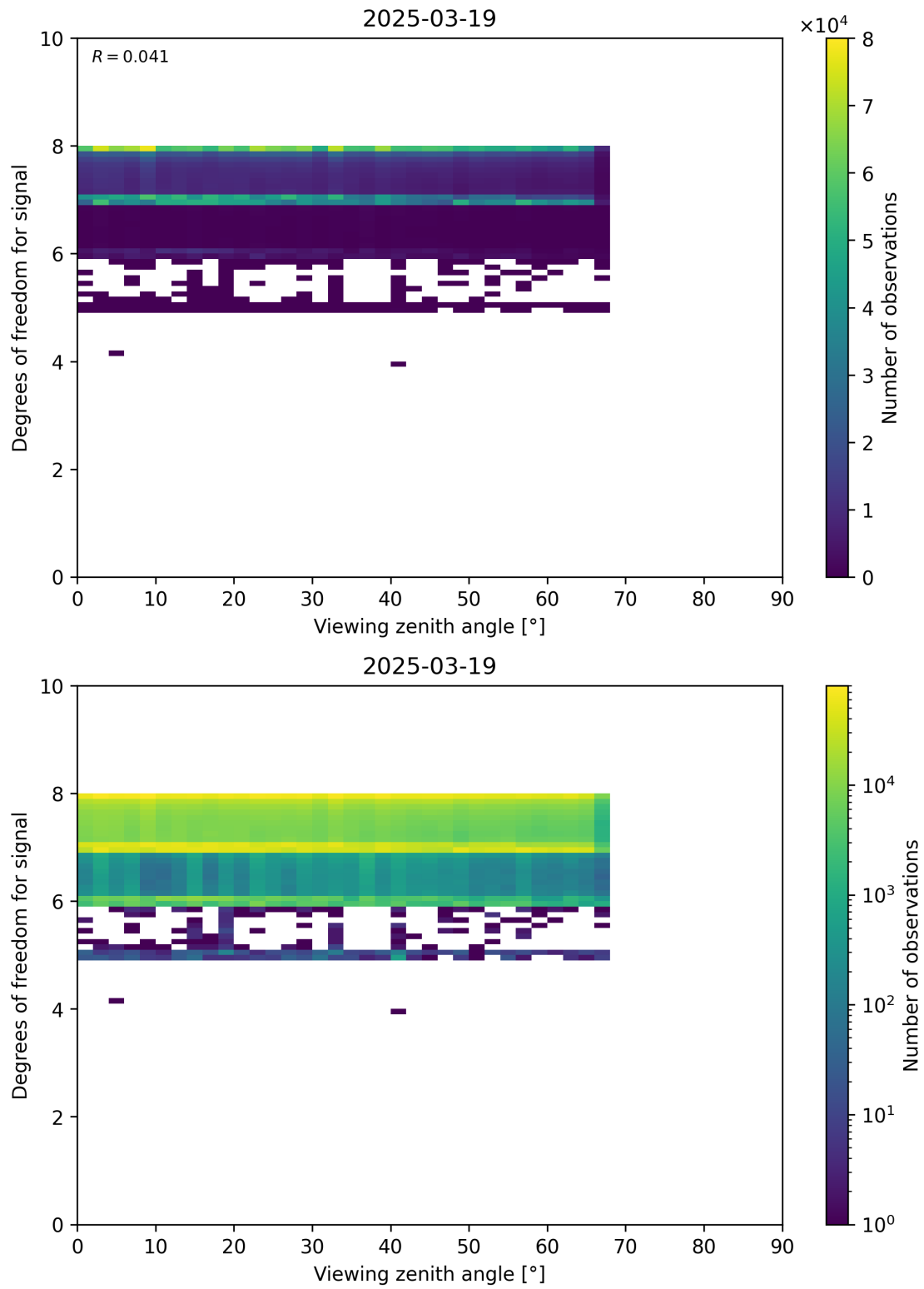
Figure 73: Scatter density plot of “Viewing zenith angle” against “Degrees of freedom for signal” for 2025-03-18 to 2025-03-20.
