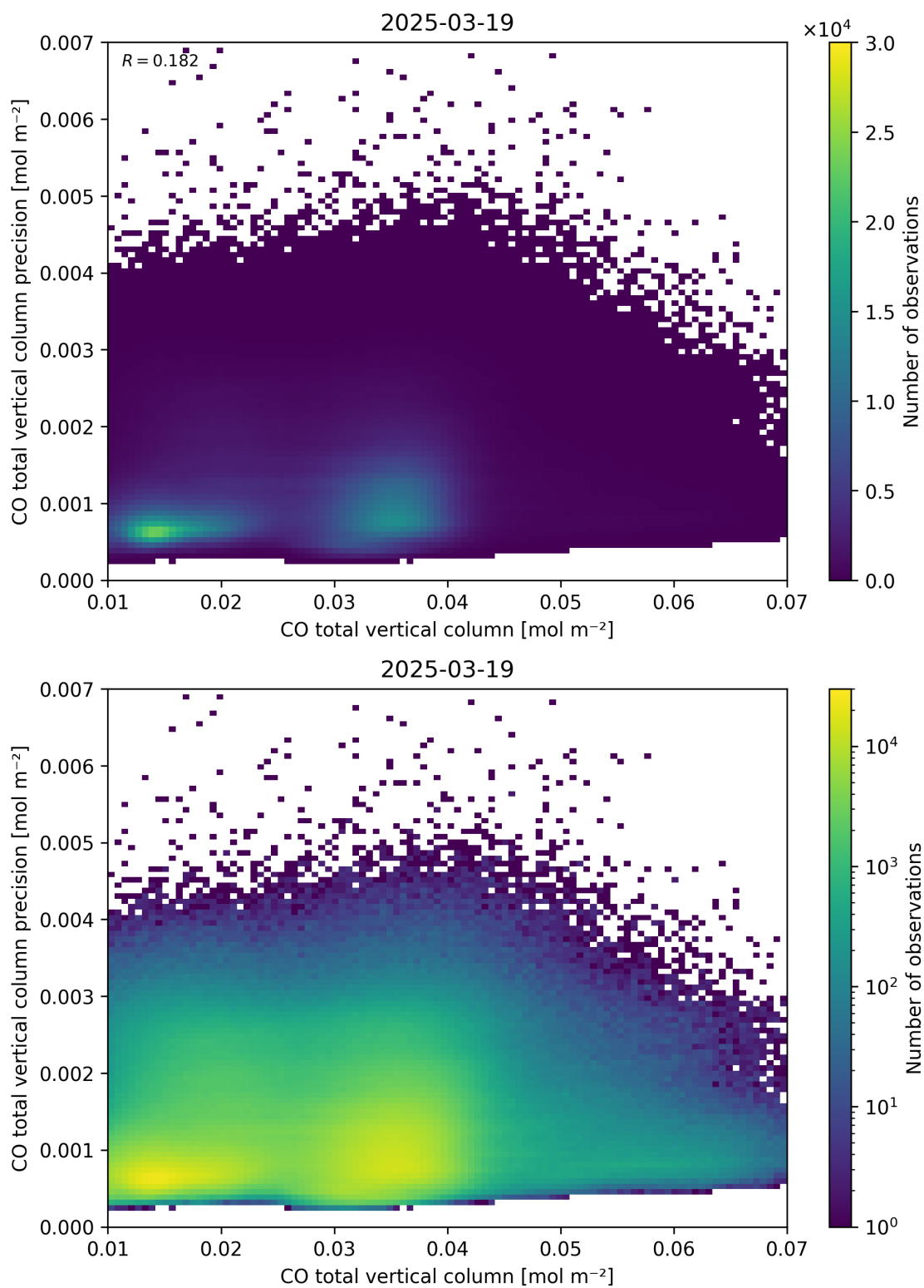
Figure 34: Scatter density plot of “CO total vertical column” against “CO total vertical column precision” for 2025-03-18 to 2025-03-20.
