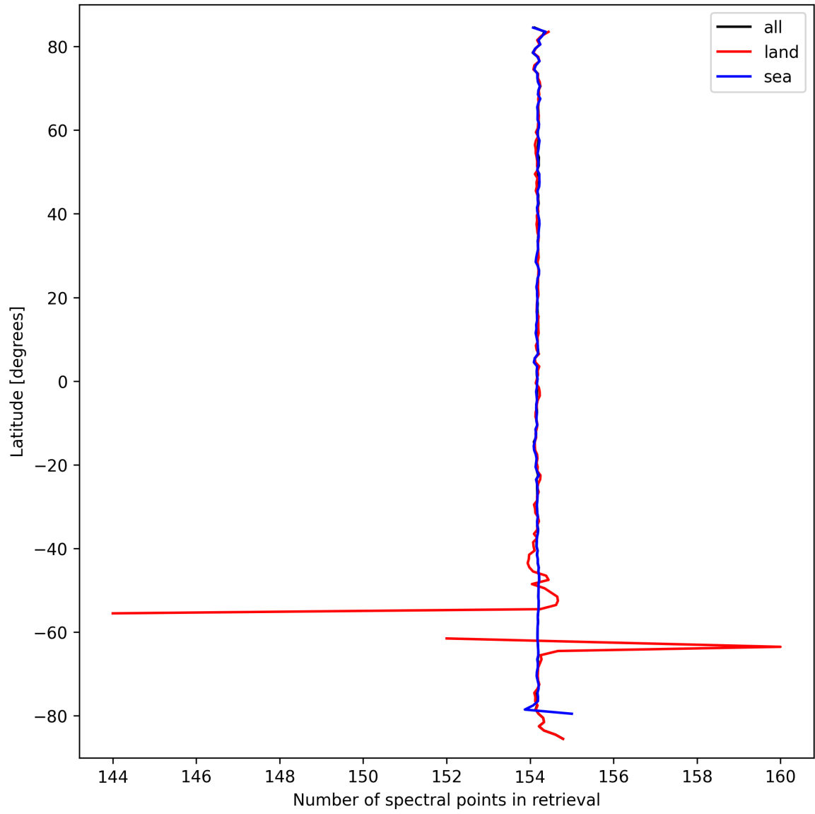
Figure 13: Zonal average of “Number of spectral points in retrieval” for 2025-03-18 to 2025-03-20.
