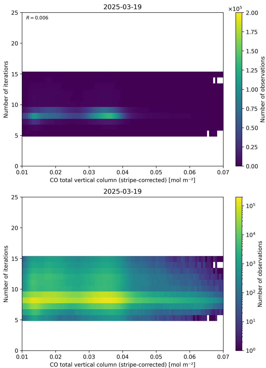
Figure 39: Scatter density plot of “CO total vertical column (stripe-corrected)” against “Number of iterations” for 2025-03-18 to 2025-03-20.
