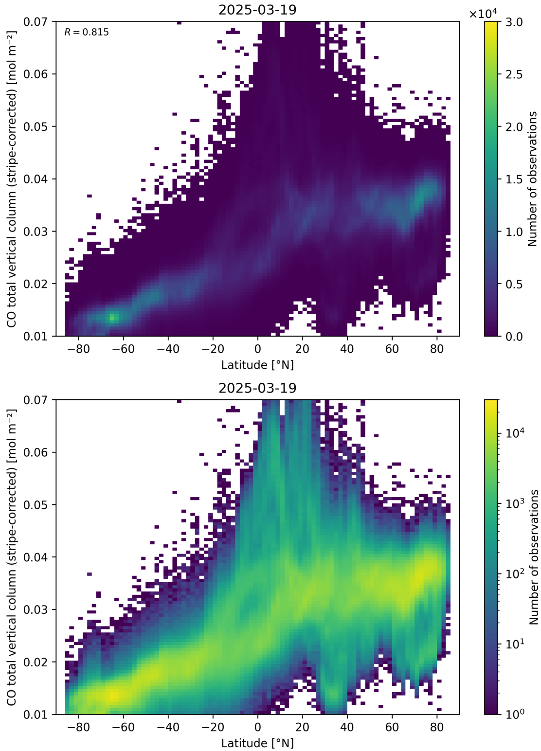
Figure 52: Scatter density plot of “Latitude” against “CO total vertical column (stripe-corrected)” for 2025-03-18 to 2025-03-20.
