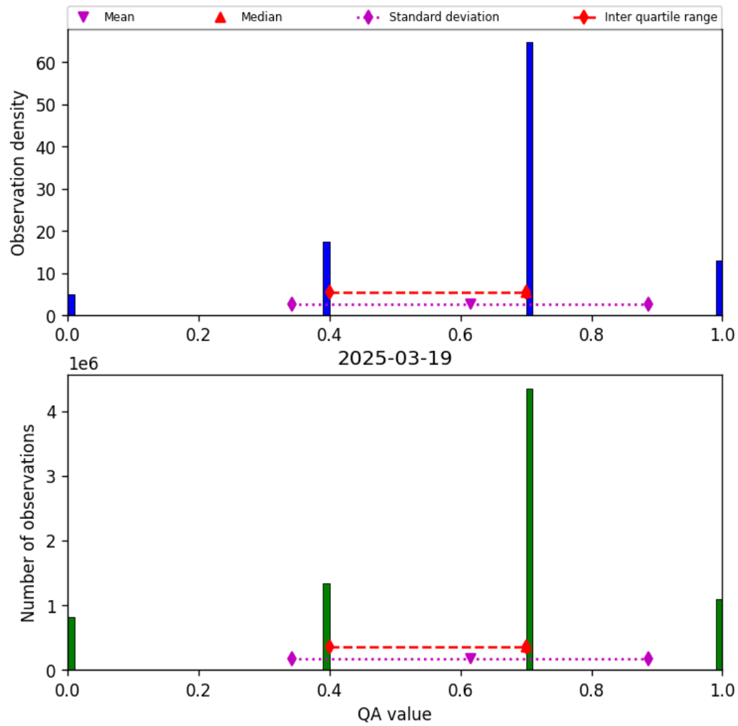
Figure 17: Histogram of “QA value” for 2025-03-18 to 2025-03-20
