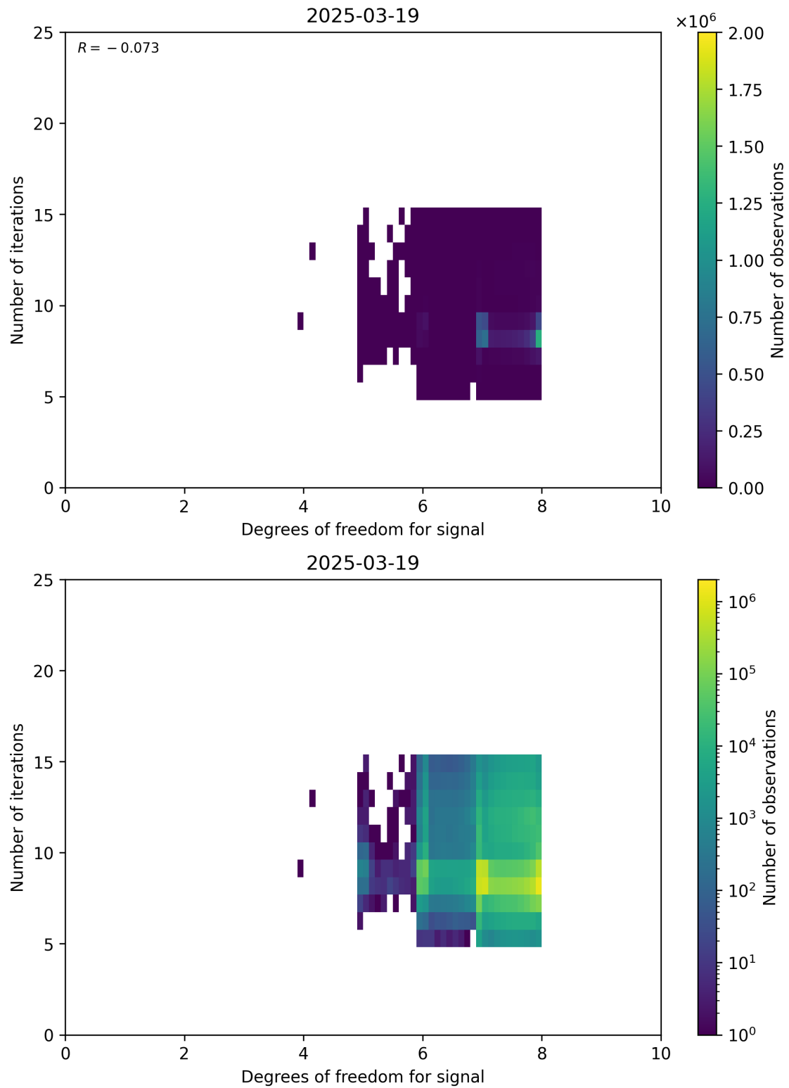
Figure 50: Scatter density plot of “Degrees of freedom for signal” against “Number of iterations” for 2025-03-18 to 2025-03-20.
