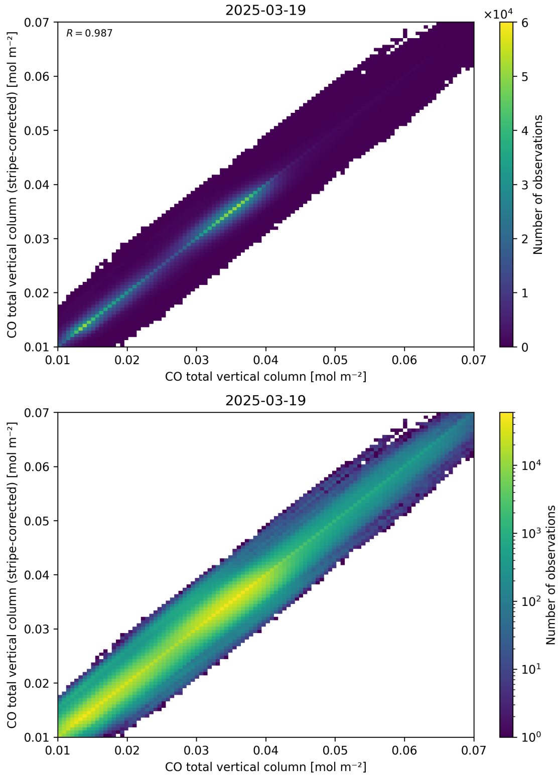
Figure 33: Scatter density plot of “CO total vertical column” against “CO total vertical column (stripe-corrected)” for 2025-03-18 to 2025-03-20.
