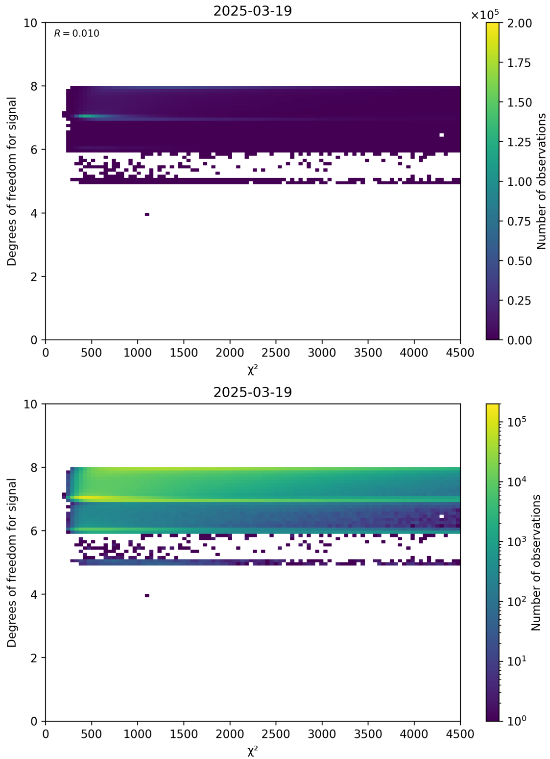
Figure 48: Scatter density plot of “ \chi^2 ” against “Degrees of freedom for signal” for 2025-03-18 to 2025-03-20.
