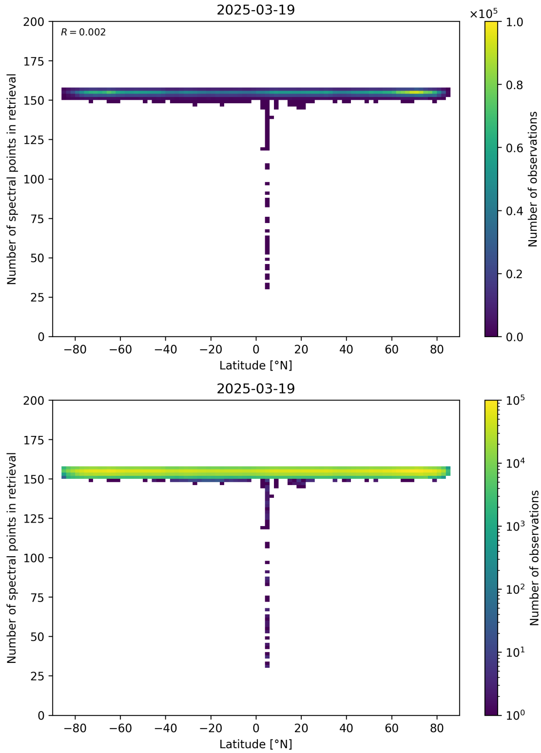
Figure 57: Scatter density plot of “Latitude” against “Number of spectral points in retrieval” for 2025-03-18 to 2025-03-20.
