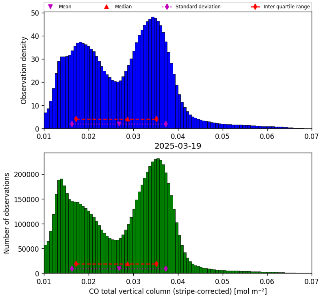
Figure 19: Histogram of “CO total vertical column (stripe-corrected)” for 2025-03-18 to 2025-03-20
