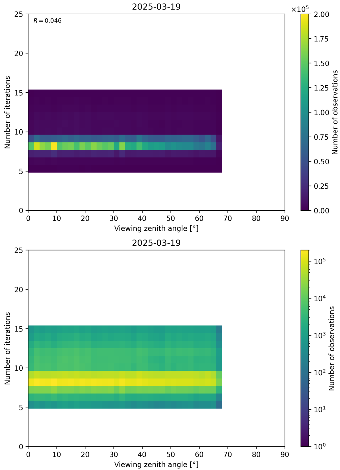
Figure 75: Scatter density plot of “Viewing zenith angle” against “Number of iterations” for 2025-03-18 to 2025-03-20.
