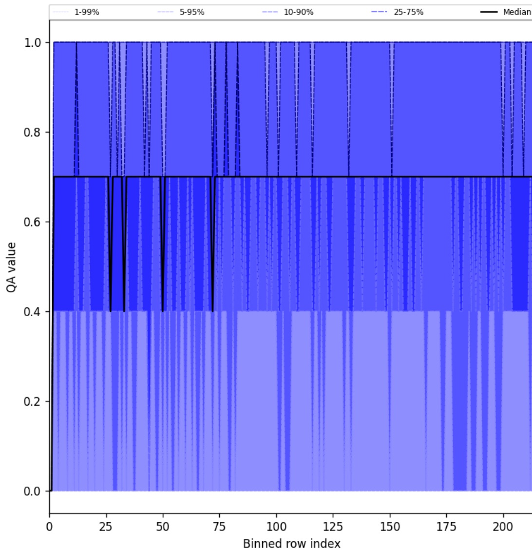
Figure 25: Along track statistics of “QA value” for 2025-03-18 to 2025-03-20
