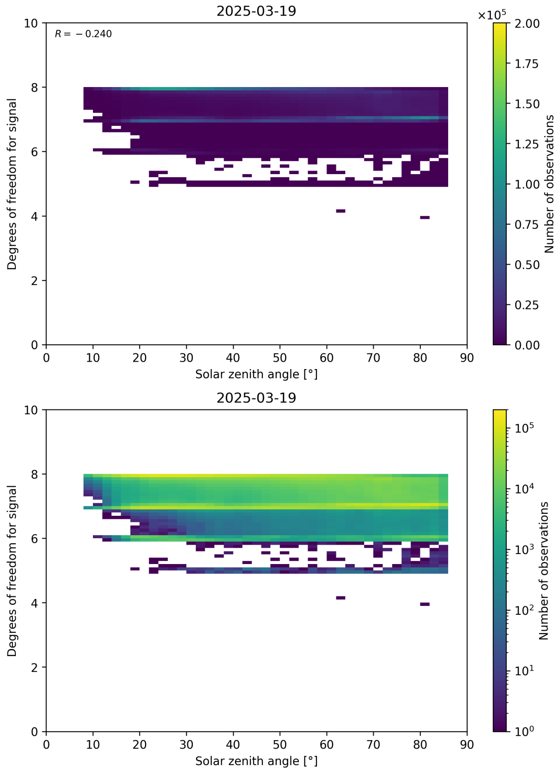
Figure 65: Scatter density plot of “Solar zenith angle” against “Degrees of freedom for signal” for 2025-03-18 to 2025-03-20.
