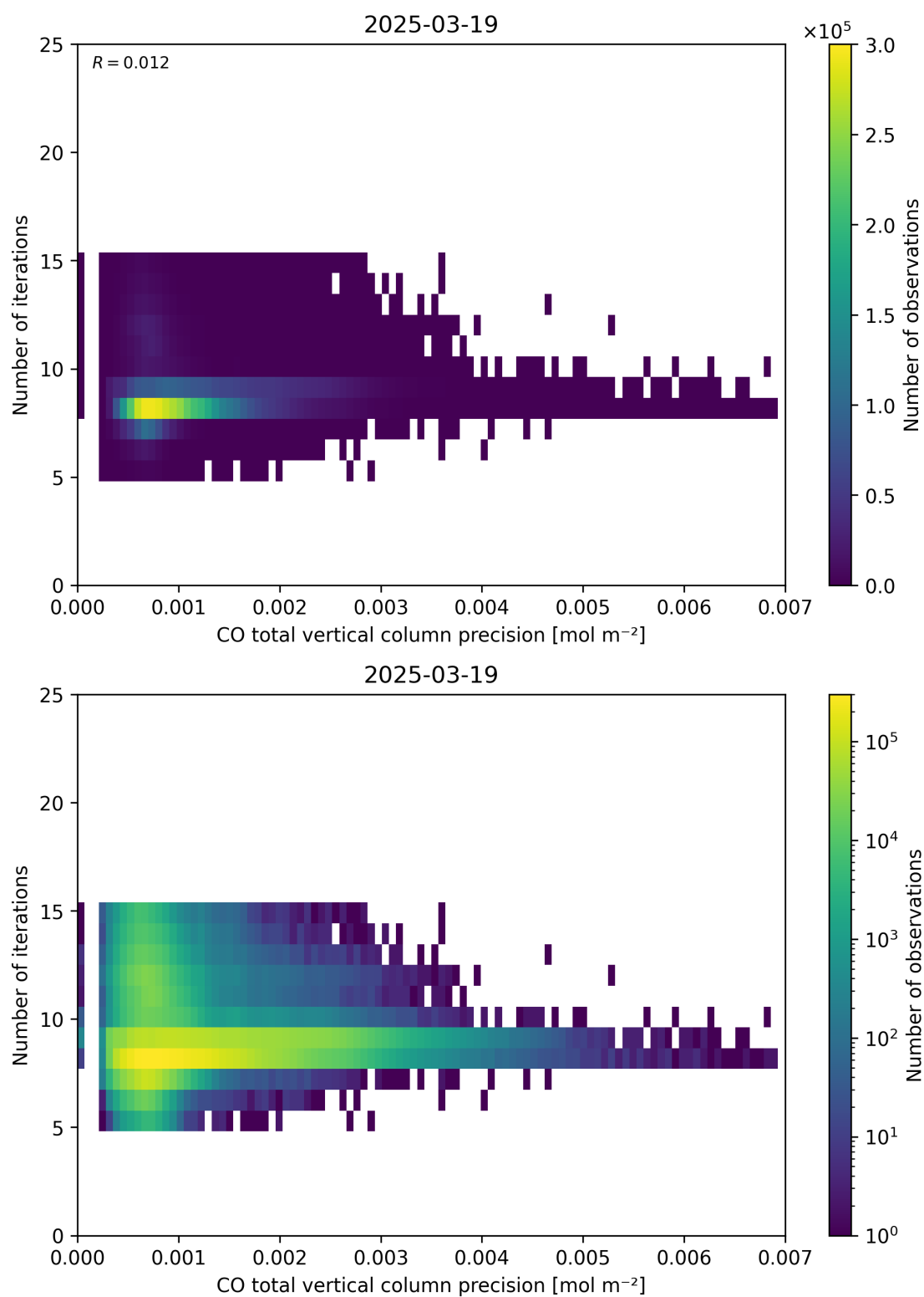
Figure 46: Scatter density plot of “CO total vertical column precision” against “Number of iterations” for 2025-03-18 to 2025-03-20.
