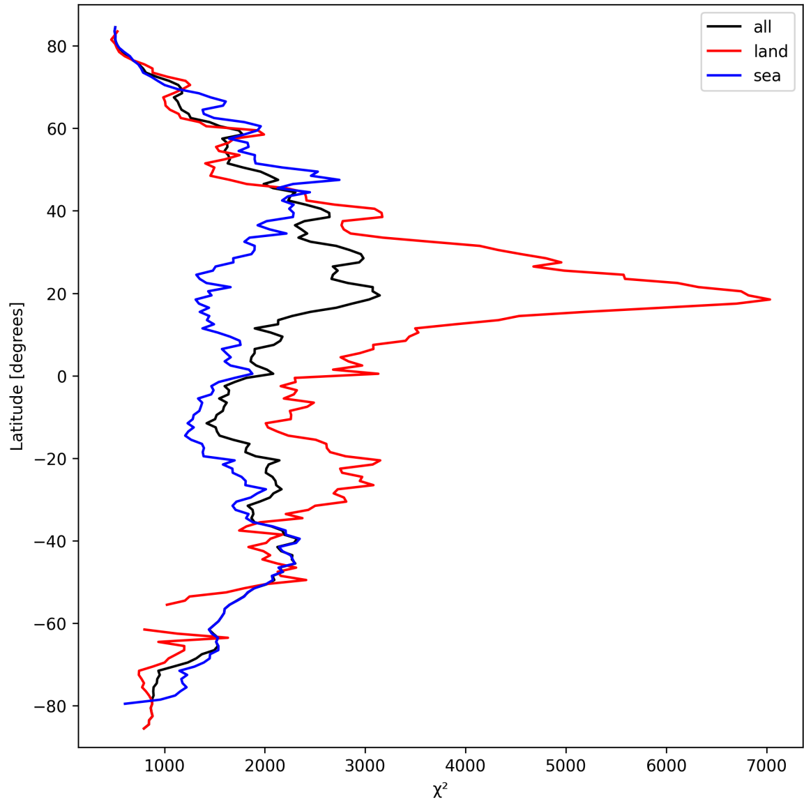
Figure 14: Zonal average of “ \chi^2 ” for 2025-03-18 to 2025-03-20.
