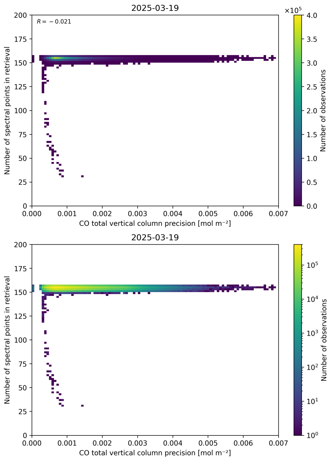
Figure 47: Scatter density plot of “CO total vertical column precision” against “Number of spectral points in retrieval” for 2025-03-18 to 2025-03-20.
