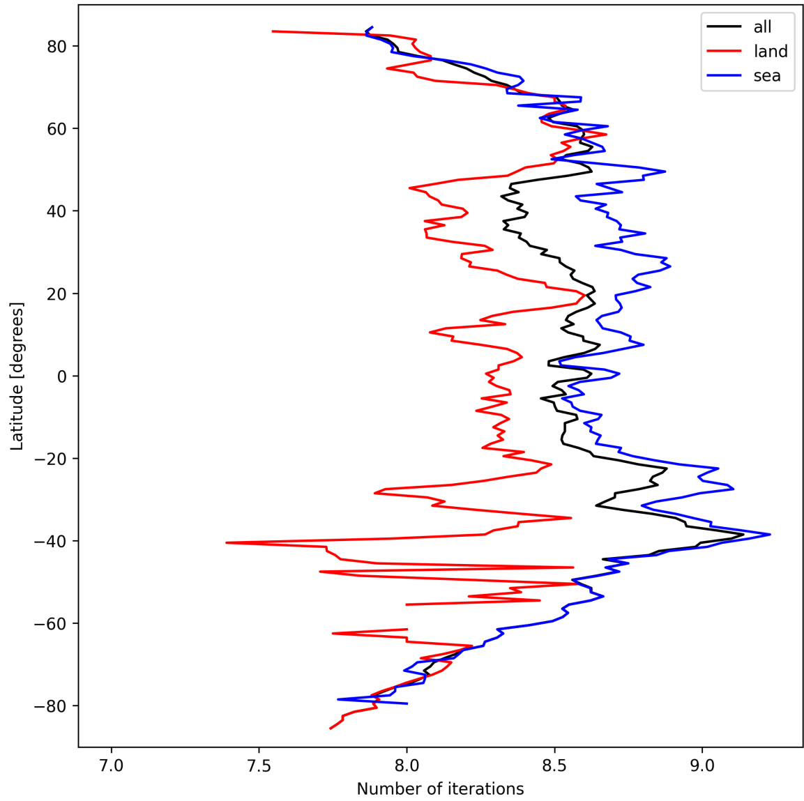
Figure 16: Zonal average of “Number of iterations” for 2025-03-18 to 2025-03-20.
