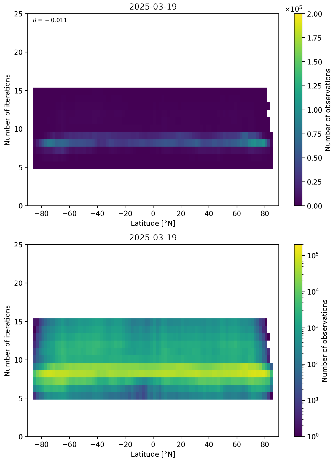
Figure 56: Scatter density plot of “Latitude” against “Number of iterations” for 2025-03-18 to 2025-03-20.
