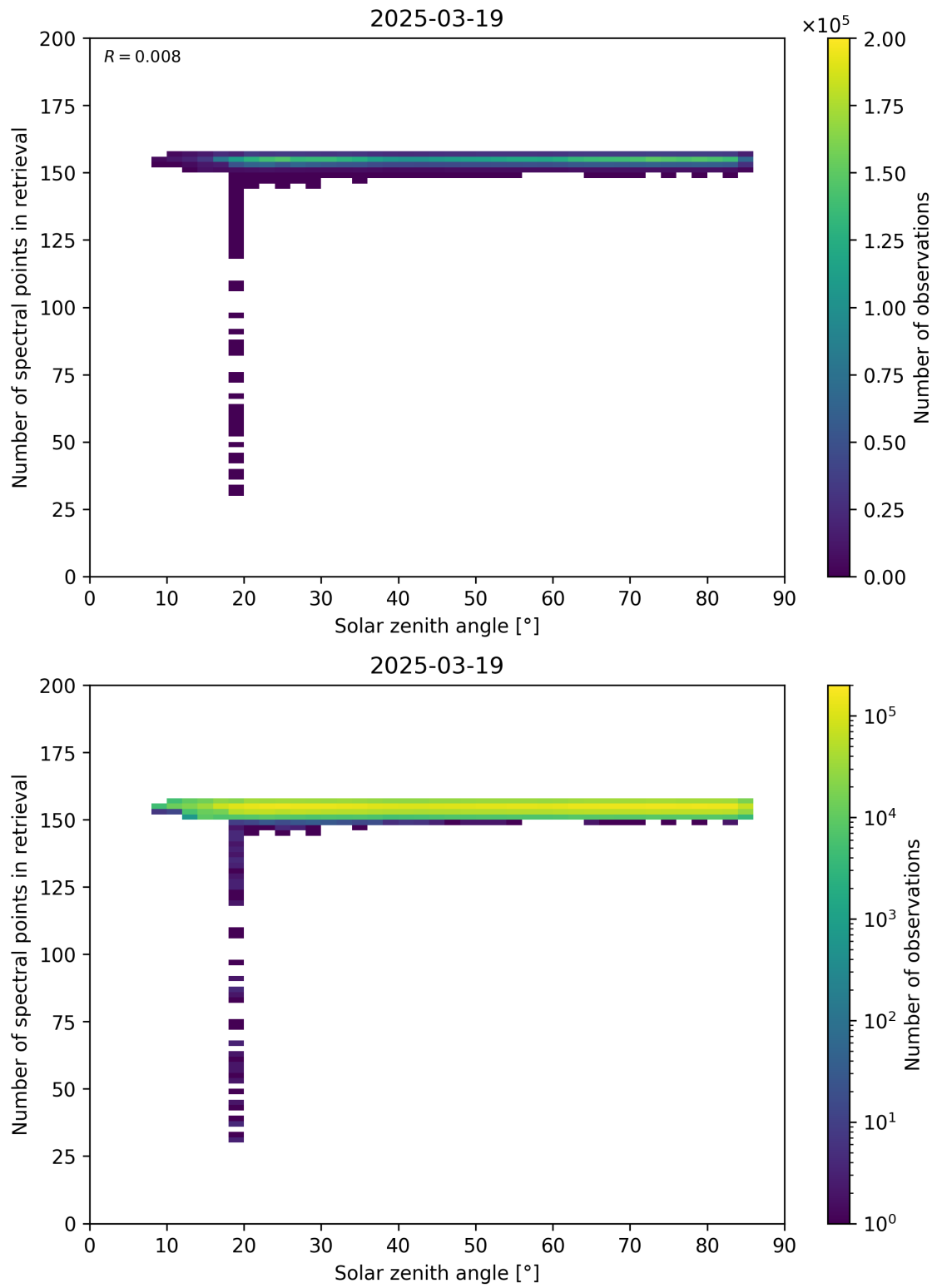
Figure 68: Scatter density plot of “Solar zenith angle” against “Number of spectral points in retrieval” for 2025-03-18 to 2025-03-20.
