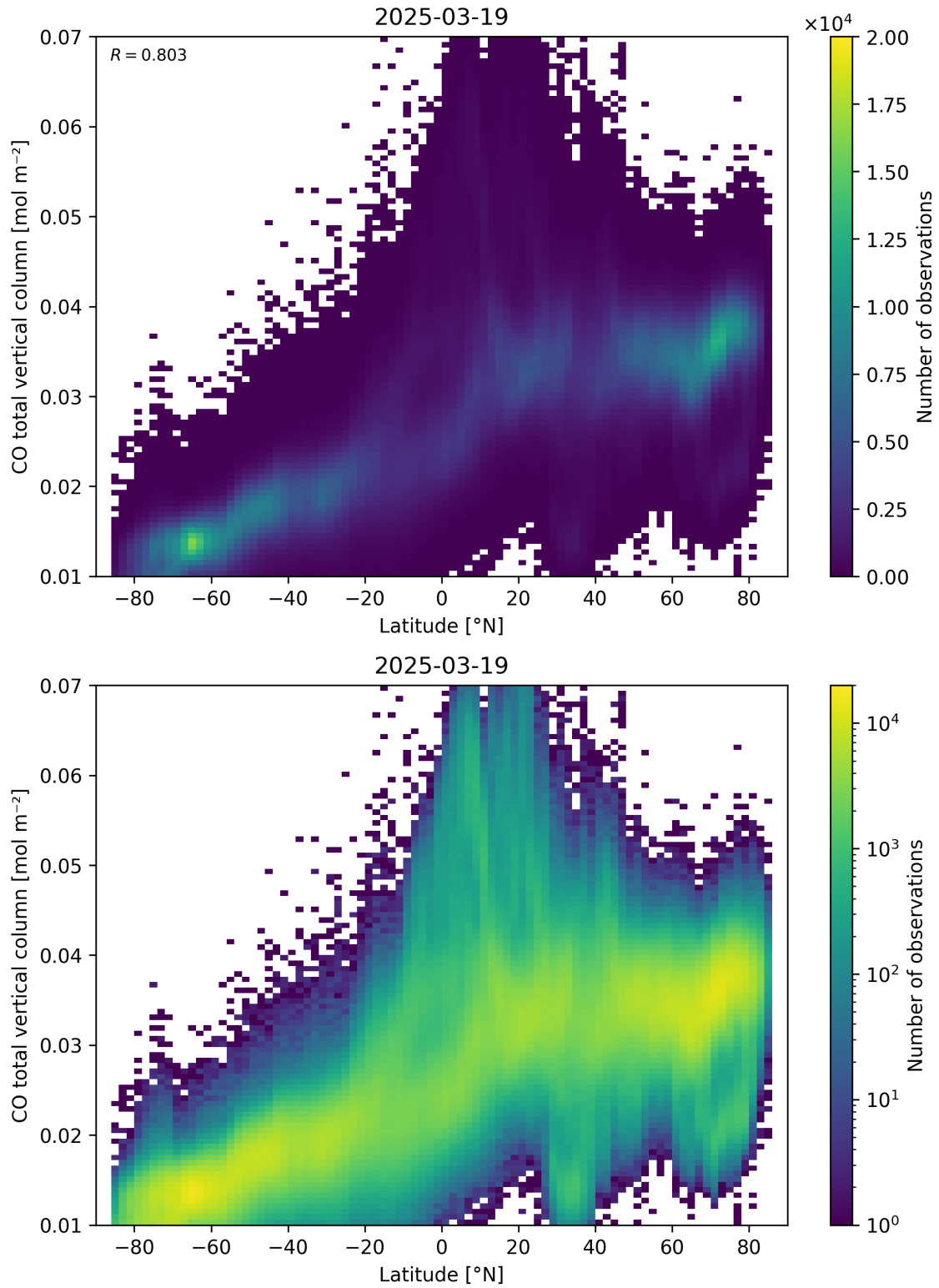
Figure 51: Scatter density plot of “Latitude” against “CO total vertical column” for 2025-03-18 to 2025-03-20.
