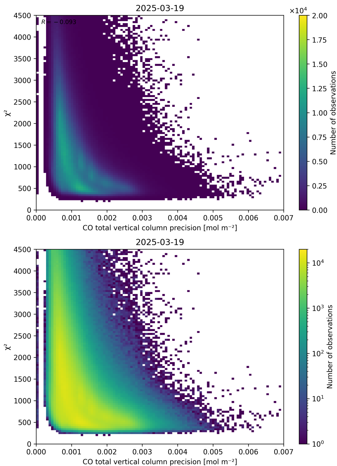
Figure 44: Scatter density plot of “CO total vertical column precision” against “ \chi^2 ” for 2025-03-18 to 2025-03-20.
