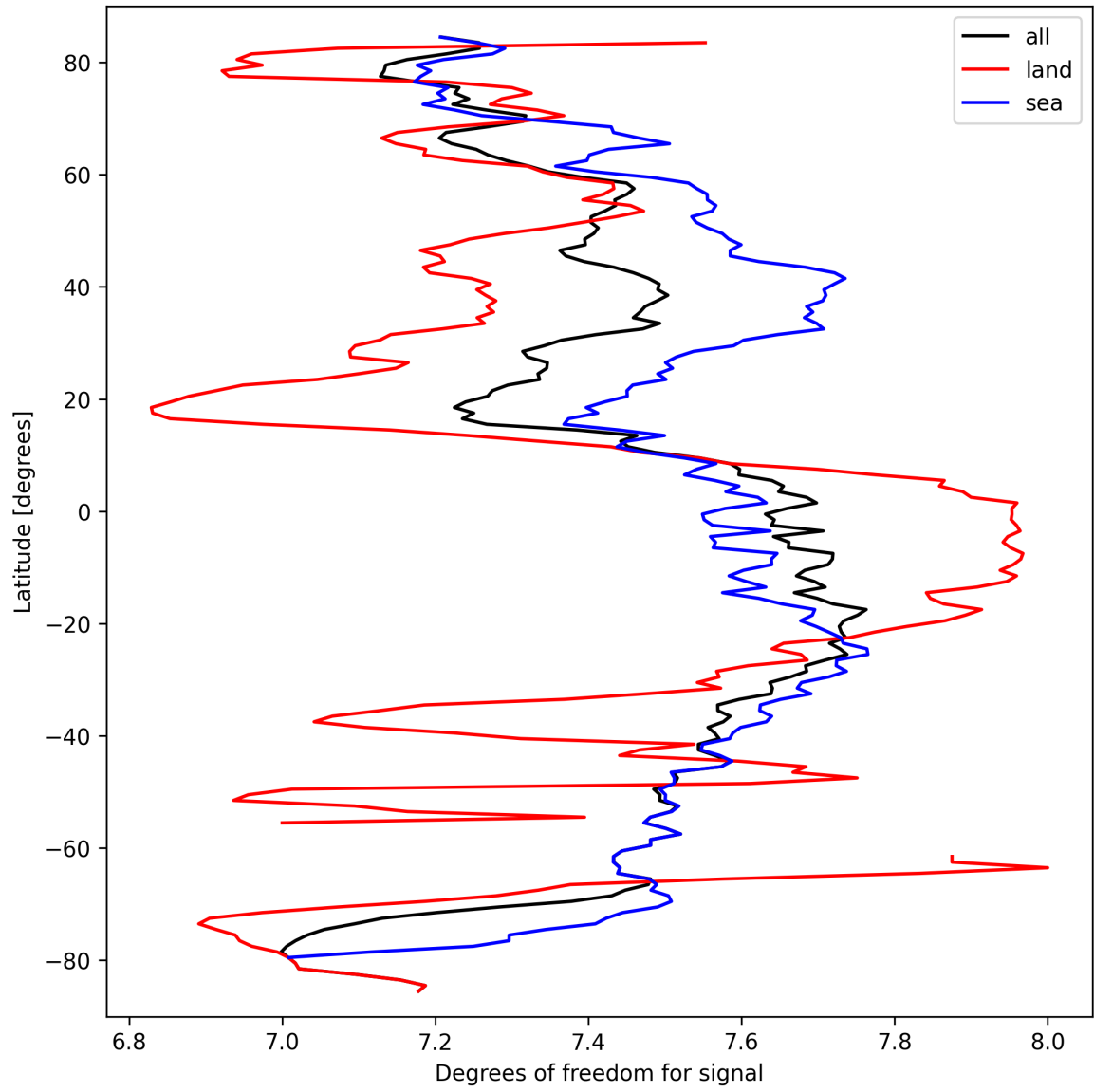
Figure 15: Zonal average of “Degrees of freedom for signal” for 2025-03-18 to 2025-03-20.
