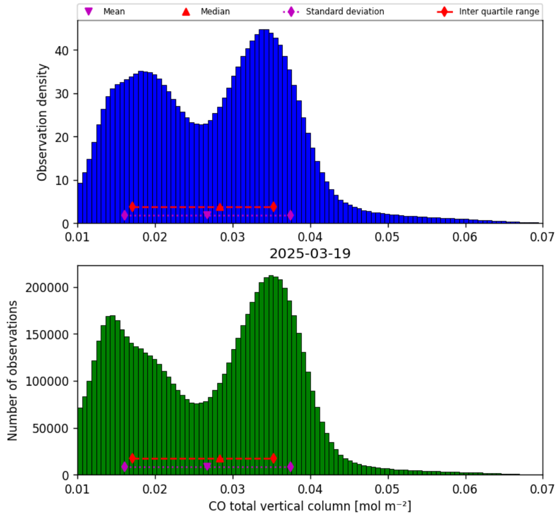
Figure 18: Histogram of “CO total vertical column” for 2025-03-18 to 2025-03-20
