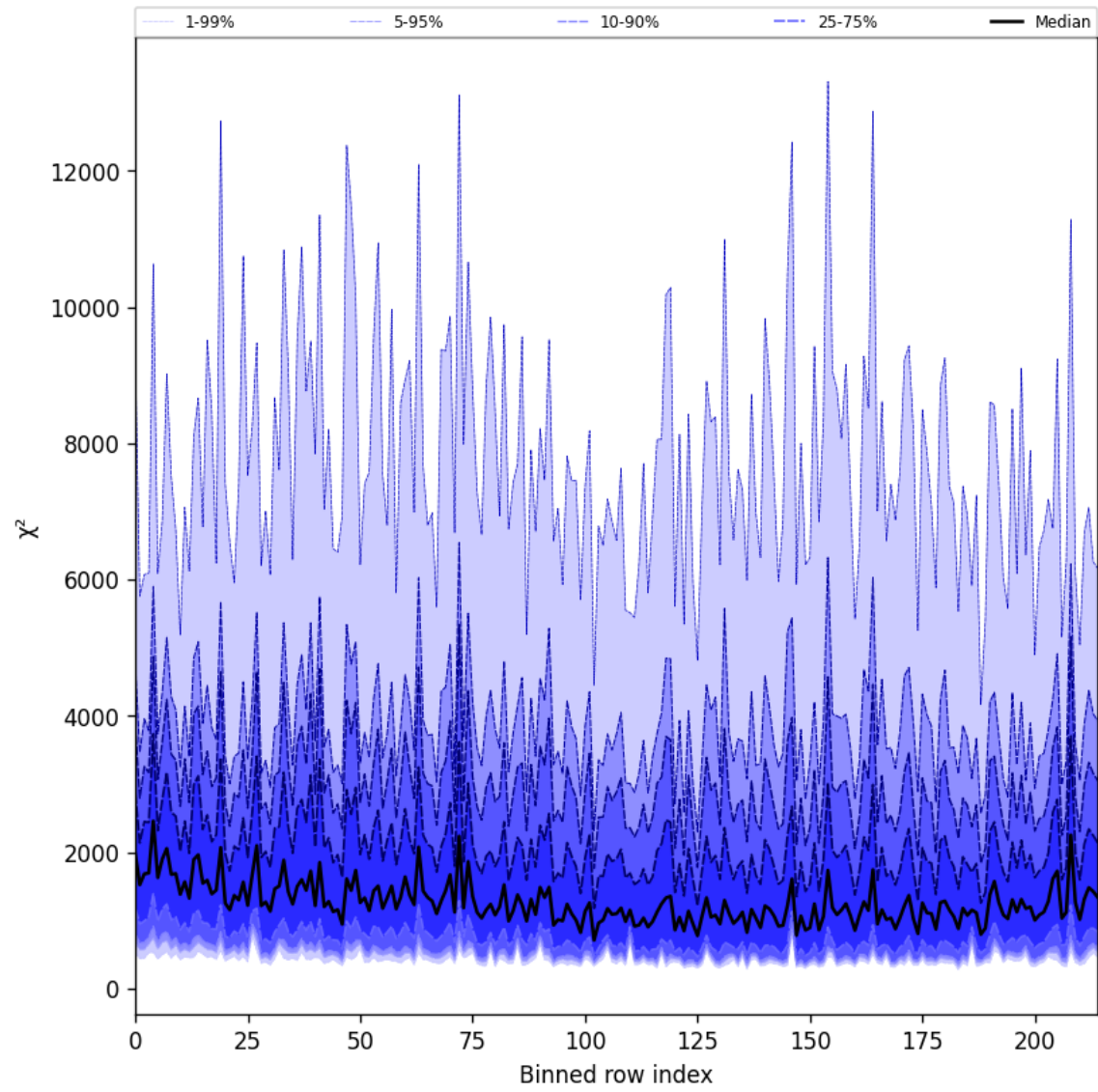
Figure 30: Along track statistics of “ \chi^2 ” for 2025-03-18 to 2025-03-20
