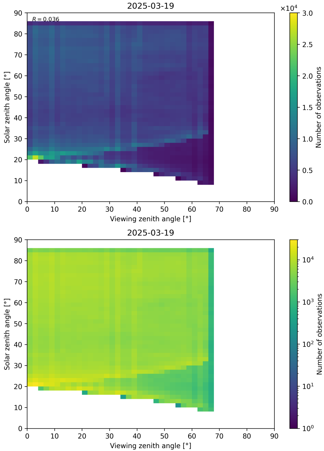
Figure 77: Scatter density plot of “Viewing zenith angle” against “Solar zenith angle” for 2025-03-18 to 2025-03-20.
