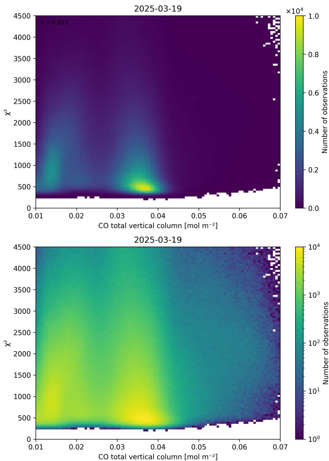
Figure 35: Scatter density plot of “CO total vertical column” against “ \chi^2 ” for 2025-03-18 to 2025-03-20.
