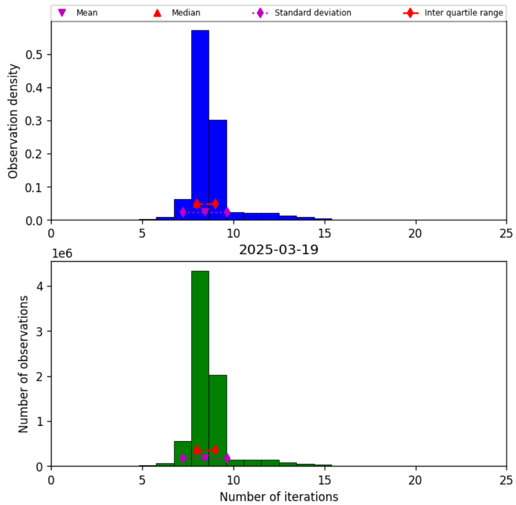
Figure 24: Histogram of “Number of iterations” for 2025-03-18 to 2025-03-20
