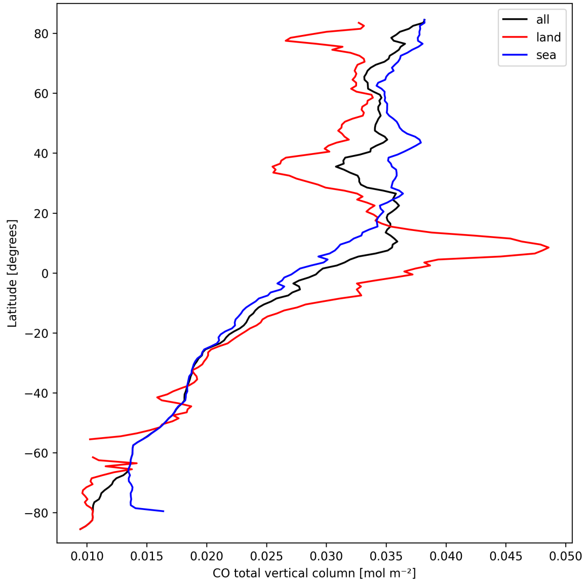
Figure 10: Zonal average of “CO total vertical column” for 2025-03-18 to 2025-03-20.
