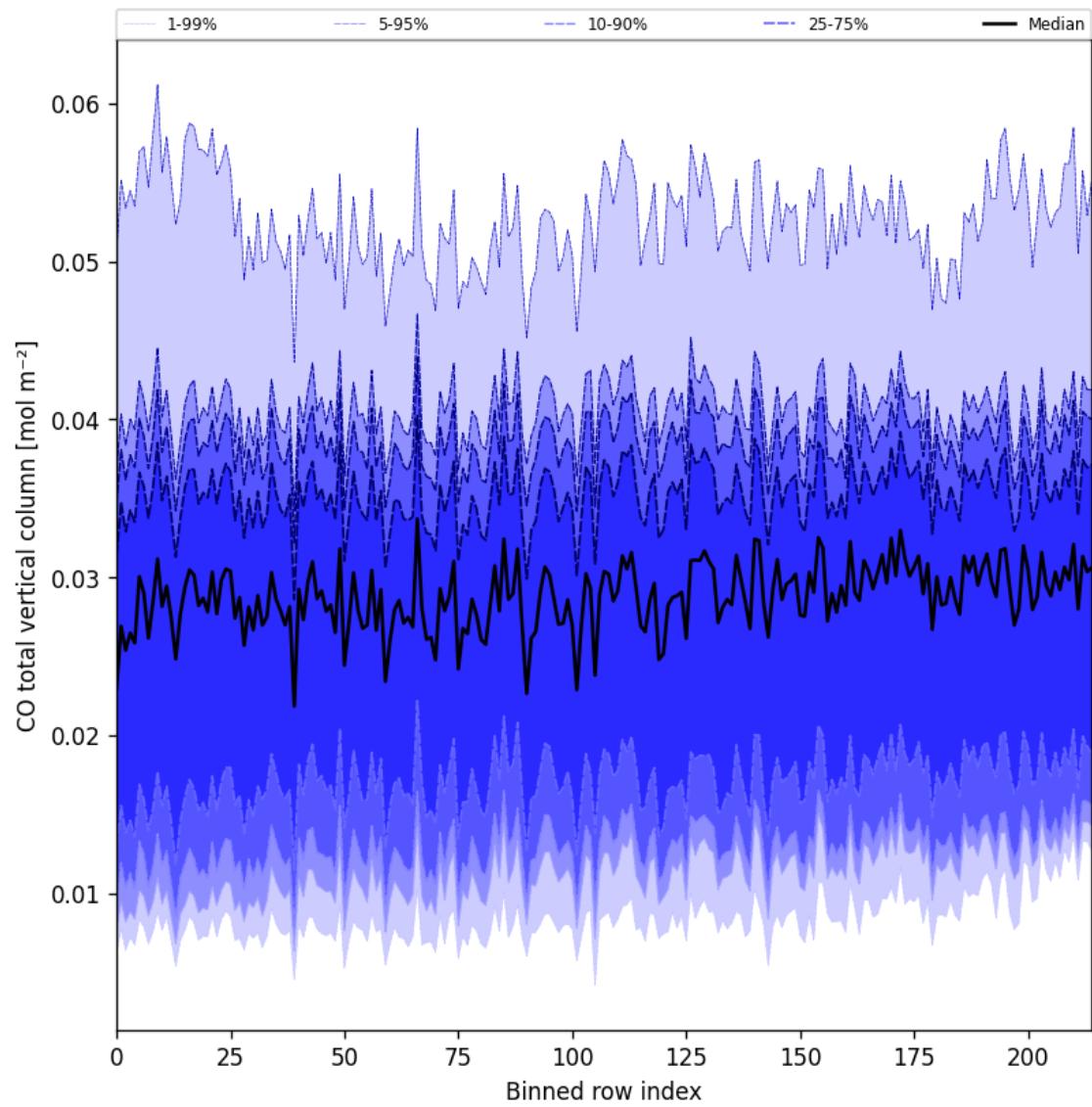
Figure 26: Along track statistics of “CO total vertical column” for 2025-03-18 to 2025-03-20
