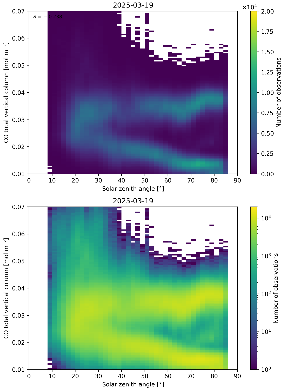
Figure 61: Scatter density plot of “Solar zenith angle” against “CO total vertical column” for 2025-03-18 to 2025-03-20.
