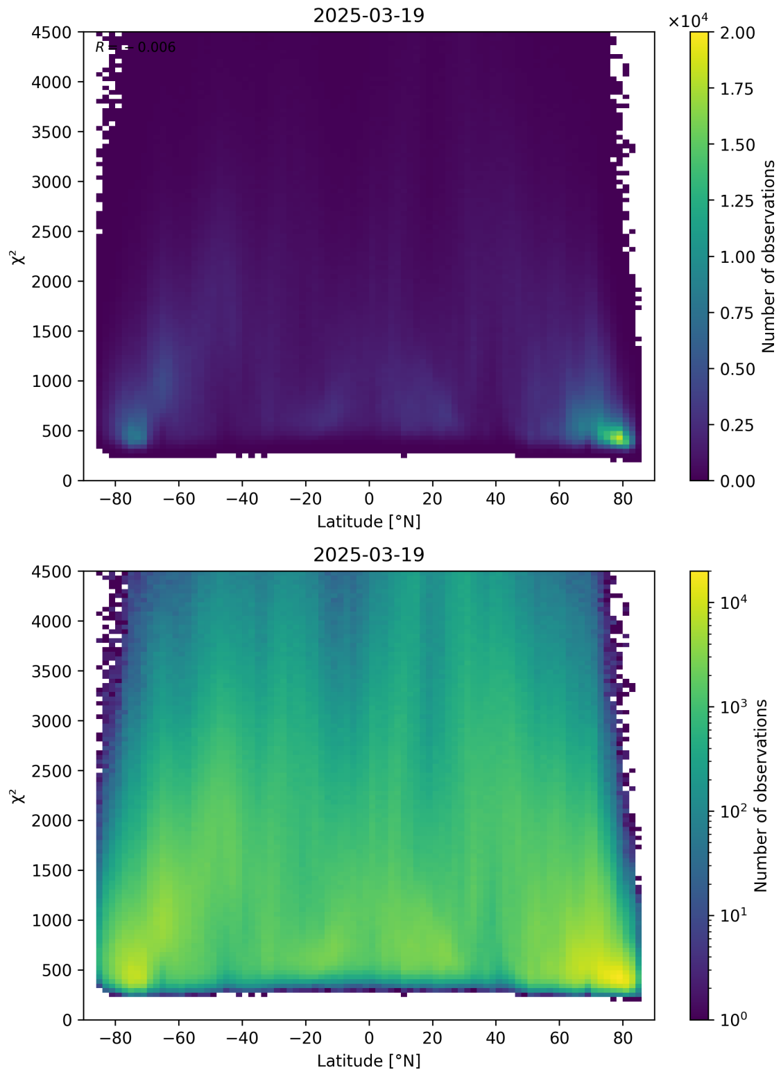
Figure 54: Scatter density plot of “Latitude” against “ \chi^2 ” for 2025-03-18 to 2025-03-20.
