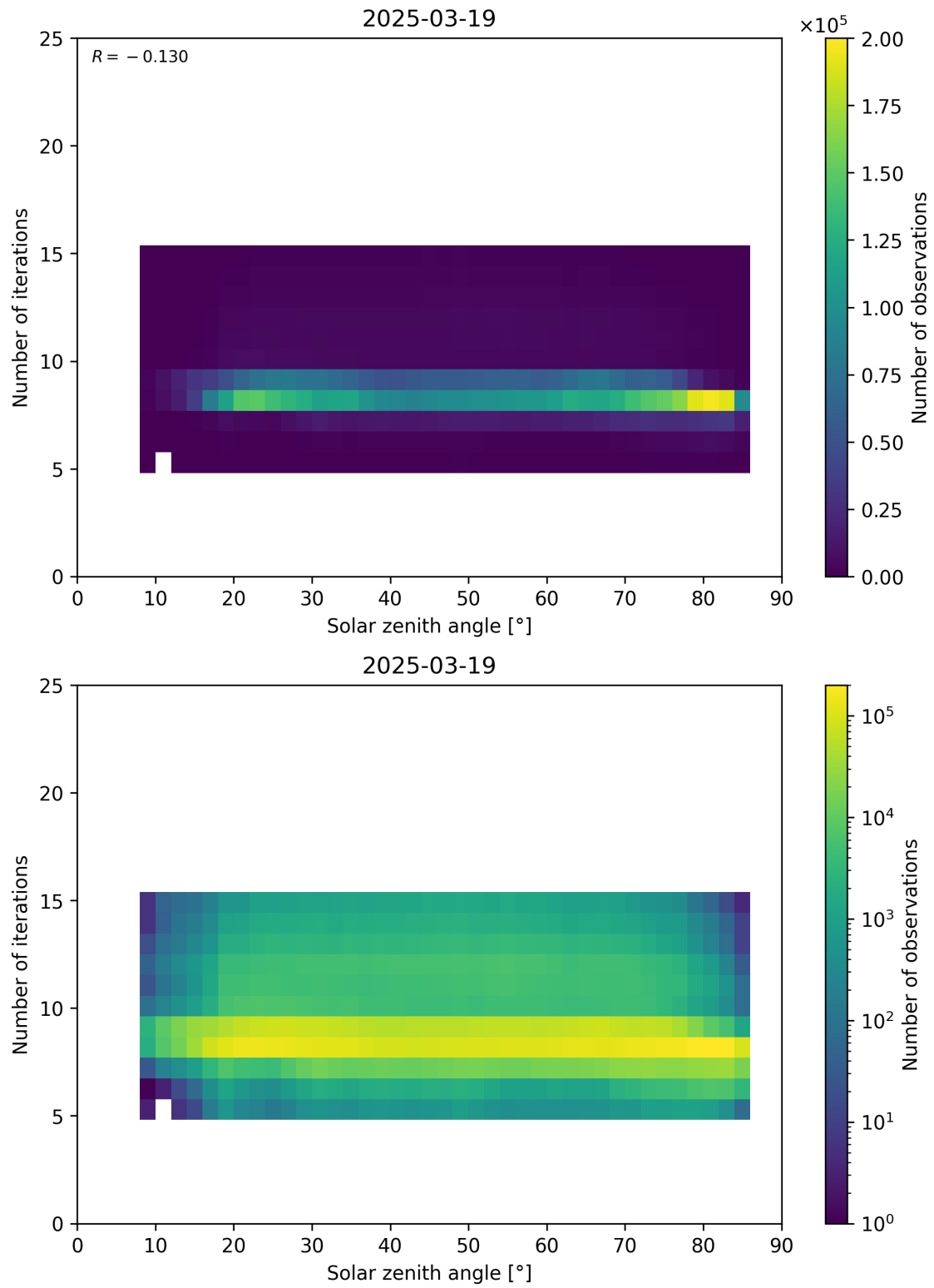
Figure 67: Scatter density plot of “Solar zenith angle” against “Number of iterations” for 2025-03-18 to 2025-03-20.
