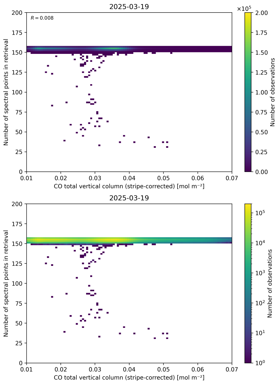
Figure 40: Scatter density plot of “CO total vertical column (stripe-corrected)” against “Number of spectral points in retrieval” for 2025-03-18 to 2025-03-20.
