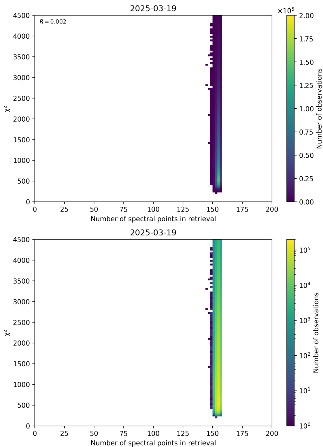
Figure 58: Scatter density plot of “Number of spectral points in retrieval” against “ \chi^2 ” for 2025-03-18 to 2025-03-20.
