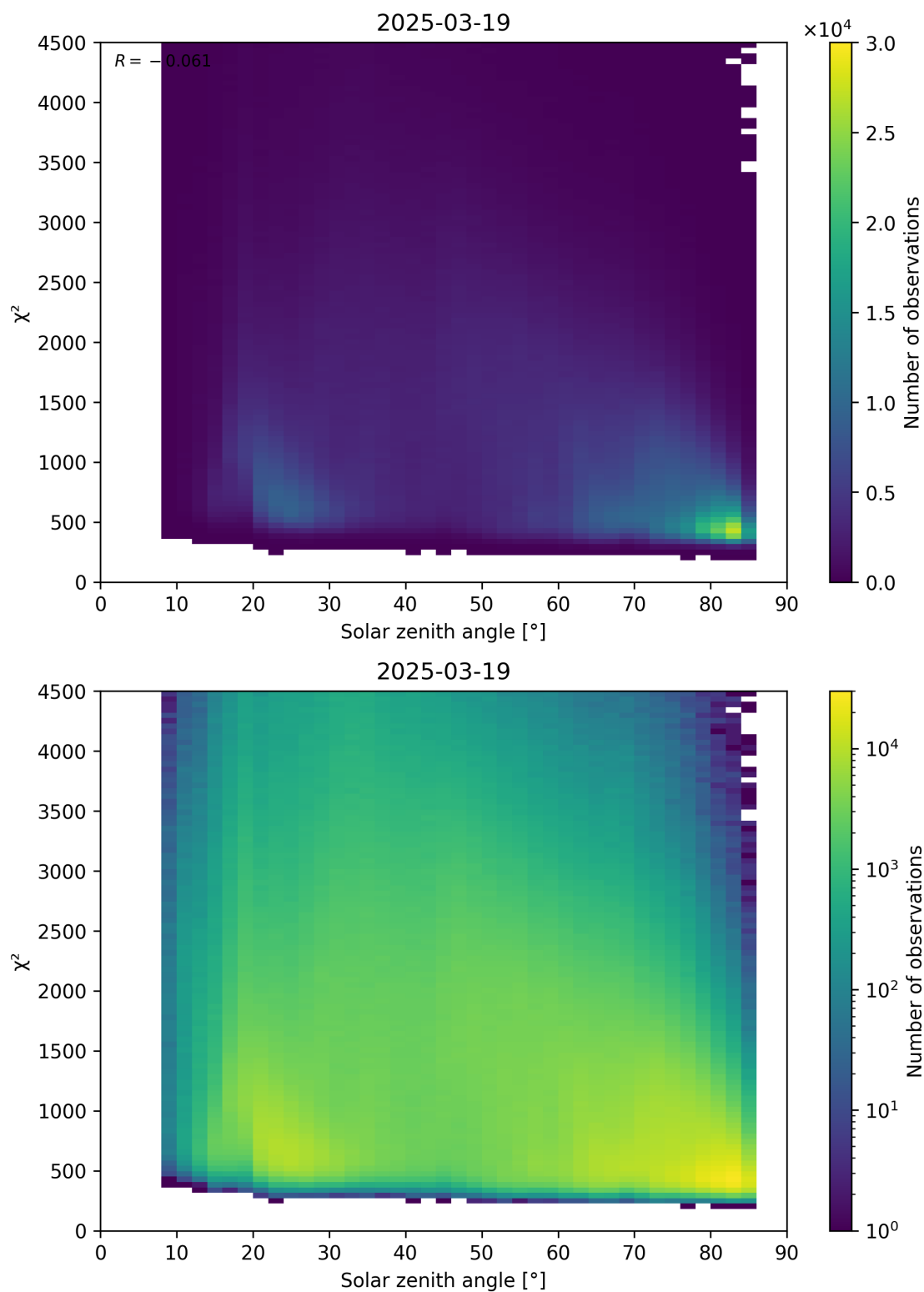
Figure 64: Scatter density plot of “Solar zenith angle” against “ \chi^2 ” for 2025-03-18 to 2025-03-20.
