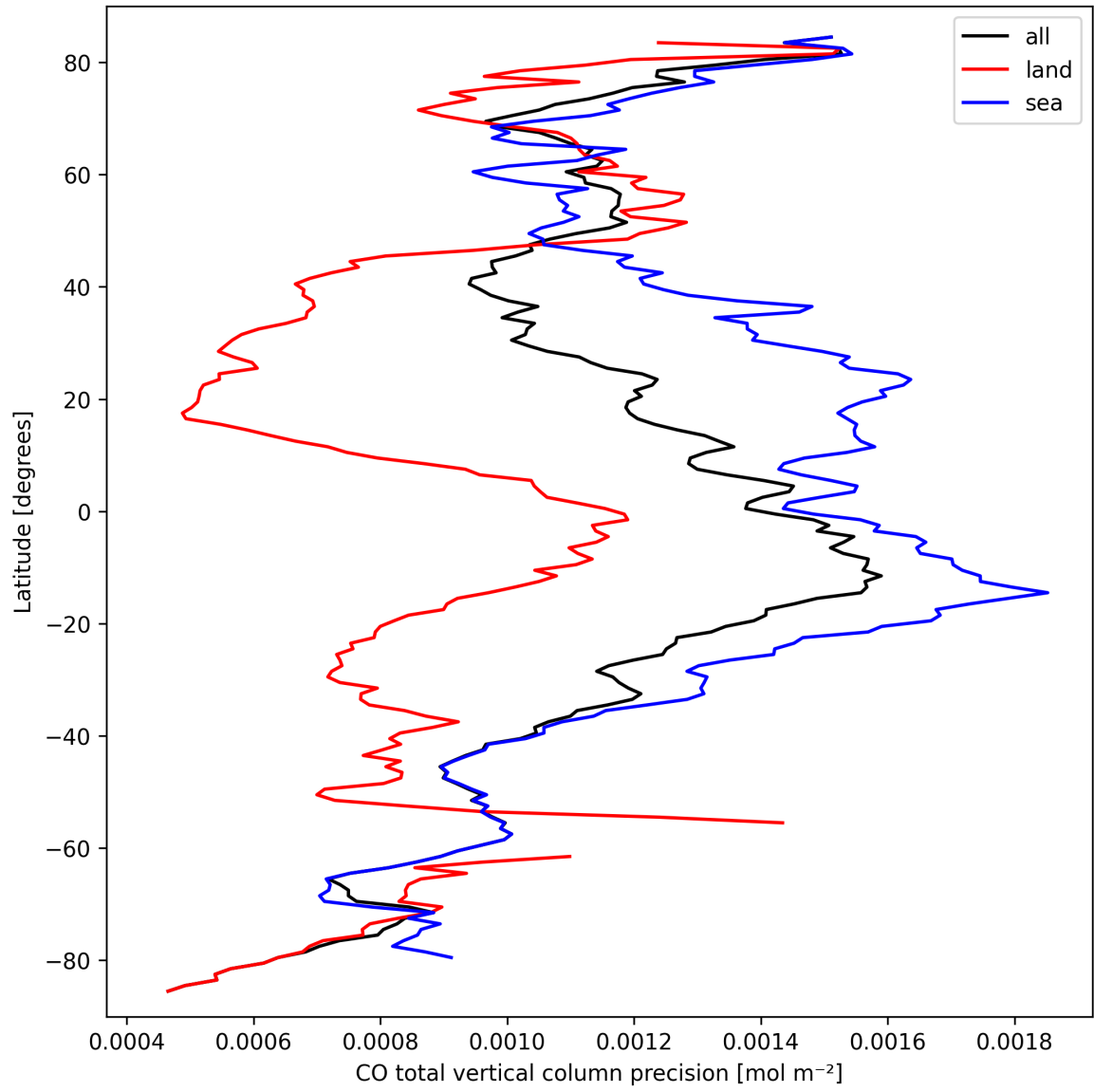
Figure 12: Zonal average of “CO total vertical column precision” for 2025-03-18 to 2025-03-20.
