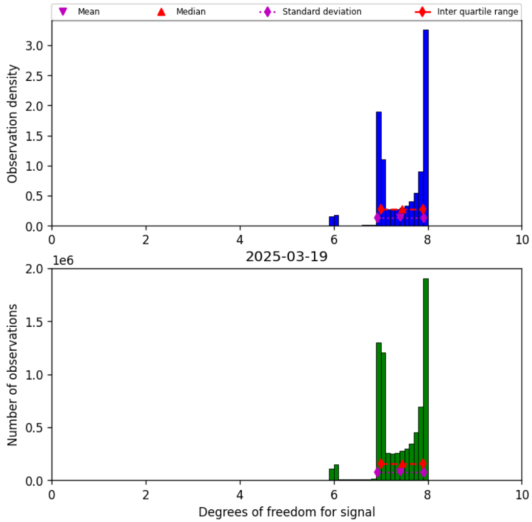
Figure 23: Histogram of “Degrees of freedom for signal” for 2025-03-18 to 2025-03-20
