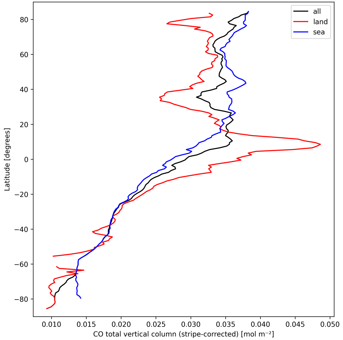
Figure 11: Zonal average of “CO total vertical column (stripe-corrected)” for 2025-03-18 to 2025-03-20.
