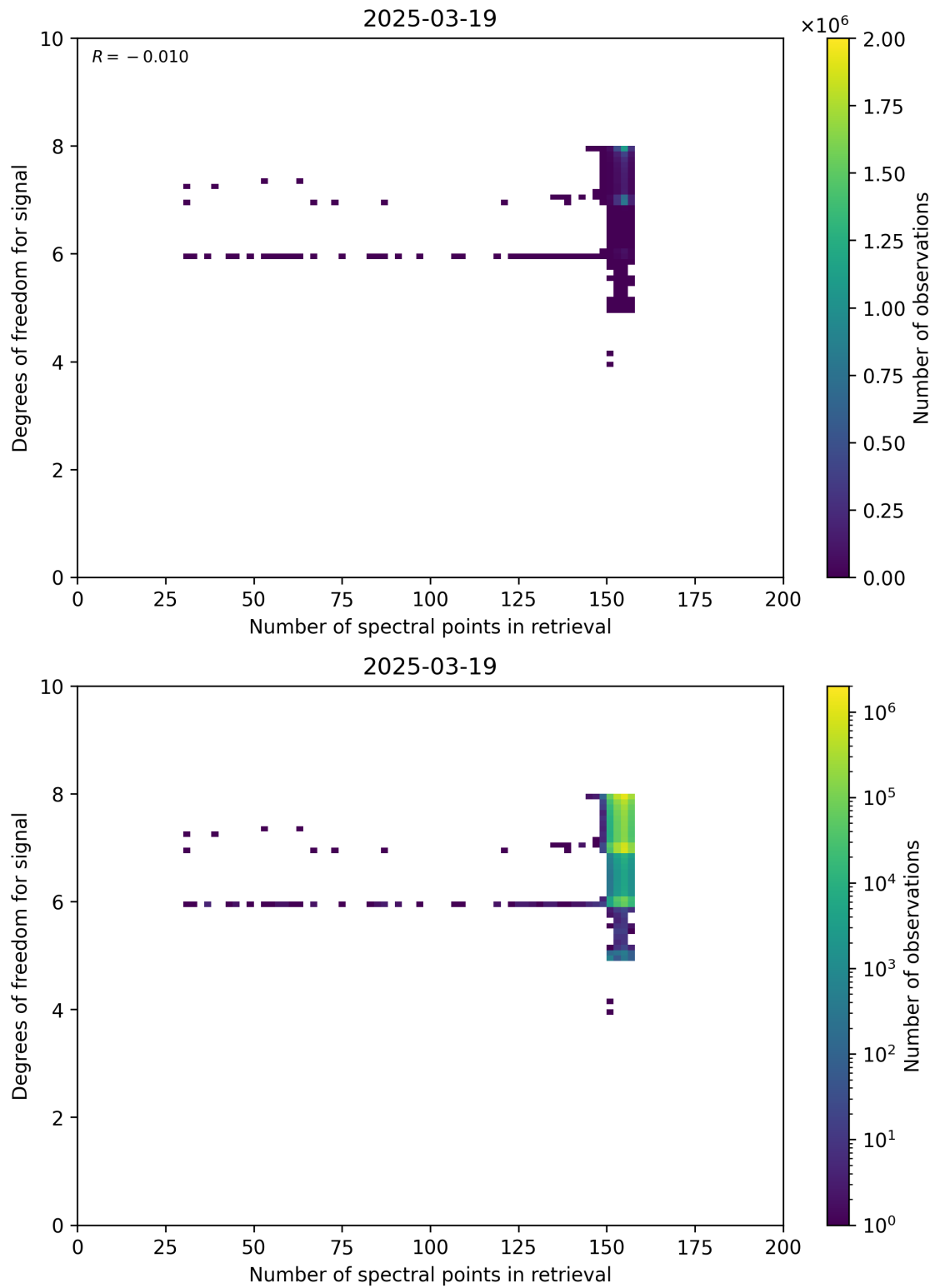
Figure 59: Scatter density plot of “Number of spectral points in retrieval” against “Degrees of freedom for signal” for 2025-03-18 to 2025-03-20.
