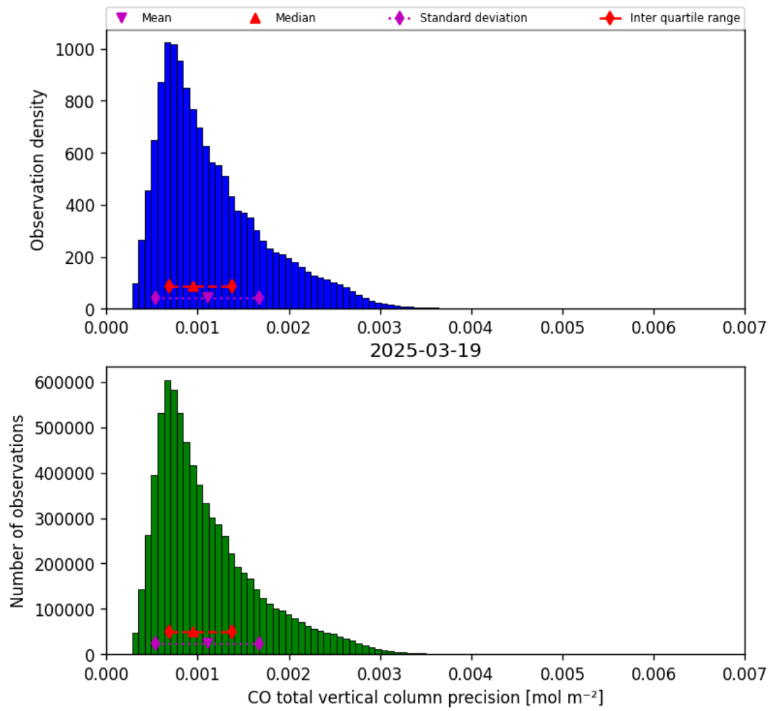
Figure 20: Histogram of “CO total vertical column precision” for 2025-03-18 to 2025-03-20
