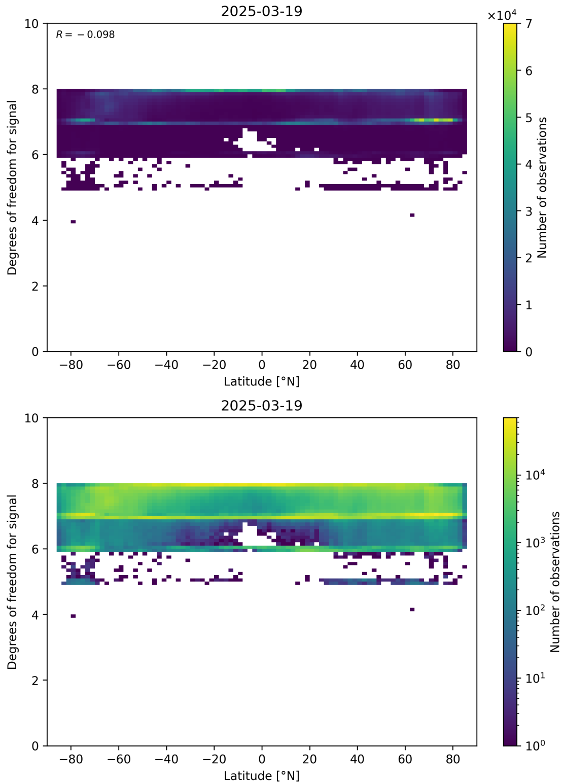
Figure 55: Scatter density plot of “Latitude” against “Degrees of freedom for signal” for 2025-03-18 to 2025-03-20.
