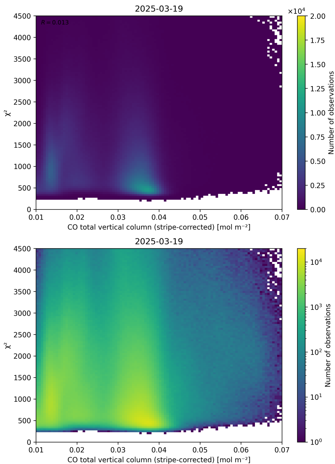
Figure 37: Scatter density plot of “CO total vertical column (stripe-corrected)” against “ \chi^2 ” for 2025-03-18 to 2025-03-20.
