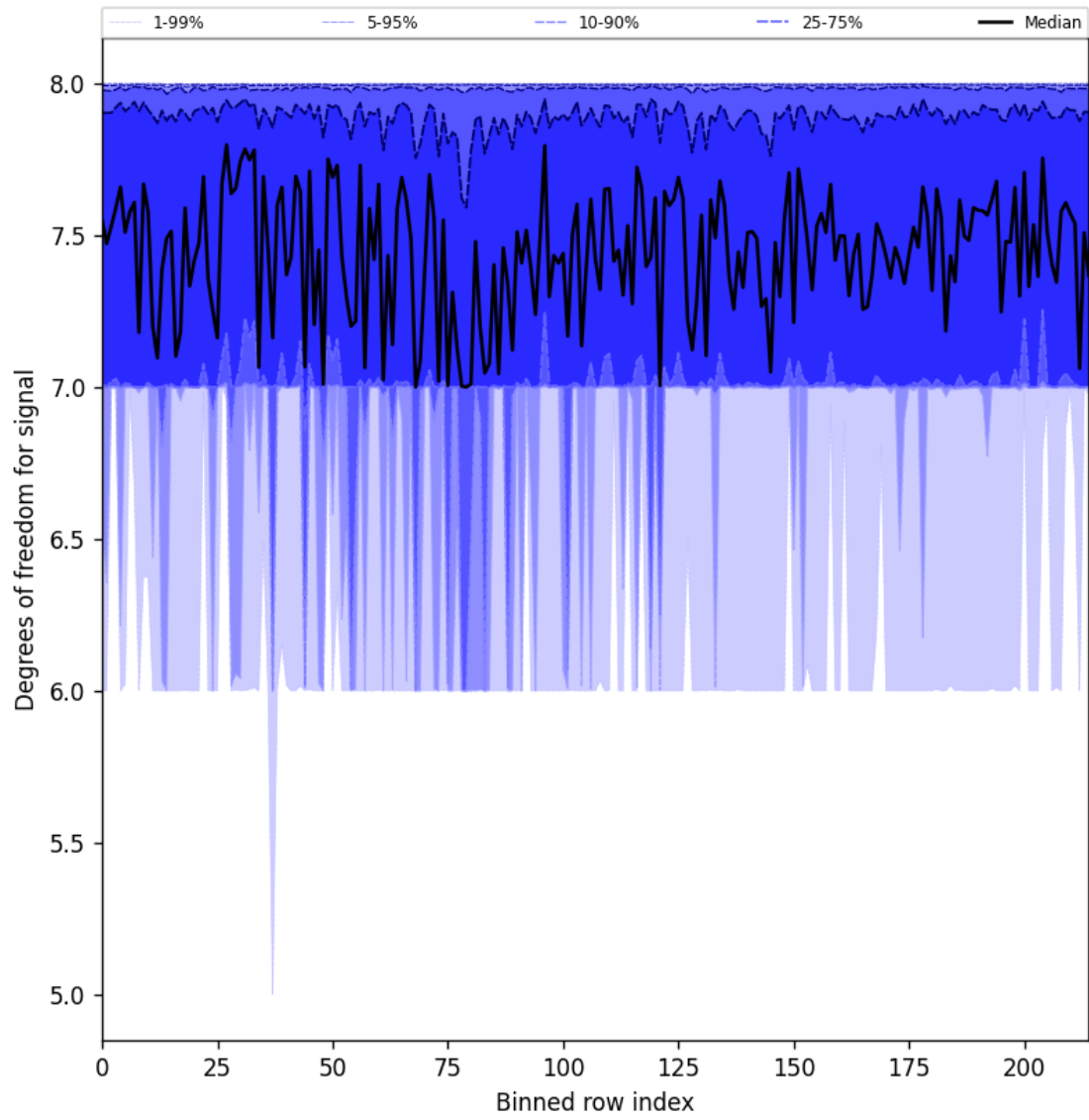
Figure 31: Along track statistics of “Degrees of freedom for signal” for 2025-03-18 to 2025-03-20
