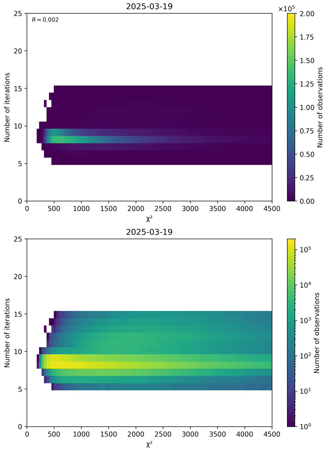
Figure 49: Scatter density plot of “ \chi^2 ” against “Number of iterations” for 2025-03-18 to 2025-03-20.
