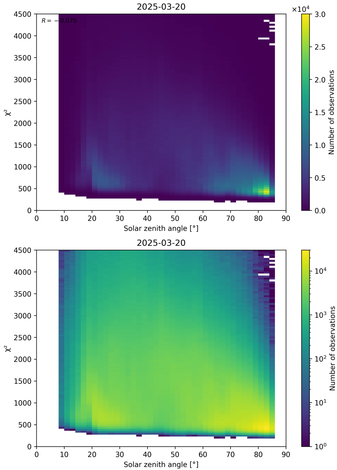
Figure 64: Scatter density plot of “Solar zenith angle” against “ \chi^2 ” for 2025-03-19 to 2025-03-21.
