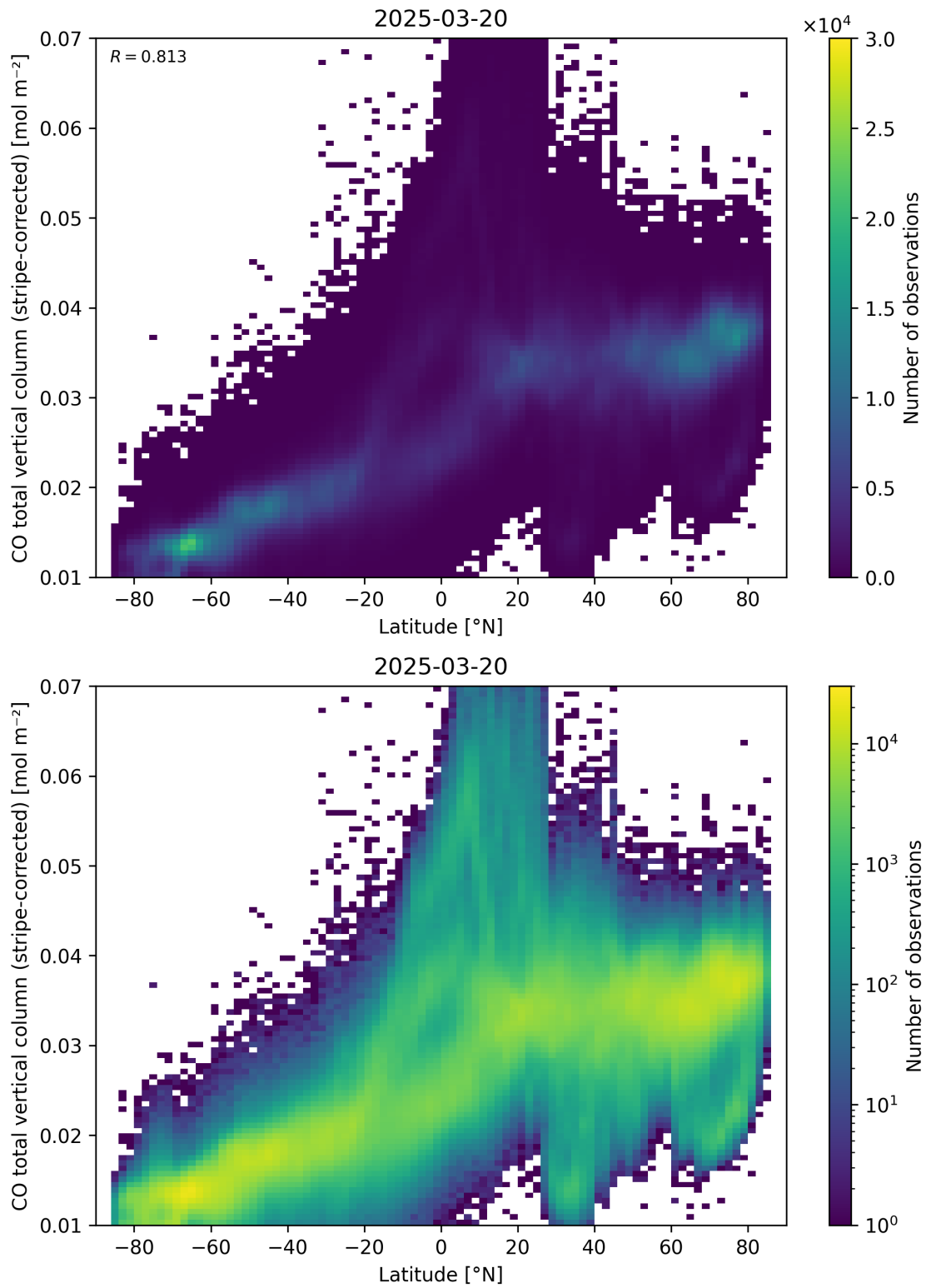
Figure 52: Scatter density plot of “Latitude” against “CO total vertical column (stripe-corrected)” for 2025-03-19 to 2025-03-21.
