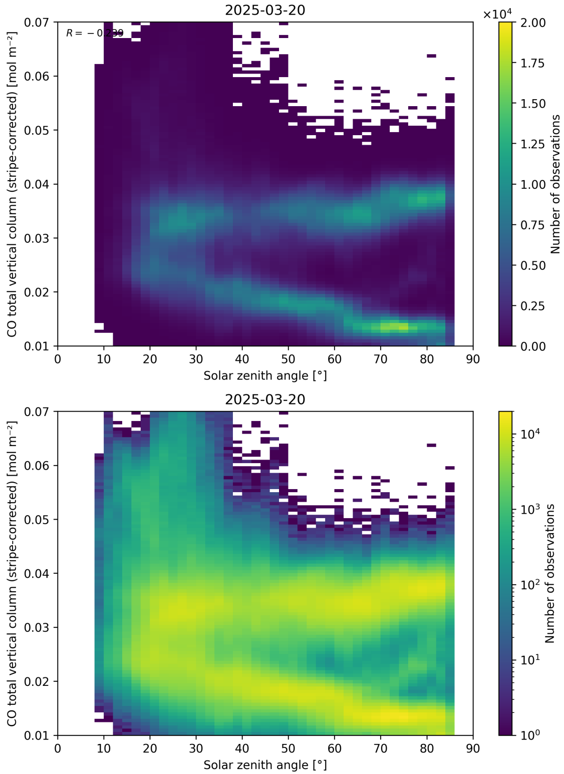
Figure 62: Scatter density plot of “Solar zenith angle” against “CO total vertical column (stripe-corrected)” for 2025-03-19 to 2025-03-21.
