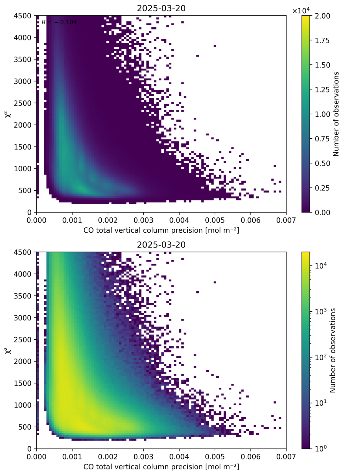
Figure 44: Scatter density plot of “CO total vertical column precision” against “ \chi^2 ” for 2025-03-19 to 2025-03-21.
