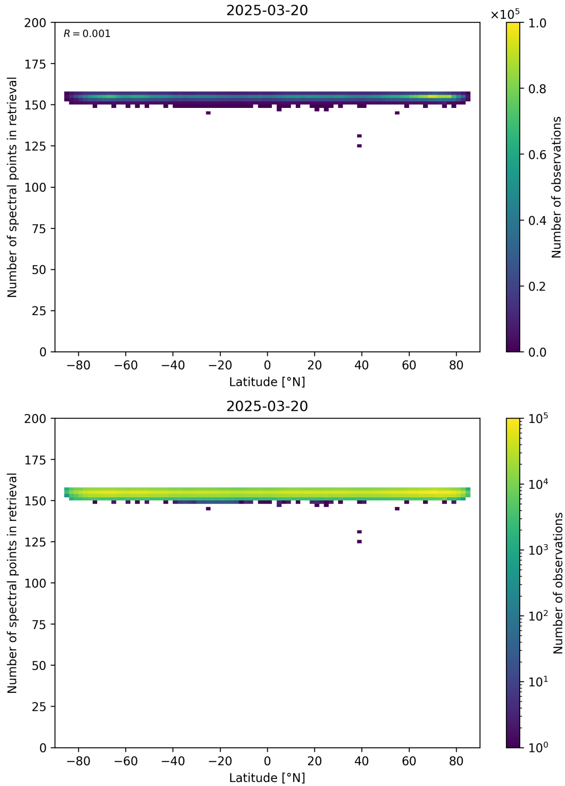
Figure 57: Scatter density plot of “Latitude” against “Number of spectral points in retrieval” for 2025-03-19 to 2025-03-21.
