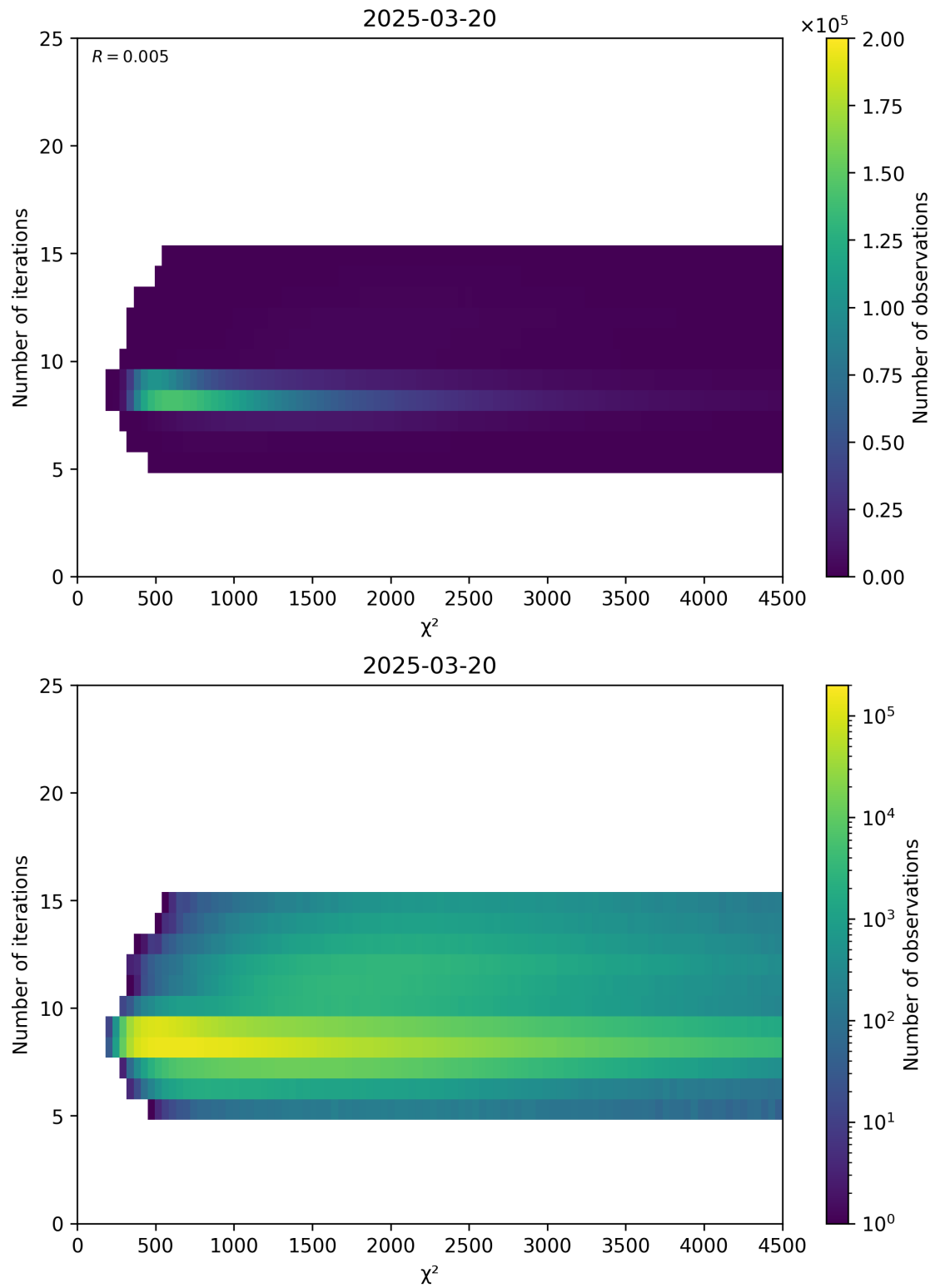
Figure 49: Scatter density plot of “ \chi^2 ” against “Number of iterations” for 2025-03-19 to 2025-03-21.
