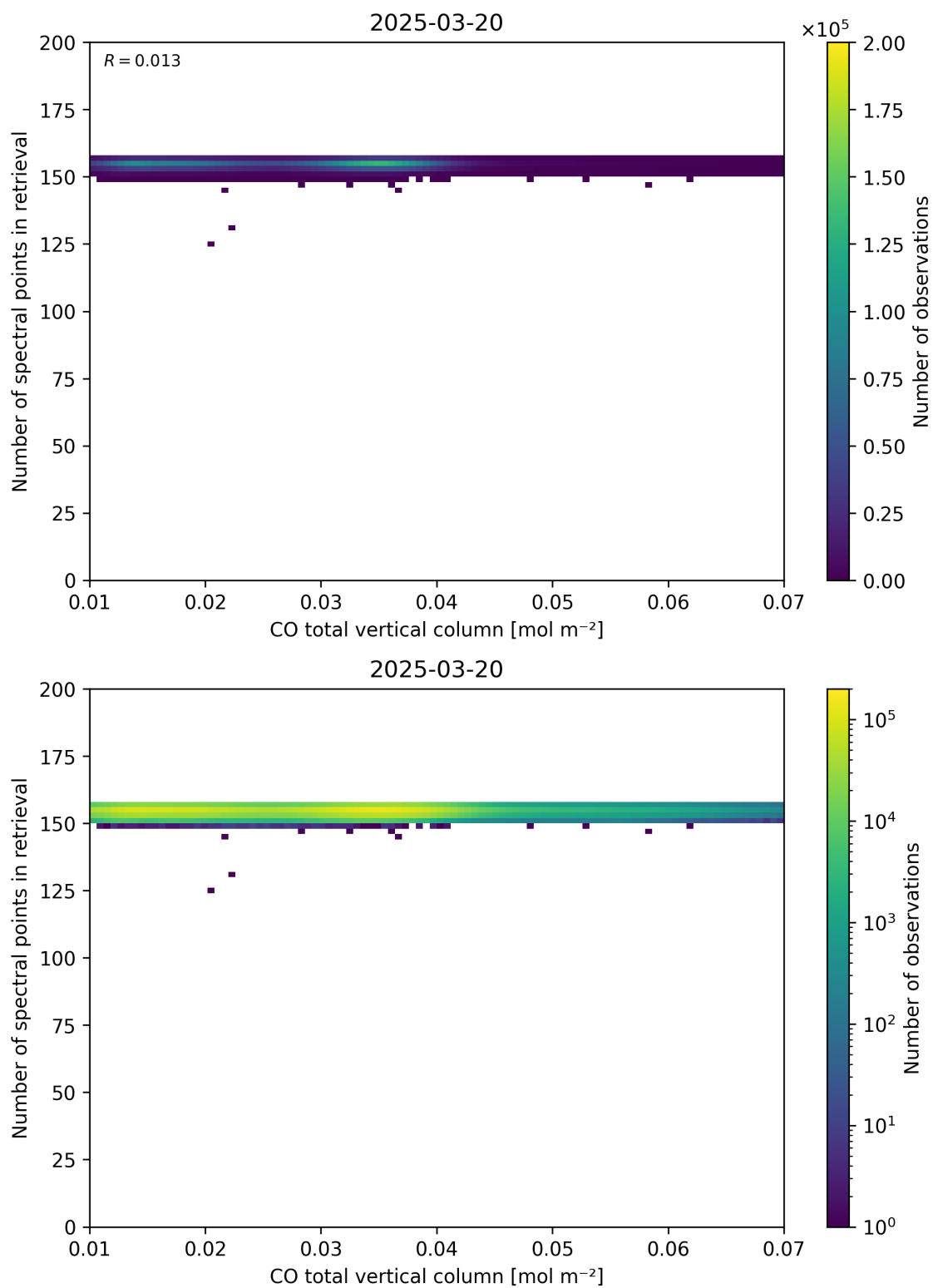
Figure 43: Scatter density plot of “CO total vertical column” against “Number of spectral points in retrieval” for 2025-03-19 to 2025-03-21.
