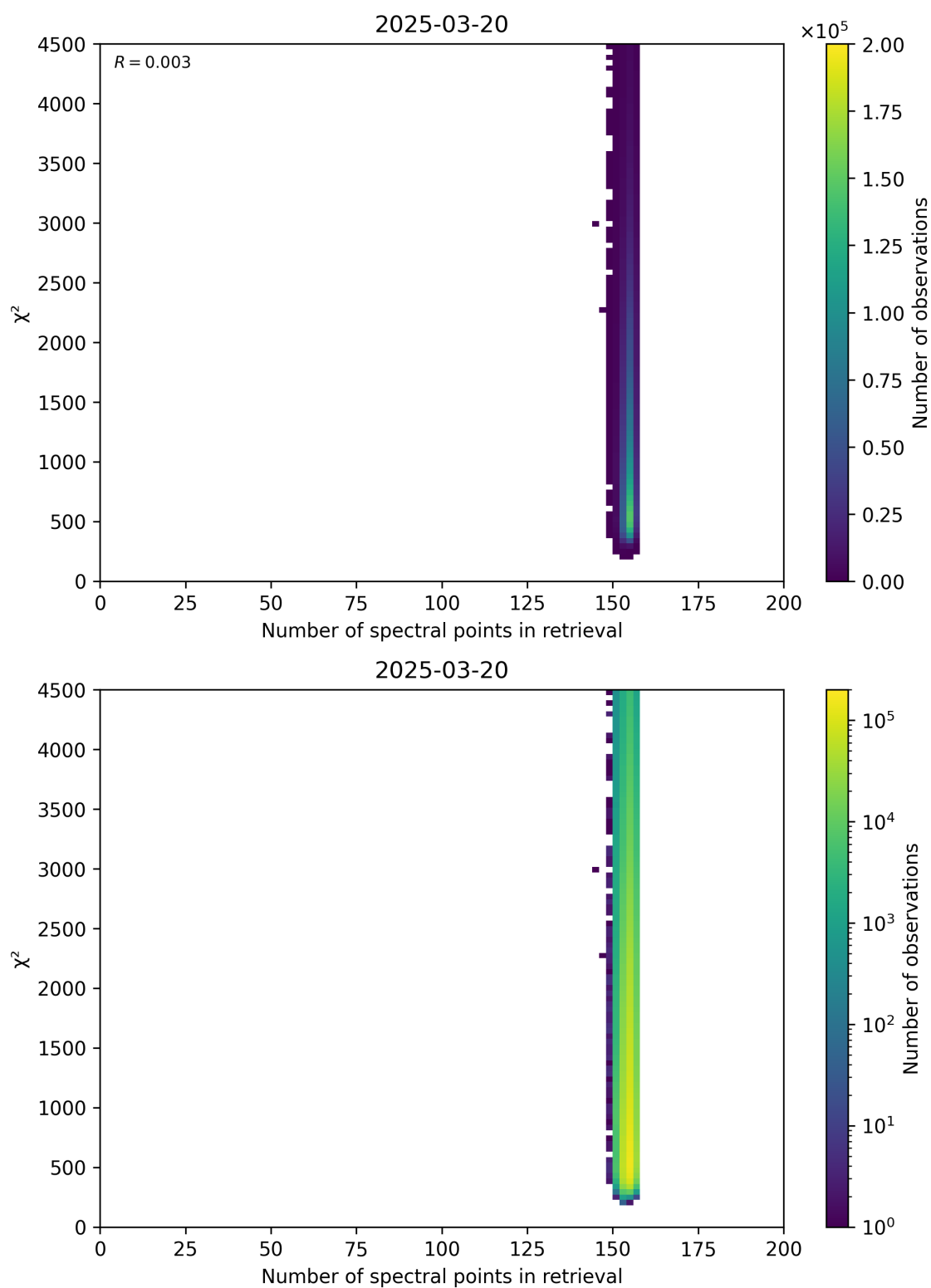
Figure 58: Scatter density plot of “Number of spectral points in retrieval” against “ \chi^2 ” for 2025-03-19 to 2025-03-21.
