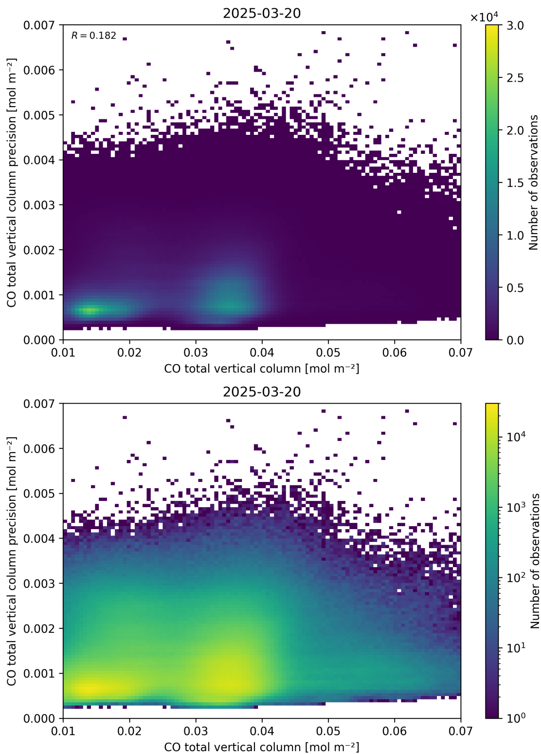
Figure 34: Scatter density plot of “CO total vertical column” against “CO total vertical column precision” for 2025-03-19 to 2025-03-21.
