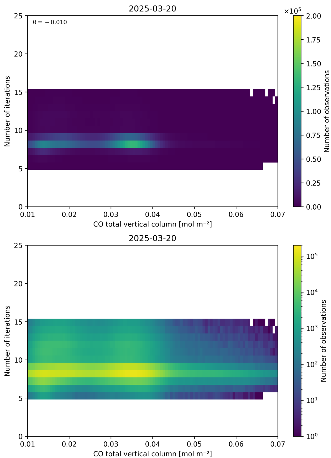
Figure 42: Scatter density plot of “CO total vertical column” against “Number of iterations” for 2025-03-19 to 2025-03-21.
