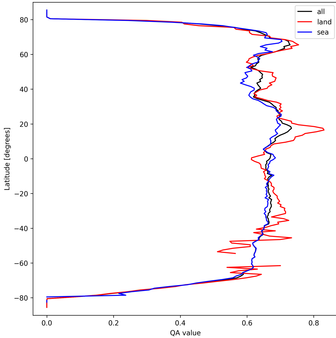
Figure 9: Zonal average of “QA value” for 2025-03-19 to 2025-03-21.
