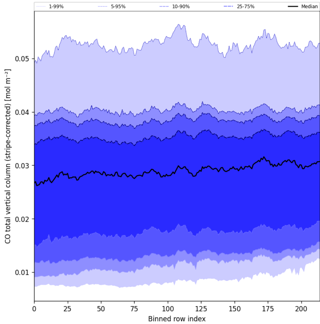
Figure 27: Along track statistics of “CO total vertical column (stripe-corrected)” for 2025-03-19 to 2025-03-21
