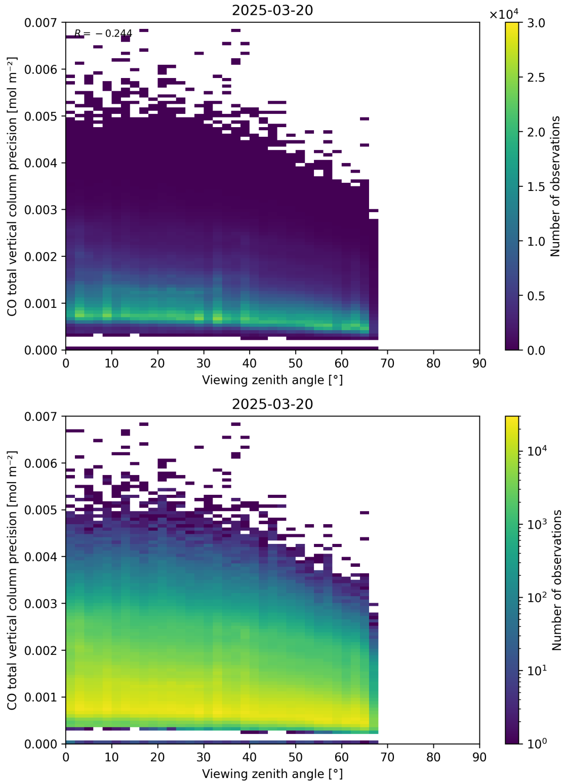
Figure 71: Scatter density plot of “Viewing zenith angle” against “CO total vertical column precision” for 2025-03-19 to 2025-03-21.
