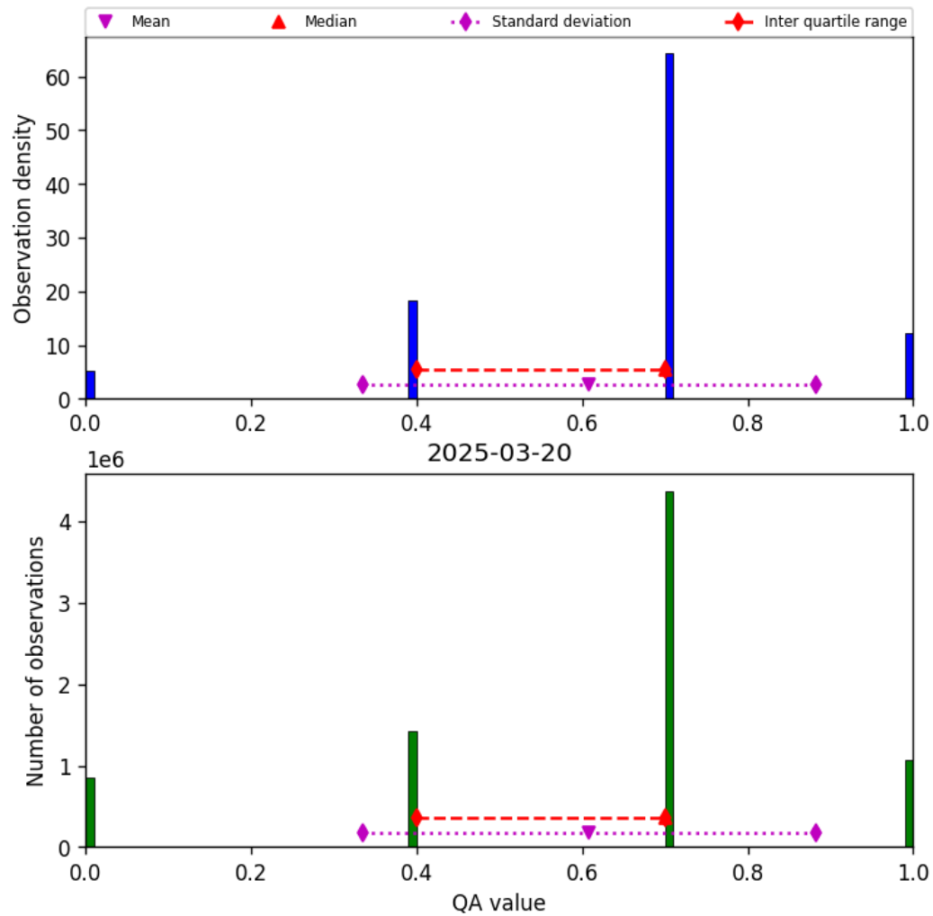
Figure 17: Histogram of “QA value” for 2025-03-19 to 2025-03-21
