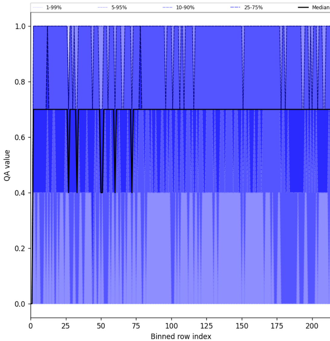
Figure 25: Along track statistics of “QA value” for 2025-03-19 to 2025-03-21
