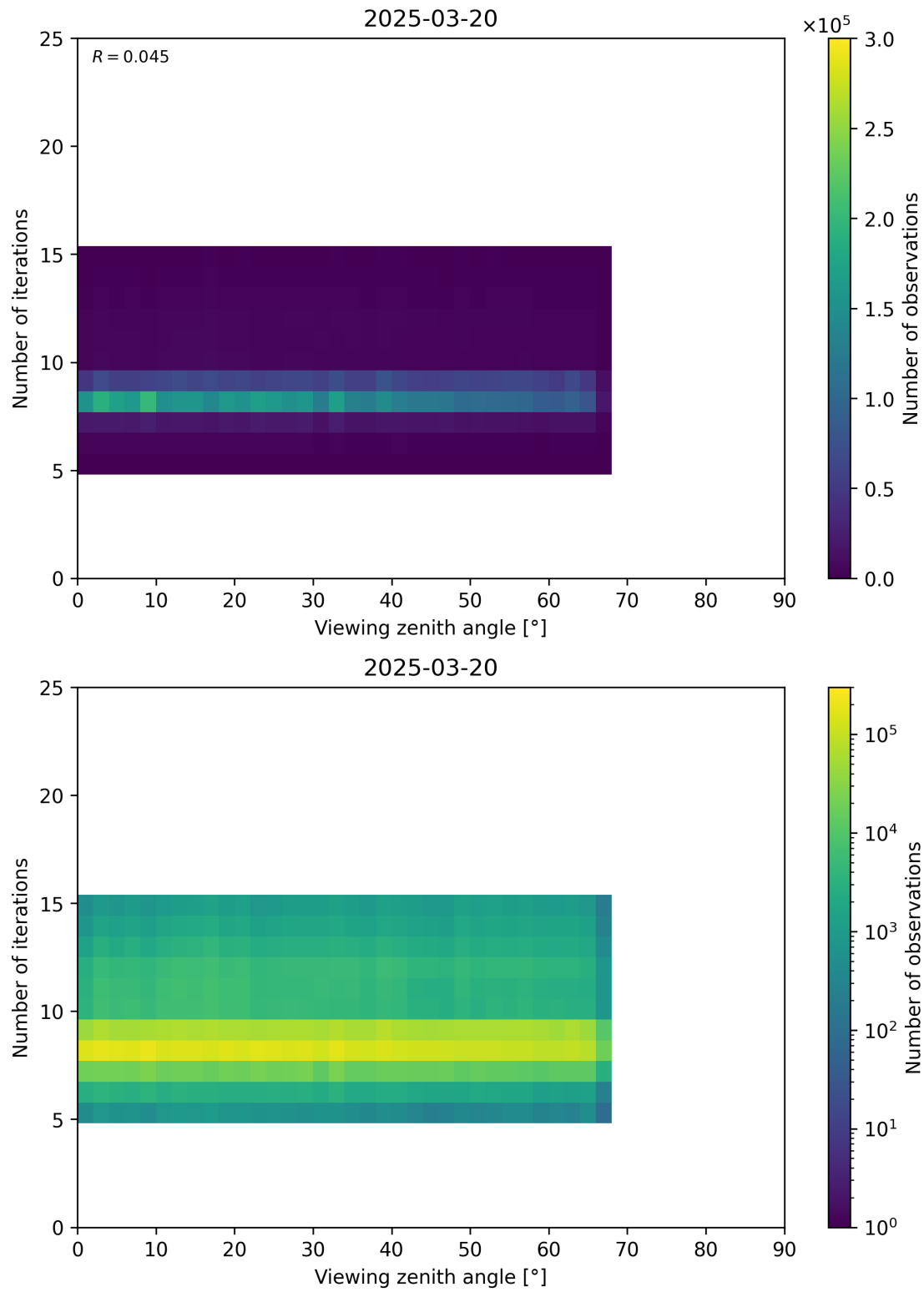
Figure 75: Scatter density plot of “Viewing zenith angle” against “Number of iterations” for 2025-03-19 to 2025-03-21.
