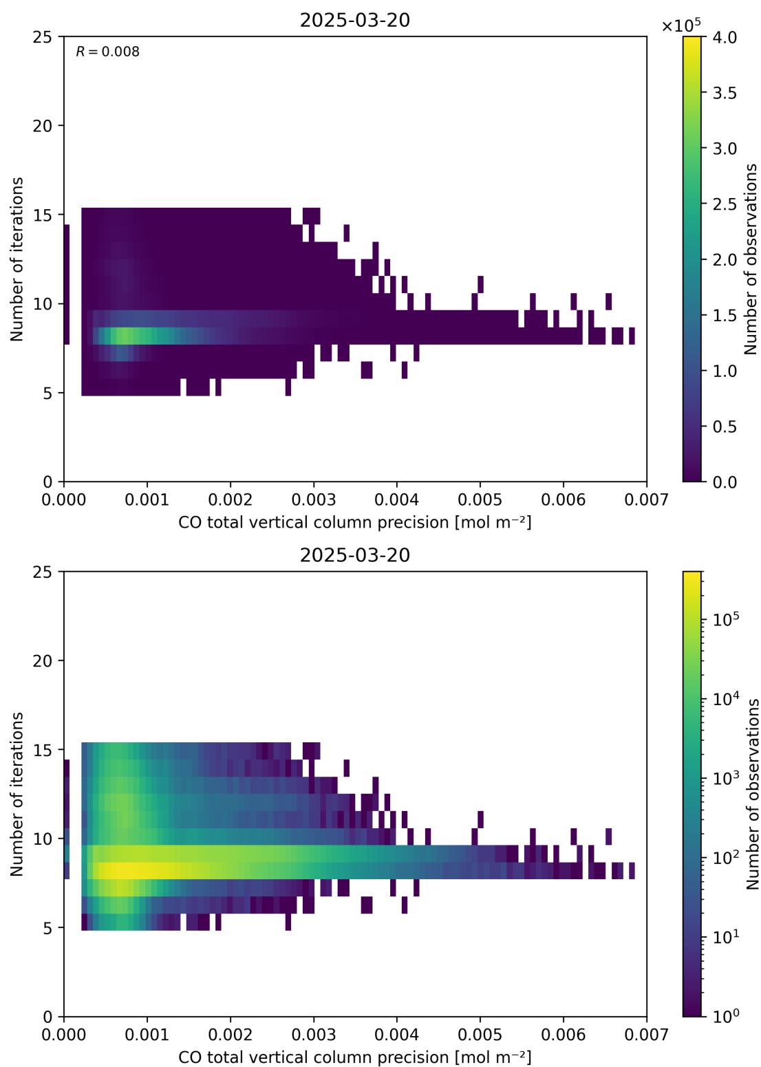
Figure 46: Scatter density plot of “CO total vertical column precision” against “Number of iterations” for 2025-03-19 to 2025-03-21.
