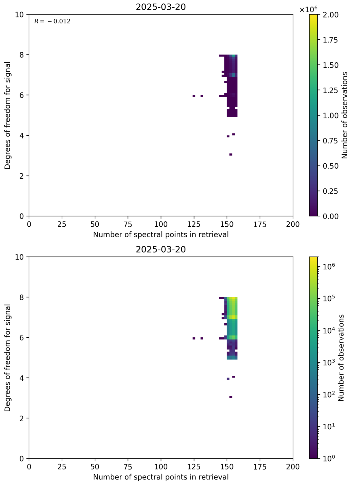
Figure 59: Scatter density plot of “Number of spectral points in retrieval” against “Degrees of freedom for signal” for 2025-03-19 to 2025-03-21.
