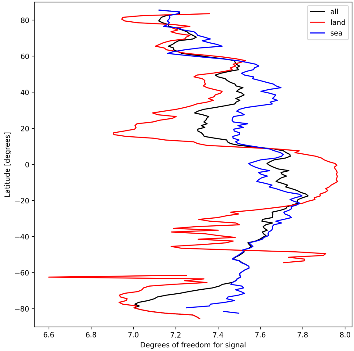
Figure 15: Zonal average of “Degrees of freedom for signal” for 2025-03-19 to 2025-03-21.
