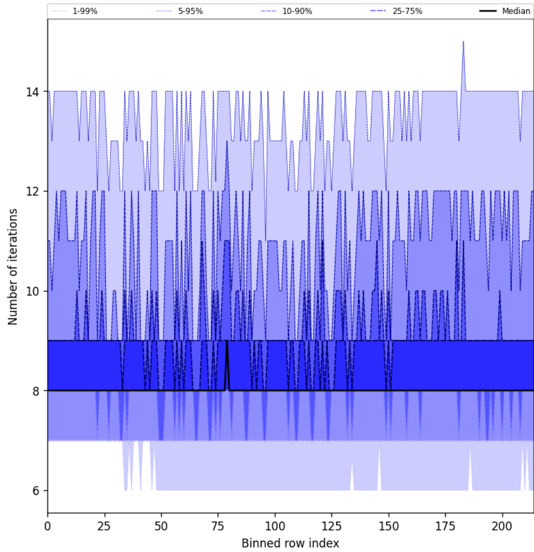
Figure 32: Along track statistics of “Number of iterations” for 2025-03-19 to 2025-03-21
