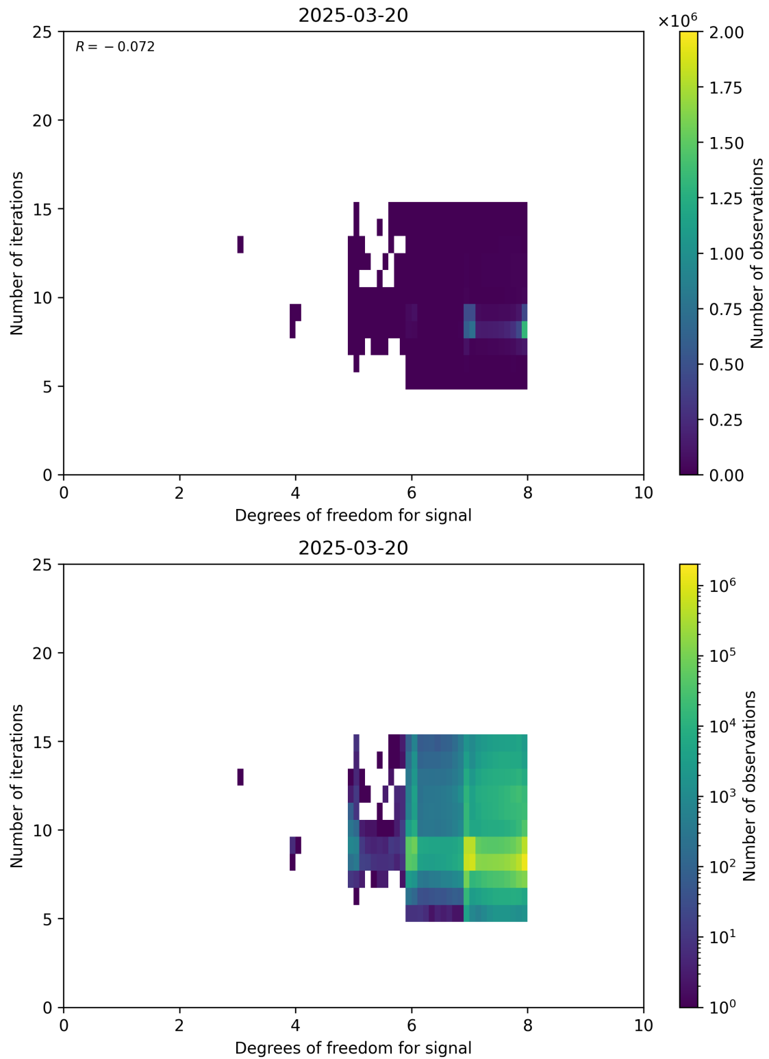
Figure 50: Scatter density plot of “Degrees of freedom for signal” against “Number of iterations” for 2025-03-19 to 2025-03-21.
