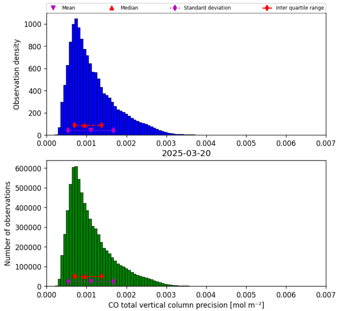
Figure 20: Histogram of “CO total vertical column precision” for 2025-03-19 to 2025-03-21
