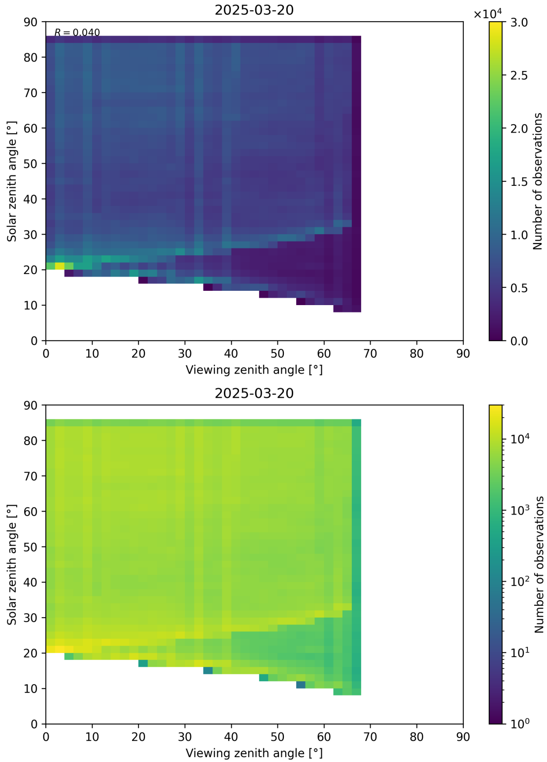
Figure 77: Scatter density plot of “Viewing zenith angle” against “Solar zenith angle” for 2025-03-19 to 2025-03-21.
