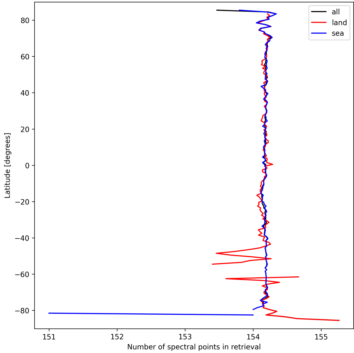
Figure 13: Zonal average of “Number of spectral points in retrieval” for 2025-03-19 to 2025-03-21.
