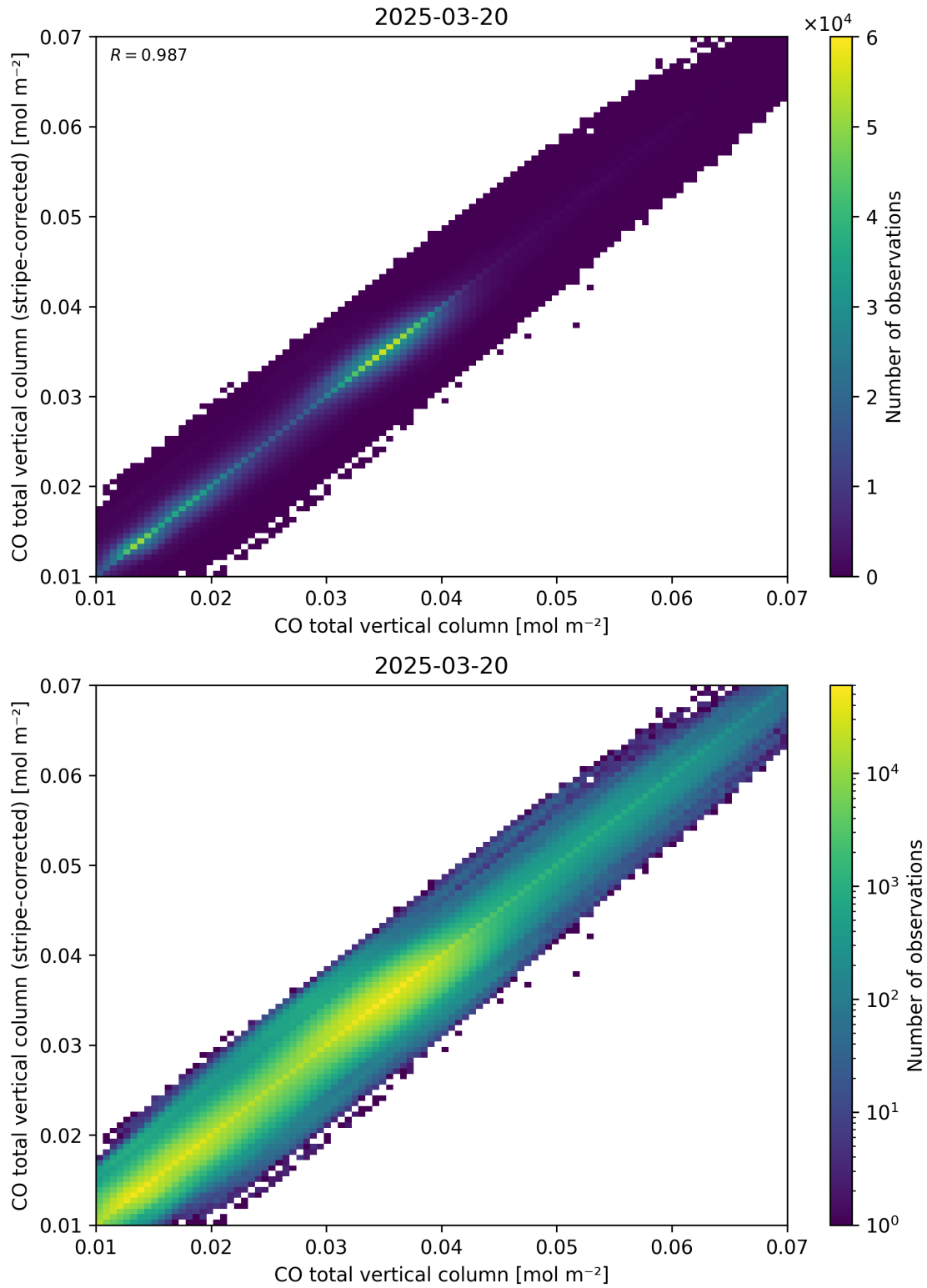
Figure 33: Scatter density plot of “CO total vertical column” against “CO total vertical column (stripe-corrected)” for 2025-03-19 to 2025-03-21.
