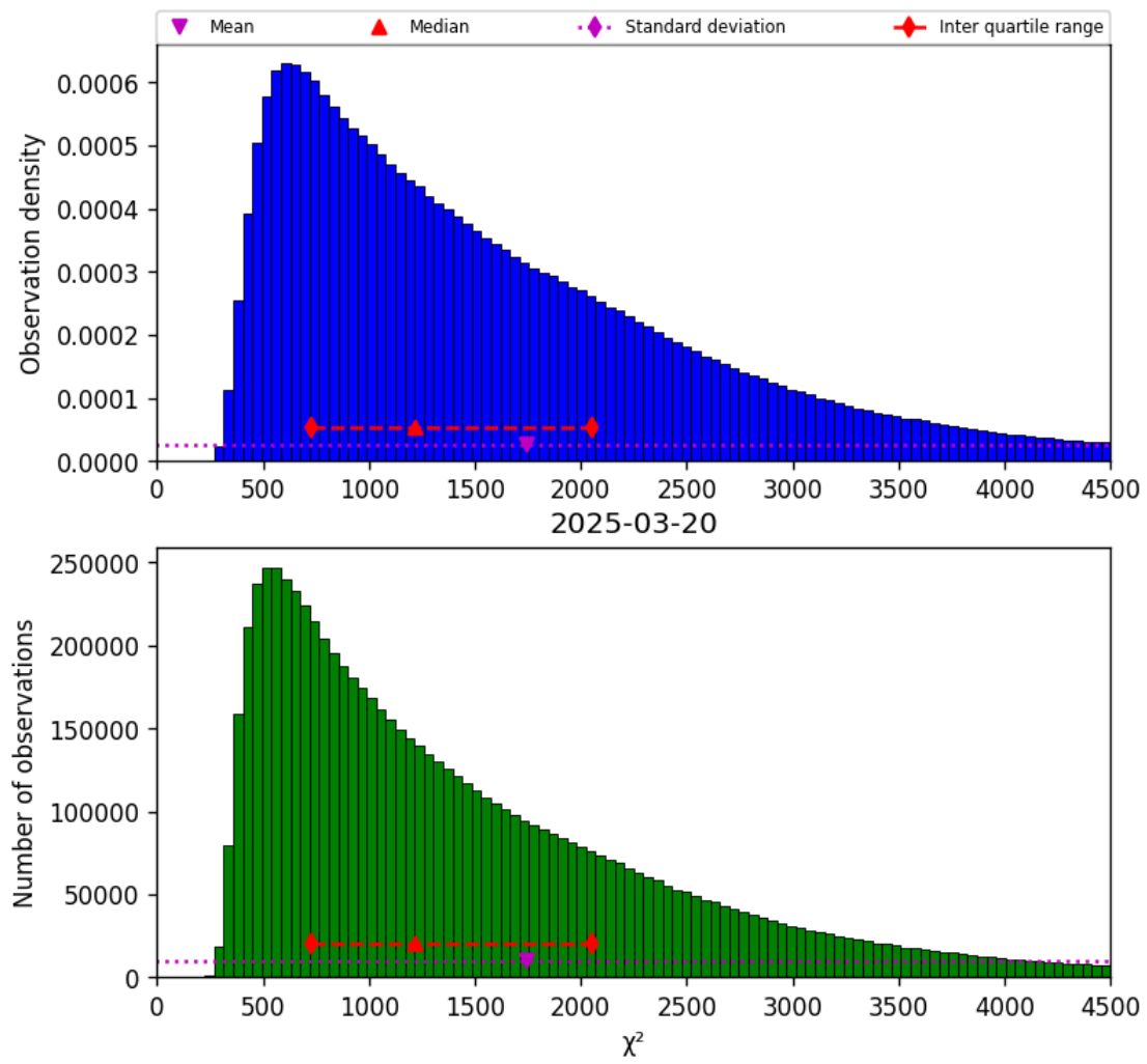
Figure 22: Histogram of “ \chi^2 ” for 2025-03-19 to 2025-03-21
