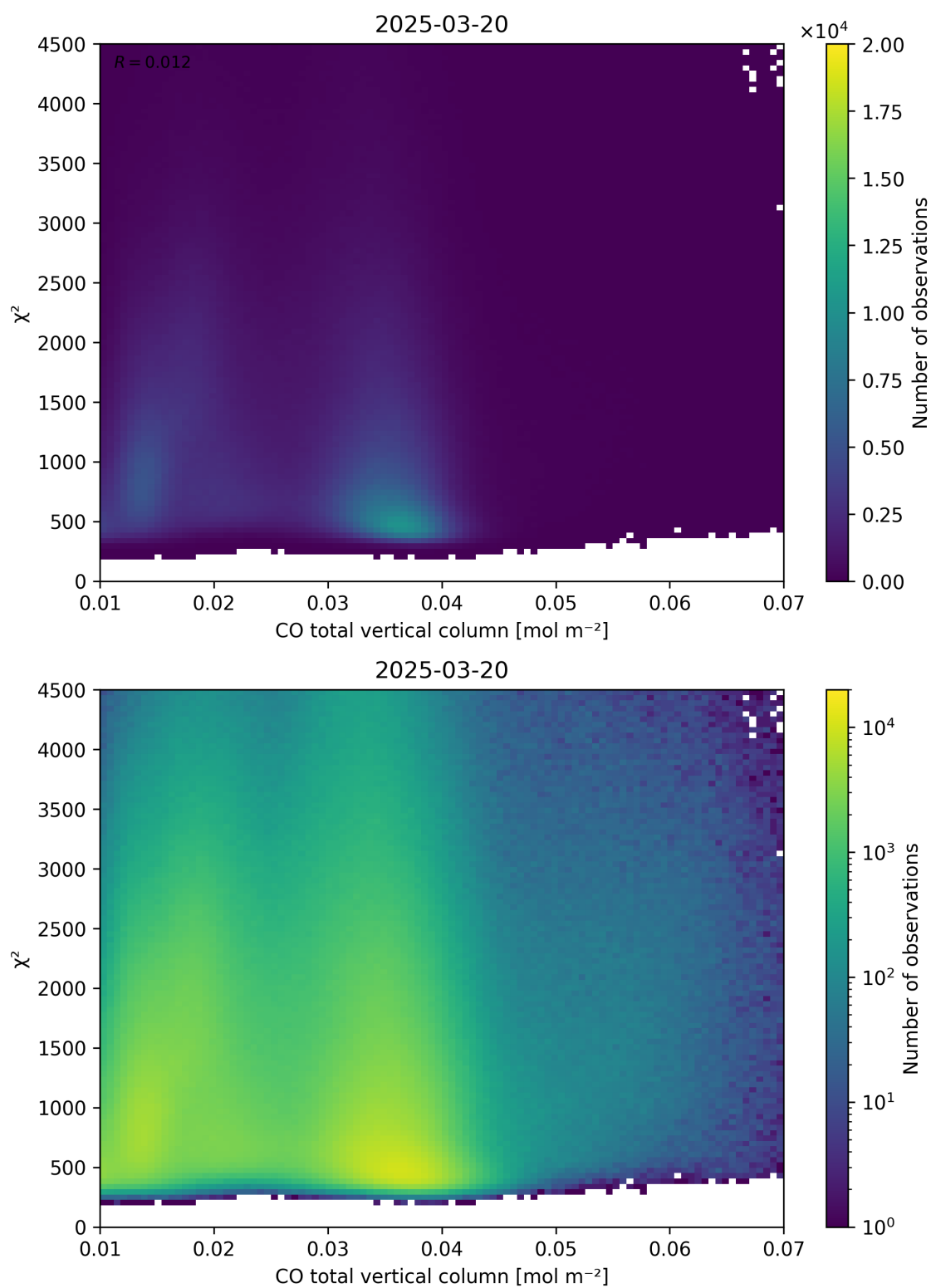
Figure 35: Scatter density plot of “CO total vertical column” against “ \chi^2 ” for 2025-03-19 to 2025-03-21.
