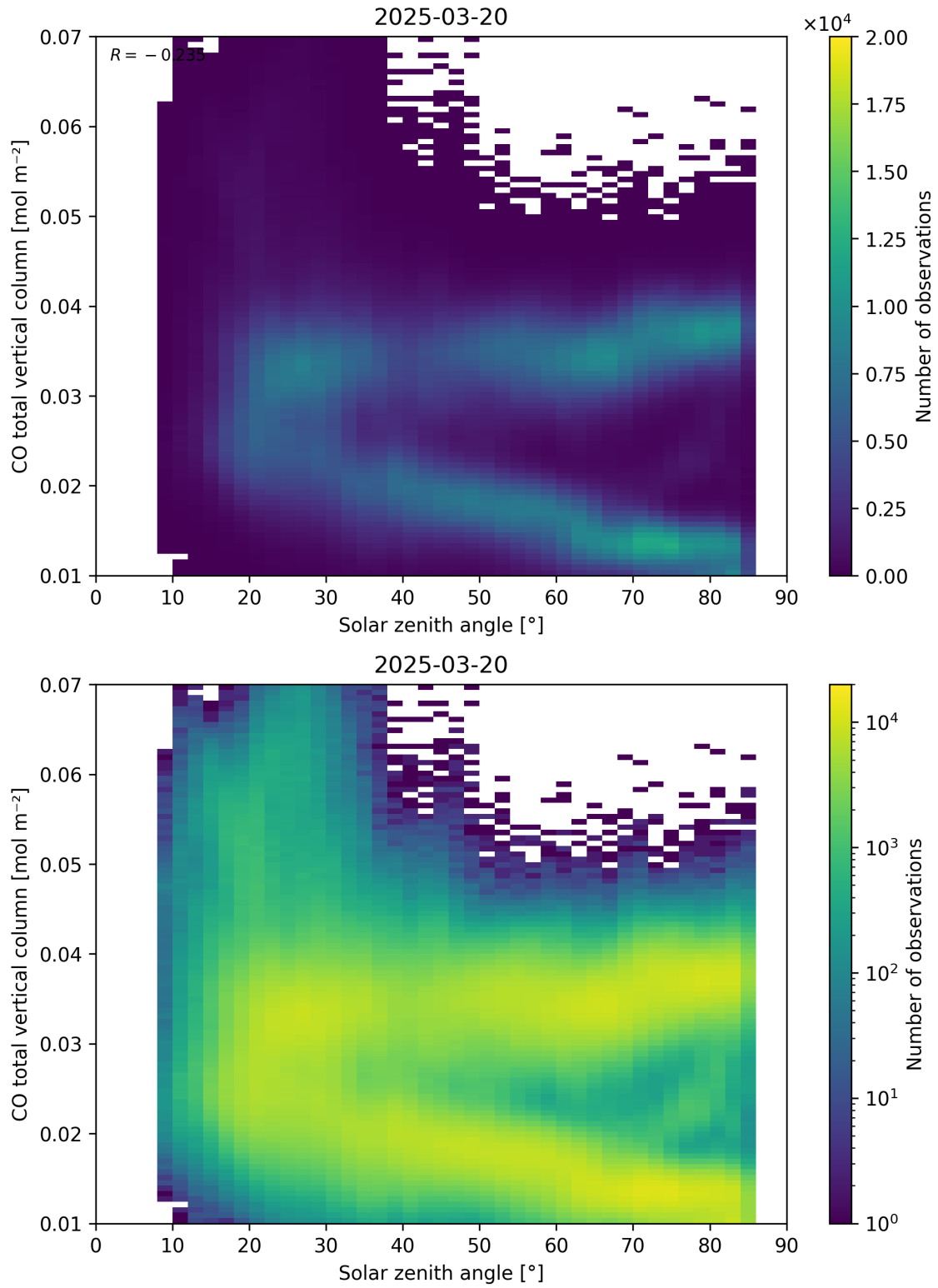
Figure 61: Scatter density plot of “Solar zenith angle” against “CO total vertical column” for 2025-03-19 to 2025-03-21.
