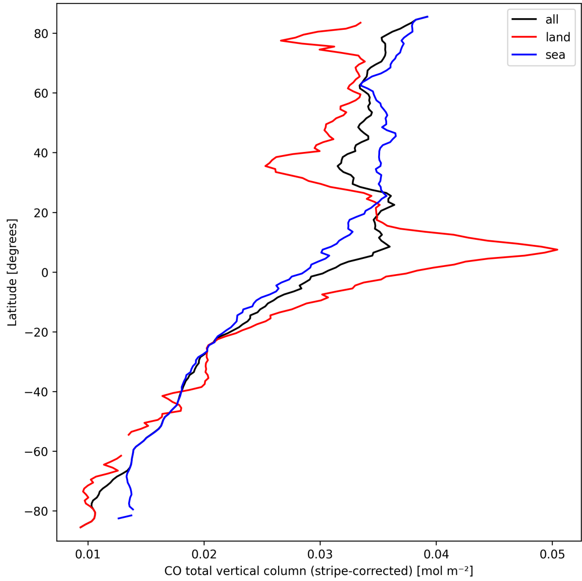
Figure 11: Zonal average of “CO total vertical column (stripe-corrected)” for 2025-03-19 to 2025-03-21.
