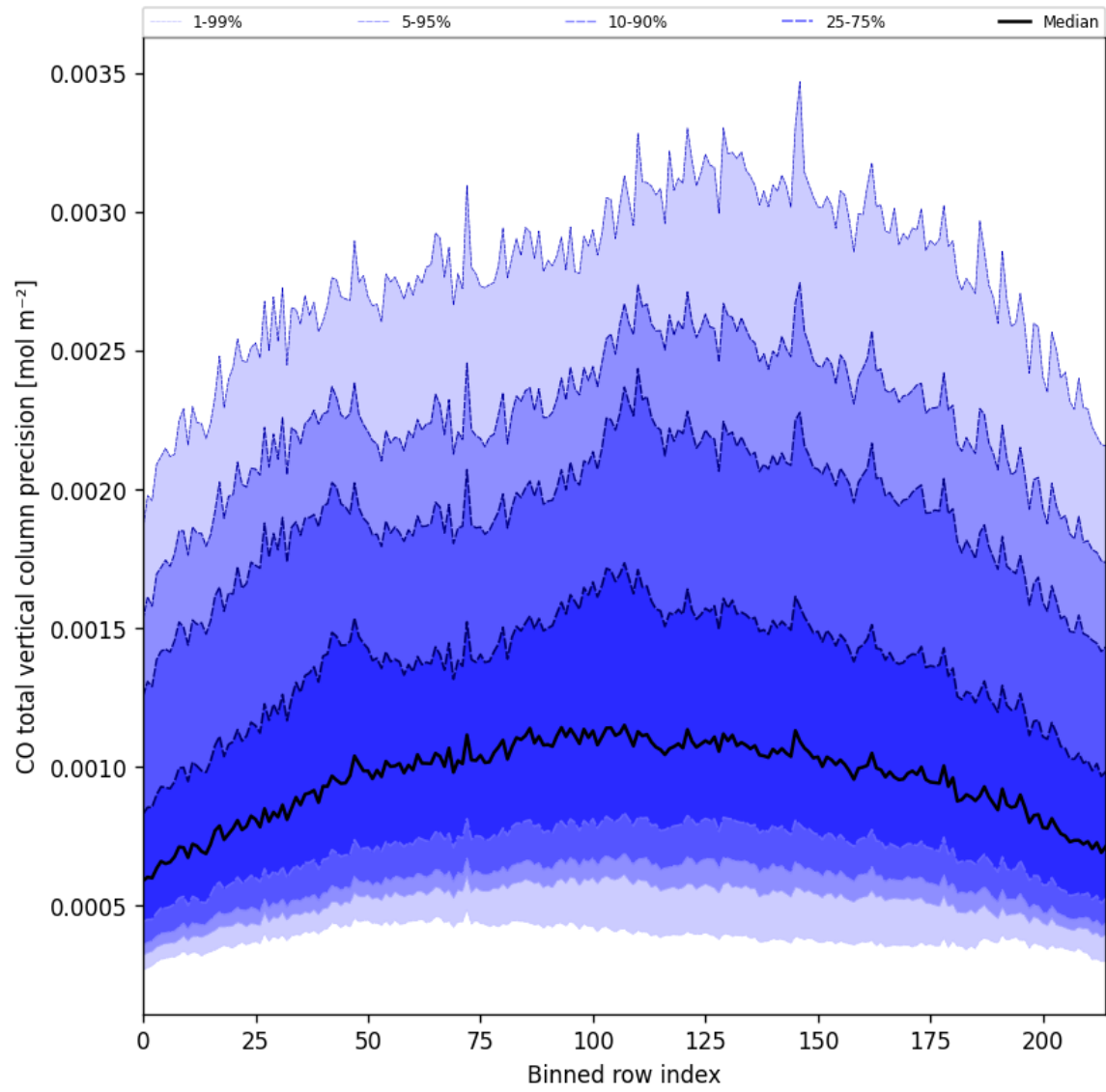
Figure 28: Along track statistics of “CO total vertical column precision” for 2025-03-19 to 2025-03-21
