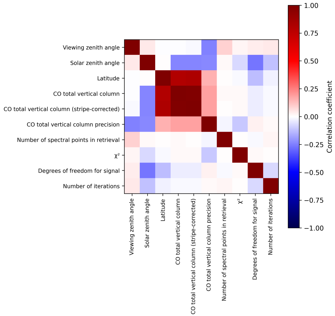
Figure 2: Map of correlation matrix for 2025-03-19 to 2025-03-21.
