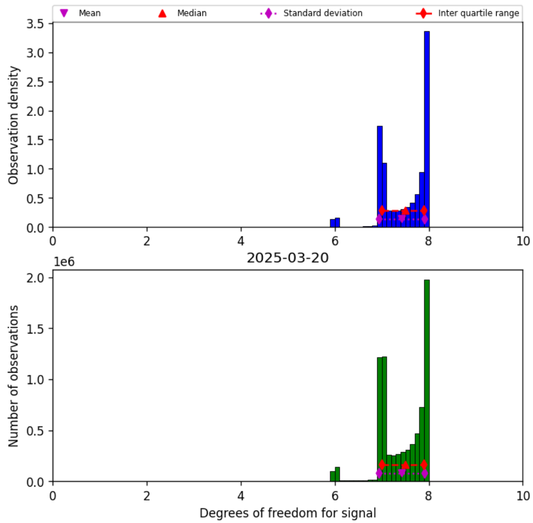
Figure 23: Histogram of “Degrees of freedom for signal” for 2025-03-19 to 2025-03-21
