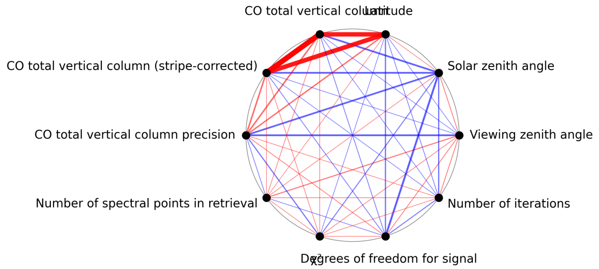
Figure 1: Map of correlation graph for 2025-03-19 to 2025-03-21.
