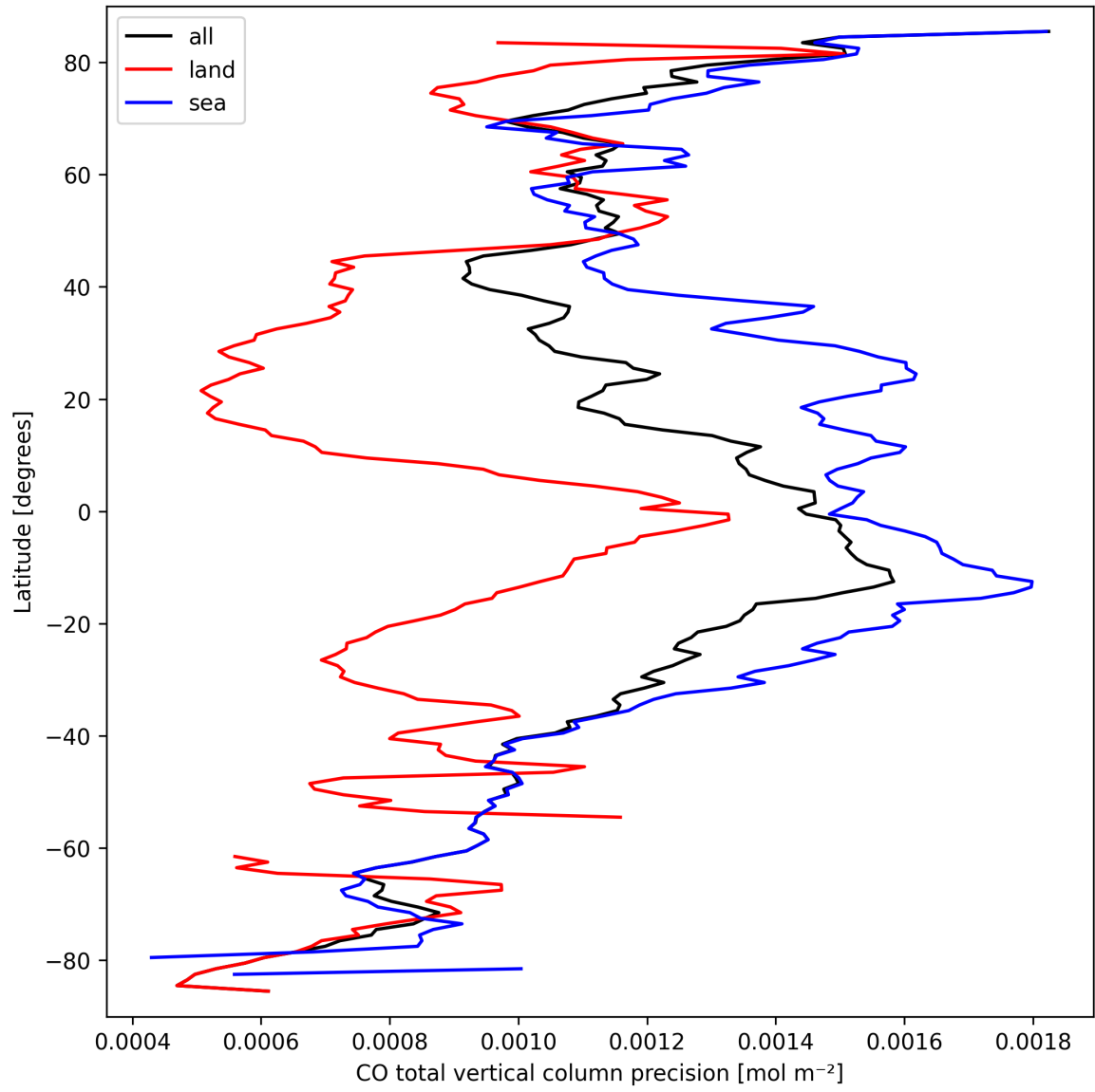
Figure 12: Zonal average of “CO total vertical column precision” for 2025-03-19 to 2025-03-21.
