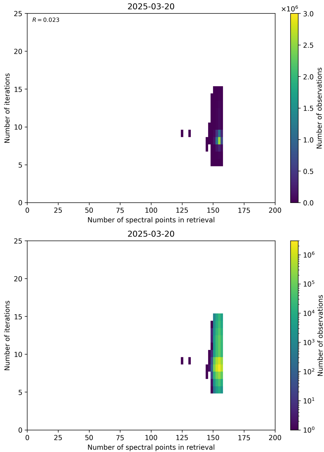
Figure 60: Scatter density plot of “Number of spectral points in retrieval” against “Number of iterations” for 2025-03-19 to 2025-03-21.
