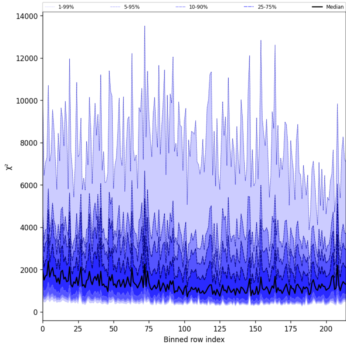
Figure 30: Along track statistics of “ \chi^2 ” for 2025-03-19 to 2025-03-21
