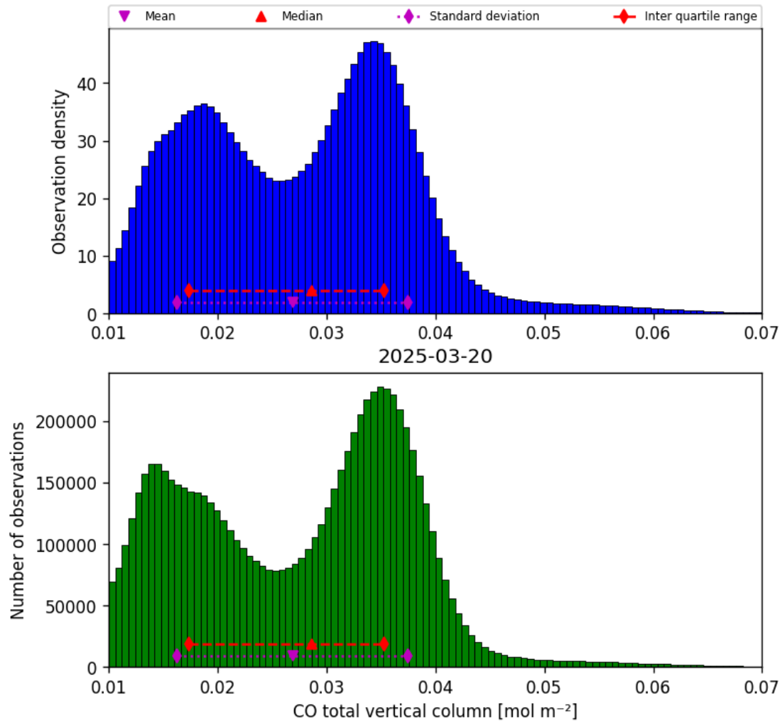
Figure 18: Histogram of “CO total vertical column” for 2025-03-19 to 2025-03-21
