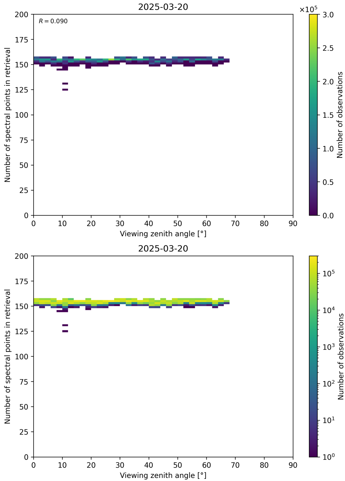
Figure 76: Scatter density plot of “Viewing zenith angle” against “Number of spectral points in retrieval” for 2025-03-19 to 2025-03-21.
