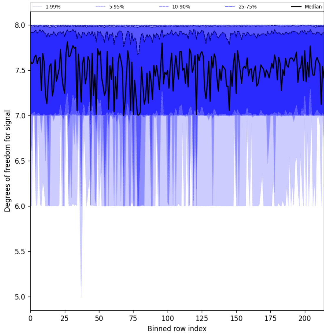
Figure 31: Along track statistics of “Degrees of freedom for signal” for 2025-03-19 to 2025-03-21
