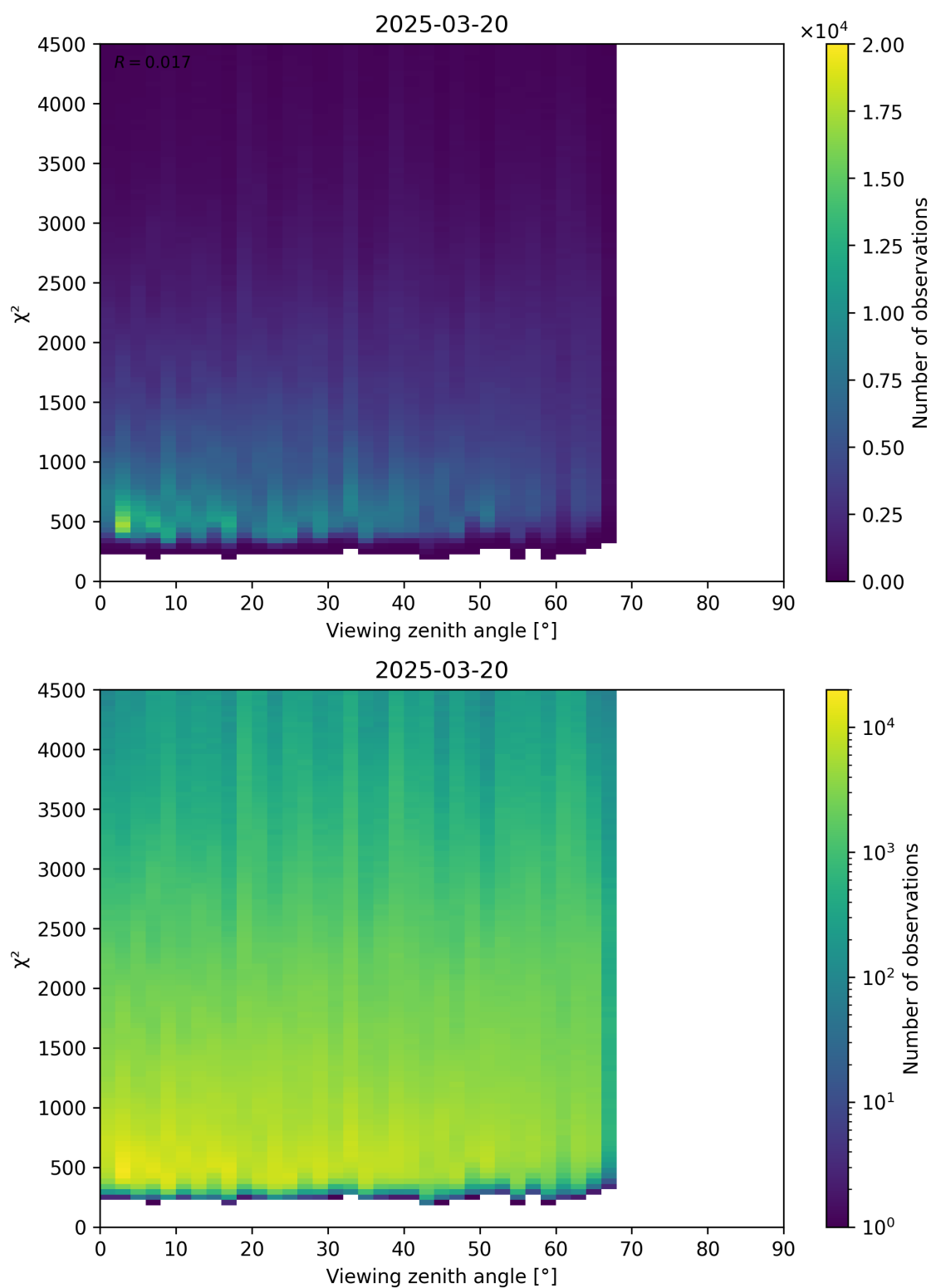
Figure 72: Scatter density plot of “Viewing zenith angle” against “ \chi^2 ” for 2025-03-19 to 2025-03-21.
