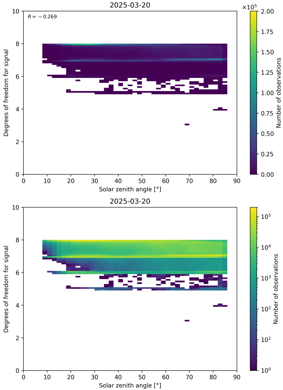
Figure 65: Scatter density plot of “Solar zenith angle” against “Degrees of freedom for signal” for 2025-03-19 to 2025-03-21.
