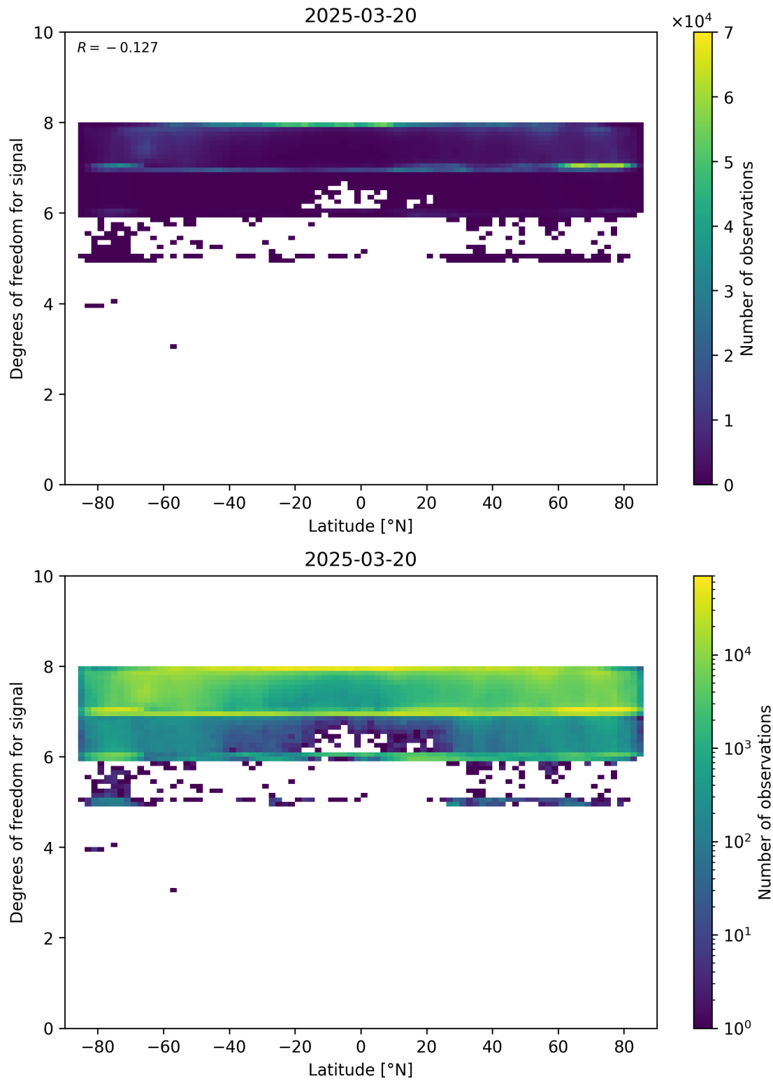
Figure 55: Scatter density plot of “Latitude” against “Degrees of freedom for signal” for 2025-03-19 to 2025-03-21.
