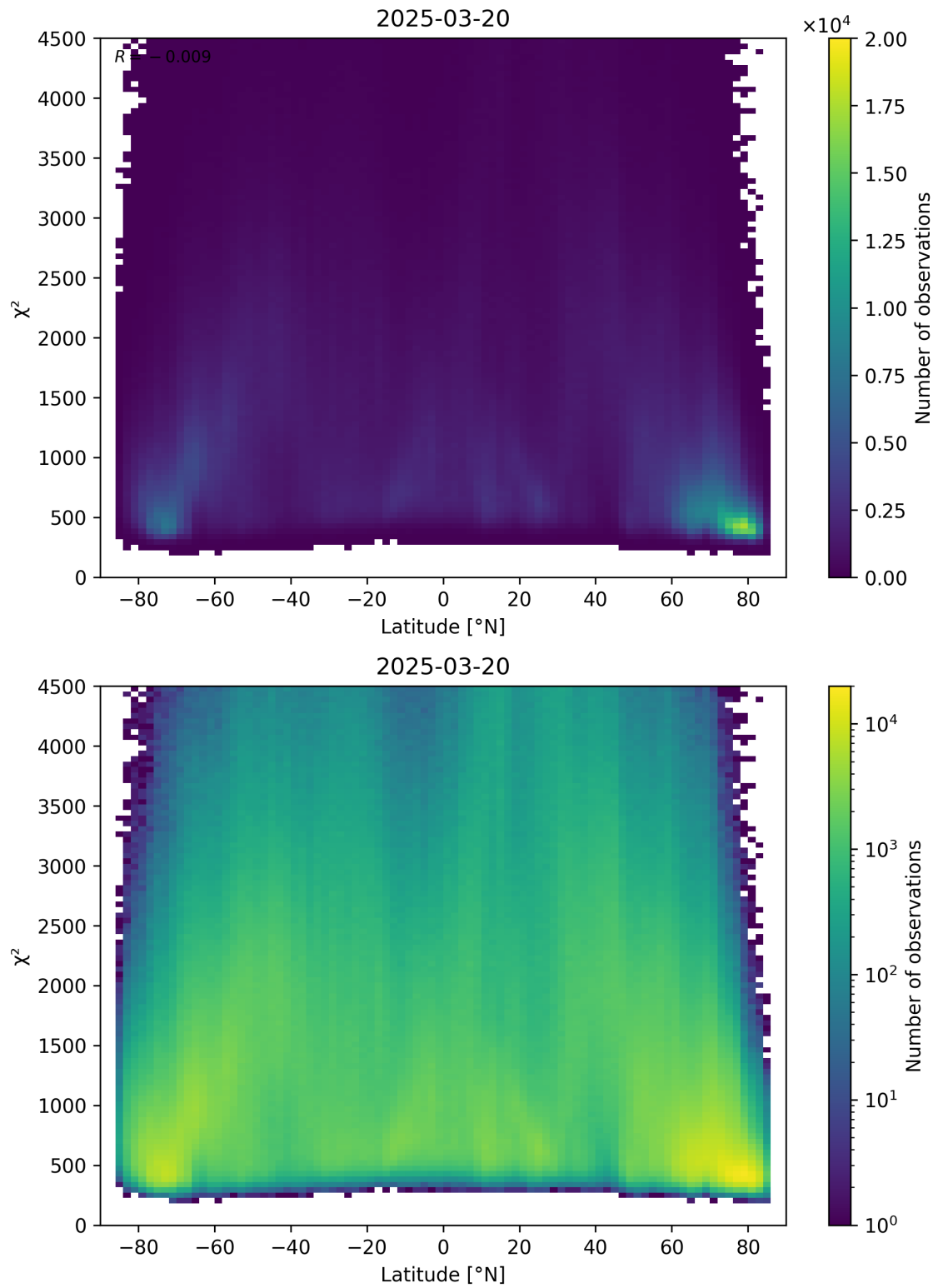
Figure 54: Scatter density plot of “Latitude” against “ \chi^2 ” for 2025-03-19 to 2025-03-21.
