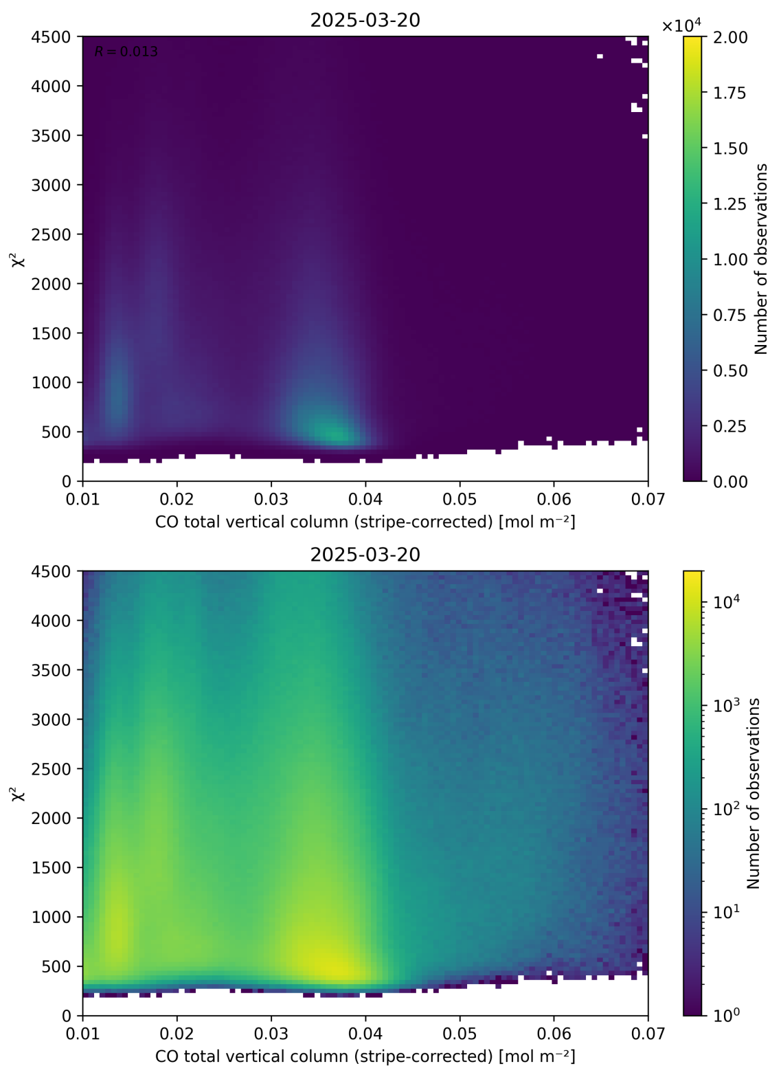
Figure 37: Scatter density plot of “CO total vertical column (stripe-corrected)” against “ \chi^2 ” for 2025-03-19 to 2025-03-21.
