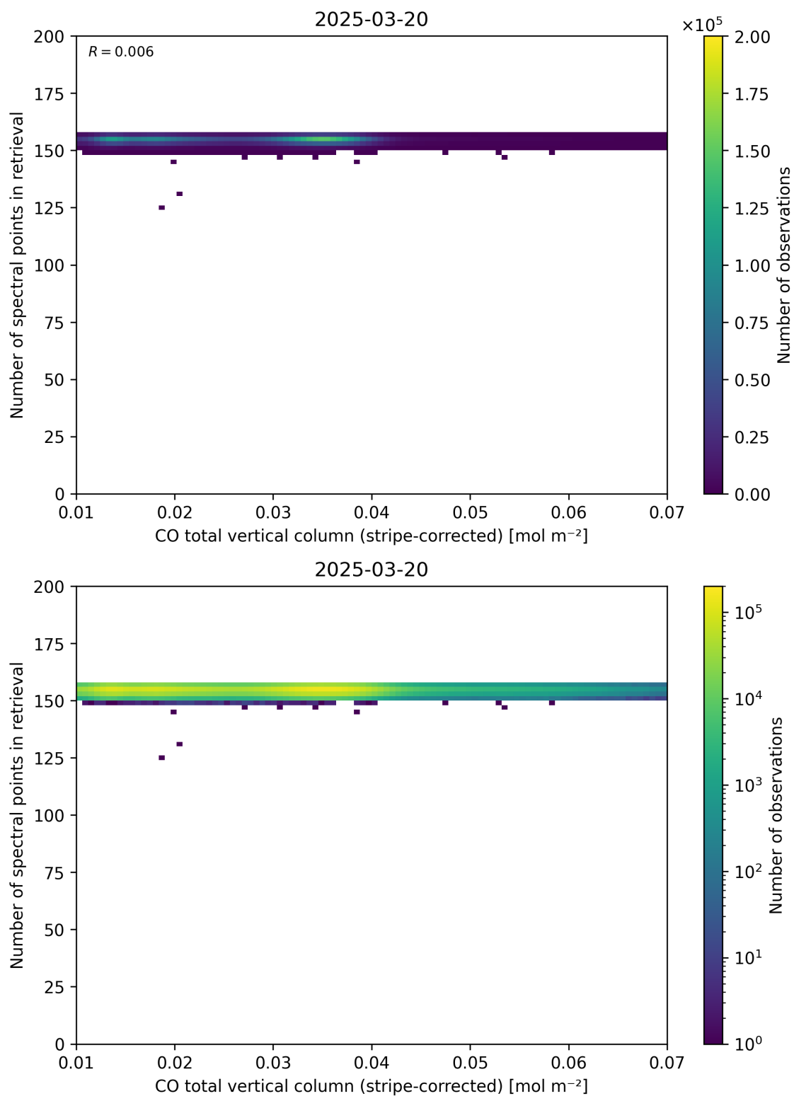
Figure 40: Scatter density plot of “CO total vertical column (stripe-corrected)” against “Number of spectral points in retrieval” for 2025-03-19 to 2025-03-21.
