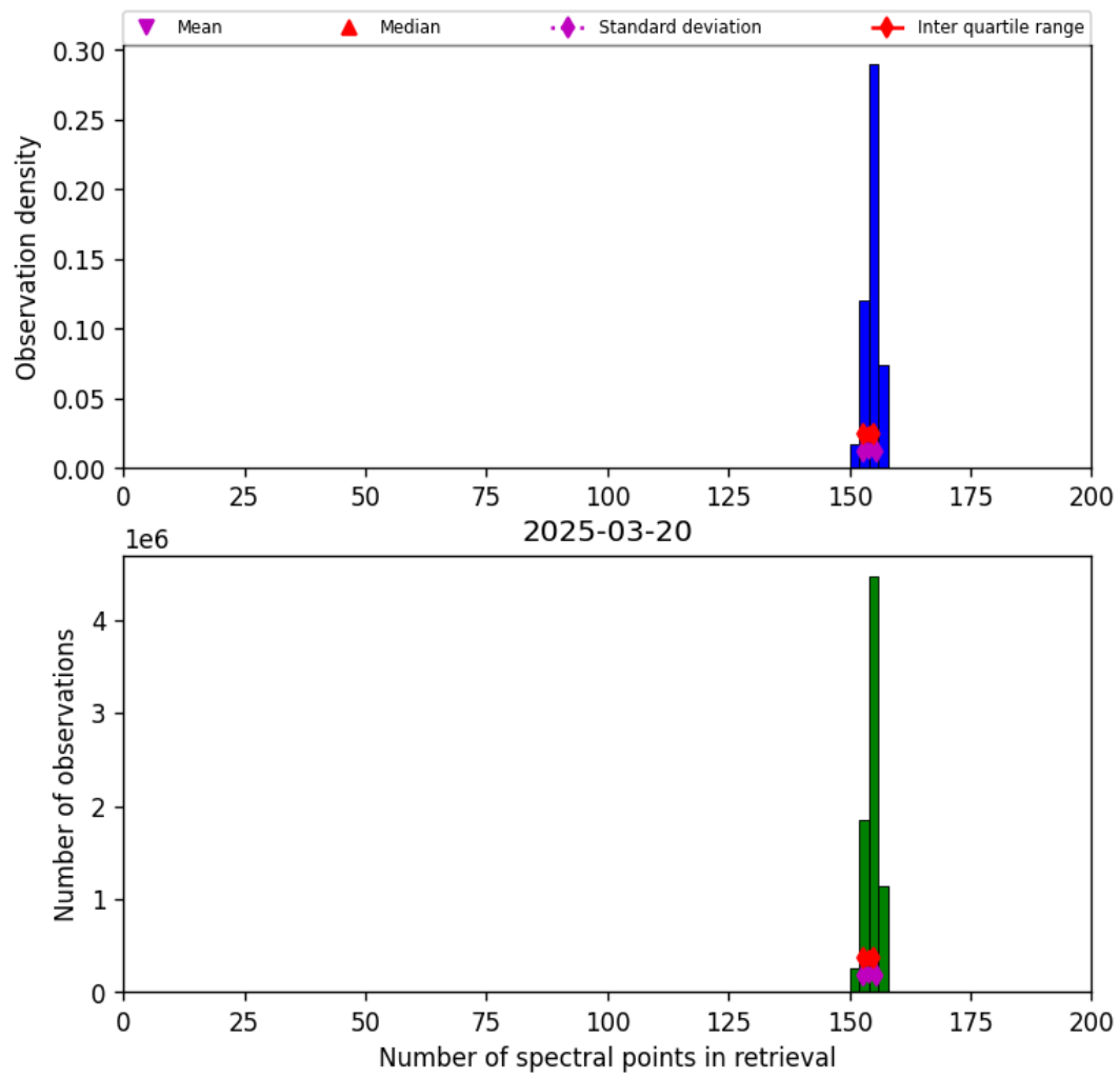
Figure 21: Histogram of “Number of spectral points in retrieval” for 2025-03-19 to 2025-03-21
