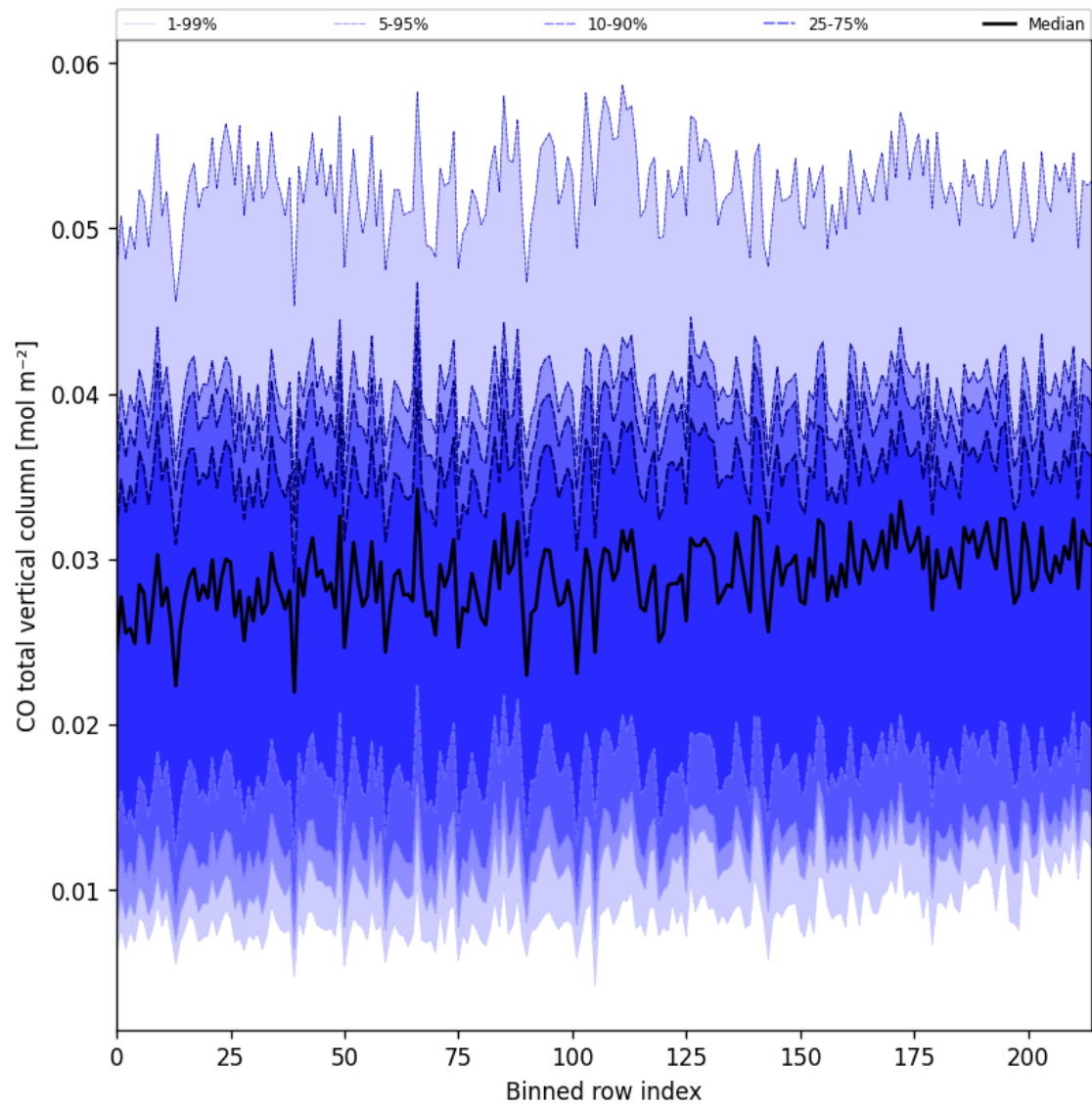
Figure 26: Along track statistics of “CO total vertical column” for 2025-03-19 to 2025-03-21
