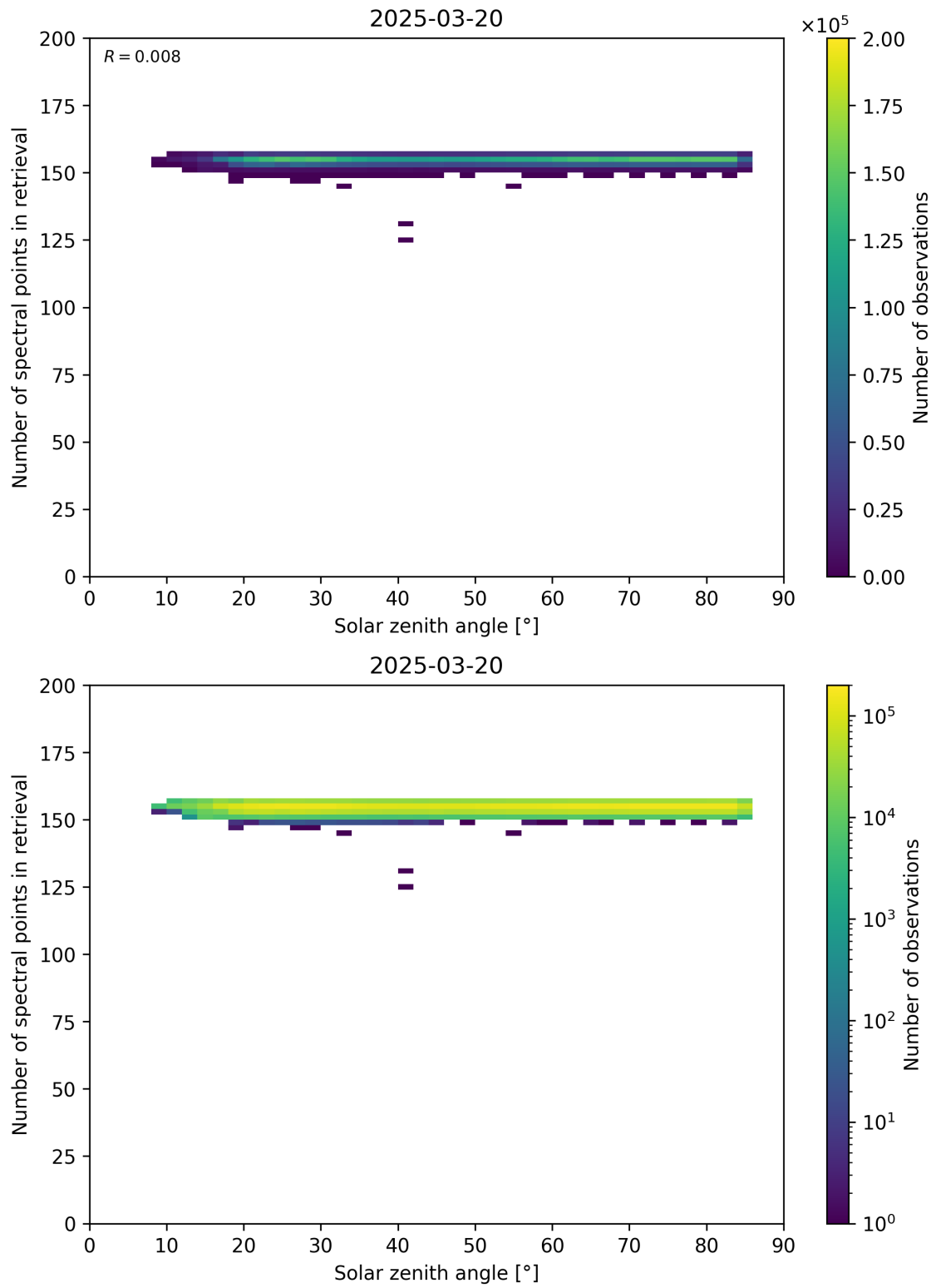
Figure 68: Scatter density plot of “Solar zenith angle” against “Number of spectral points in retrieval” for 2025-03-19 to 2025-03-21.
