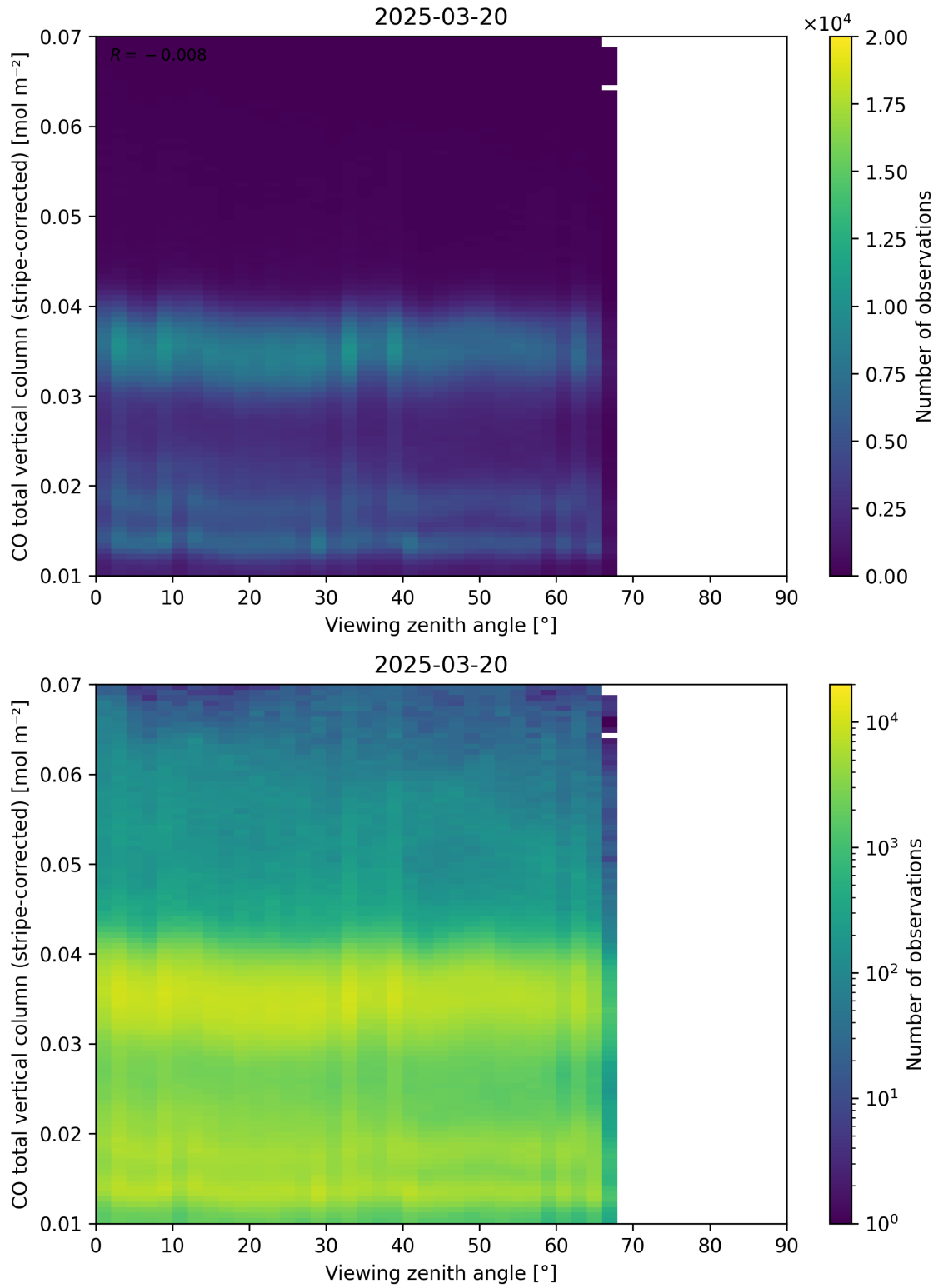
Figure 70: Scatter density plot of “Viewing zenith angle” against “CO total vertical column (stripe-corrected)” for 2025-03-19 to 2025-03-21.
