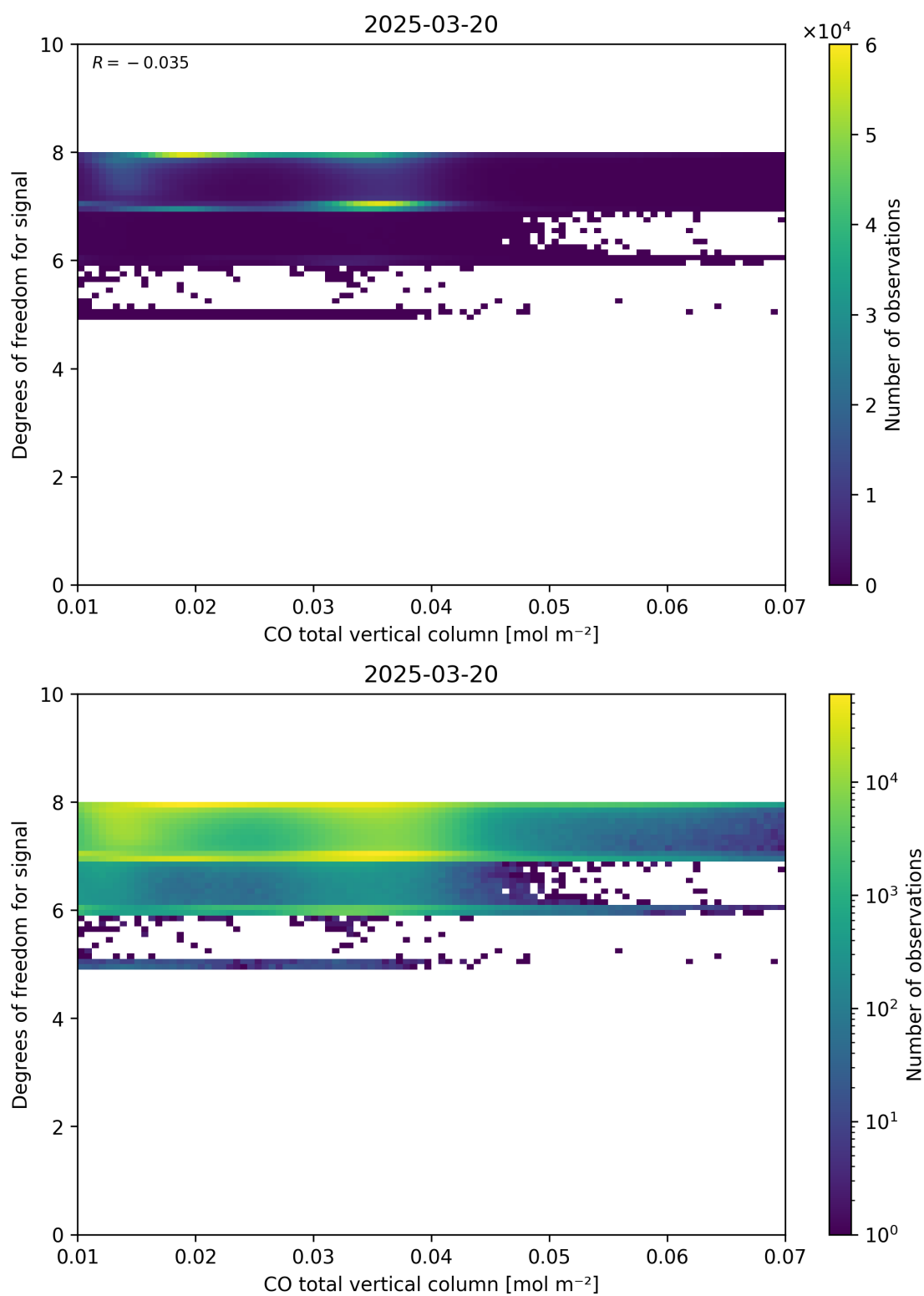
Figure 41: Scatter density plot of “CO total vertical column” against “Degrees of freedom for signal” for 2025-03-19 to 2025-03-21.
