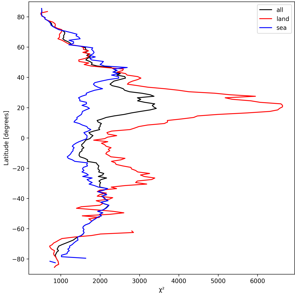
Figure 14: Zonal average of “ \chi^2 ” for 2025-03-19 to 2025-03-21.
