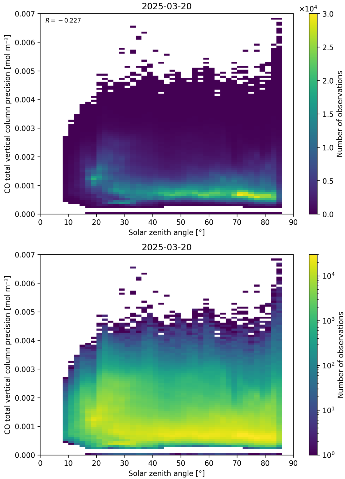
Figure 63: Scatter density plot of “Solar zenith angle” against “CO total vertical column precision” for 2025-03-19 to 2025-03-21.
