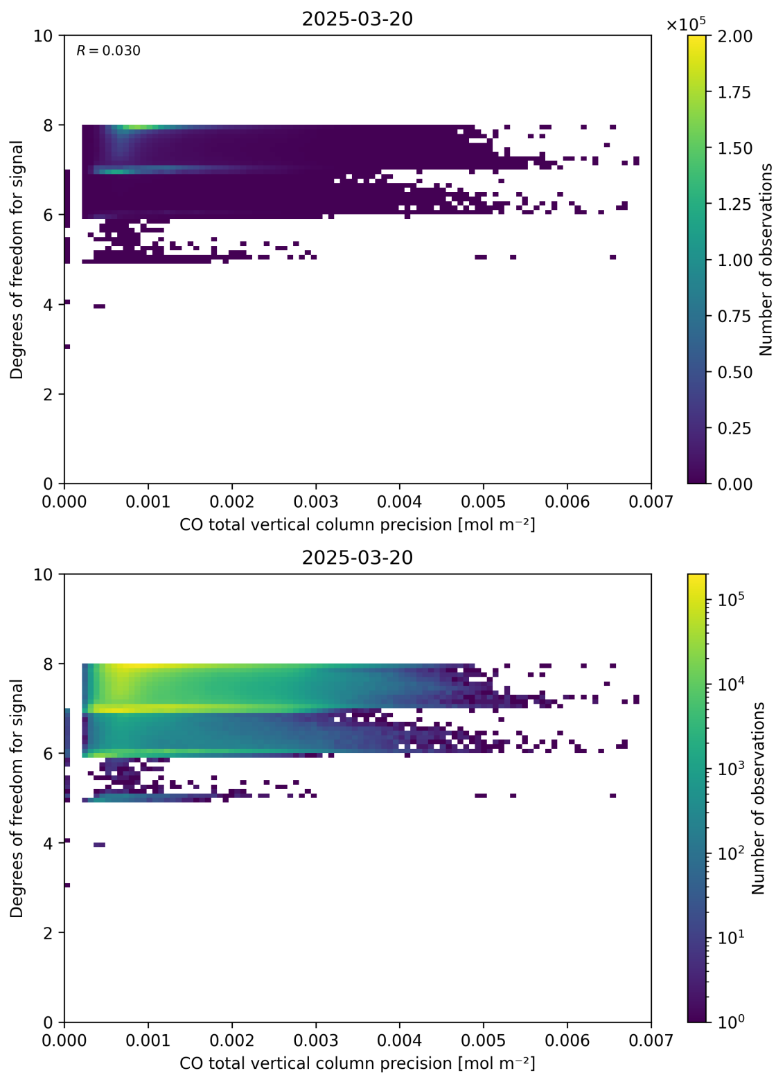
Figure 45: Scatter density plot of “CO total vertical column precision” against “Degrees of freedom for signal” for 2025-03-19 to 2025-03-21.
