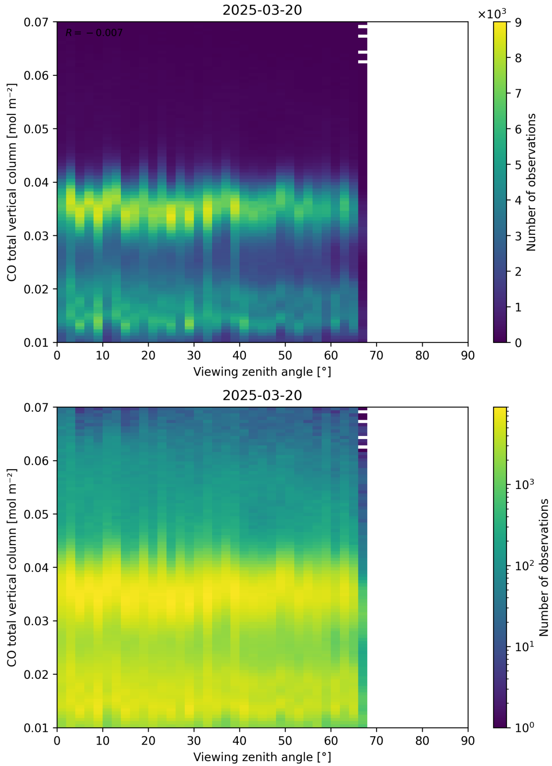
Figure 69: Scatter density plot of “Viewing zenith angle” against “CO total vertical column” for 2025-03-19 to 2025-03-21.
