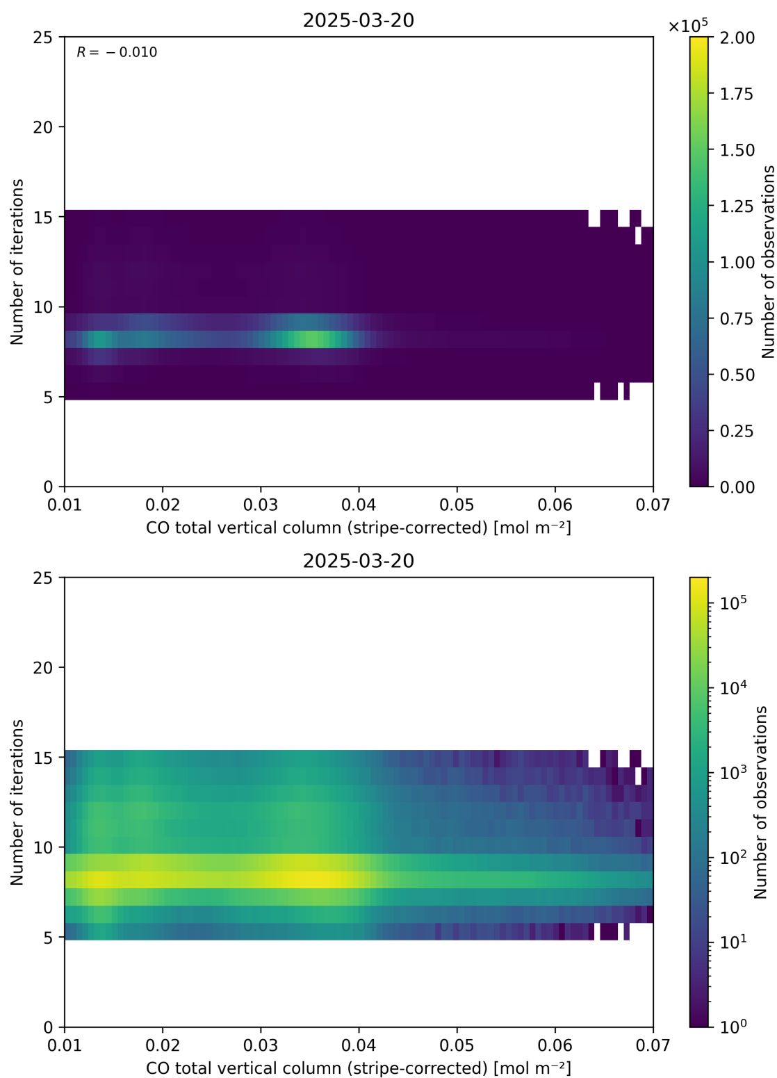
Figure 39: Scatter density plot of “CO total vertical column (stripe-corrected)” against “Number of iterations” for 2025-03-19 to 2025-03-21.
