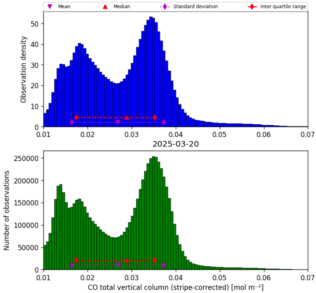
Figure 19: Histogram of “CO total vertical column (stripe-corrected)” for 2025-03-19 to 2025-03-21
