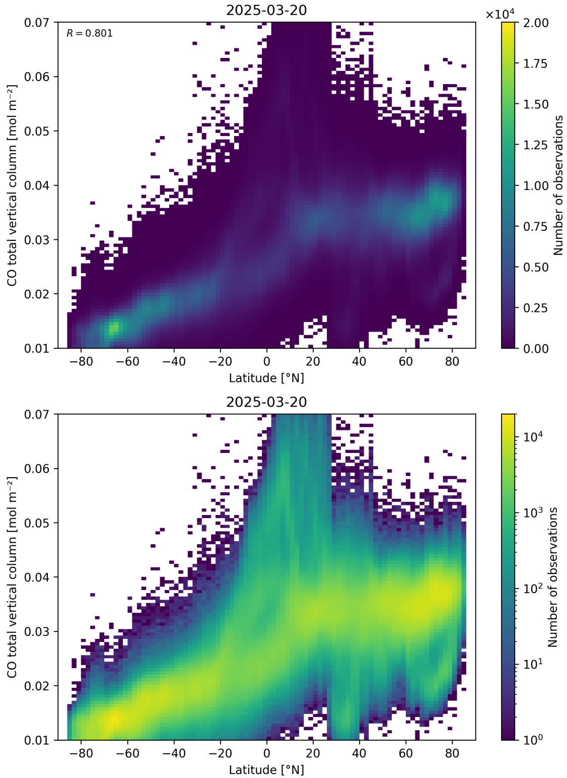
Figure 51: Scatter density plot of “Latitude” against “CO total vertical column” for 2025-03-19 to 2025-03-21.
