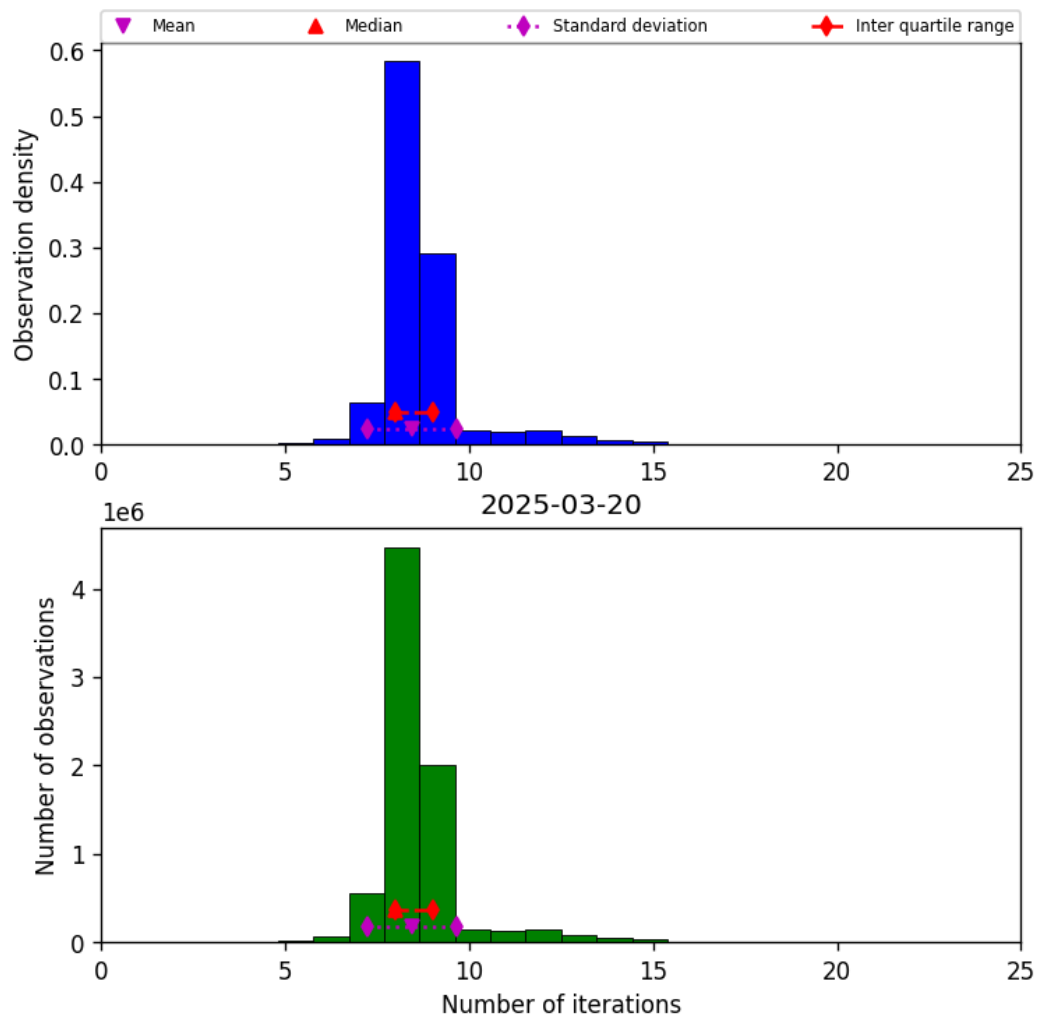
Figure 24: Histogram of “Number of iterations” for 2025-03-19 to 2025-03-21
