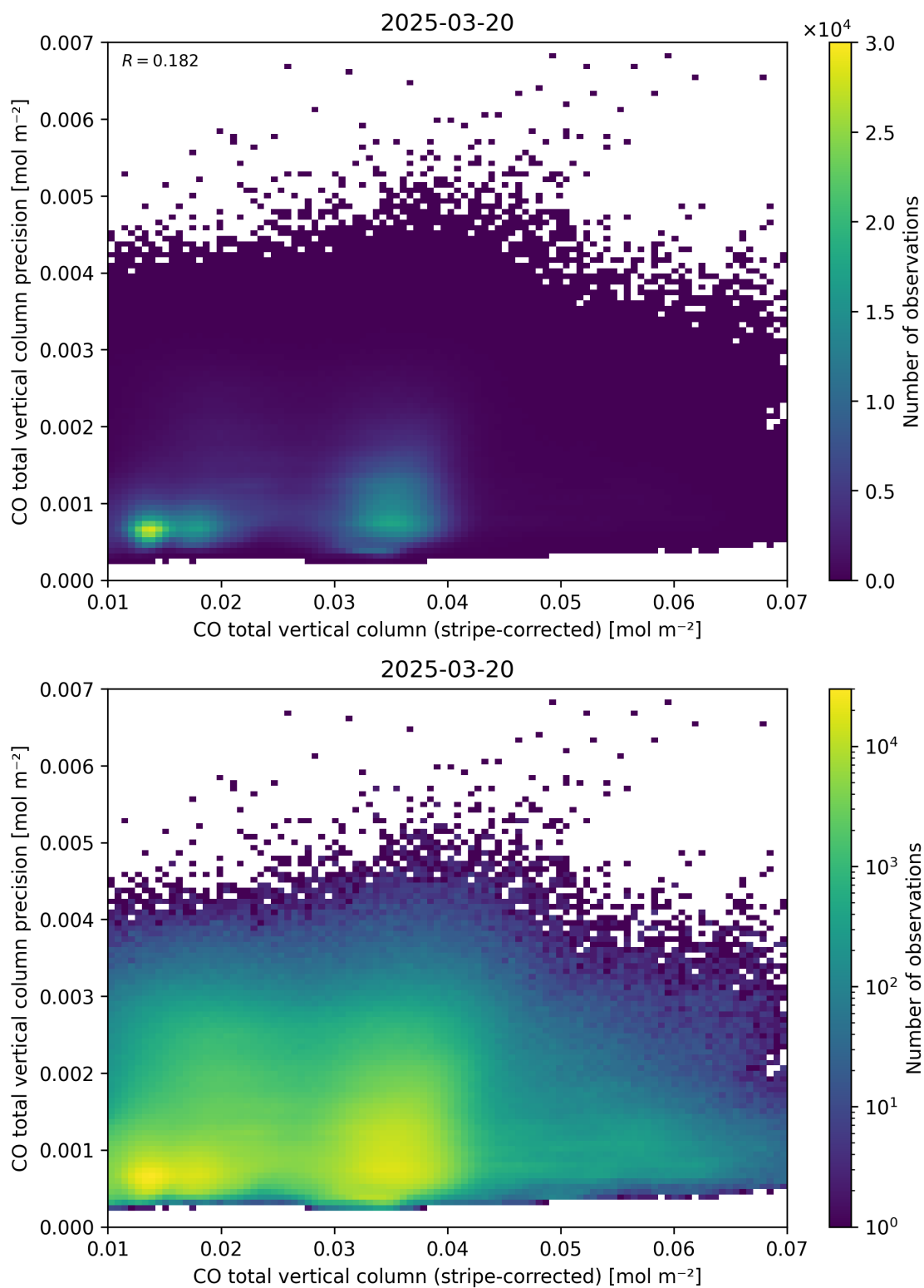
Figure 36: Scatter density plot of “CO total vertical column (stripe-corrected)” against “CO total vertical column precision” for 2025-03-19 to 2025-03-21.
