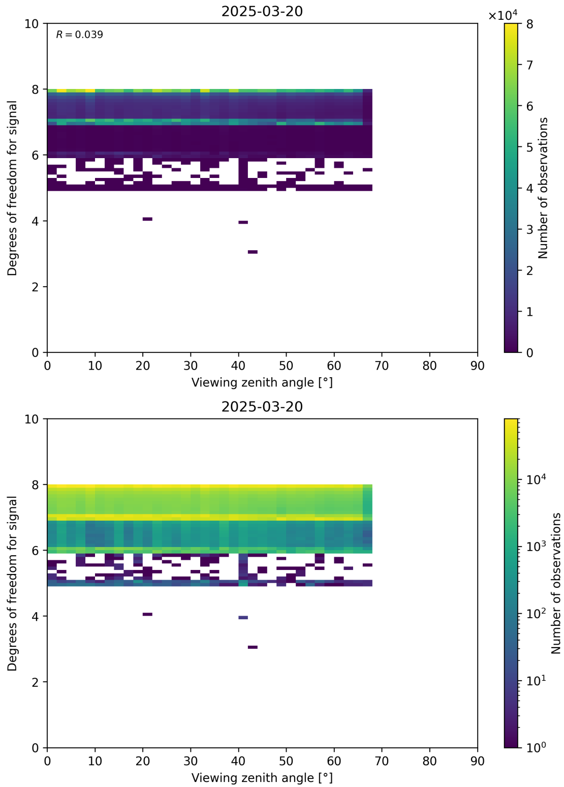
Figure 73: Scatter density plot of “Viewing zenith angle” against “Degrees of freedom for signal” for 2025-03-19 to 2025-03-21.
