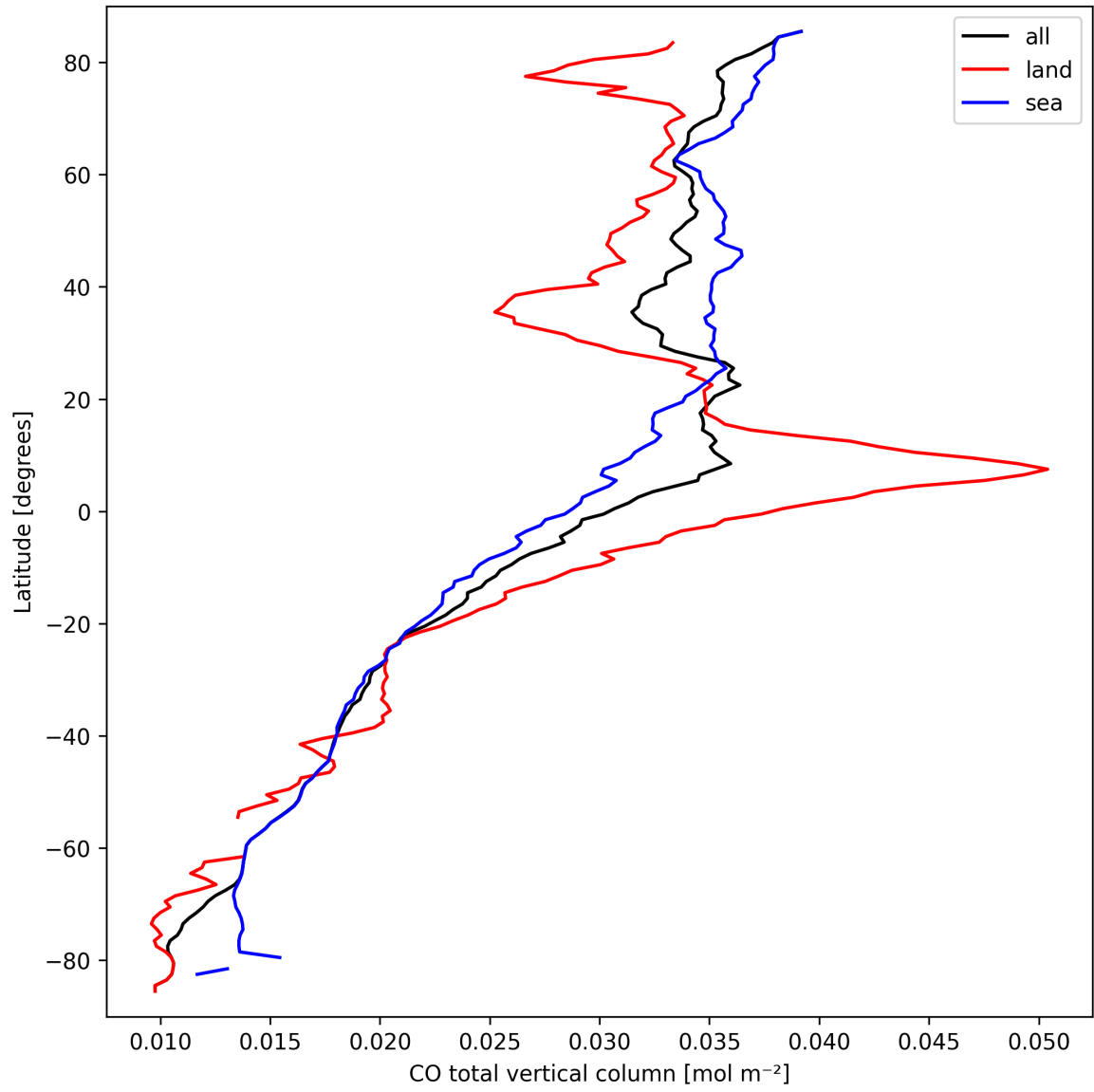
Figure 10: Zonal average of “CO total vertical column” for 2025-03-19 to 2025-03-21.
