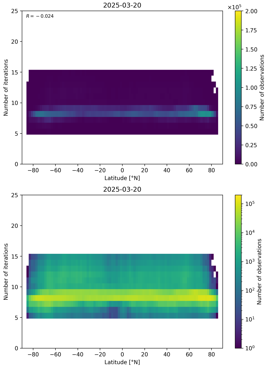
Figure 56: Scatter density plot of “Latitude” against “Number of iterations” for 2025-03-19 to 2025-03-21.
