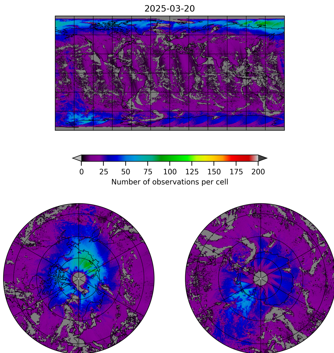
Figure 8: Map of the number of observations for 2025-03-19 to 2025-03-21
