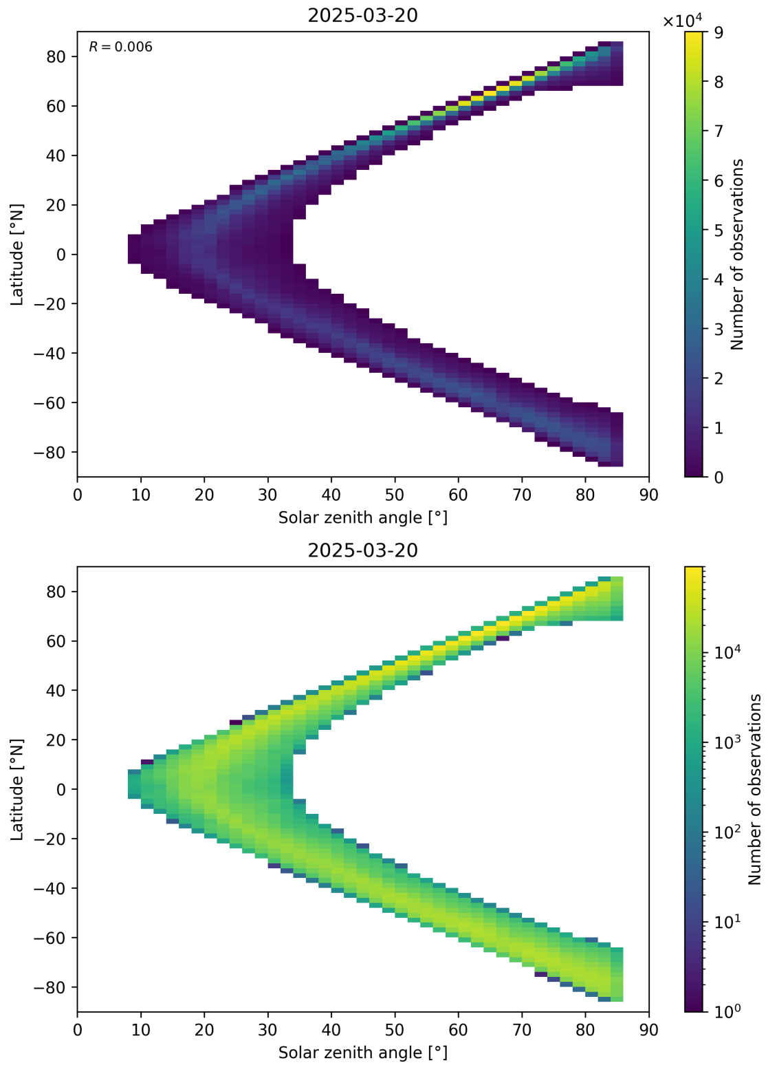
Figure 66: Scatter density plot of “Solar zenith angle” against “Latitude” for 2025-03-19 to 2025-03-21.
