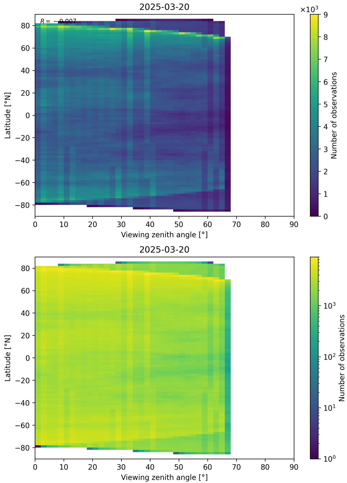
Figure 74: Scatter density plot of “Viewing zenith angle” against “Latitude” for 2025-03-19 to 2025-03-21.
