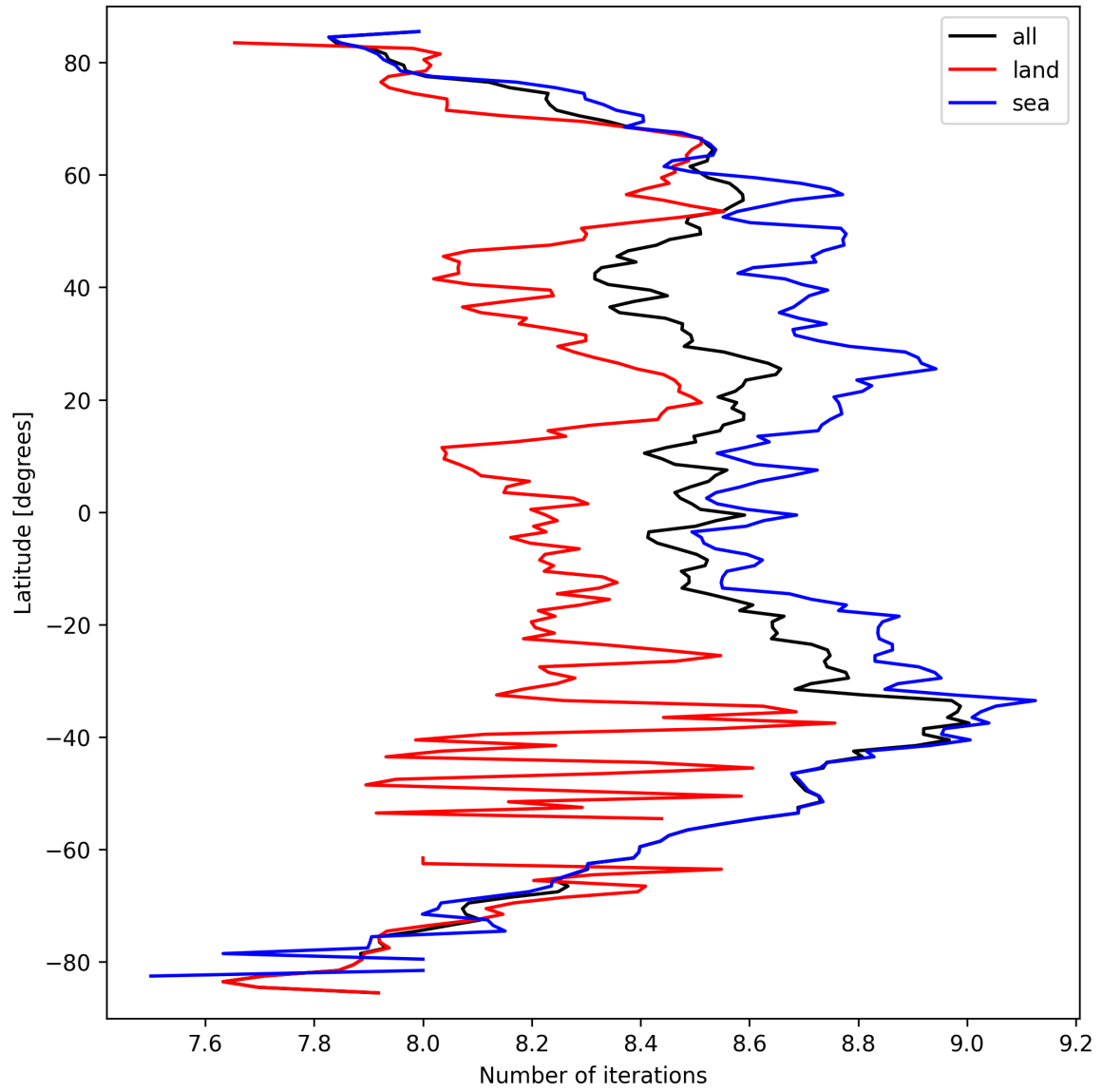
Figure 16: Zonal average of “Number of iterations” for 2025-03-19 to 2025-03-21.
