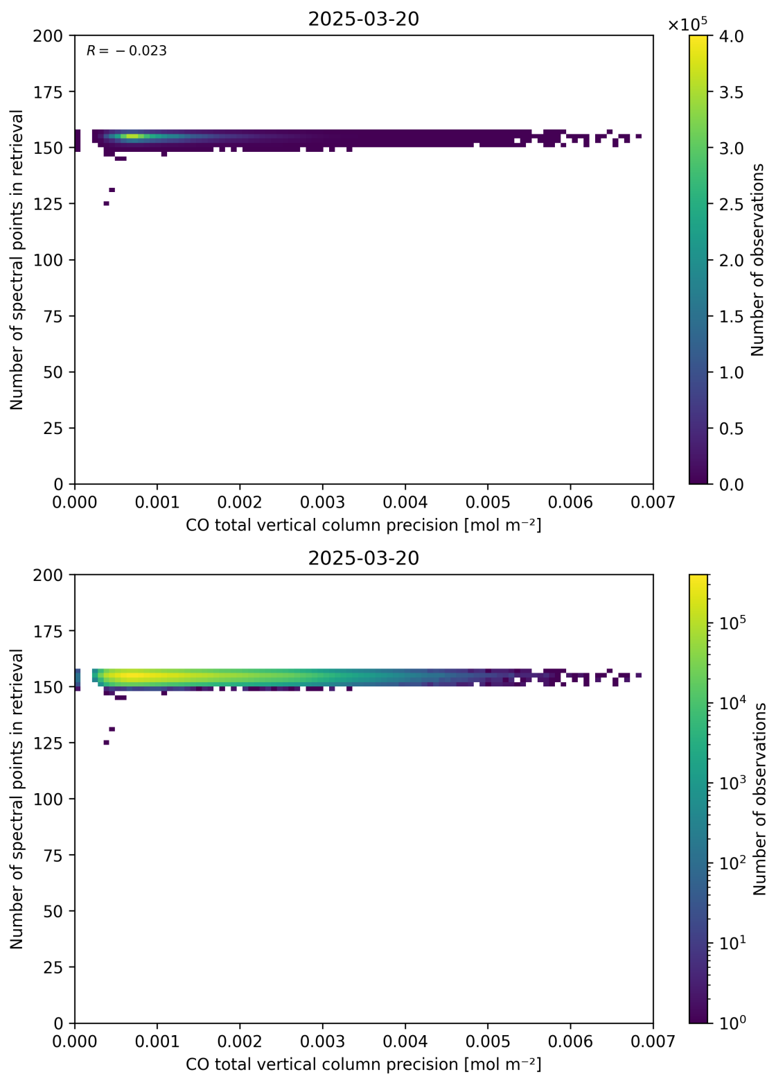
Figure 47: Scatter density plot of “CO total vertical column precision” against “Number of spectral points in retrieval” for 2025-03-19 to 2025-03-21.
