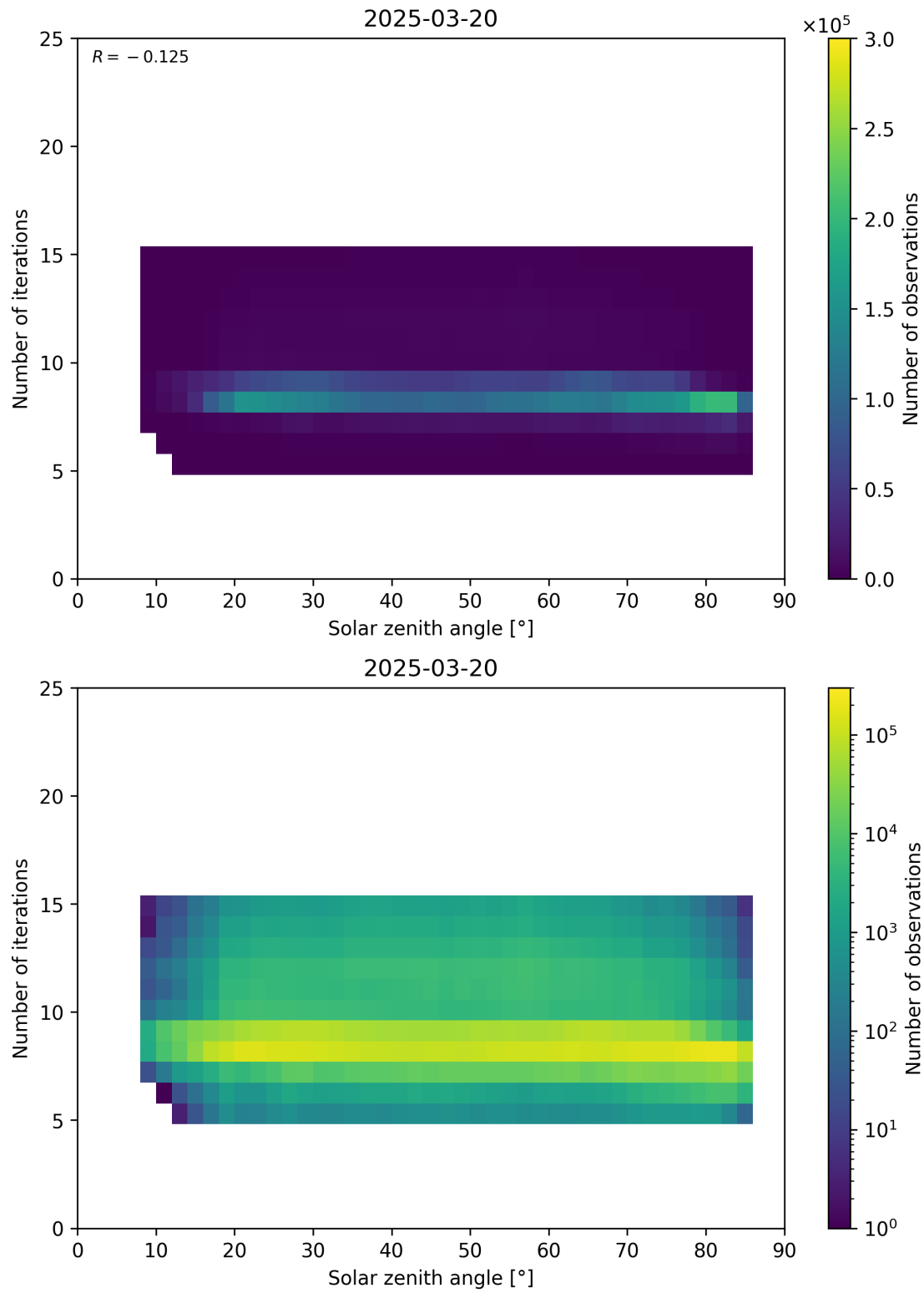
Figure 67: Scatter density plot of “Solar zenith angle” against “Number of iterations” for 2025-03-19 to 2025-03-21.
