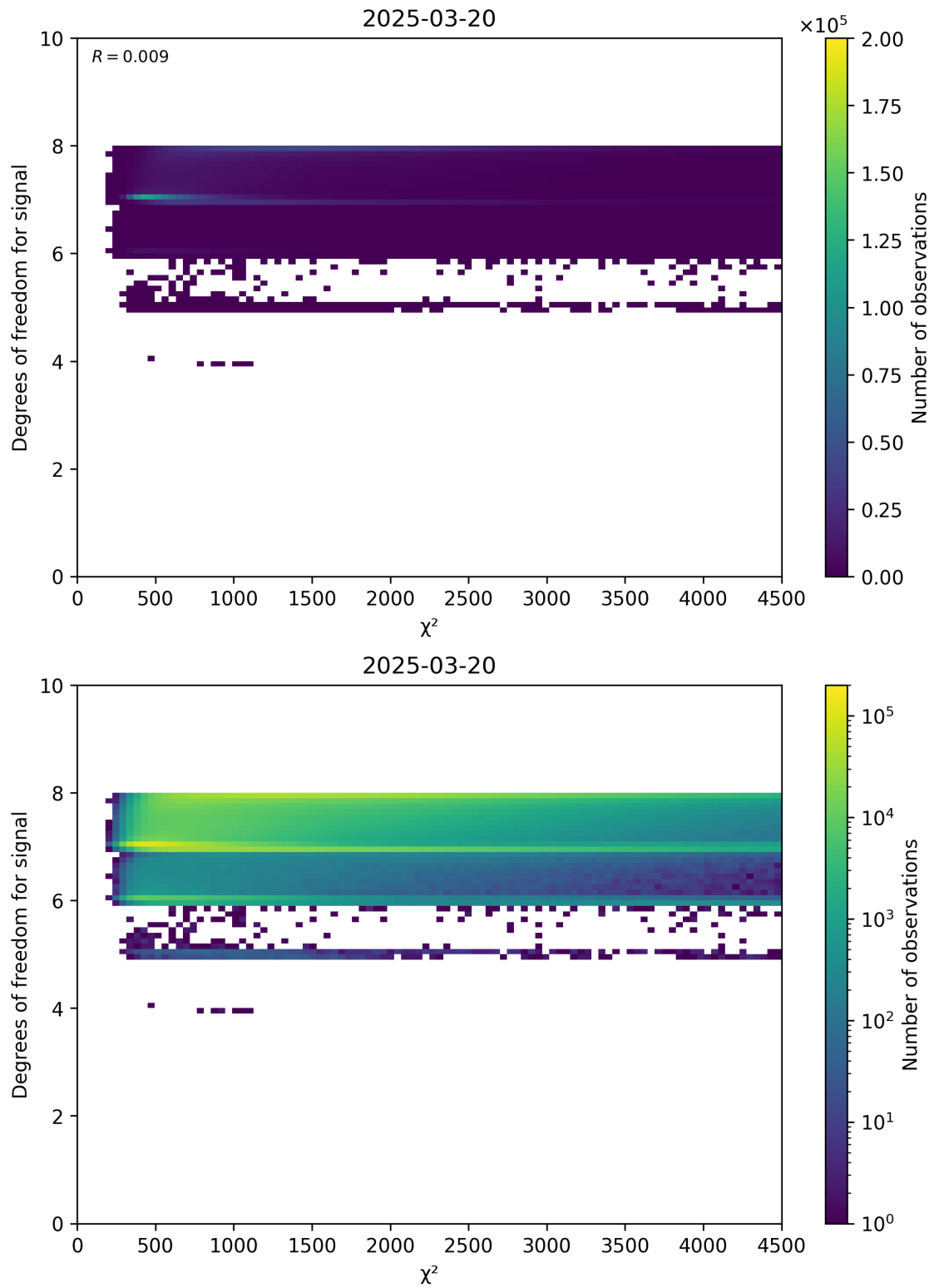
Figure 48: Scatter density plot of “ \chi^2 ” against “Degrees of freedom for signal” for 2025-03-19 to 2025-03-21.
