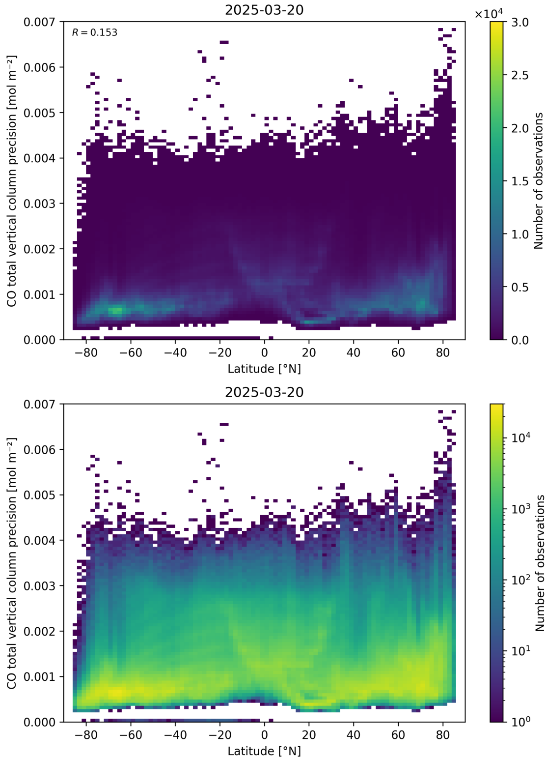
Figure 53: Scatter density plot of “Latitude” against “CO total vertical column precision” for 2025-03-19 to 2025-03-21.
