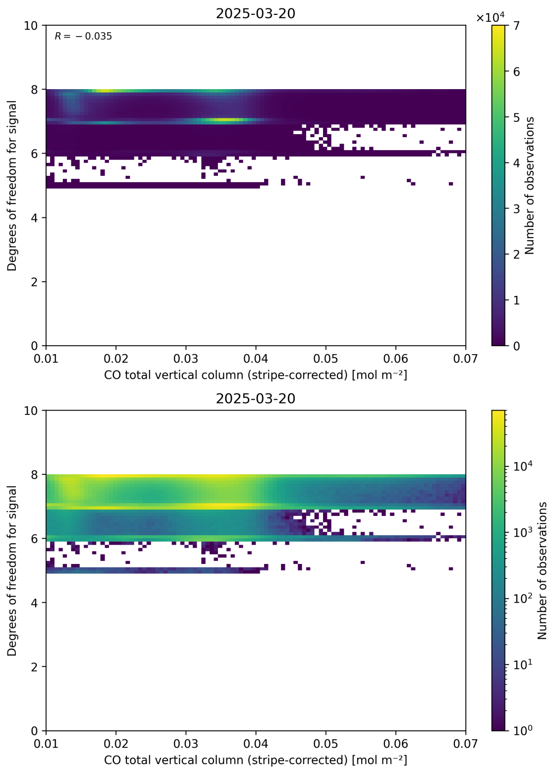
Figure 38: Scatter density plot of “CO total vertical column (stripe-corrected)” against “Degrees of freedom for signal” for 2025-03-19 to 2025-03-21.
