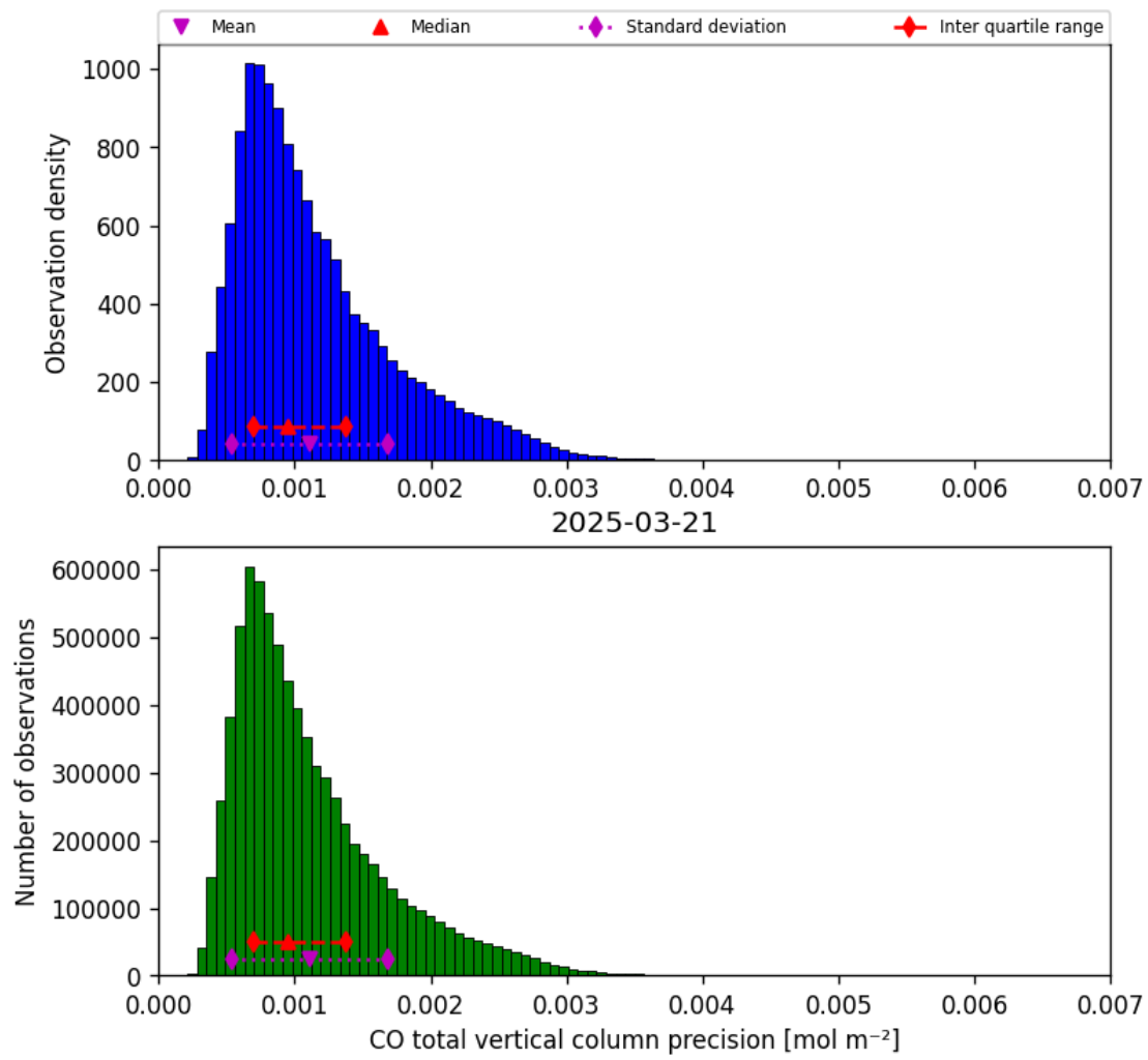
Figure 20: Histogram of “CO total vertical column precision” for 2025-03-20 to 2025-03-22
