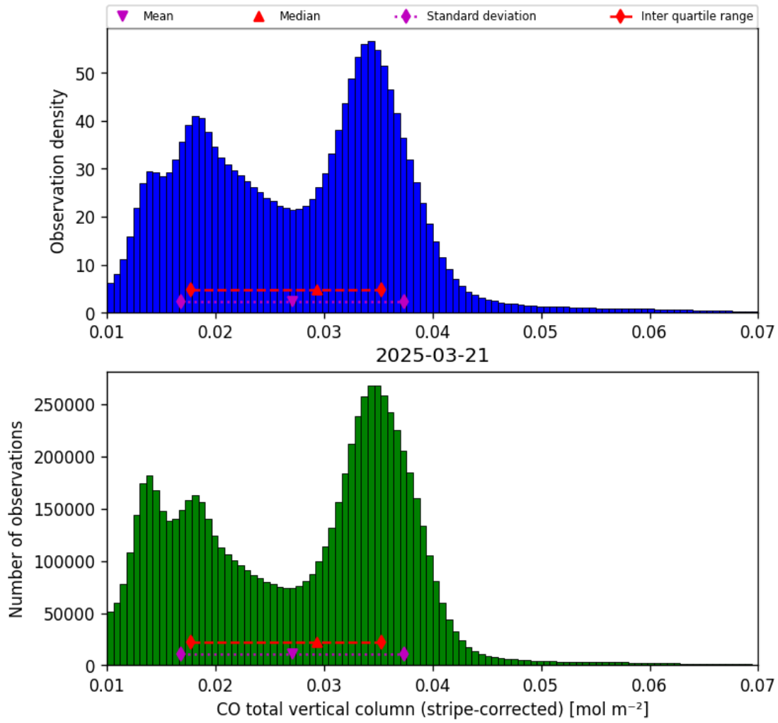
Figure 19: Histogram of “CO total vertical column (stripe-corrected)” for 2025-03-20 to 2025-03-22
