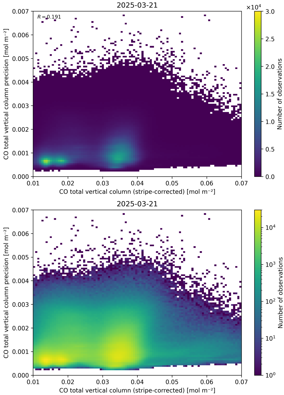
Figure 36: Scatter density plot of “CO total vertical column (stripe-corrected)” against “CO total vertical column precision” for 2025-03-20 to 2025-03-22.
