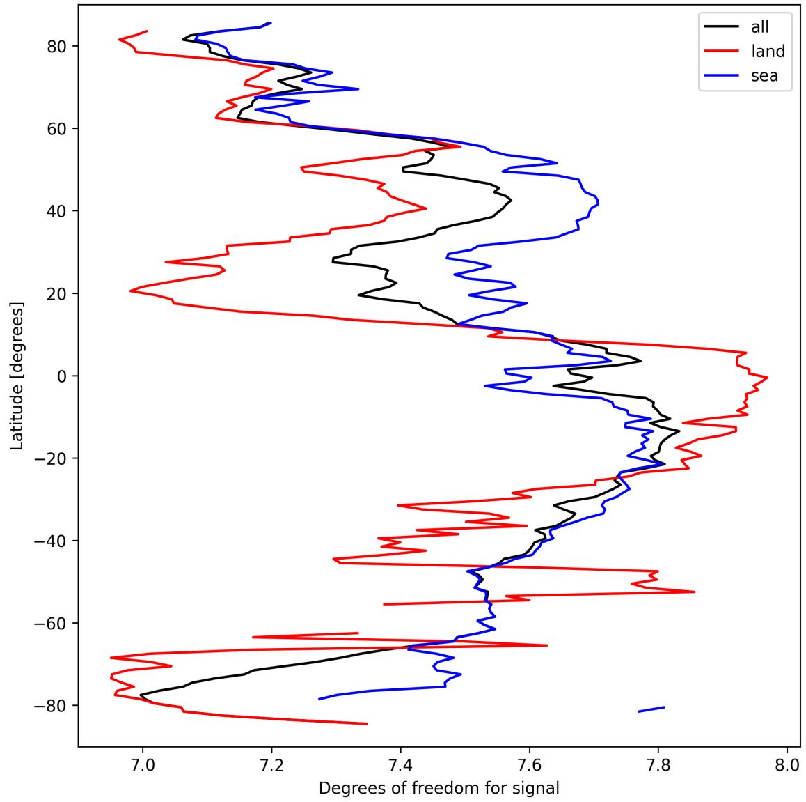
Figure 15: Zonal average of “Degrees of freedom for signal” for 2025-03-20 to 2025-03-22.
