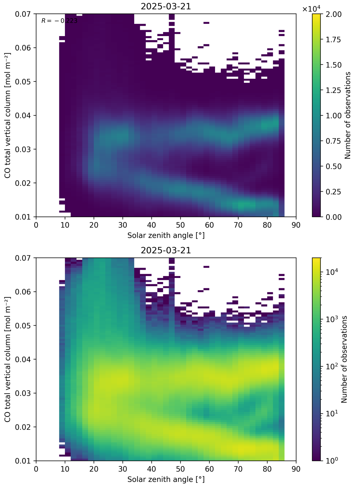
Figure 61: Scatter density plot of “Solar zenith angle” against “CO total vertical column” for 2025-03-20 to 2025-03-22.
