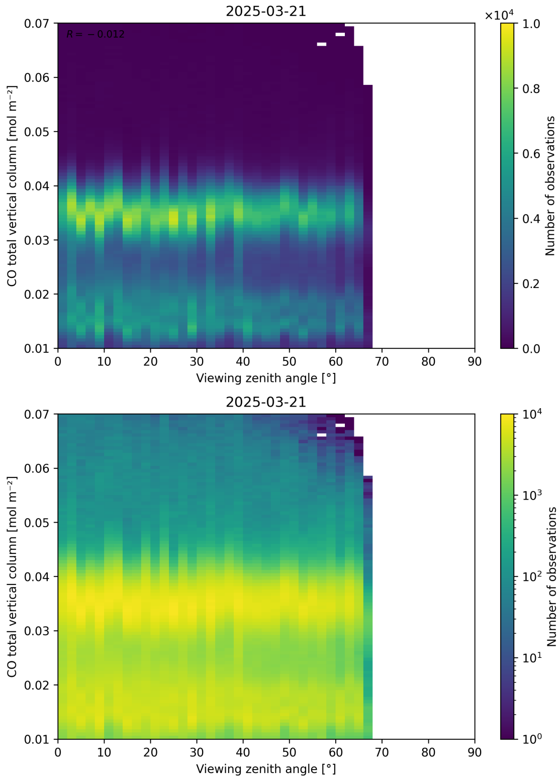
Figure 69: Scatter density plot of “Viewing zenith angle” against “CO total vertical column” for 2025-03-20 to 2025-03-22.
