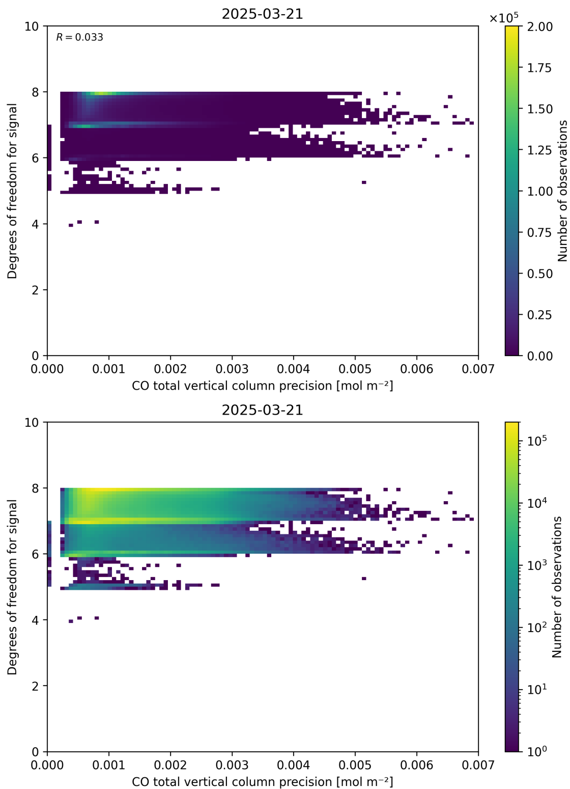
Figure 45: Scatter density plot of “CO total vertical column precision” against “Degrees of freedom for signal” for 2025-03-20 to 2025-03-22.
