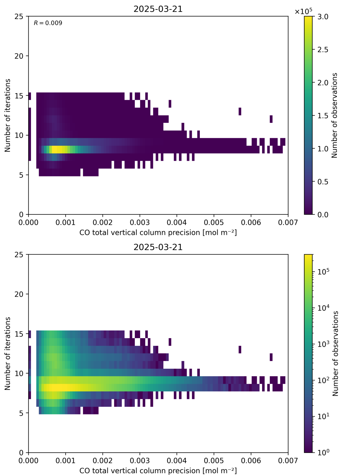
Figure 46: Scatter density plot of “CO total vertical column precision” against “Number of iterations” for 2025-03-20 to 2025-03-22.
