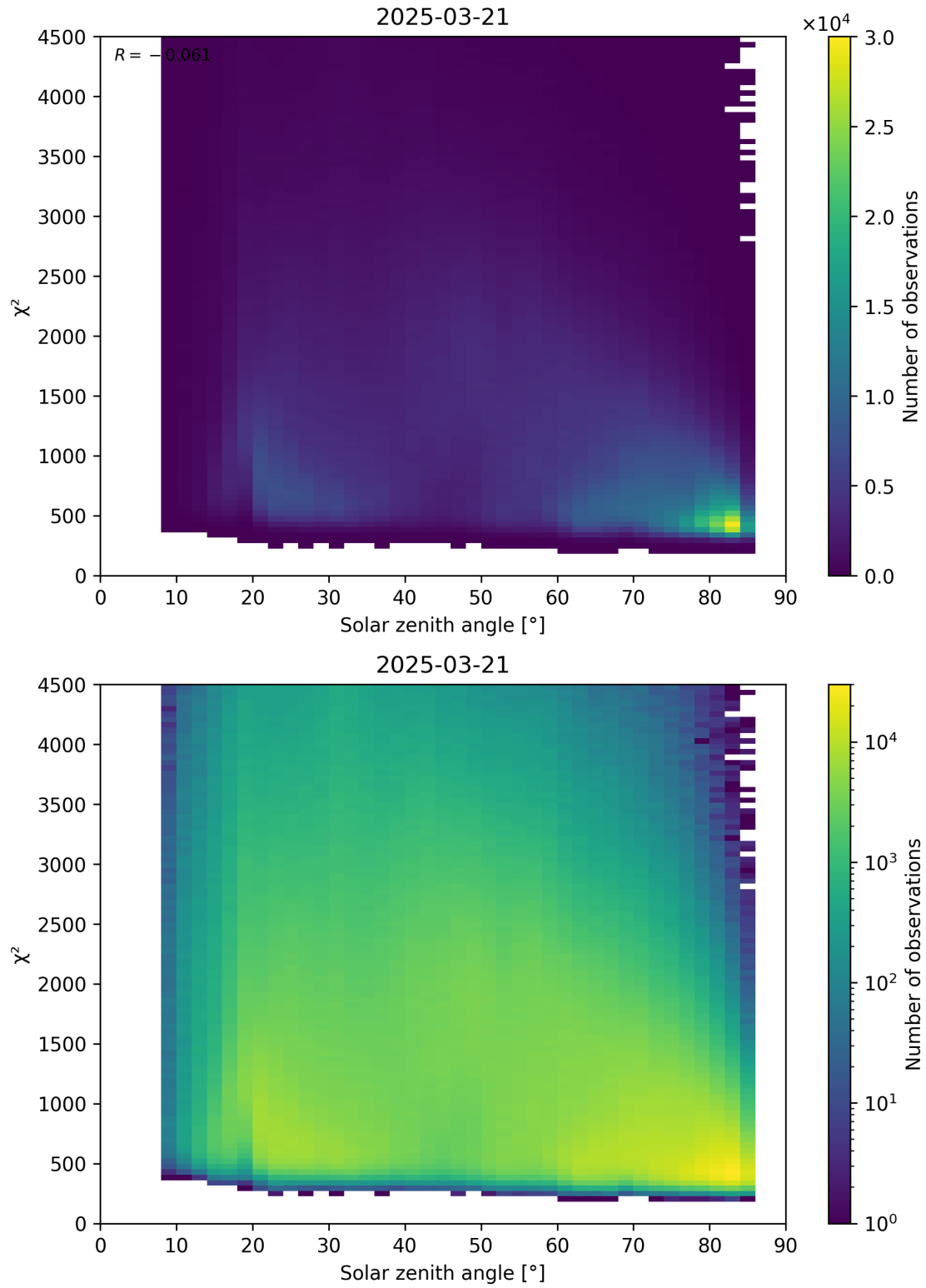
Figure 64: Scatter density plot of “Solar zenith angle” against “ \chi^2 ” for 2025-03-20 to 2025-03-22.
