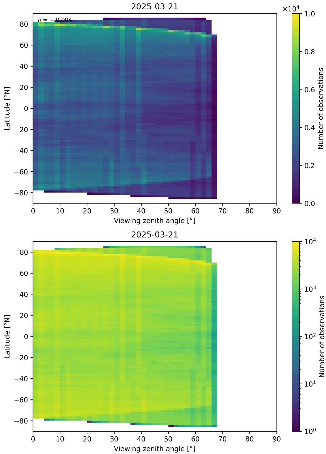
Figure 74: Scatter density plot of “Viewing zenith angle” against “Latitude” for 2025-03-20 to 2025-03-22.
