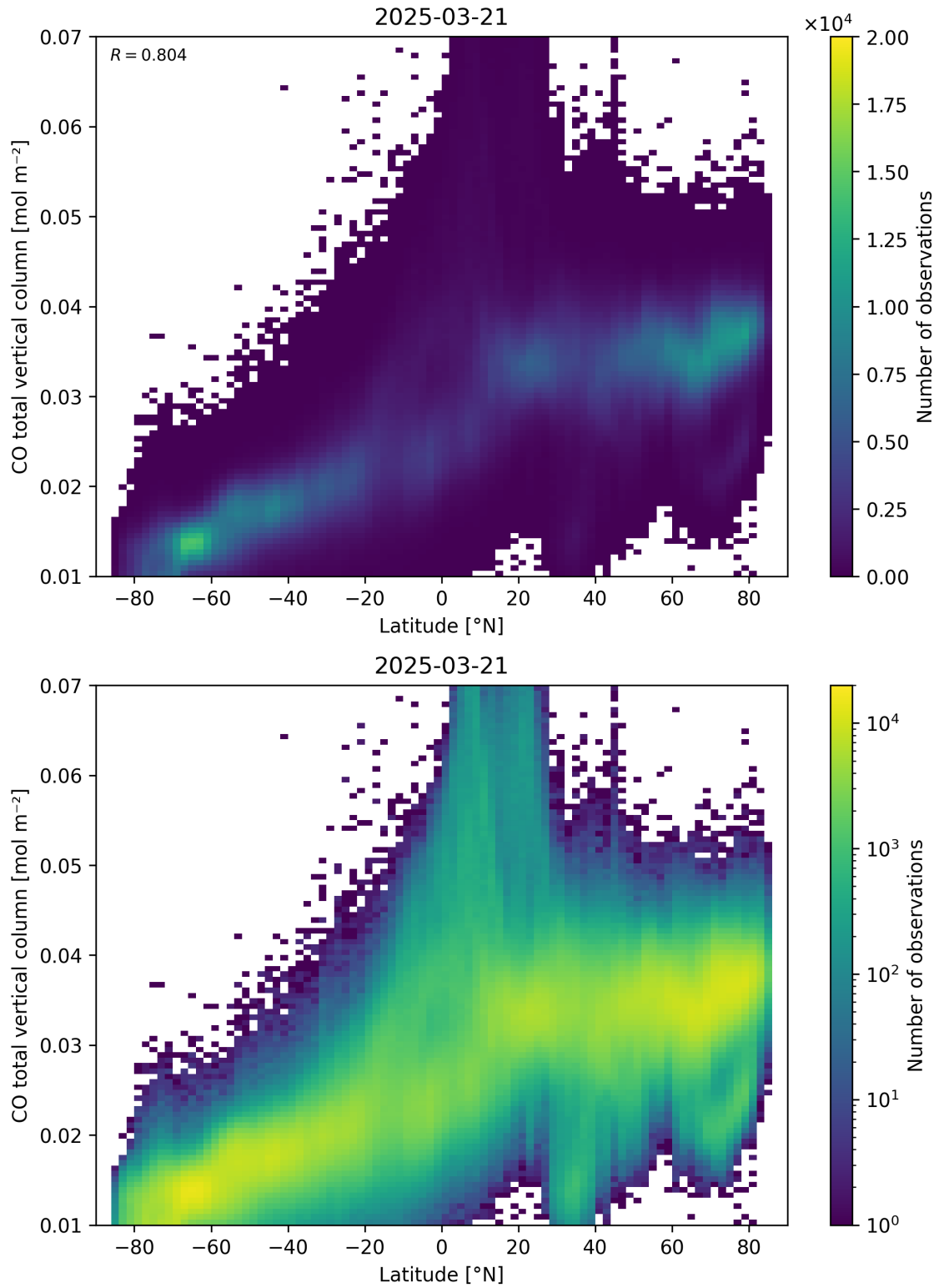
Figure 51: Scatter density plot of “Latitude” against “CO total vertical column” for 2025-03-20 to 2025-03-22.
