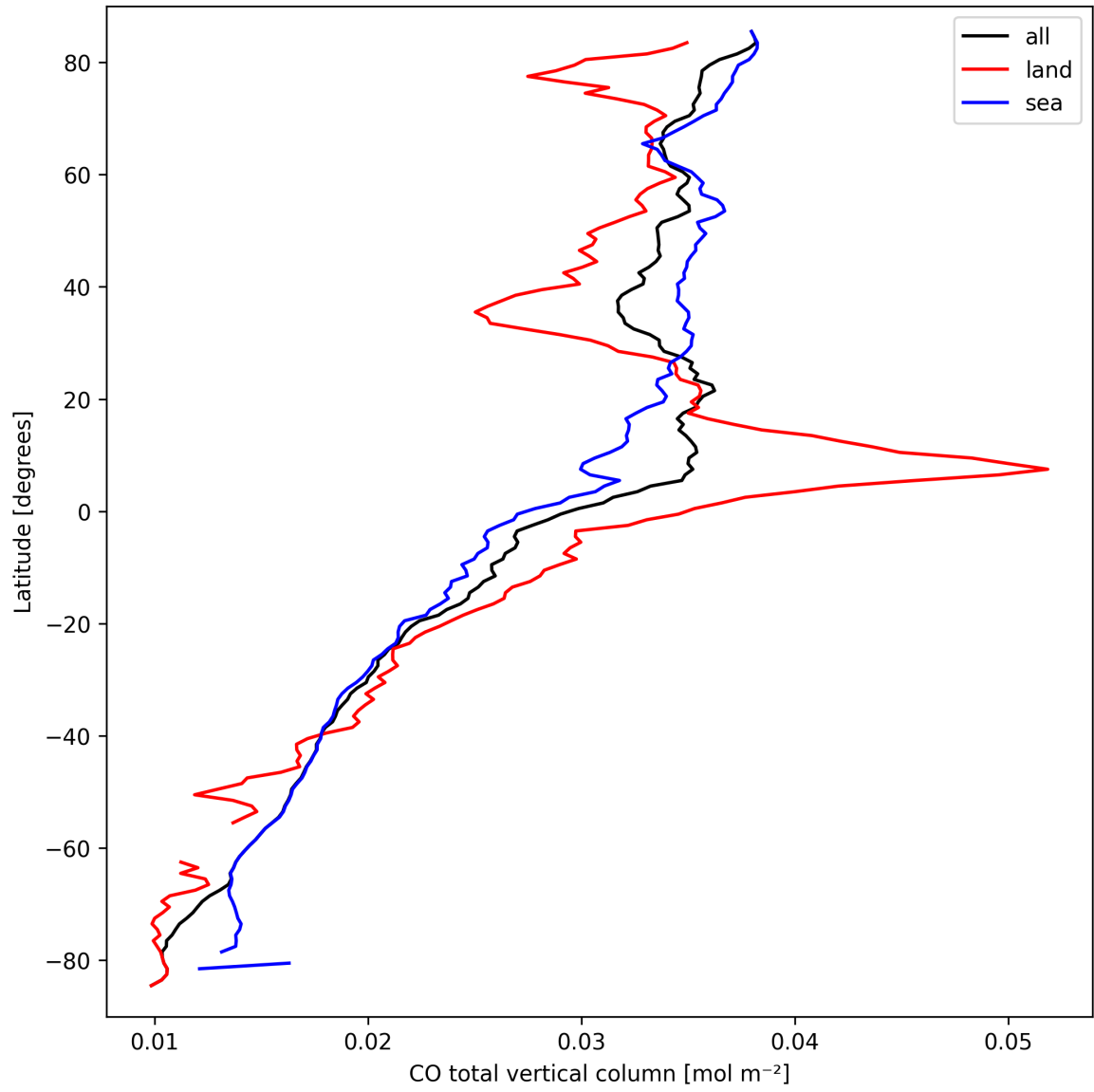
Figure 10: Zonal average of “CO total vertical column” for 2025-03-20 to 2025-03-22.
