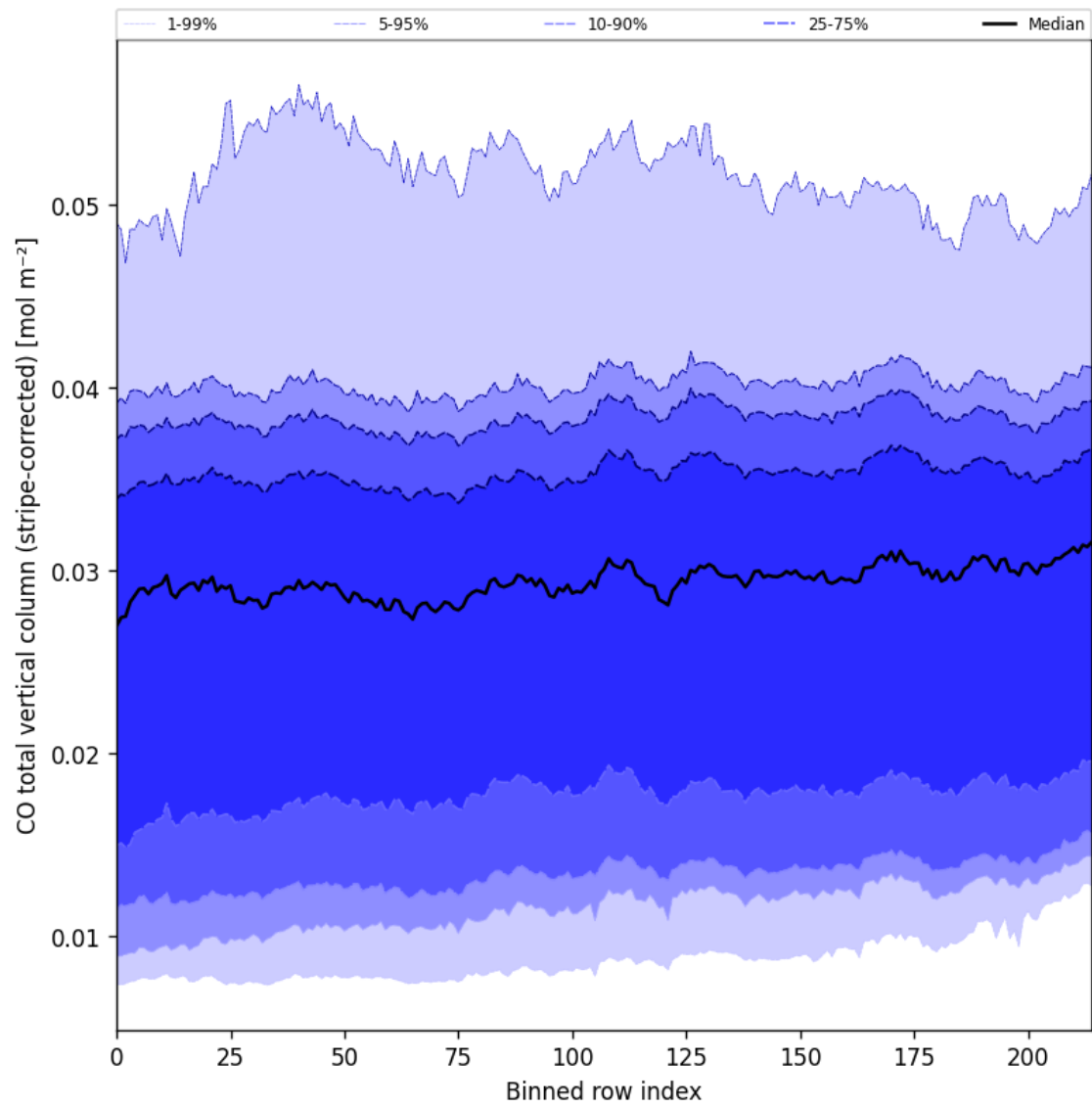
Figure 27: Along track statistics of “CO total vertical column (stripe-corrected)” for 2025-03-20 to 2025-03-22
