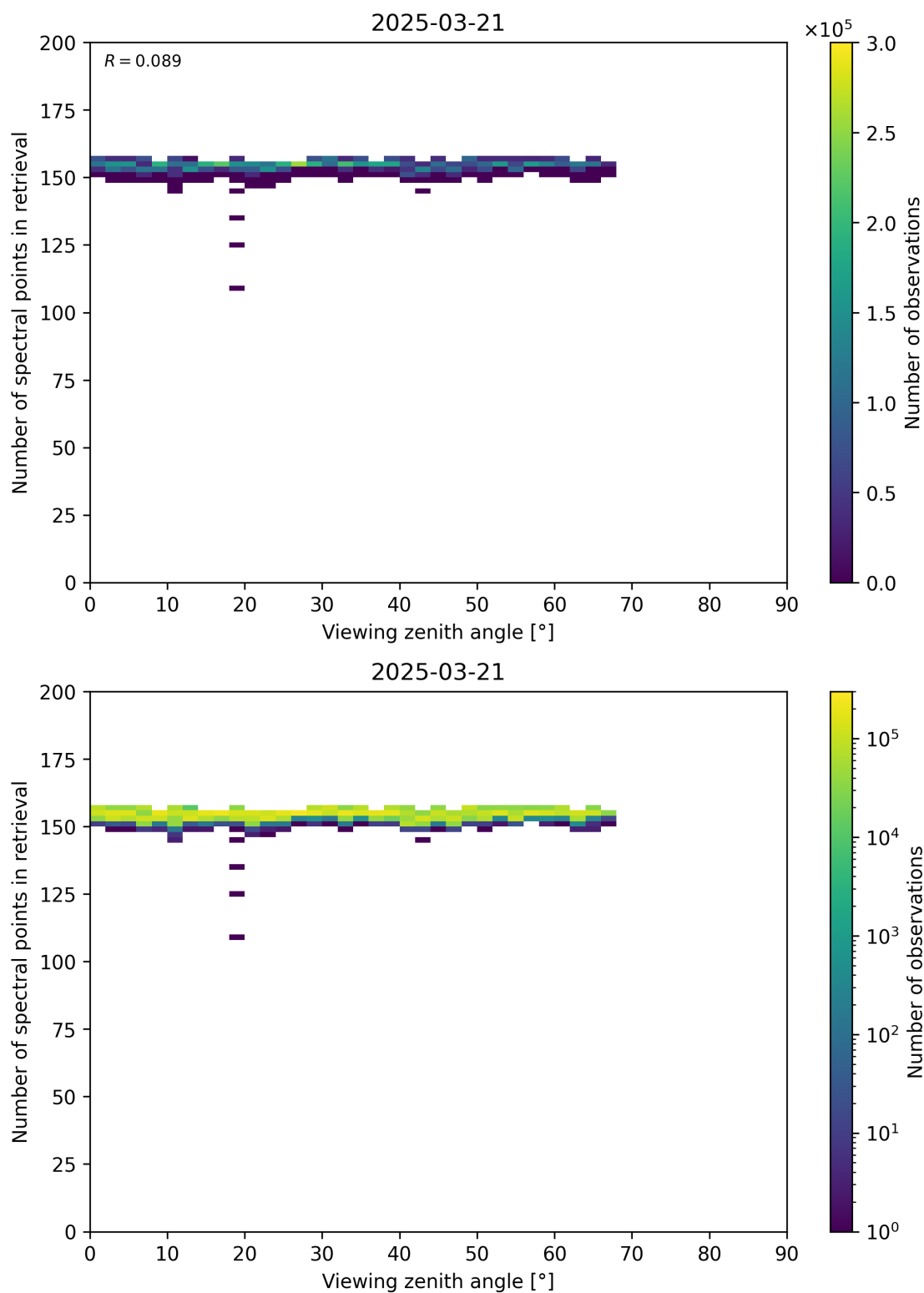
Figure 76: Scatter density plot of “Viewing zenith angle” against “Number of spectral points in retrieval” for 2025-03-20 to 2025-03-22.
