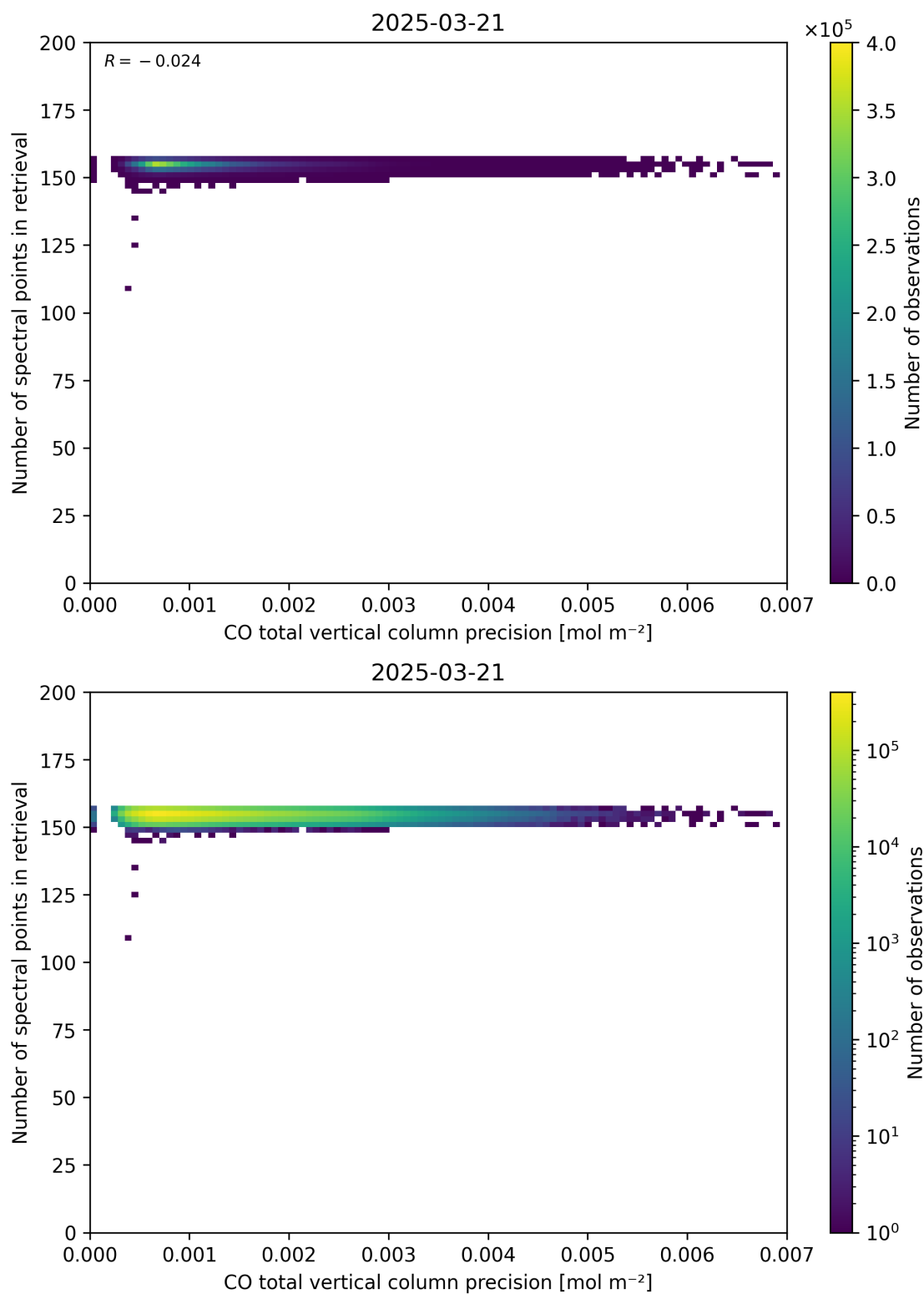
Figure 47: Scatter density plot of “CO total vertical column precision” against “Number of spectral points in retrieval” for 2025-03-20 to 2025-03-22.
