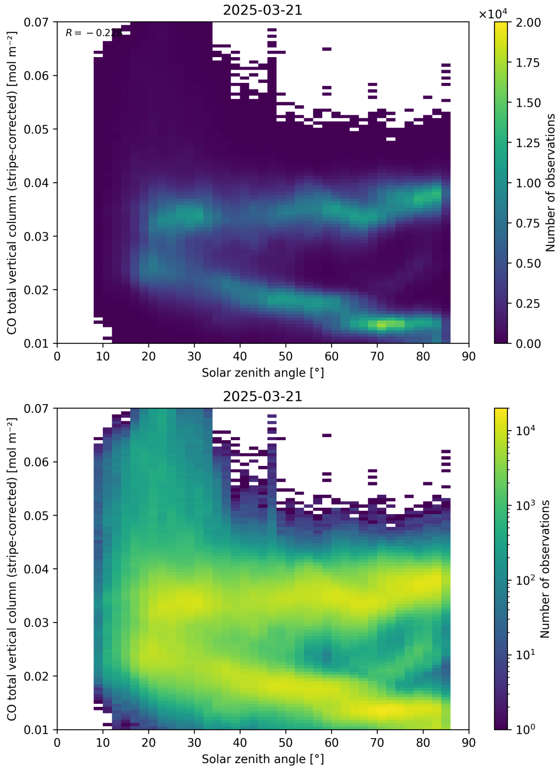
Figure 62: Scatter density plot of “Solar zenith angle” against “CO total vertical column (stripe-corrected)” for 2025-03-20 to 2025-03-22.
