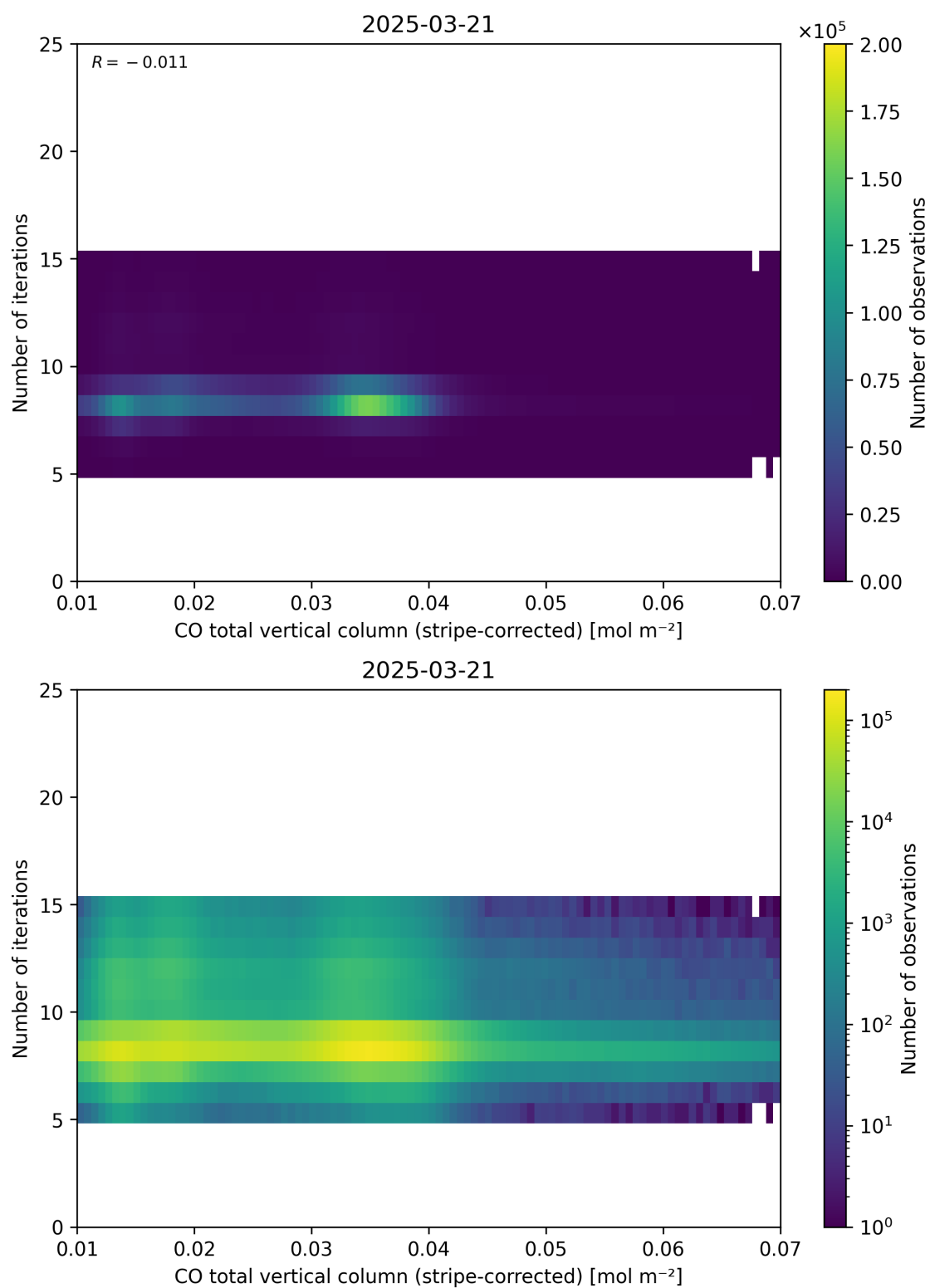
Figure 39: Scatter density plot of “CO total vertical column (stripe-corrected)” against “Number of iterations” for 2025-03-20 to 2025-03-22.
