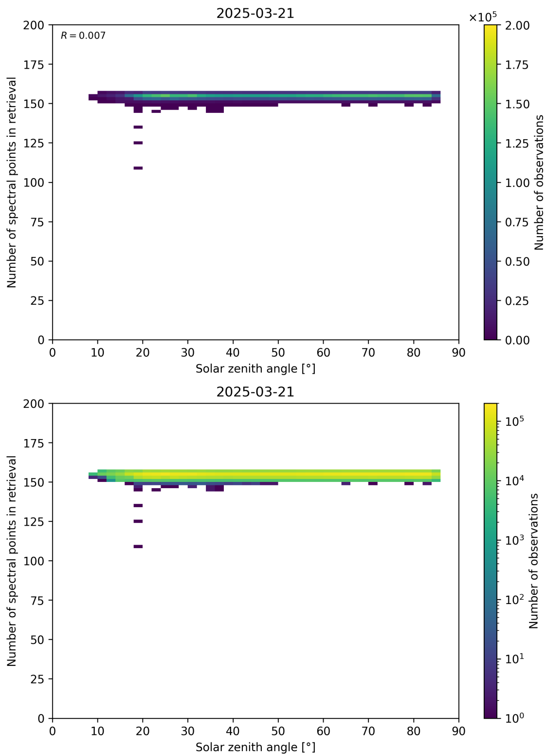
Figure 68: Scatter density plot of “Solar zenith angle” against “Number of spectral points in retrieval” for 2025-03-20 to 2025-03-22.
