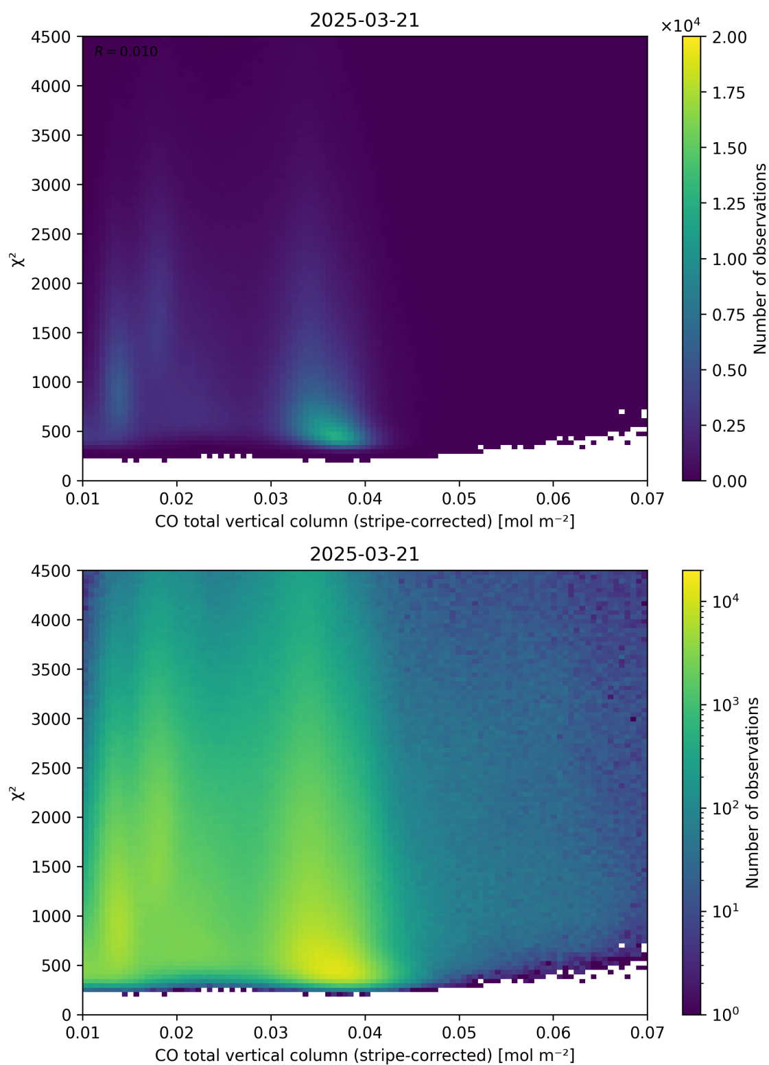
Figure 37: Scatter density plot of “CO total vertical column (stripe-corrected)” against “ \chi^2 ” for 2025-03-20 to 2025-03-22.
