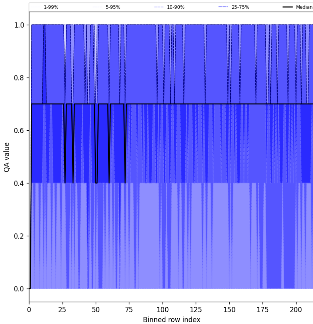
Figure 25: Along track statistics of “QA value” for 2025-03-20 to 2025-03-22
