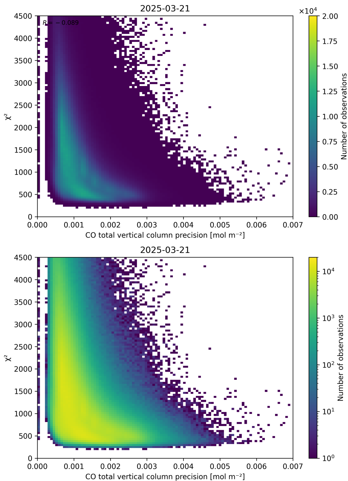
Figure 44: Scatter density plot of “CO total vertical column precision” against “ \chi^2 ” for 2025-03-20 to 2025-03-22.
