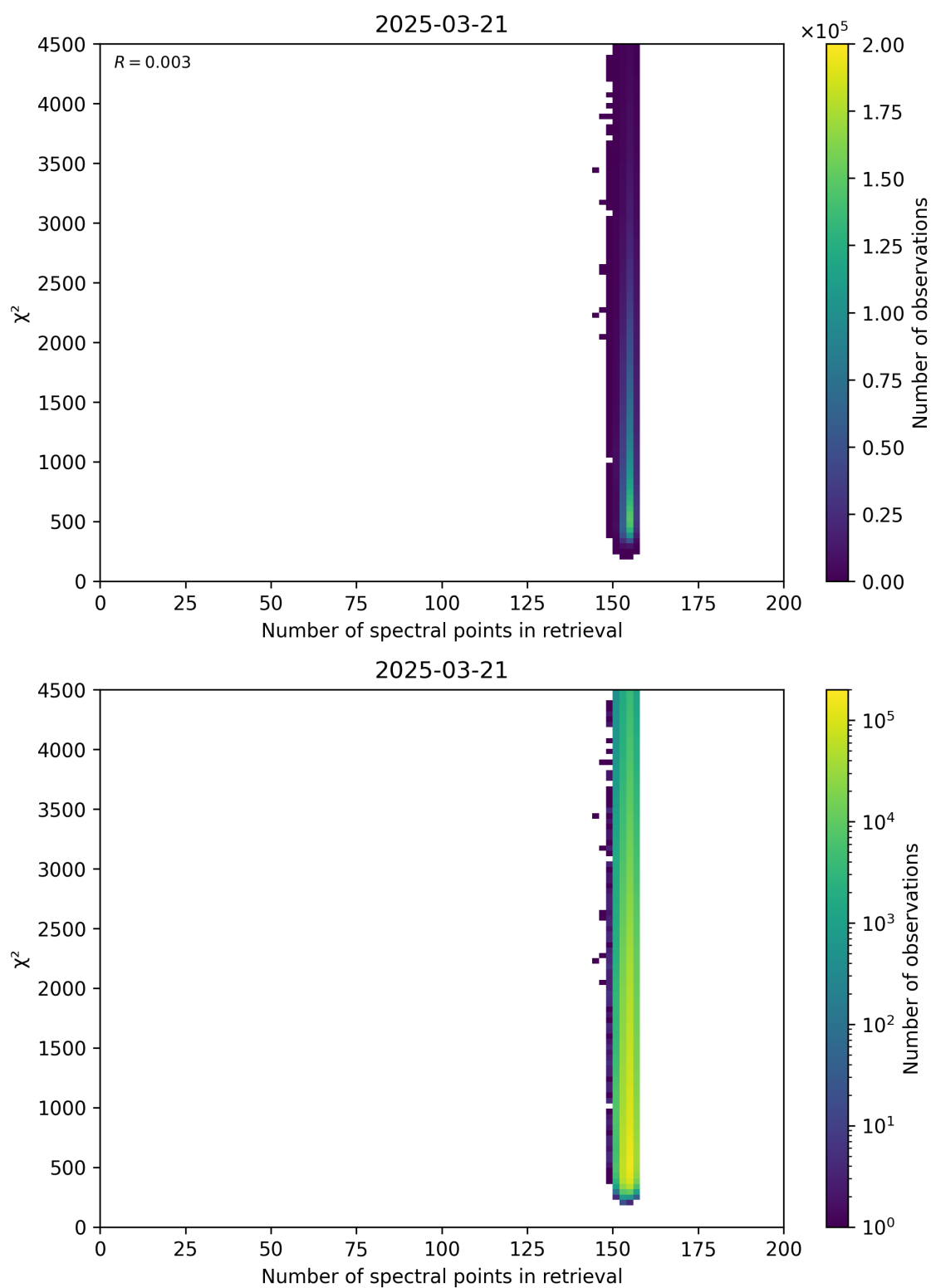
Figure 58: Scatter density plot of “Number of spectral points in retrieval” against “ \chi^2 ” for 2025-03-20 to 2025-03-22.
