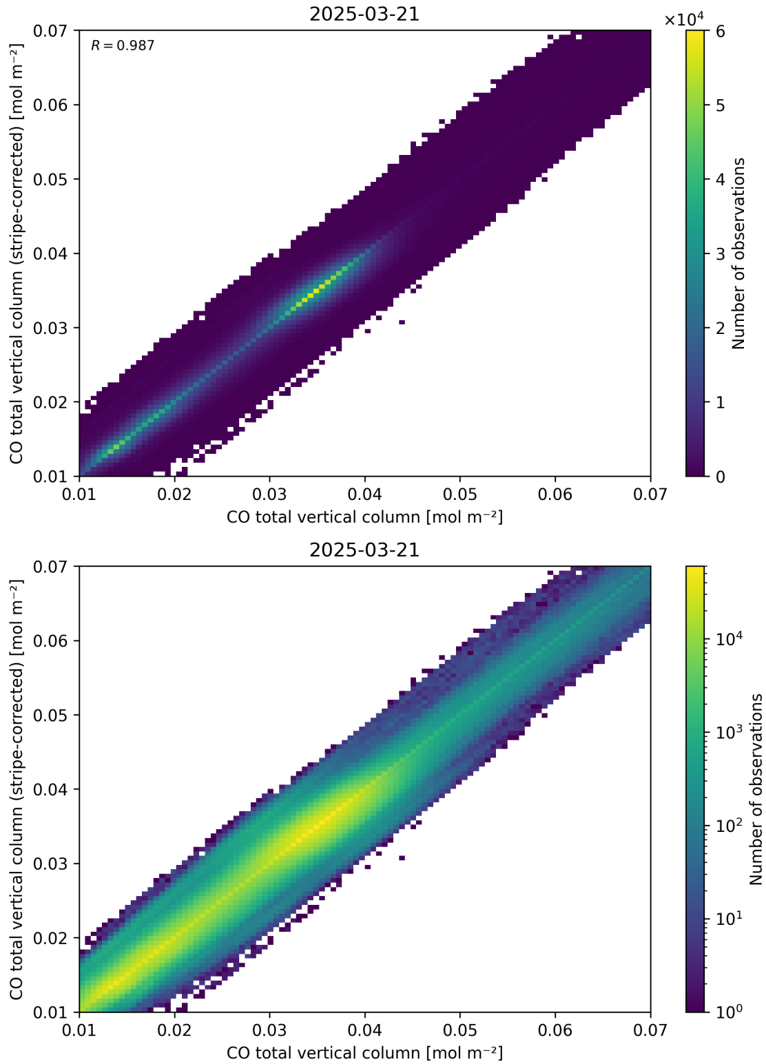
Figure 33: Scatter density plot of “CO total vertical column” against “CO total vertical column (stripe-corrected)” for 2025-03-20 to 2025-03-22.
