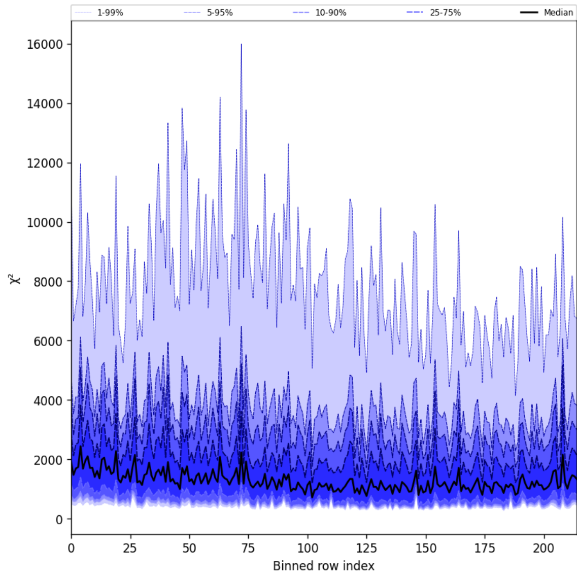
Figure 30: Along track statistics of “ \chi^2 ” for 2025-03-20 to 2025-03-22
