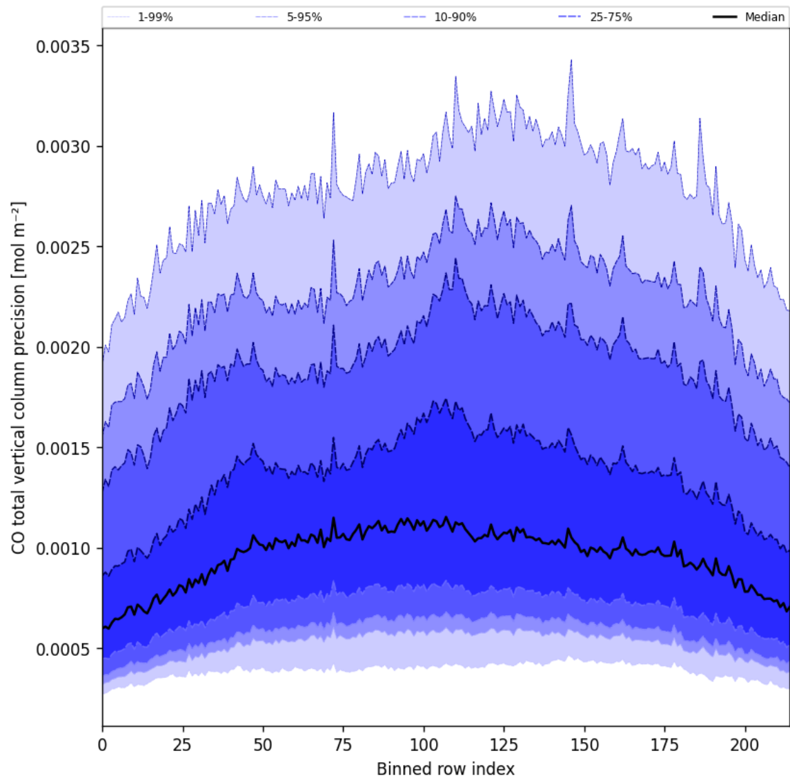
Figure 28: Along track statistics of “CO total vertical column precision” for 2025-03-20 to 2025-03-22
