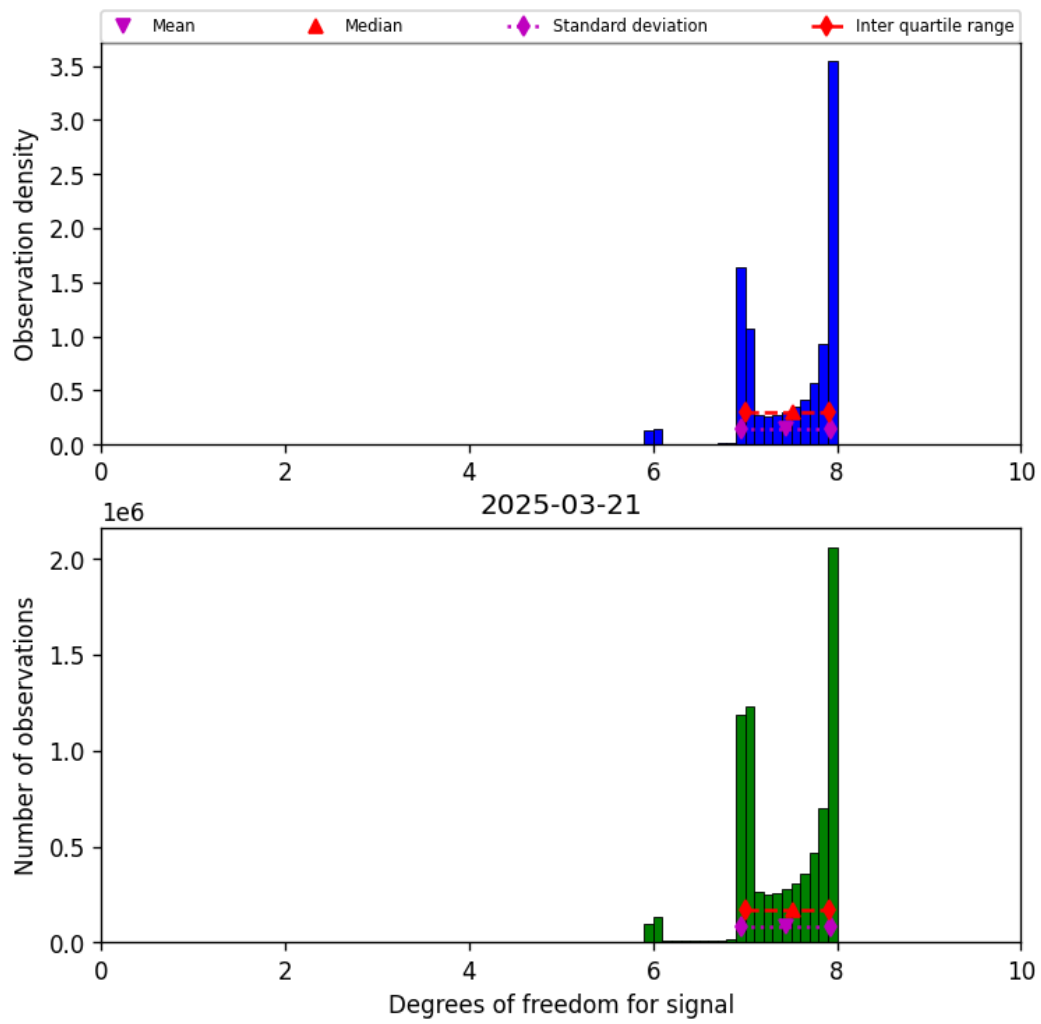
Figure 23: Histogram of “Degrees of freedom for signal” for 2025-03-20 to 2025-03-22
