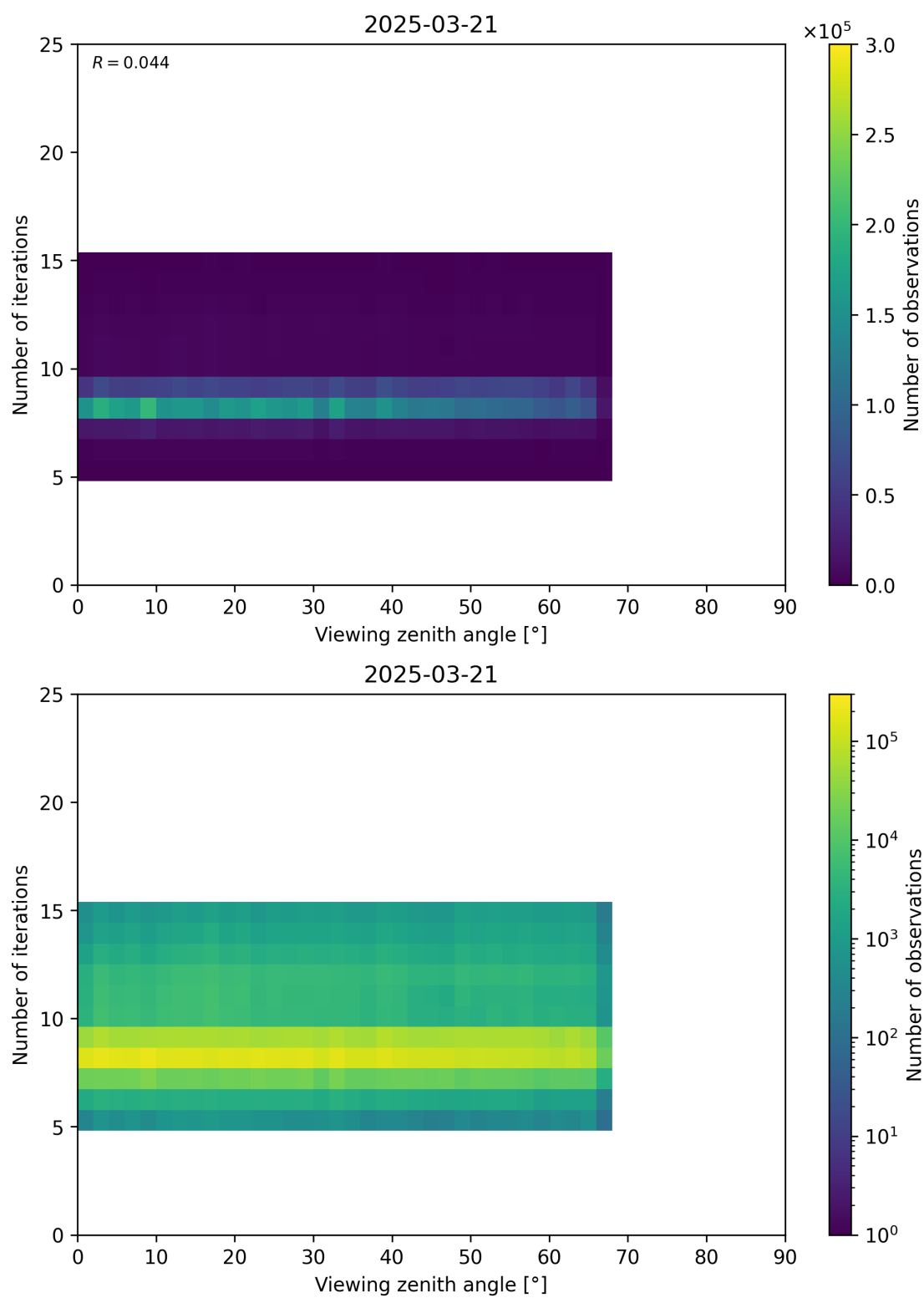
Figure 75: Scatter density plot of “Viewing zenith angle” against “Number of iterations” for 2025-03-20 to 2025-03-22.
