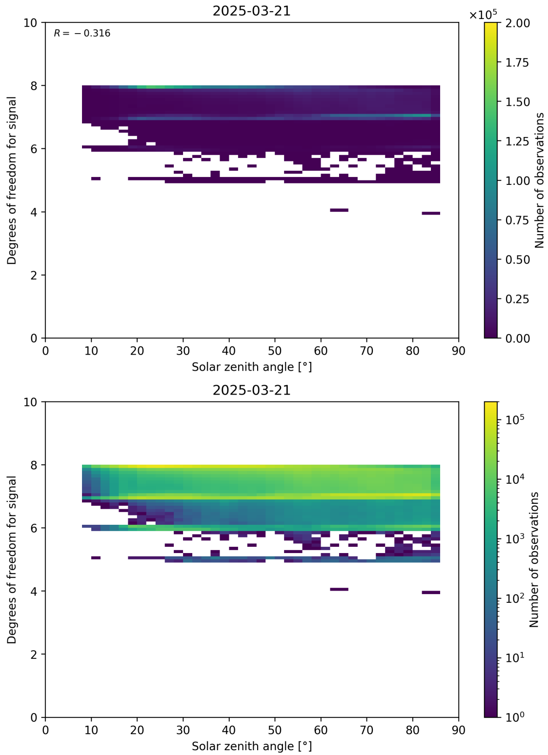
Figure 65: Scatter density plot of “Solar zenith angle” against “Degrees of freedom for signal” for 2025-03-20 to 2025-03-22.
