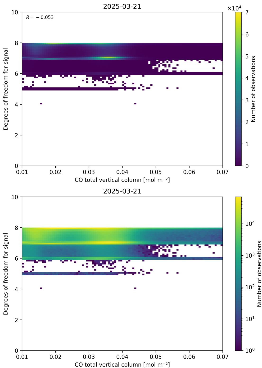
Figure 41: Scatter density plot of “CO total vertical column” against “Degrees of freedom for signal” for 2025-03-20 to 2025-03-22.
