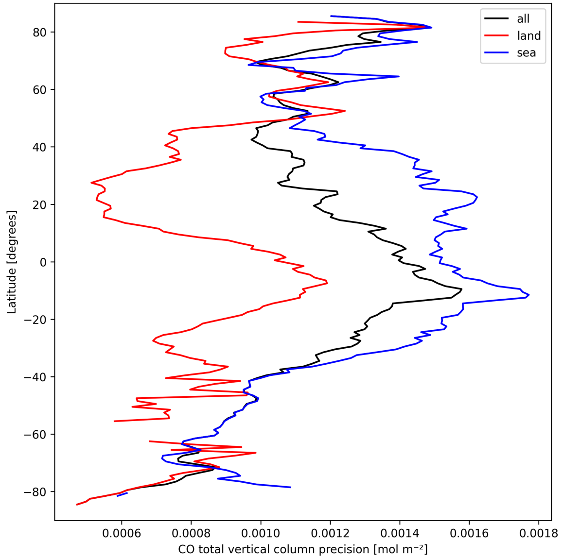
Figure 12: Zonal average of “CO total vertical column precision” for 2025-03-20 to 2025-03-22.
