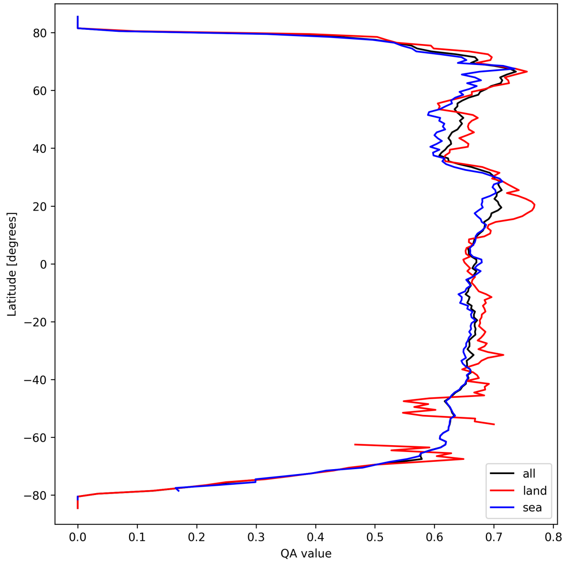
Figure 9: Zonal average of “QA value” for 2025-03-20 to 2025-03-22.
