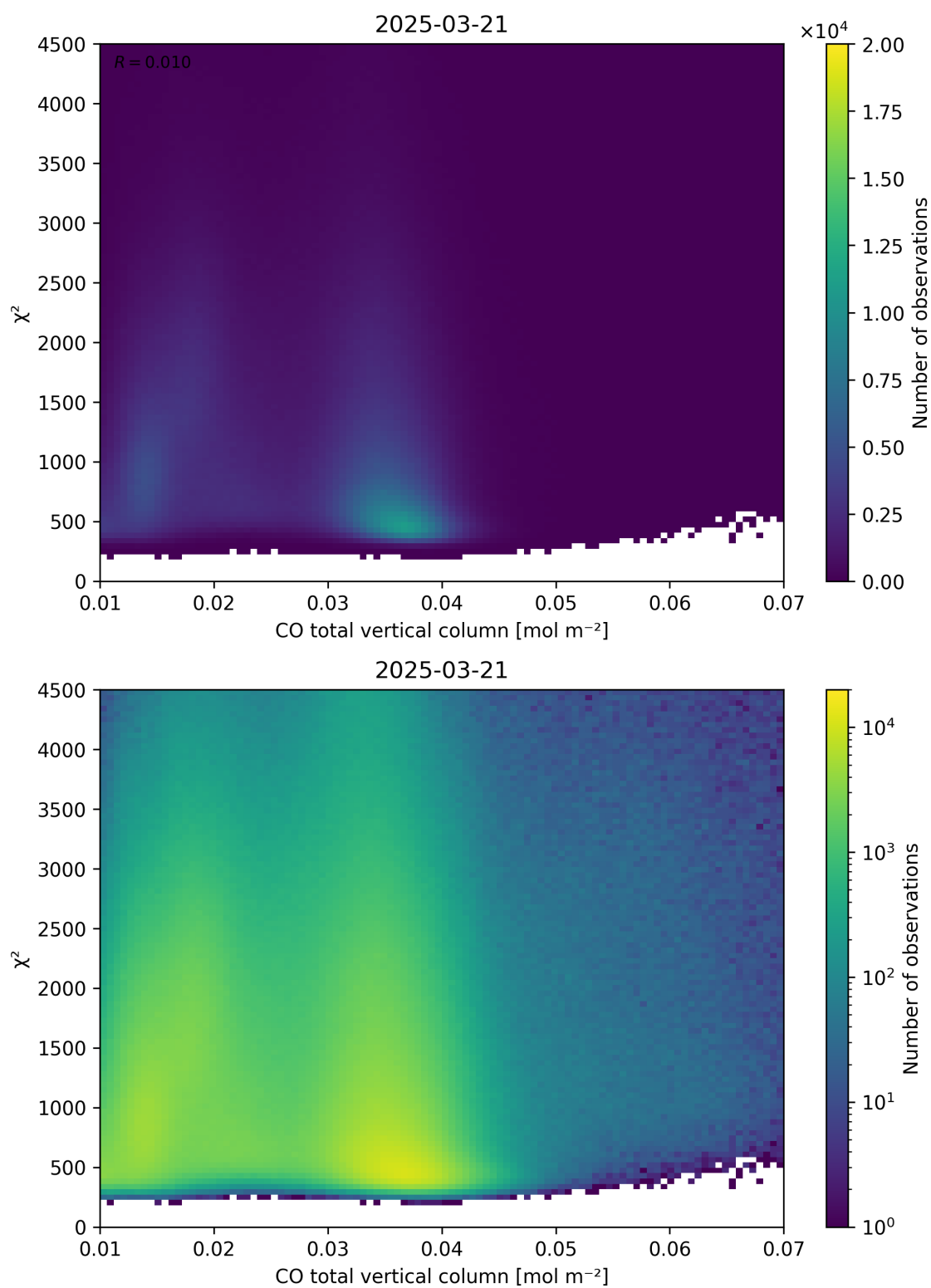
Figure 35: Scatter density plot of “CO total vertical column” against “ \chi^2 ” for 2025-03-20 to 2025-03-22.
