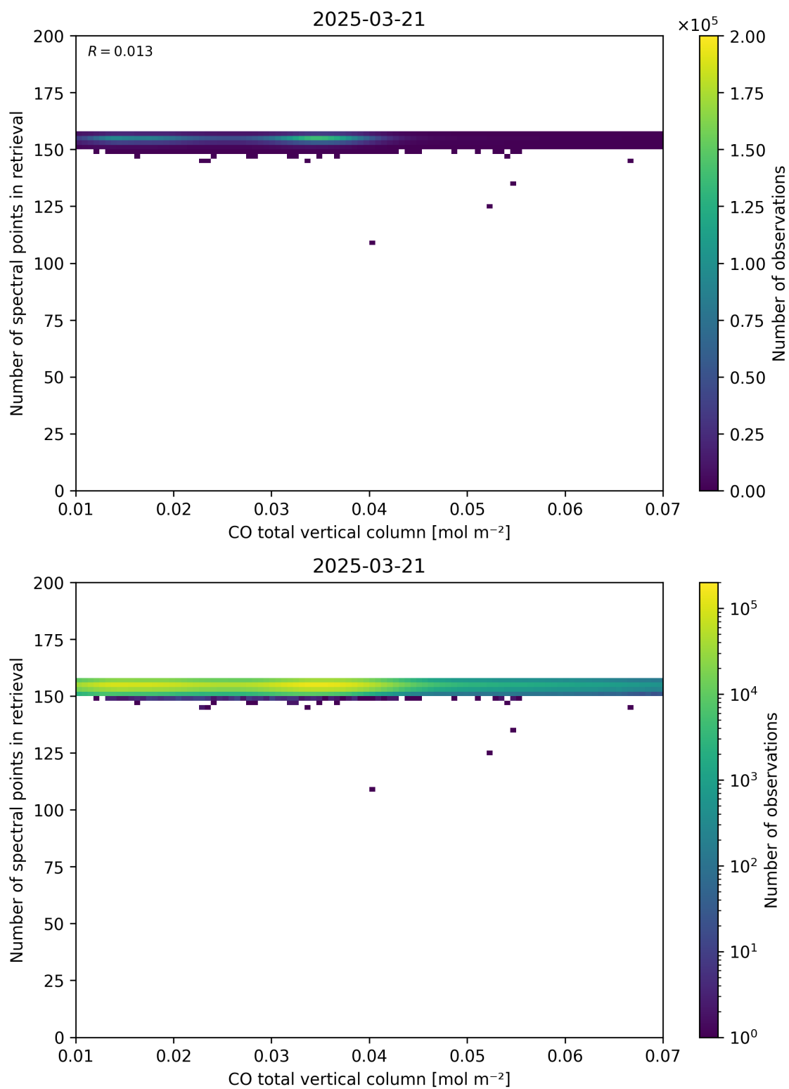
Figure 43: Scatter density plot of “CO total vertical column” against “Number of spectral points in retrieval” for 2025-03-20 to 2025-03-22.
