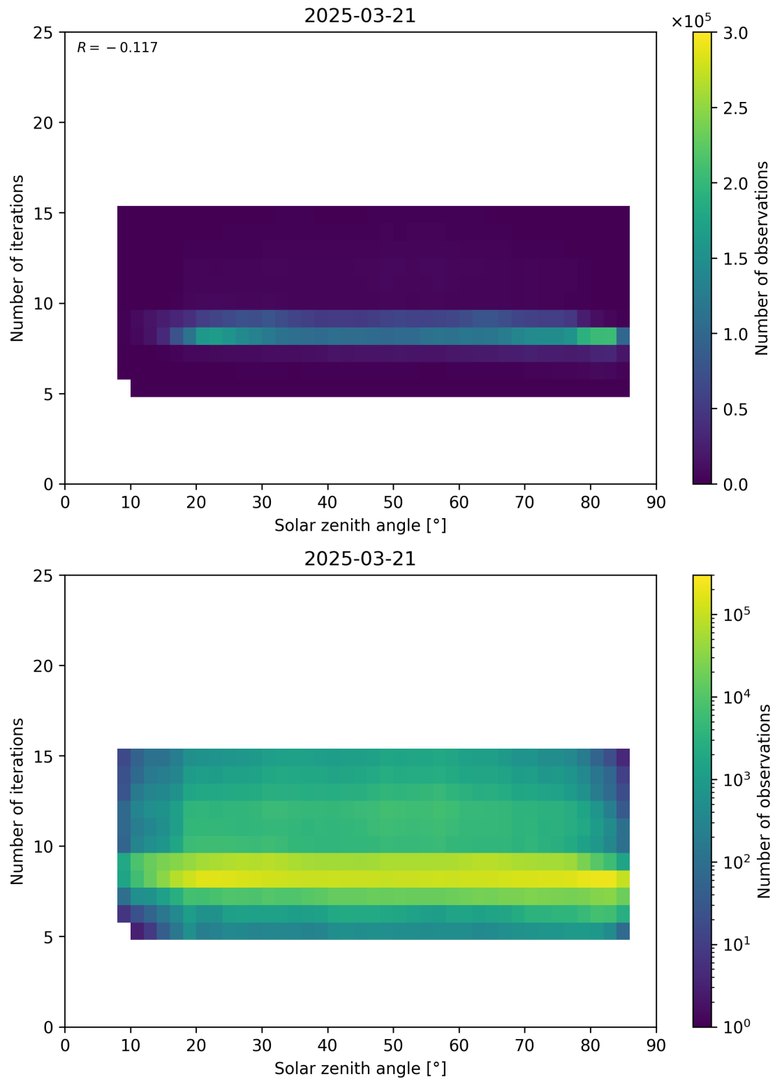
Figure 67: Scatter density plot of “Solar zenith angle” against “Number of iterations” for 2025-03-20 to 2025-03-22.
