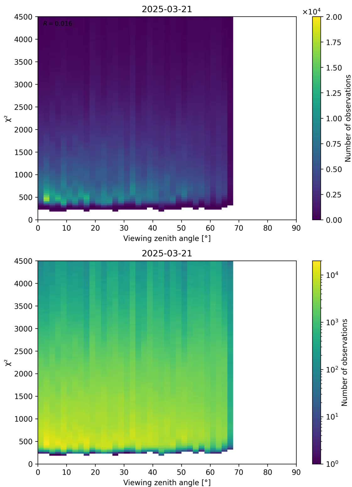
Figure 72: Scatter density plot of “Viewing zenith angle” against “ \chi^2 ” for 2025-03-20 to 2025-03-22.
