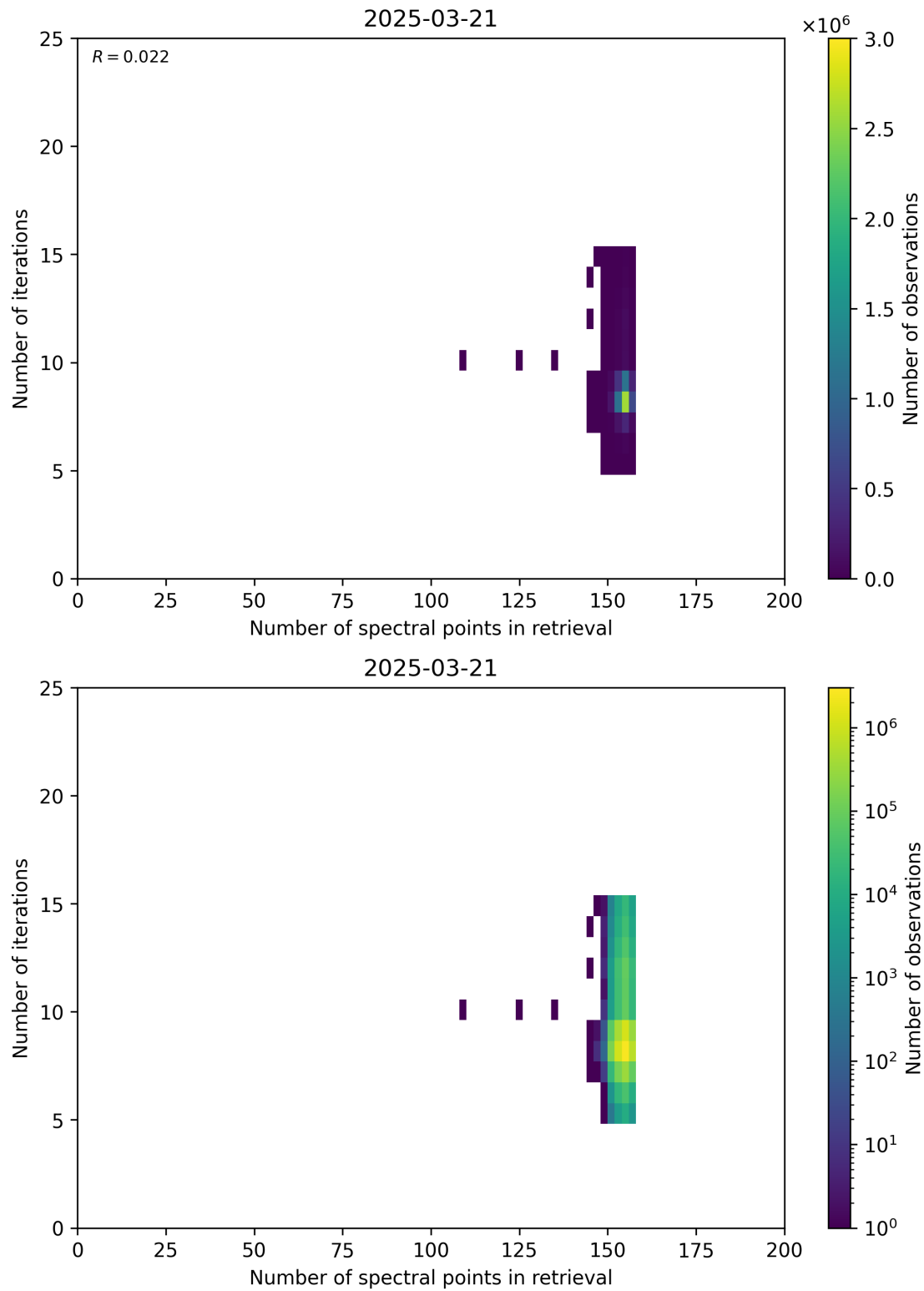
Figure 60: Scatter density plot of “Number of spectral points in retrieval” against “Number of iterations” for 2025-03-20 to 2025-03-22.
