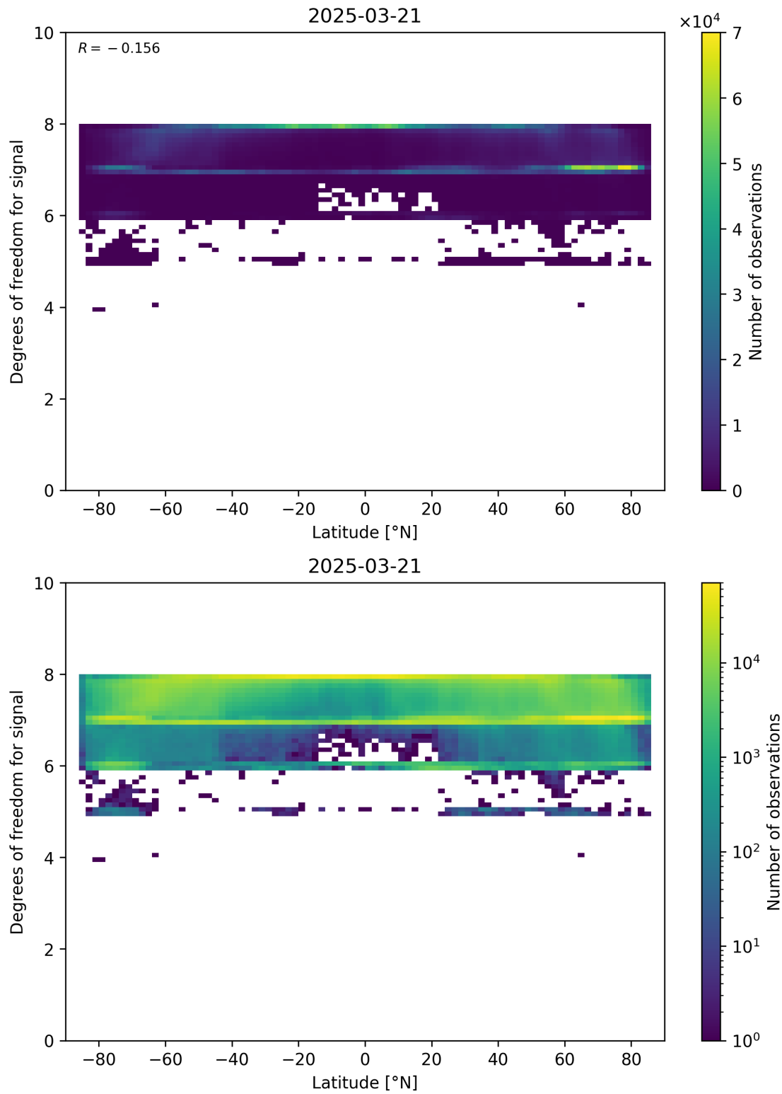
Figure 55: Scatter density plot of “Latitude” against “Degrees of freedom for signal” for 2025-03-20 to 2025-03-22.
