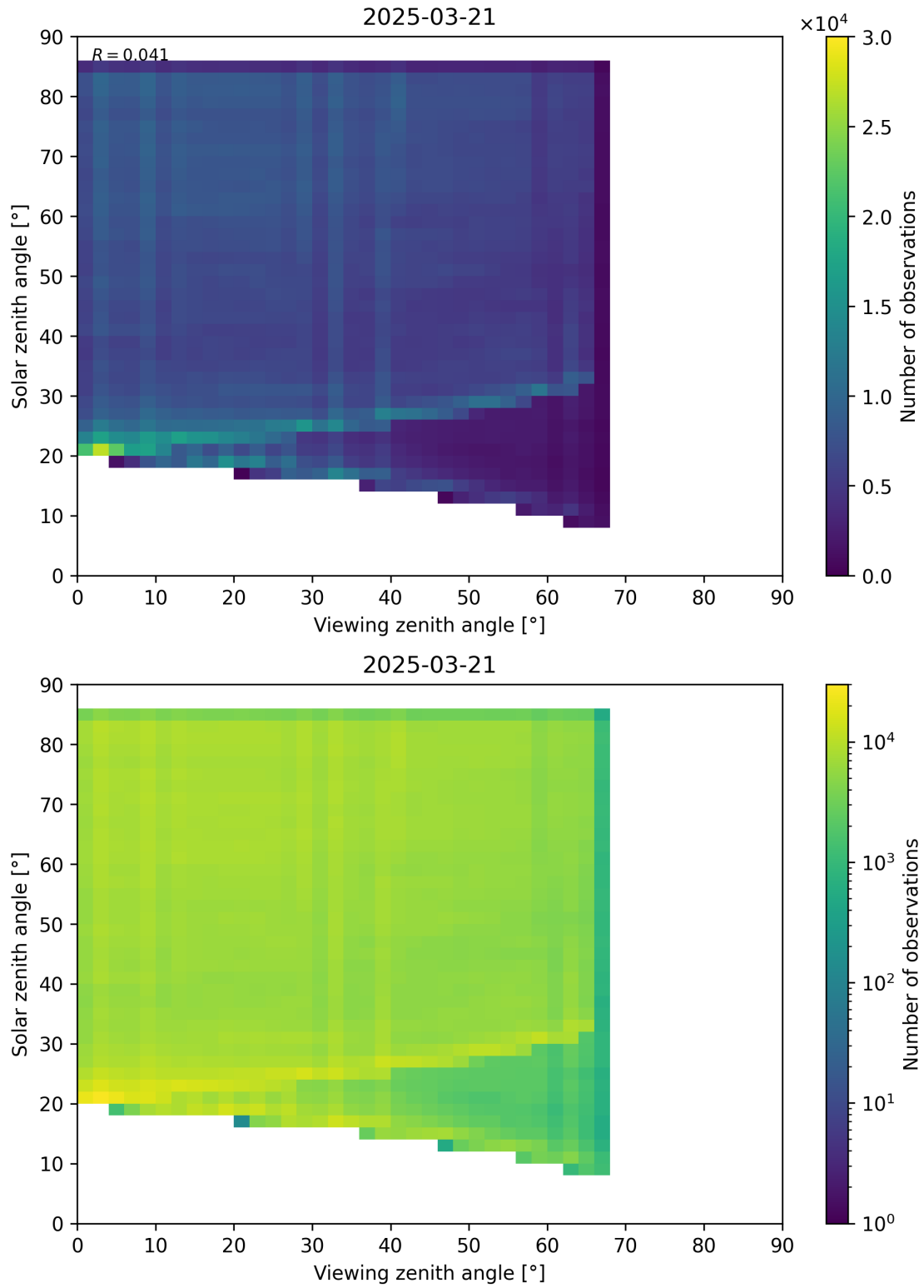
Figure 77: Scatter density plot of “Viewing zenith angle” against “Solar zenith angle” for 2025-03-20 to 2025-03-22.
