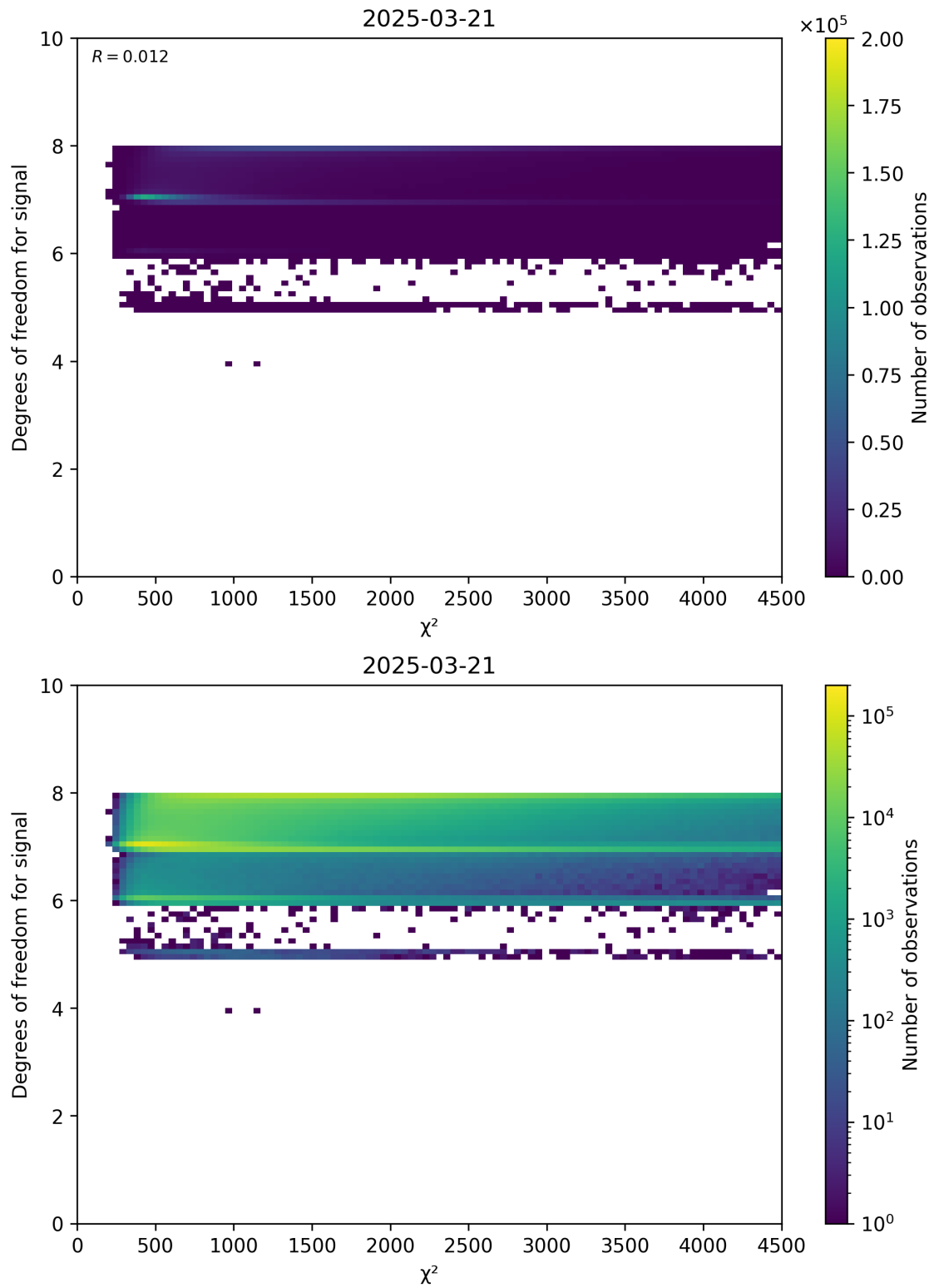
Figure 48: Scatter density plot of “ \chi^2 ” against “Degrees of freedom for signal” for 2025-03-20 to 2025-03-22.
