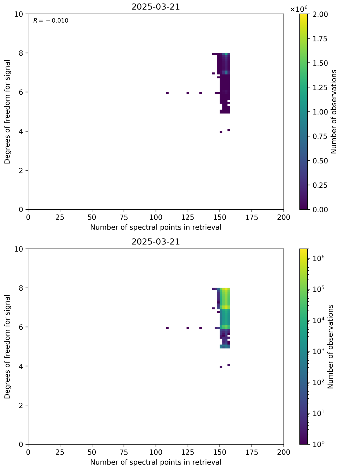
Figure 59: Scatter density plot of “Number of spectral points in retrieval” against “Degrees of freedom for signal” for 2025-03-20 to 2025-03-22.
