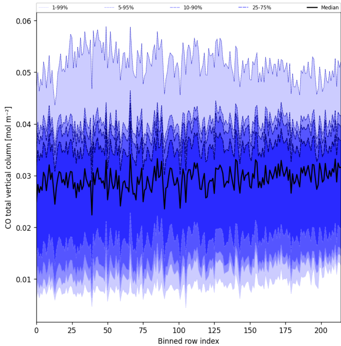
Figure 26: Along track statistics of “CO total vertical column” for 2025-03-20 to 2025-03-22
