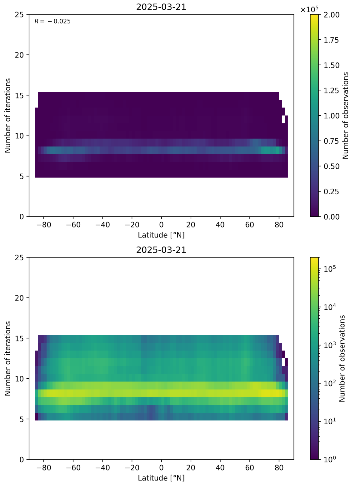
Figure 56: Scatter density plot of “Latitude” against “Number of iterations” for 2025-03-20 to 2025-03-22.
