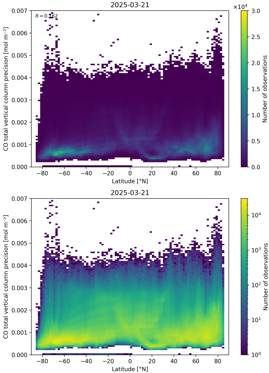
Figure 53: Scatter density plot of “Latitude” against “CO total vertical column precision” for 2025-03-20 to 2025-03-22.
