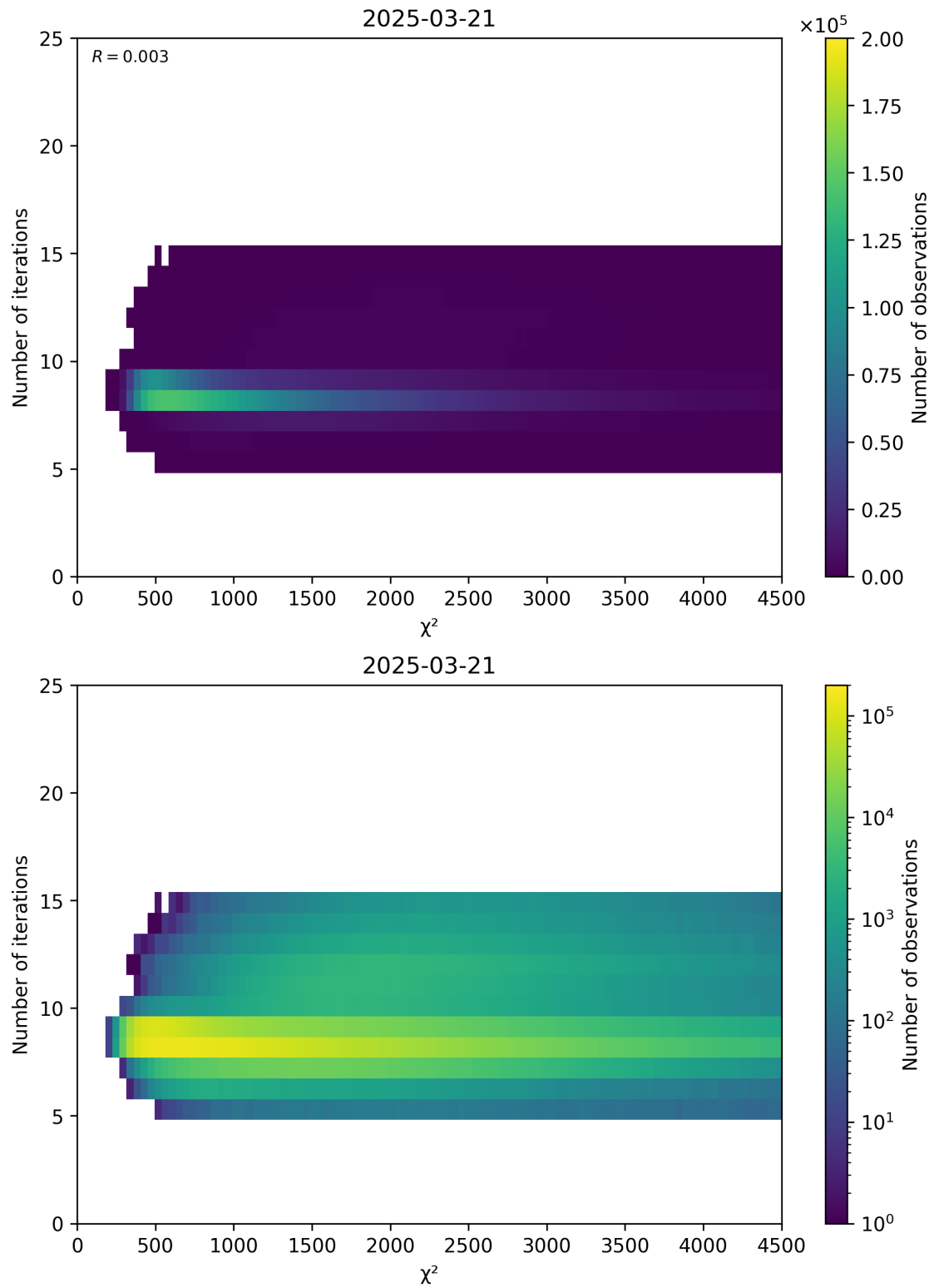
Figure 49: Scatter density plot of “ \chi^2 ” against “Number of iterations” for 2025-03-20 to 2025-03-22.
