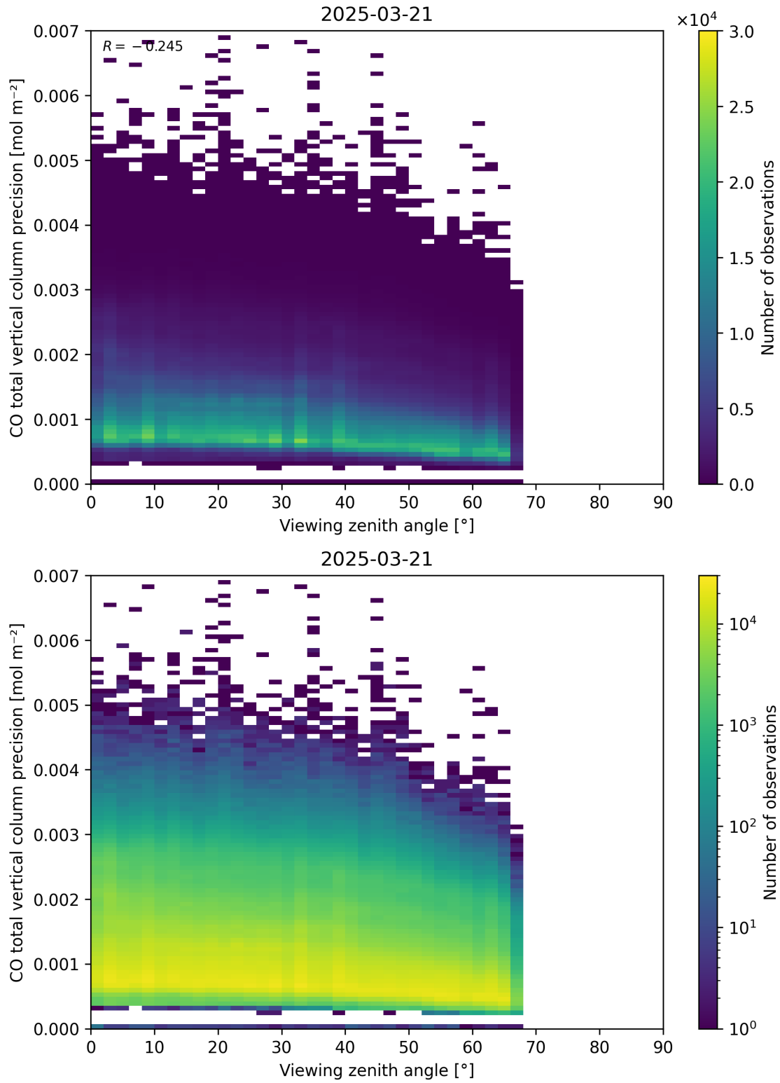
Figure 71: Scatter density plot of “Viewing zenith angle” against “CO total vertical column precision” for 2025-03-20 to 2025-03-22.
