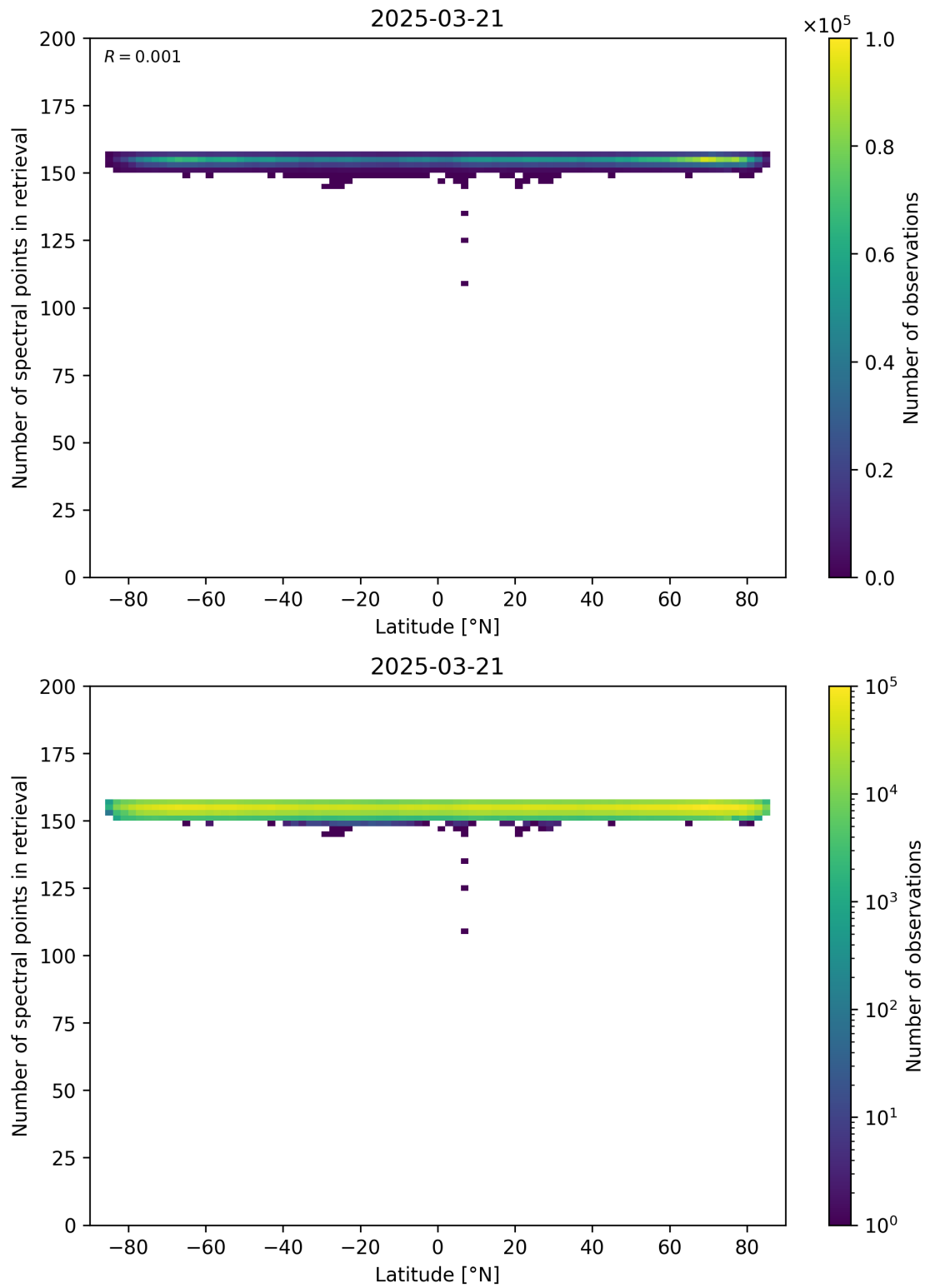
Figure 57: Scatter density plot of “Latitude” against “Number of spectral points in retrieval” for 2025-03-20 to 2025-03-22.
