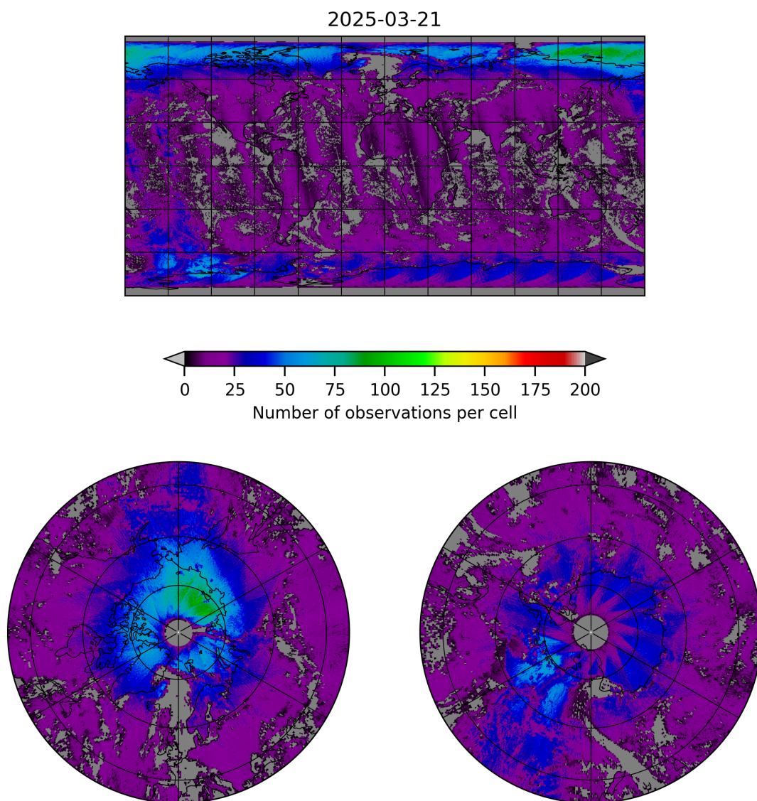
Figure 8: Map of the number of observations for 2025-03-20 to 2025-03-22
