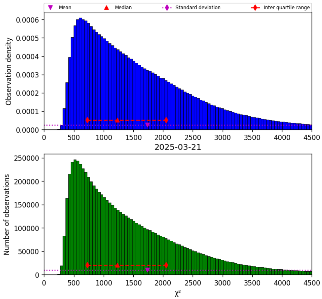
Figure 22: Histogram of “ \chi^2 ” for 2025-03-20 to 2025-03-22
