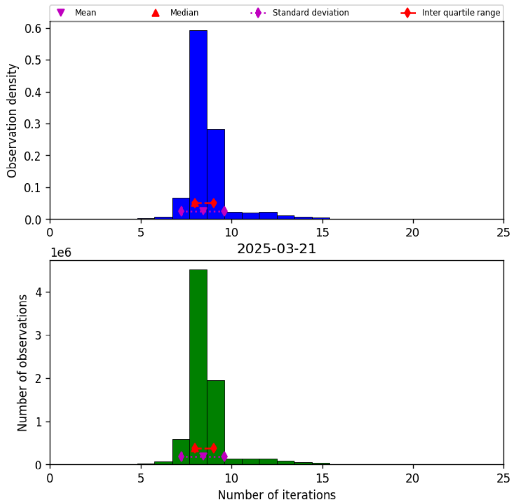
Figure 24: Histogram of “Number of iterations” for 2025-03-20 to 2025-03-22
