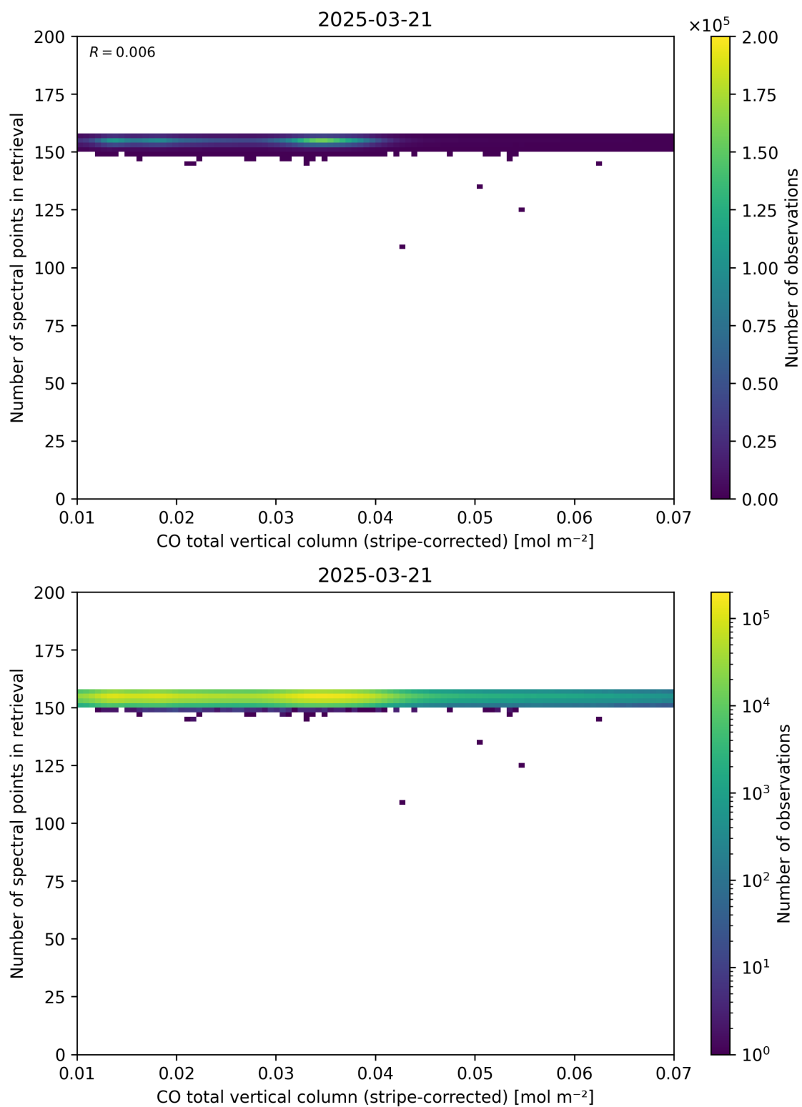
Figure 40: Scatter density plot of “CO total vertical column (stripe-corrected)” against “Number of spectral points in retrieval” for 2025-03-20 to 2025-03-22.
