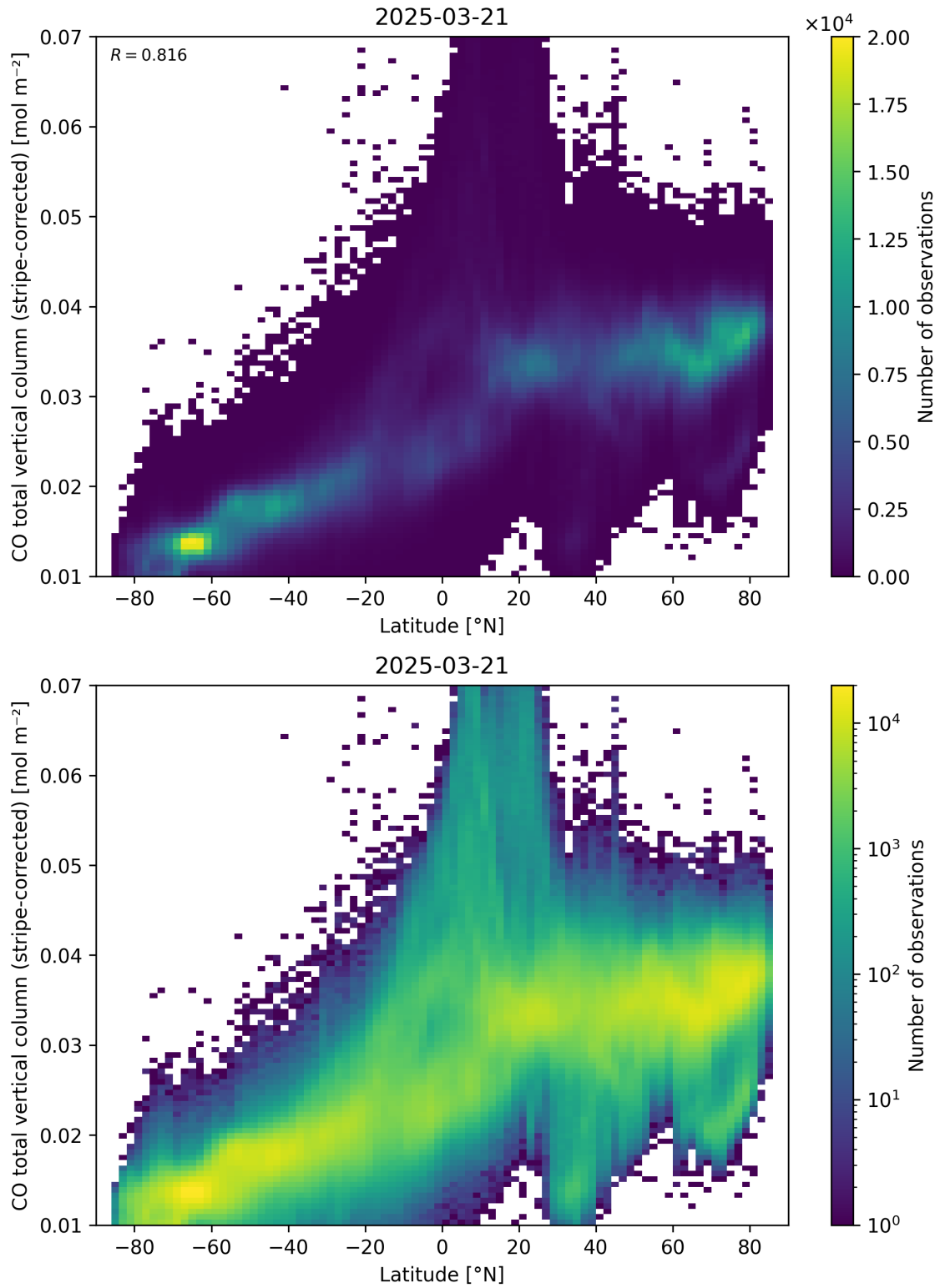
Figure 52: Scatter density plot of “Latitude” against “CO total vertical column (stripe-corrected)” for 2025-03-20 to 2025-03-22.
