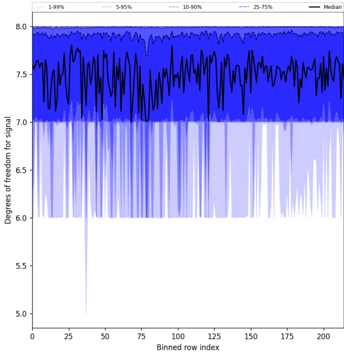
Figure 31: Along track statistics of “Degrees of freedom for signal” for 2025-03-20 to 2025-03-22
