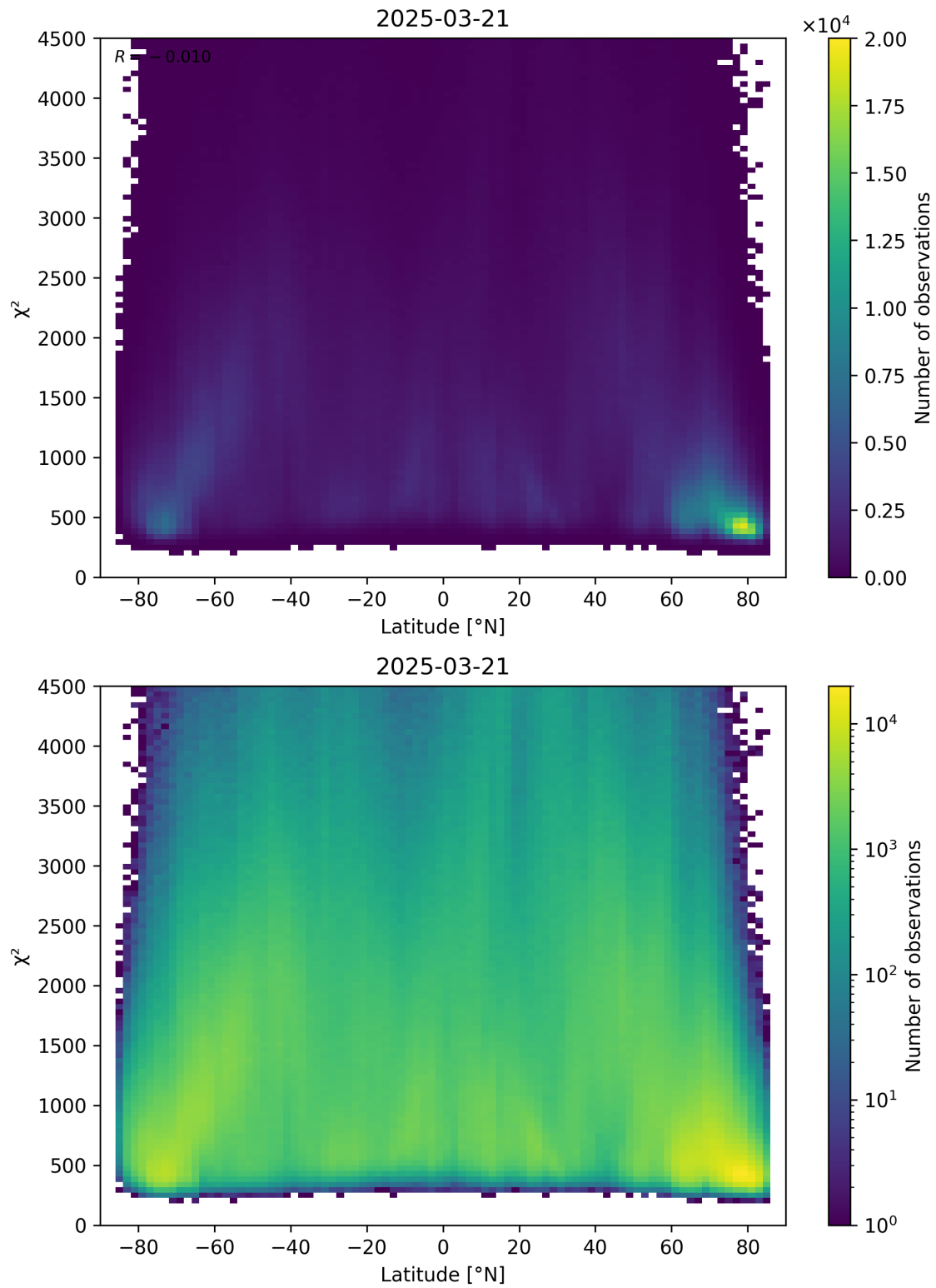
Figure 54: Scatter density plot of “Latitude” against “ \chi^2 ” for 2025-03-20 to 2025-03-22.
