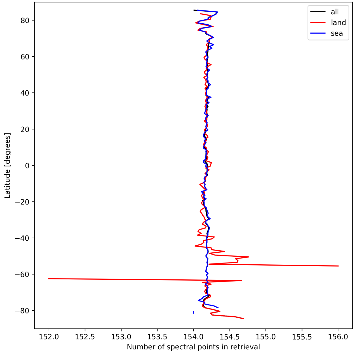
Figure 13: Zonal average of “Number of spectral points in retrieval” for 2025-03-20 to 2025-03-22.
