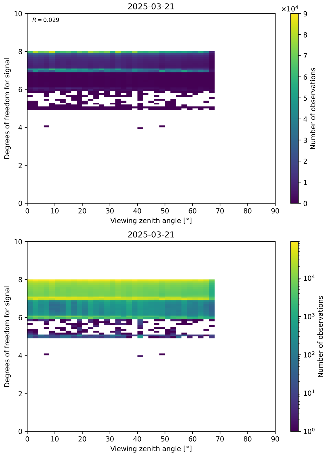
Figure 73: Scatter density plot of “Viewing zenith angle” against “Degrees of freedom for signal” for 2025-03-20 to 2025-03-22.
