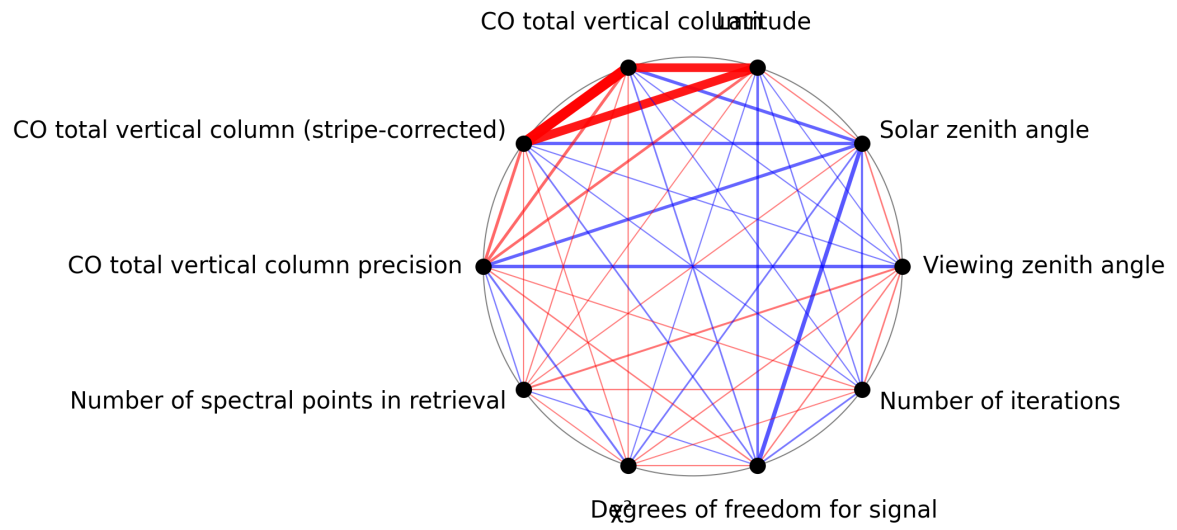
Figure 1: Map of correlation graph for 2025-03-20 to 2025-03-22.
