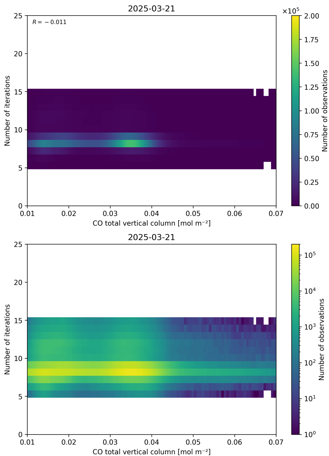
Figure 42: Scatter density plot of “CO total vertical column” against “Number of iterations” for 2025-03-20 to 2025-03-22.
