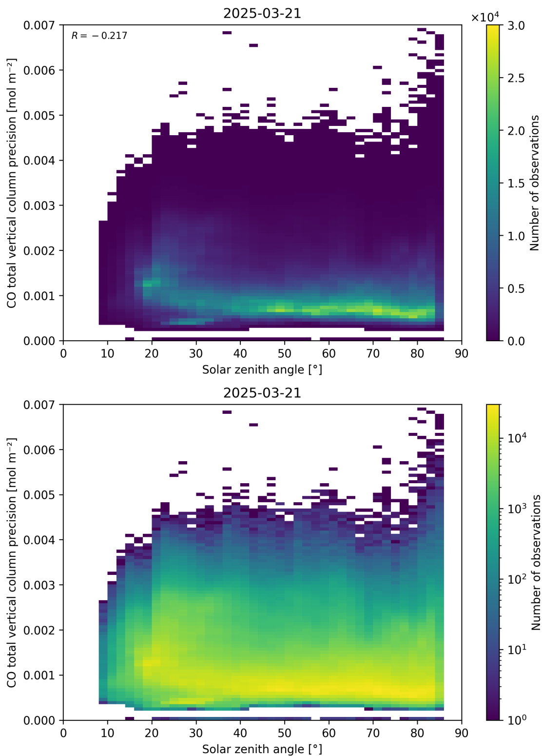
Figure 63: Scatter density plot of “Solar zenith angle” against “CO total vertical column precision” for 2025-03-20 to 2025-03-22.
