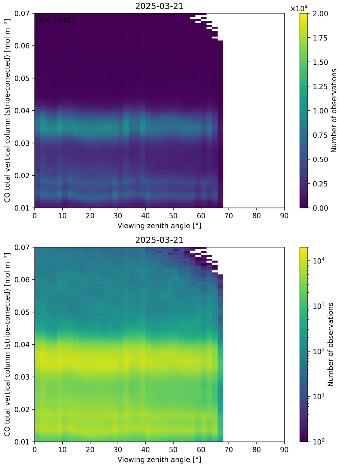
Figure 70: Scatter density plot of “Viewing zenith angle” against “CO total vertical column (stripe-corrected)” for 2025-03-20 to 2025-03-22.
