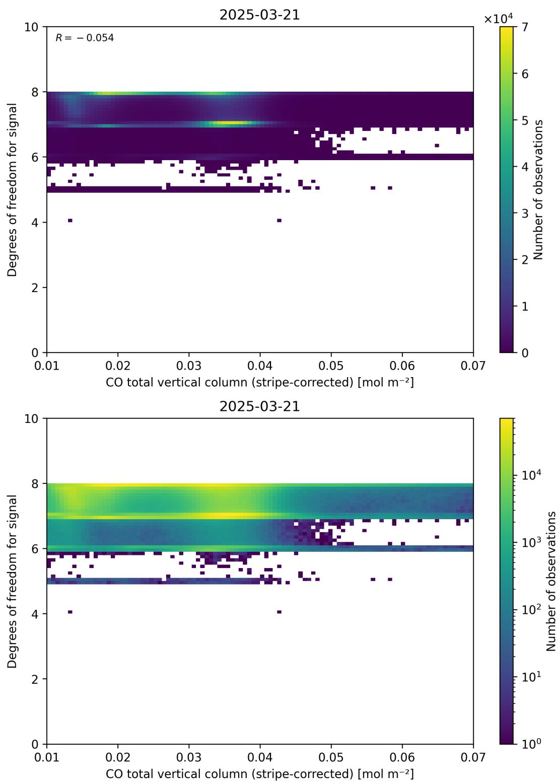
Figure 38: Scatter density plot of “CO total vertical column (stripe-corrected)” against “Degrees of freedom for signal” for 2025-03-20 to 2025-03-22.
