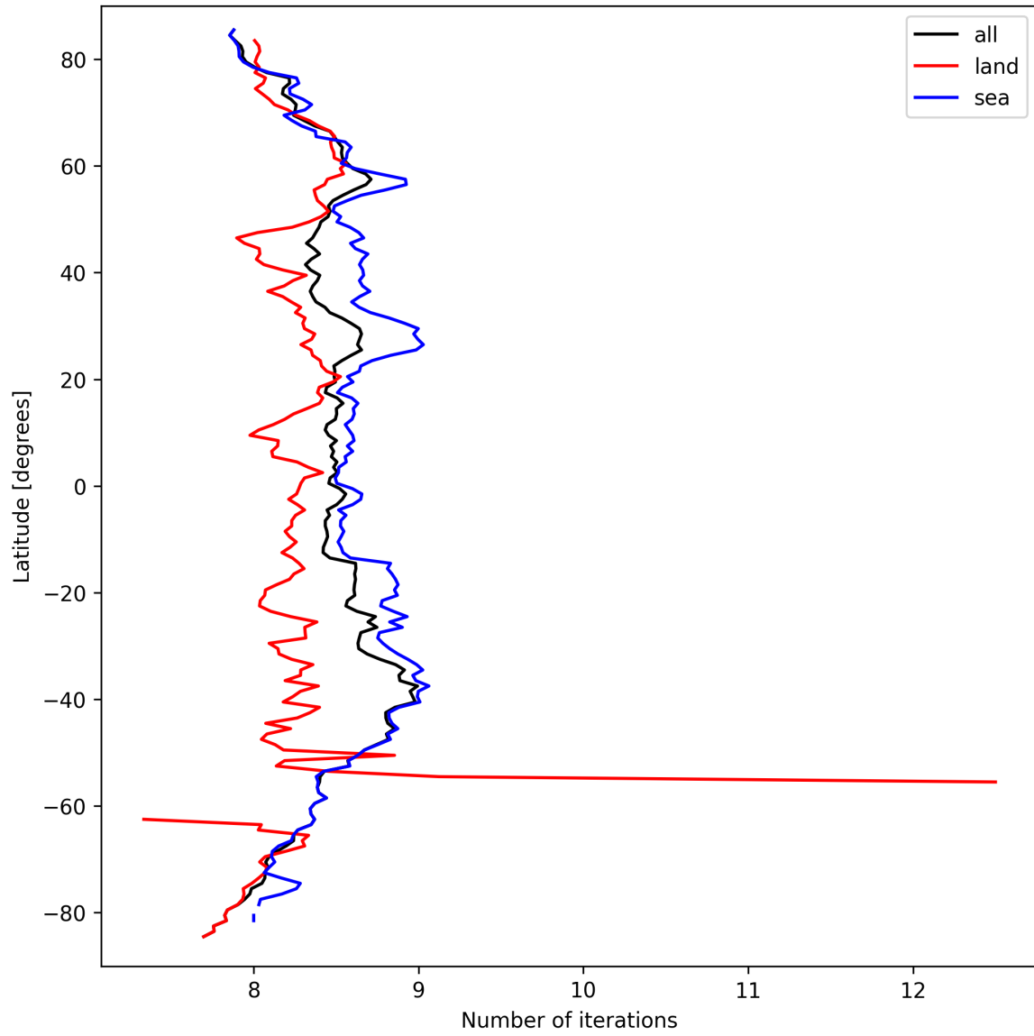
Figure 16: Zonal average of “Number of iterations” for 2025-03-20 to 2025-03-22.
