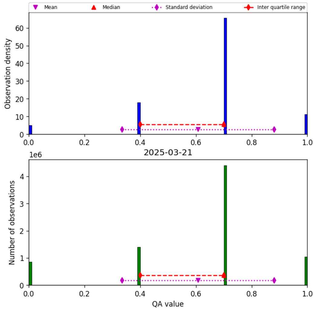
Figure 17: Histogram of “QA value” for 2025-03-20 to 2025-03-22
