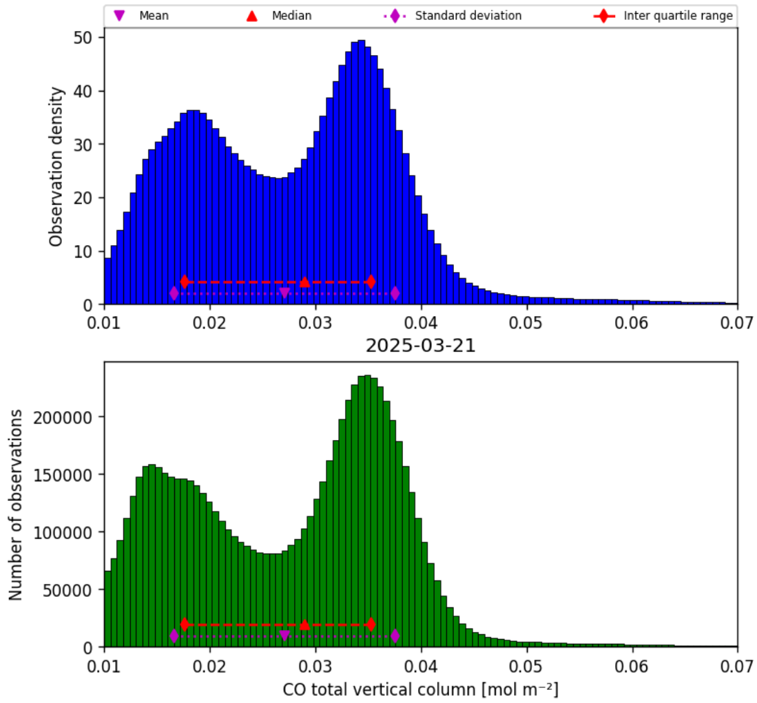
Figure 18: Histogram of “CO total vertical column” for 2025-03-20 to 2025-03-22
