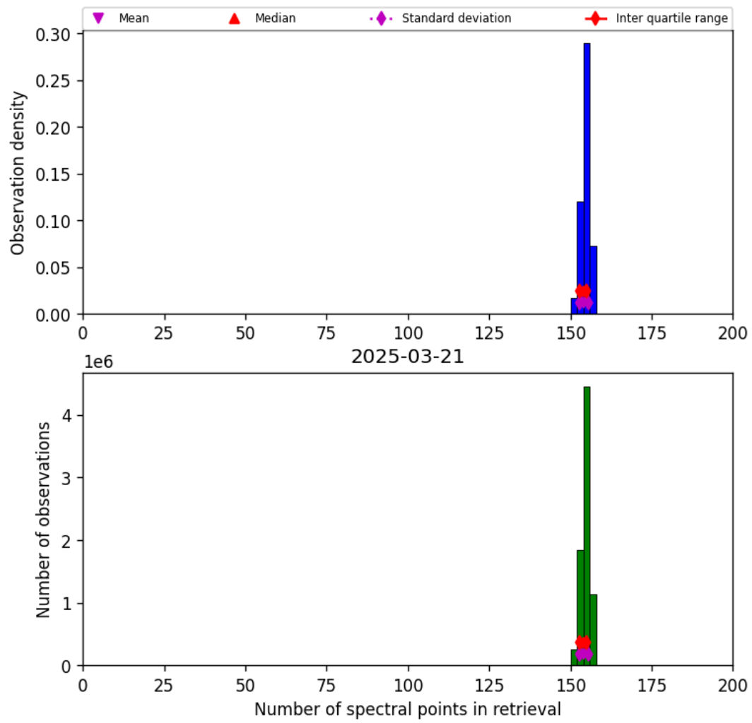
Figure 21: Histogram of “Number of spectral points in retrieval” for 2025-03-20 to 2025-03-22
