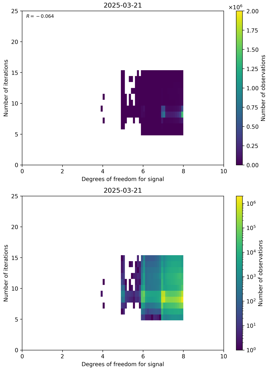
Figure 50: Scatter density plot of “Degrees of freedom for signal” against “Number of iterations” for 2025-03-20 to 2025-03-22.
