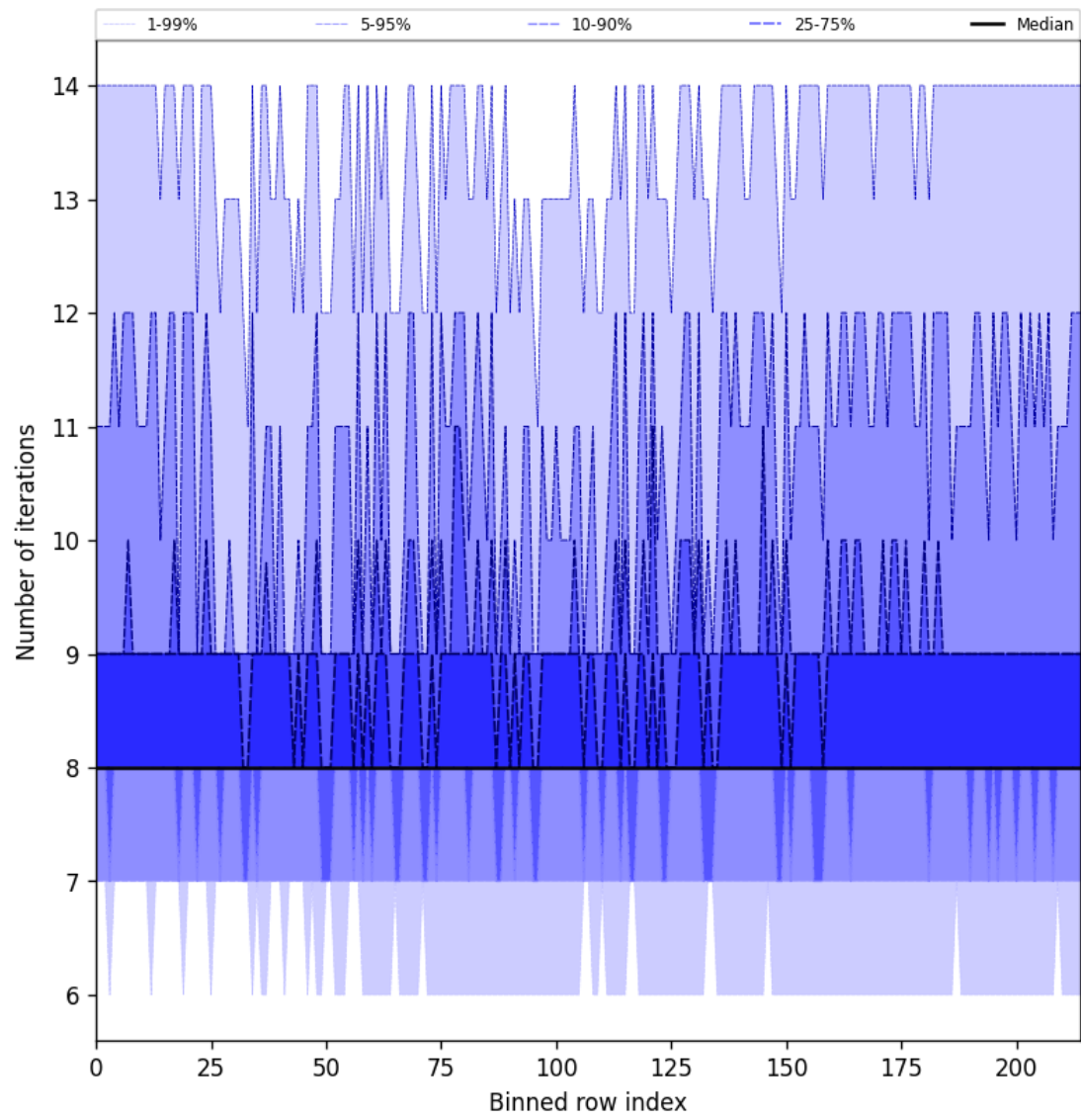
Figure 32: Along track statistics of “Number of iterations” for 2025-03-20 to 2025-03-22
