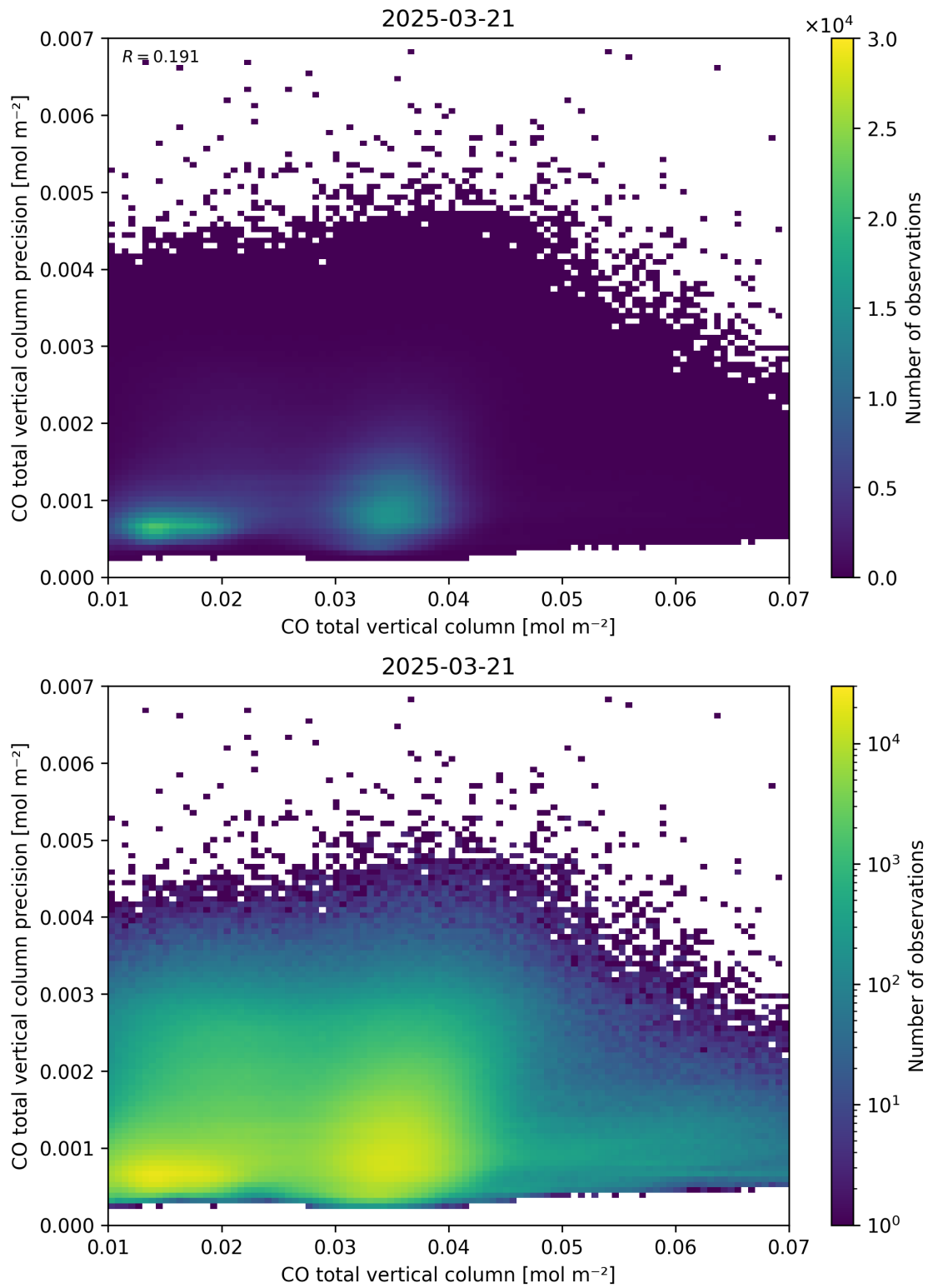
Figure 34: Scatter density plot of “CO total vertical column” against “CO total vertical column precision” for 2025-03-20 to 2025-03-22.
