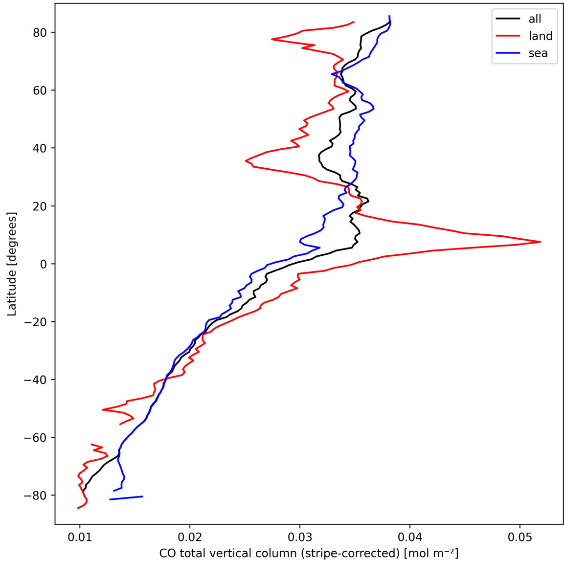
Figure 11: Zonal average of “CO total vertical column (stripe-corrected)” for 2025-03-20 to 2025-03-22.
