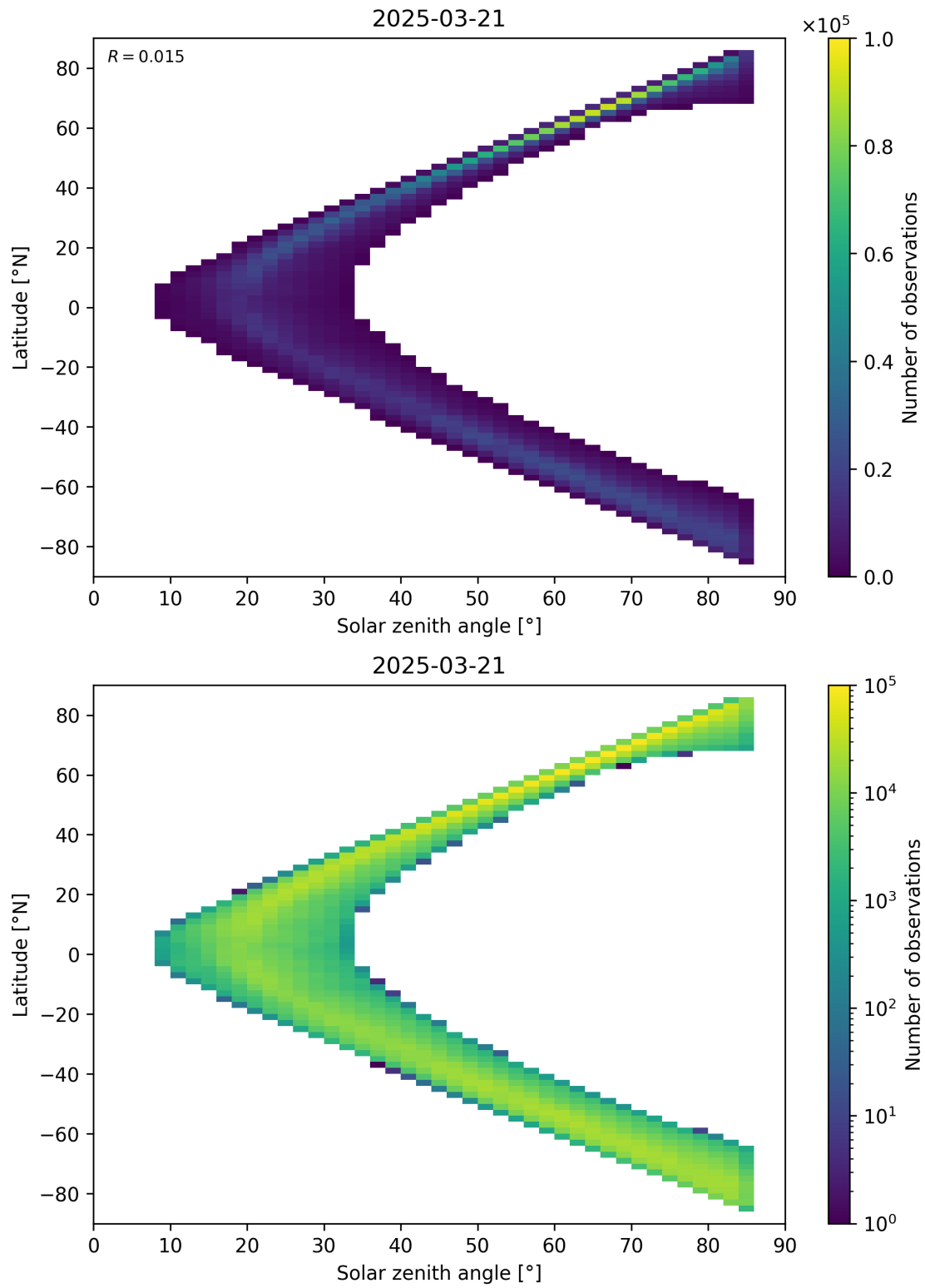
Figure 66: Scatter density plot of “Solar zenith angle” against “Latitude” for 2025-03-20 to 2025-03-22.
