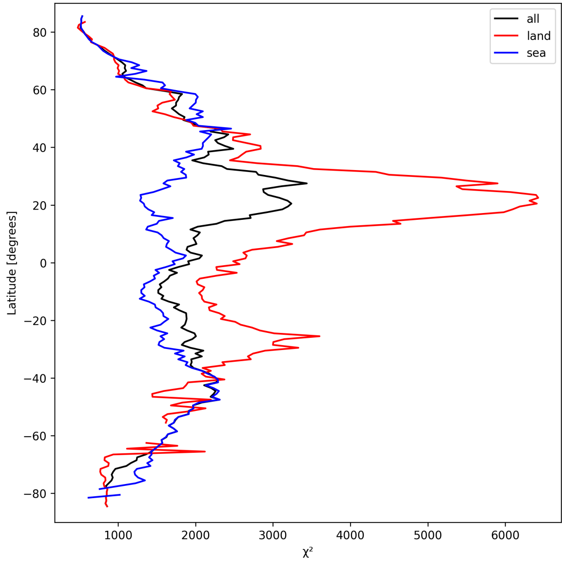
Figure 14: Zonal average of “ \chi^2 ” for 2025-03-20 to 2025-03-22.
