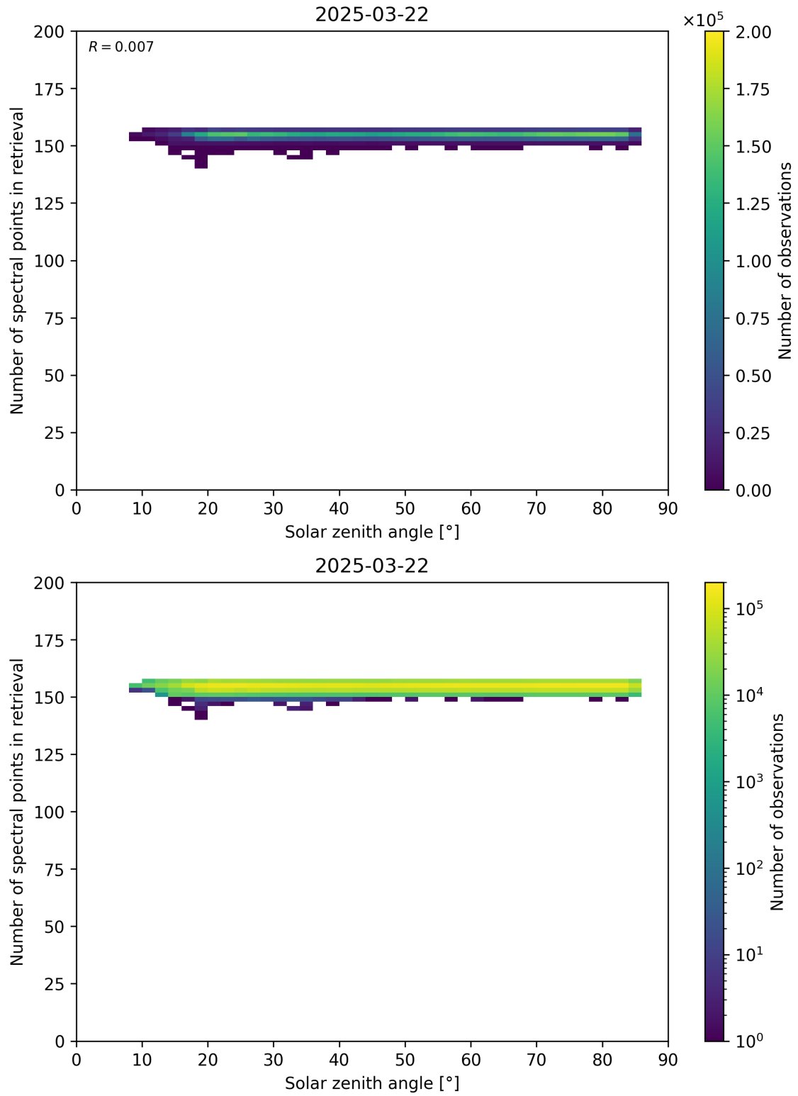
Figure 68: Scatter density plot of “Solar zenith angle” against “Number of spectral points in retrieval” for 2025-03-21 to 2025-03-23.
