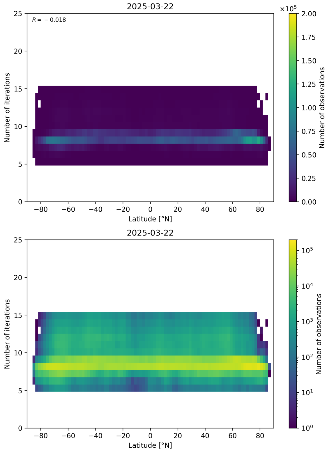
Figure 56: Scatter density plot of “Latitude” against “Number of iterations” for 2025-03-21 to 2025-03-23.
