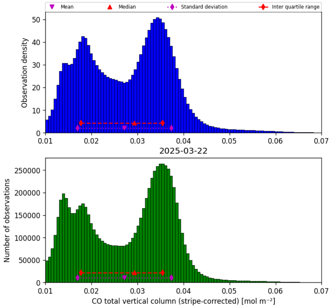
Figure 19: Histogram of “CO total vertical column (stripe-corrected)” for 2025-03-21 to 2025-03-23
