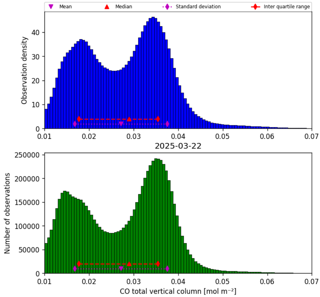
Figure 18: Histogram of “CO total vertical column” for 2025-03-21 to 2025-03-23
