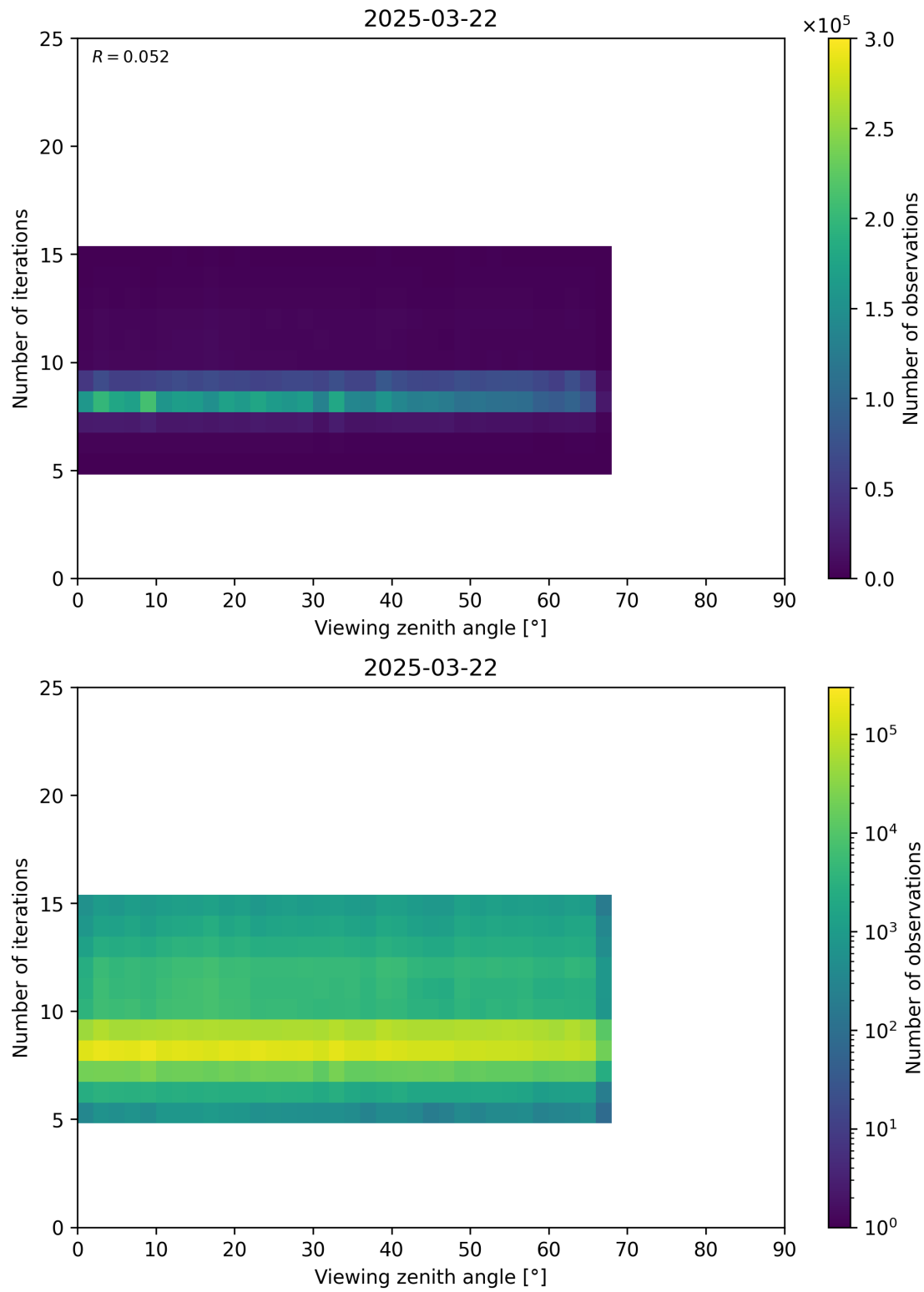
Figure 75: Scatter density plot of “Viewing zenith angle” against “Number of iterations” for 2025-03-21 to 2025-03-23.
