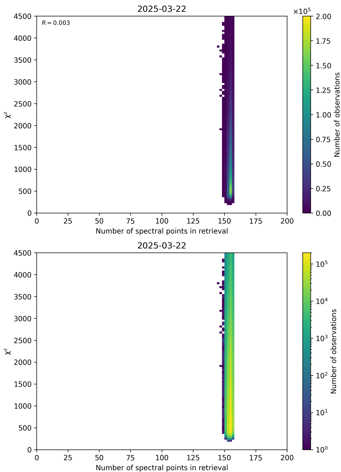
Figure 58: Scatter density plot of “Number of spectral points in retrieval” against “ \chi^2 ” for 2025-03-21 to 2025-03-23.
