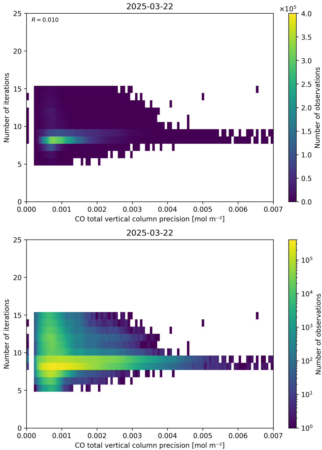
Figure 46: Scatter density plot of “CO total vertical column precision” against “Number of iterations” for 2025-03-21 to 2025-03-23.
