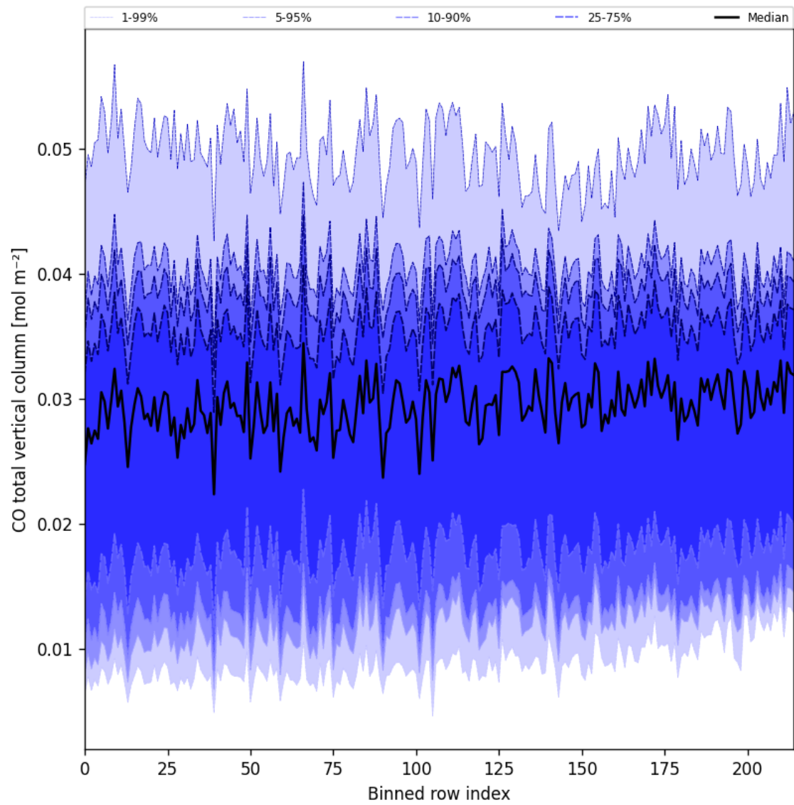
Figure 26: Along track statistics of “CO total vertical column” for 2025-03-21 to 2025-03-23
