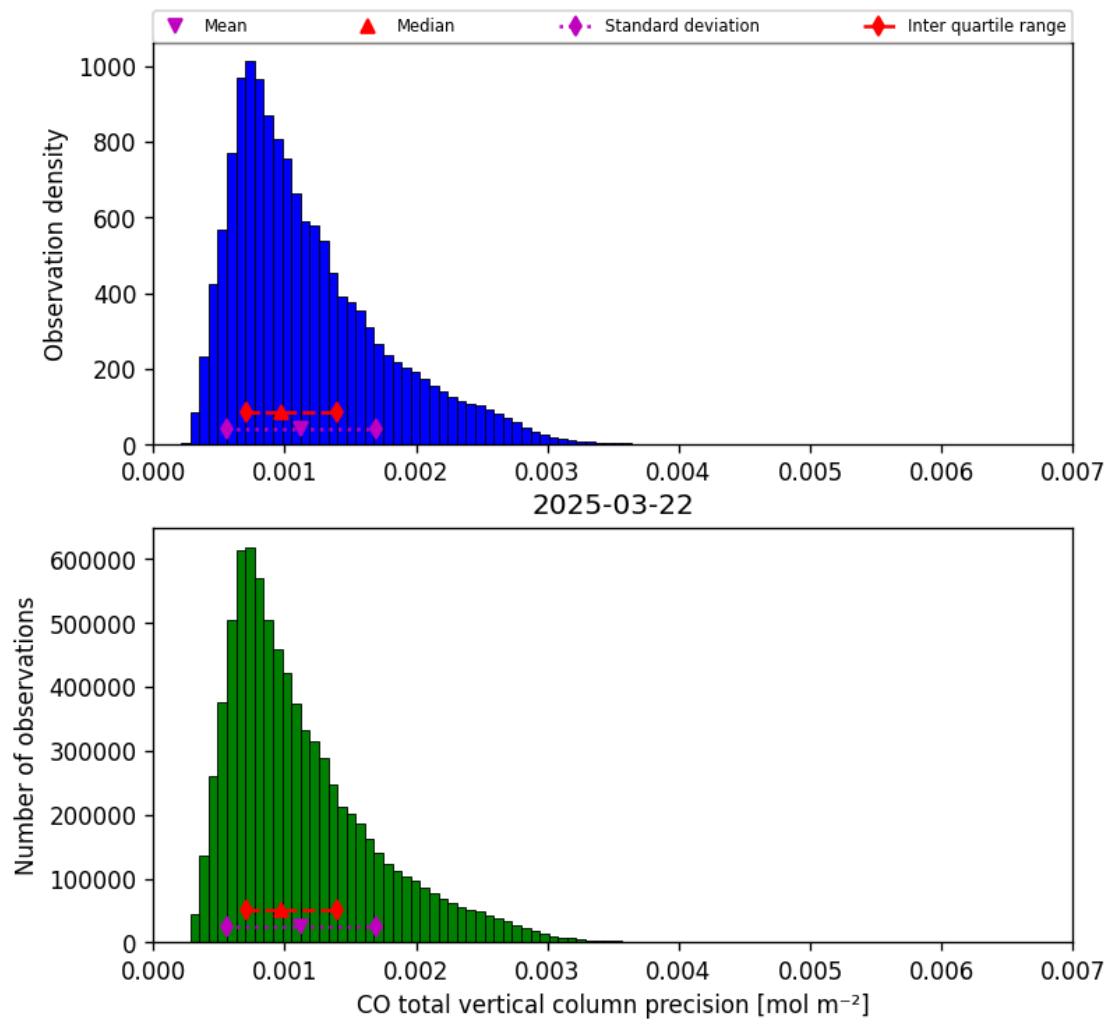
Figure 20: Histogram of “CO total vertical column precision” for 2025-03-21 to 2025-03-23
