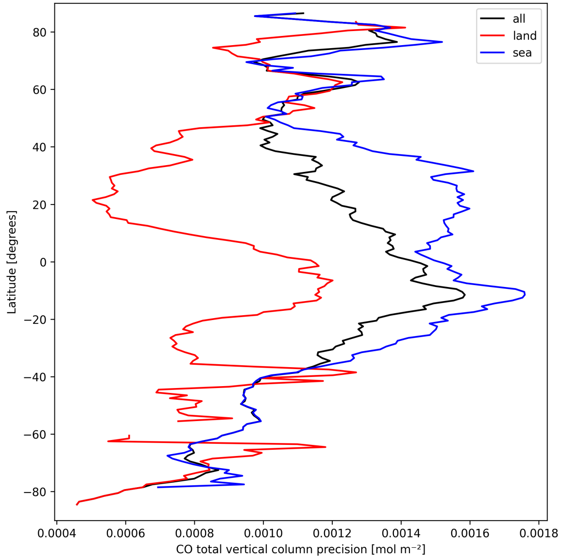
Figure 12: Zonal average of “CO total vertical column precision” for 2025-03-21 to 2025-03-23.
