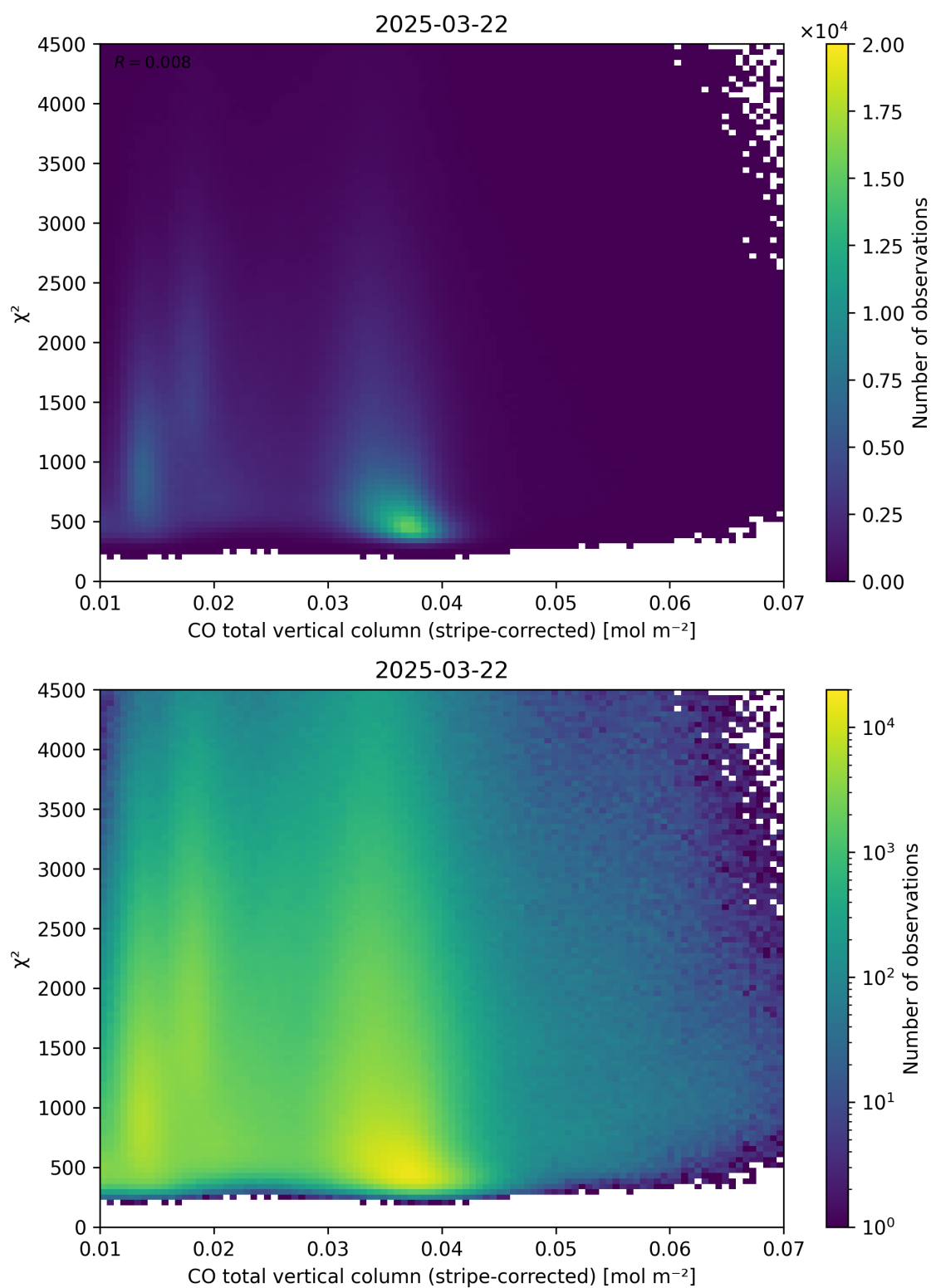
Figure 37: Scatter density plot of “CO total vertical column (stripe-corrected)” against “ \chi^2 ” for 2025-03-21 to 2025-03-23.
