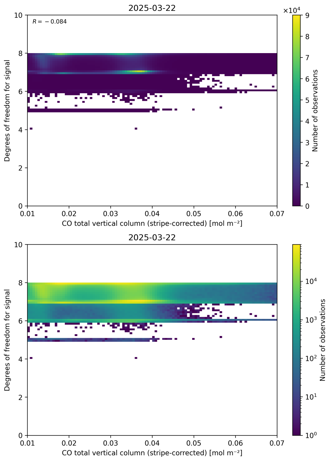
Figure 38: Scatter density plot of “CO total vertical column (stripe-corrected)” against “Degrees of freedom for signal” for 2025-03-21 to 2025-03-23.
