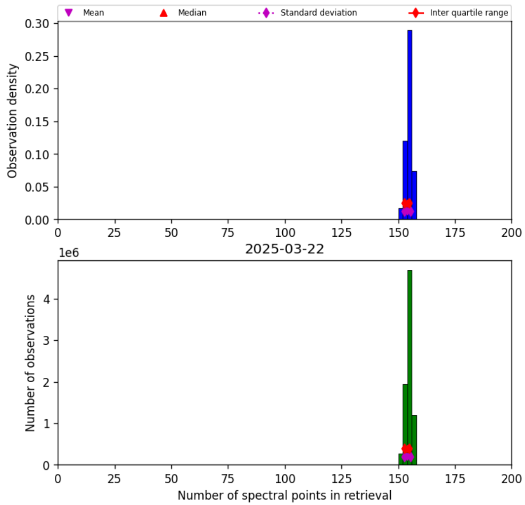
Figure 21: Histogram of “Number of spectral points in retrieval” for 2025-03-21 to 2025-03-23
