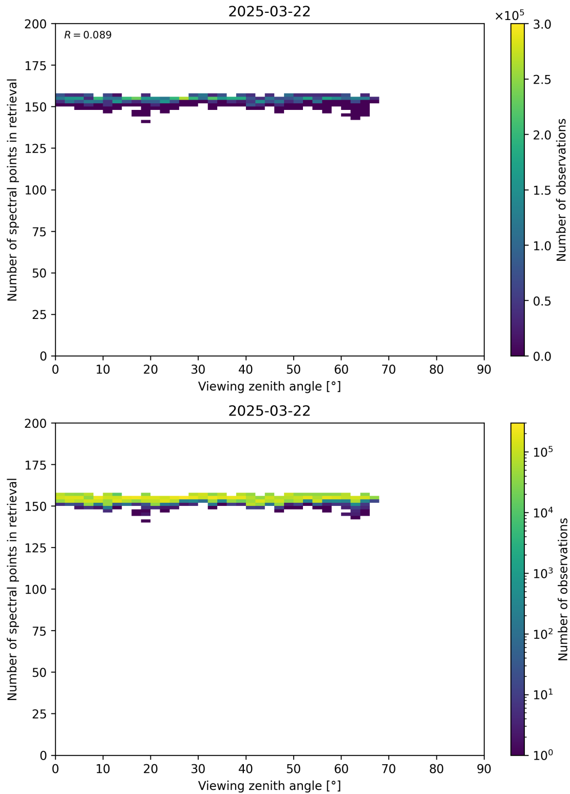
Figure 76: Scatter density plot of “Viewing zenith angle” against “Number of spectral points in retrieval” for 2025-03-21 to 2025-03-23.
