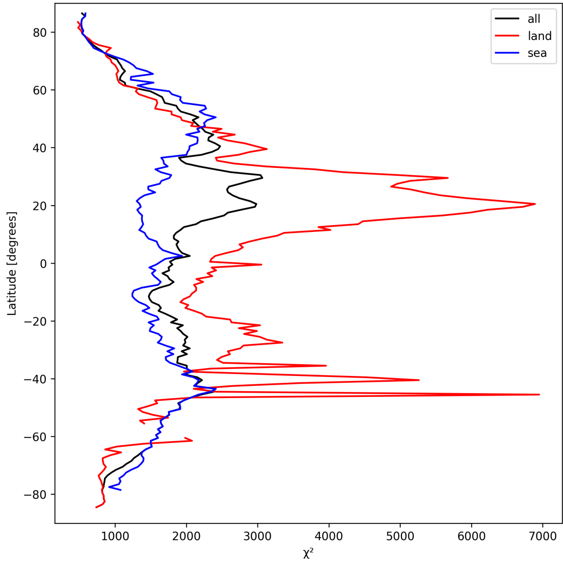
Figure 14: Zonal average of “ \chi^2 ” for 2025-03-21 to 2025-03-23.
