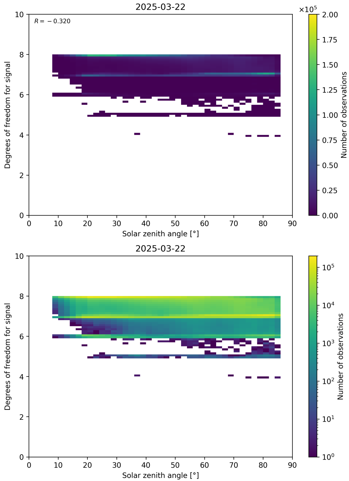
Figure 65: Scatter density plot of “Solar zenith angle” against “Degrees of freedom for signal” for 2025-03-21 to 2025-03-23.
