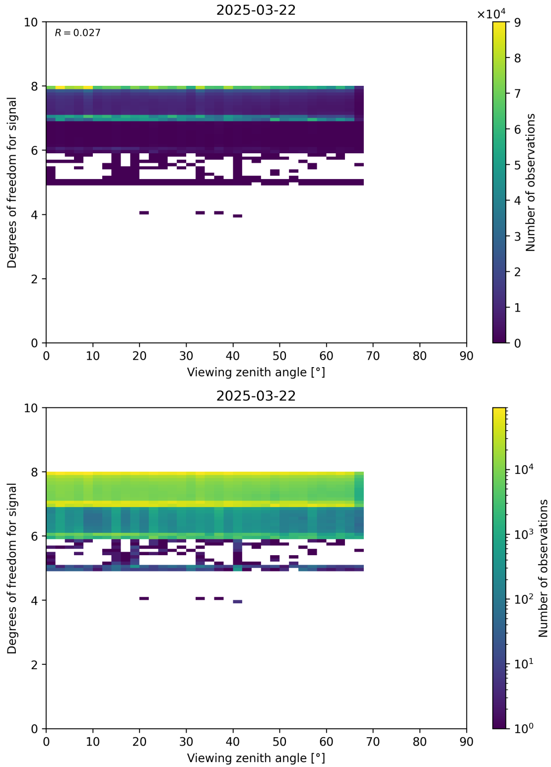
Figure 73: Scatter density plot of “Viewing zenith angle” against “Degrees of freedom for signal” for 2025-03-21 to 2025-03-23.
