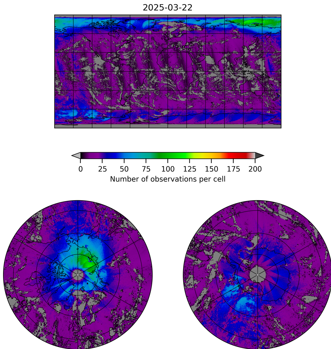
Figure 8: Map of the number of observations for 2025-03-21 to 2025-03-23
