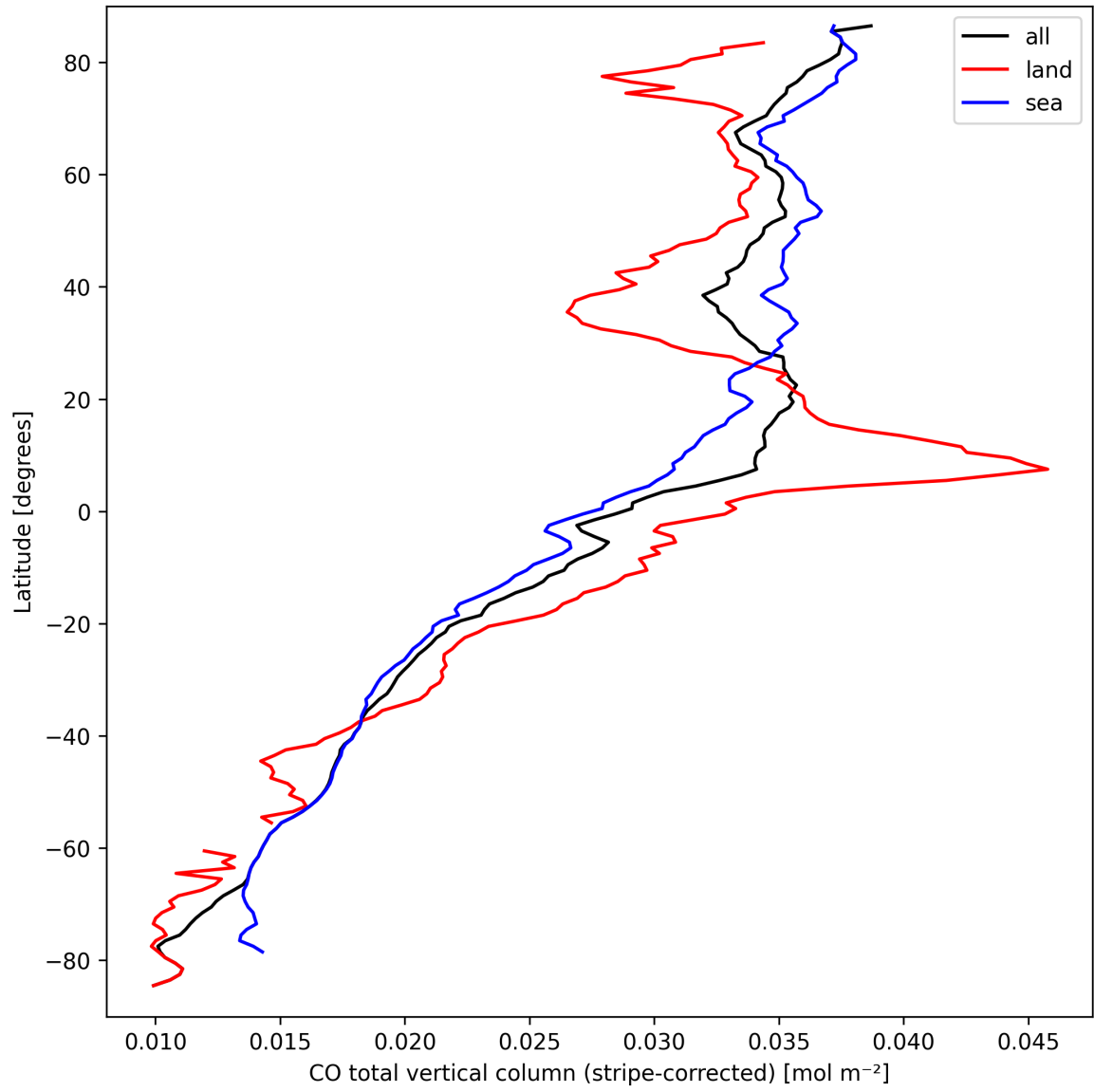
Figure 11: Zonal average of “CO total vertical column (stripe-corrected)” for 2025-03-21 to 2025-03-23.
