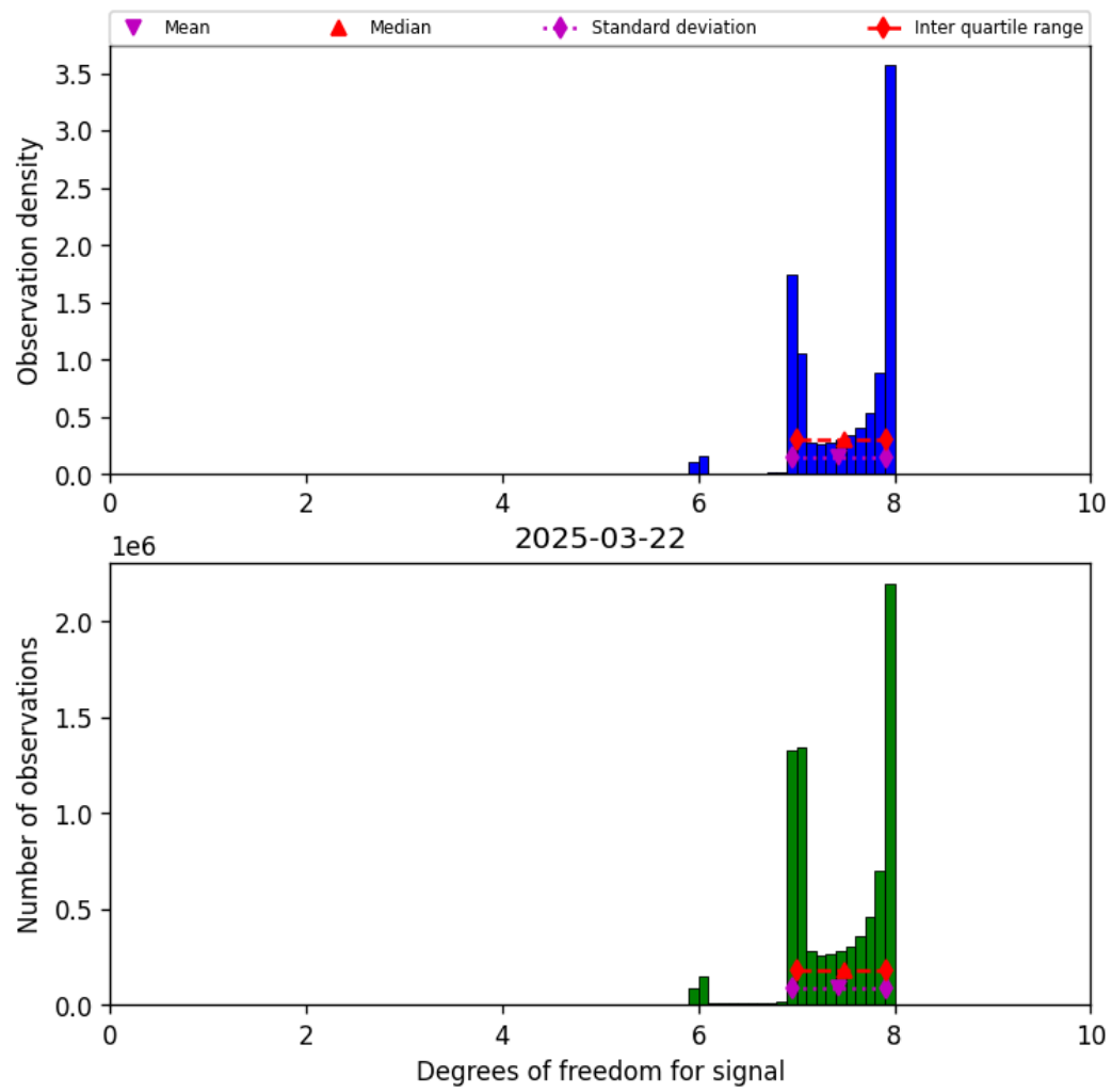
Figure 23: Histogram of “Degrees of freedom for signal” for 2025-03-21 to 2025-03-23
