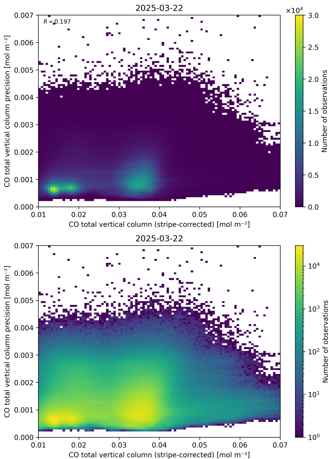
Figure 36: Scatter density plot of “CO total vertical column (stripe-corrected)” against “CO total vertical column precision” for 2025-03-21 to 2025-03-23.
