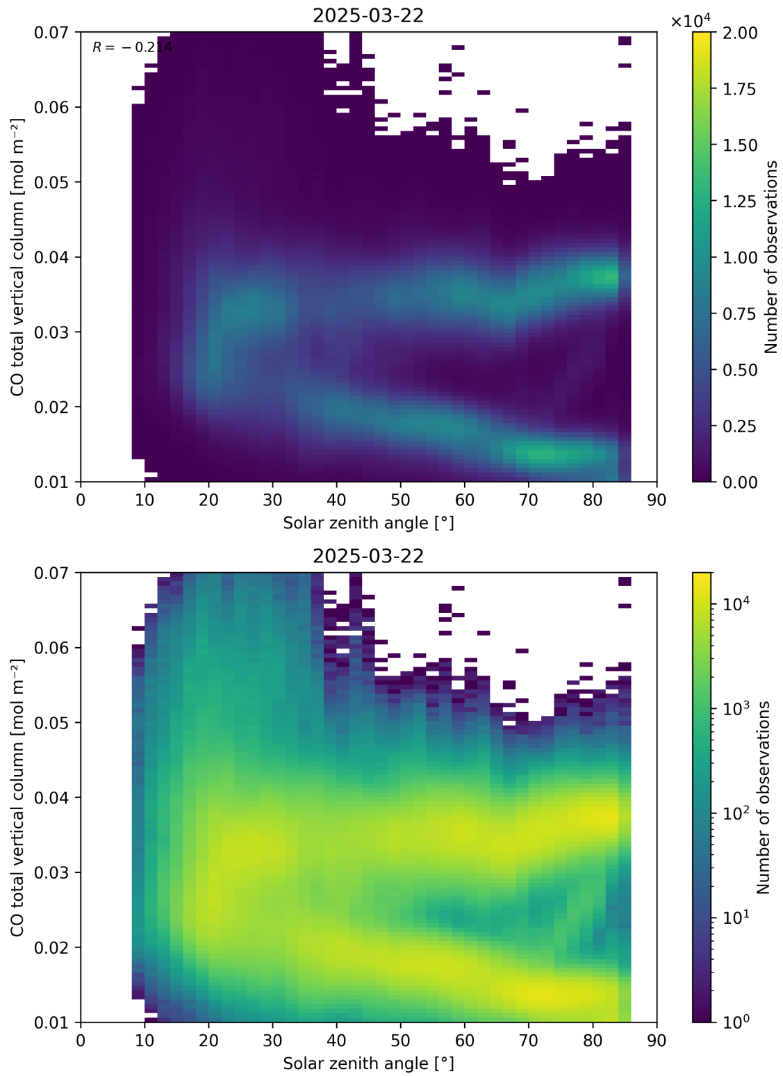
Figure 61: Scatter density plot of “Solar zenith angle” against “CO total vertical column” for 2025-03-21 to 2025-03-23.
