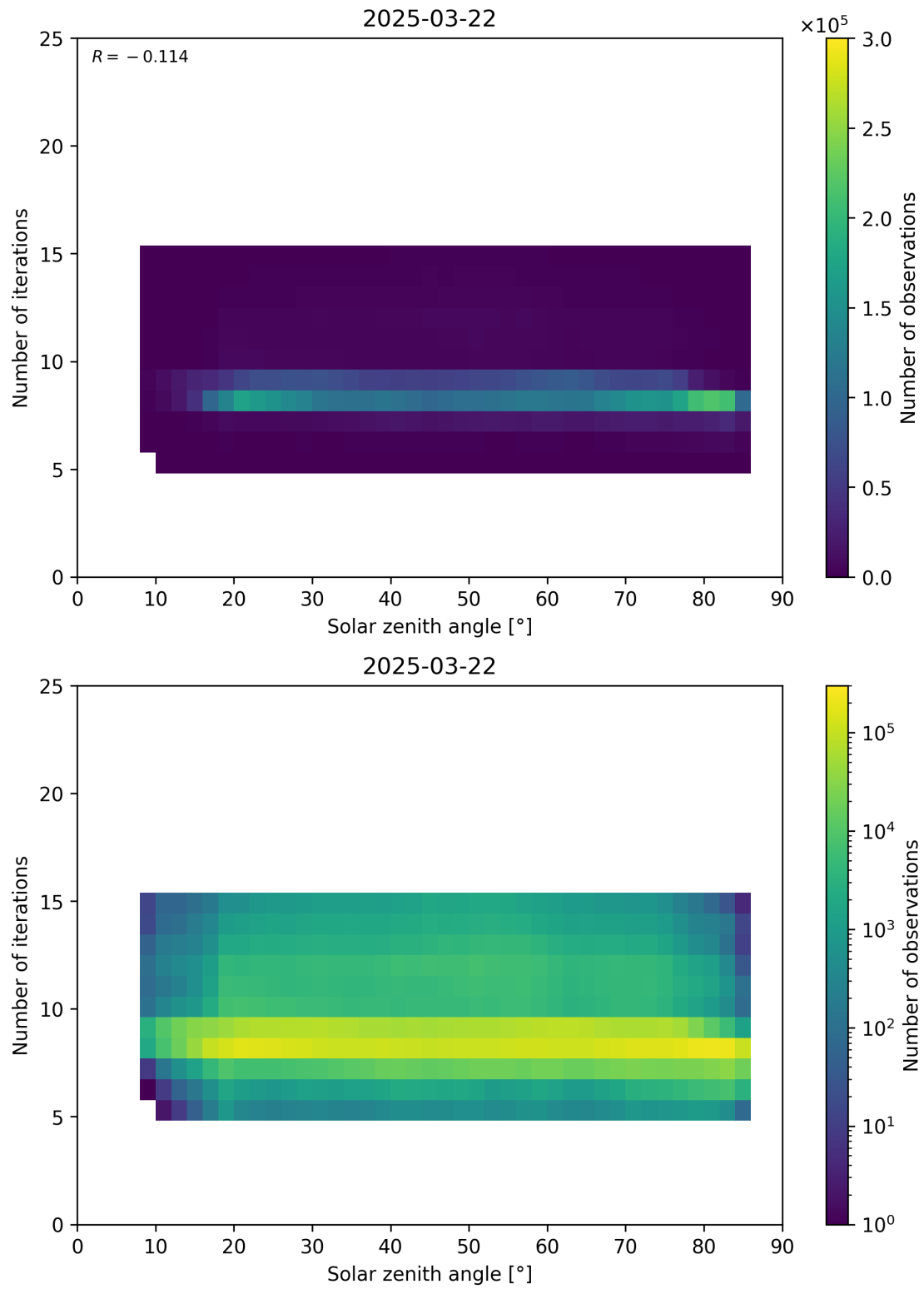
Figure 67: Scatter density plot of “Solar zenith angle” against “Number of iterations” for 2025-03-21 to 2025-03-23.
