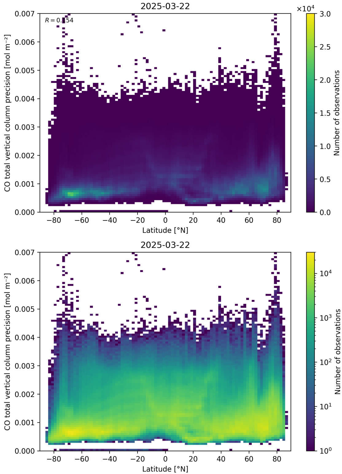
Figure 53: Scatter density plot of “Latitude” against “CO total vertical column precision” for 2025-03-21 to 2025-03-23.
