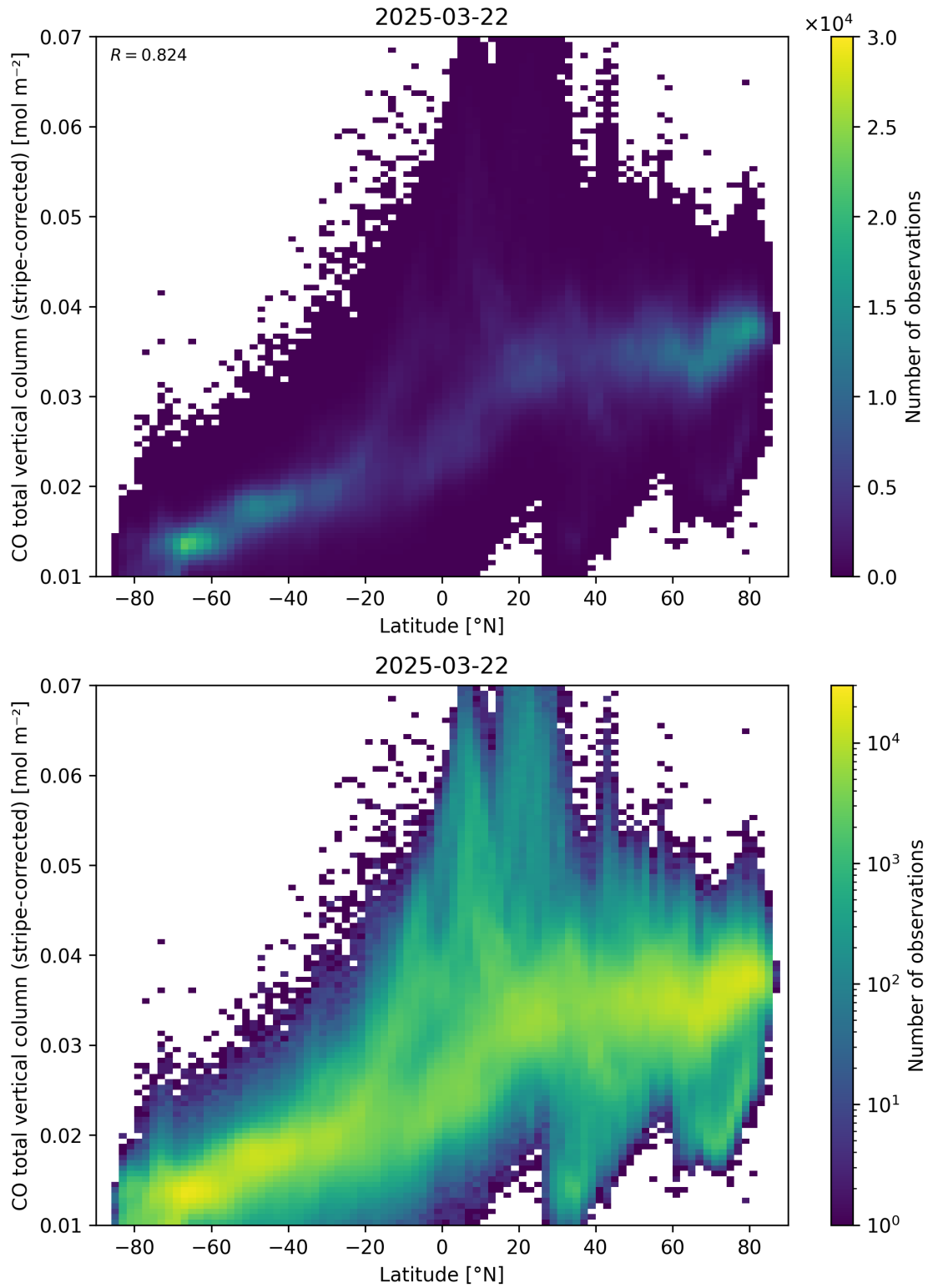
Figure 52: Scatter density plot of “Latitude” against “CO total vertical column (stripe-corrected)” for 2025-03-21 to 2025-03-23.
