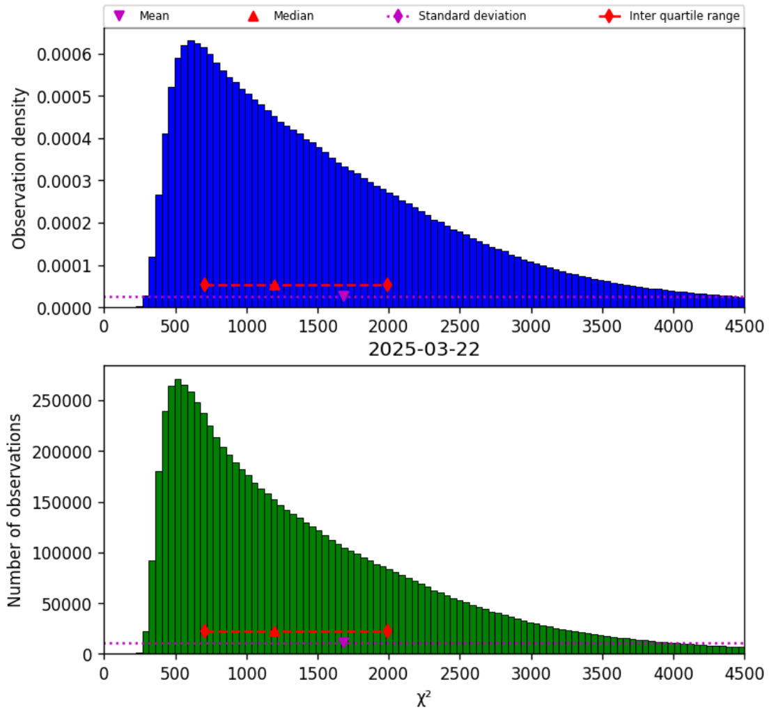
Figure 22: Histogram of “ \chi^2 ” for 2025-03-21 to 2025-03-23
