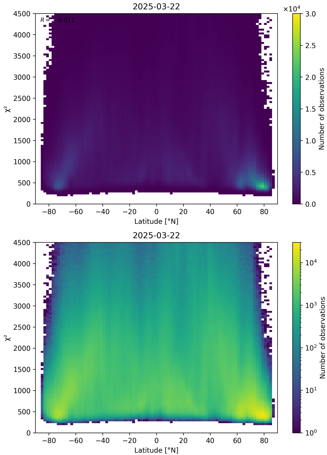
Figure 54: Scatter density plot of “Latitude” against “ \chi^2 ” for 2025-03-21 to 2025-03-23.
