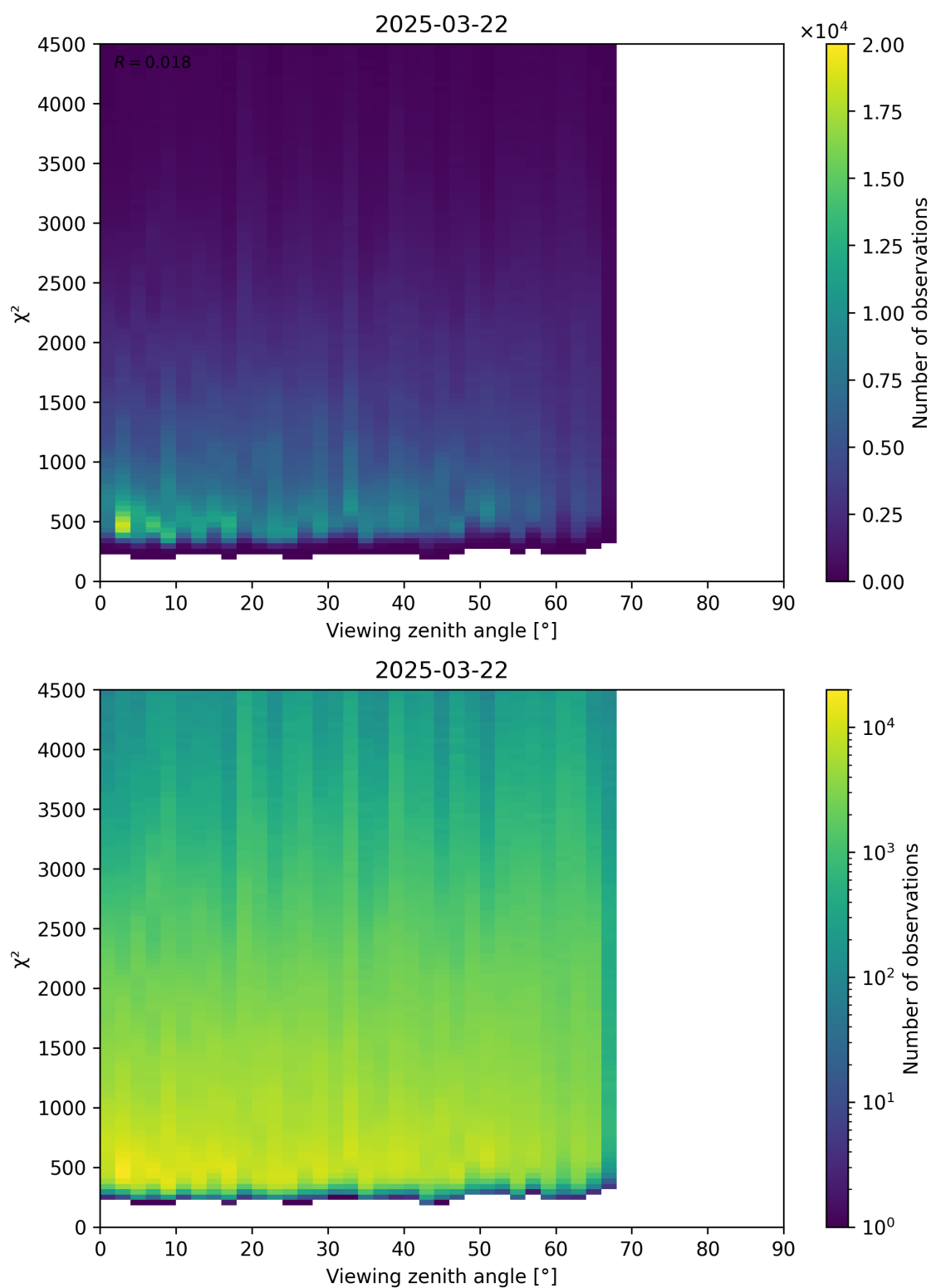
Figure 72: Scatter density plot of “Viewing zenith angle” against “ \chi^2 ” for 2025-03-21 to 2025-03-23.
