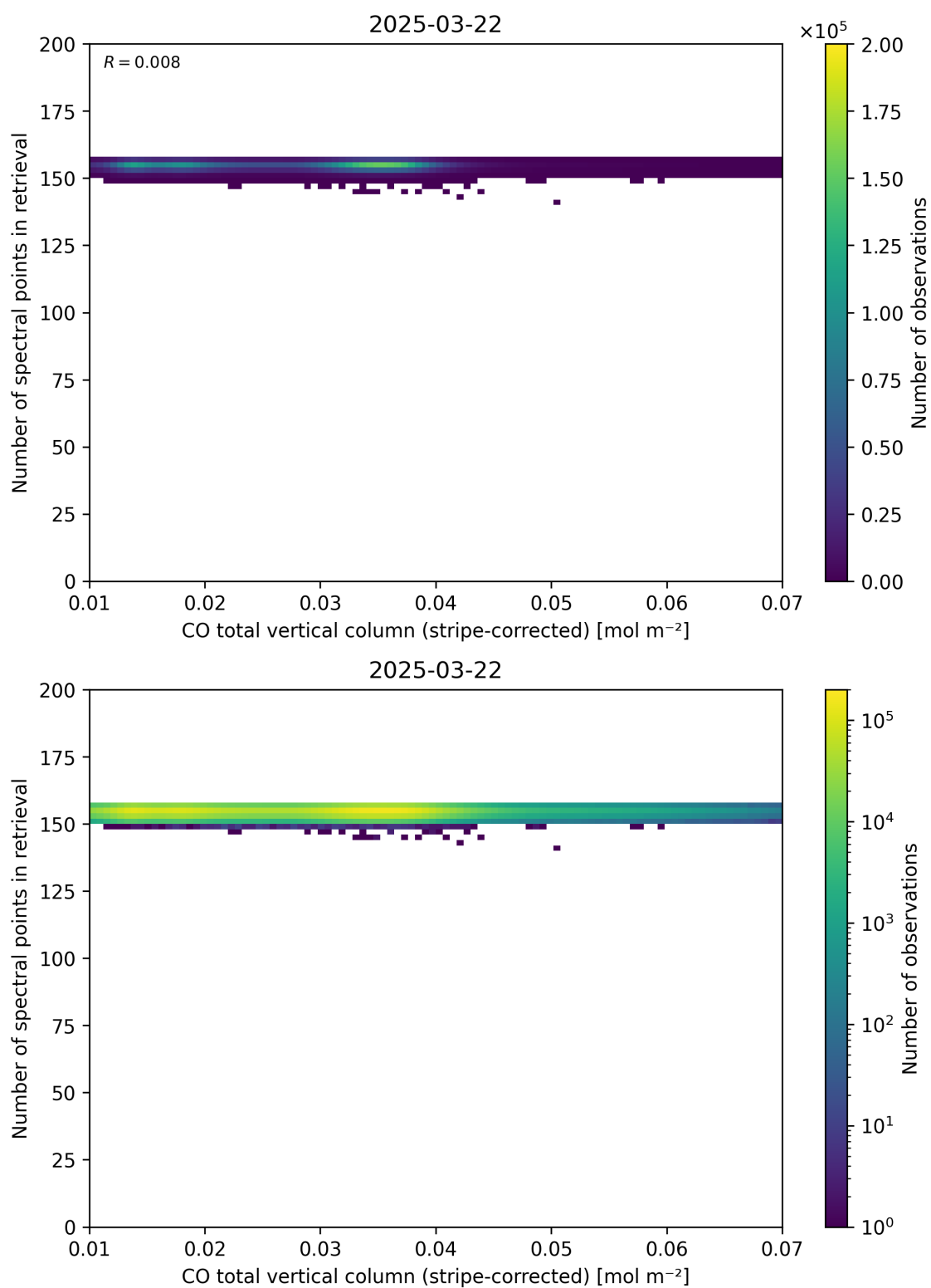
Figure 40: Scatter density plot of “CO total vertical column (stripe-corrected)” against “Number of spectral points in retrieval” for 2025-03-21 to 2025-03-23.
