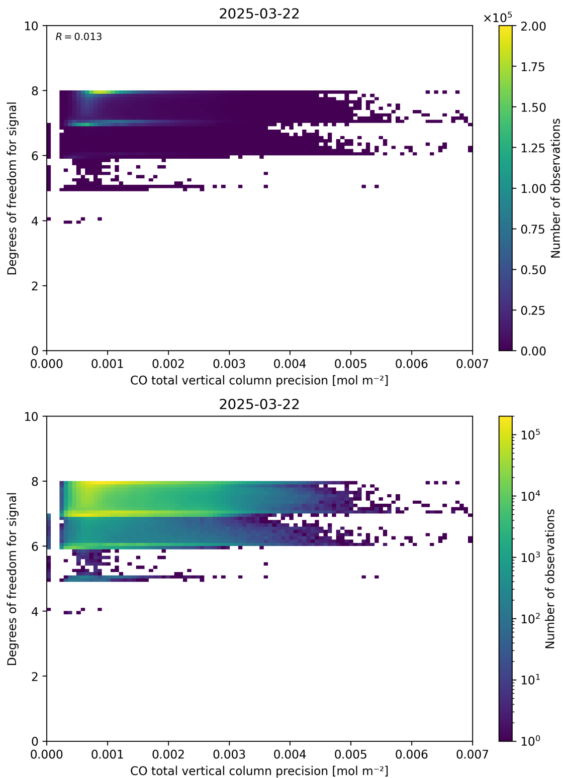
Figure 45: Scatter density plot of “CO total vertical column precision” against “Degrees of freedom for signal” for 2025-03-21 to 2025-03-23.
