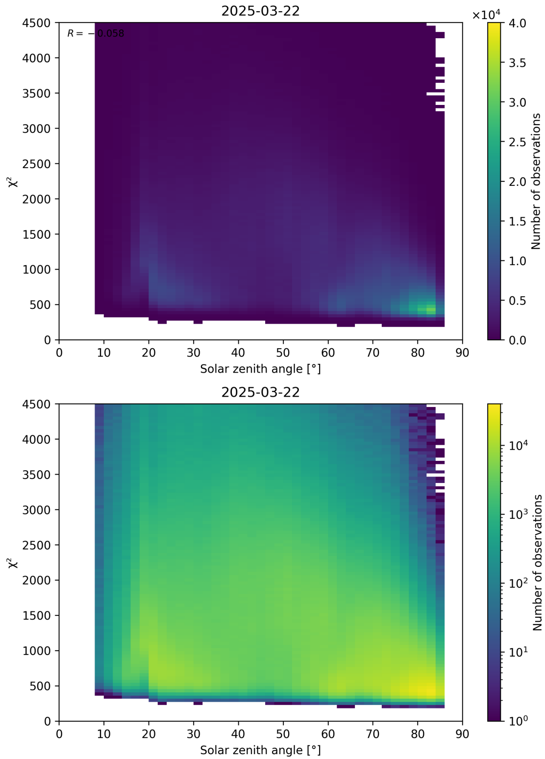
Figure 64: Scatter density plot of “Solar zenith angle” against “ \chi^2 ” for 2025-03-21 to 2025-03-23.
