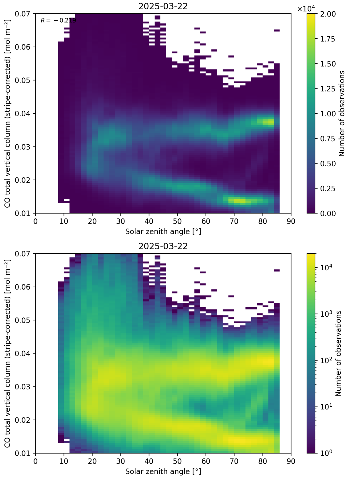
Figure 62: Scatter density plot of “Solar zenith angle” against “CO total vertical column (stripe-corrected)” for 2025-03-21 to 2025-03-23.
