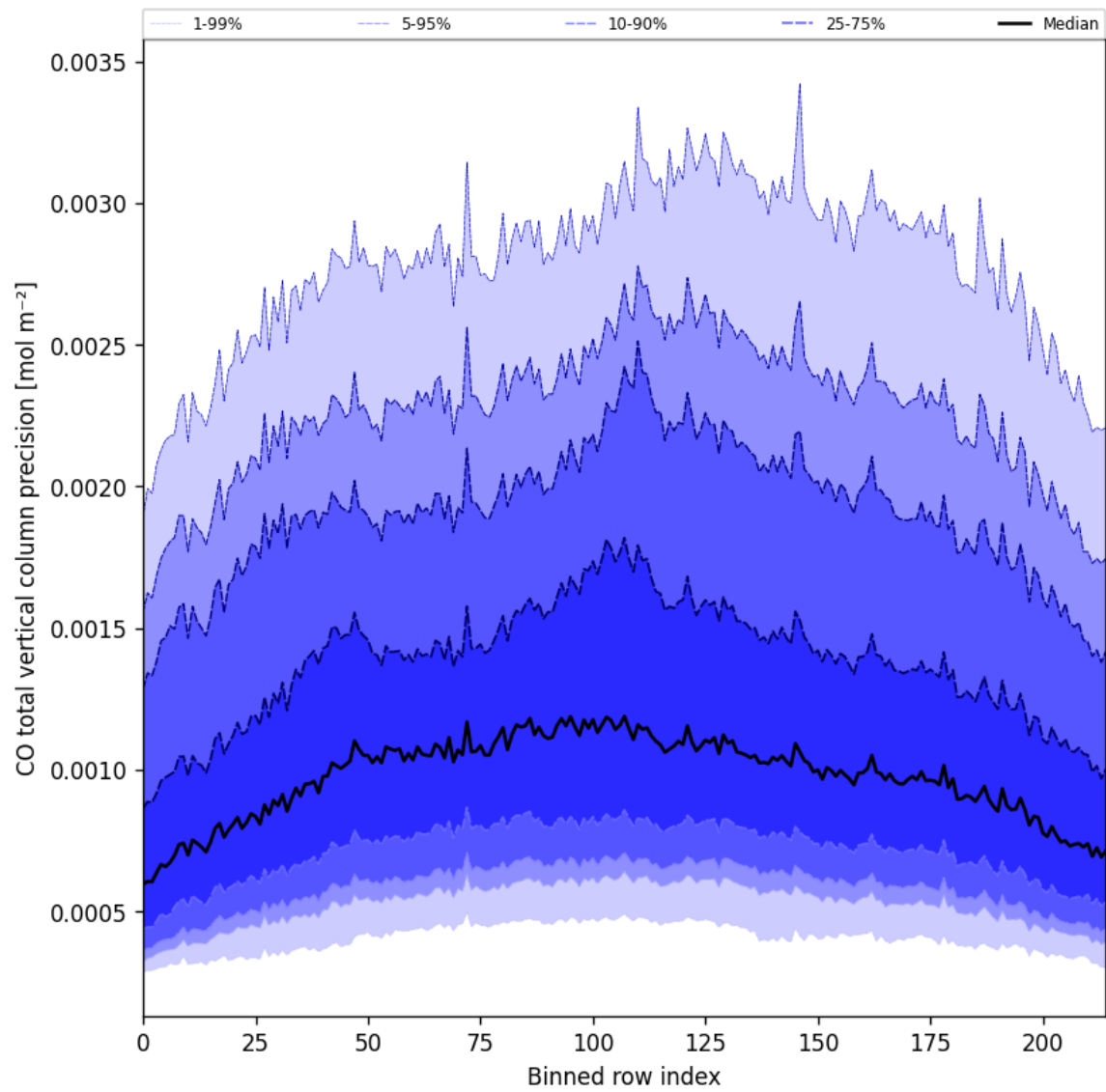
Figure 28: Along track statistics of “CO total vertical column precision” for 2025-03-21 to 2025-03-23
