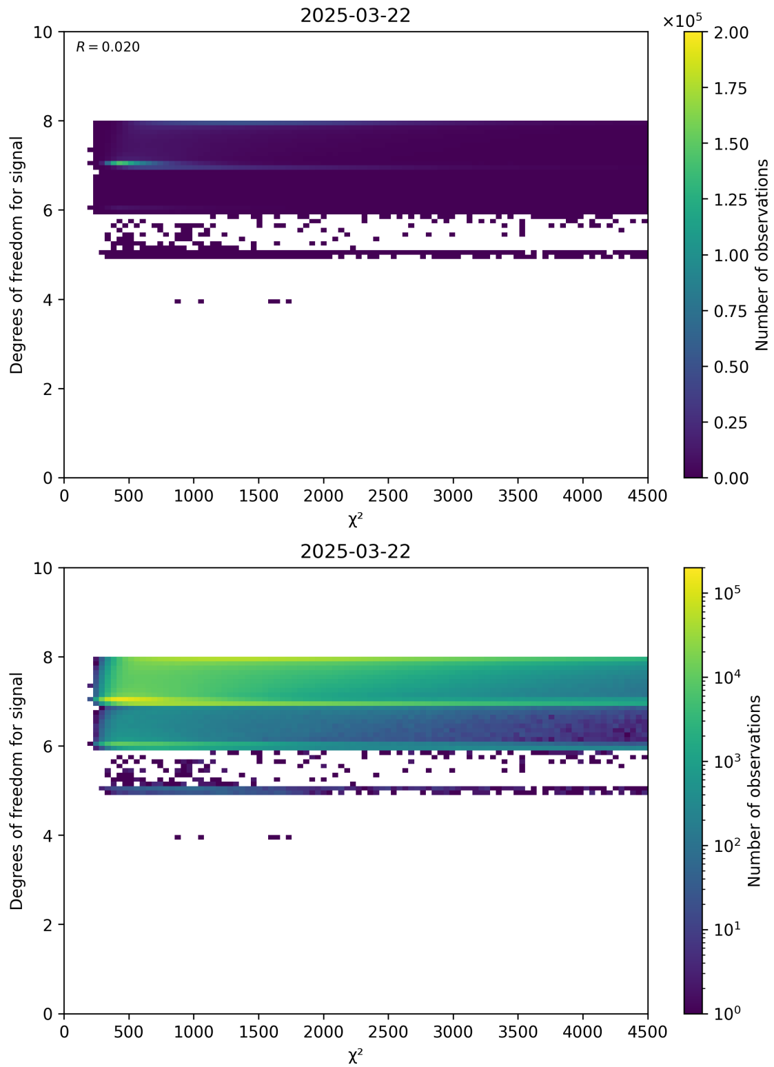
Figure 48: Scatter density plot of “ \chi^2 ” against “Degrees of freedom for signal” for 2025-03-21 to 2025-03-23.
