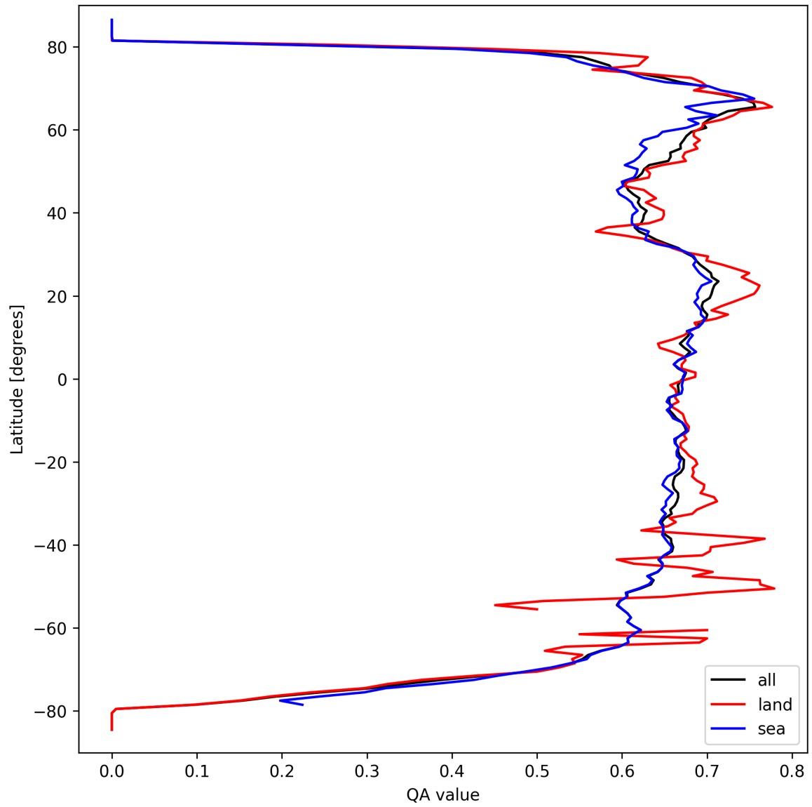
Figure 9: Zonal average of “QA value” for 2025-03-21 to 2025-03-23.
