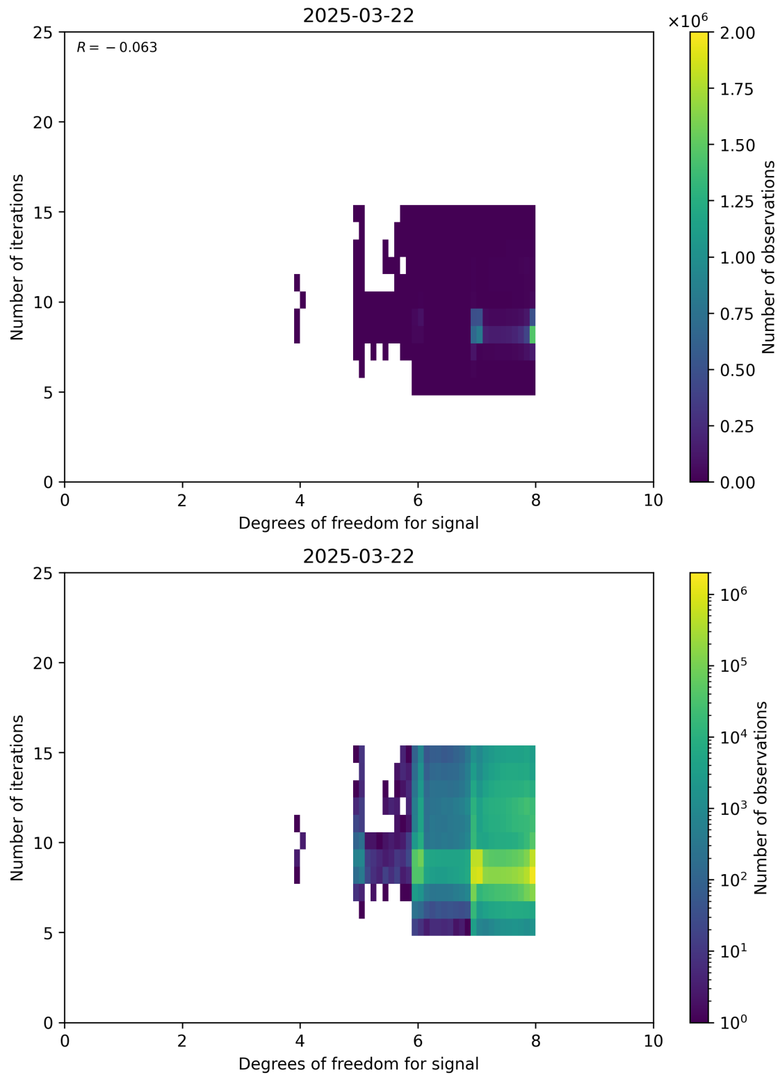
Figure 50: Scatter density plot of “Degrees of freedom for signal” against “Number of iterations” for 2025-03-21 to 2025-03-23.
