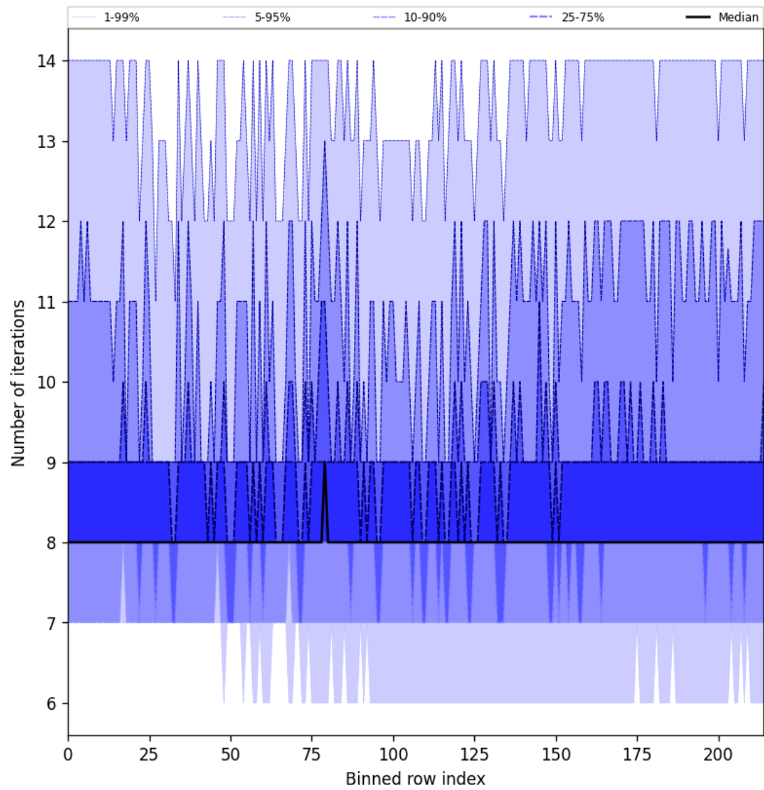
Figure 32: Along track statistics of “Number of iterations” for 2025-03-21 to 2025-03-23
