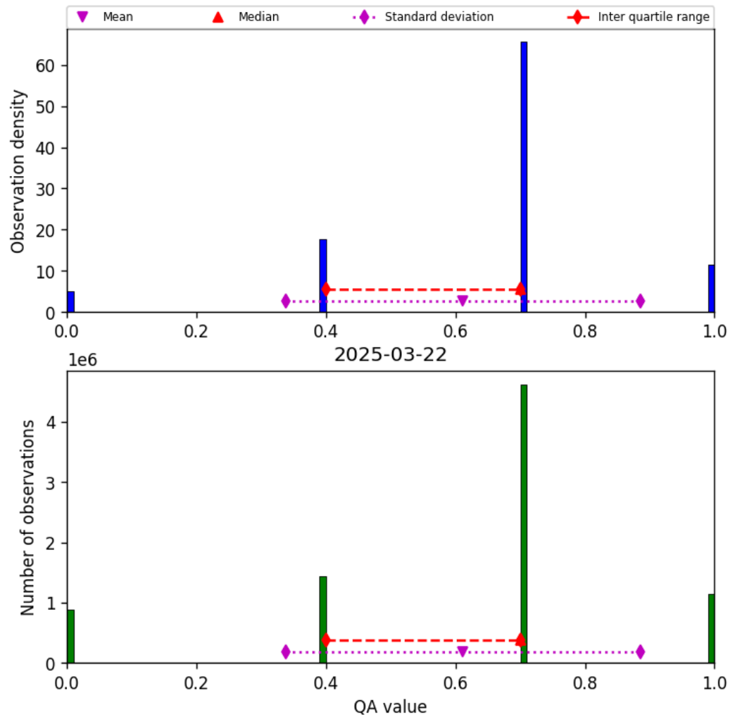
Figure 17: Histogram of “QA value” for 2025-03-21 to 2025-03-23
