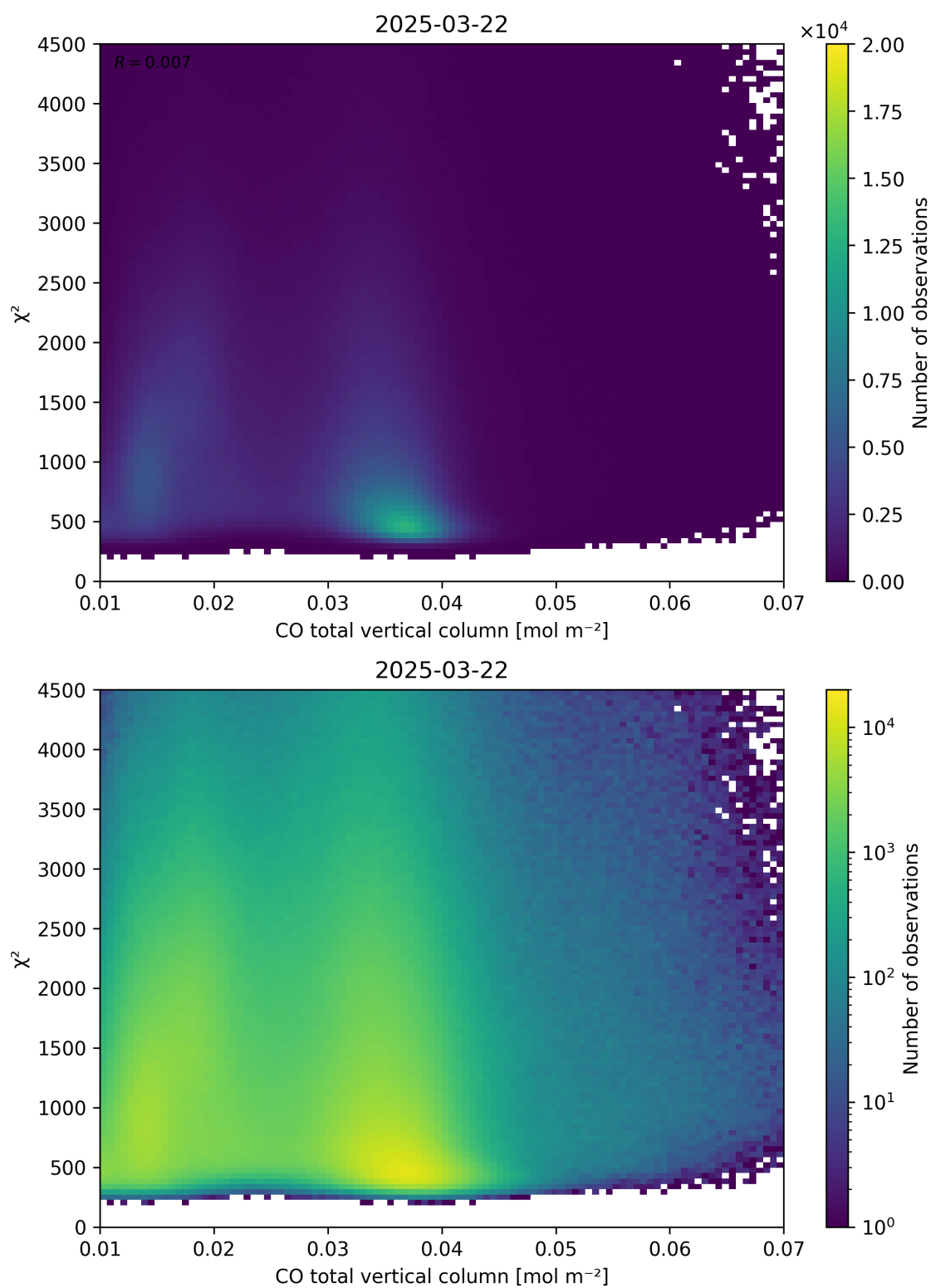
Figure 35: Scatter density plot of “CO total vertical column” against “ \chi^2 ” for 2025-03-21 to 2025-03-23.
