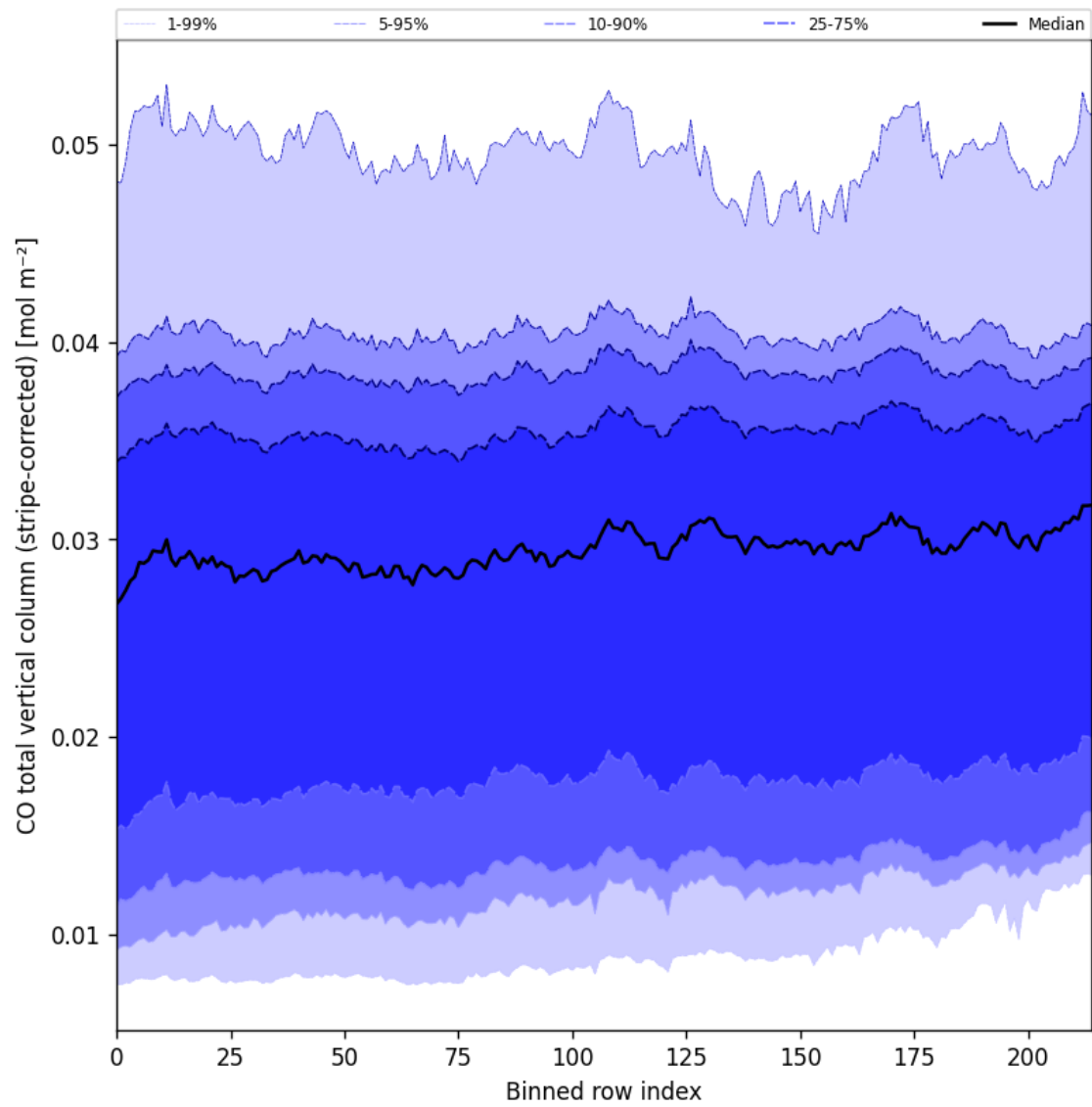
Figure 27: Along track statistics of “CO total vertical column (stripe-corrected)” for 2025-03-21 to 2025-03-23
