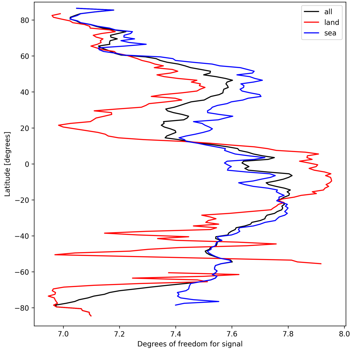
Figure 15: Zonal average of “Degrees of freedom for signal” for 2025-03-21 to 2025-03-23.
