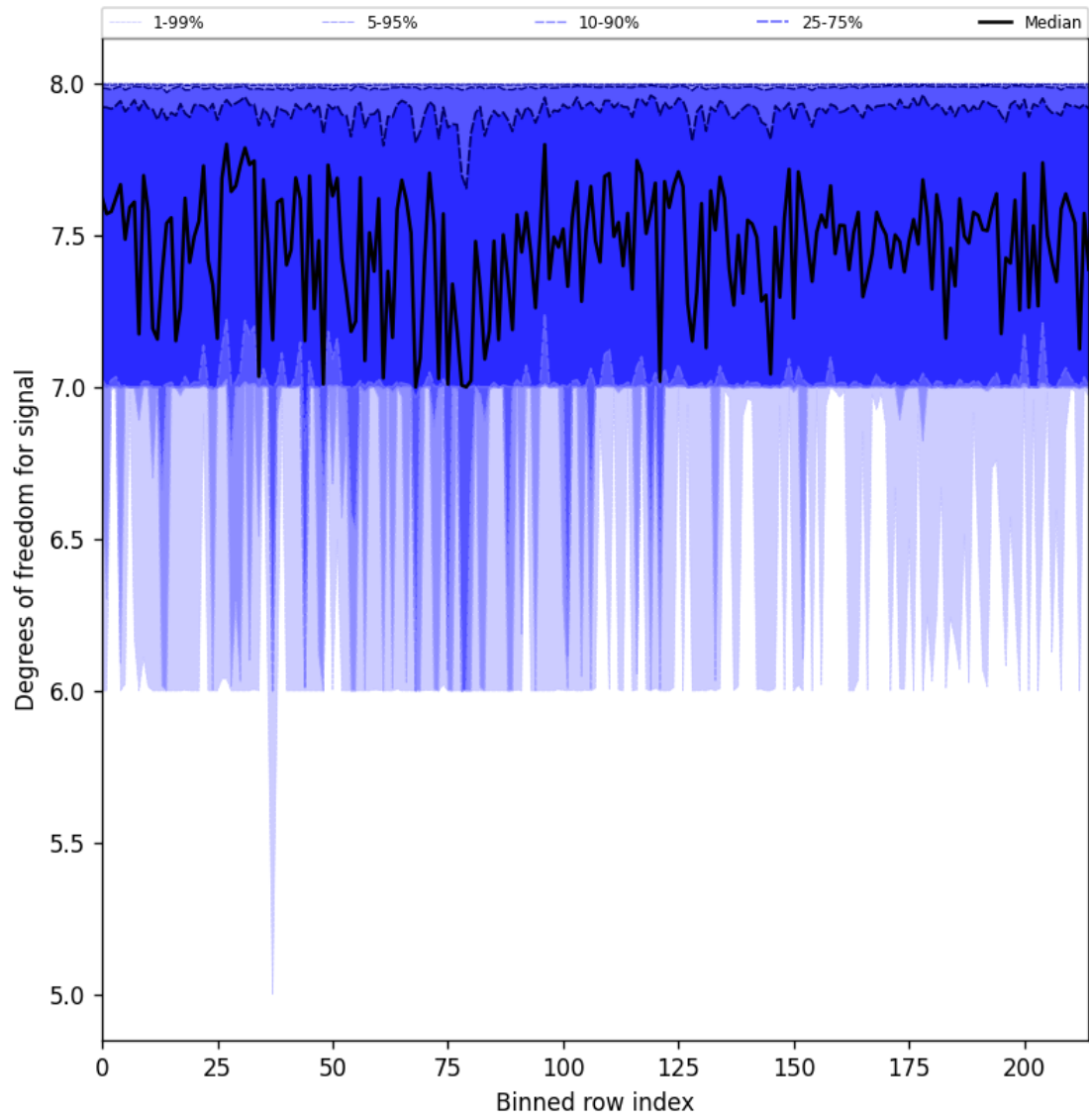
Figure 31: Along track statistics of “Degrees of freedom for signal” for 2025-03-21 to 2025-03-23
