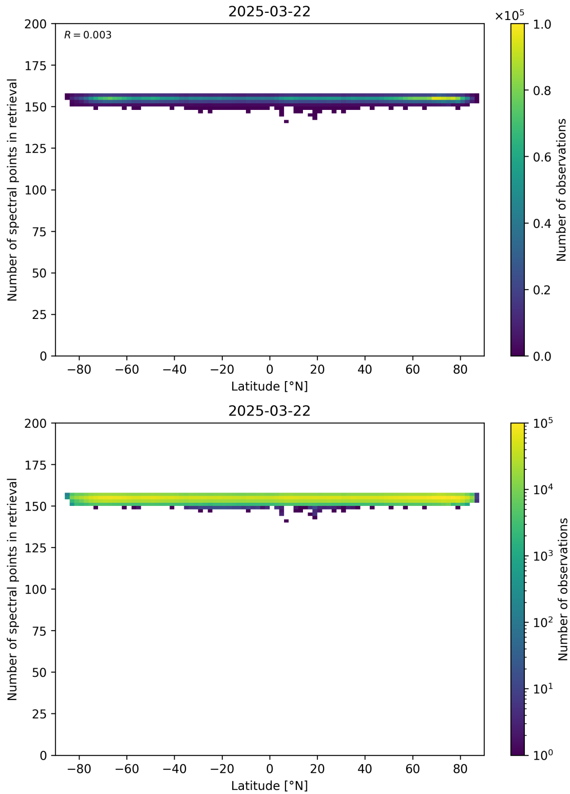
Figure 57: Scatter density plot of “Latitude” against “Number of spectral points in retrieval” for 2025-03-21 to 2025-03-23.
