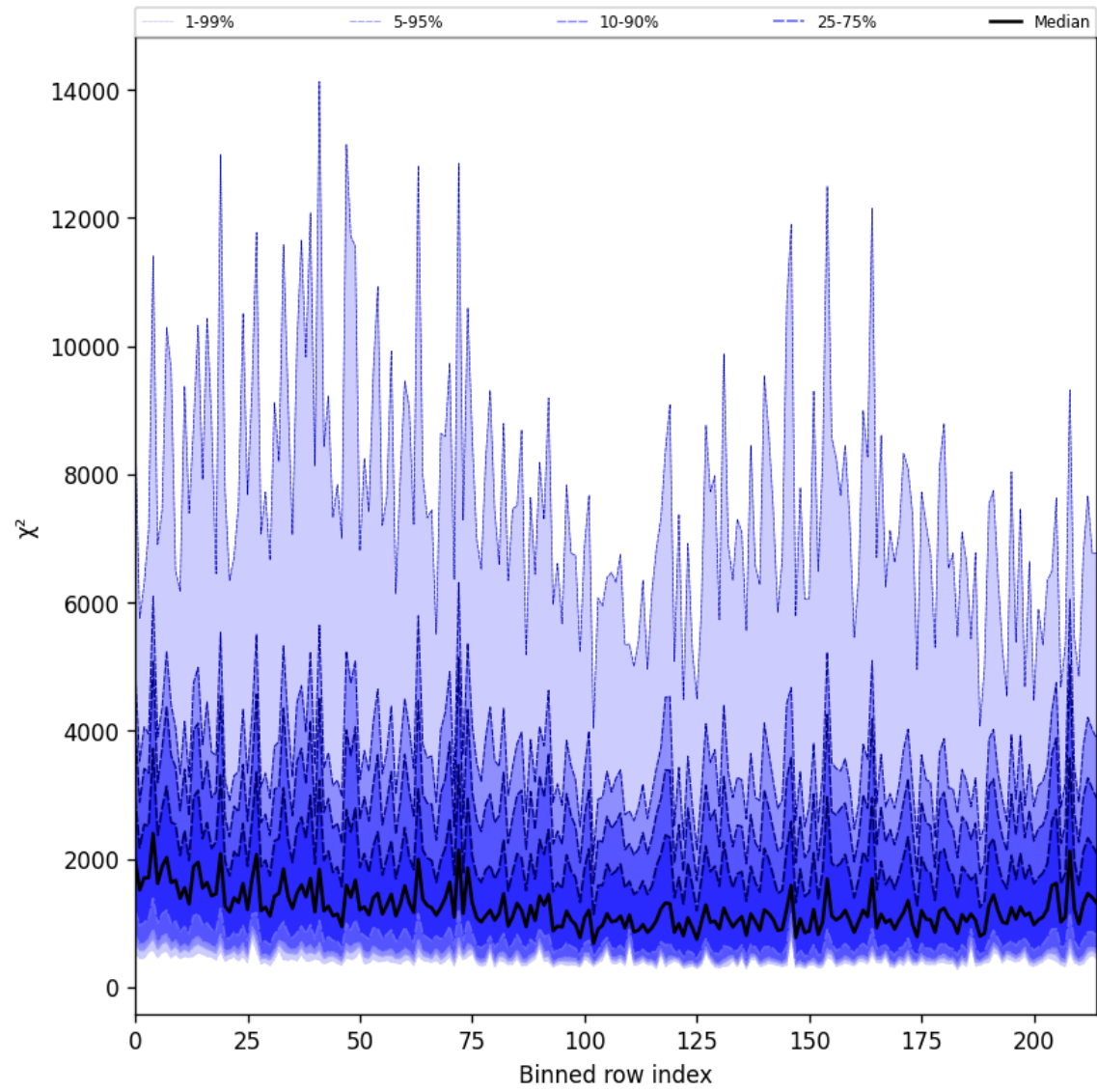
Figure 30: Along track statistics of “ \chi^2 ” for 2025-03-21 to 2025-03-23
