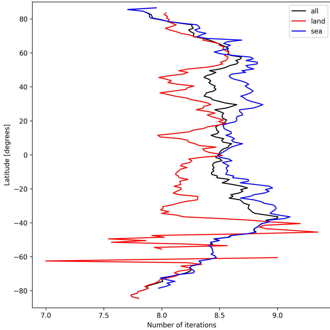
Figure 16: Zonal average of “Number of iterations” for 2025-03-21 to 2025-03-23.
