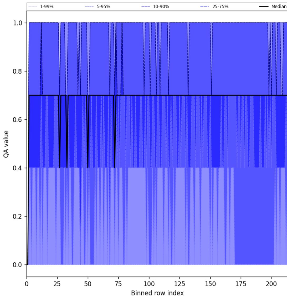
Figure 25: Along track statistics of “QA value” for 2025-03-21 to 2025-03-23
