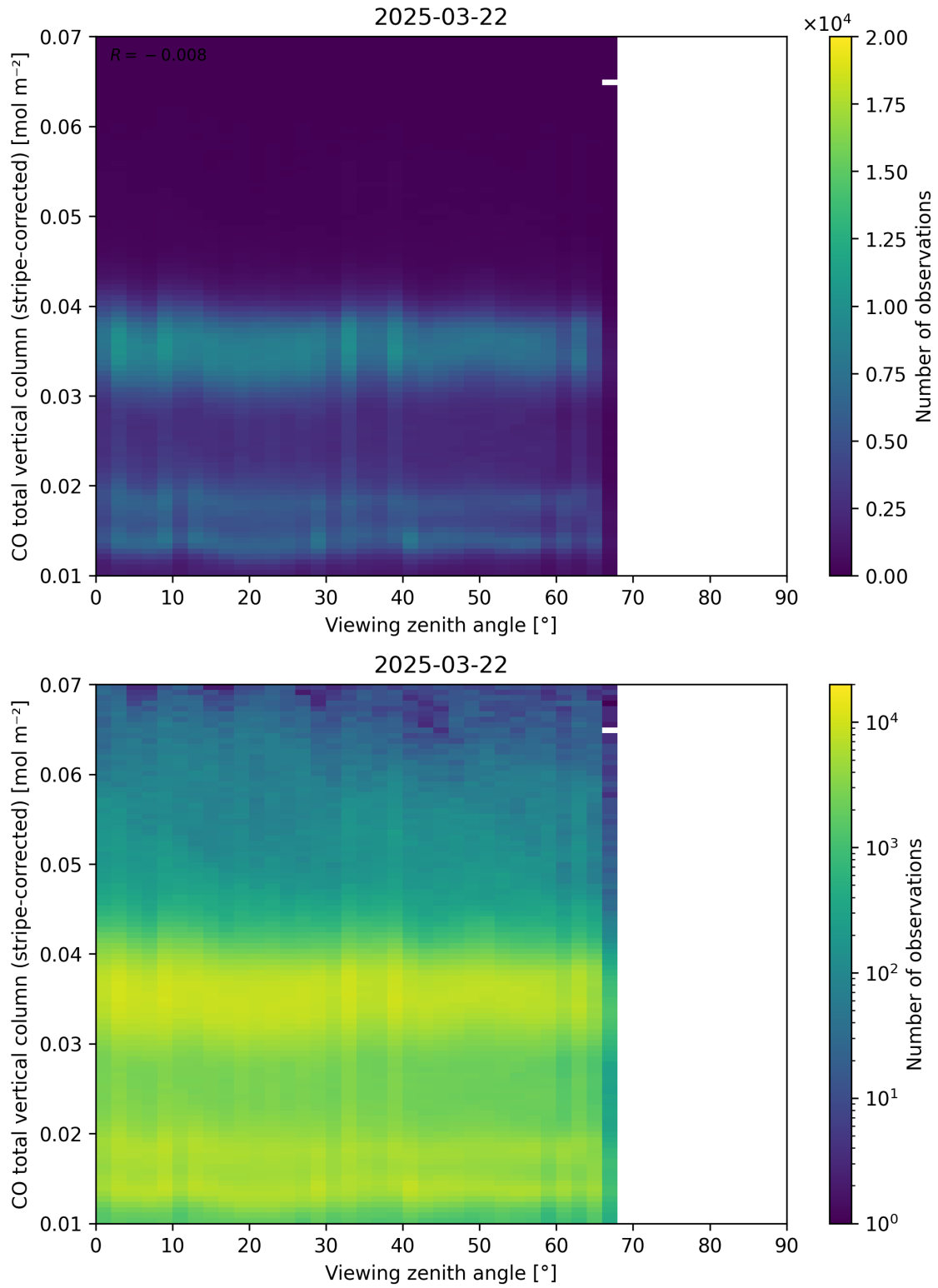
Figure 70: Scatter density plot of “Viewing zenith angle” against “CO total vertical column (stripe-corrected)” for 2025-03-21 to 2025-03-23.
