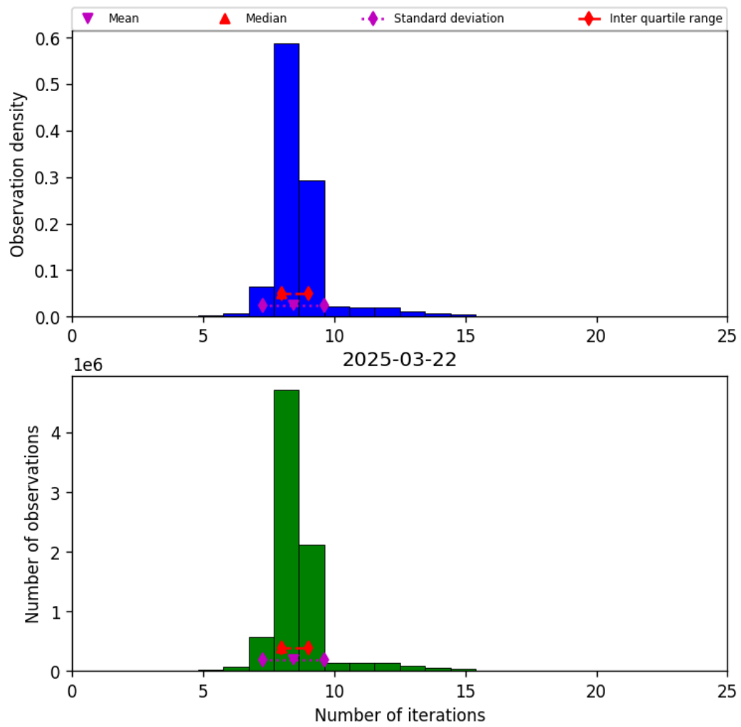
Figure 24: Histogram of “Number of iterations” for 2025-03-21 to 2025-03-23
