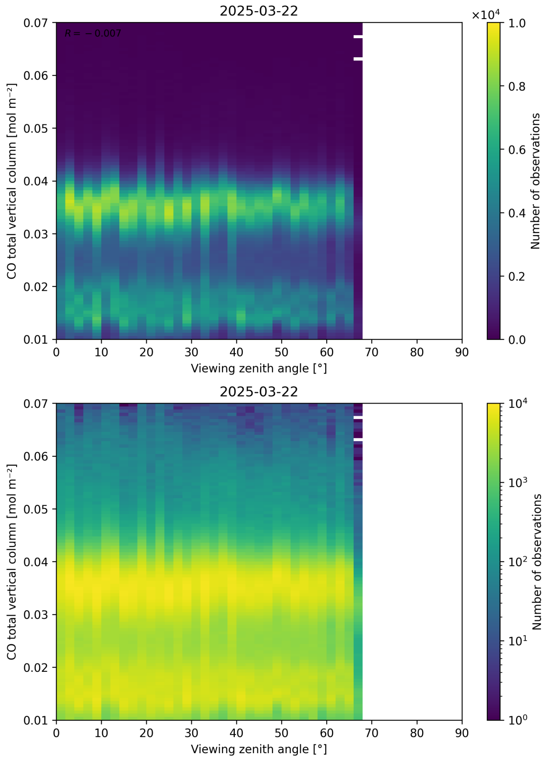
Figure 69: Scatter density plot of “Viewing zenith angle” against “CO total vertical column” for 2025-03-21 to 2025-03-23.
