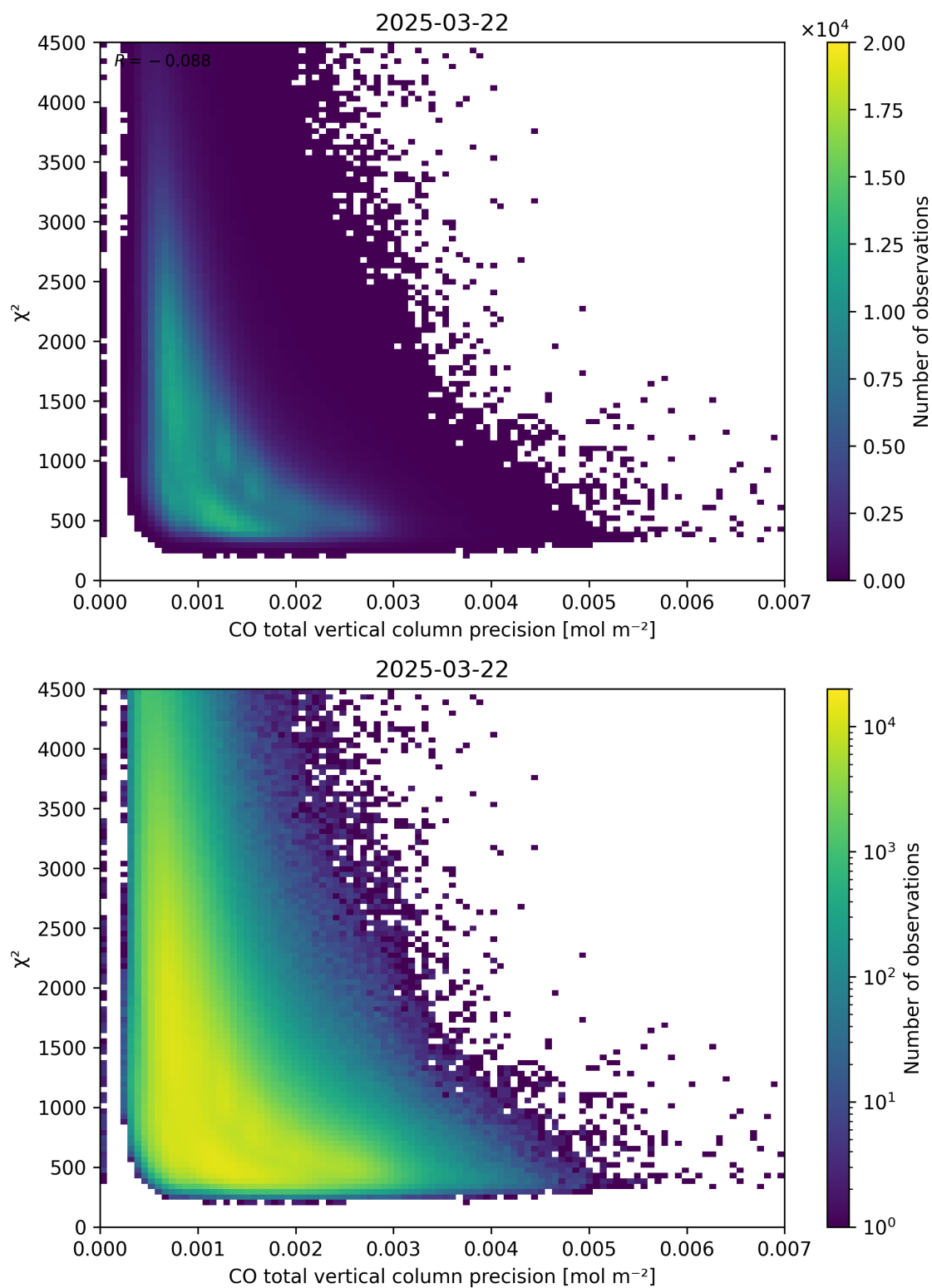
Figure 44: Scatter density plot of “CO total vertical column precision” against “ \chi^2 ” for 2025-03-21 to 2025-03-23.
