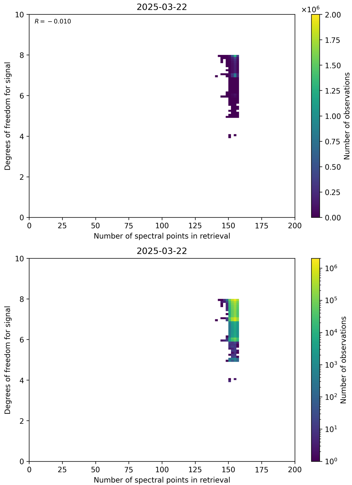
Figure 59: Scatter density plot of “Number of spectral points in retrieval” against “Degrees of freedom for signal” for 2025-03-21 to 2025-03-23.
