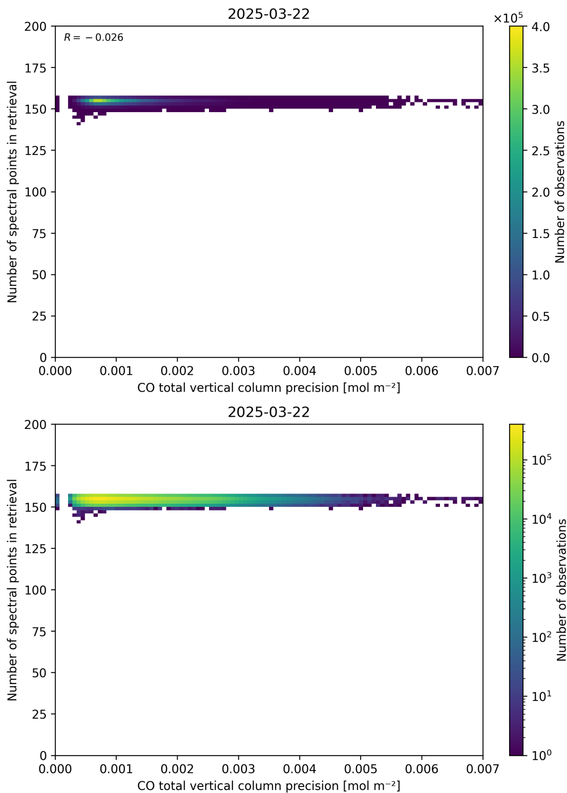
Figure 47: Scatter density plot of “CO total vertical column precision” against “Number of spectral points in retrieval” for 2025-03-21 to 2025-03-23.
