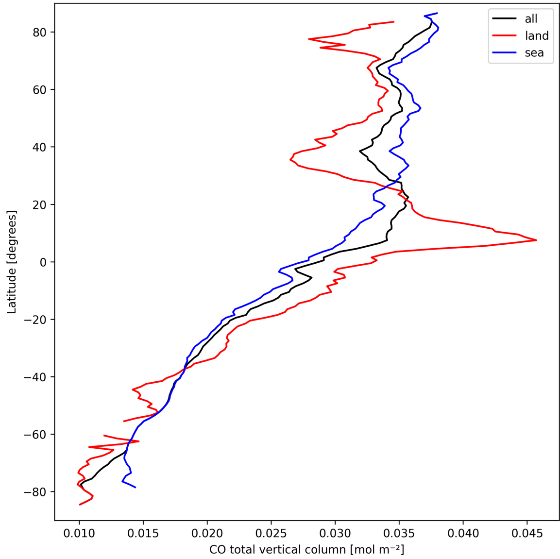
Figure 10: Zonal average of “CO total vertical column” for 2025-03-21 to 2025-03-23.
