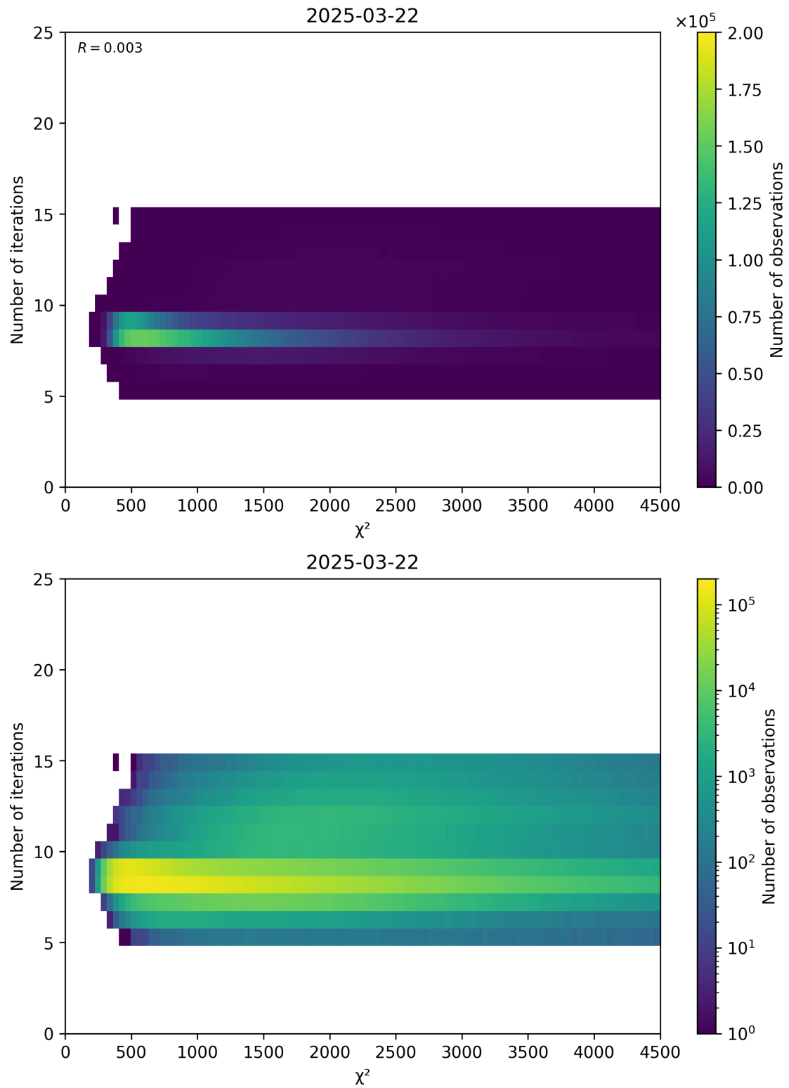
Figure 49: Scatter density plot of “ \chi^2 ” against “Number of iterations” for 2025-03-21 to 2025-03-23.
