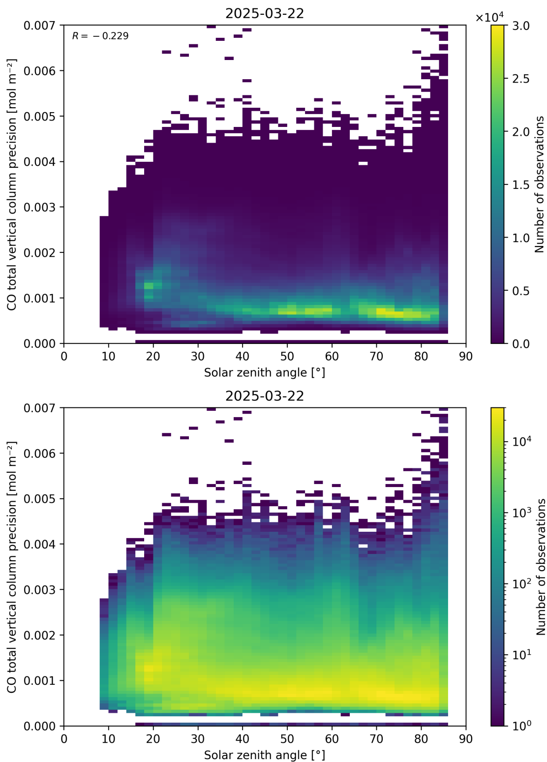
Figure 63: Scatter density plot of “Solar zenith angle” against “CO total vertical column precision” for 2025-03-21 to 2025-03-23.
