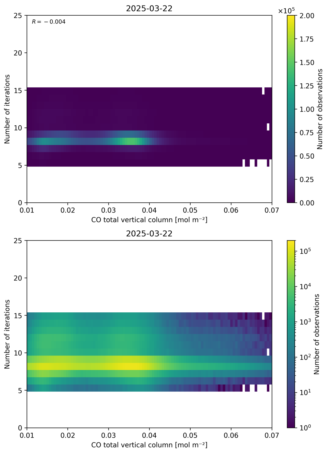
Figure 42: Scatter density plot of “CO total vertical column” against “Number of iterations” for 2025-03-21 to 2025-03-23.
