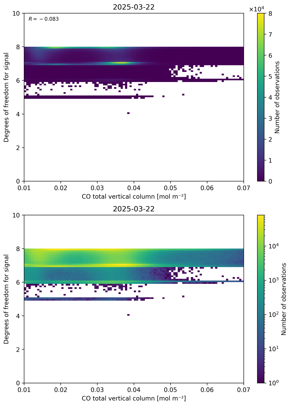
Figure 41: Scatter density plot of “CO total vertical column” against “Degrees of freedom for signal” for 2025-03-21 to 2025-03-23.
