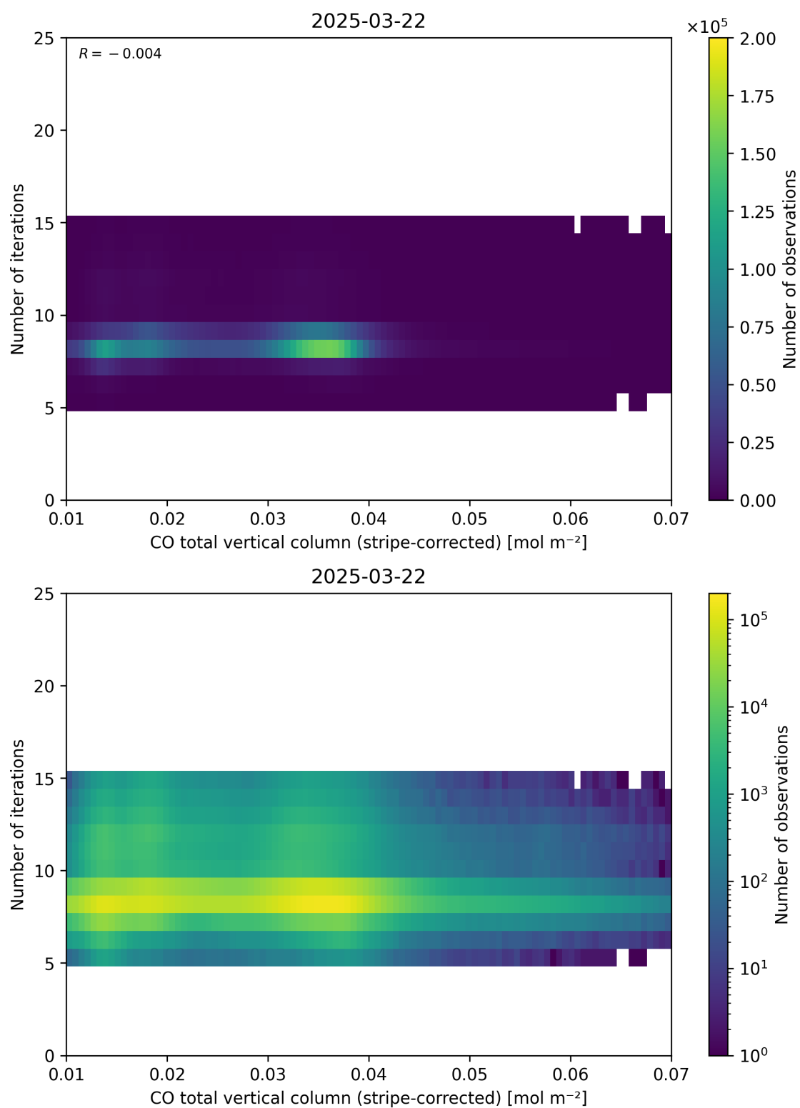
Figure 39: Scatter density plot of “CO total vertical column (stripe-corrected)” against “Number of iterations” for 2025-03-21 to 2025-03-23.
