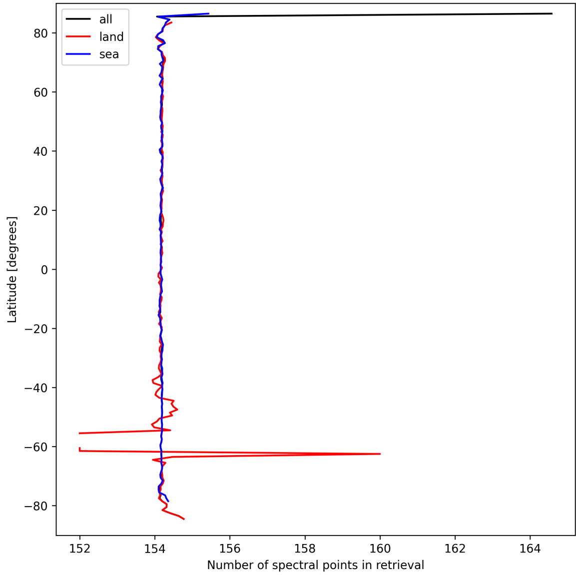
Figure 13: Zonal average of “Number of spectral points in retrieval” for 2025-03-21 to 2025-03-23.
