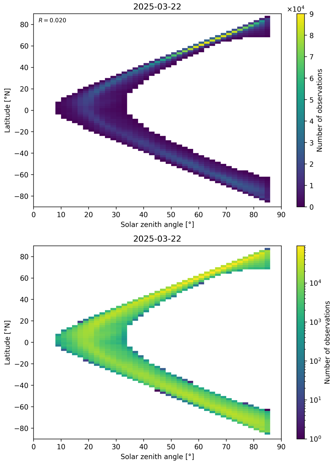
Figure 66: Scatter density plot of “Solar zenith angle” against “Latitude” for 2025-03-21 to 2025-03-23.
