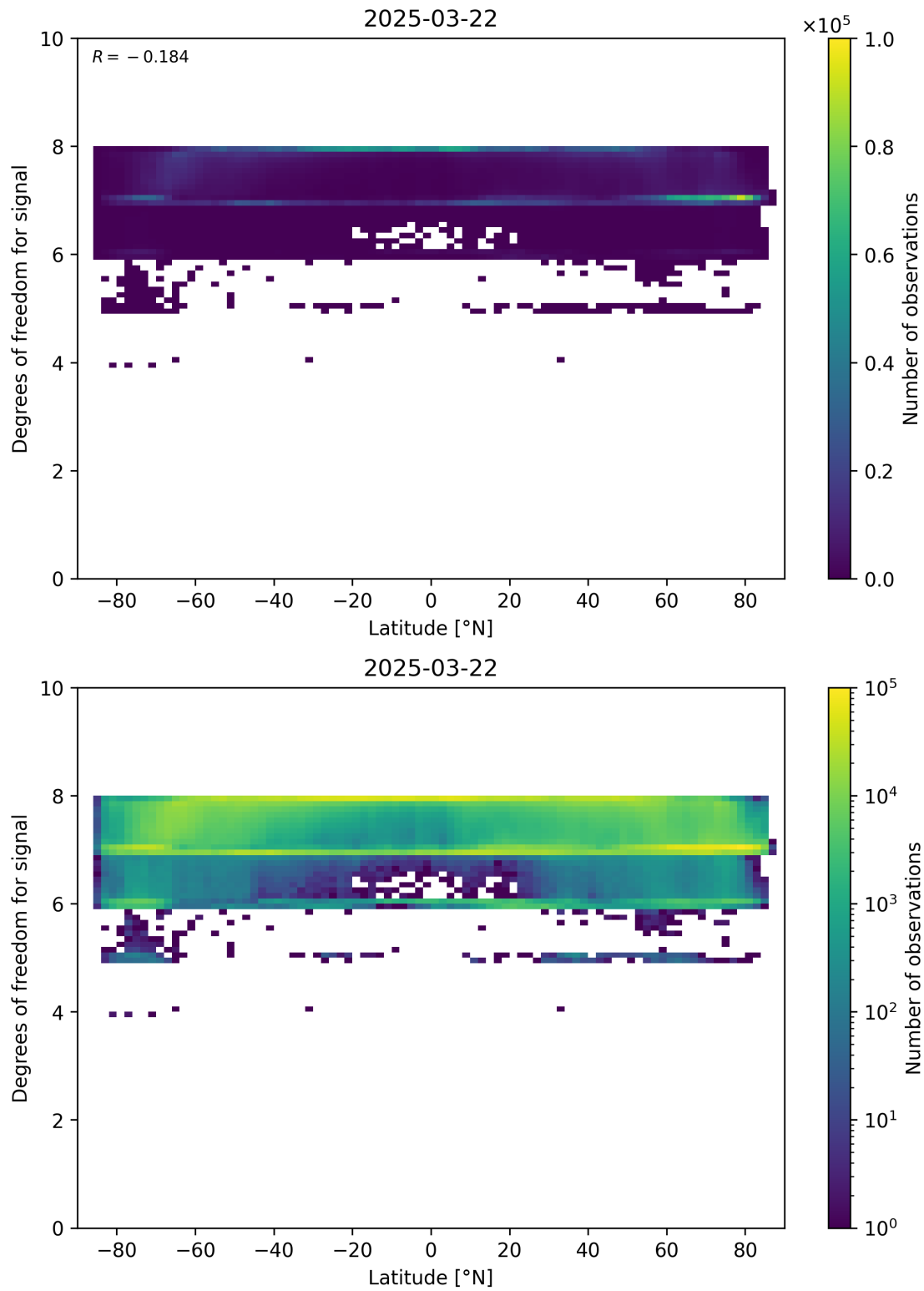
Figure 55: Scatter density plot of “Latitude” against “Degrees of freedom for signal” for 2025-03-21 to 2025-03-23.
