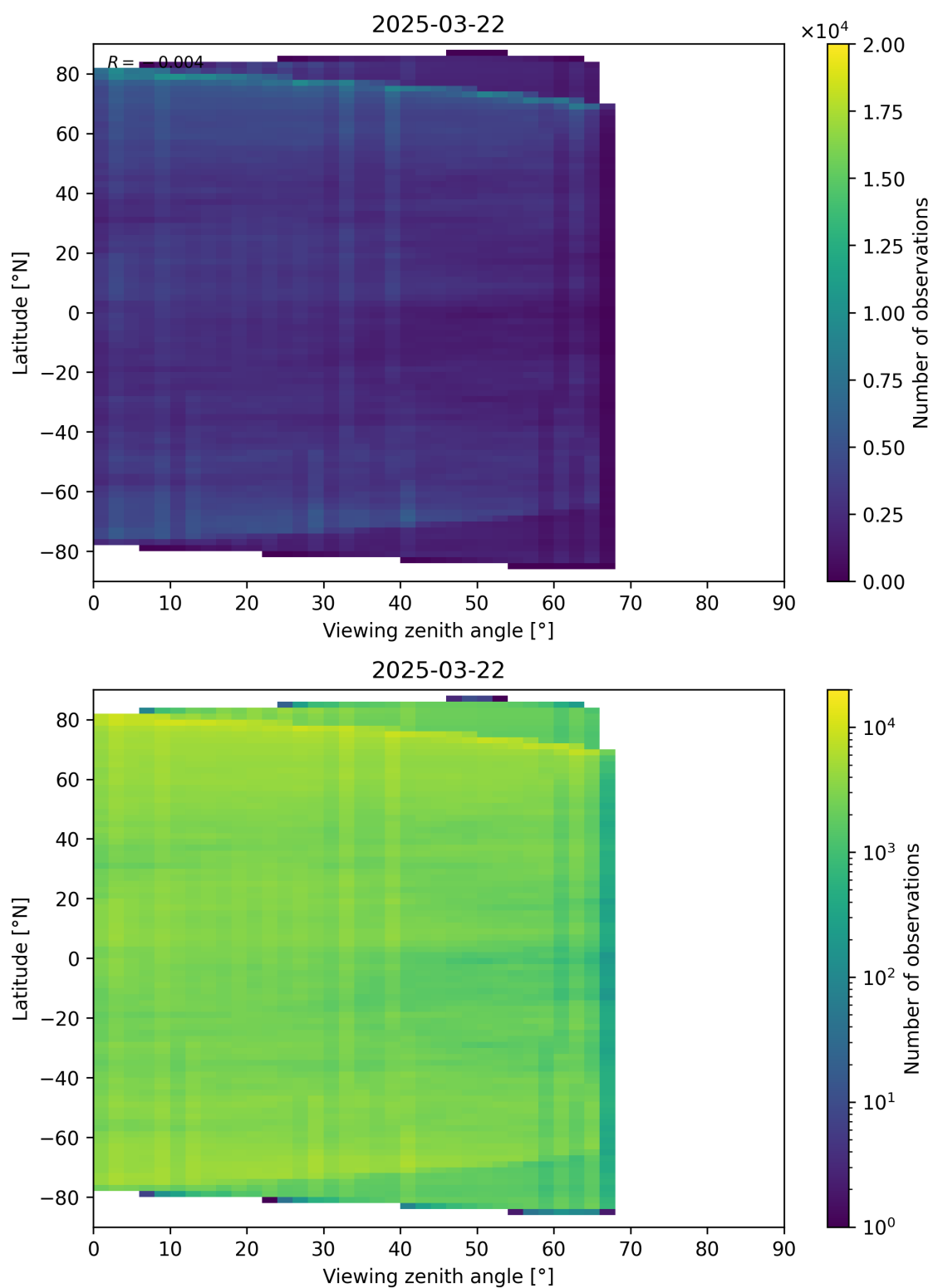
Figure 74: Scatter density plot of “Viewing zenith angle” against “Latitude” for 2025-03-21 to 2025-03-23.
