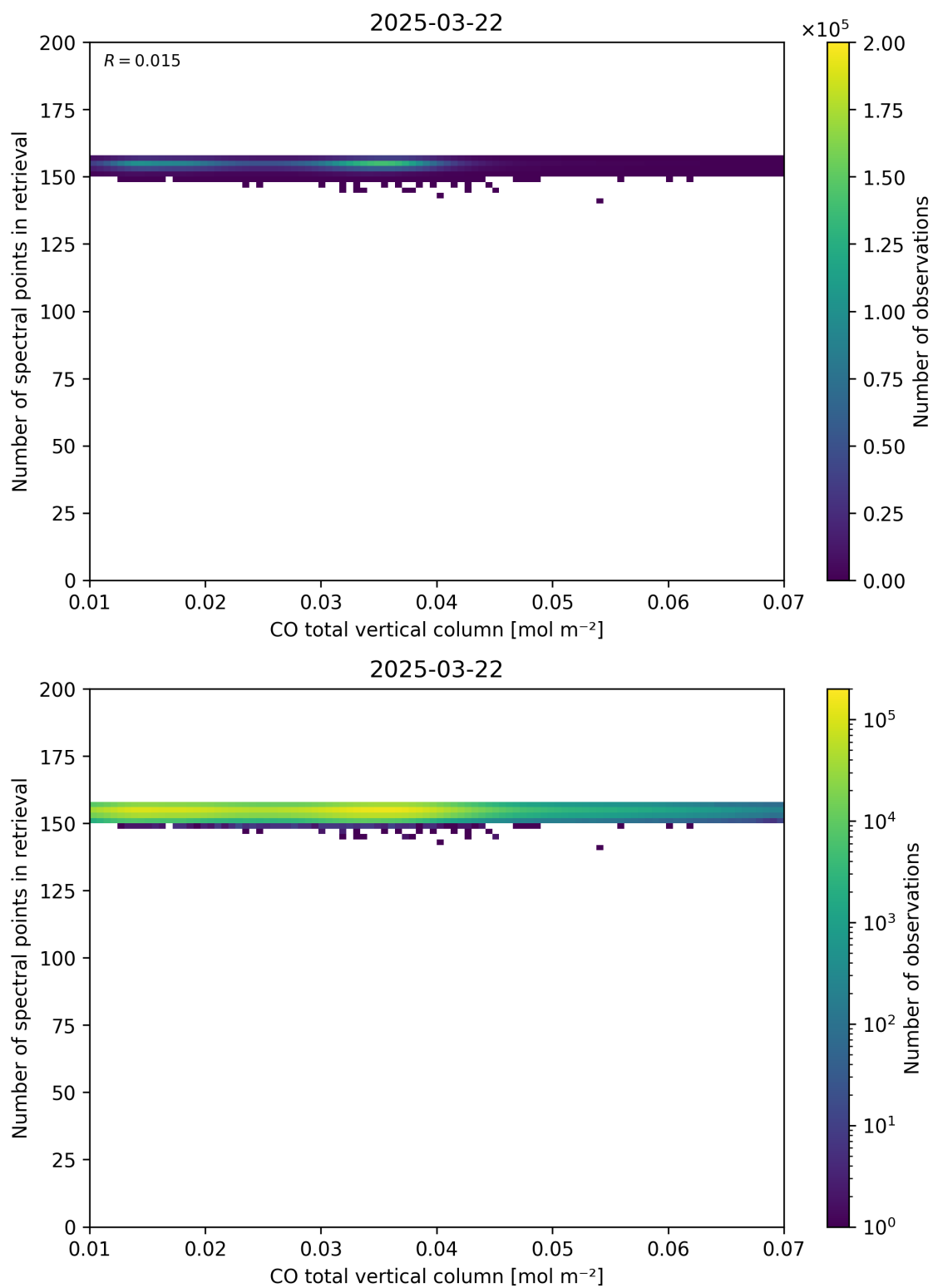
Figure 43: Scatter density plot of “CO total vertical column” against “Number of spectral points in retrieval” for 2025-03-21 to 2025-03-23.
