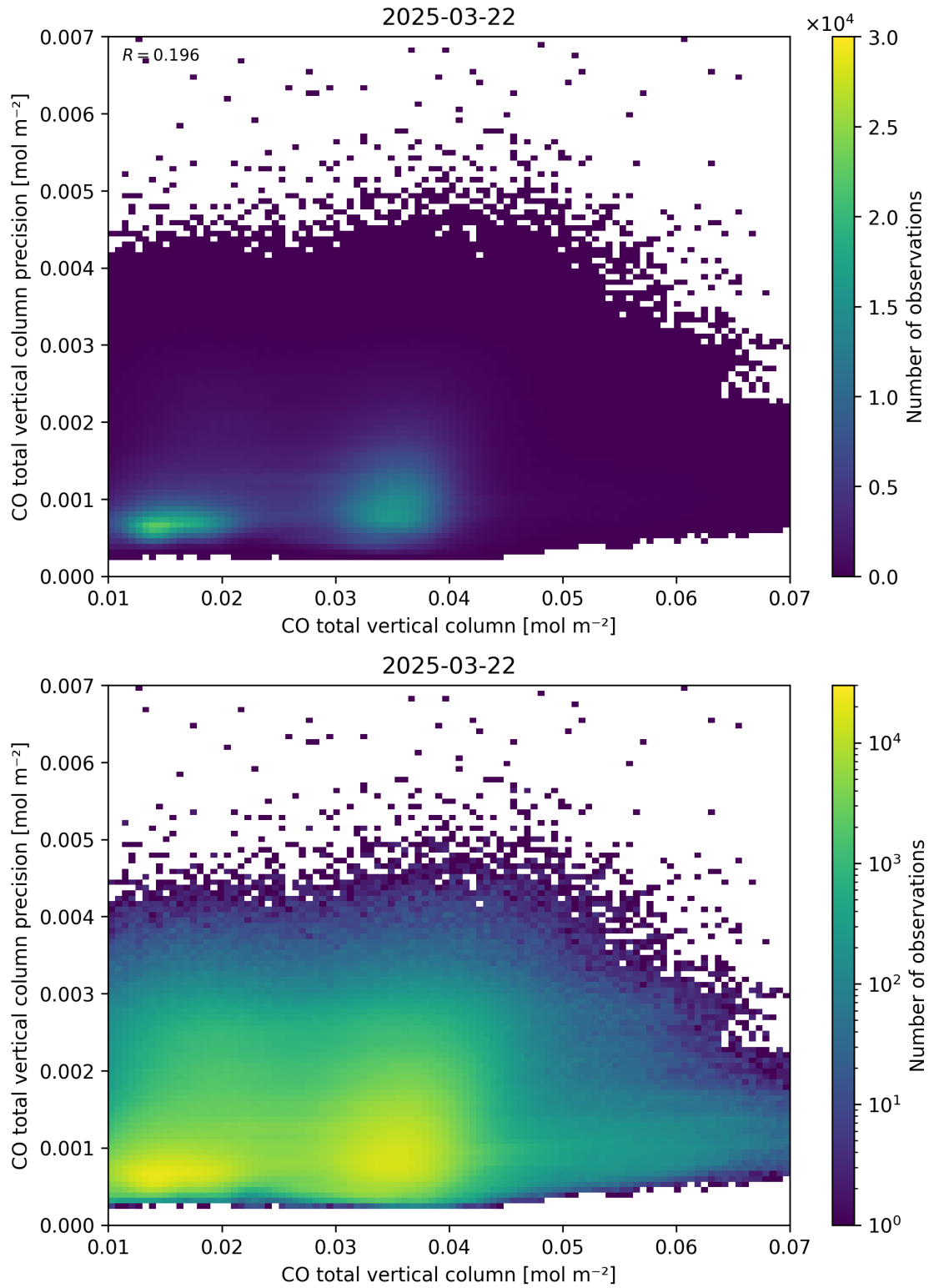
Figure 34: Scatter density plot of “CO total vertical column” against “CO total vertical column precision” for 2025-03-21 to 2025-03-23.
