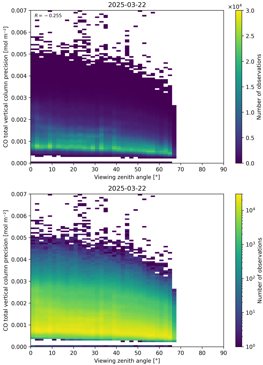
Figure 71: Scatter density plot of “Viewing zenith angle” against “CO total vertical column precision” for 2025-03-21 to 2025-03-23.
