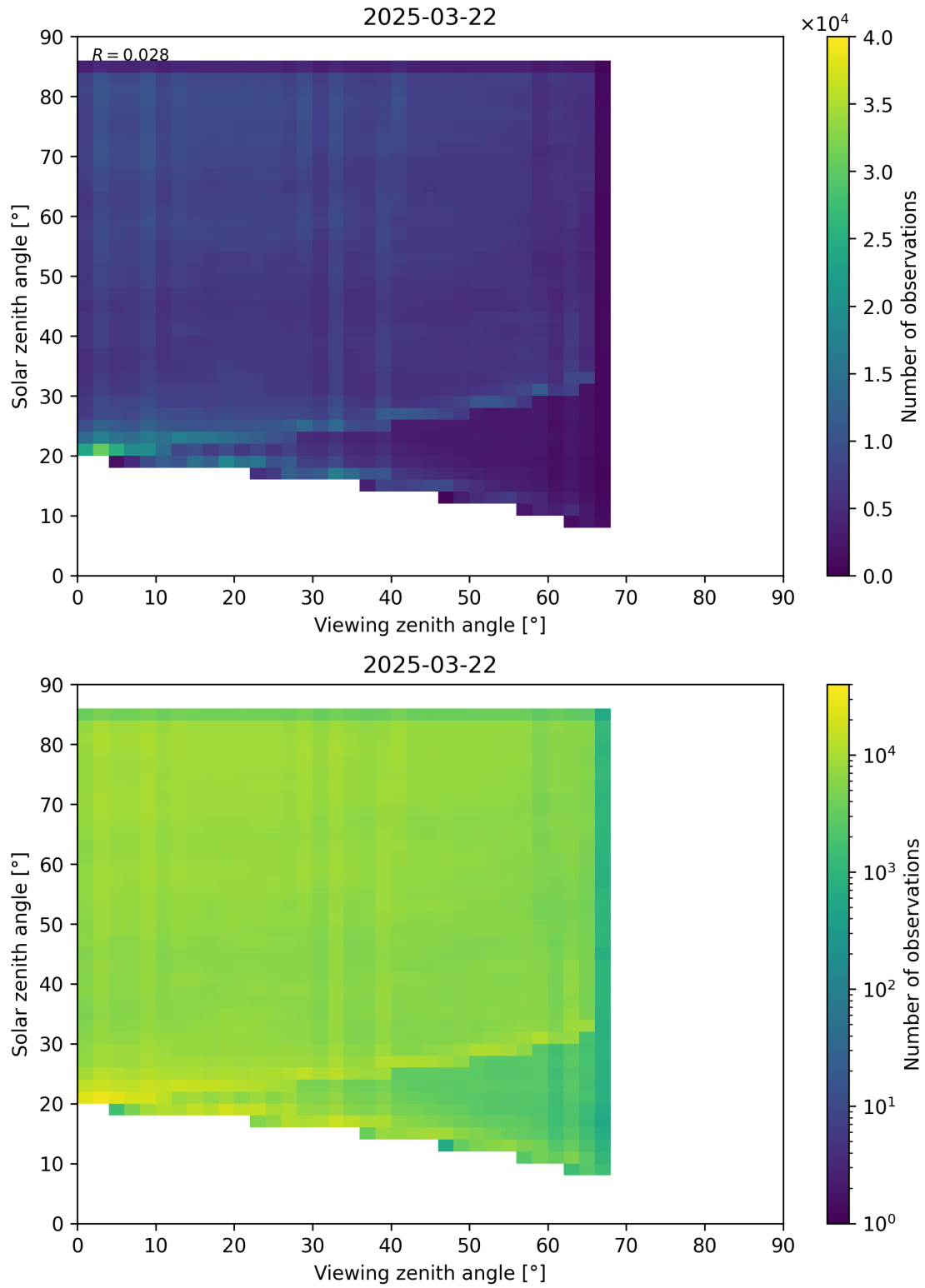
Figure 77: Scatter density plot of “Viewing zenith angle” against “Solar zenith angle” for 2025-03-21 to 2025-03-23.
