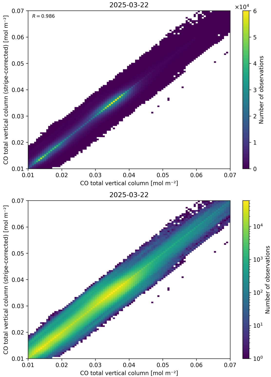
Figure 33: Scatter density plot of “CO total vertical column” against “CO total vertical column (stripe-corrected)” for 2025-03-21 to 2025-03-23.
