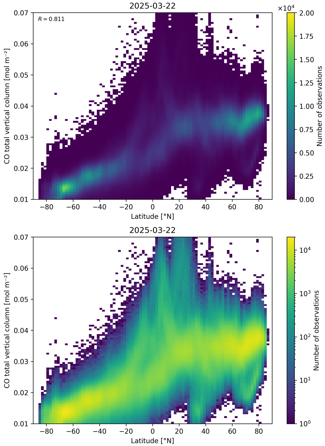
Figure 51: Scatter density plot of “Latitude” against “CO total vertical column” for 2025-03-21 to 2025-03-23.
