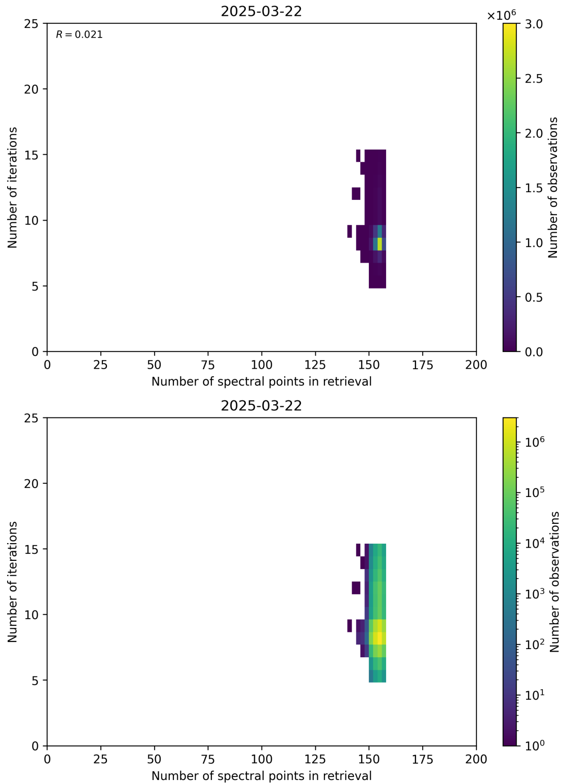
Figure 60: Scatter density plot of “Number of spectral points in retrieval” against “Number of iterations” for 2025-03-21 to 2025-03-23.
