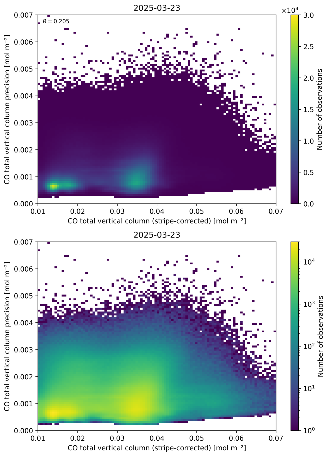
Figure 36: Scatter density plot of “CO total vertical column (stripe-corrected)” against “CO total vertical column precision” for 2025-03-23 to 2025-03-24.
