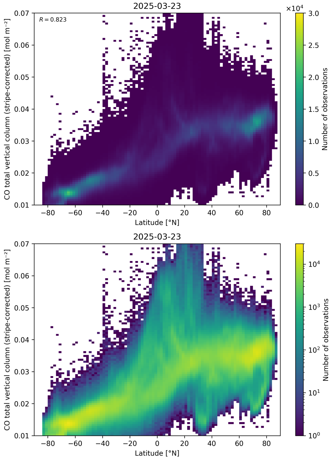
Figure 52: Scatter density plot of “Latitude” against “CO total vertical column (stripe-corrected)” for 2025-03-23 to 2025-03-24.
