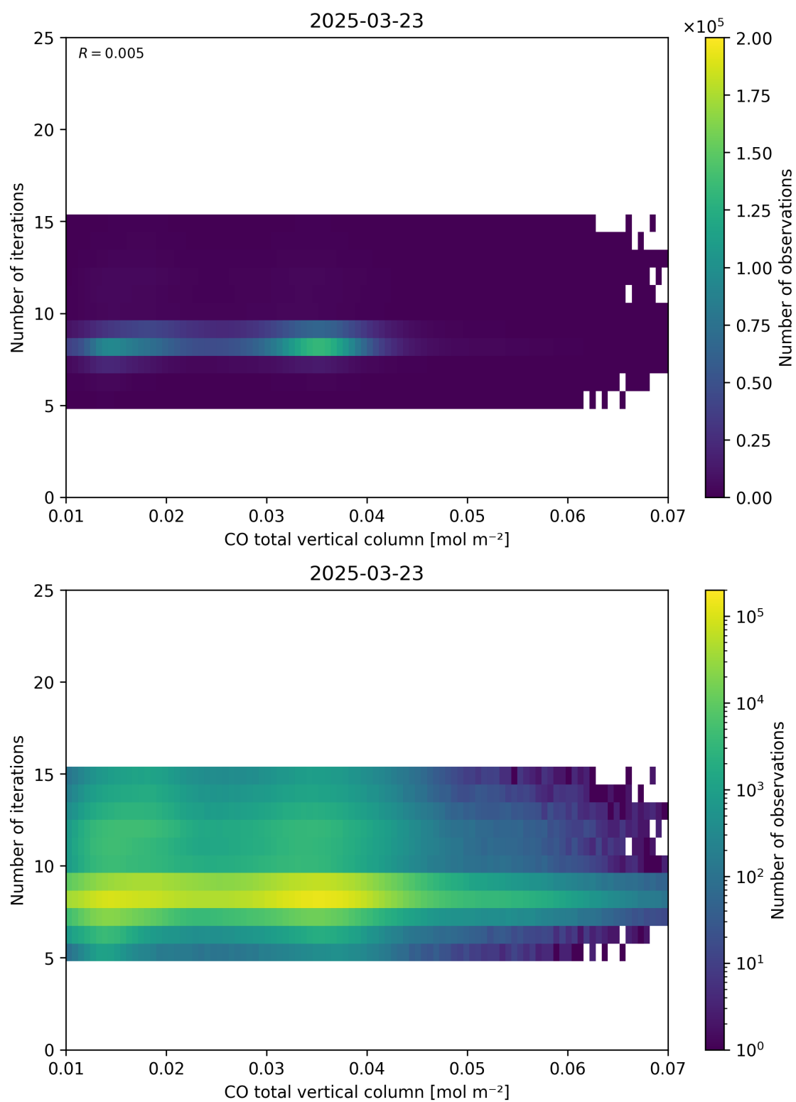
Figure 42: Scatter density plot of “CO total vertical column” against “Number of iterations” for 2025-03-23 to 2025-03-24.
