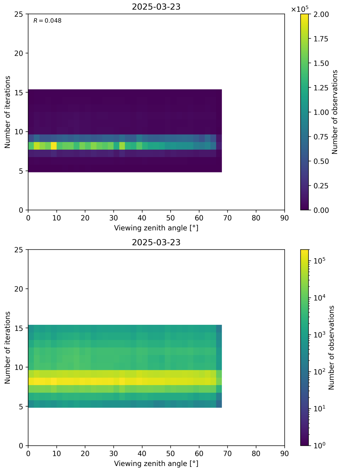
Figure 75: Scatter density plot of “Viewing zenith angle” against “Number of iterations” for 2025-03-23 to 2025-03-24.
