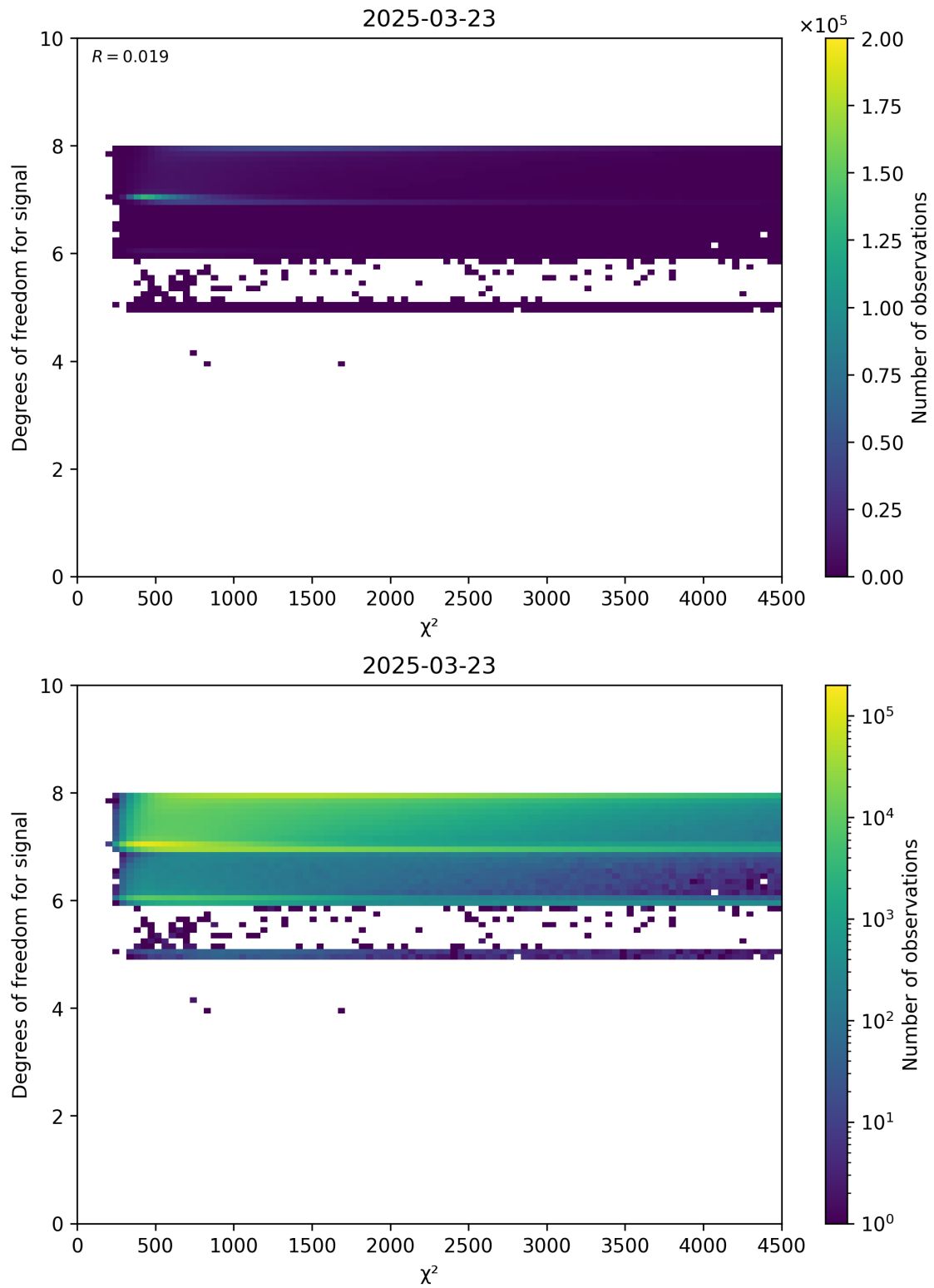
Figure 48: Scatter density plot of “ \chi^2 ” against “Degrees of freedom for signal” for 2025-03-23 to 2025-03-24.
