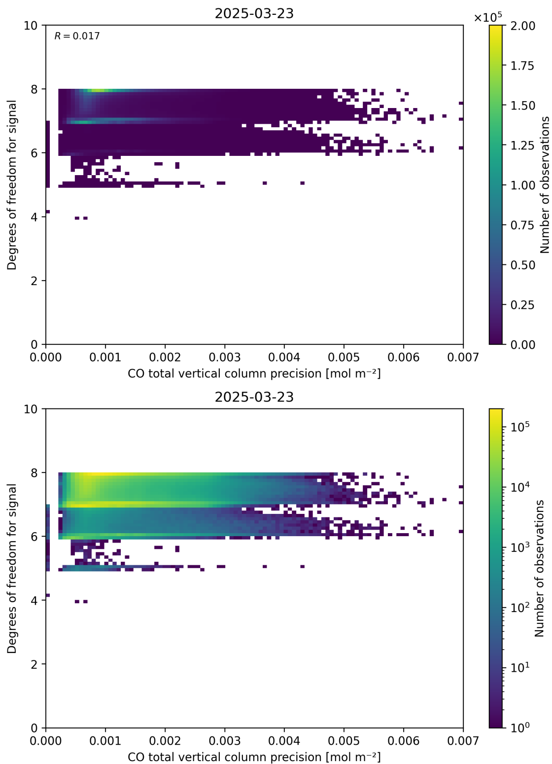
Figure 45: Scatter density plot of “CO total vertical column precision” against “Degrees of freedom for signal” for 2025-03-23 to 2025-03-24.
