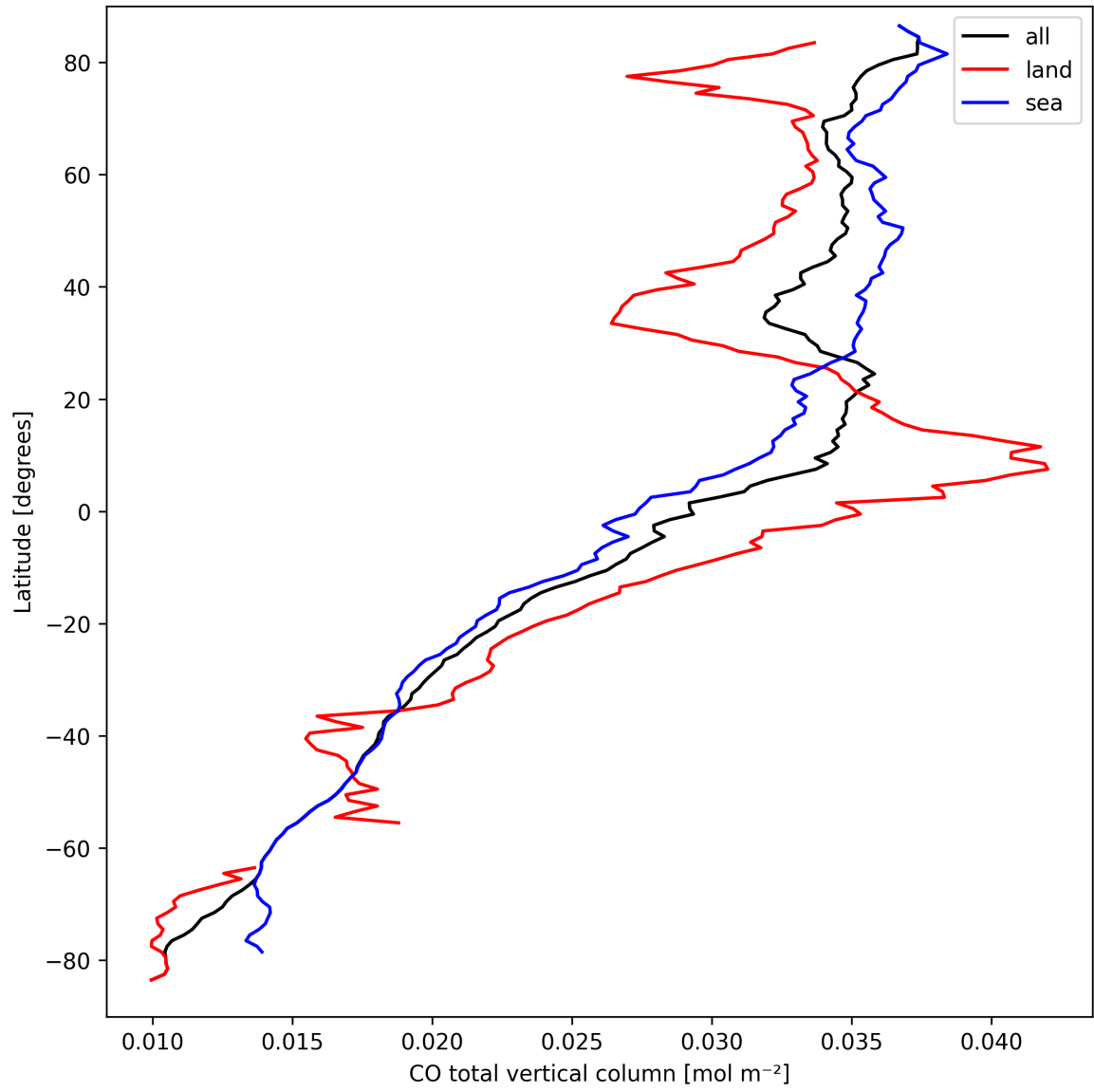
Figure 10: Zonal average of “CO total vertical column” for 2025-03-23 to 2025-03-24.
