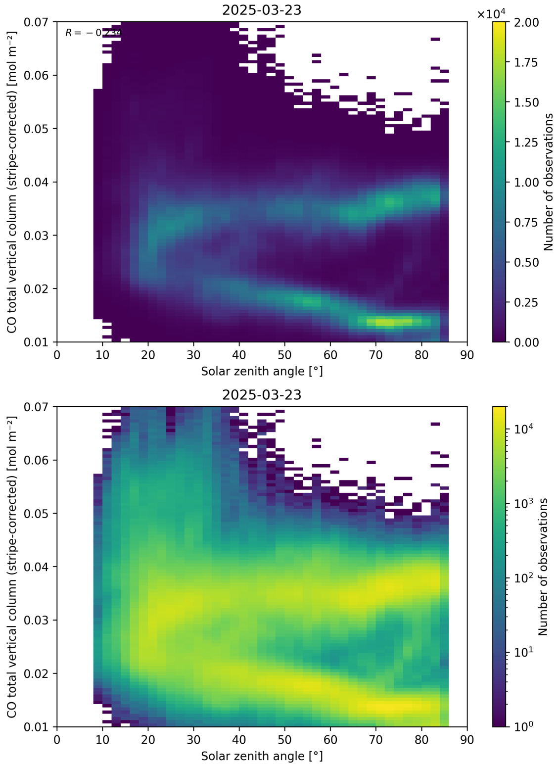
Figure 62: Scatter density plot of “Solar zenith angle” against “CO total vertical column (stripe-corrected)” for 2025-03-23 to 2025-03-24.
