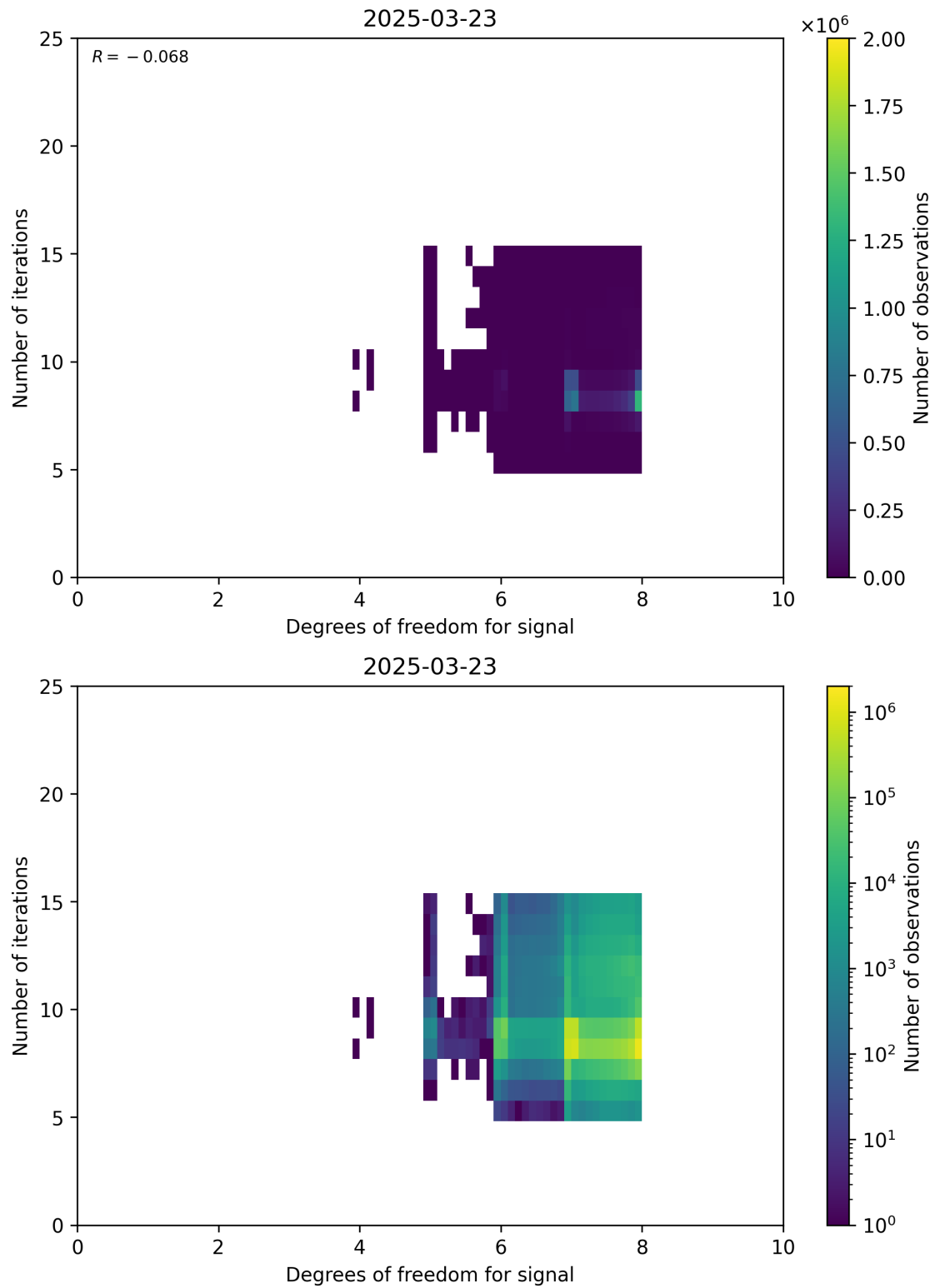
Figure 50: Scatter density plot of “Degrees of freedom for signal” against “Number of iterations” for 2025-03-23 to 2025-03-24.
