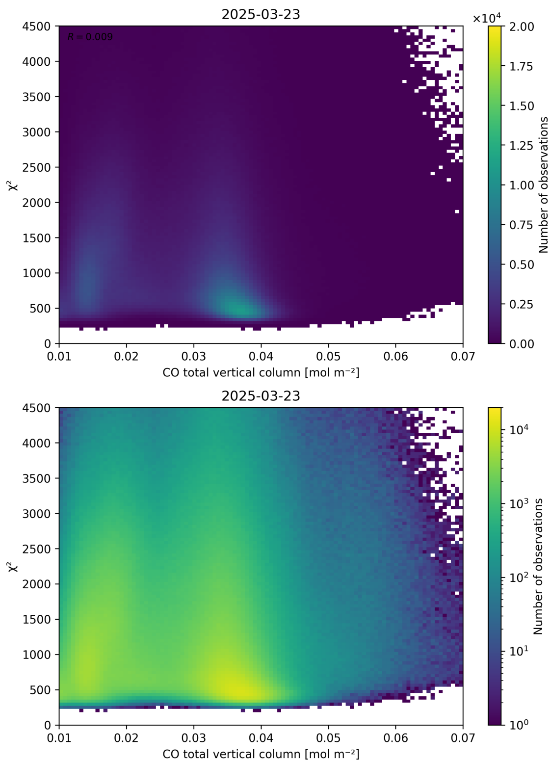
Figure 35: Scatter density plot of “CO total vertical column” against “ \chi^2 ” for 2025-03-23 to 2025-03-24.
