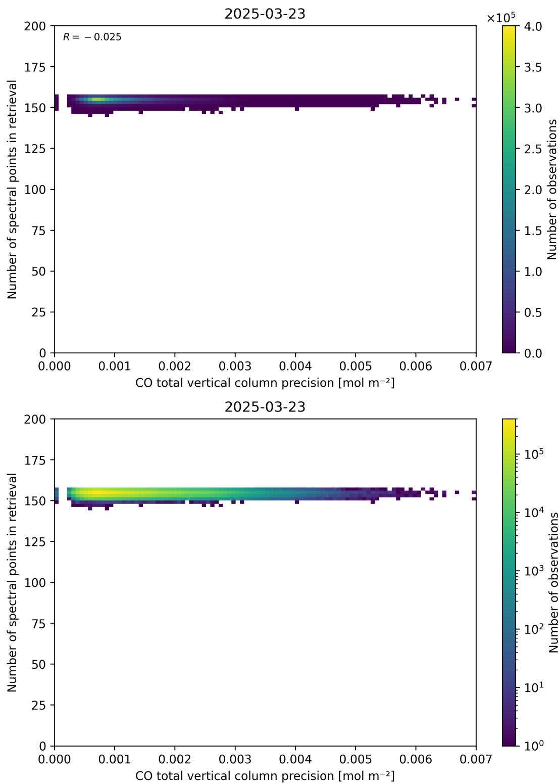
Figure 47: Scatter density plot of “CO total vertical column precision” against “Number of spectral points in retrieval” for 2025-03-23 to 2025-03-24.
