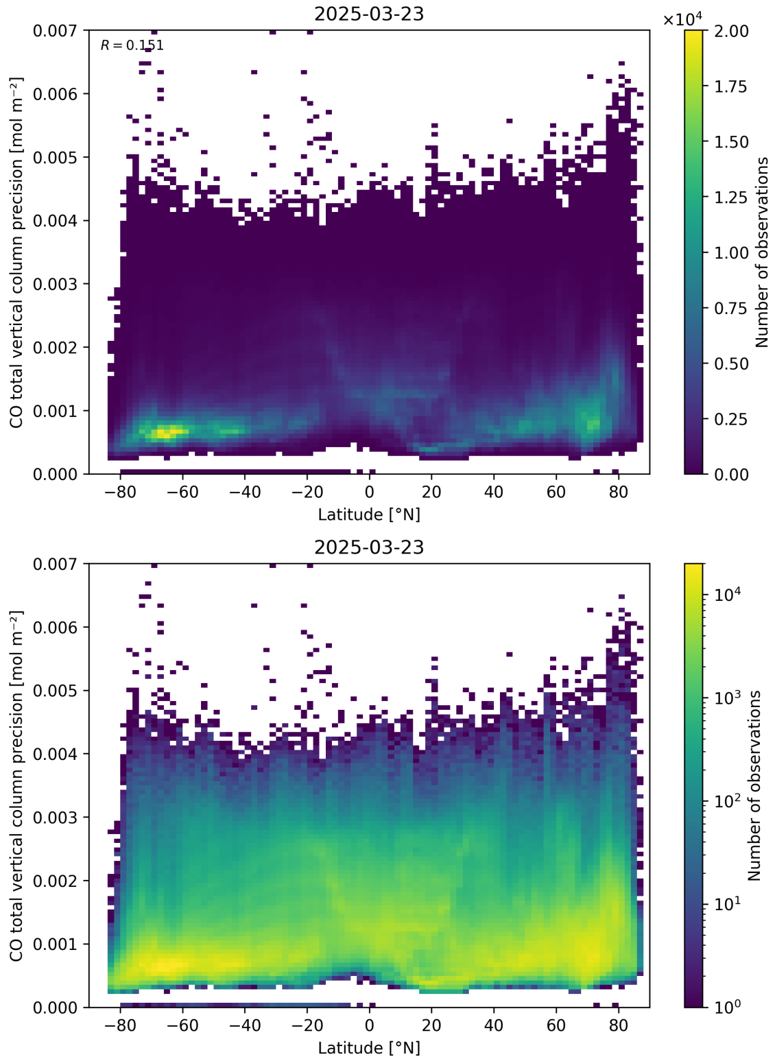
Figure 53: Scatter density plot of “Latitude” against “CO total vertical column precision” for 2025-03-23 to 2025-03-24.
