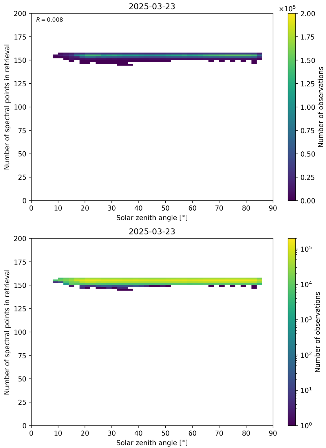
Figure 68: Scatter density plot of “Solar zenith angle” against “Number of spectral points in retrieval” for 2025-03-23 to 2025-03-24.
