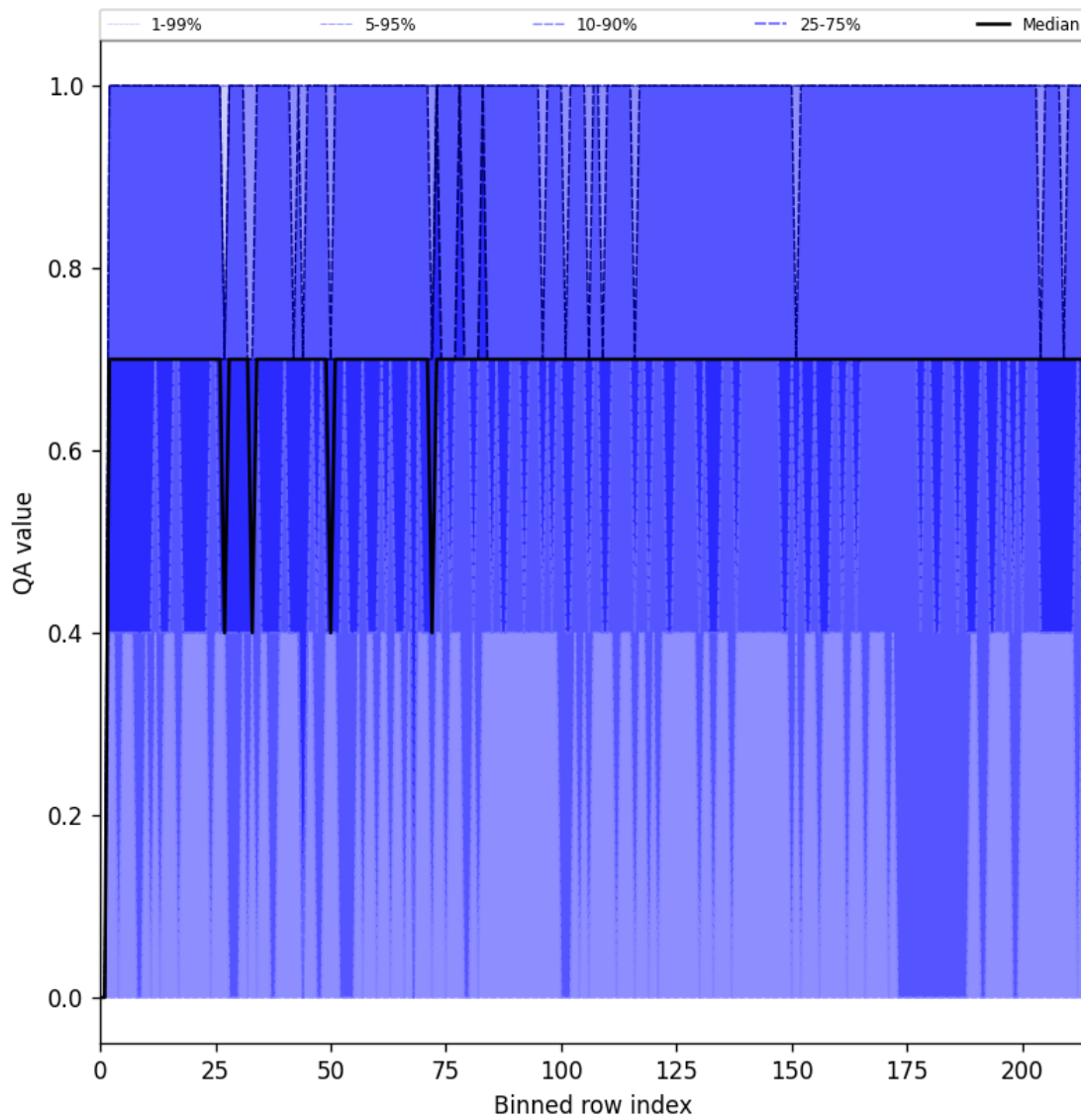
Figure 25: Along track statistics of “QA value” for 2025-03-23 to 2025-03-24
