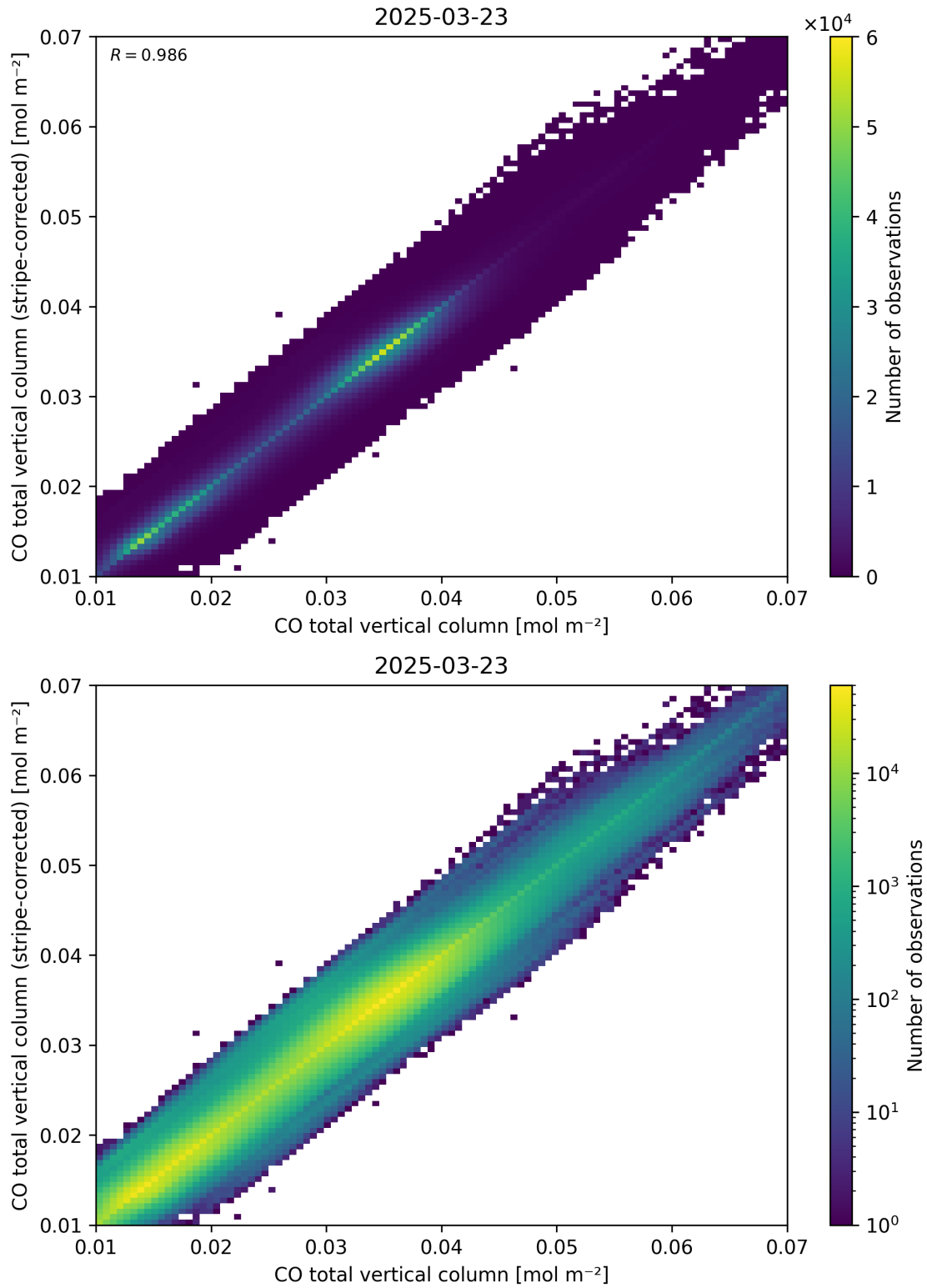
Figure 33: Scatter density plot of “CO total vertical column” against “CO total vertical column (stripe-corrected)” for 2025-03-23 to 2025-03-24.
