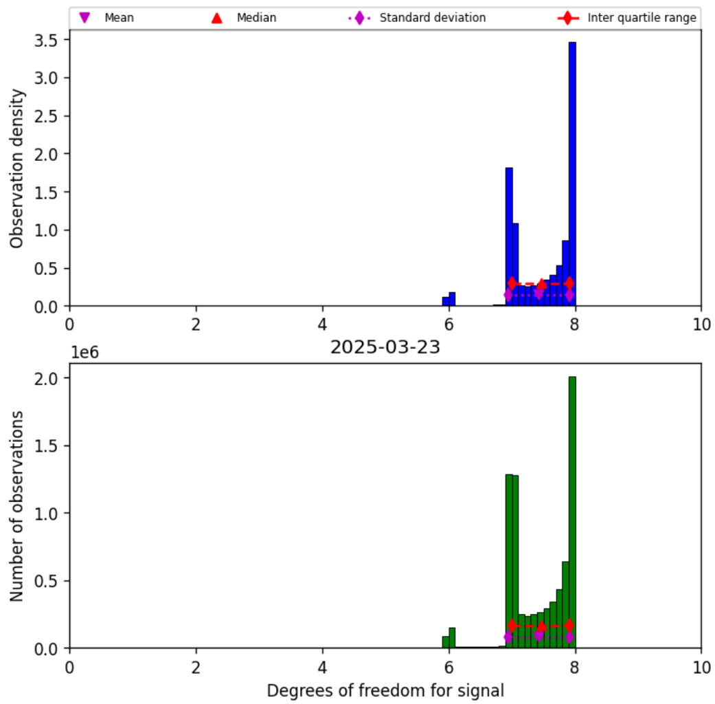
Figure 23: Histogram of “Degrees of freedom for signal” for 2025-03-23 to 2025-03-24
