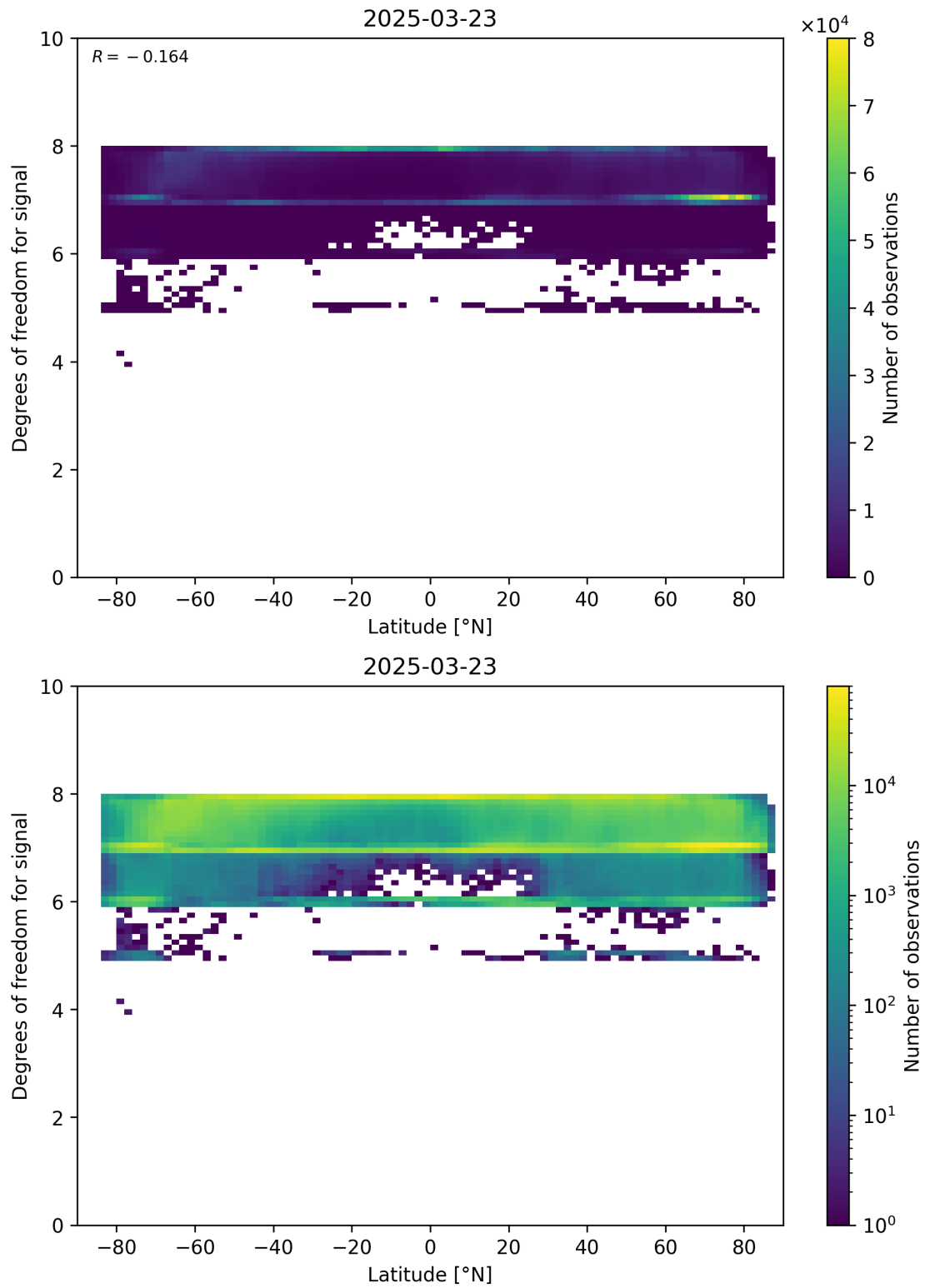
Figure 55: Scatter density plot of “Latitude” against “Degrees of freedom for signal” for 2025-03-23 to 2025-03-24.
