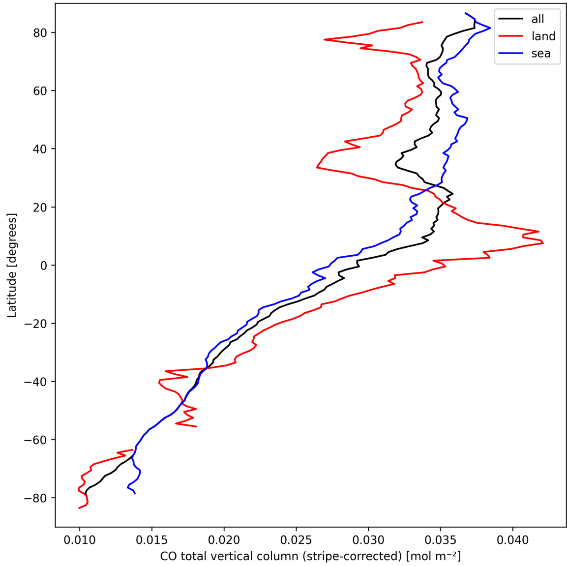
Figure 11: Zonal average of “CO total vertical column (stripe-corrected)” for 2025-03-23 to 2025-03-24.
