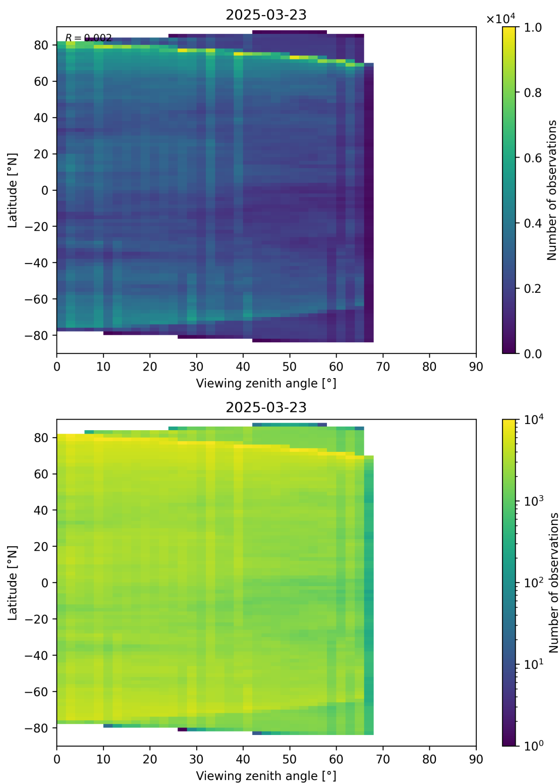
Figure 74: Scatter density plot of “Viewing zenith angle” against “Latitude” for 2025-03-23 to 2025-03-24.
