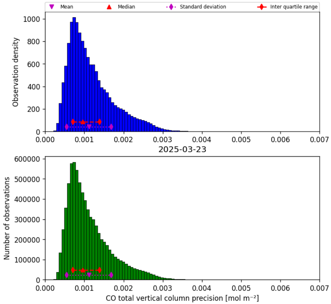
Figure 20: Histogram of “CO total vertical column precision” for 2025-03-23 to 2025-03-24
