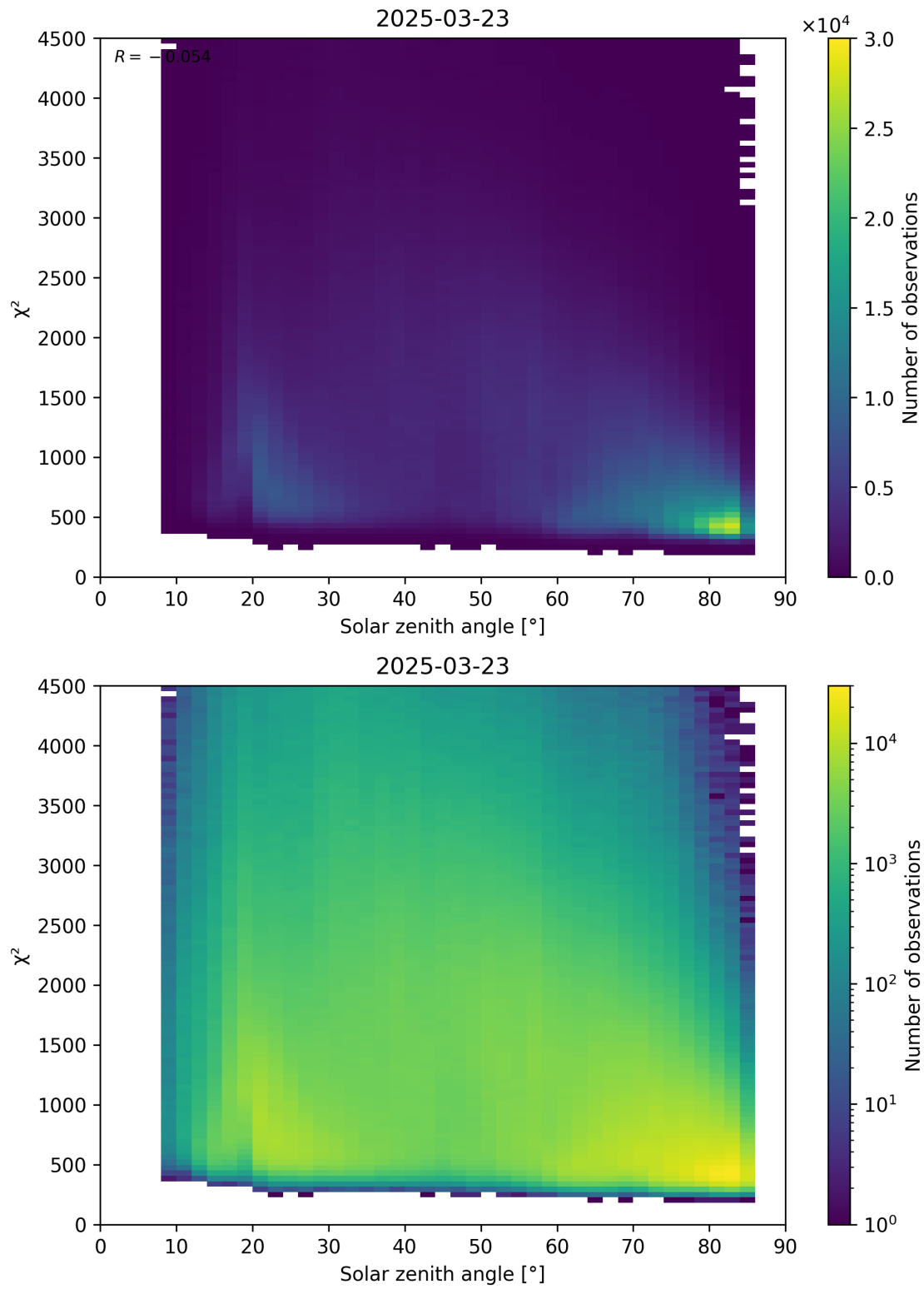
Figure 64: Scatter density plot of “Solar zenith angle” against “ \chi^2 ” for 2025-03-23 to 2025-03-24.
