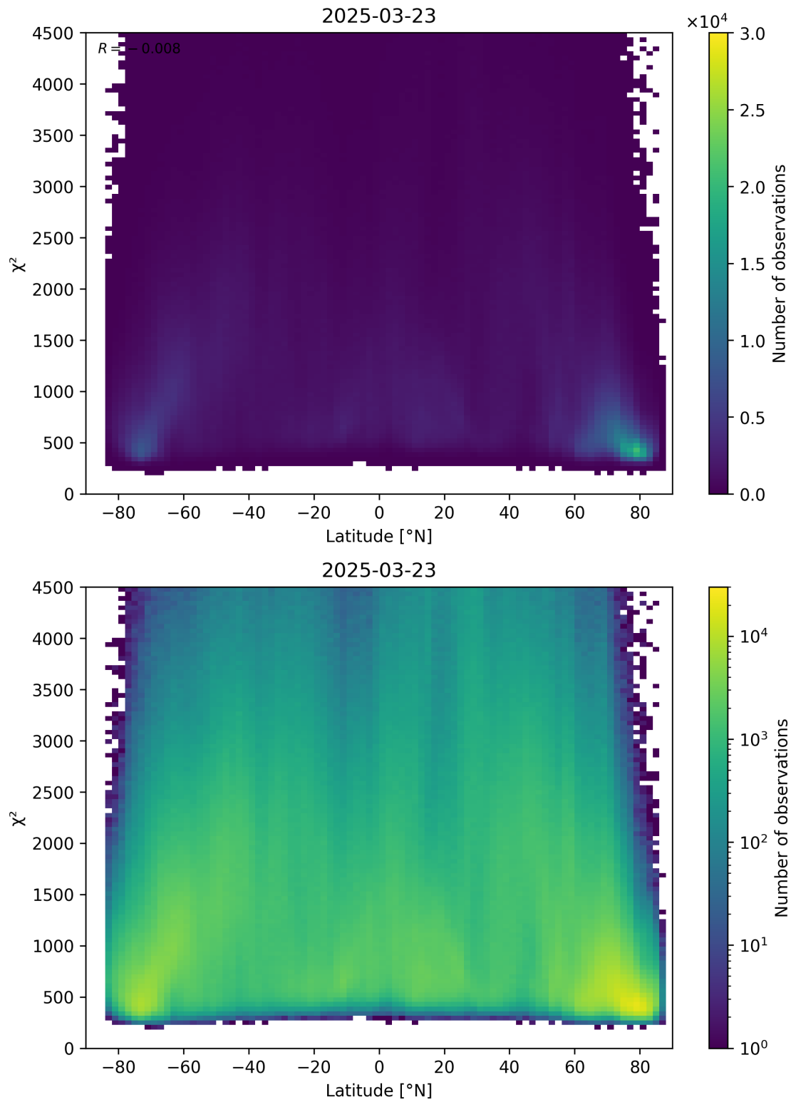
Figure 54: Scatter density plot of “Latitude” against “ \chi^2 ” for 2025-03-23 to 2025-03-24.
