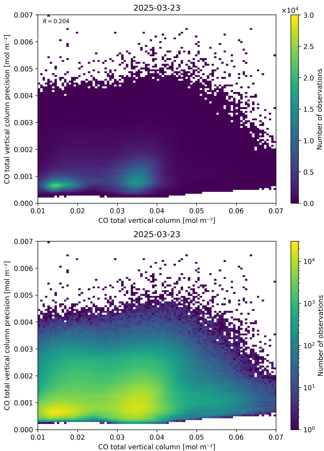
Figure 34: Scatter density plot of “CO total vertical column” against “CO total vertical column precision” for 2025-03-23 to 2025-03-24.
