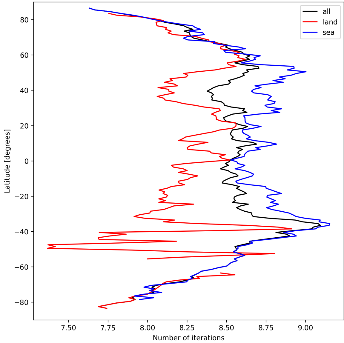
Figure 16: Zonal average of “Number of iterations” for 2025-03-23 to 2025-03-24.
