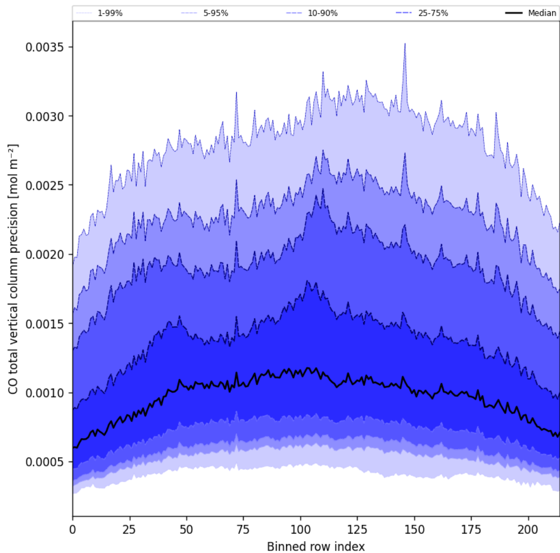
Figure 28: Along track statistics of “CO total vertical column precision” for 2025-03-23 to 2025-03-24
