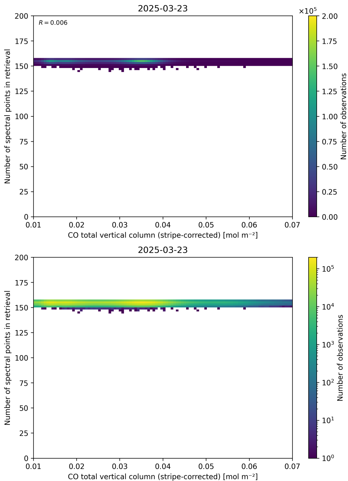
Figure 40: Scatter density plot of “CO total vertical column (stripe-corrected)” against “Number of spectral points in retrieval” for 2025-03-23 to 2025-03-24.
