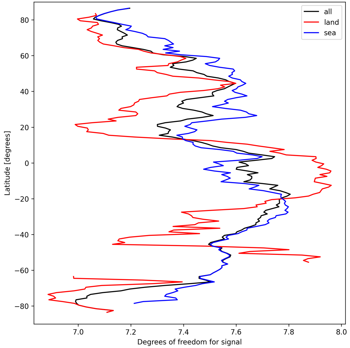
Figure 15: Zonal average of “Degrees of freedom for signal” for 2025-03-23 to 2025-03-24.
