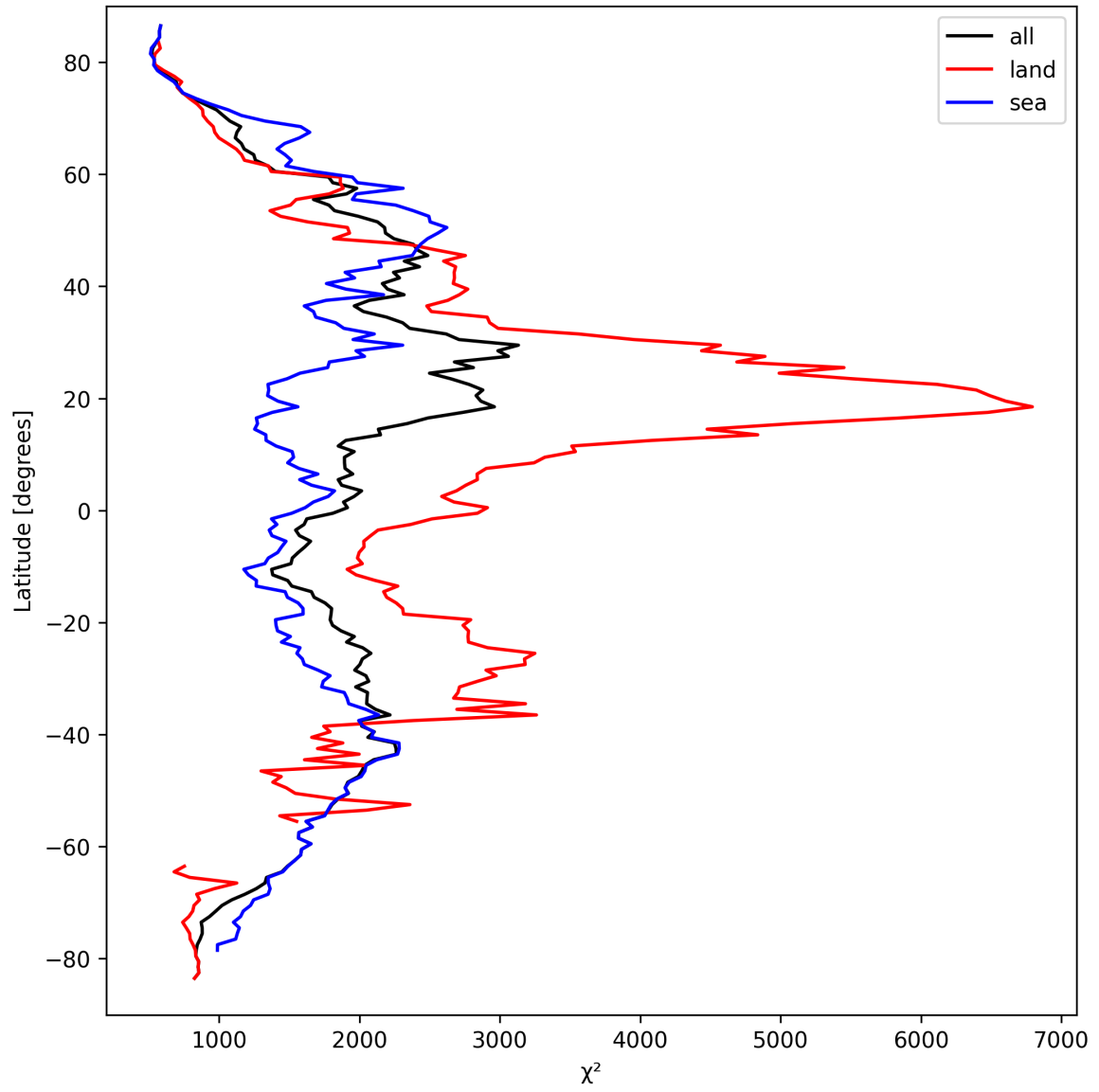
Figure 14: Zonal average of “ \chi^2 ” for 2025-03-23 to 2025-03-24.
