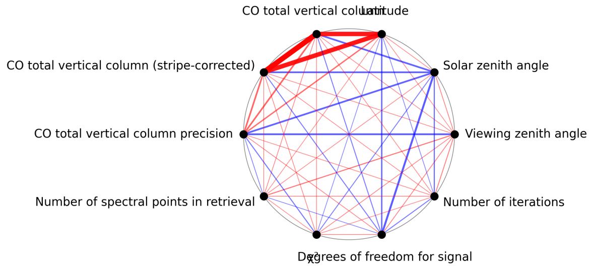
Figure 1: Map of correlation graph for 2025-03-23 to 2025-03-24.
