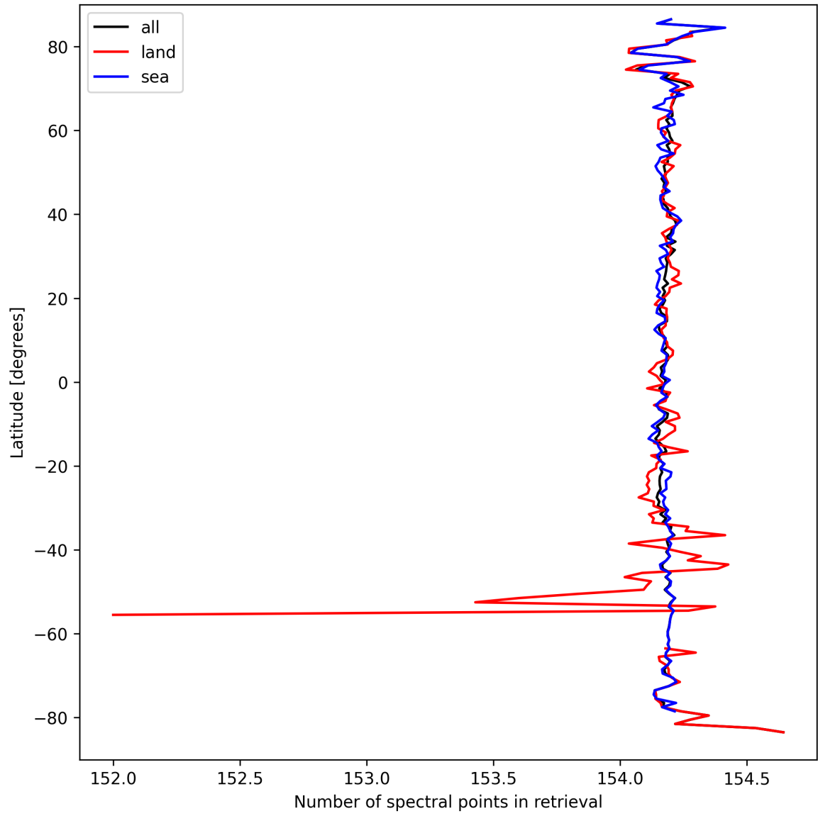
Figure 13: Zonal average of “Number of spectral points in retrieval” for 2025-03-23 to 2025-03-24.
