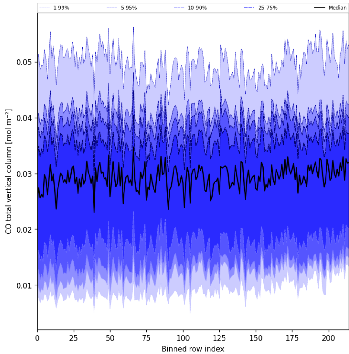
Figure 26: Along track statistics of “CO total vertical column” for 2025-03-23 to 2025-03-24
