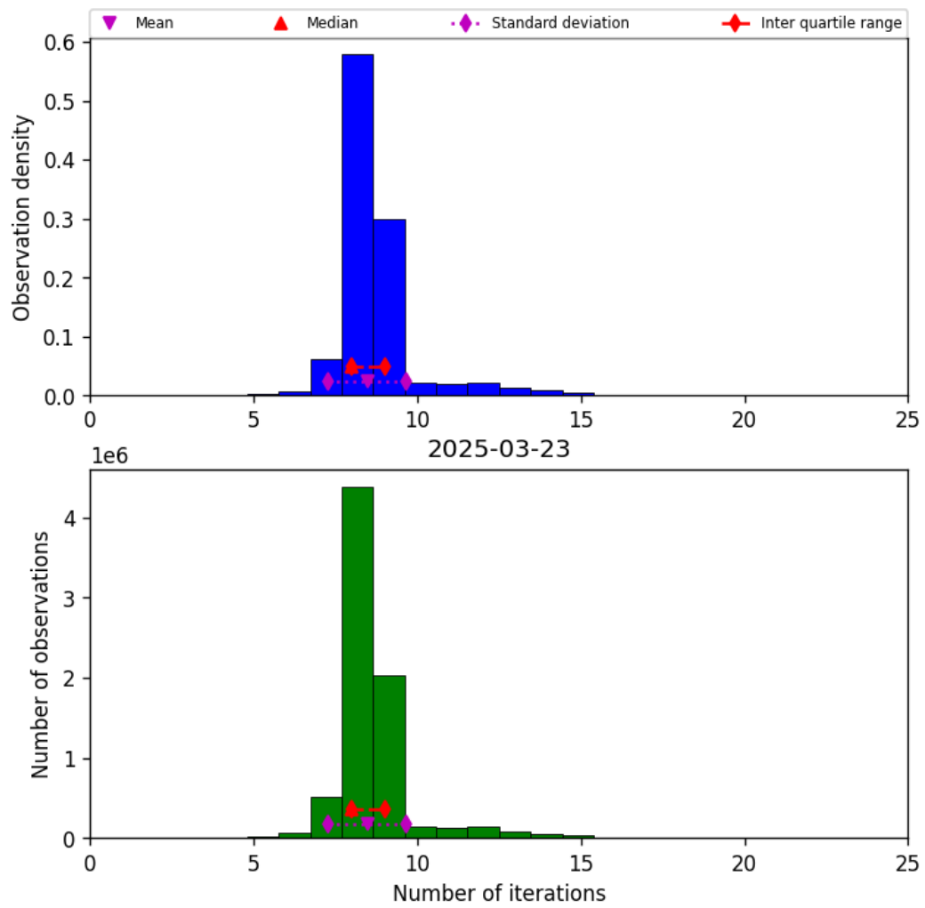
Figure 24: Histogram of “Number of iterations” for 2025-03-23 to 2025-03-24
