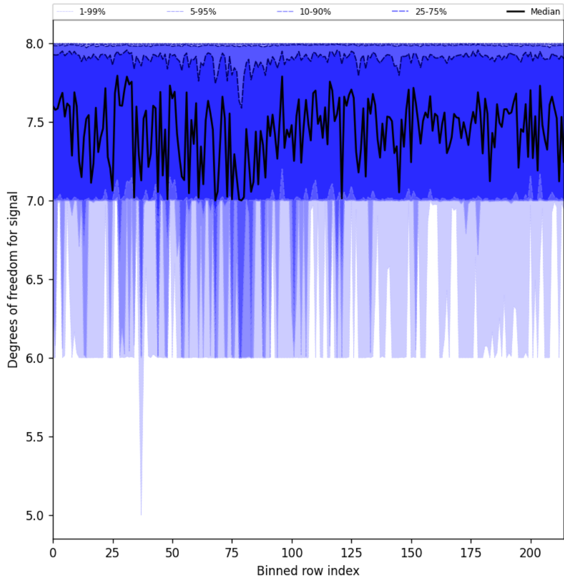
Figure 31: Along track statistics of “Degrees of freedom for signal” for 2025-03-23 to 2025-03-24
