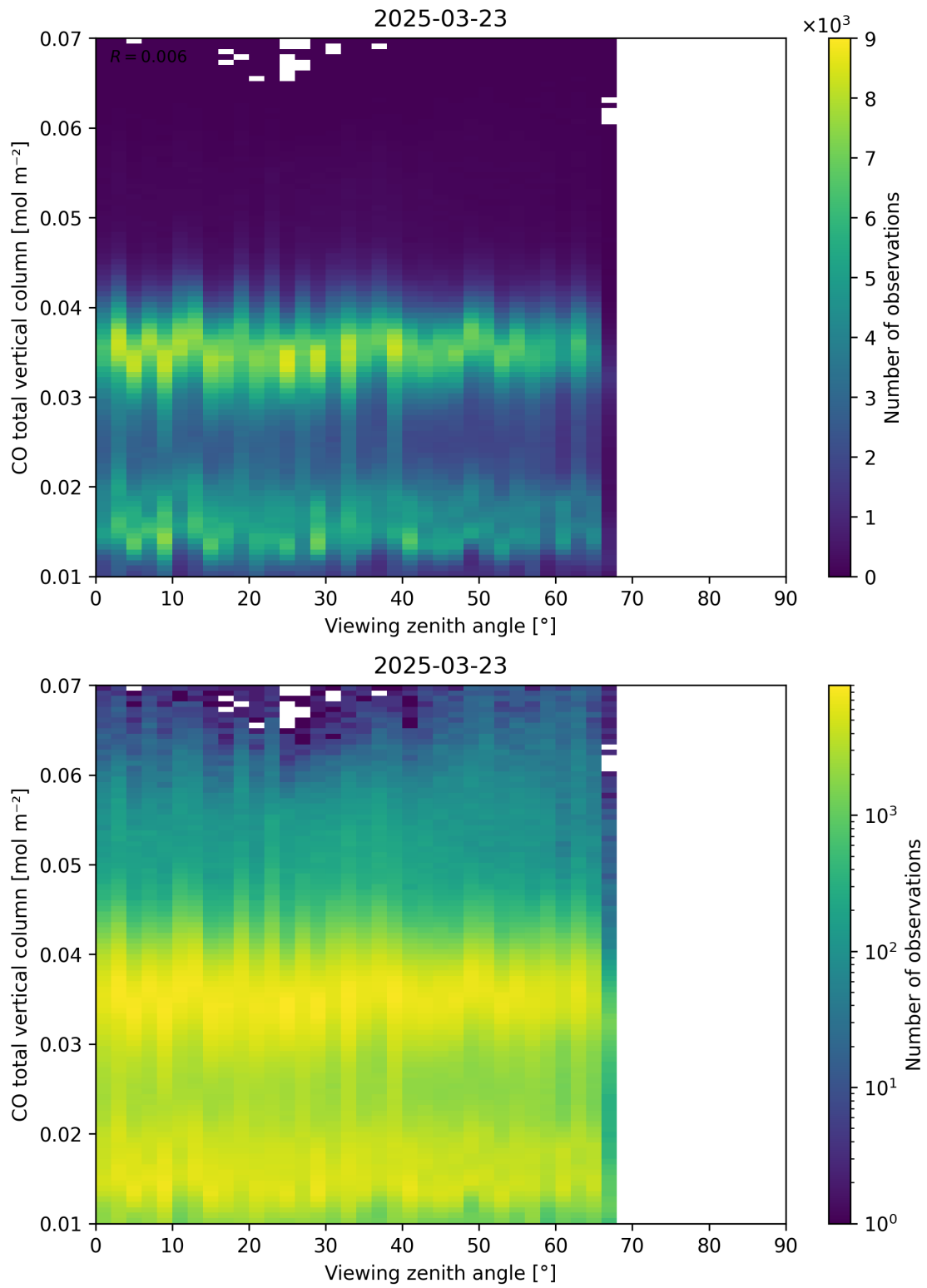
Figure 69: Scatter density plot of “Viewing zenith angle” against “CO total vertical column” for 2025-03-23 to 2025-03-24.
