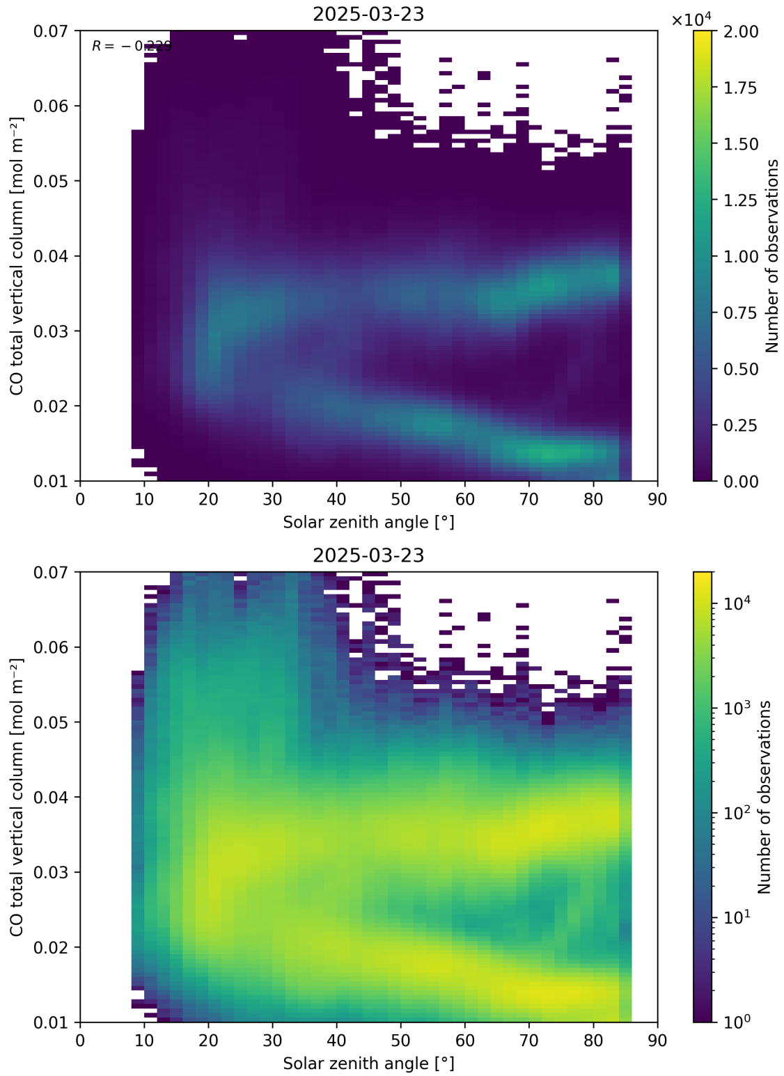
Figure 61: Scatter density plot of “Solar zenith angle” against “CO total vertical column” for 2025-03-23 to 2025-03-24.
