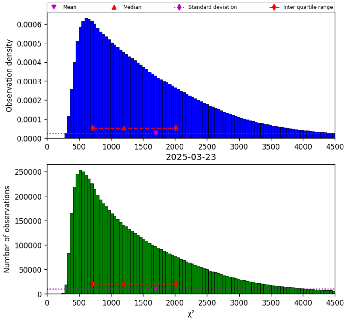
Figure 22: Histogram of “ \chi^2 ” for 2025-03-23 to 2025-03-24
