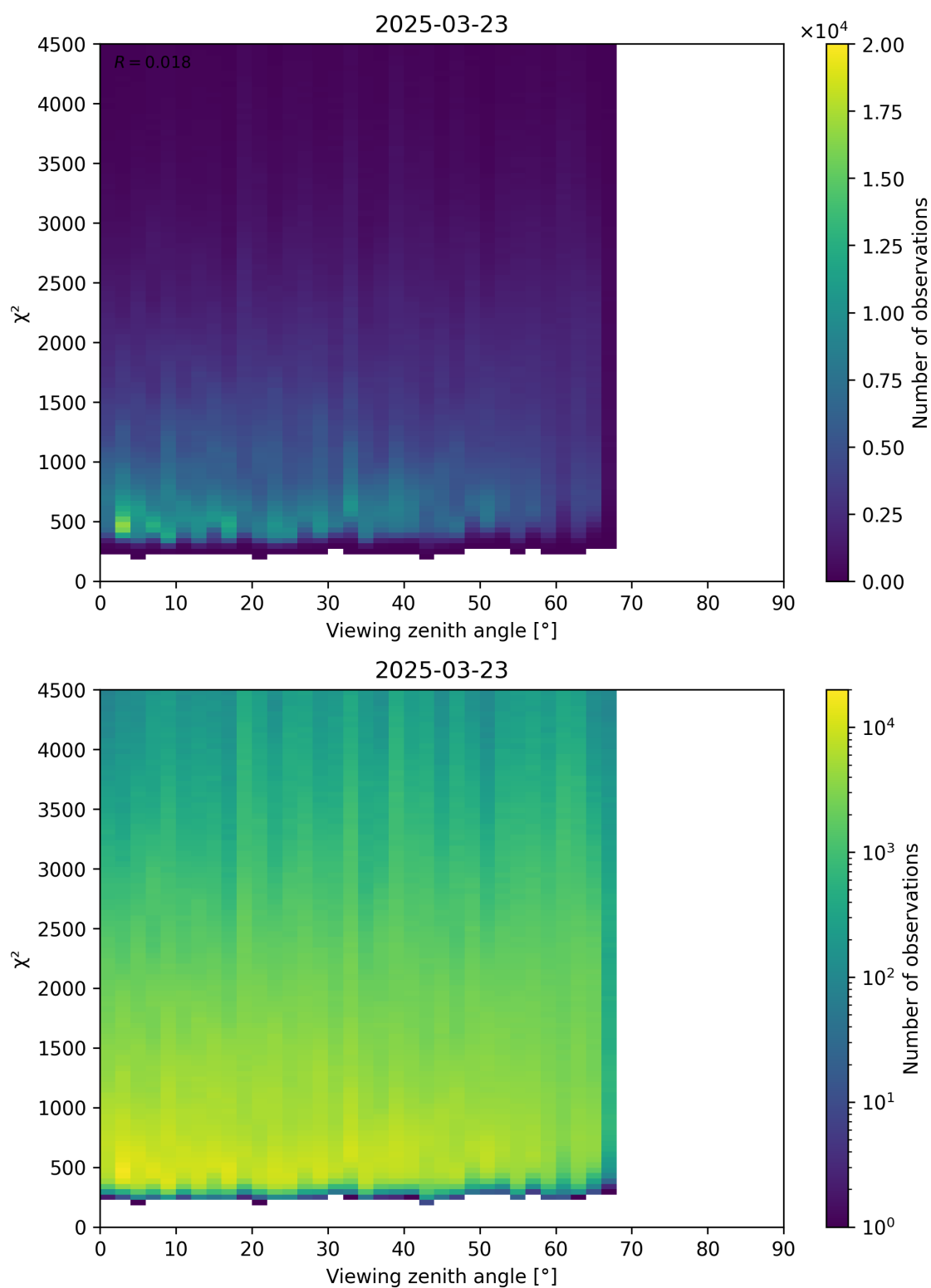
Figure 72: Scatter density plot of “Viewing zenith angle” against “ \chi^2 ” for 2025-03-23 to 2025-03-24.
