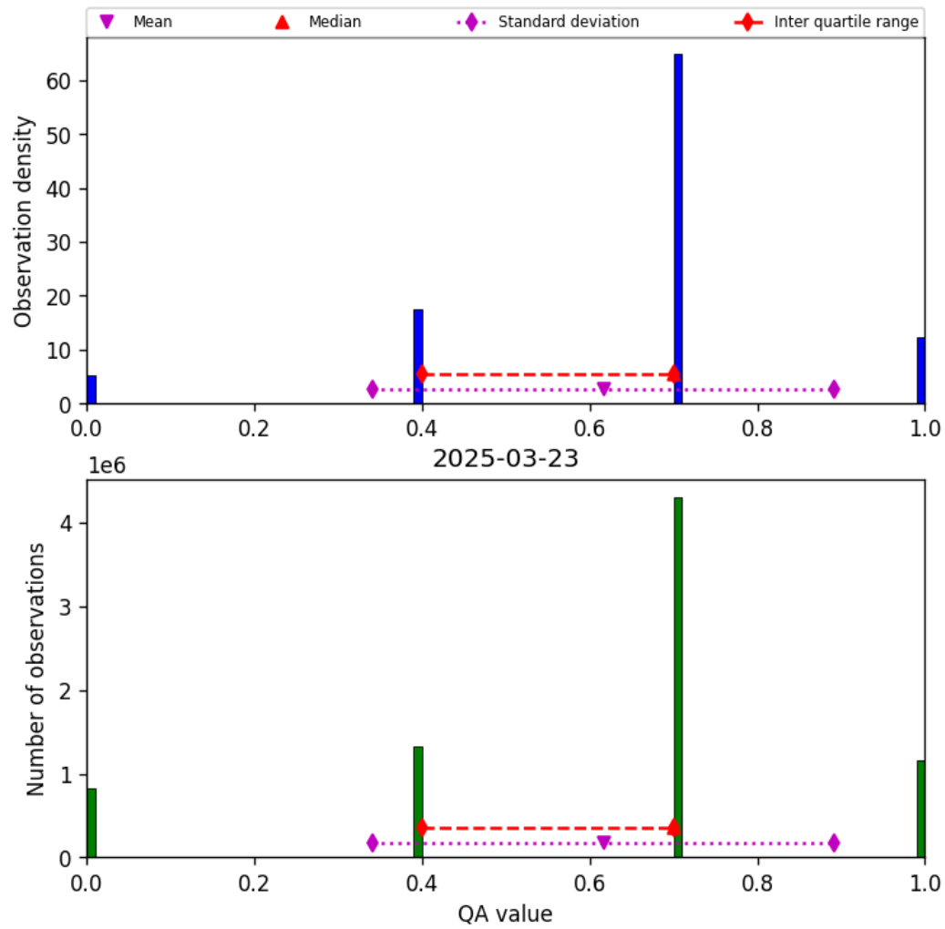
Figure 17: Histogram of “QA value” for 2025-03-23 to 2025-03-24
