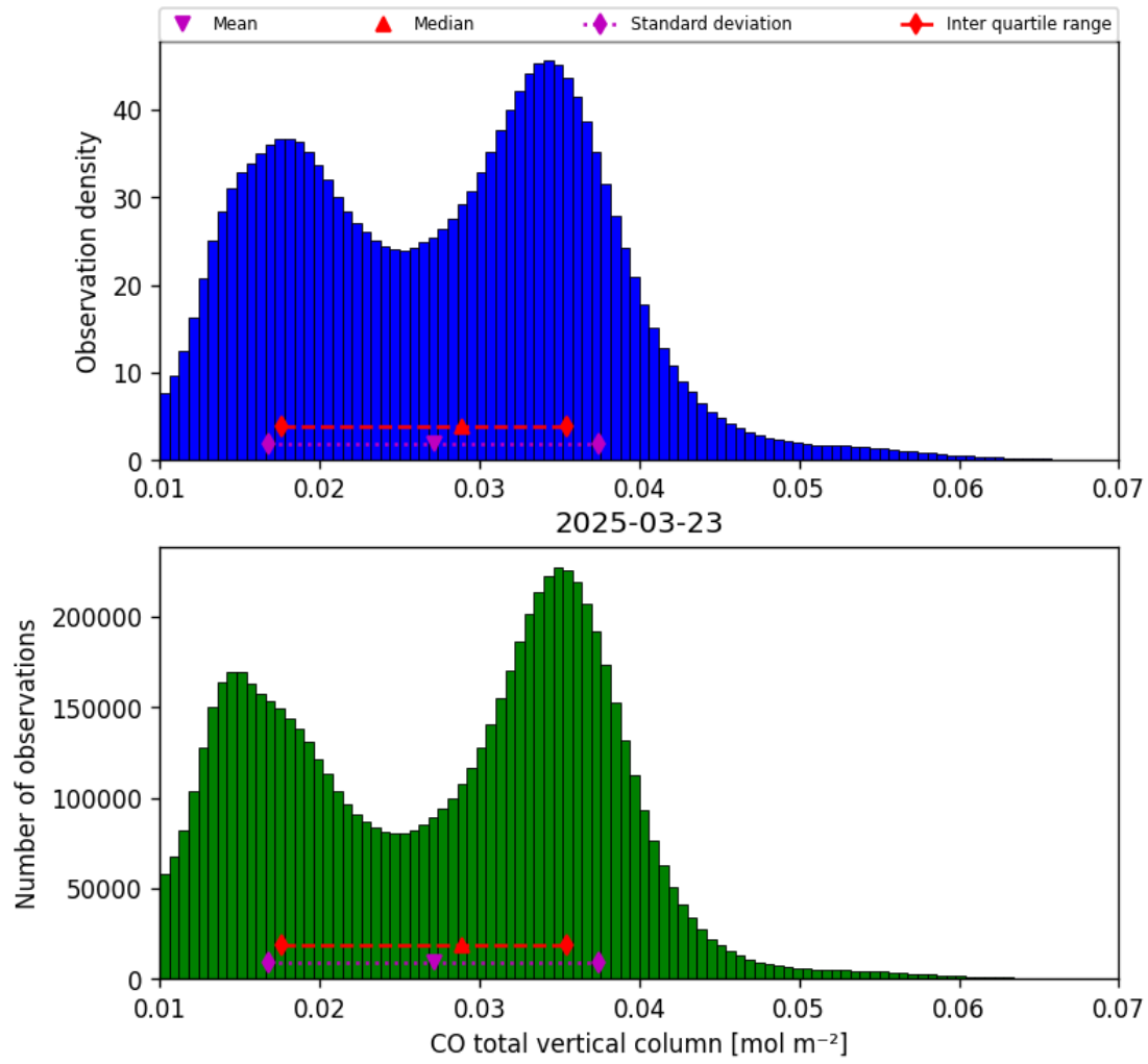
Figure 18: Histogram of “CO total vertical column” for 2025-03-23 to 2025-03-24
