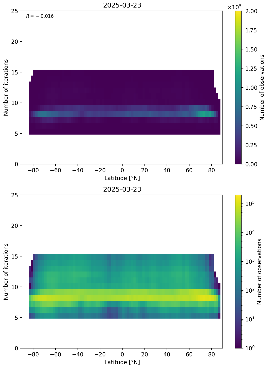
Figure 56: Scatter density plot of “Latitude” against “Number of iterations” for 2025-03-23 to 2025-03-24.
