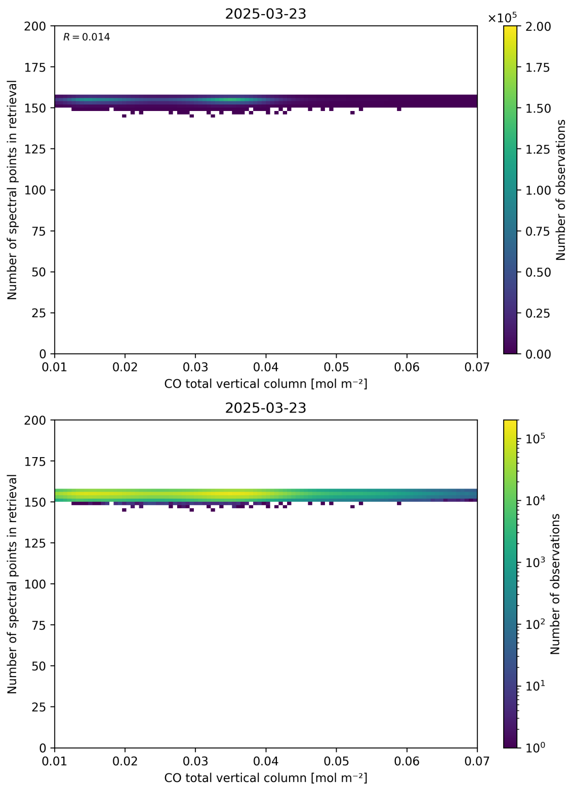
Figure 43: Scatter density plot of “CO total vertical column” against “Number of spectral points in retrieval” for 2025-03-23 to 2025-03-24.
