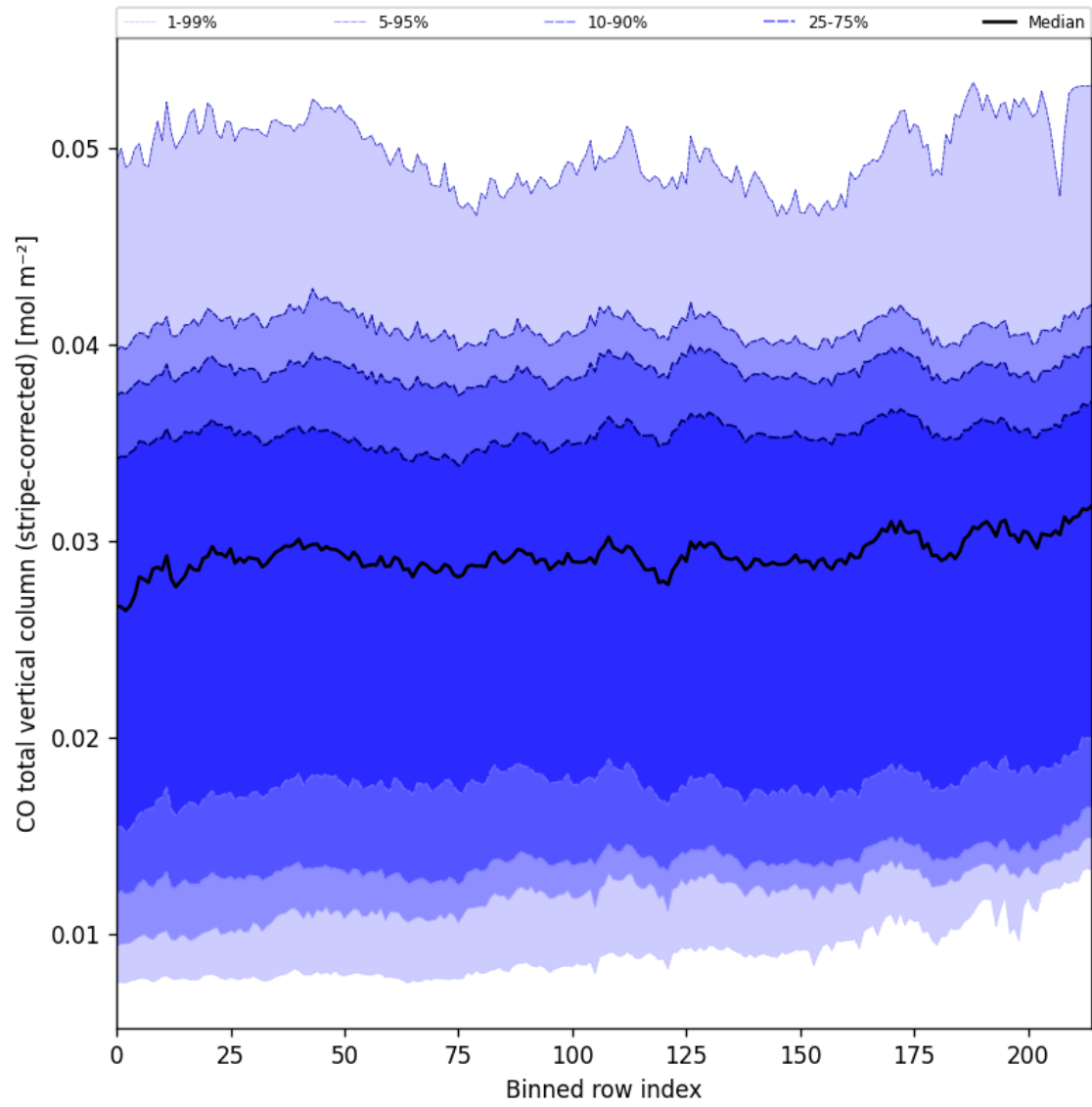
Figure 27: Along track statistics of “CO total vertical column (stripe-corrected)” for 2025-03-23 to 2025-03-24
