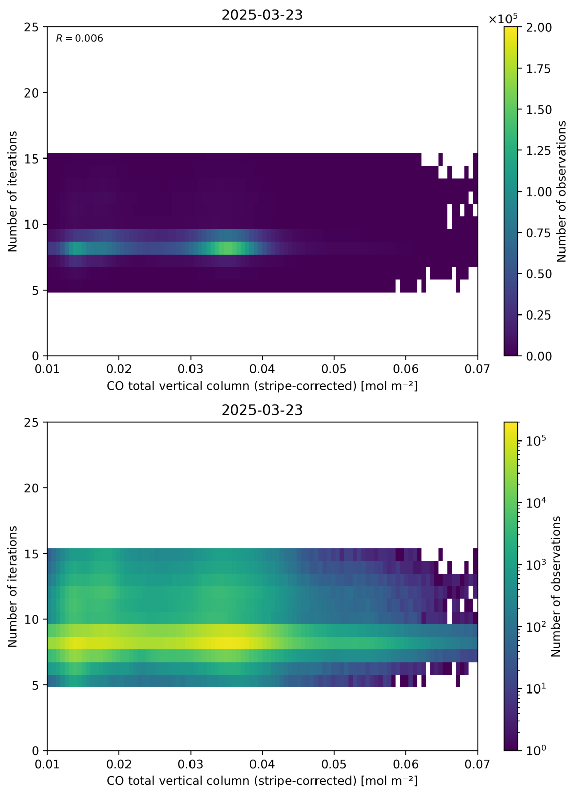
Figure 39: Scatter density plot of “CO total vertical column (stripe-corrected)” against “Number of iterations” for 2025-03-23 to 2025-03-24.
