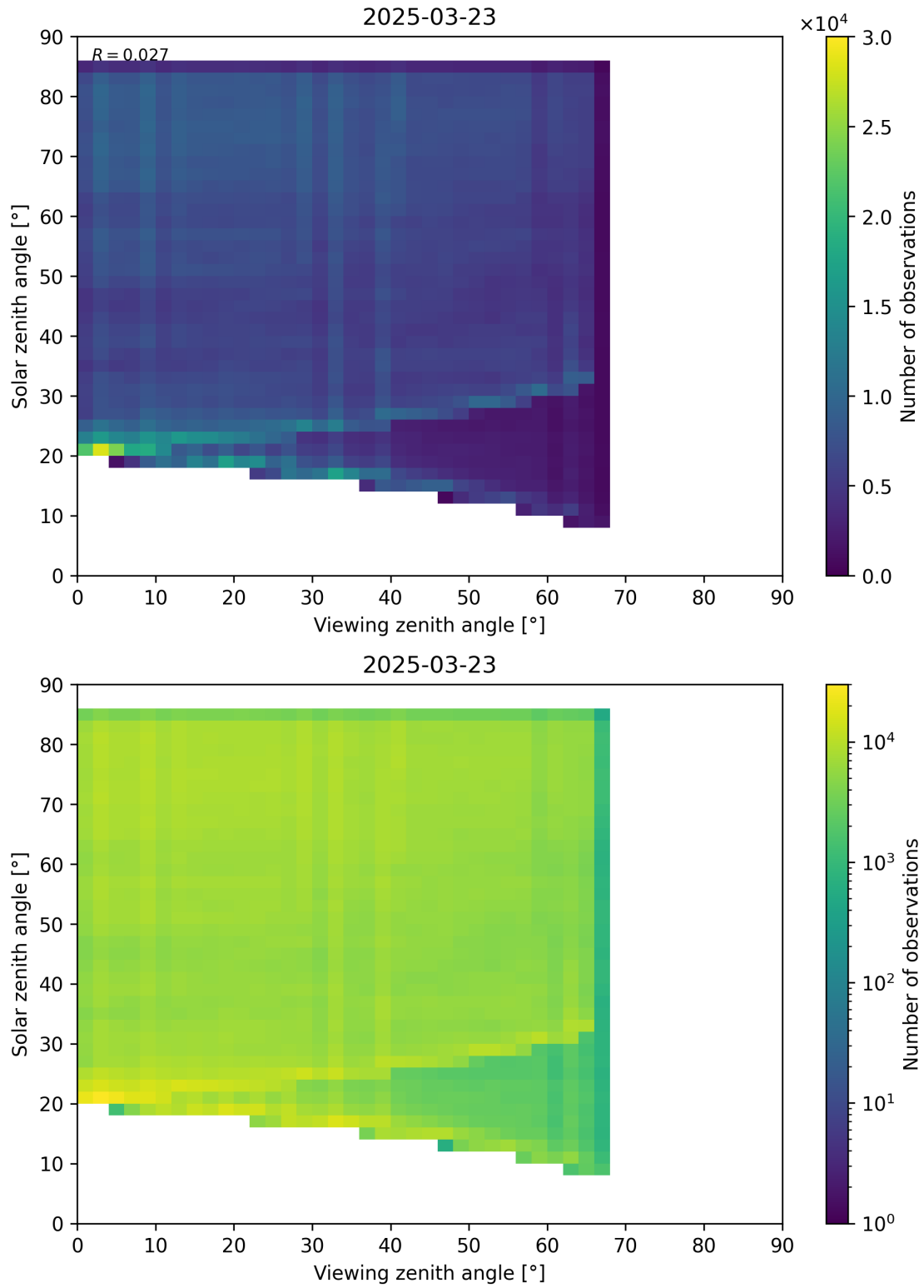
Figure 77: Scatter density plot of “Viewing zenith angle” against “Solar zenith angle” for 2025-03-23 to 2025-03-24.
