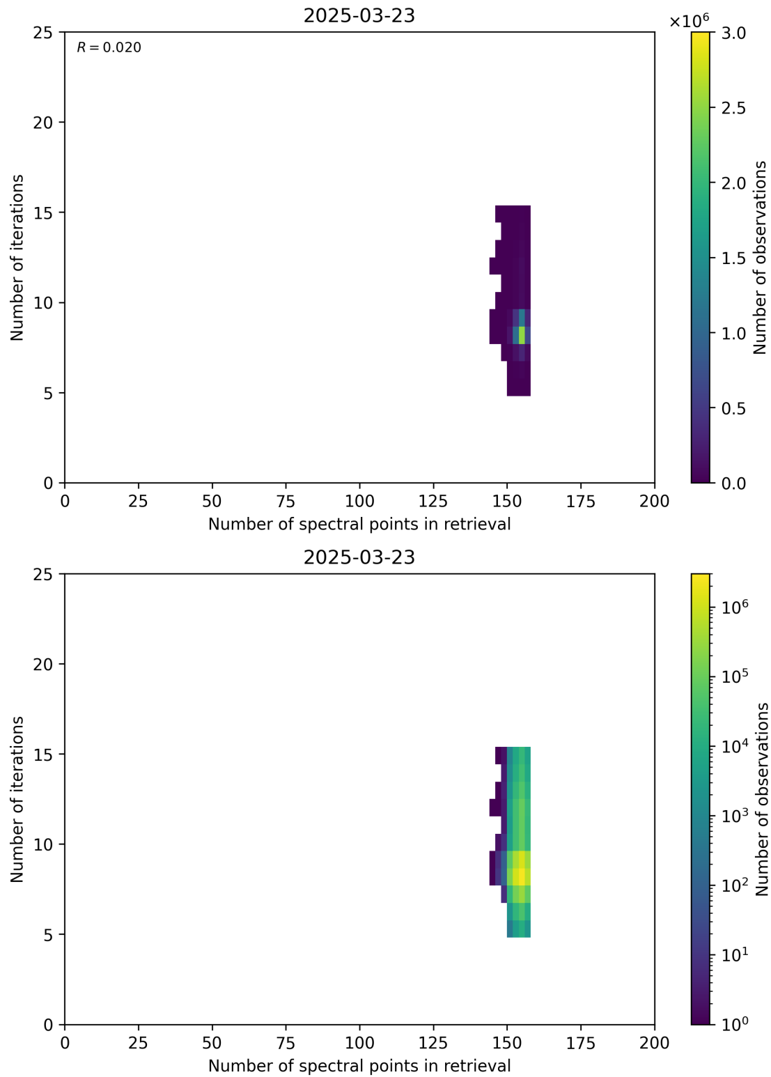
Figure 60: Scatter density plot of “Number of spectral points in retrieval” against “Number of iterations” for 2025-03-23 to 2025-03-24.
