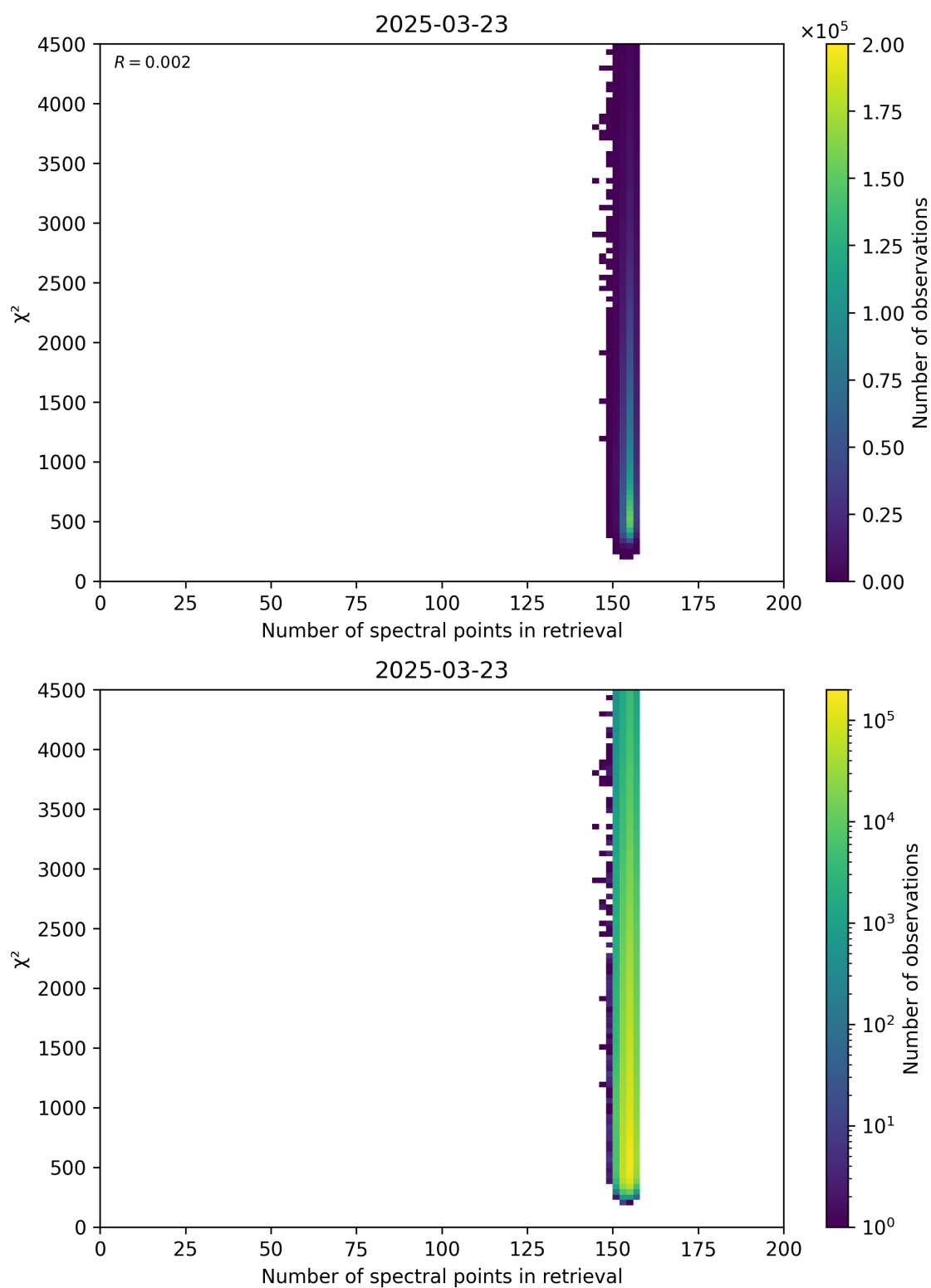
Figure 58: Scatter density plot of “Number of spectral points in retrieval” against “ \chi^2 ” for 2025-03-23 to 2025-03-24.
