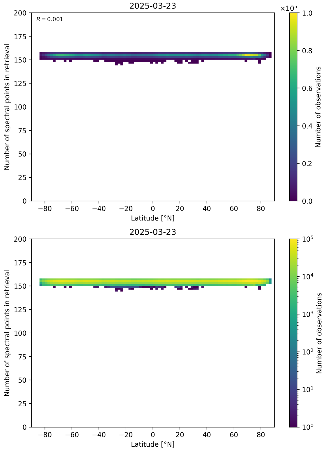
Figure 57: Scatter density plot of “Latitude” against “Number of spectral points in retrieval” for 2025-03-23 to 2025-03-24.
