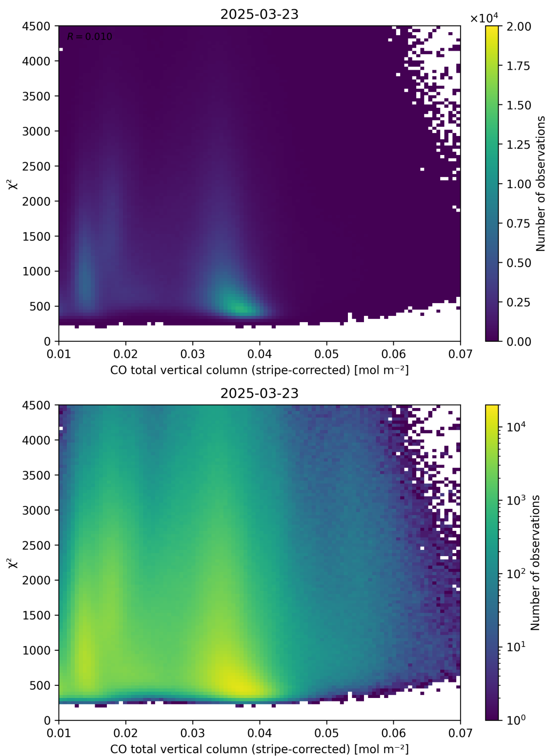
Figure 37: Scatter density plot of “CO total vertical column (stripe-corrected)” against “ \chi^2 ” for 2025-03-23 to 2025-03-24.
