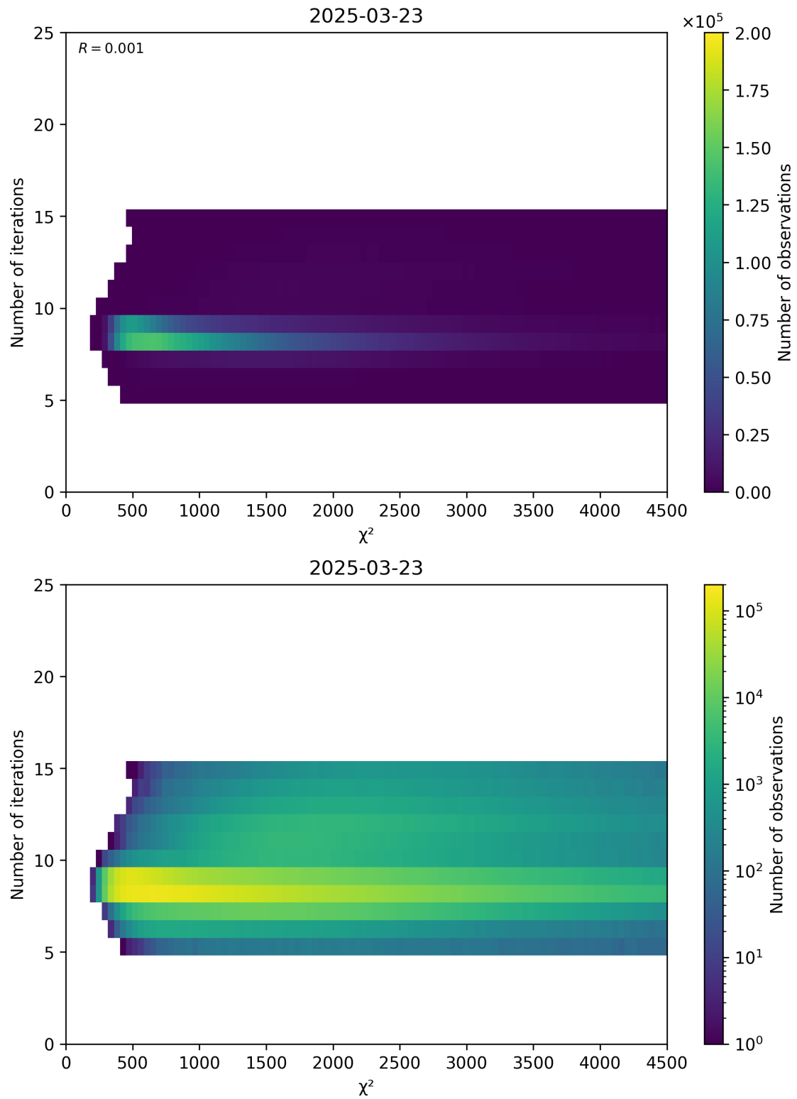
Figure 49: Scatter density plot of “ \chi^2 ” against “Number of iterations” for 2025-03-23 to 2025-03-24.
