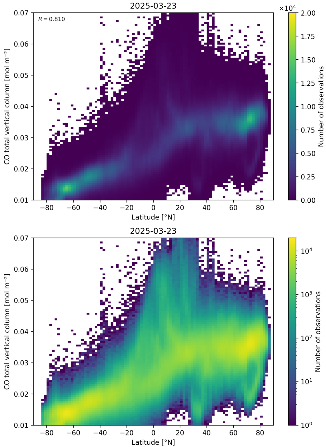
Figure 51: Scatter density plot of “Latitude” against “CO total vertical column” for 2025-03-23 to 2025-03-24.
