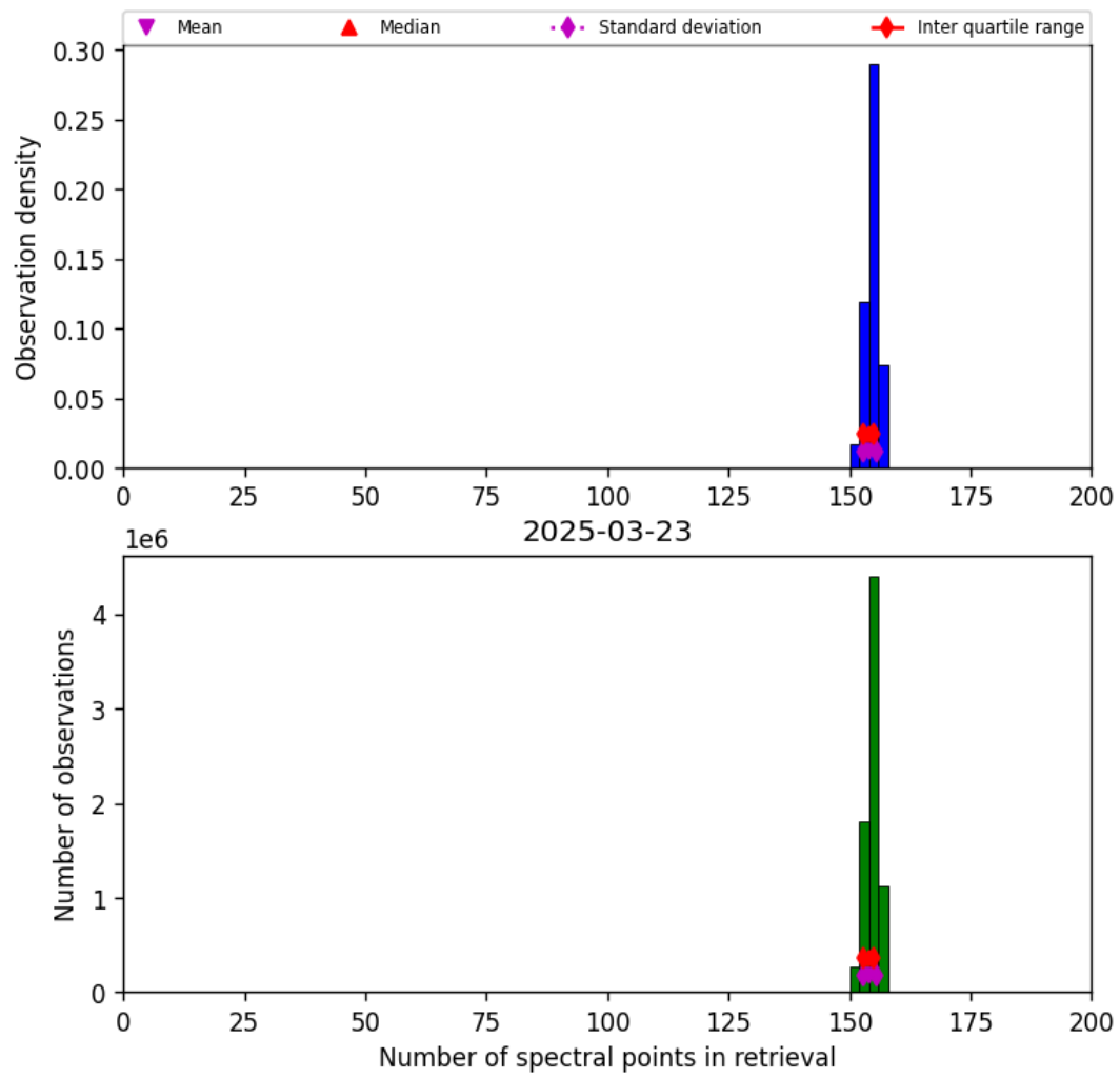
Figure 21: Histogram of “Number of spectral points in retrieval” for 2025-03-23 to 2025-03-24
