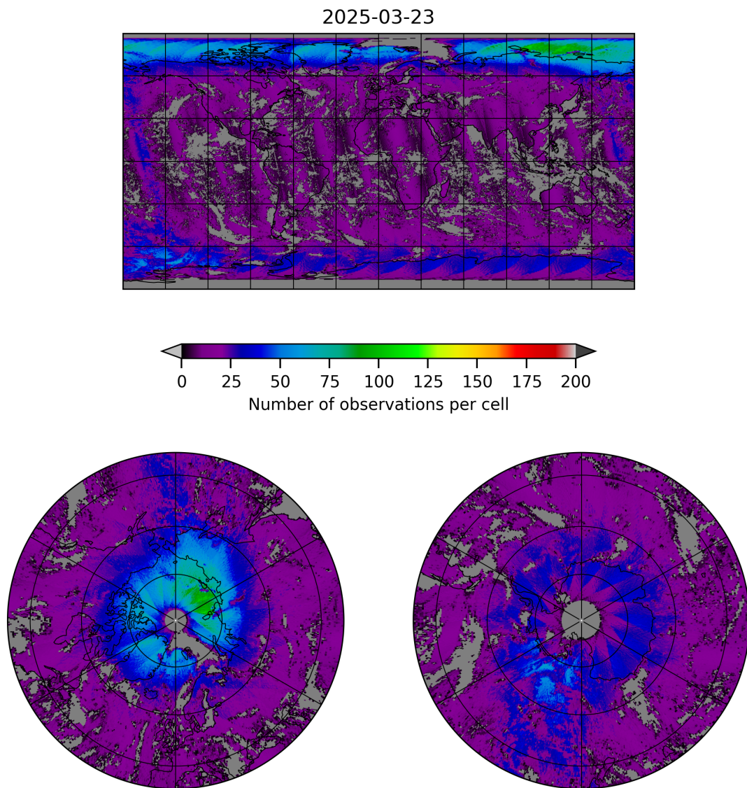
Figure 8: Map of the number of observations for 2025-03-23 to 2025-03-24
