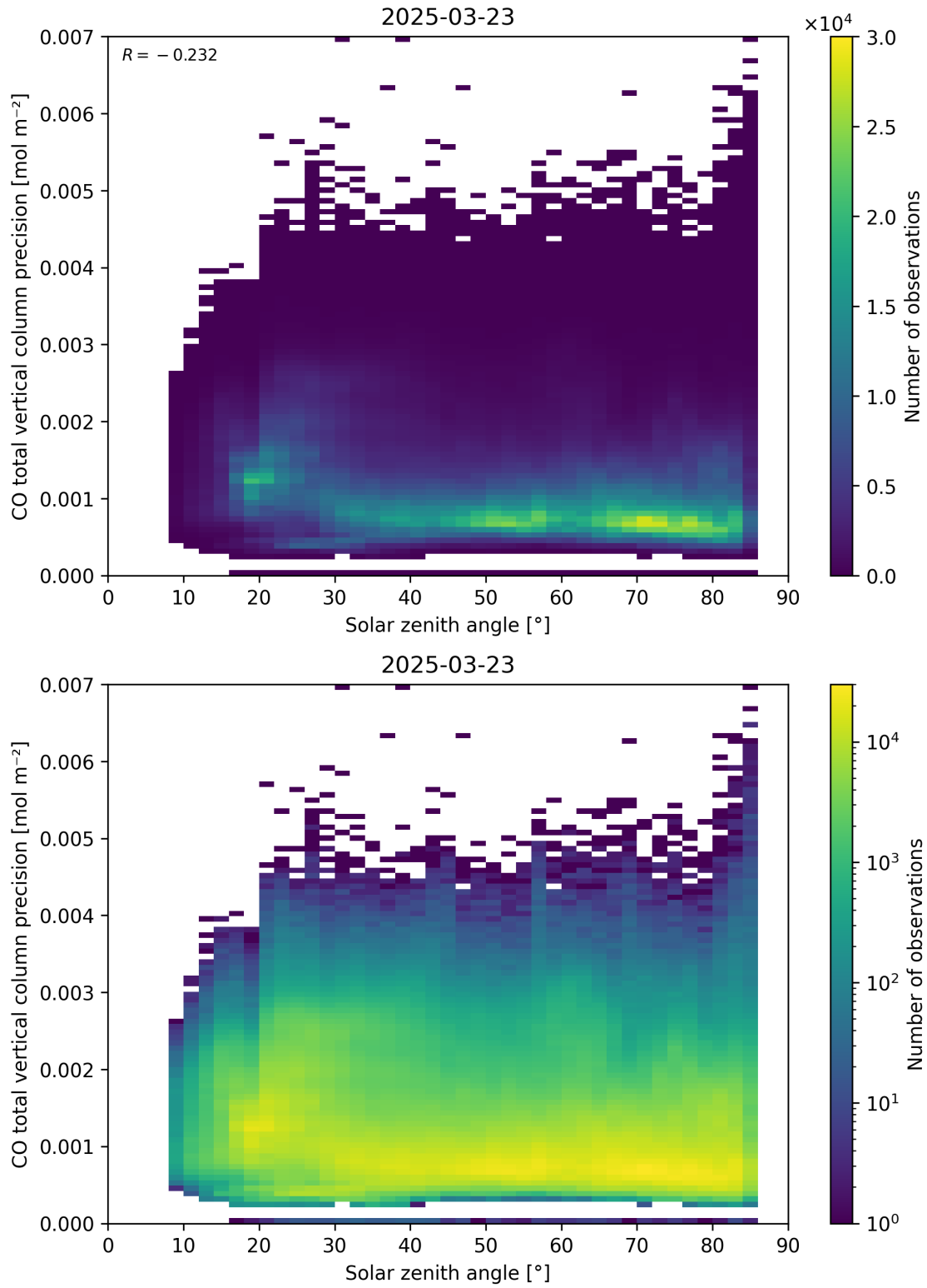
Figure 63: Scatter density plot of “Solar zenith angle” against “CO total vertical column precision” for 2025-03-23 to 2025-03-24.
