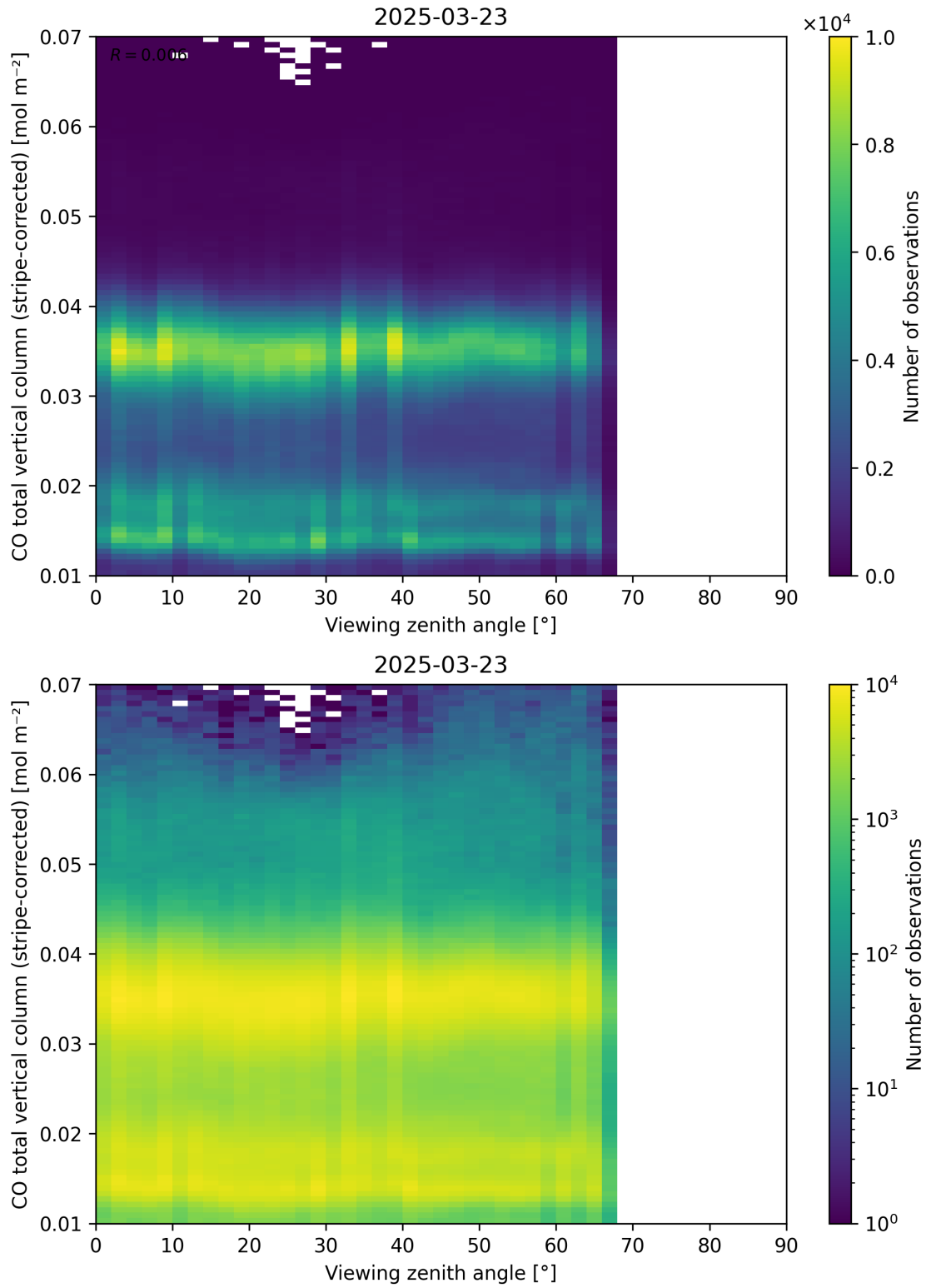
Figure 70: Scatter density plot of “Viewing zenith angle” against “CO total vertical column (stripe-corrected)” for 2025-03-23 to 2025-03-24.
