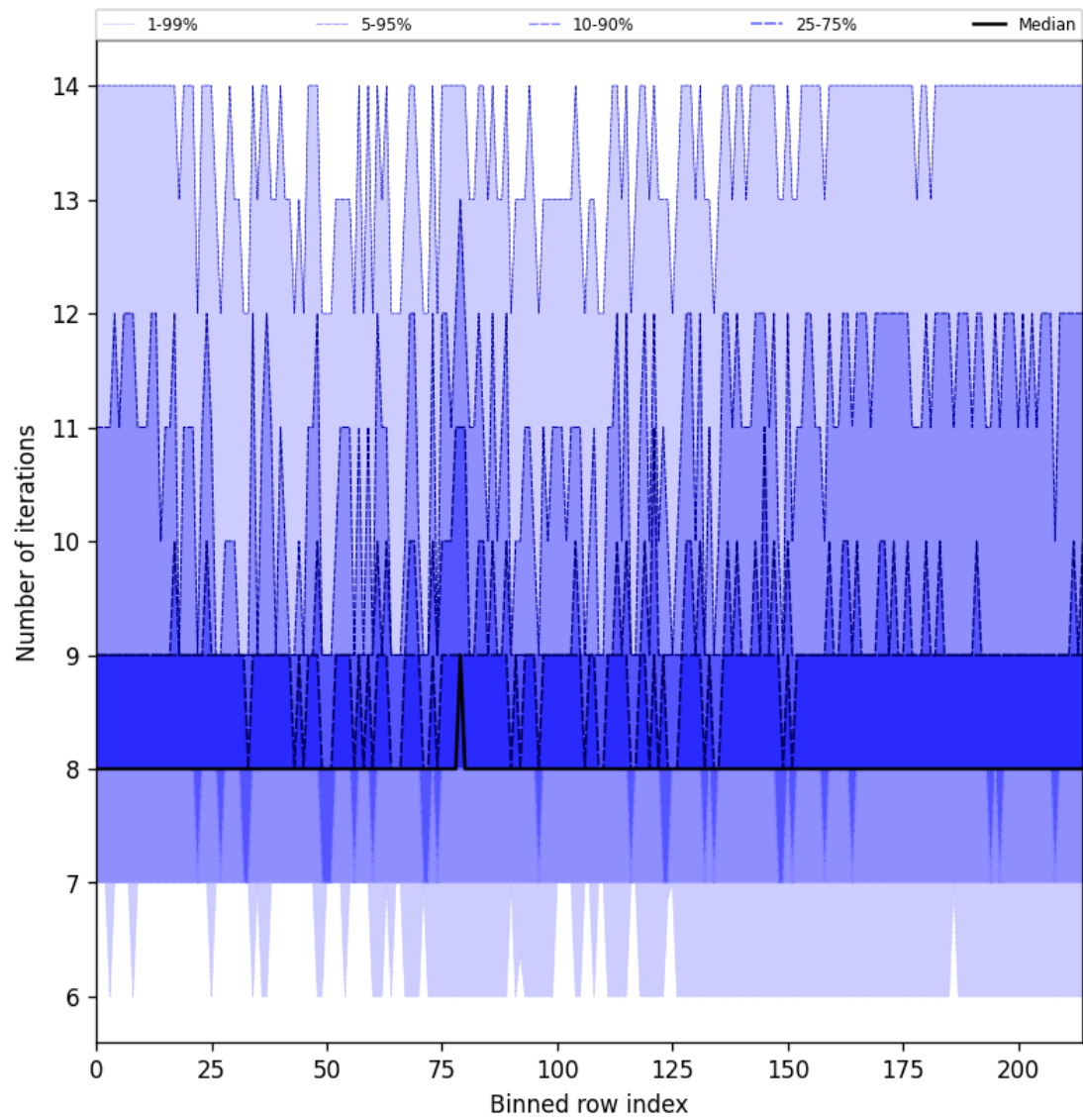
Figure 32: Along track statistics of “Number of iterations” for 2025-03-23 to 2025-03-24
