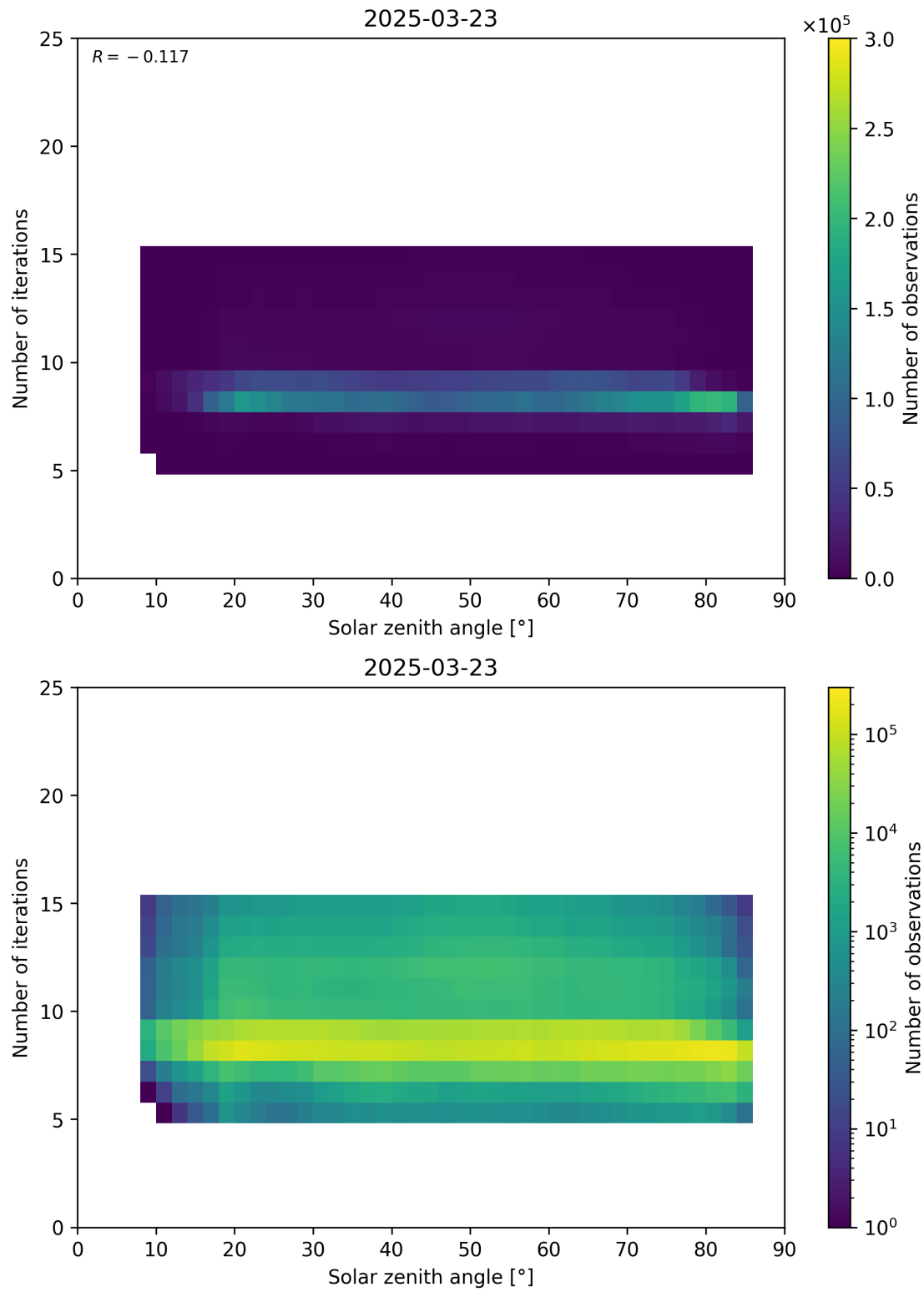
Figure 67: Scatter density plot of “Solar zenith angle” against “Number of iterations” for 2025-03-23 to 2025-03-24.
