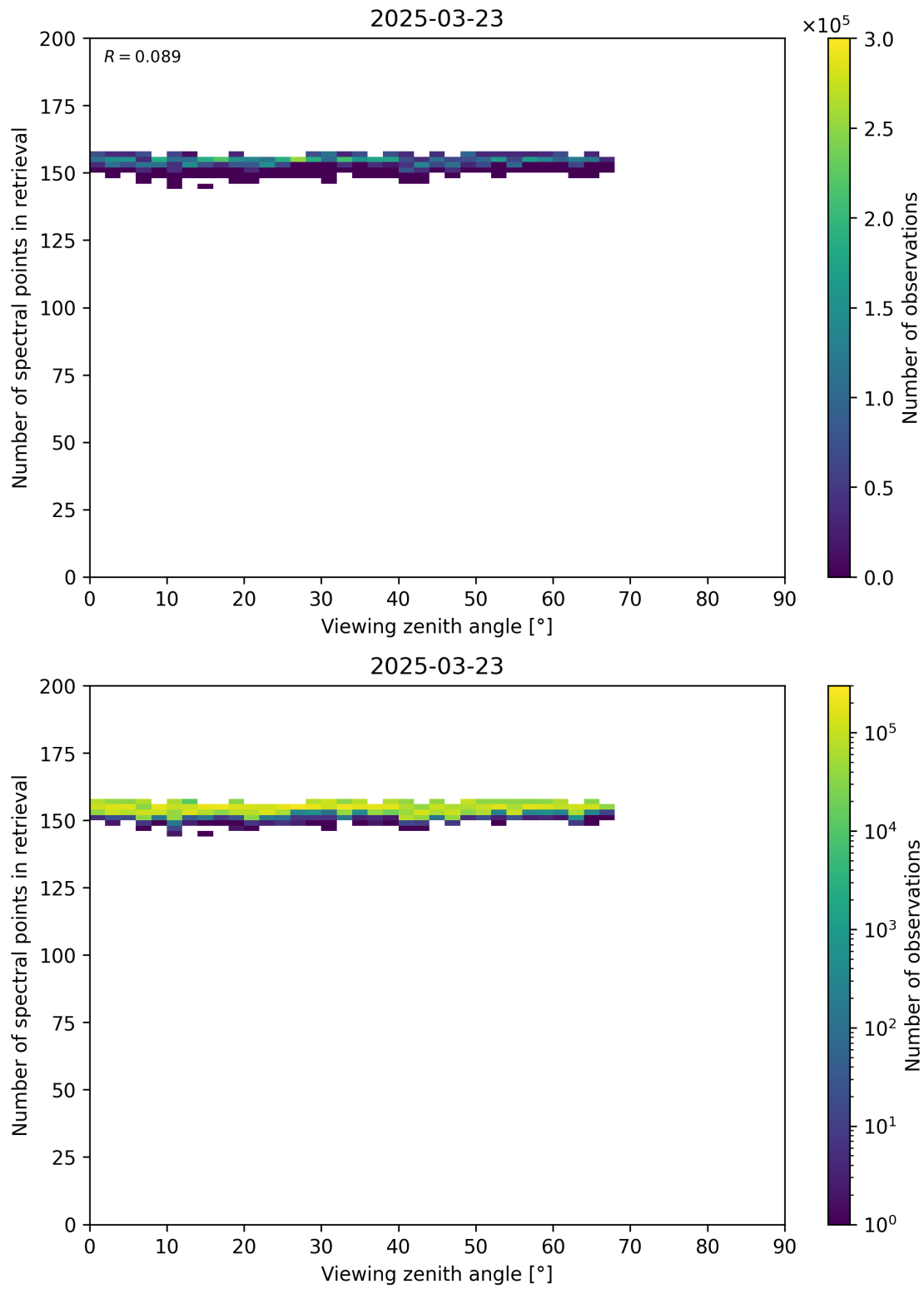
Figure 76: Scatter density plot of “Viewing zenith angle” against “Number of spectral points in retrieval” for 2025-03-23 to 2025-03-24.
