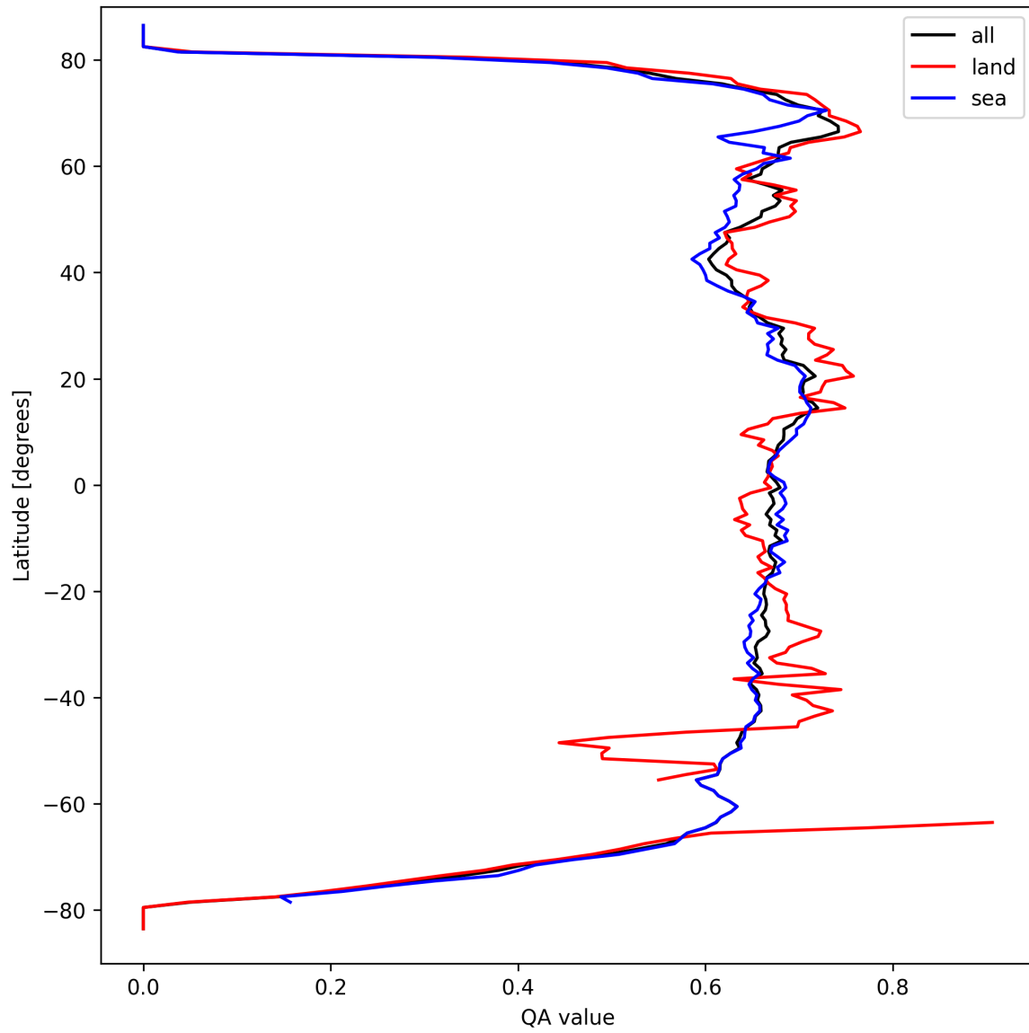
Figure 9: Zonal average of “QA value” for 2025-03-23 to 2025-03-24.
