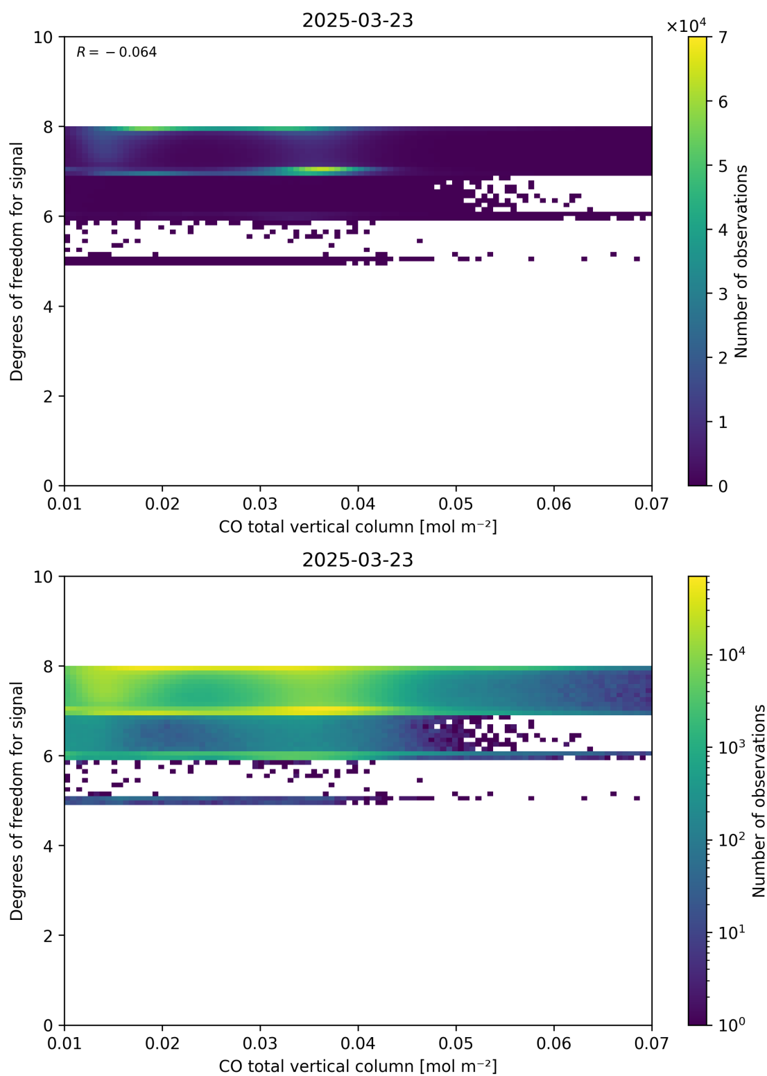
Figure 41: Scatter density plot of “CO total vertical column” against “Degrees of freedom for signal” for 2025-03-23 to 2025-03-24.
