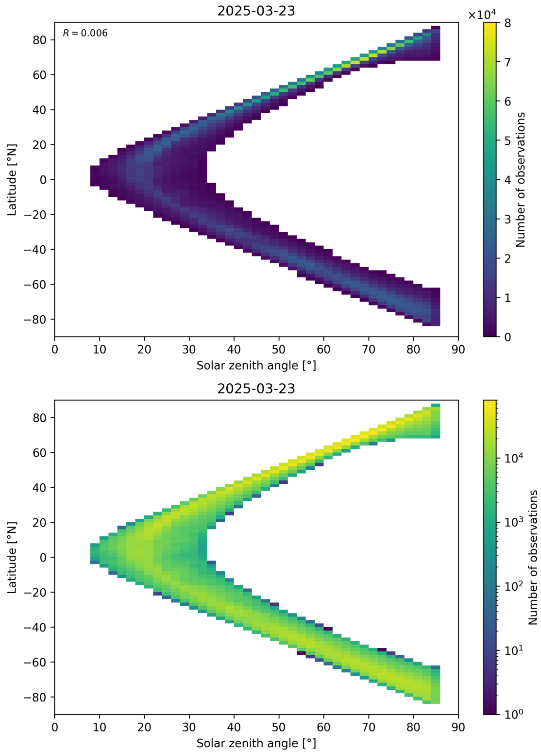
Figure 66: Scatter density plot of “Solar zenith angle” against “Latitude” for 2025-03-23 to 2025-03-24.
