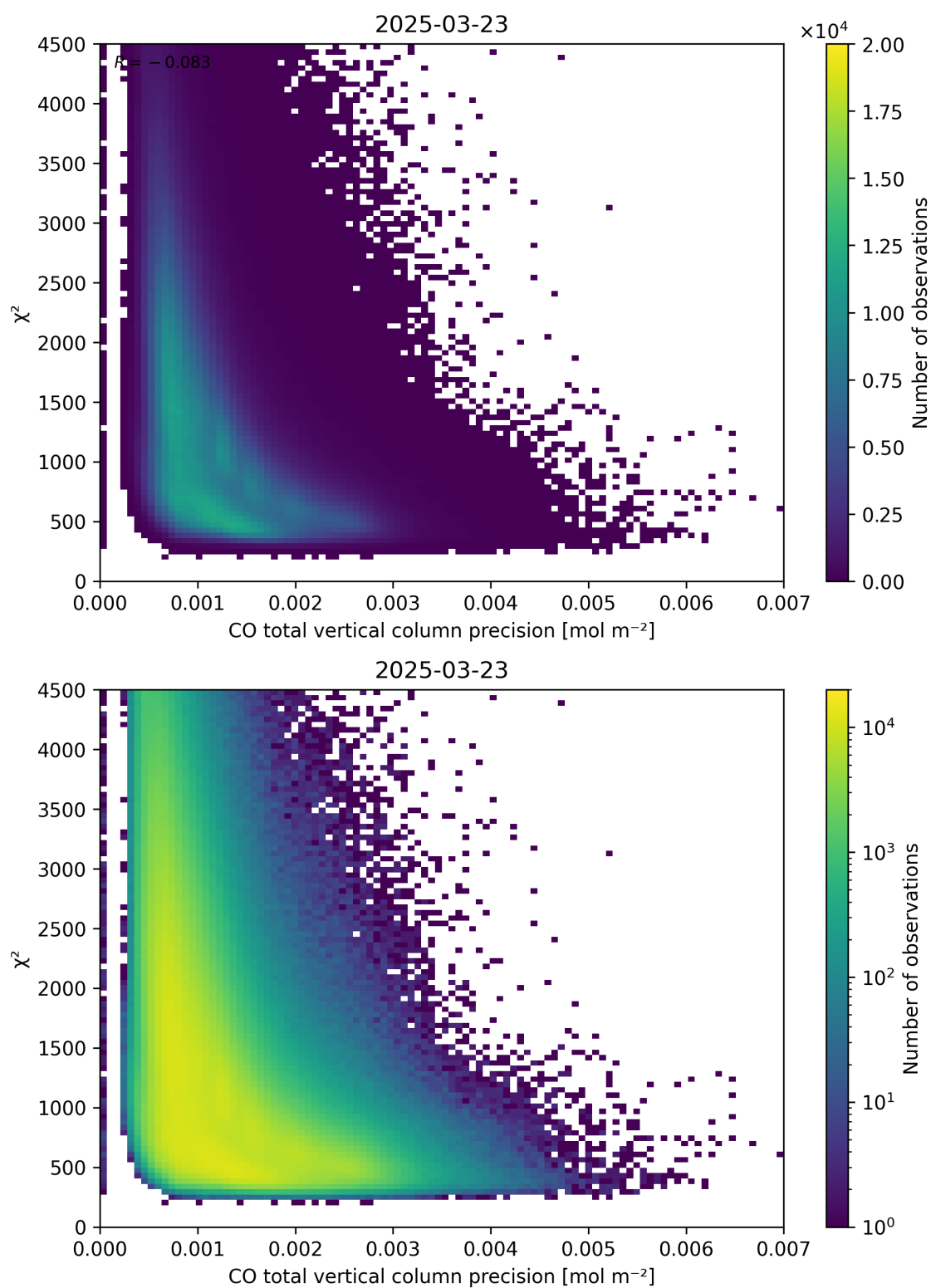
Figure 44: Scatter density plot of “CO total vertical column precision” against “ \chi^2 ” for 2025-03-23 to 2025-03-24.
