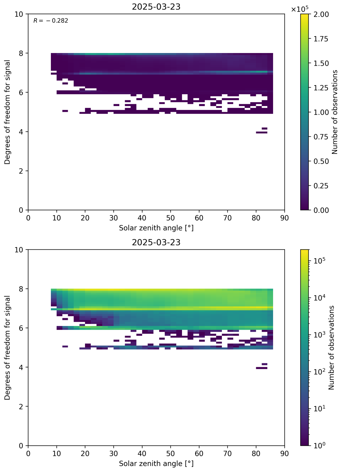
Figure 65: Scatter density plot of “Solar zenith angle” against “Degrees of freedom for signal” for 2025-03-23 to 2025-03-24.
