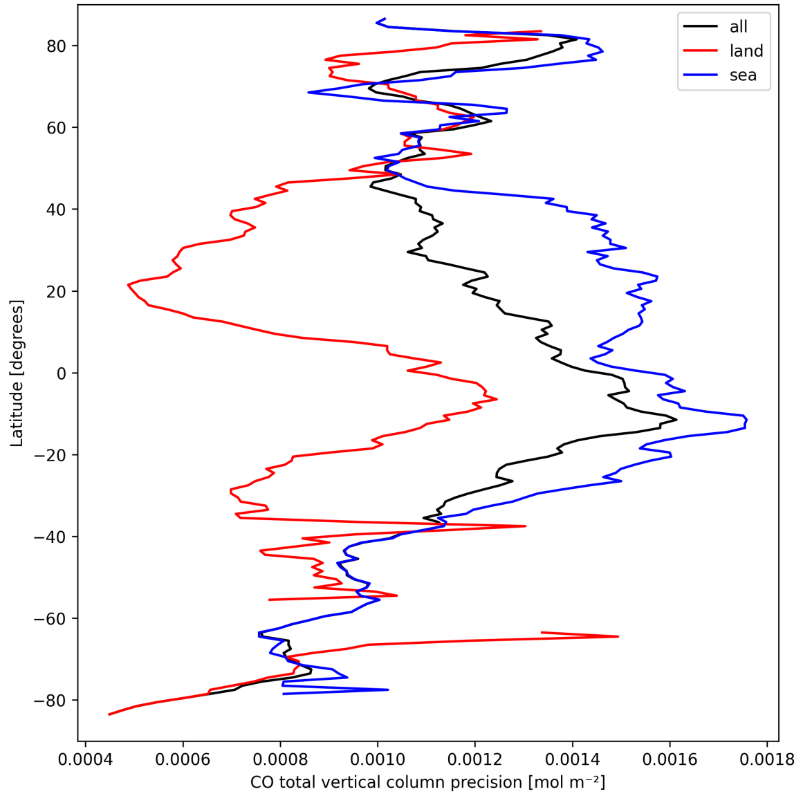
Figure 12: Zonal average of "CO total vertical column precision" for 2025-03-23 to 2025-03-24.
