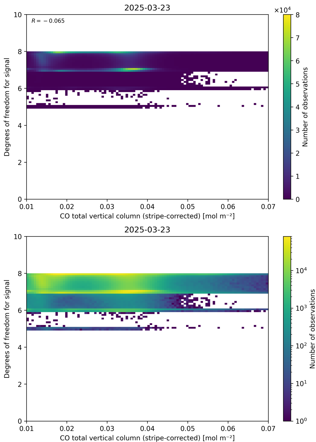
Figure 38: Scatter density plot of “CO total vertical column (stripe-corrected)” against “Degrees of freedom for signal” for 2025-03-23 to 2025-03-24.
