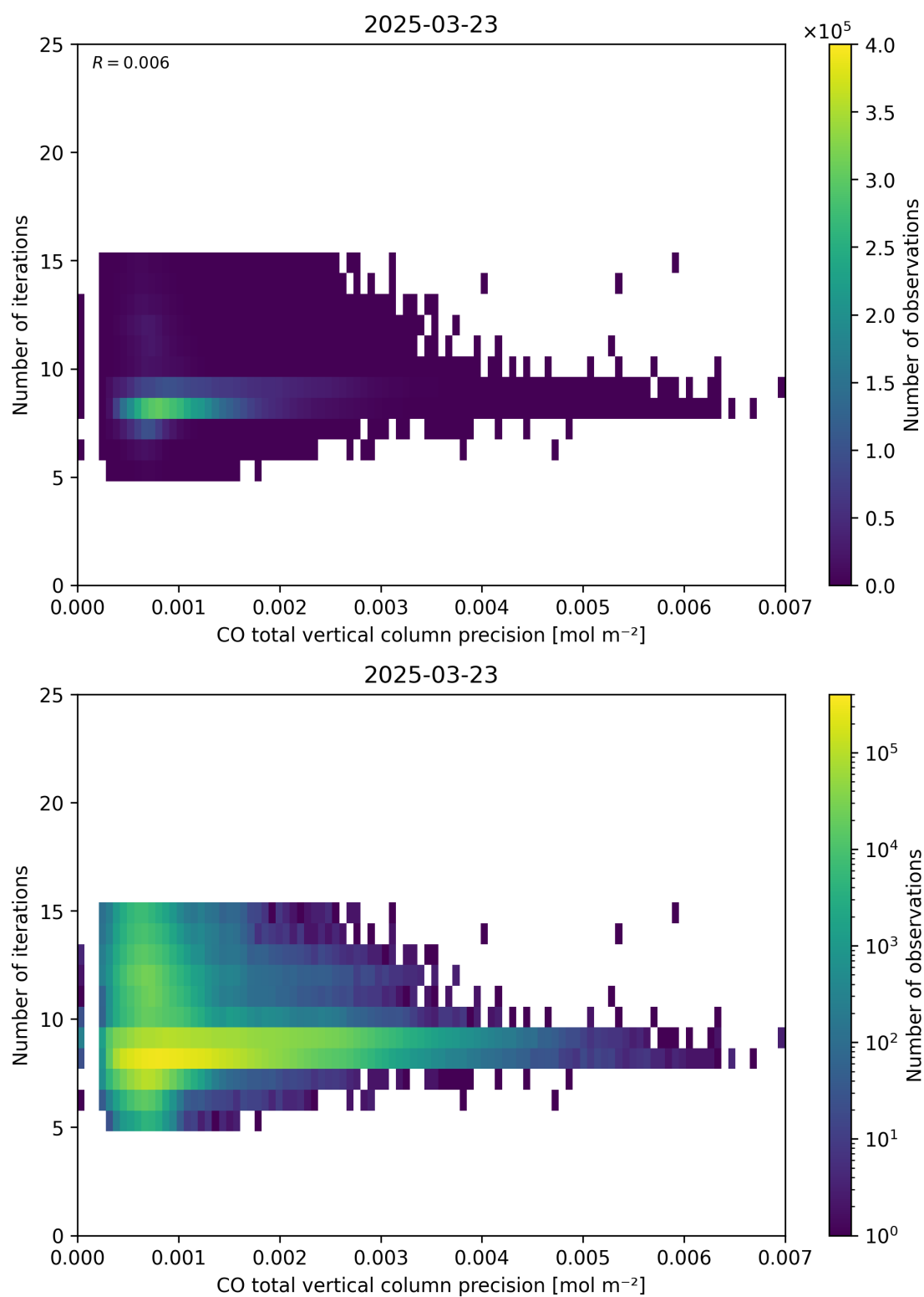
Figure 46: Scatter density plot of “CO total vertical column precision” against “Number of iterations” for 2025-03-23 to 2025-03-24.
