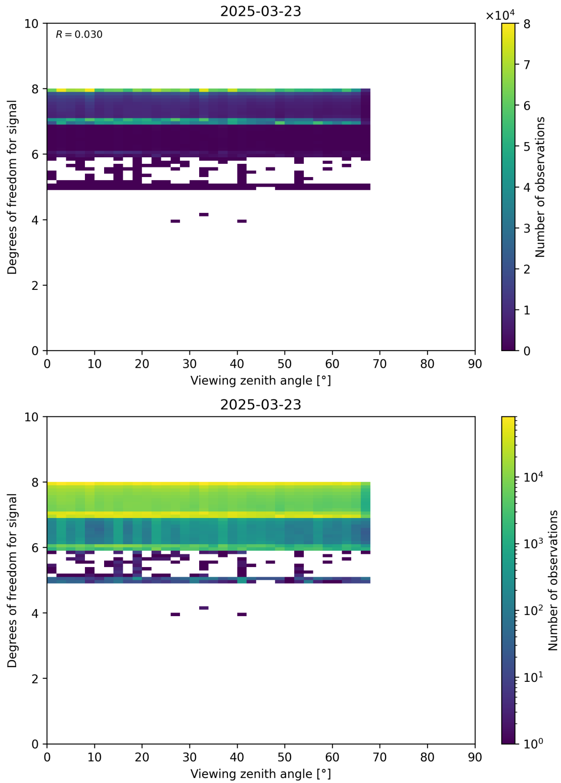
Figure 73: Scatter density plot of “Viewing zenith angle” against “Degrees of freedom for signal” for 2025-03-23 to 2025-03-24.
