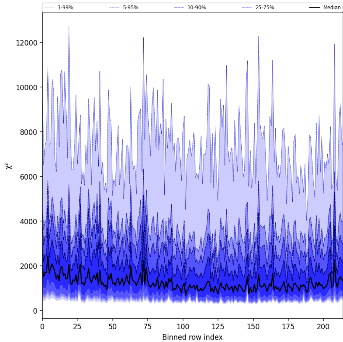
Figure 30: Along track statistics of “ \chi^2 ” for 2025-03-23 to 2025-03-24
