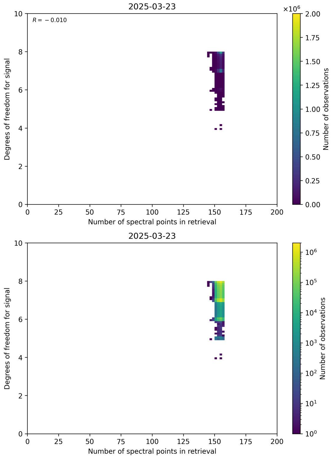
Figure 59: Scatter density plot of “Number of spectral points in retrieval” against “Degrees of freedom for signal” for 2025-03-23 to 2025-03-24.
