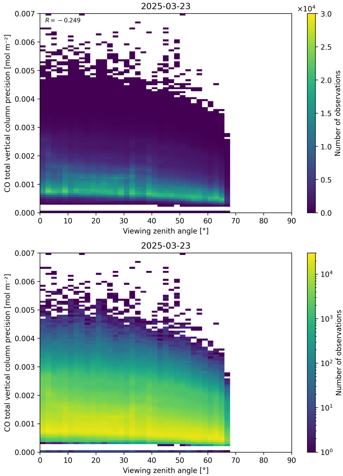
Figure 71: Scatter density plot of “Viewing zenith angle” against “CO total vertical column precision” for 2025-03-23 to 2025-03-24.
