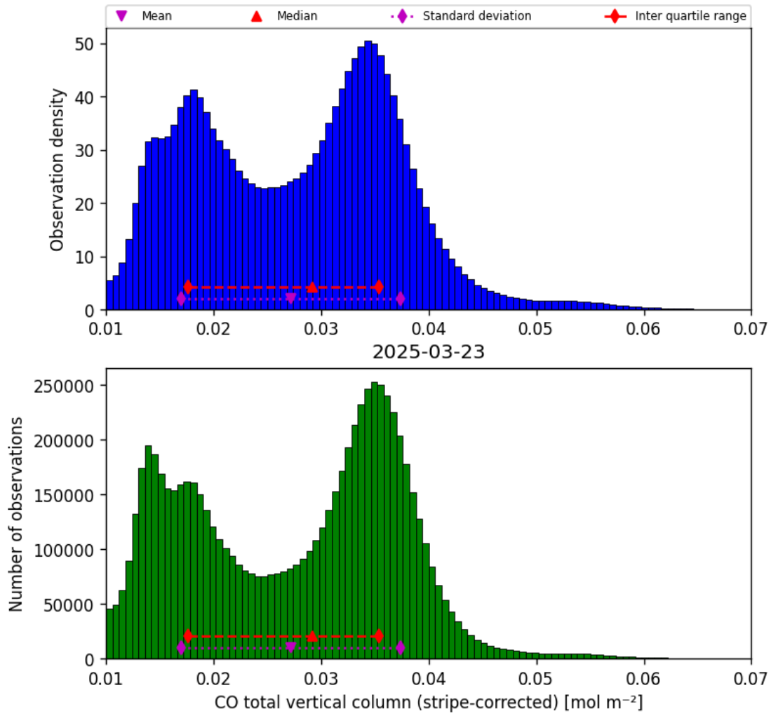
Figure 19: Histogram of “CO total vertical column (stripe-corrected)” for 2025-03-23 to 2025-03-24
