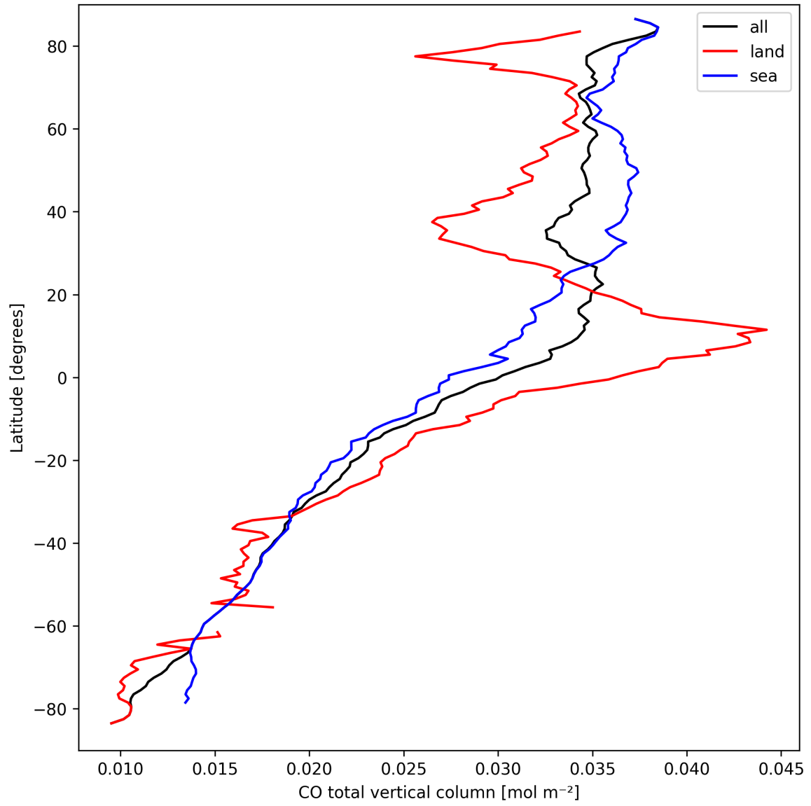
Figure 10: Zonal average of “CO total vertical column” for 2025-03-23 to 2025-03-25.
