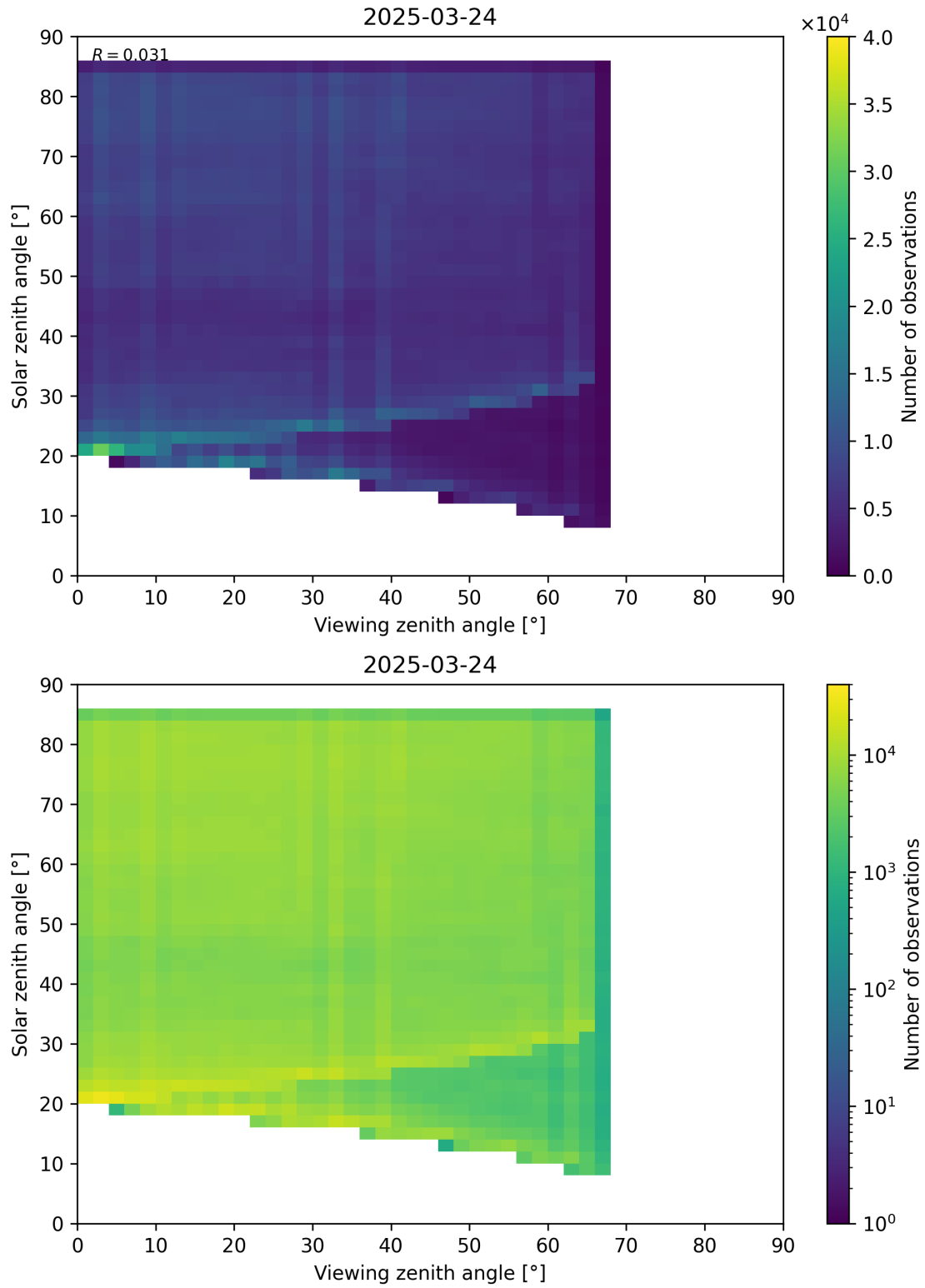
Figure 77: Scatter density plot of “Viewing zenith angle” against “Solar zenith angle” for 2025-03-23 to 2025-03-25.
