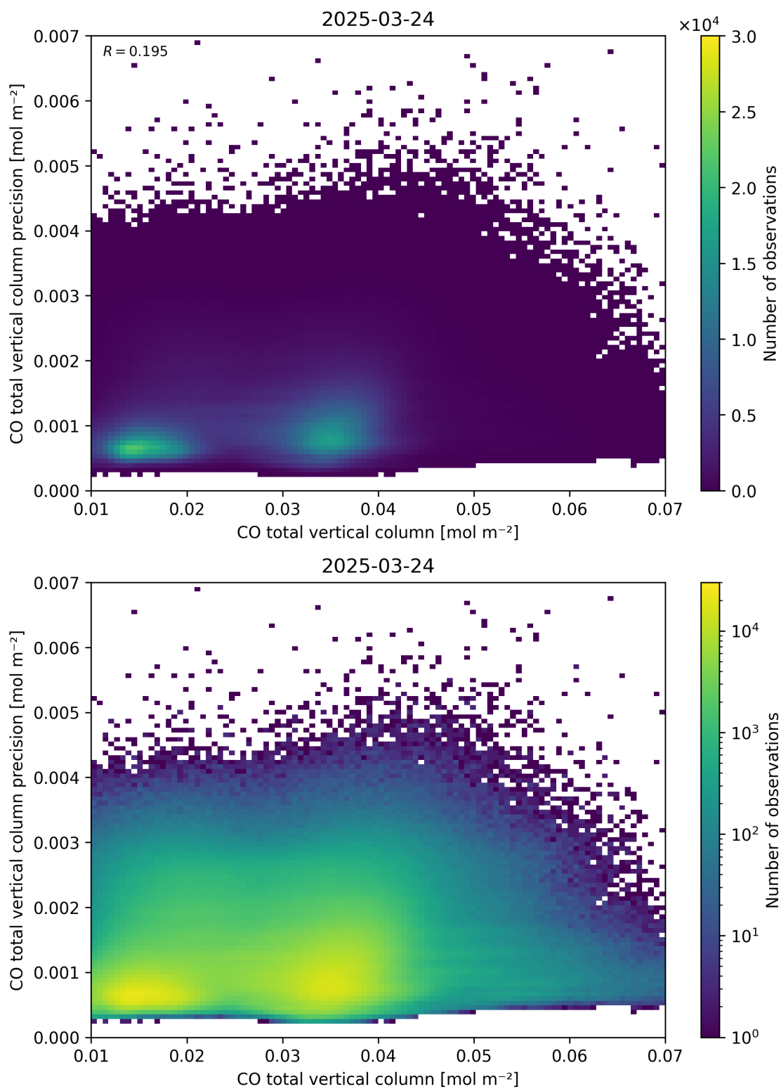
Figure 34: Scatter density plot of “CO total vertical column” against “CO total vertical column precision” for 2025-03-23 to 2025-03-25.
