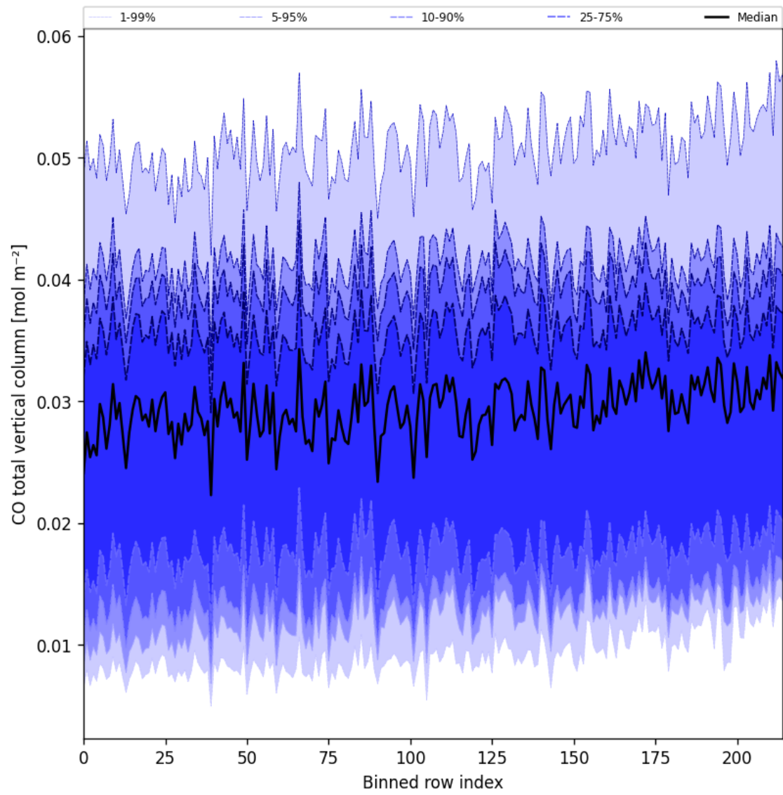
Figure 26: Along track statistics of “CO total vertical column” for 2025-03-23 to 2025-03-25
