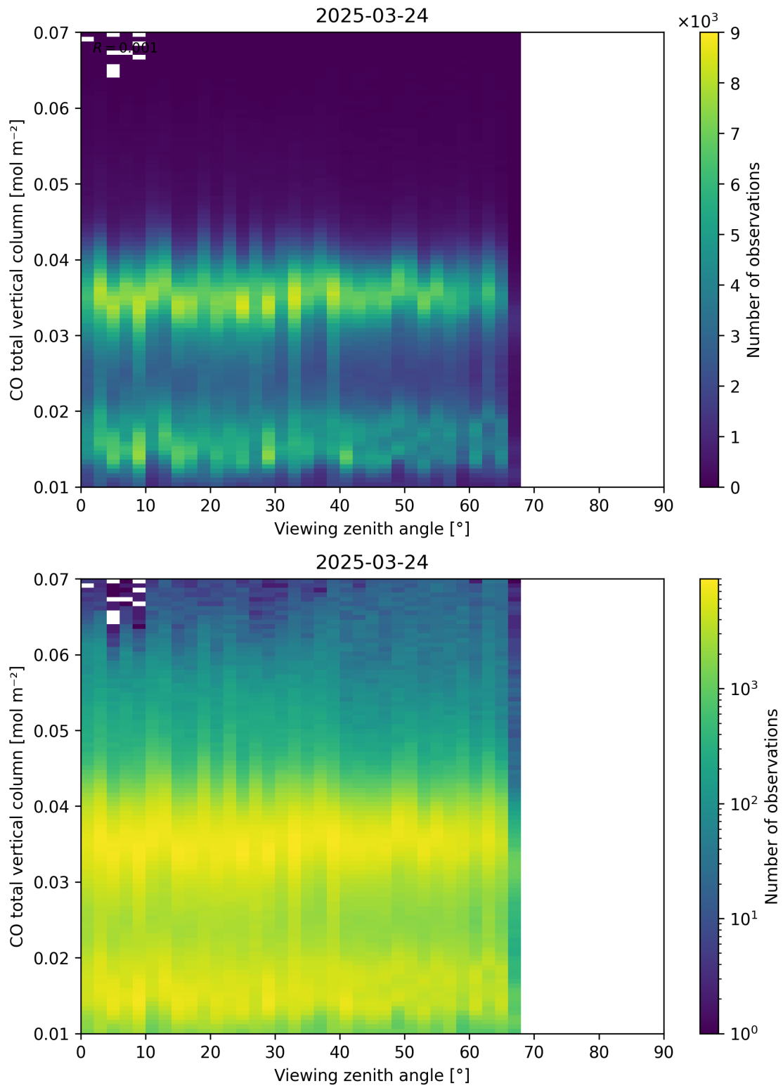
Figure 69: Scatter density plot of “Viewing zenith angle” against “CO total vertical column” for 2025-03-23 to 2025-03-25.
