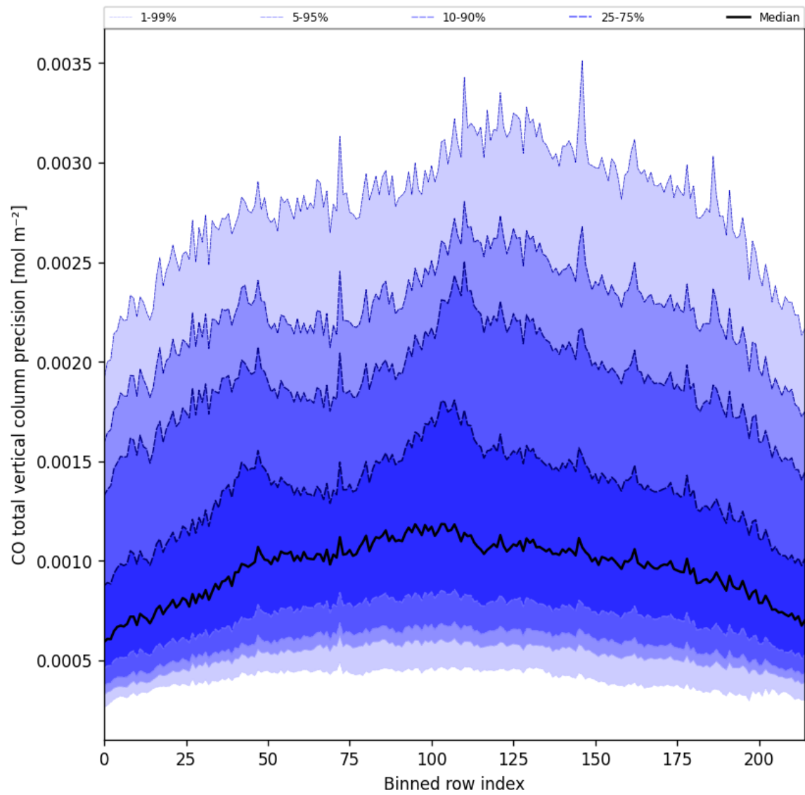
Figure 28: Along track statistics of “CO total vertical column precision” for 2025-03-23 to 2025-03-25
