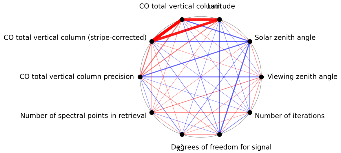
Figure 1: Map of correlation graph for 2025-03-23 to 2025-03-25.
