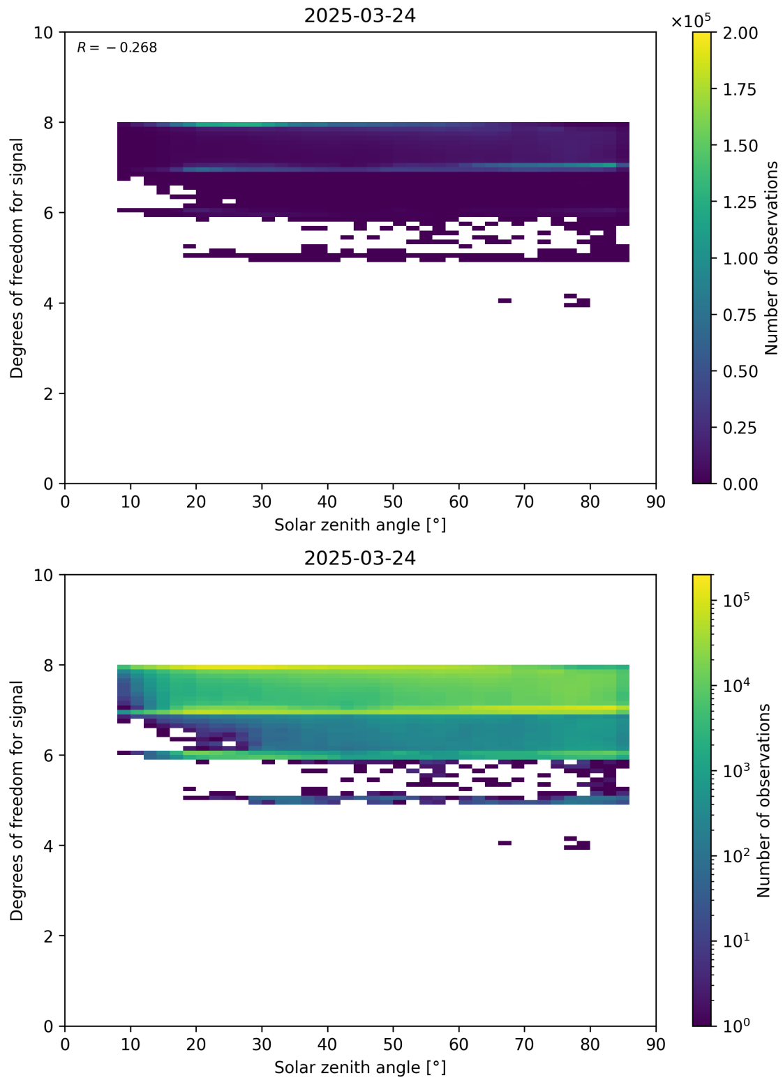
Figure 65: Scatter density plot of “Solar zenith angle” against “Degrees of freedom for signal” for 2025-03-23 to 2025-03-25.
