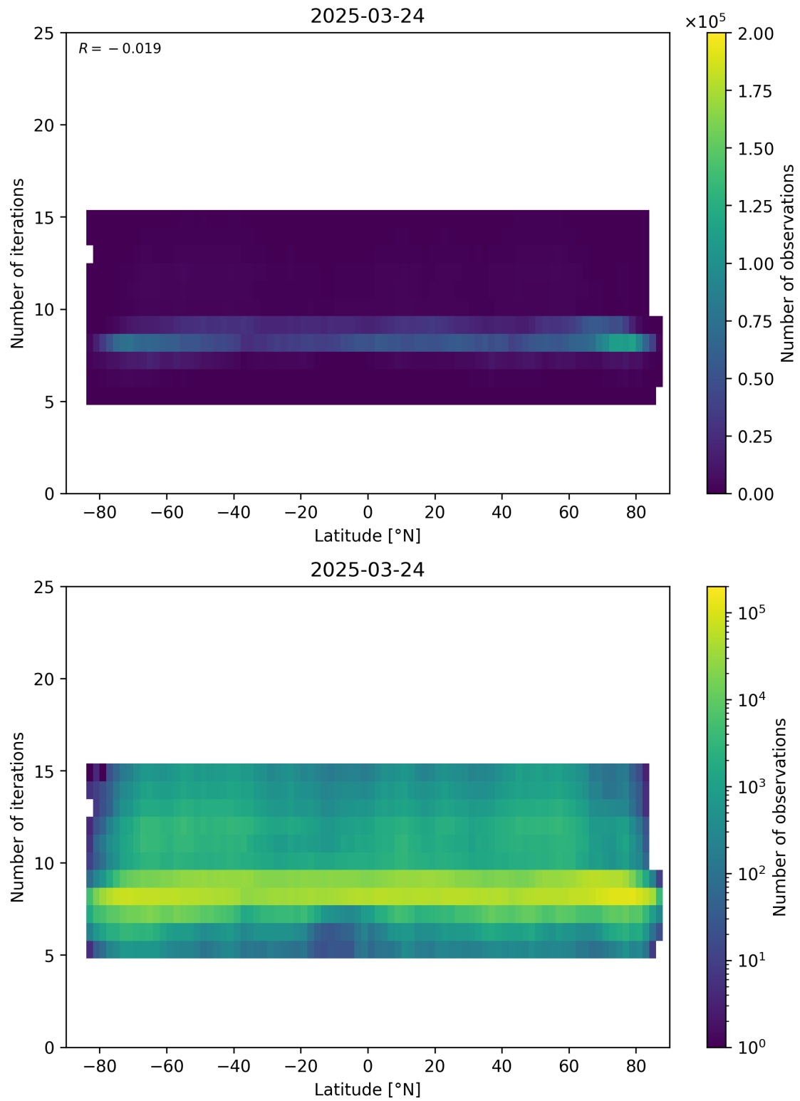
Figure 56: Scatter density plot of “Latitude” against “Number of iterations” for 2025-03-23 to 2025-03-25.
