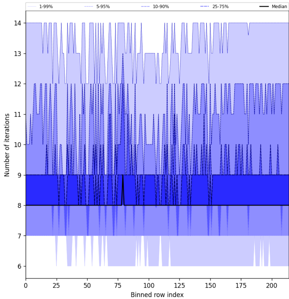
Figure 32: Along track statistics of “Number of iterations” for 2025-03-23 to 2025-03-25
