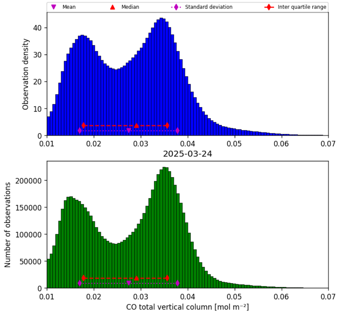
Figure 18: Histogram of “CO total vertical column” for 2025-03-23 to 2025-03-25
