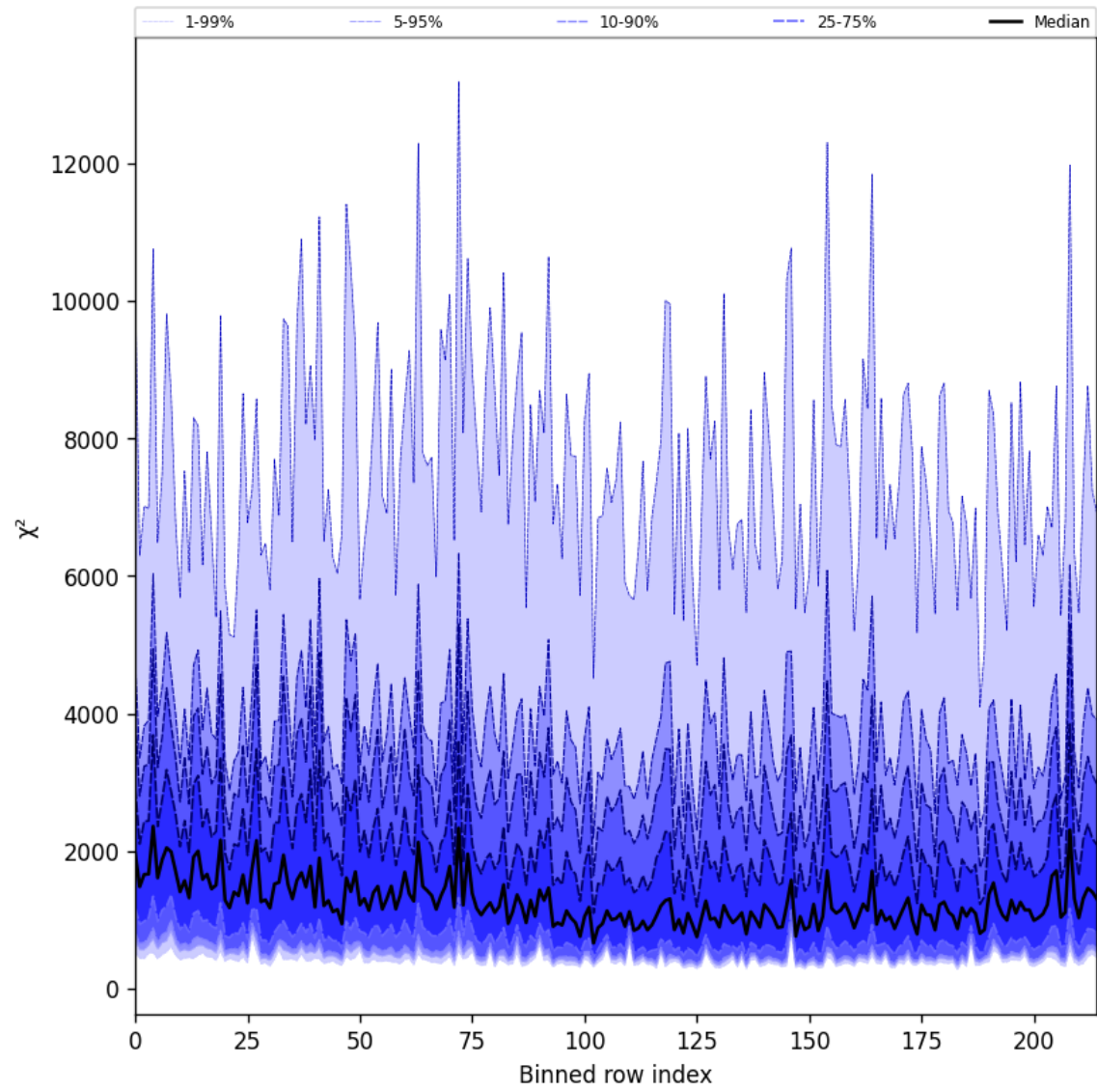
Figure 30: Along track statistics of “ \chi^2 ” for 2025-03-23 to 2025-03-25
