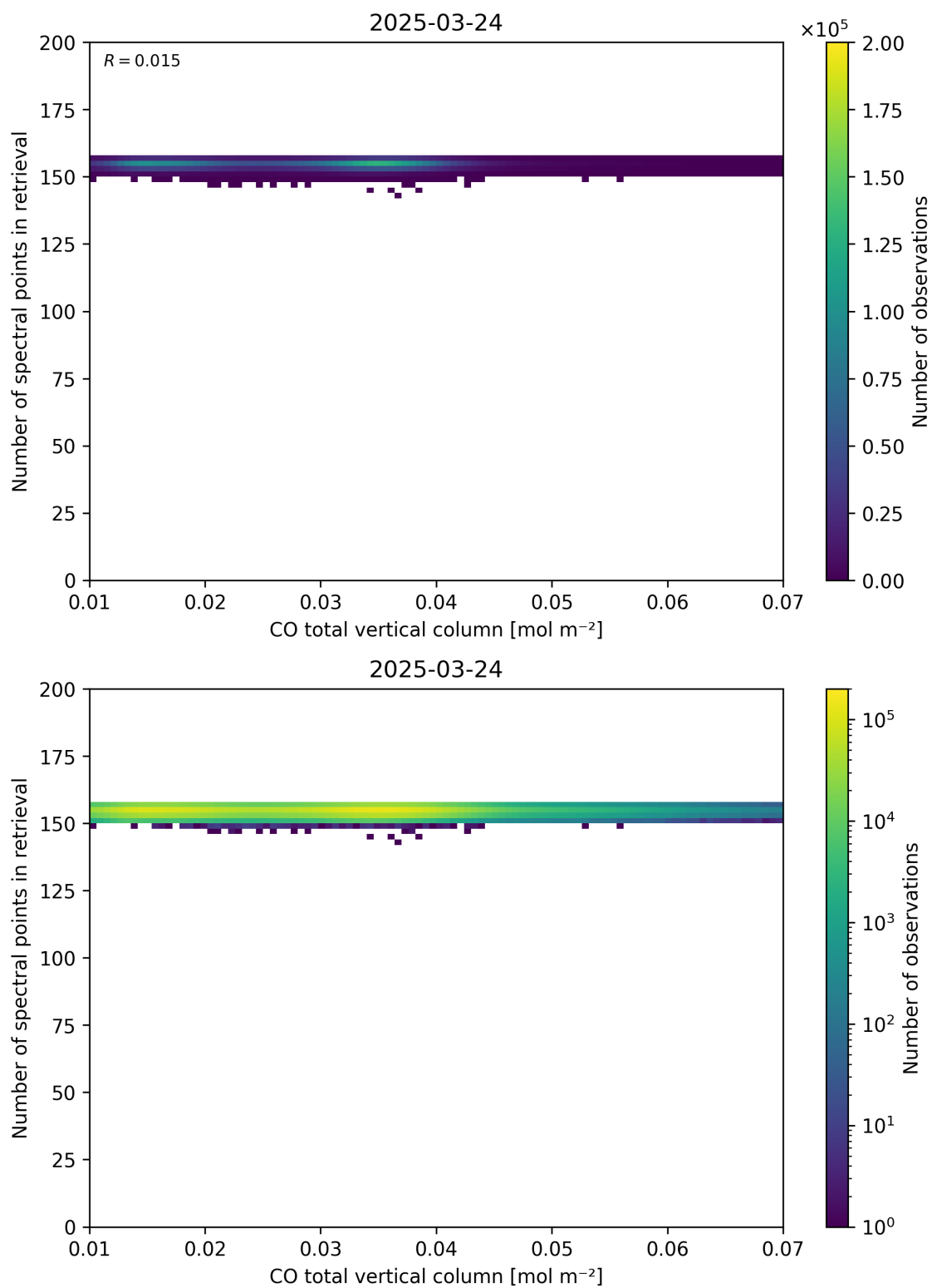
Figure 43: Scatter density plot of “CO total vertical column” against “Number of spectral points in retrieval” for 2025-03-23 to 2025-03-25.
