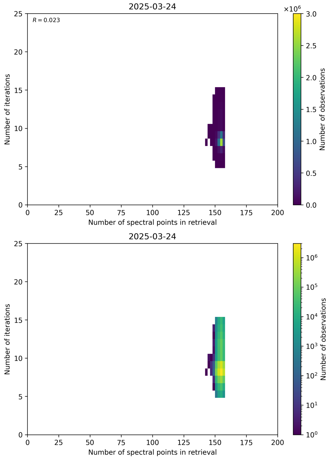
Figure 60: Scatter density plot of “Number of spectral points in retrieval” against “Number of iterations” for 2025-03-23 to 2025-03-25.
