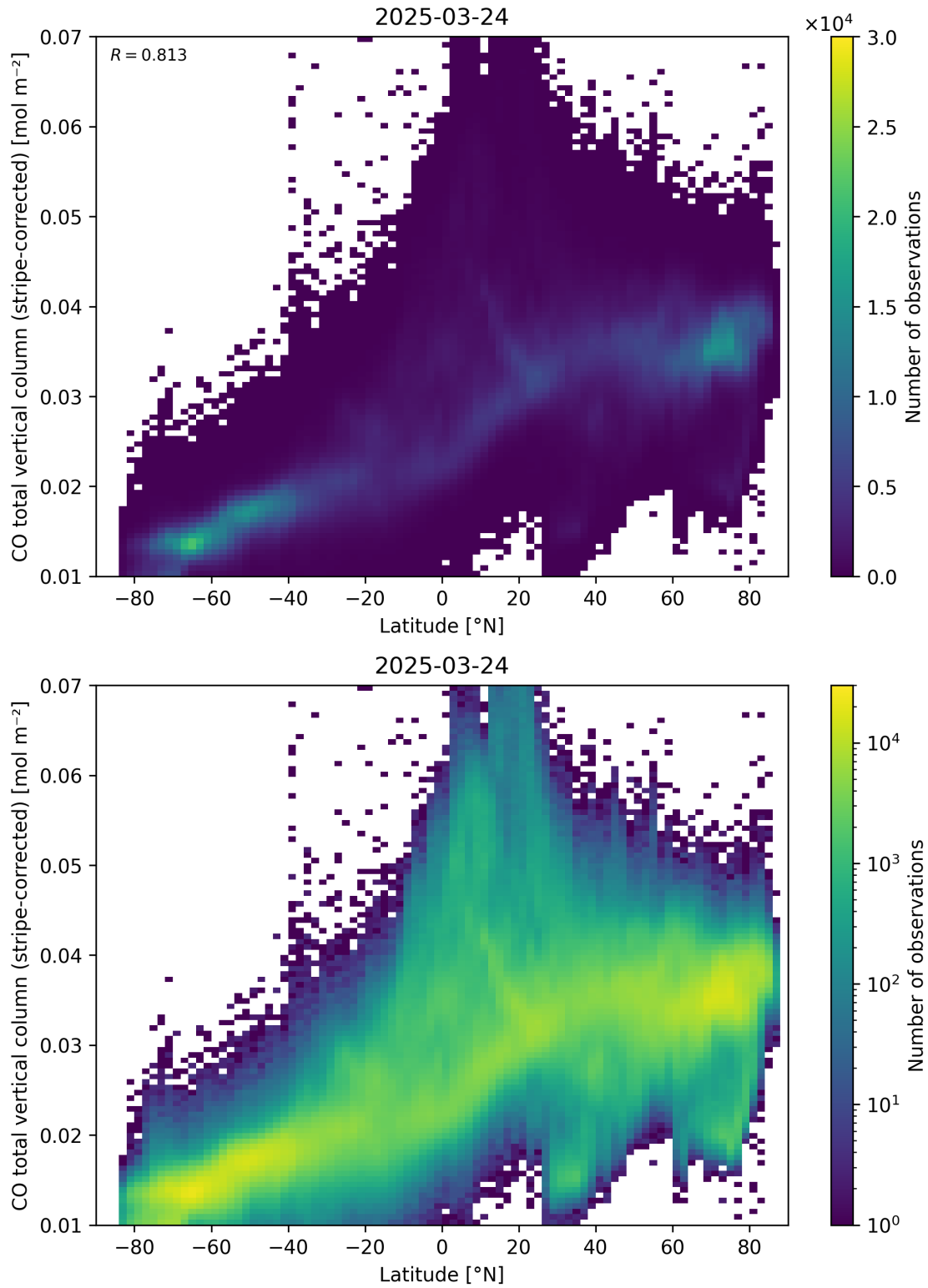
Figure 52: Scatter density plot of “Latitude” against “CO total vertical column (stripe-corrected)” for 2025-03-23 to 2025-03-25.
