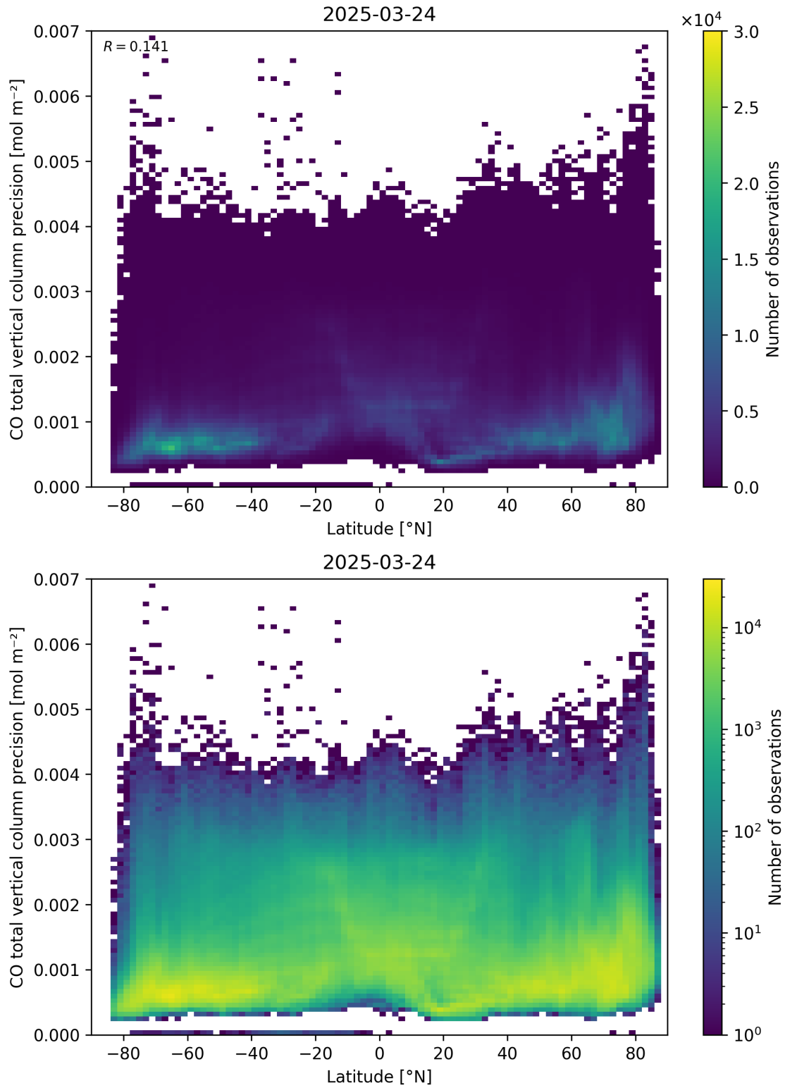
Figure 53: Scatter density plot of “Latitude” against “CO total vertical column precision” for 2025-03-23 to 2025-03-25.
