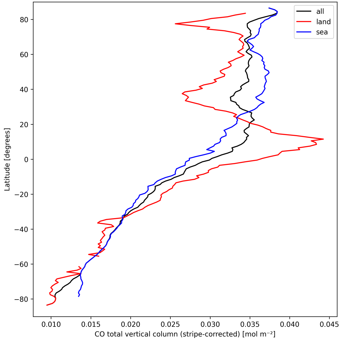
Figure 11: Zonal average of “CO total vertical column (stripe-corrected)” for 2025-03-23 to 2025-03-25.
