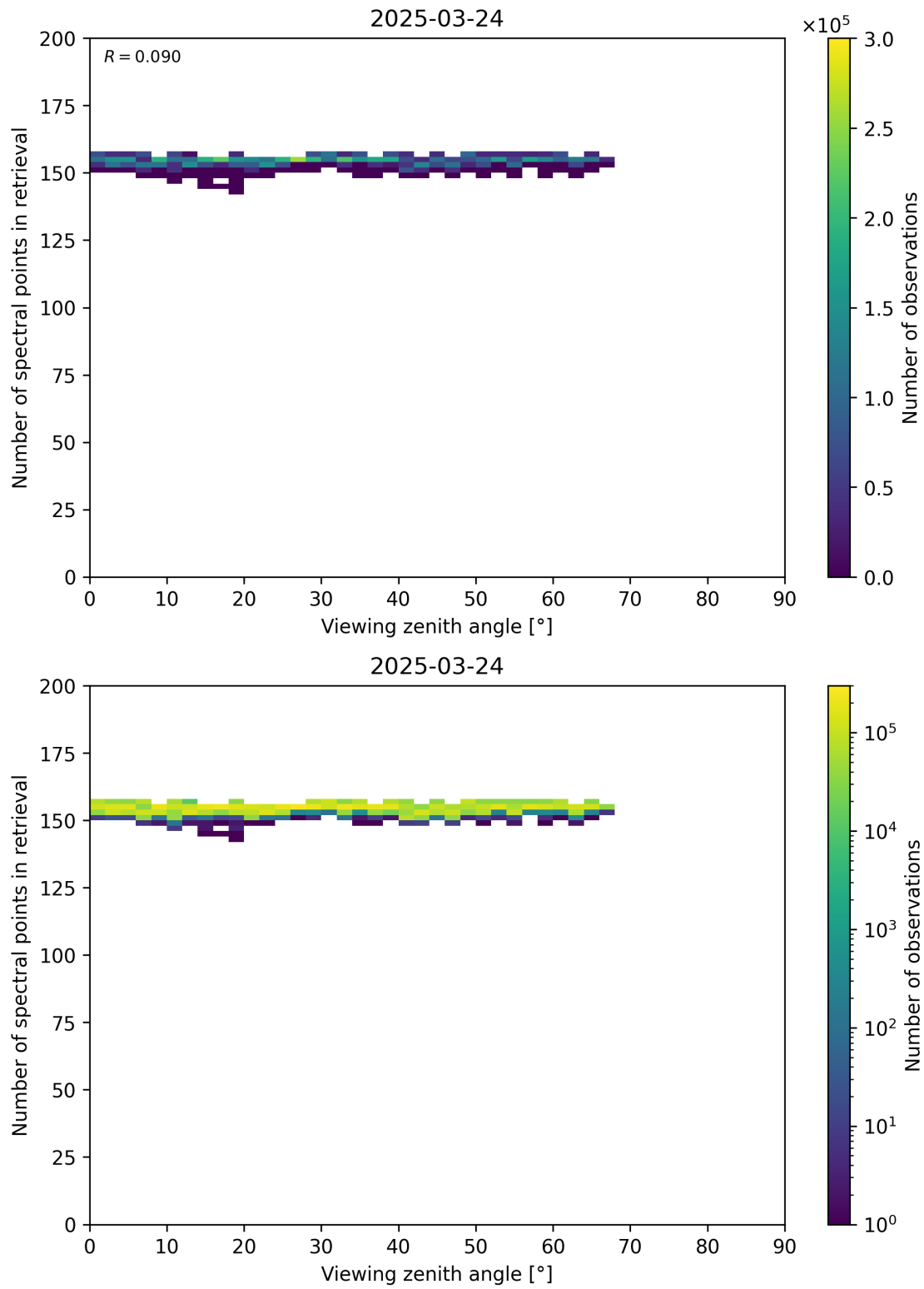
Figure 76: Scatter density plot of “Viewing zenith angle” against “Number of spectral points in retrieval” for 2025-03-23 to 2025-03-25.
