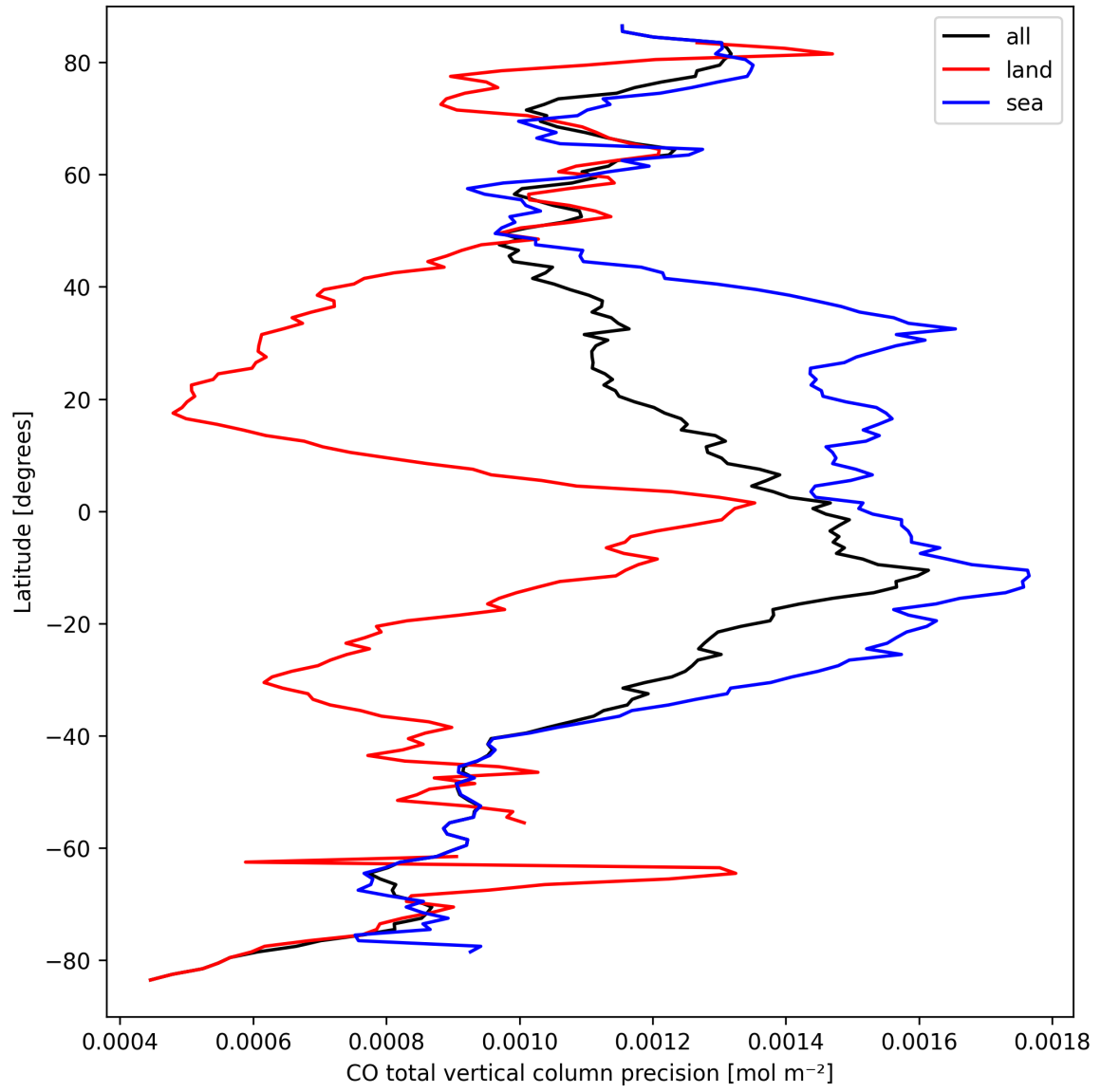
Figure 12: Zonal average of “CO total vertical column precision” for 2025-03-23 to 2025-03-25.
