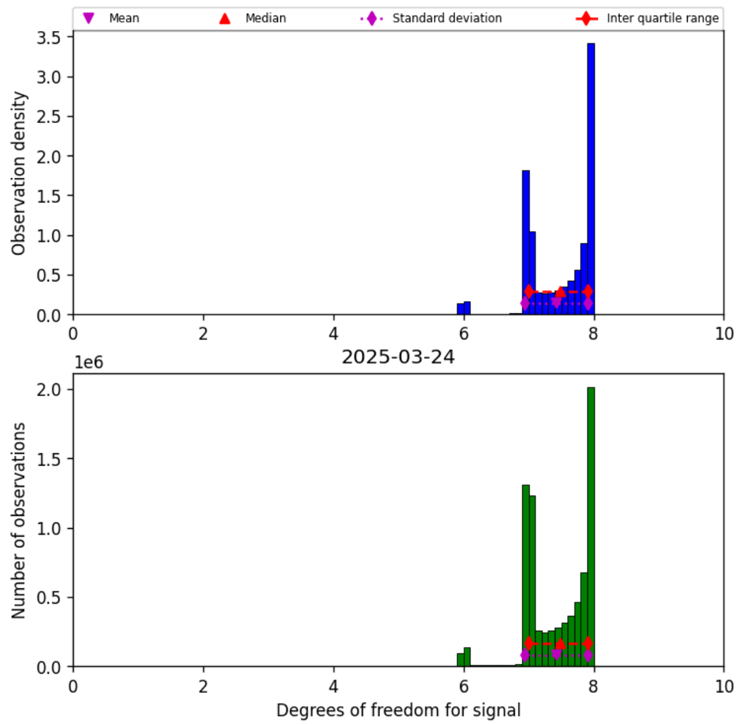
Figure 23: Histogram of “Degrees of freedom for signal” for 2025-03-23 to 2025-03-25
