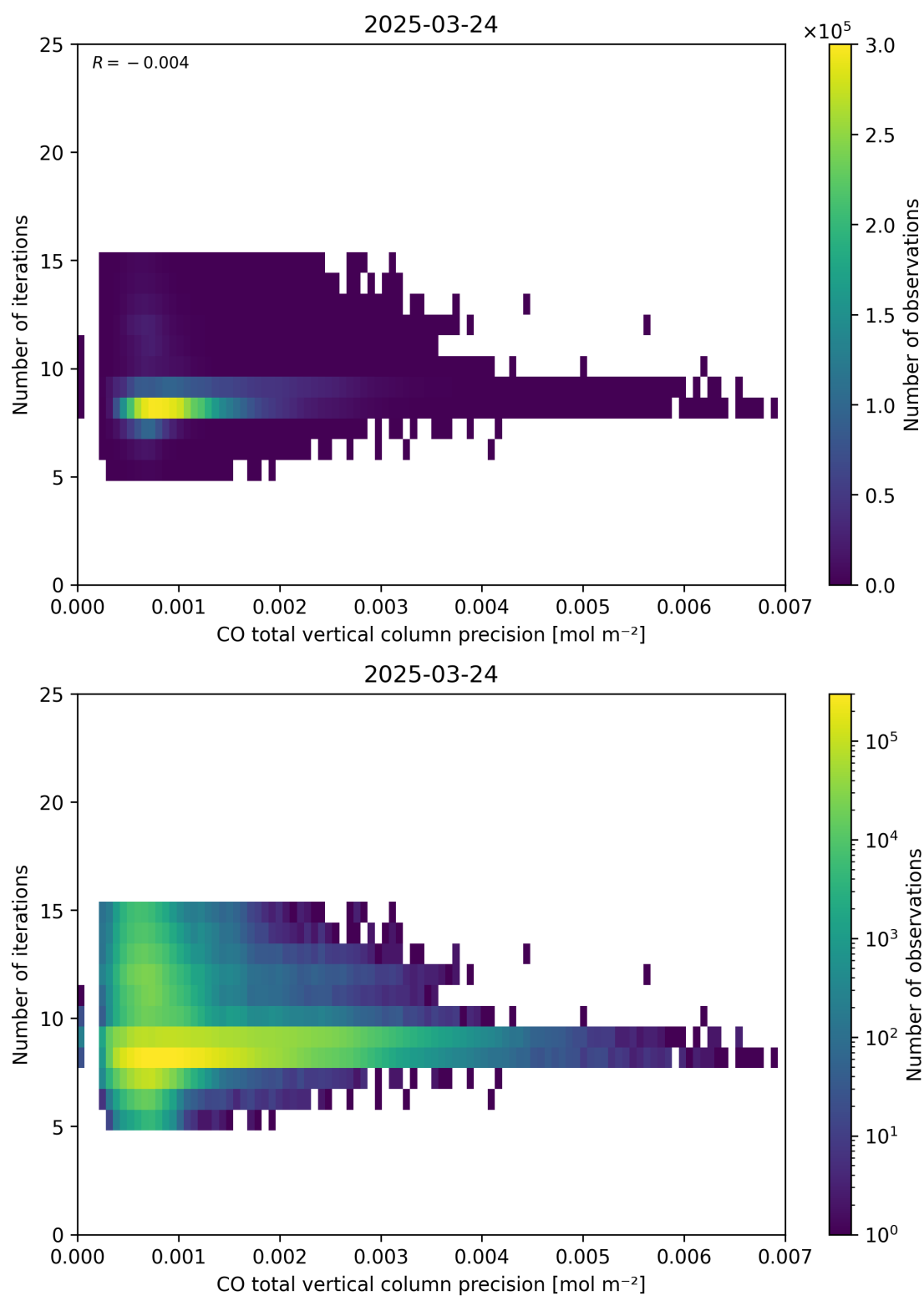
Figure 46: Scatter density plot of “CO total vertical column precision” against “Number of iterations” for 2025-03-23 to 2025-03-25.
