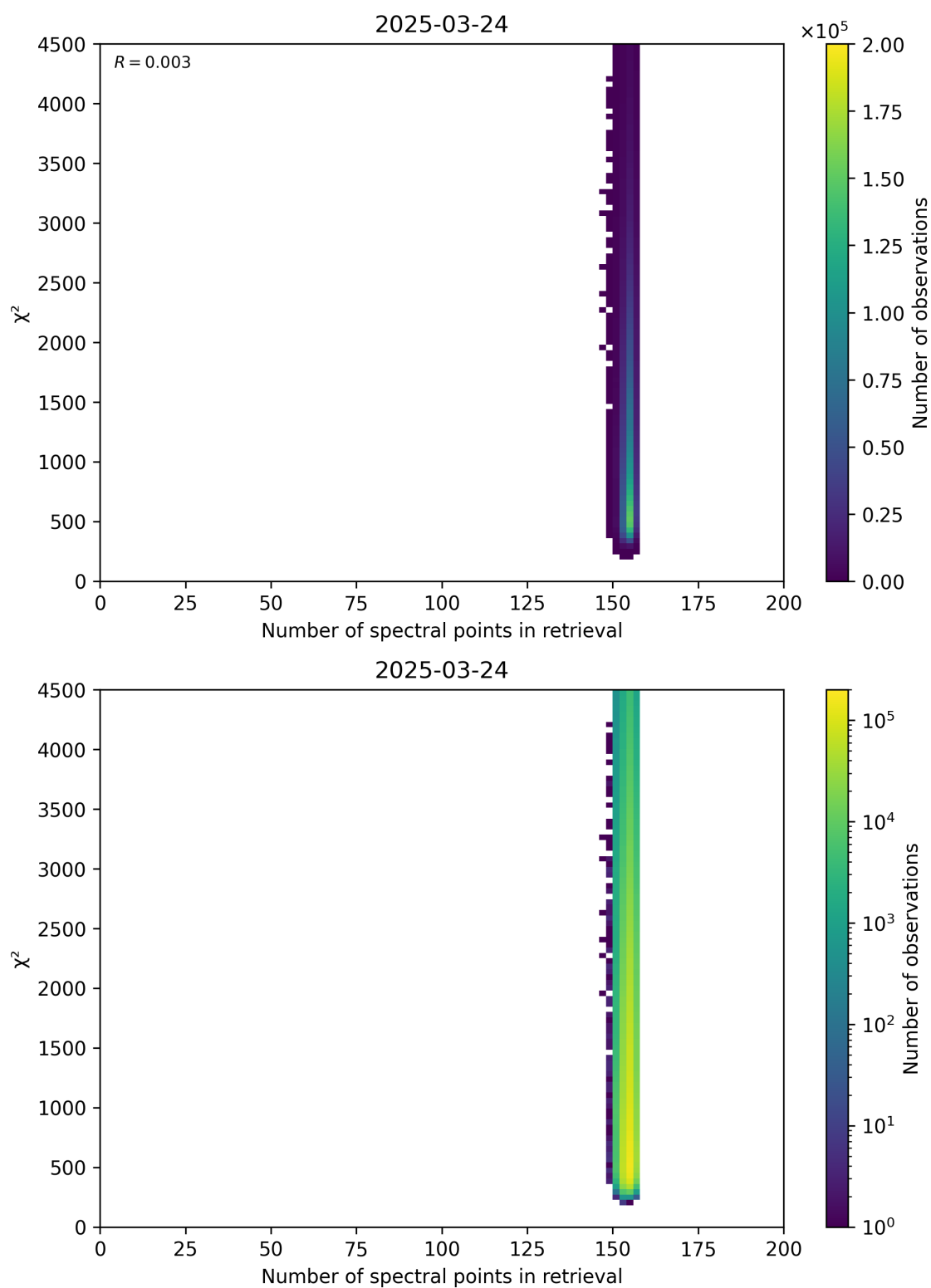
Figure 58: Scatter density plot of “Number of spectral points in retrieval” against “ \chi^2 ” for 2025-03-23 to 2025-03-25.
