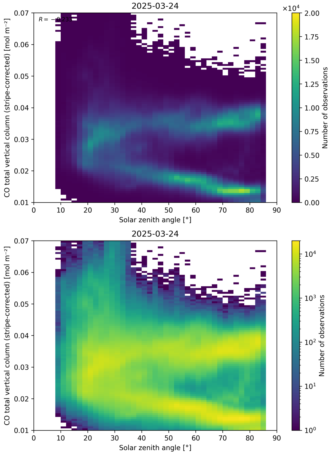
Figure 62: Scatter density plot of “Solar zenith angle” against “CO total vertical column (stripe-corrected)” for 2025-03-23 to 2025-03-25.
