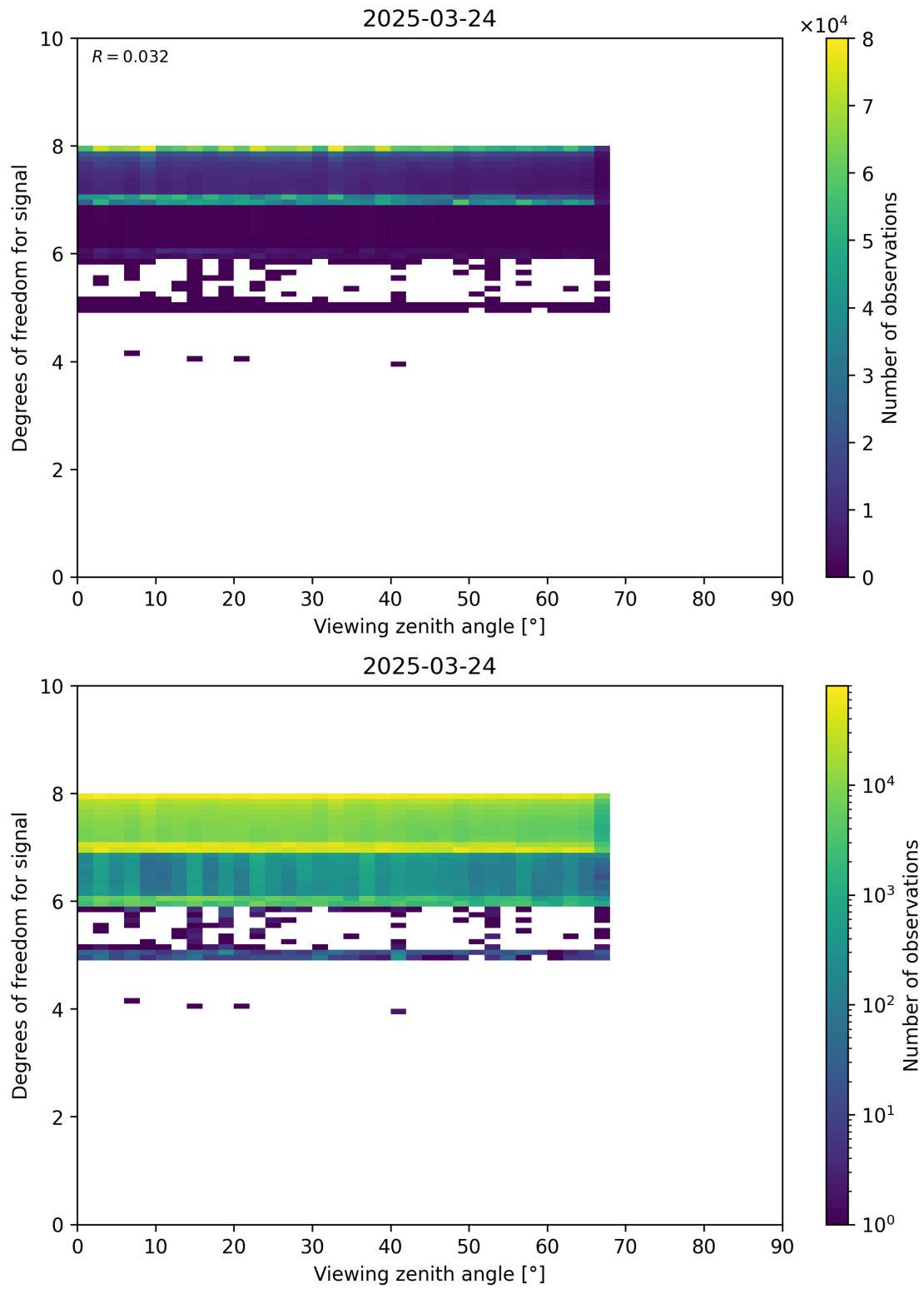
Figure 73: Scatter density plot of “Viewing zenith angle” against “Degrees of freedom for signal” for 2025-03-23 to 2025-03-25.
