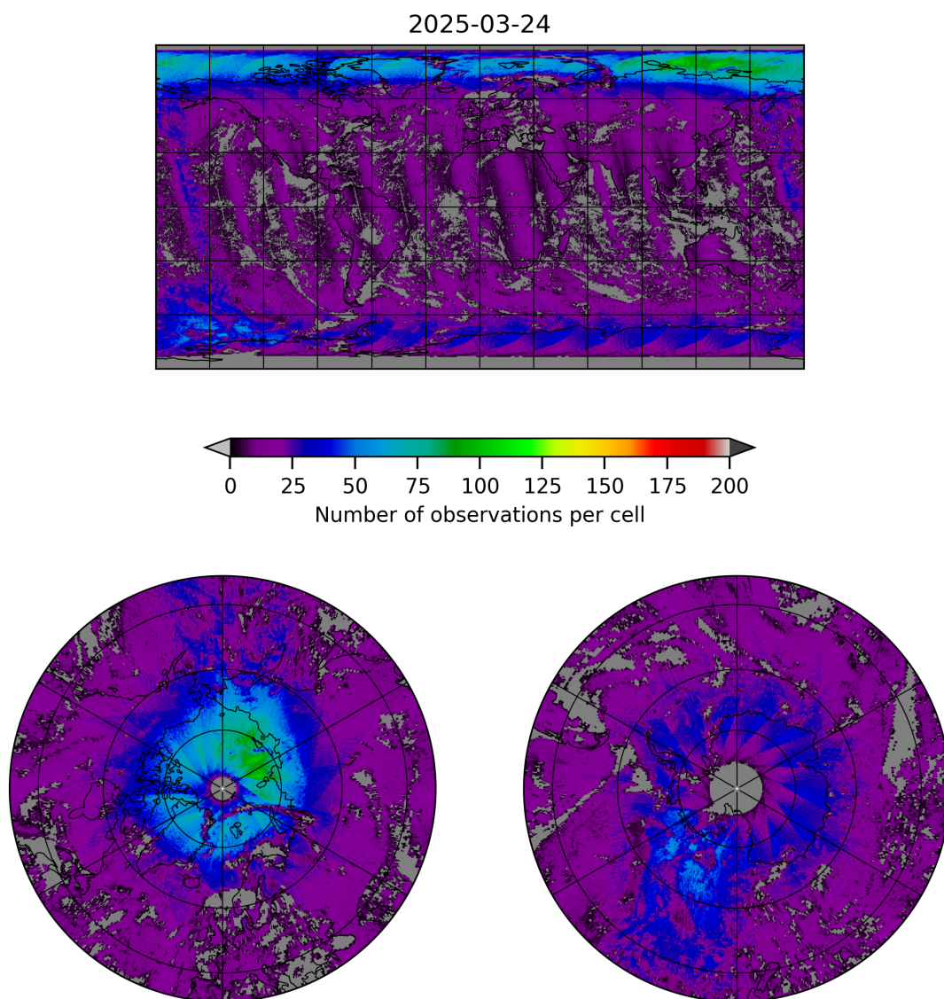
Figure 8: Map of the number of observations for 2025-03-23 to 2025-03-25
