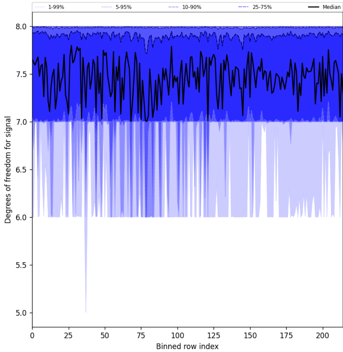
Figure 31: Along track statistics of “Degrees of freedom for signal” for 2025-03-23 to 2025-03-25
