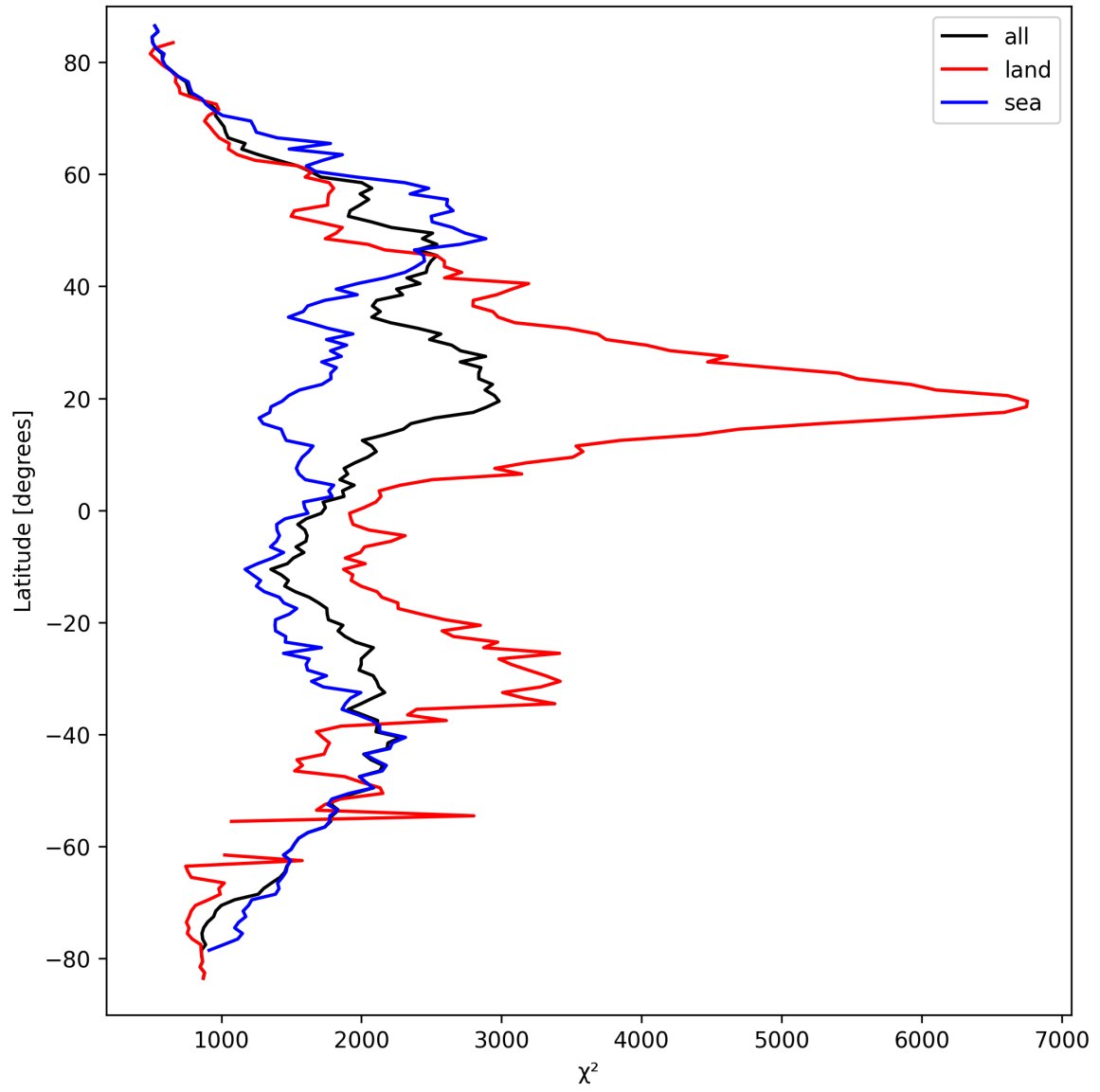
Figure 14: Zonal average of “ \chi^2 ” for 2025-03-23 to 2025-03-25.
