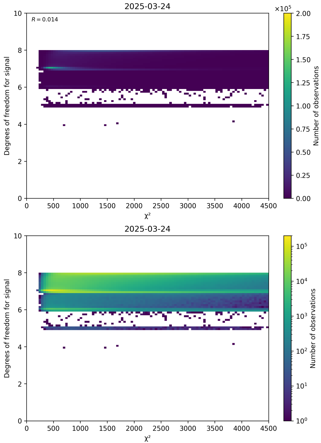
Figure 48: Scatter density plot of " \chi^2 " against "Degrees of freedom for signal" for 2025-03-23 to 2025-03-25.
