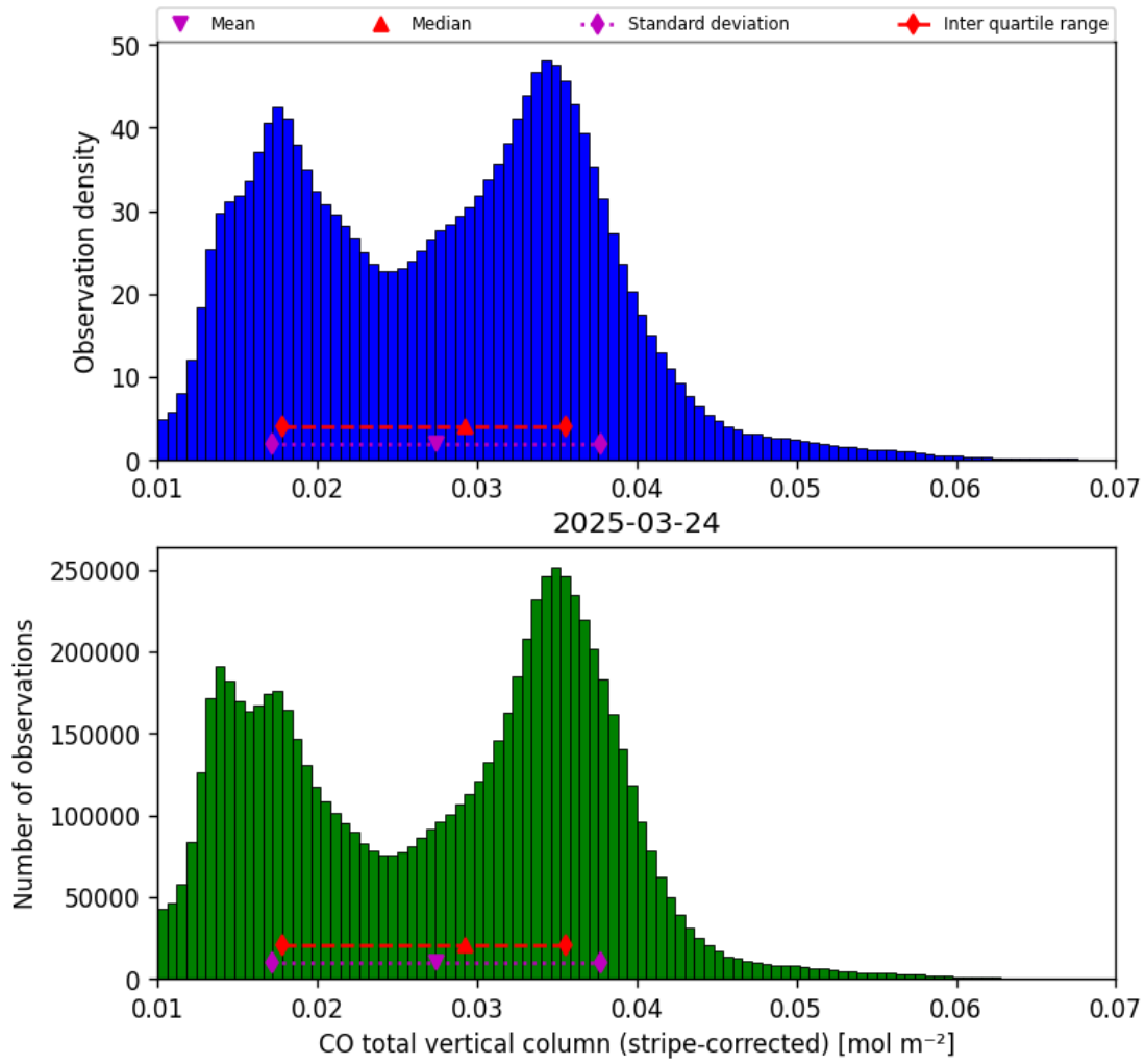
Figure 19: Histogram of “CO total vertical column (stripe-corrected)” for 2025-03-23 to 2025-03-25
