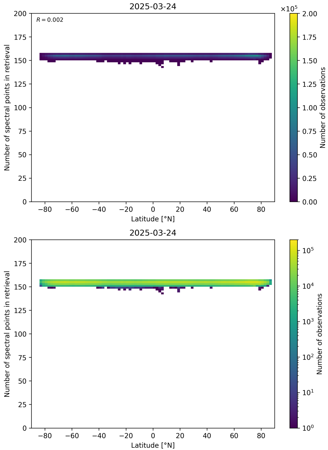
Figure 57: Scatter density plot of “Latitude” against “Number of spectral points in retrieval” for 2025-03-23 to 2025-03-25.
