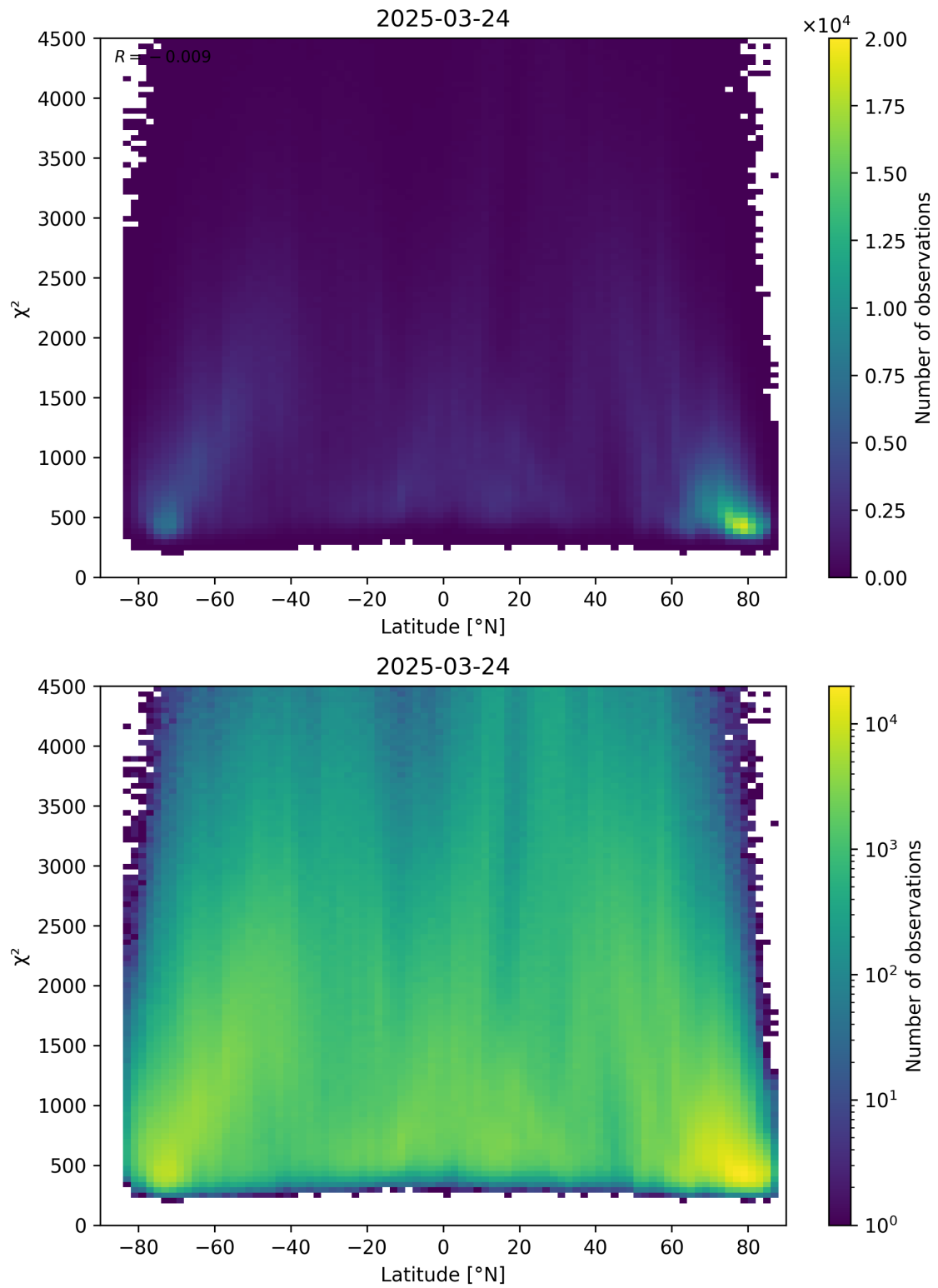
Figure 54: Scatter density plot of “Latitude” against “ \chi^2 ” for 2025-03-23 to 2025-03-25.
