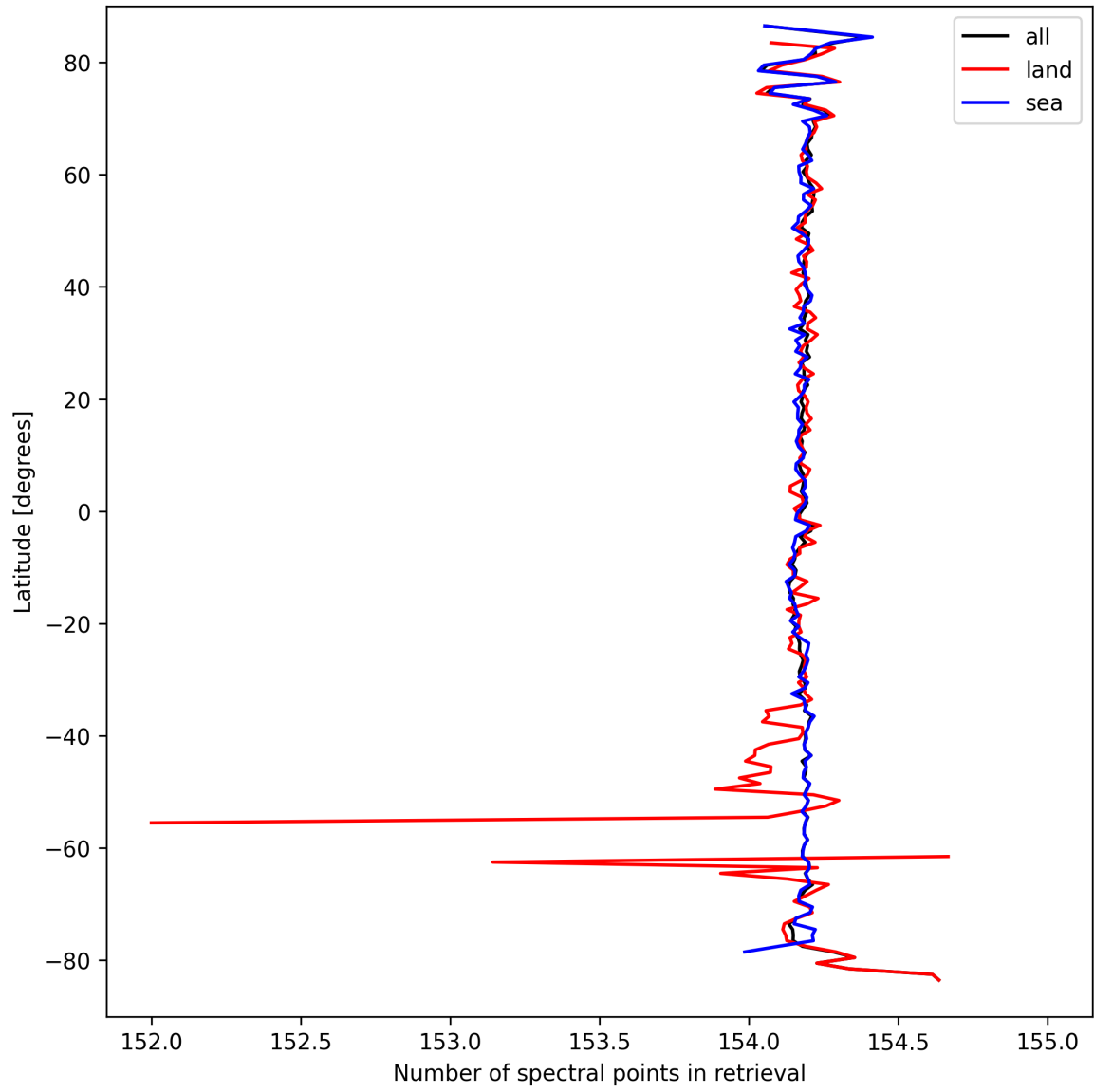
Figure 13: Zonal average of “Number of spectral points in retrieval” for 2025-03-23 to 2025-03-25.
