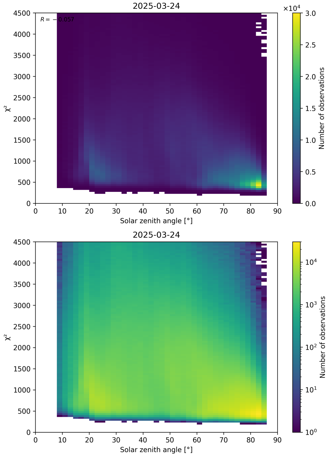
Figure 64: Scatter density plot of “Solar zenith angle” against “ \chi^2 ” for 2025-03-23 to 2025-03-25.
