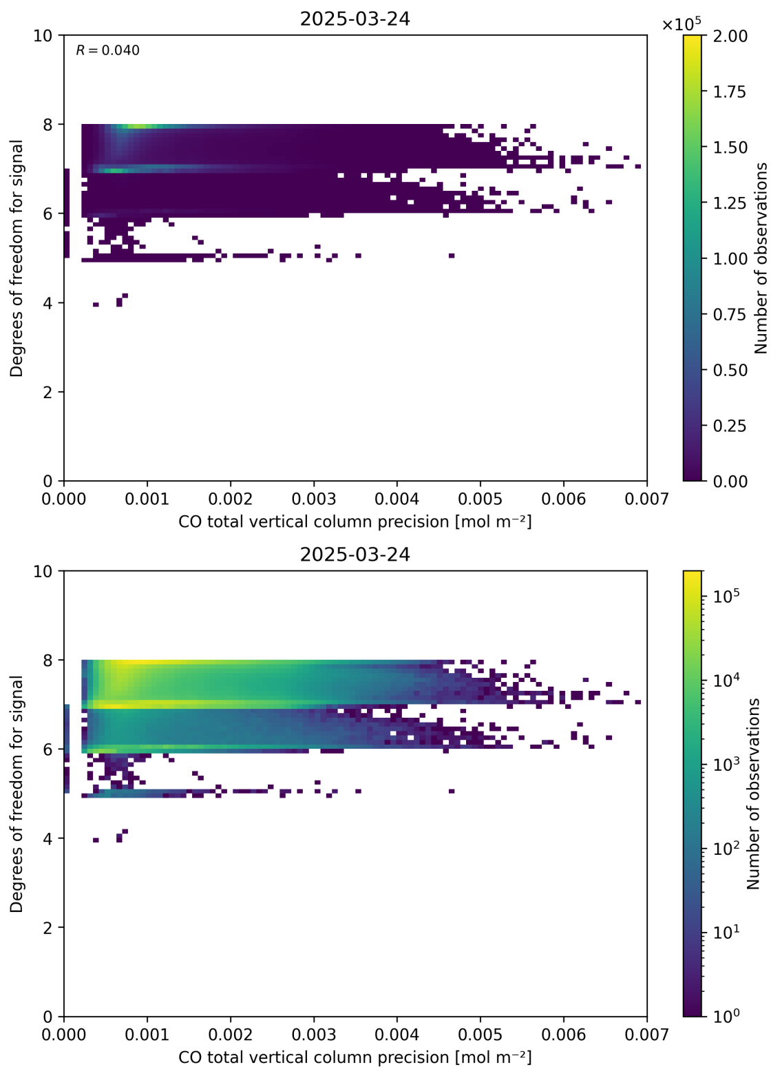
Figure 45: Scatter density plot of “CO total vertical column precision” against “Degrees of freedom for signal” for 2025-03-23 to 2025-03-25.
