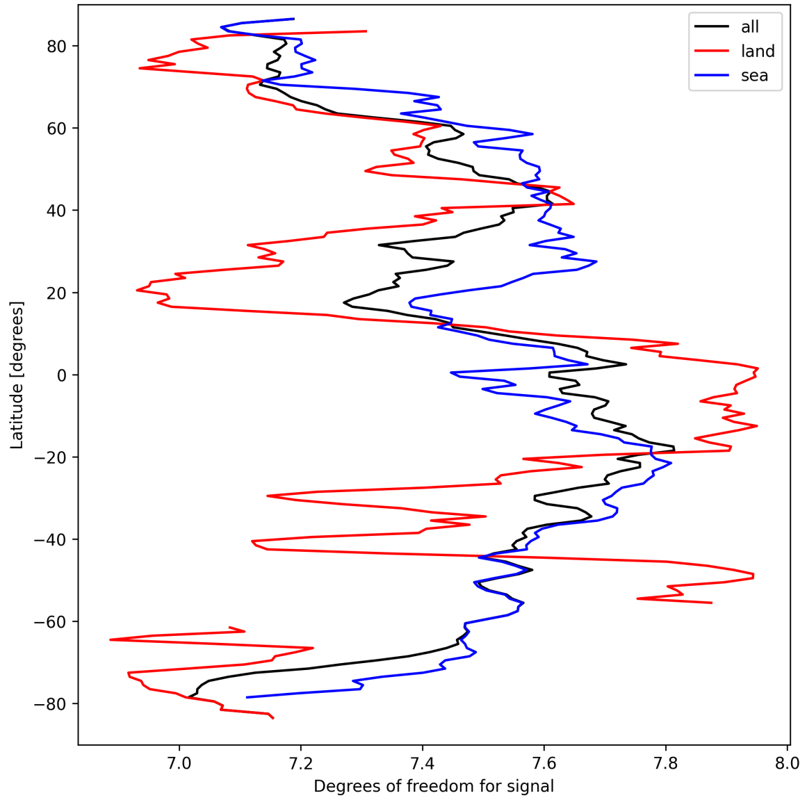
Figure 15: Zonal average of “Degrees of freedom for signal” for 2025-03-23 to 2025-03-25.
