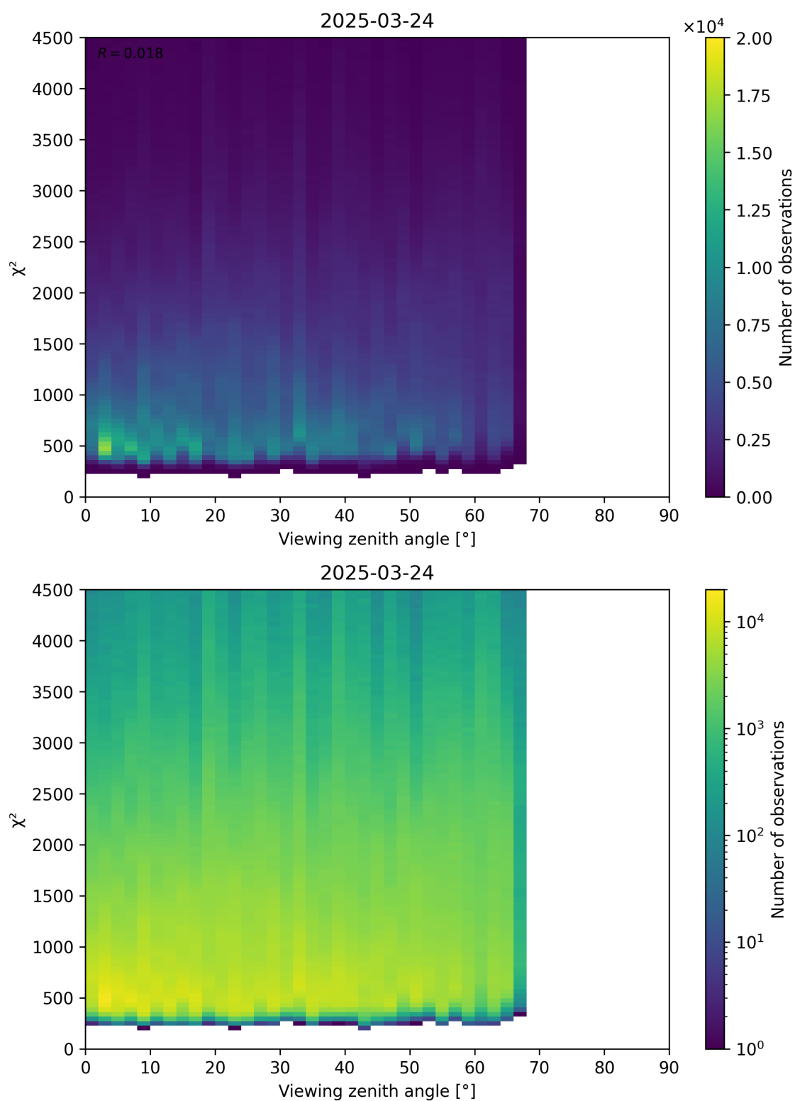
Figure 72: Scatter density plot of “Viewing zenith angle” against “ \chi^2 ” for 2025-03-23 to 2025-03-25.
