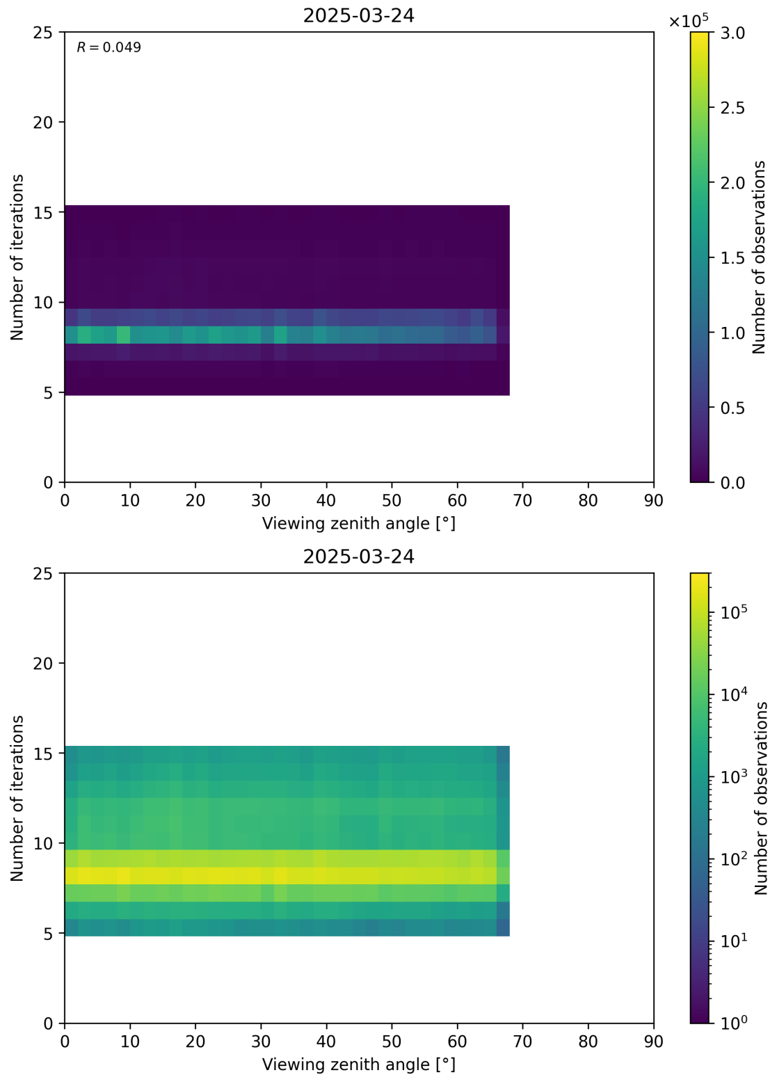
Figure 75: Scatter density plot of “Viewing zenith angle” against “Number of iterations” for 2025-03-23 to 2025-03-25.
