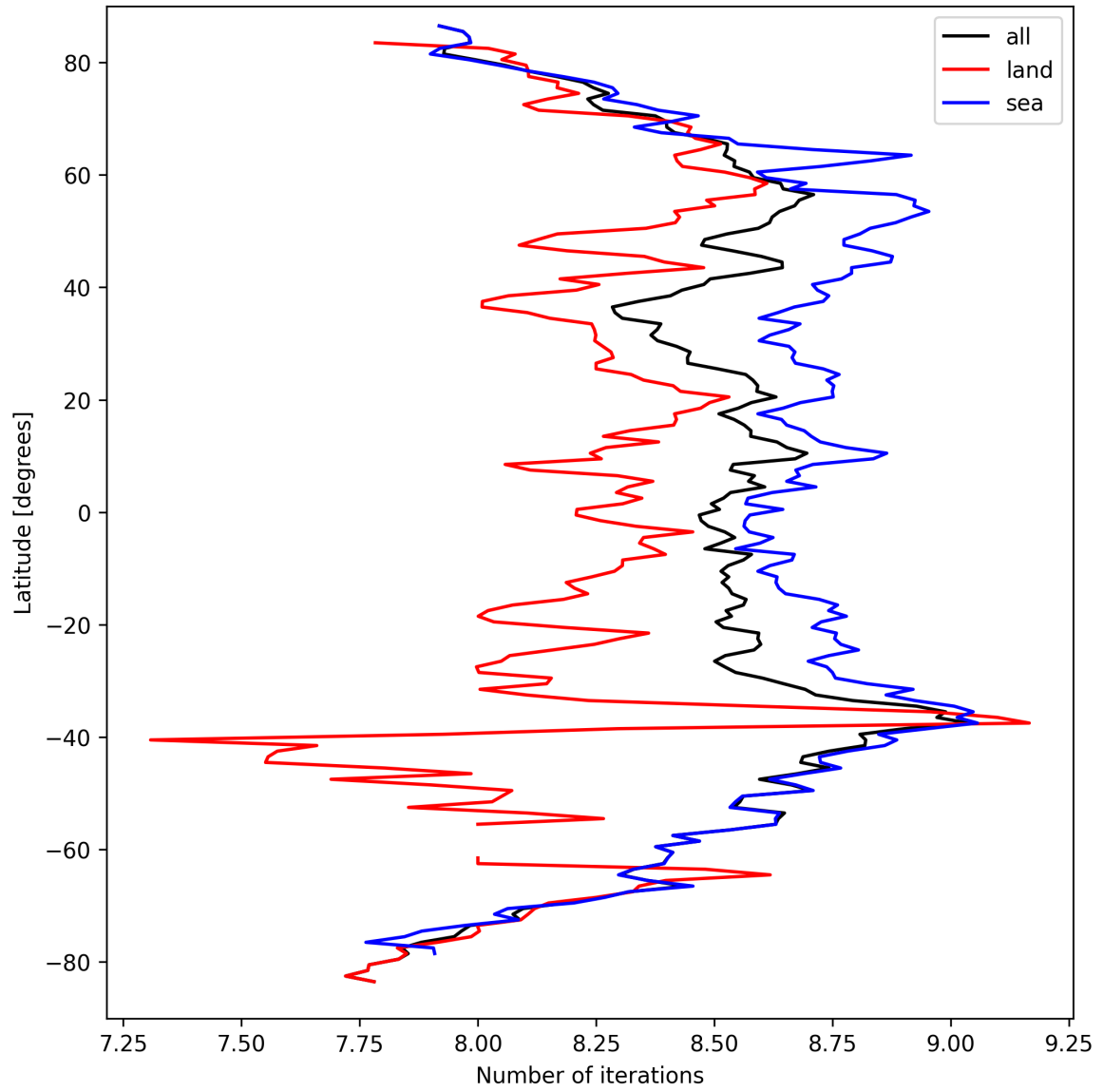
Figure 16: Zonal average of “Number of iterations” for 2025-03-23 to 2025-03-25.
