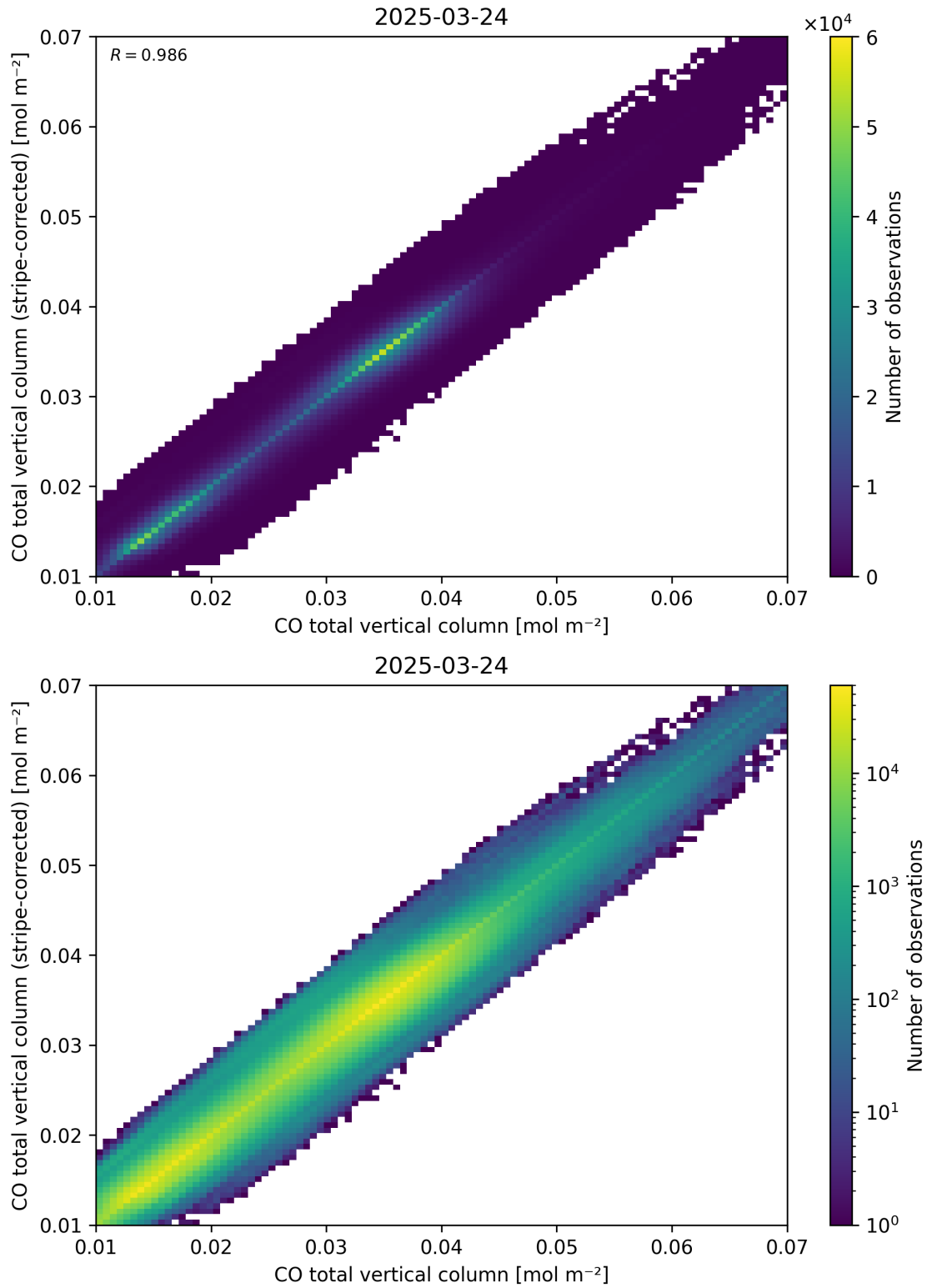
Figure 33: Scatter density plot of “CO total vertical column” against “CO total vertical column (stripe-corrected)” for 2025-03-23 to 2025-03-25.
