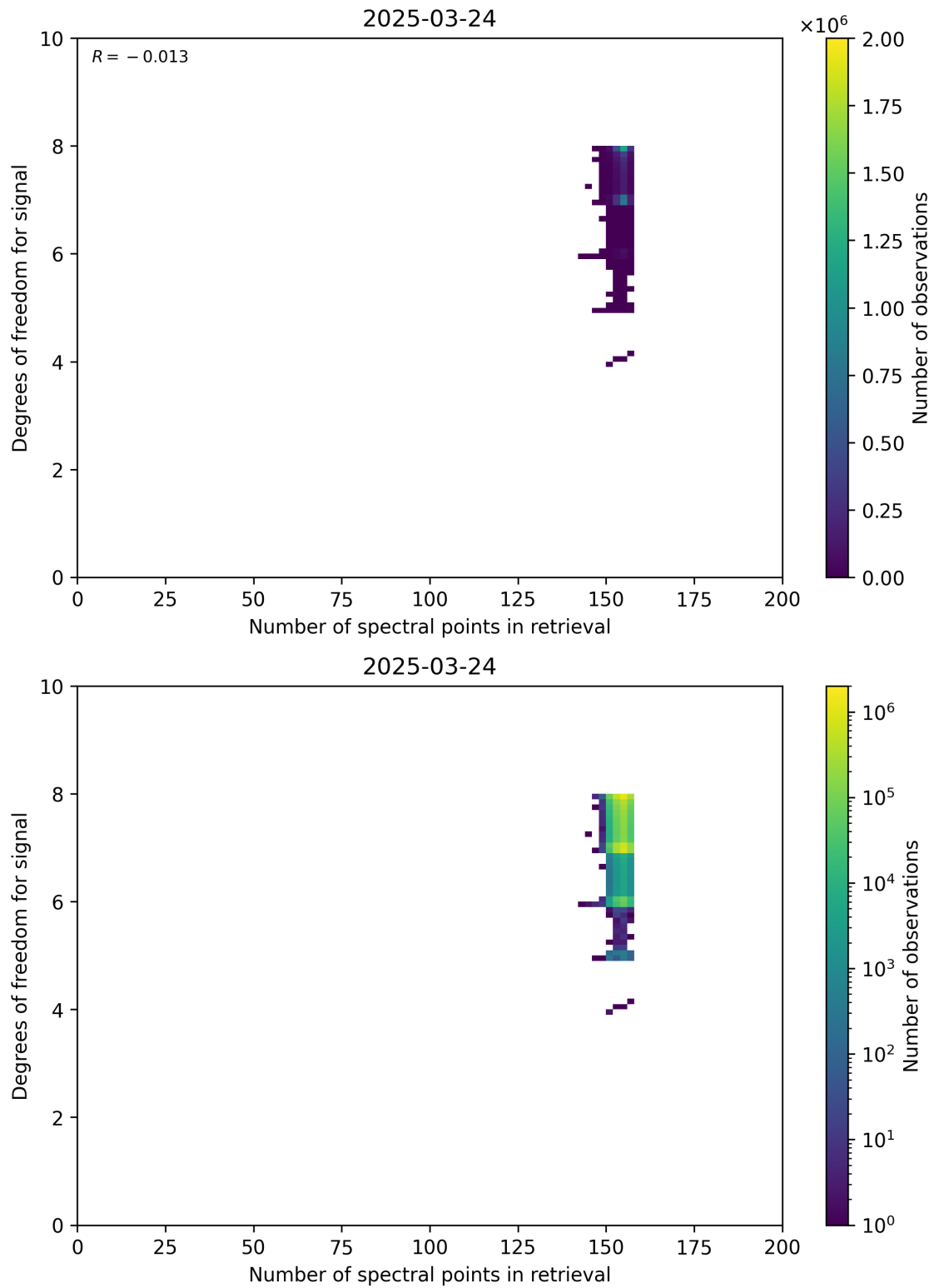
Figure 59: Scatter density plot of “Number of spectral points in retrieval” against “Degrees of freedom for signal” for 2025-03-23 to 2025-03-25.
