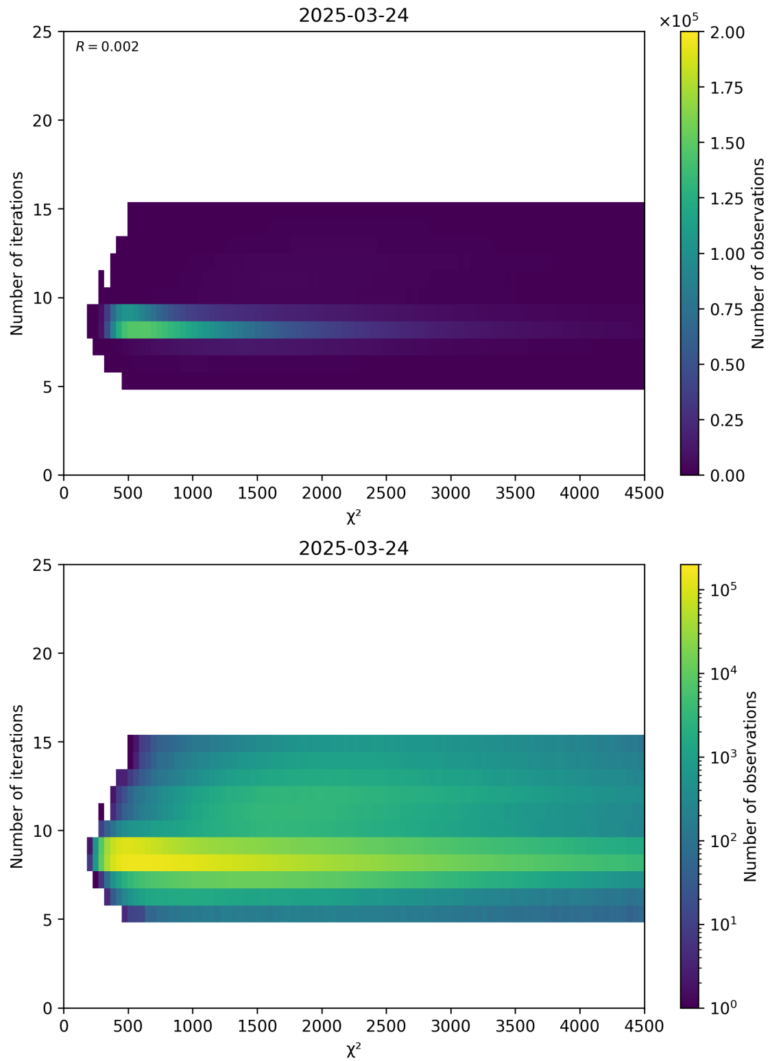
Figure 49: Scatter density plot of “ \chi^2 ” against “Number of iterations” for 2025-03-23 to 2025-03-25.
