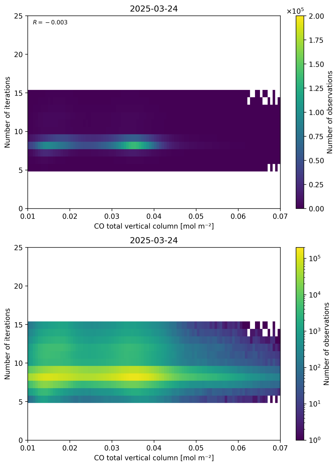
Figure 42: Scatter density plot of “CO total vertical column” against “Number of iterations” for 2025-03-23 to 2025-03-25.
