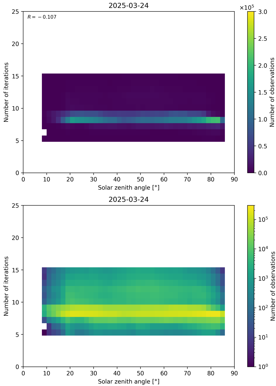
Figure 67: Scatter density plot of “Solar zenith angle” against “Number of iterations” for 2025-03-23 to 2025-03-25.
