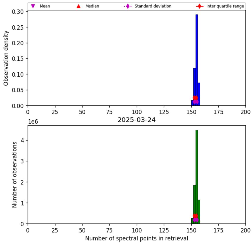
Figure 21: Histogram of “Number of spectral points in retrieval” for 2025-03-23 to 2025-03-25
