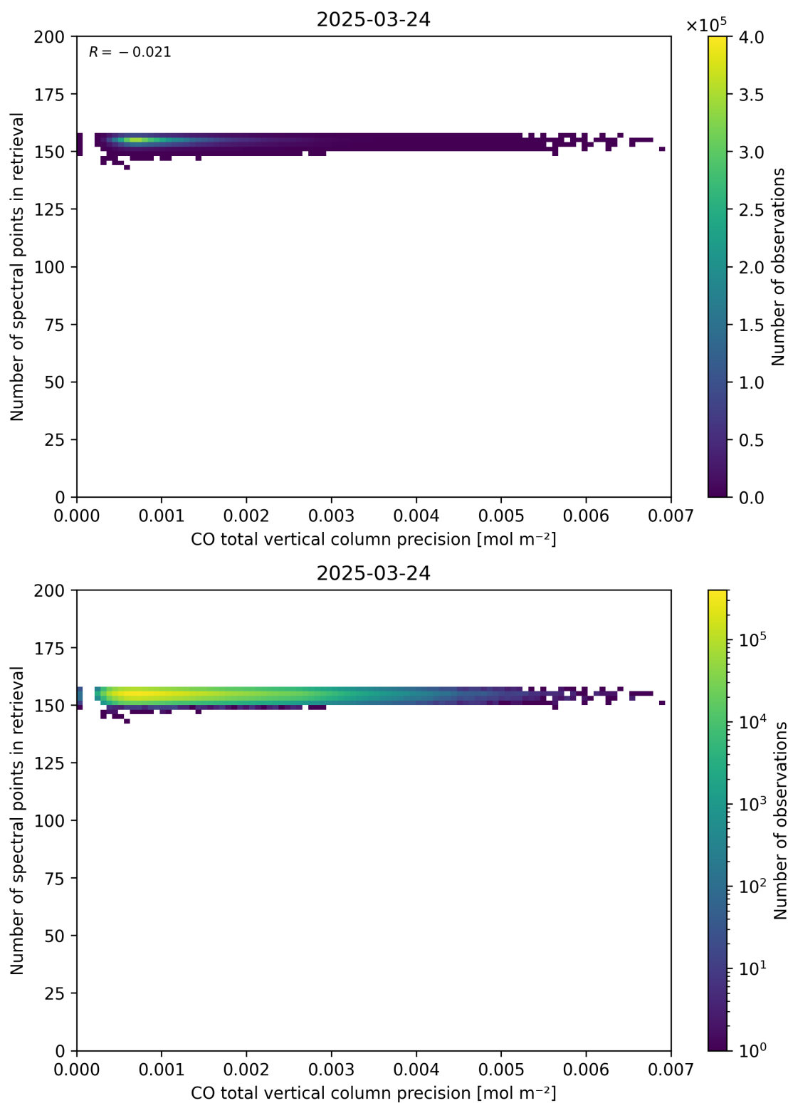
Figure 47: Scatter density plot of “CO total vertical column precision” against “Number of spectral points in retrieval” for 2025-03-23 to 2025-03-25.
