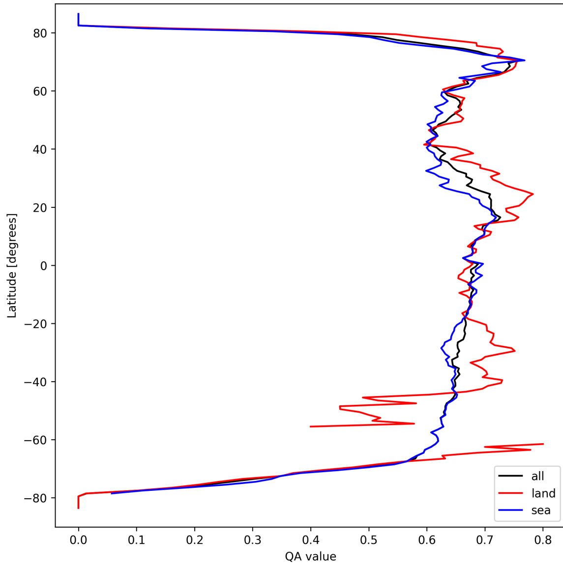
Figure 9: Zonal average of “QA value” for 2025-03-23 to 2025-03-25.
