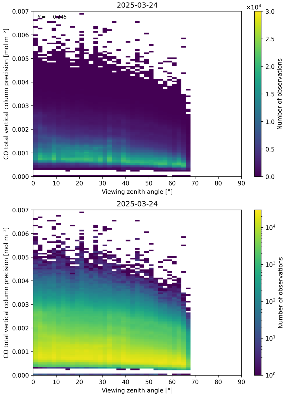
Figure 71: Scatter density plot of “Viewing zenith angle” against “CO total vertical column precision” for 2025-03-23 to 2025-03-25.
