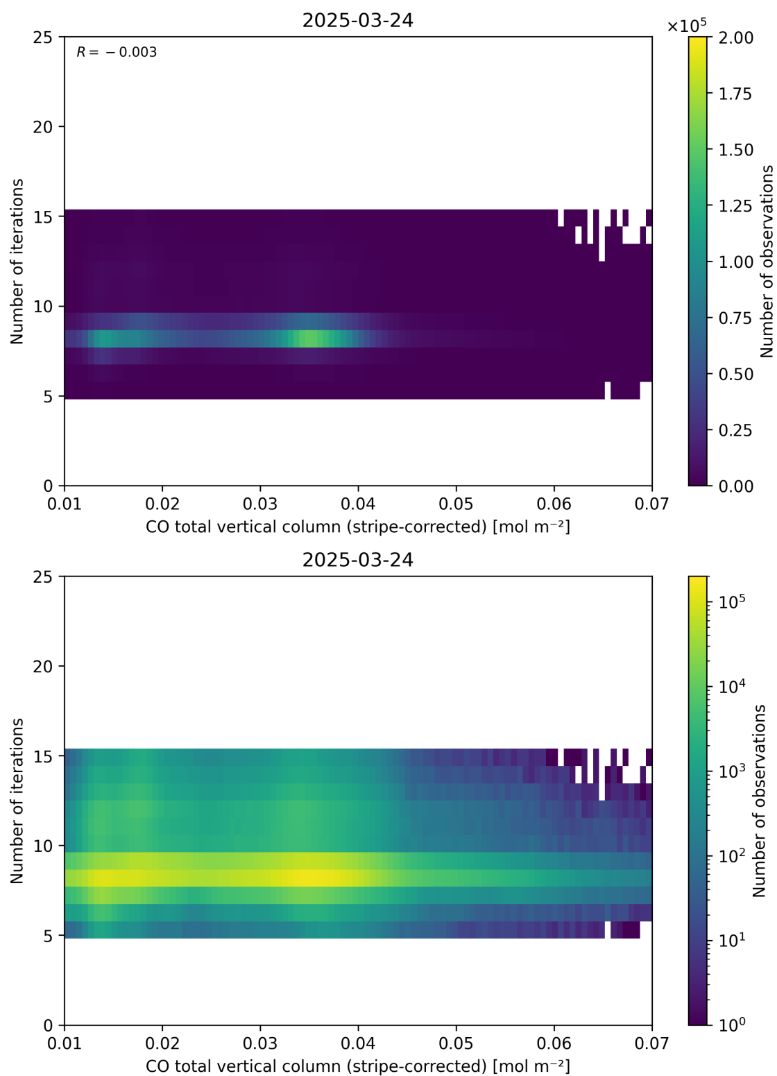
Figure 39: Scatter density plot of “CO total vertical column (stripe-corrected)” against “Number of iterations” for 2025-03-23 to 2025-03-25.
