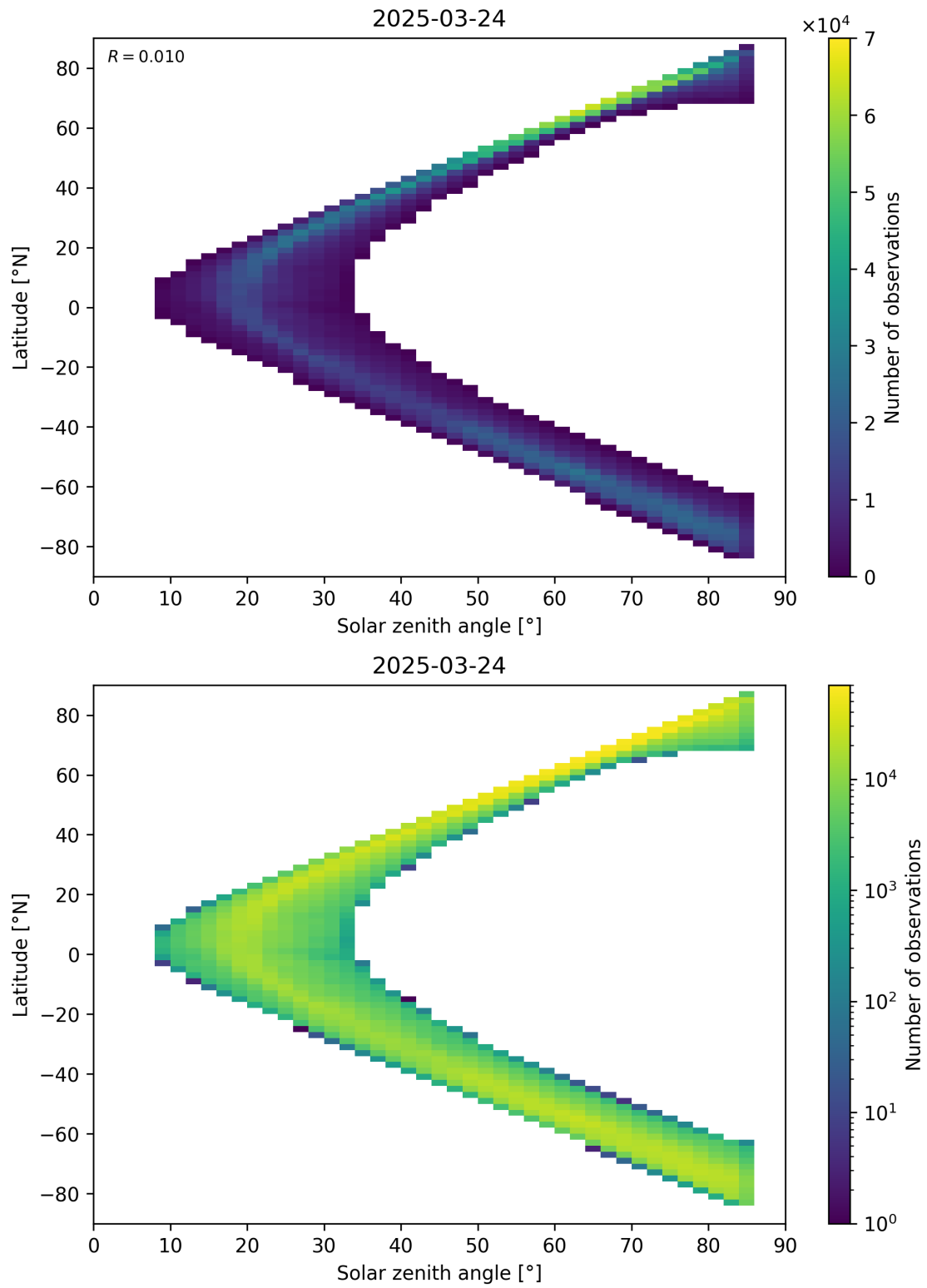
Figure 66: Scatter density plot of “Solar zenith angle” against “Latitude” for 2025-03-23 to 2025-03-25.
