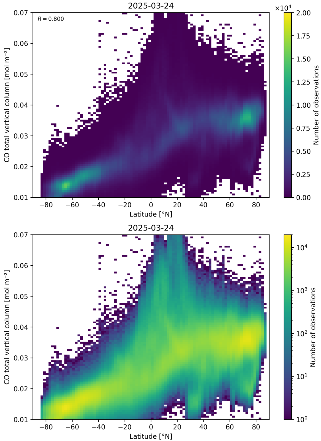
Figure 51: Scatter density plot of “Latitude” against “CO total vertical column” for 2025-03-23 to 2025-03-25.
