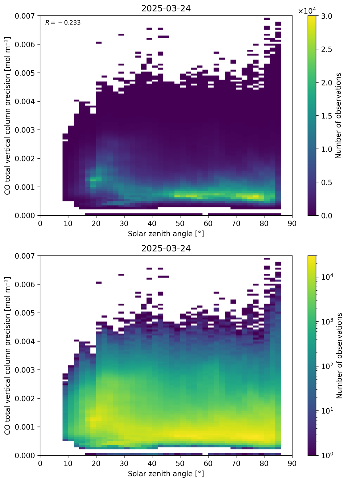
Figure 63: Scatter density plot of “Solar zenith angle” against “CO total vertical column precision” for 2025-03-23 to 2025-03-25.
