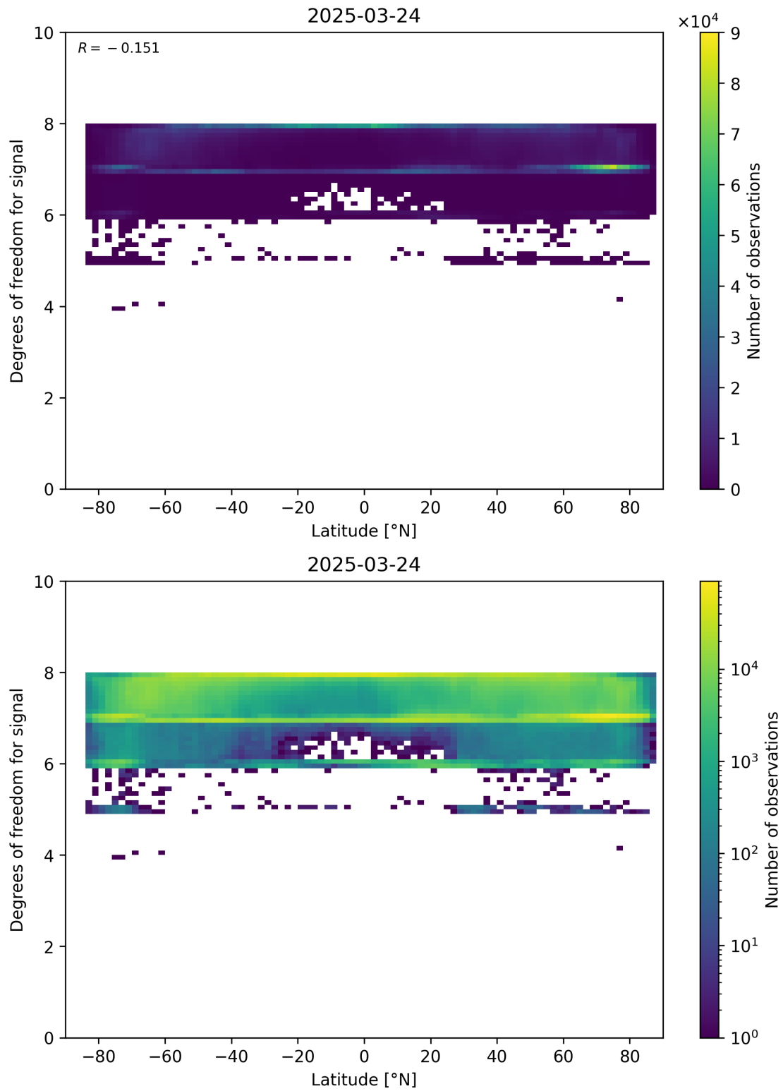
Figure 55: Scatter density plot of “Latitude” against “Degrees of freedom for signal” for 2025-03-23 to 2025-03-25.
