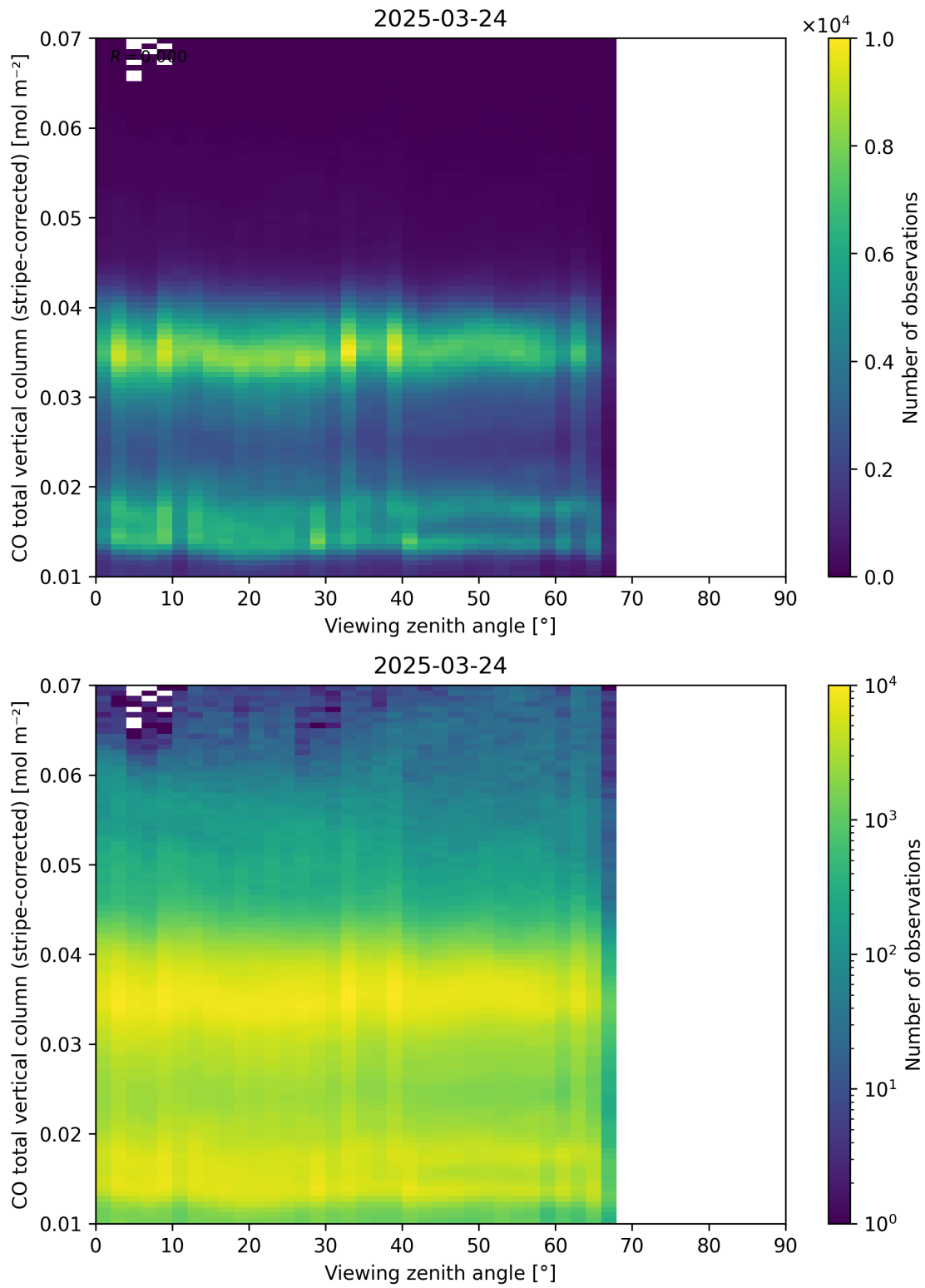
Figure 70: Scatter density plot of “Viewing zenith angle” against “CO total vertical column (stripe-corrected)” for 2025-03-23 to 2025-03-25.
