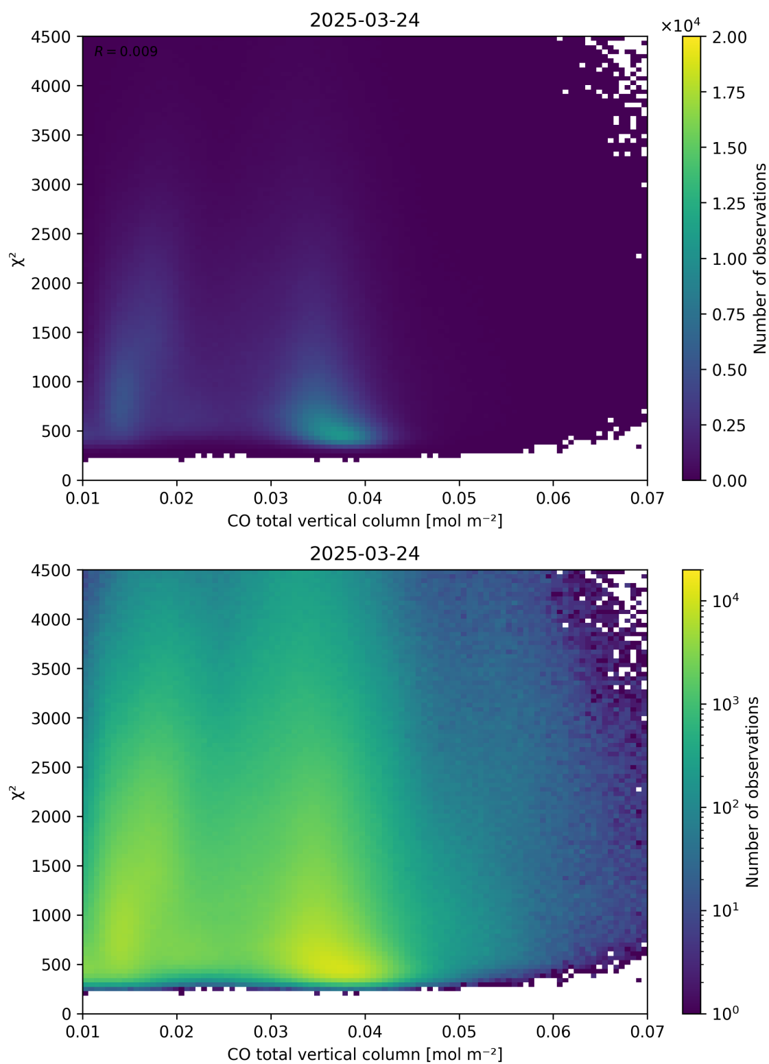
Figure 35: Scatter density plot of “CO total vertical column” against “ \chi^2 ” for 2025-03-23 to 2025-03-25.
