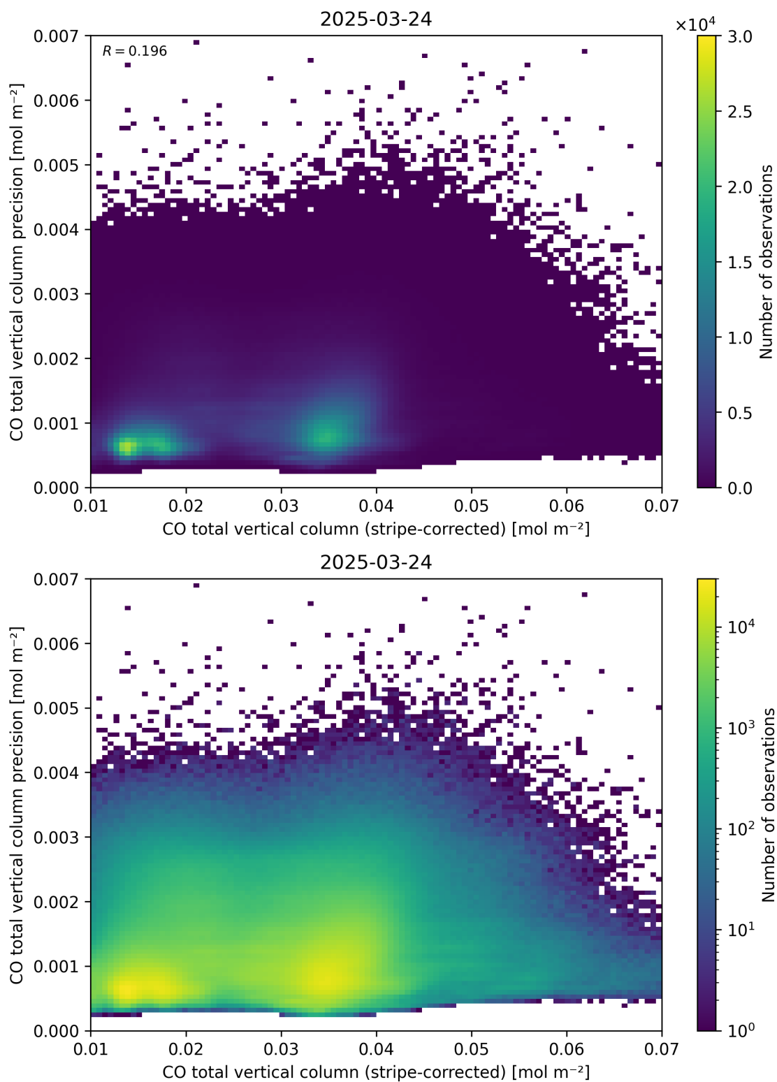
Figure 36: Scatter density plot of “CO total vertical column (stripe-corrected)” against “CO total vertical column precision” for 2025-03-23 to 2025-03-25.
