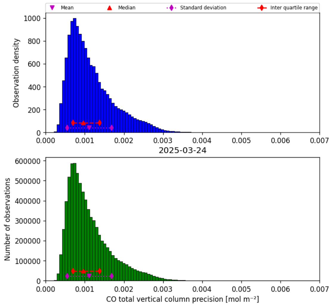
Figure 20: Histogram of “CO total vertical column precision” for 2025-03-23 to 2025-03-25
