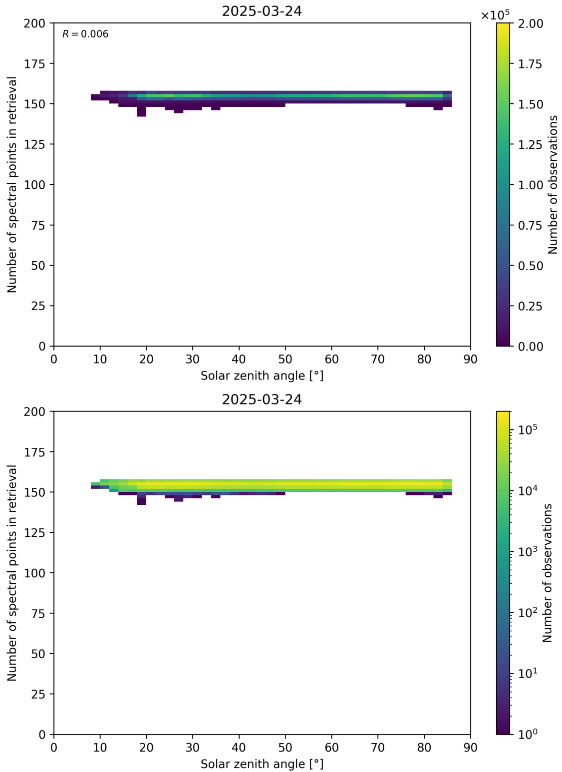
Figure 68: Scatter density plot of “Solar zenith angle” against “Number of spectral points in retrieval” for 2025-03-23 to 2025-03-25.
