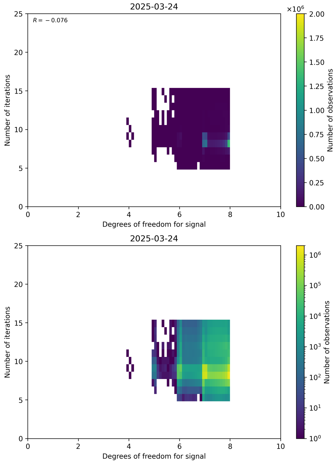
Figure 50: Scatter density plot of “Degrees of freedom for signal” against “Number of iterations” for 2025-03-23 to 2025-03-25.
