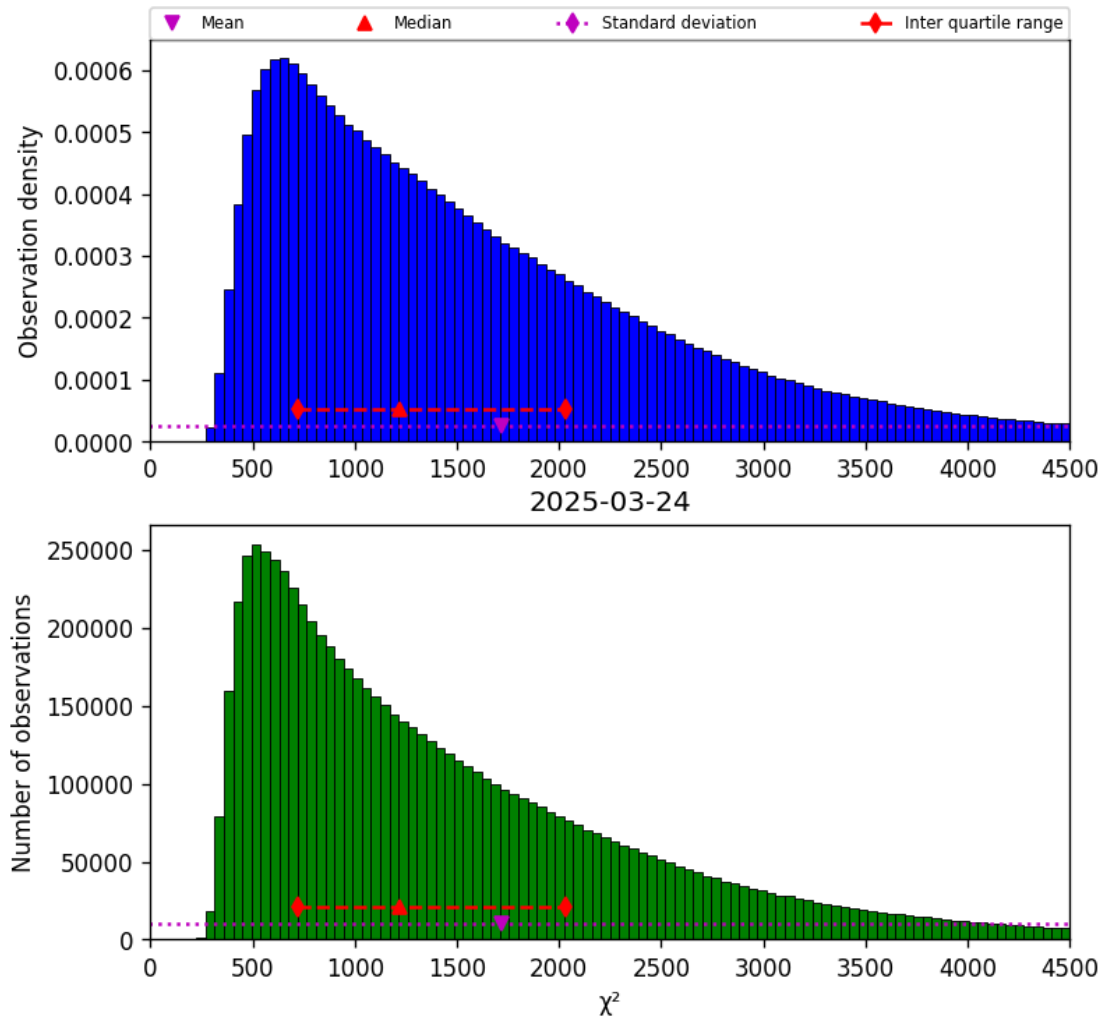
Figure 22: Histogram of “ \chi^2 ” for 2025-03-23 to 2025-03-25
