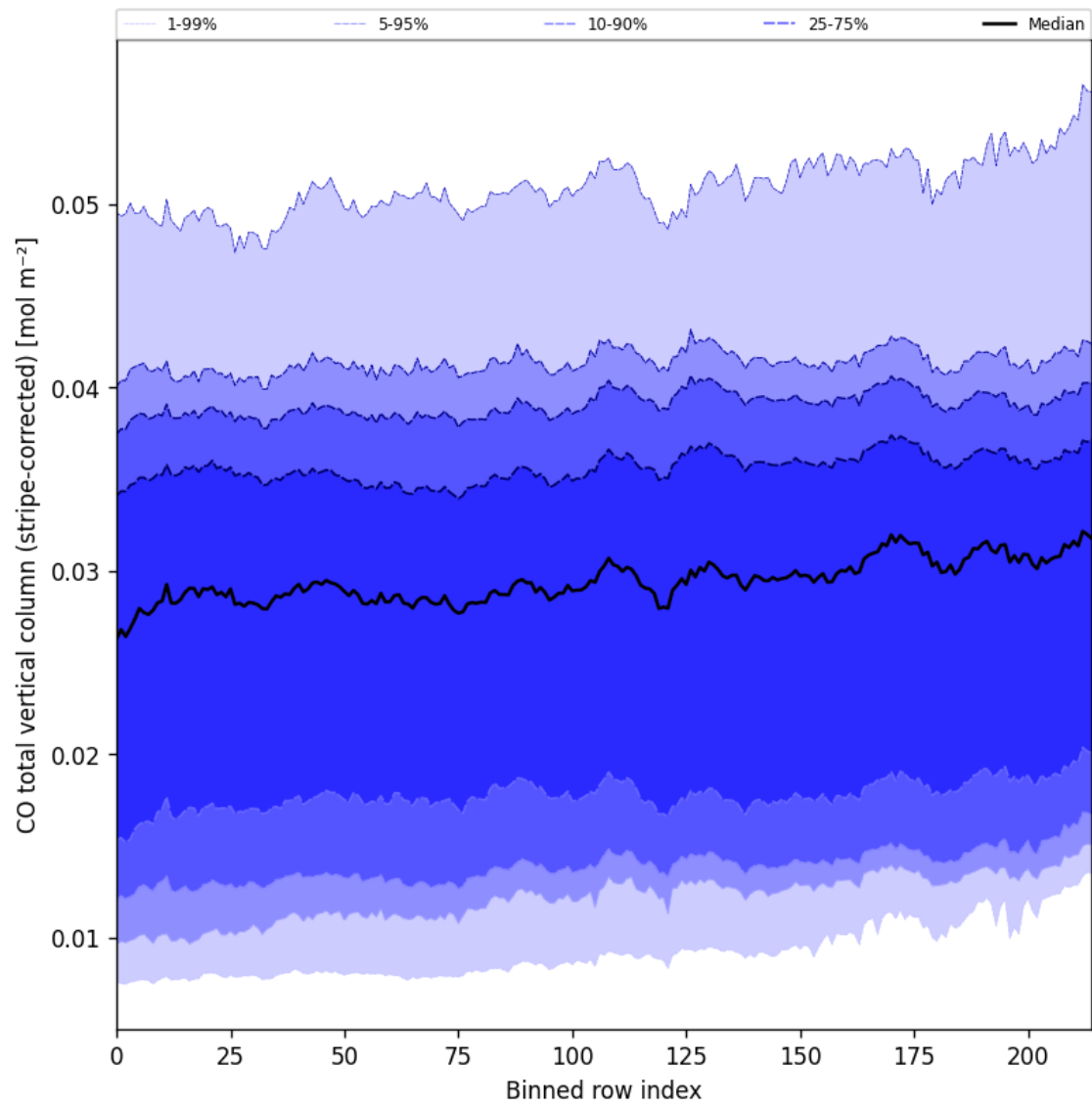
Figure 27: Along track statistics of “CO total vertical column (stripe-corrected)” for 2025-03-23 to 2025-03-25
