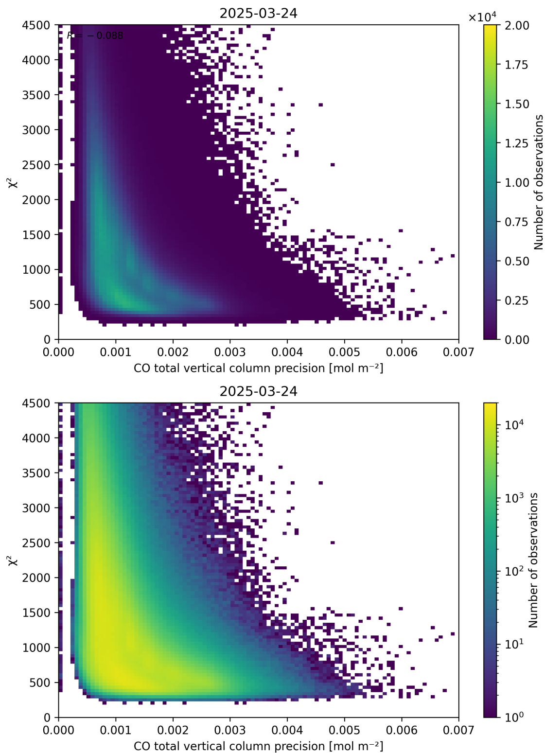
Figure 44: Scatter density plot of “CO total vertical column precision” against “ \chi^2 ” for 2025-03-23 to 2025-03-25.
