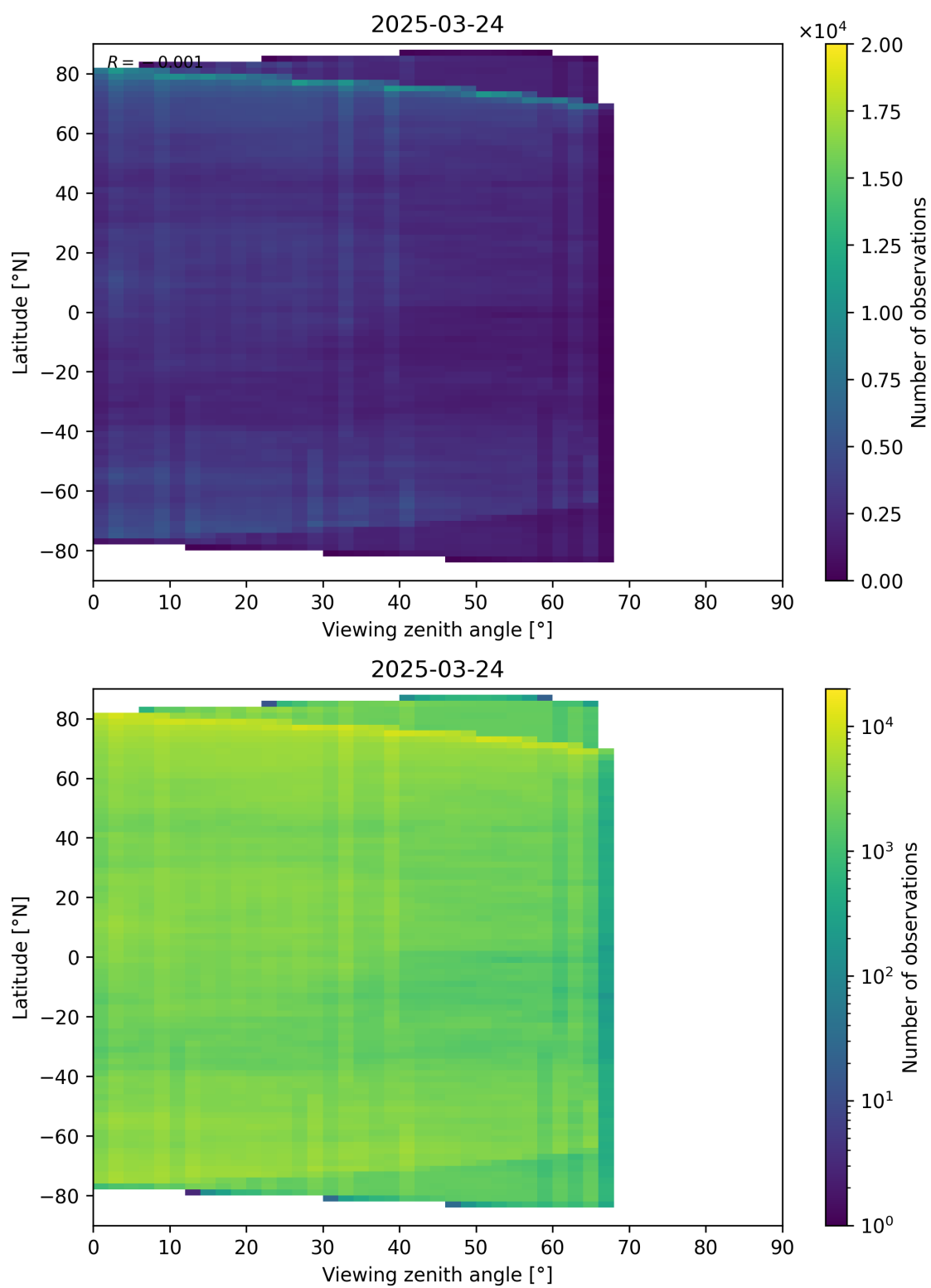
Figure 74: Scatter density plot of “Viewing zenith angle” against “Latitude” for 2025-03-23 to 2025-03-25.
