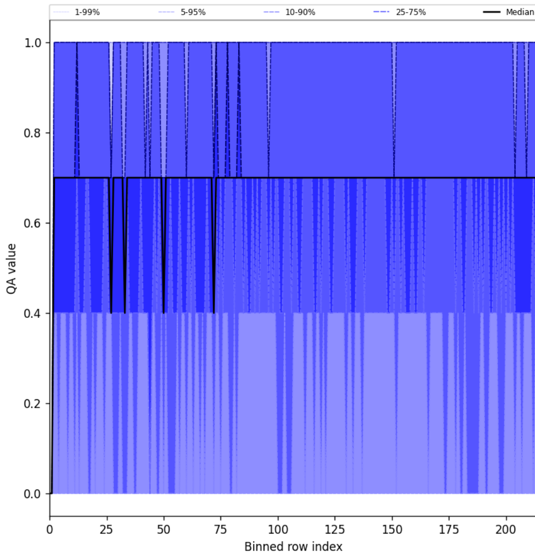
Figure 25: Along track statistics of “QA value” for 2025-03-23 to 2025-03-25
