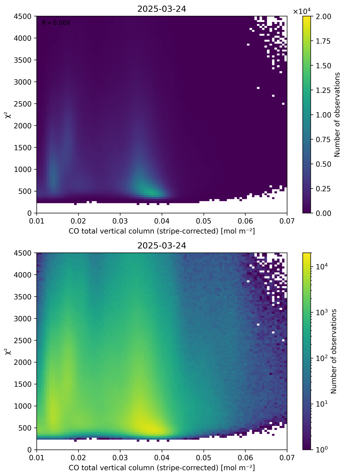
Figure 37: Scatter density plot of “CO total vertical column (stripe-corrected)” against “ \chi^2 ” for 2025-03-23 to 2025-03-25.
