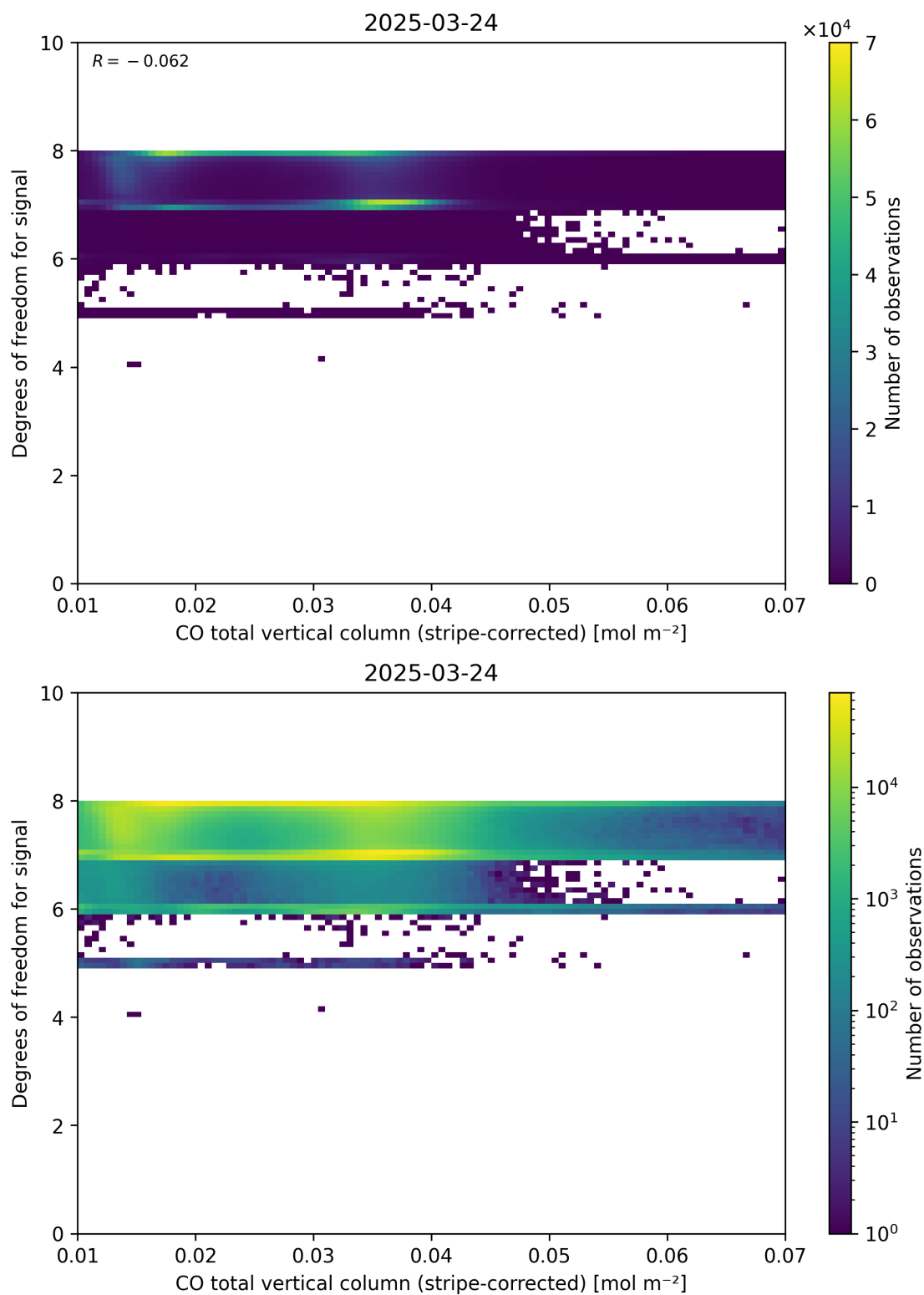
Figure 38: Scatter density plot of “CO total vertical column (stripe-corrected)” against “Degrees of freedom for signal” for 2025-03-23 to 2025-03-25.
