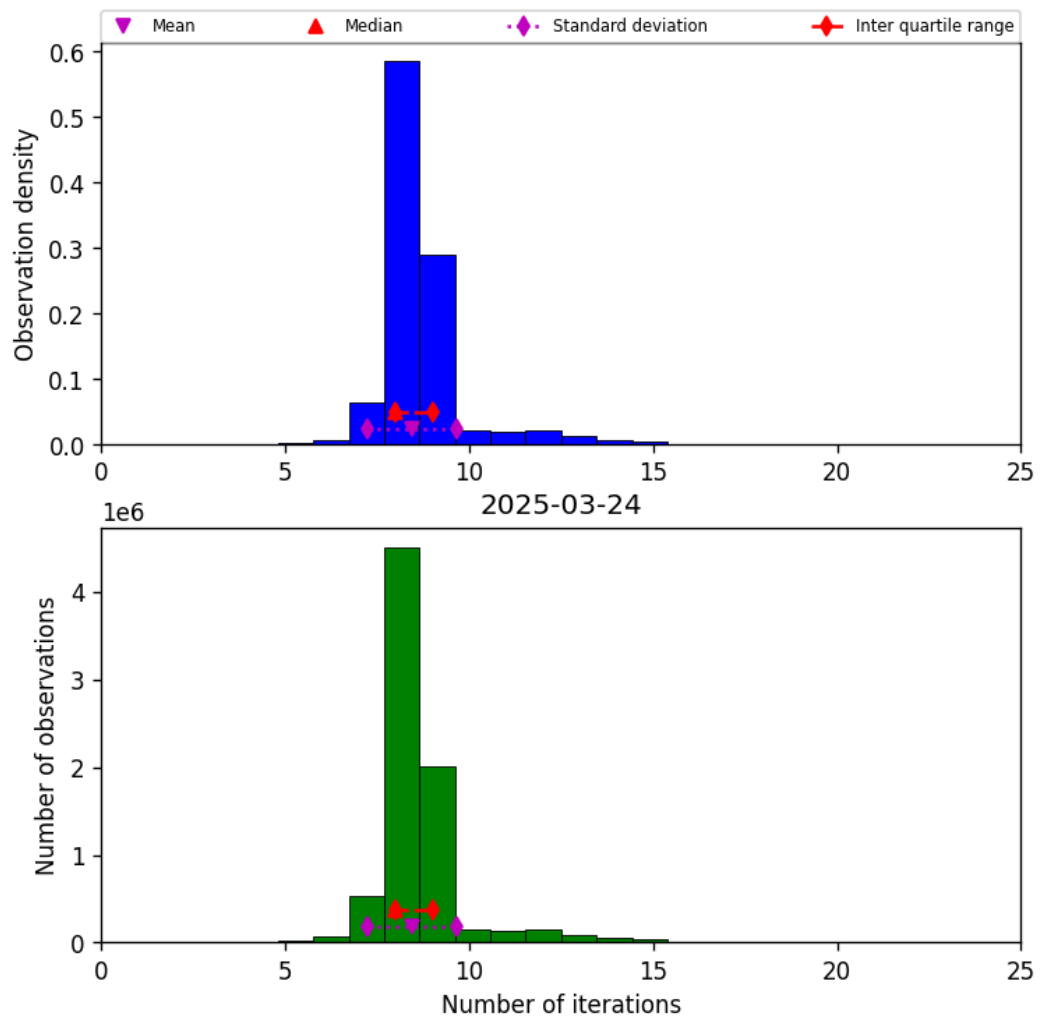
Figure 24: Histogram of “Number of iterations” for 2025-03-23 to 2025-03-25
