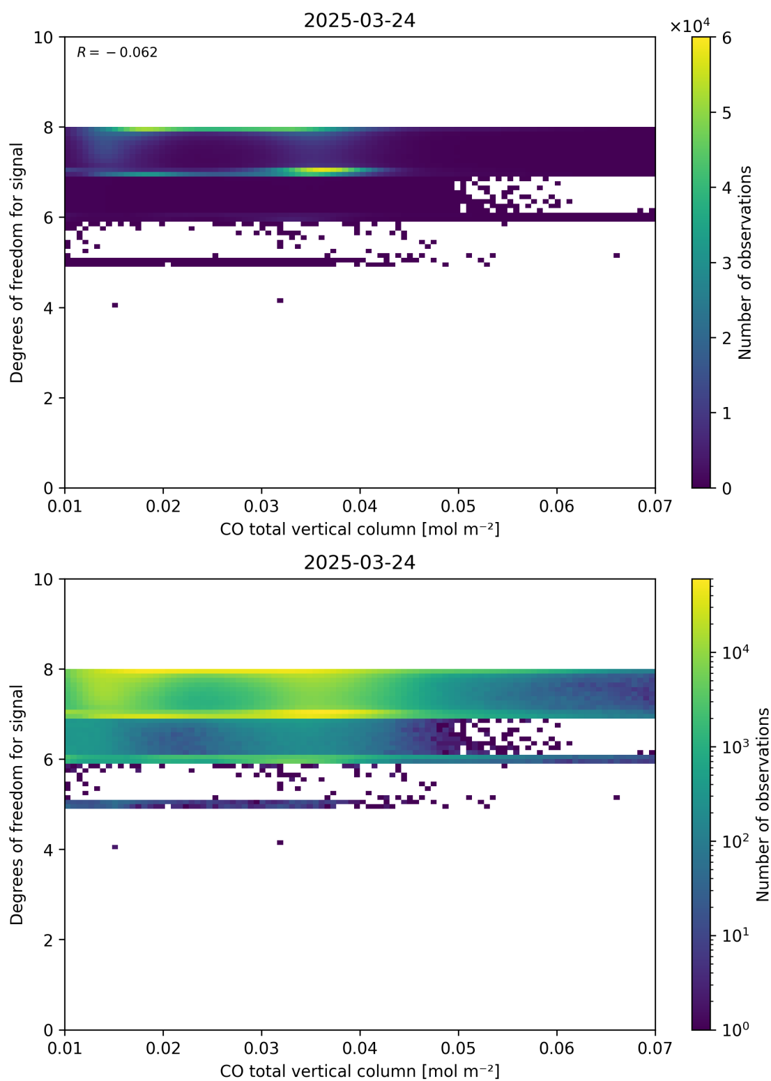
Figure 41: Scatter density plot of “CO total vertical column” against “Degrees of freedom for signal” for 2025-03-23 to 2025-03-25.
