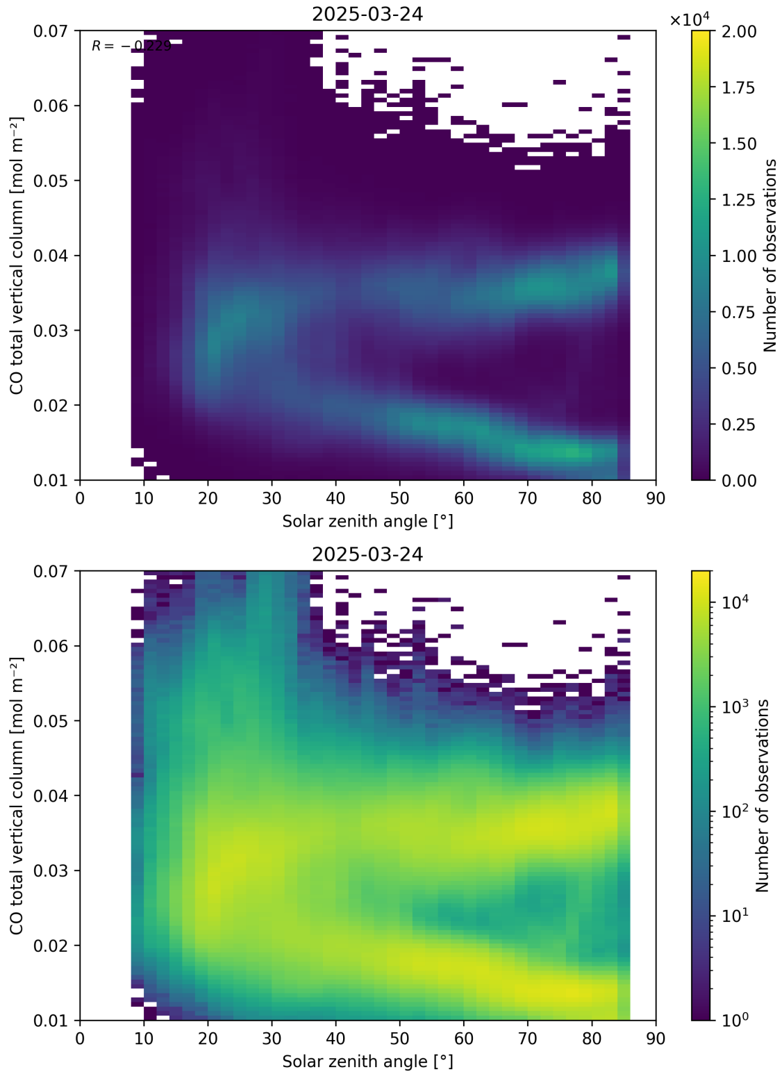
Figure 61: Scatter density plot of “Solar zenith angle” against “CO total vertical column” for 2025-03-23 to 2025-03-25.
