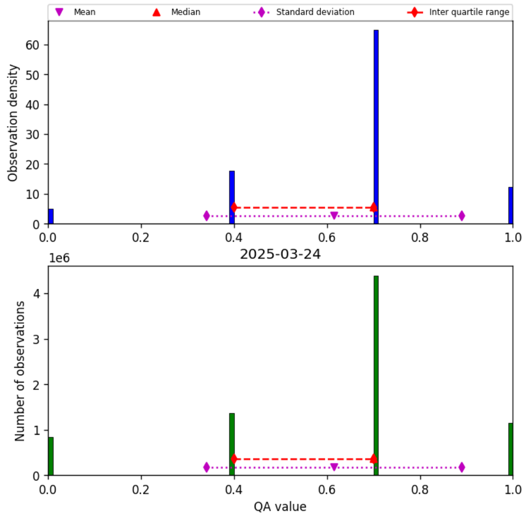
Figure 17: Histogram of “QA value” for 2025-03-23 to 2025-03-25
