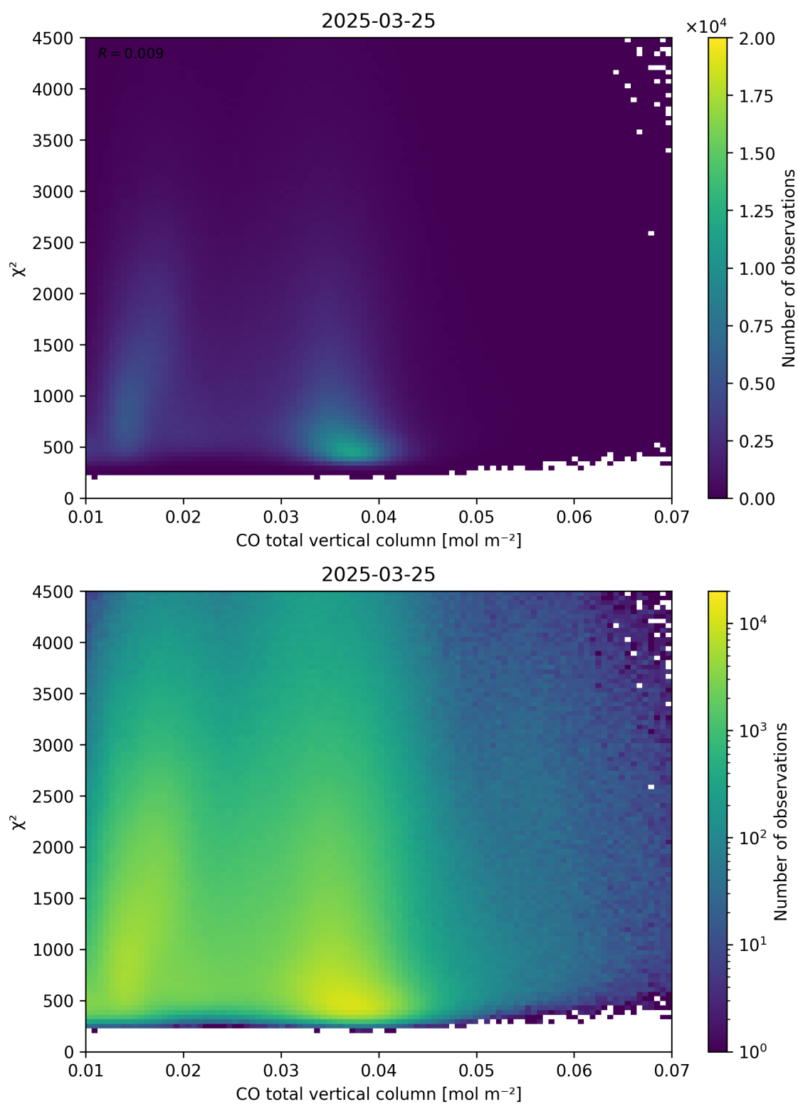
Figure 35: Scatter density plot of “CO total vertical column” against “ \chi^2 ” for 2025-03-24 to 2025-03-26.
