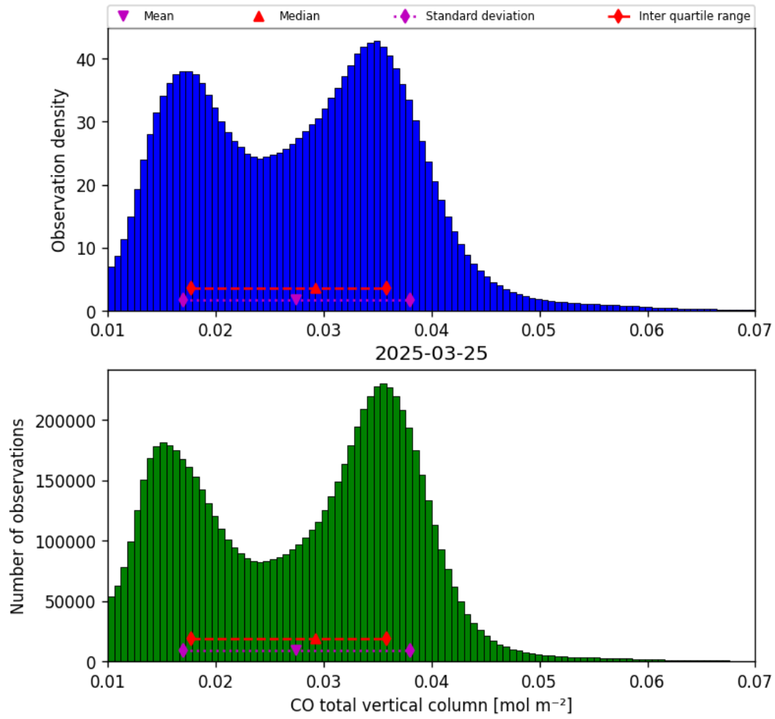
Figure 18: Histogram of “CO total vertical column” for 2025-03-24 to 2025-03-26
