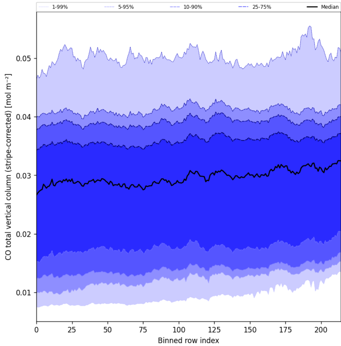
Figure 27: Along track statistics of “CO total vertical column (stripe-corrected)” for 2025-03-24 to 2025-03-26
