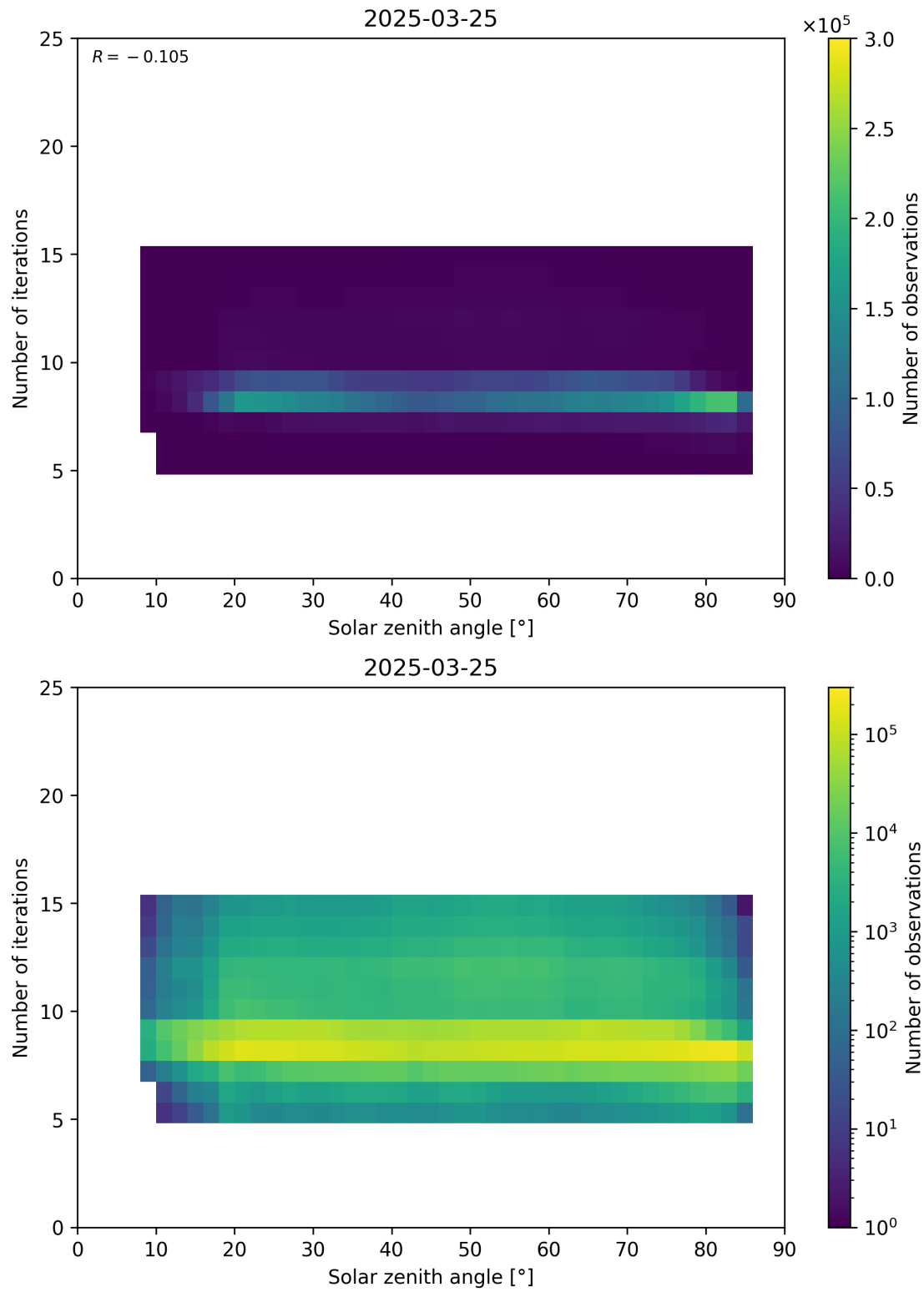
Figure 67: Scatter density plot of “Solar zenith angle” against “Number of iterations” for 2025-03-24 to 2025-03-26.
