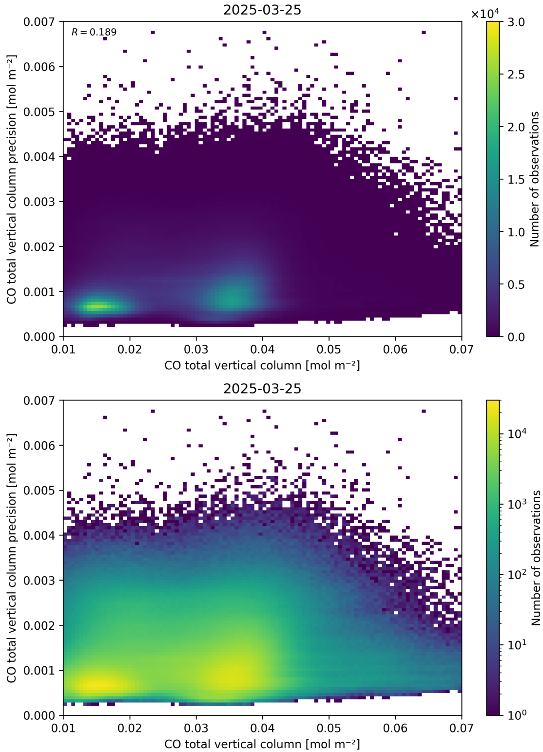
Figure 34: Scatter density plot of “CO total vertical column” against “CO total vertical column precision” for 2025-03-24 to 2025-03-26.
