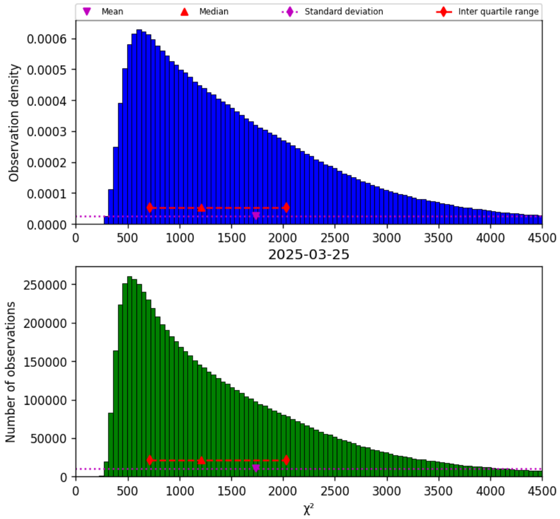
Figure 22: Histogram of “ \chi^2 ” for 2025-03-24 to 2025-03-26
