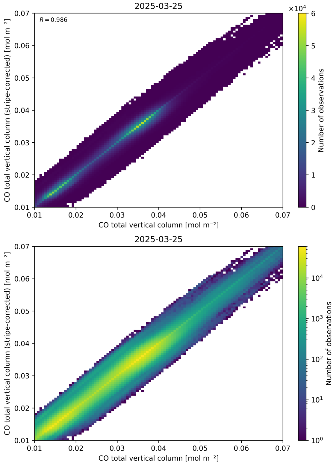
Figure 33: Scatter density plot of “CO total vertical column” against “CO total vertical column (stripe-corrected)” for 2025-03-24 to 2025-03-26.
