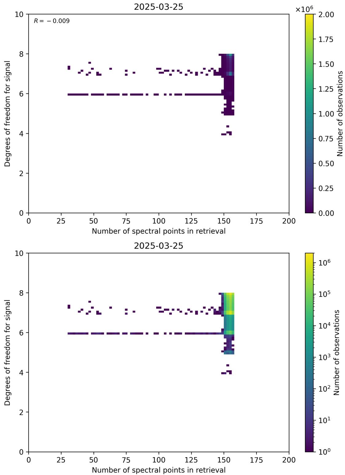
Figure 59: Scatter density plot of “Number of spectral points in retrieval” against “Degrees of freedom for signal” for 2025-03-24 to 2025-03-26.
