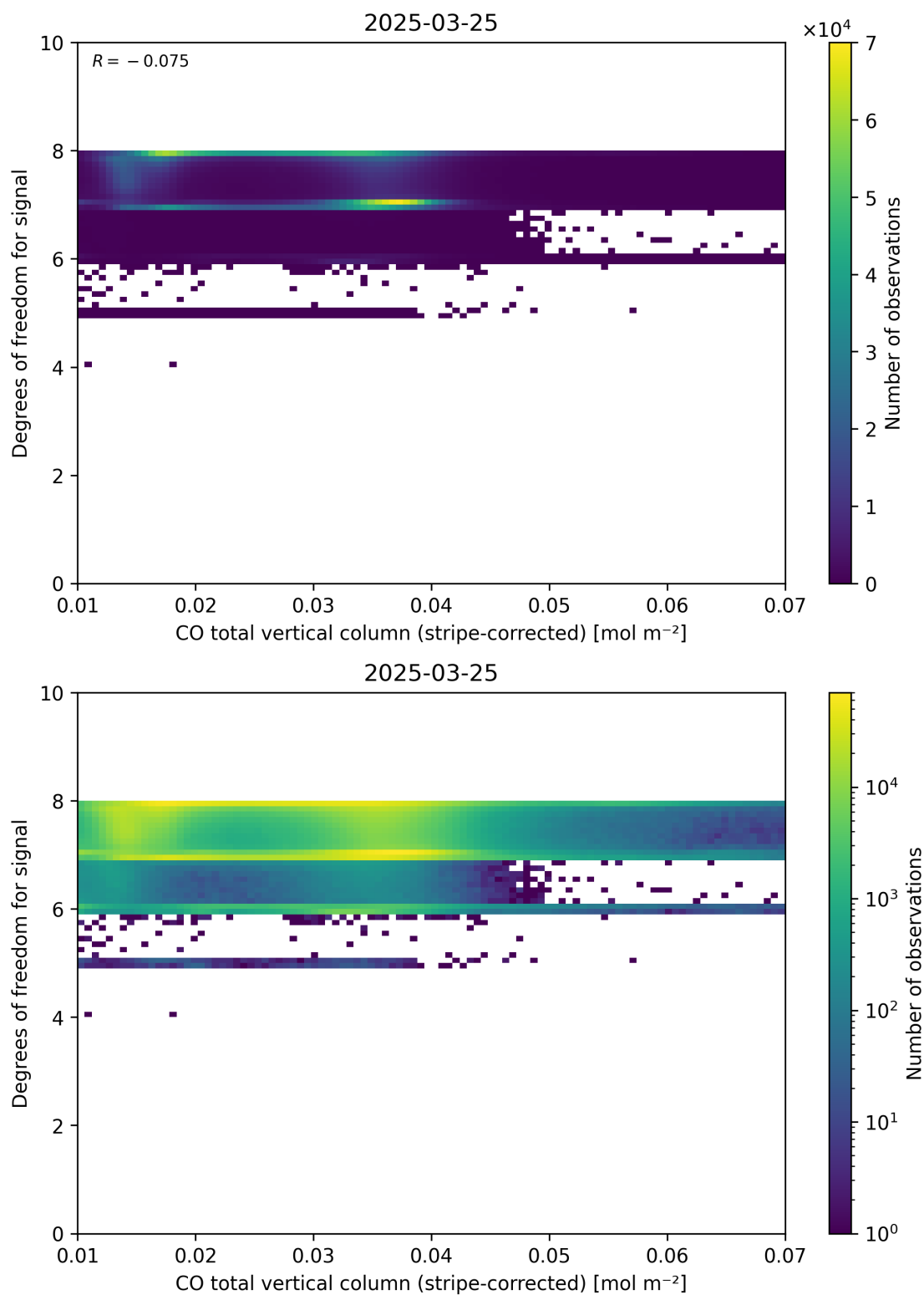
Figure 38: Scatter density plot of “CO total vertical column (stripe-corrected)” against “Degrees of freedom for signal” for 2025-03-24 to 2025-03-26.
