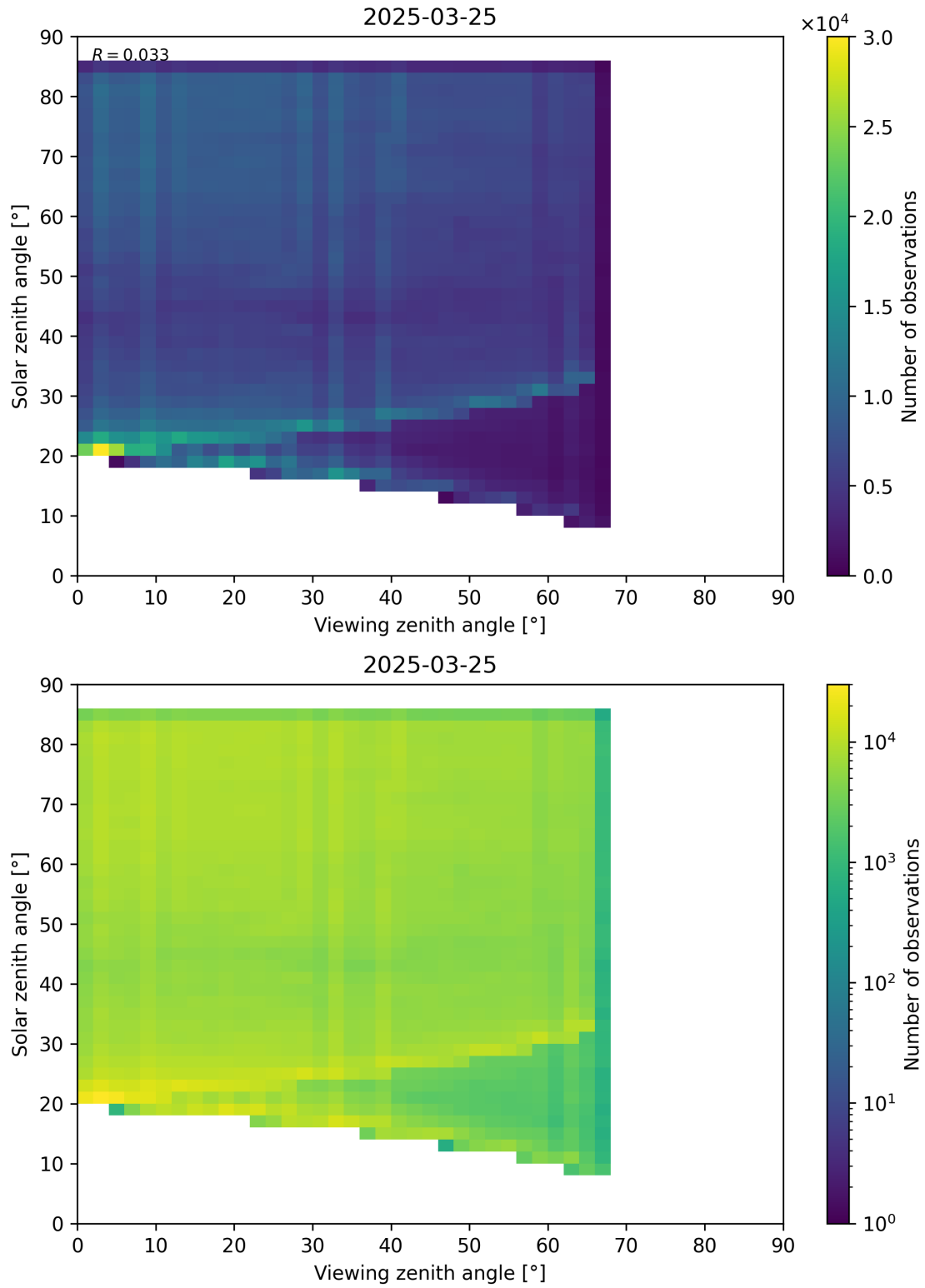
Figure 77: Scatter density plot of “Viewing zenith angle” against “Solar zenith angle” for 2025-03-24 to 2025-03-26.
