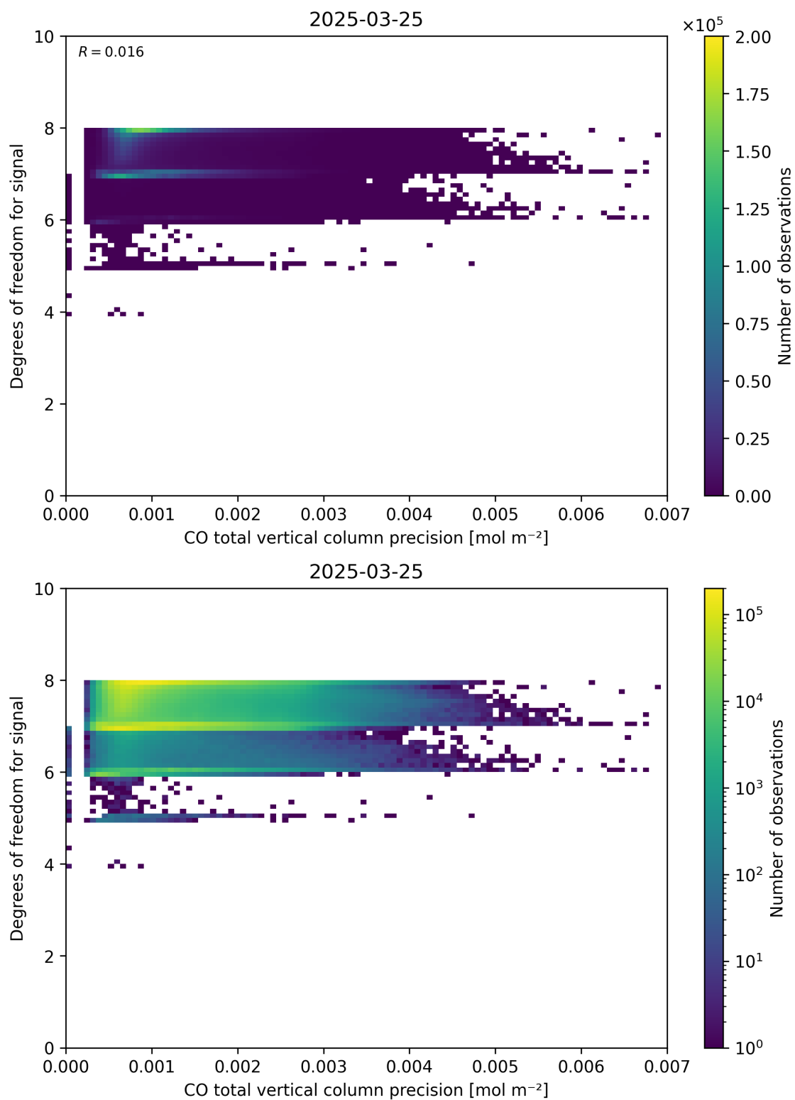
Figure 45: Scatter density plot of “CO total vertical column precision” against “Degrees of freedom for signal” for 2025-03-24 to 2025-03-26.
