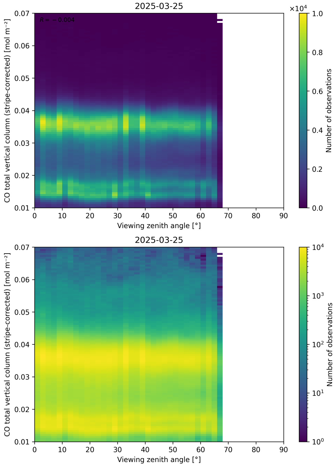
Figure 70: Scatter density plot of “Viewing zenith angle” against “CO total vertical column (stripe-corrected)” for 2025-03-24 to 2025-03-26.
