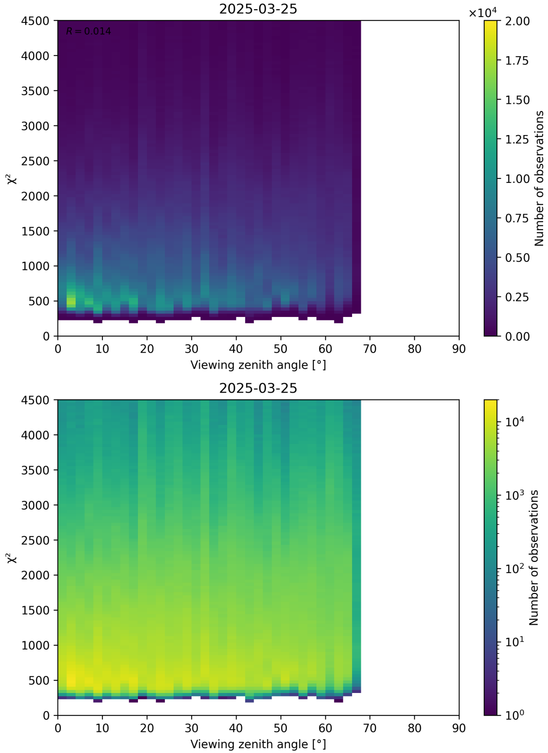
Figure 72: Scatter density plot of “Viewing zenith angle” against “ \chi^2 ” for 2025-03-24 to 2025-03-26.
