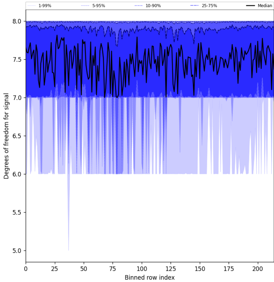
Figure 31: Along track statistics of “Degrees of freedom for signal” for 2025-03-24 to 2025-03-26
