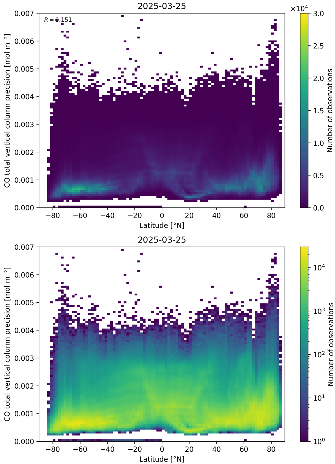
Figure 53: Scatter density plot of “Latitude” against “CO total vertical column precision” for 2025-03-24 to 2025-03-26.
