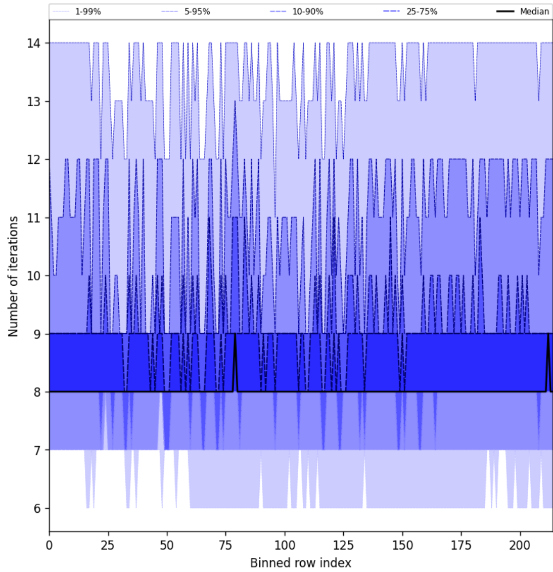
Figure 32: Along track statistics of “Number of iterations” for 2025-03-24 to 2025-03-26
