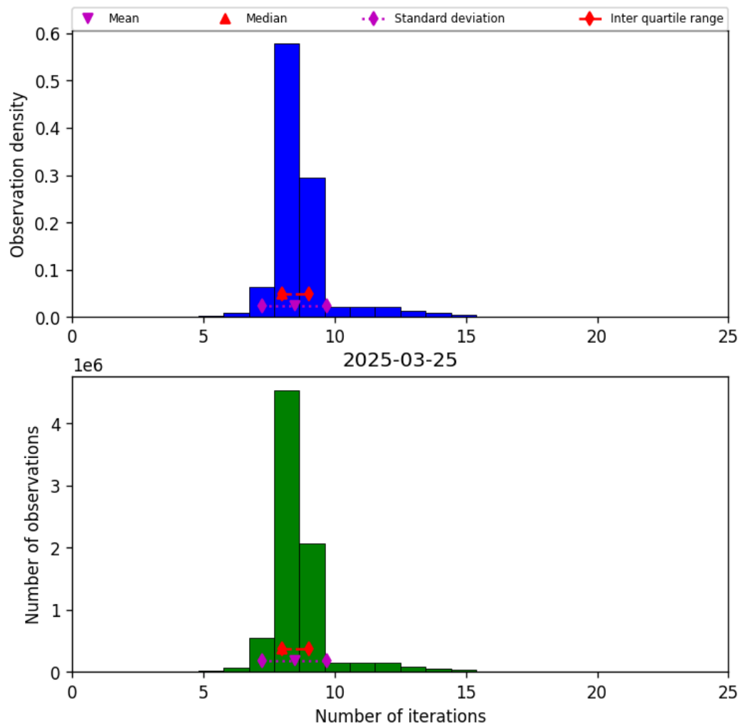
Figure 24: Histogram of “Number of iterations” for 2025-03-24 to 2025-03-26
