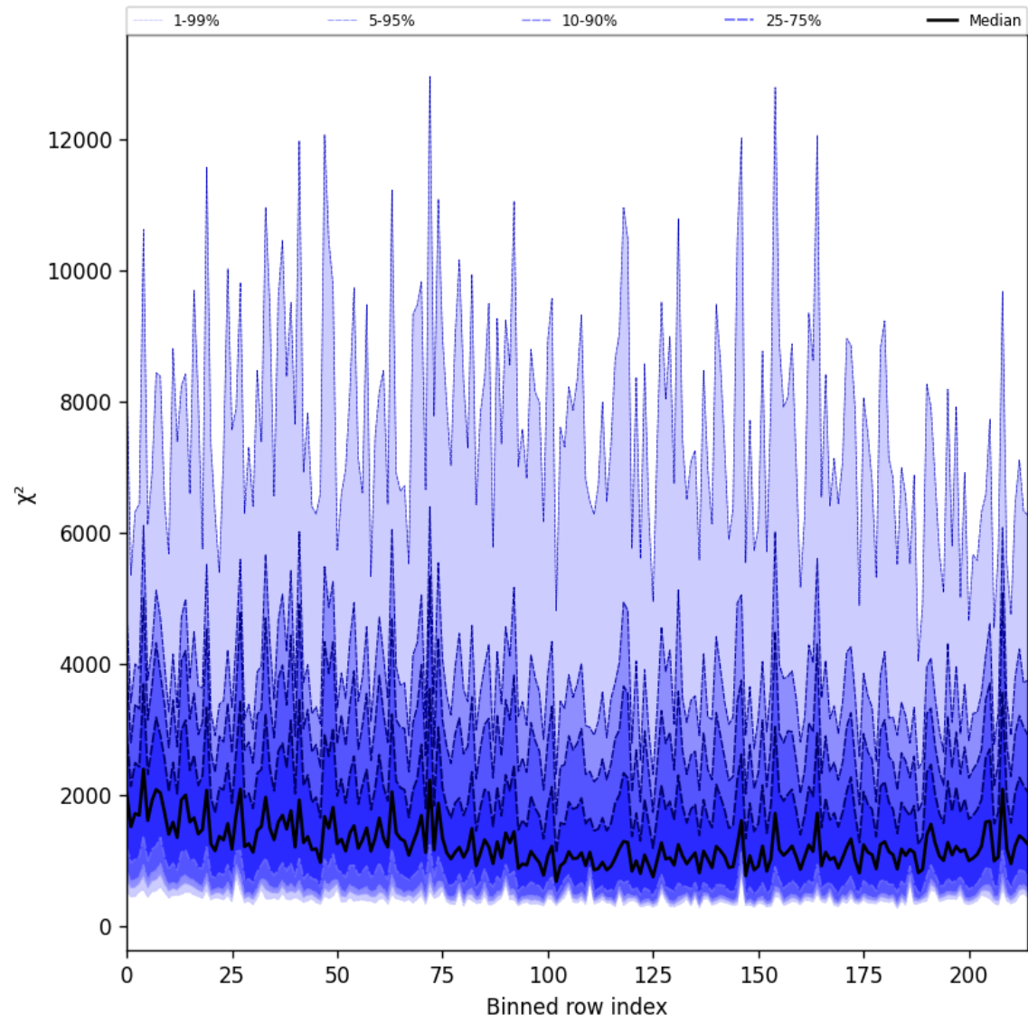
Figure 30: Along track statistics of “ \chi^2 ” for 2025-03-24 to 2025-03-26
