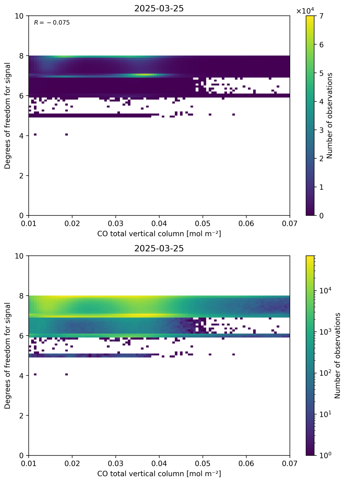
Figure 41: Scatter density plot of “CO total vertical column” against “Degrees of freedom for signal” for 2025-03-24 to 2025-03-26.
