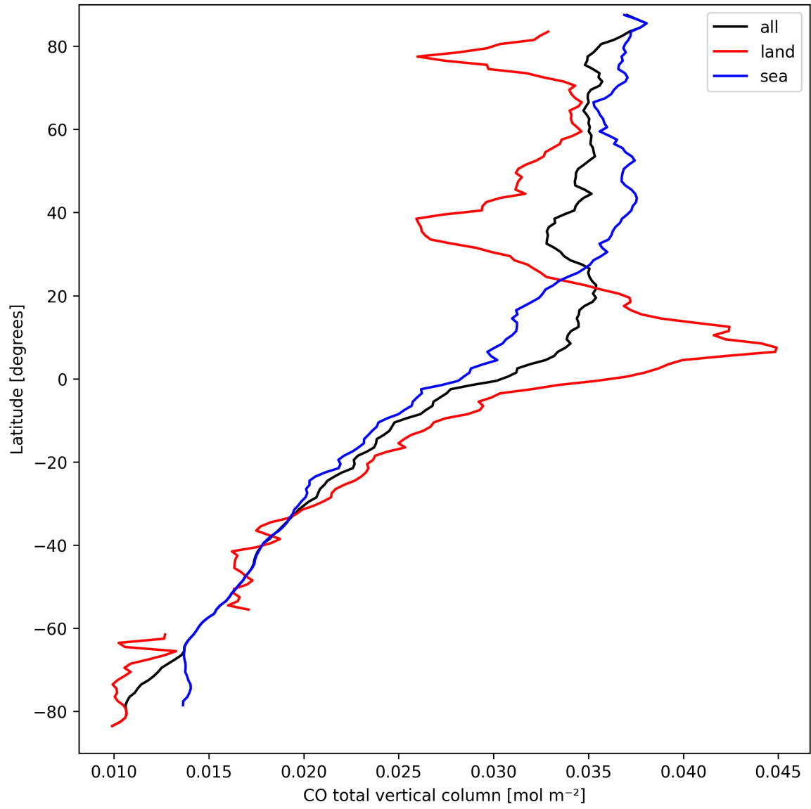
Figure 10: Zonal average of “CO total vertical column” for 2025-03-24 to 2025-03-26.
