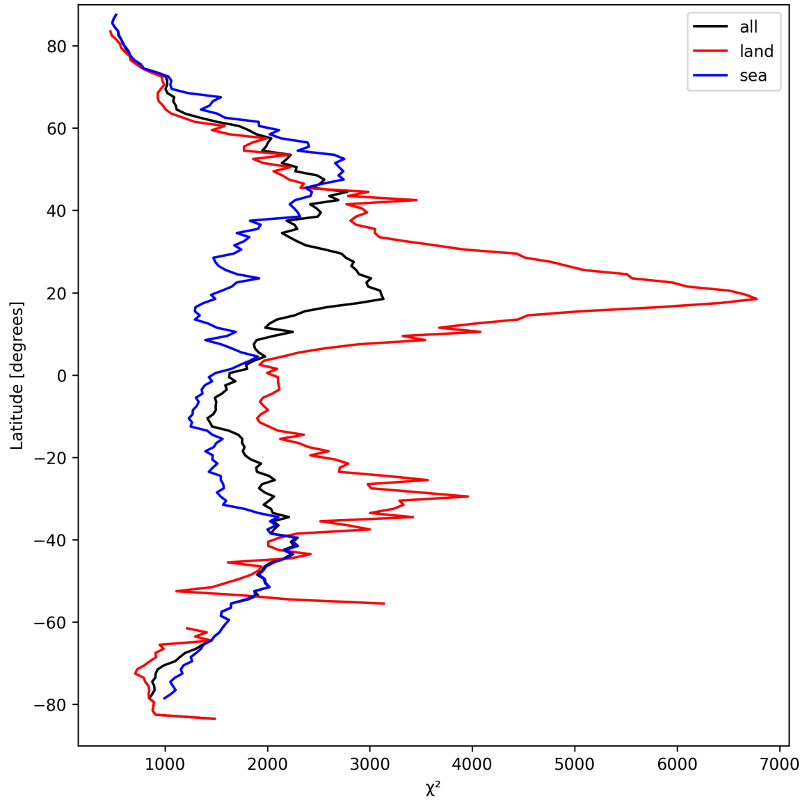
Figure 14: Zonal average of “ \chi^2 ” for 2025-03-24 to 2025-03-26.
