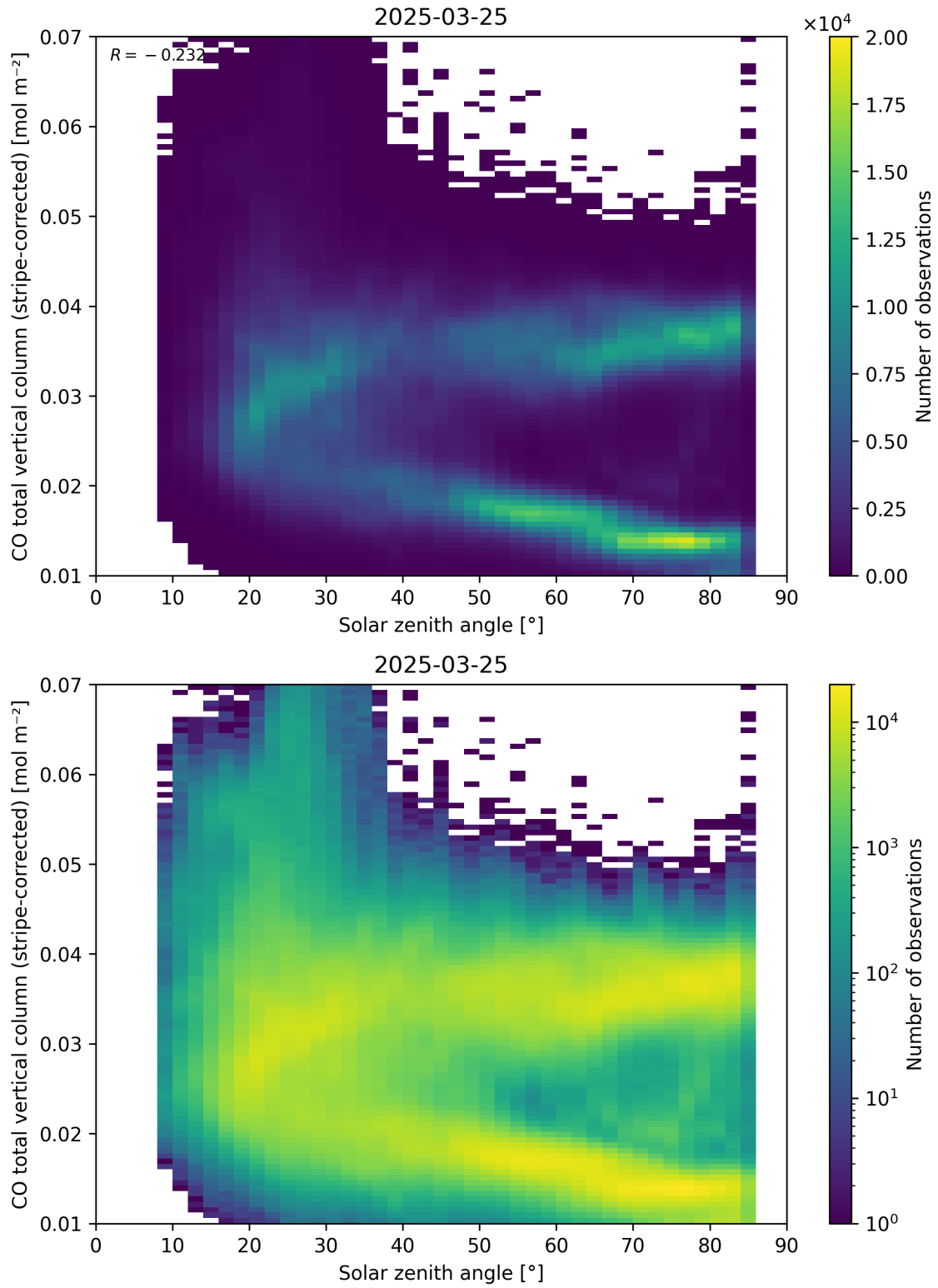
Figure 62: Scatter density plot of “Solar zenith angle” against “CO total vertical column (stripe-corrected)” for 2025-03-24 to 2025-03-26.
