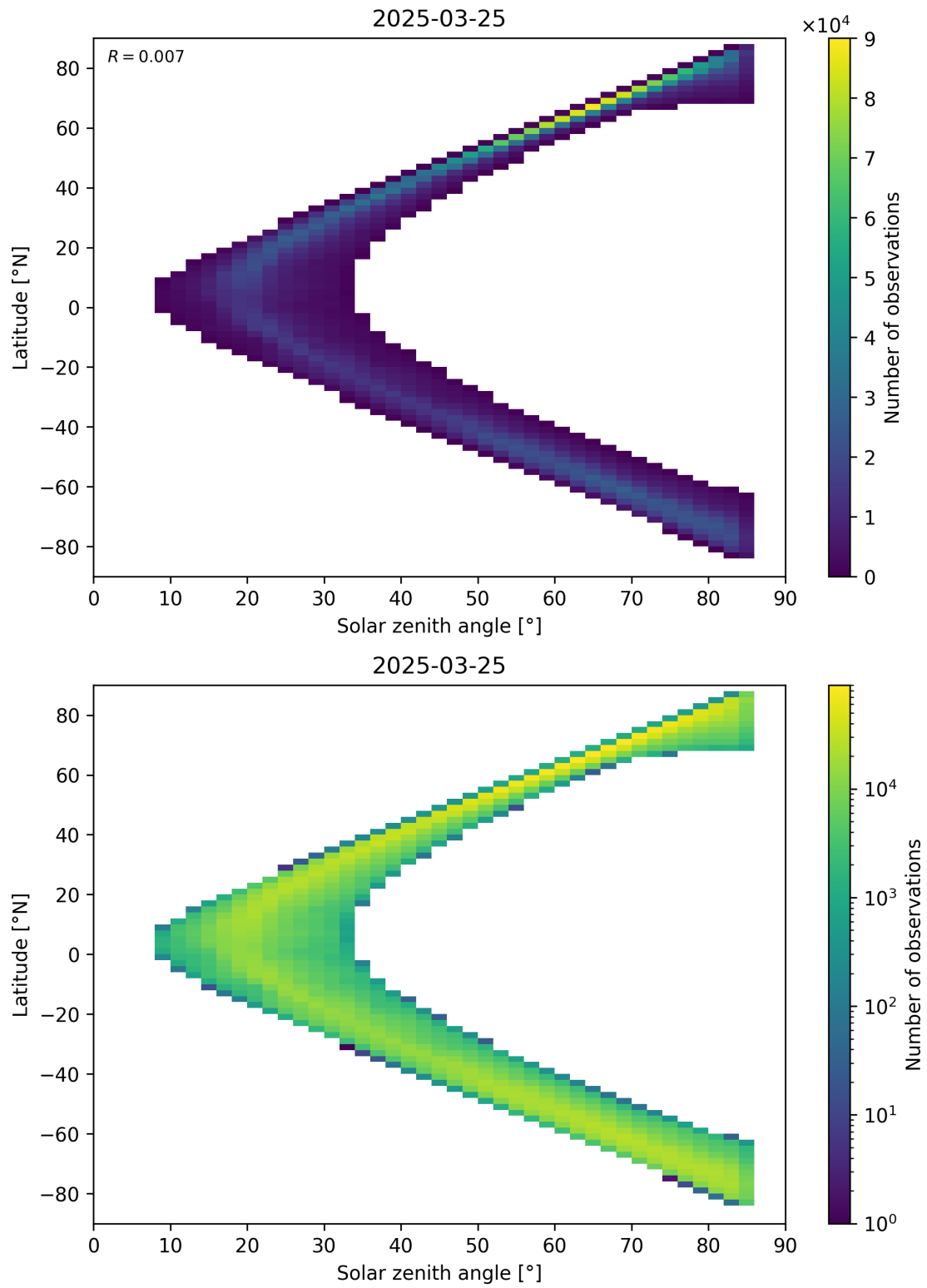
Figure 66: Scatter density plot of “Solar zenith angle” against “Latitude” for 2025-03-24 to 2025-03-26.
