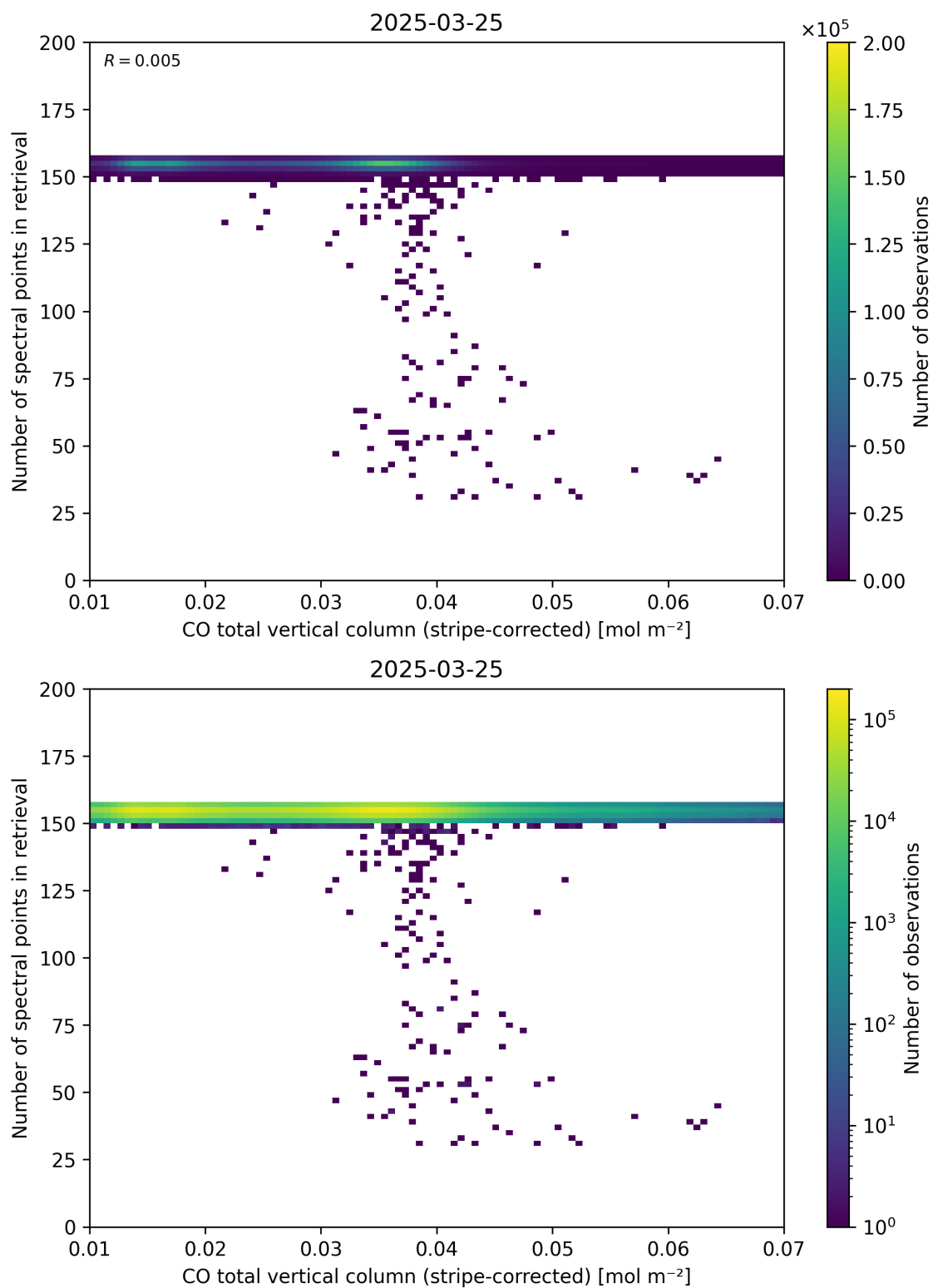
Figure 40: Scatter density plot of “CO total vertical column (stripe-corrected)” against “Number of spectral points in retrieval” for 2025-03-24 to 2025-03-26.
