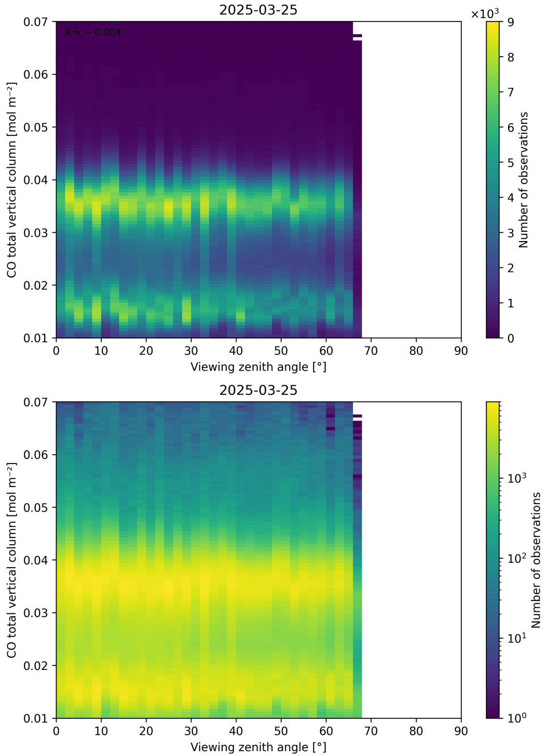
Figure 69: Scatter density plot of “Viewing zenith angle” against “CO total vertical column” for 2025-03-24 to 2025-03-26.
