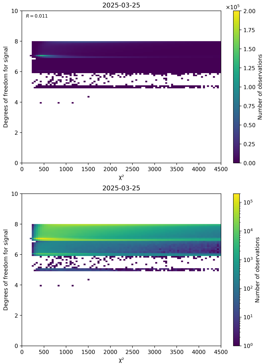
Figure 48: Scatter density plot of “ \chi^2 ” against “Degrees of freedom for signal” for 2025-03-24 to 2025-03-26.
