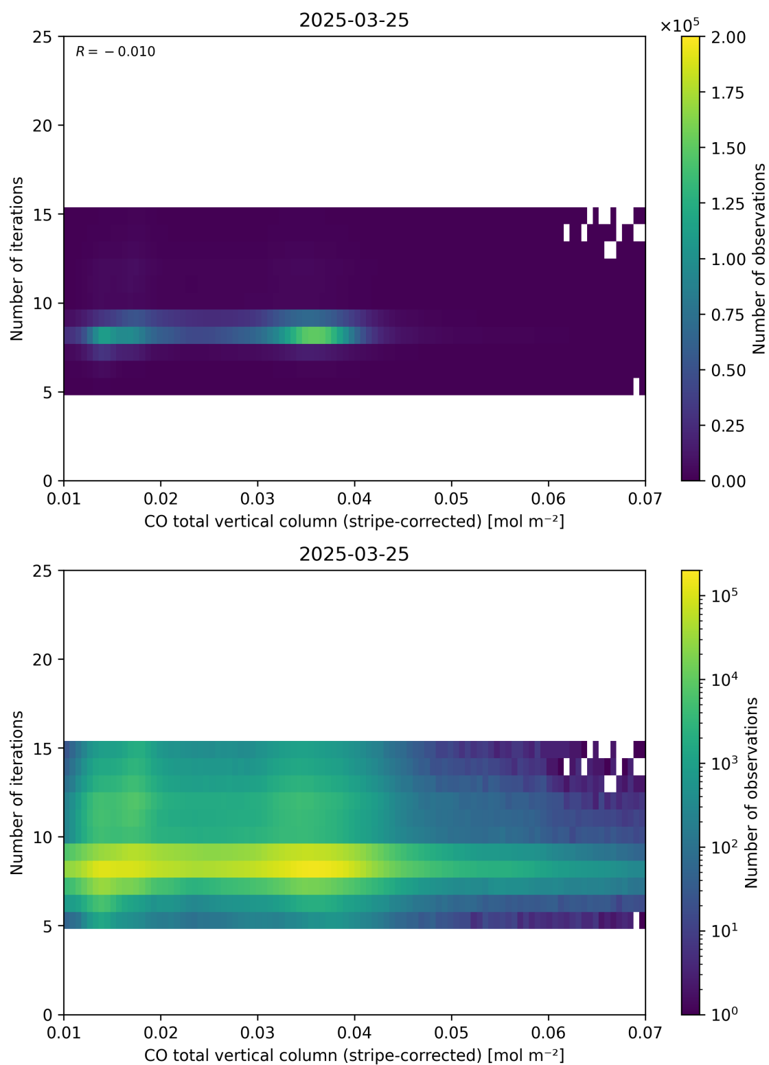
Figure 39: Scatter density plot of “CO total vertical column (stripe-corrected)” against “Number of iterations” for 2025-03-24 to 2025-03-26.
