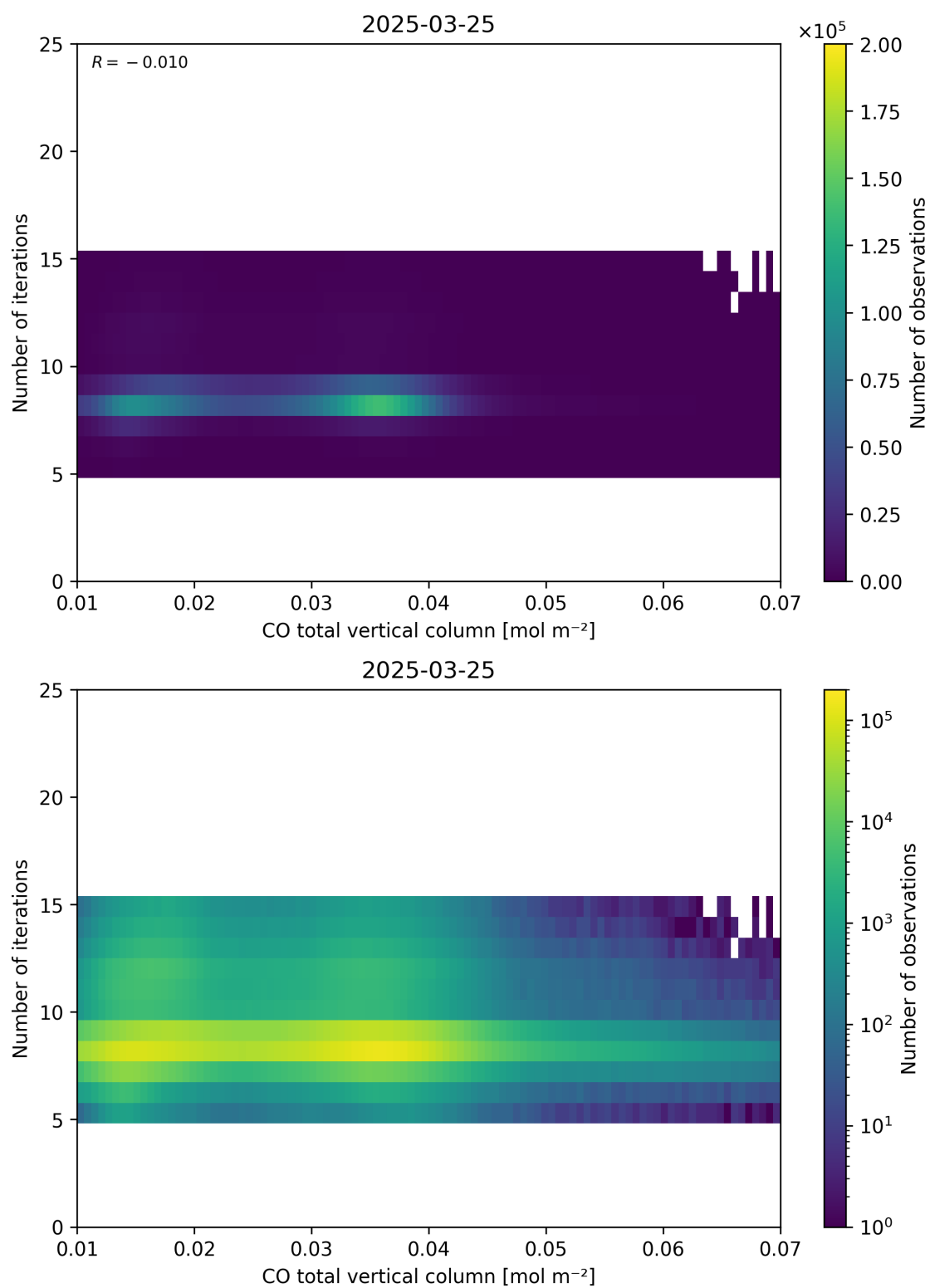
Figure 42: Scatter density plot of “CO total vertical column” against “Number of iterations” for 2025-03-24 to 2025-03-26.
