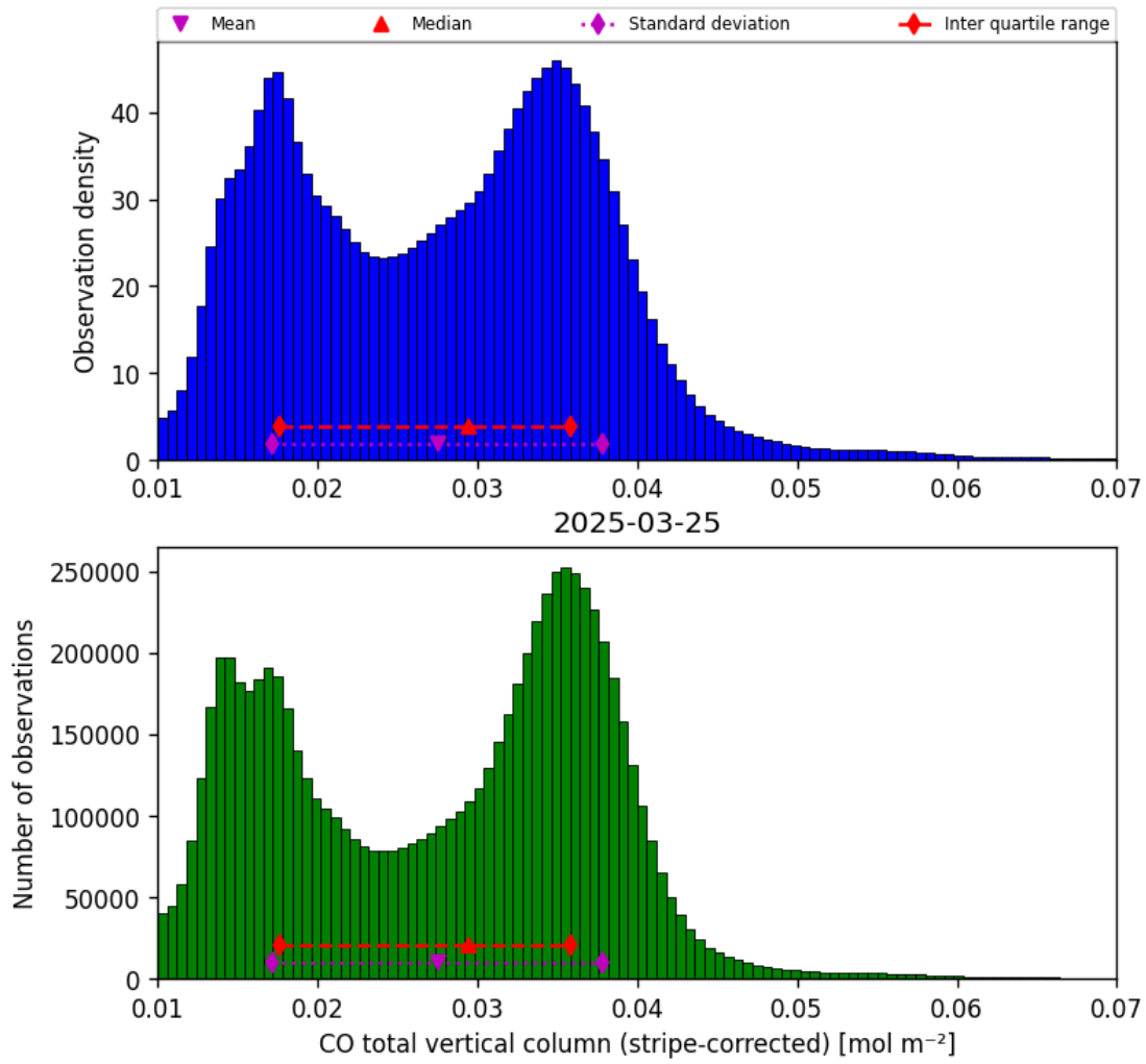
Figure 19: Histogram of “CO total vertical column (stripe-corrected)” for 2025-03-24 to 2025-03-26
