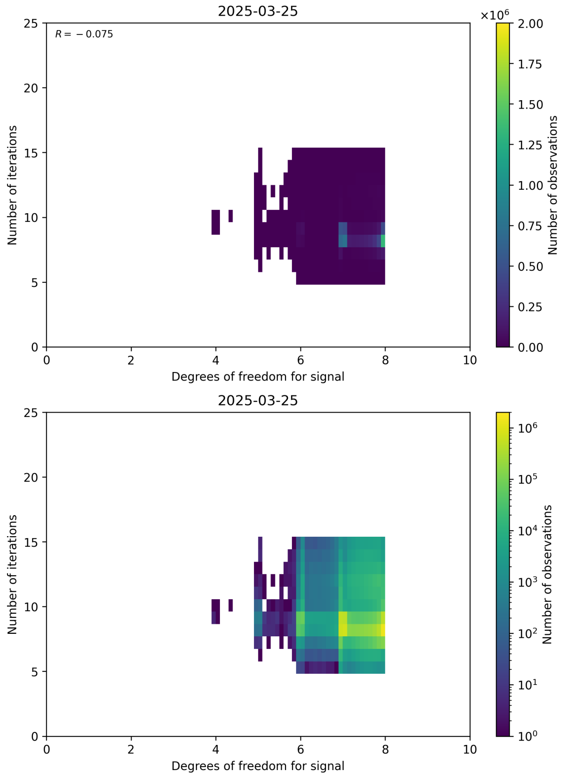
Figure 50: Scatter density plot of “Degrees of freedom for signal” against “Number of iterations” for 2025-03-24 to 2025-03-26.
