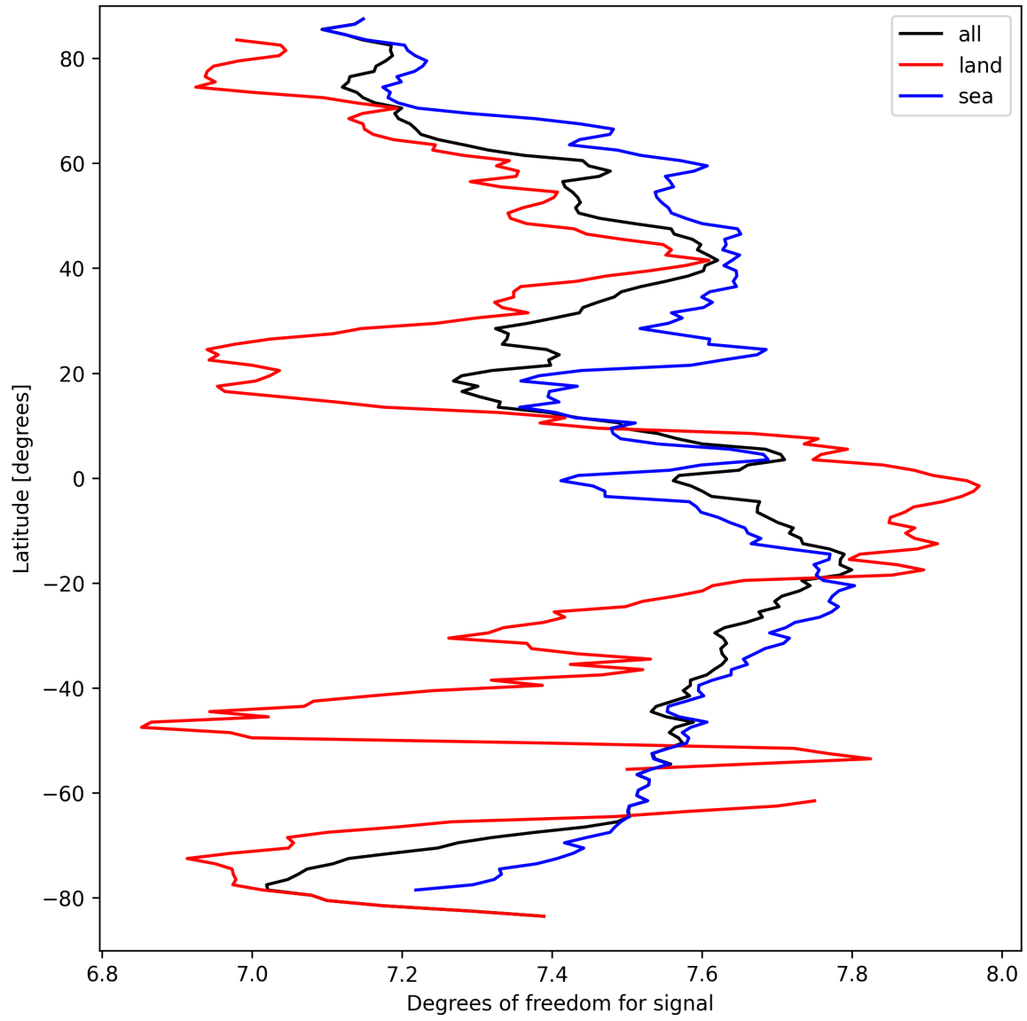
Figure 15: Zonal average of “Degrees of freedom for signal” for 2025-03-24 to 2025-03-26.
