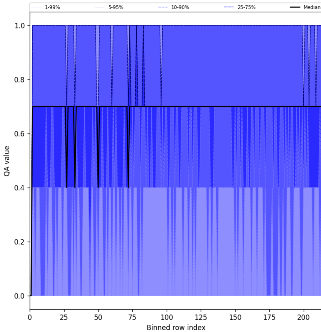
Figure 25: Along track statistics of “QA value” for 2025-03-24 to 2025-03-26
