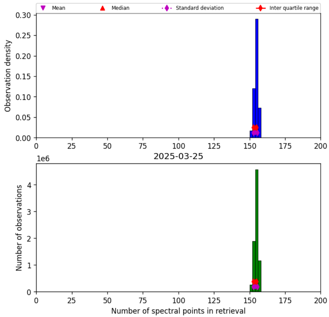
Figure 21: Histogram of “Number of spectral points in retrieval” for 2025-03-24 to 2025-03-26
