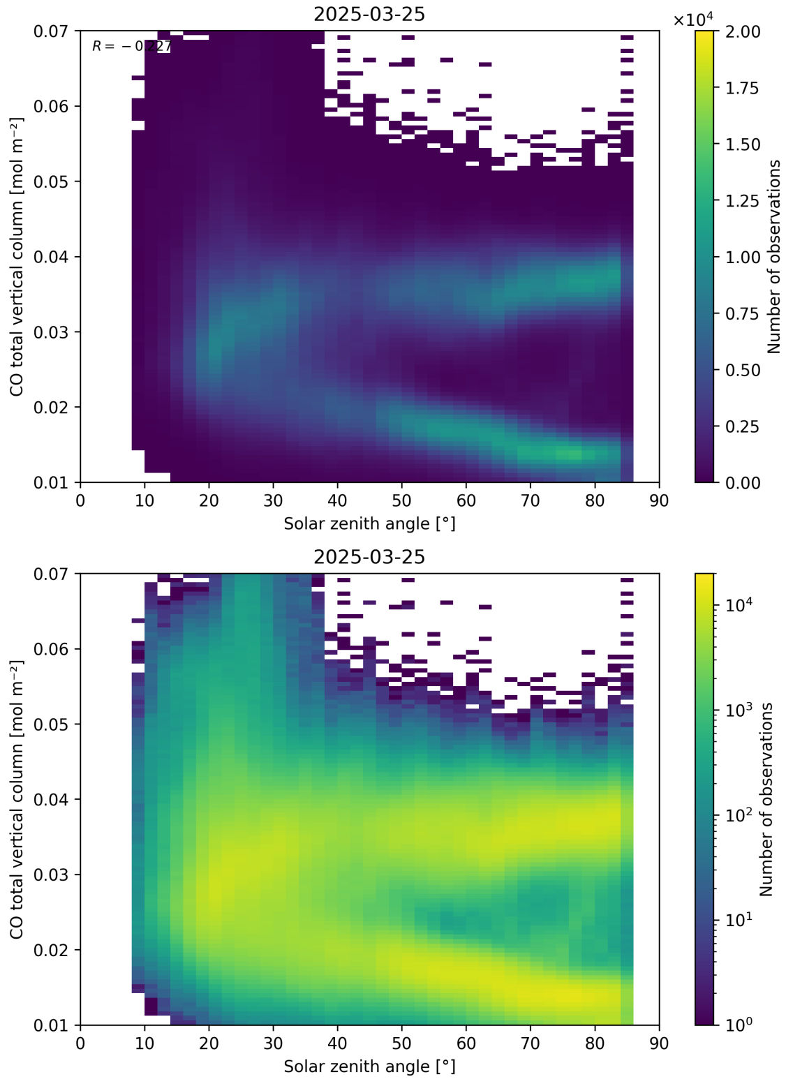
Figure 61: Scatter density plot of “Solar zenith angle” against “CO total vertical column” for 2025-03-24 to 2025-03-26.
