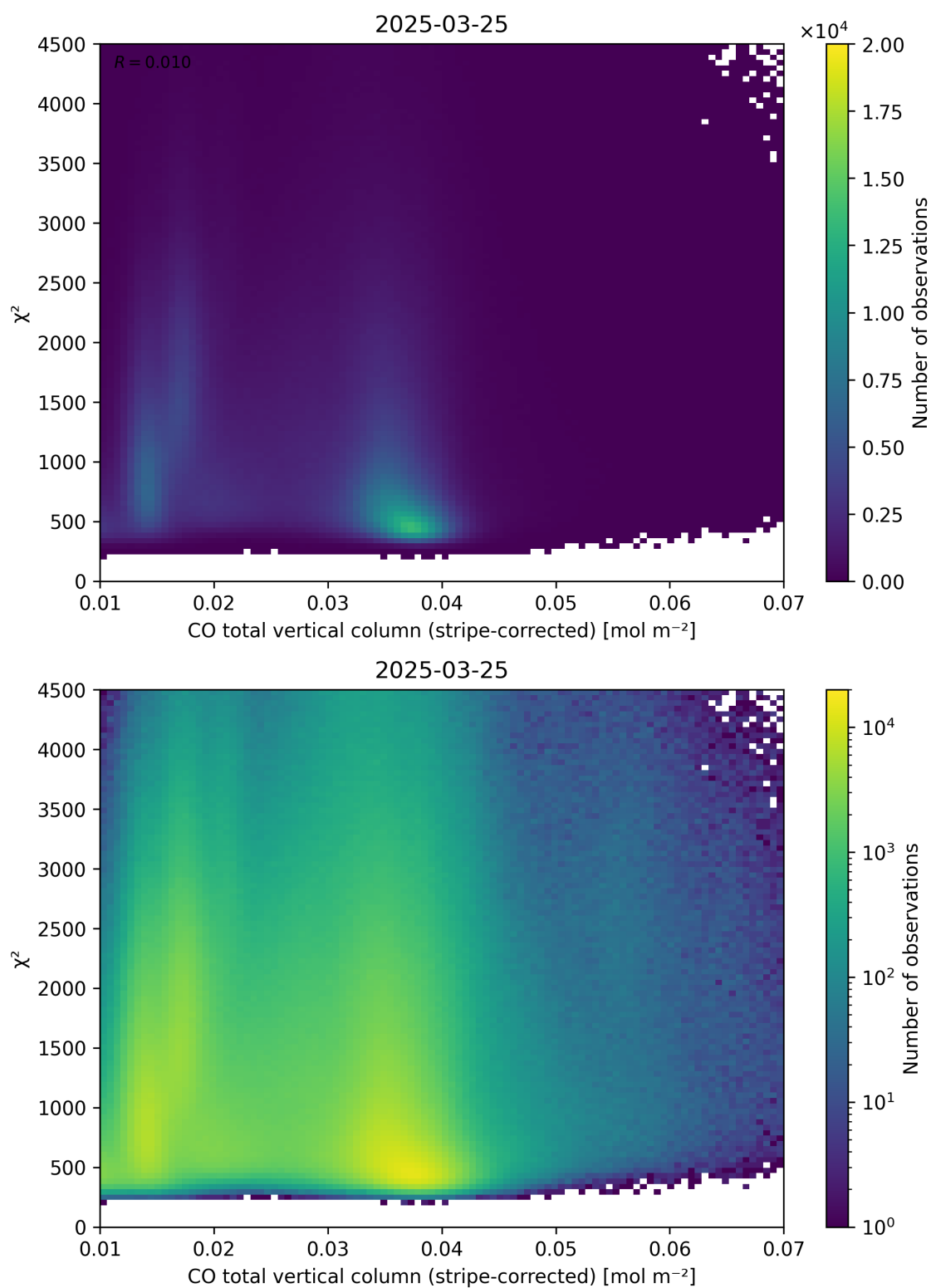
Figure 37: Scatter density plot of “CO total vertical column (stripe-corrected)” against “ \chi^2 ” for 2025-03-24 to 2025-03-26.
