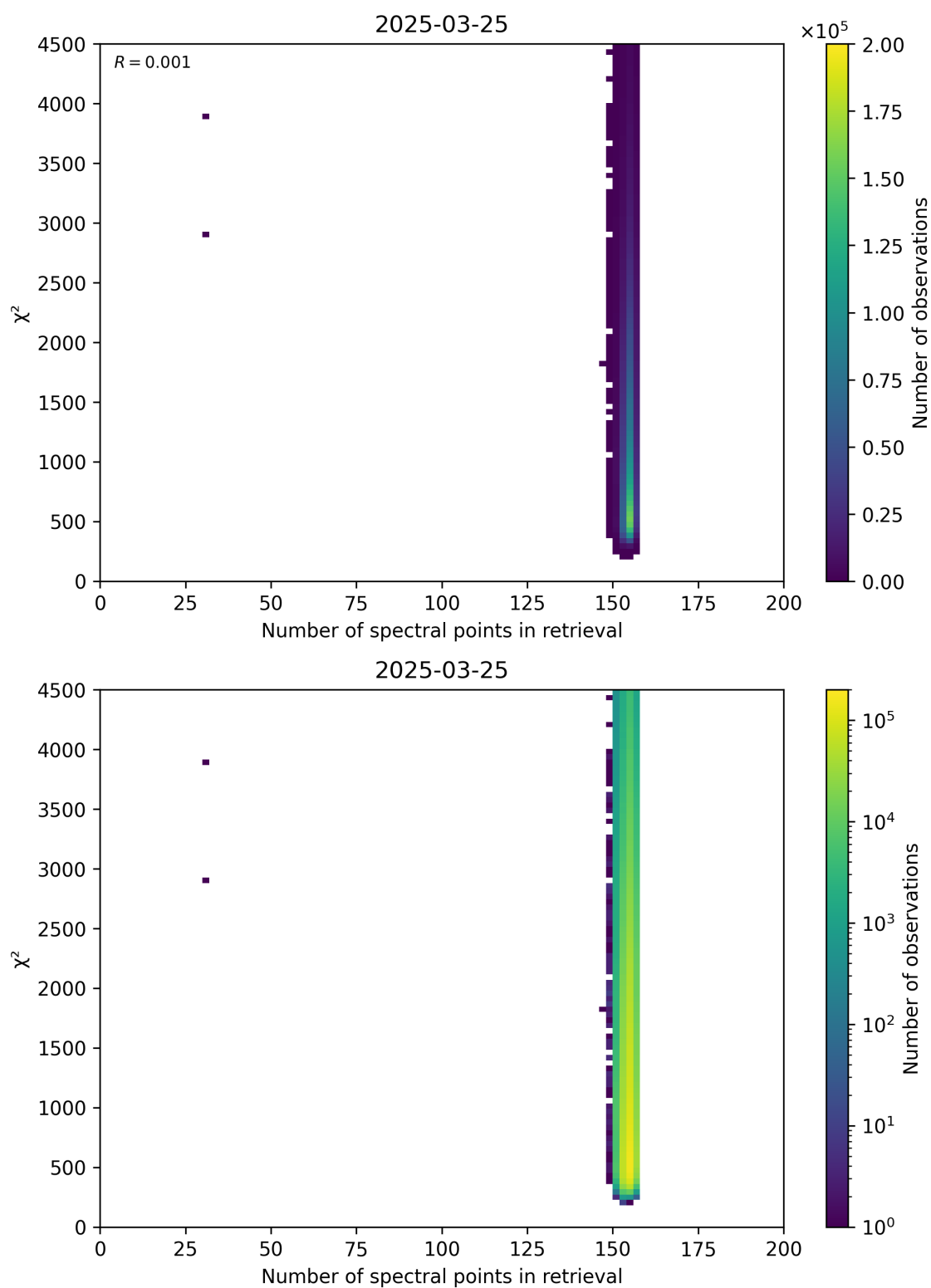
Figure 58: Scatter density plot of “Number of spectral points in retrieval” against “ \chi^2 ” for 2025-03-24 to 2025-03-26.
