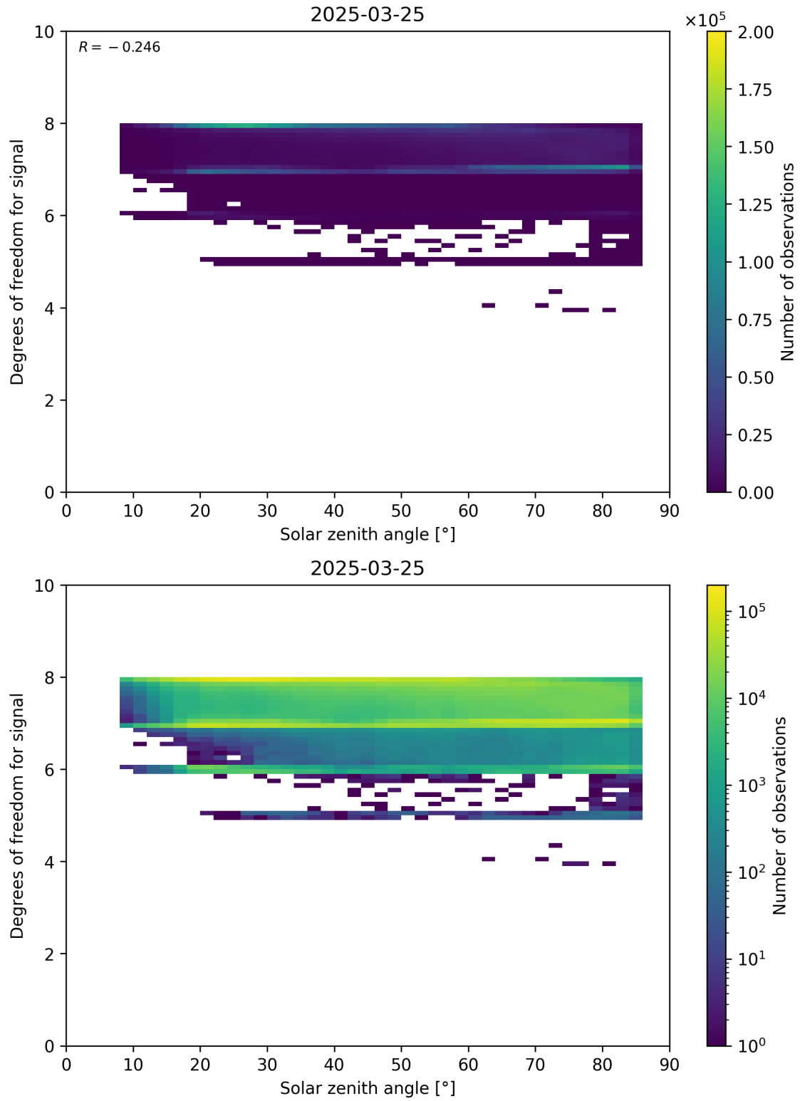
Figure 65: Scatter density plot of “Solar zenith angle” against “Degrees of freedom for signal” for 2025-03-24 to 2025-03-26.
