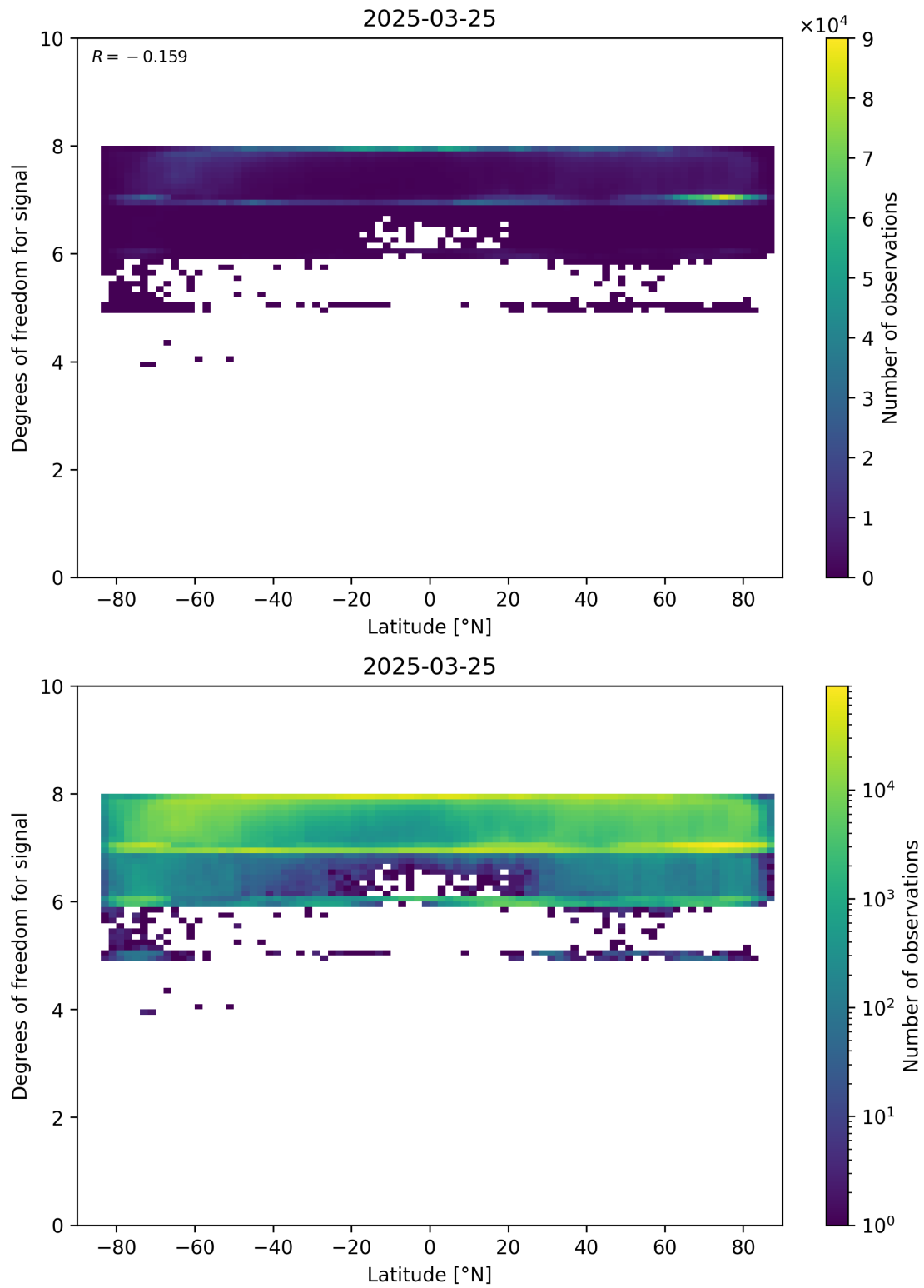
Figure 55: Scatter density plot of “Latitude” against “Degrees of freedom for signal” for 2025-03-24 to 2025-03-26.
