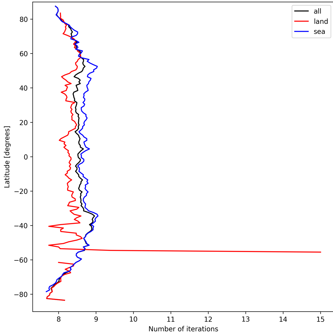
Figure 16: Zonal average of “Number of iterations” for 2025-03-24 to 2025-03-26.
