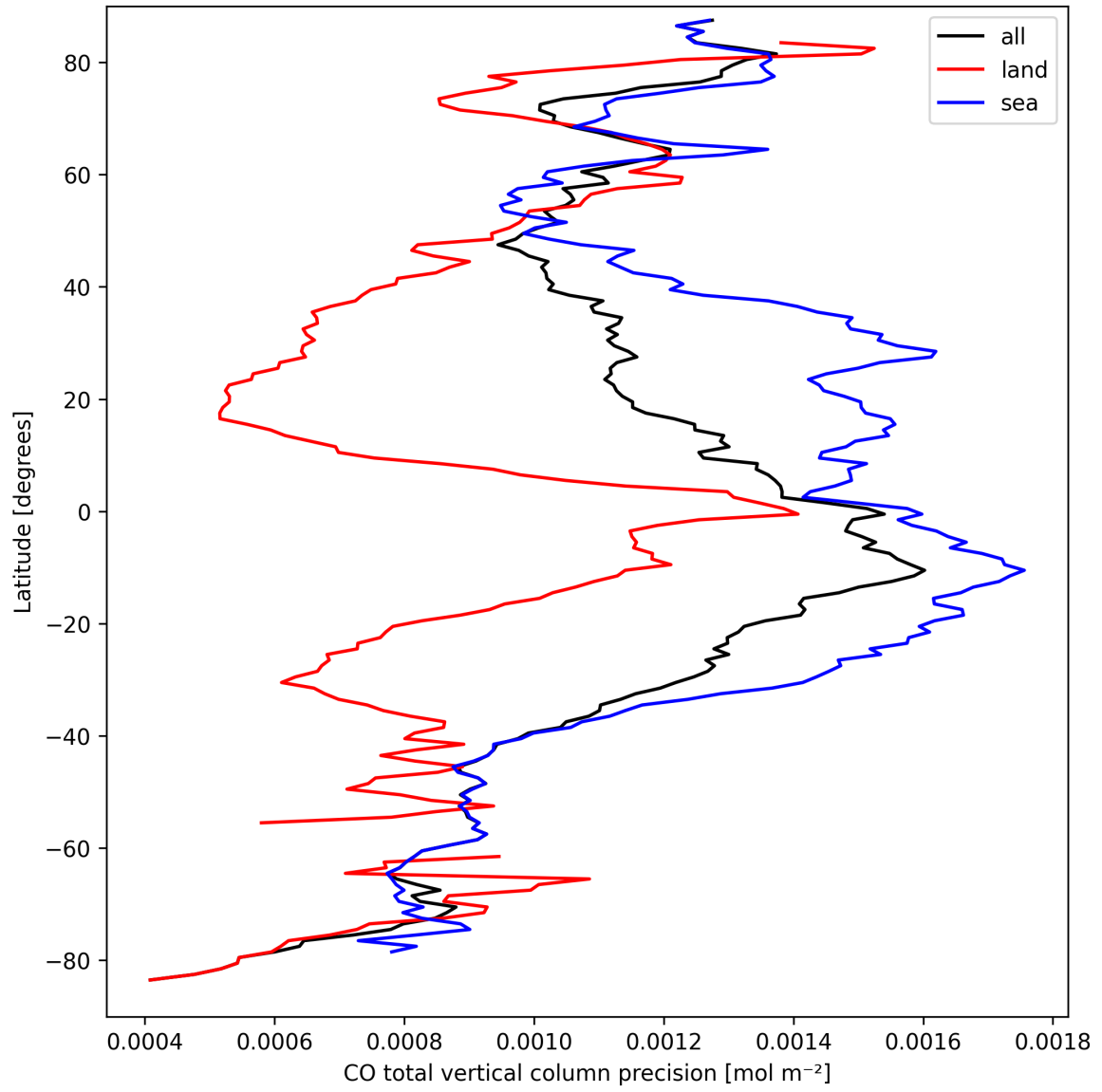
Figure 12: Zonal average of "CO total vertical column precision" for 2025-03-24 to 2025-03-26.
