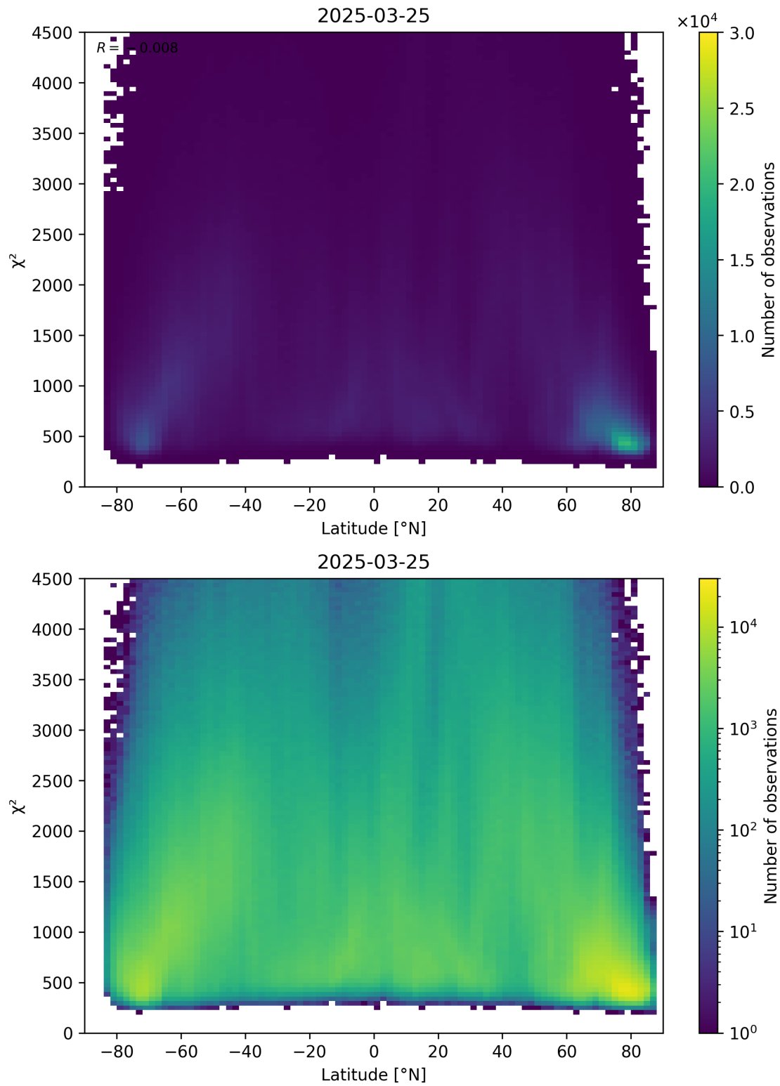
Figure 54: Scatter density plot of “Latitude” against “ \chi^2 ” for 2025-03-24 to 2025-03-26.
