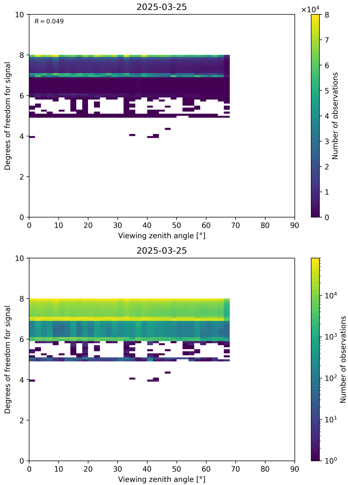
Figure 73: Scatter density plot of “Viewing zenith angle” against “Degrees of freedom for signal” for 2025-03-24 to 2025-03-26.
