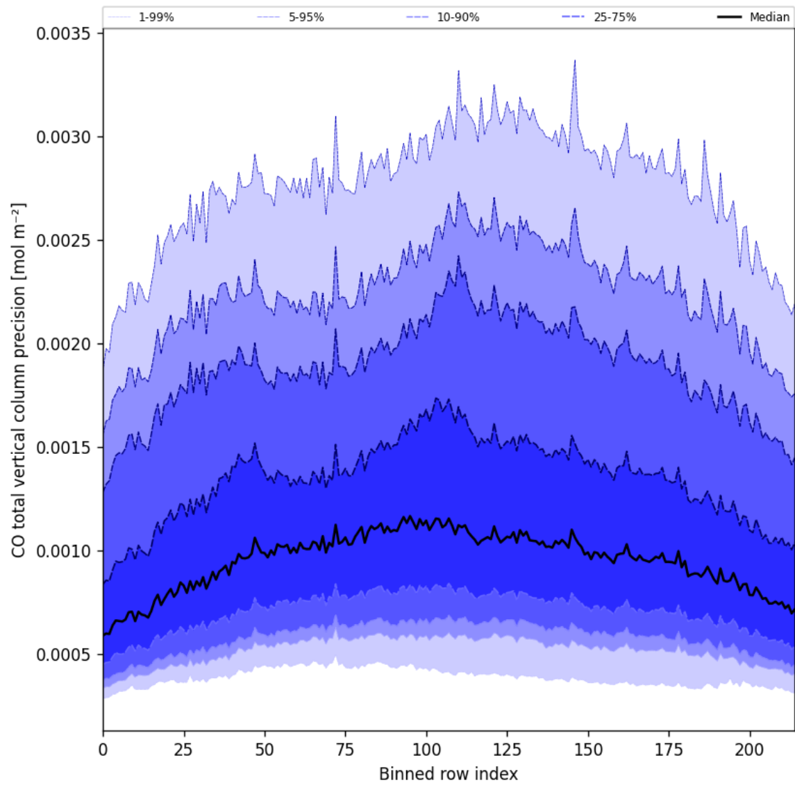
Figure 28: Along track statistics of “CO total vertical column precision” for 2025-03-24 to 2025-03-26
