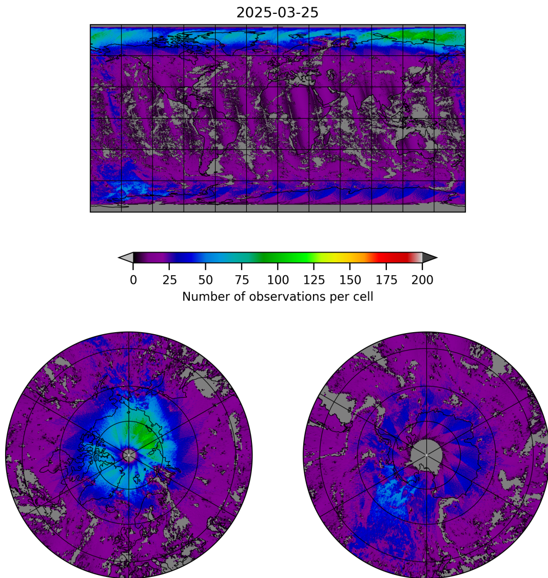
Figure 8: Map of the number of observations for 2025-03-24 to 2025-03-26
