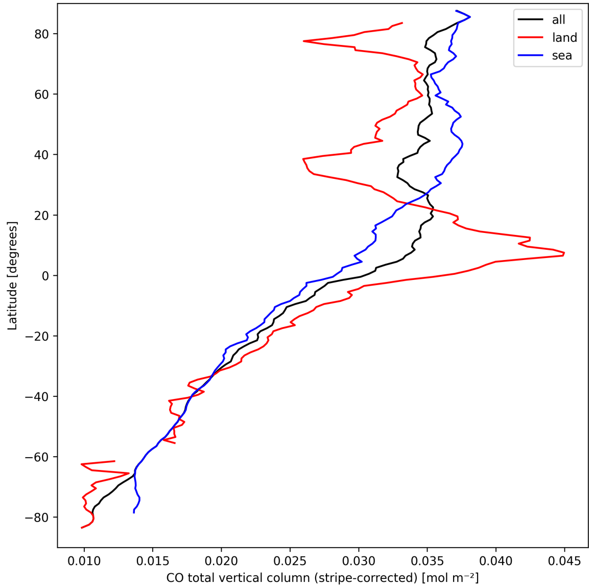
Figure 11: Zonal average of “CO total vertical column (stripe-corrected)” for 2025-03-24 to 2025-03-26.
