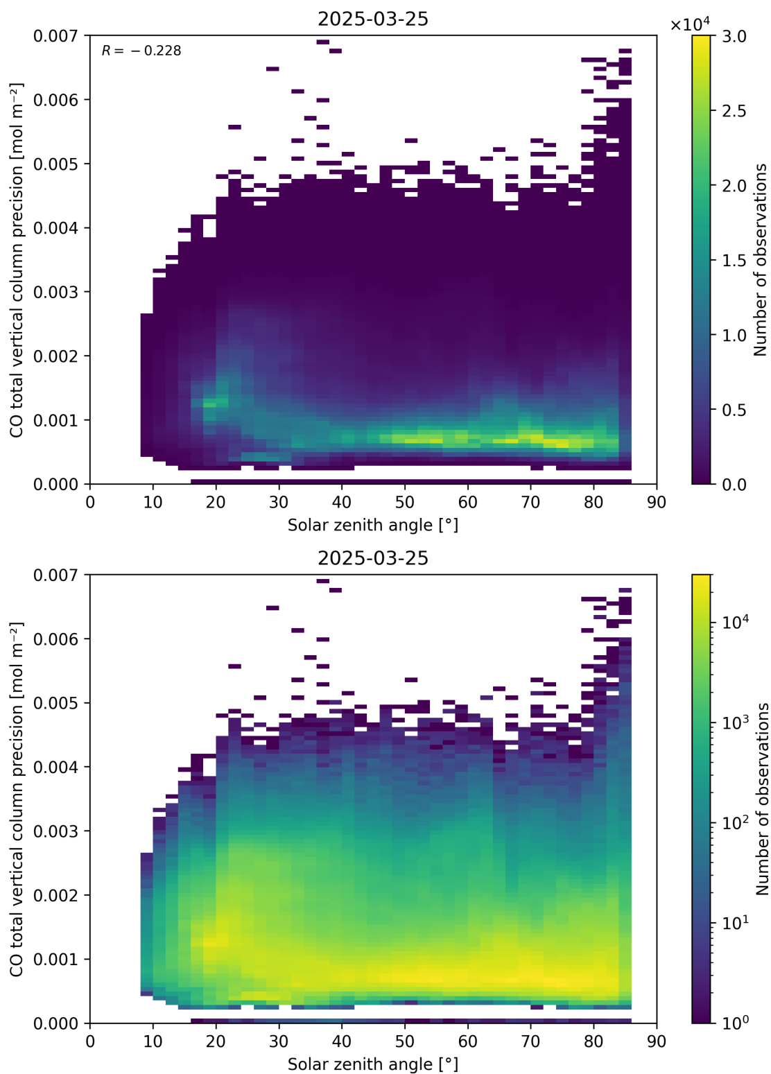
Figure 63: Scatter density plot of “Solar zenith angle” against “CO total vertical column precision” for 2025-03-24 to 2025-03-26.
