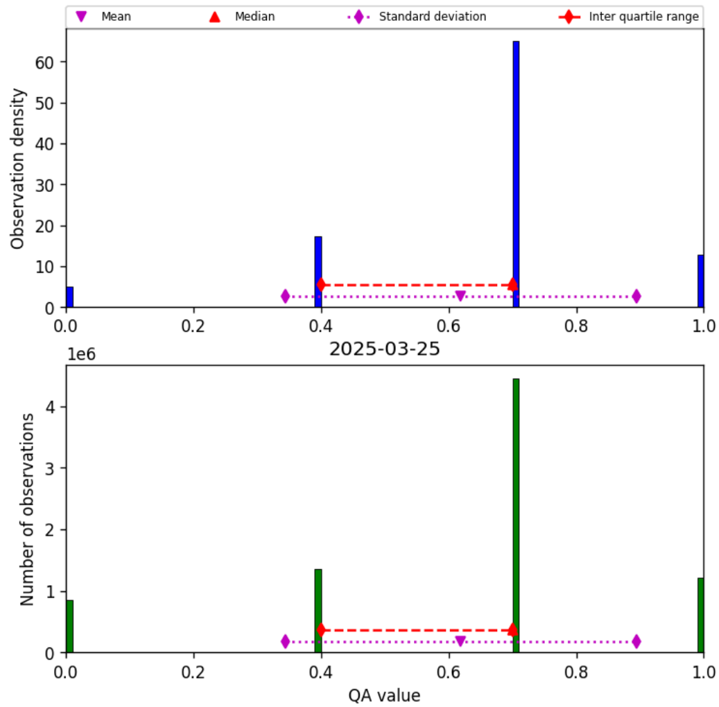
Figure 17: Histogram of “QA value” for 2025-03-24 to 2025-03-26
