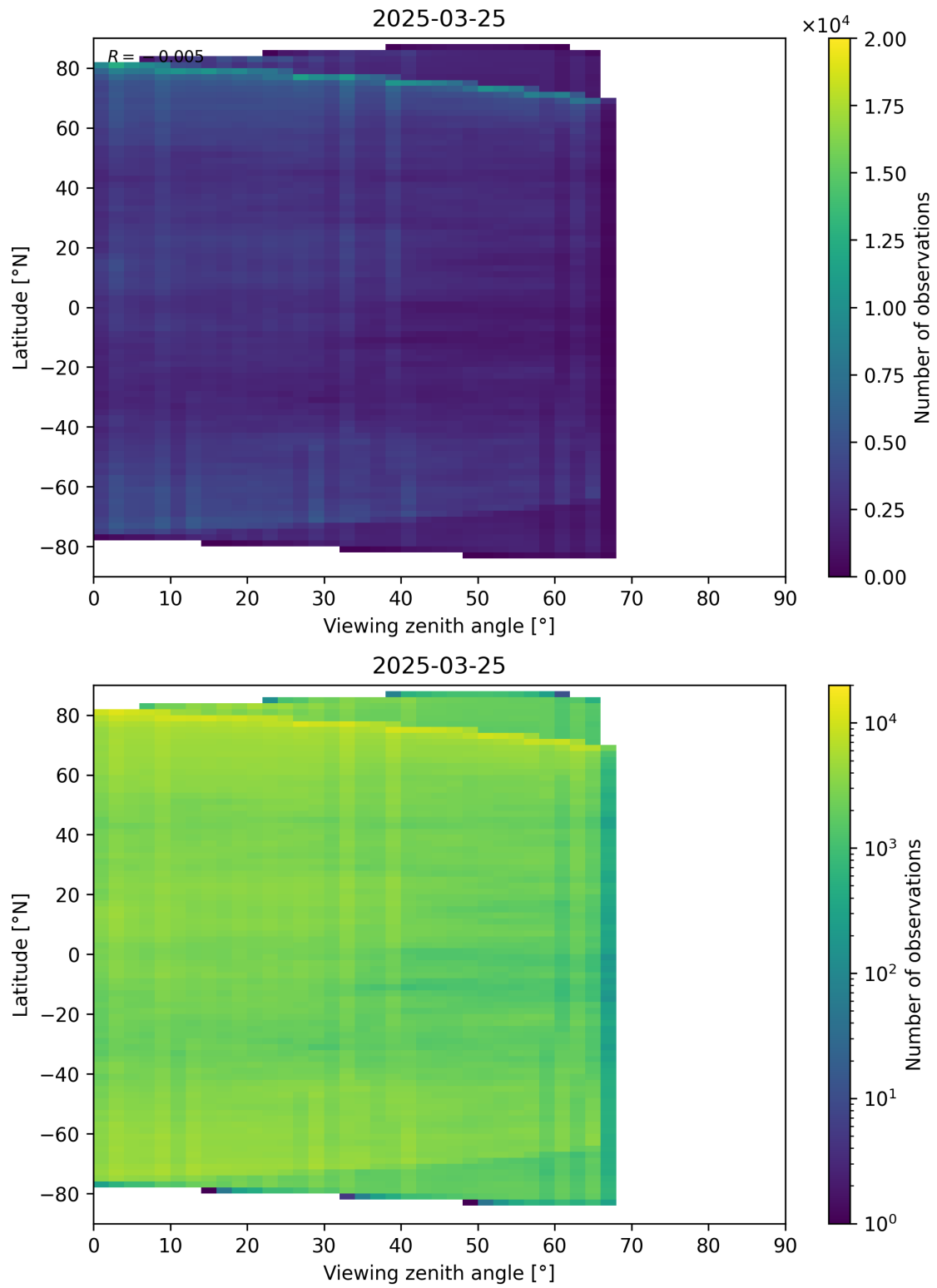
Figure 74: Scatter density plot of “Viewing zenith angle” against “Latitude” for 2025-03-24 to 2025-03-26.
