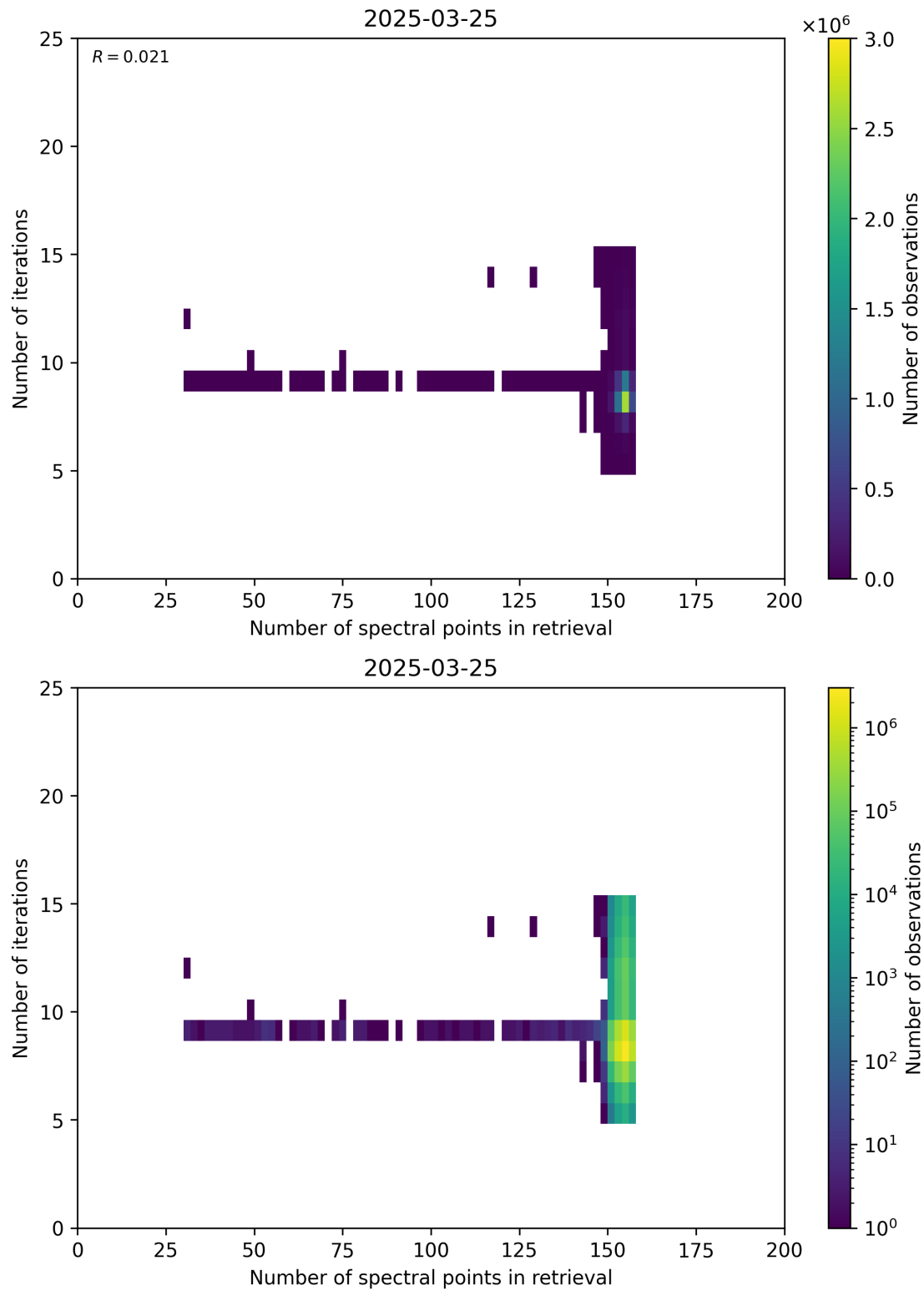
Figure 60: Scatter density plot of “Number of spectral points in retrieval” against “Number of iterations” for 2025-03-24 to 2025-03-26.
