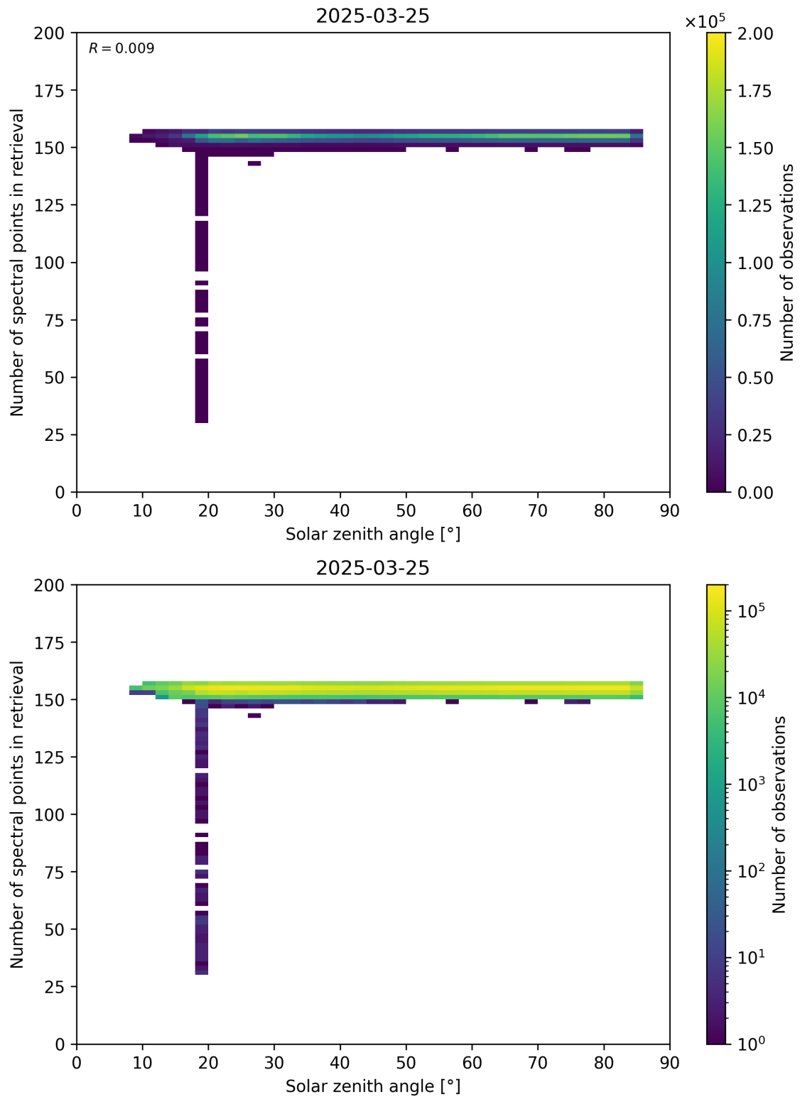
Figure 68: Scatter density plot of “Solar zenith angle” against “Number of spectral points in retrieval” for 2025-03-24 to 2025-03-26.
