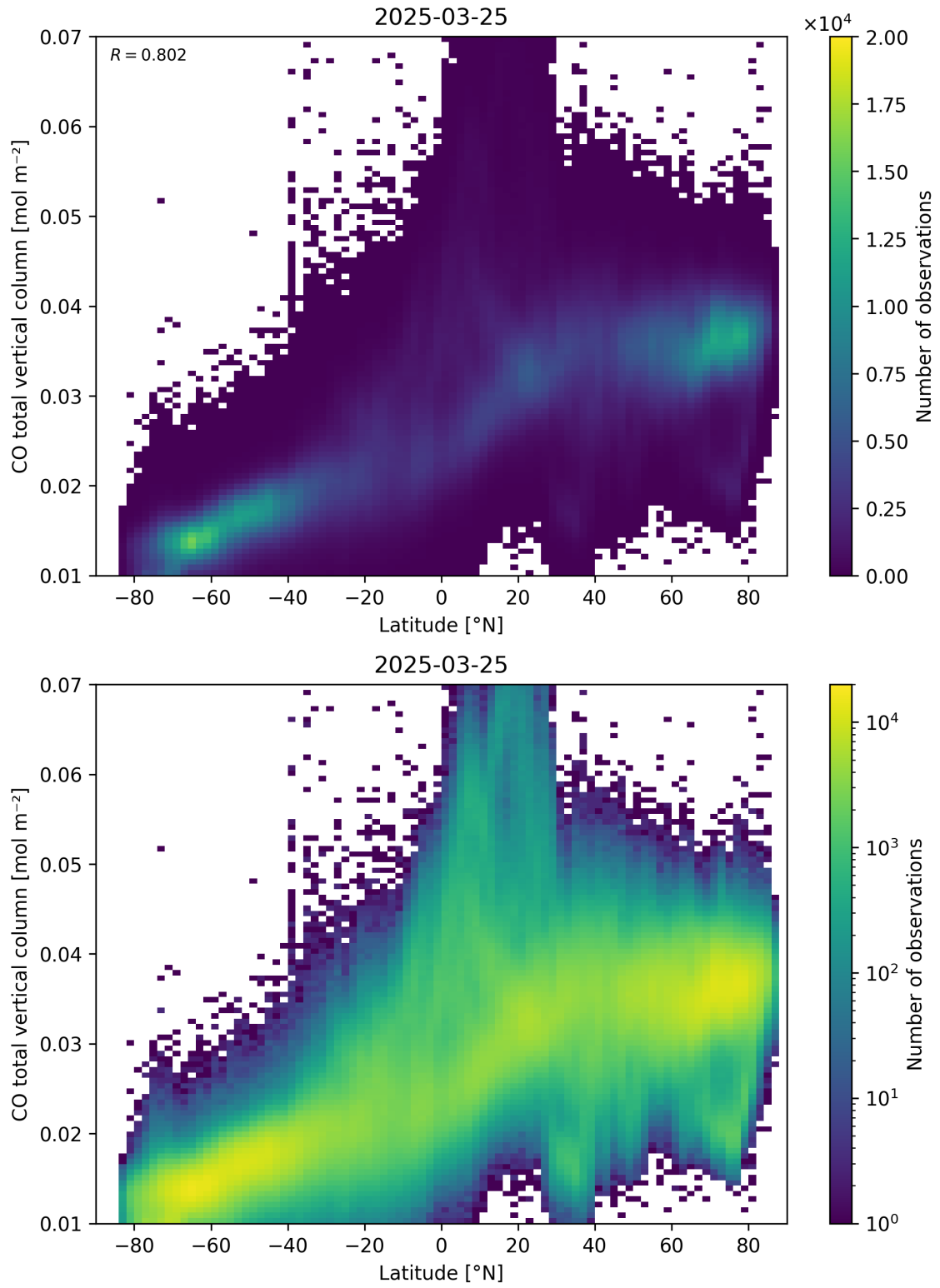
Figure 51: Scatter density plot of “Latitude” against “CO total vertical column” for 2025-03-24 to 2025-03-26.
