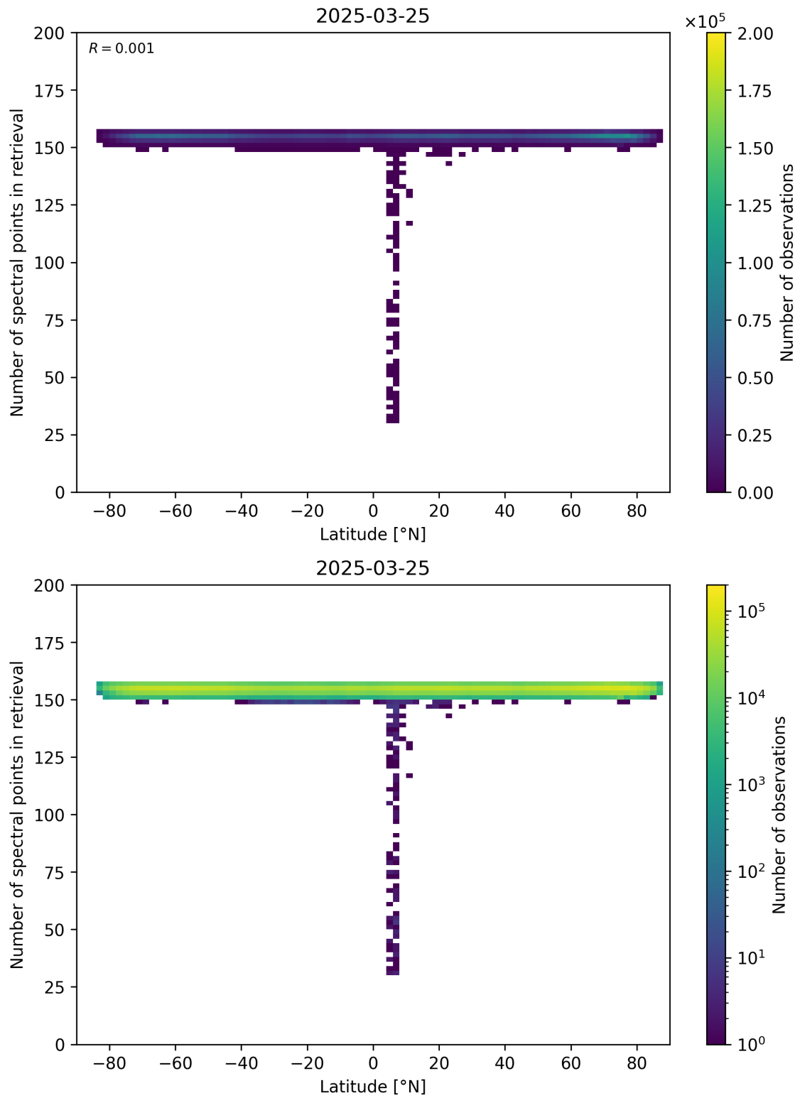
Figure 57: Scatter density plot of “Latitude” against “Number of spectral points in retrieval” for 2025-03-24 to 2025-03-26.
