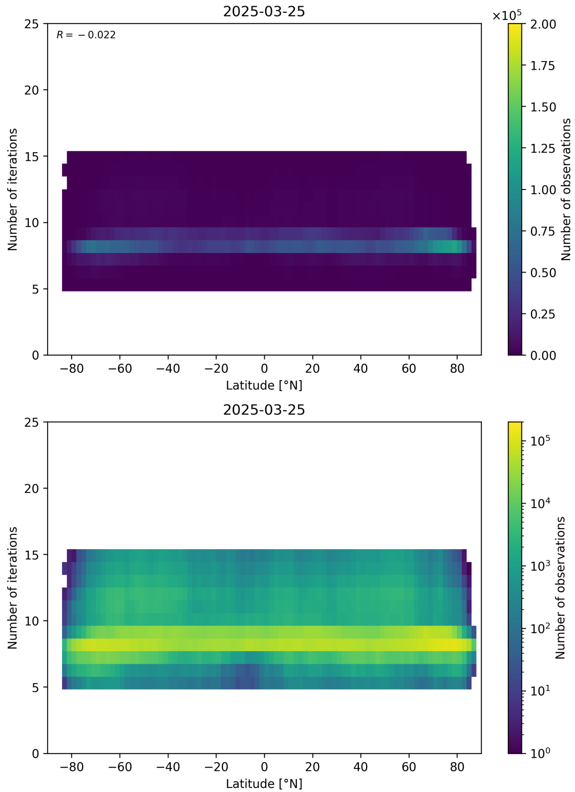
Figure 56: Scatter density plot of “Latitude” against “Number of iterations” for 2025-03-24 to 2025-03-26.
