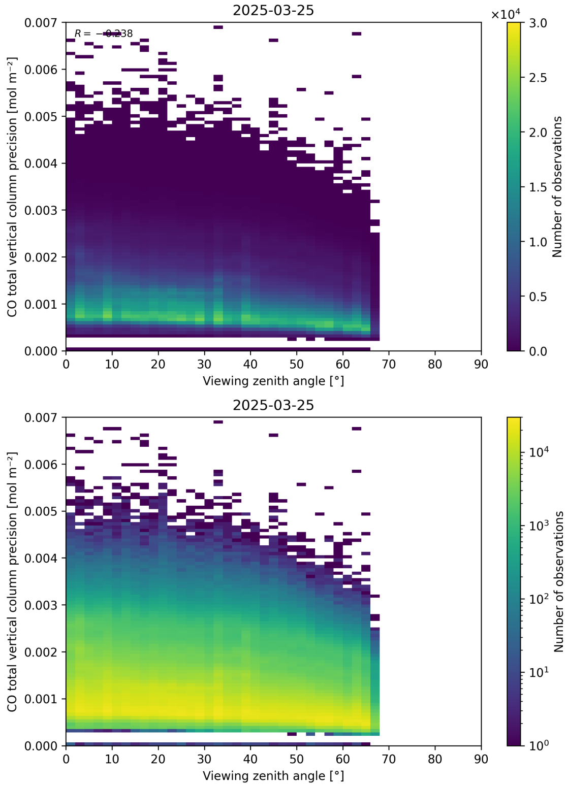
Figure 71: Scatter density plot of “Viewing zenith angle” against “CO total vertical column precision” for 2025-03-24 to 2025-03-26.
