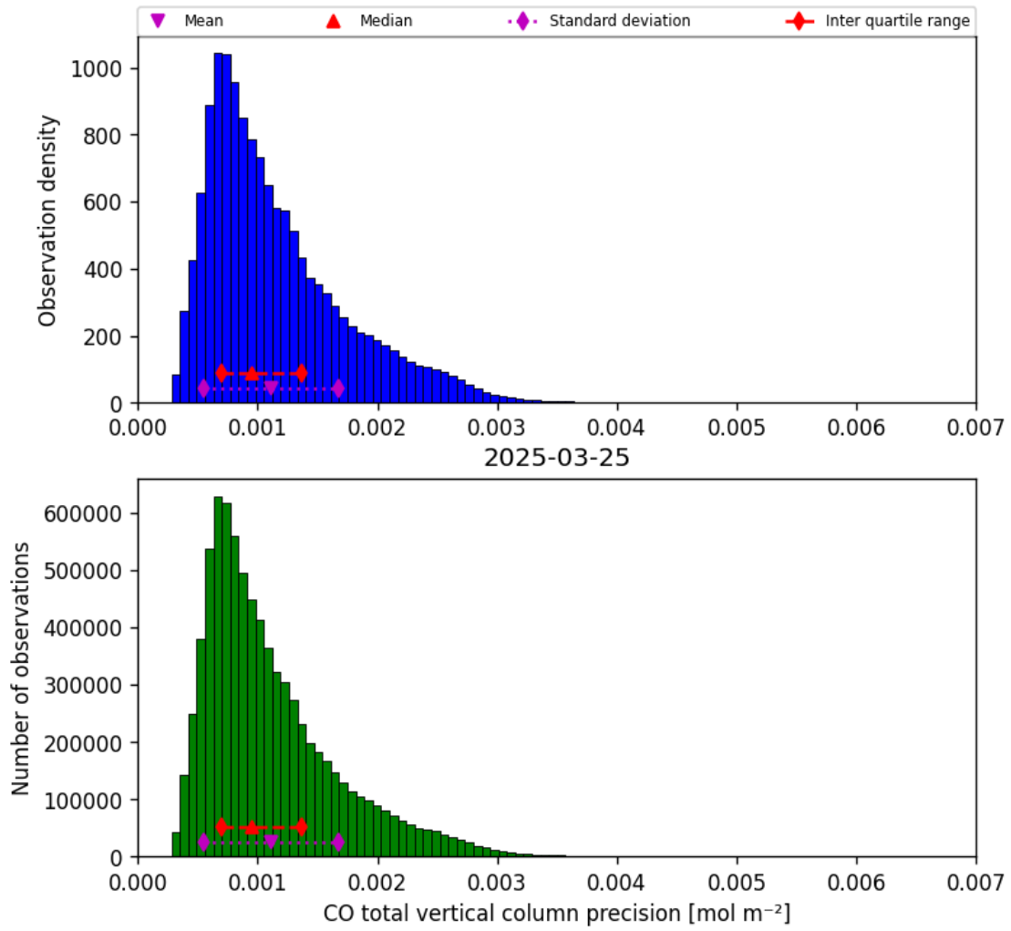
Figure 20: Histogram of “CO total vertical column precision” for 2025-03-24 to 2025-03-26
