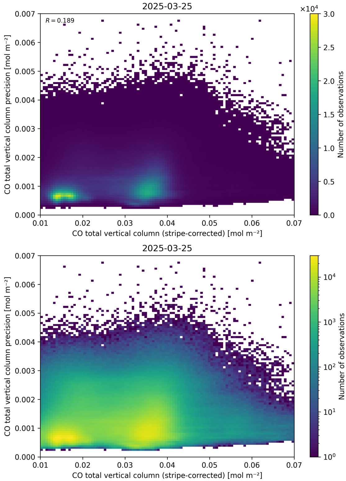
Figure 36: Scatter density plot of “CO total vertical column (stripe-corrected)” against “CO total vertical column precision” for 2025-03-24 to 2025-03-26.
