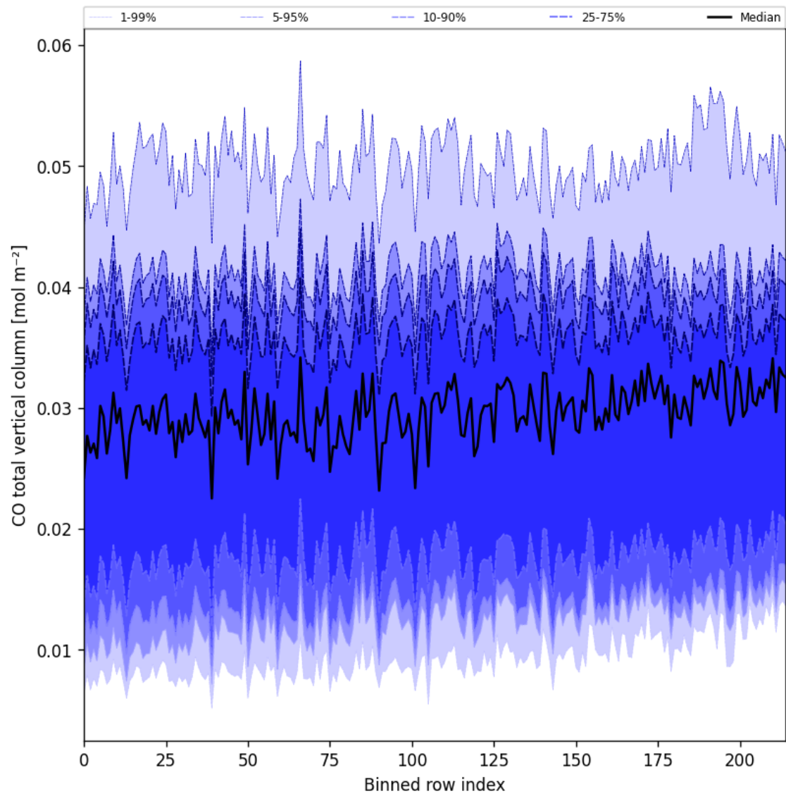
Figure 26: Along track statistics of “CO total vertical column” for 2025-03-24 to 2025-03-26
