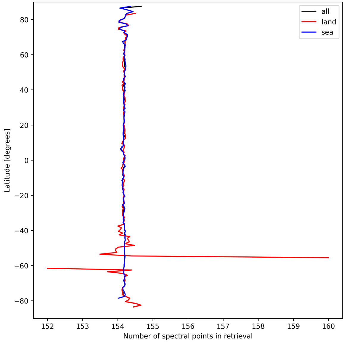
Figure 13: Zonal average of “Number of spectral points in retrieval” for 2025-03-24 to 2025-03-26.
