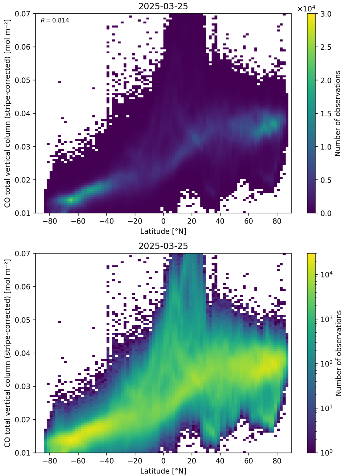
Figure 52: Scatter density plot of “Latitude” against “CO total vertical column (stripe-corrected)” for 2025-03-24 to 2025-03-26.
