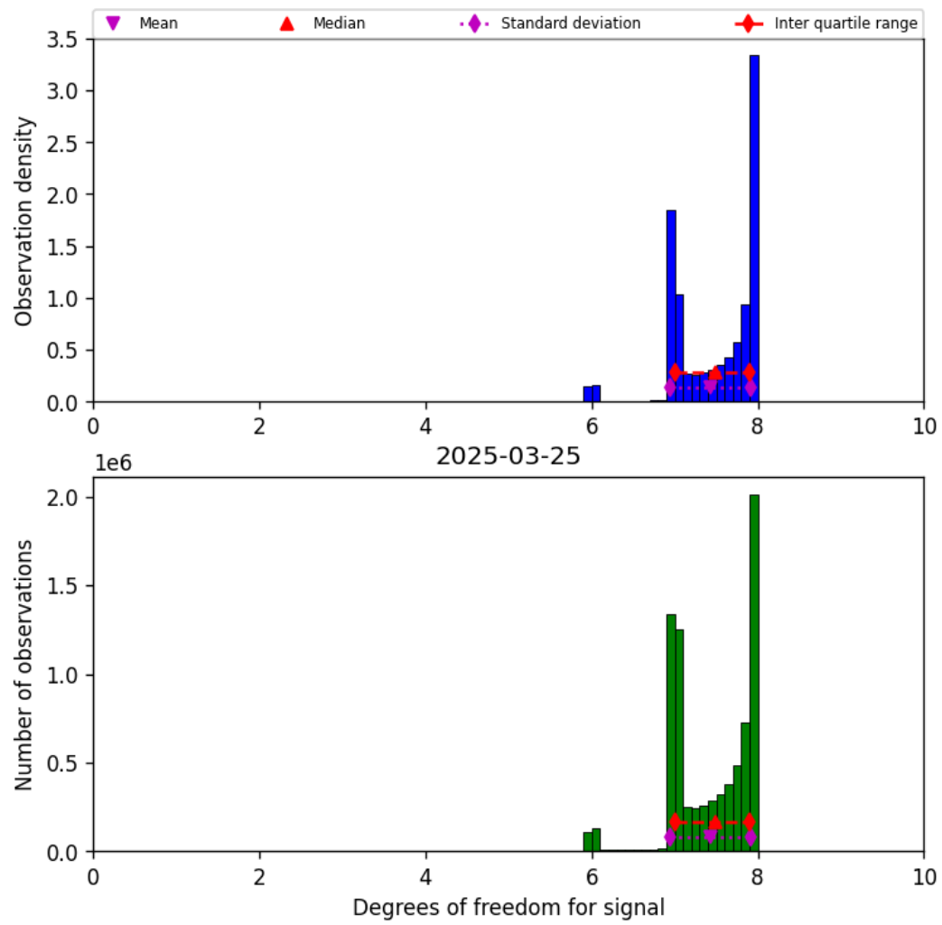
Figure 23: Histogram of “Degrees of freedom for signal” for 2025-03-24 to 2025-03-26
