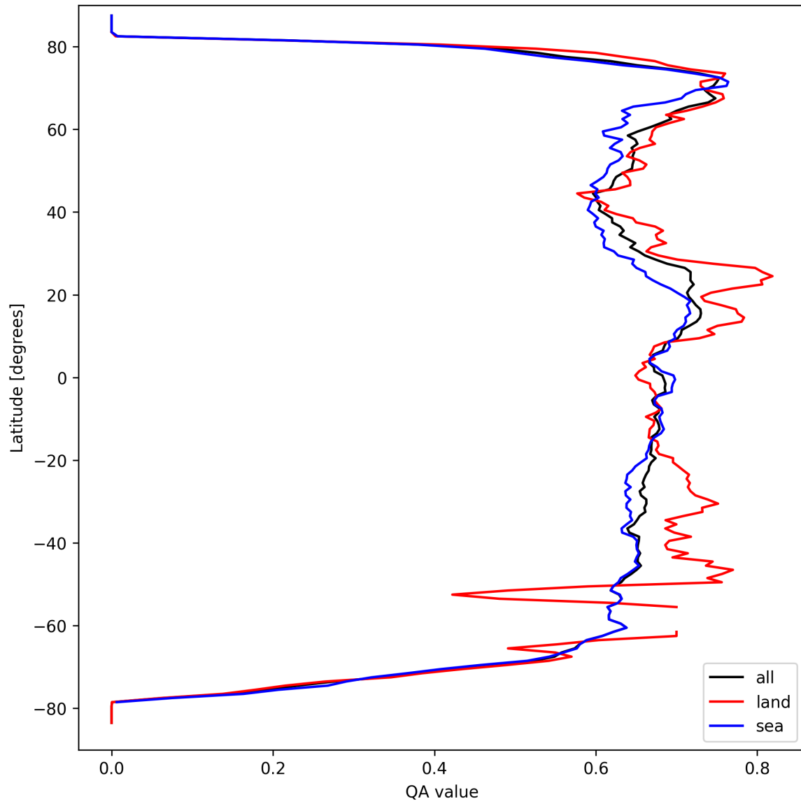
Figure 9: Zonal average of “QA value” for 2025-03-24 to 2025-03-26.
