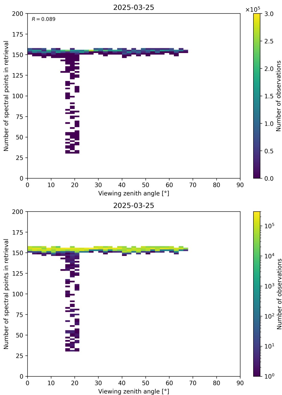
Figure 76: Scatter density plot of “Viewing zenith angle” against “Number of spectral points in retrieval” for 2025-03-24 to 2025-03-26.
