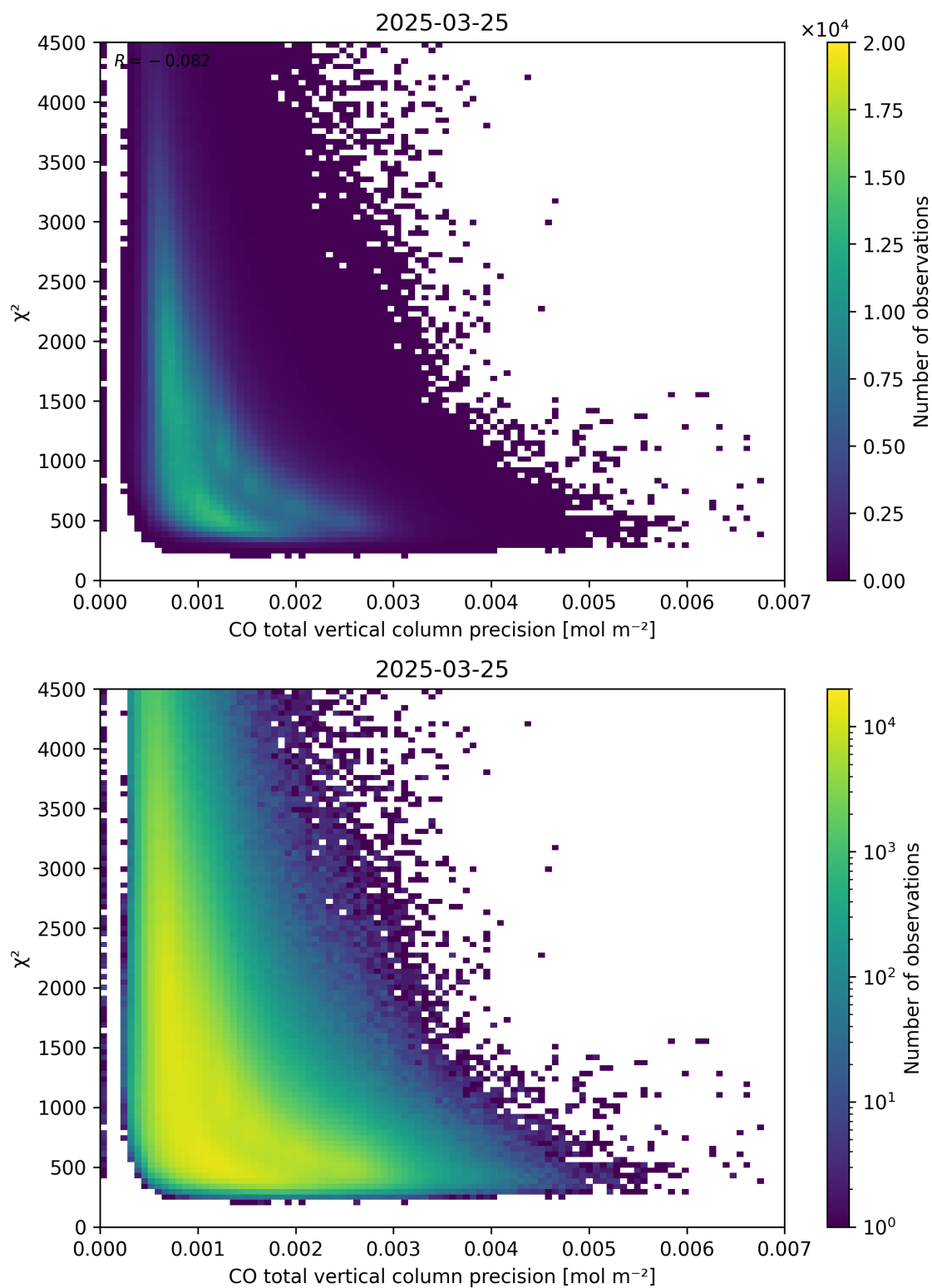
Figure 44: Scatter density plot of “CO total vertical column precision” against “ \chi^2 ” for 2025-03-24 to 2025-03-26.
