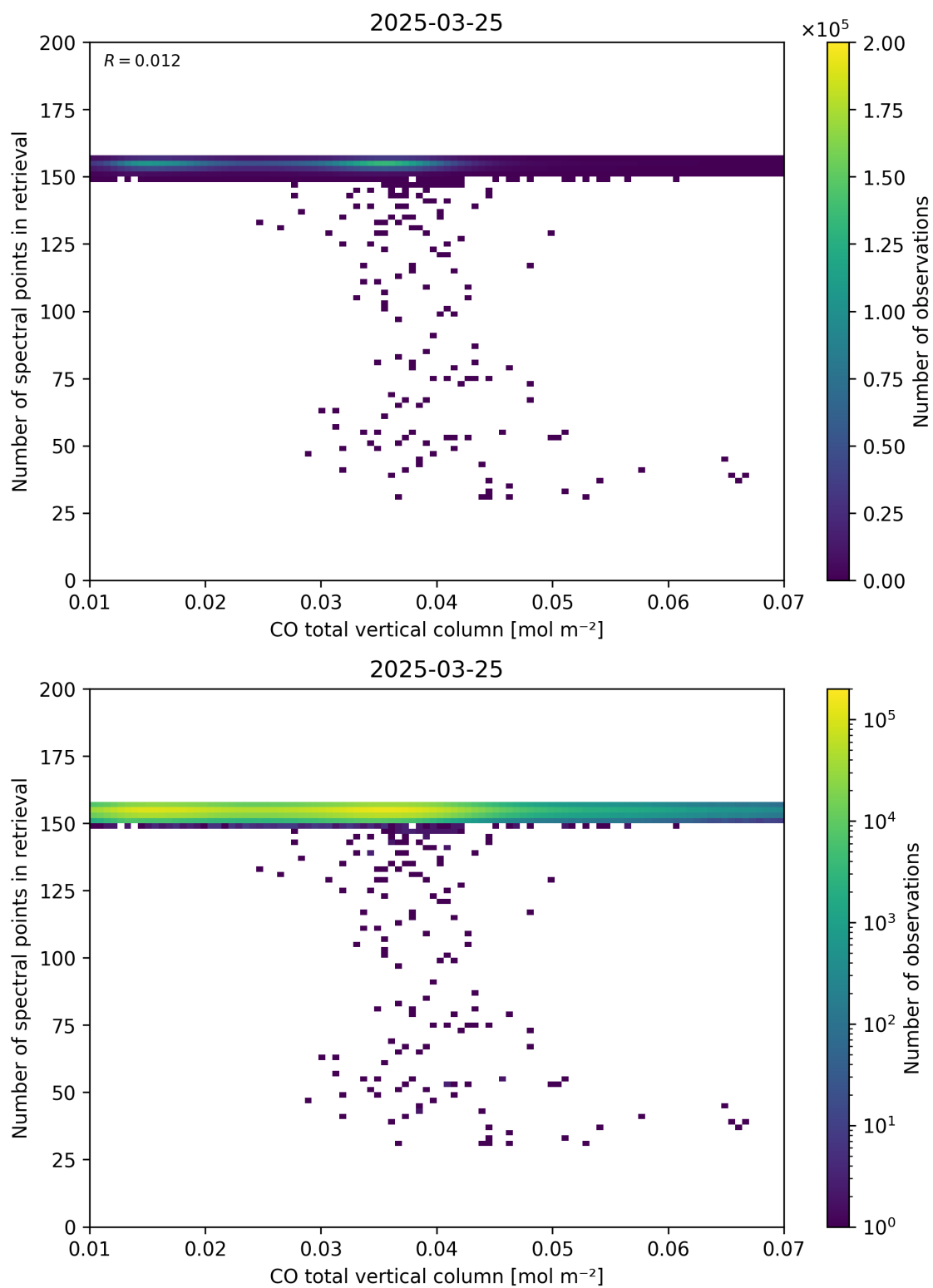
Figure 43: Scatter density plot of “CO total vertical column” against “Number of spectral points in retrieval” for 2025-03-24 to 2025-03-26.
