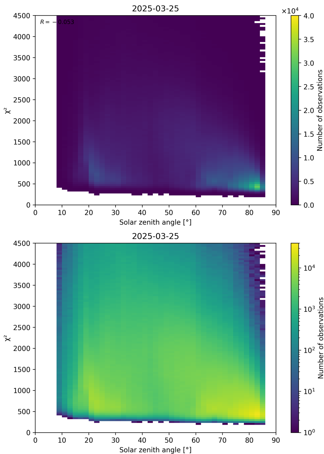
Figure 64: Scatter density plot of “Solar zenith angle” against “ \chi^2 ” for 2025-03-24 to 2025-03-26.
