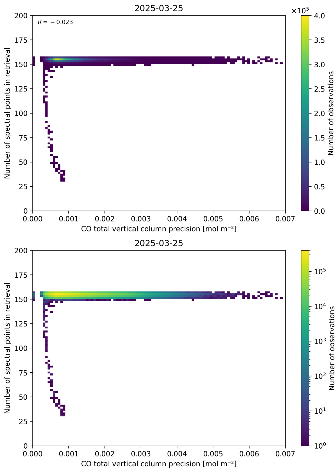
Figure 47: Scatter density plot of “CO total vertical column precision” against “Number of spectral points in retrieval” for 2025-03-24 to 2025-03-26.
