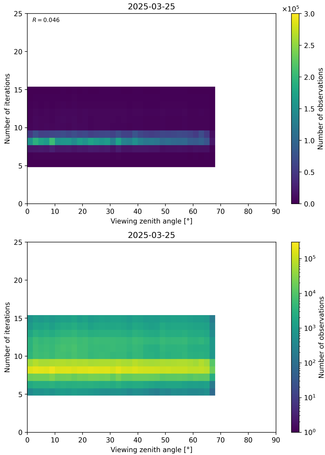
Figure 75: Scatter density plot of “Viewing zenith angle” against “Number of iterations” for 2025-03-24 to 2025-03-26.
