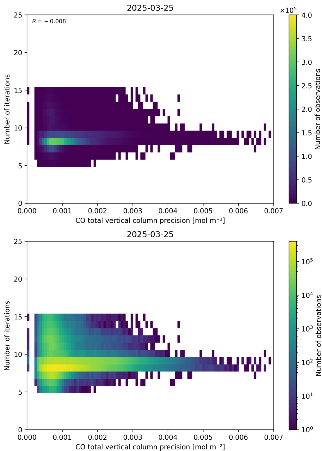
Figure 46: Scatter density plot of “CO total vertical column precision” against “Number of iterations” for 2025-03-24 to 2025-03-26.
