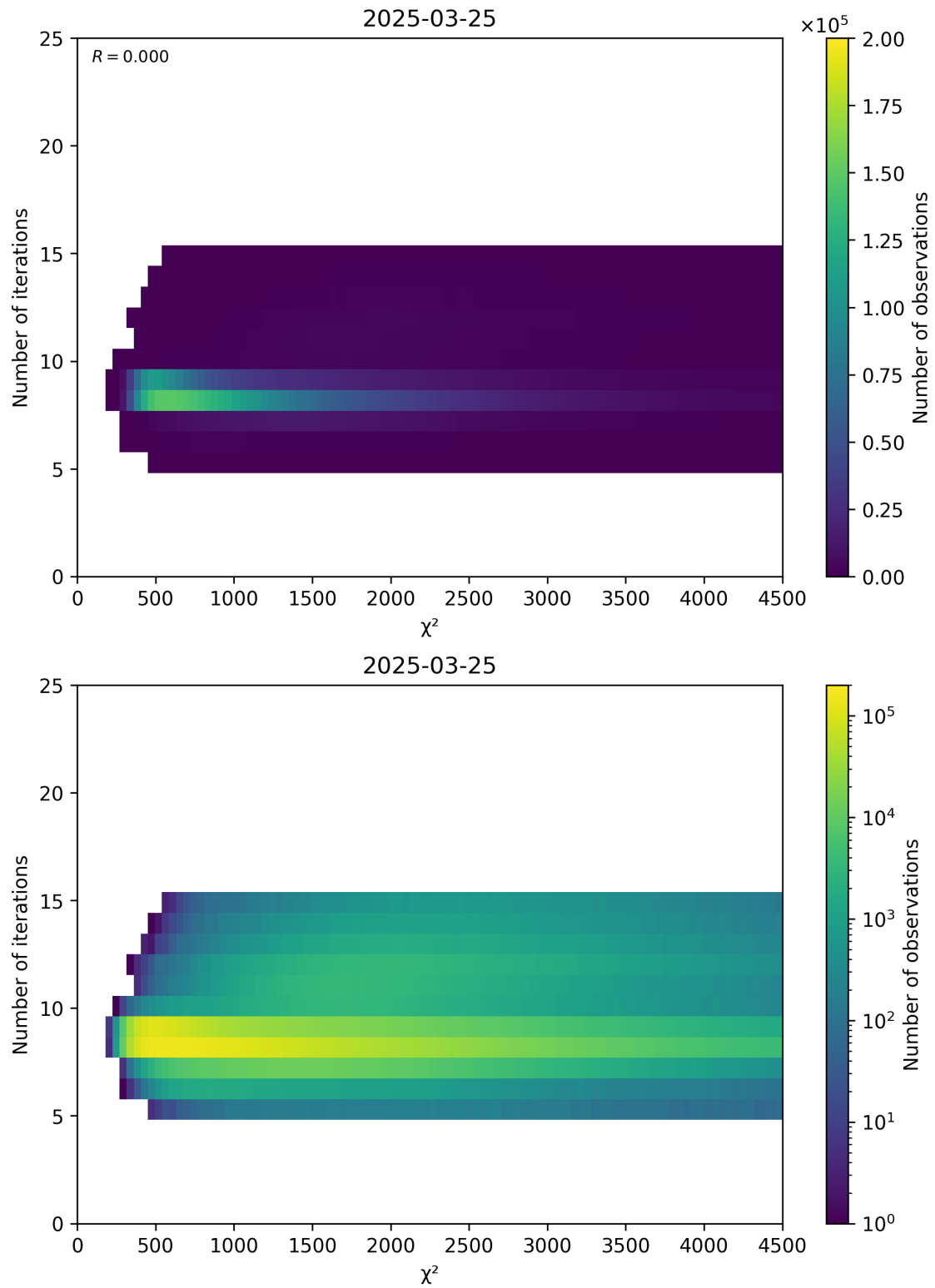
Figure 49: Scatter density plot of “ \chi^2 ” against “Number of iterations” for 2025-03-24 to 2025-03-26.
