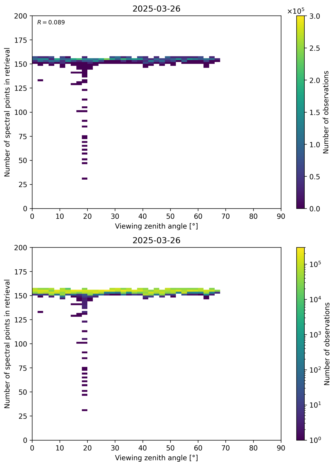
Figure 76: Scatter density plot of “Viewing zenith angle” against “Number of spectral points in retrieval” for 2025-03-25 to 2025-03-27.
