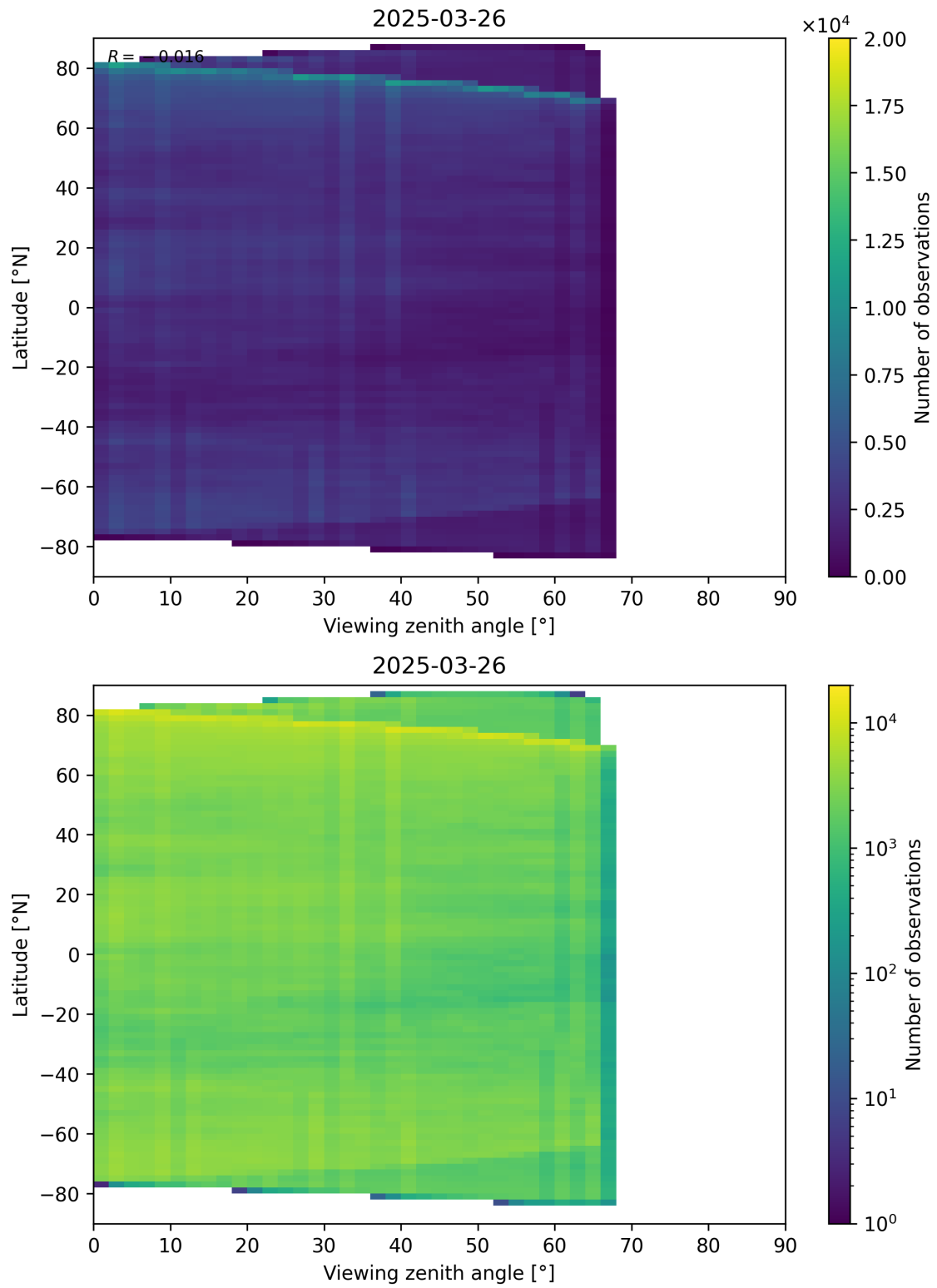
Figure 74: Scatter density plot of “Viewing zenith angle” against “Latitude” for 2025-03-25 to 2025-03-27.
