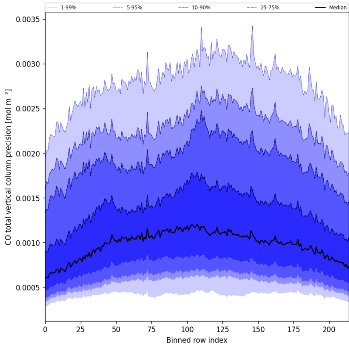
Figure 28: Along track statistics of “CO total vertical column precision” for 2025-03-25 to 2025-03-27
