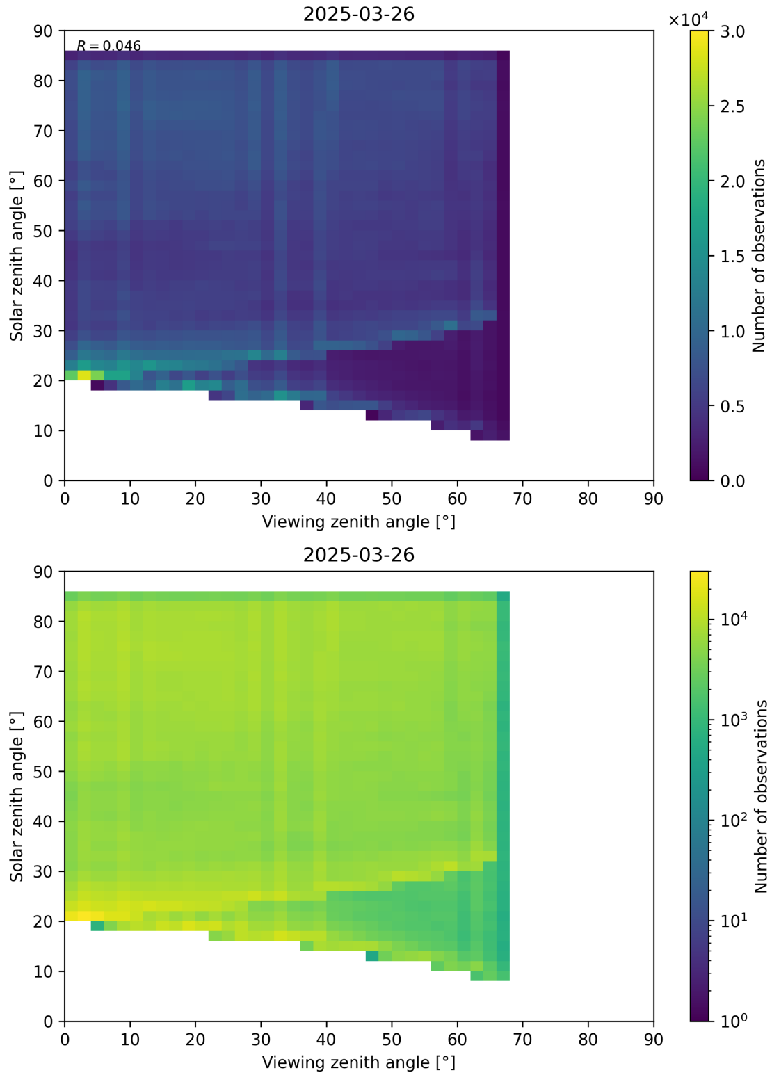
Figure 77: Scatter density plot of “Viewing zenith angle” against “Solar zenith angle” for 2025-03-25 to 2025-03-27.
