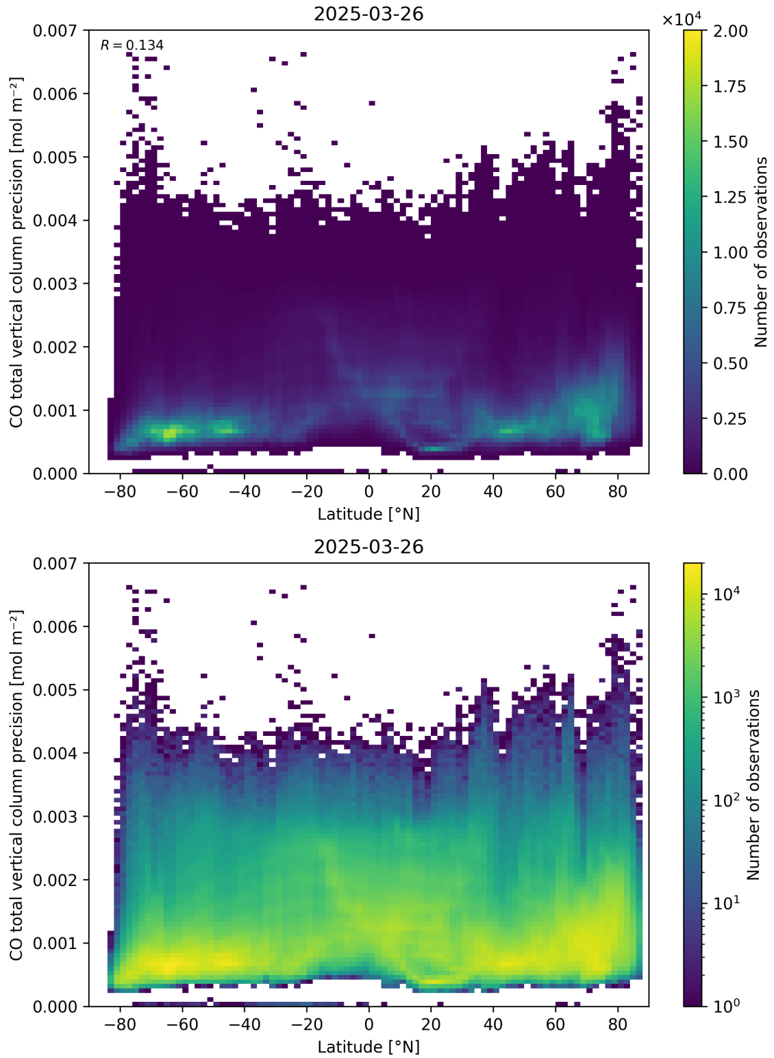
Figure 53: Scatter density plot of “Latitude” against “CO total vertical column precision” for 2025-03-25 to 2025-03-27.
