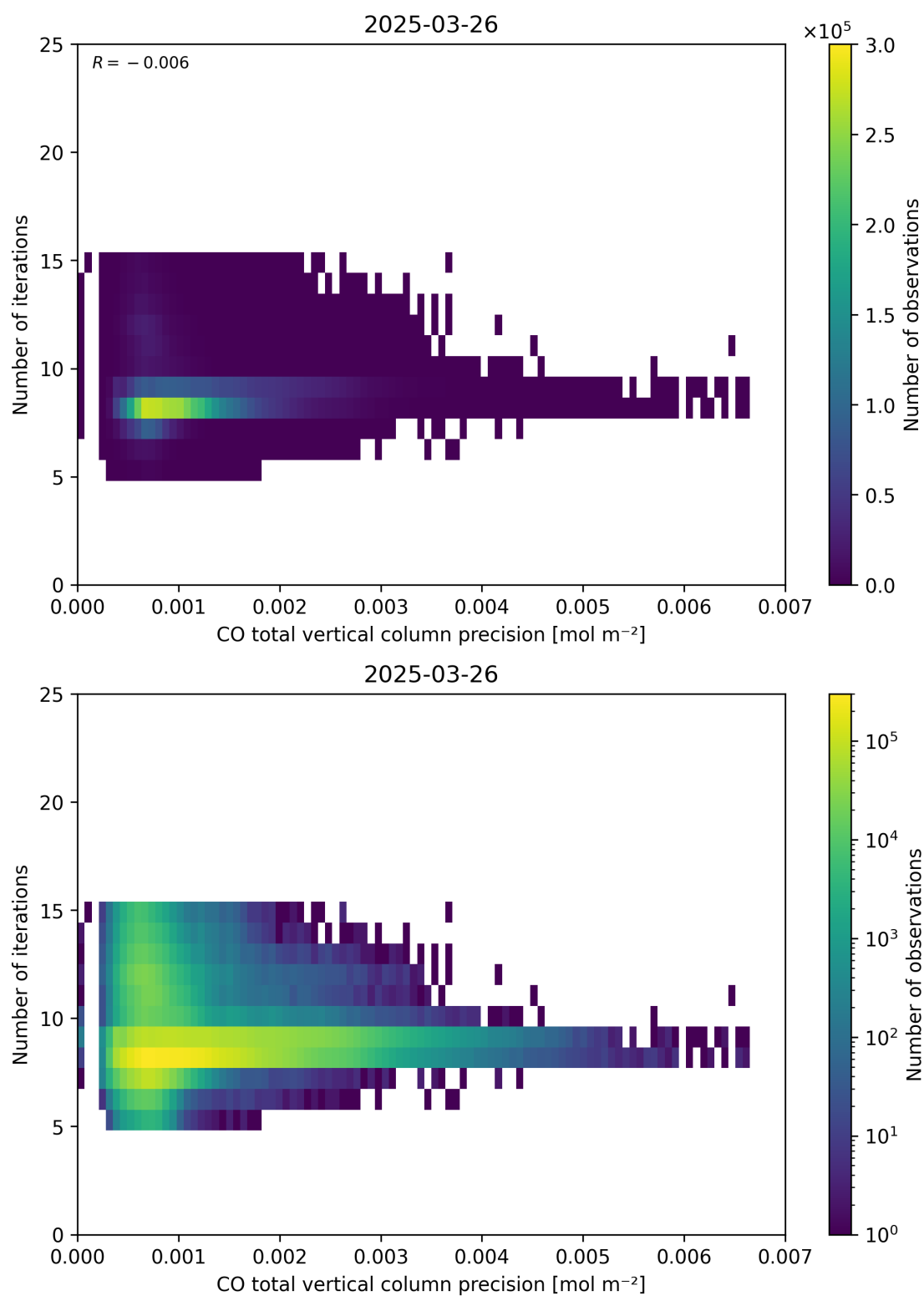
Figure 46: Scatter density plot of “CO total vertical column precision” against “Number of iterations” for 2025-03-25 to 2025-03-27.
