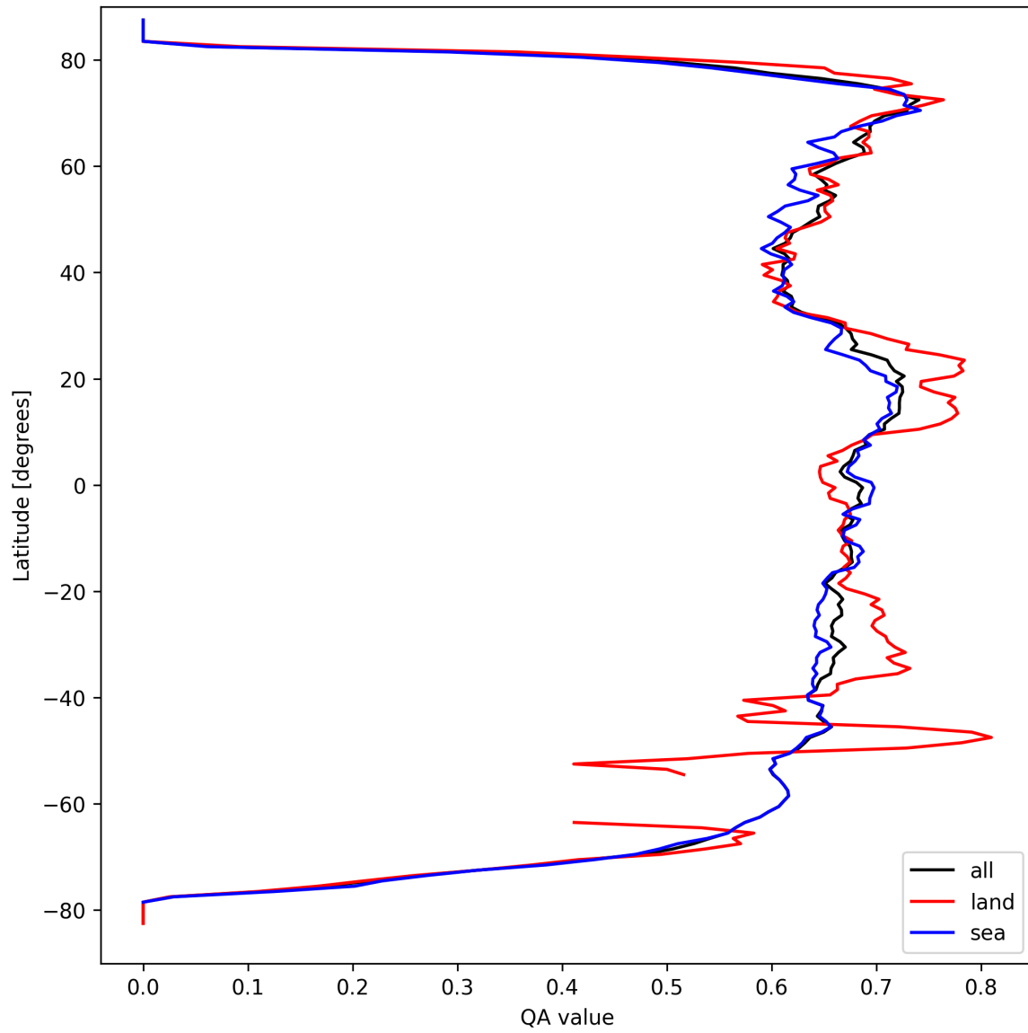
Figure 9: Zonal average of “QA value” for 2025-03-25 to 2025-03-27.
