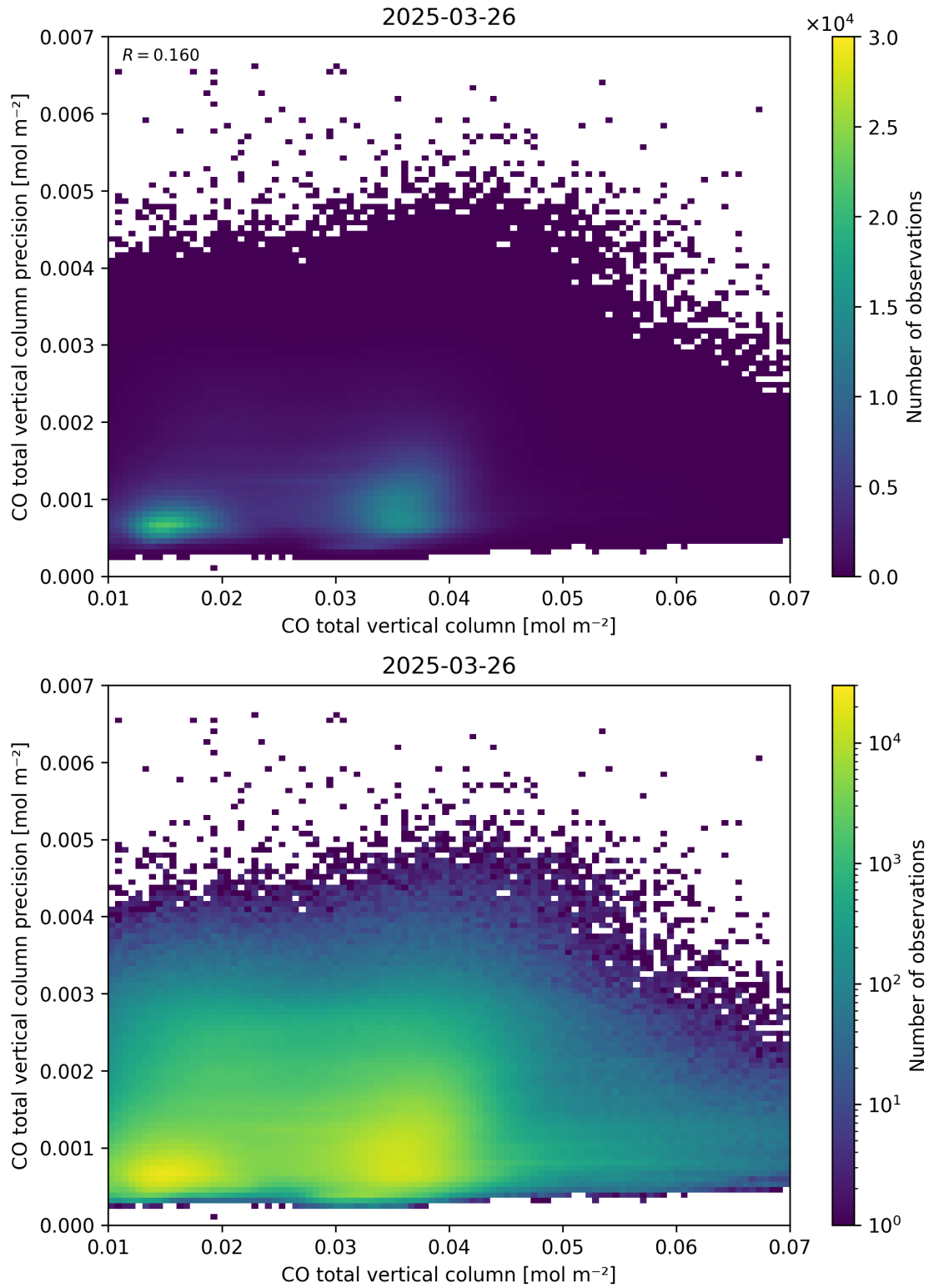
Figure 34: Scatter density plot of “CO total vertical column” against “CO total vertical column precision” for 2025-03-25 to 2025-03-27.
