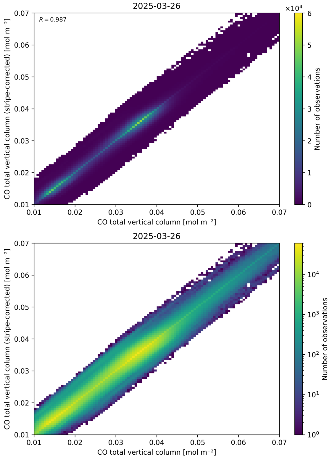
Figure 33: Scatter density plot of “CO total vertical column” against “CO total vertical column (stripe-corrected)” for 2025-03-25 to 2025-03-27.
