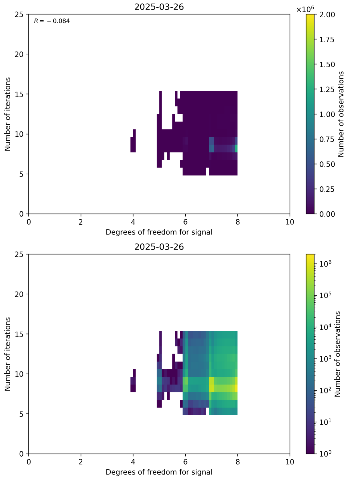
Figure 50: Scatter density plot of “Degrees of freedom for signal” against “Number of iterations” for 2025-03-25 to 2025-03-27.
