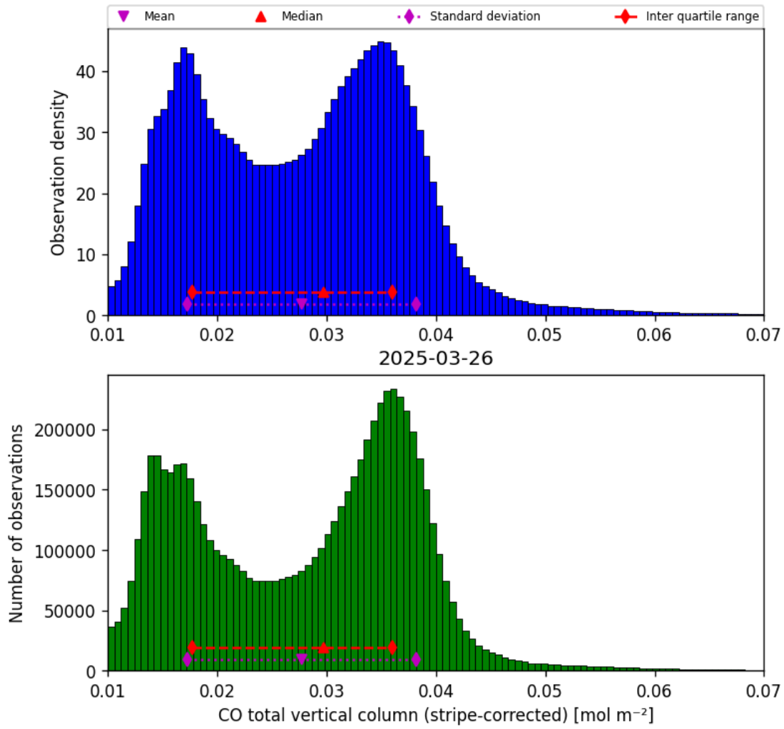
Figure 19: Histogram of “CO total vertical column (stripe-corrected)” for 2025-03-25 to 2025-03-27
