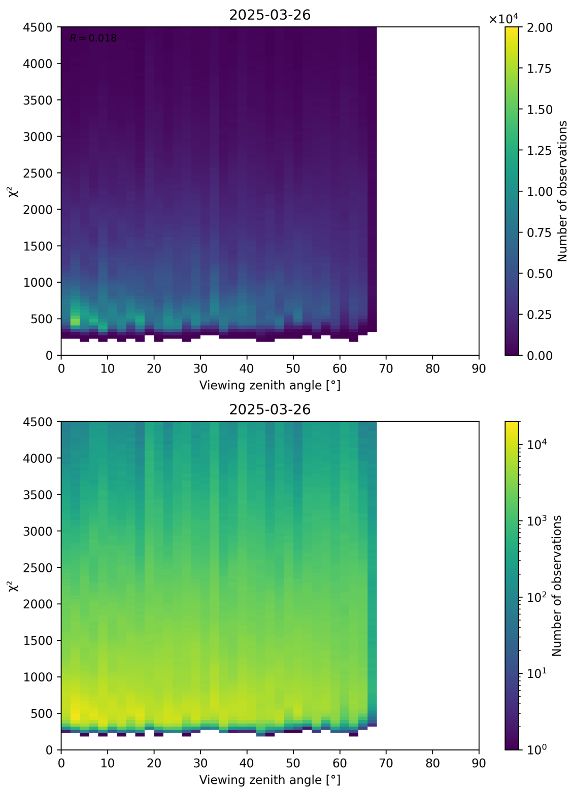
Figure 72: Scatter density plot of “Viewing zenith angle” against “ \chi^2 ” for 2025-03-25 to 2025-03-27.
