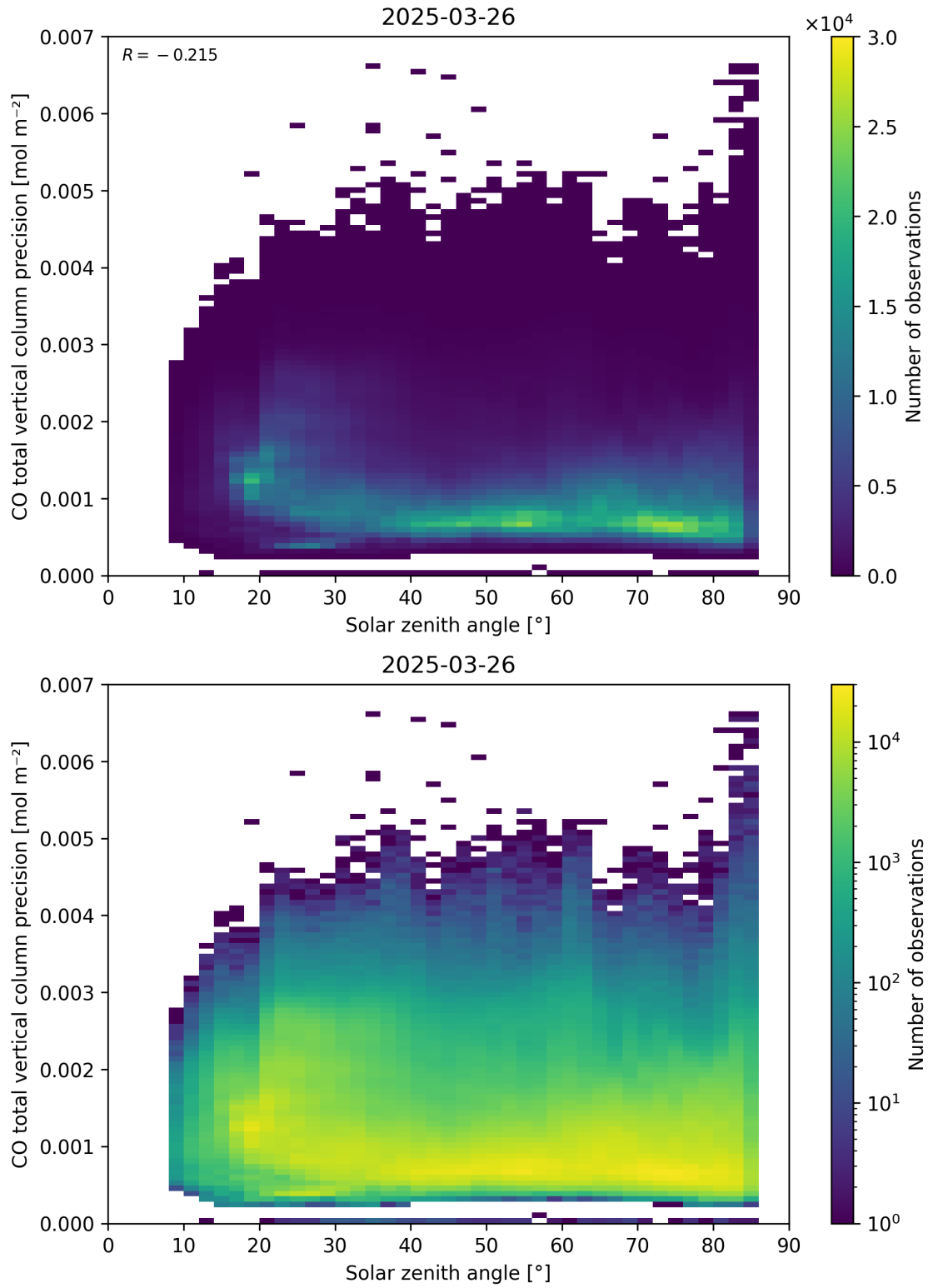
Figure 63: Scatter density plot of “Solar zenith angle” against “CO total vertical column precision” for 2025-03-25 to 2025-03-27.
