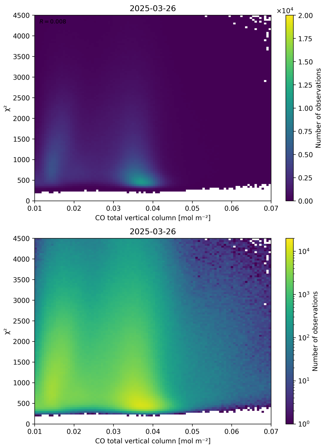
Figure 35: Scatter density plot of “CO total vertical column” against “ \chi^2 ” for 2025-03-25 to 2025-03-27.
