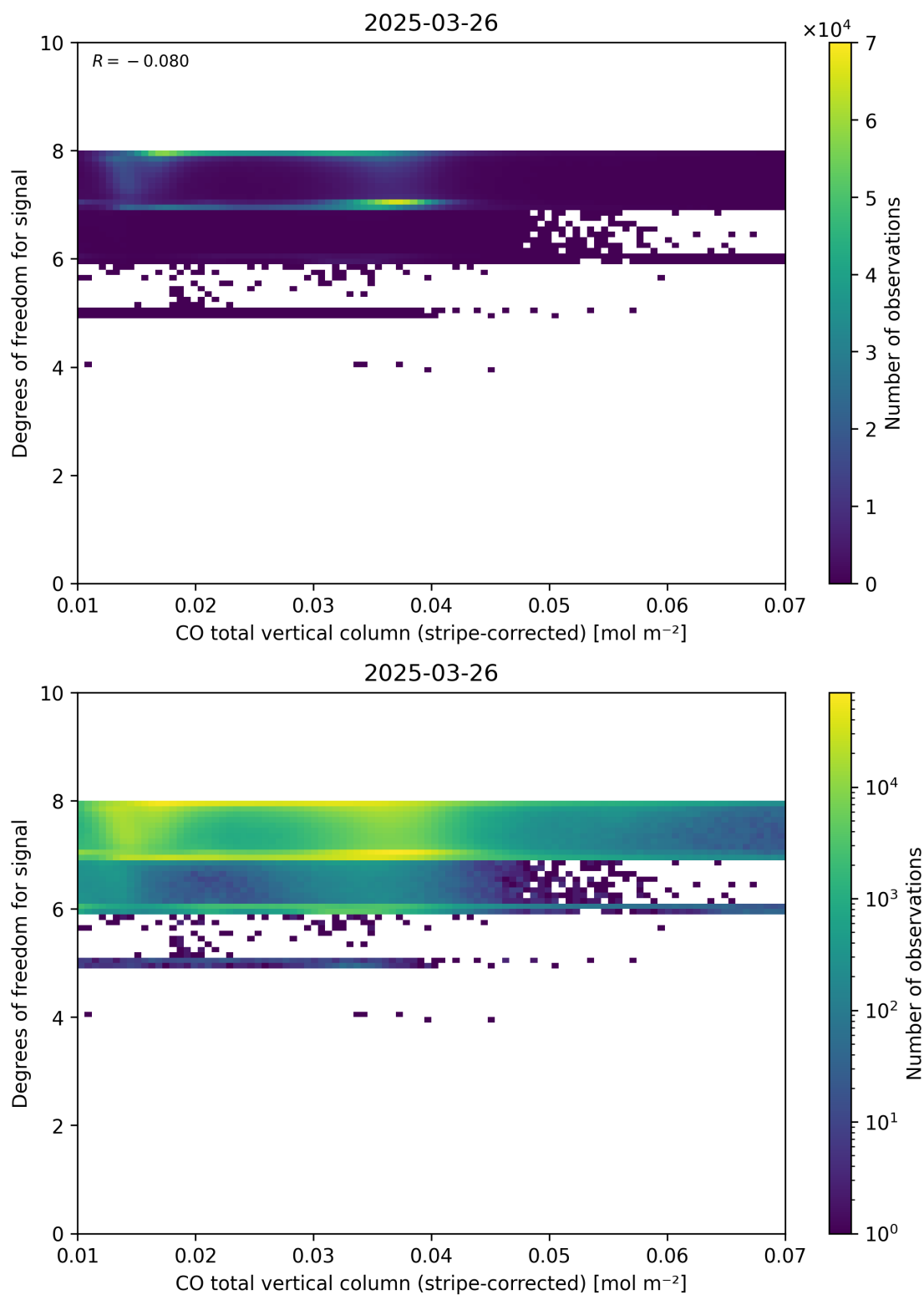
Figure 38: Scatter density plot of “CO total vertical column (stripe-corrected)” against “Degrees of freedom for signal” for 2025-03-25 to 2025-03-27.
