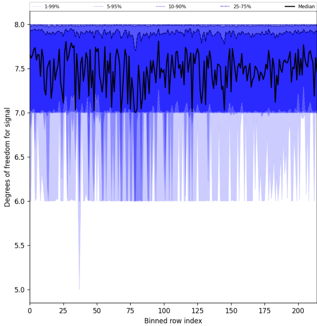
Figure 31: Along track statistics of “Degrees of freedom for signal” for 2025-03-25 to 2025-03-27
