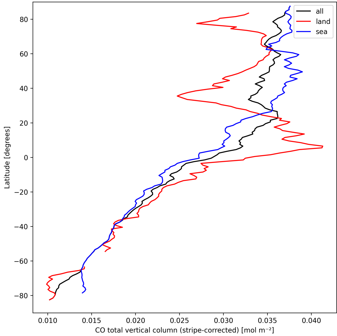
Figure 11: Zonal average of “CO total vertical column (stripe-corrected)” for 2025-03-25 to 2025-03-27.
