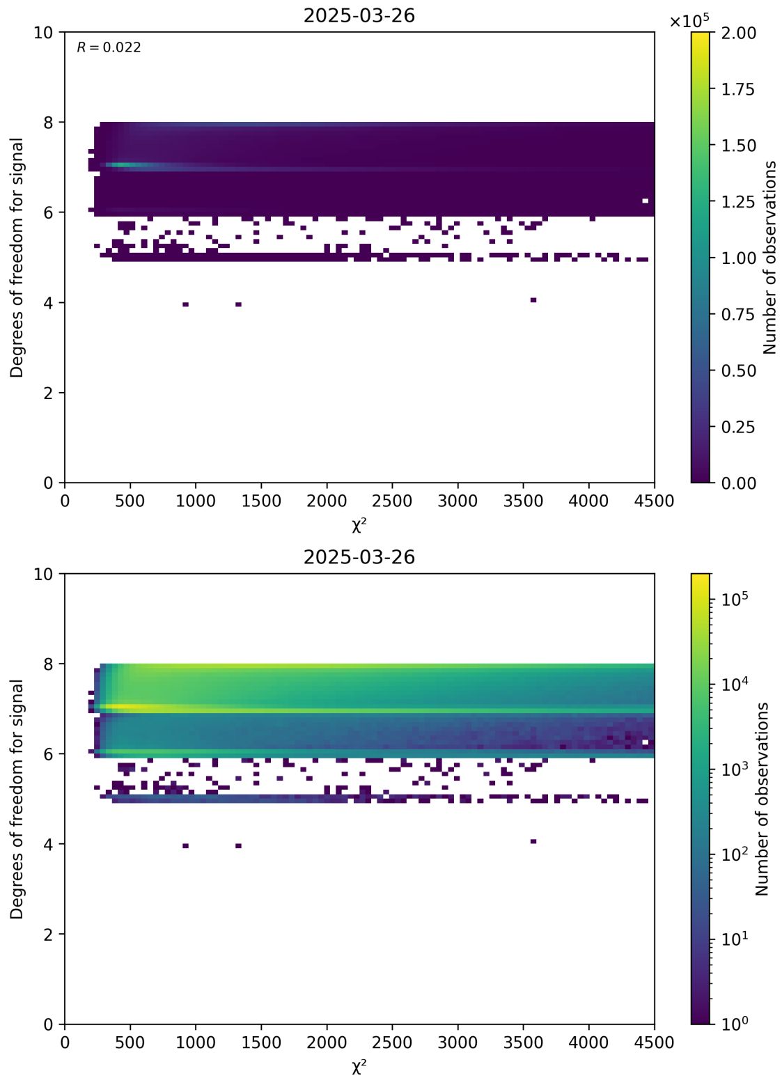
Figure 48: Scatter density plot of “ \chi^2 ” against “Degrees of freedom for signal” for 2025-03-25 to 2025-03-27.
