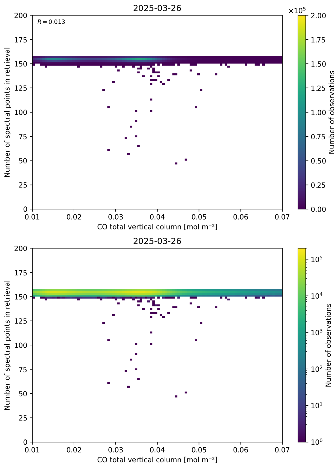
Figure 43: Scatter density plot of “CO total vertical column” against “Number of spectral points in retrieval” for 2025-03-25 to 2025-03-27.
