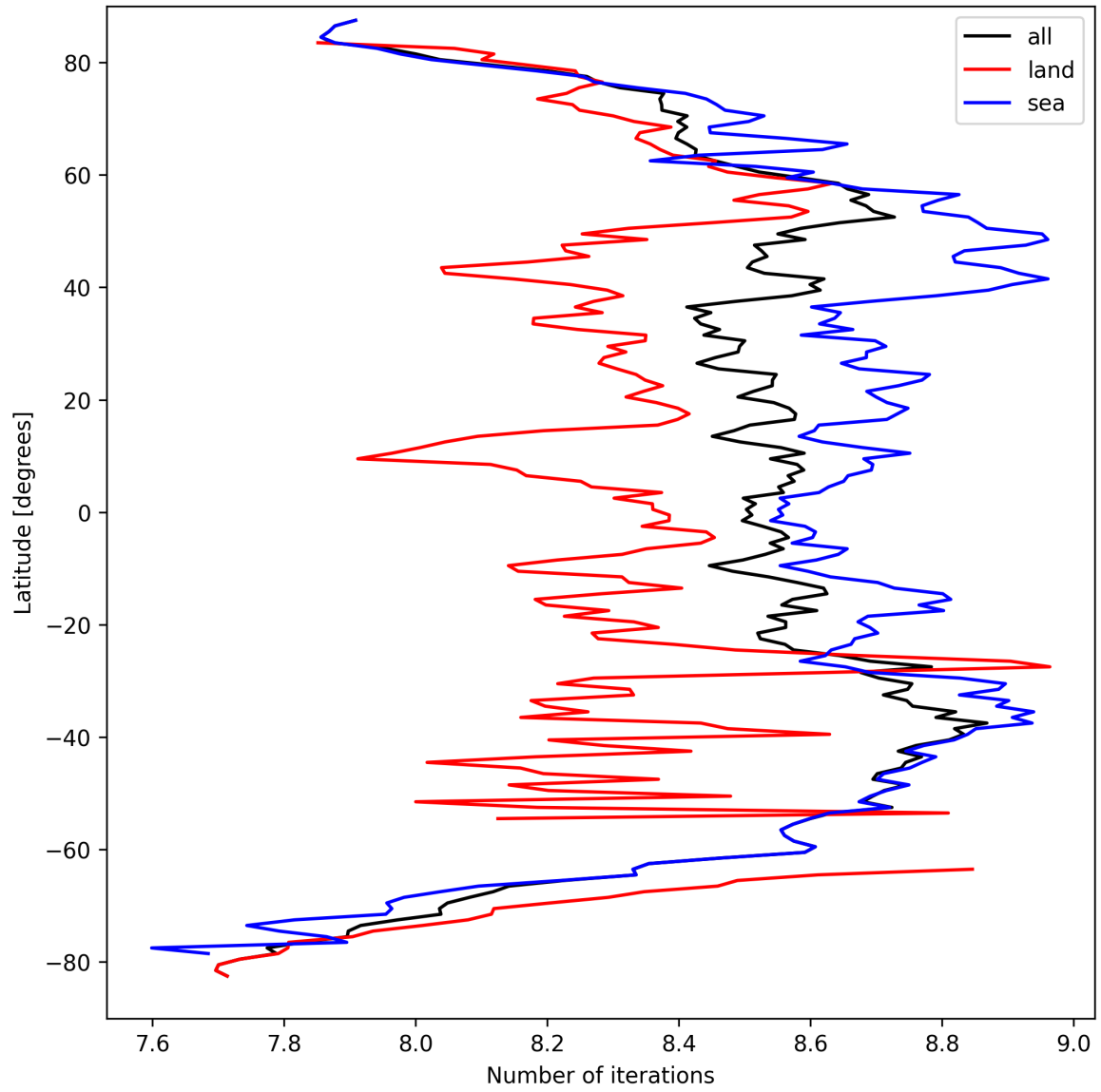
Figure 16: Zonal average of “Number of iterations” for 2025-03-25 to 2025-03-27.
