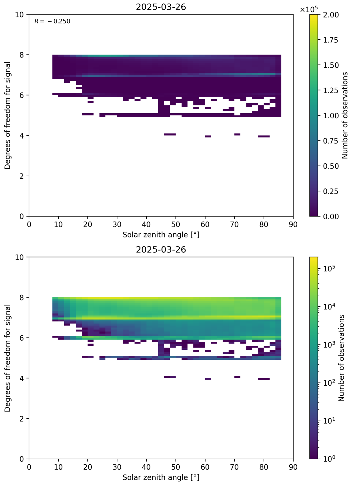
Figure 65: Scatter density plot of “Solar zenith angle” against “Degrees of freedom for signal” for 2025-03-25 to 2025-03-27.
