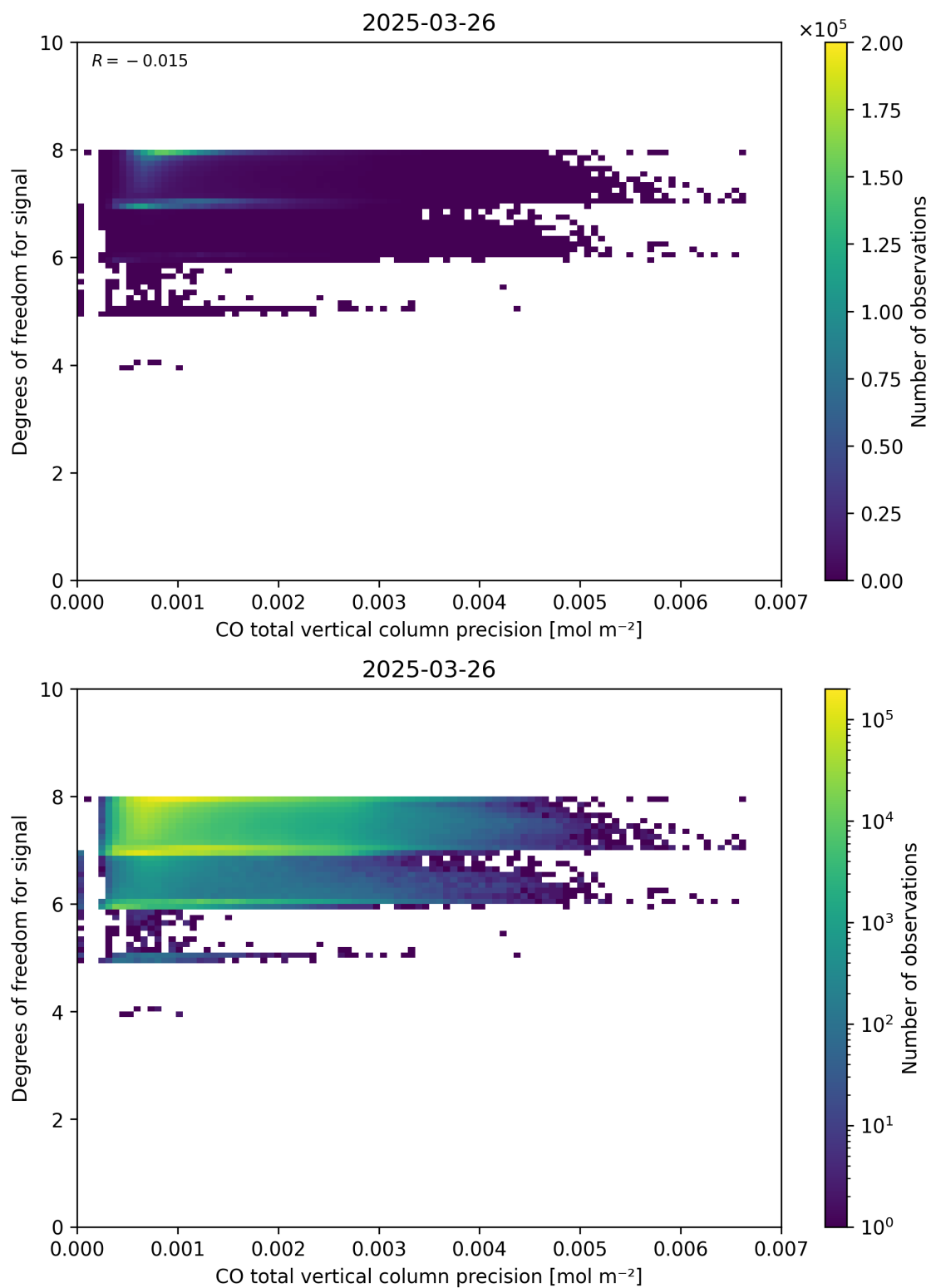
Figure 45: Scatter density plot of “CO total vertical column precision” against “Degrees of freedom for signal” for 2025-03-25 to 2025-03-27.
