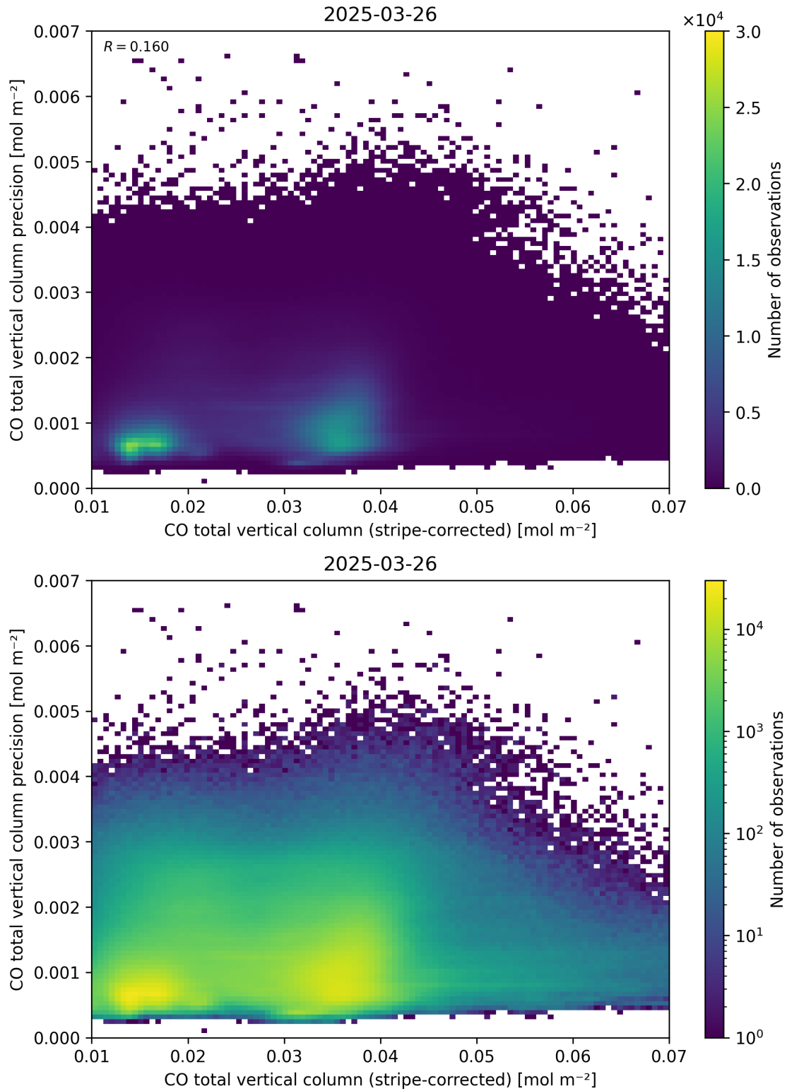
Figure 36: Scatter density plot of “CO total vertical column (stripe-corrected)” against “CO total vertical column precision” for 2025-03-25 to 2025-03-27.
