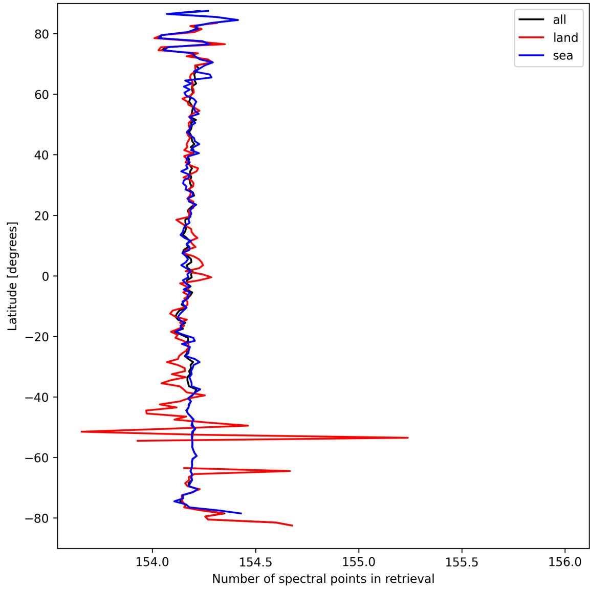
Figure 13: Zonal average of “Number of spectral points in retrieval” for 2025-03-25 to 2025-03-27.
