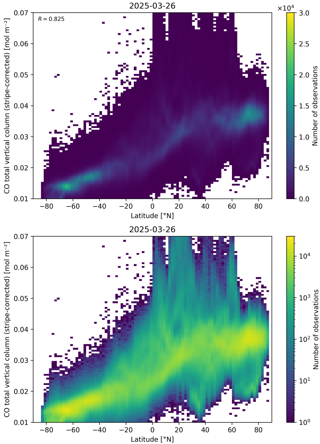
Figure 52: Scatter density plot of “Latitude” against “CO total vertical column (stripe-corrected)” for 2025-03-25 to 2025-03-27.
