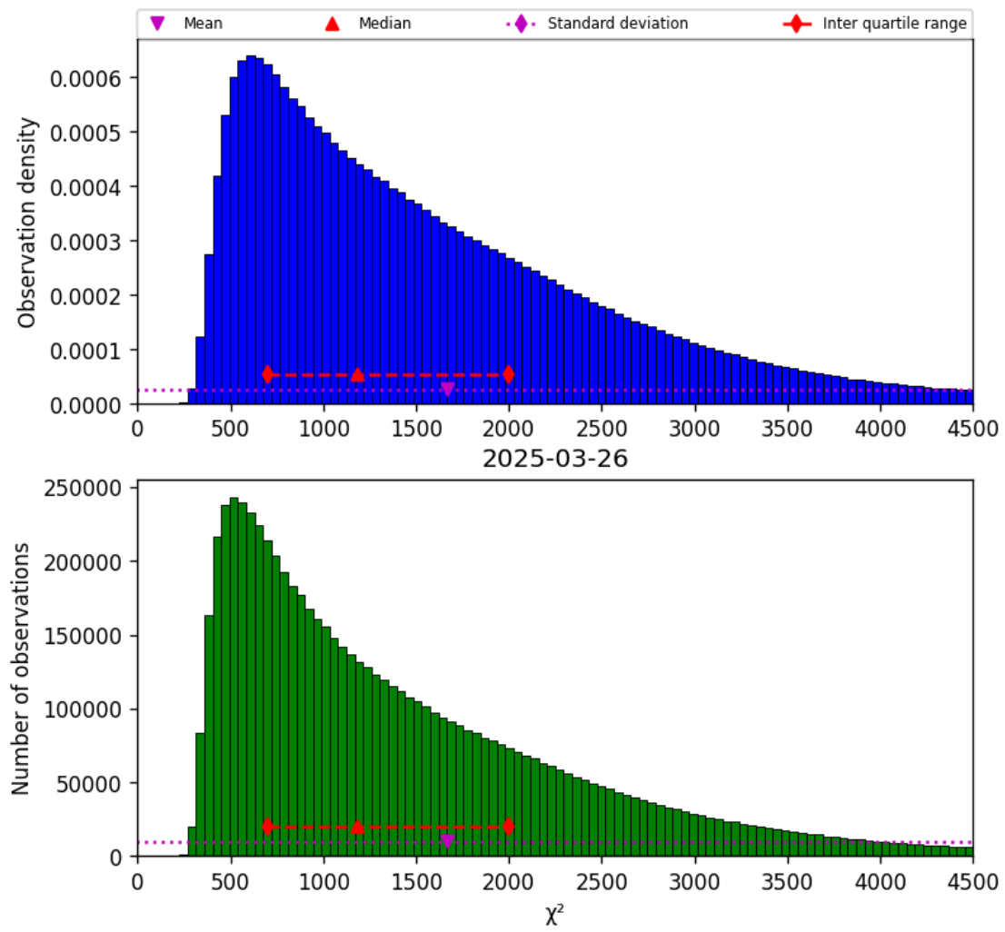
Figure 22: Histogram of “ \chi^2 ” for 2025-03-25 to 2025-03-27
