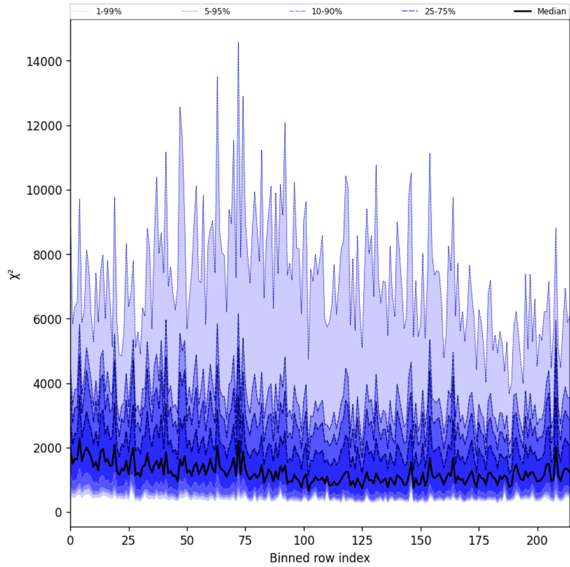
Figure 30: Along track statistics of “ \chi^2 ” for 2025-03-25 to 2025-03-27
