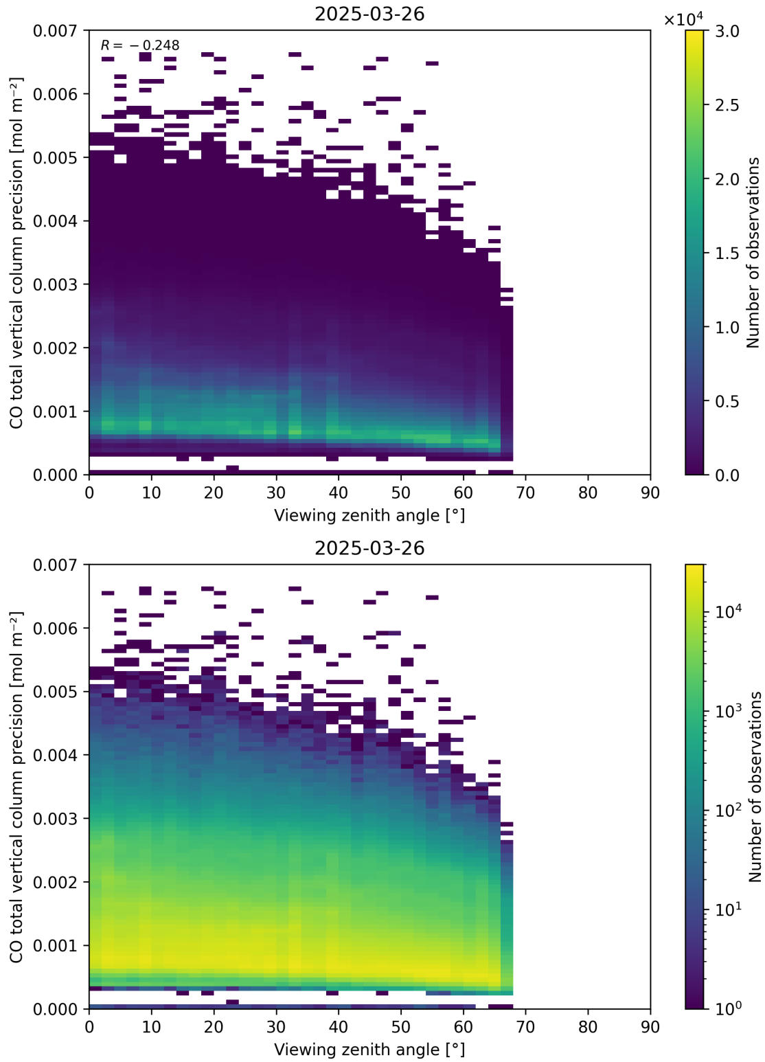
Figure 71: Scatter density plot of “Viewing zenith angle” against “CO total vertical column precision” for 2025-03-25 to 2025-03-27.
