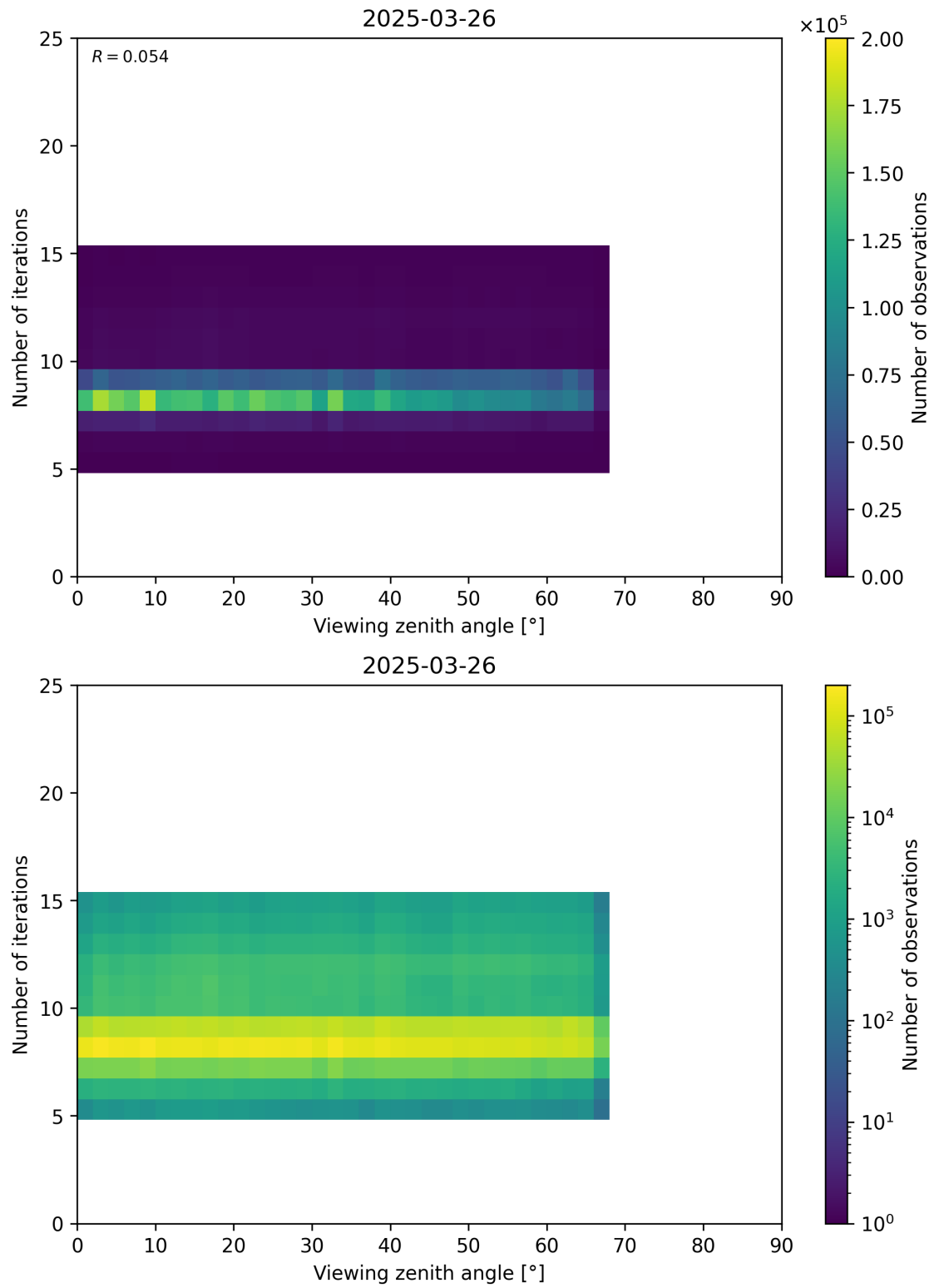
Figure 75: Scatter density plot of “Viewing zenith angle” against “Number of iterations” for 2025-03-25 to 2025-03-27.
