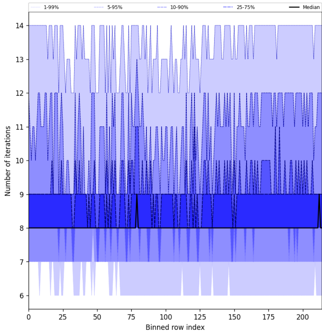
Figure 32: Along track statistics of “Number of iterations” for 2025-03-25 to 2025-03-27
