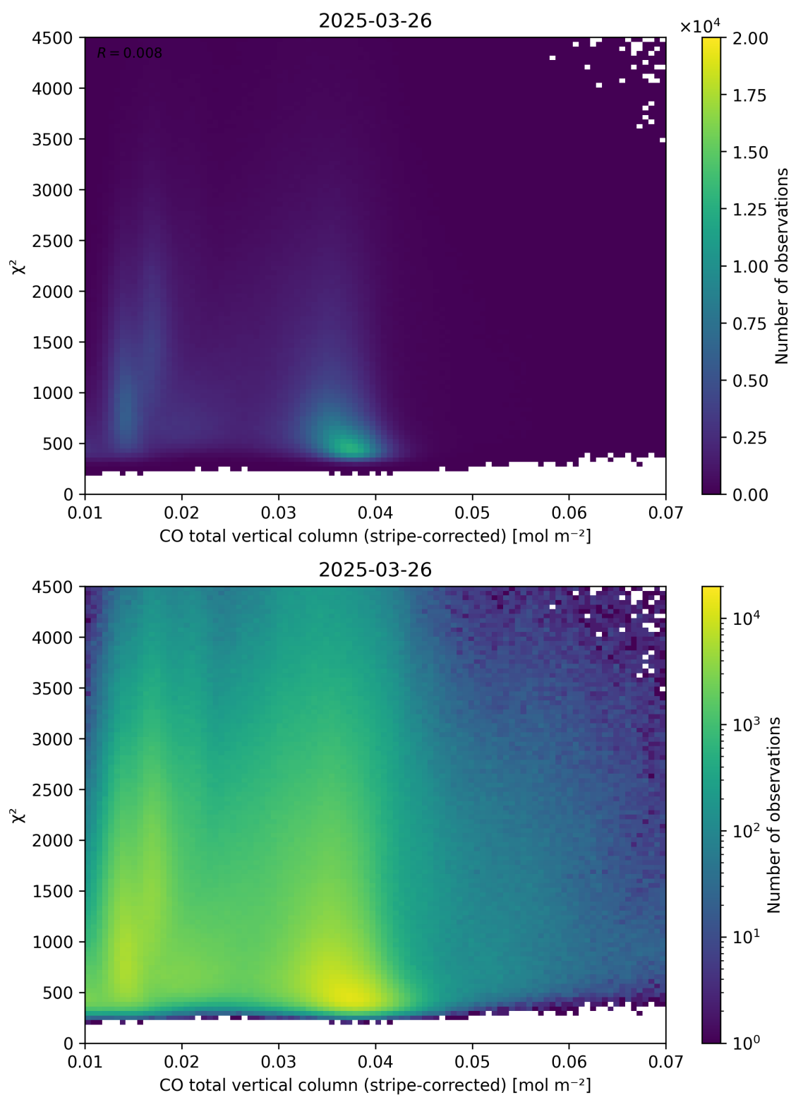
Figure 37: Scatter density plot of “CO total vertical column (stripe-corrected)” against “ \chi^2 ” for 2025-03-25 to 2025-03-27.
