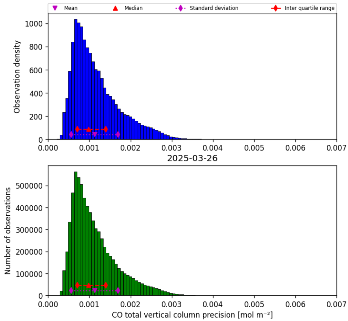
Figure 20: Histogram of “CO total vertical column precision” for 2025-03-25 to 2025-03-27
