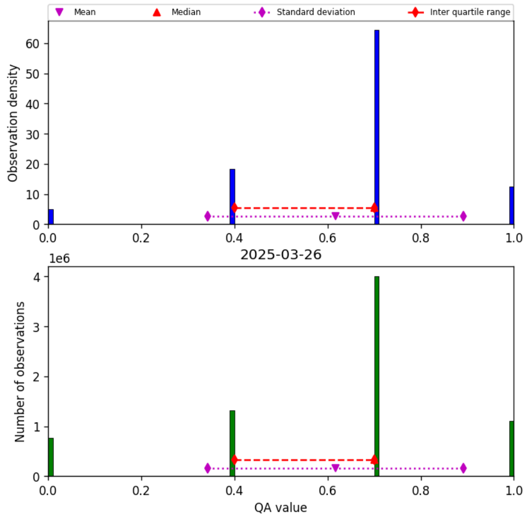
Figure 17: Histogram of “QA value” for 2025-03-25 to 2025-03-27
