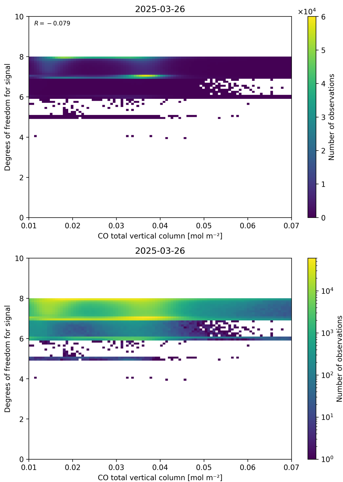
Figure 41: Scatter density plot of “CO total vertical column” against “Degrees of freedom for signal” for 2025-03-25 to 2025-03-27.
