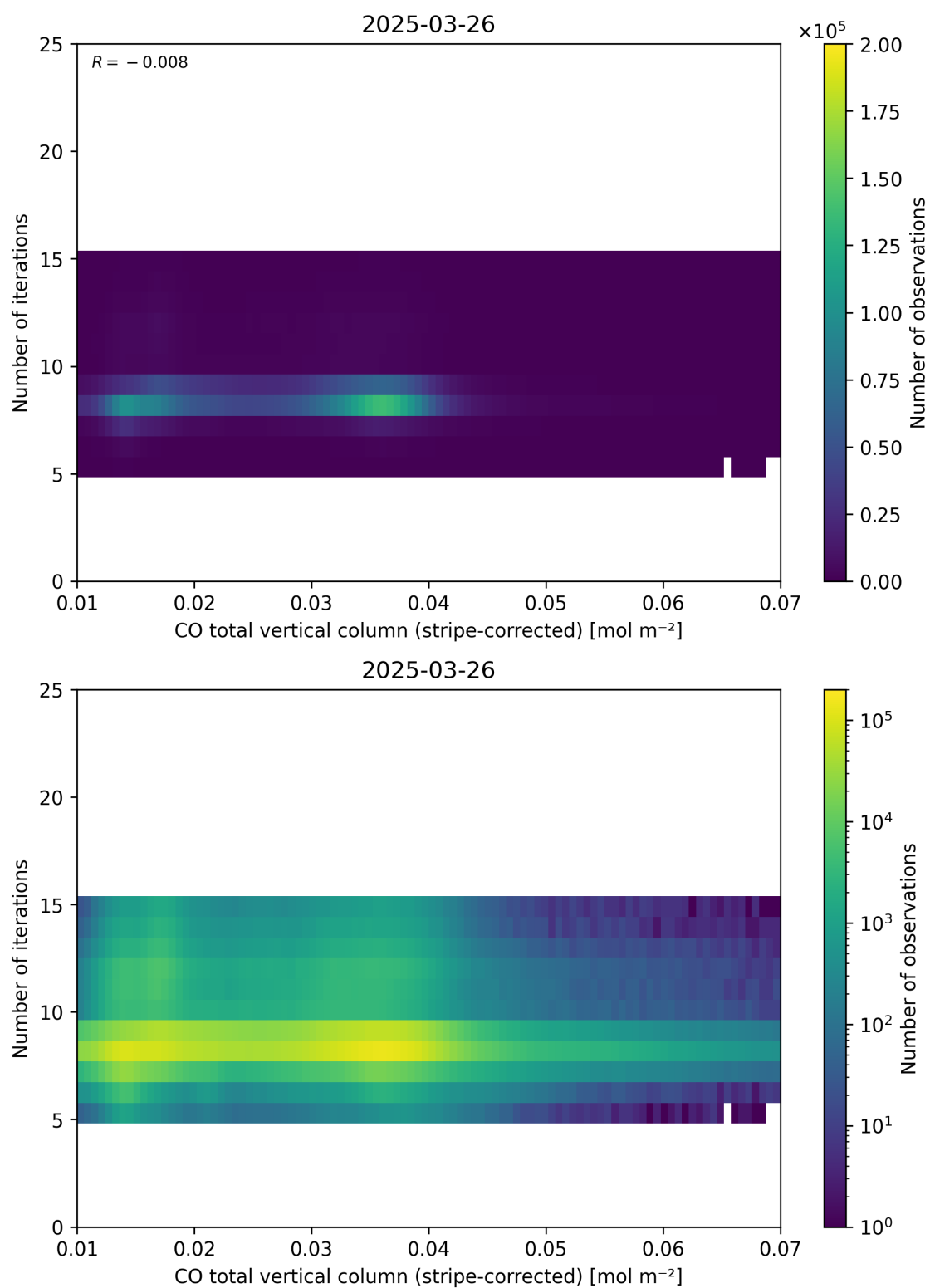
Figure 39: Scatter density plot of “CO total vertical column (stripe-corrected)” against “Number of iterations” for 2025-03-25 to 2025-03-27.
