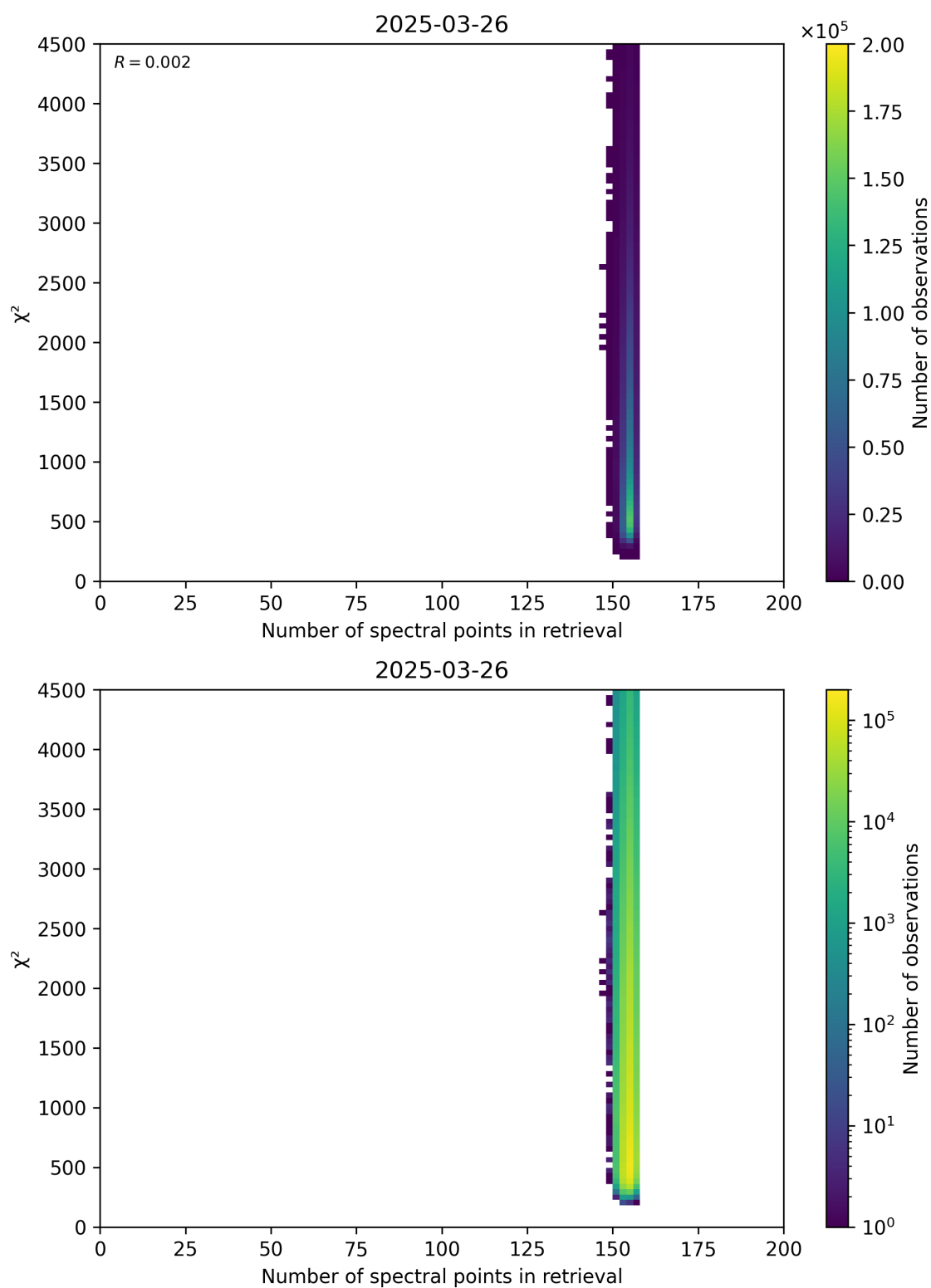
Figure 58: Scatter density plot of “Number of spectral points in retrieval” against “ \chi^2 ” for 2025-03-25 to 2025-03-27.
