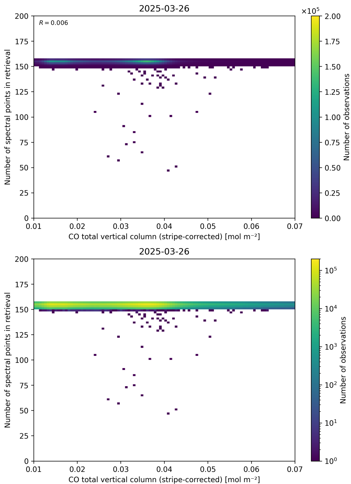
Figure 40: Scatter density plot of “CO total vertical column (stripe-corrected)” against “Number of spectral points in retrieval” for 2025-03-25 to 2025-03-27.
