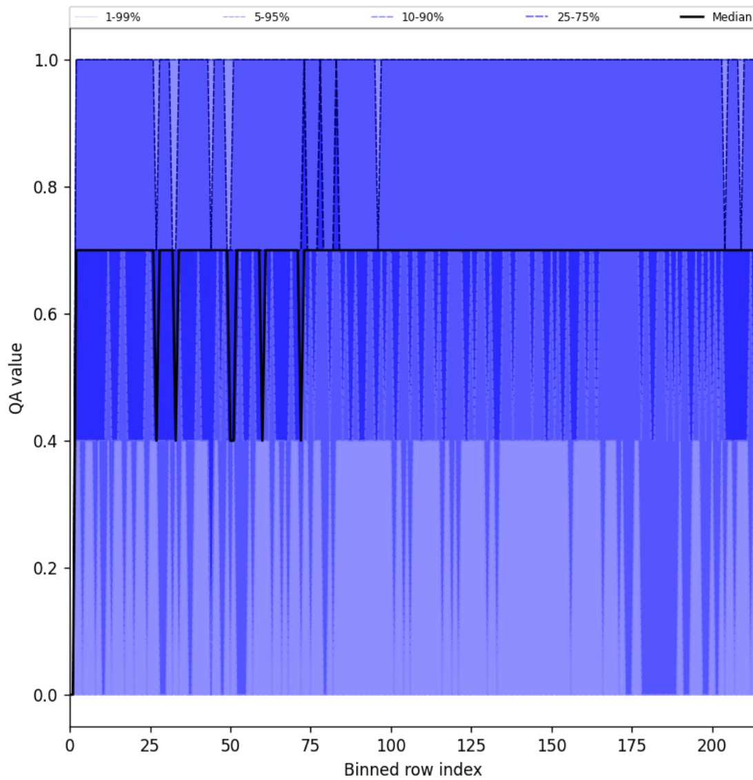
Figure 25: Along track statistics of “QA value” for 2025-03-25 to 2025-03-27
