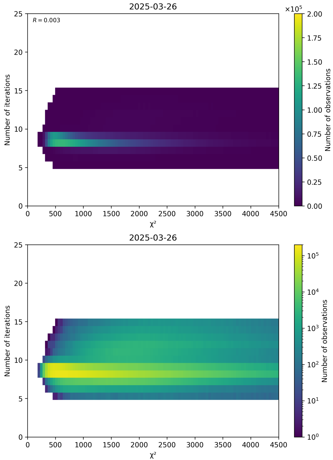
Figure 49: Scatter density plot of “ \chi^2 ” against “Number of iterations” for 2025-03-25 to 2025-03-27.
