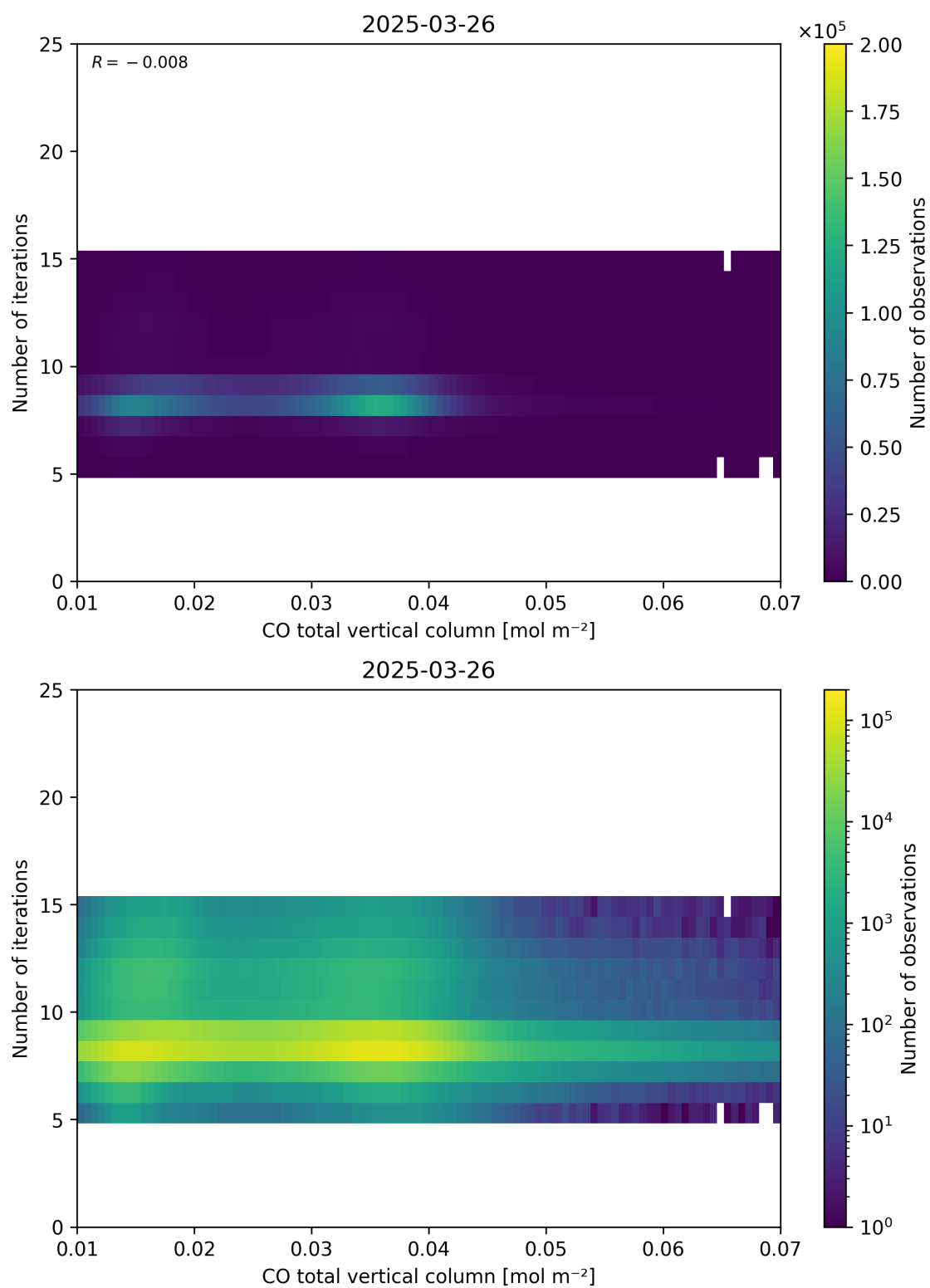
Figure 42: Scatter density plot of “CO total vertical column” against “Number of iterations” for 2025-03-25 to 2025-03-27.
