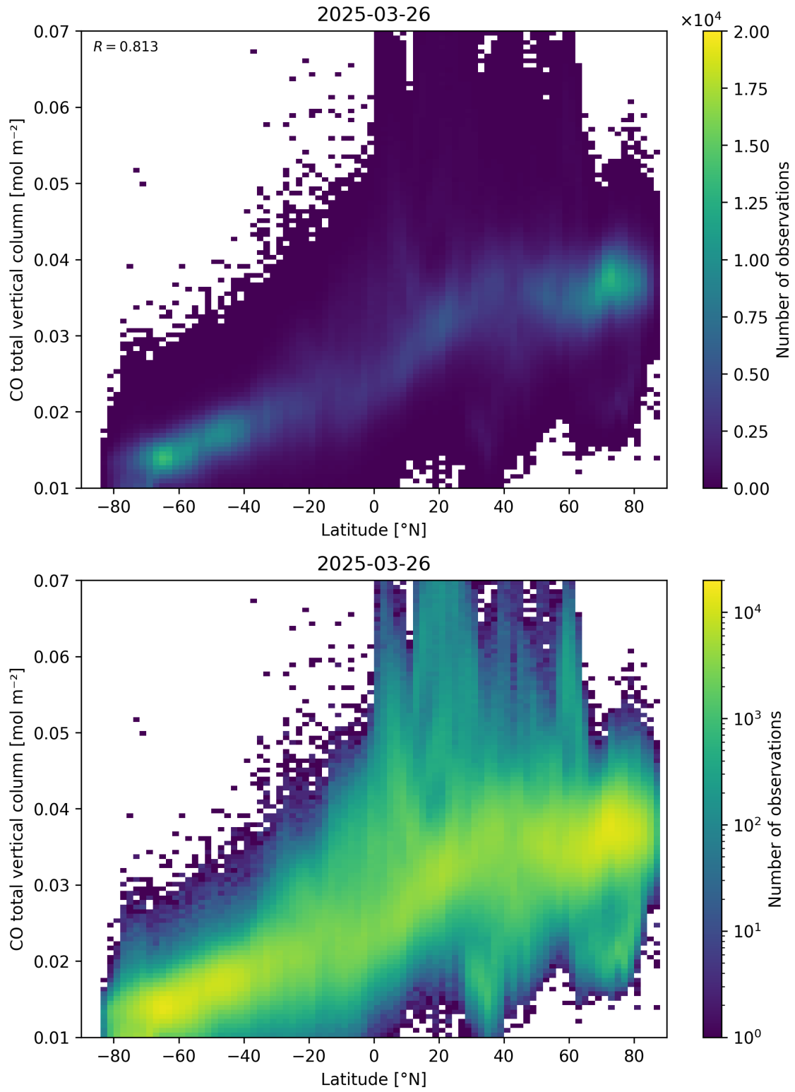
Figure 51: Scatter density plot of “Latitude” against “CO total vertical column” for 2025-03-25 to 2025-03-27.
