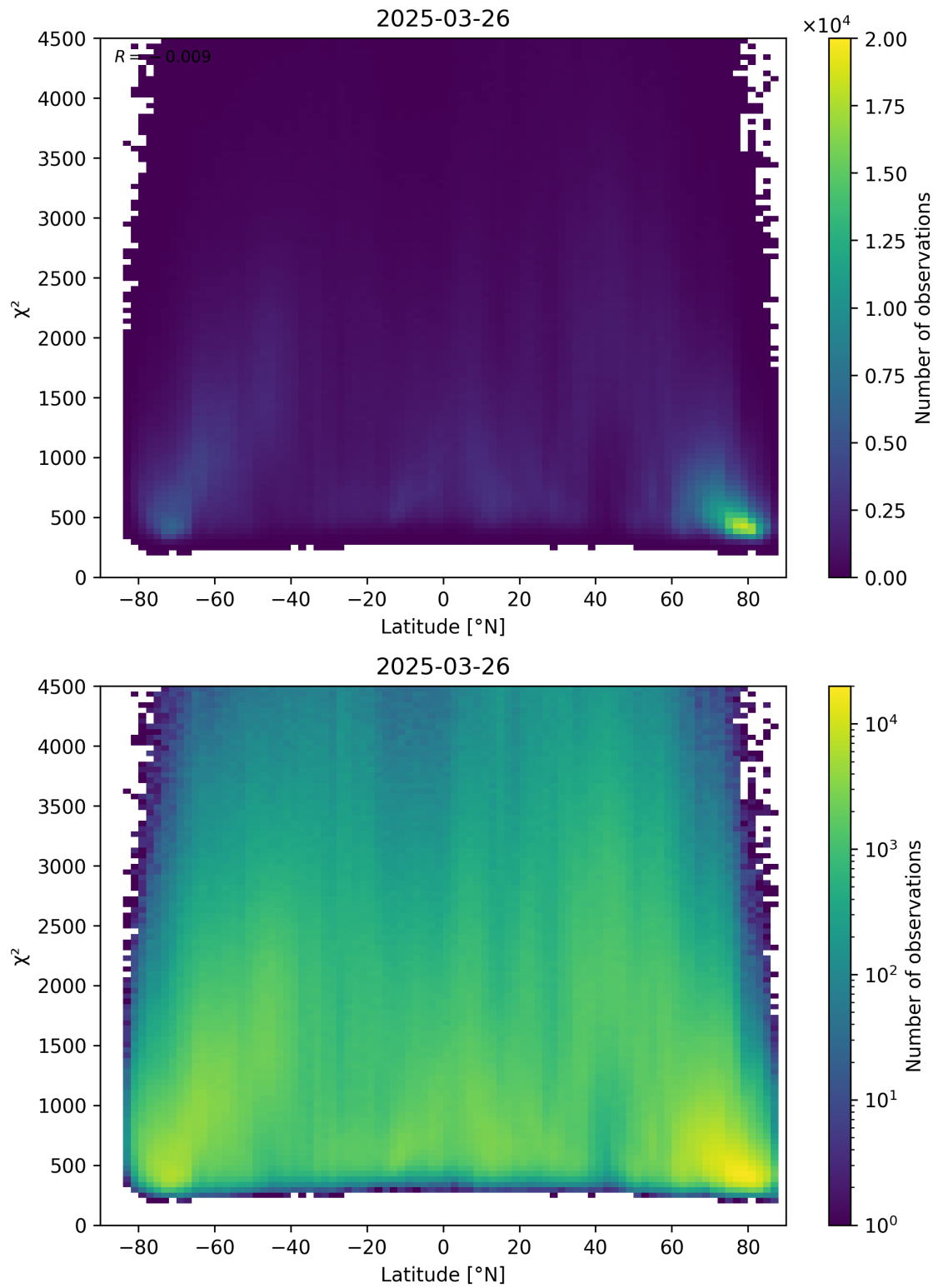
Figure 54: Scatter density plot of “Latitude” against “ \chi^2 ” for 2025-03-25 to 2025-03-27.
