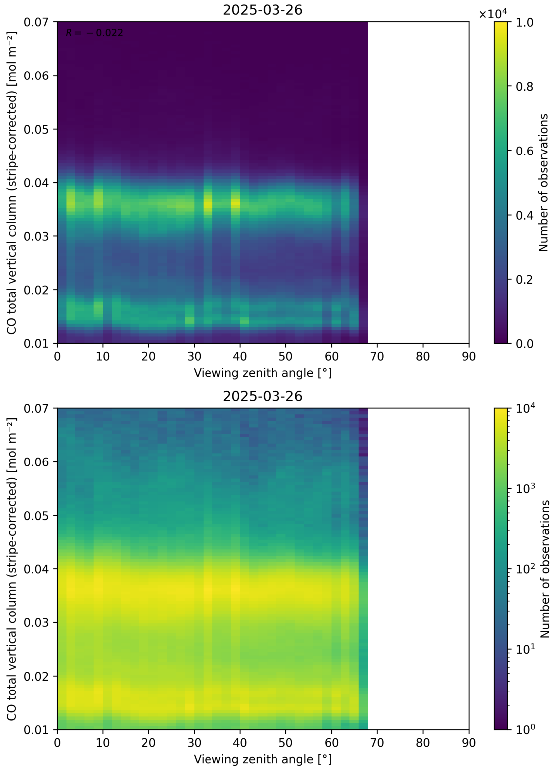
Figure 70: Scatter density plot of “Viewing zenith angle” against “CO total vertical column (stripe-corrected)” for 2025-03-25 to 2025-03-27.
