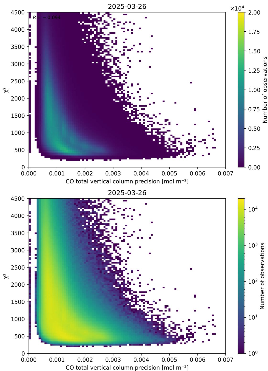
Figure 44: Scatter density plot of “CO total vertical column precision” against “ \chi^2 ” for 2025-03-25 to 2025-03-27.
