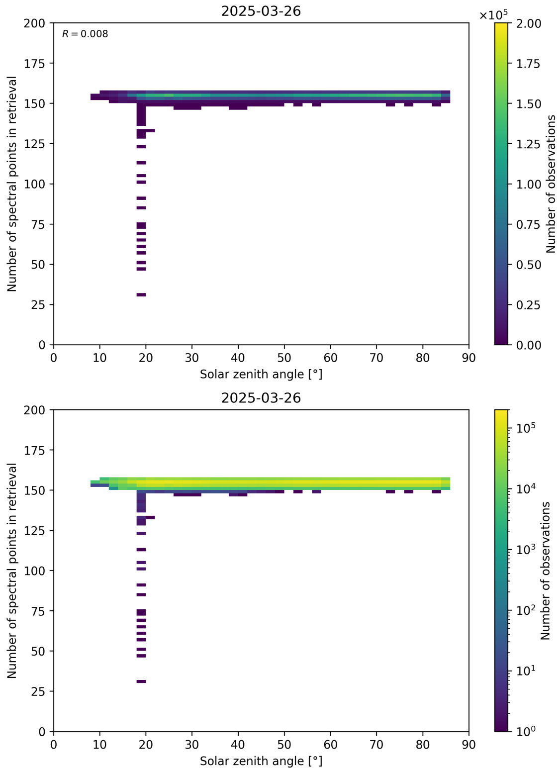
Figure 68: Scatter density plot of “Solar zenith angle” against “Number of spectral points in retrieval” for 2025-03-25 to 2025-03-27.
