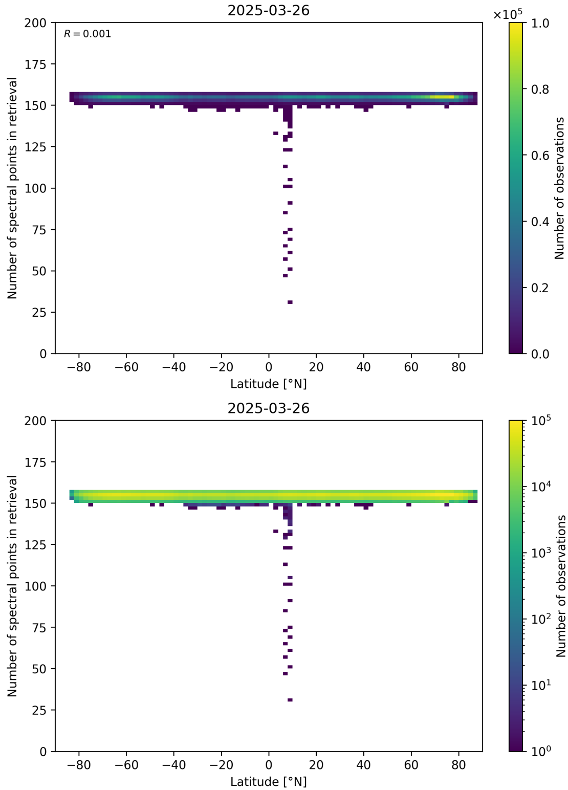
Figure 57: Scatter density plot of “Latitude” against “Number of spectral points in retrieval” for 2025-03-25 to 2025-03-27.
