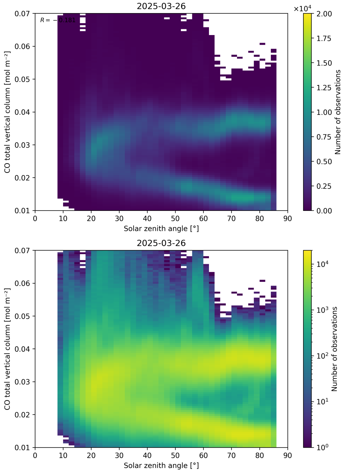
Figure 61: Scatter density plot of “Solar zenith angle” against “CO total vertical column” for 2025-03-25 to 2025-03-27.
