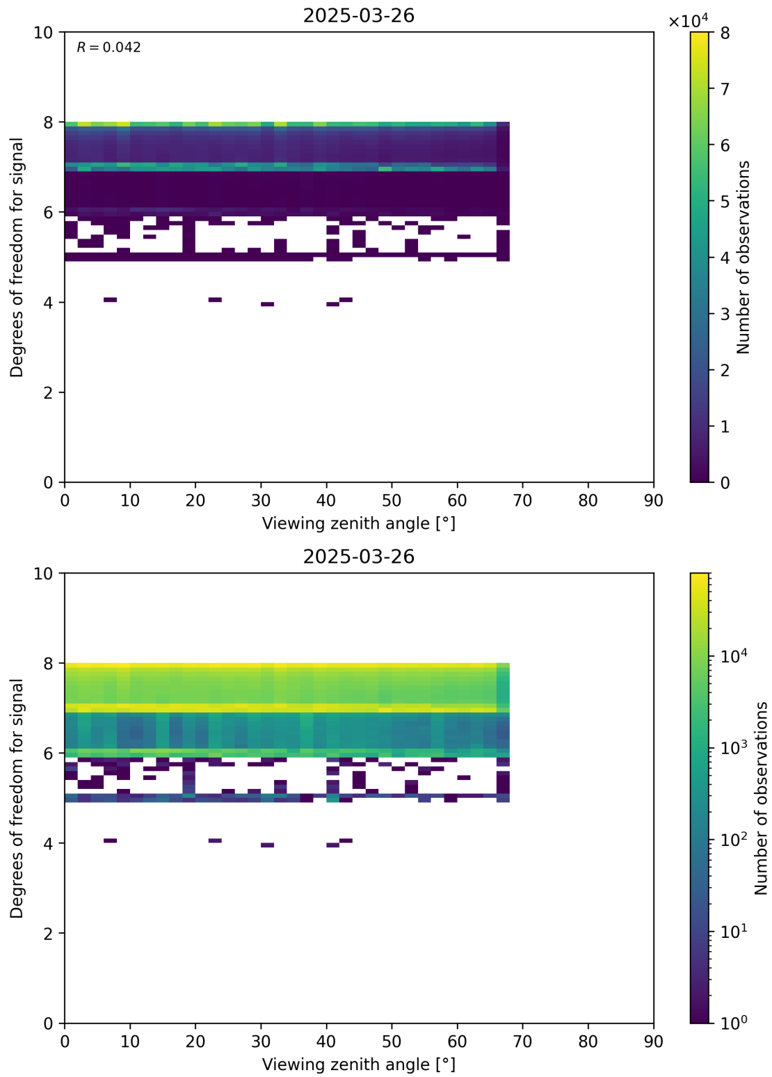
Figure 73: Scatter density plot of “Viewing zenith angle” against “Degrees of freedom for signal” for 2025-03-25 to 2025-03-27.
