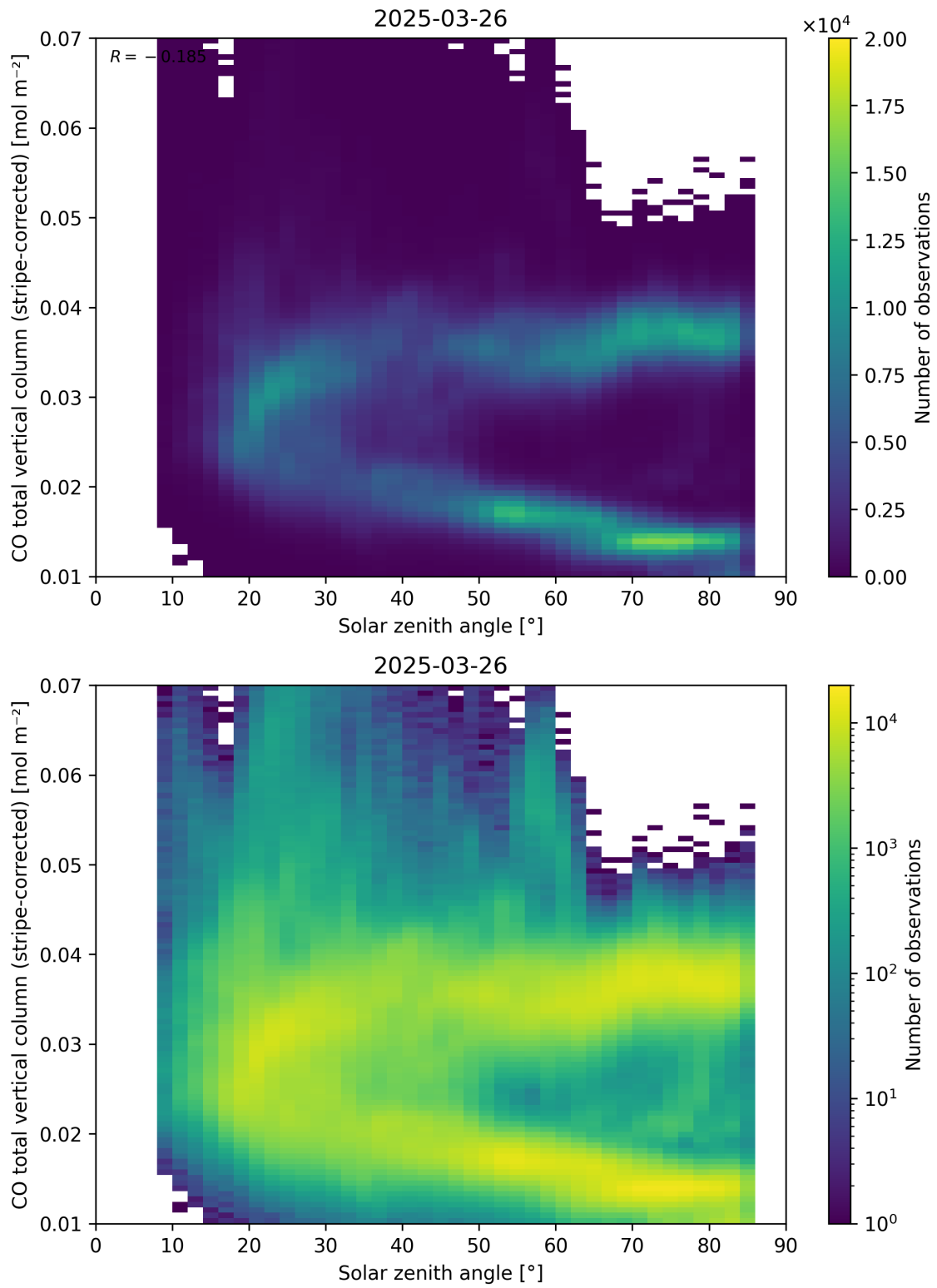
Figure 62: Scatter density plot of “Solar zenith angle” against “CO total vertical column (stripe-corrected)” for 2025-03-25 to 2025-03-27.
