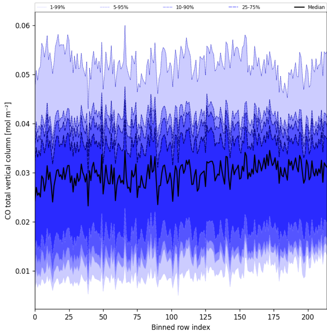
Figure 26: Along track statistics of “CO total vertical column” for 2025-03-25 to 2025-03-27
