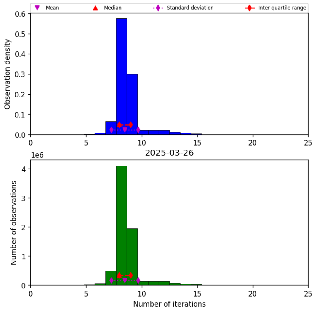
Figure 24: Histogram of “Number of iterations” for 2025-03-25 to 2025-03-27
