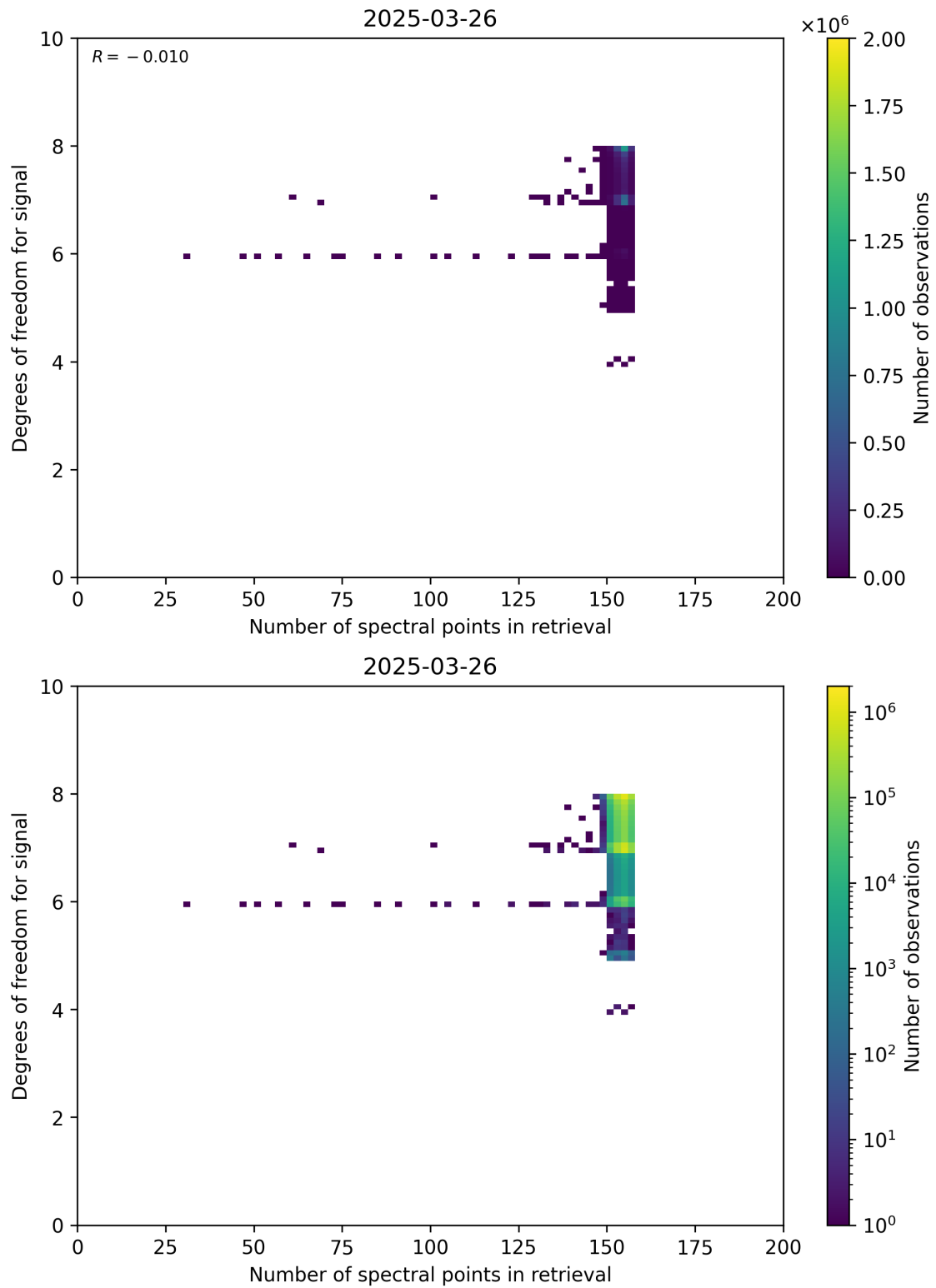
Figure 59: Scatter density plot of “Number of spectral points in retrieval” against “Degrees of freedom for signal” for 2025-03-25 to 2025-03-27.
