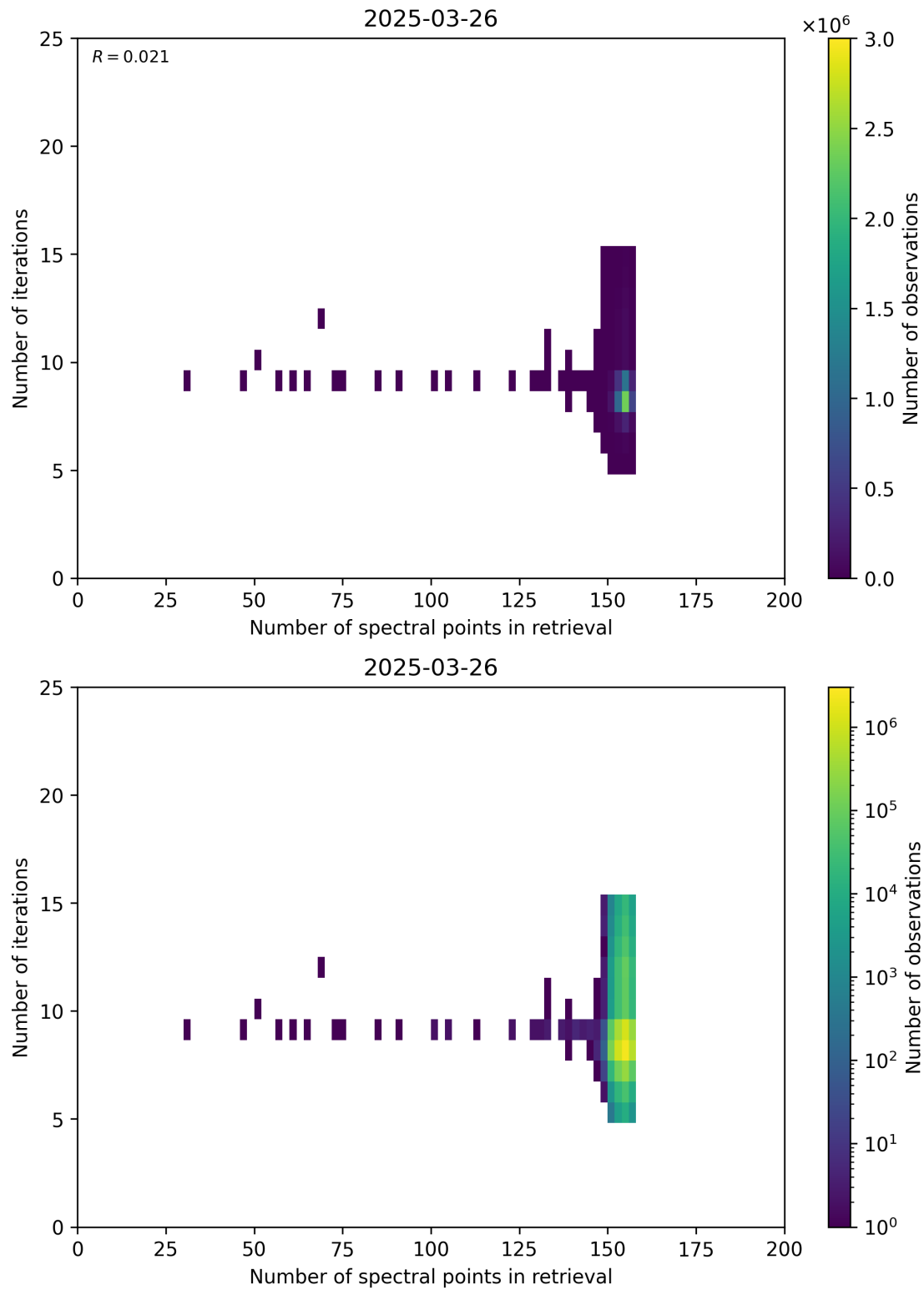
Figure 60: Scatter density plot of “Number of spectral points in retrieval” against “Number of iterations” for 2025-03-25 to 2025-03-27.
