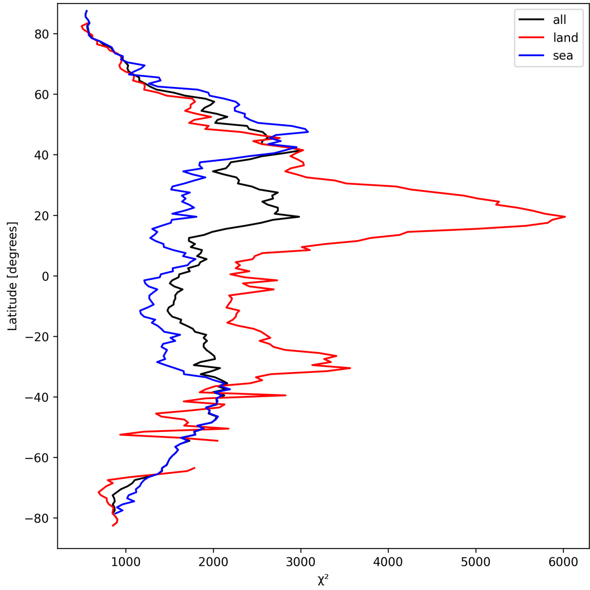
Figure 14: Zonal average of “ \chi^2 ” for 2025-03-25 to 2025-03-27.
