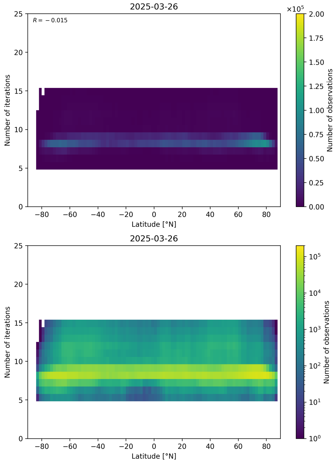
Figure 56: Scatter density plot of “Latitude” against “Number of iterations” for 2025-03-25 to 2025-03-27.
