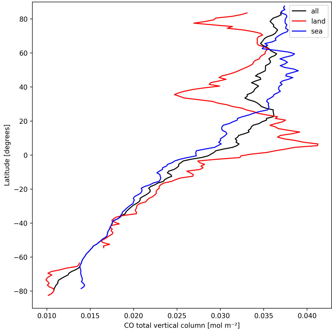
Figure 10: Zonal average of “CO total vertical column” for 2025-03-25 to 2025-03-27.
