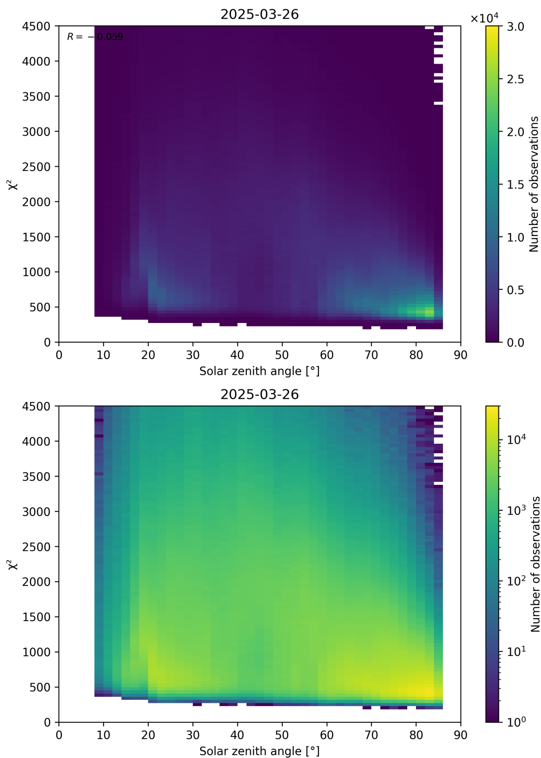
Figure 64: Scatter density plot of “Solar zenith angle” against “ \chi^2 ” for 2025-03-25 to 2025-03-27.
