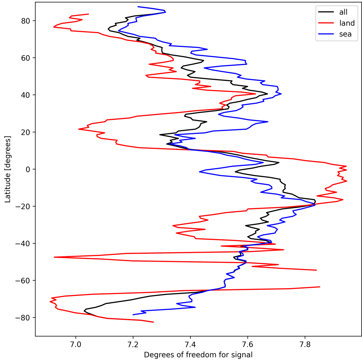
Figure 15: Zonal average of “Degrees of freedom for signal” for 2025-03-25 to 2025-03-27.
