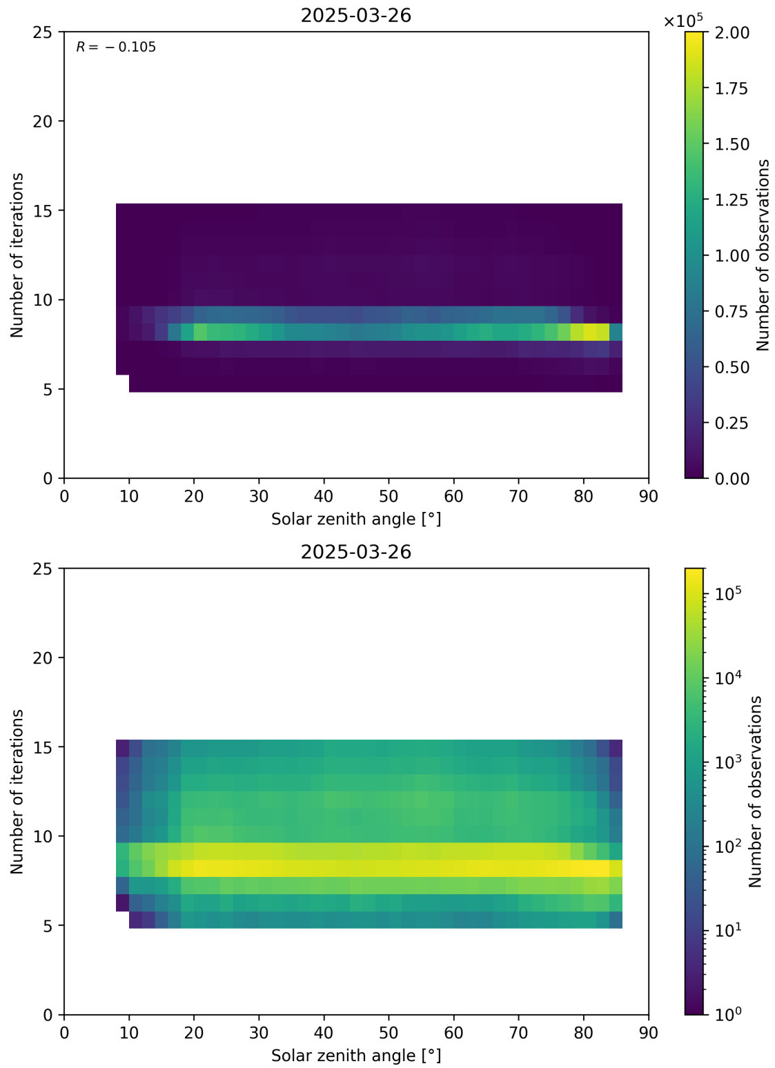
Figure 67: Scatter density plot of “Solar zenith angle” against “Number of iterations” for 2025-03-25 to 2025-03-27.
