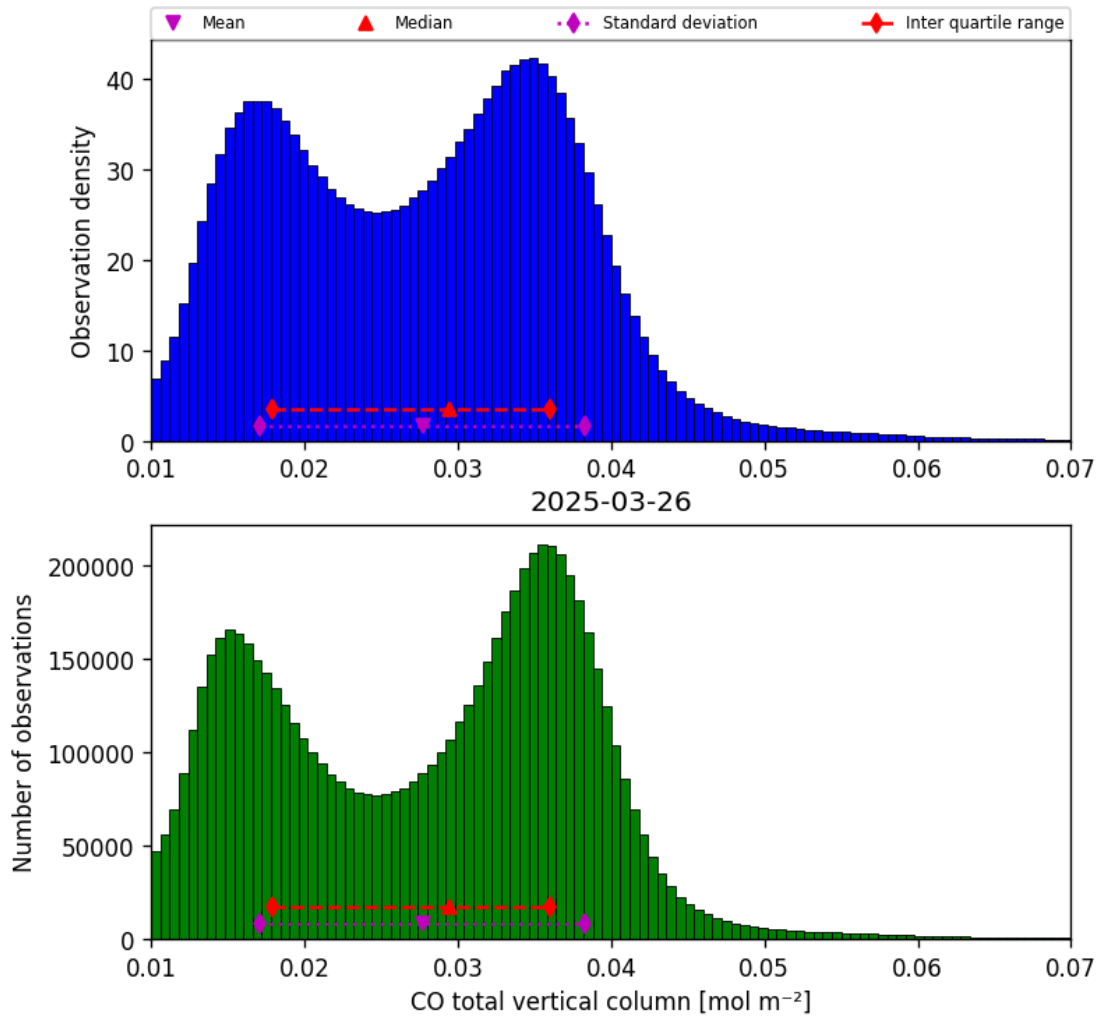
Figure 18: Histogram of “CO total vertical column” for 2025-03-25 to 2025-03-27
