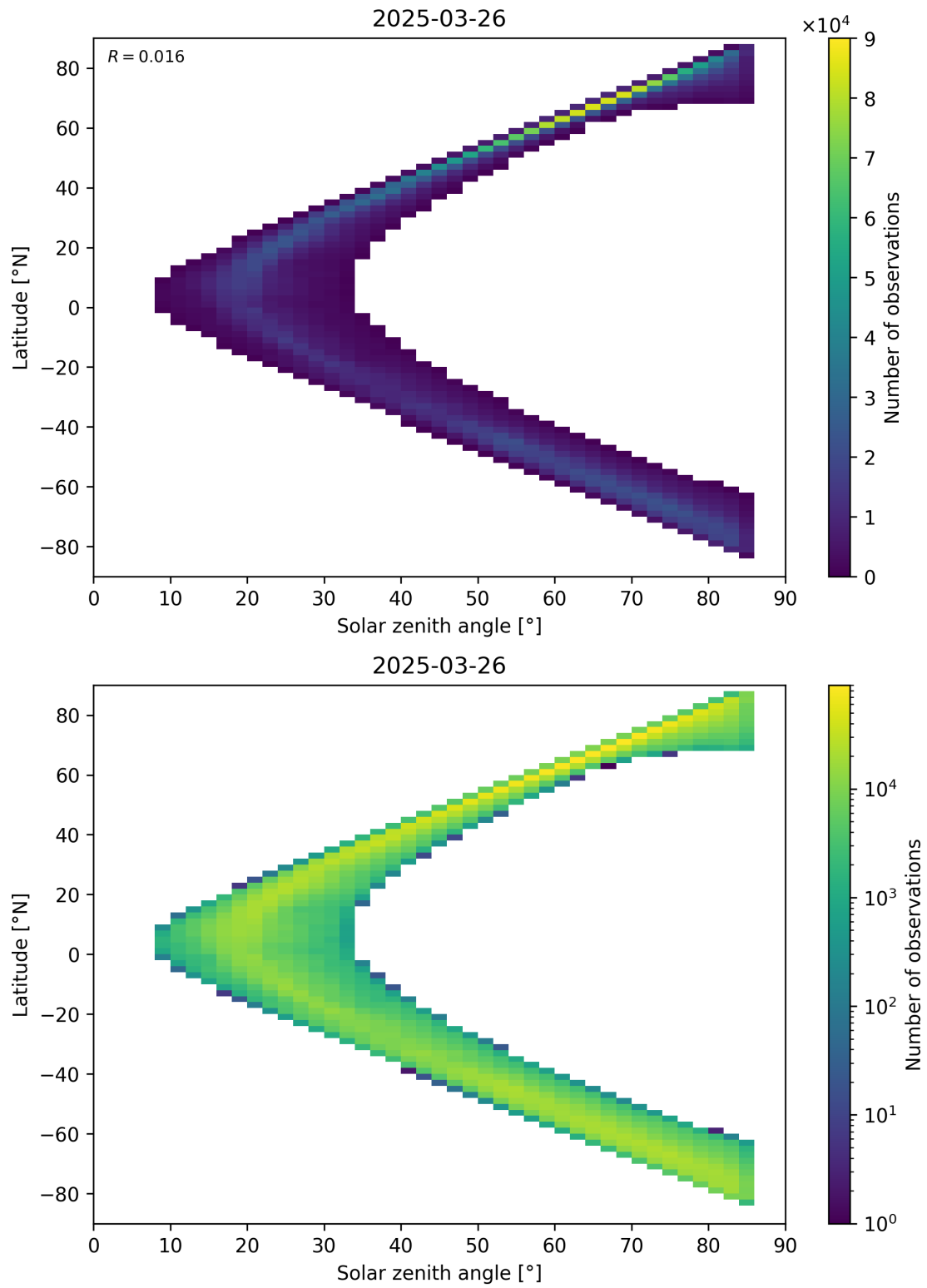
Figure 66: Scatter density plot of “Solar zenith angle” against “Latitude” for 2025-03-25 to 2025-03-27.
