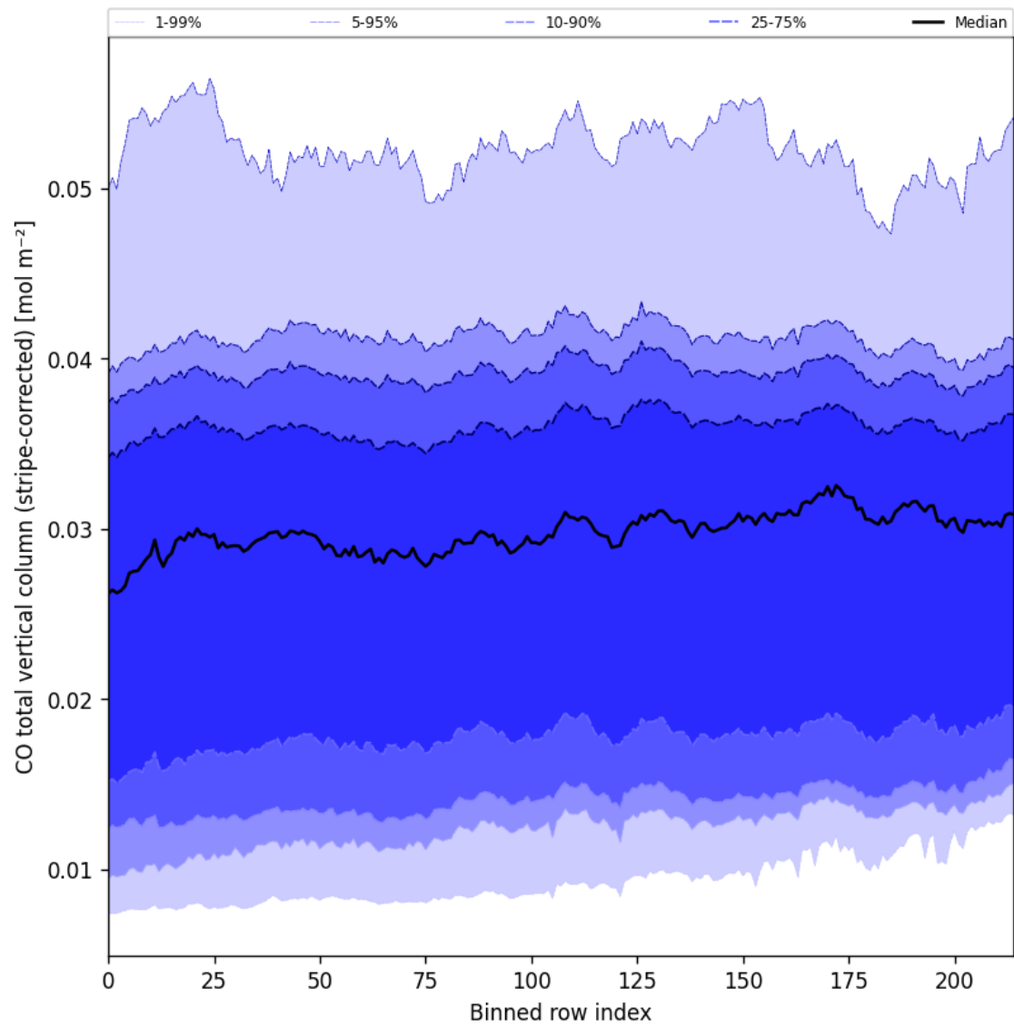
Figure 27: Along track statistics of “CO total vertical column (stripe-corrected)” for 2025-03-25 to 2025-03-27
