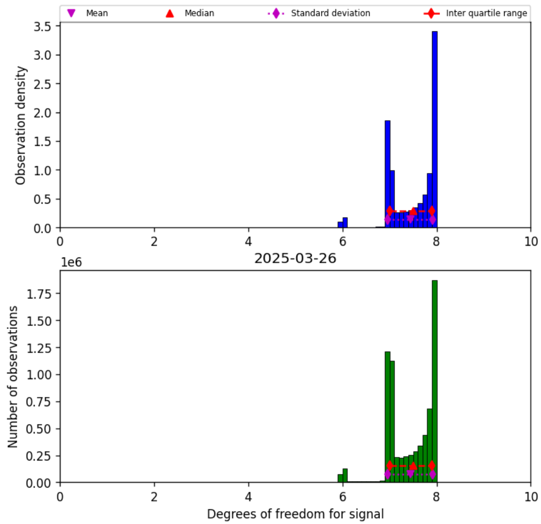
Figure 23: Histogram of “Degrees of freedom for signal” for 2025-03-25 to 2025-03-27
