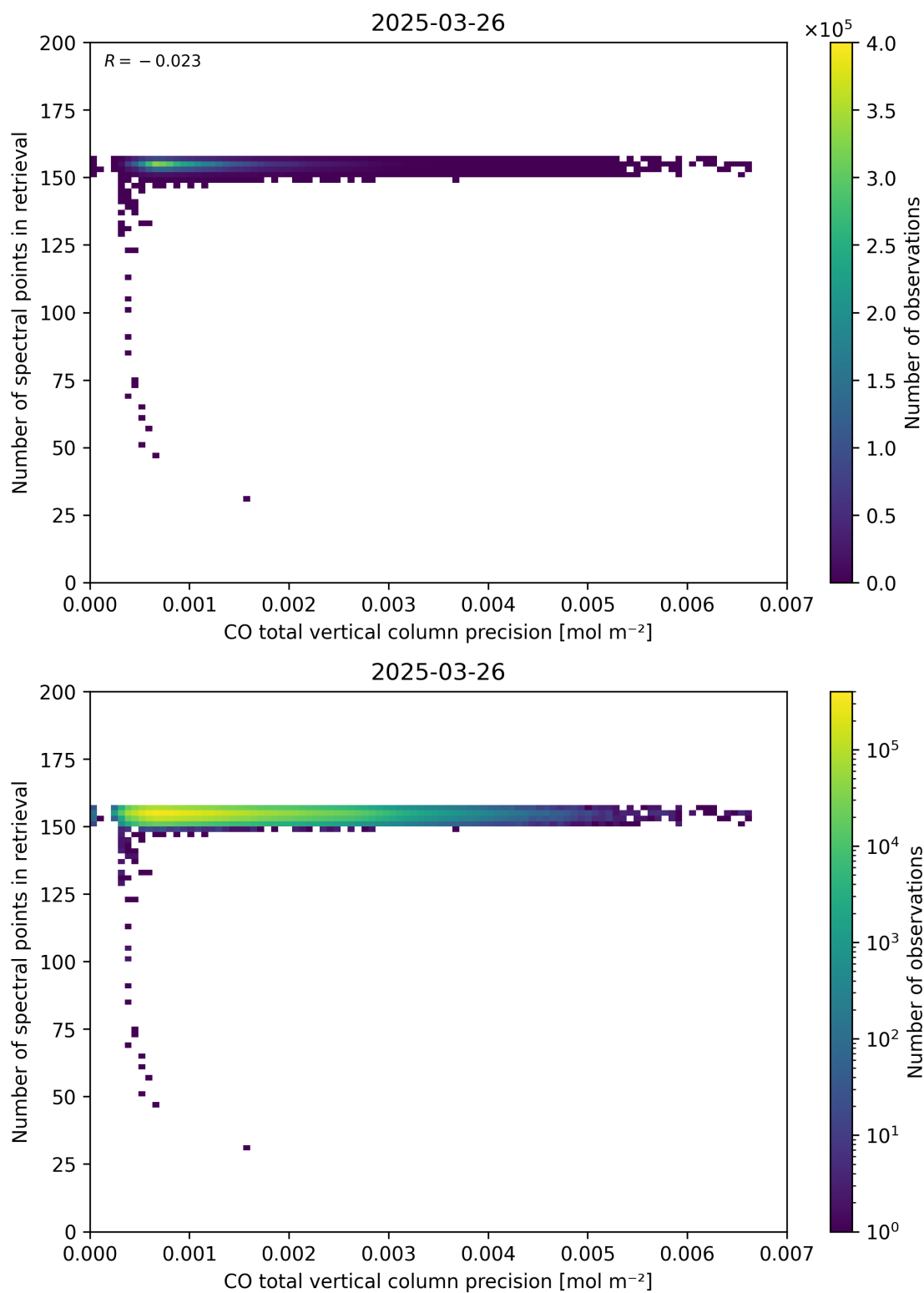
Figure 47: Scatter density plot of “CO total vertical column precision” against “Number of spectral points in retrieval” for 2025-03-25 to 2025-03-27.
