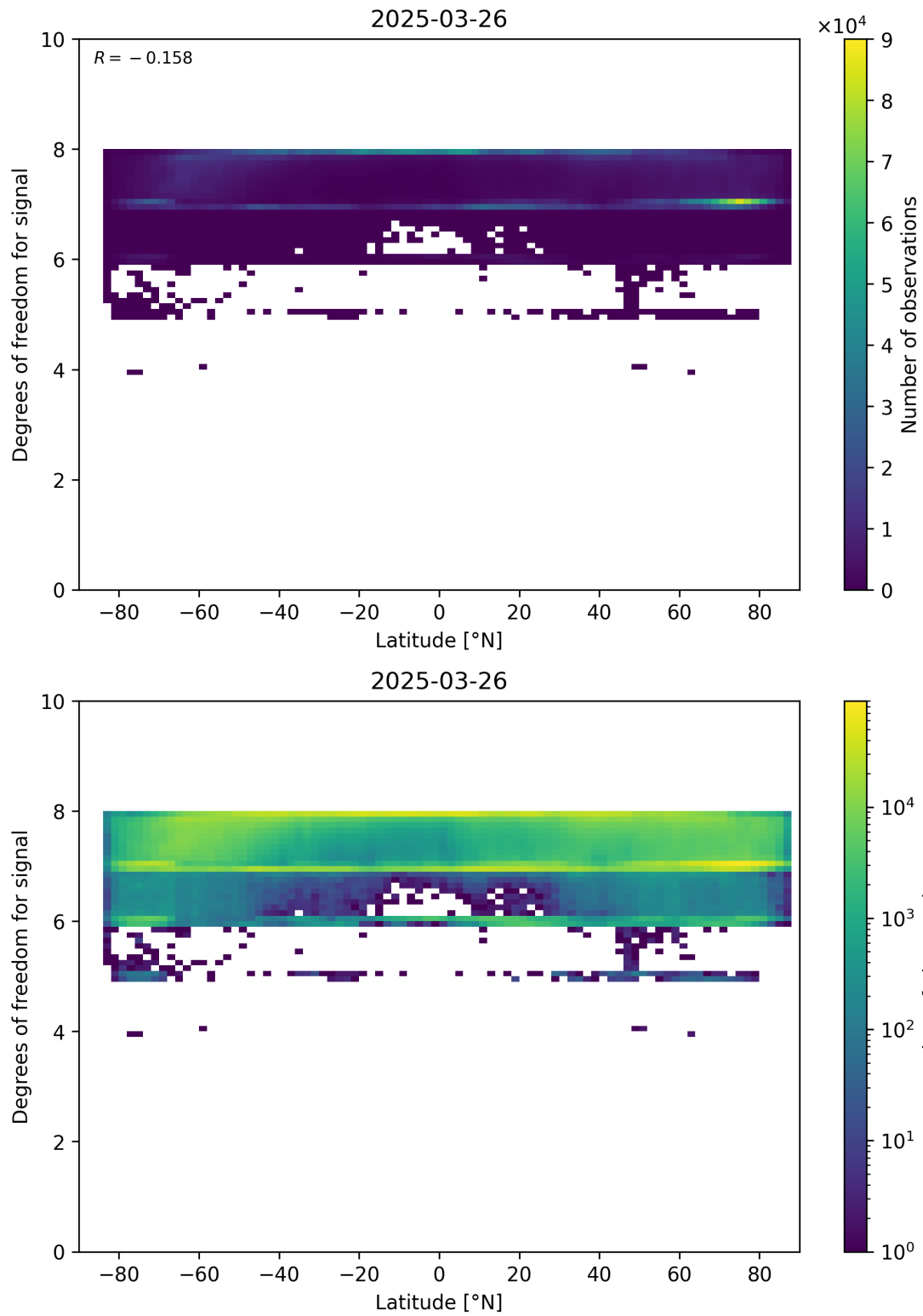
Figure 55: Scatter density plot of “Latitude” against “Degrees of freedom for signal” for 2025-03-25 to 2025-03-27.
