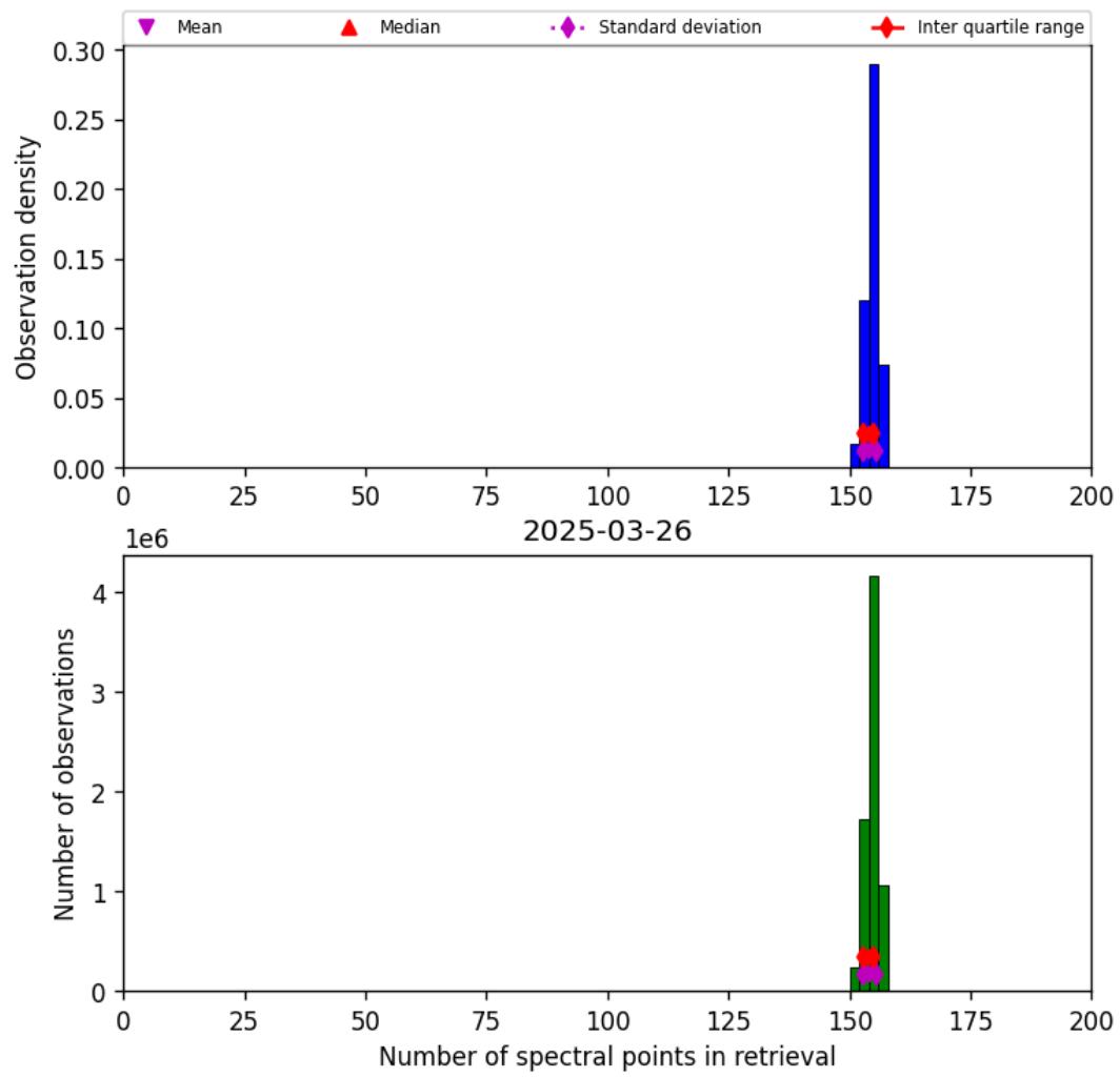
Figure 21: Histogram of “Number of spectral points in retrieval” for 2025-03-25 to 2025-03-27
