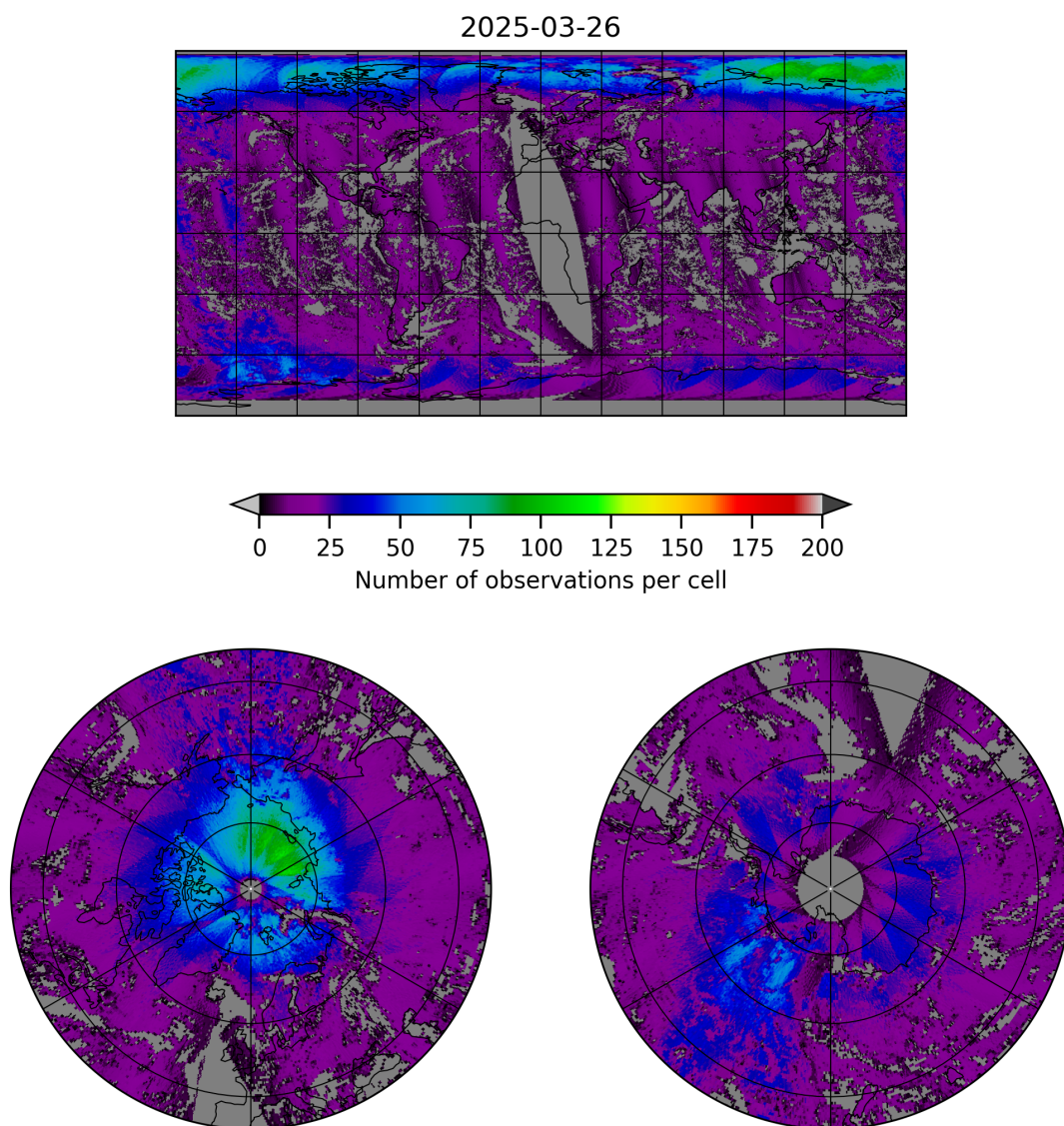
Figure 8: Map of the number of observations for 2025-03-25 to 2025-03-27
