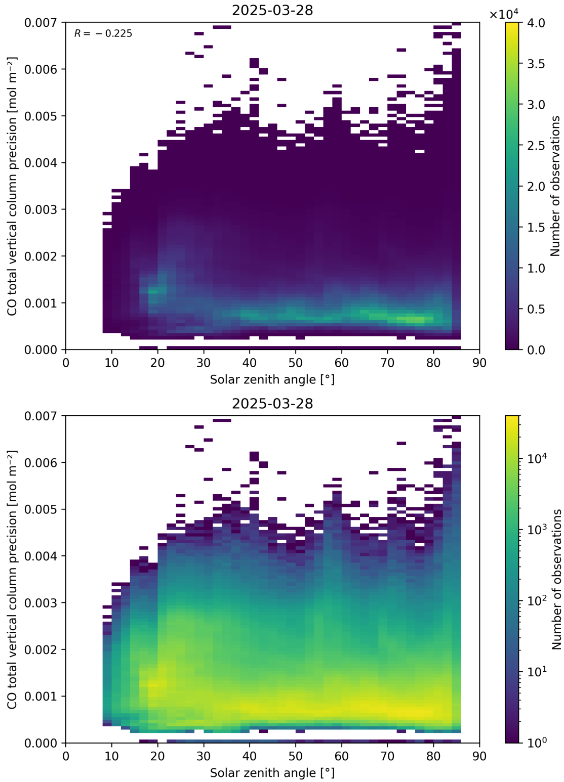
Figure 63: Scatter density plot of “Solar zenith angle” against “CO total vertical column precision” for 2025-03-28 to 2025-03-29.
