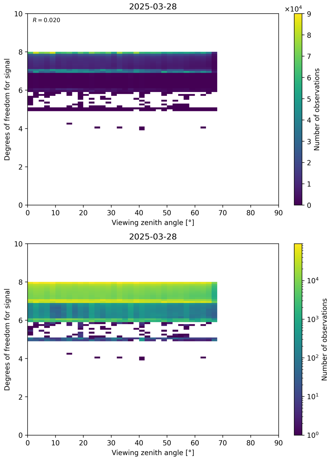
Figure 73: Scatter density plot of “Viewing zenith angle” against “Degrees of freedom for signal” for 2025-03-28 to 2025-03-29.
