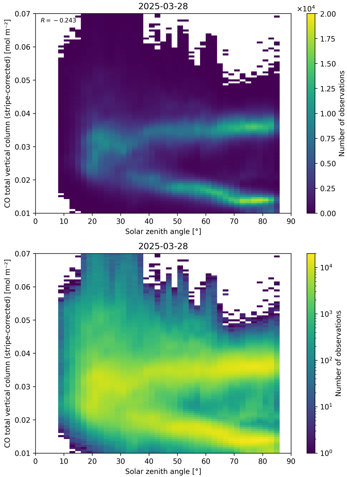
Figure 62: Scatter density plot of “Solar zenith angle” against “CO total vertical column (stripe-corrected)” for 2025-03-28 to 2025-03-29.
