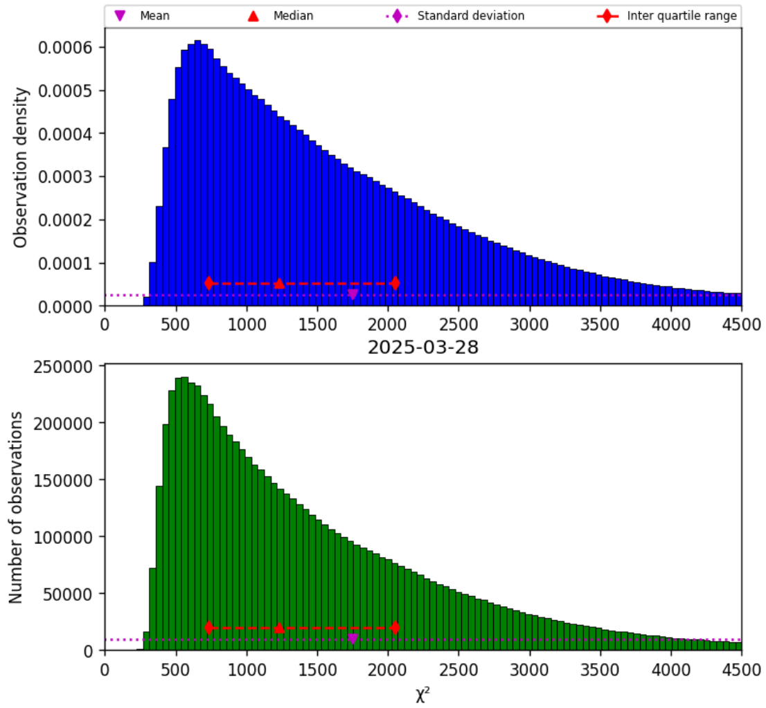
Figure 22: Histogram of “ \chi^2 ” for 2025-03-28 to 2025-03-29
