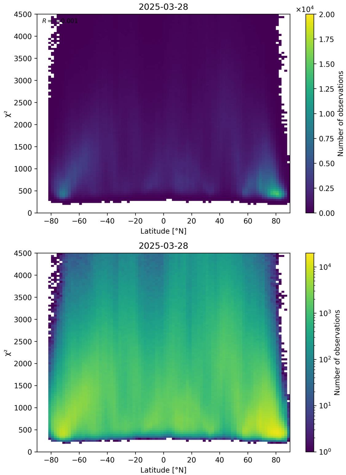
Figure 54: Scatter density plot of “Latitude” against “ \chi^2 ” for 2025-03-28 to 2025-03-29.
