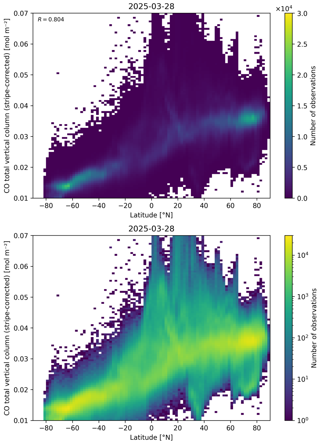
Figure 52: Scatter density plot of “Latitude” against “CO total vertical column (stripe-corrected)” for 2025-03-28 to 2025-03-29.
