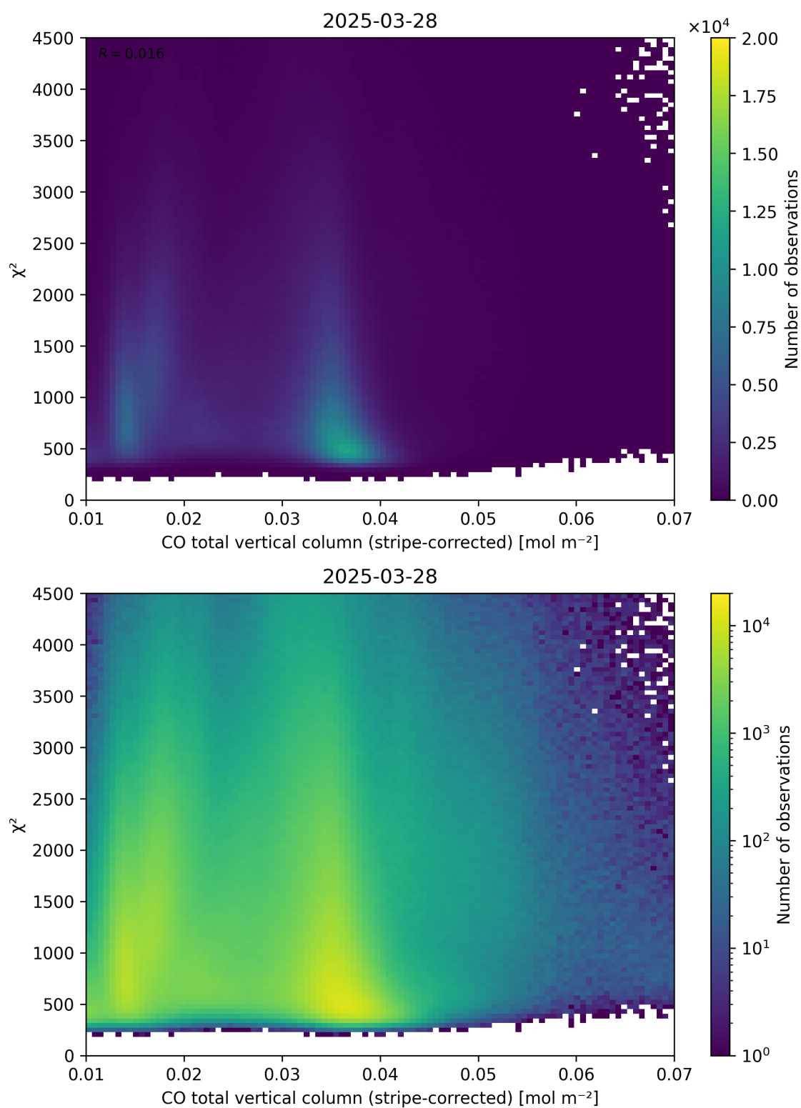
Figure 37: Scatter density plot of “CO total vertical column (stripe-corrected)” against “ \chi^2 ” for 2025-03-28 to 2025-03-29.
