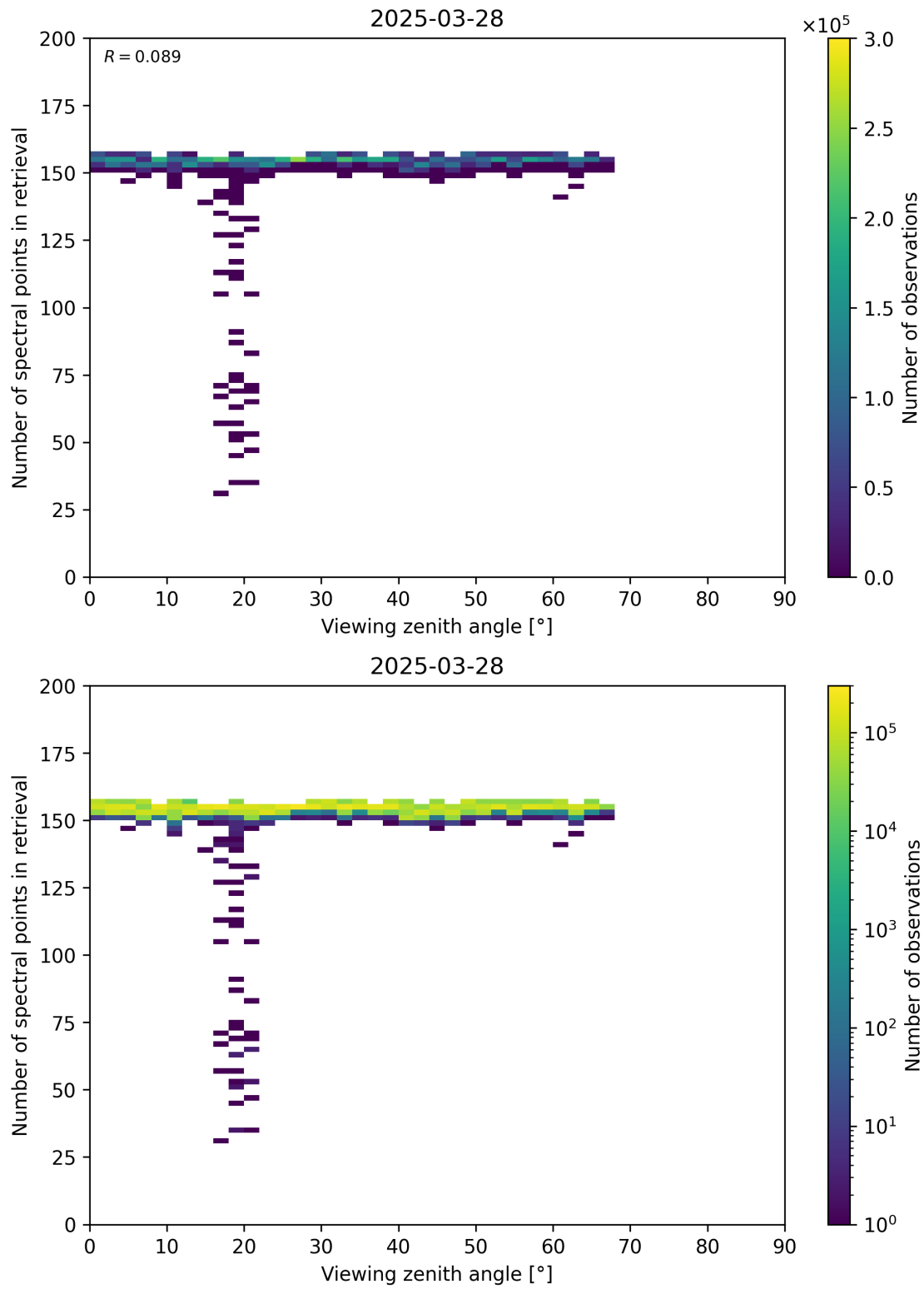
Figure 76: Scatter density plot of “Viewing zenith angle” against “Number of spectral points in retrieval” for 2025-03-28 to 2025-03-29.
