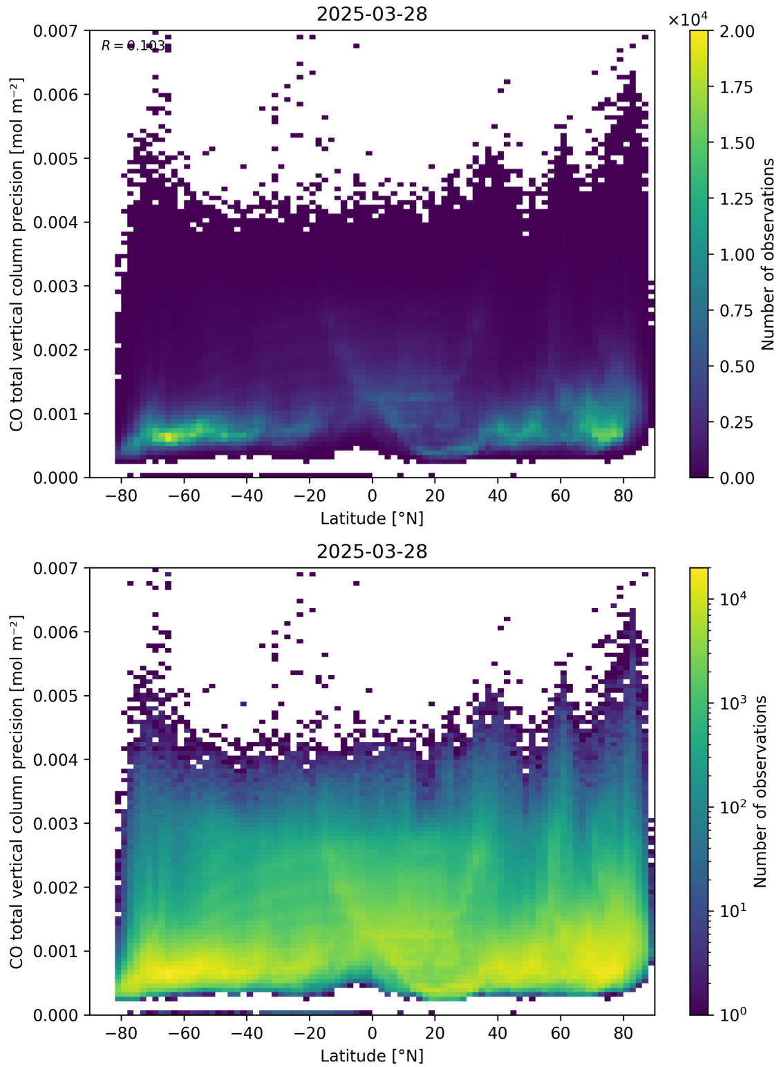
Figure 53: Scatter density plot of “Latitude” against “CO total vertical column precision” for 2025-03-28 to 2025-03-29.
