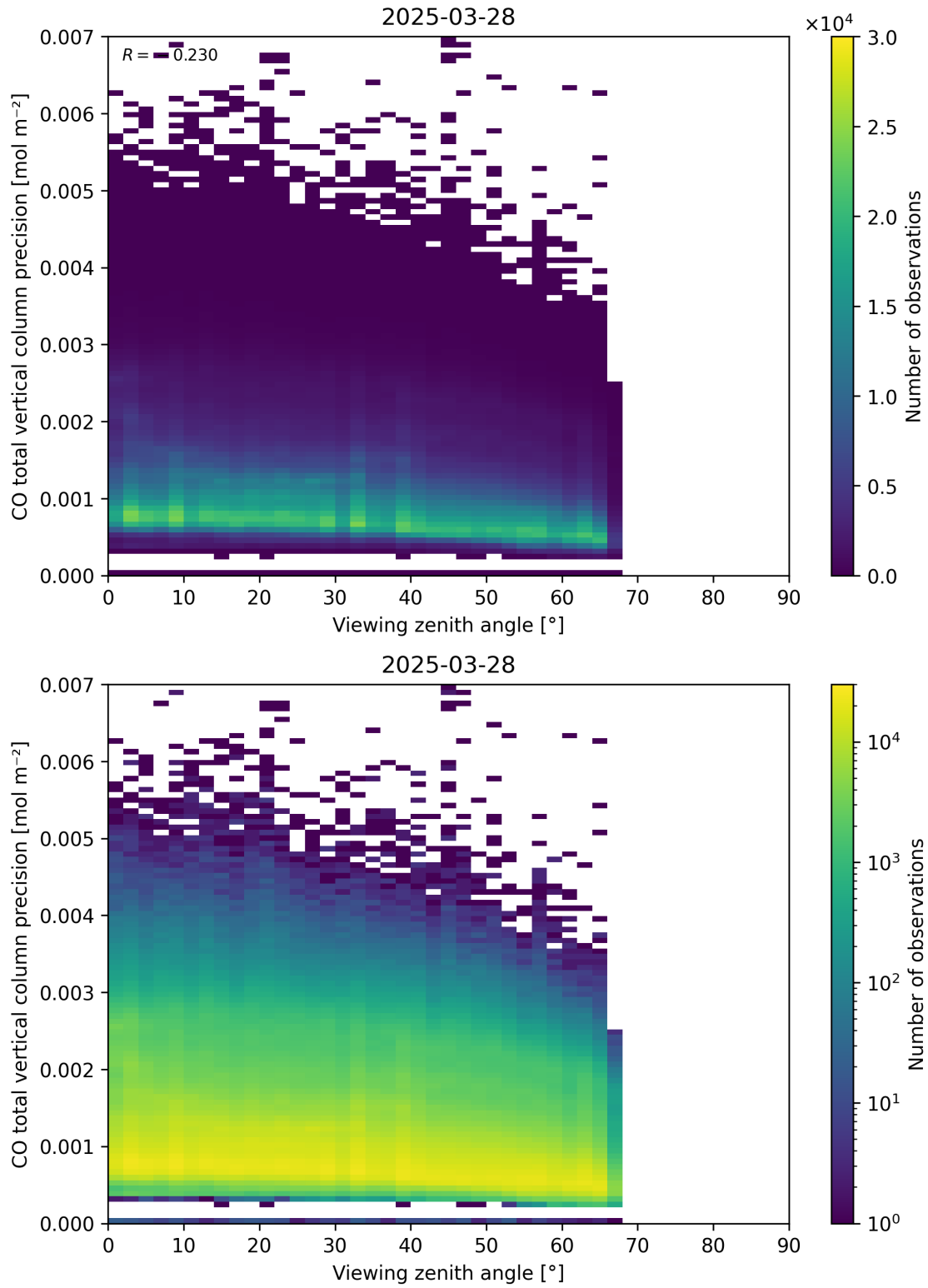
Figure 71: Scatter density plot of “Viewing zenith angle” against “CO total vertical column precision” for 2025-03-28 to 2025-03-29.
