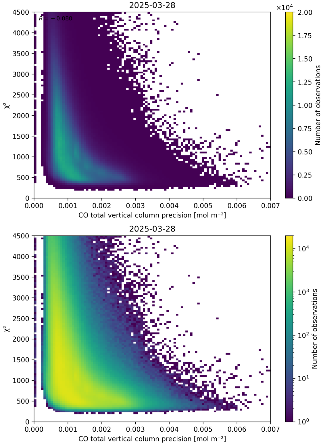
Figure 44: Scatter density plot of “CO total vertical column precision” against “ \chi^2 ” for 2025-03-28 to 2025-03-29.
