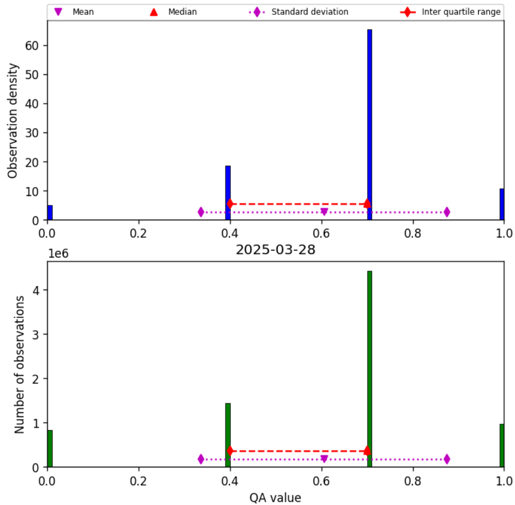
Figure 17: Histogram of “QA value” for 2025-03-28 to 2025-03-29
