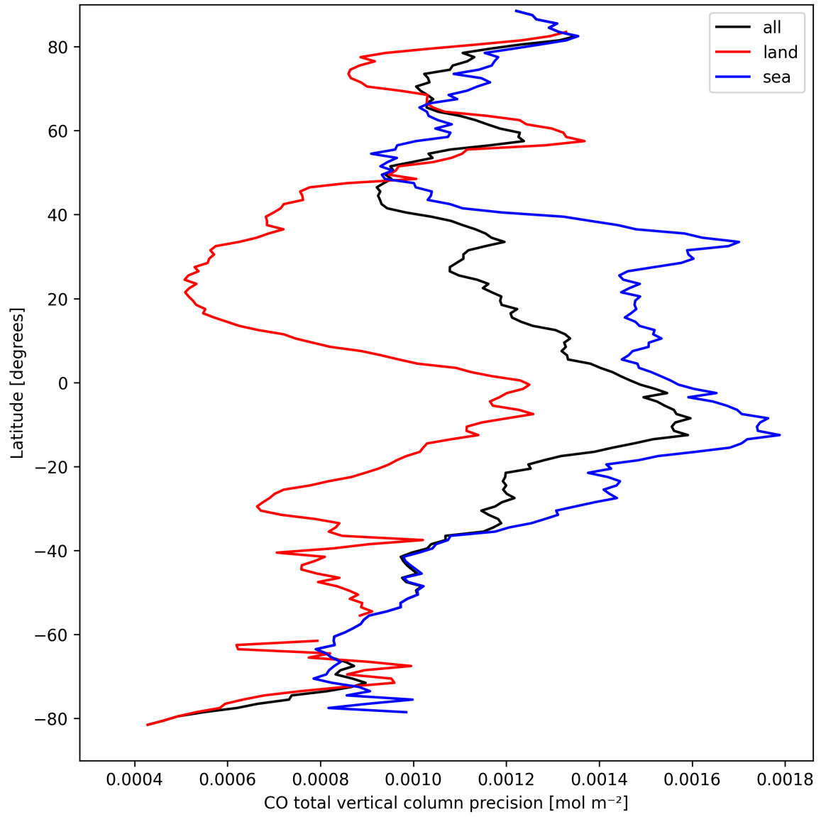
Figure 12: Zonal average of “CO total vertical column precision” for 2025-03-28 to 2025-03-29.
