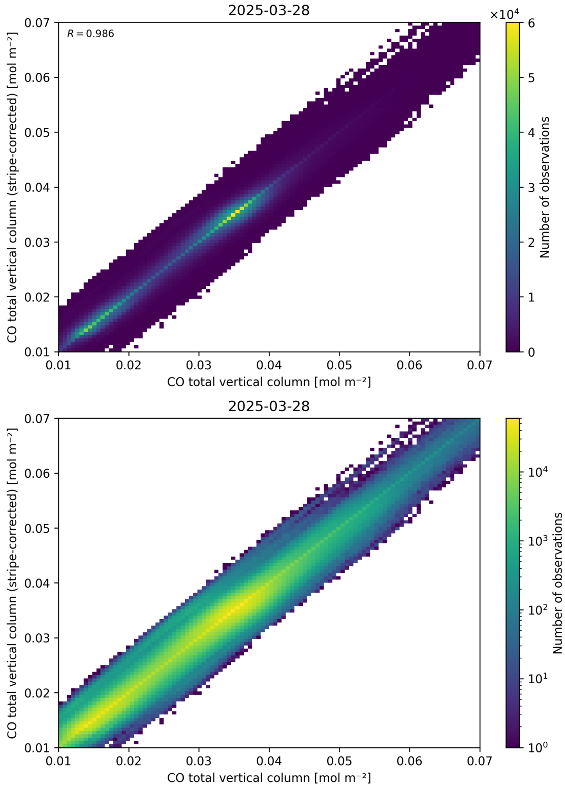
Figure 33: Scatter density plot of “CO total vertical column” against “CO total vertical column (stripe-corrected)” for 2025-03-28 to 2025-03-29.
