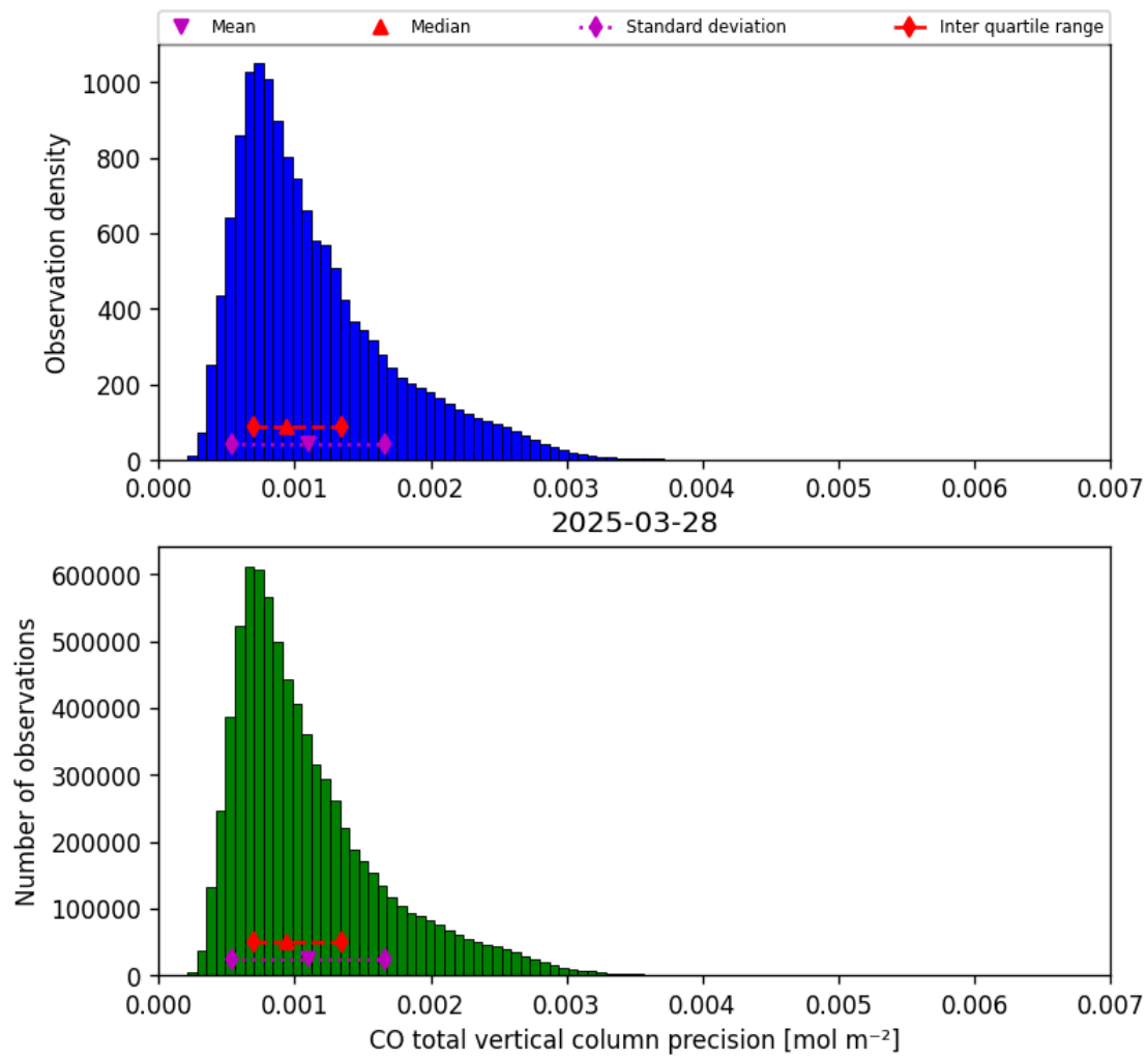
Figure 20: Histogram of “CO total vertical column precision” for 2025-03-28 to 2025-03-29
