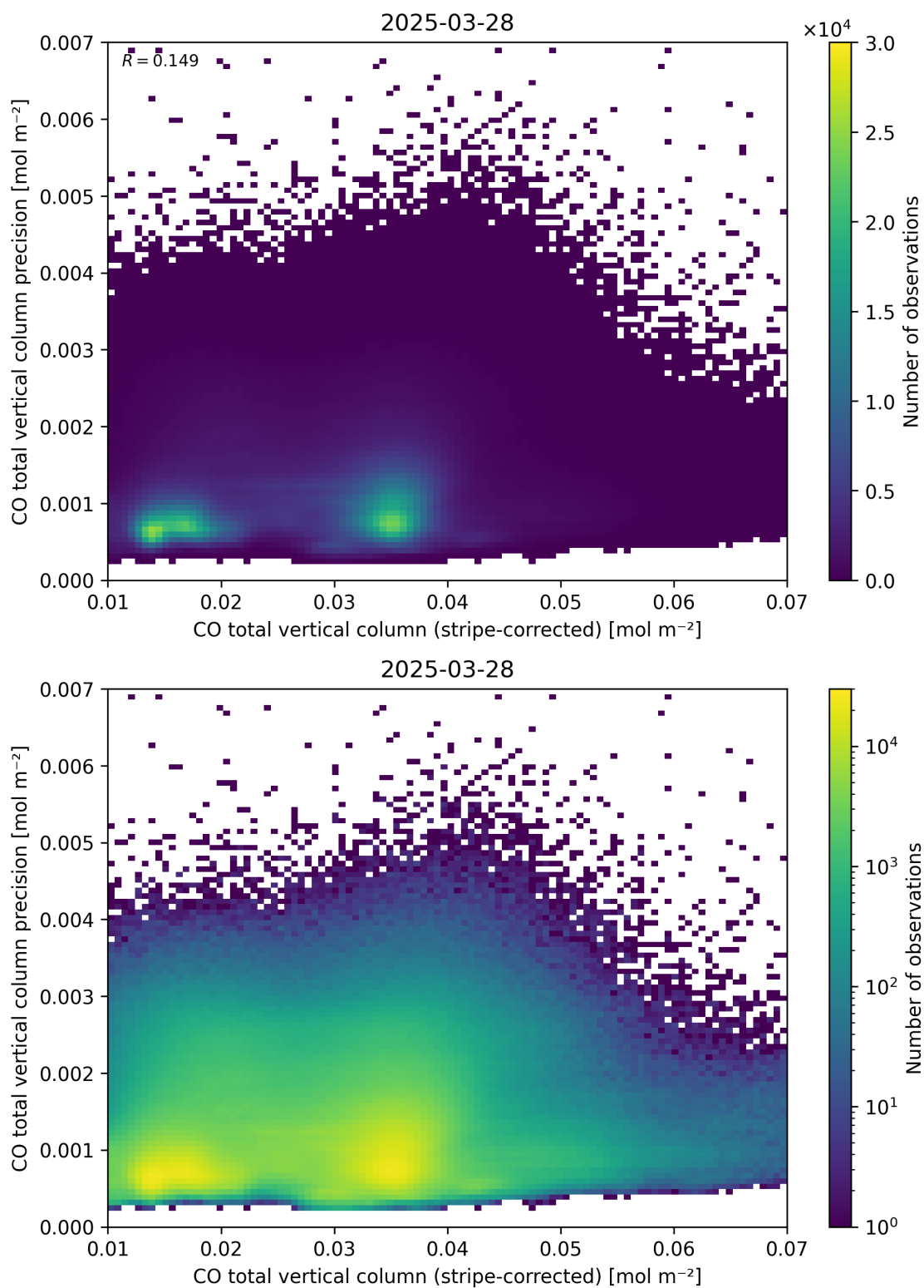
Figure 36: Scatter density plot of “CO total vertical column (stripe-corrected)” against “CO total vertical column precision” for 2025-03-28 to 2025-03-29.
