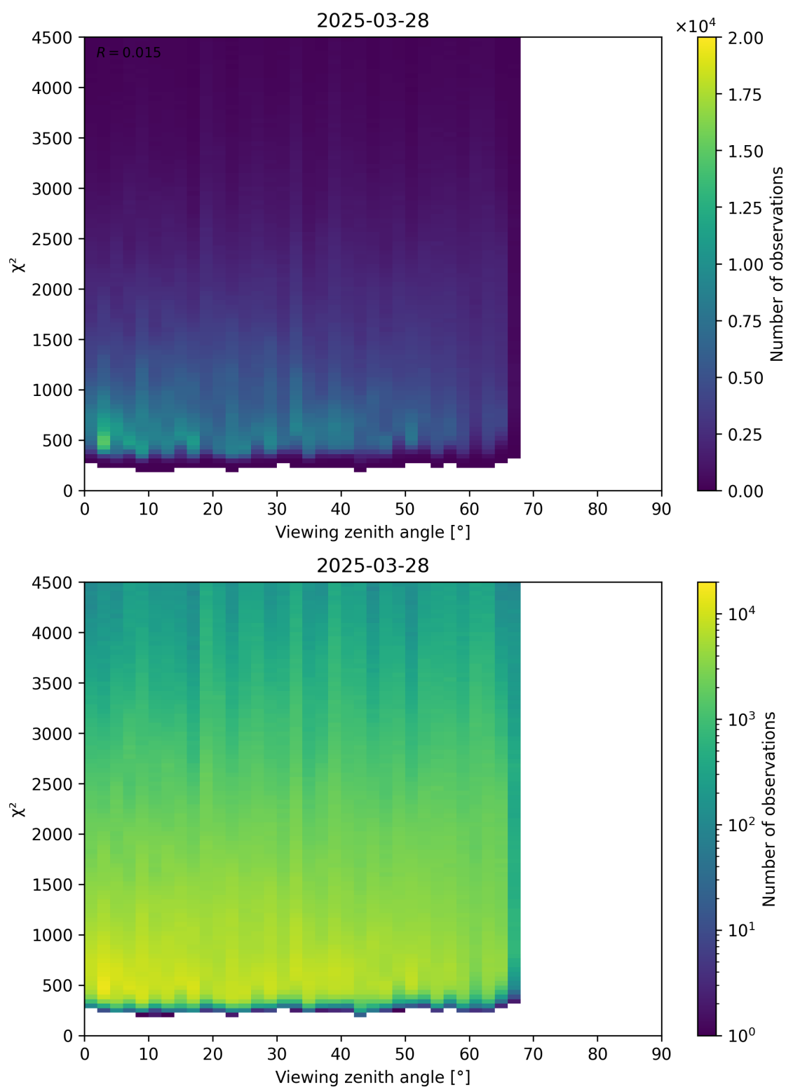
Figure 72: Scatter density plot of “Viewing zenith angle” against “ \chi^2 ” for 2025-03-28 to 2025-03-29.
