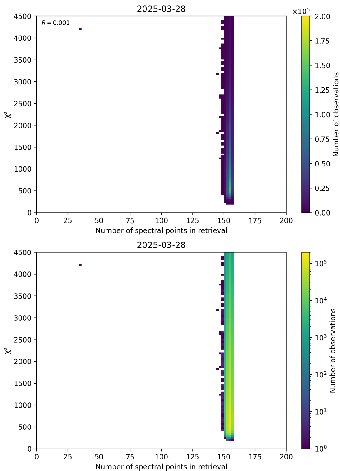
Figure 58: Scatter density plot of “Number of spectral points in retrieval” against “ \chi^2 ” for 2025-03-28 to 2025-03-29.
