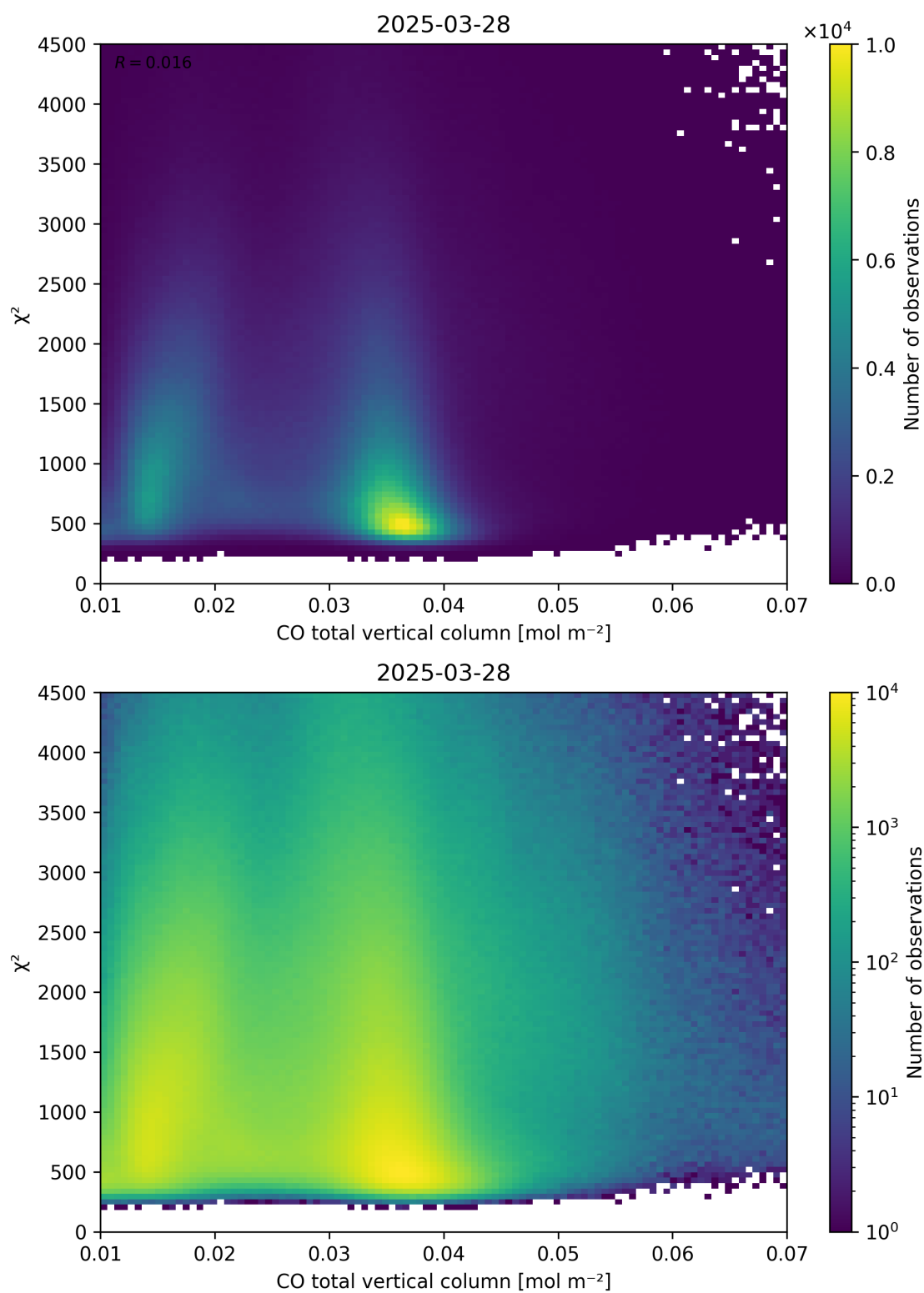
Figure 35: Scatter density plot of “CO total vertical column” against “ \chi^2 ” for 2025-03-28 to 2025-03-29.
