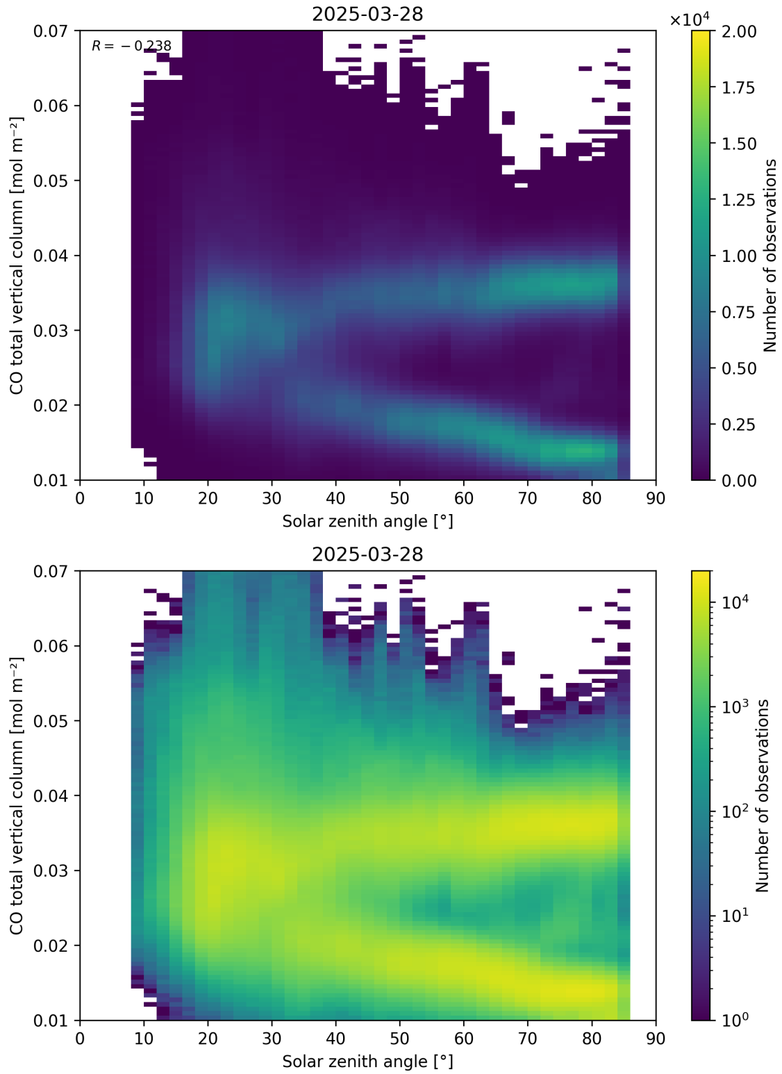
Figure 61: Scatter density plot of “Solar zenith angle” against “CO total vertical column” for 2025-03-28 to 2025-03-29.
