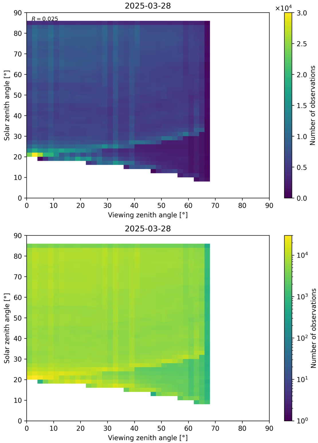
Figure 77: Scatter density plot of “Viewing zenith angle” against “Solar zenith angle” for 2025-03-28 to 2025-03-29.
