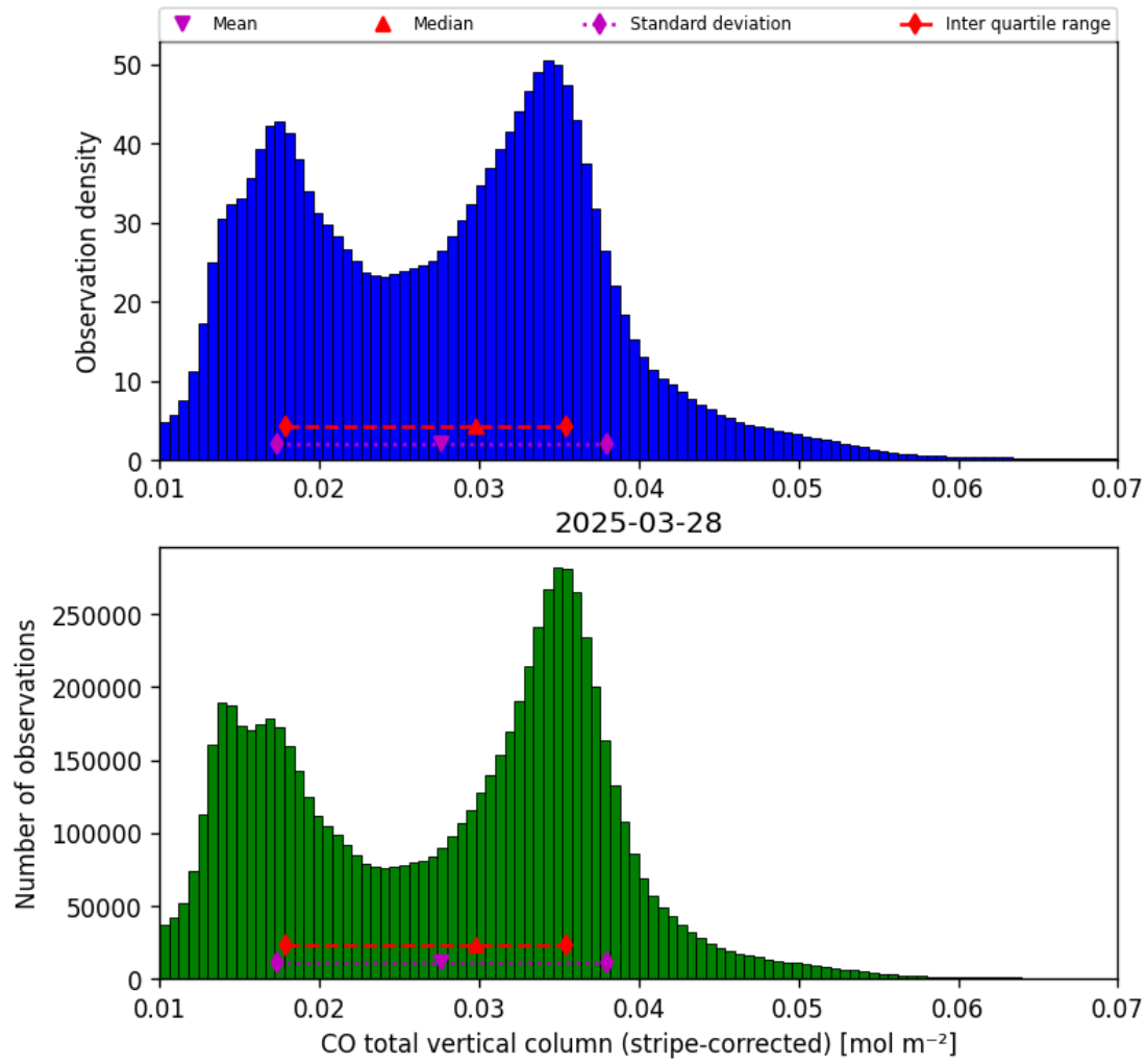
Figure 19: Histogram of “CO total vertical column (stripe-corrected)” for 2025-03-28 to 2025-03-29
