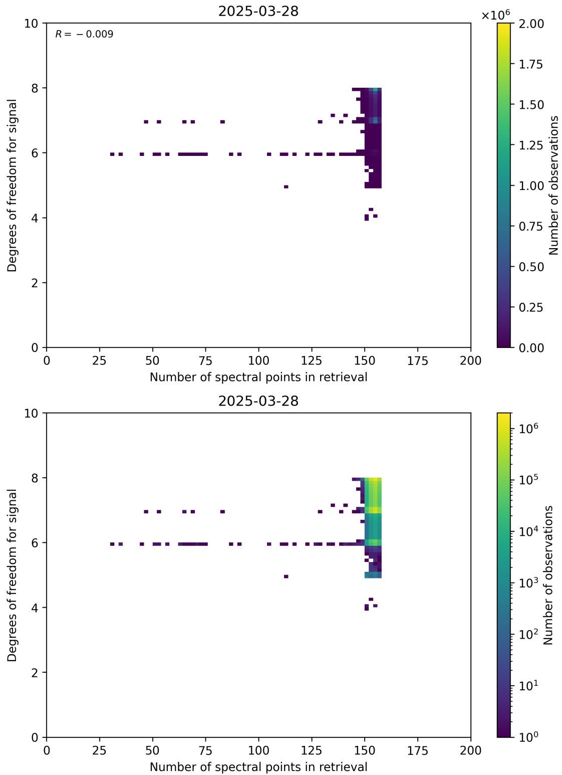
Figure 59: Scatter density plot of “Number of spectral points in retrieval” against “Degrees of freedom for signal” for 2025-03-28 to 2025-03-29.
