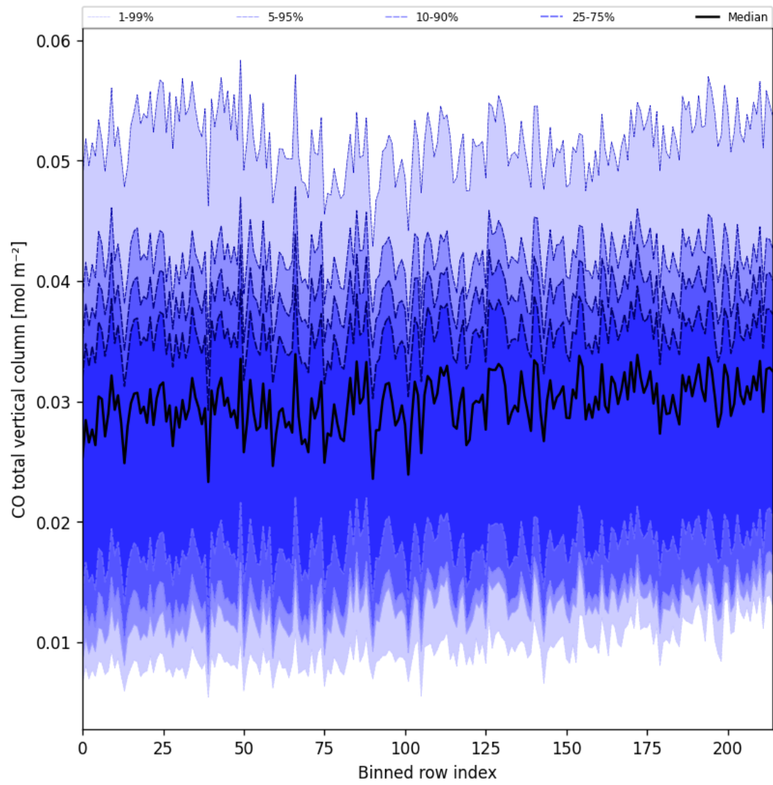
Figure 26: Along track statistics of “CO total vertical column” for 2025-03-28 to 2025-03-29
