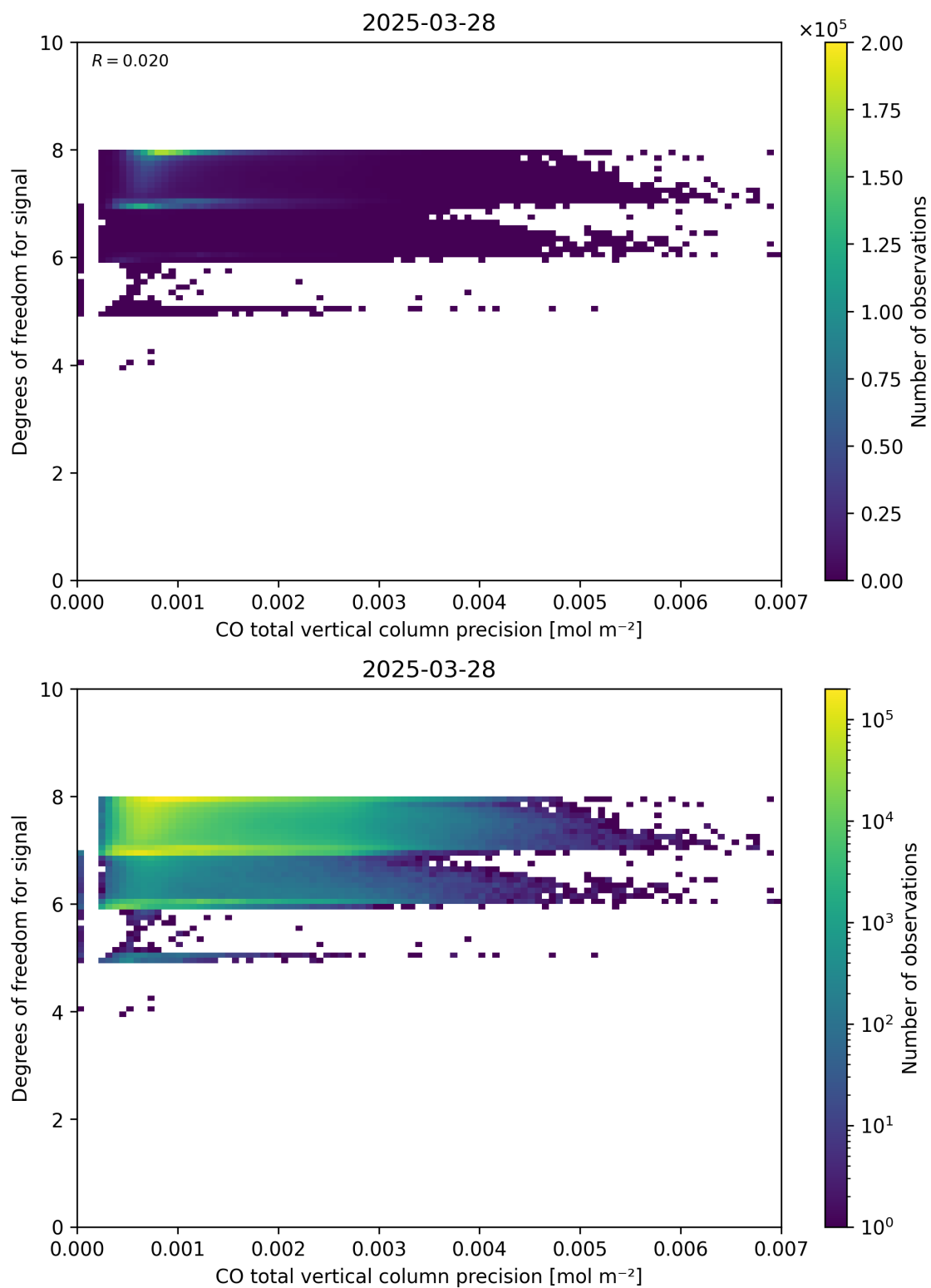
Figure 45: Scatter density plot of “CO total vertical column precision” against “Degrees of freedom for signal” for 2025-03-28 to 2025-03-29.
