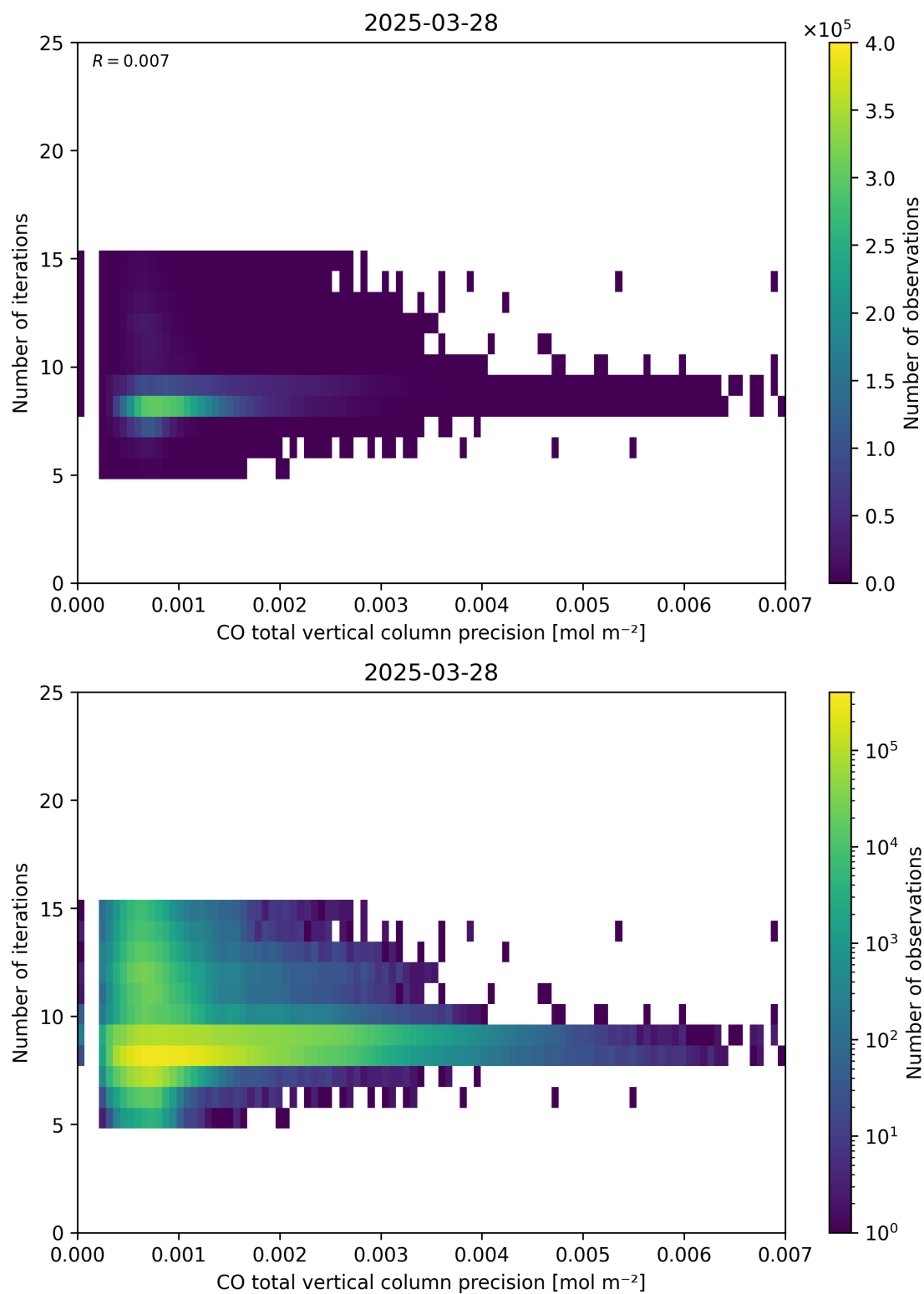
Figure 46: Scatter density plot of “CO total vertical column precision” against “Number of iterations” for 2025-03-28 to 2025-03-29.
