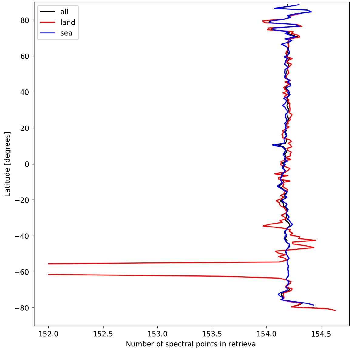
Figure 13: Zonal average of “Number of spectral points in retrieval” for 2025-03-28 to 2025-03-29.
