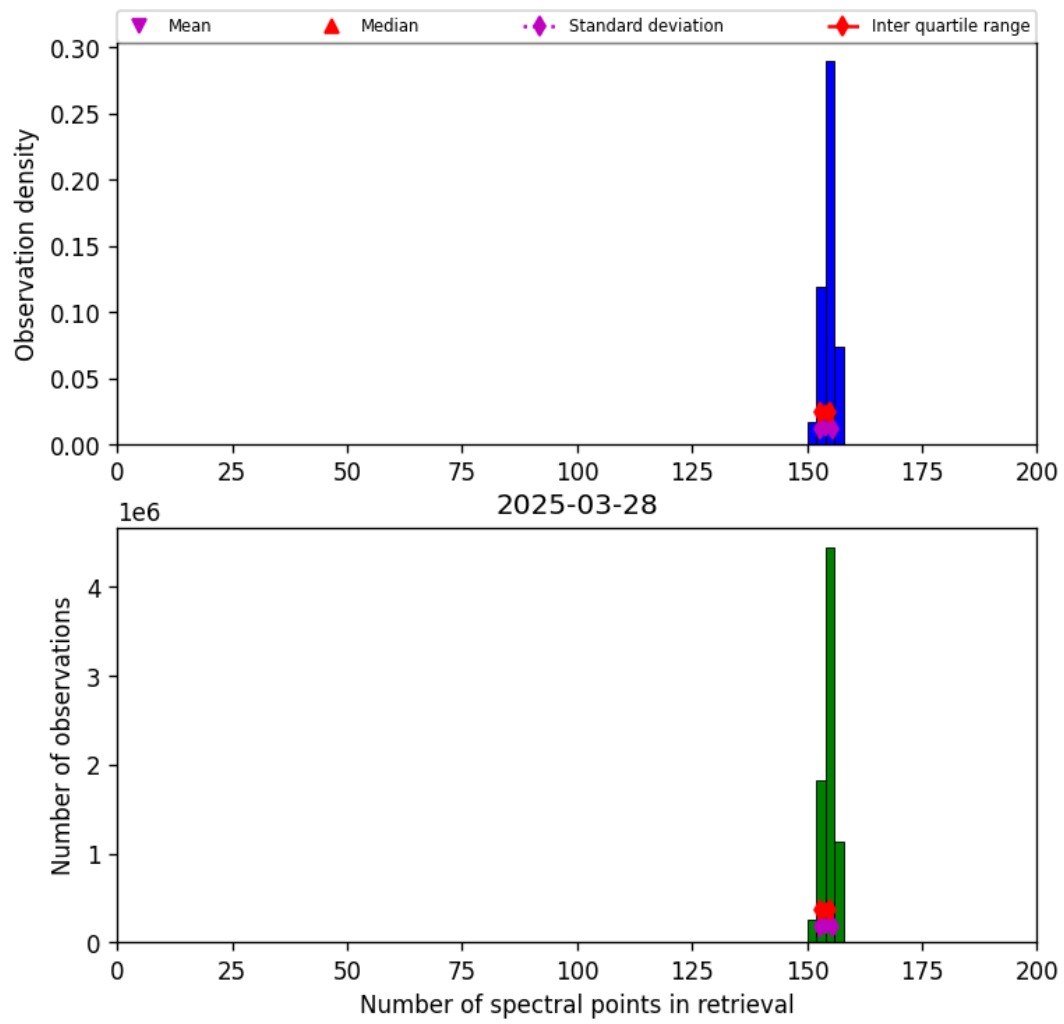
Figure 21: Histogram of “Number of spectral points in retrieval” for 2025-03-28 to 2025-03-29
