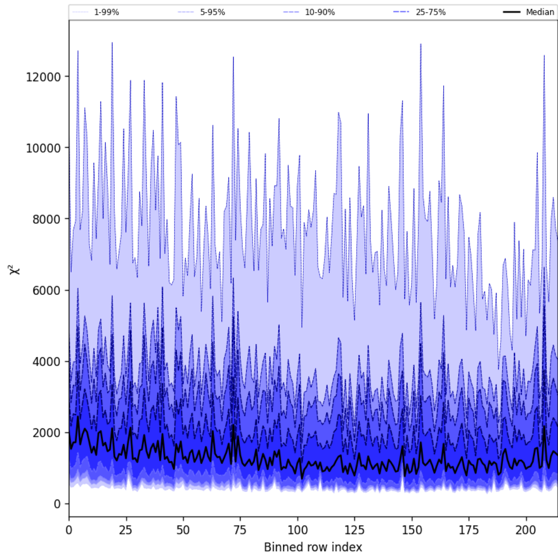
Figure 30: Along track statistics of “ \chi^2 ” for 2025-03-28 to 2025-03-29
