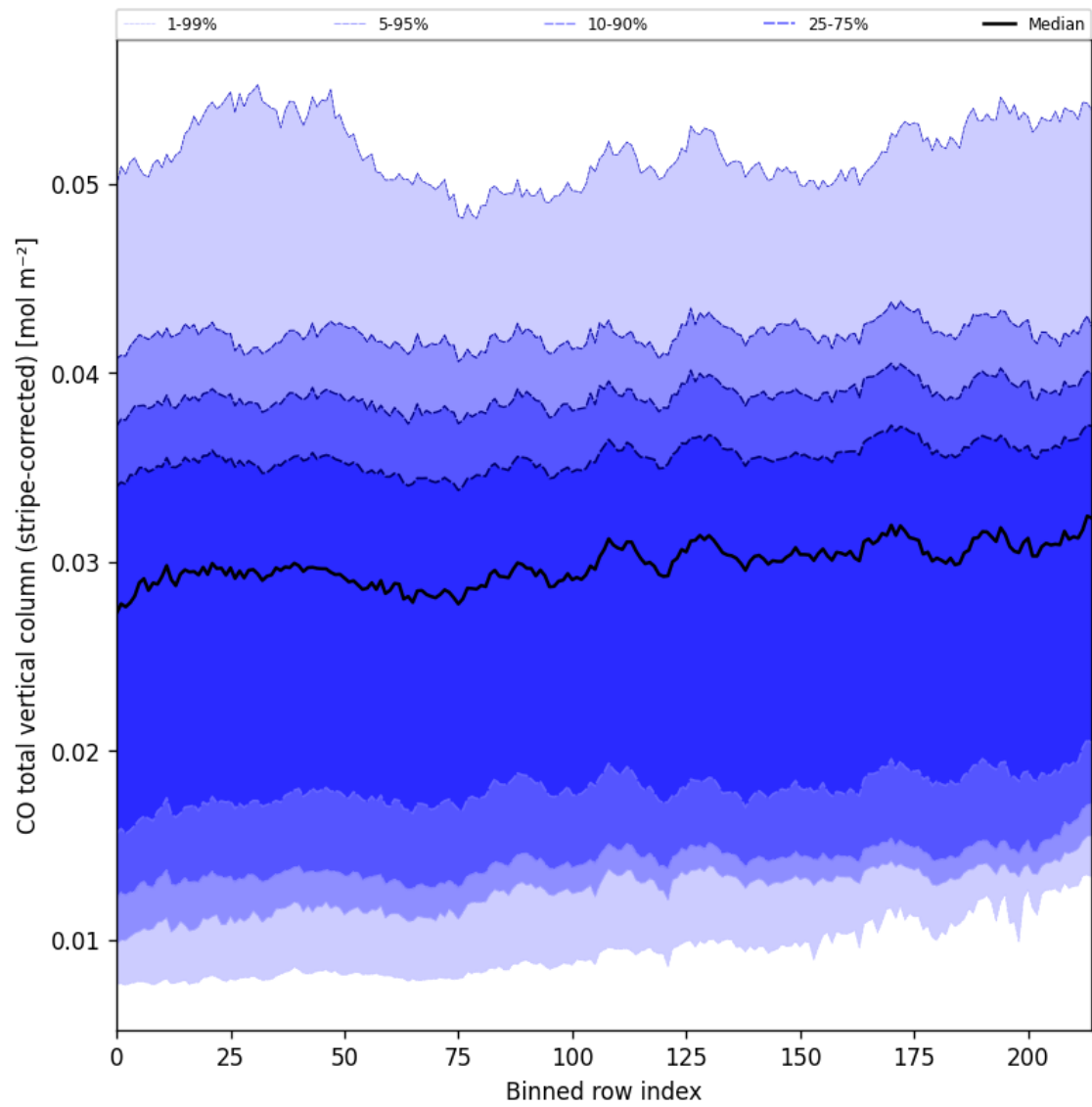
Figure 27: Along track statistics of “CO total vertical column (stripe-corrected)” for 2025-03-28 to 2025-03-29
