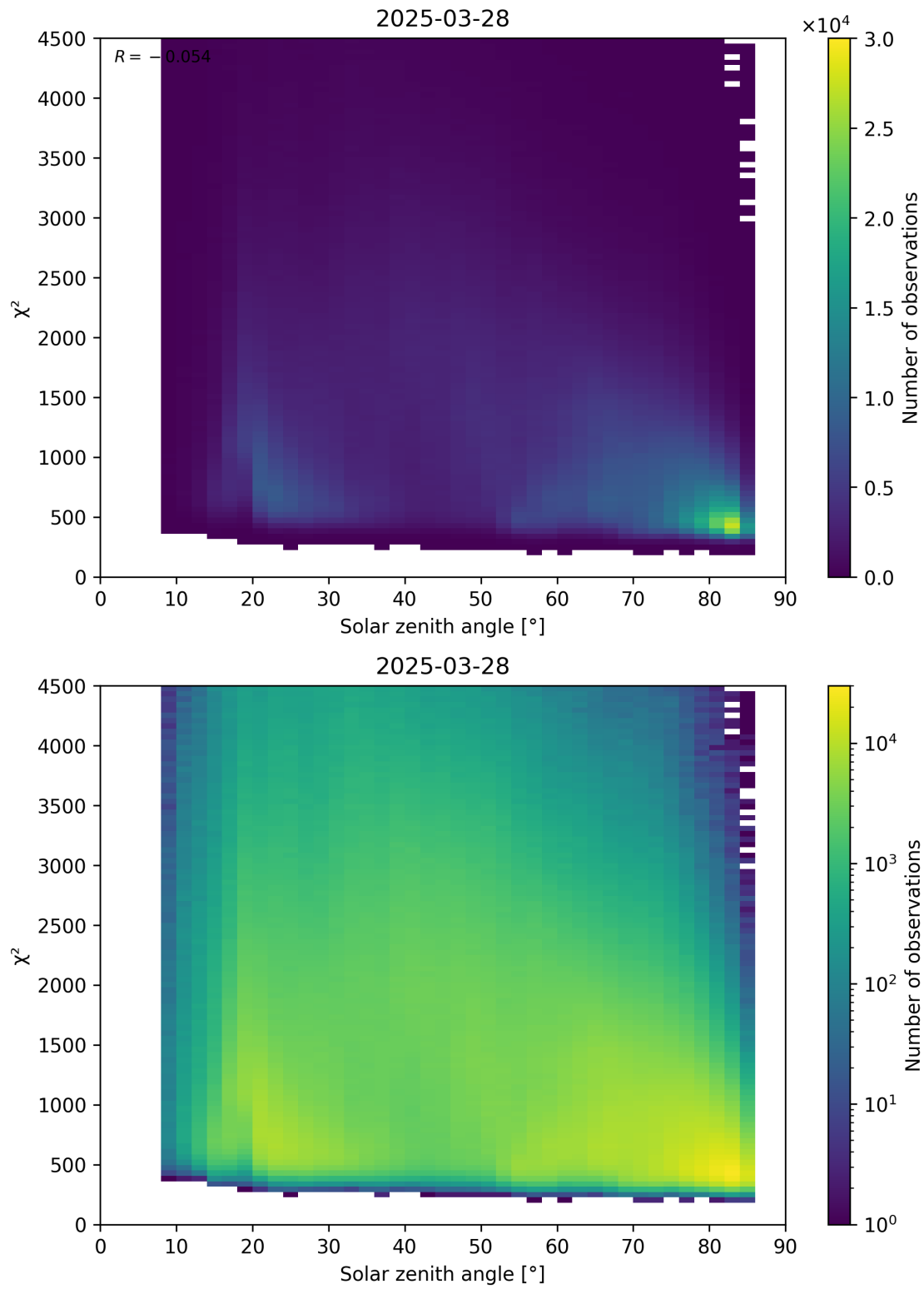
Figure 64: Scatter density plot of “Solar zenith angle” against “ \chi^2 ” for 2025-03-28 to 2025-03-29.
