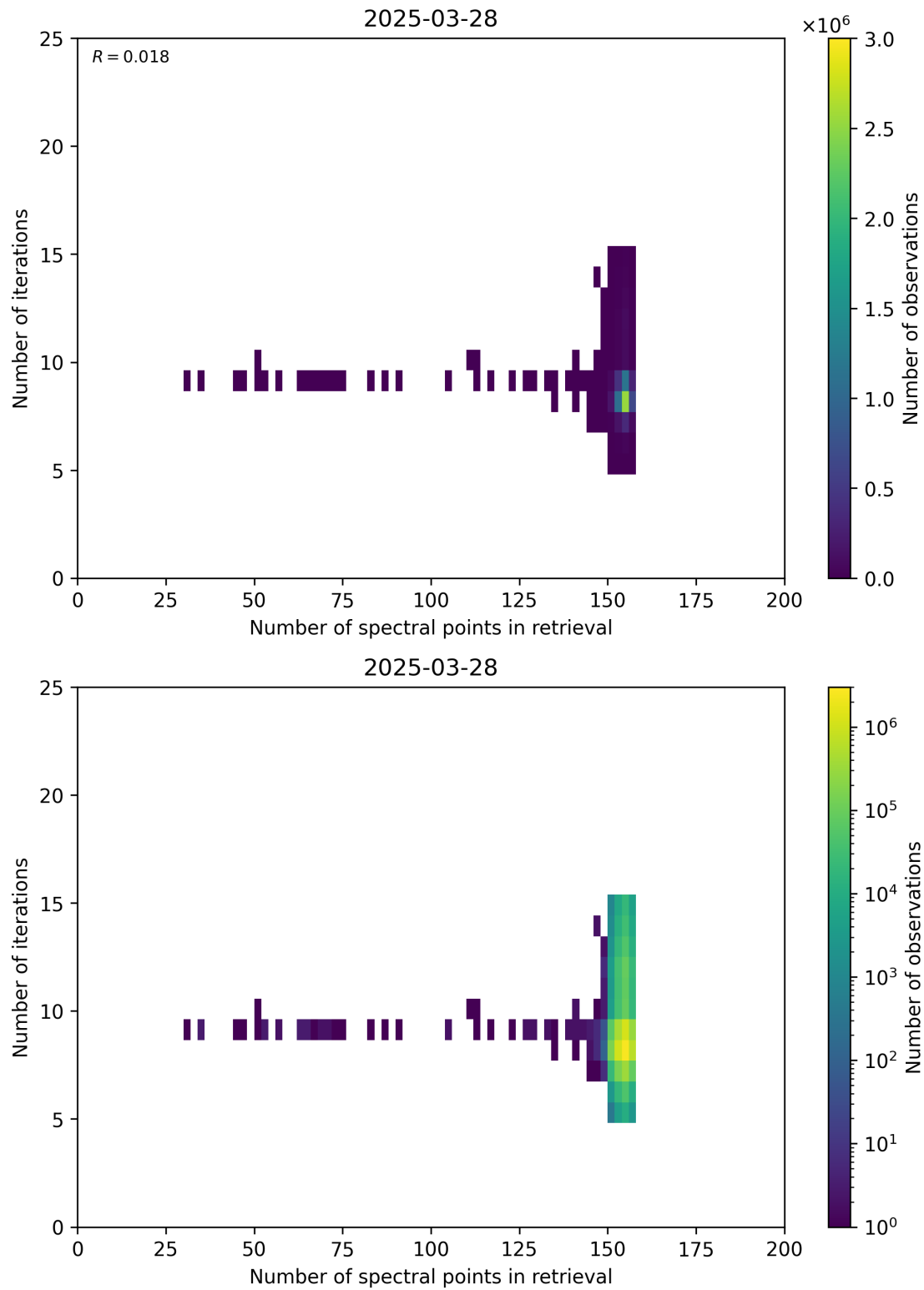
Figure 60: Scatter density plot of “Number of spectral points in retrieval” against “Number of iterations” for 2025-03-28 to 2025-03-29.
