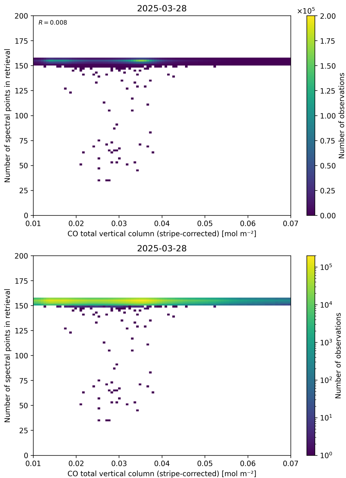
Figure 40: Scatter density plot of “CO total vertical column (stripe-corrected)” against “Number of spectral points in retrieval” for 2025-03-28 to 2025-03-29.
