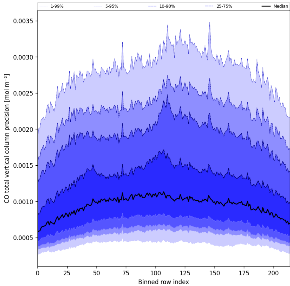
Figure 28: Along track statistics of “CO total vertical column precision” for 2025-03-28 to 2025-03-29
