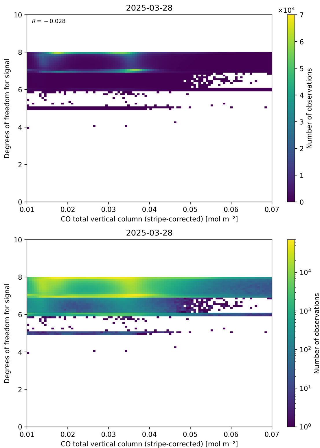
Figure 38: Scatter density plot of “CO total vertical column (stripe-corrected)” against “Degrees of freedom for signal” for 2025-03-28 to 2025-03-29.
