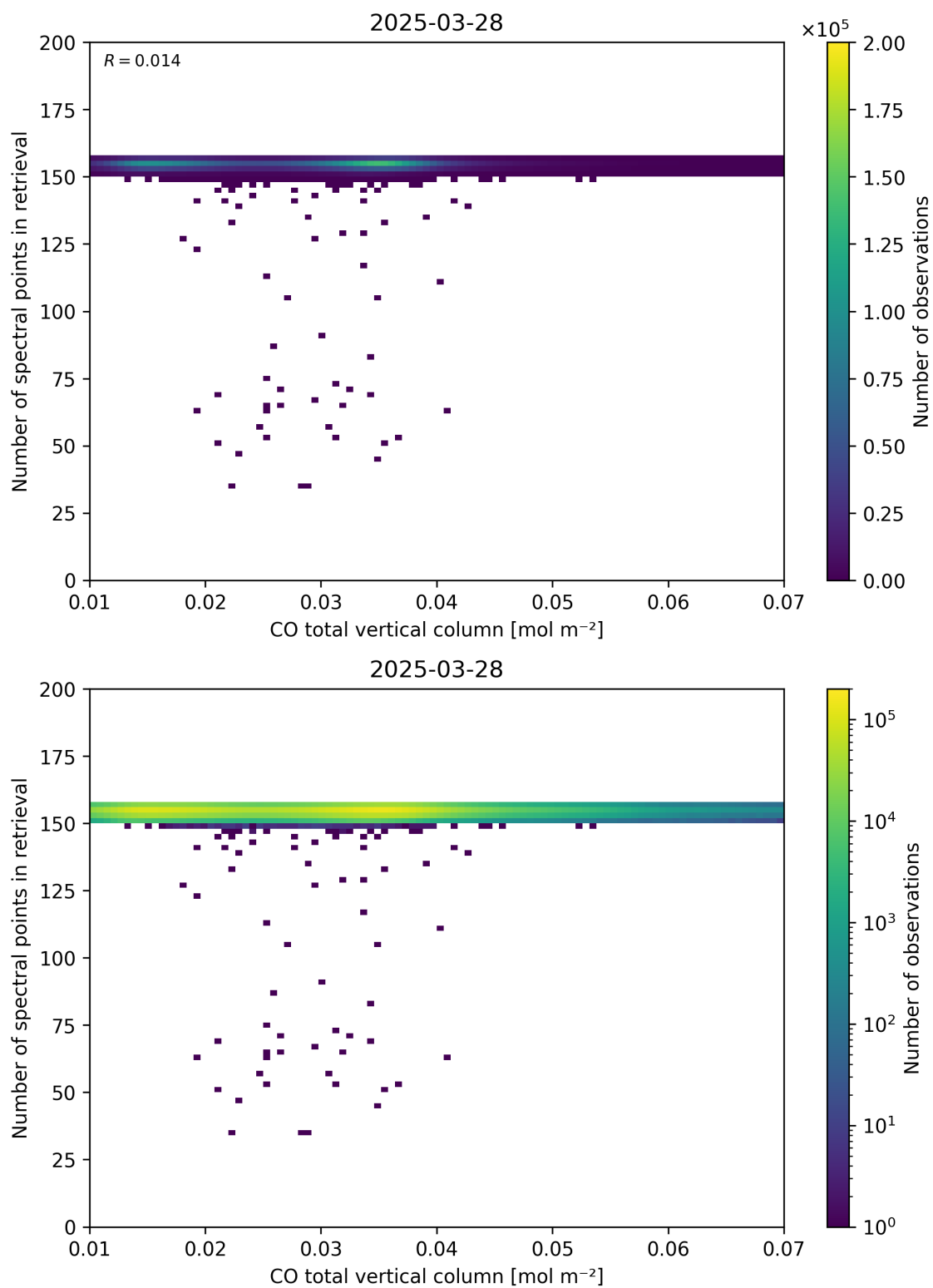
Figure 43: Scatter density plot of “CO total vertical column” against “Number of spectral points in retrieval” for 2025-03-28 to 2025-03-29.
