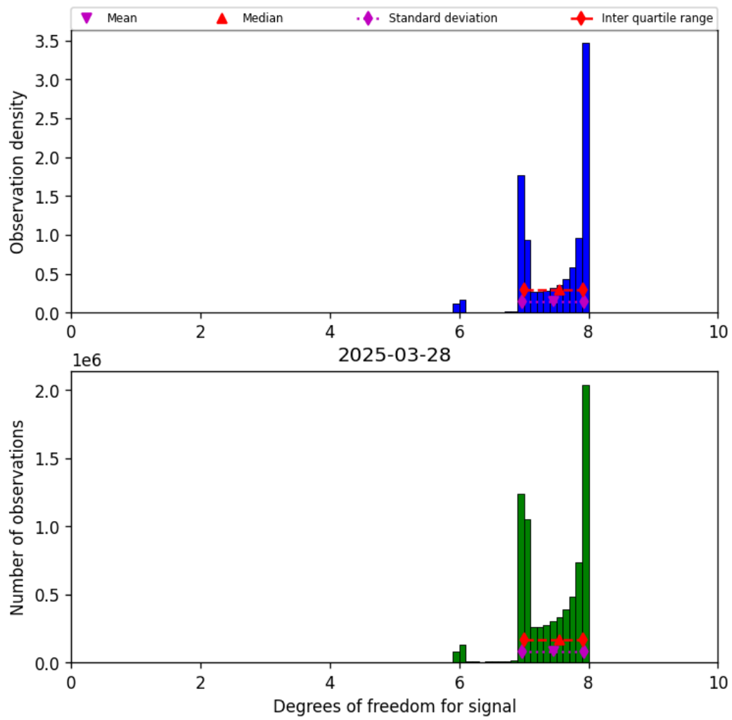
Figure 23: Histogram of “Degrees of freedom for signal” for 2025-03-28 to 2025-03-29
