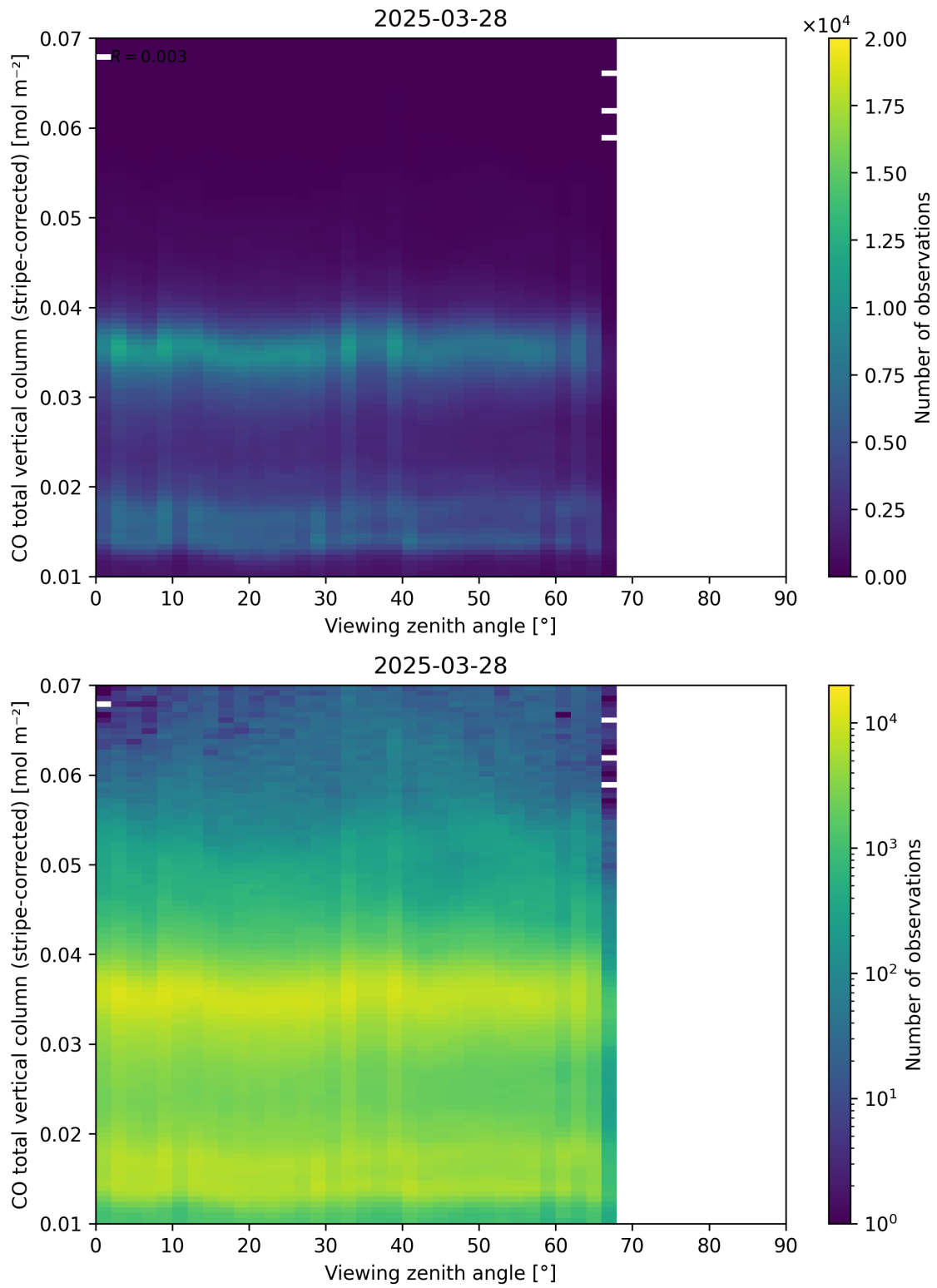
Figure 70: Scatter density plot of “Viewing zenith angle” against “CO total vertical column (stripe-corrected)” for 2025-03-28 to 2025-03-29.
