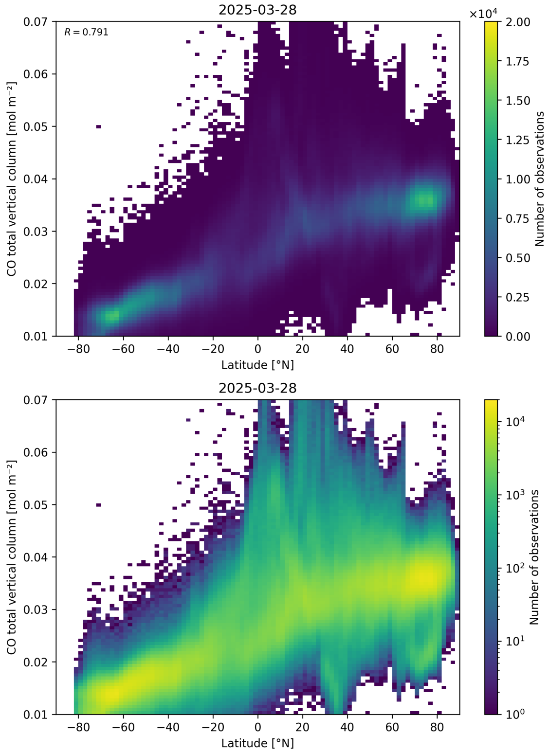
Figure 51: Scatter density plot of “Latitude” against “CO total vertical column” for 2025-03-28 to 2025-03-29.
