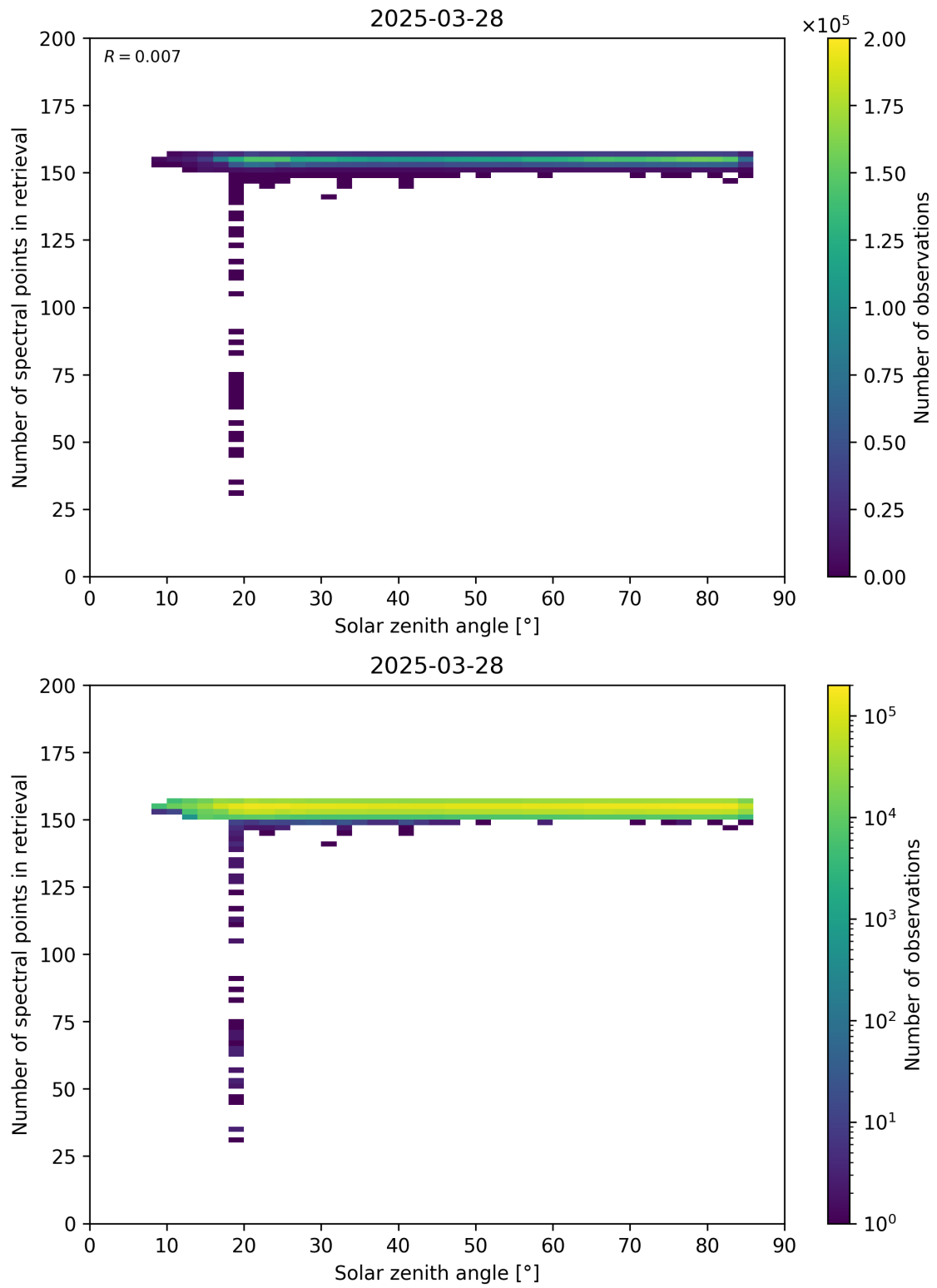
Figure 68: Scatter density plot of “Solar zenith angle” against “Number of spectral points in retrieval” for 2025-03-28 to 2025-03-29.
