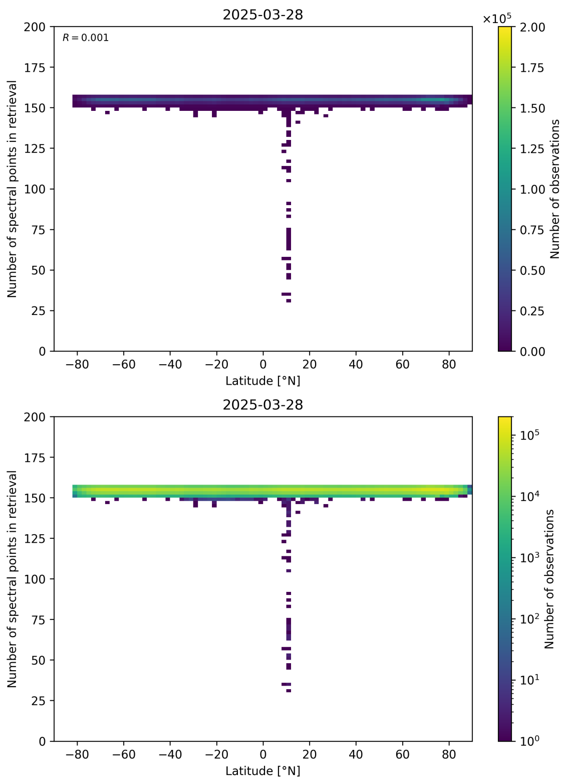
Figure 57: Scatter density plot of “Latitude” against “Number of spectral points in retrieval” for 2025-03-28 to 2025-03-29.
