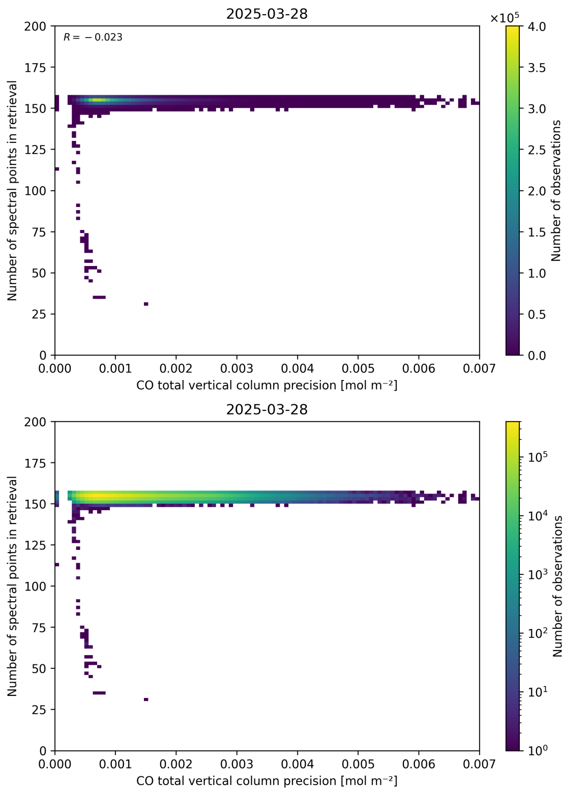
Figure 47: Scatter density plot of “CO total vertical column precision” against “Number of spectral points in retrieval” for 2025-03-28 to 2025-03-29.
