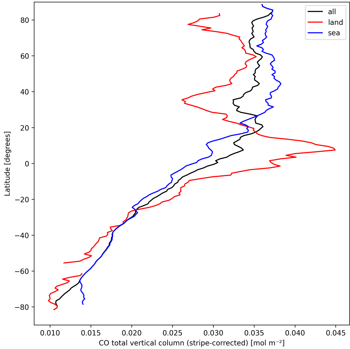
Figure 11: Zonal average of “CO total vertical column (stripe-corrected)” for 2025-03-28 to 2025-03-29.
