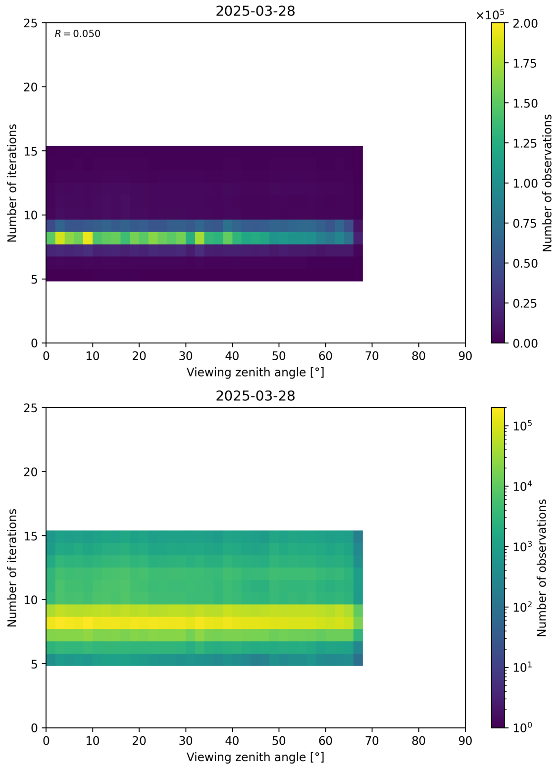
Figure 75: Scatter density plot of “Viewing zenith angle” against “Number of iterations” for 2025-03-28 to 2025-03-29.
