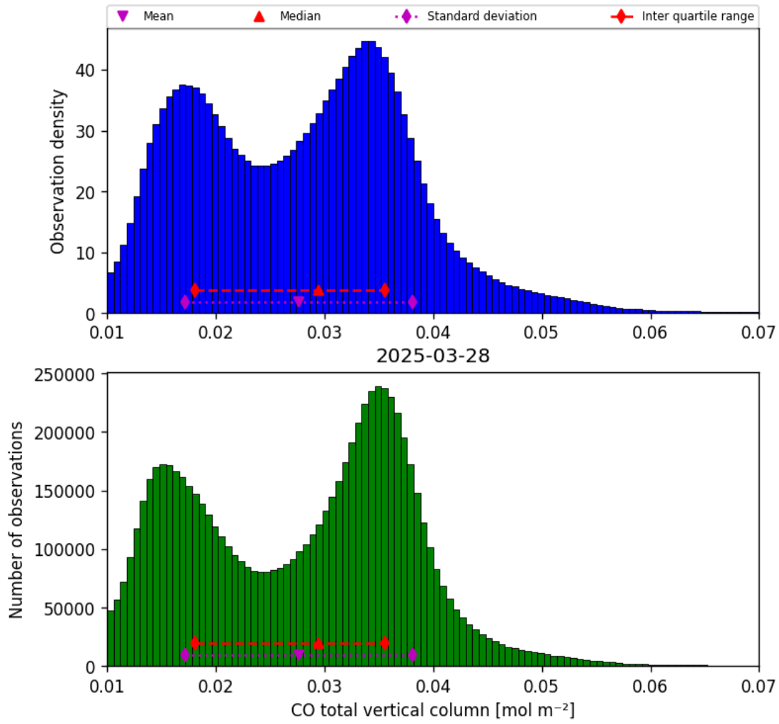
Figure 18: Histogram of “CO total vertical column” for 2025-03-28 to 2025-03-29
