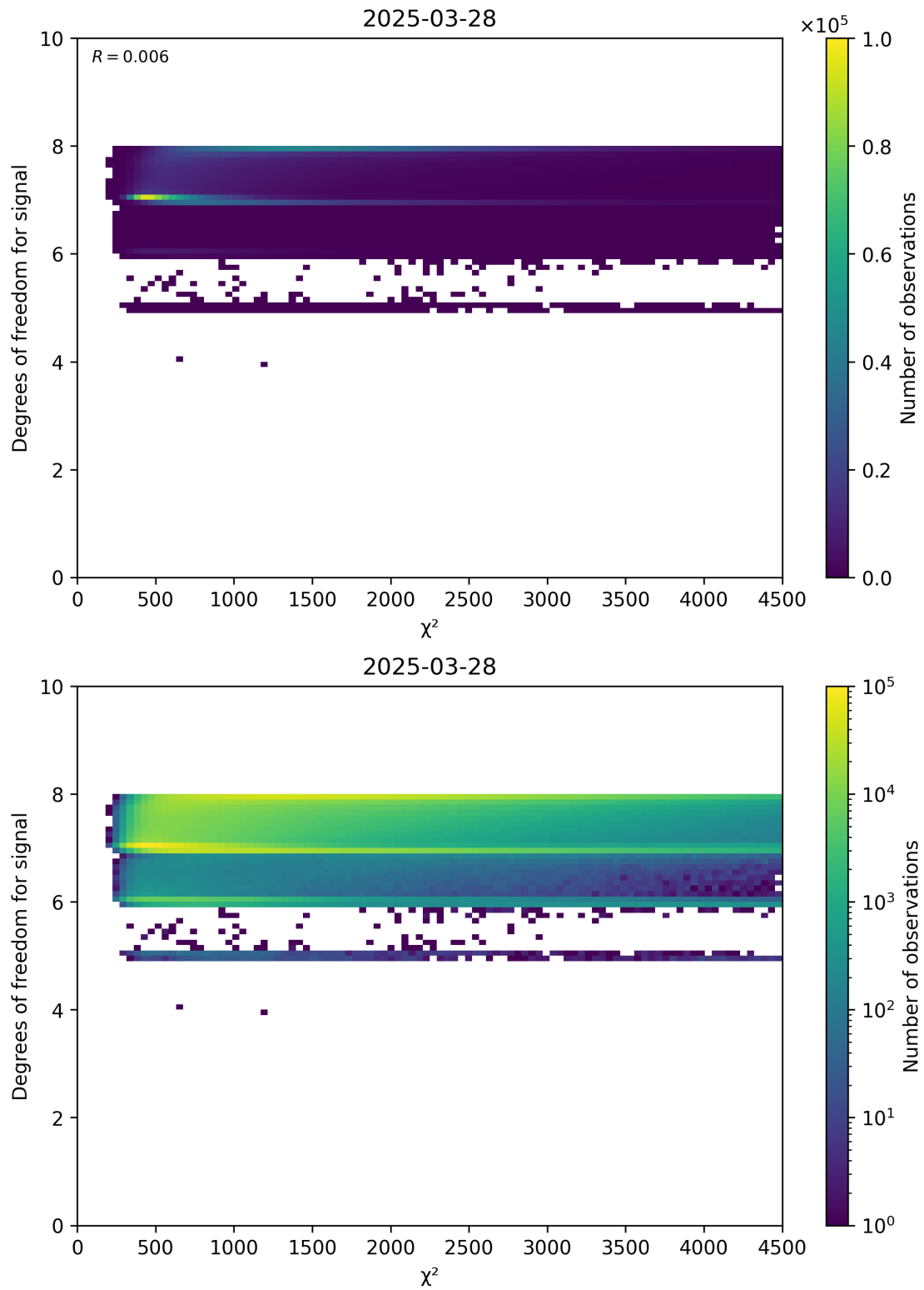
Figure 48: Scatter density plot of “ \chi^2 ” against “Degrees of freedom for signal” for 2025-03-28 to 2025-03-29.
