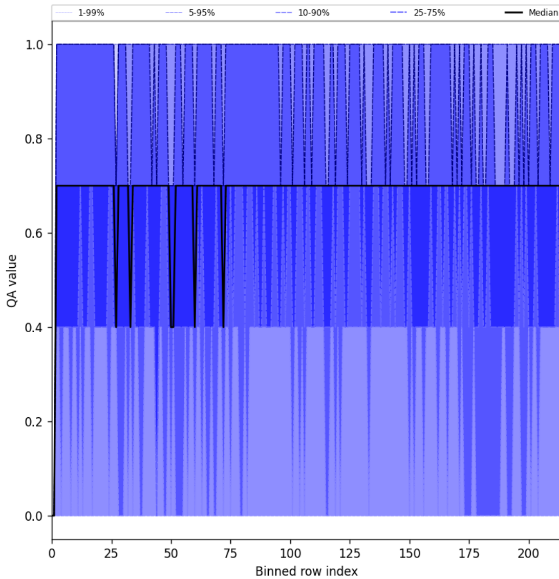
Figure 25: Along track statistics of “QA value” for 2025-03-28 to 2025-03-29
