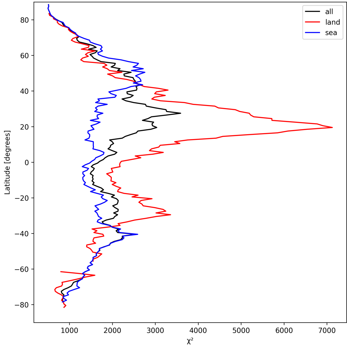
Figure 14: Zonal average of “ \chi^2 ” for 2025-03-28 to 2025-03-29.
