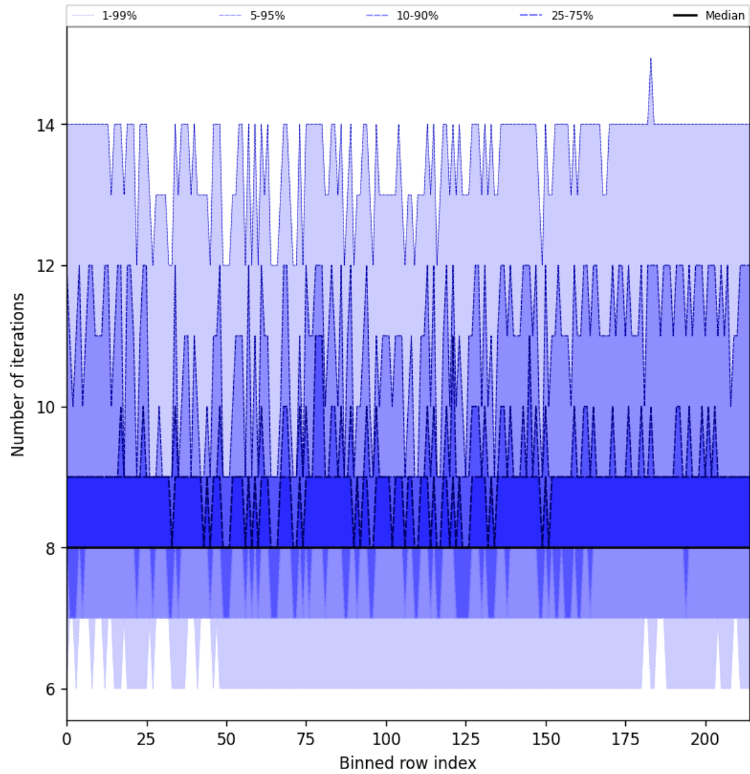
Figure 32: Along track statistics of “Number of iterations” for 2025-03-28 to 2025-03-29
