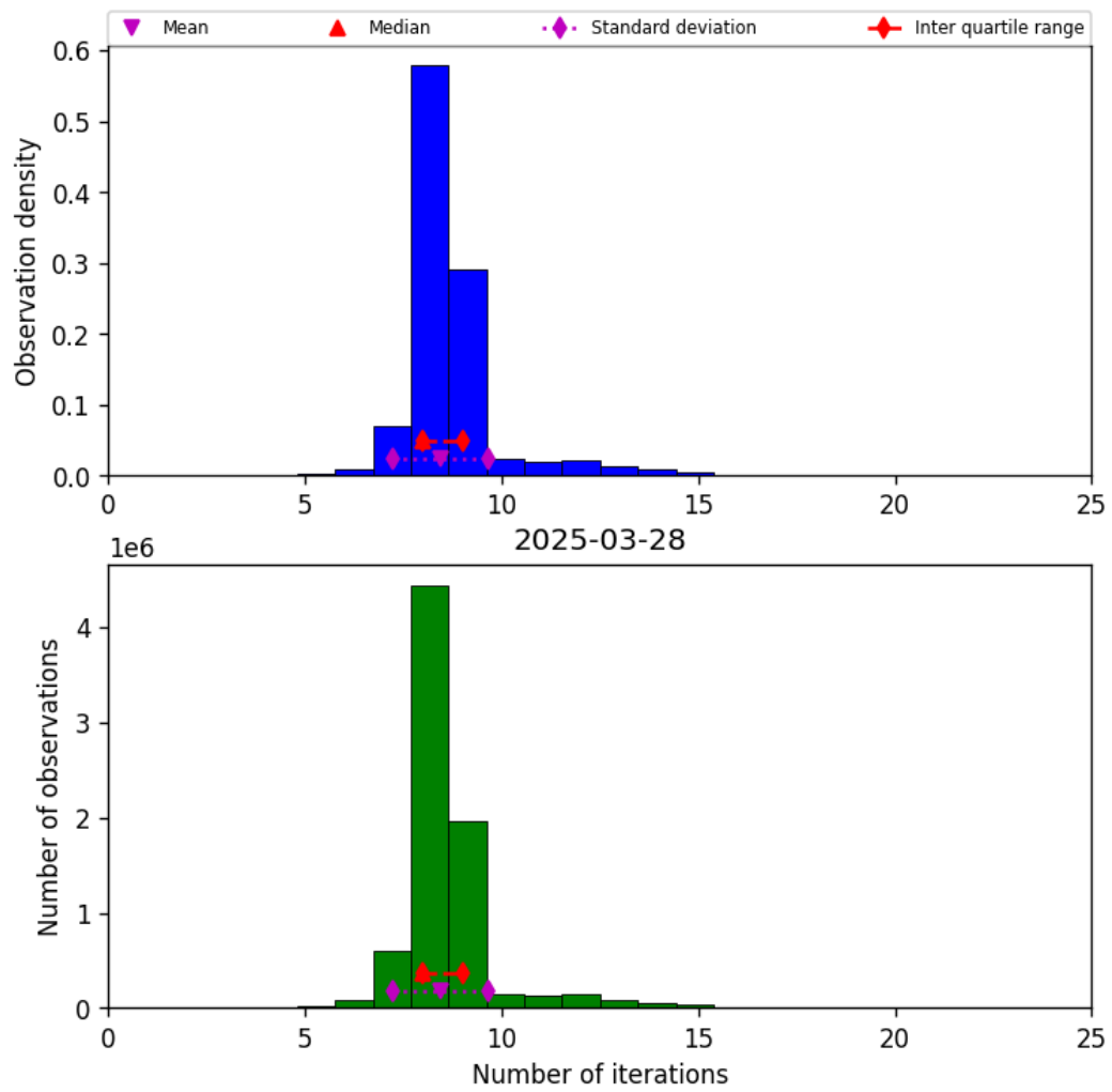
Figure 24: Histogram of “Number of iterations” for 2025-03-28 to 2025-03-29
