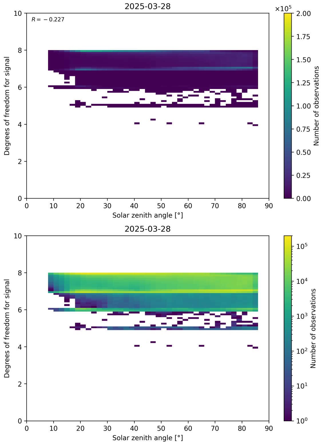
Figure 65: Scatter density plot of “Solar zenith angle” against “Degrees of freedom for signal” for 2025-03-28 to 2025-03-29.
