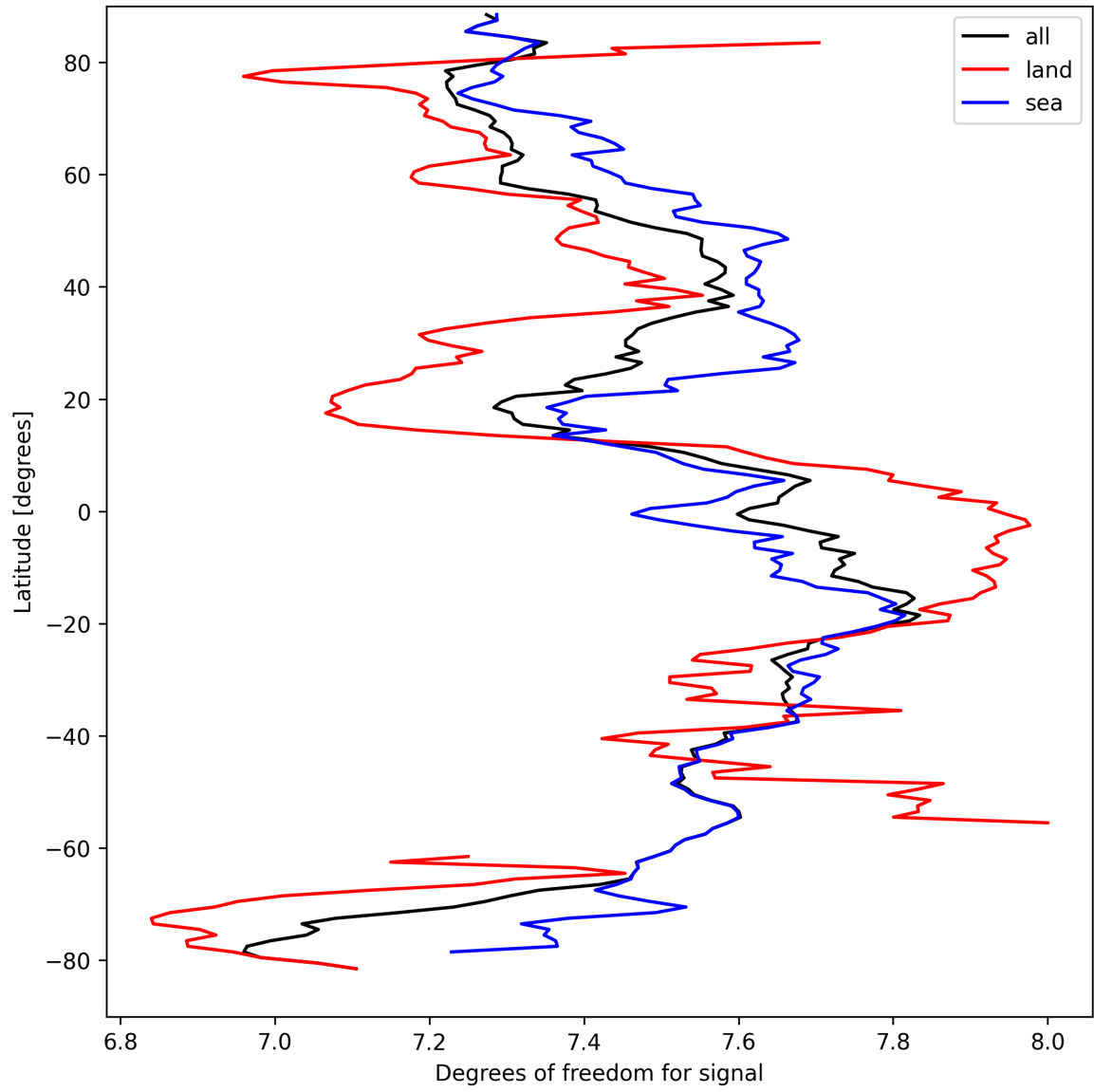
Figure 15: Zonal average of “Degrees of freedom for signal” for 2025-03-28 to 2025-03-29.
