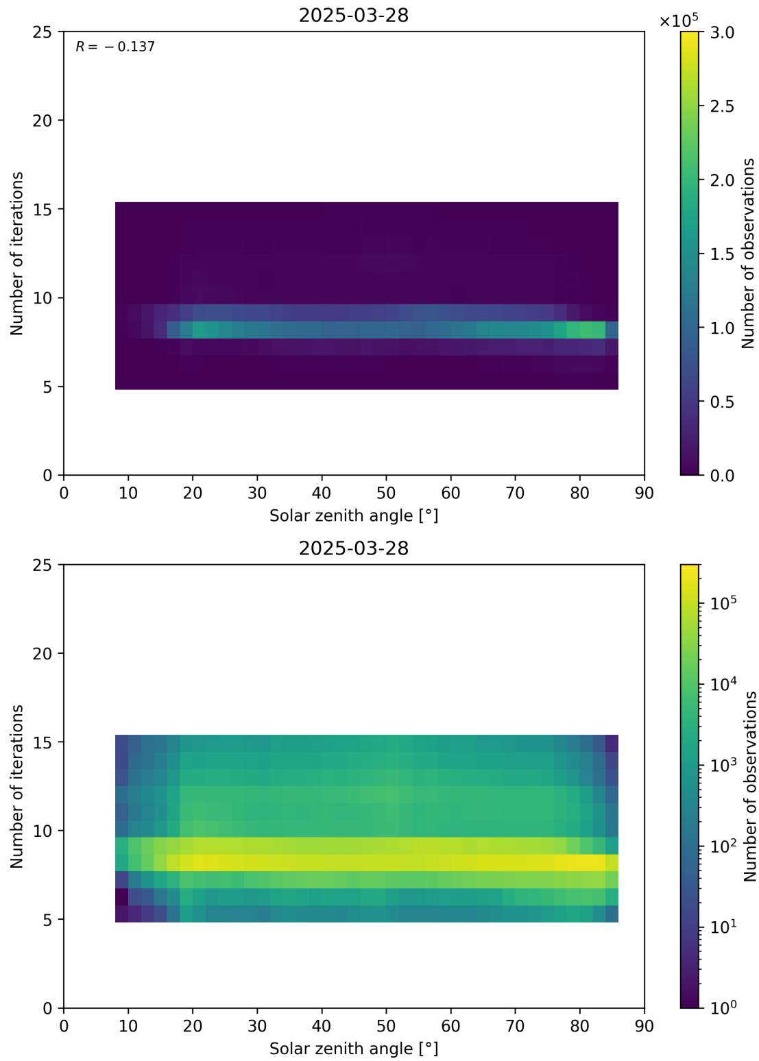
Figure 67: Scatter density plot of “Solar zenith angle” against “Number of iterations” for 2025-03-28 to 2025-03-29.
