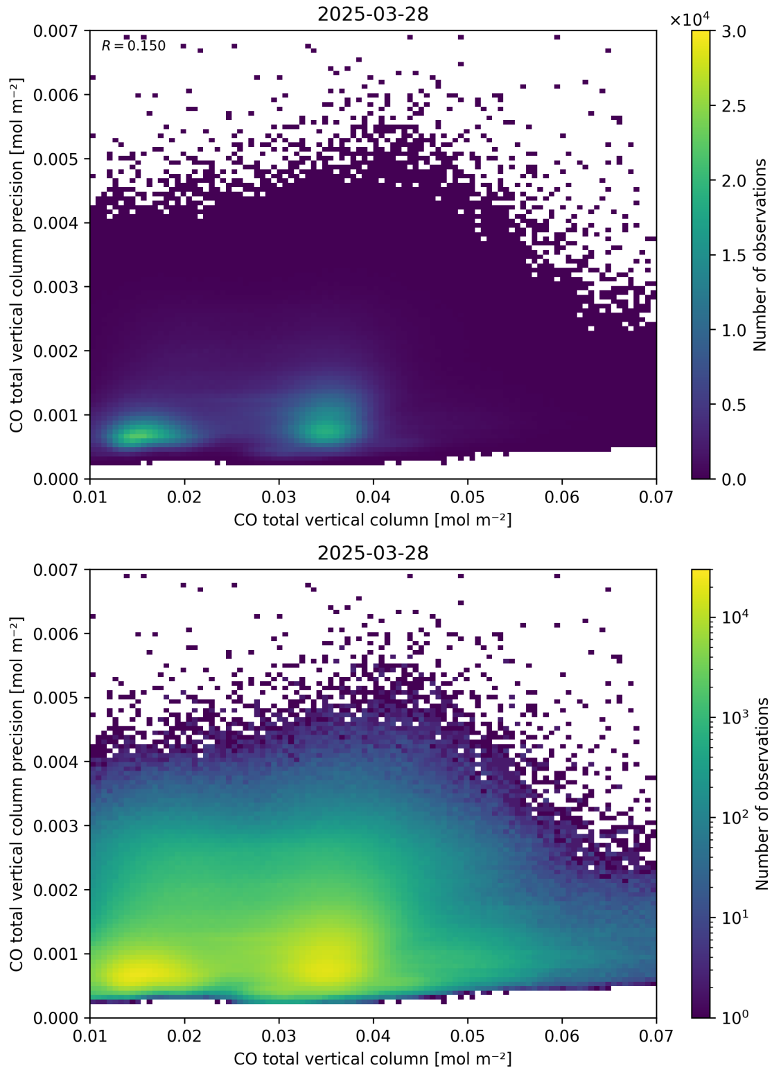
Figure 34: Scatter density plot of “CO total vertical column” against “CO total vertical column precision” for 2025-03-28 to 2025-03-29.
