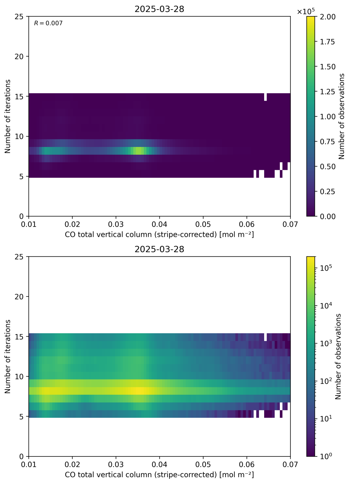
Figure 39: Scatter density plot of “CO total vertical column (stripe-corrected)” against “Number of iterations” for 2025-03-28 to 2025-03-29.
