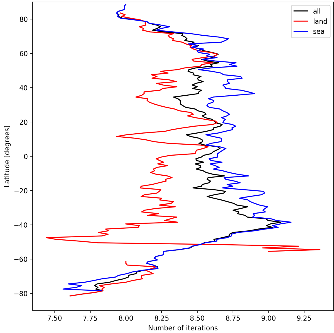
Figure 16: Zonal average of “Number of iterations” for 2025-03-28 to 2025-03-29.
