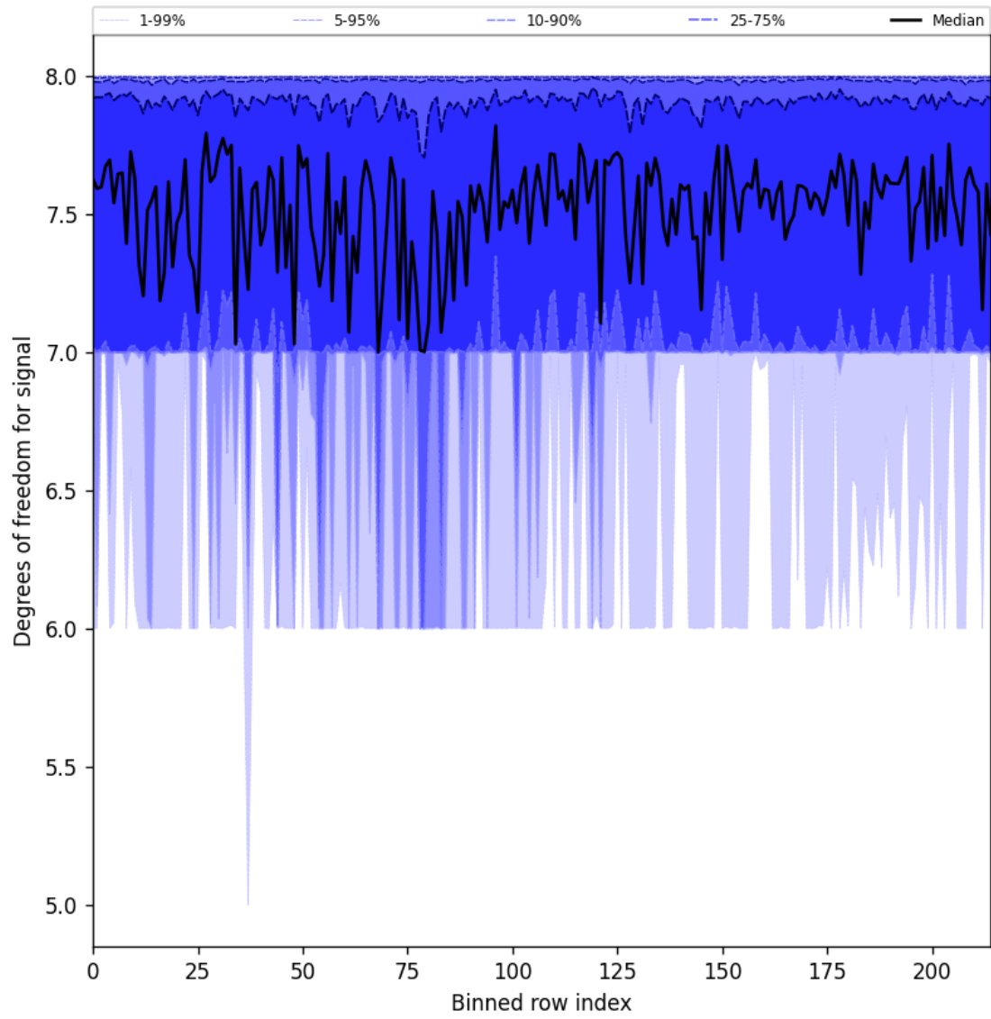
Figure 31: Along track statistics of “Degrees of freedom for signal” for 2025-03-28 to 2025-03-29
