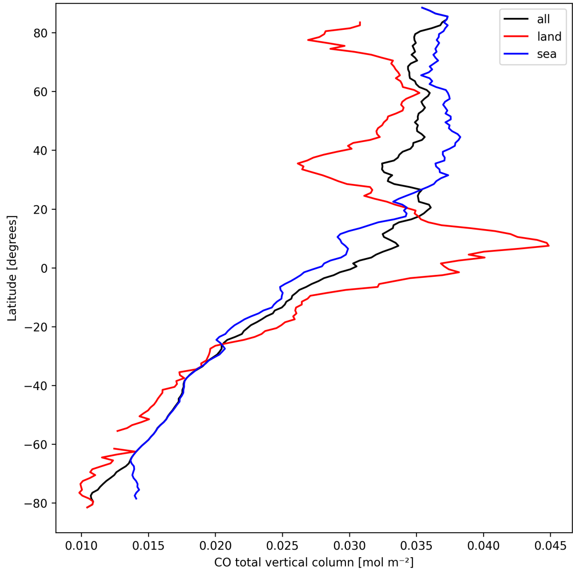
Figure 10: Zonal average of “CO total vertical column” for 2025-03-28 to 2025-03-29.
