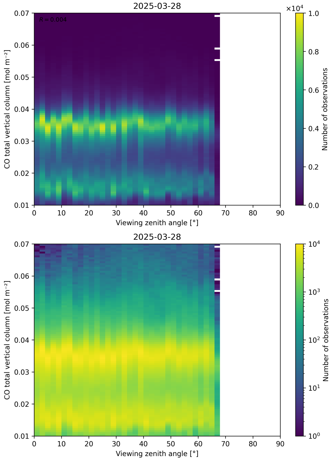
Figure 69: Scatter density plot of “Viewing zenith angle” against “CO total vertical column” for 2025-03-28 to 2025-03-29.
