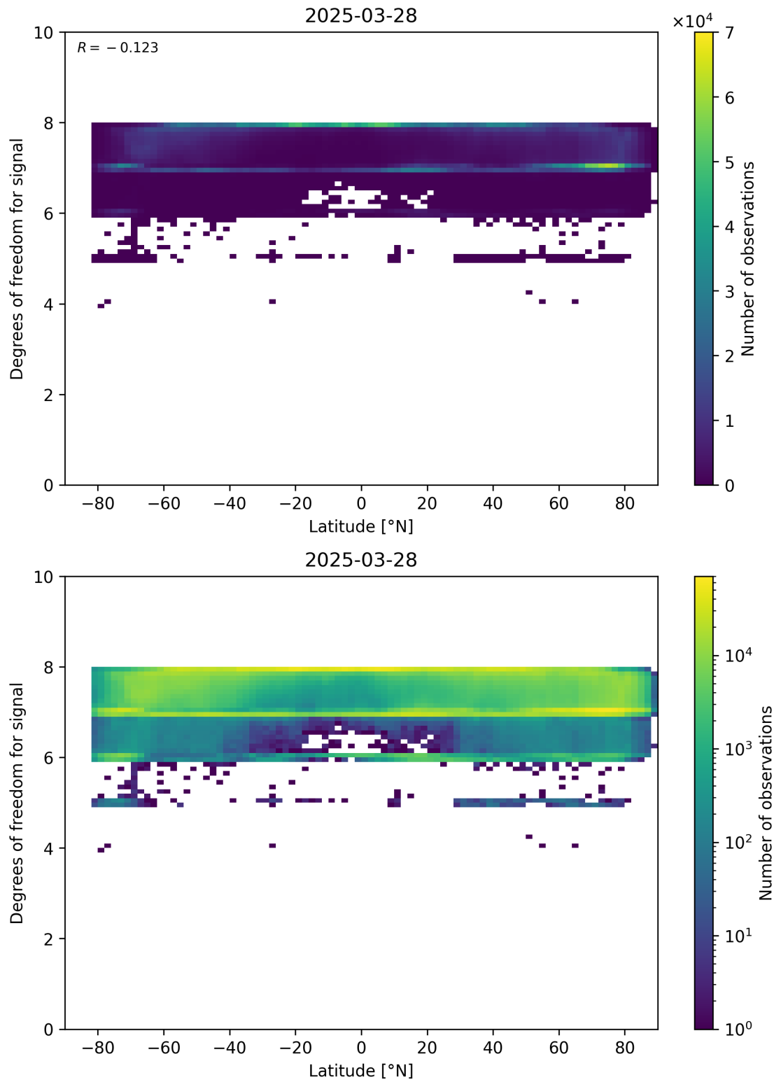
Figure 55: Scatter density plot of “Latitude” against “Degrees of freedom for signal” for 2025-03-28 to 2025-03-29.
