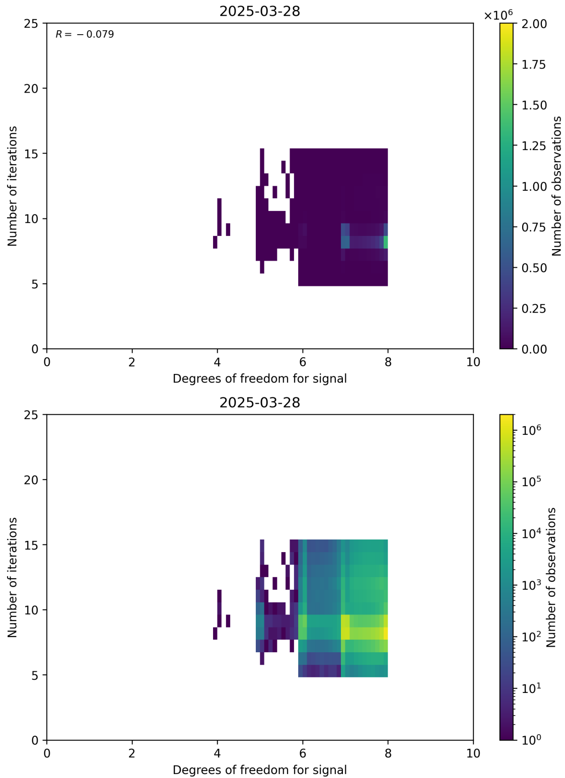
Figure 50: Scatter density plot of “Degrees of freedom for signal” against “Number of iterations” for 2025-03-28 to 2025-03-29.
