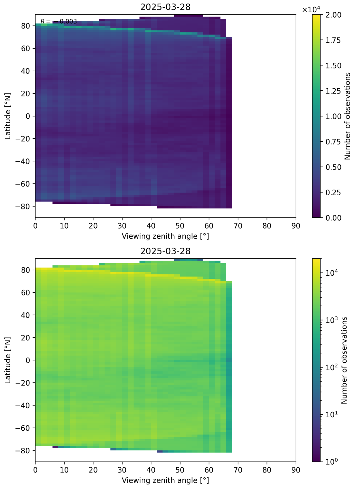
Figure 74: Scatter density plot of “Viewing zenith angle” against “Latitude” for 2025-03-28 to 2025-03-29.
