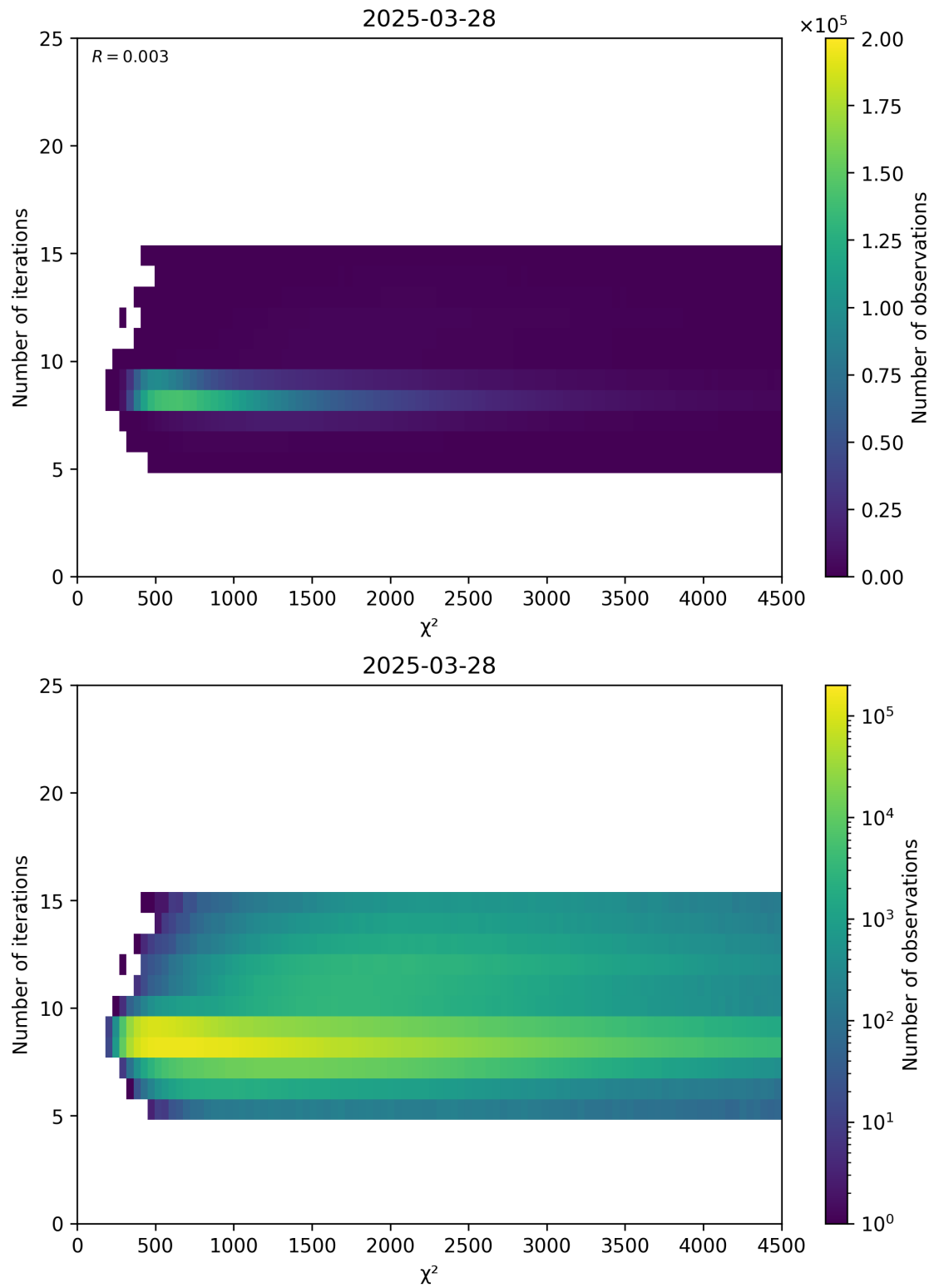
Figure 49: Scatter density plot of “ \chi^2 ” against “Number of iterations” for 2025-03-28 to 2025-03-29.
