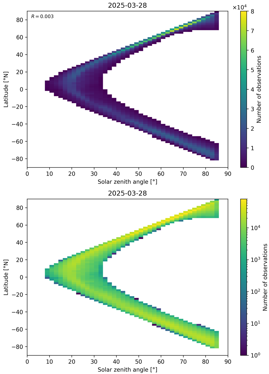
Figure 66: Scatter density plot of “Solar zenith angle” against “Latitude” for 2025-03-28 to 2025-03-29.
