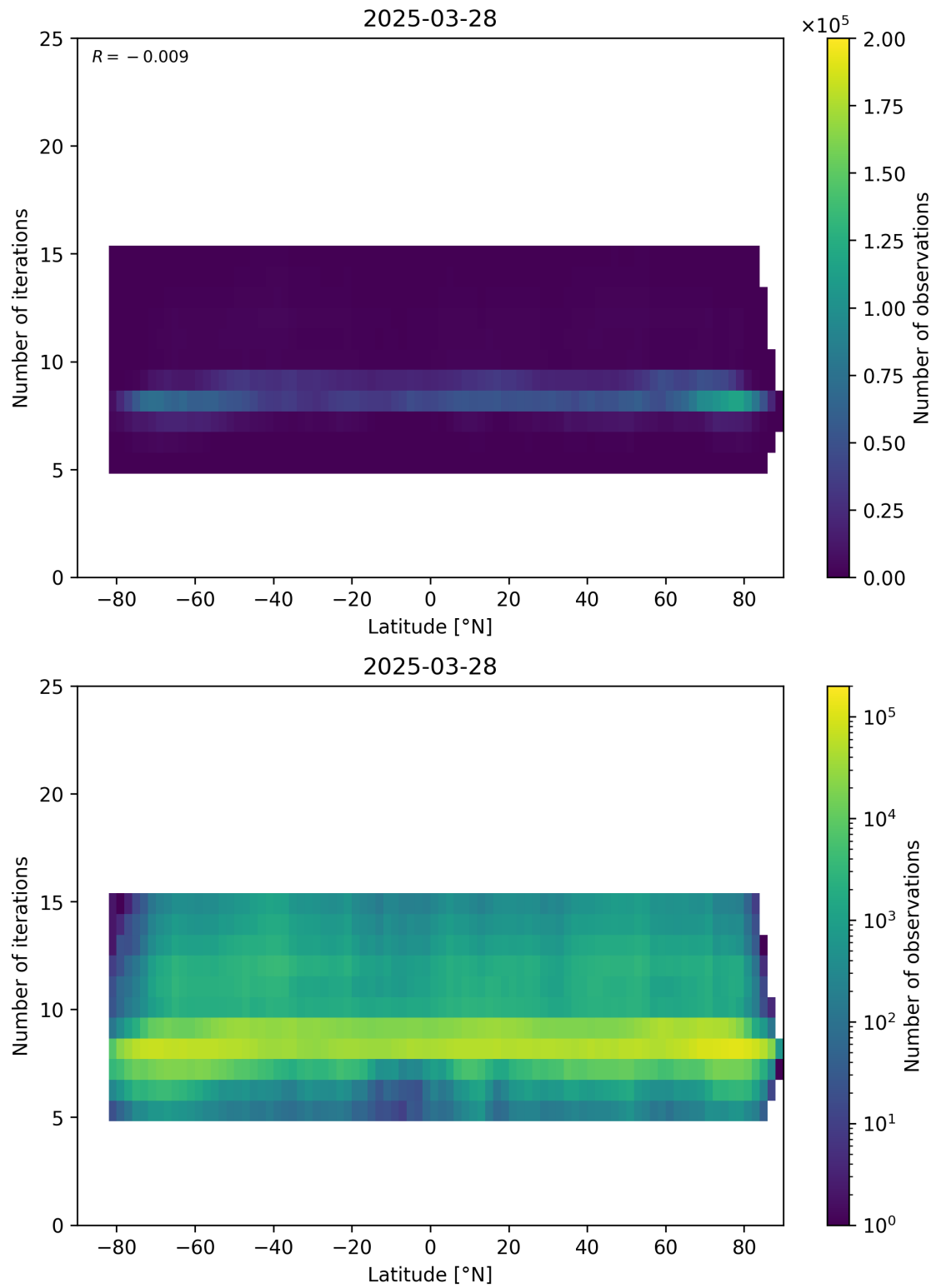
Figure 56: Scatter density plot of “Latitude” against “Number of iterations” for 2025-03-28 to 2025-03-29.
