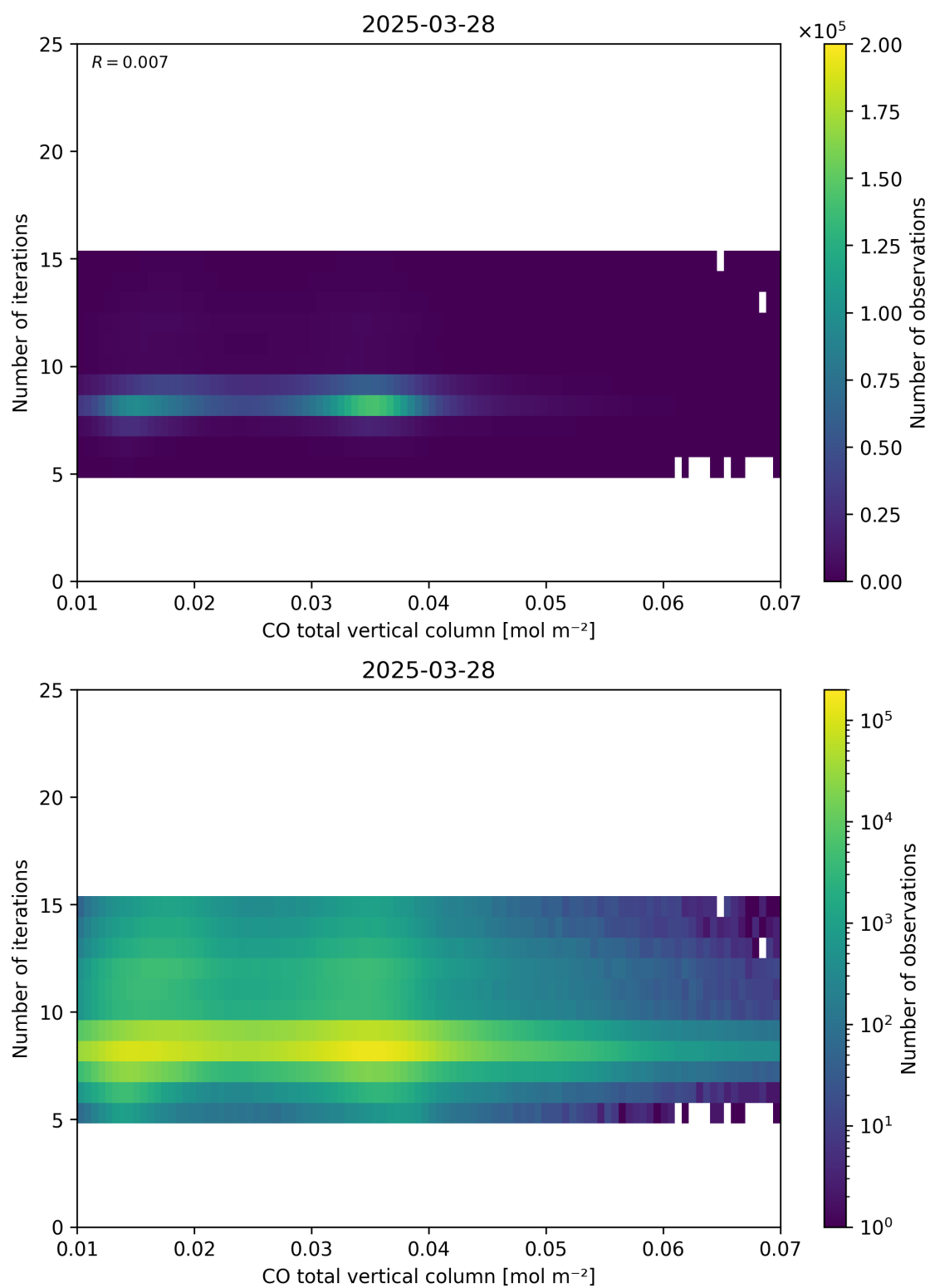
Figure 42: Scatter density plot of “CO total vertical column” against “Number of iterations” for 2025-03-28 to 2025-03-29.
