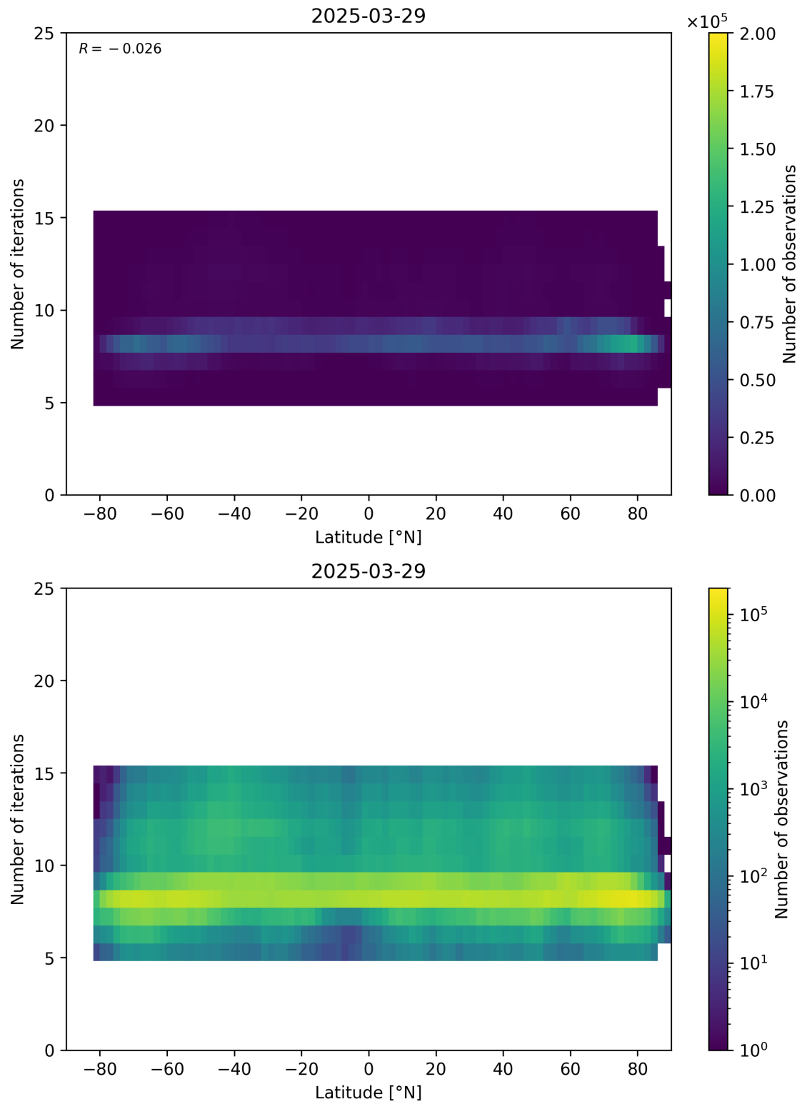
Figure 56: Scatter density plot of “Latitude” against “Number of iterations” for 2025-03-28 to 2025-03-30.
