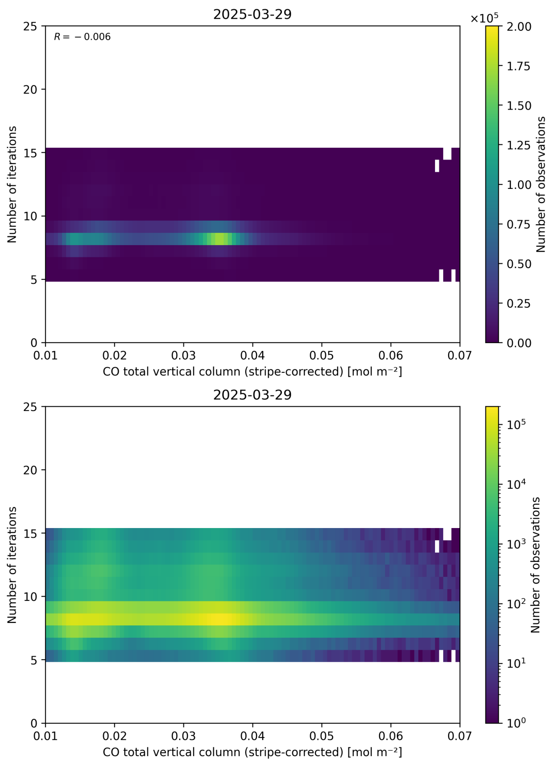
Figure 39: Scatter density plot of “CO total vertical column (stripe-corrected)” against “Number of iterations” for 2025-03-28 to 2025-03-30.
