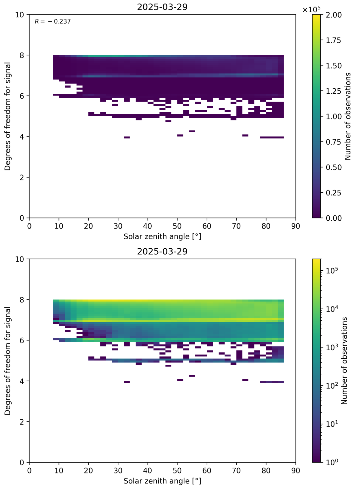
Figure 65: Scatter density plot of “Solar zenith angle” against “Degrees of freedom for signal” for 2025-03-28 to 2025-03-30.
