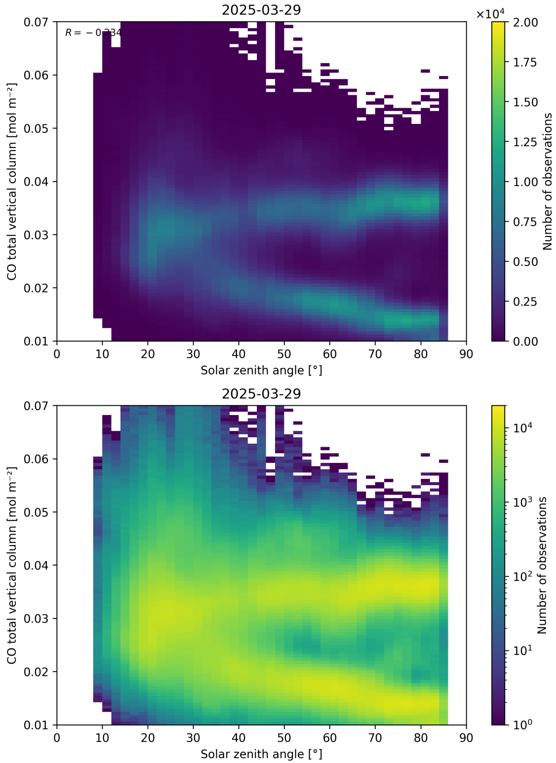
Figure 61: Scatter density plot of “Solar zenith angle” against “CO total vertical column” for 2025-03-28 to 2025-03-30.
