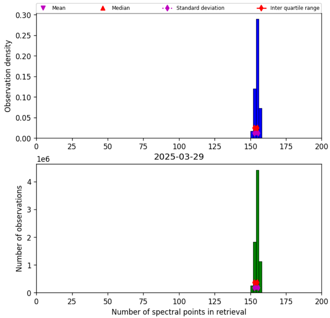
Figure 21: Histogram of “Number of spectral points in retrieval” for 2025-03-28 to 2025-03-30
