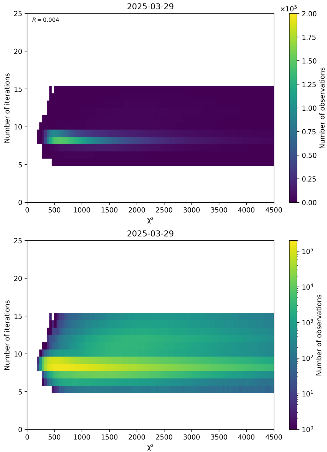
Figure 49: Scatter density plot of “ \chi^2 ” against “Number of iterations” for 2025-03-28 to 2025-03-30.
