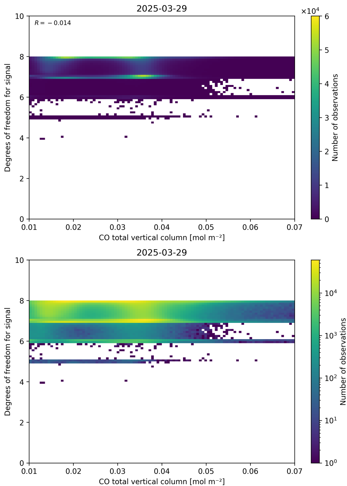
Figure 41: Scatter density plot of “CO total vertical column” against “Degrees of freedom for signal” for 2025-03-28 to 2025-03-30.
