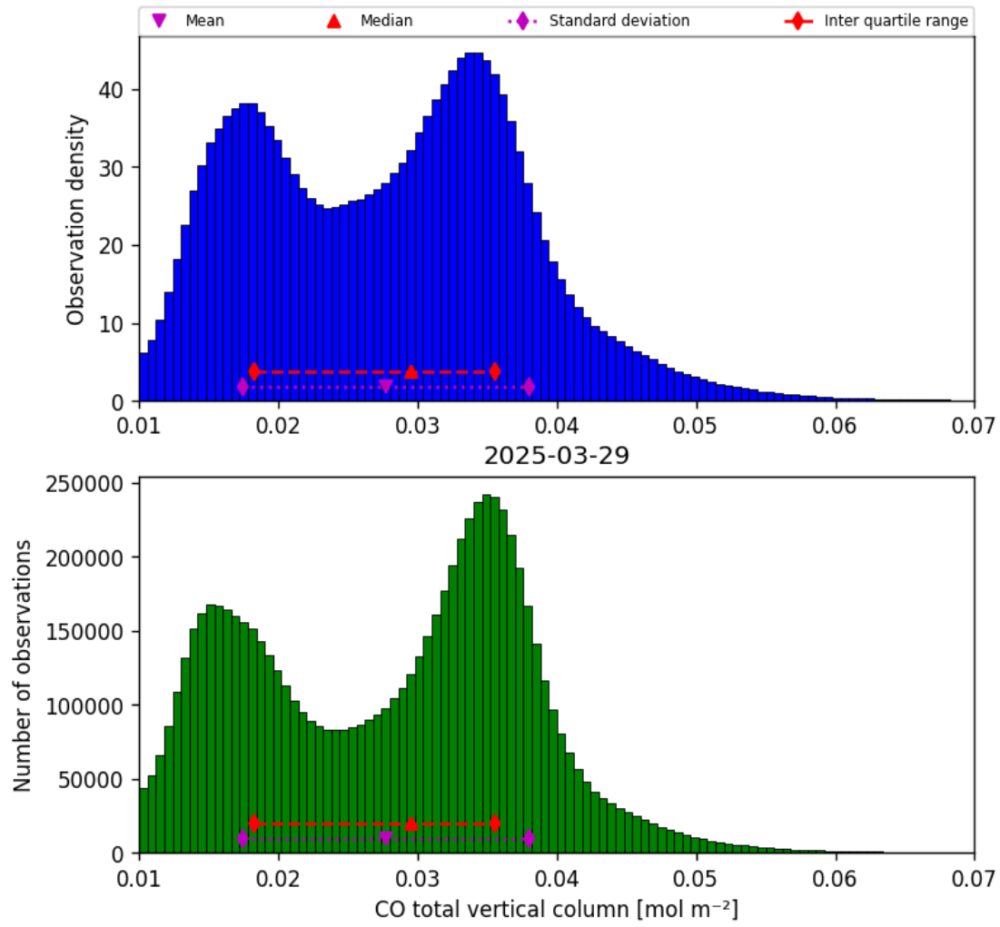
Figure 18: Histogram of “CO total vertical column” for 2025-03-28 to 2025-03-30
