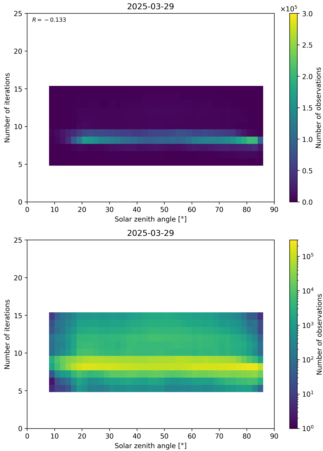
Figure 67: Scatter density plot of “Solar zenith angle” against “Number of iterations” for 2025-03-28 to 2025-03-30.
