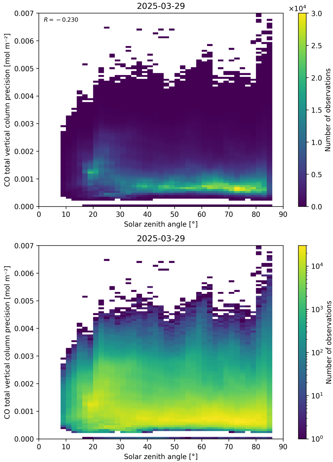
Figure 63: Scatter density plot of “Solar zenith angle” against “CO total vertical column precision” for 2025-03-28 to 2025-03-30.
