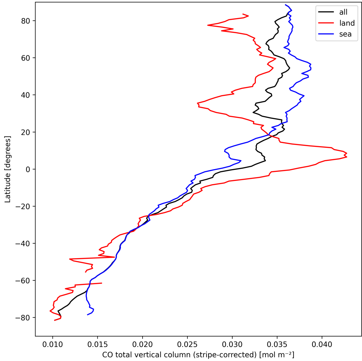
Figure 11: Zonal average of “CO total vertical column (stripe-corrected)” for 2025-03-28 to 2025-03-30.
