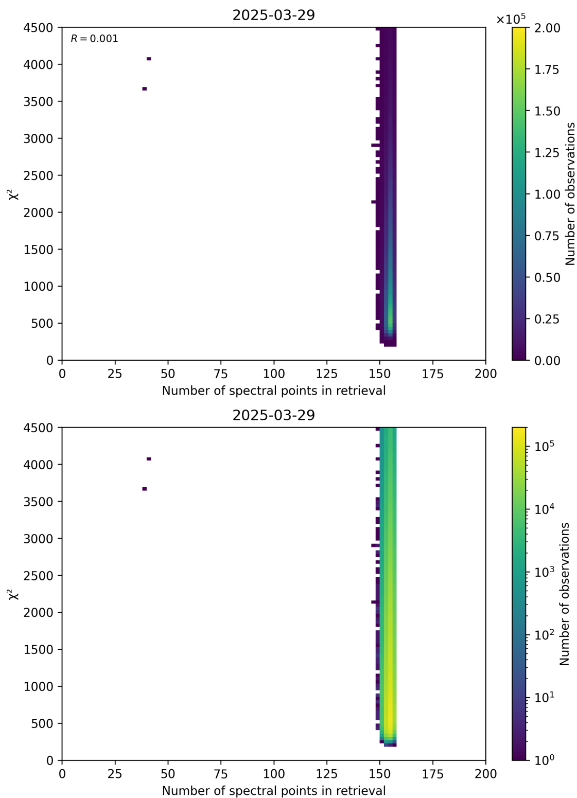
Figure 58: Scatter density plot of “Number of spectral points in retrieval” against “ \chi^2 ” for 2025-03-28 to 2025-03-30.
