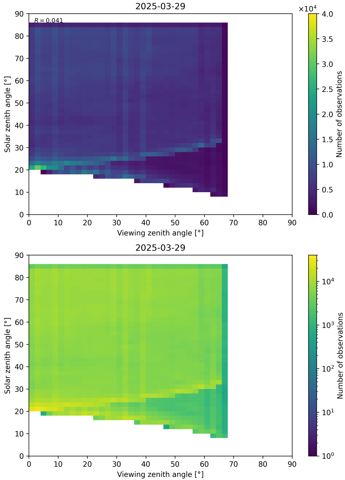
Figure 77: Scatter density plot of “Viewing zenith angle” against “Solar zenith angle” for 2025-03-28 to 2025-03-30.
