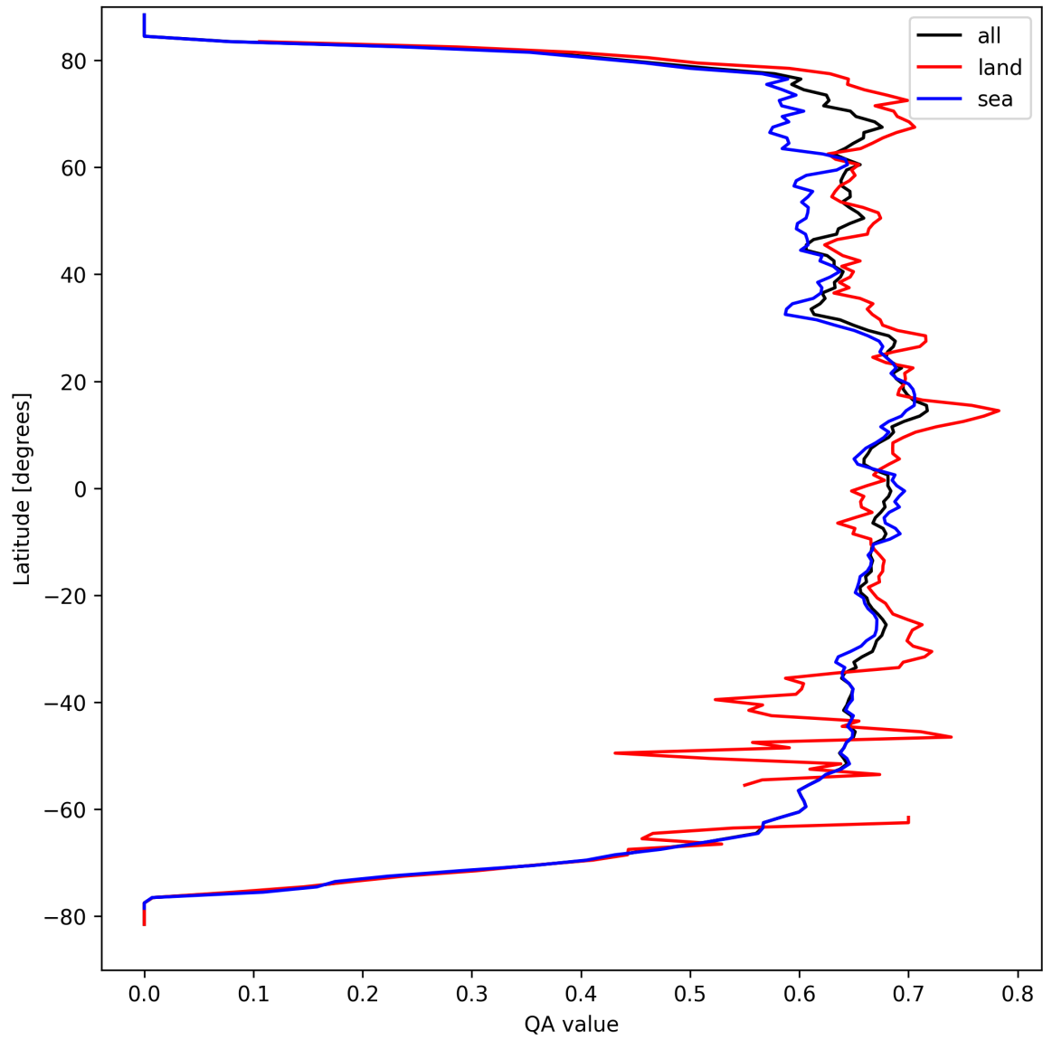
Figure 9: Zonal average of “QA value” for 2025-03-28 to 2025-03-30.
