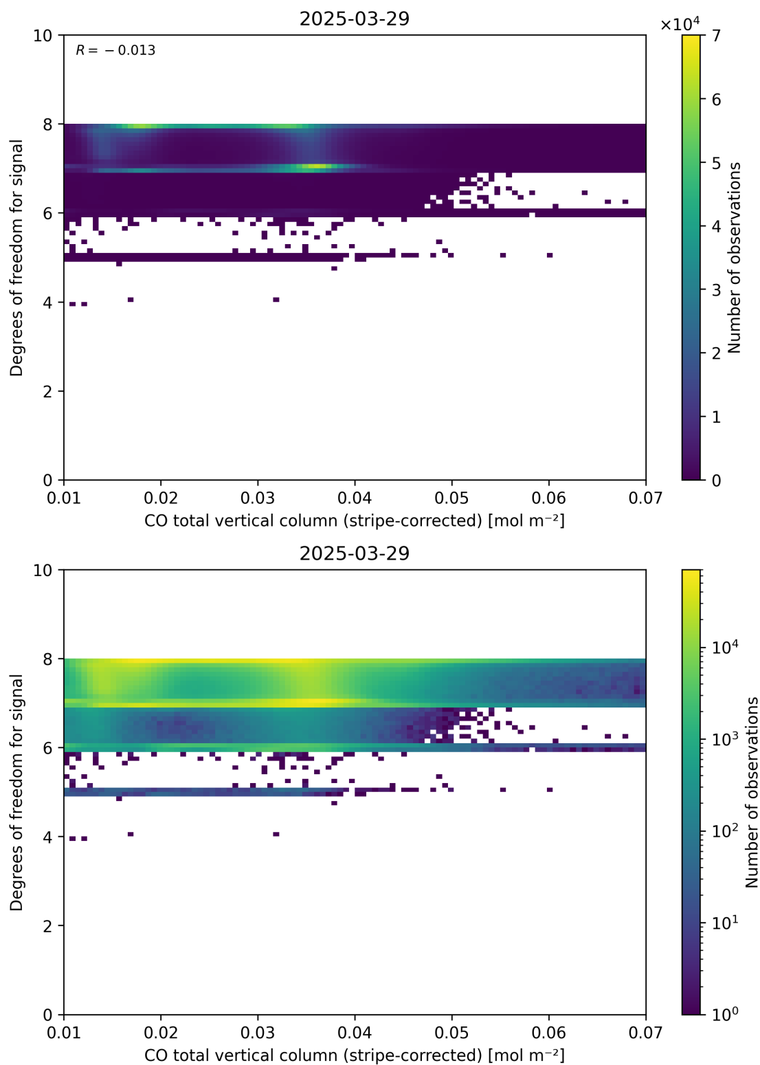
Figure 38: Scatter density plot of “CO total vertical column (stripe-corrected)” against “Degrees of freedom for signal” for 2025-03-28 to 2025-03-30.
