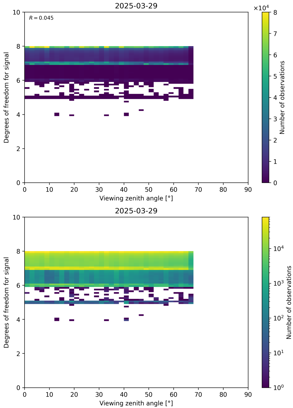
Figure 73: Scatter density plot of “Viewing zenith angle” against “Degrees of freedom for signal” for 2025-03-28 to 2025-03-30.
