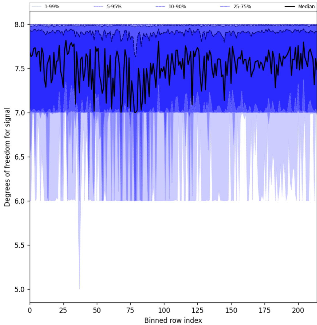
Figure 31: Along track statistics of “Degrees of freedom for signal” for 2025-03-28 to 2025-03-30
