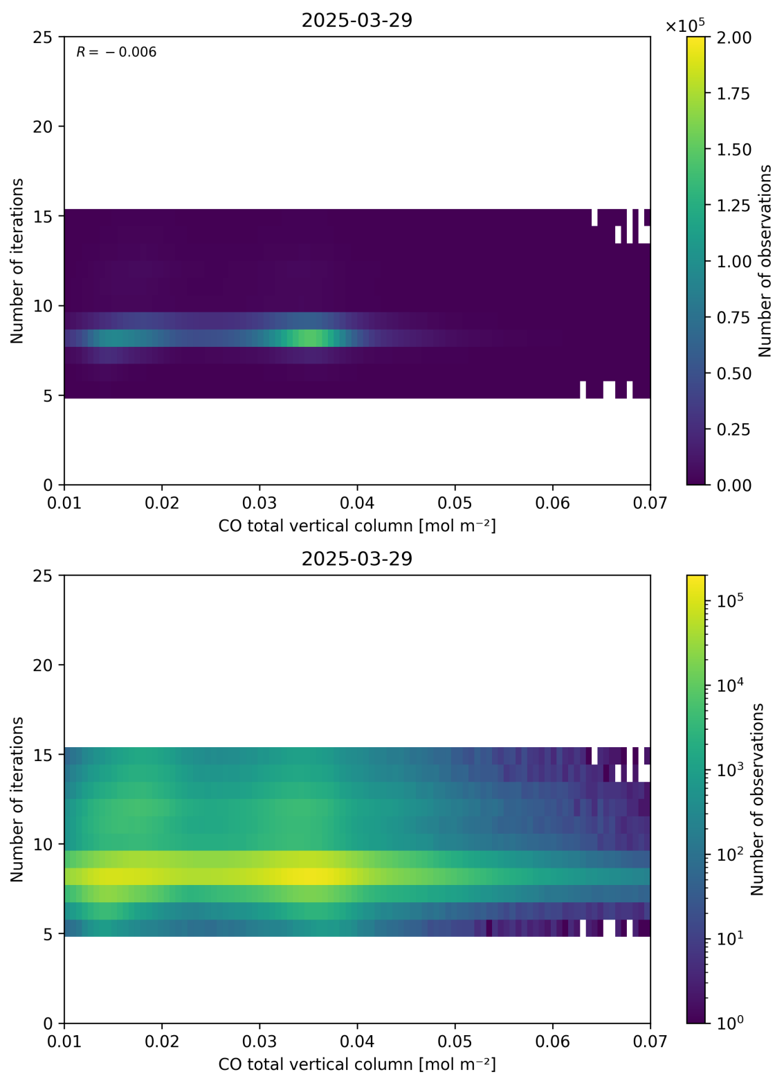
Figure 42: Scatter density plot of “CO total vertical column” against “Number of iterations” for 2025-03-28 to 2025-03-30.
