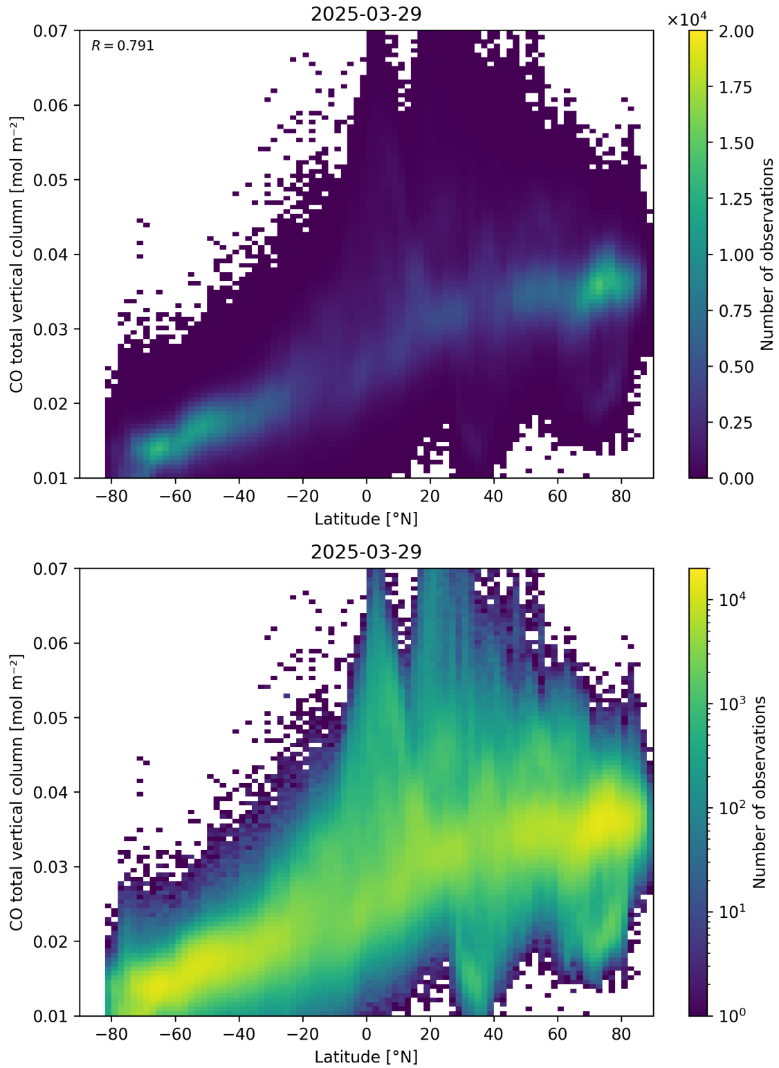
Figure 51: Scatter density plot of “Latitude” against “CO total vertical column” for 2025-03-28 to 2025-03-30.
