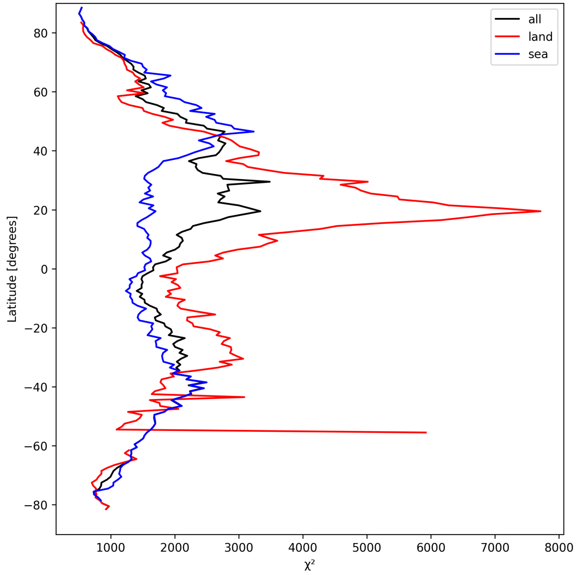
Figure 14: Zonal average of “ \chi^2 ” for 2025-03-28 to 2025-03-30.
