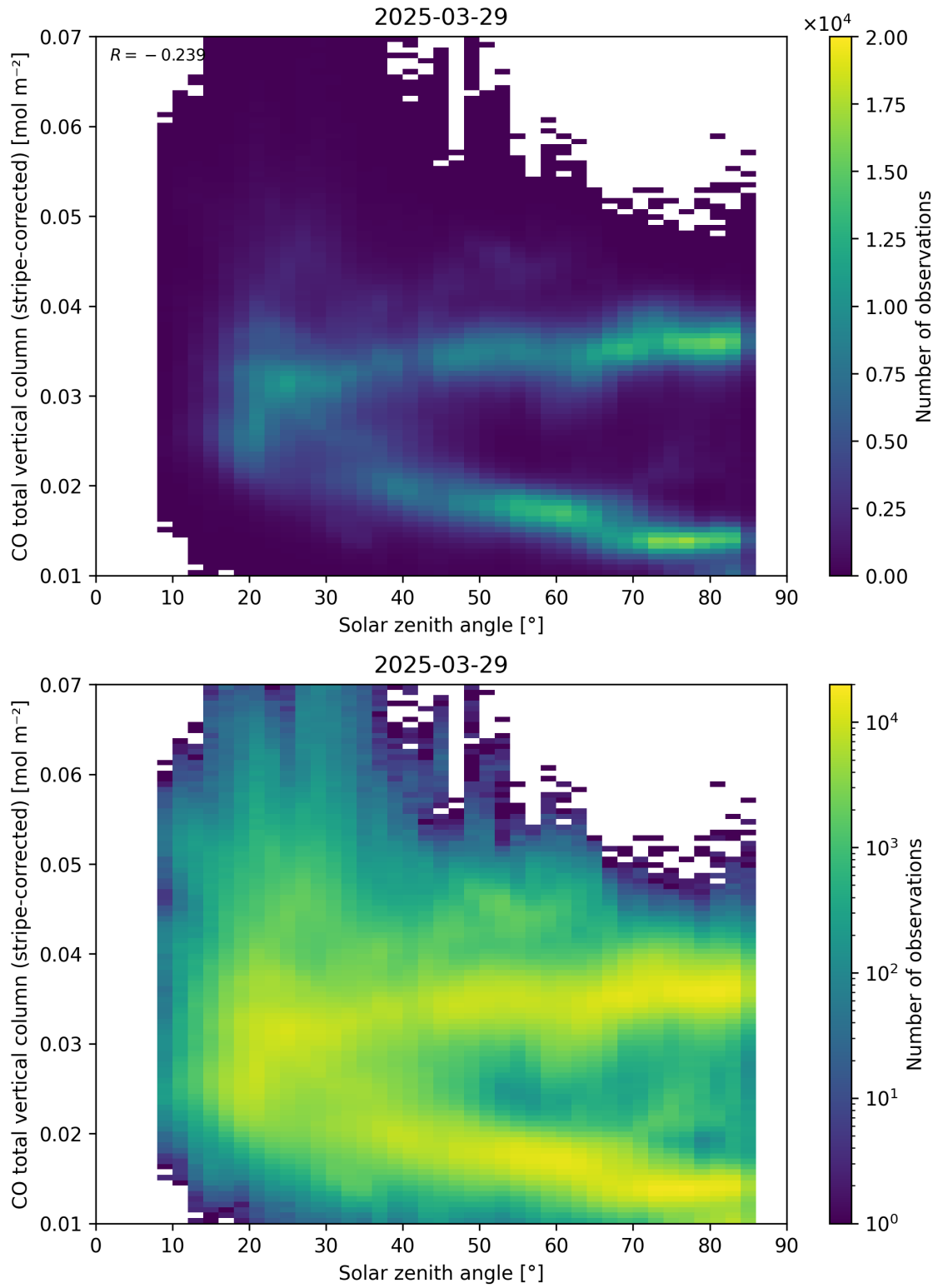
Figure 62: Scatter density plot of “Solar zenith angle” against “CO total vertical column (stripe-corrected)” for 2025-03-28 to 2025-03-30.
