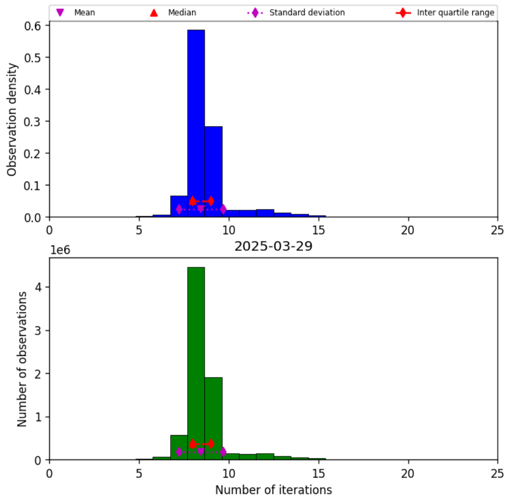
Figure 24: Histogram of “Number of iterations” for 2025-03-28 to 2025-03-30
