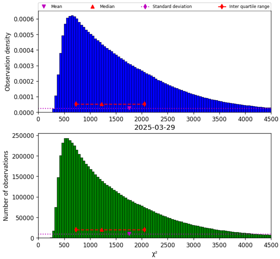
Figure 22: Histogram of “ \chi^2 ” for 2025-03-28 to 2025-03-30
