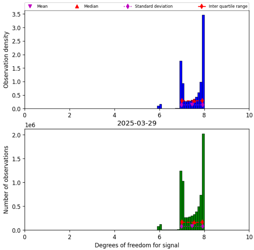
Figure 23: Histogram of “Degrees of freedom for signal” for 2025-03-28 to 2025-03-30
