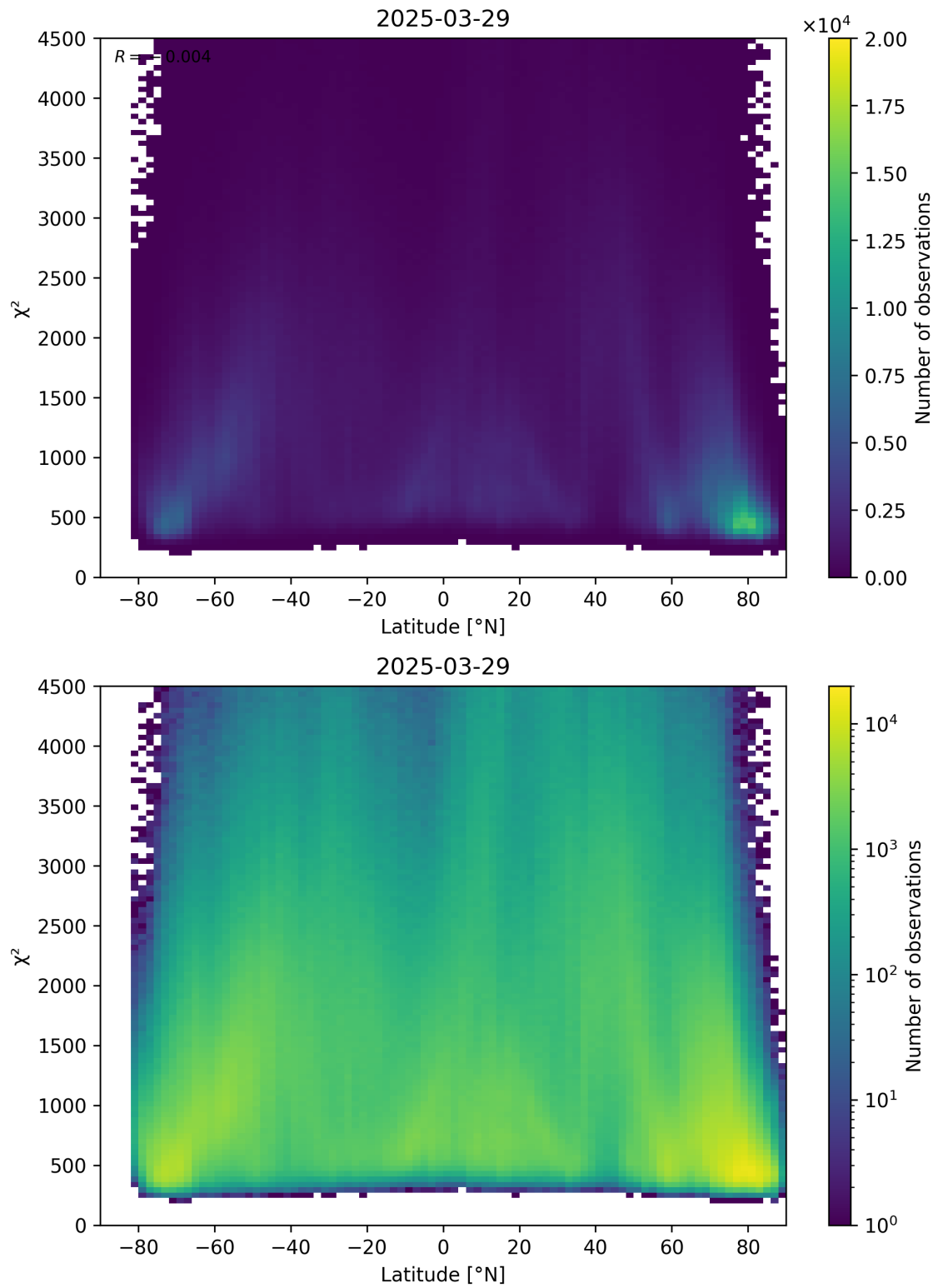
Figure 54: Scatter density plot of “Latitude” against “ \chi^2 ” for 2025-03-28 to 2025-03-30.
