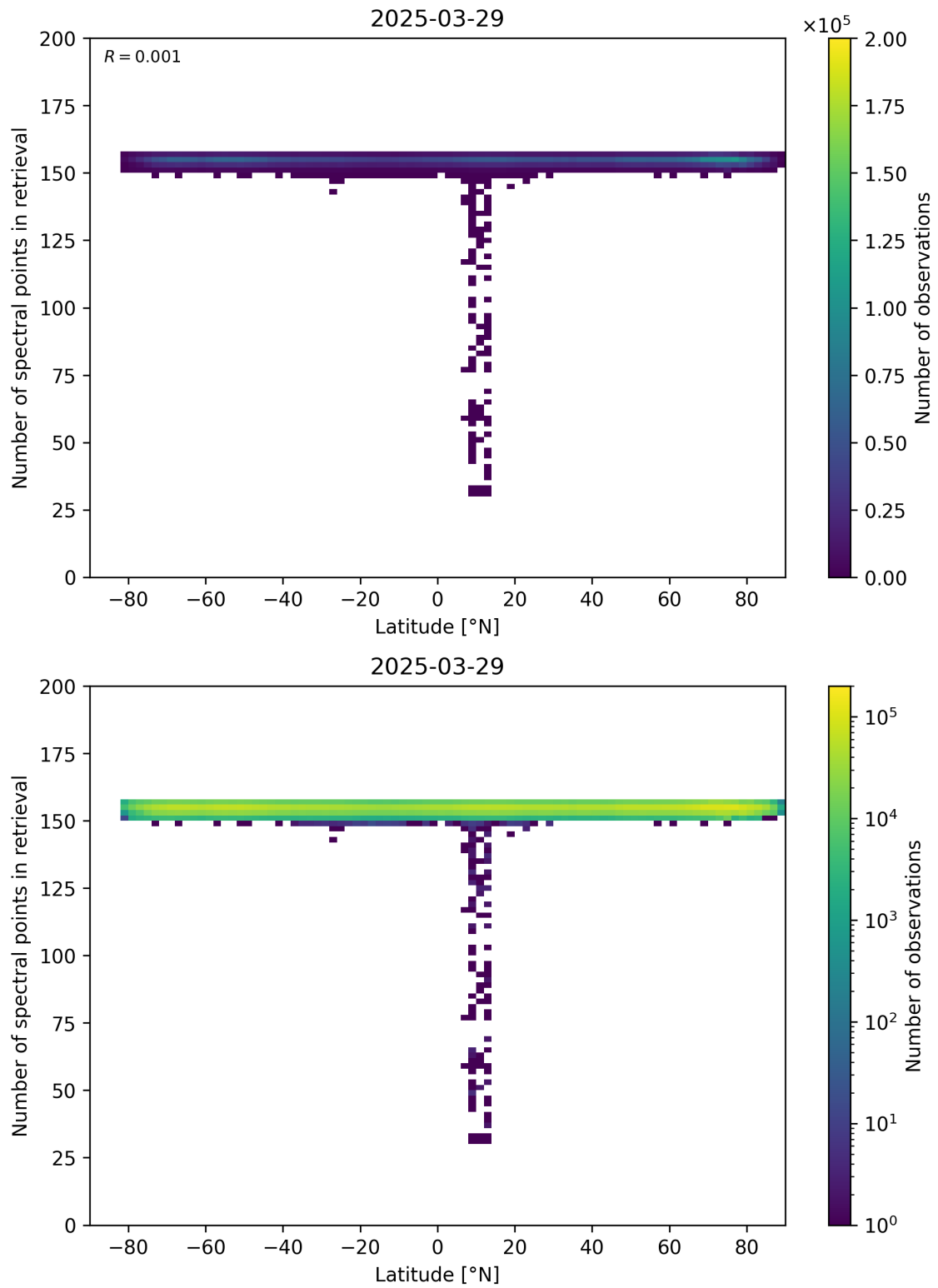
Figure 57: Scatter density plot of “Latitude” against “Number of spectral points in retrieval” for 2025-03-28 to 2025-03-30.
