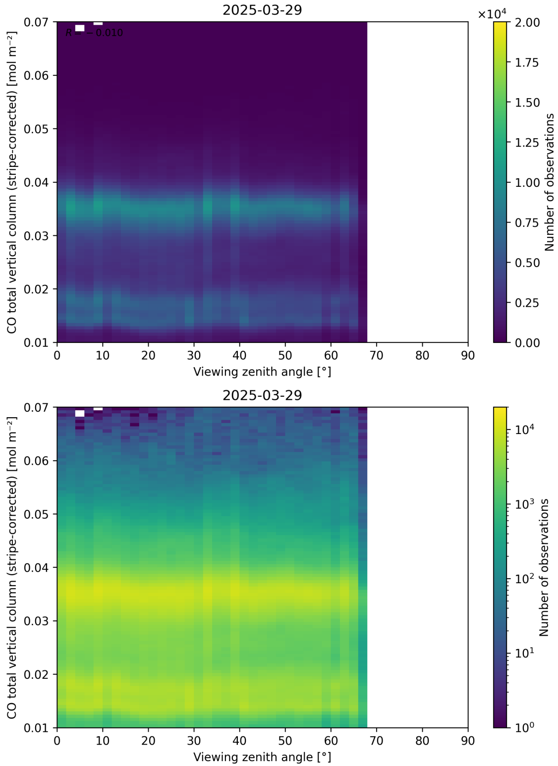
Figure 70: Scatter density plot of “Viewing zenith angle” against “CO total vertical column (stripe-corrected)” for 2025-03-28 to 2025-03-30.
