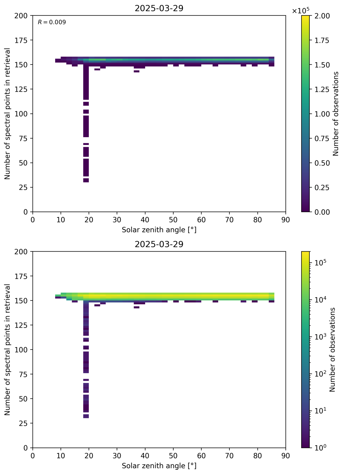
Figure 68: Scatter density plot of “Solar zenith angle” against “Number of spectral points in retrieval” for 2025-03-28 to 2025-03-30.
