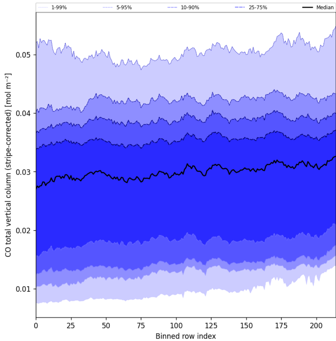
Figure 27: Along track statistics of “CO total vertical column (stripe-corrected)” for 2025-03-28 to 2025-03-30
