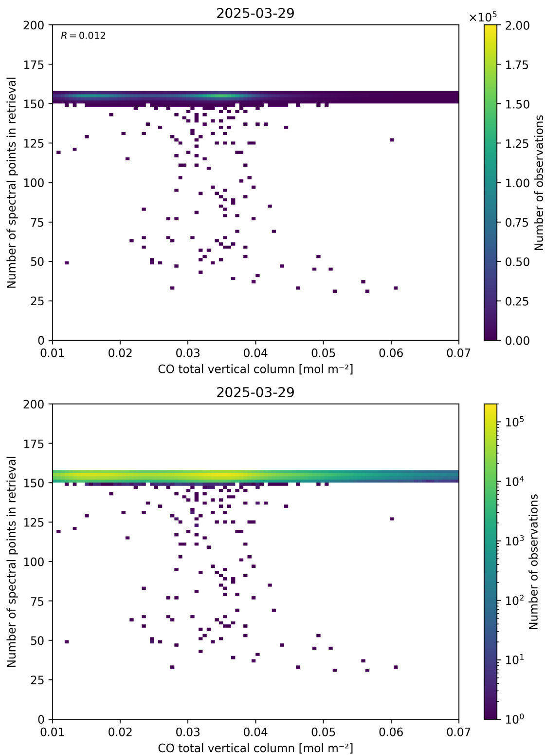
Figure 43: Scatter density plot of “CO total vertical column” against “Number of spectral points in retrieval” for 2025-03-28 to 2025-03-30.
