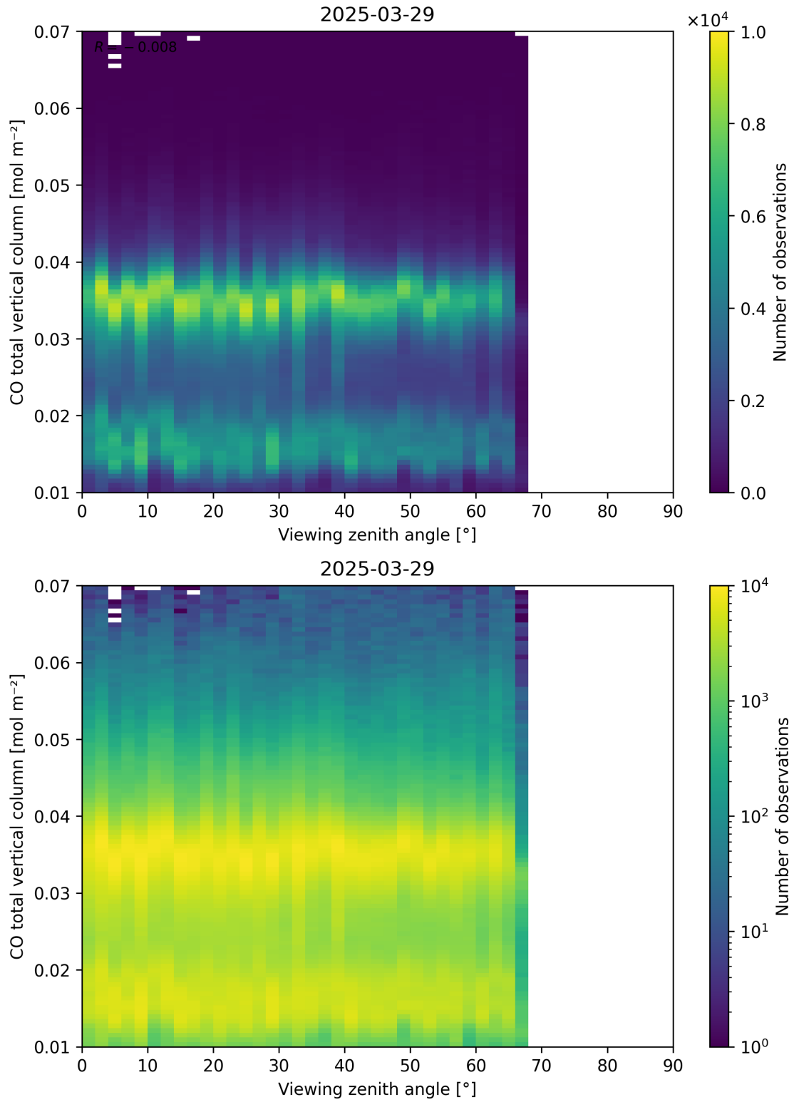
Figure 69: Scatter density plot of “Viewing zenith angle” against “CO total vertical column” for 2025-03-28 to 2025-03-30.
