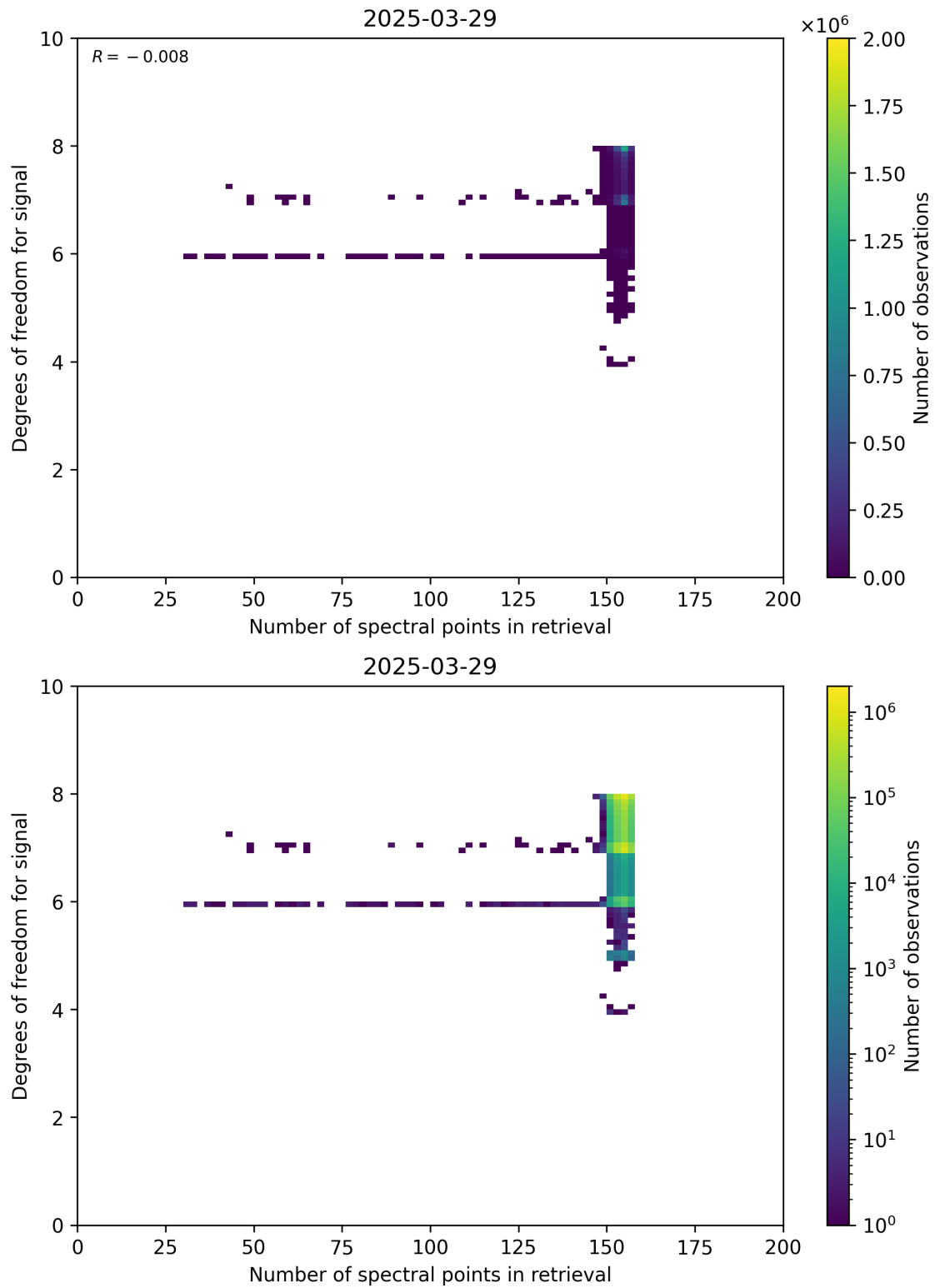
Figure 59: Scatter density plot of “Number of spectral points in retrieval” against “Degrees of freedom for signal” for 2025-03-28 to 2025-03-30.
