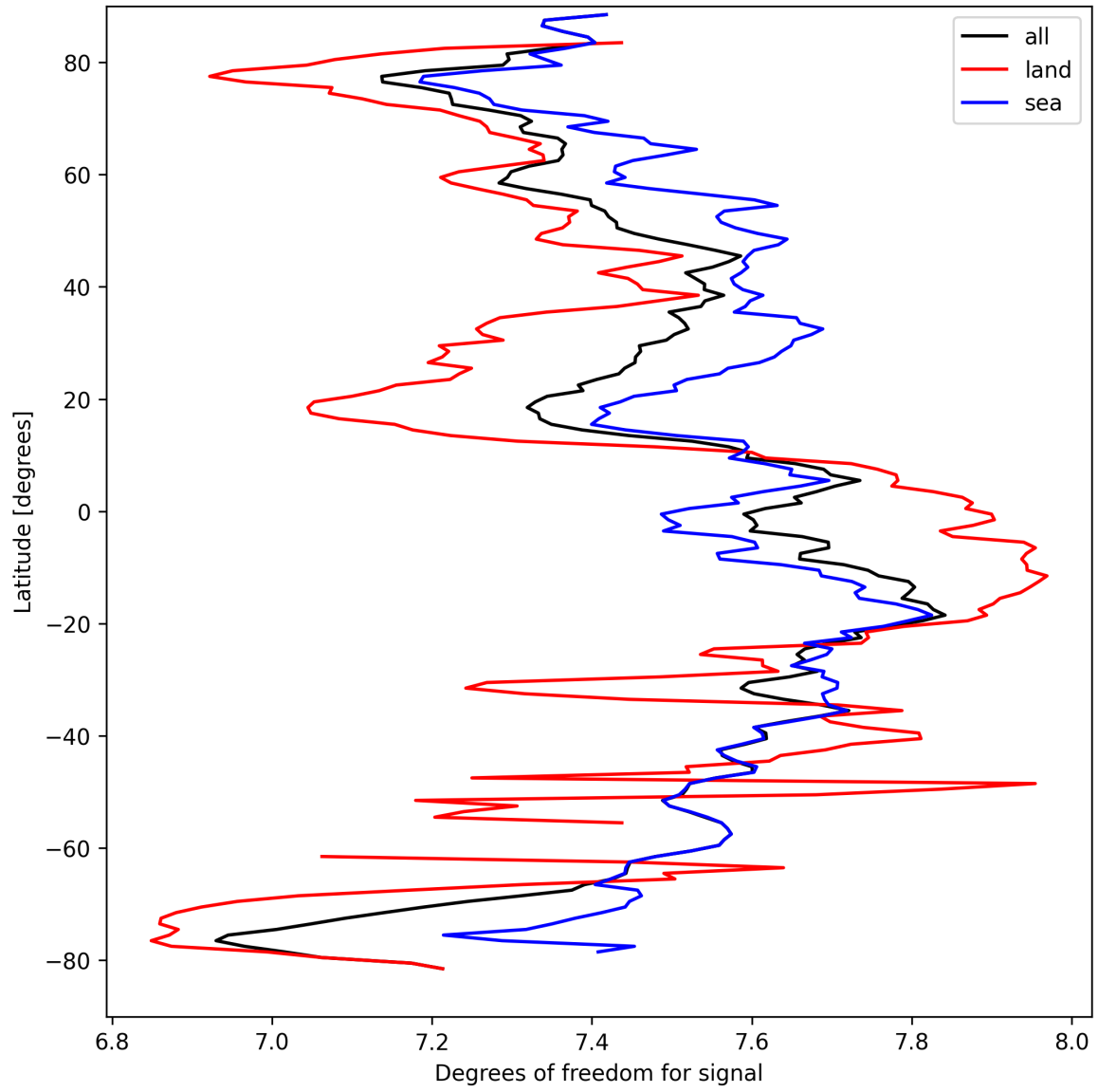
Figure 15: Zonal average of “Degrees of freedom for signal” for 2025-03-28 to 2025-03-30.
