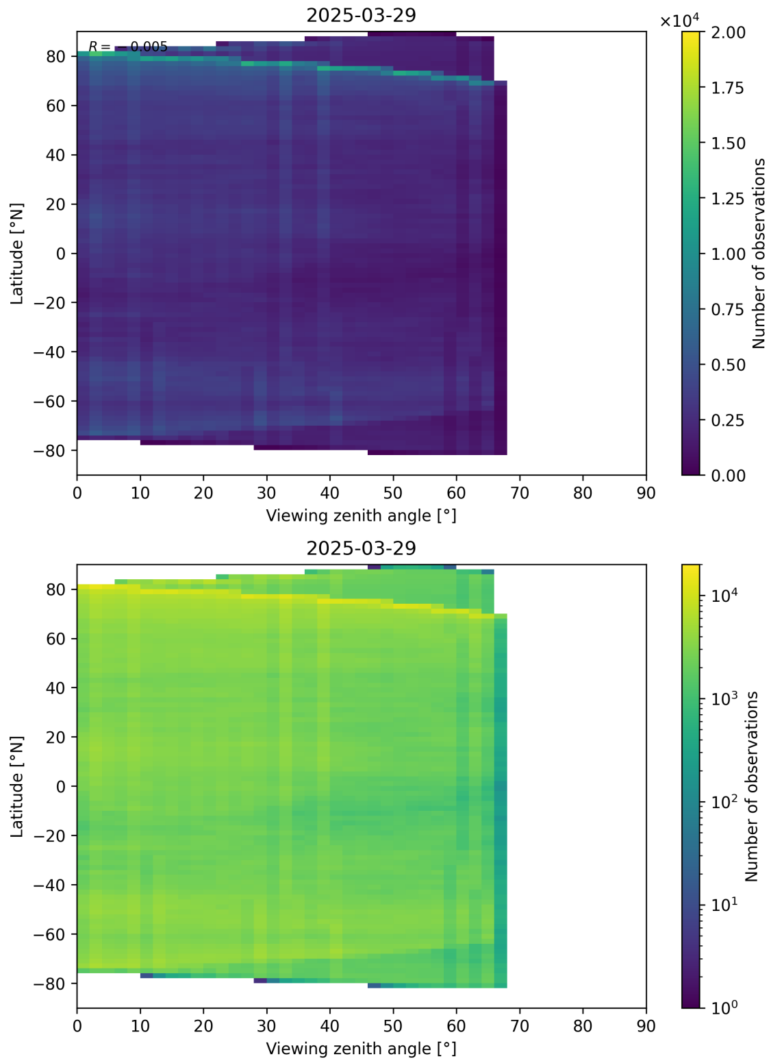
Figure 74: Scatter density plot of “Viewing zenith angle” against “Latitude” for 2025-03-28 to 2025-03-30.
