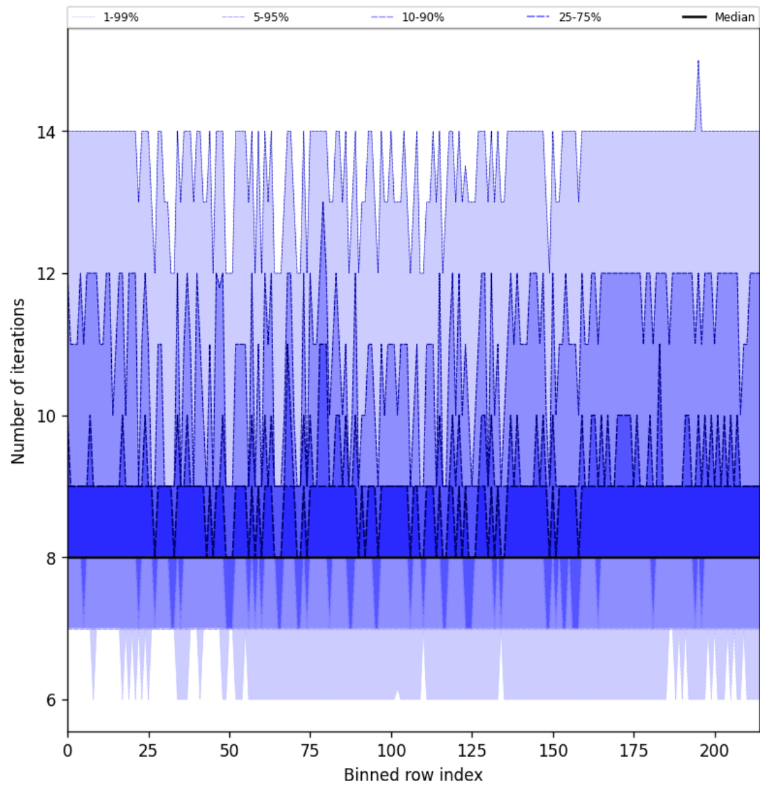
Figure 32: Along track statistics of “Number of iterations” for 2025-03-28 to 2025-03-30
