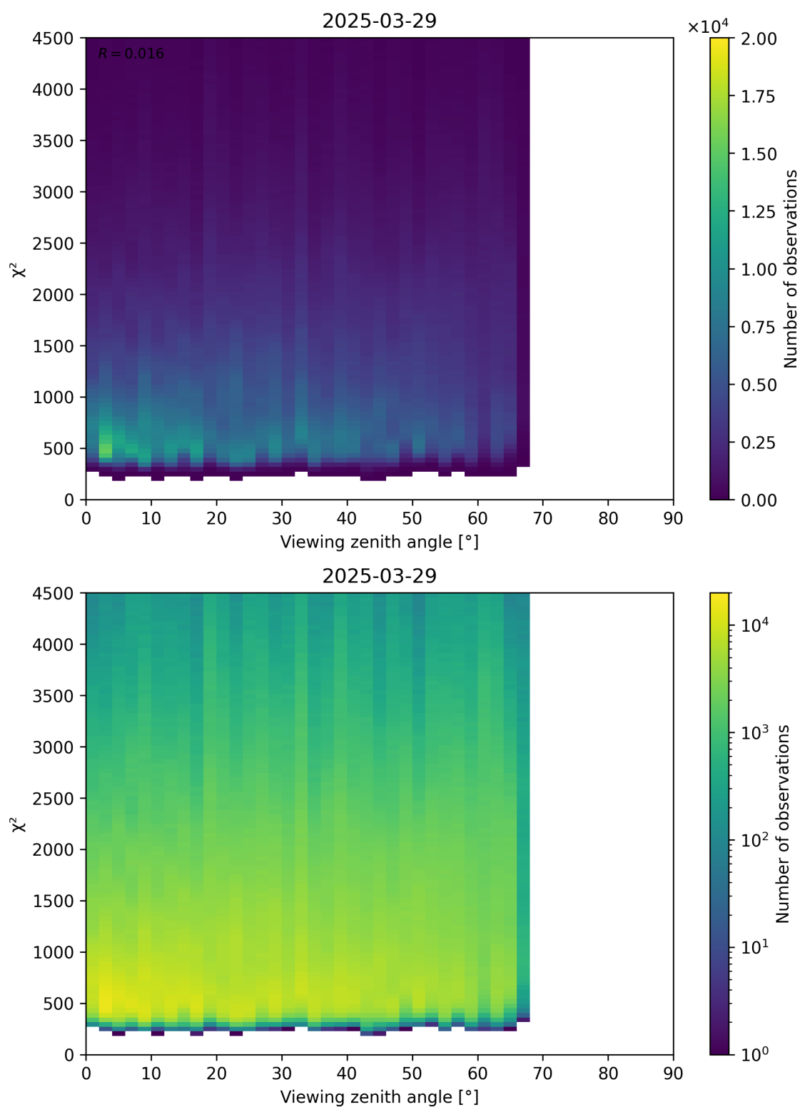
Figure 72: Scatter density plot of “Viewing zenith angle” against “ \chi^2 ” for 2025-03-28 to 2025-03-30.
