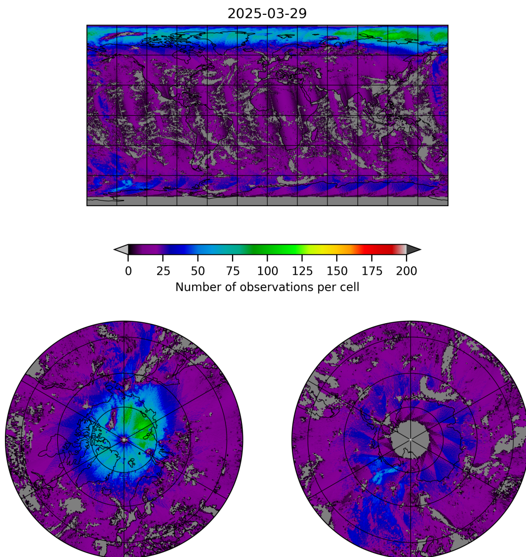
Figure 8: Map of the number of observations for 2025-03-28 to 2025-03-30
