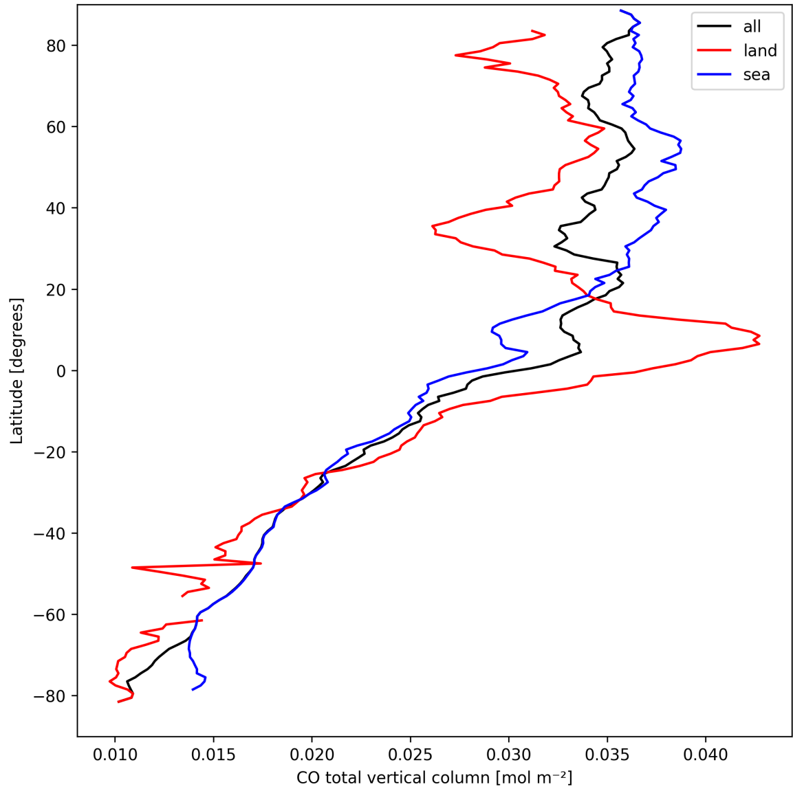
Figure 10: Zonal average of “CO total vertical column” for 2025-03-28 to 2025-03-30.
