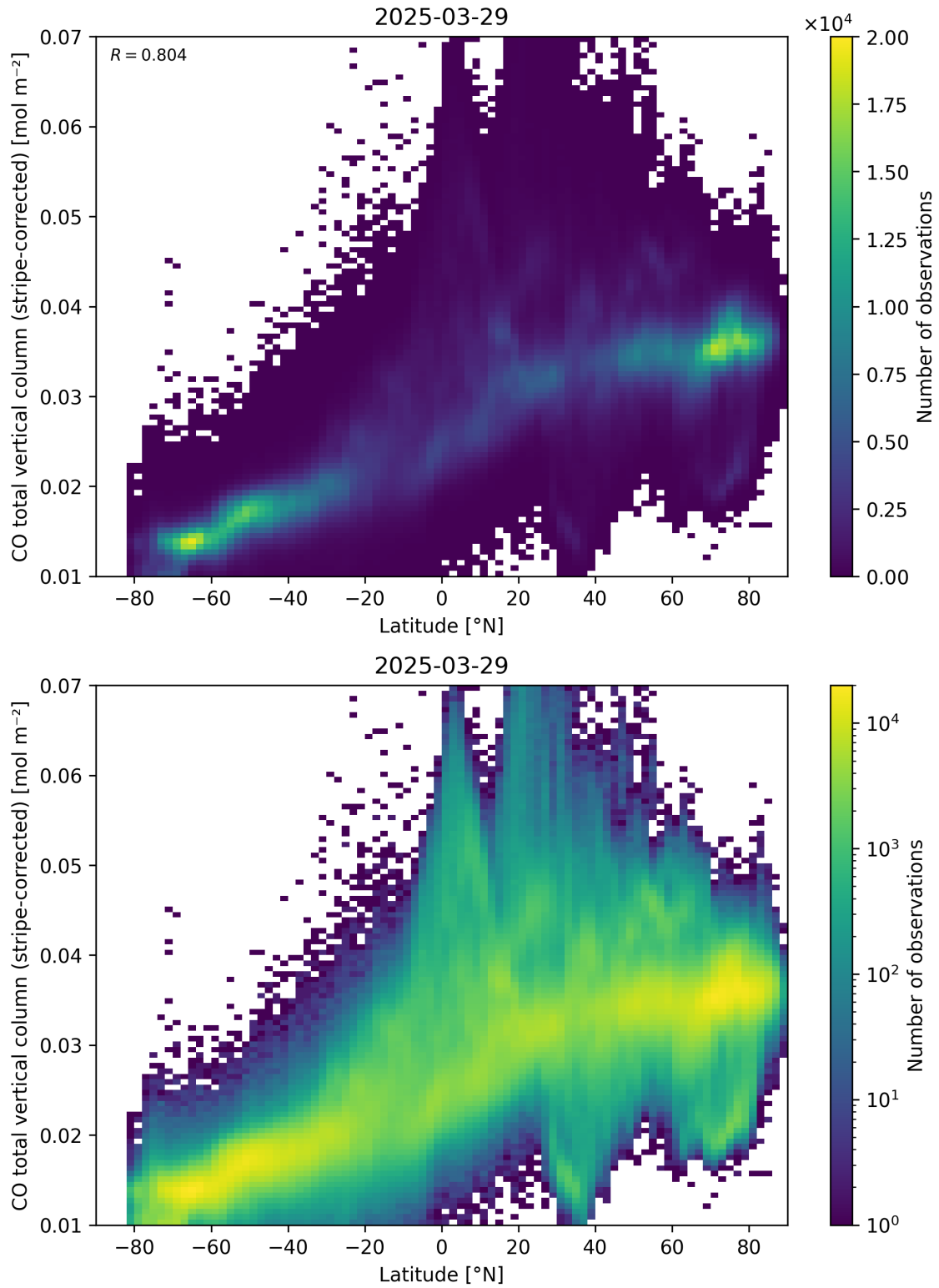
Figure 52: Scatter density plot of “Latitude” against “CO total vertical column (stripe-corrected)” for 2025-03-28 to 2025-03-30.
