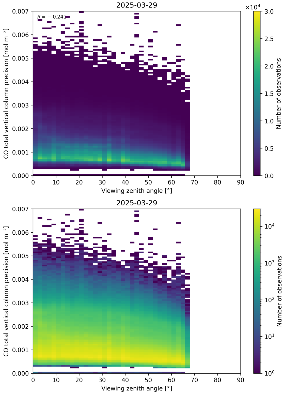
Figure 71: Scatter density plot of “Viewing zenith angle” against “CO total vertical column precision” for 2025-03-28 to 2025-03-30.
