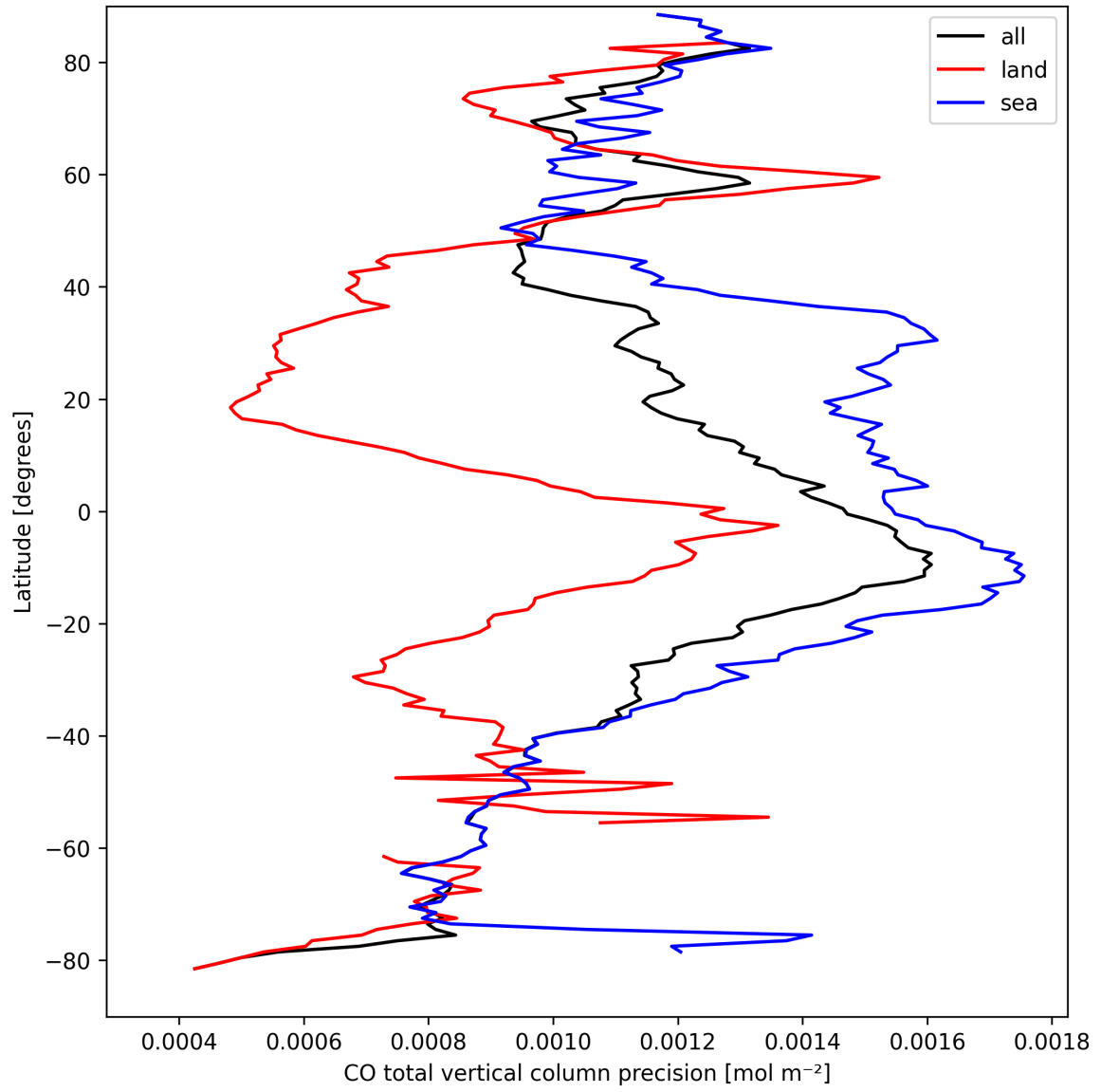
Figure 12: Zonal average of “CO total vertical column precision” for 2025-03-28 to 2025-03-30.
