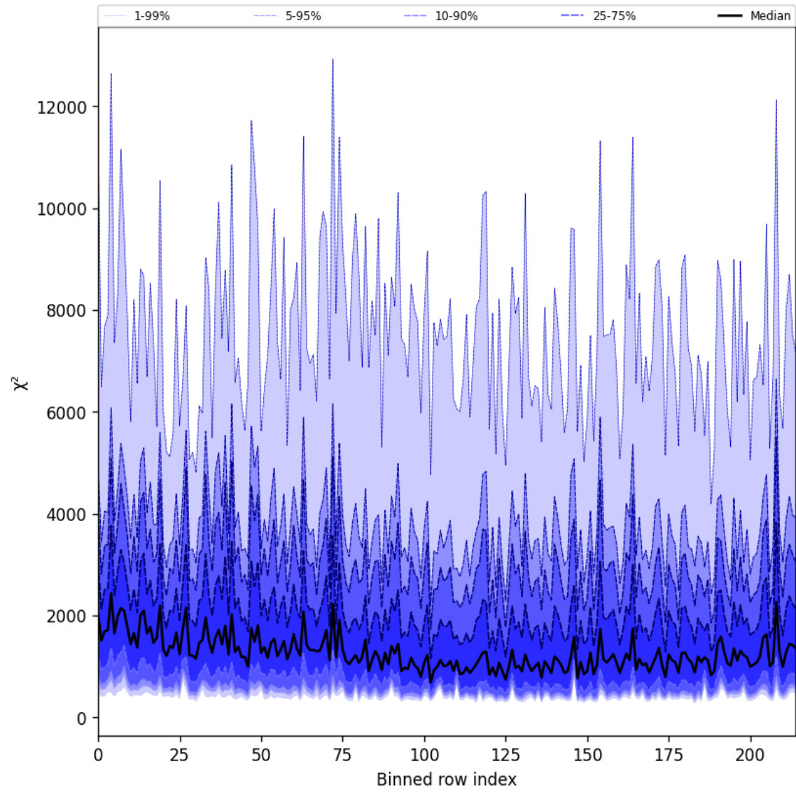
Figure 30: Along track statistics of “ \chi^2 ” for 2025-03-28 to 2025-03-30
