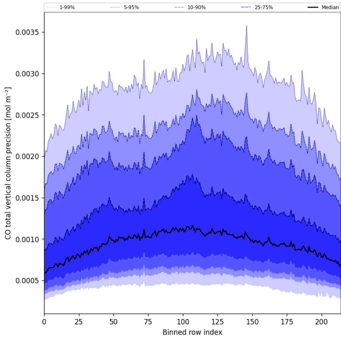
Figure 28: Along track statistics of “CO total vertical column precision” for 2025-03-28 to 2025-03-30
