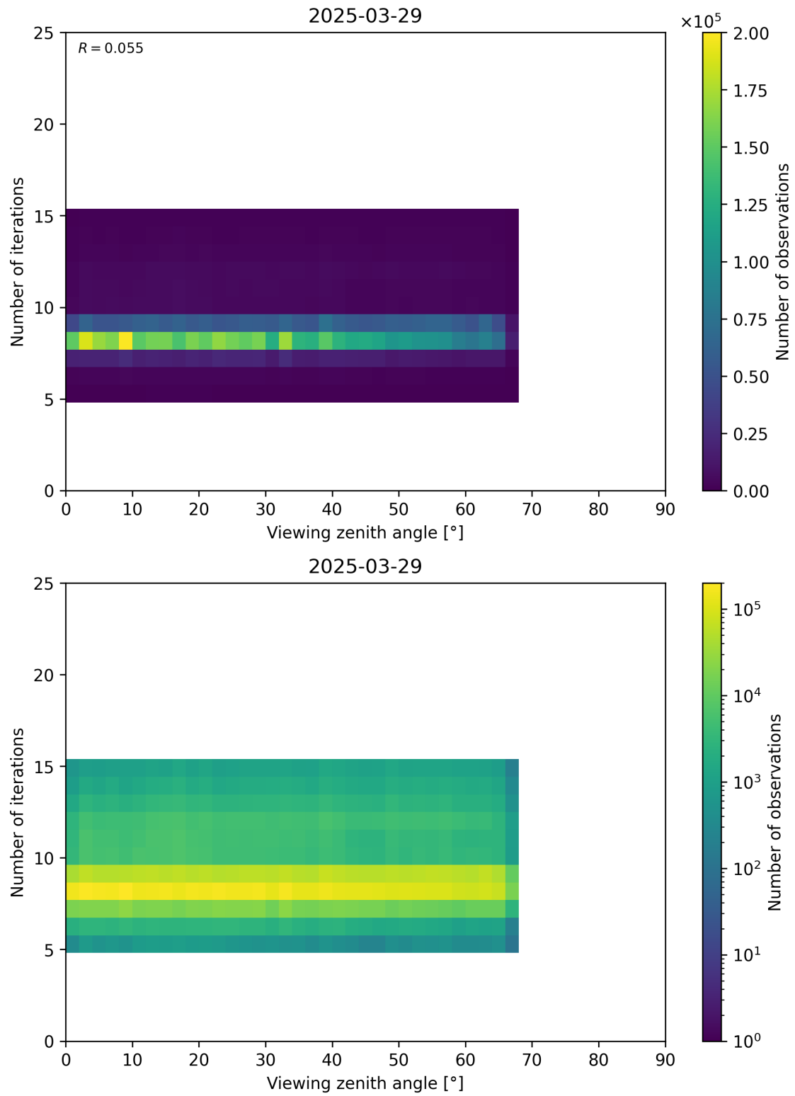
Figure 75: Scatter density plot of “Viewing zenith angle” against “Number of iterations” for 2025-03-28 to 2025-03-30.
