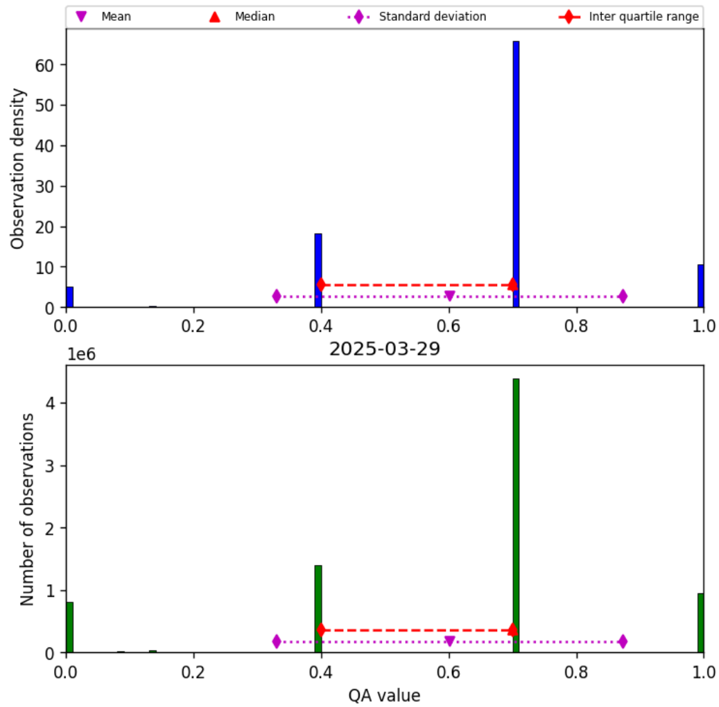
Figure 17: Histogram of “QA value” for 2025-03-28 to 2025-03-30
