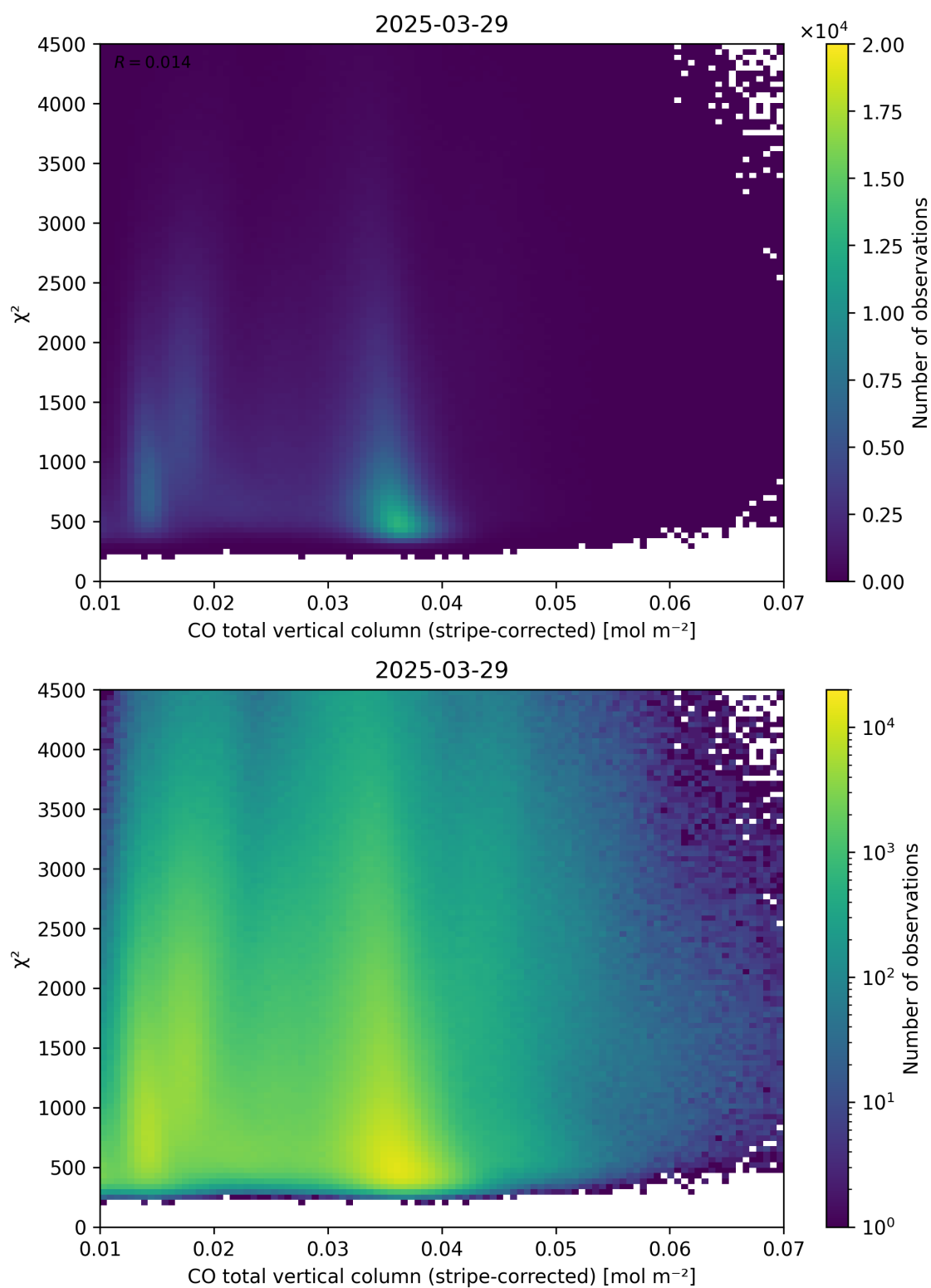
Figure 37: Scatter density plot of “CO total vertical column (stripe-corrected)” against “ \chi^2 ” for 2025-03-28 to 2025-03-30.
