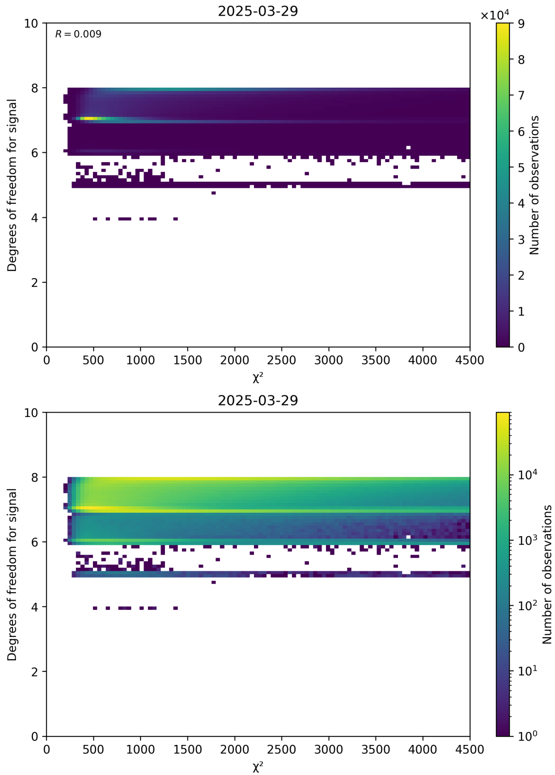
Figure 48: Scatter density plot of “ \chi^2 ” against “Degrees of freedom for signal” for 2025-03-28 to 2025-03-30.
