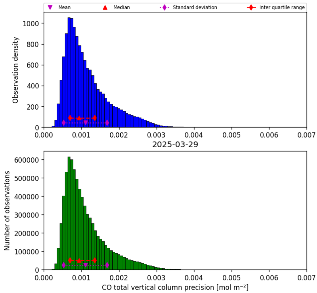
Figure 20: Histogram of “CO total vertical column precision” for 2025-03-28 to 2025-03-30
