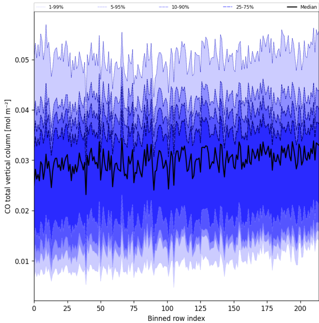
Figure 26: Along track statistics of “CO total vertical column” for 2025-03-28 to 2025-03-30
