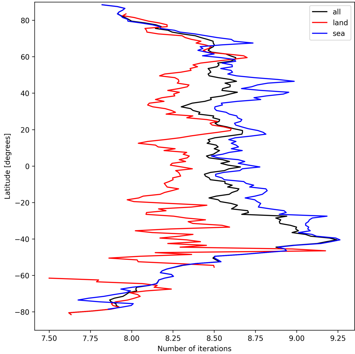
Figure 16: Zonal average of “Number of iterations” for 2025-03-28 to 2025-03-30.
