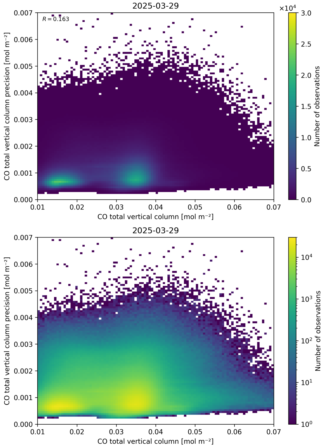
Figure 34: Scatter density plot of “CO total vertical column” against “CO total vertical column precision” for 2025-03-28 to 2025-03-30.
