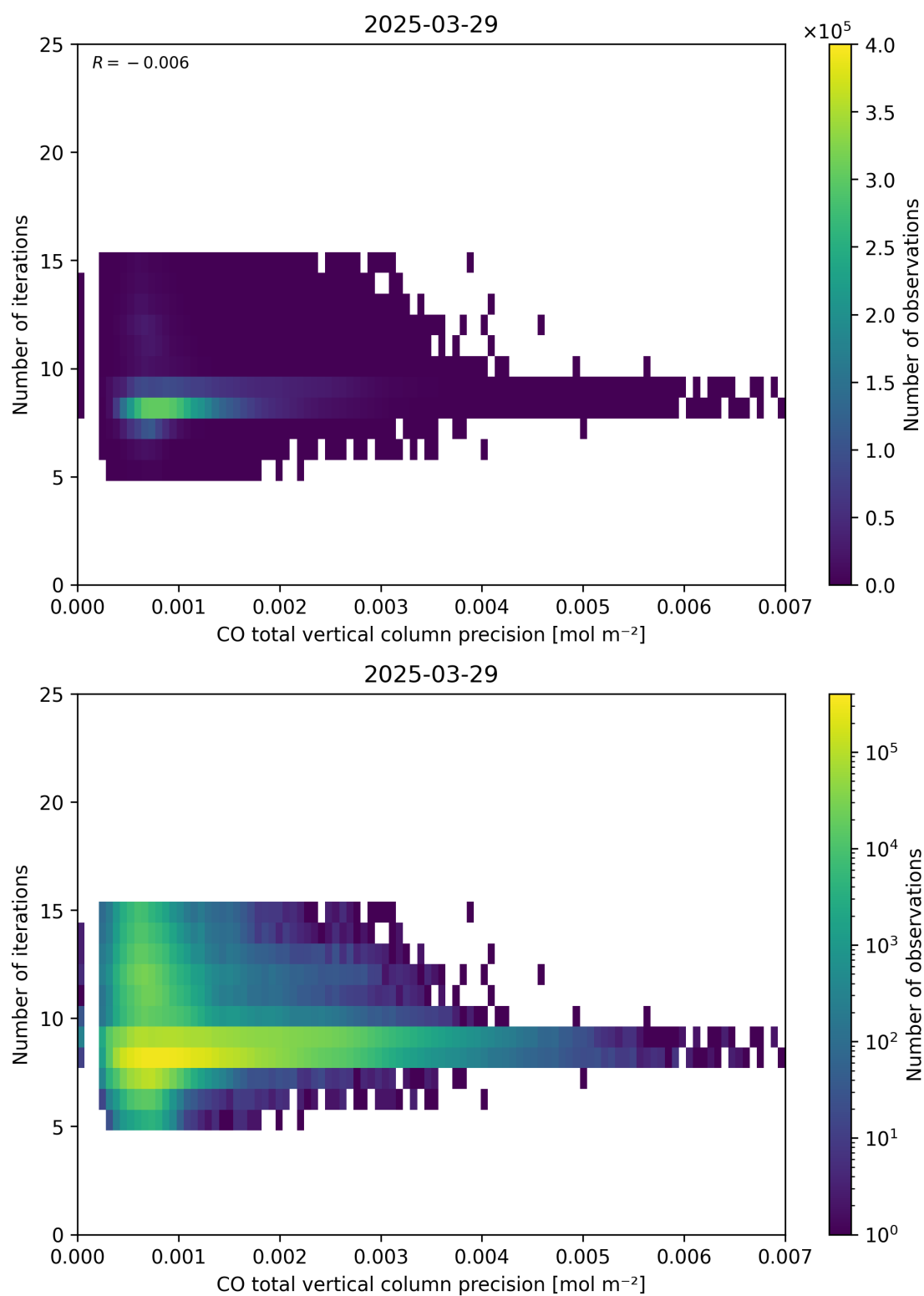
Figure 46: Scatter density plot of “CO total vertical column precision” against “Number of iterations” for 2025-03-28 to 2025-03-30.
