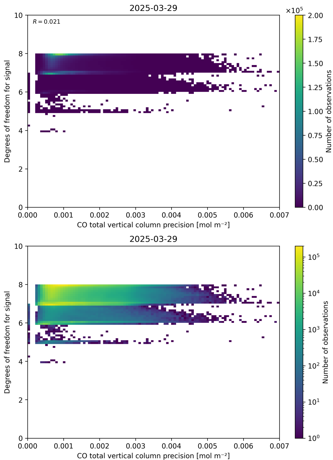
Figure 45: Scatter density plot of “CO total vertical column precision” against “Degrees of freedom for signal” for 2025-03-28 to 2025-03-30.
