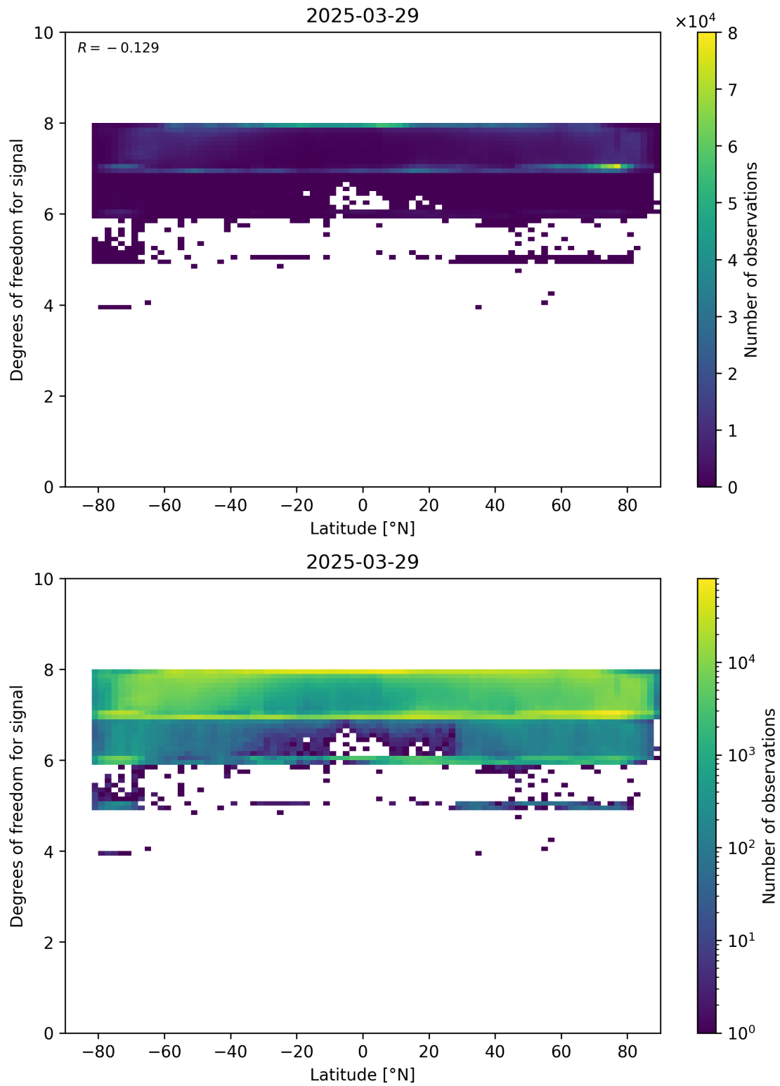
Figure 55: Scatter density plot of “Latitude” against “Degrees of freedom for signal” for 2025-03-28 to 2025-03-30.
