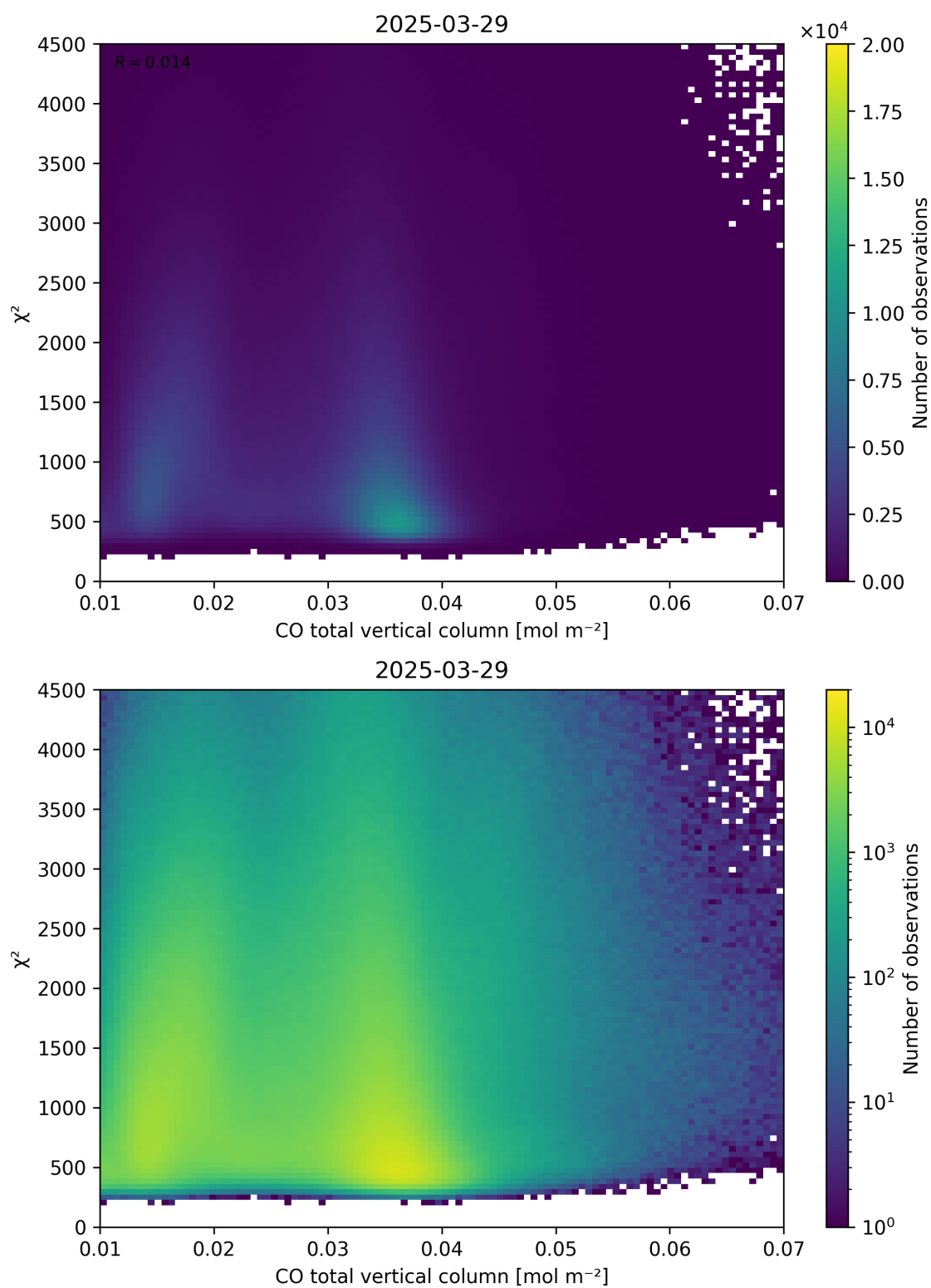
Figure 35: Scatter density plot of “CO total vertical column” against “ \chi^2 ” for 2025-03-28 to 2025-03-30.
