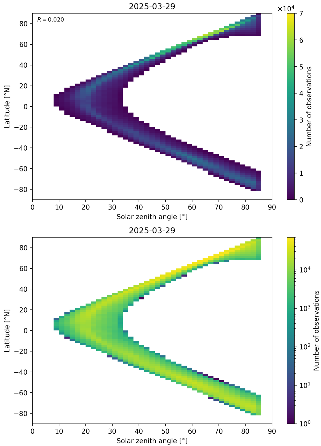
Figure 66: Scatter density plot of “Solar zenith angle” against “Latitude” for 2025-03-28 to 2025-03-30.
