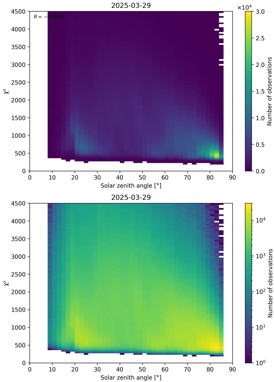
Figure 64: Scatter density plot of “Solar zenith angle” against “ \chi^2 ” for 2025-03-28 to 2025-03-30.
