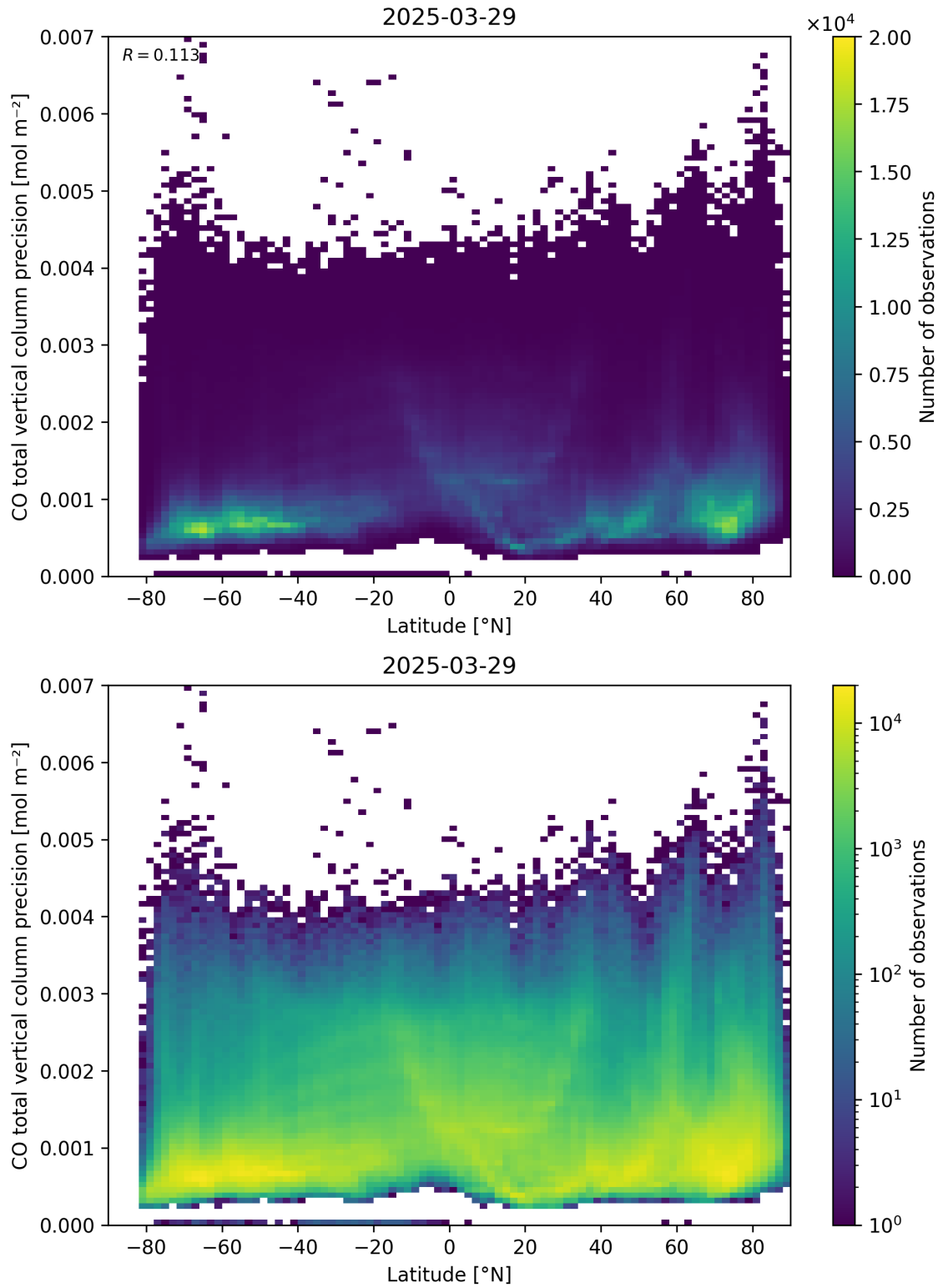
Figure 53: Scatter density plot of “Latitude” against “CO total vertical column precision” for 2025-03-28 to 2025-03-30.
