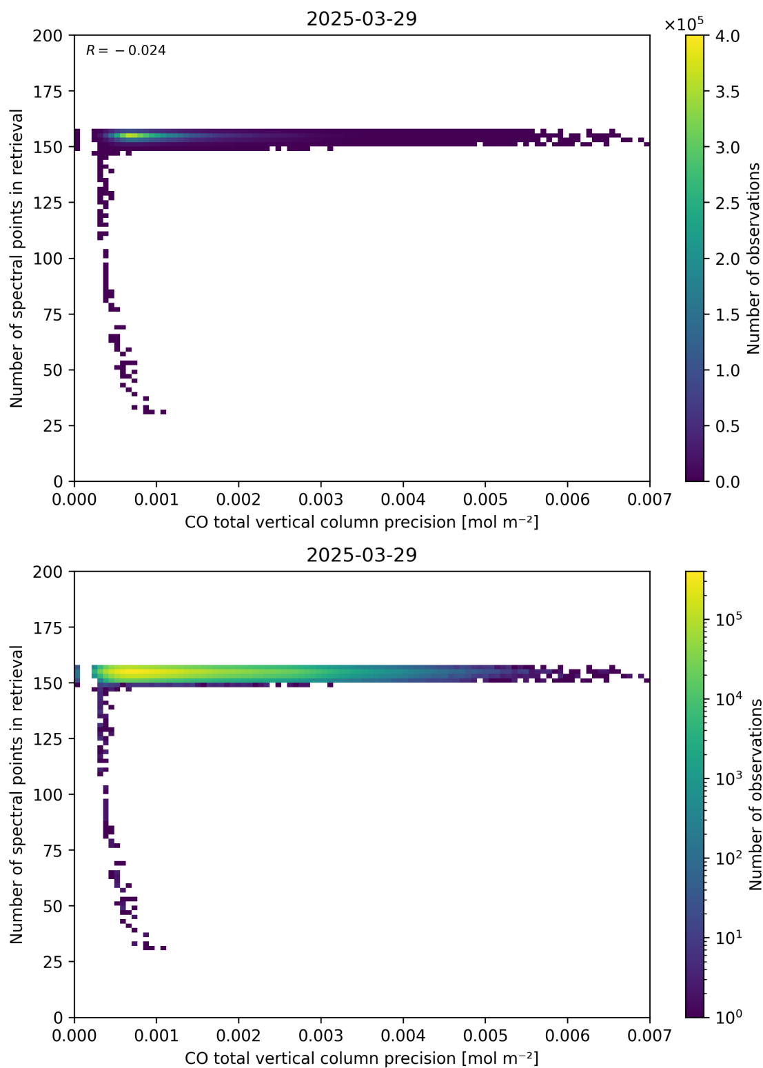
Figure 47: Scatter density plot of “CO total vertical column precision” against “Number of spectral points in retrieval” for 2025-03-28 to 2025-03-30.
