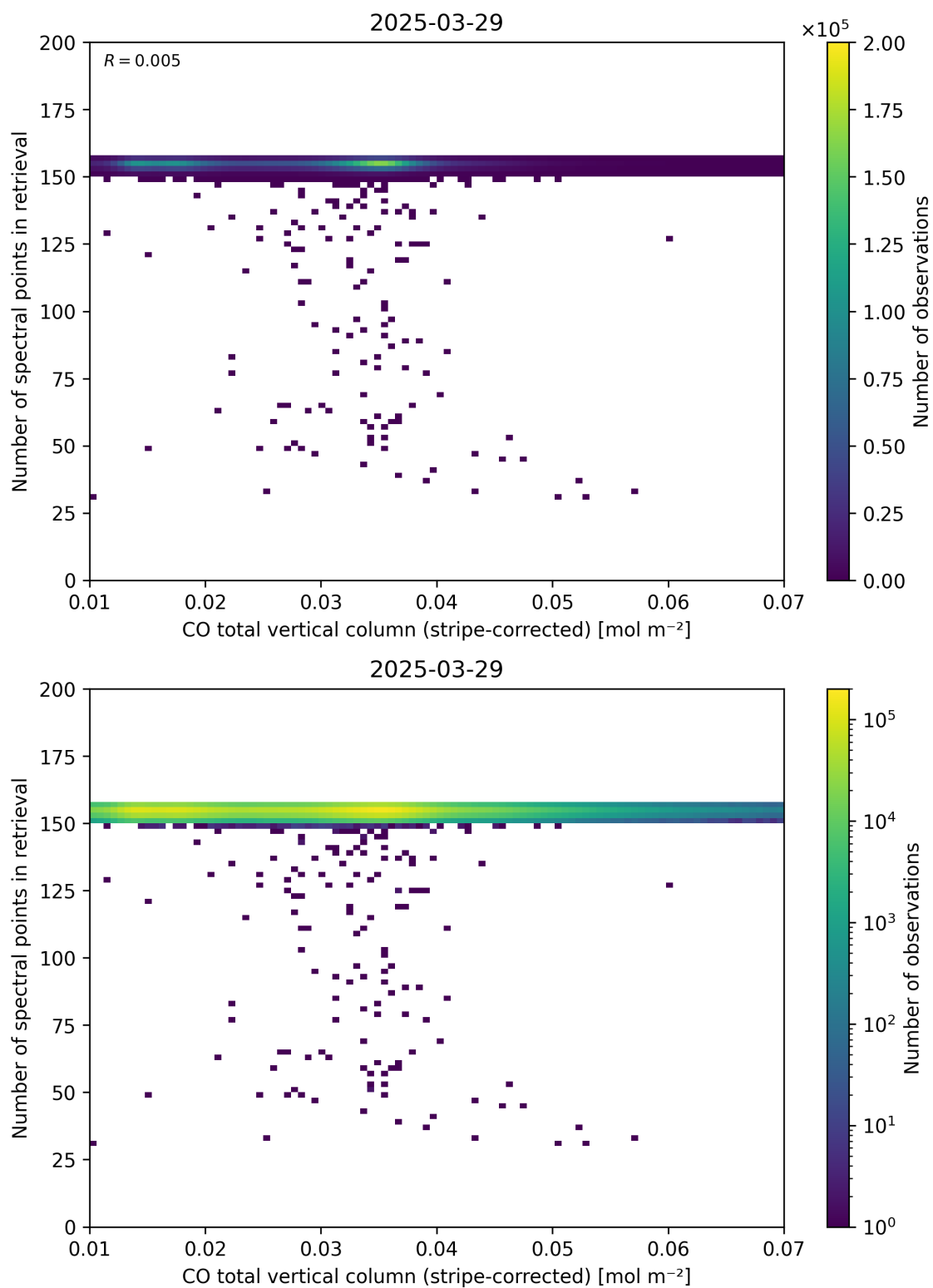
Figure 40: Scatter density plot of “CO total vertical column (stripe-corrected)” against “Number of spectral points in retrieval” for 2025-03-28 to 2025-03-30.
