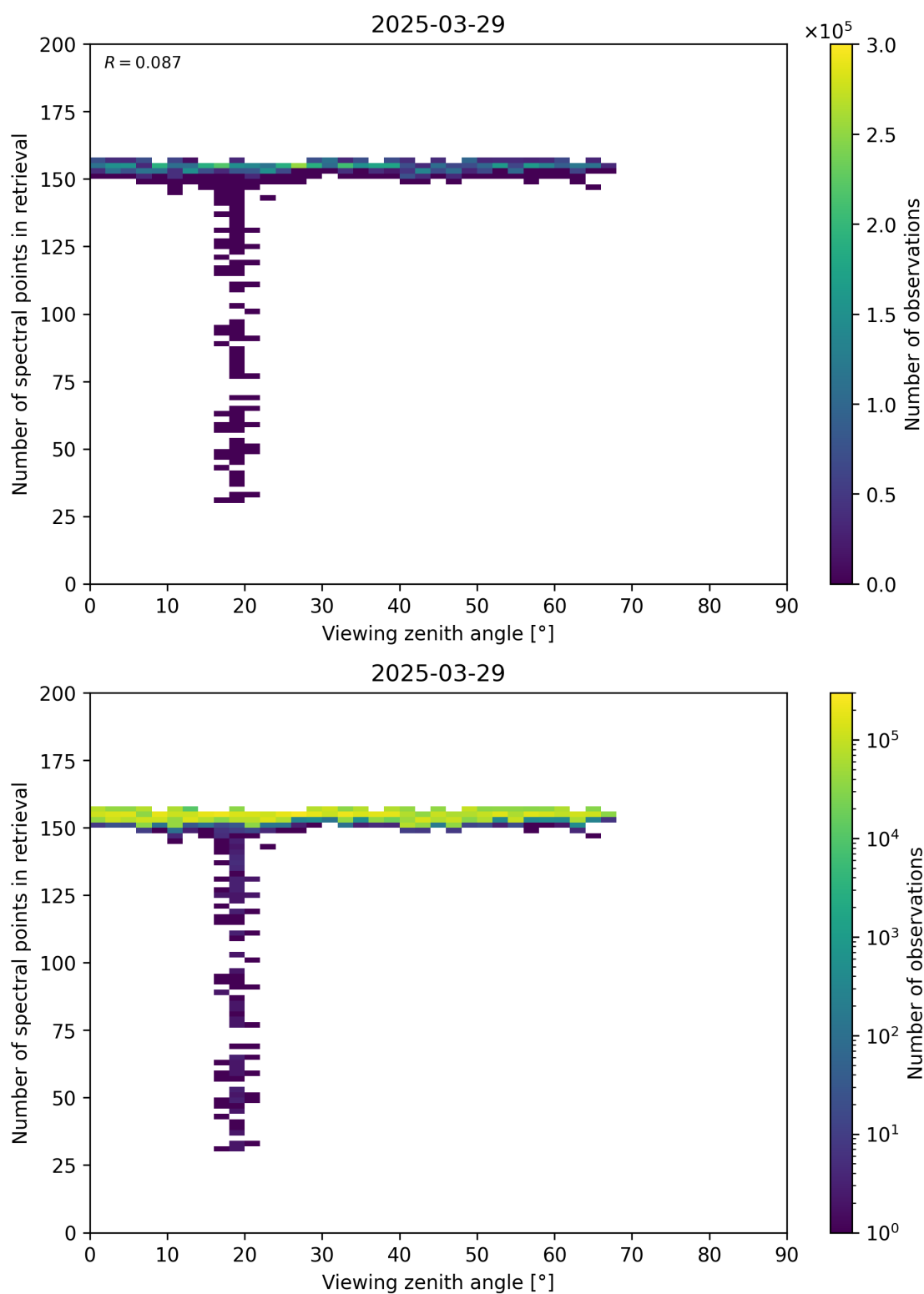
Figure 76: Scatter density plot of “Viewing zenith angle” against “Number of spectral points in retrieval” for 2025-03-28 to 2025-03-30.
