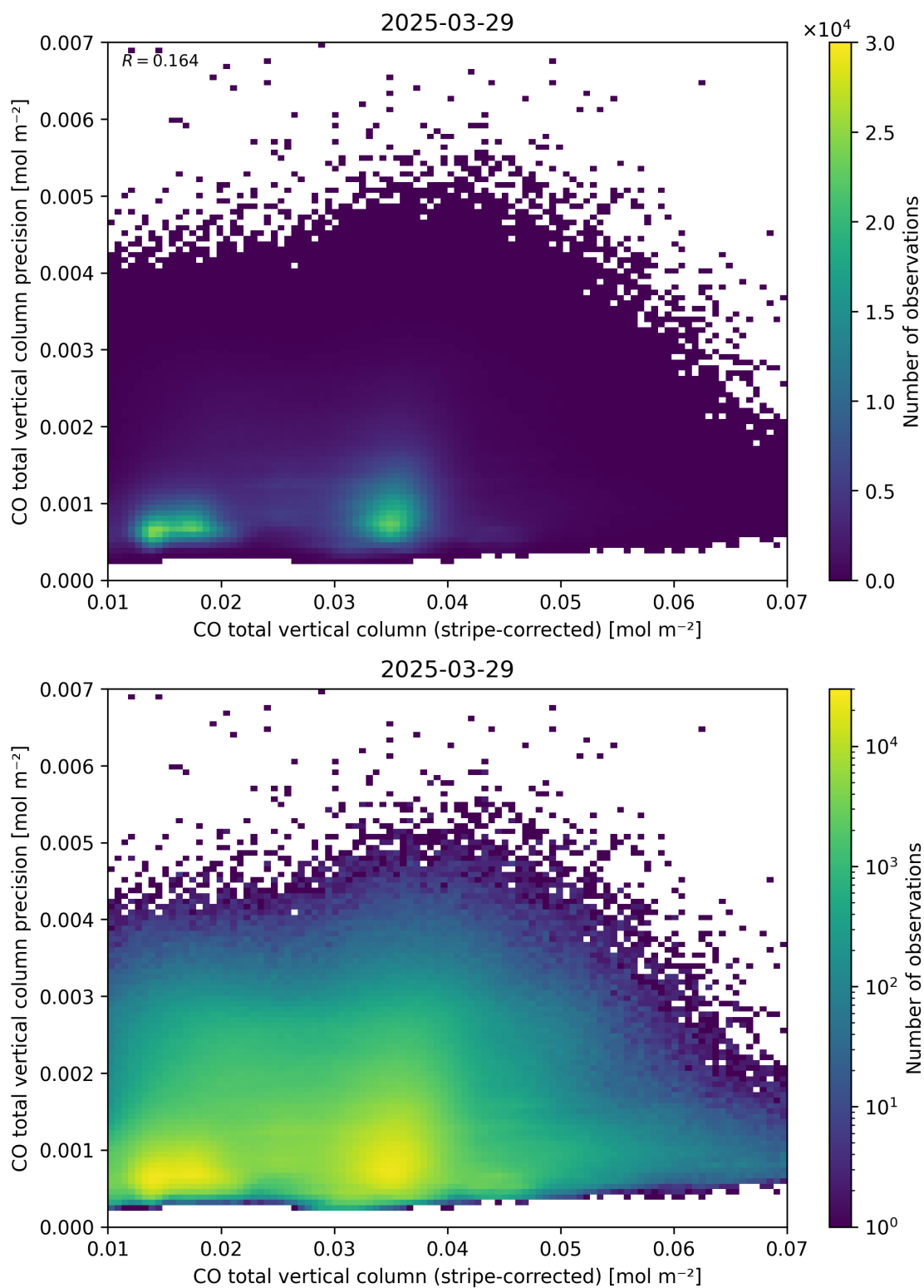
Figure 36: Scatter density plot of “CO total vertical column (stripe-corrected)” against “CO total vertical column precision” for 2025-03-28 to 2025-03-30.
