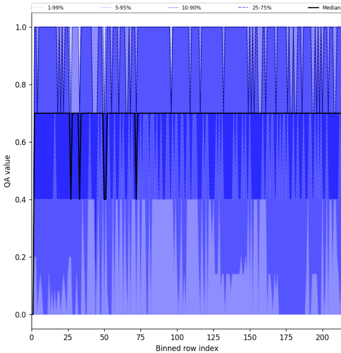
Figure 25: Along track statistics of “QA value” for 2025-03-28 to 2025-03-30
