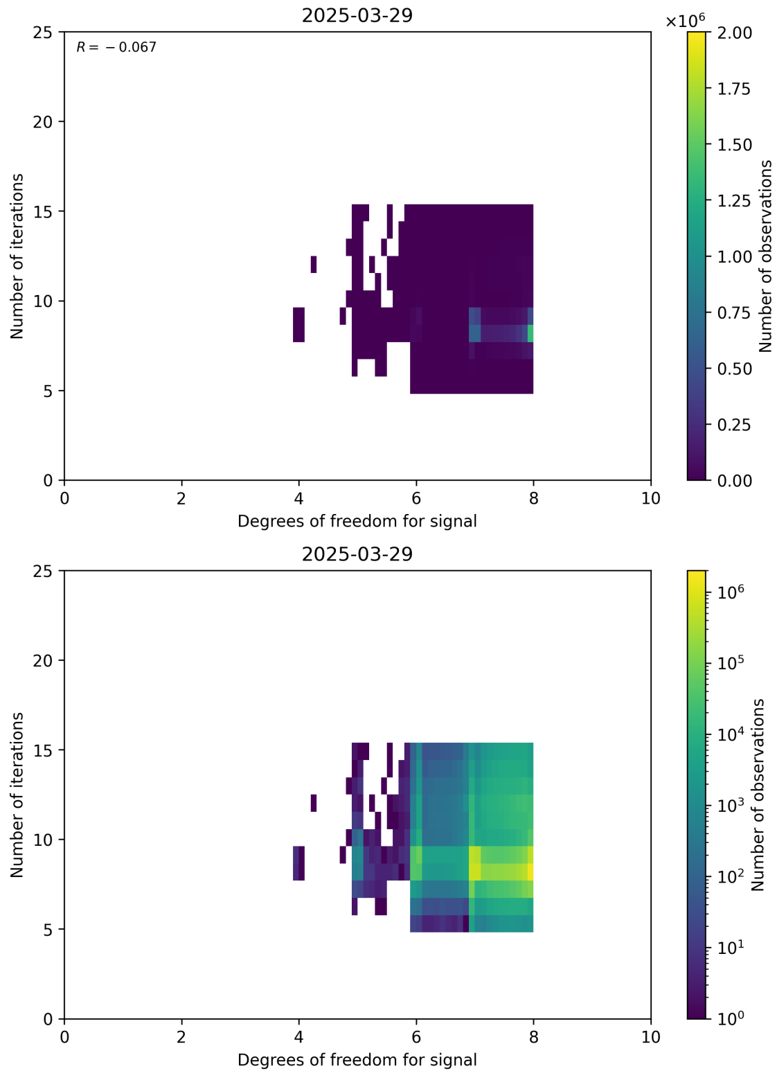
Figure 50: Scatter density plot of “Degrees of freedom for signal” against “Number of iterations” for 2025-03-28 to 2025-03-30.
