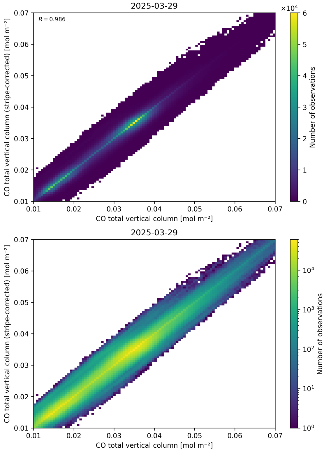
Figure 33: Scatter density plot of “CO total vertical column” against “CO total vertical column (stripe-corrected)” for 2025-03-28 to 2025-03-30.
