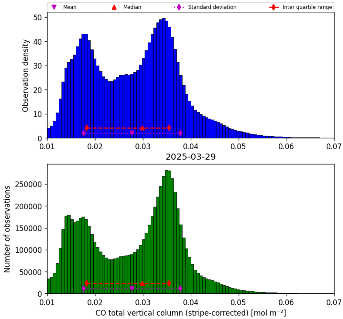
Figure 19: Histogram of “CO total vertical column (stripe-corrected)” for 2025-03-28 to 2025-03-30
