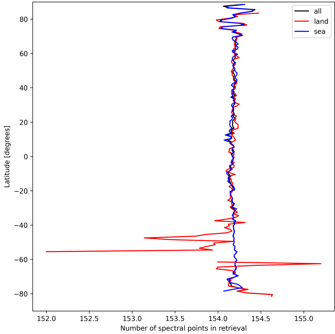
Figure 13: Zonal average of “Number of spectral points in retrieval” for 2025-03-28 to 2025-03-30.
