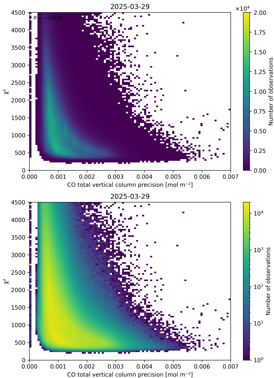
Figure 44: Scatter density plot of “CO total vertical column precision” against “ \chi^2 ” for 2025-03-28 to 2025-03-30.
