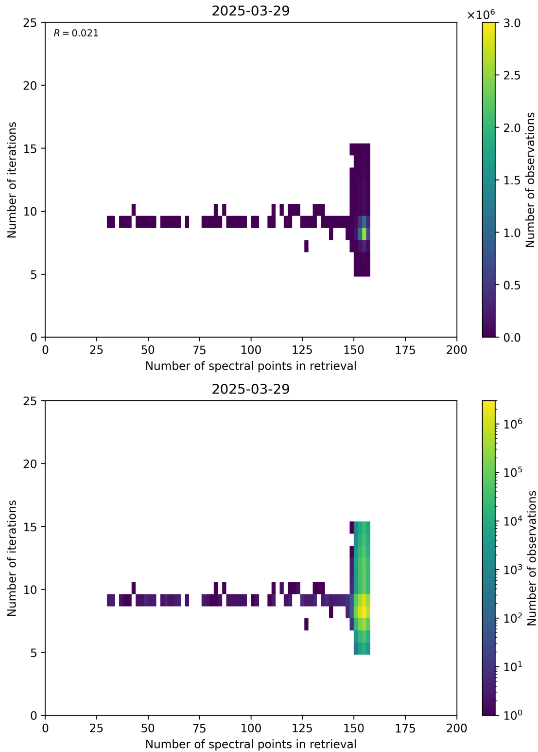
Figure 60: Scatter density plot of “Number of spectral points in retrieval” against “Number of iterations” for 2025-03-28 to 2025-03-30.
