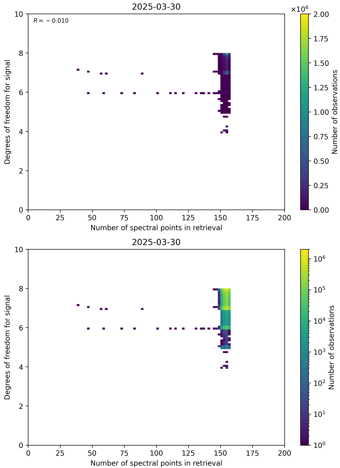
Figure 59: Scatter density plot of “Number of spectral points in retrieval” against “Degrees of freedom for signal” for 2025-03-29 to 2025-03-31.
