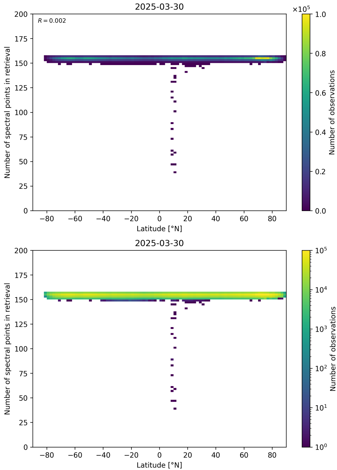
Figure 57: Scatter density plot of “Latitude” against “Number of spectral points in retrieval” for 2025-03-29 to 2025-03-31.
