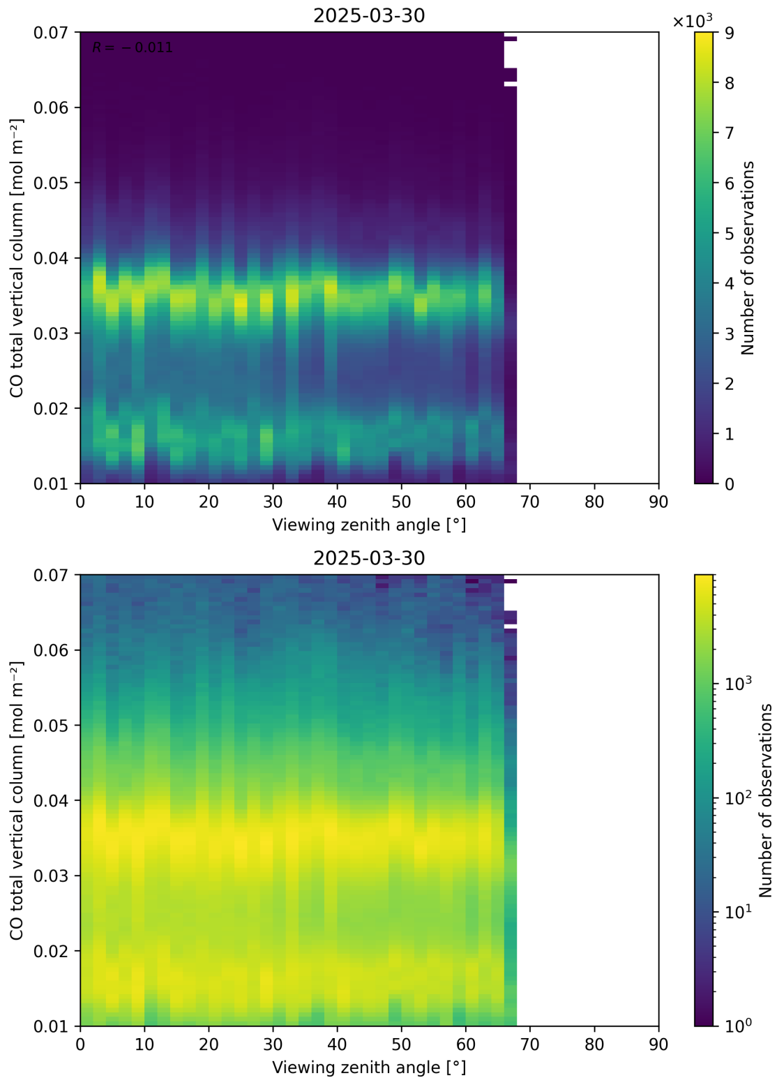
Figure 69: Scatter density plot of “Viewing zenith angle” against “CO total vertical column” for 2025-03-29 to 2025-03-31.
