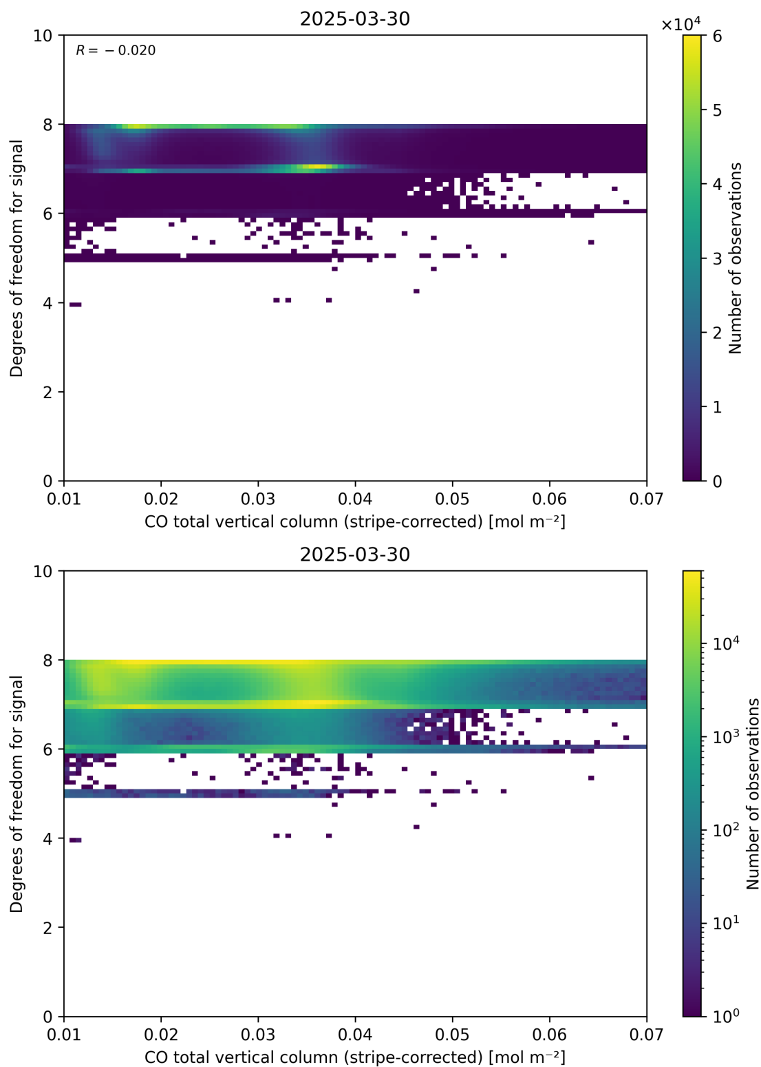
Figure 38: Scatter density plot of “CO total vertical column (stripe-corrected)” against “Degrees of freedom for signal” for 2025-03-29 to 2025-03-31.
