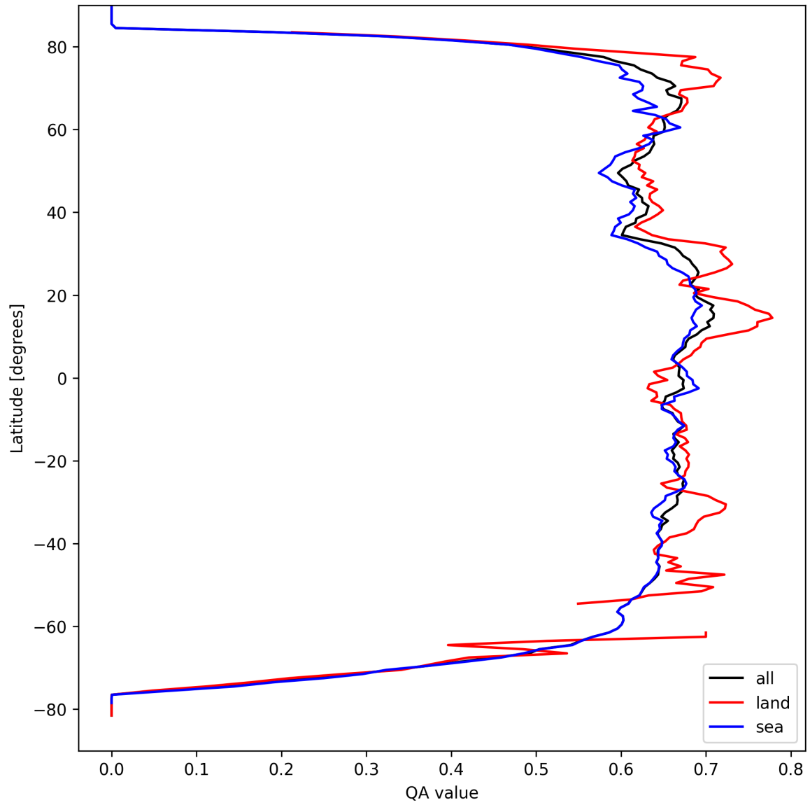
Figure 9: Zonal average of “QA value” for 2025-03-29 to 2025-03-31.
