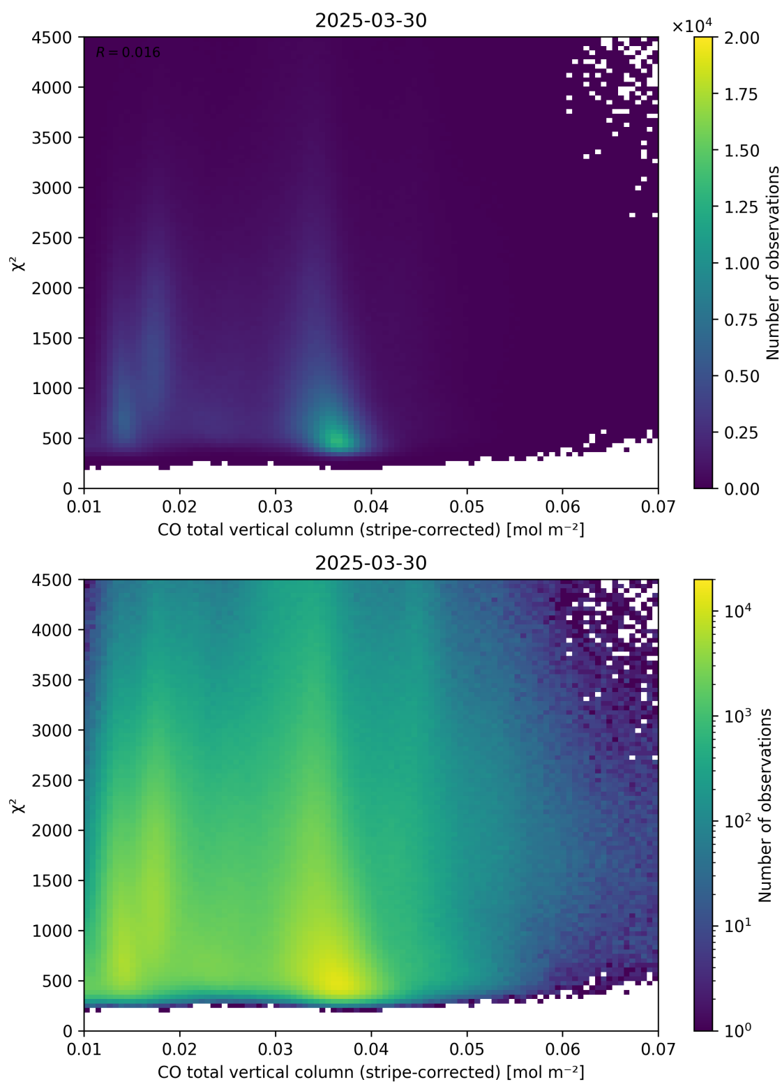
Figure 37: Scatter density plot of “CO total vertical column (stripe-corrected)” against “ \chi^2 ” for 2025-03-29 to 2025-03-31.
