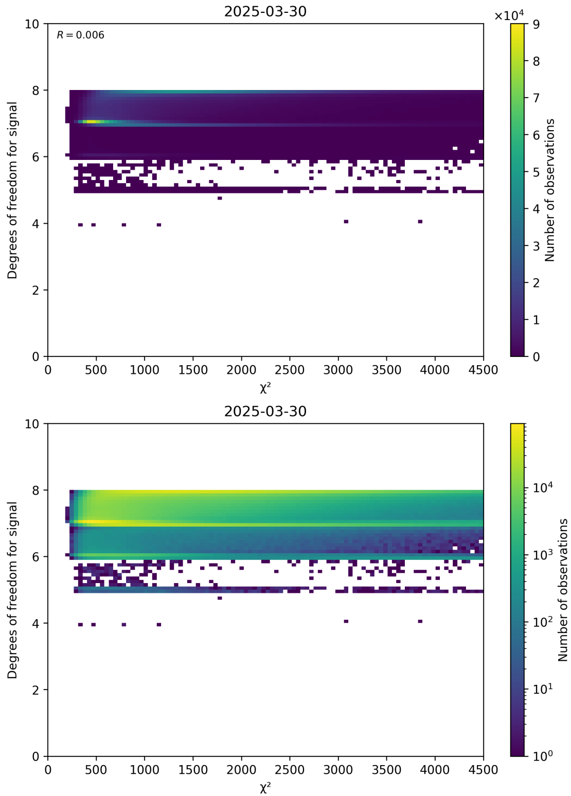
Figure 48: Scatter density plot of “ \chi^2 ” against “Degrees of freedom for signal” for 2025-03-29 to 2025-03-31.
