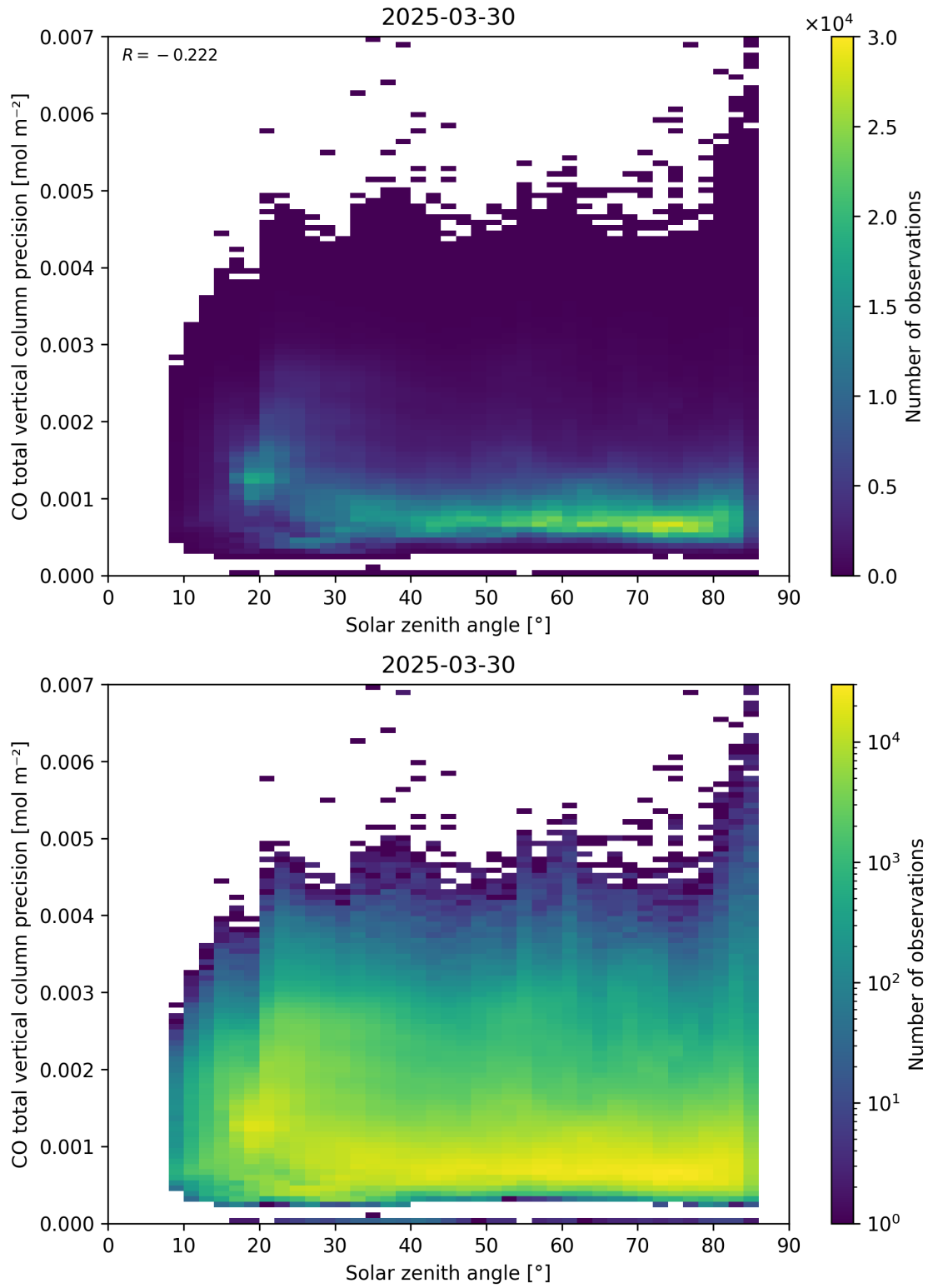
Figure 63: Scatter density plot of “Solar zenith angle” against “CO total vertical column precision” for 2025-03-29 to 2025-03-31.
