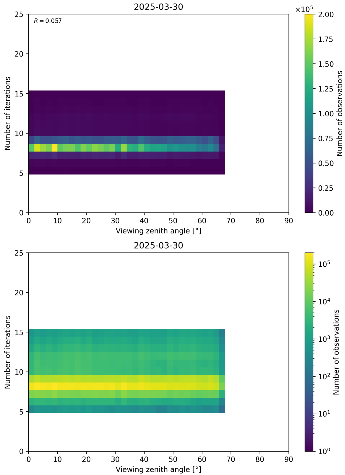
Figure 75: Scatter density plot of “Viewing zenith angle” against “Number of iterations” for 2025-03-29 to 2025-03-31.
