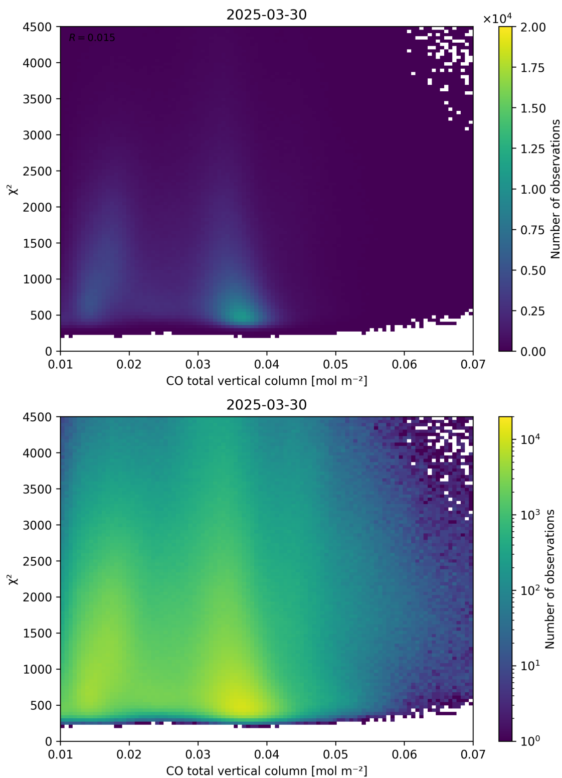
Figure 35: Scatter density plot of “CO total vertical column” against “ \chi^2 ” for 2025-03-29 to 2025-03-31.
