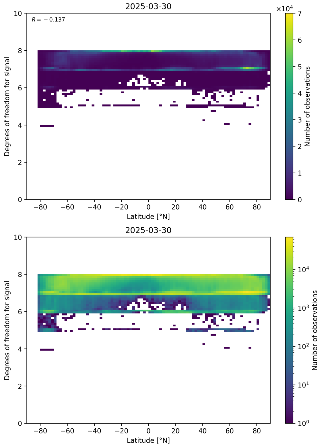
Figure 55: Scatter density plot of “Latitude” against “Degrees of freedom for signal” for 2025-03-29 to 2025-03-31.
