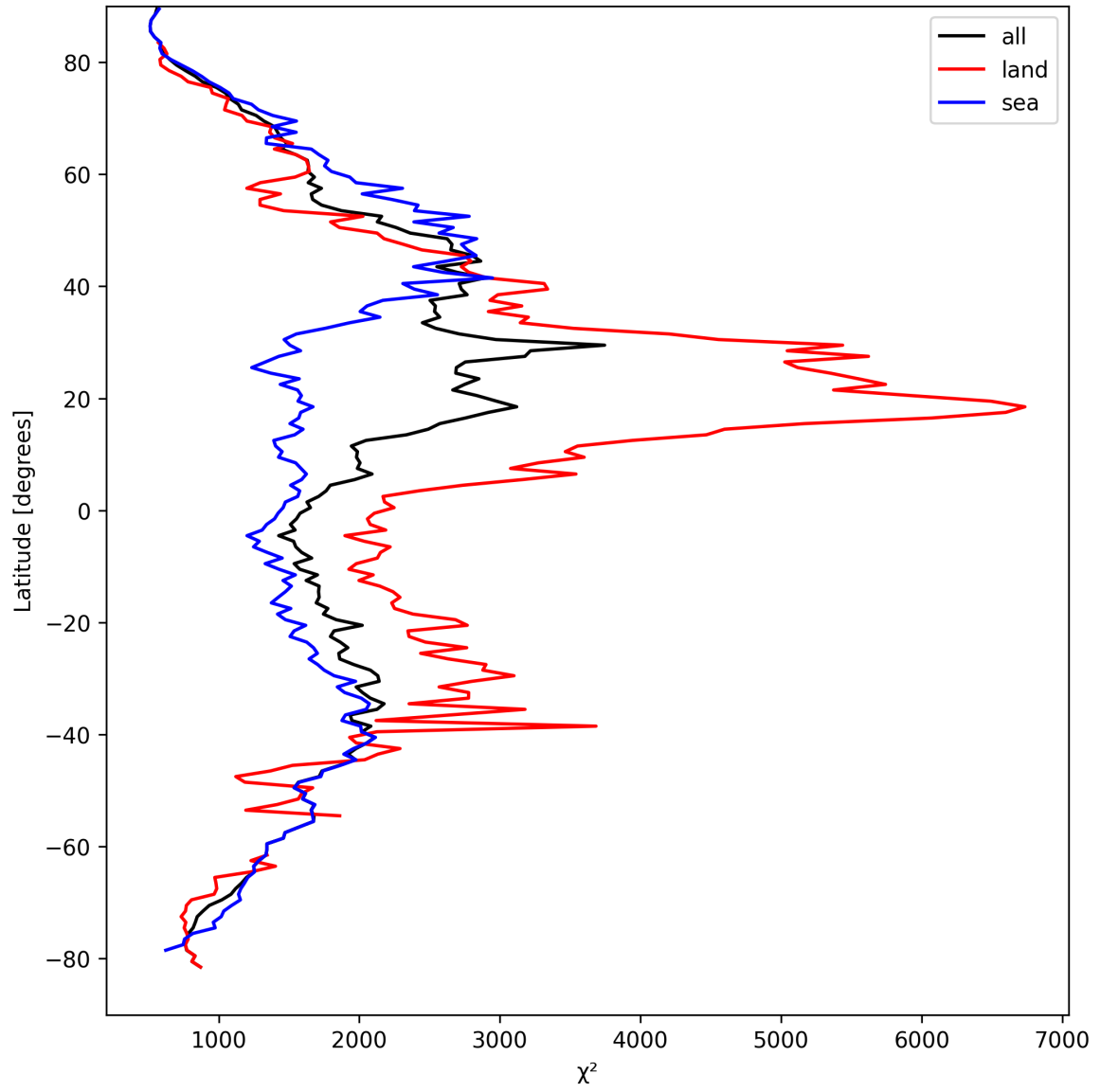
Figure 14: Zonal average of “ \chi^2 ” for 2025-03-29 to 2025-03-31.
