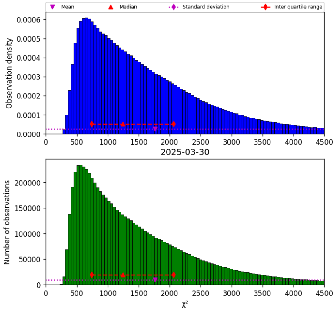
Figure 22: Histogram of “ \chi^2 ” for 2025-03-29 to 2025-03-31
