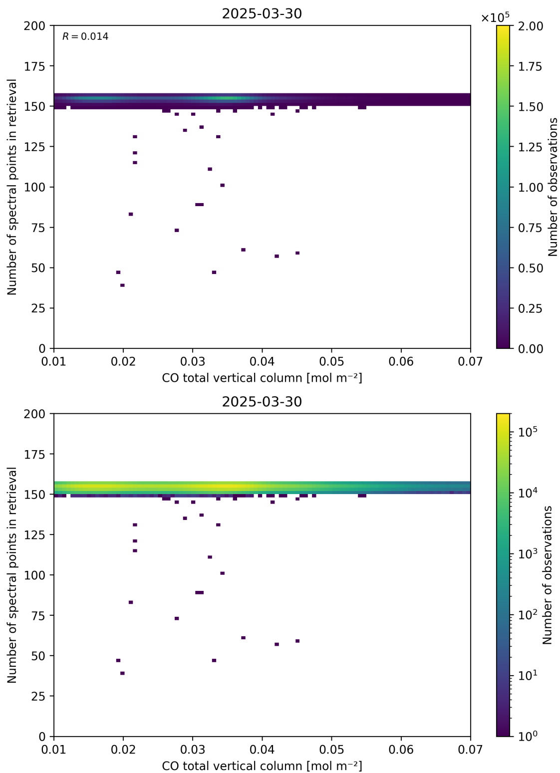
Figure 43: Scatter density plot of “CO total vertical column” against “Number of spectral points in retrieval” for 2025-03-29 to 2025-03-31.
