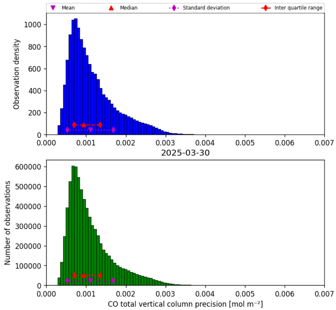
Figure 20: Histogram of “CO total vertical column precision” for 2025-03-29 to 2025-03-31
