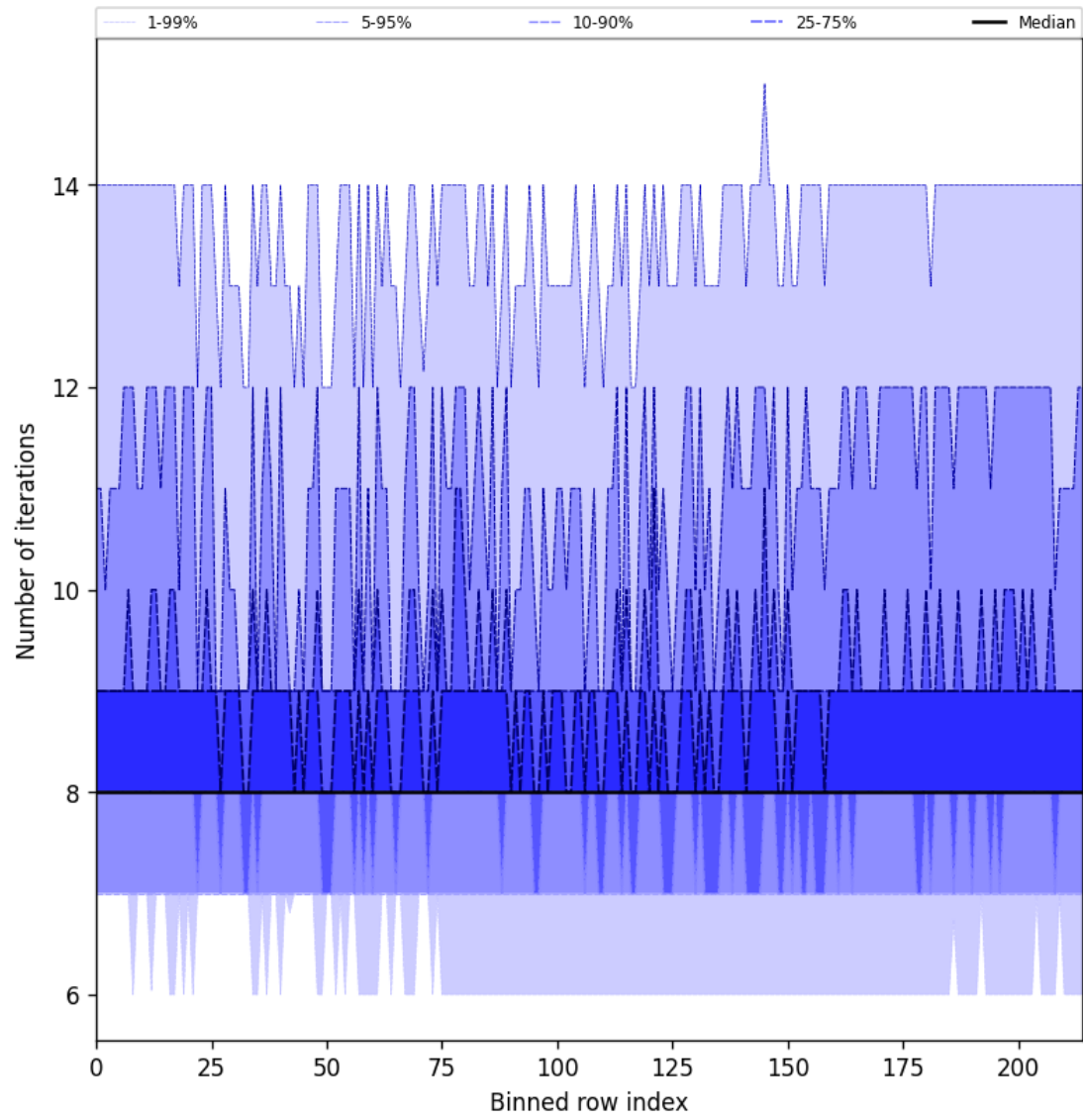
Figure 32: Along track statistics of “Number of iterations” for 2025-03-29 to 2025-03-31
