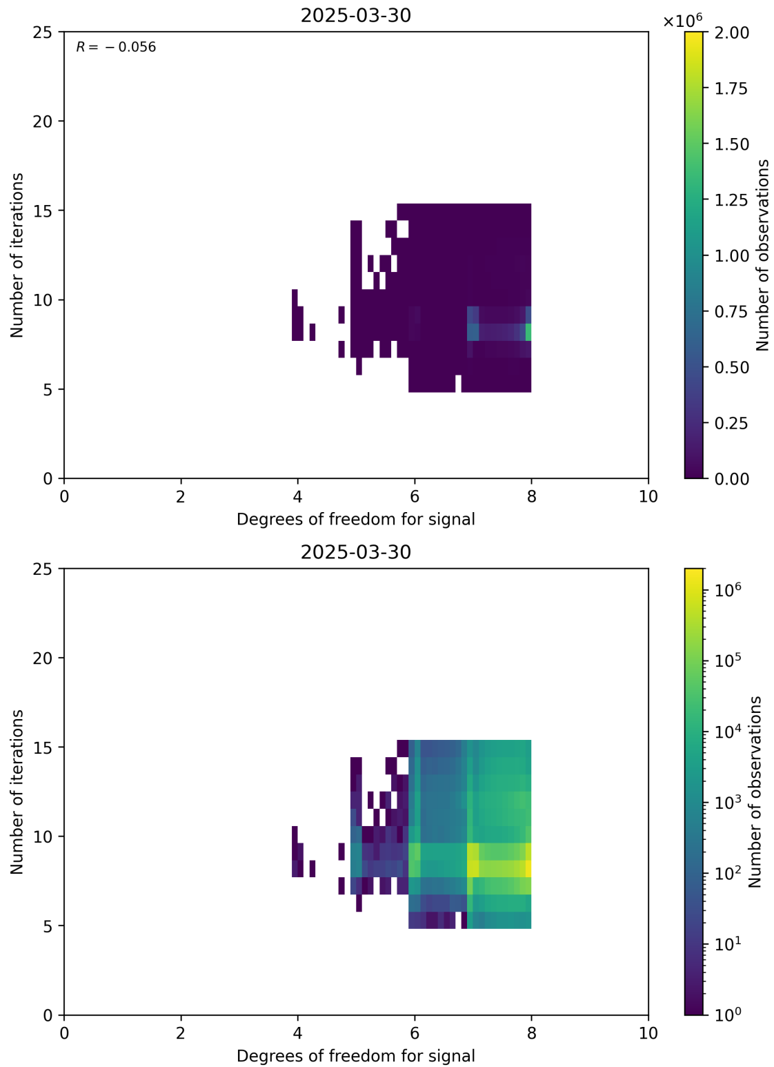
Figure 50: Scatter density plot of “Degrees of freedom for signal” against “Number of iterations” for 2025-03-29 to 2025-03-31.
