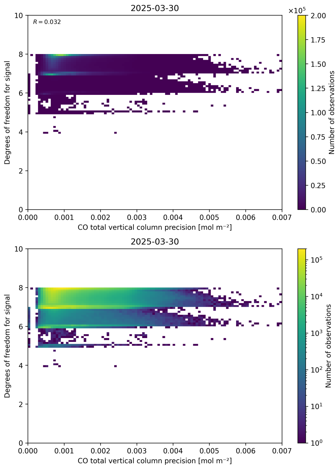
Figure 45: Scatter density plot of “CO total vertical column precision” against “Degrees of freedom for signal” for 2025-03-29 to 2025-03-31.
