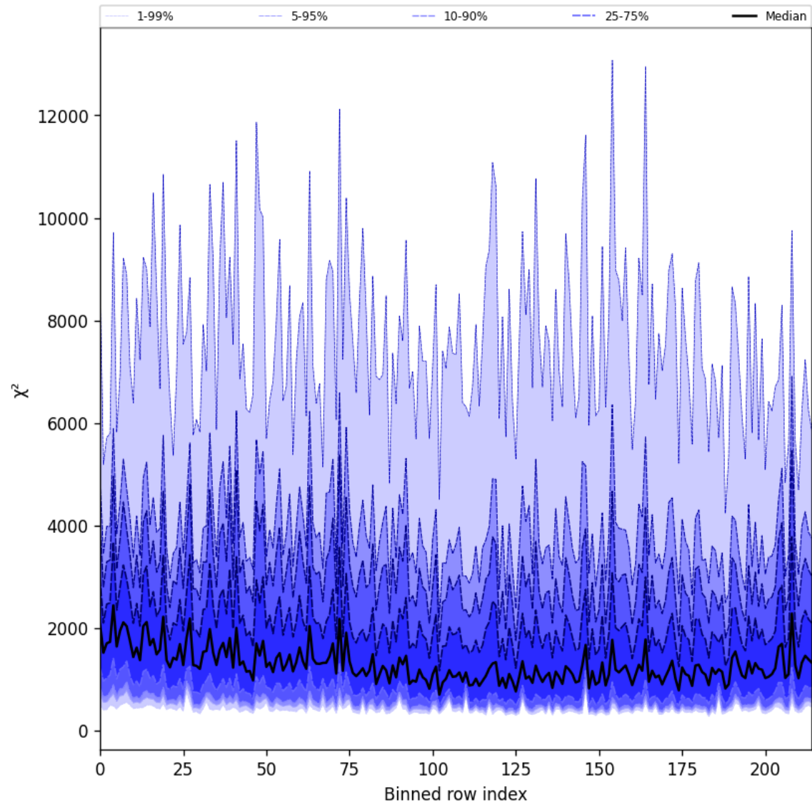
Figure 30: Along track statistics of “ \chi^2 ” for 2025-03-29 to 2025-03-31
