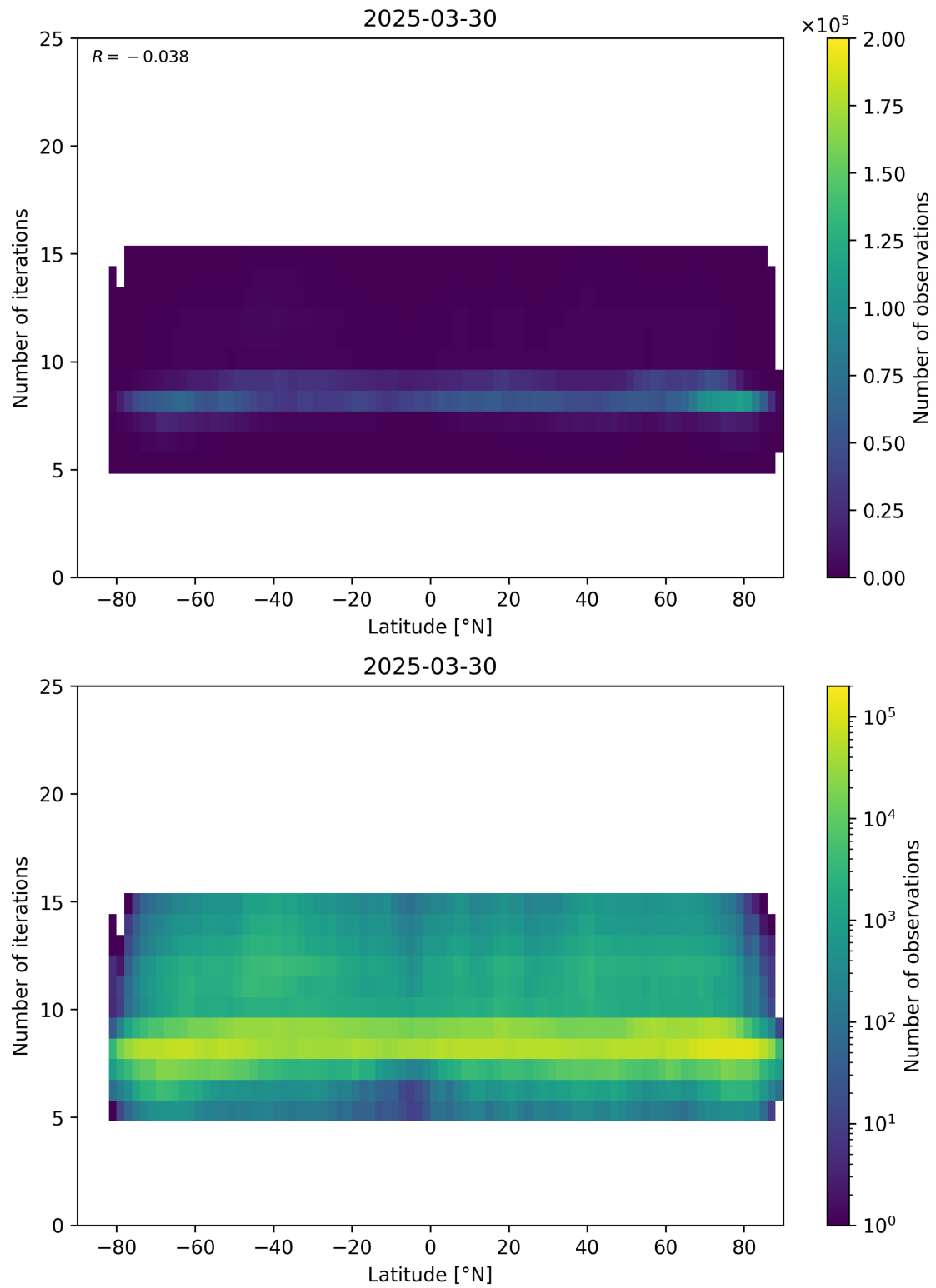
Figure 56: Scatter density plot of “Latitude” against “Number of iterations” for 2025-03-29 to 2025-03-31.
