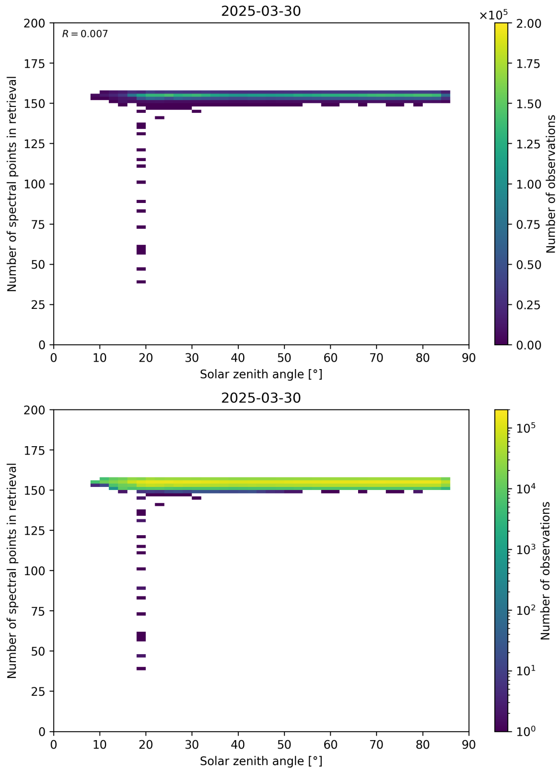
Figure 68: Scatter density plot of “Solar zenith angle” against “Number of spectral points in retrieval” for 2025-03-29 to 2025-03-31.
