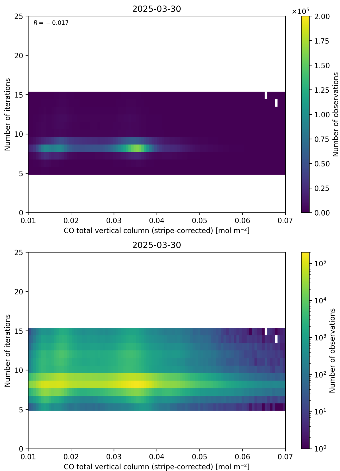
Figure 39: Scatter density plot of “CO total vertical column (stripe-corrected)” against “Number of iterations” for 2025-03-29 to 2025-03-31.
