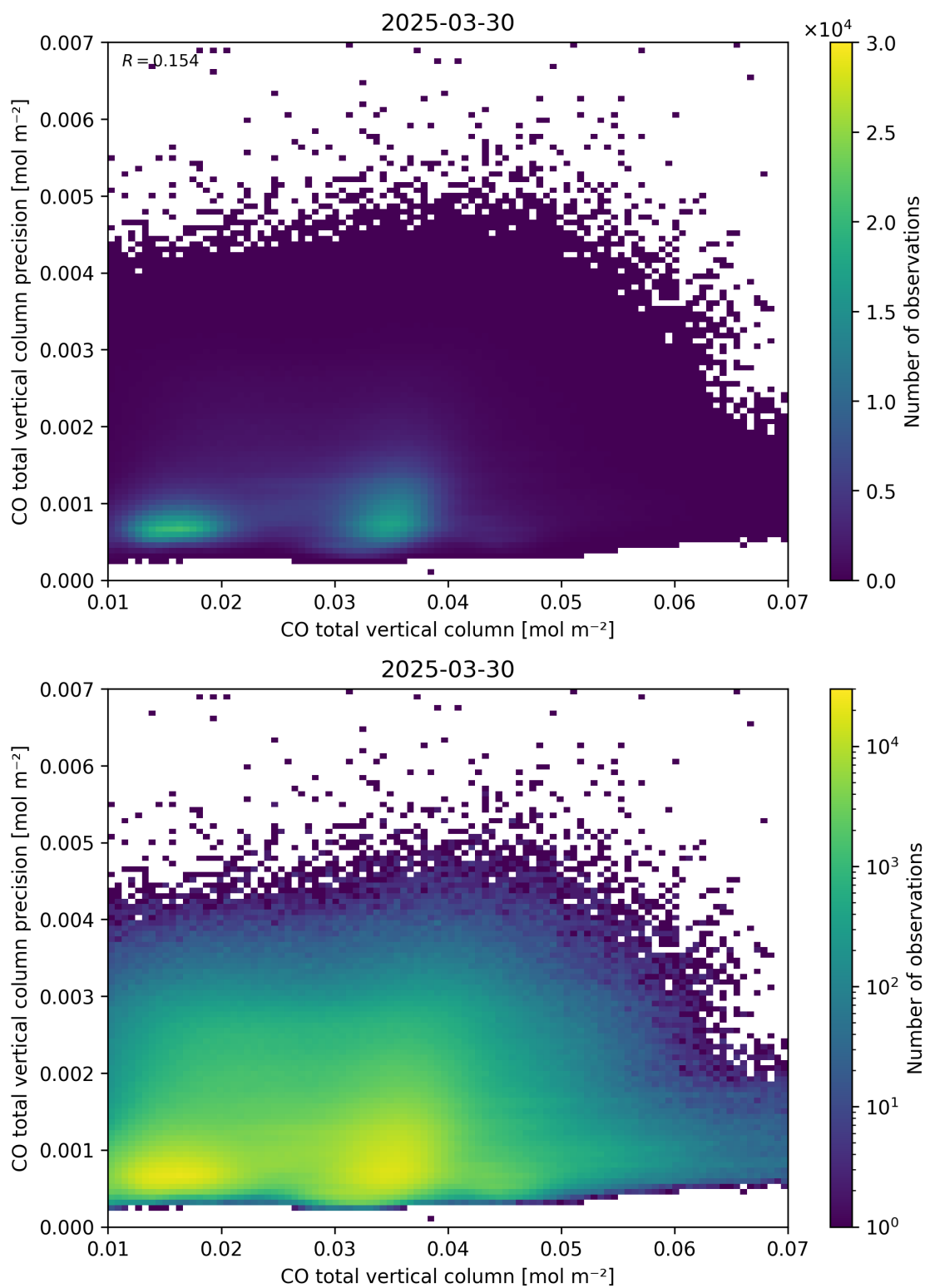
Figure 34: Scatter density plot of “CO total vertical column” against “CO total vertical column precision” for 2025-03-29 to 2025-03-31.
