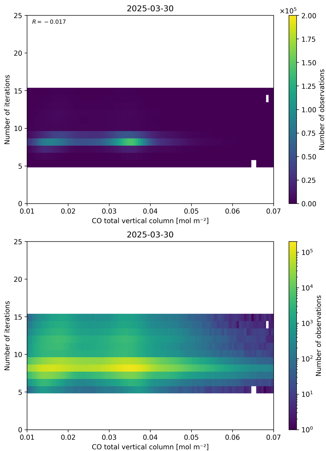
Figure 42: Scatter density plot of “CO total vertical column” against “Number of iterations” for 2025-03-29 to 2025-03-31.
