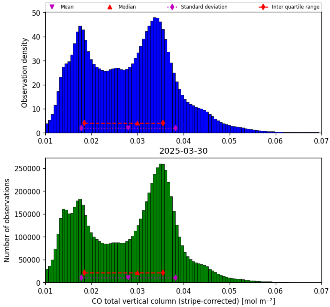
Figure 19: Histogram of “CO total vertical column (stripe-corrected)” for 2025-03-29 to 2025-03-31
