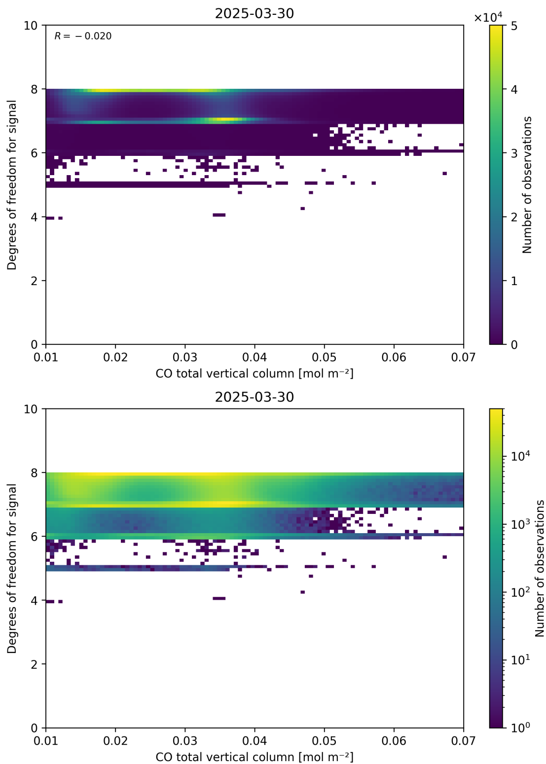
Figure 41: Scatter density plot of “CO total vertical column” against “Degrees of freedom for signal” for 2025-03-29 to 2025-03-31.
