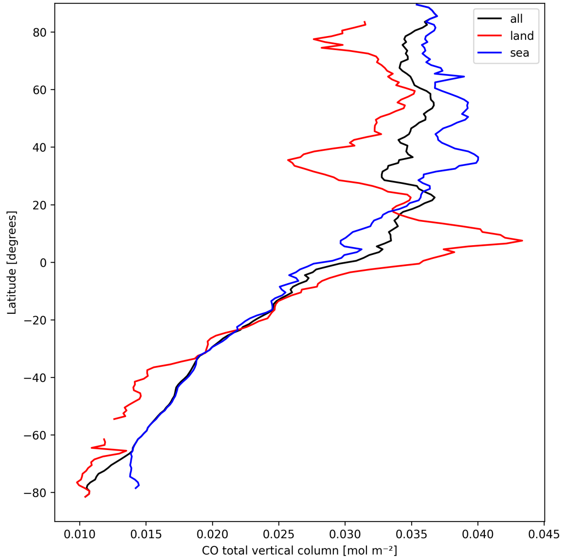
Figure 10: Zonal average of “CO total vertical column” for 2025-03-29 to 2025-03-31.
