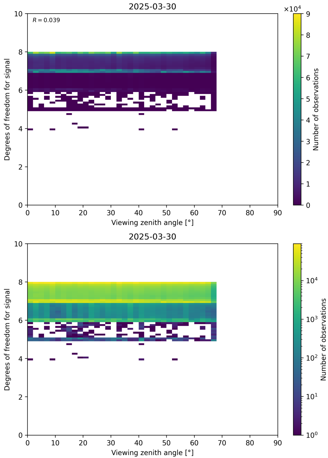
Figure 73: Scatter density plot of “Viewing zenith angle” against “Degrees of freedom for signal” for 2025-03-29 to 2025-03-31.
