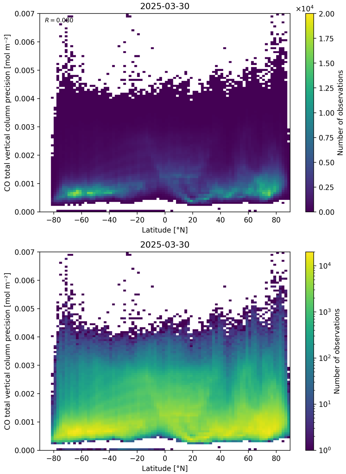
Figure 53: Scatter density plot of “Latitude” against “CO total vertical column precision” for 2025-03-29 to 2025-03-31.
