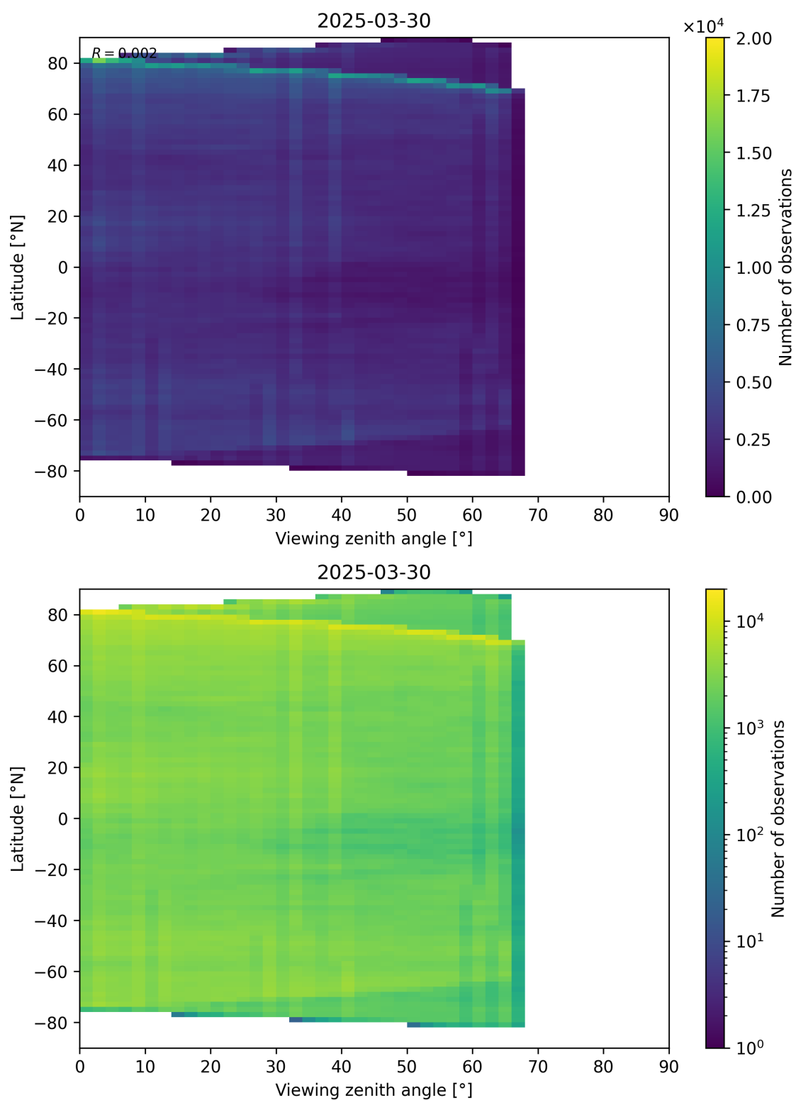
Figure 74: Scatter density plot of “Viewing zenith angle” against “Latitude” for 2025-03-29 to 2025-03-31.
