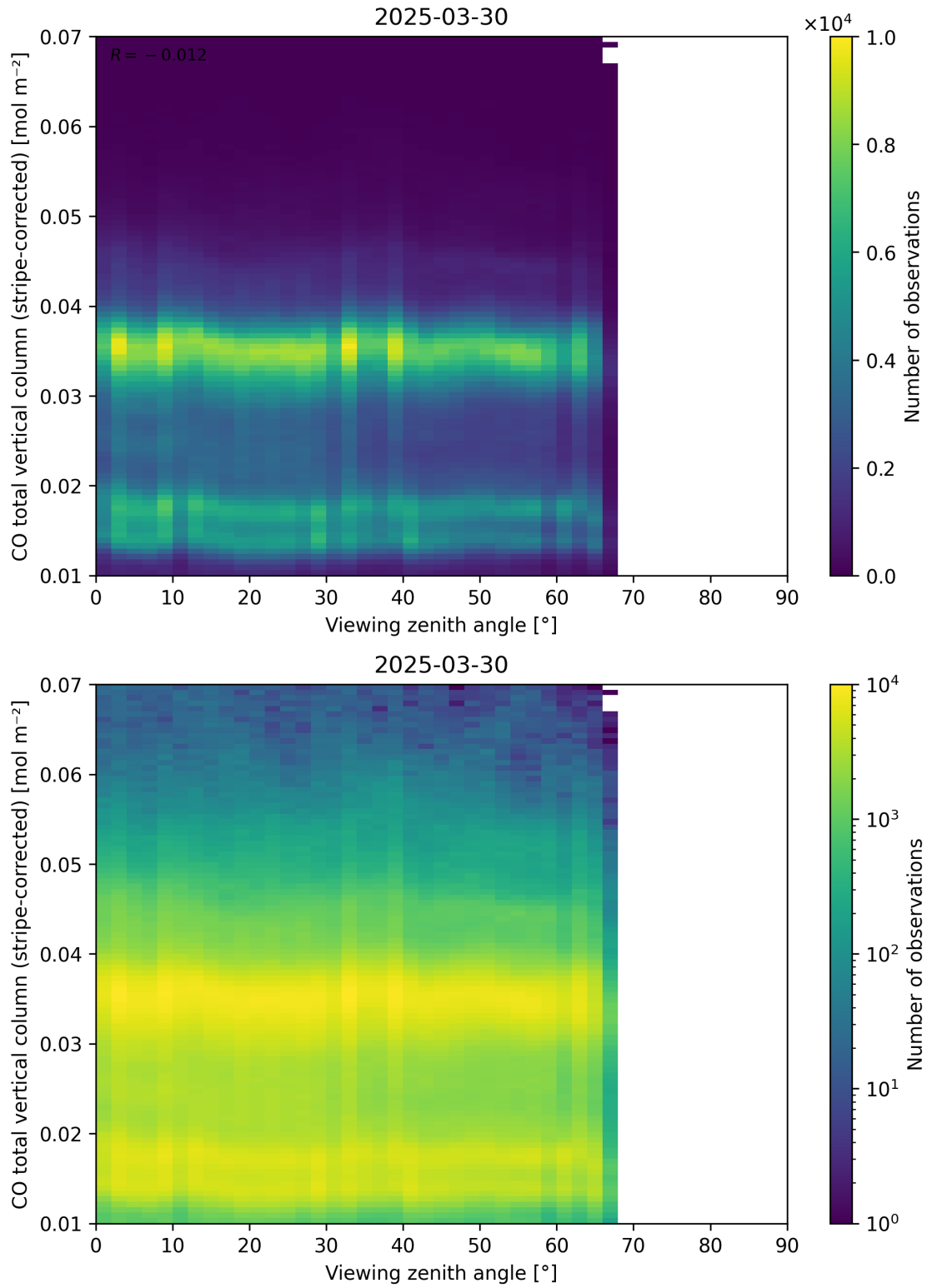
Figure 70: Scatter density plot of “Viewing zenith angle” against “CO total vertical column (stripe-corrected)” for 2025-03-29 to 2025-03-31.
