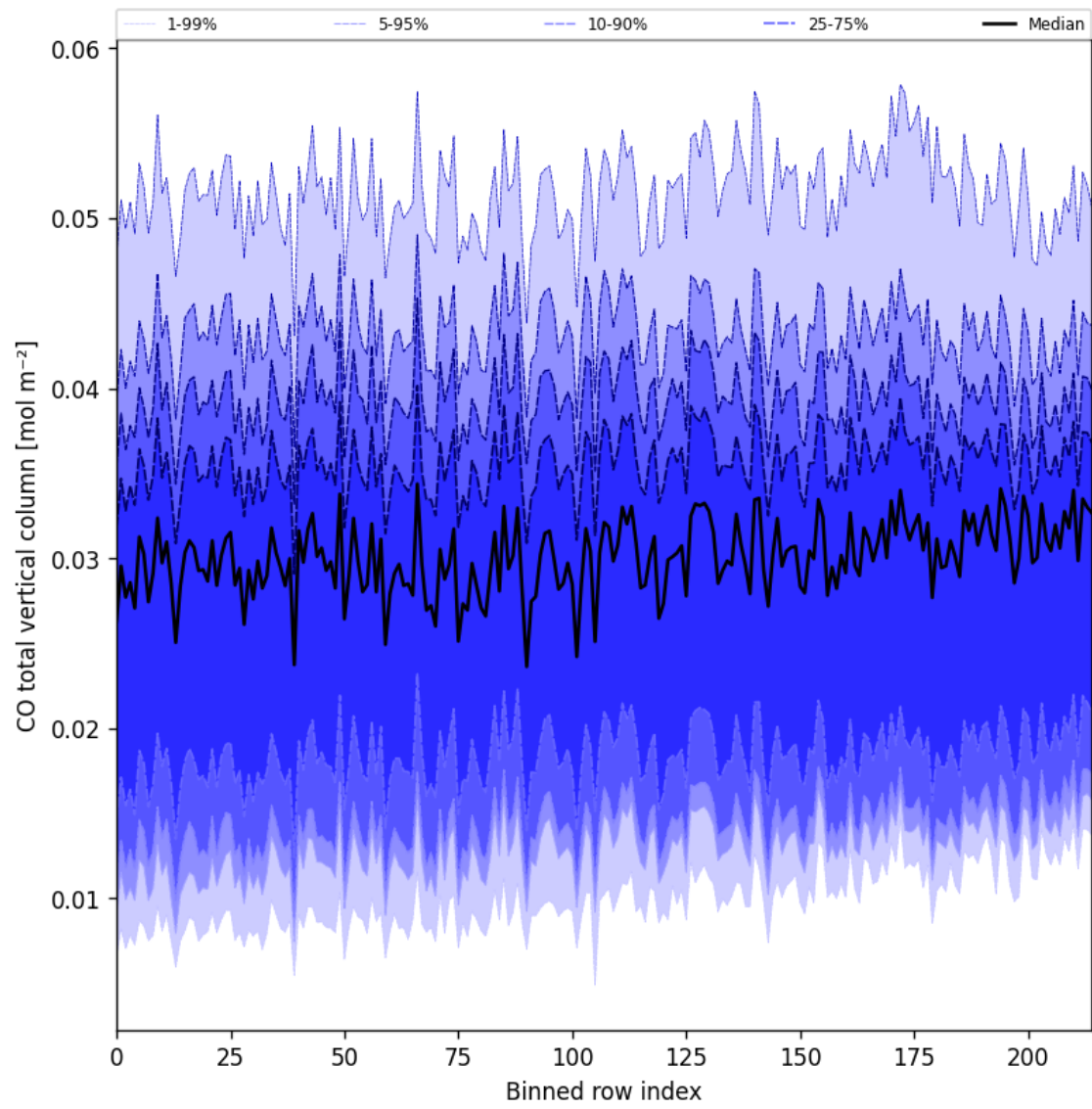
Figure 26: Along track statistics of “CO total vertical column” for 2025-03-29 to 2025-03-31
