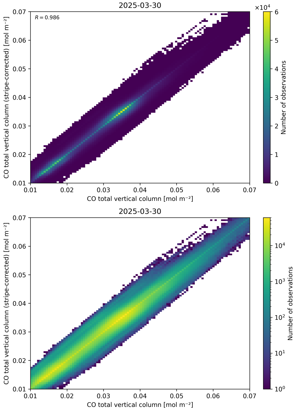
Figure 33: Scatter density plot of “CO total vertical column” against “CO total vertical column (stripe-corrected)” for 2025-03-29 to 2025-03-31.
