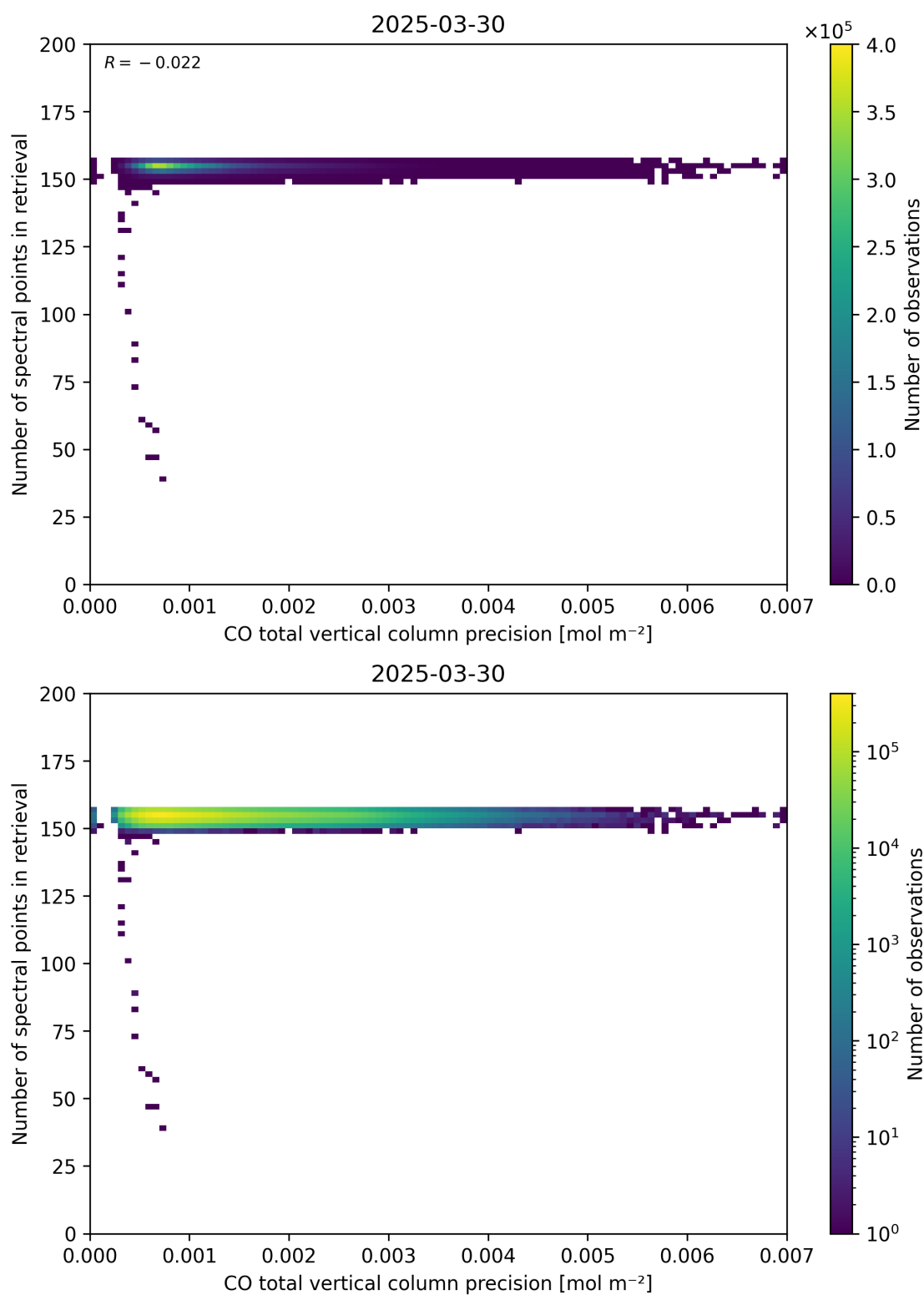
Figure 47: Scatter density plot of “CO total vertical column precision” against “Number of spectral points in retrieval” for 2025-03-29 to 2025-03-31.
