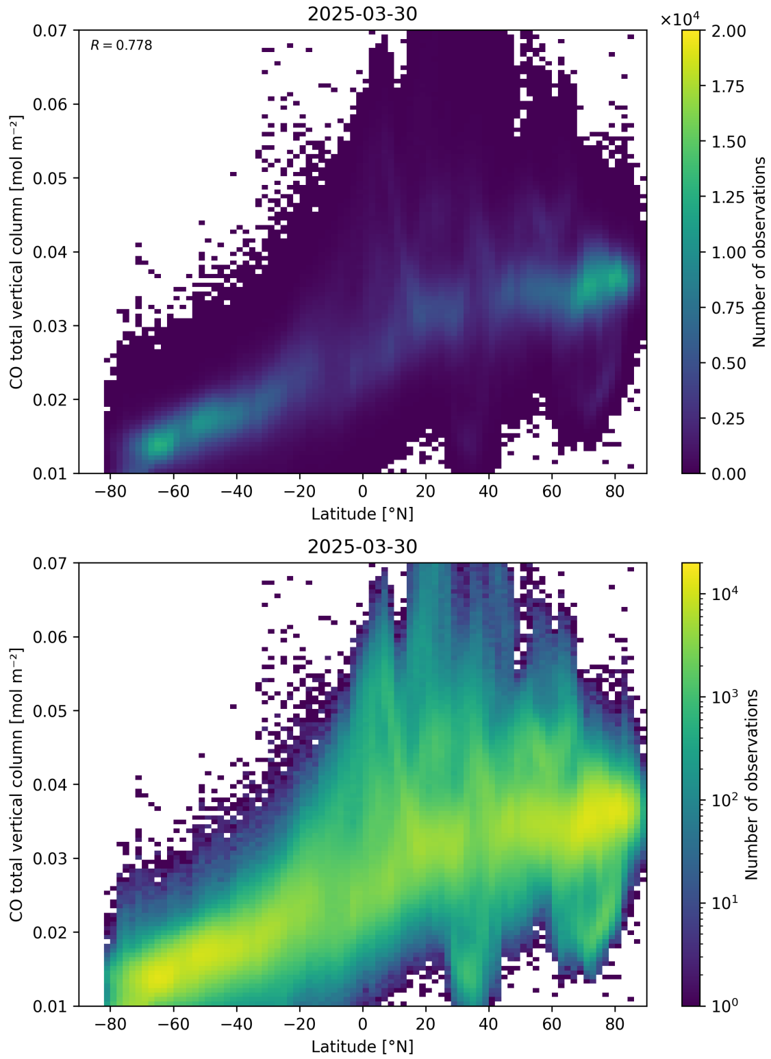
Figure 51: Scatter density plot of “Latitude” against “CO total vertical column” for 2025-03-29 to 2025-03-31.
