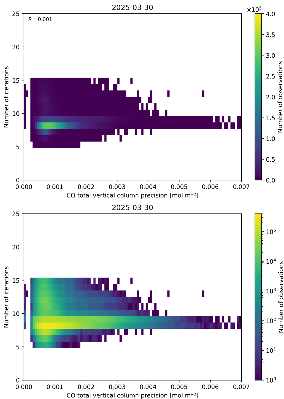
Figure 46: Scatter density plot of “CO total vertical column precision” against “Number of iterations” for 2025-03-29 to 2025-03-31.
