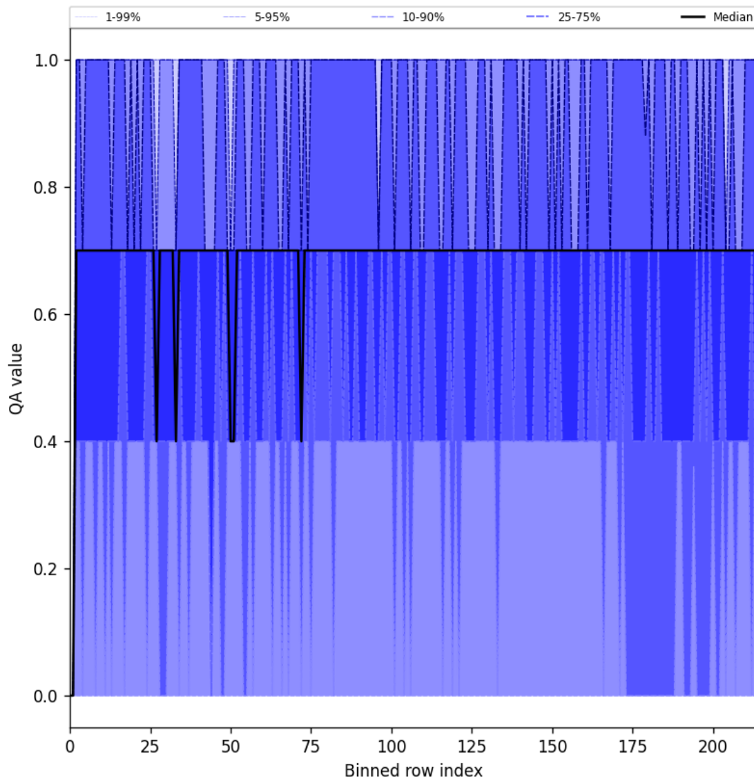
Figure 25: Along track statistics of “QA value” for 2025-03-29 to 2025-03-31
