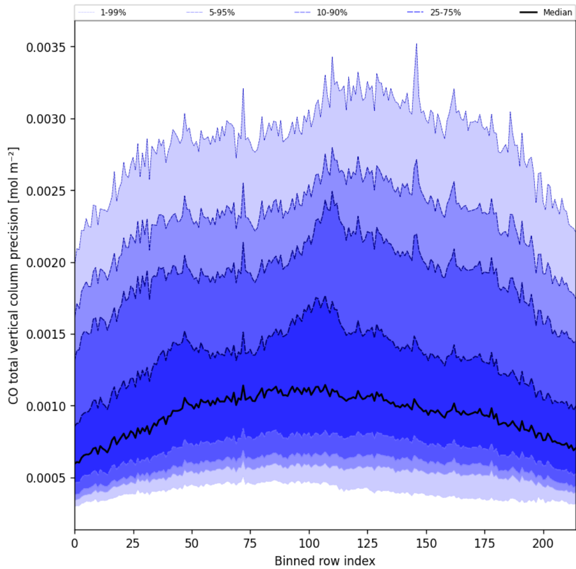
Figure 28: Along track statistics of “CO total vertical column precision” for 2025-03-29 to 2025-03-31
