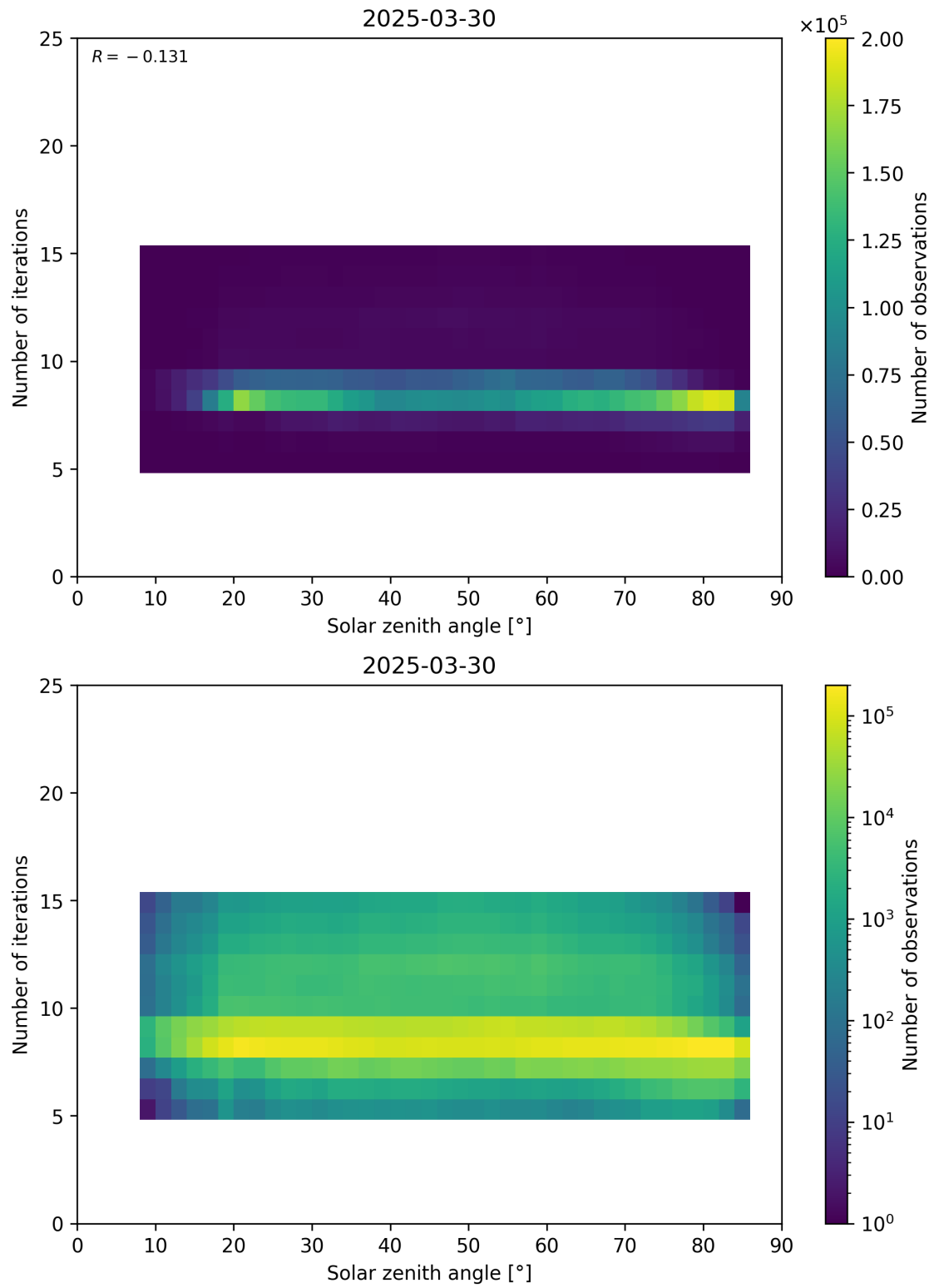
Figure 67: Scatter density plot of “Solar zenith angle” against “Number of iterations” for 2025-03-29 to 2025-03-31.
