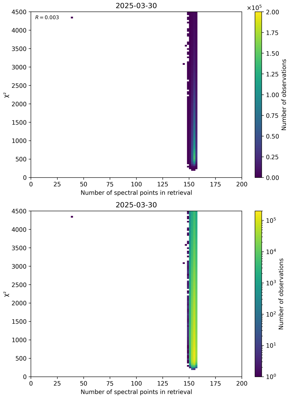
Figure 58: Scatter density plot of “Number of spectral points in retrieval” against “ \chi^2 ” for 2025-03-29 to 2025-03-31.
