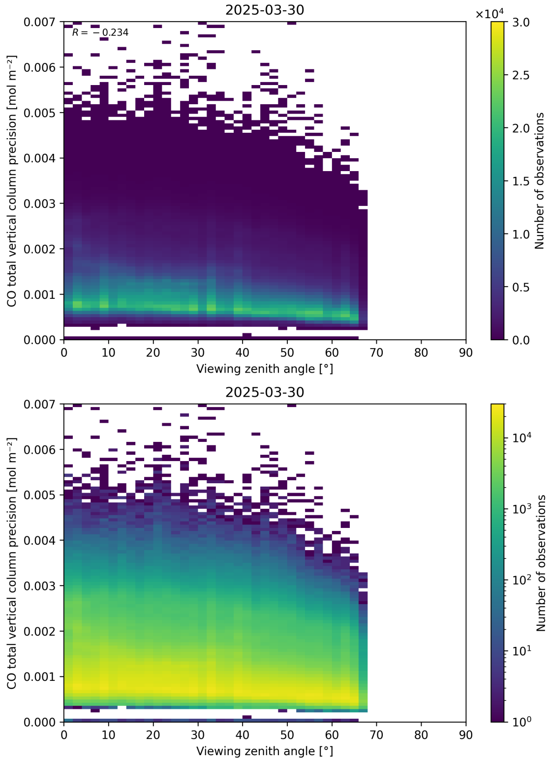
Figure 71: Scatter density plot of “Viewing zenith angle” against “CO total vertical column precision” for 2025-03-29 to 2025-03-31.
