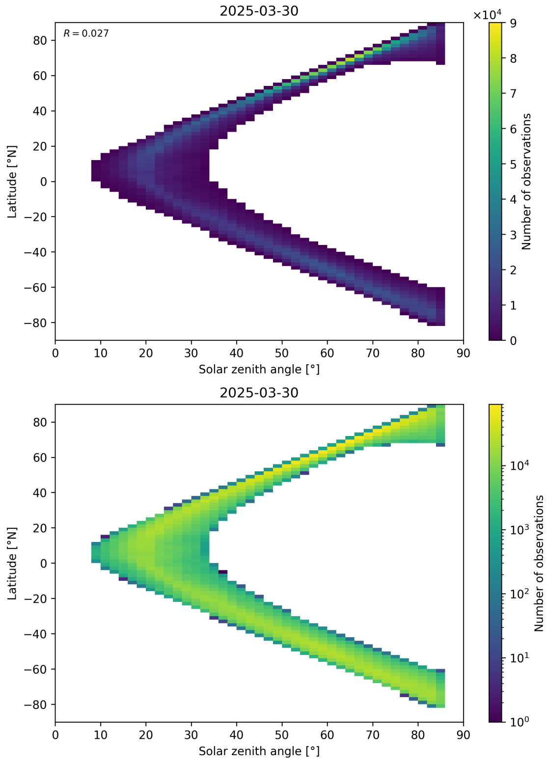
Figure 66: Scatter density plot of “Solar zenith angle” against “Latitude” for 2025-03-29 to 2025-03-31.
