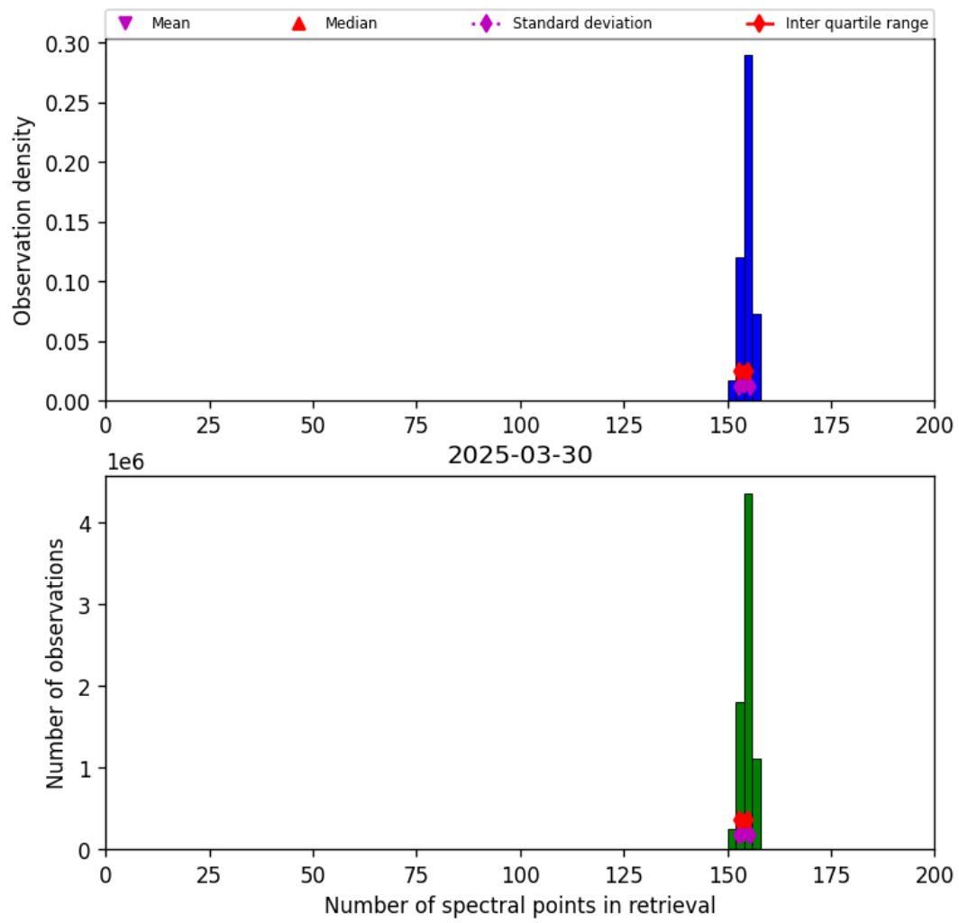
Figure 21: Histogram of “Number of spectral points in retrieval” for 2025-03-29 to 2025-03-31
