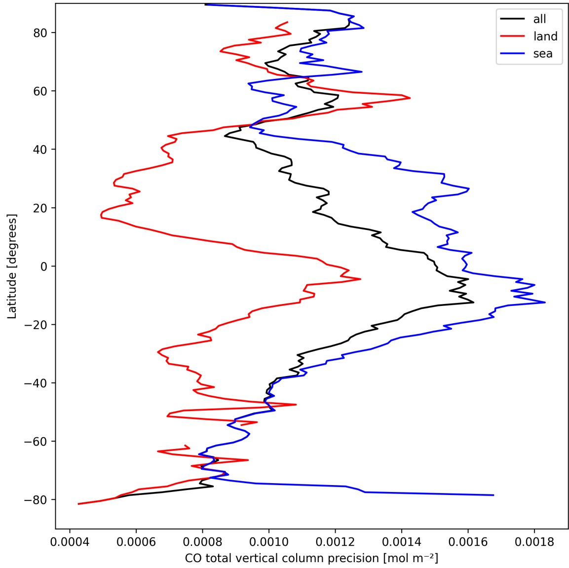
Figure 12: Zonal average of “CO total vertical column precision” for 2025-03-29 to 2025-03-31.
