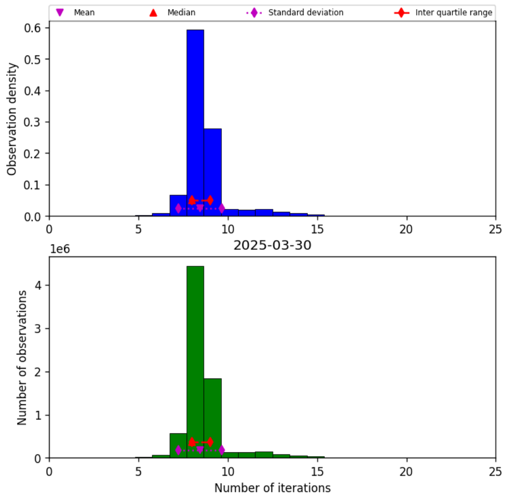
Figure 24: Histogram of “Number of iterations” for 2025-03-29 to 2025-03-31
