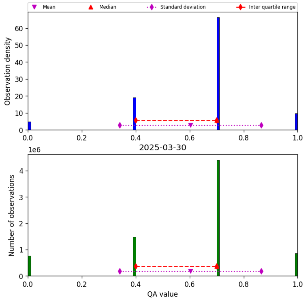
Figure 17: Histogram of “QA value” for 2025-03-29 to 2025-03-31
