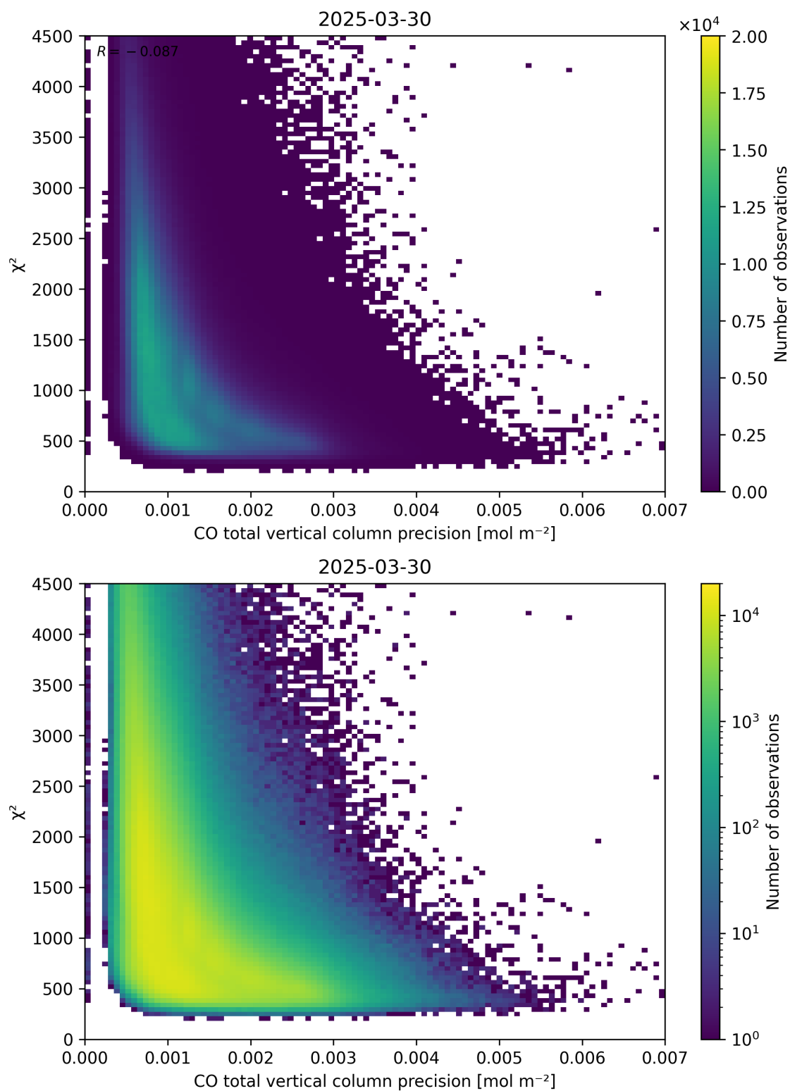
Figure 44: Scatter density plot of “CO total vertical column precision” against “ \chi^2 ” for 2025-03-29 to 2025-03-31.
