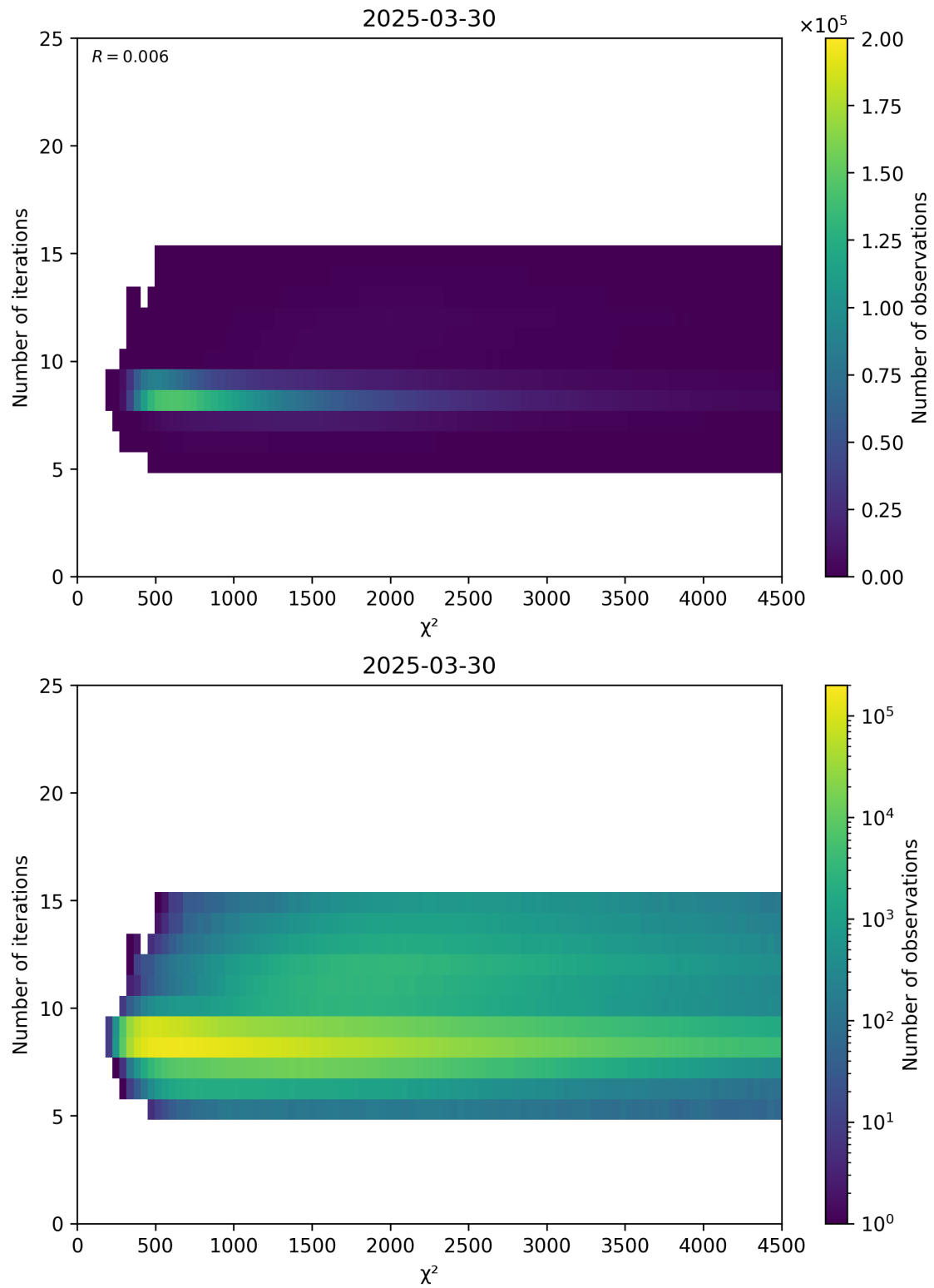
Figure 49: Scatter density plot of “ \chi^2 ” against “Number of iterations” for 2025-03-29 to 2025-03-31.
