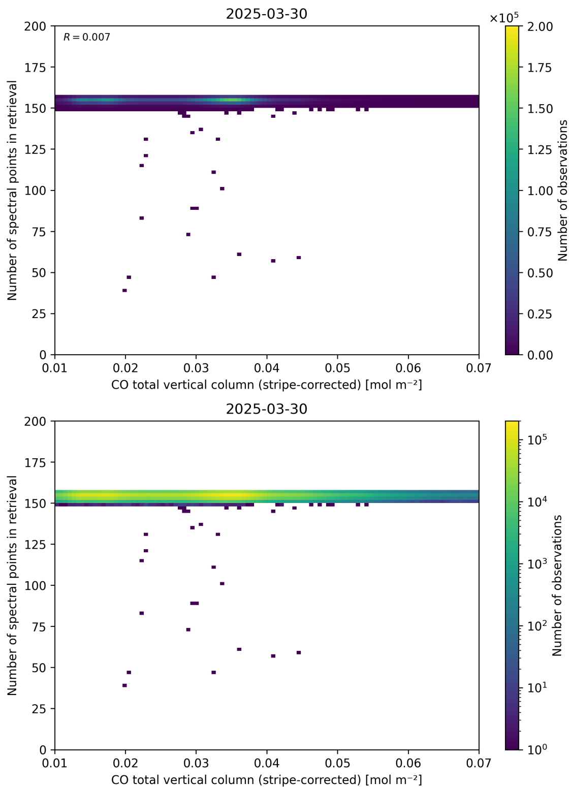
Figure 40: Scatter density plot of “CO total vertical column (stripe-corrected)” against “Number of spectral points in retrieval” for 2025-03-29 to 2025-03-31.
