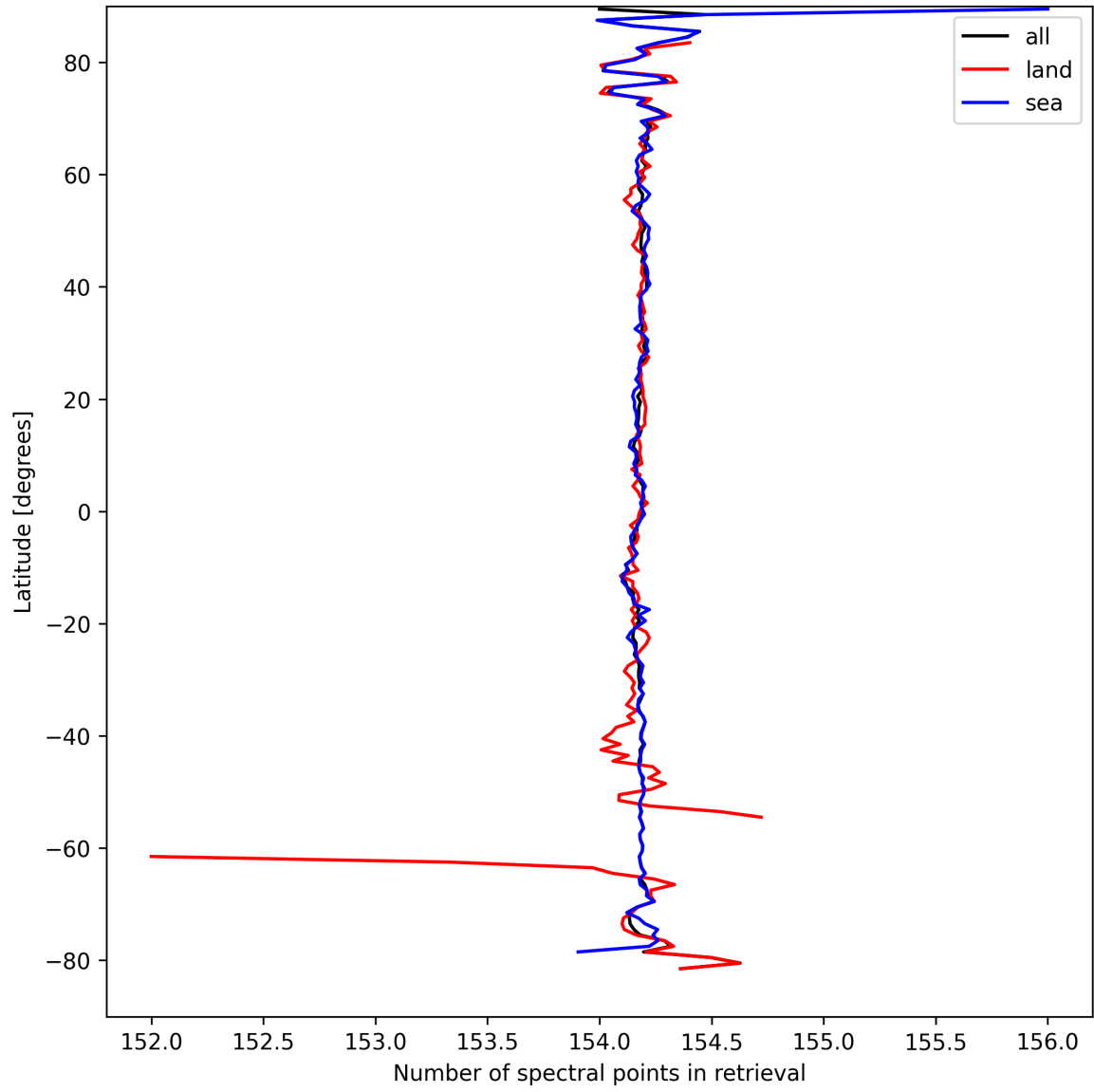
Figure 13: Zonal average of “Number of spectral points in retrieval” for 2025-03-29 to 2025-03-31.
