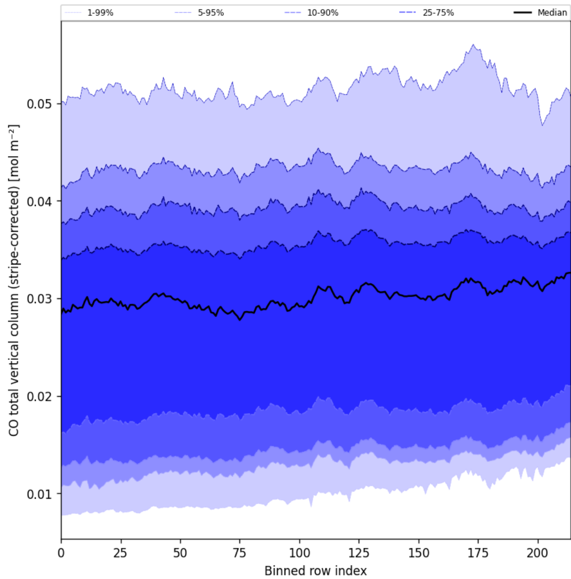
Figure 27: Along track statistics of “CO total vertical column (stripe-corrected)” for 2025-03-29 to 2025-03-31
