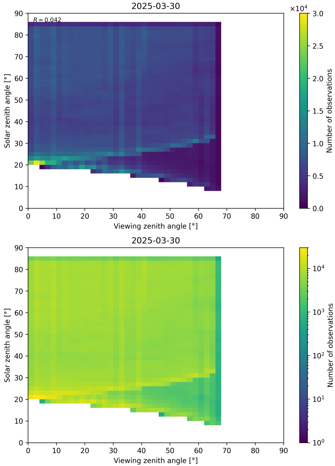
Figure 77: Scatter density plot of “Viewing zenith angle” against “Solar zenith angle” for 2025-03-29 to 2025-03-31.
