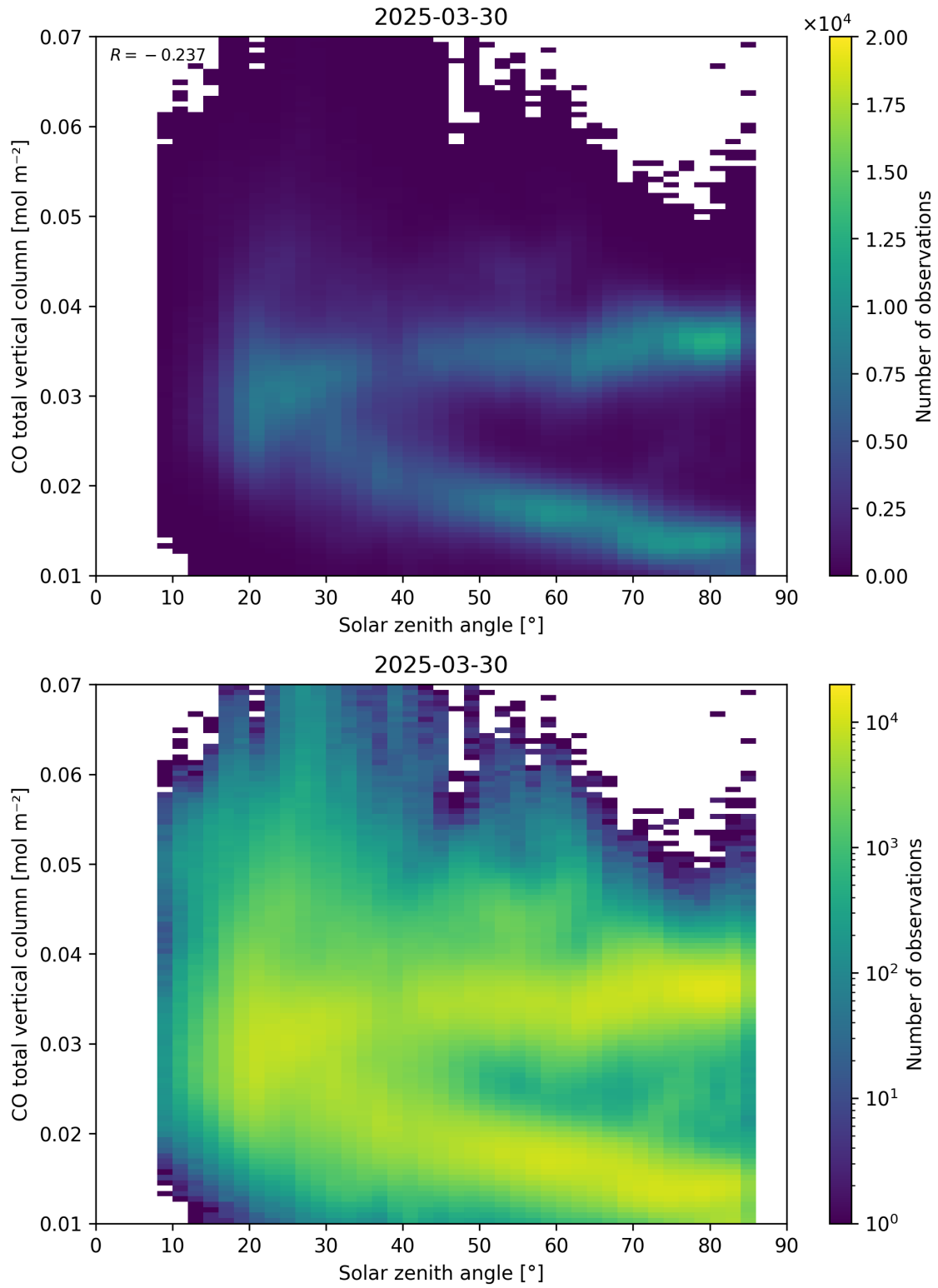
Figure 61: Scatter density plot of “Solar zenith angle” against “CO total vertical column” for 2025-03-29 to 2025-03-31.
