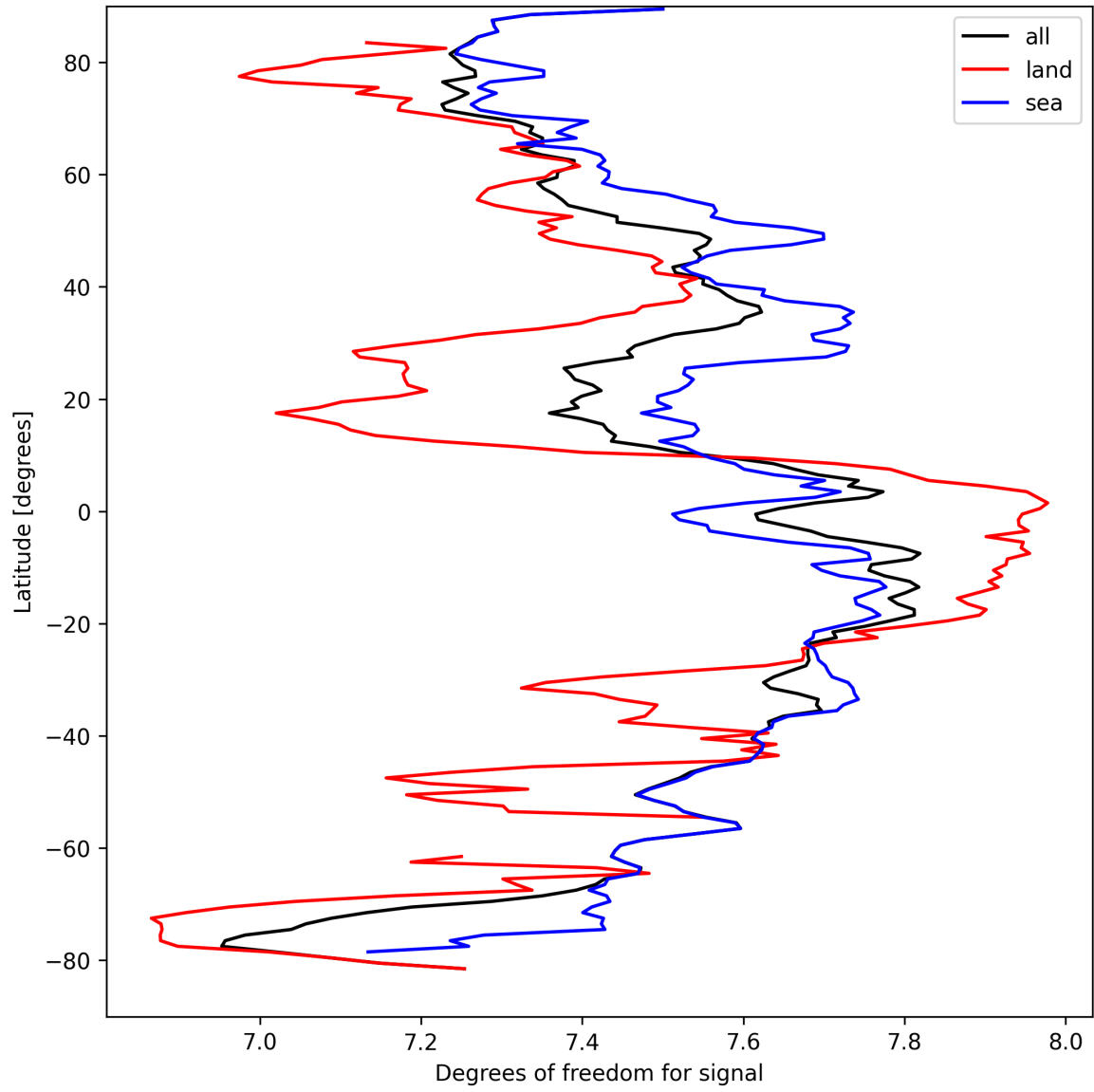
Figure 15: Zonal average of “Degrees of freedom for signal” for 2025-03-29 to 2025-03-31.
