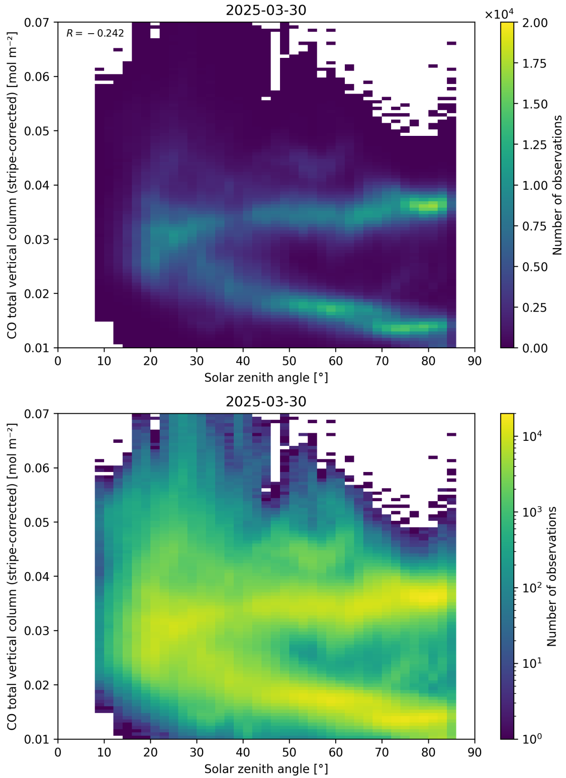
Figure 62: Scatter density plot of “Solar zenith angle” against “CO total vertical column (stripe-corrected)” for 2025-03-29 to 2025-03-31.
