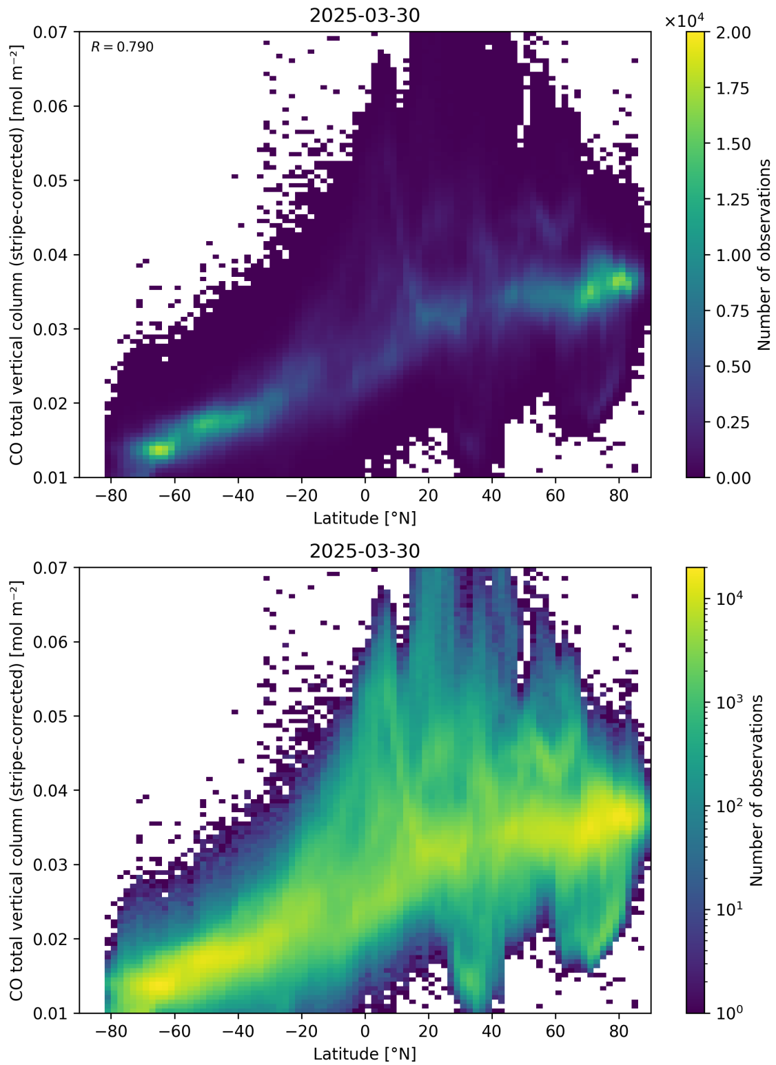
Figure 52: Scatter density plot of “Latitude” against “CO total vertical column (stripe-corrected)” for 2025-03-29 to 2025-03-31.
