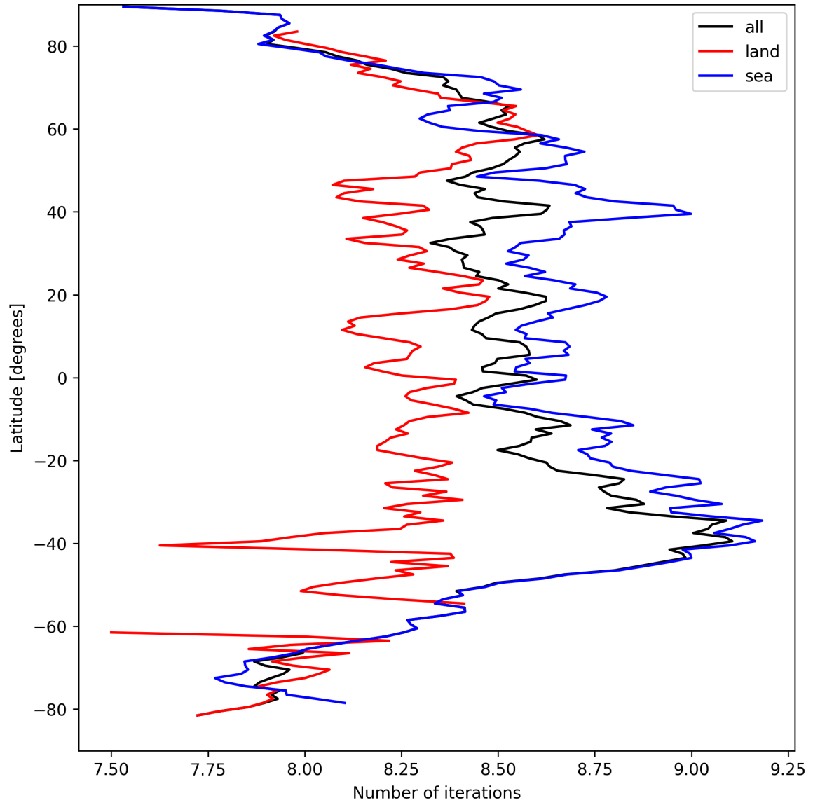
Figure 16: Zonal average of “Number of iterations” for 2025-03-29 to 2025-03-31.
