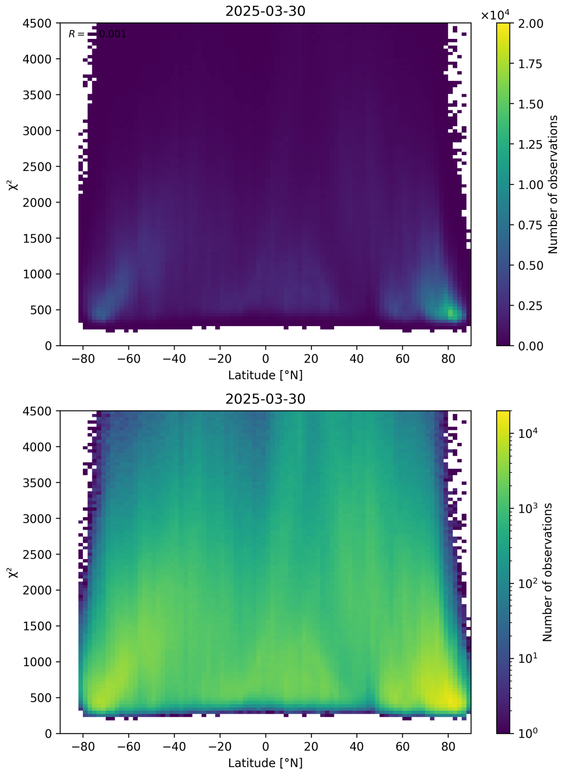
Figure 54: Scatter density plot of “Latitude” against “ \chi^2 ” for 2025-03-29 to 2025-03-31.
