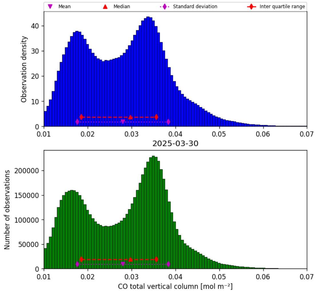
Figure 18: Histogram of “CO total vertical column” for 2025-03-29 to 2025-03-31
