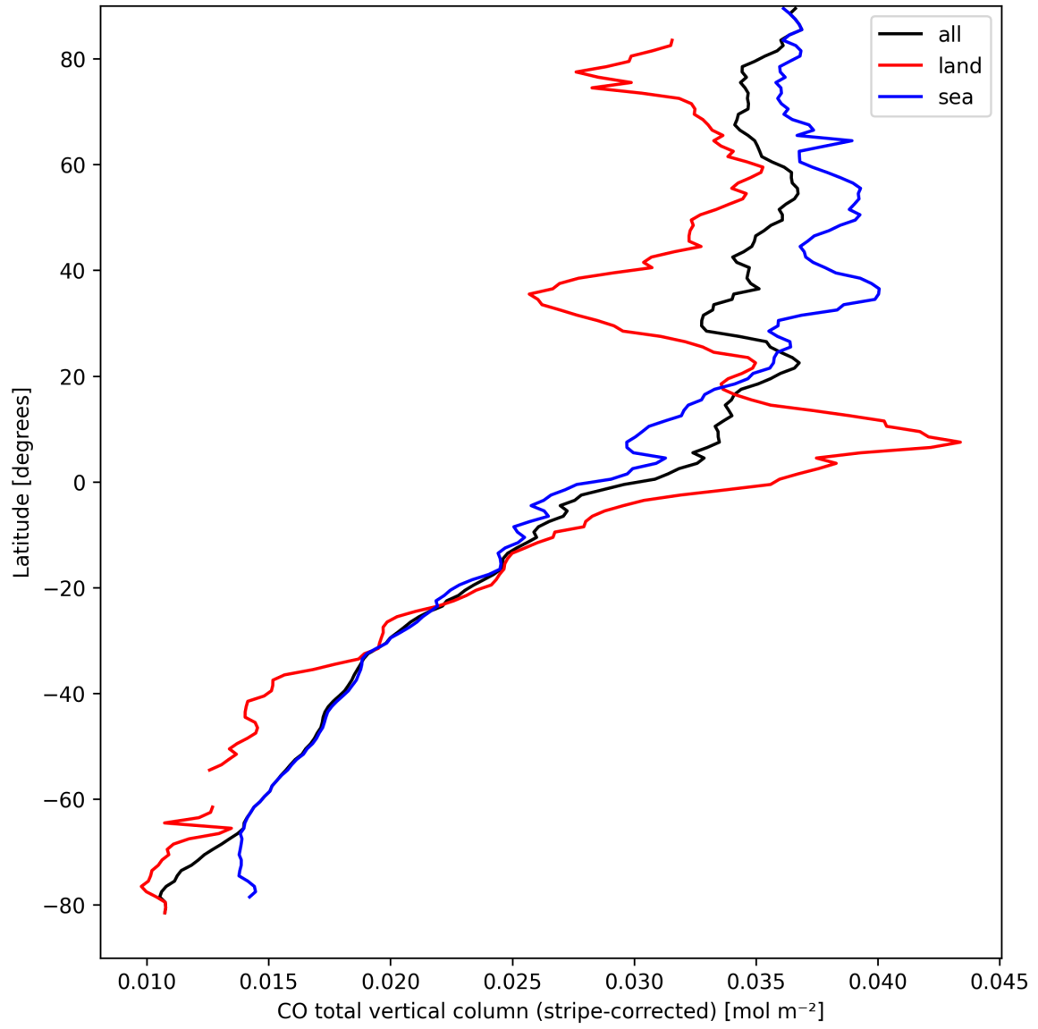
Figure 11: Zonal average of “CO total vertical column (stripe-corrected)” for 2025-03-29 to 2025-03-31.
