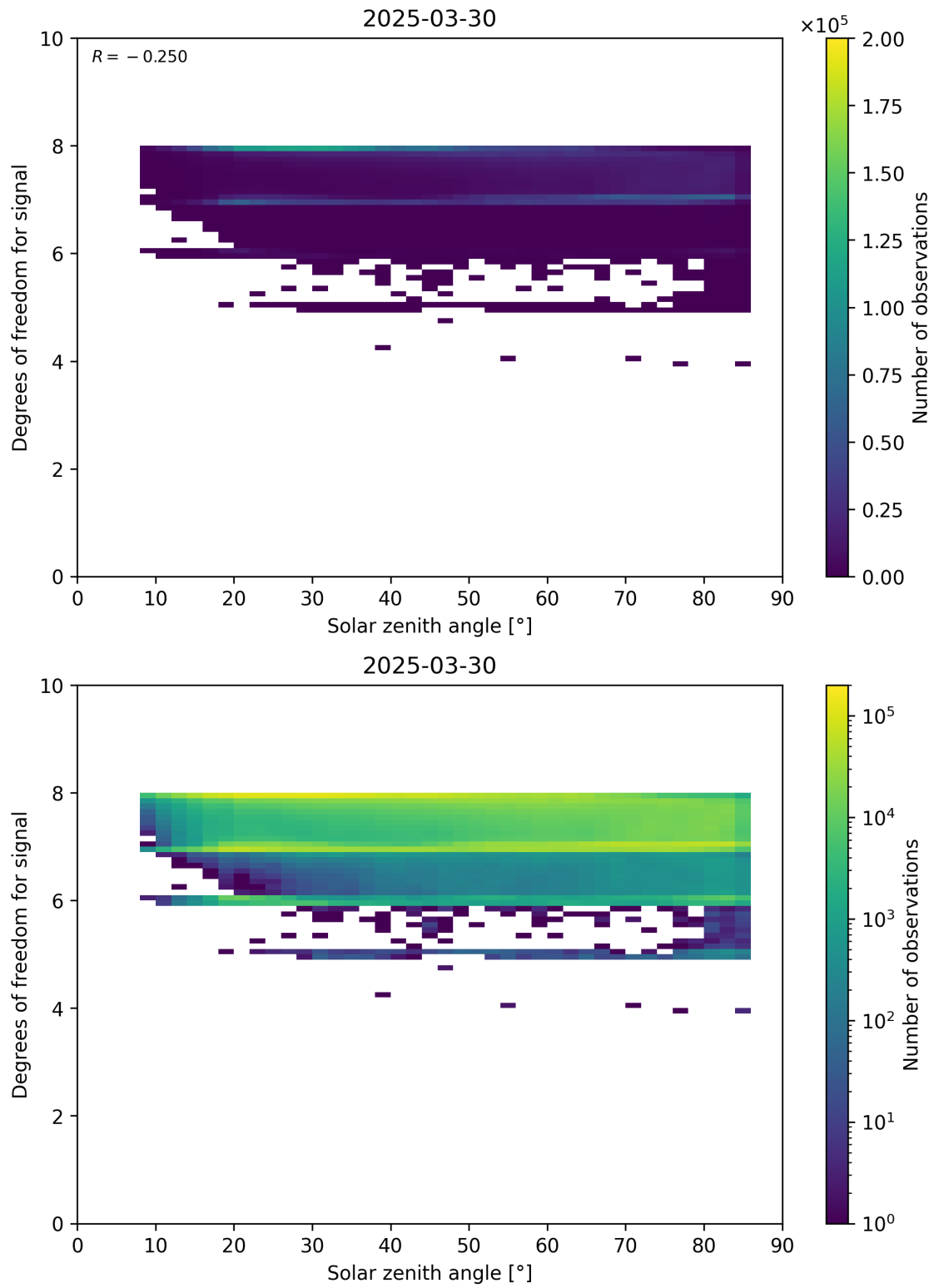
Figure 65: Scatter density plot of “Solar zenith angle” against “Degrees of freedom for signal” for 2025-03-29 to 2025-03-31.
