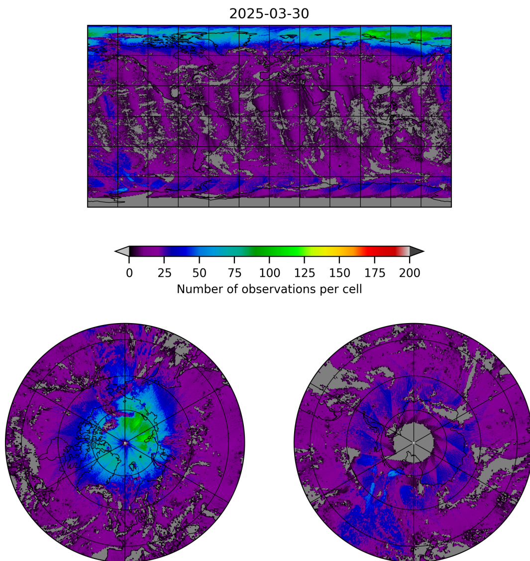
Figure 8: Map of the number of observations for 2025-03-29 to 2025-03-31
