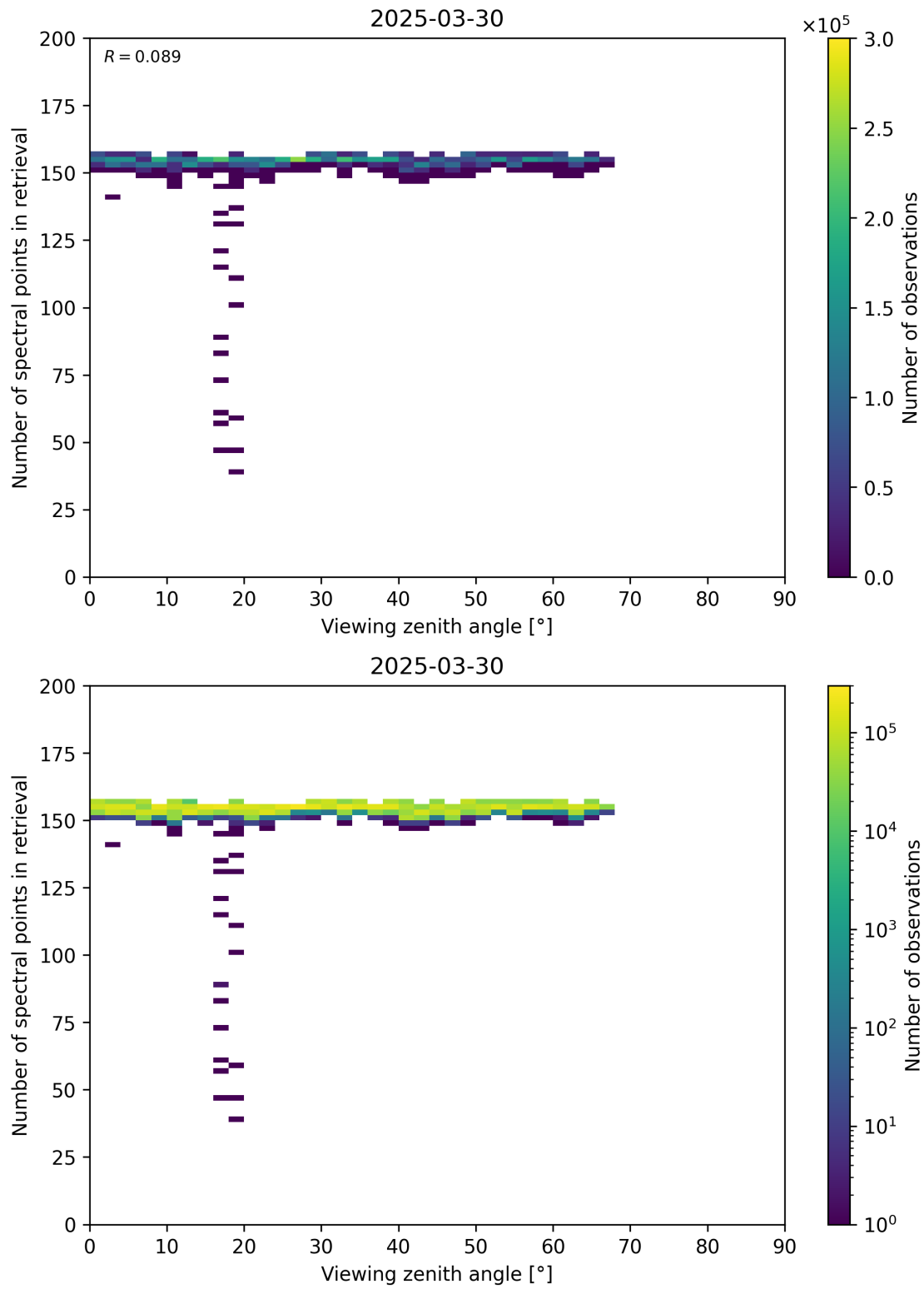
Figure 76: Scatter density plot of “Viewing zenith angle” against “Number of spectral points in retrieval” for 2025-03-29 to 2025-03-31.
