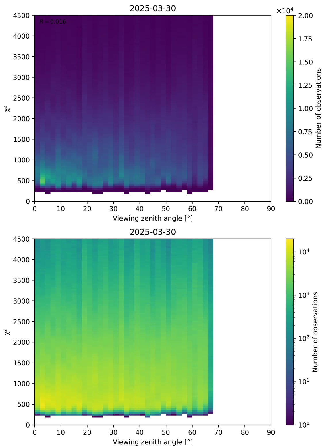
Figure 72: Scatter density plot of “Viewing zenith angle” against “ \chi^2 ” for 2025-03-29 to 2025-03-31.
