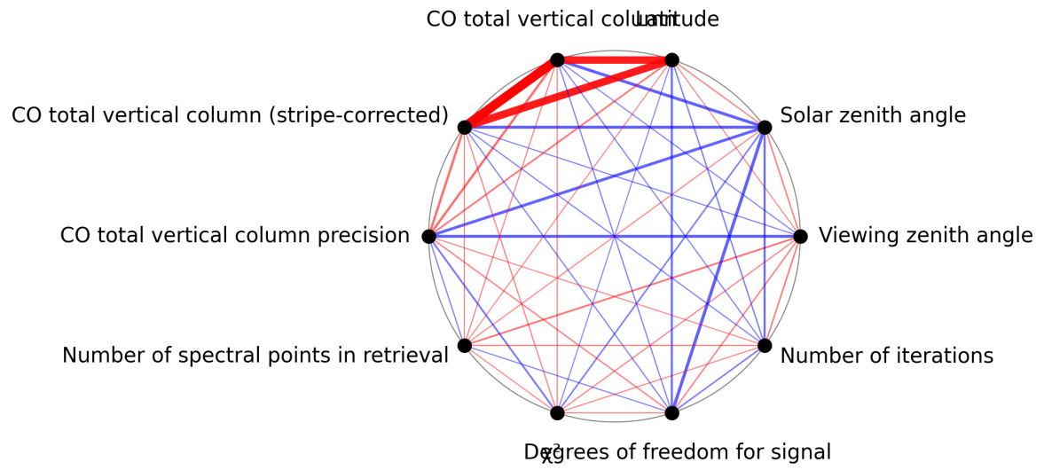
Figure 1: Map of correlation graph for 2025-03-29 to 2025-03-31.
