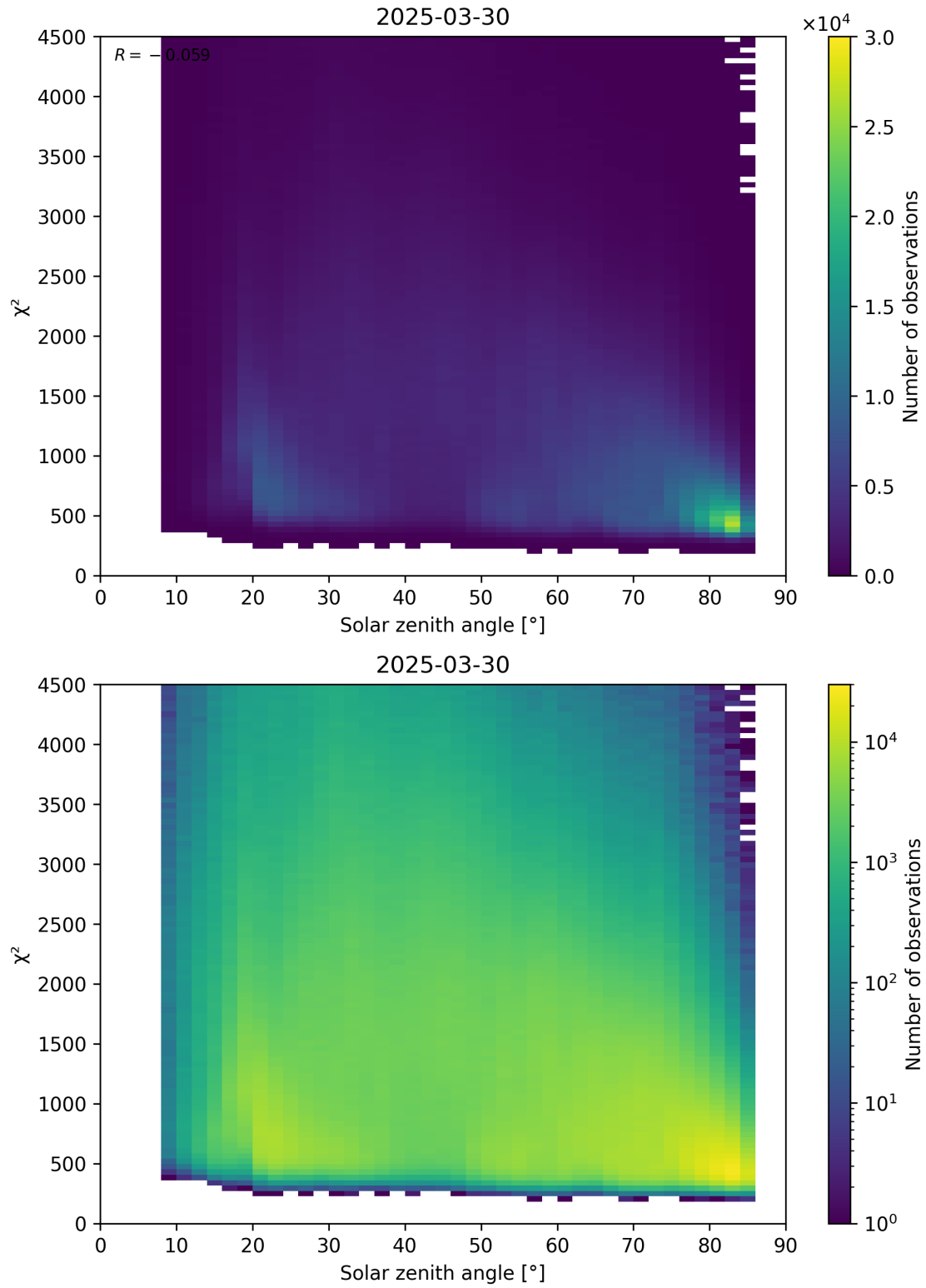
Figure 64: Scatter density plot of “Solar zenith angle” against “ \chi^2 ” for 2025-03-29 to 2025-03-31.
