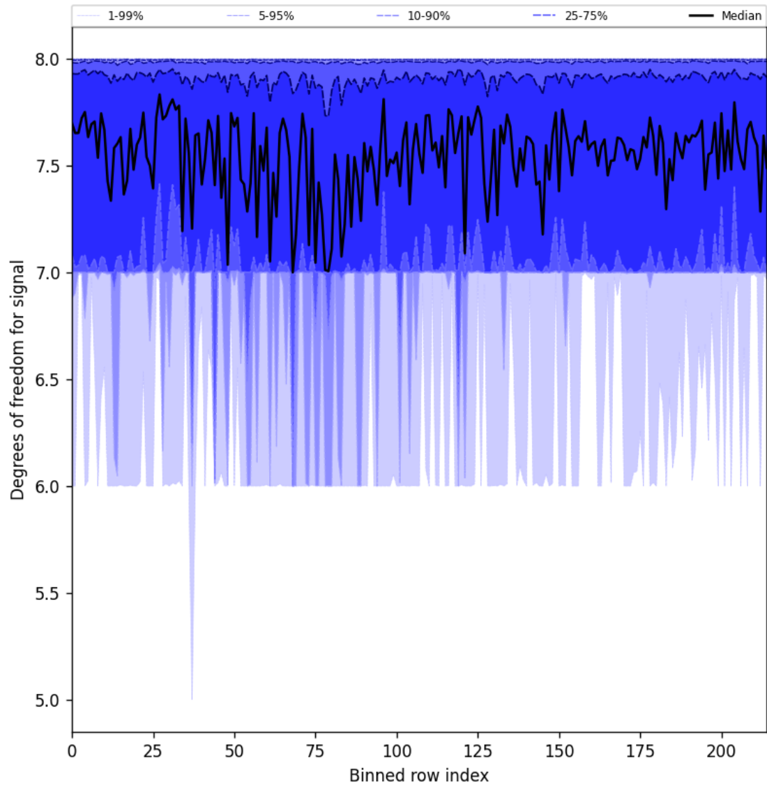
Figure 31: Along track statistics of “Degrees of freedom for signal” for 2025-03-29 to 2025-03-31
