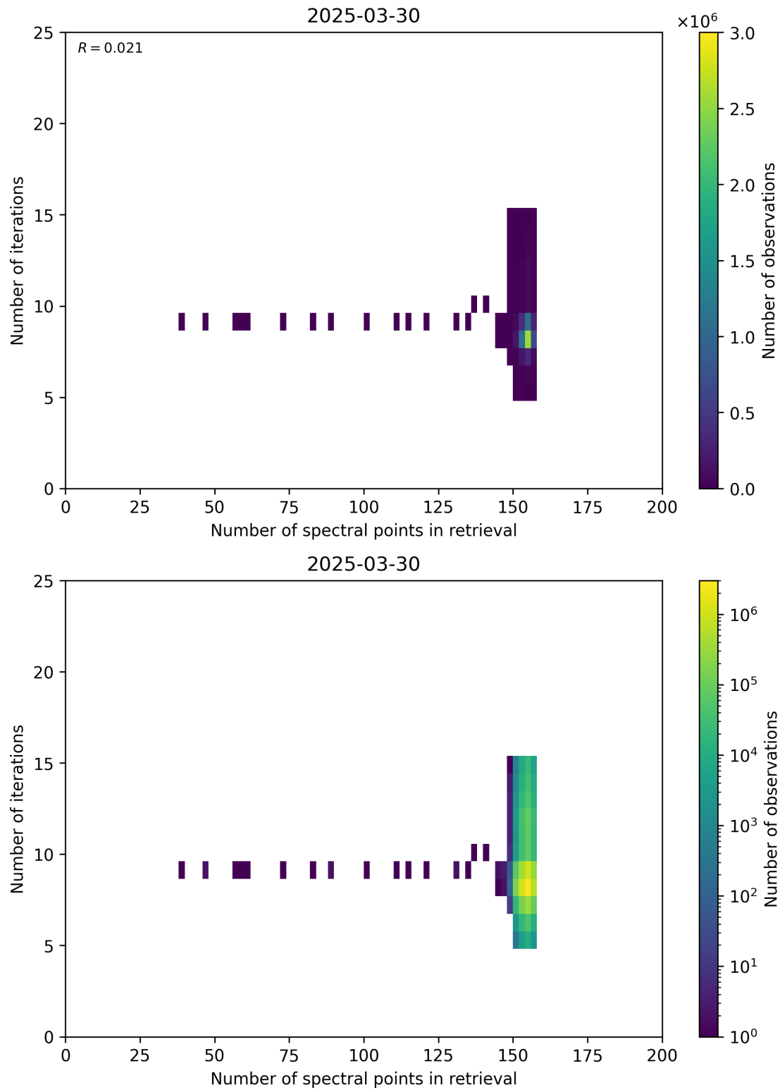
Figure 60: Scatter density plot of “Number of spectral points in retrieval” against “Number of iterations” for 2025-03-29 to 2025-03-31.
