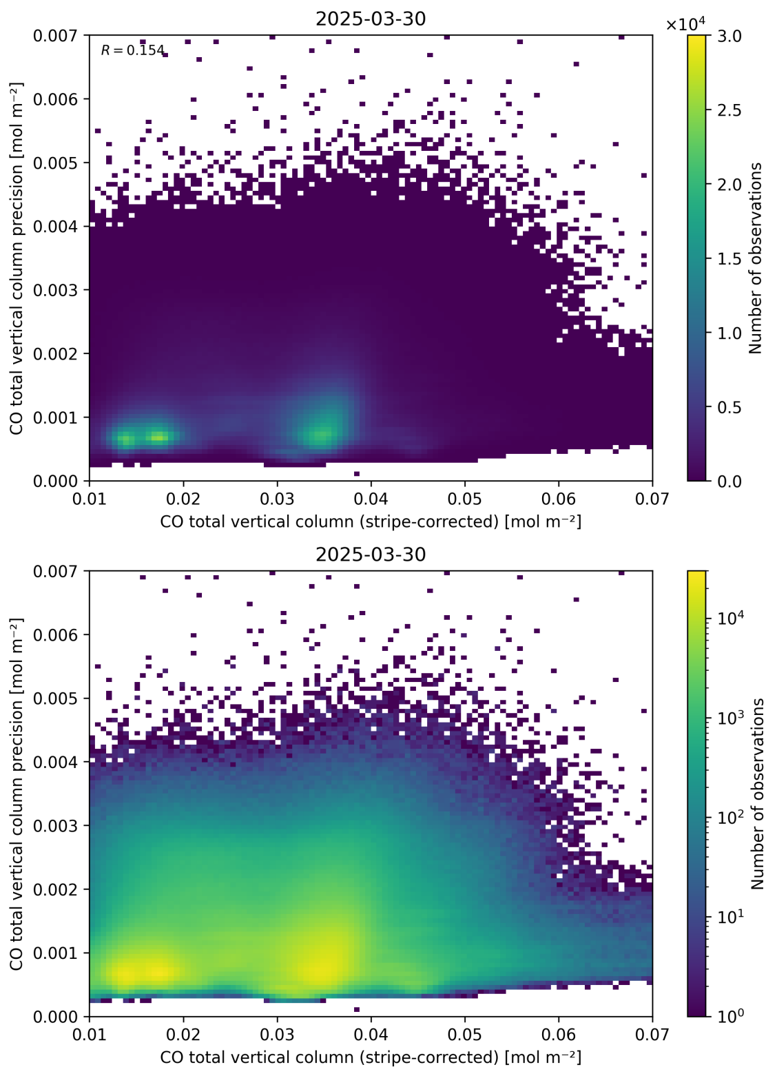
Figure 36: Scatter density plot of “CO total vertical column (stripe-corrected)” against “CO total vertical column precision” for 2025-03-29 to 2025-03-31.
