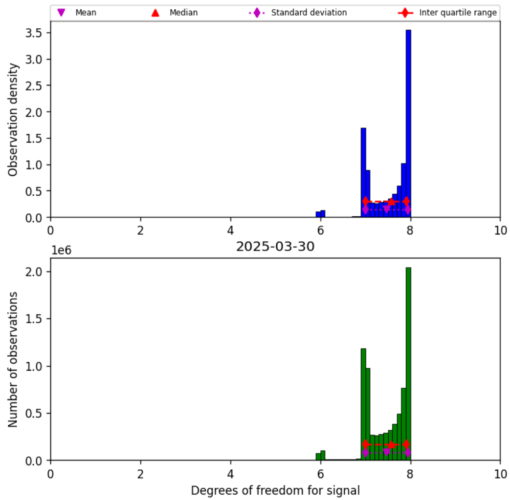
Figure 23: Histogram of “Degrees of freedom for signal” for 2025-03-29 to 2025-03-31
