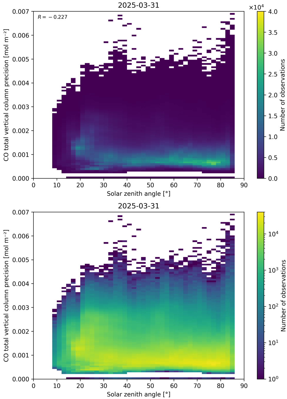
Figure 63: Scatter density plot of “Solar zenith angle” against “CO total vertical column precision” for 2025-03-30 to 2025-04-01.
