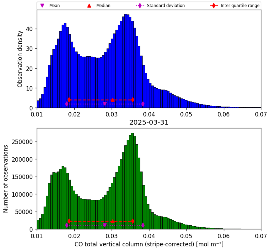
Figure 19: Histogram of “CO total vertical column (stripe-corrected)” for 2025-03-30 to 2025-04-01
