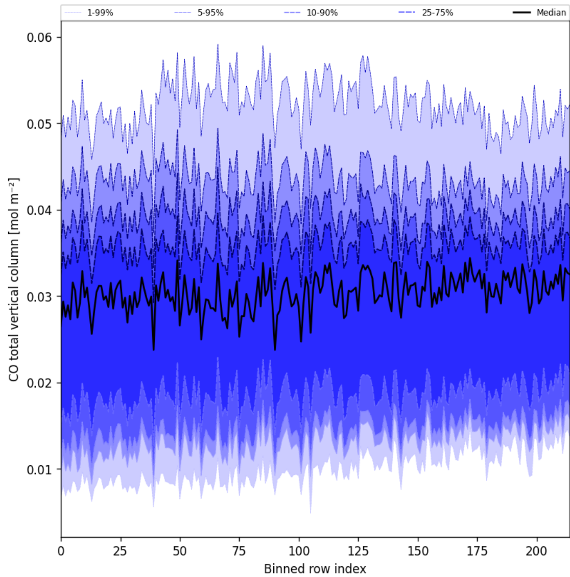
Figure 26: Along track statistics of “CO total vertical column” for 2025-03-30 to 2025-04-01
