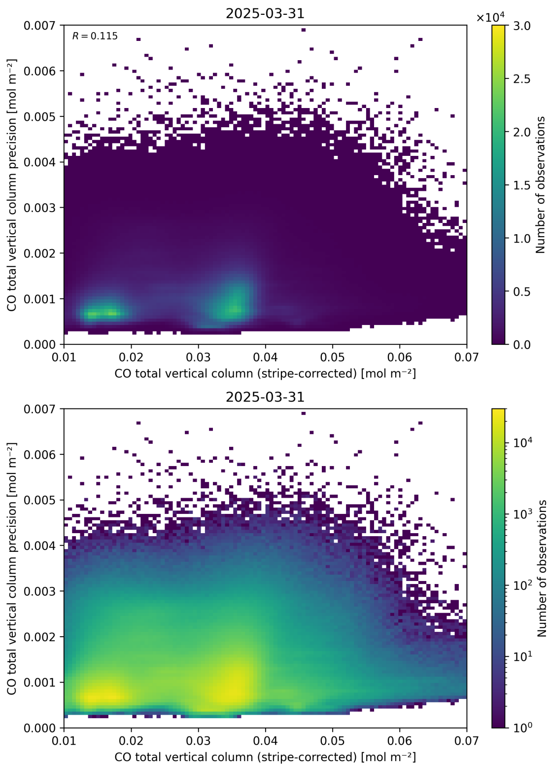
Figure 36: Scatter density plot of “CO total vertical column (stripe-corrected)” against “CO total vertical column precision” for 2025-03-30 to 2025-04-01.
