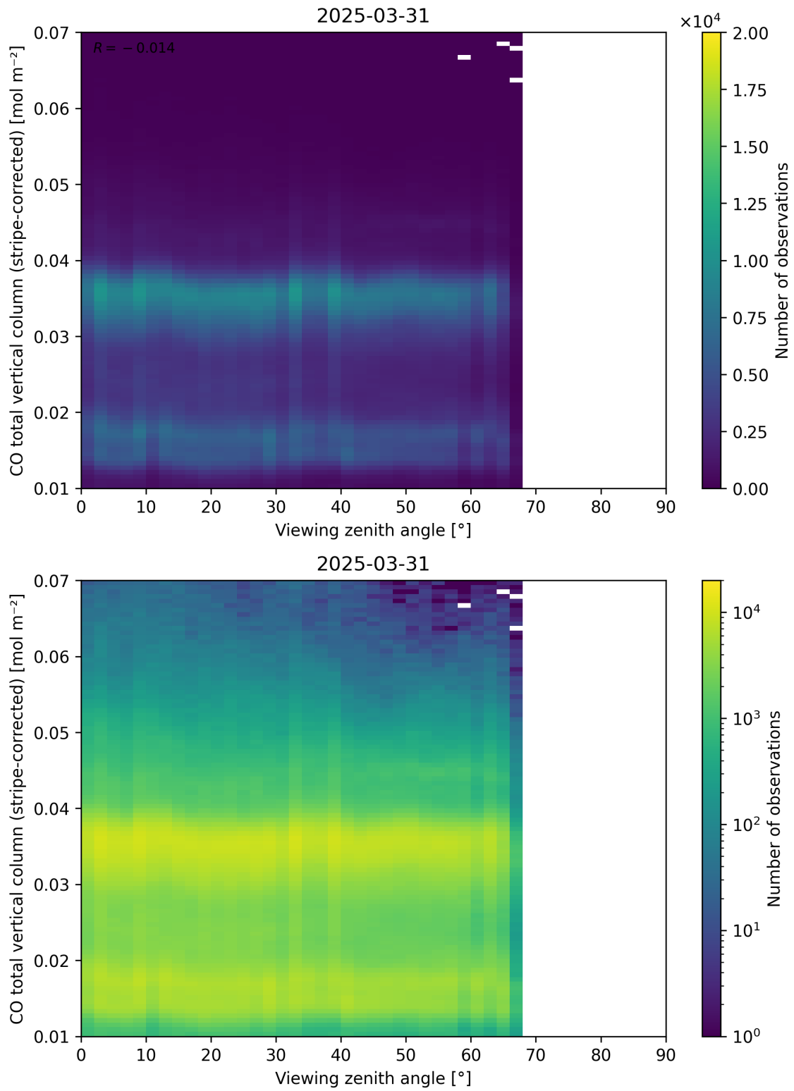
Figure 70: Scatter density plot of “Viewing zenith angle” against “CO total vertical column (stripe-corrected)” for 2025-03-30 to 2025-04-01.
