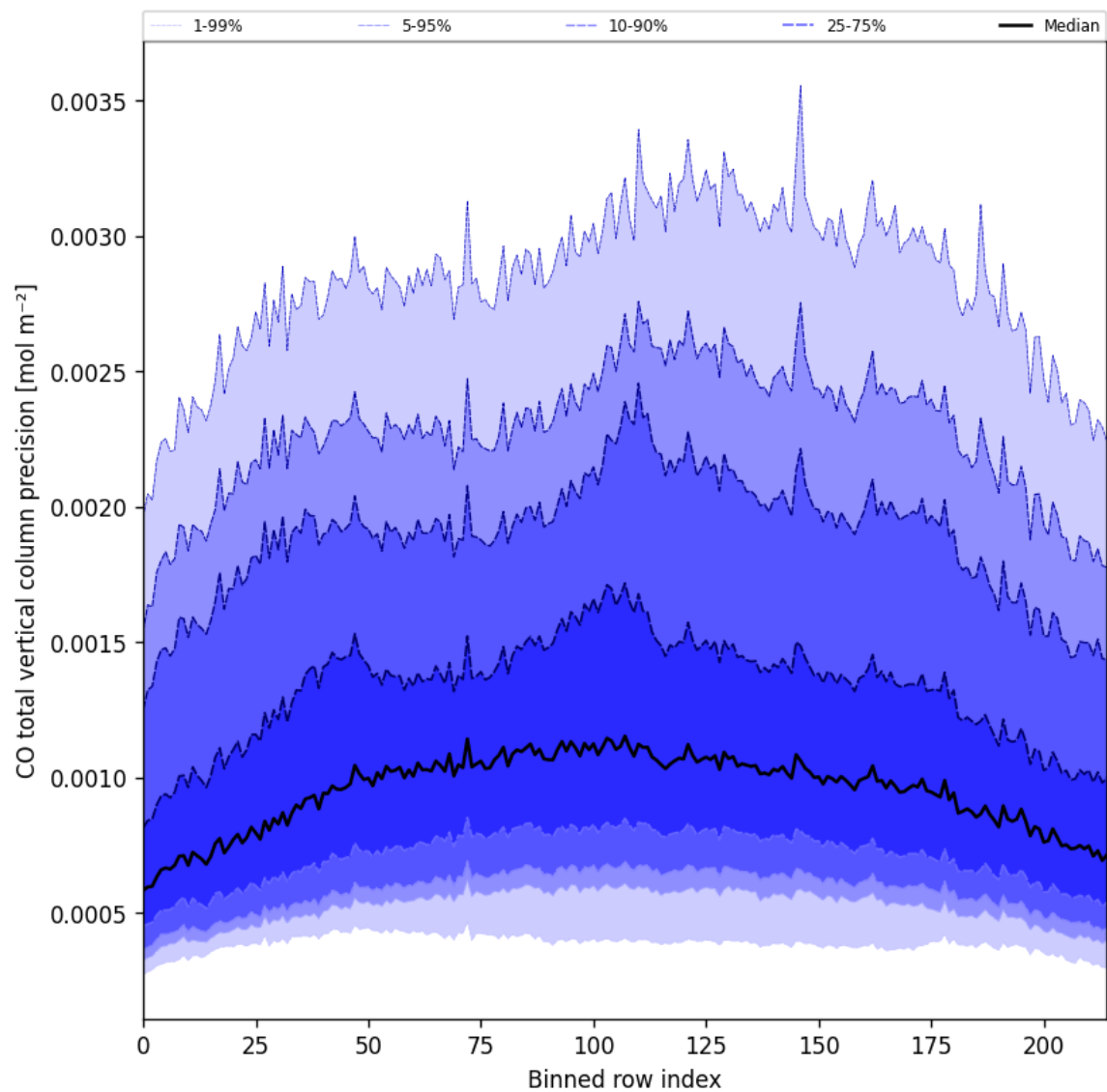
Figure 28: Along track statistics of “CO total vertical column precision” for 2025-03-30 to 2025-04-01
