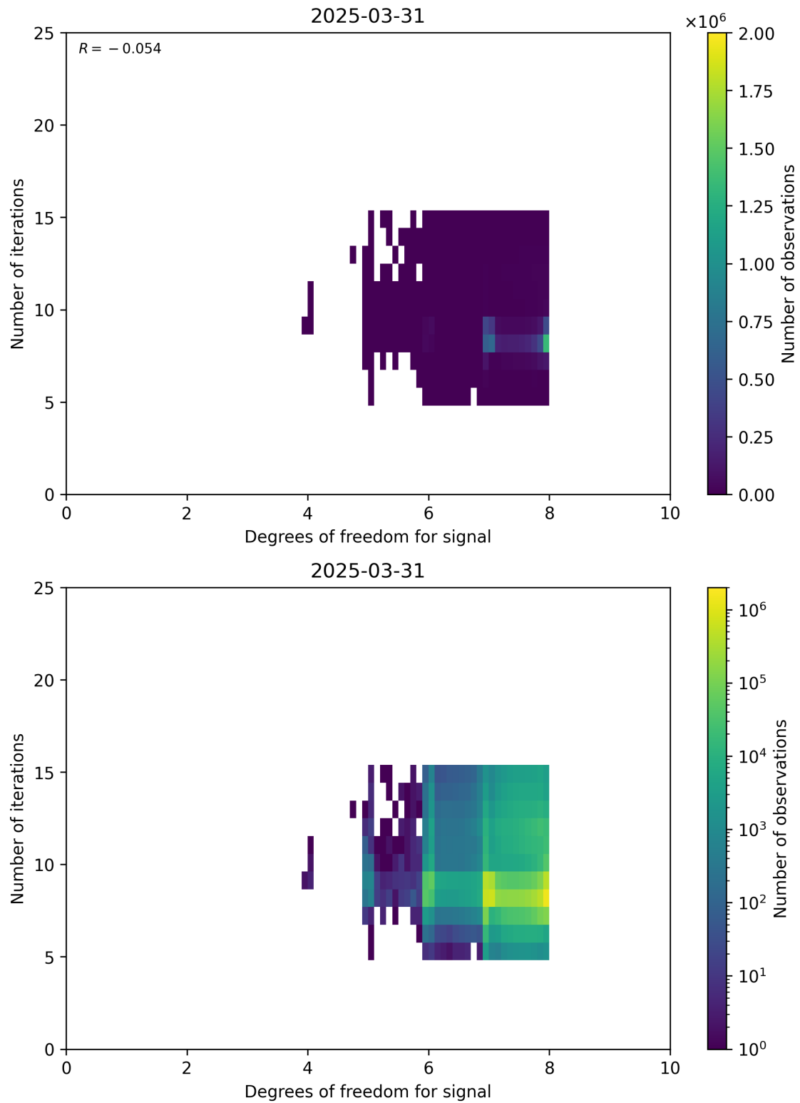
Figure 50: Scatter density plot of “Degrees of freedom for signal” against “Number of iterations” for 2025-03-30 to 2025-04-01.
