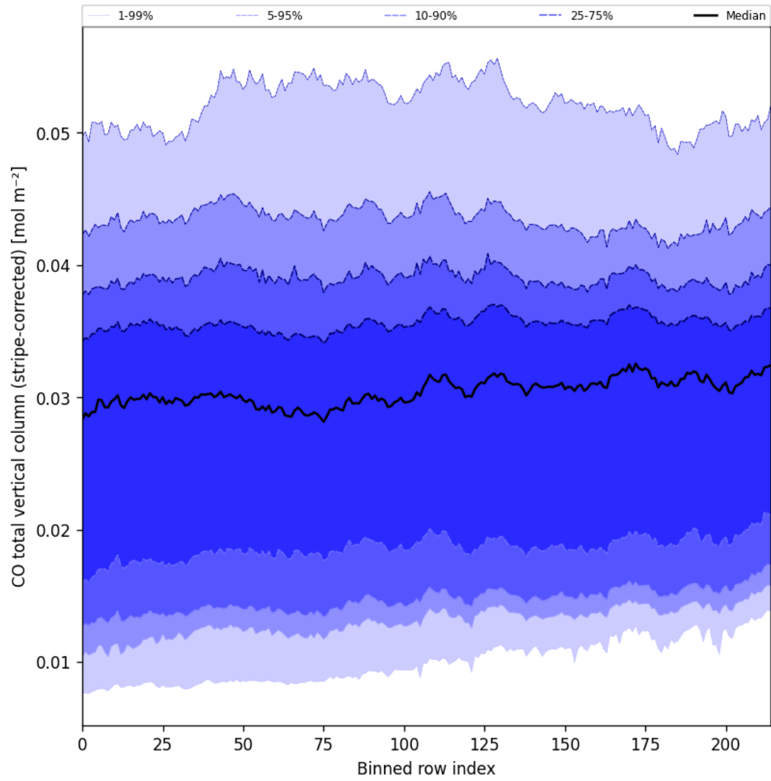
Figure 27: Along track statistics of “CO total vertical column (stripe-corrected)” for 2025-03-30 to 2025-04-01
