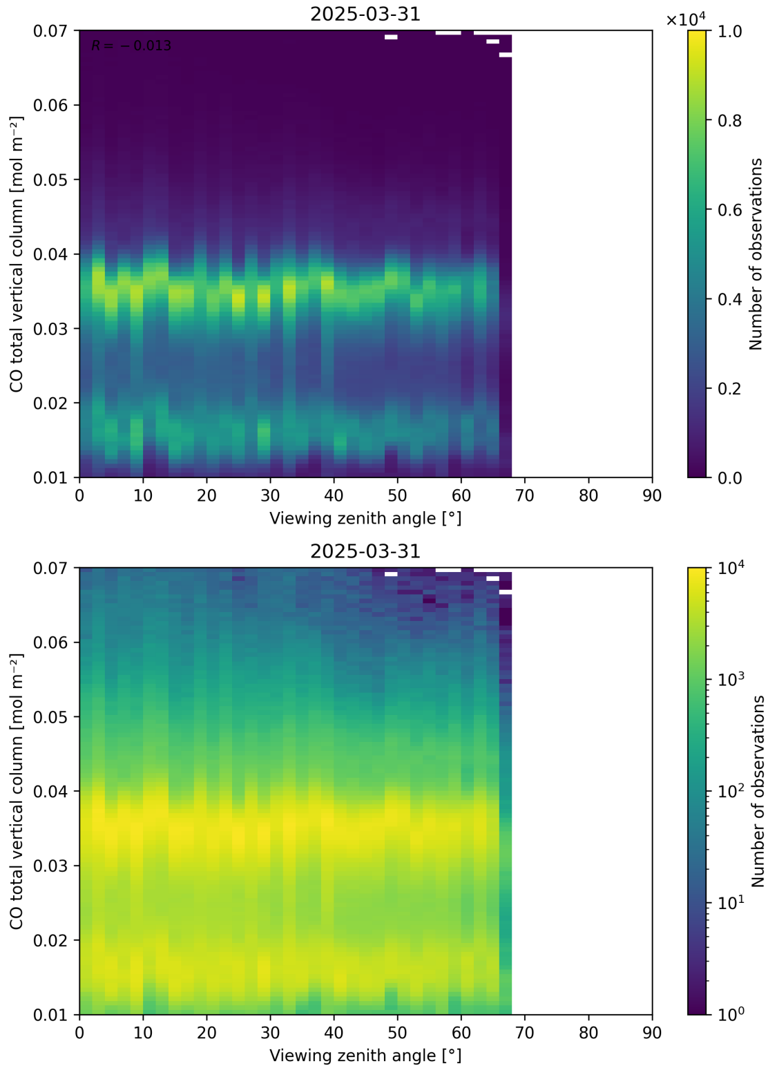
Figure 69: Scatter density plot of “Viewing zenith angle” against “CO total vertical column” for 2025-03-30 to 2025-04-01.
