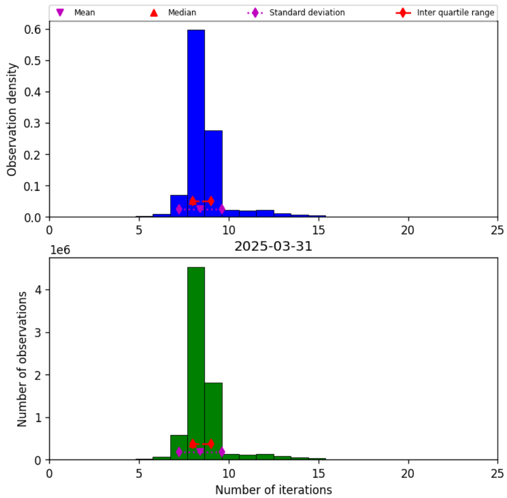
Figure 24: Histogram of “Number of iterations” for 2025-03-30 to 2025-04-01
