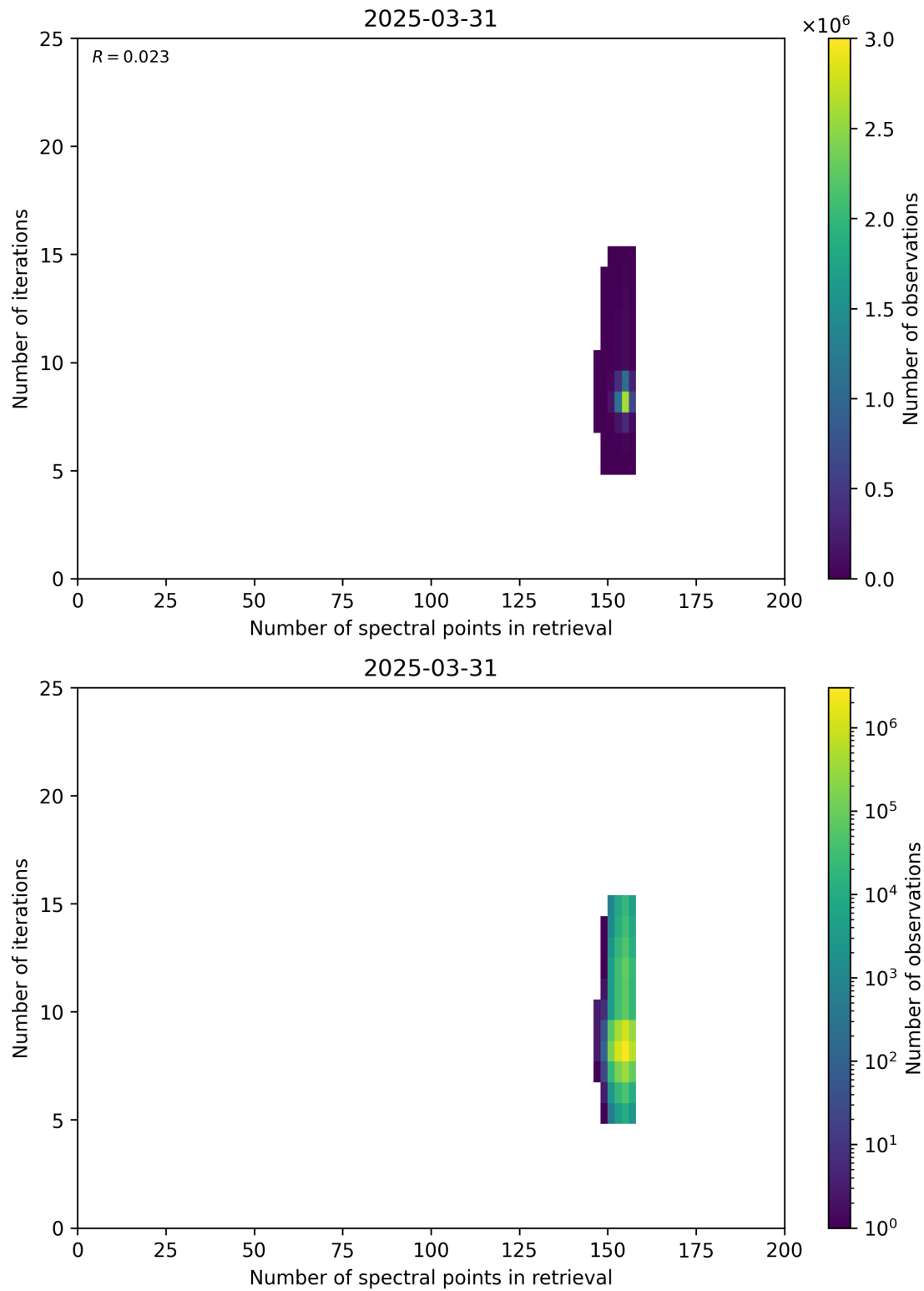
Figure 60: Scatter density plot of “Number of spectral points in retrieval” against “Number of iterations” for 2025-03-30 to 2025-04-01.
