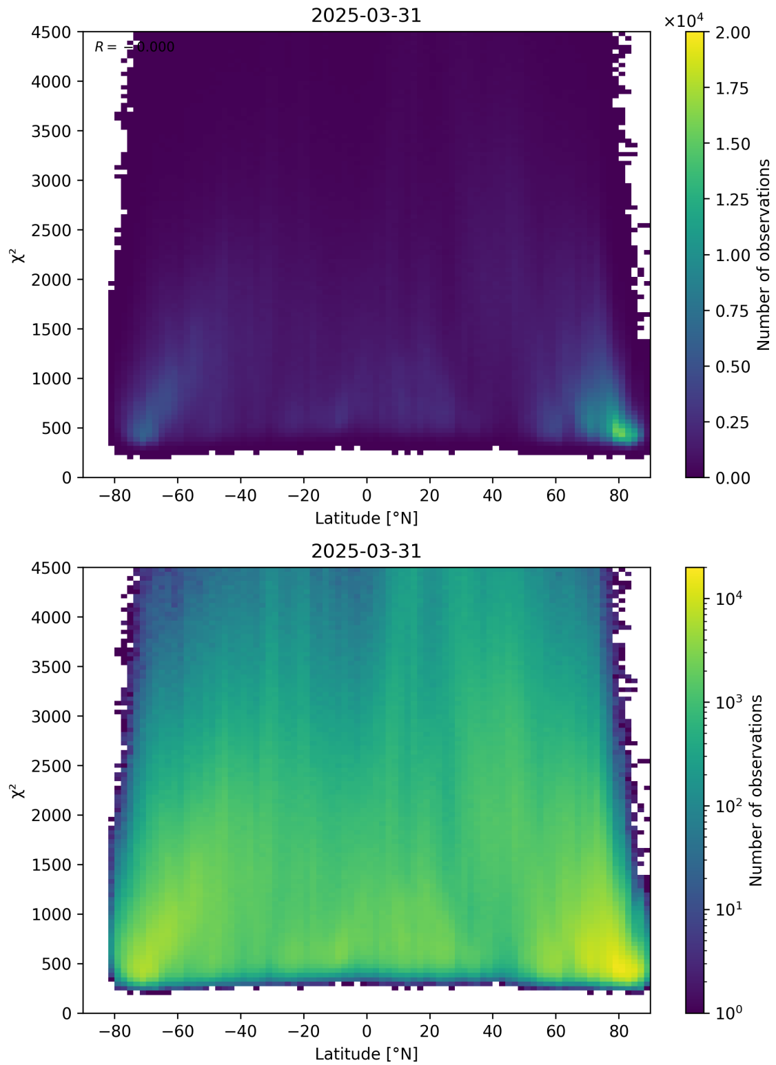
Figure 54: Scatter density plot of “Latitude” against “ \chi^2 ” for 2025-03-30 to 2025-04-01.
