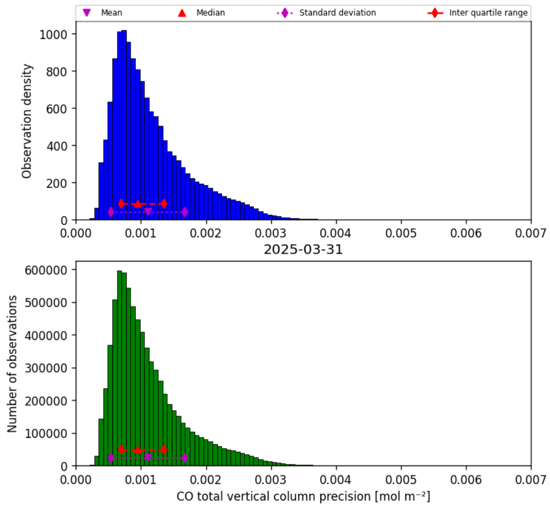
Figure 20: Histogram of “CO total vertical column precision” for 2025-03-30 to 2025-04-01
