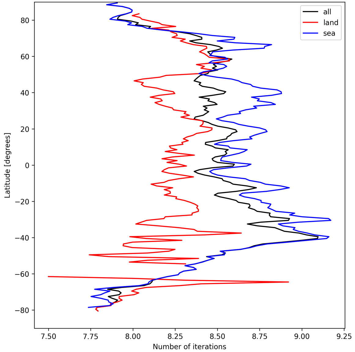
Figure 16: Zonal average of “Number of iterations” for 2025-03-30 to 2025-04-01.
