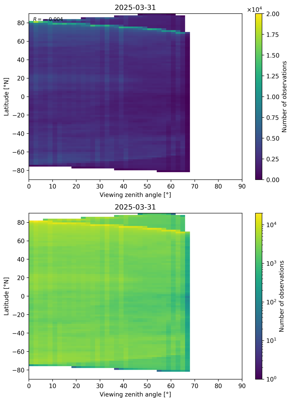
Figure 74: Scatter density plot of “Viewing zenith angle” against “Latitude” for 2025-03-30 to 2025-04-01.
