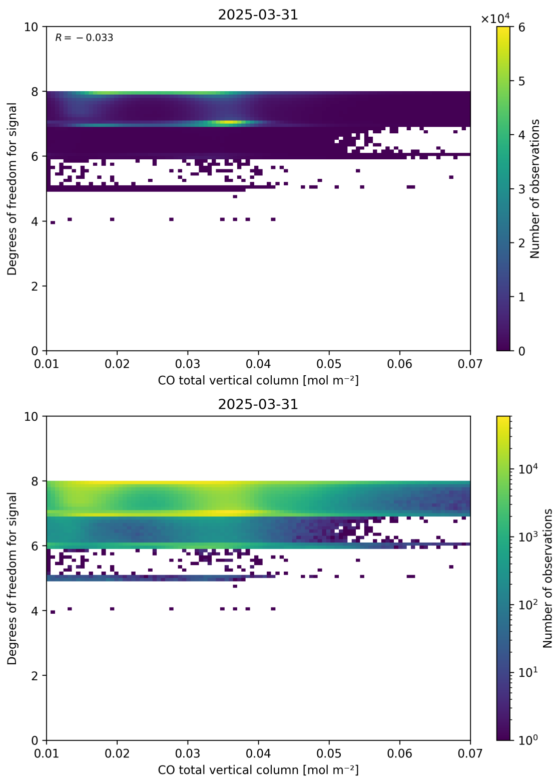
Figure 41: Scatter density plot of “CO total vertical column” against “Degrees of freedom for signal” for 2025-03-30 to 2025-04-01.
