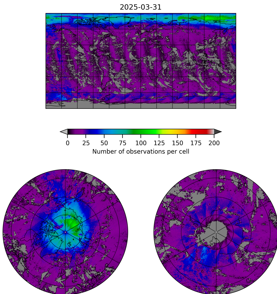
Figure 8: Map of the number of observations for 2025-03-30 to 2025-04-01
