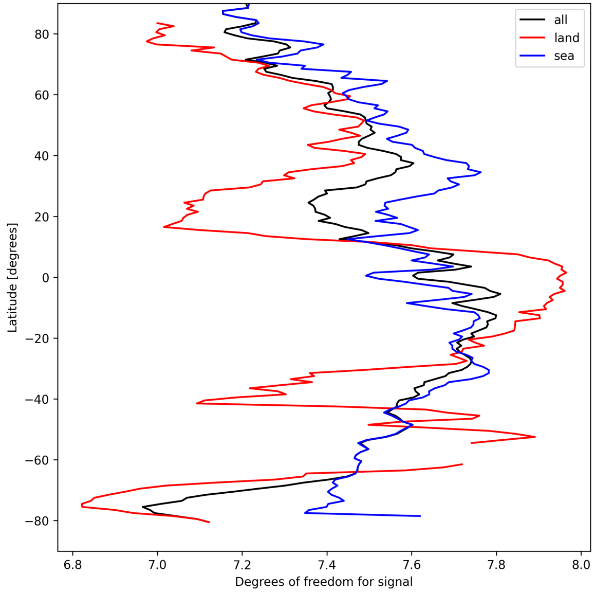
Figure 15: Zonal average of “Degrees of freedom for signal” for 2025-03-30 to 2025-04-01.
