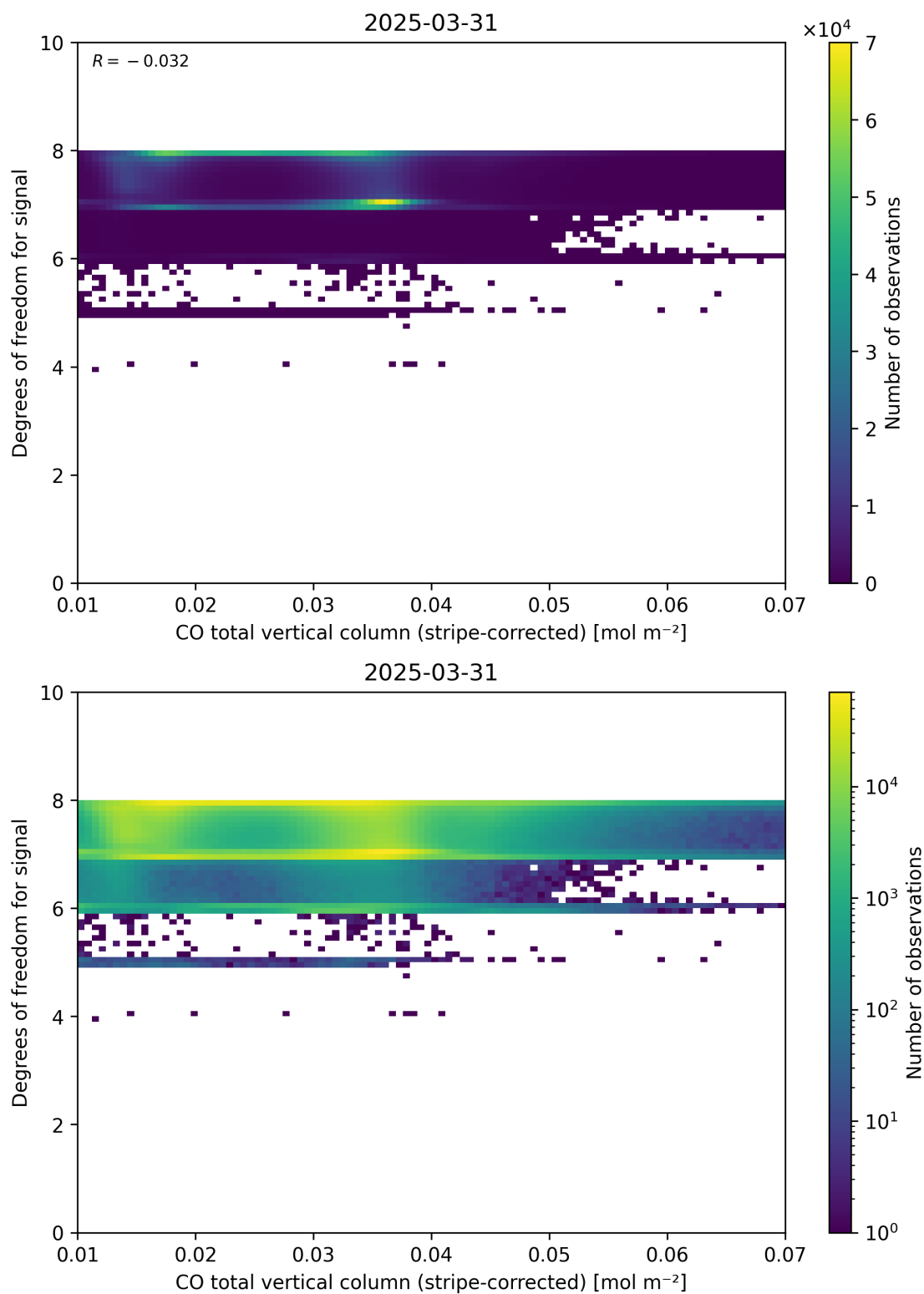
Figure 38: Scatter density plot of “CO total vertical column (stripe-corrected)” against “Degrees of freedom for signal” for 2025-03-30 to 2025-04-01.
