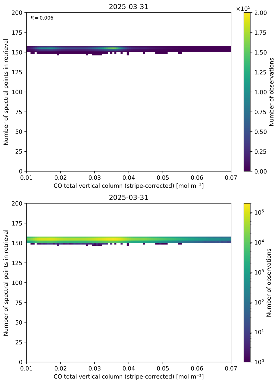
Figure 40: Scatter density plot of “CO total vertical column (stripe-corrected)” against “Number of spectral points in retrieval” for 2025-03-30 to 2025-04-01.
