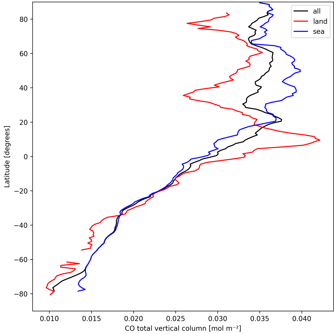
Figure 10: Zonal average of “CO total vertical column” for 2025-03-30 to 2025-04-01.
