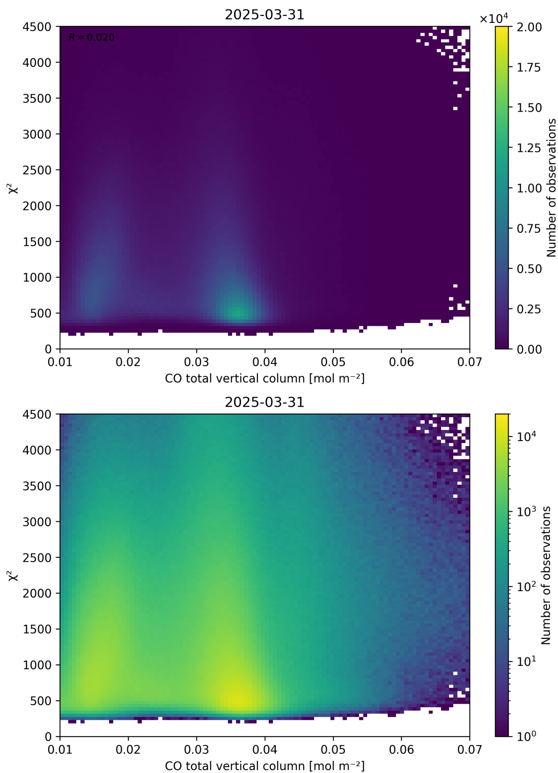
Figure 35: Scatter density plot of “CO total vertical column” against “ \chi^2 ” for 2025-03-30 to 2025-04-01.
