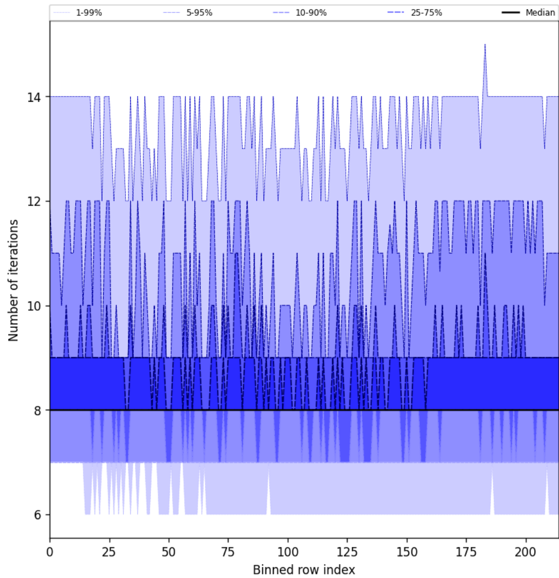
Figure 32: Along track statistics of “Number of iterations” for 2025-03-30 to 2025-04-01
