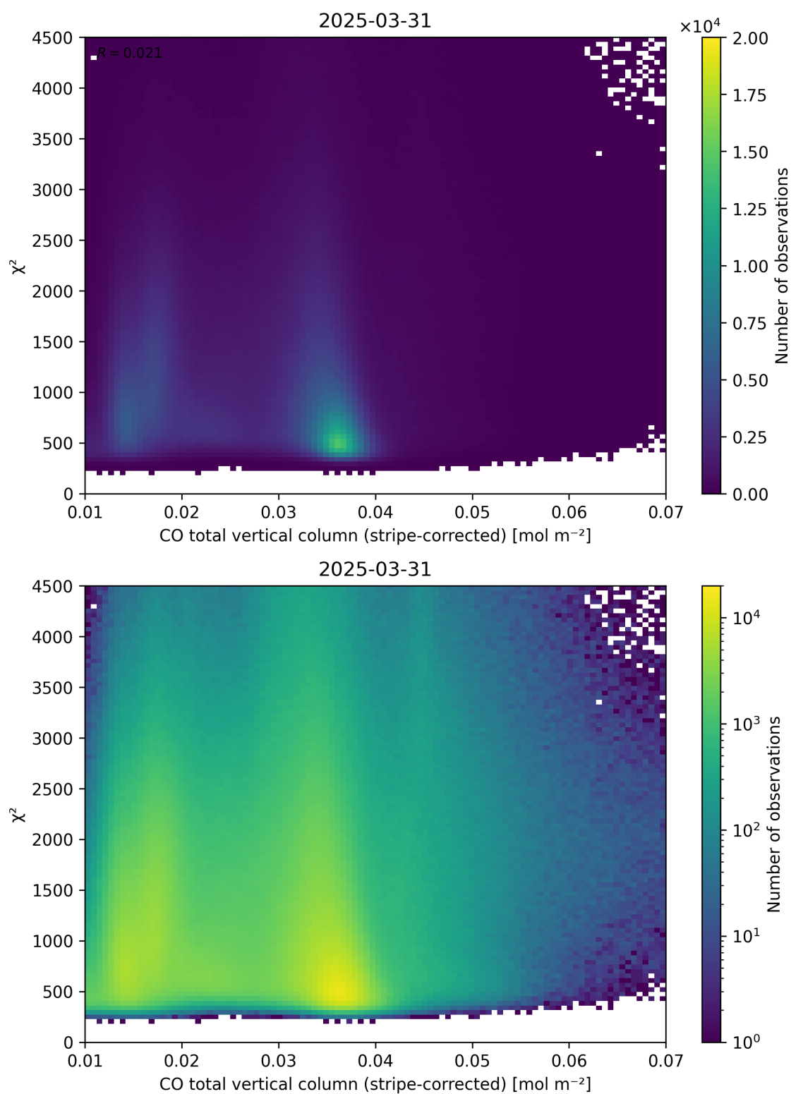
Figure 37: Scatter density plot of “CO total vertical column (stripe-corrected)” against “ \chi^2 ” for 2025-03-30 to 2025-04-01.
