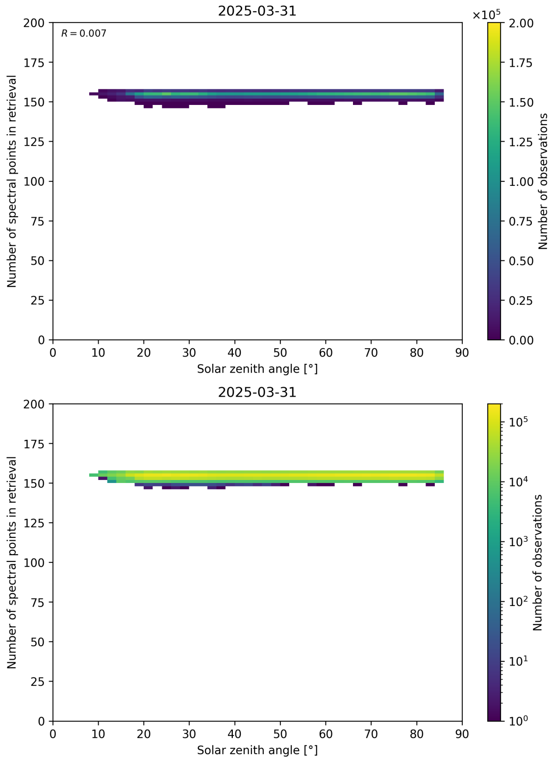
Figure 68: Scatter density plot of “Solar zenith angle” against “Number of spectral points in retrieval” for 2025-03-30 to 2025-04-01.
