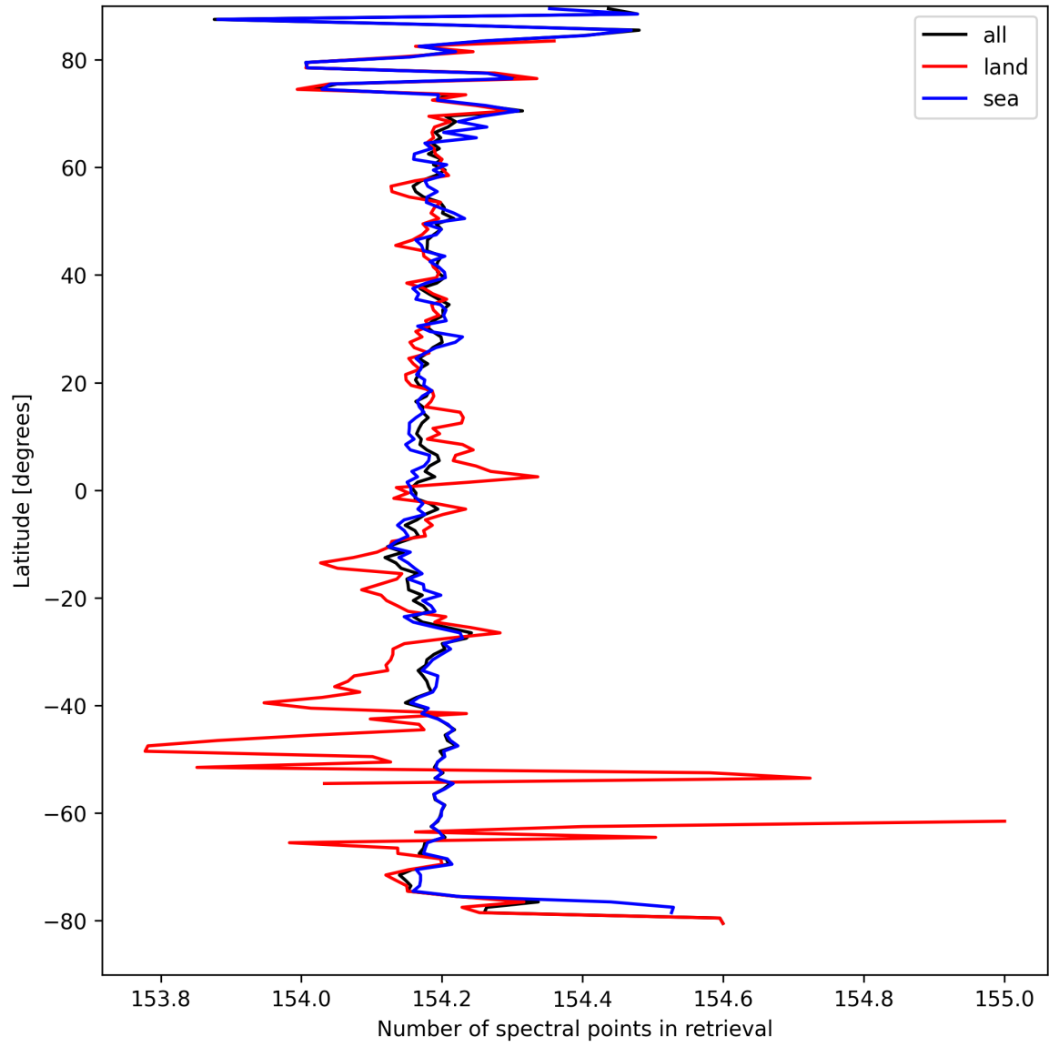
Figure 13: Zonal average of “Number of spectral points in retrieval” for 2025-03-30 to 2025-04-01.
