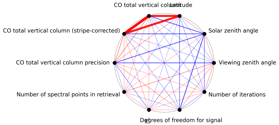
Figure 1: Map of correlation graph for 2025-03-30 to 2025-04-01.
