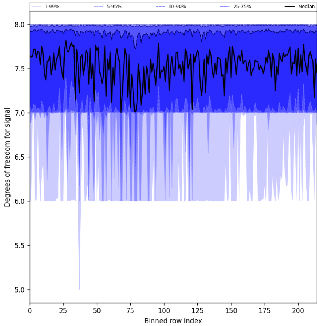
Figure 31: Along track statistics of “Degrees of freedom for signal” for 2025-03-30 to 2025-04-01
