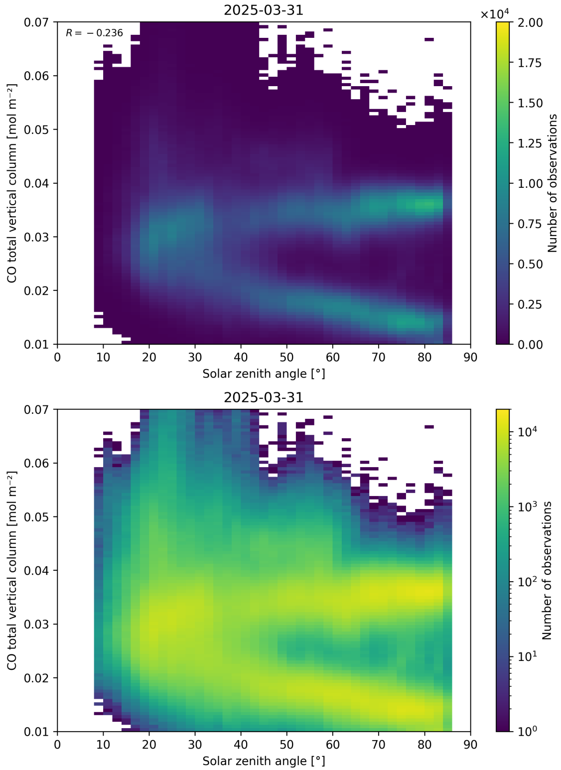
Figure 61: Scatter density plot of “Solar zenith angle” against “CO total vertical column” for 2025-03-30 to 2025-04-01.
