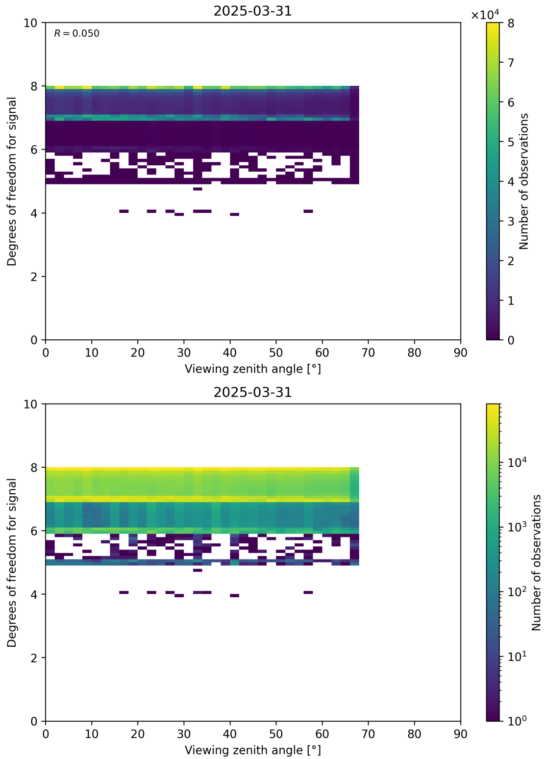
Figure 73: Scatter density plot of “Viewing zenith angle” against “Degrees of freedom for signal” for 2025-03-30 to 2025-04-01.
