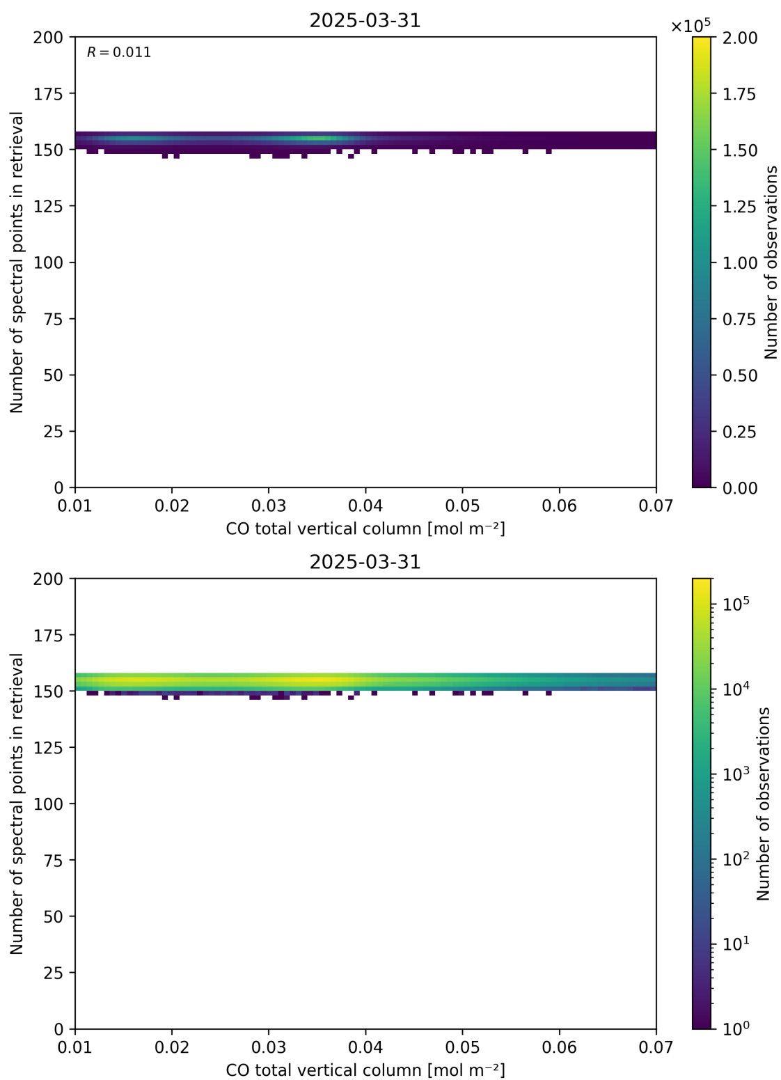
Figure 43: Scatter density plot of “CO total vertical column” against “Number of spectral points in retrieval” for 2025-03-30 to 2025-04-01.
