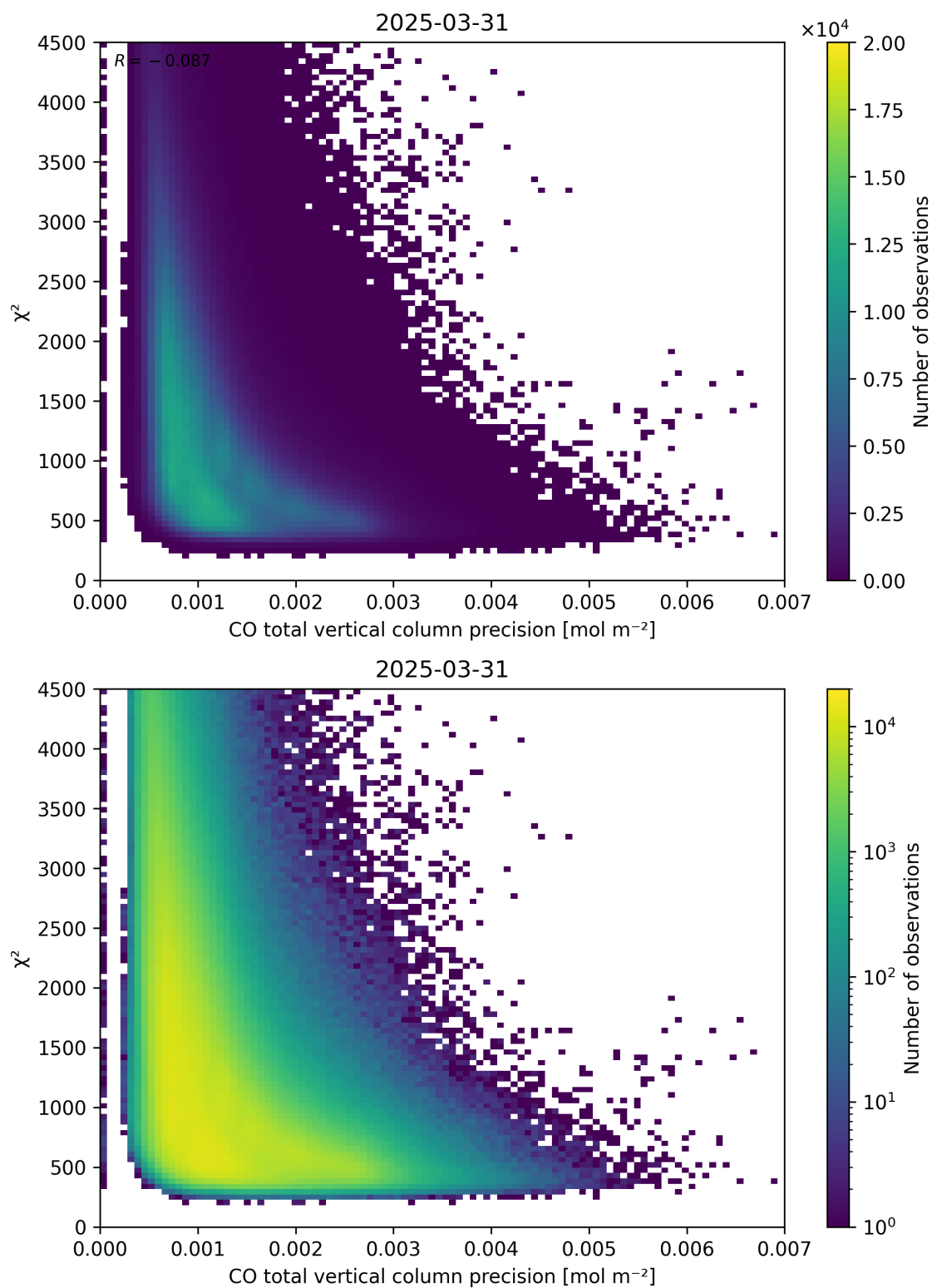
Figure 44: Scatter density plot of “CO total vertical column precision” against “ \chi^2 ” for 2025-03-30 to 2025-04-01.
