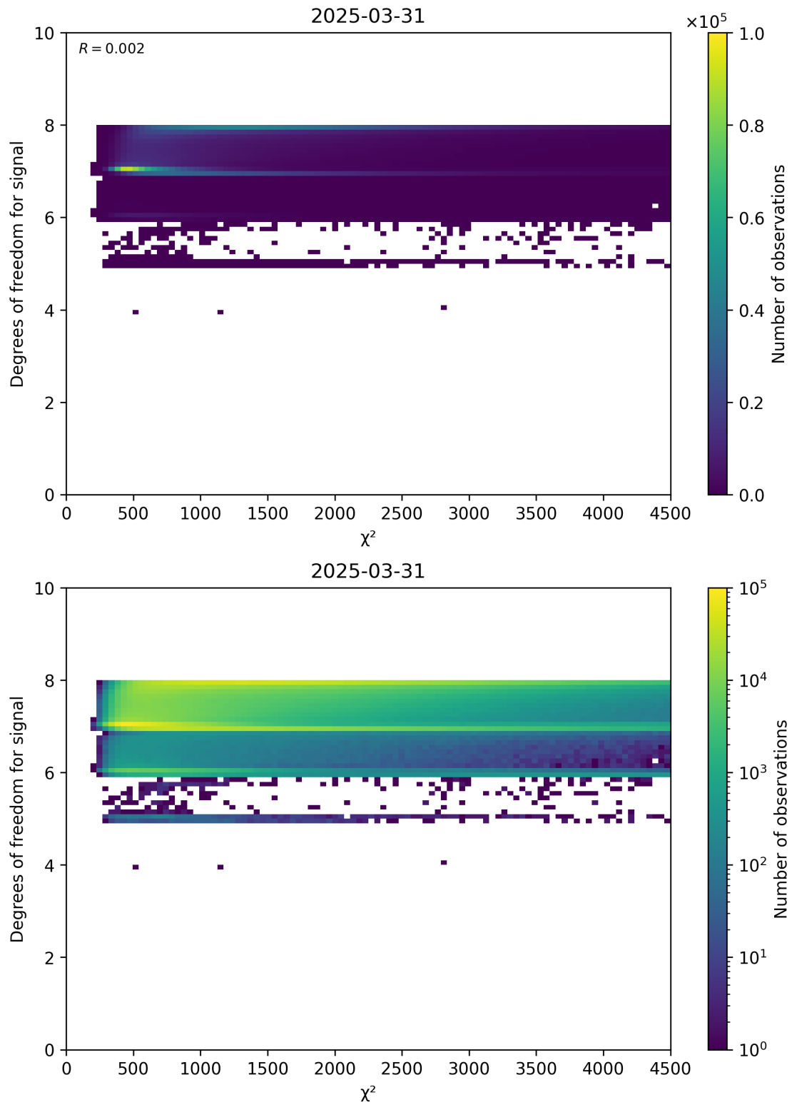
Figure 48: Scatter density plot of “ \chi^2 ” against “Degrees of freedom for signal” for 2025-03-30 to 2025-04-01.
