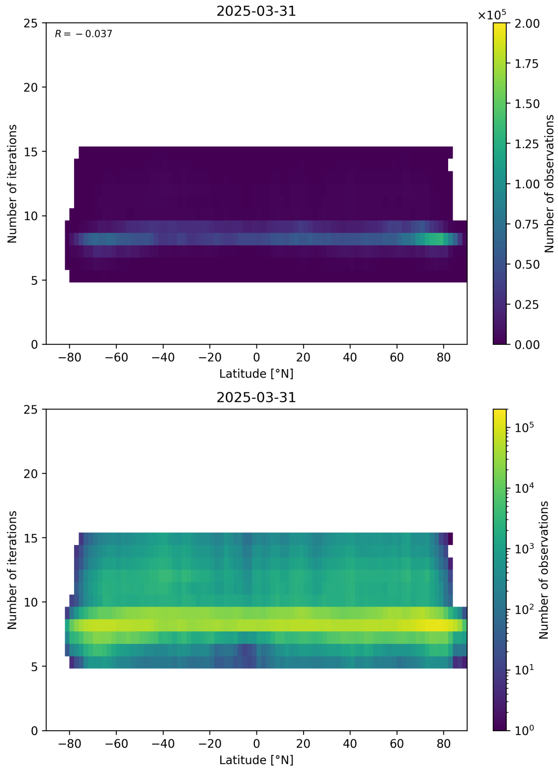
Figure 56: Scatter density plot of “Latitude” against “Number of iterations” for 2025-03-30 to 2025-04-01.
