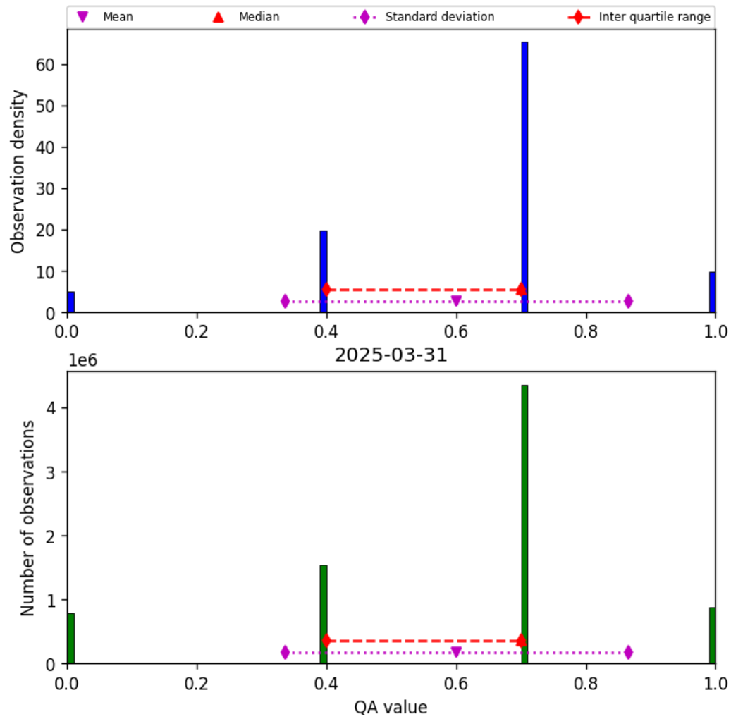
Figure 17: Histogram of “QA value” for 2025-03-30 to 2025-04-01
