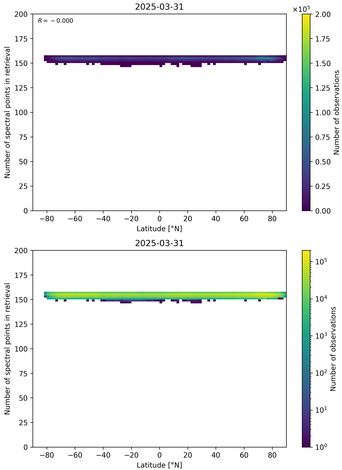
Figure 57: Scatter density plot of “Latitude” against “Number of spectral points in retrieval” for 2025-03-30 to 2025-04-01.
