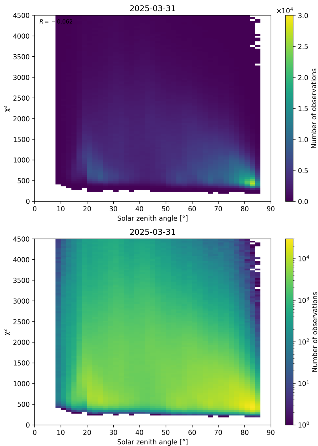
Figure 64: Scatter density plot of “Solar zenith angle” against “ \chi^2 ” for 2025-03-30 to 2025-04-01.
