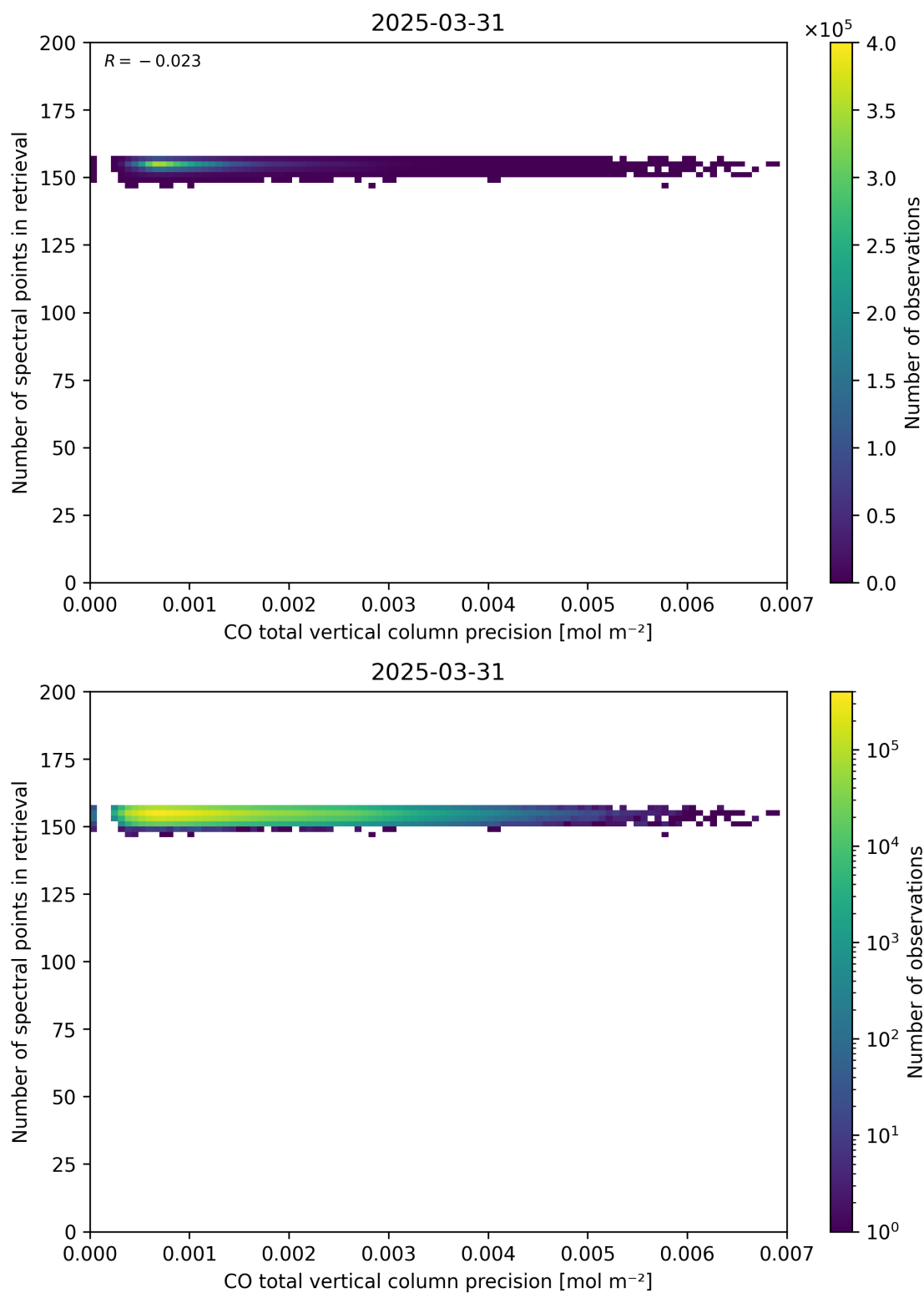
Figure 47: Scatter density plot of “CO total vertical column precision” against “Number of spectral points in retrieval” for 2025-03-30 to 2025-04-01.
