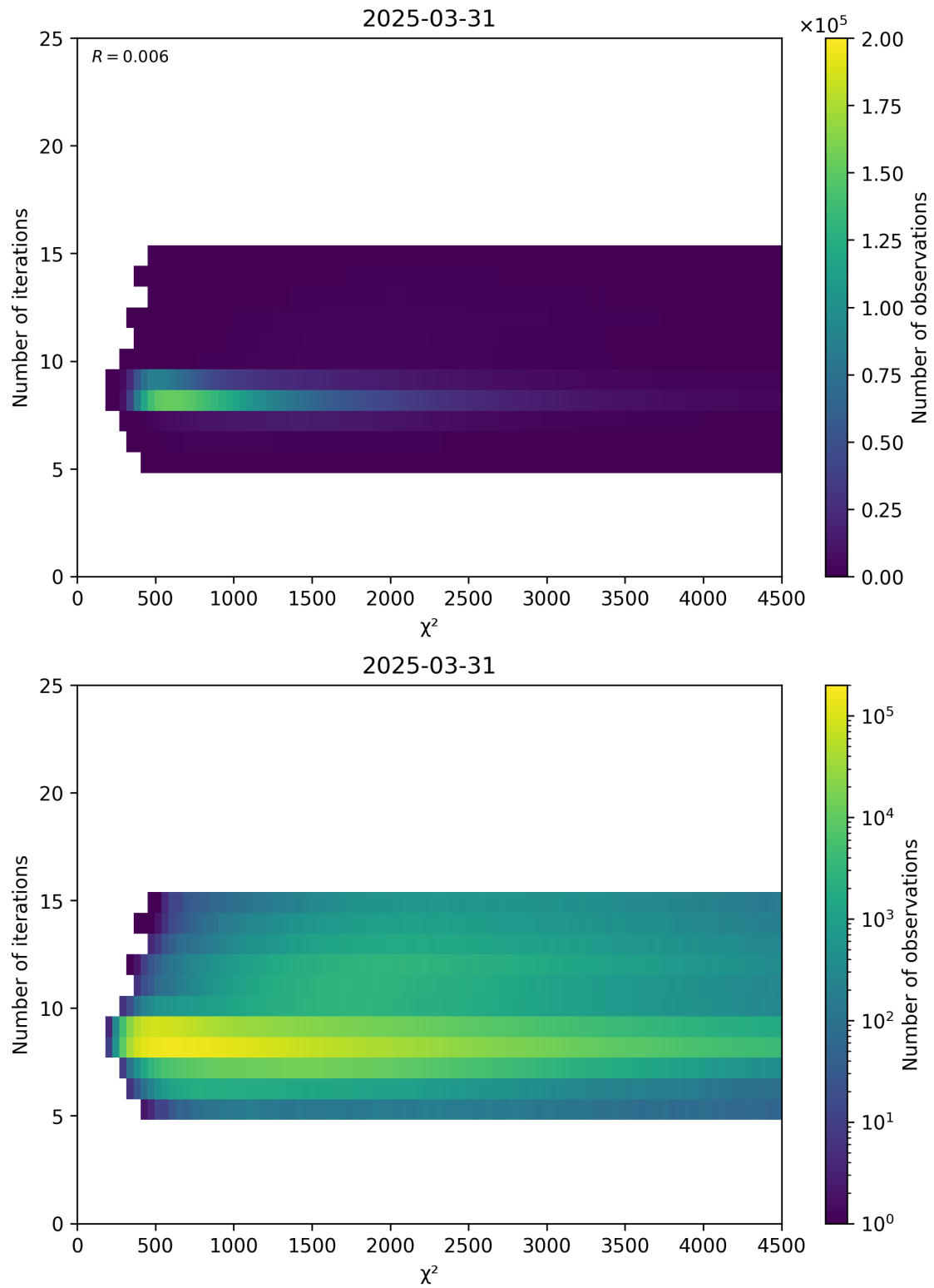
Figure 49: Scatter density plot of “ \chi^2 ” against “Number of iterations” for 2025-03-30 to 2025-04-01.
