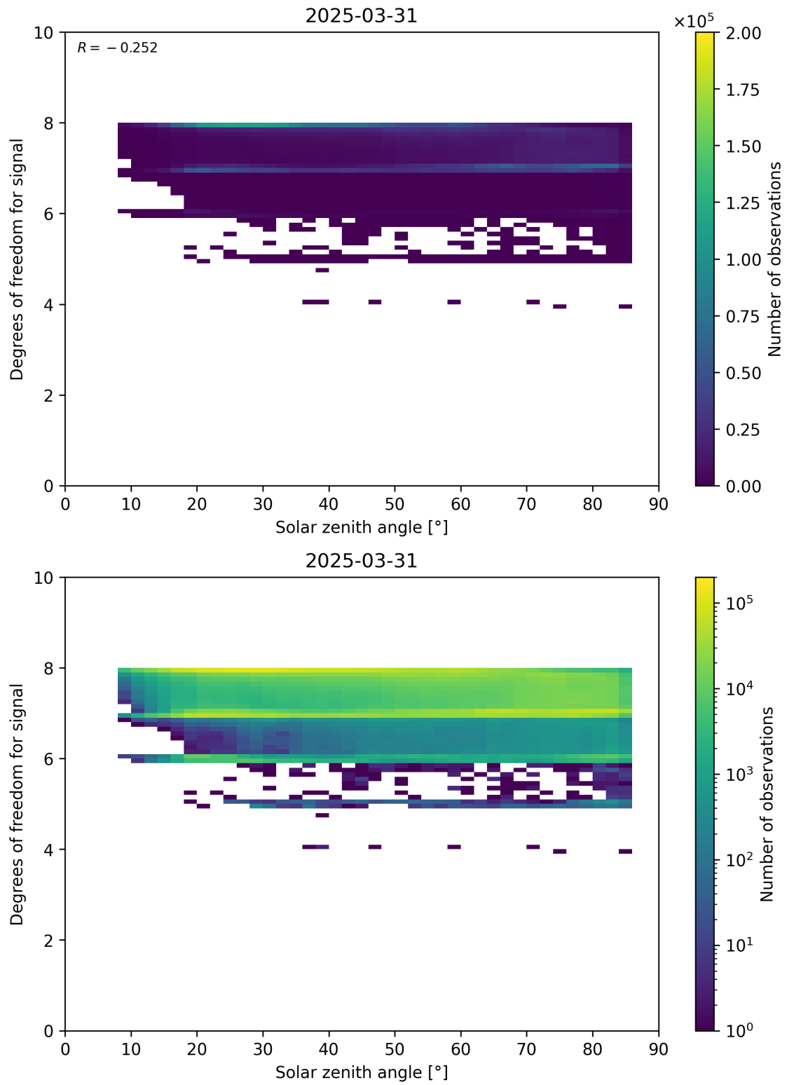
Figure 65: Scatter density plot of “Solar zenith angle” against “Degrees of freedom for signal” for 2025-03-30 to 2025-04-01.
