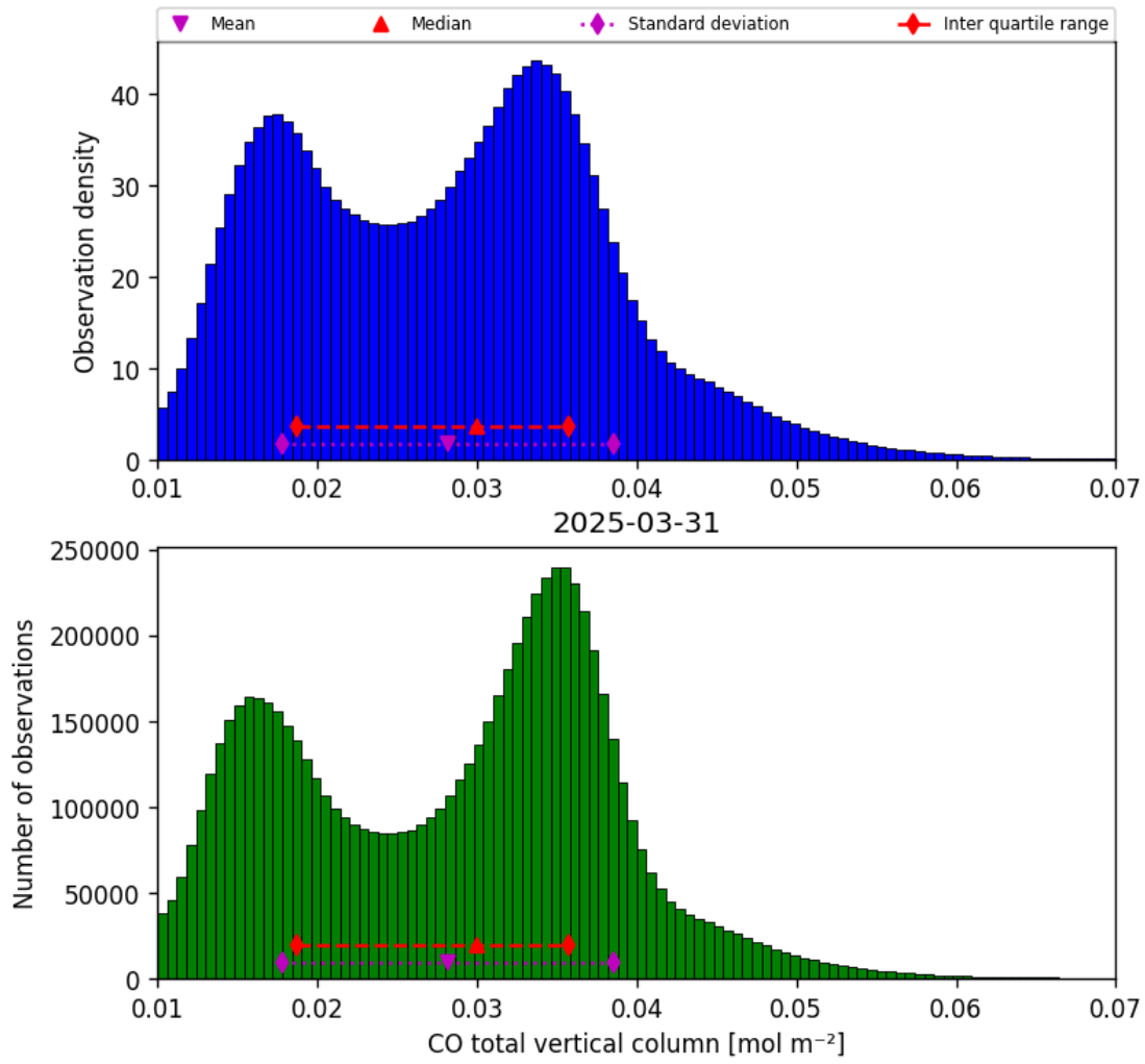
Figure 18: Histogram of “CO total vertical column” for 2025-03-30 to 2025-04-01
