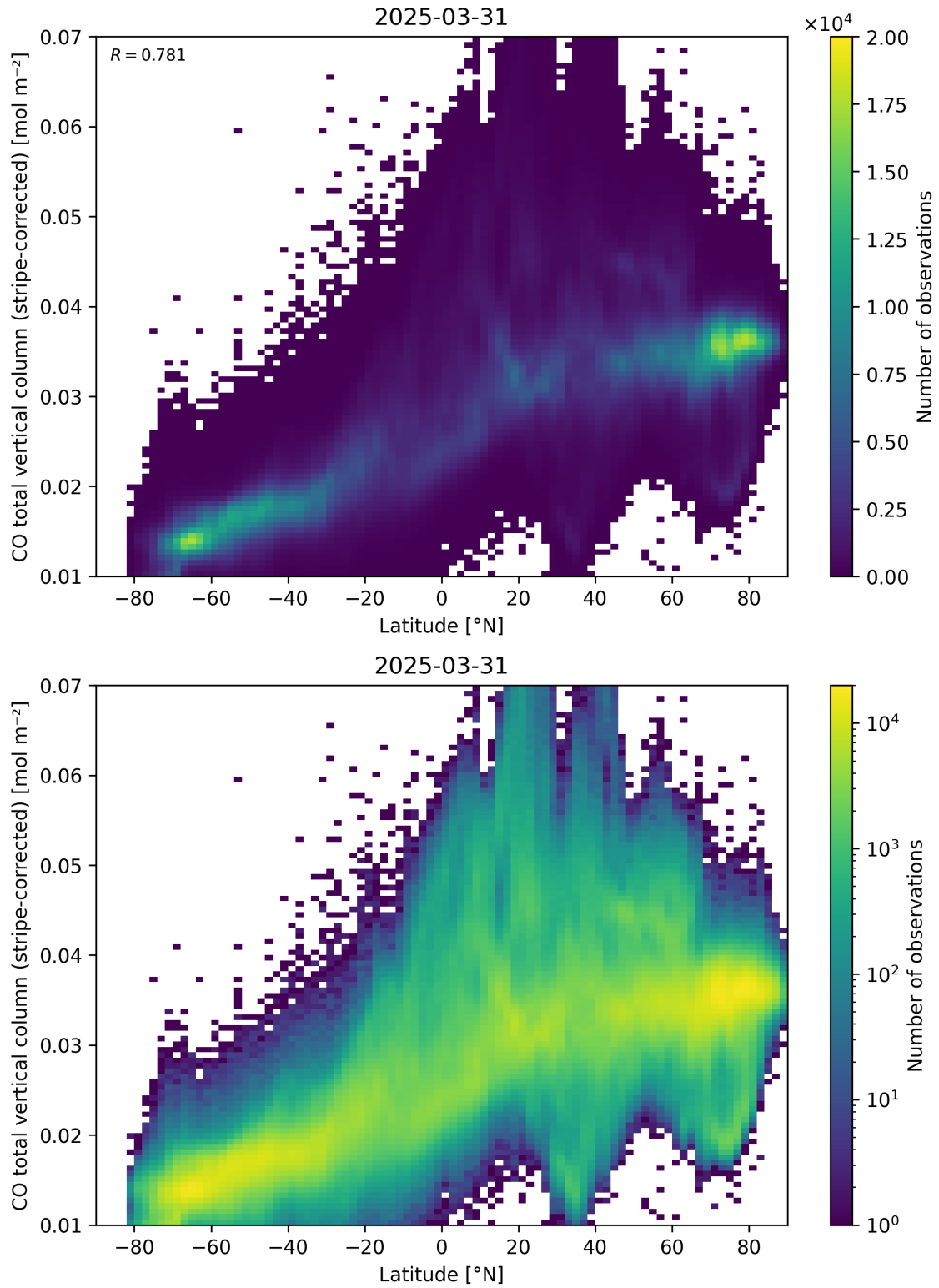
Figure 52: Scatter density plot of “Latitude” against “CO total vertical column (stripe-corrected)” for 2025-03-30 to 2025-04-01.
