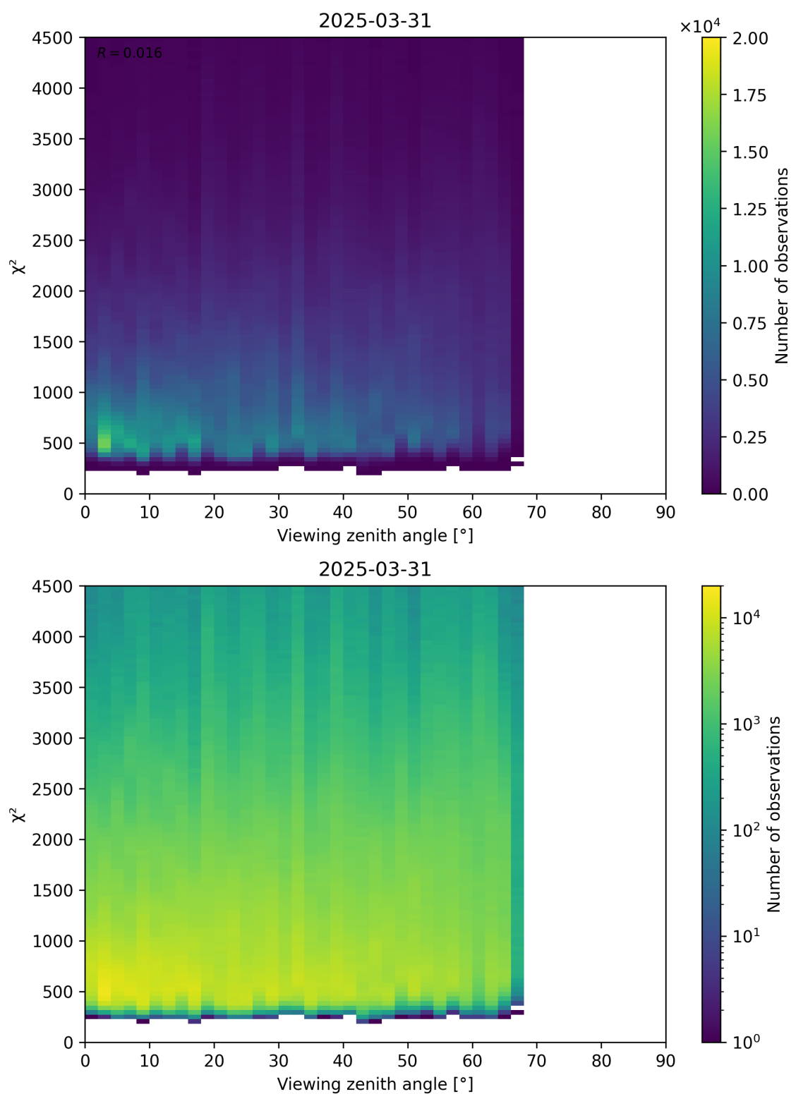
Figure 72: Scatter density plot of “Viewing zenith angle” against “ \chi^2 ” for 2025-03-30 to 2025-04-01.
