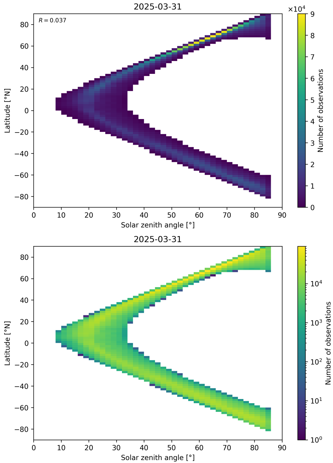
Figure 66: Scatter density plot of “Solar zenith angle” against “Latitude” for 2025-03-30 to 2025-04-01.
