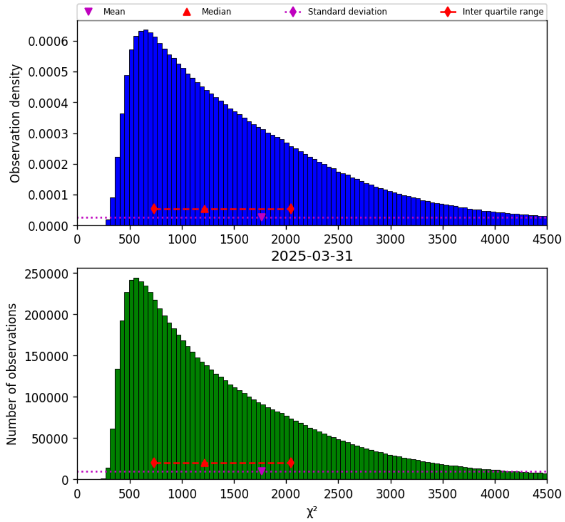
Figure 22: Histogram of “ \chi^2 ” for 2025-03-30 to 2025-04-01
