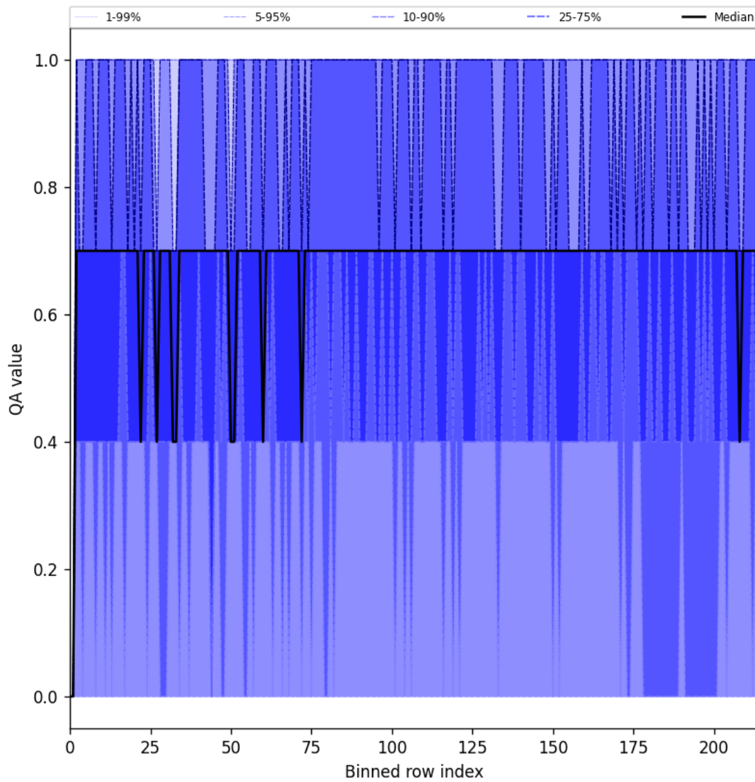
Figure 25: Along track statistics of “QA value” for 2025-03-30 to 2025-04-01
