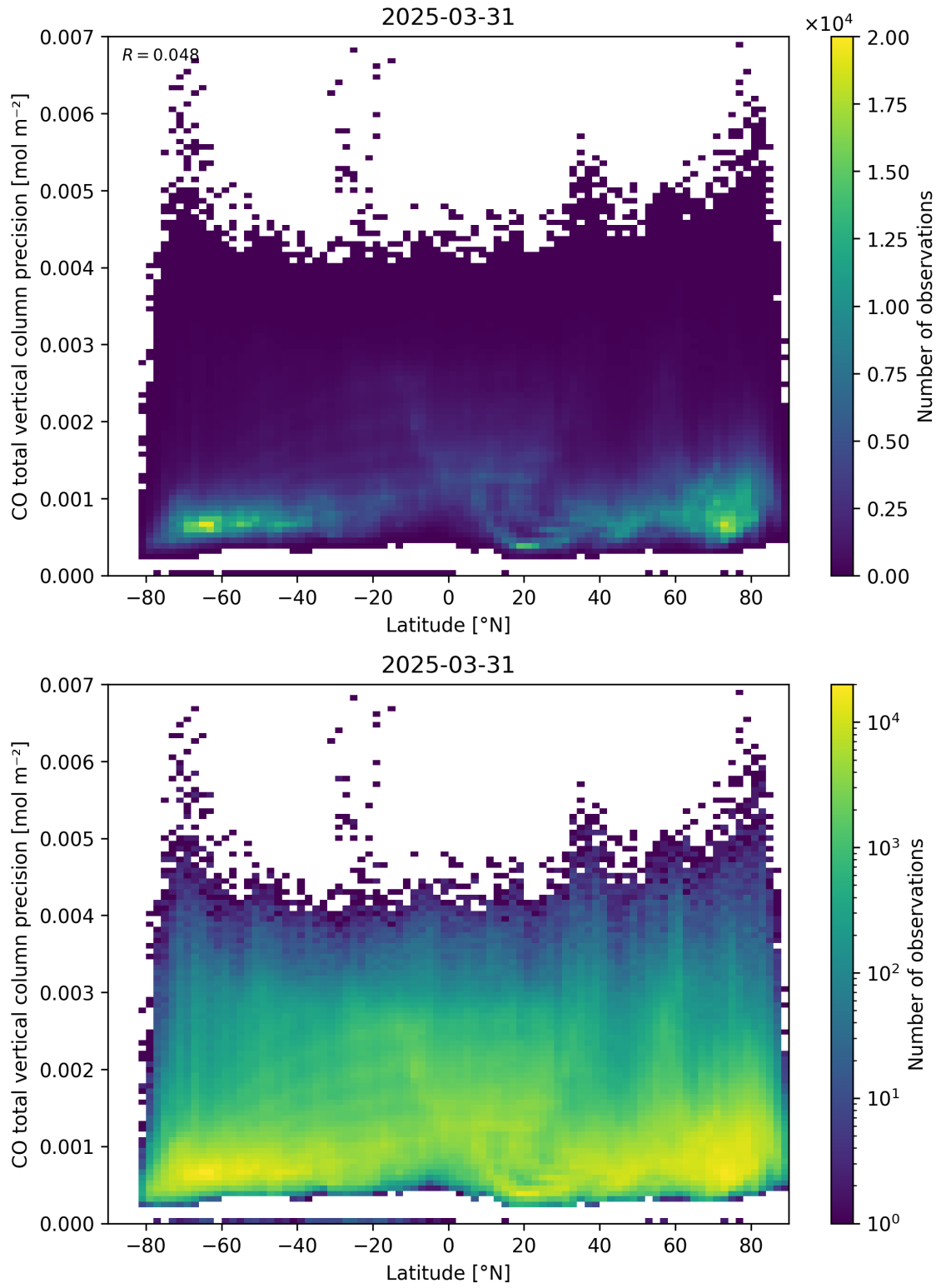
Figure 53: Scatter density plot of “Latitude” against “CO total vertical column precision” for 2025-03-30 to 2025-04-01.
