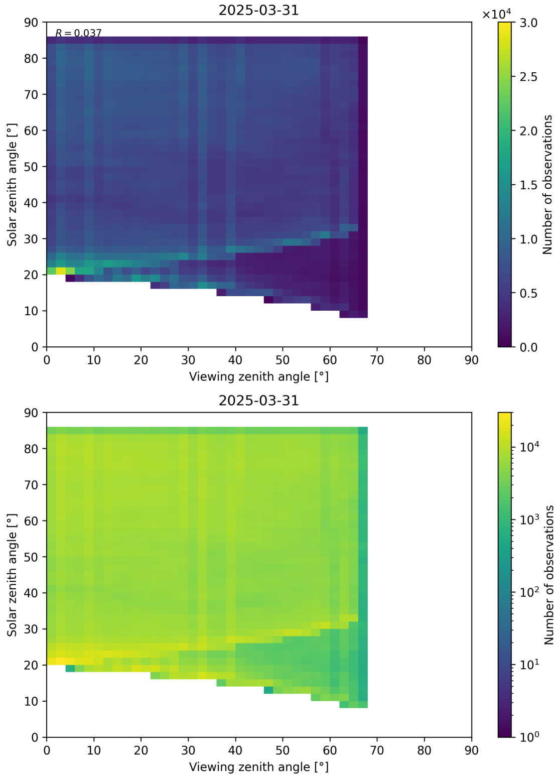
Figure 77: Scatter density plot of “Viewing zenith angle” against “Solar zenith angle” for 2025-03-30 to 2025-04-01.
