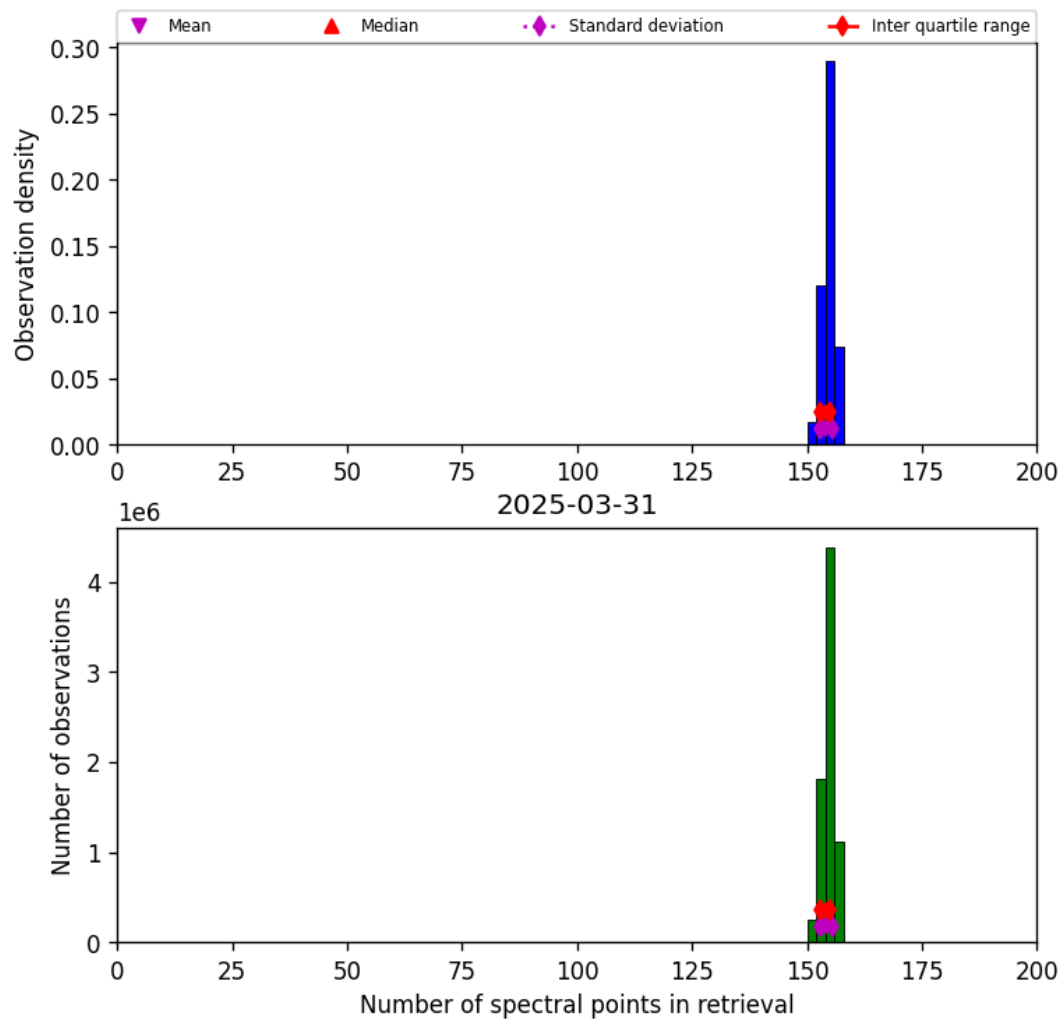
Figure 21: Histogram of “Number of spectral points in retrieval” for 2025-03-30 to 2025-04-01
