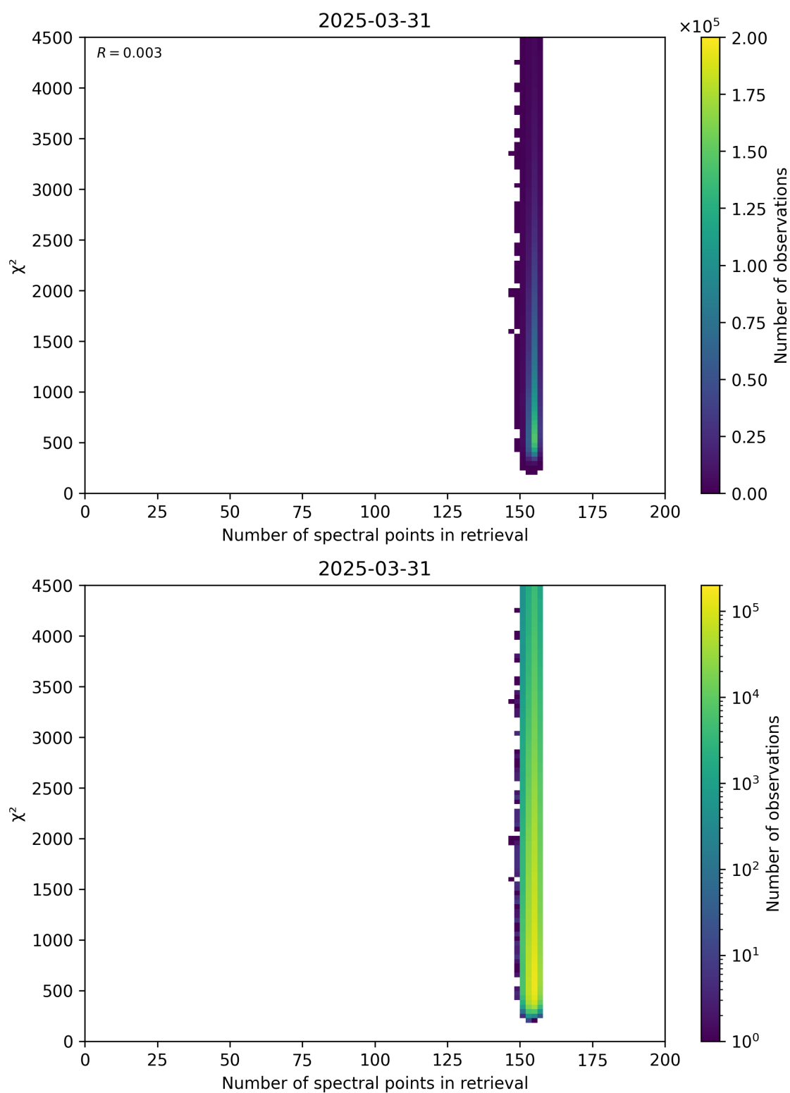
Figure 58: Scatter density plot of “Number of spectral points in retrieval” against “ \chi^2 ” for 2025-03-30 to 2025-04-01.
