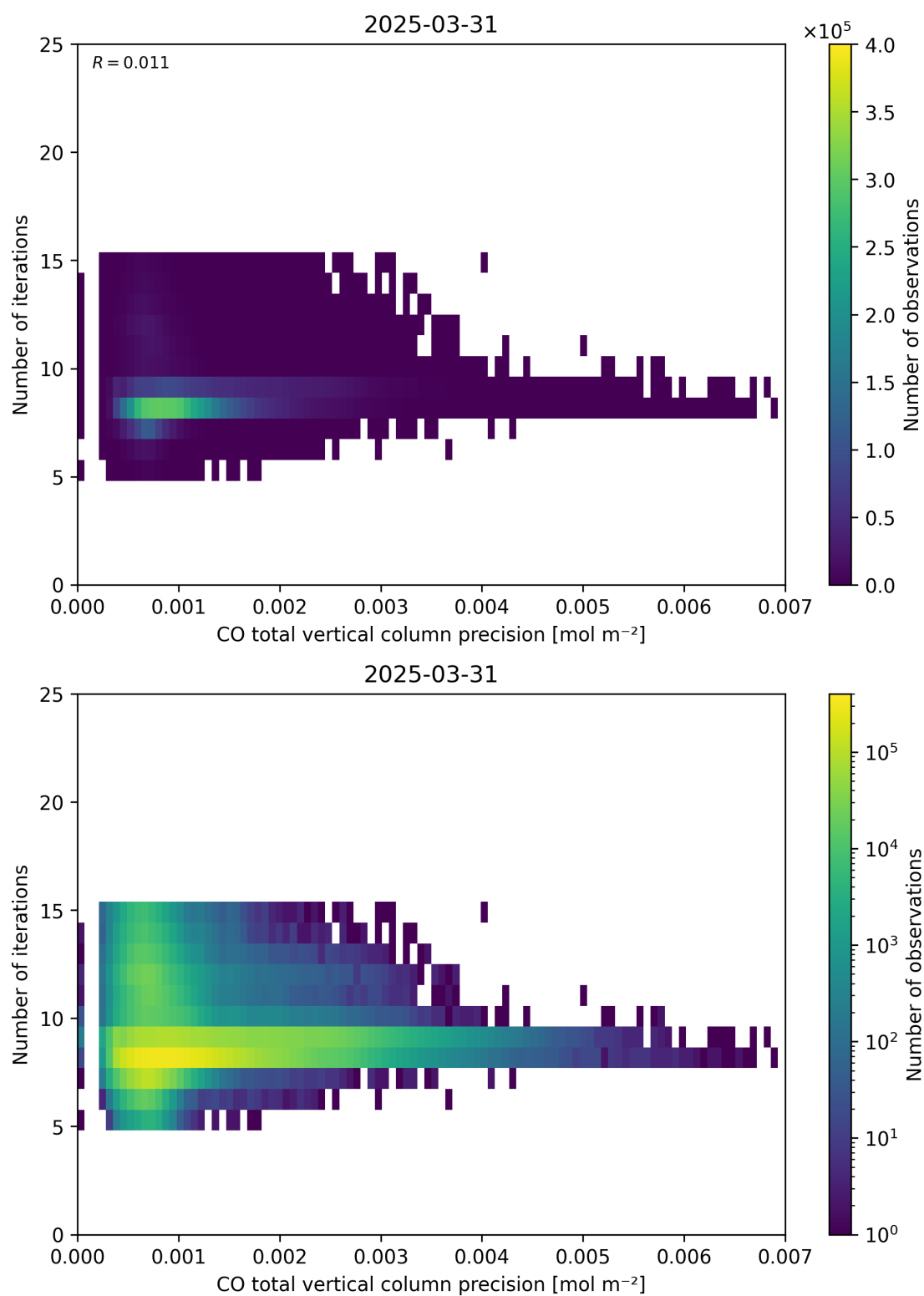
Figure 46: Scatter density plot of “CO total vertical column precision” against “Number of iterations” for 2025-03-30 to 2025-04-01.
