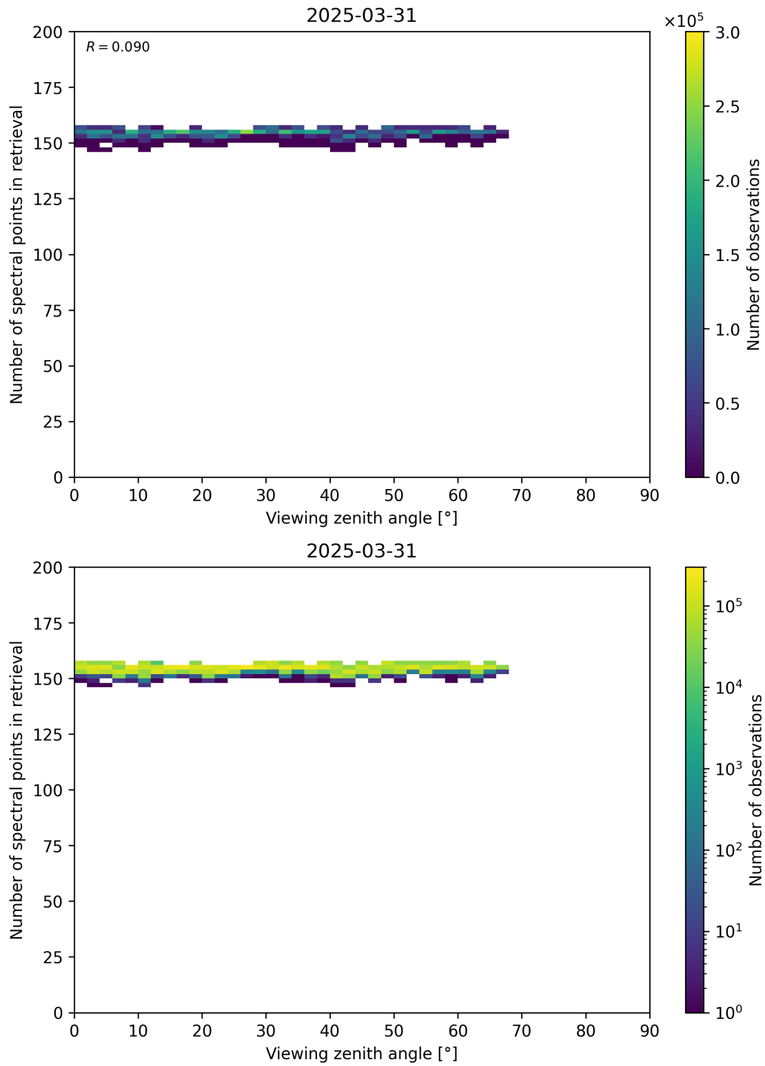
Figure 76: Scatter density plot of “Viewing zenith angle” against “Number of spectral points in retrieval” for 2025-03-30 to 2025-04-01.
