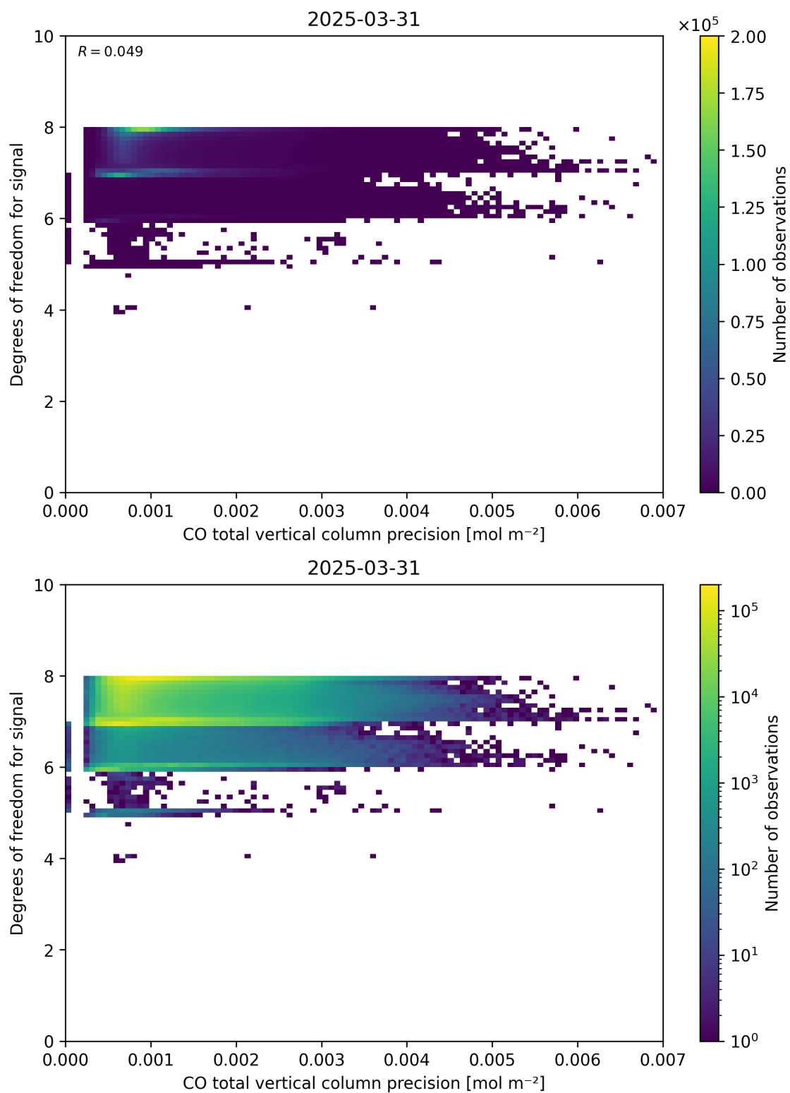
Figure 45: Scatter density plot of “CO total vertical column precision” against “Degrees of freedom for signal” for 2025-03-30 to 2025-04-01.
