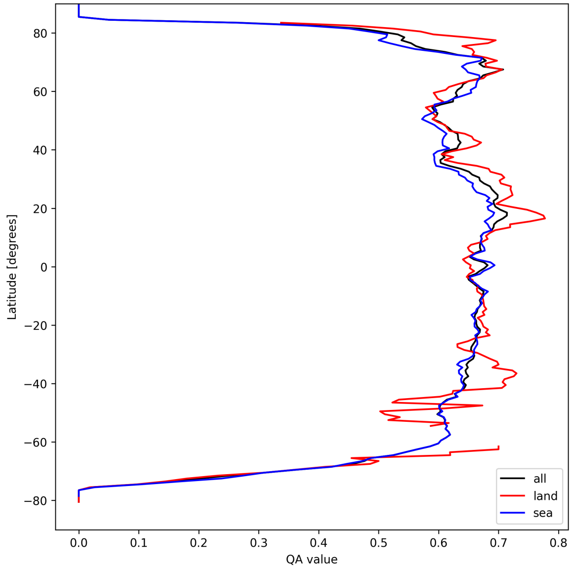
Figure 9: Zonal average of “QA value” for 2025-03-30 to 2025-04-01.
