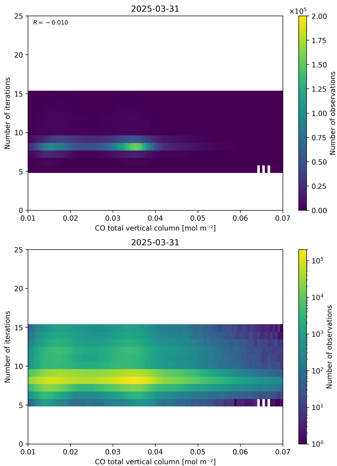
Figure 42: Scatter density plot of “CO total vertical column” against “Number of iterations” for 2025-03-30 to 2025-04-01.
