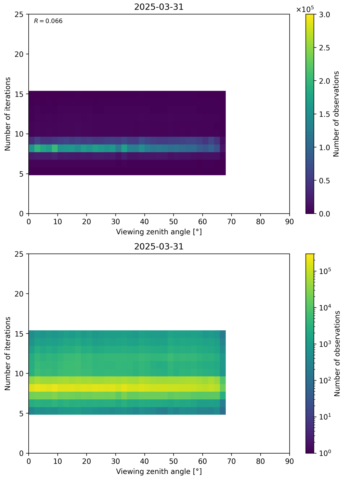
Figure 75: Scatter density plot of “Viewing zenith angle” against “Number of iterations” for 2025-03-30 to 2025-04-01.
