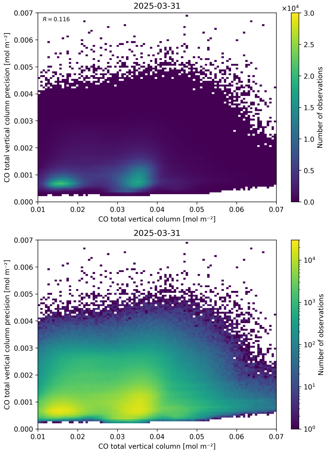
Figure 34: Scatter density plot of “CO total vertical column” against “CO total vertical column precision” for 2025-03-30 to 2025-04-01.
