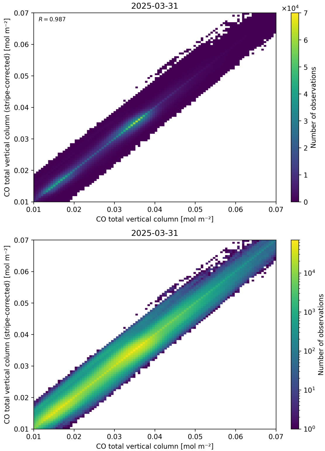
Figure 33: Scatter density plot of “CO total vertical column” against “CO total vertical column (stripe-corrected)” for 2025-03-30 to 2025-04-01.
