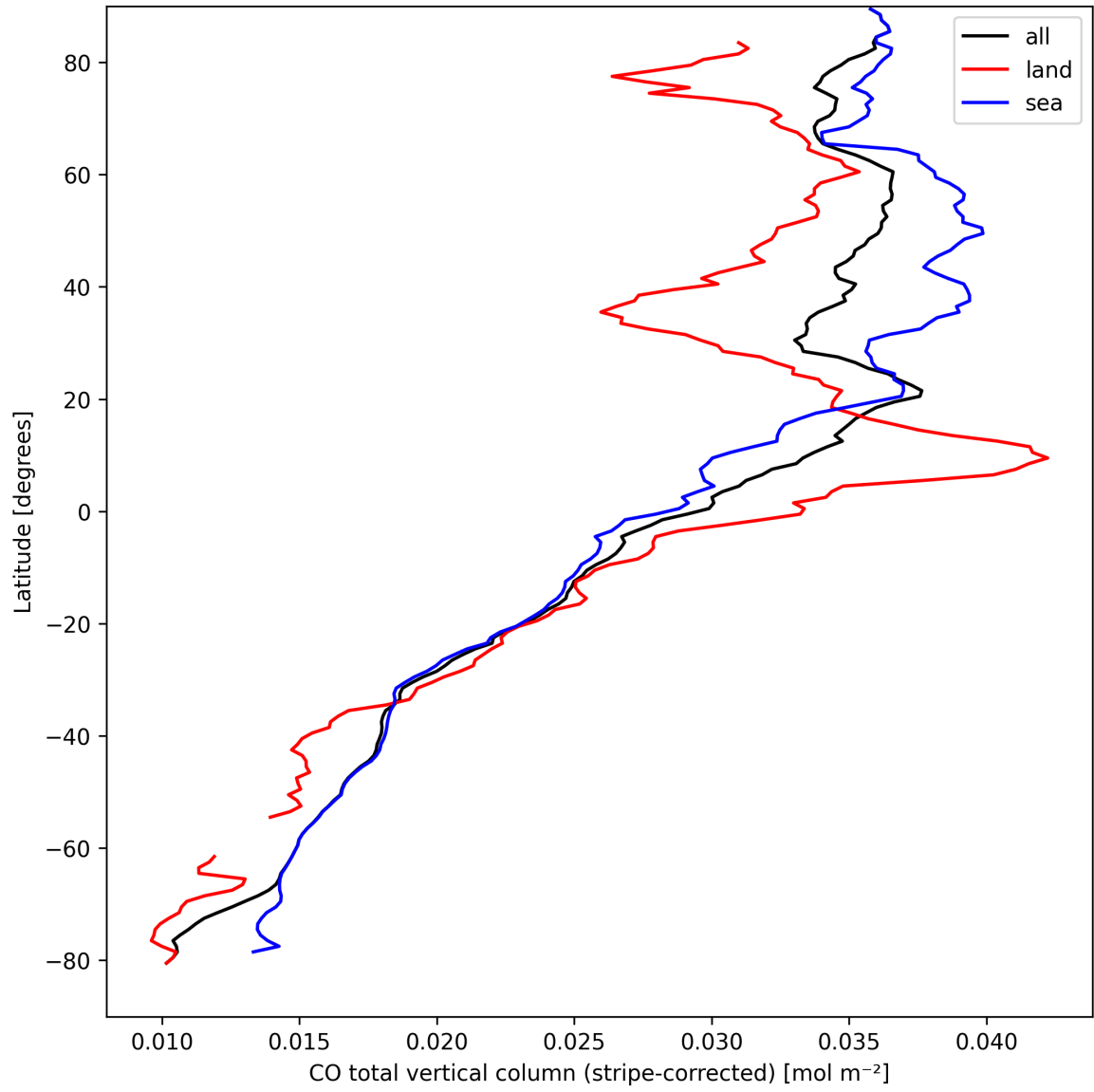
Figure 11: Zonal average of “CO total vertical column (stripe-corrected)” for 2025-03-30 to 2025-04-01.
