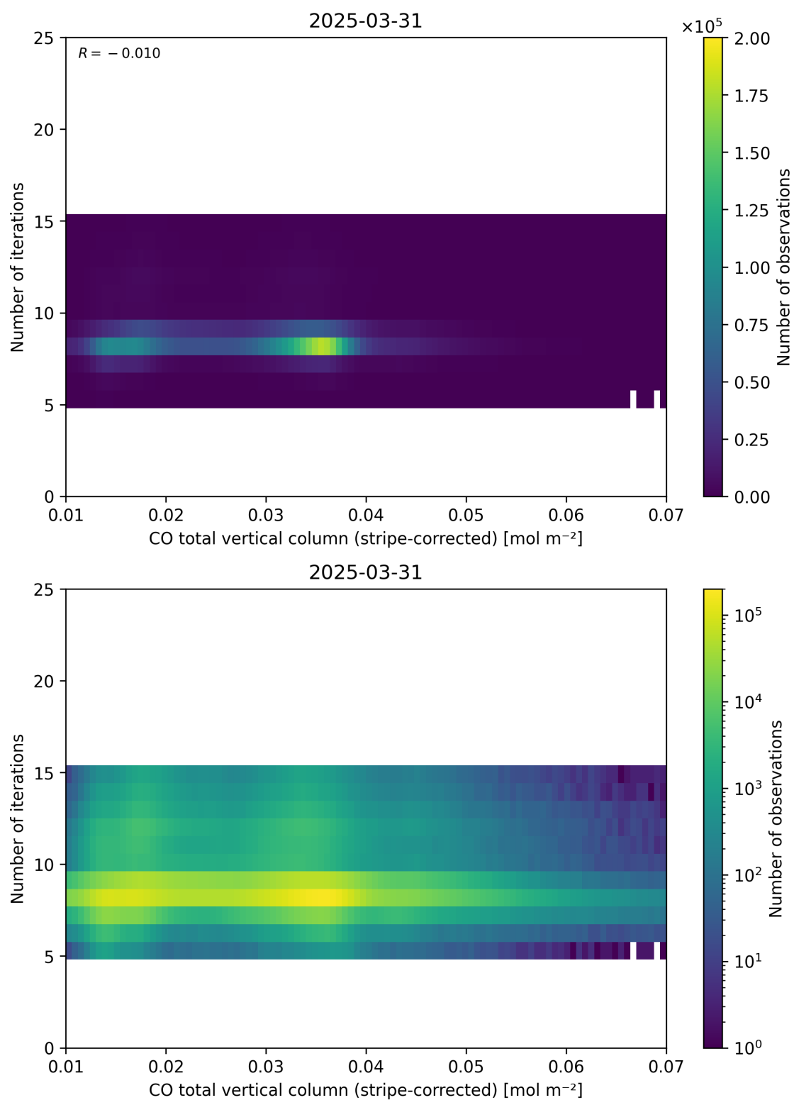
Figure 39: Scatter density plot of “CO total vertical column (stripe-corrected)” against “Number of iterations” for 2025-03-30 to 2025-04-01.
