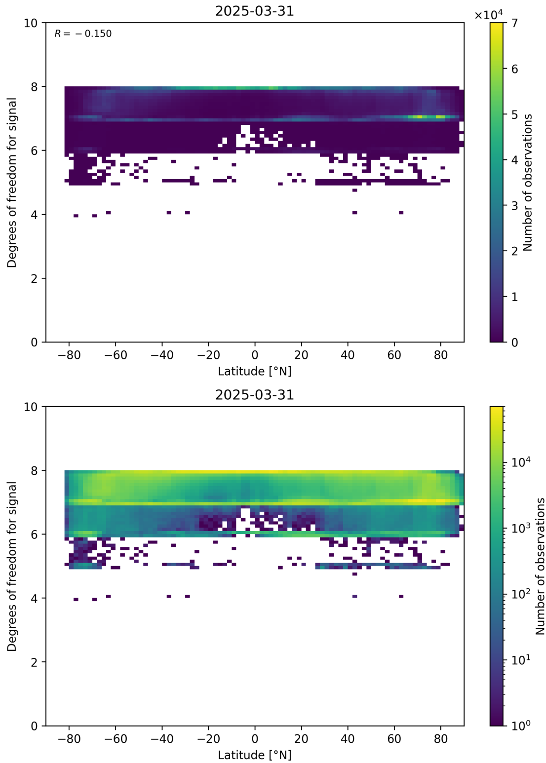
Figure 55: Scatter density plot of “Latitude” against “Degrees of freedom for signal” for 2025-03-30 to 2025-04-01.
