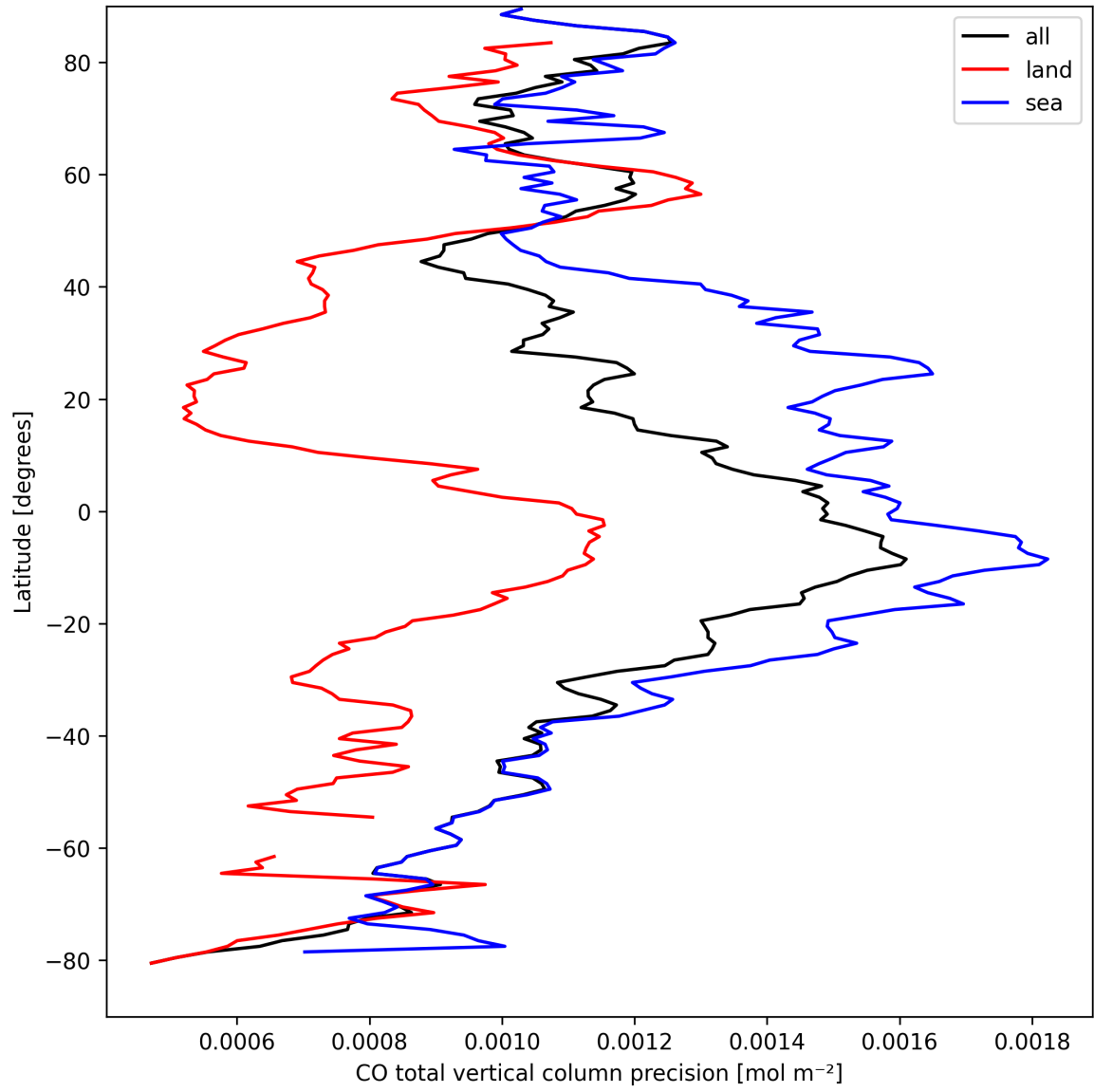
Figure 12: Zonal average of “CO total vertical column precision” for 2025-03-30 to 2025-04-01.
