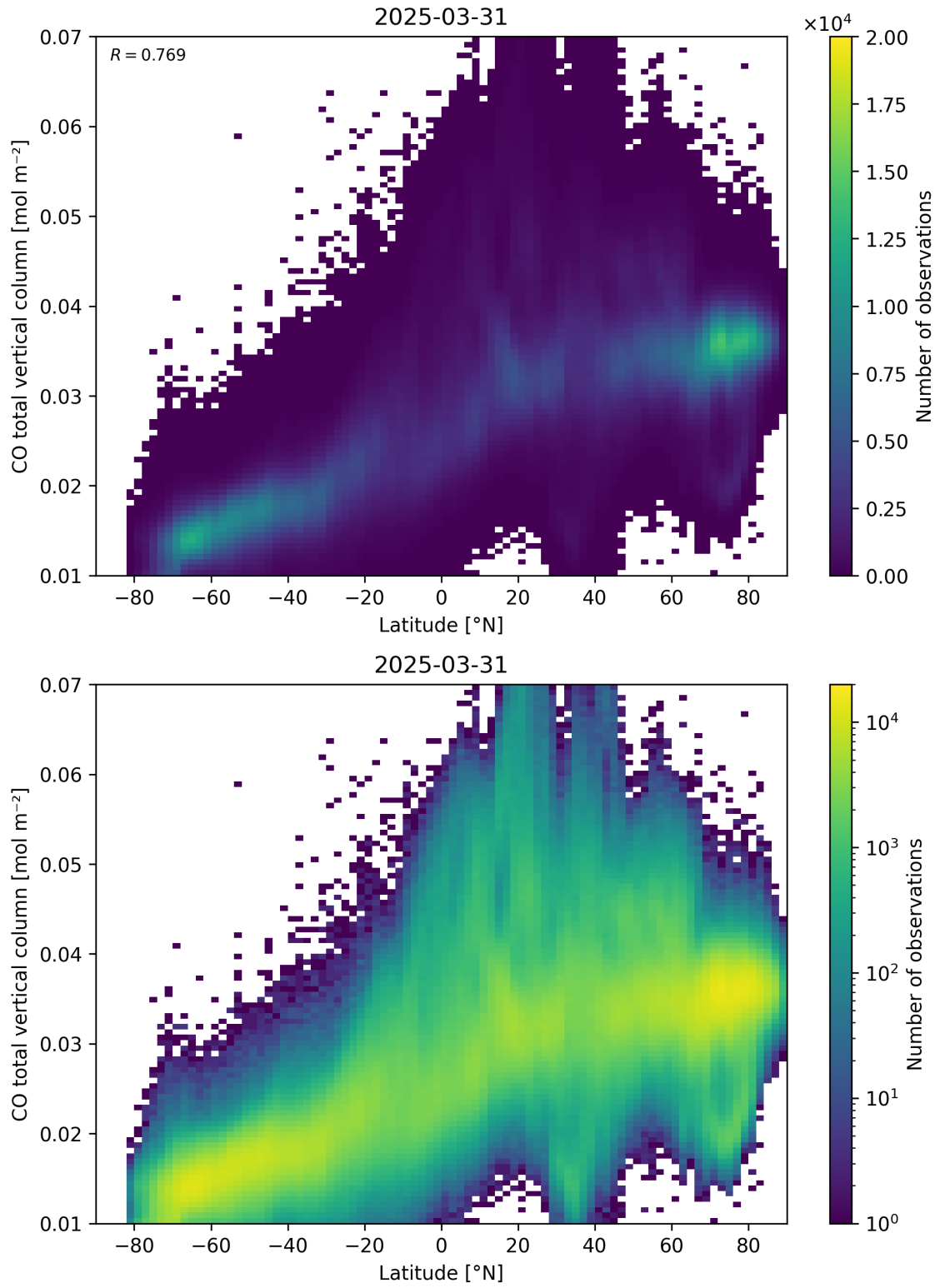
Figure 51: Scatter density plot of “Latitude” against “CO total vertical column” for 2025-03-30 to 2025-04-01.
