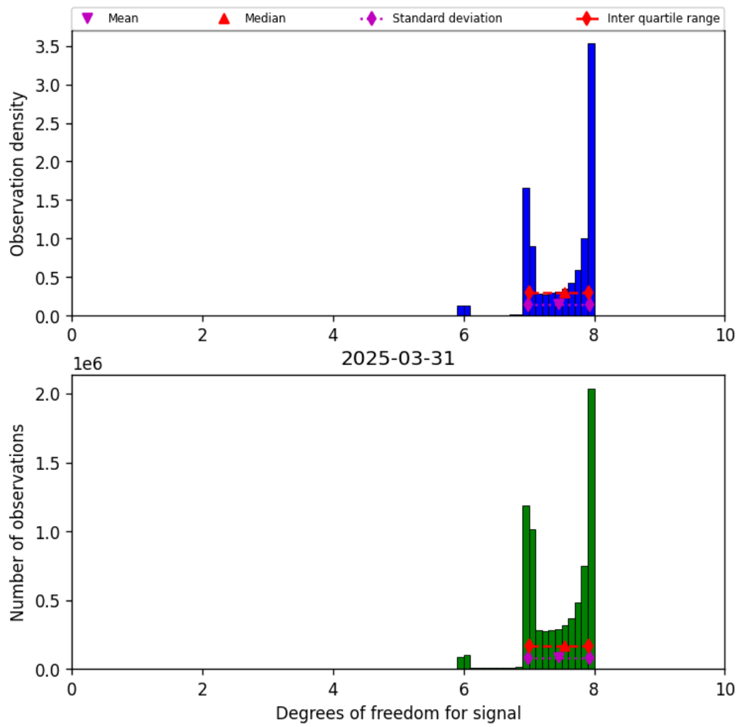
Figure 23: Histogram of “Degrees of freedom for signal” for 2025-03-30 to 2025-04-01
