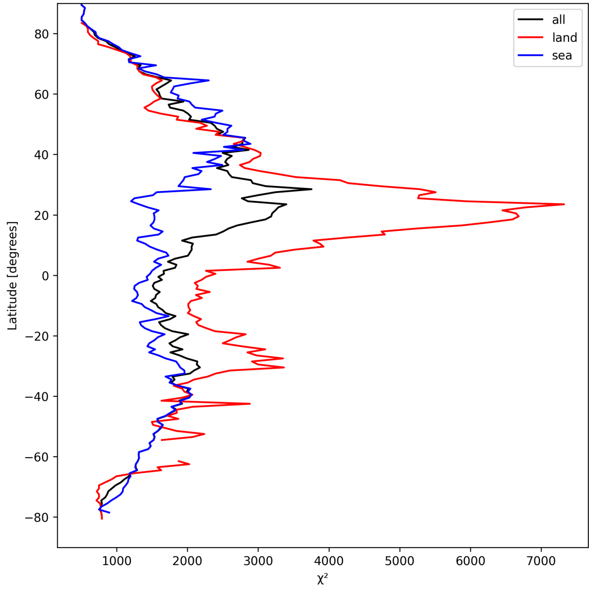
Figure 14: Zonal average of “ \chi^2 ” for 2025-03-30 to 2025-04-01.
