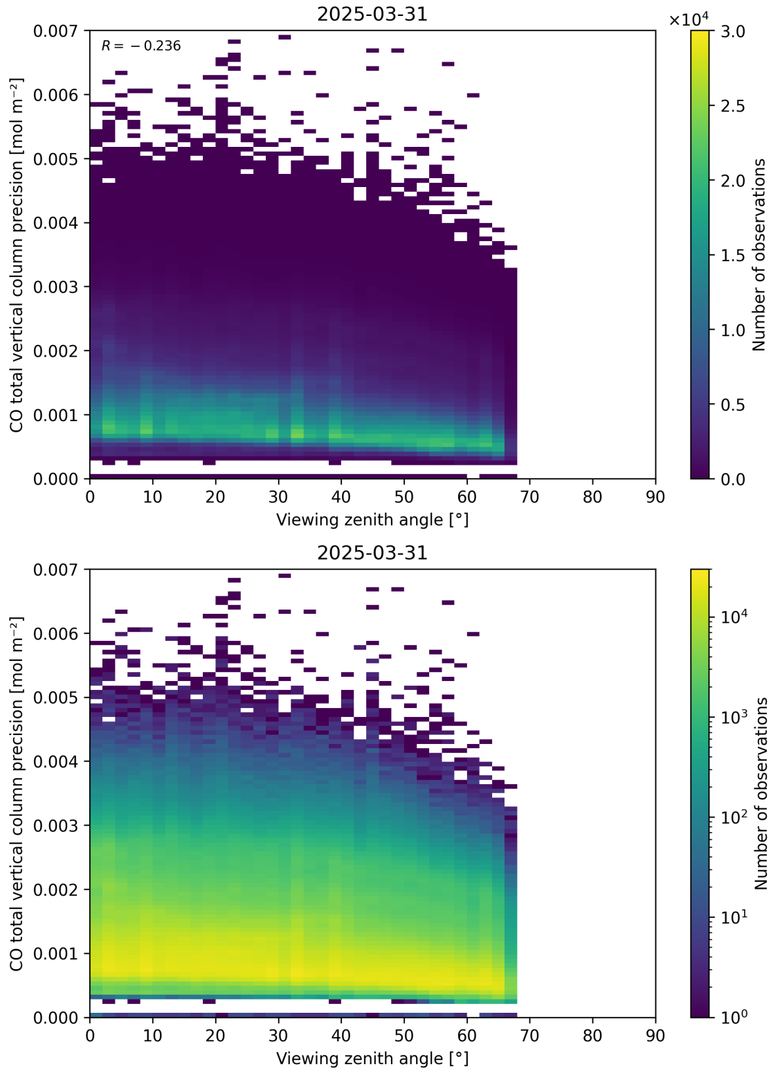
Figure 71: Scatter density plot of “Viewing zenith angle” against “CO total vertical column precision” for 2025-03-30 to 2025-04-01.
