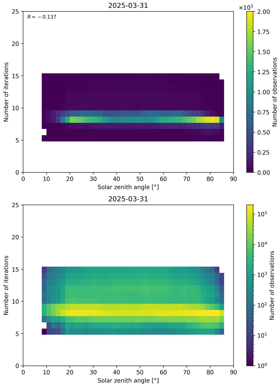
Figure 67: Scatter density plot of “Solar zenith angle” against “Number of iterations” for 2025-03-30 to 2025-04-01.
