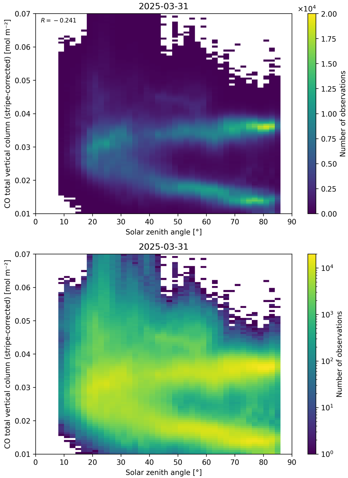
Figure 62: Scatter density plot of “Solar zenith angle” against “CO total vertical column (stripe-corrected)” for 2025-03-30 to 2025-04-01.
