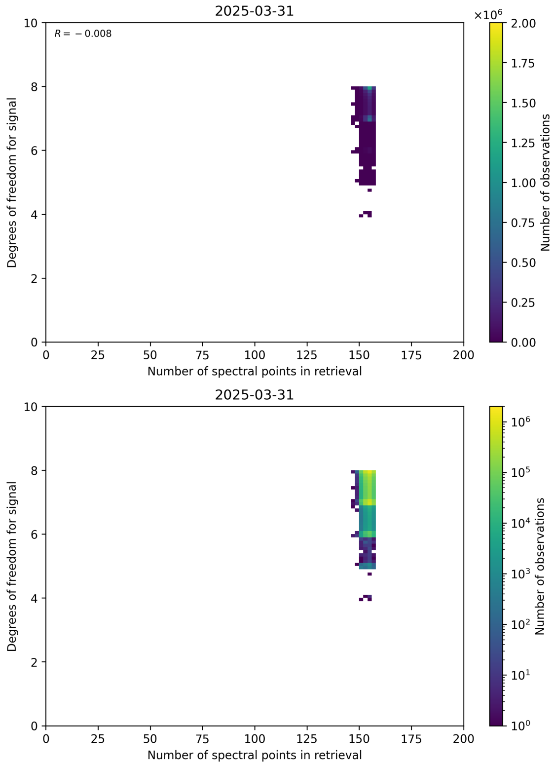
Figure 59: Scatter density plot of “Number of spectral points in retrieval” against “Degrees of freedom for signal” for 2025-03-30 to 2025-04-01.
