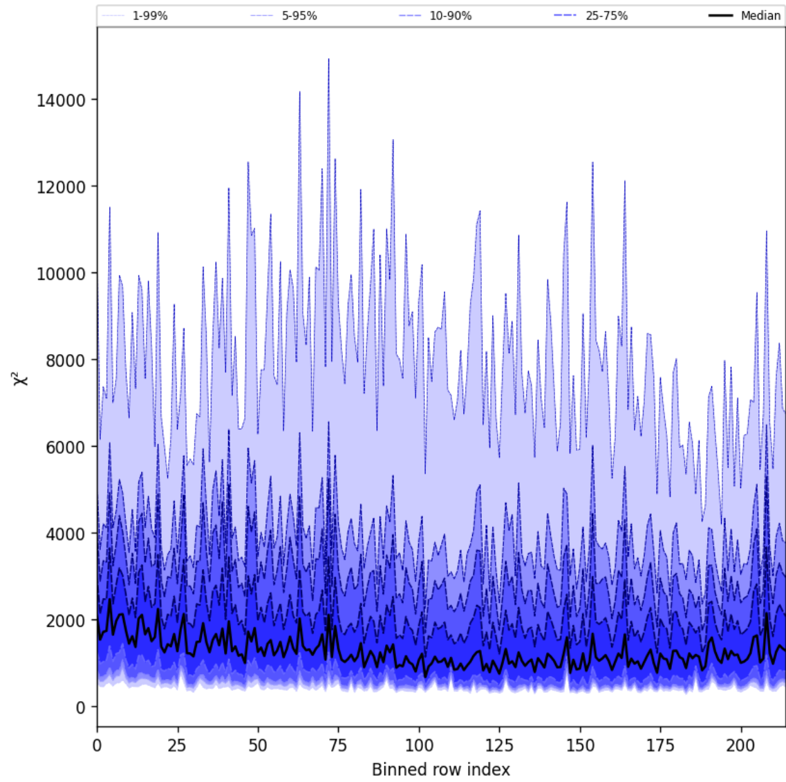
Figure 30: Along track statistics of “ \chi^2 ” for 2025-03-30 to 2025-04-01
