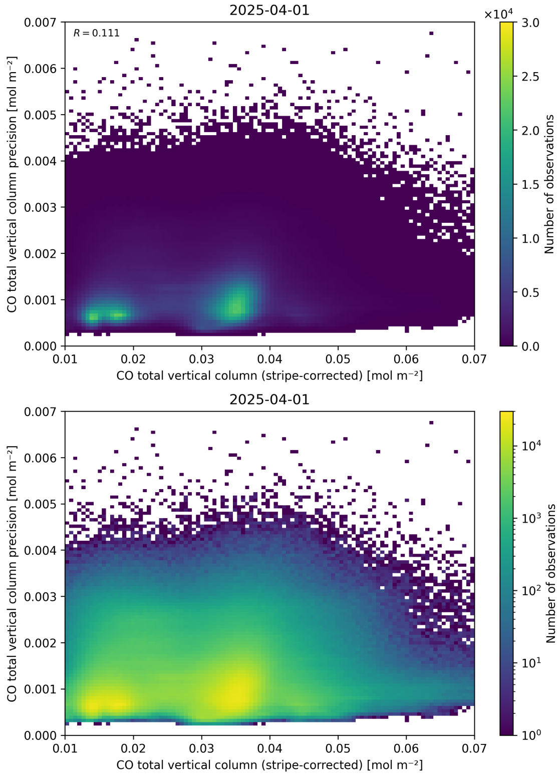
Figure 36: Scatter density plot of “CO total vertical column (stripe-corrected)” against “CO total vertical column precision” for 2025-03-31 to 2025-04-02.
