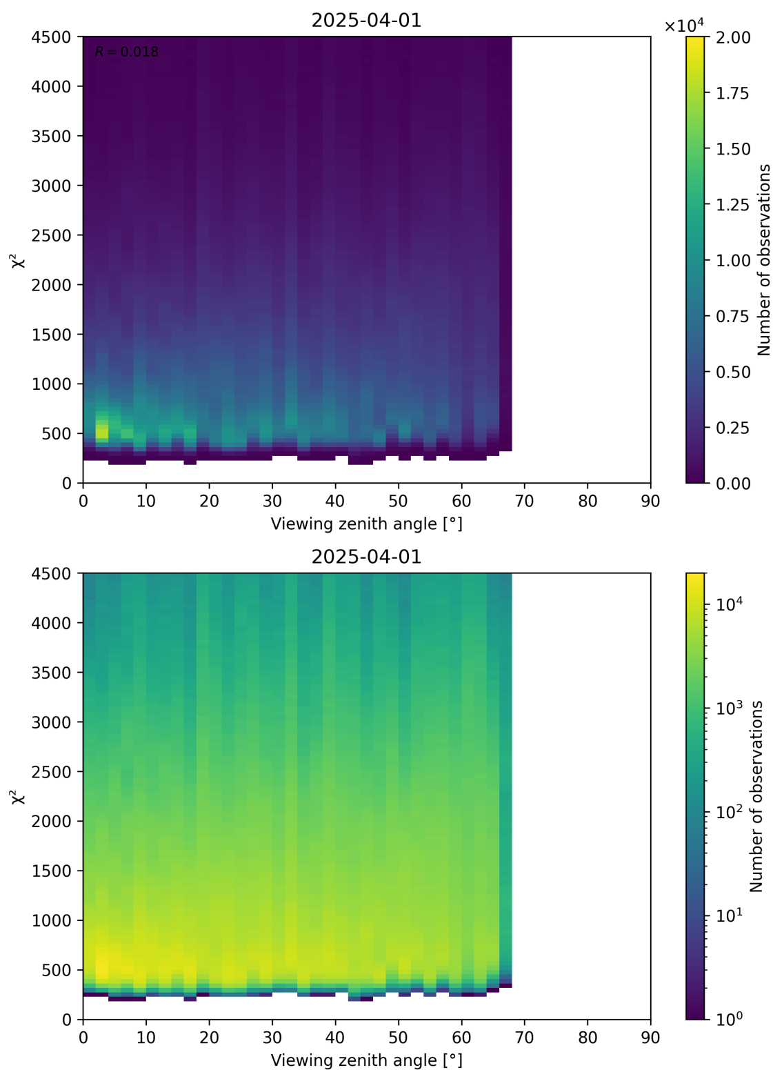
Figure 72: Scatter density plot of “Viewing zenith angle” against “ \chi^2 ” for 2025-03-31 to 2025-04-02.
