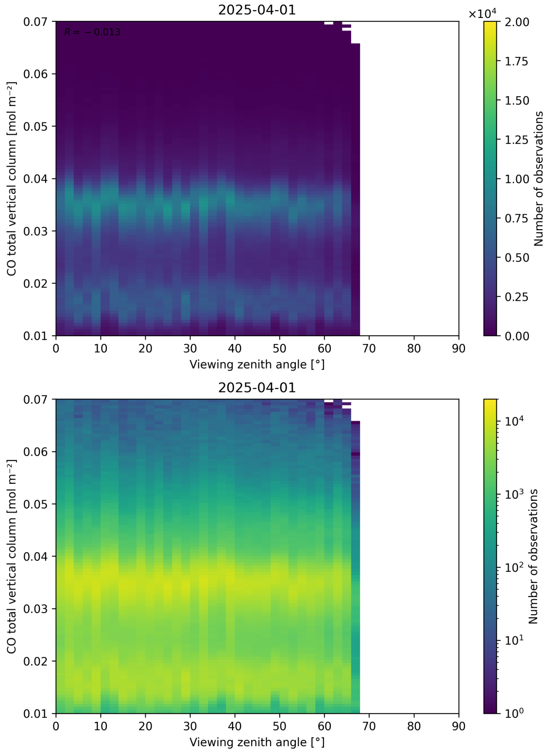
Figure 69: Scatter density plot of “Viewing zenith angle” against “CO total vertical column” for 2025-03-31 to 2025-04-02.
