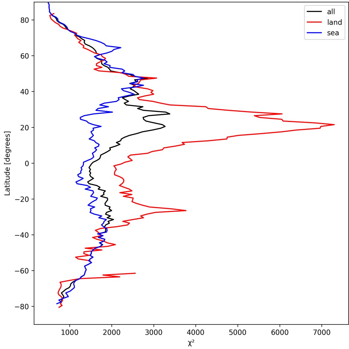
Figure 14: Zonal average of “ \chi^2 ” for 2025-03-31 to 2025-04-02.
