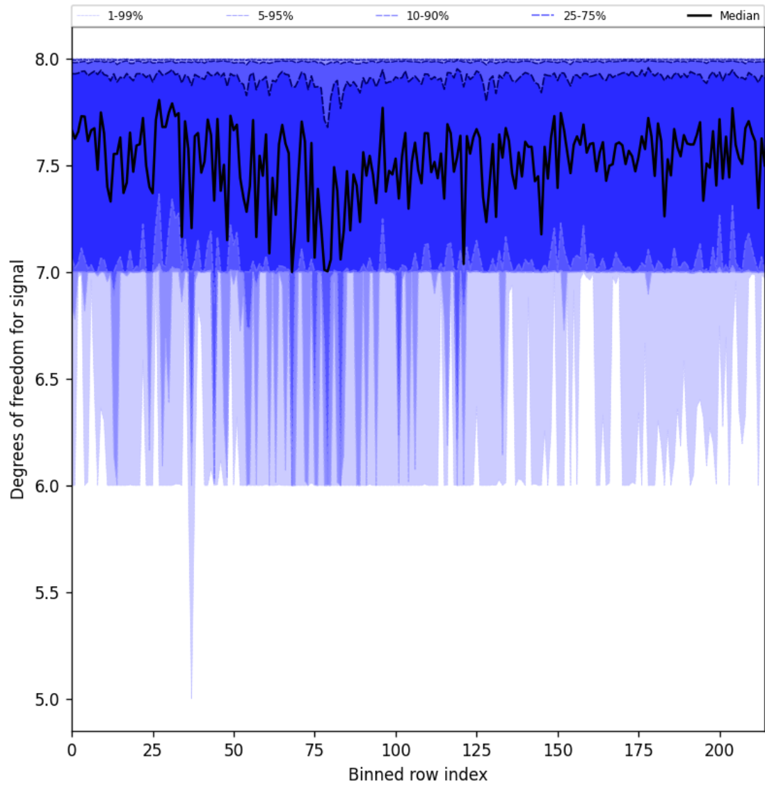
Figure 31: Along track statistics of “Degrees of freedom for signal” for 2025-03-31 to 2025-04-02
