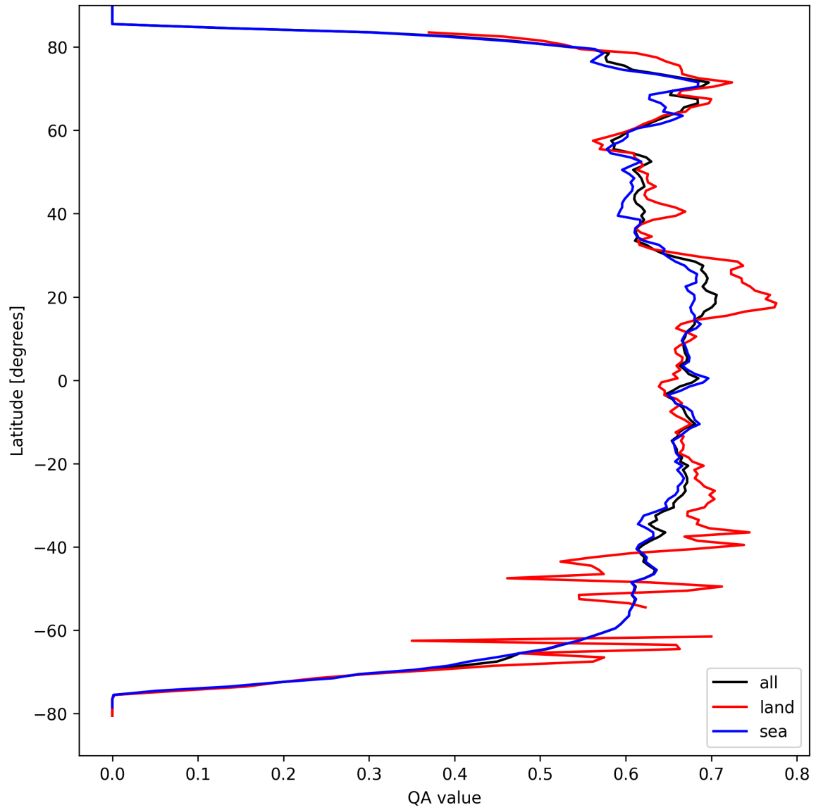
Figure 9: Zonal average of “QA value” for 2025-03-31 to 2025-04-02.
