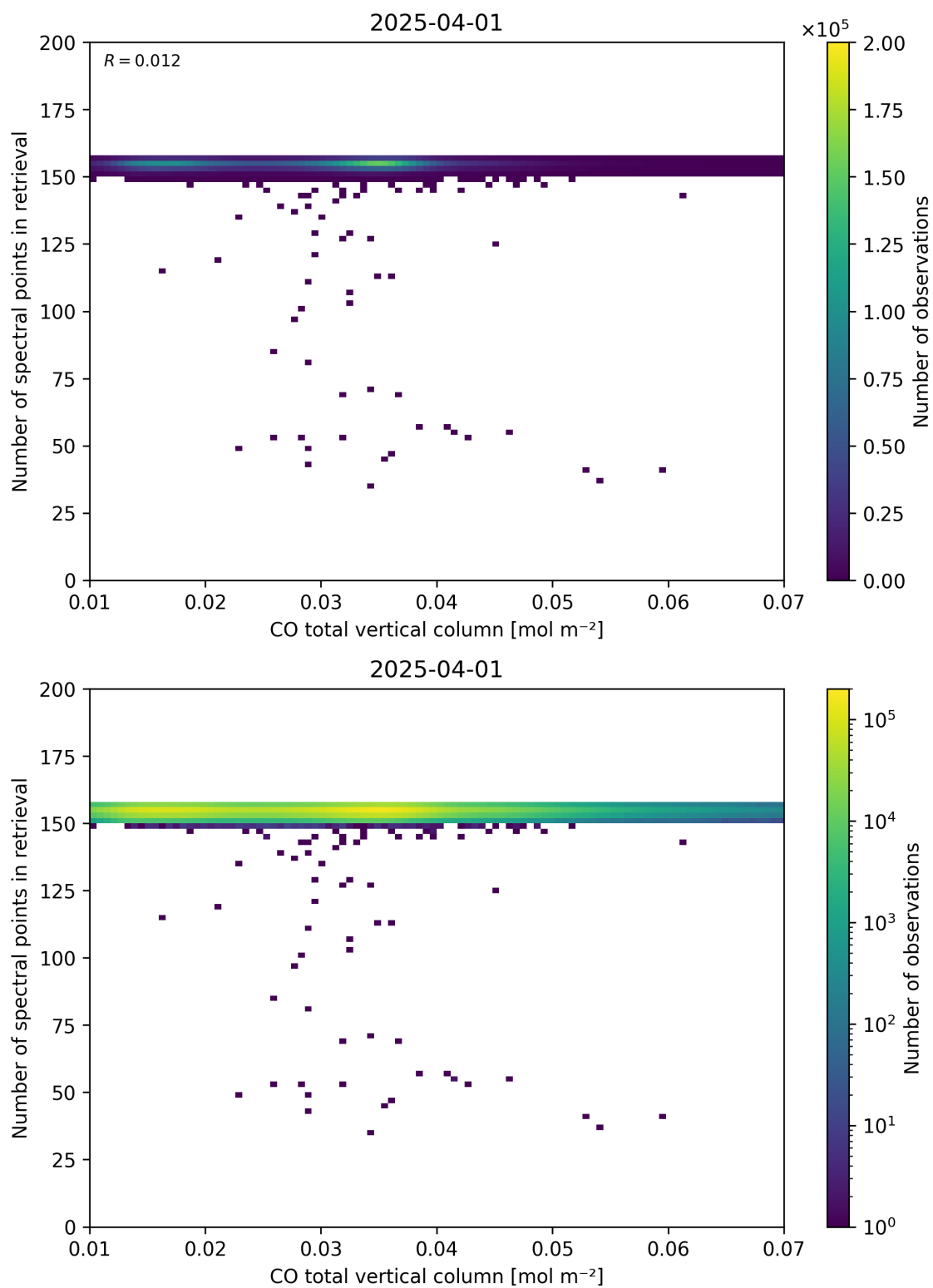
Figure 43: Scatter density plot of “CO total vertical column” against “Number of spectral points in retrieval” for 2025-03-31 to 2025-04-02.
