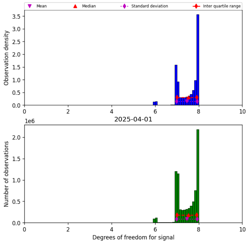
Figure 23: Histogram of “Degrees of freedom for signal” for 2025-03-31 to 2025-04-02
