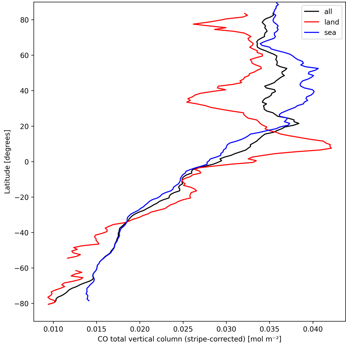
Figure 11: Zonal average of “CO total vertical column (stripe-corrected)” for 2025-03-31 to 2025-04-02.
