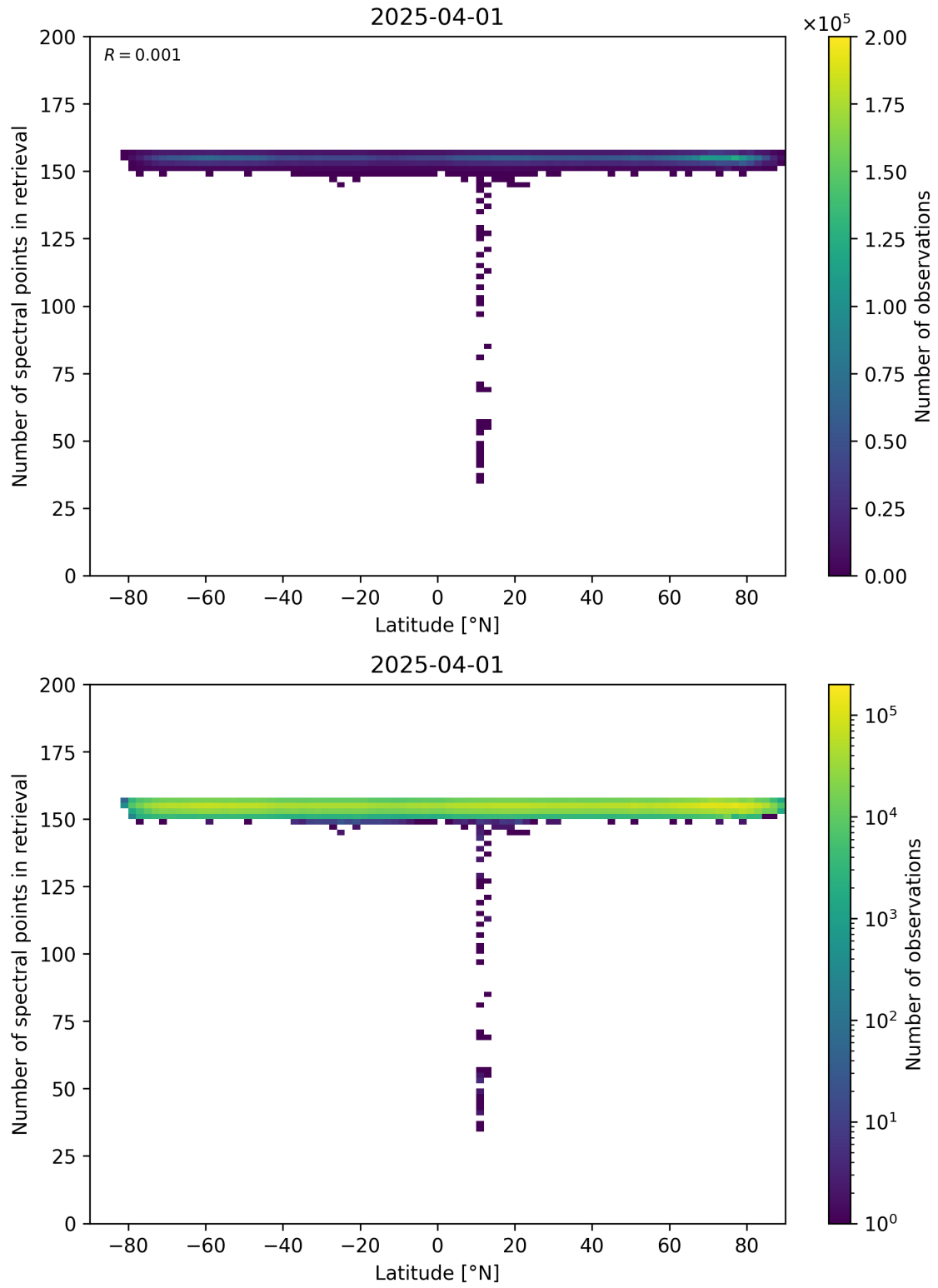
Figure 57: Scatter density plot of “Latitude” against “Number of spectral points in retrieval” for 2025-03-31 to 2025-04-02.
