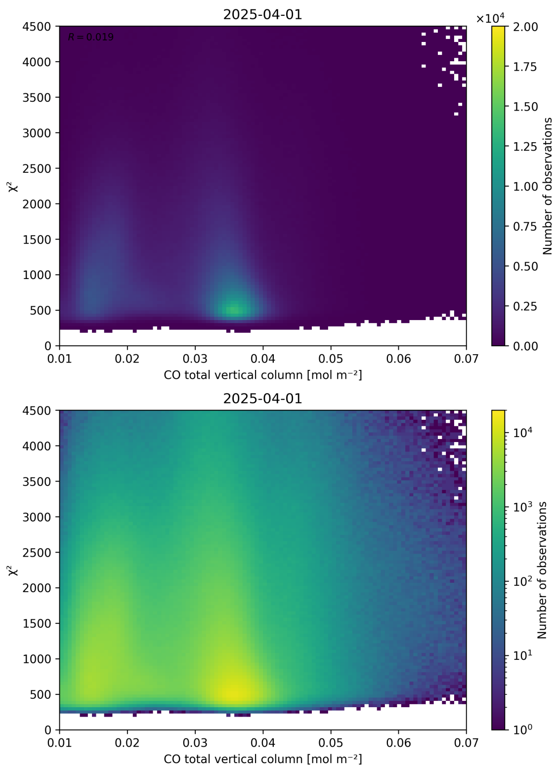
Figure 35: Scatter density plot of “CO total vertical column” against “ \chi^2 ” for 2025-03-31 to 2025-04-02.
