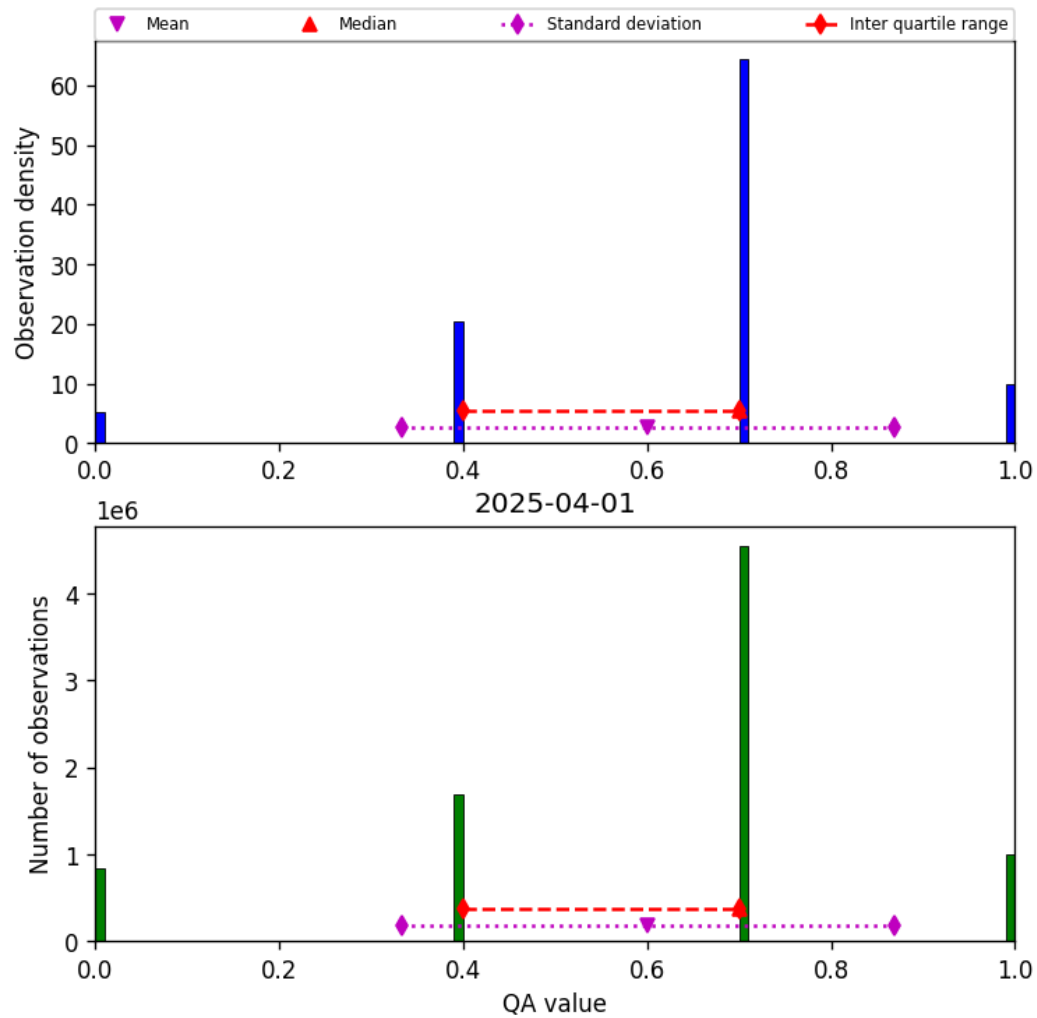
Figure 17: Histogram of “QA value” for 2025-03-31 to 2025-04-02
