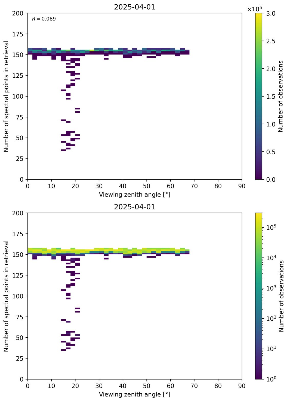
Figure 76: Scatter density plot of “Viewing zenith angle” against “Number of spectral points in retrieval” for 2025-03-31 to 2025-04-02.
