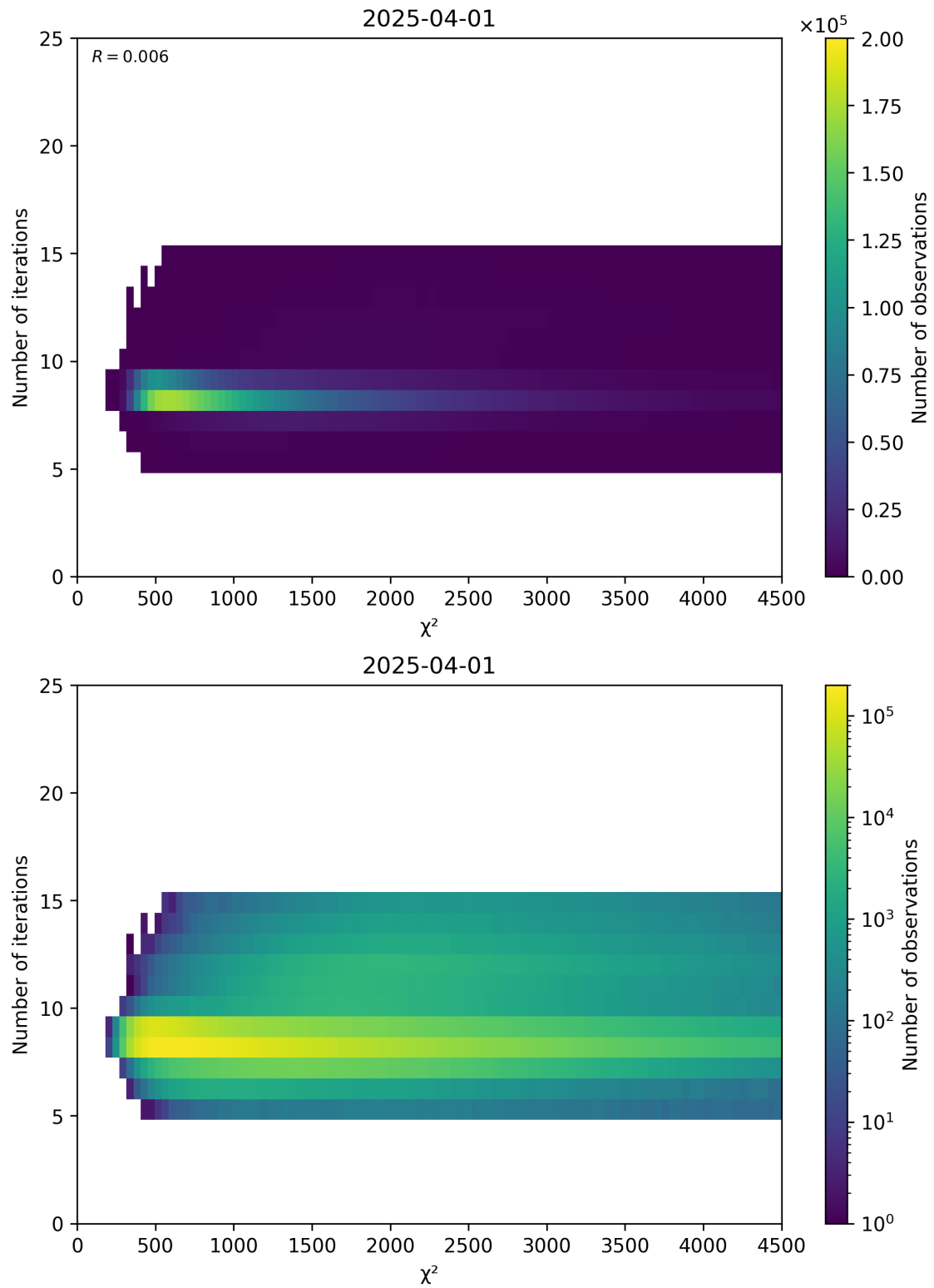
Figure 49: Scatter density plot of “ \chi^2 ” against “Number of iterations” for 2025-03-31 to 2025-04-02.
