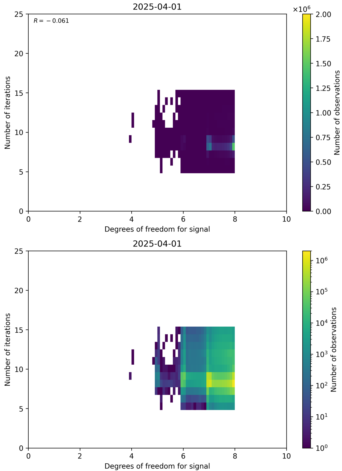
Figure 50: Scatter density plot of “Degrees of freedom for signal” against “Number of iterations” for 2025-03-31 to 2025-04-02.
