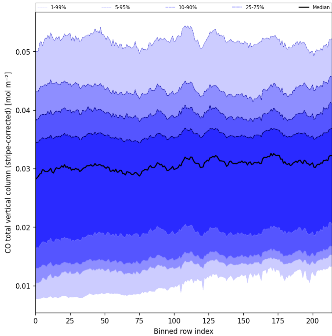
Figure 27: Along track statistics of “CO total vertical column (stripe-corrected)” for 2025-03-31 to 2025-04-02
