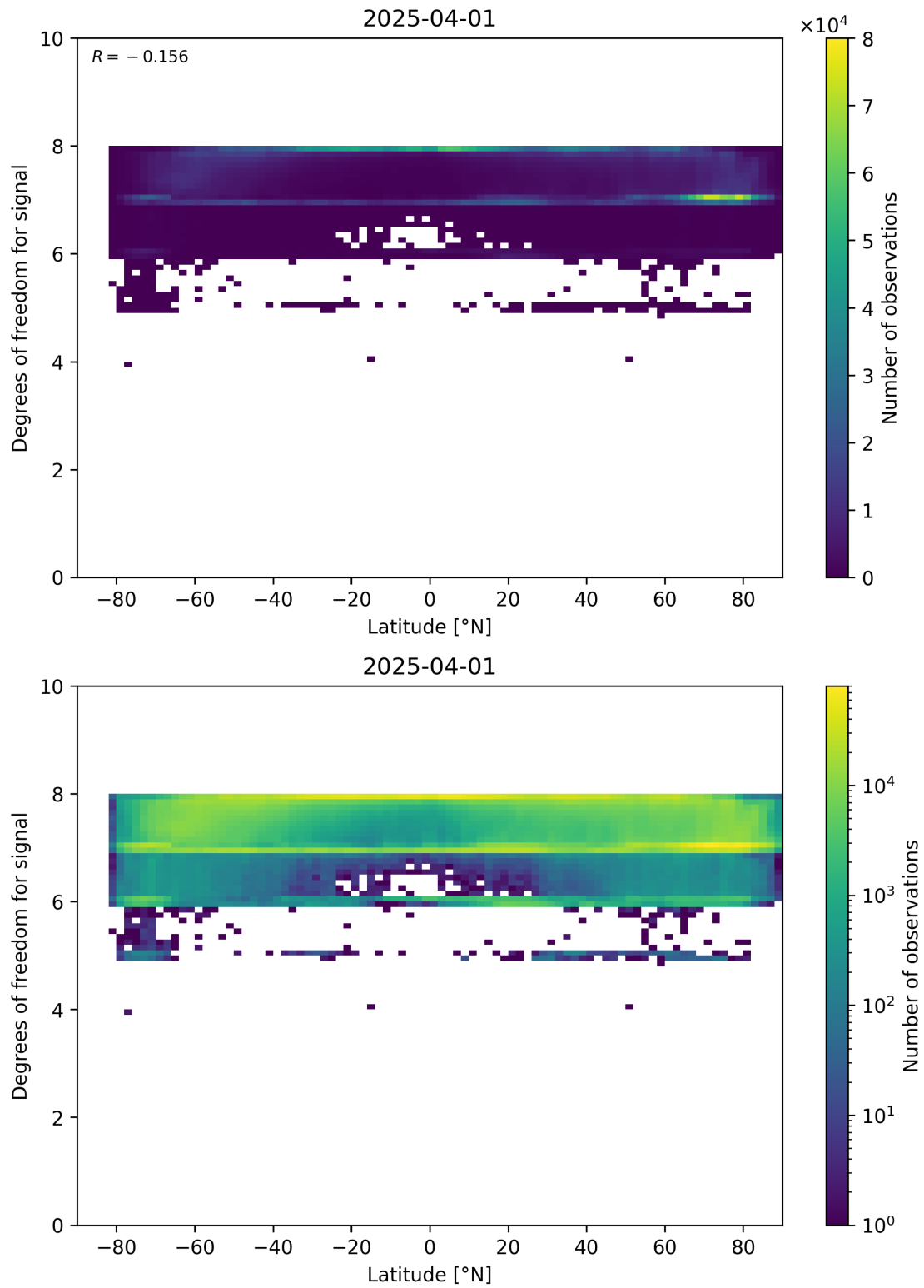
Figure 55: Scatter density plot of “Latitude” against “Degrees of freedom for signal” for 2025-03-31 to 2025-04-02.
