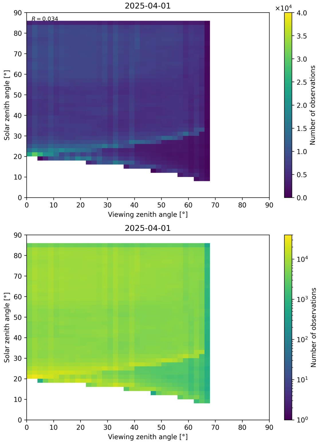
Figure 77: Scatter density plot of “Viewing zenith angle” against “Solar zenith angle” for 2025-03-31 to 2025-04-02.
