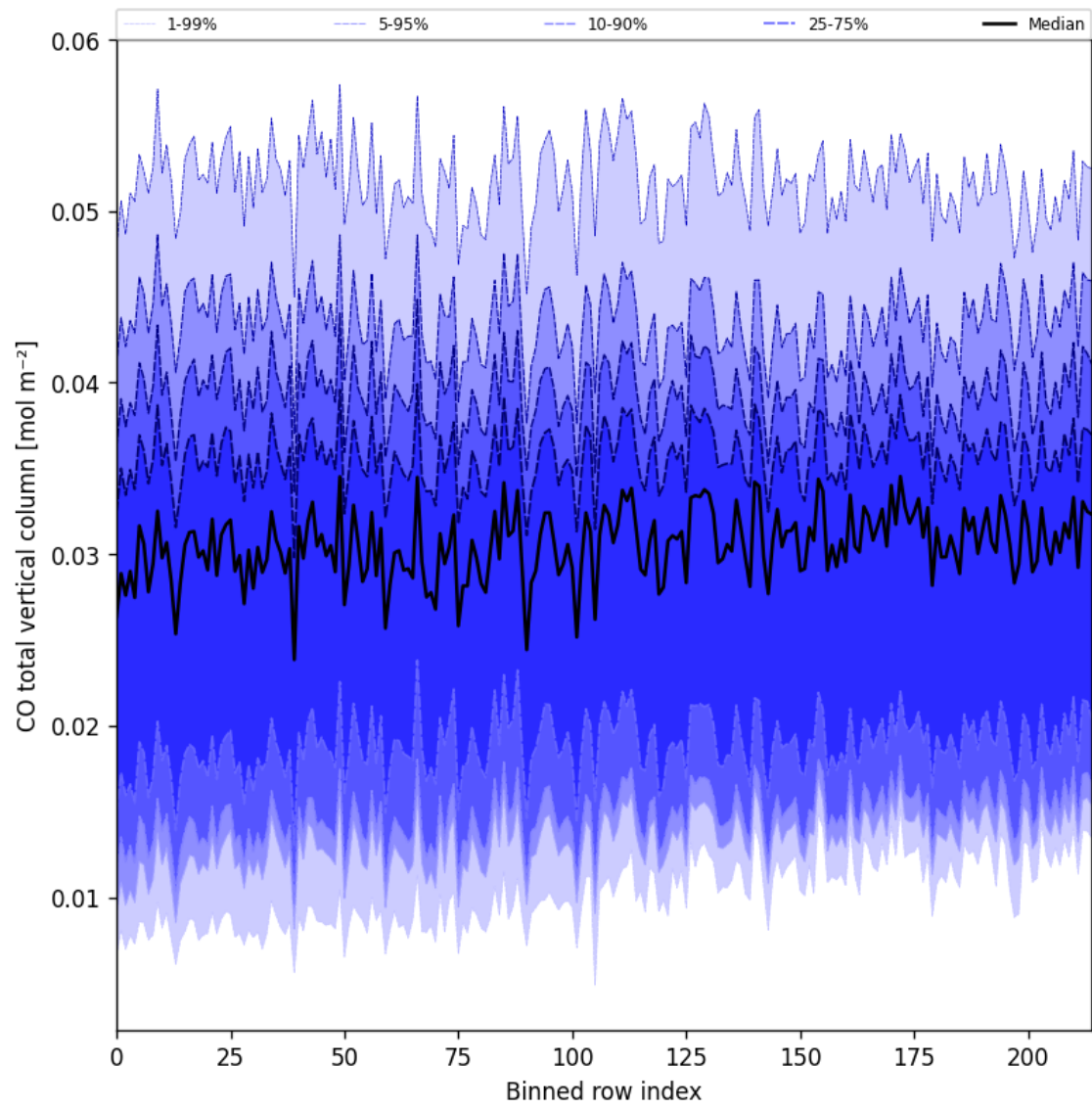
Figure 26: Along track statistics of "CO total vertical column" for 2025-03-31 to 2025-04-02
