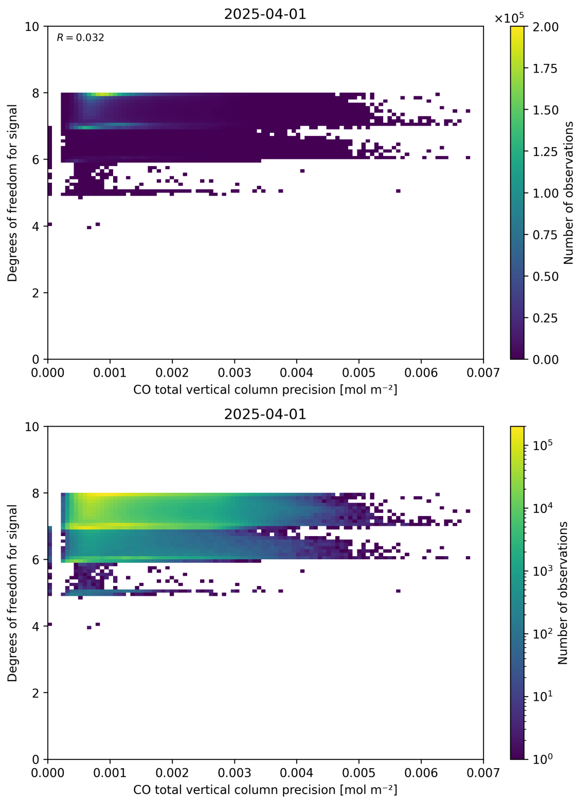
Figure 45: Scatter density plot of “CO total vertical column precision” against “Degrees of freedom for signal” for 2025-03-31 to 2025-04-02.
