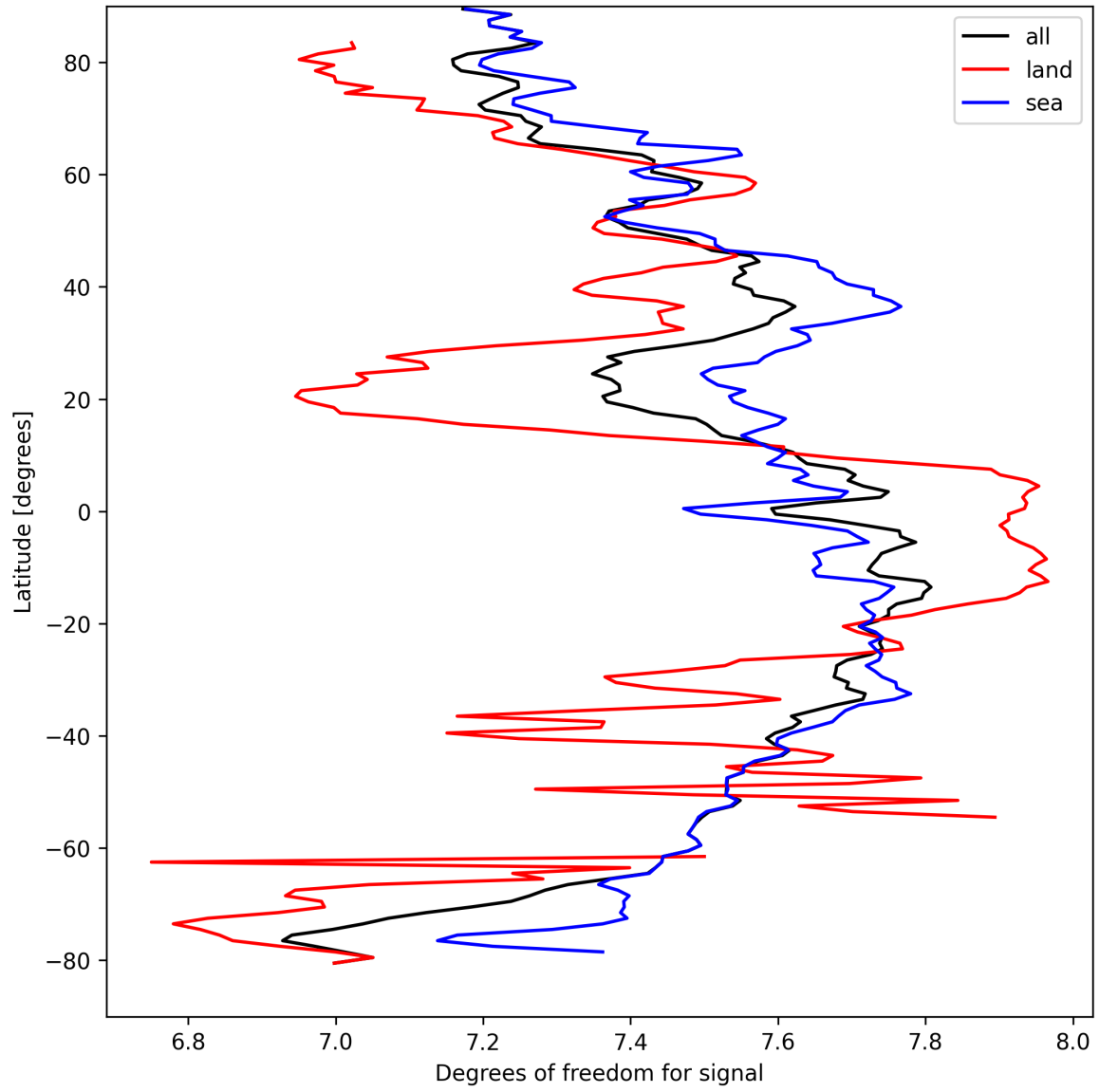
Figure 15: Zonal average of “Degrees of freedom for signal” for 2025-03-31 to 2025-04-02.
