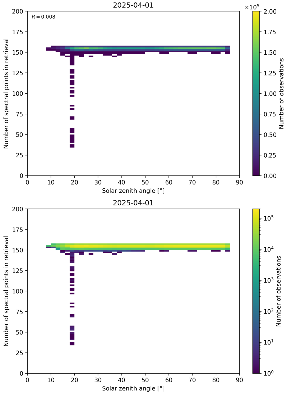
Figure 68: Scatter density plot of “Solar zenith angle” against “Number of spectral points in retrieval” for 2025-03-31 to 2025-04-02.
