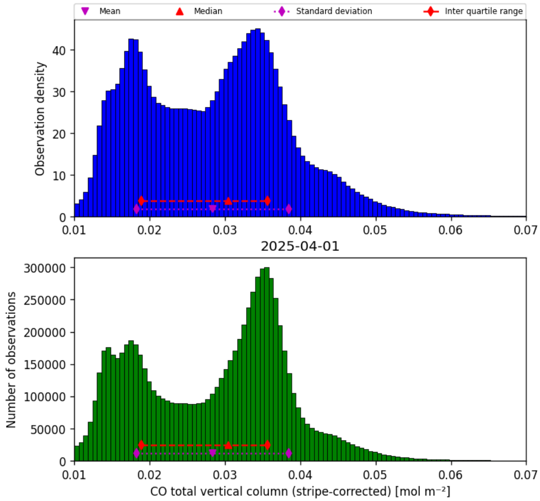
Figure 19: Histogram of “CO total vertical column (stripe-corrected)” for 2025-03-31 to 2025-04-02
