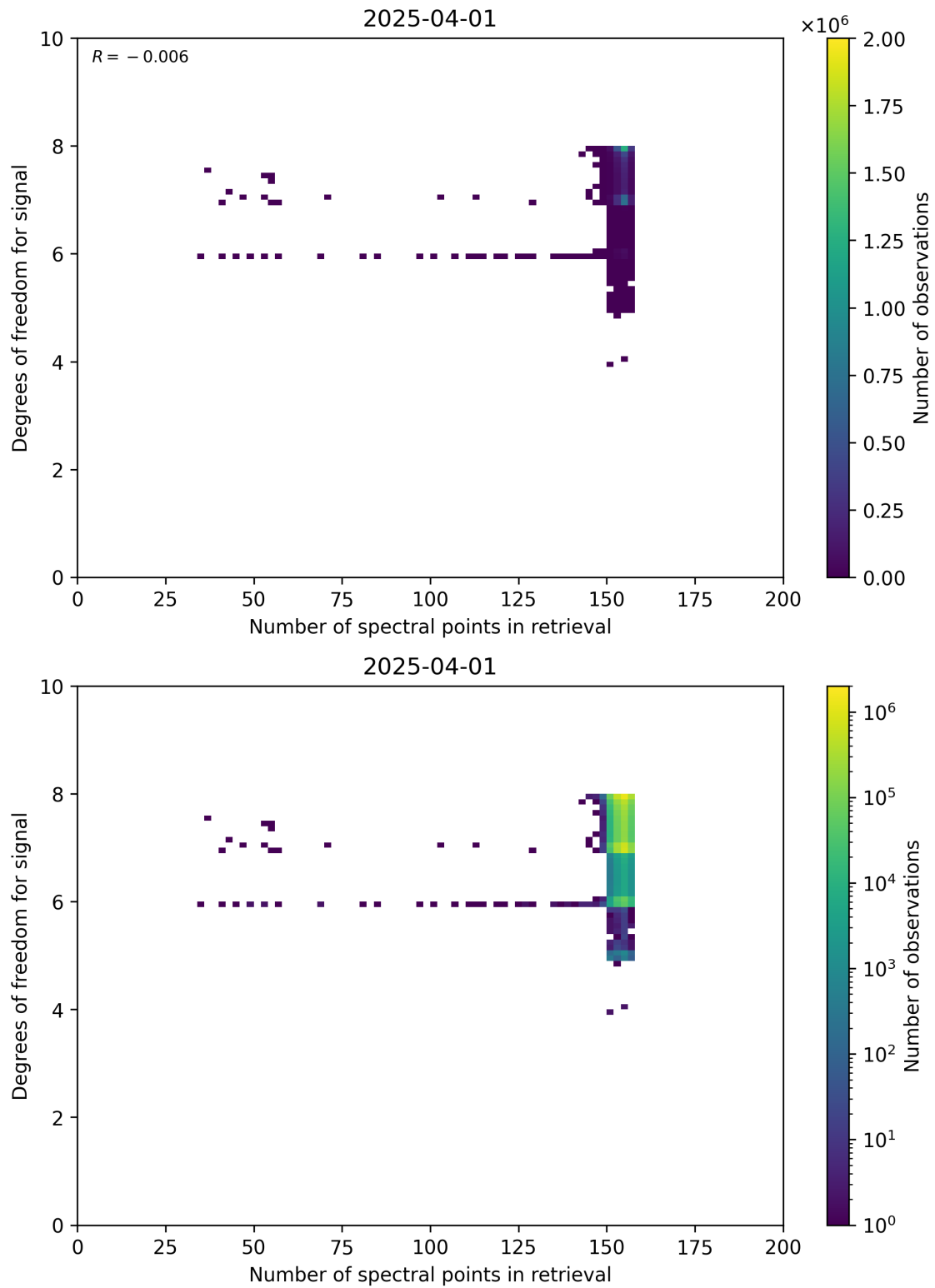
Figure 59: Scatter density plot of “Number of spectral points in retrieval” against “Degrees of freedom for signal” for 2025-03-31 to 2025-04-02.
