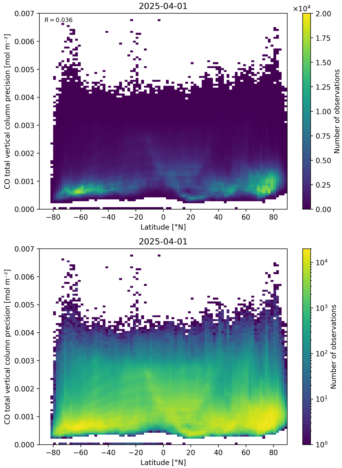
Figure 53: Scatter density plot of “Latitude” against “CO total vertical column precision” for 2025-03-31 to 2025-04-02.
