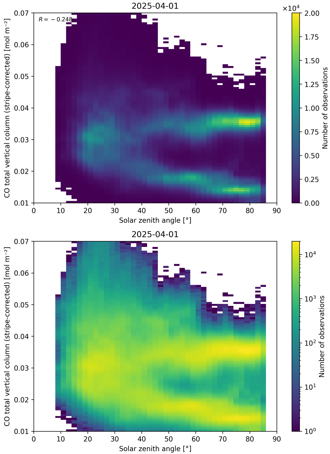
Figure 62: Scatter density plot of “Solar zenith angle” against “CO total vertical column (stripe-corrected)” for 2025-03-31 to 2025-04-02.
