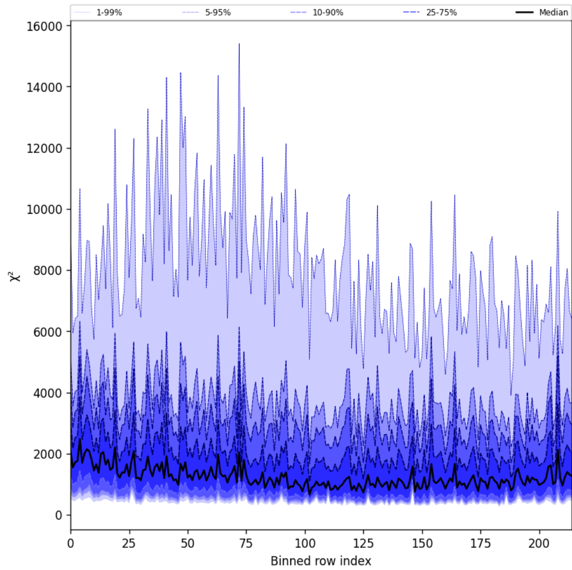
Figure 30: Along track statistics of “ \chi^2 ” for 2025-03-31 to 2025-04-02
