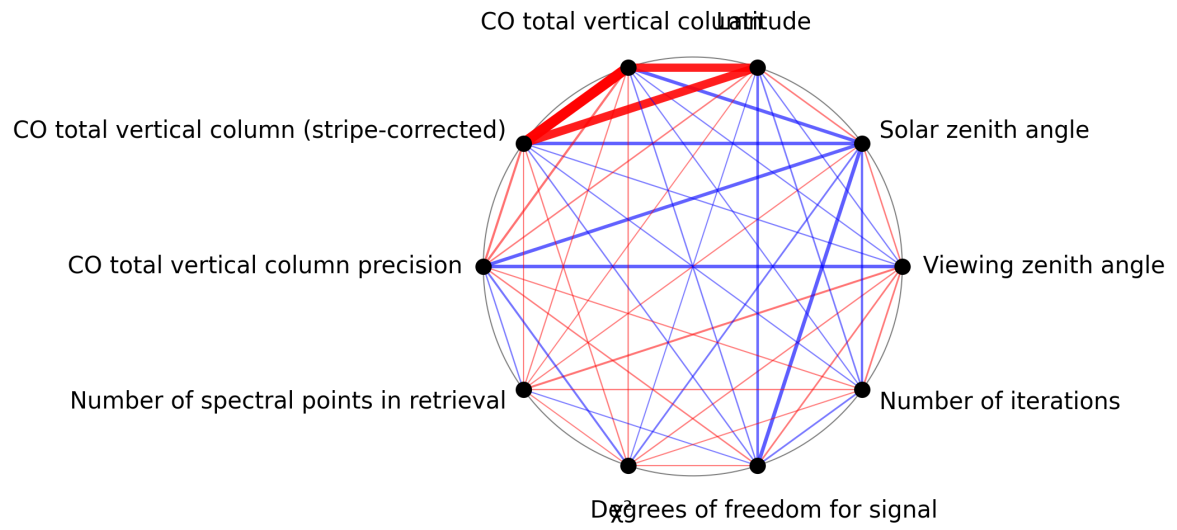
Figure 1: Map of correlation graph for 2025-03-31 to 2025-04-02.
