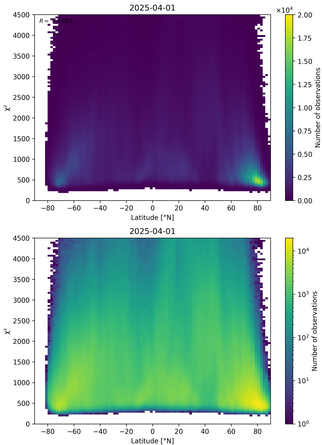
Figure 54: Scatter density plot of “Latitude” against “ \chi^2 ” for 2025-03-31 to 2025-04-02.
