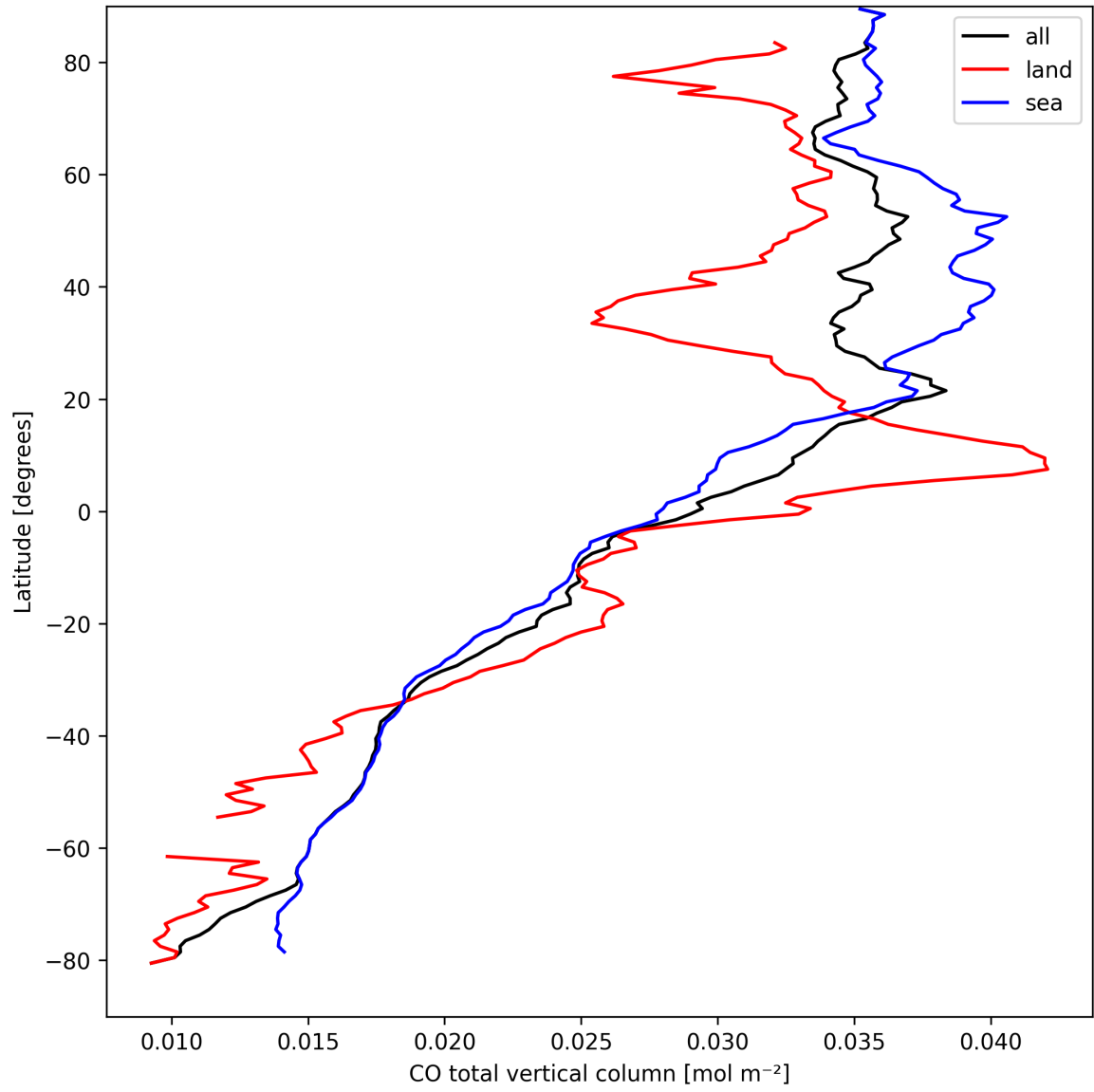
Figure 10: Zonal average of “CO total vertical column” for 2025-03-31 to 2025-04-02.
