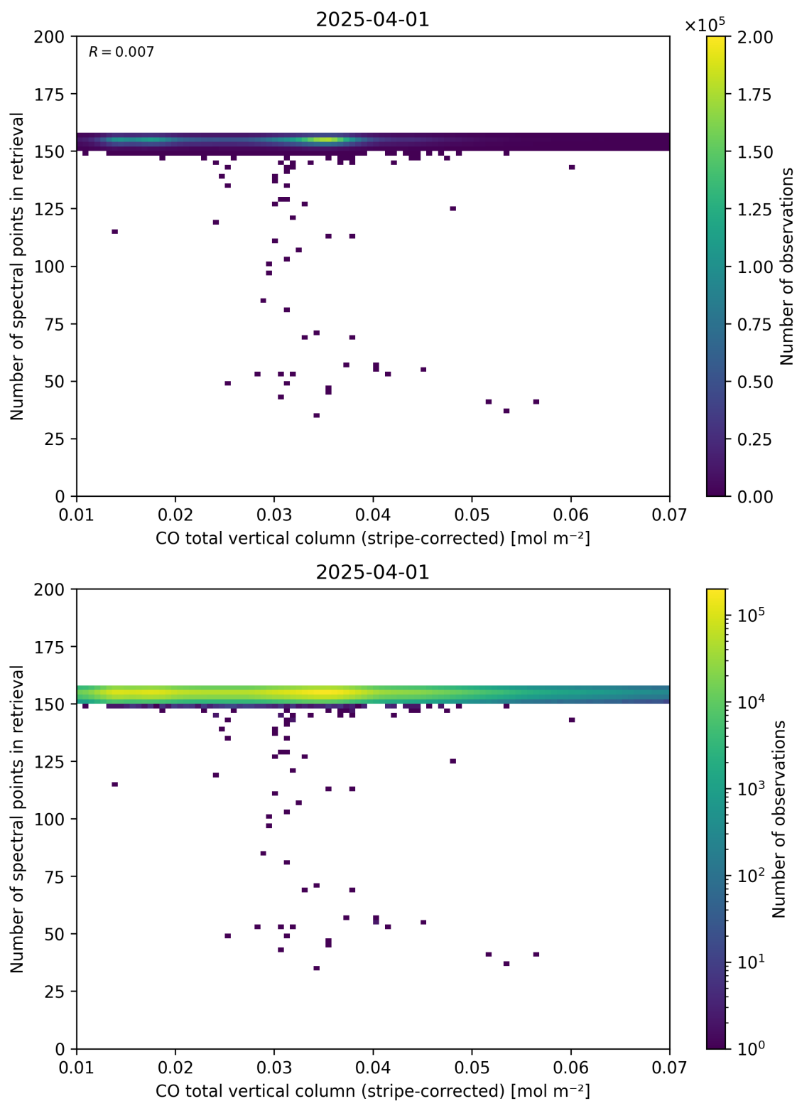
Figure 40: Scatter density plot of “CO total vertical column (stripe-corrected)” against “Number of spectral points in retrieval” for 2025-03-31 to 2025-04-02.
