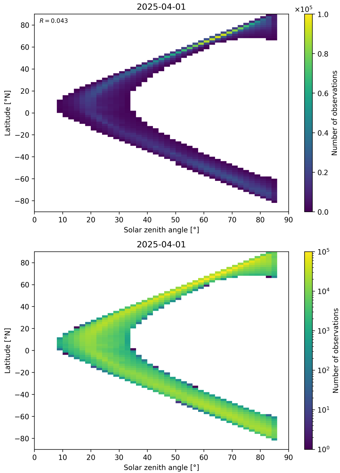
Figure 66: Scatter density plot of “Solar zenith angle” against “Latitude” for 2025-03-31 to 2025-04-02.
