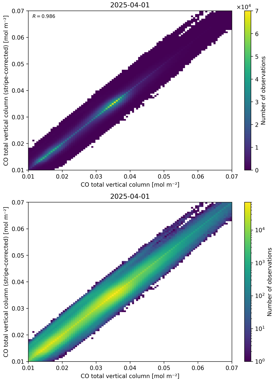
Figure 33: Scatter density plot of “CO total vertical column” against “CO total vertical column (stripe-corrected)” for 2025-03-31 to 2025-04-02.
