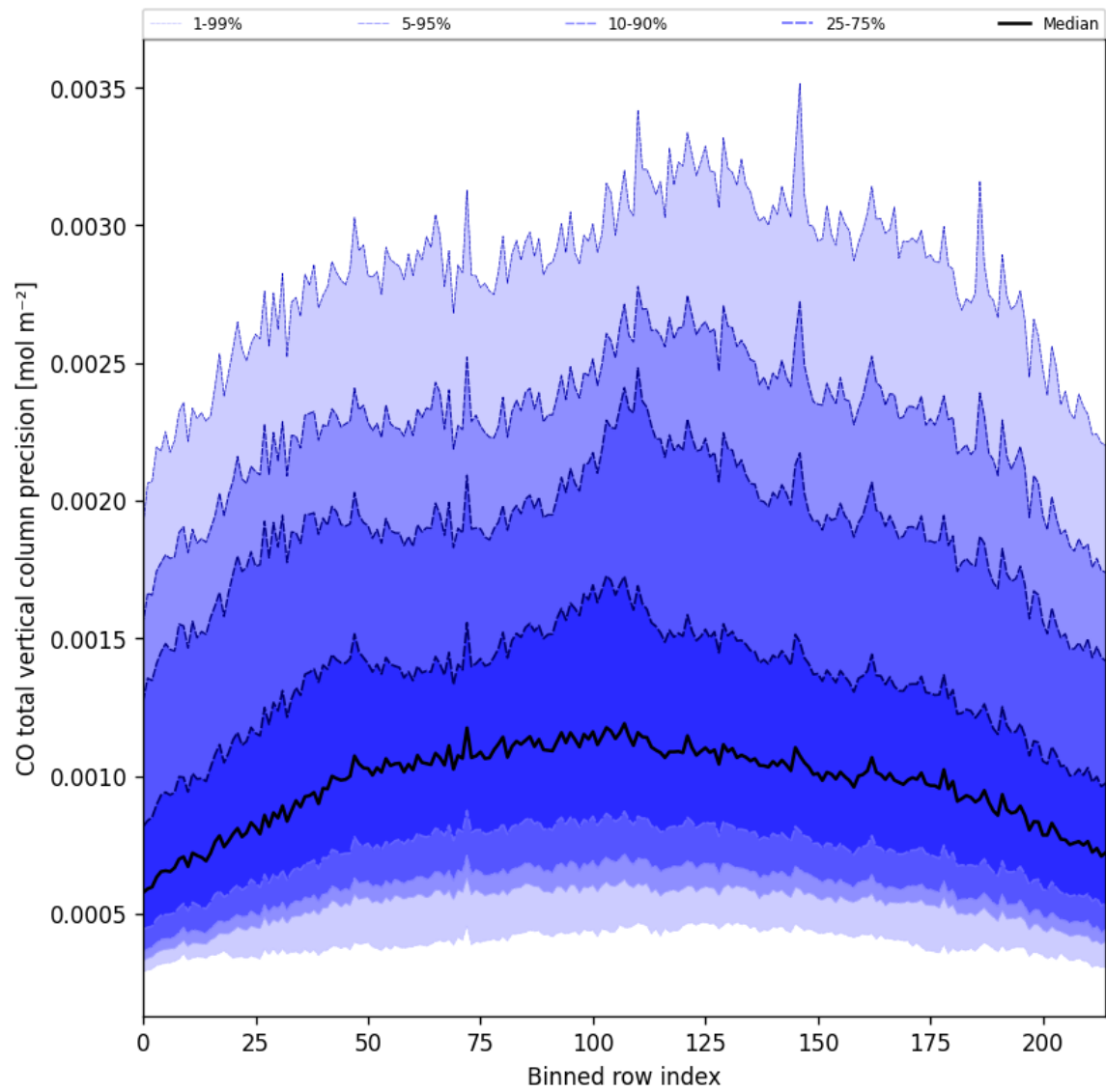
Figure 28: Along track statistics of “CO total vertical column precision” for 2025-03-31 to 2025-04-02
