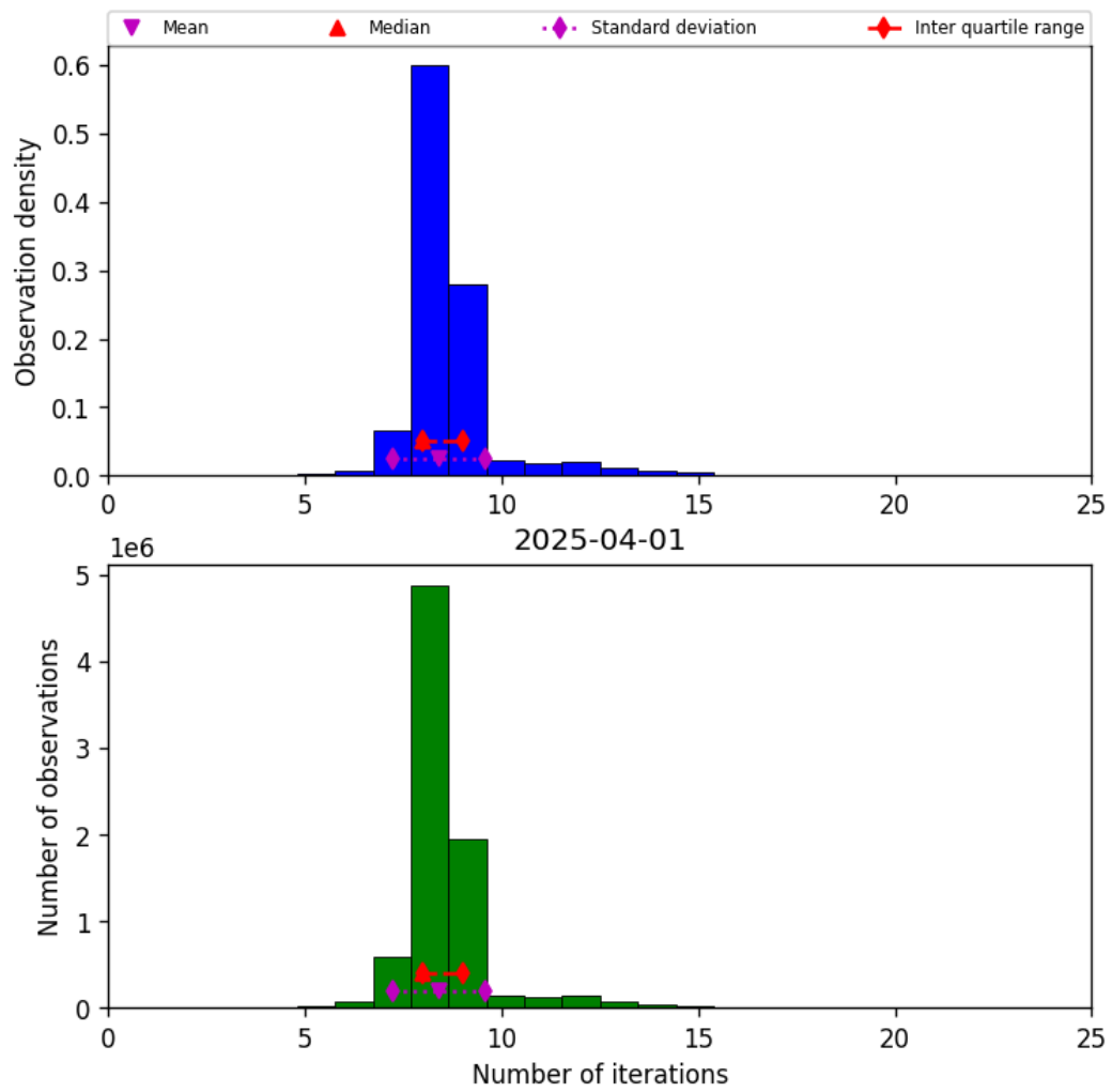
Figure 24: Histogram of “Number of iterations” for 2025-03-31 to 2025-04-02
