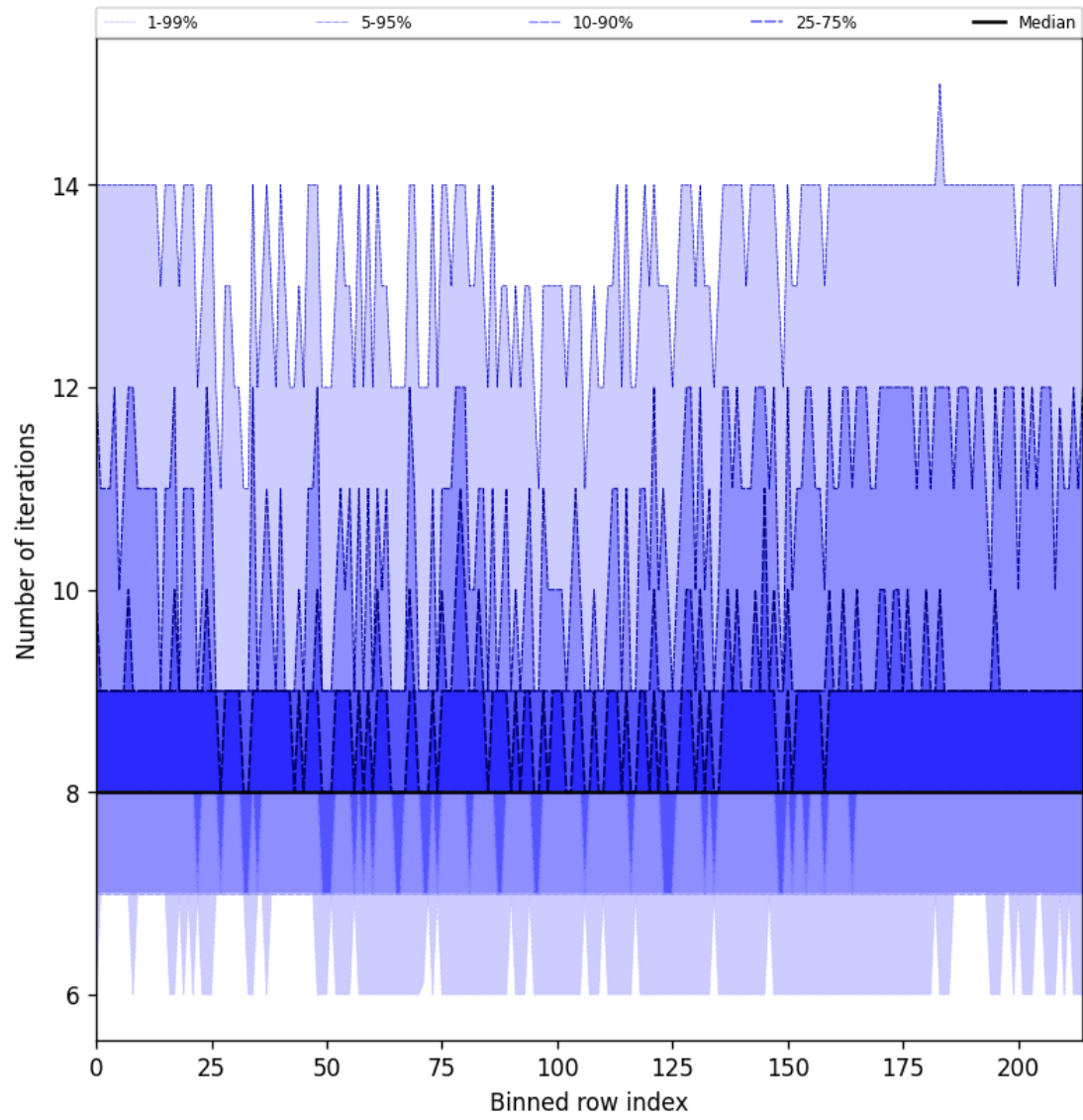
Figure 32: Along track statistics of “Number of iterations” for 2025-03-31 to 2025-04-02
