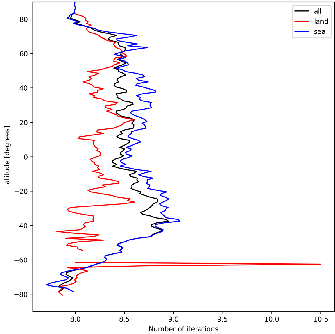
Figure 16: Zonal average of “Number of iterations” for 2025-03-31 to 2025-04-02.
