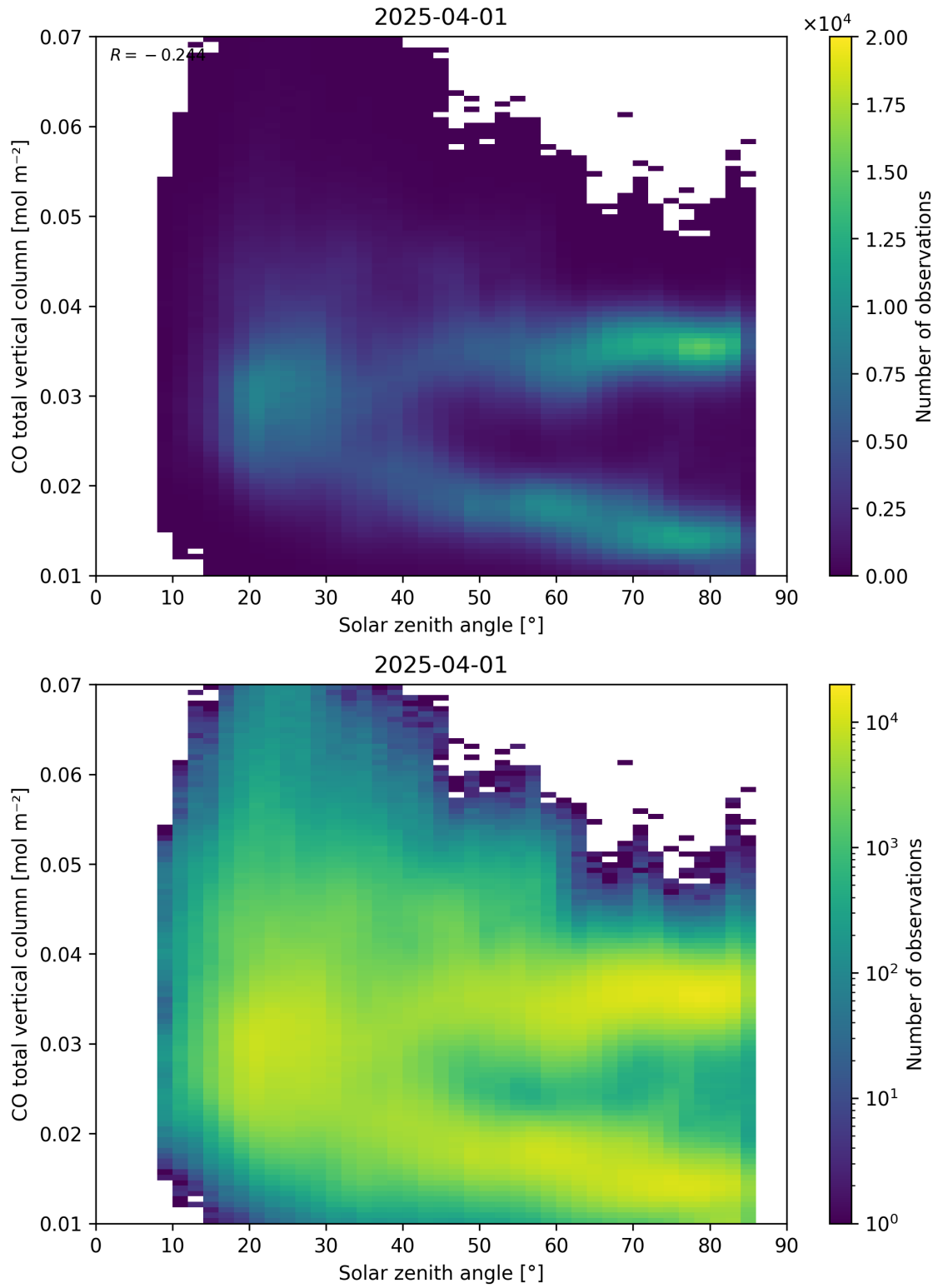
Figure 61: Scatter density plot of “Solar zenith angle” against “CO total vertical column” for 2025-03-31 to 2025-04-02.
