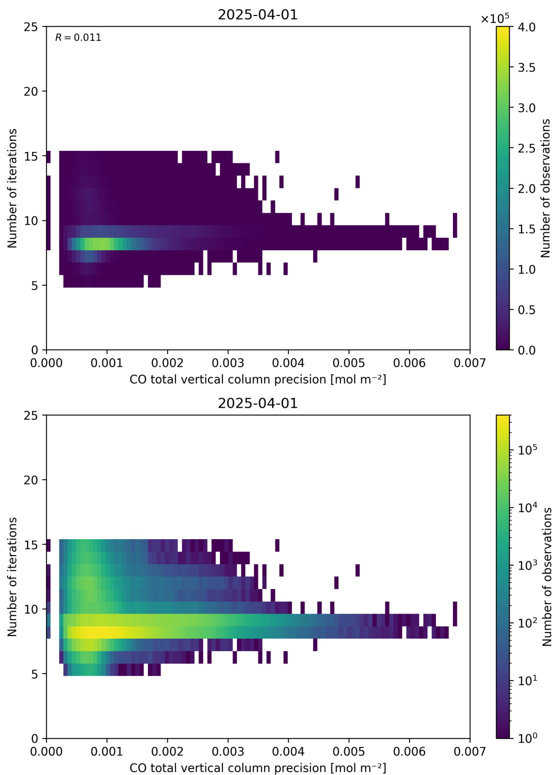
Figure 46: Scatter density plot of “CO total vertical column precision” against “Number of iterations” for 2025-03-31 to 2025-04-02.
