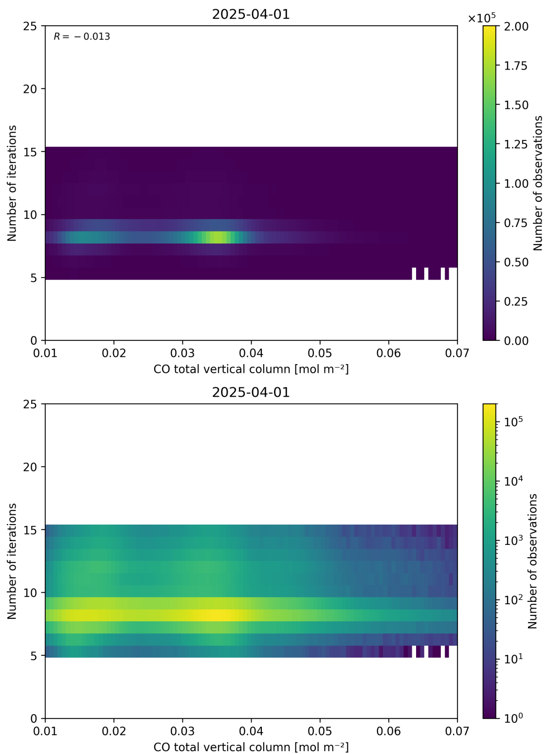
Figure 42: Scatter density plot of “CO total vertical column” against “Number of iterations” for 2025-03-31 to 2025-04-02.
