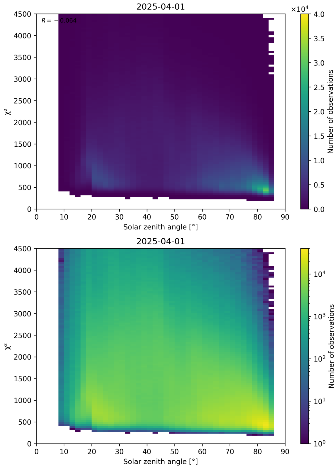
Figure 64: Scatter density plot of “Solar zenith angle” against “ \chi^2 ” for 2025-03-31 to 2025-04-02.
