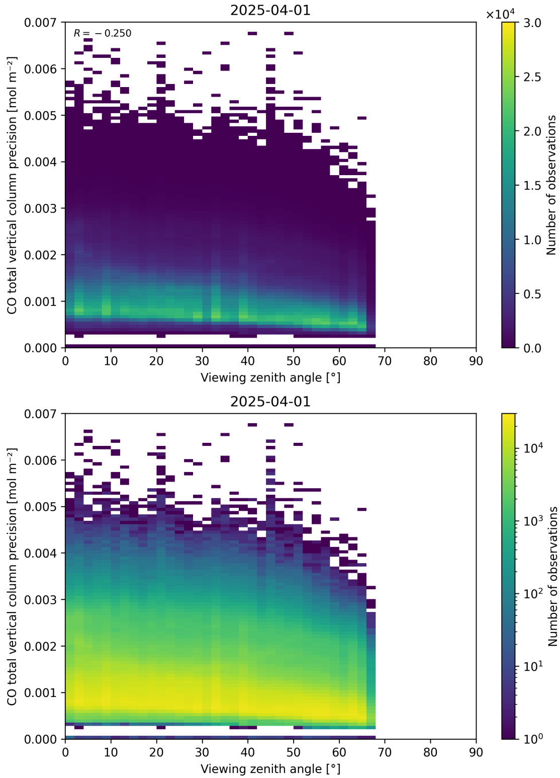
Figure 71: Scatter density plot of “Viewing zenith angle” against “CO total vertical column precision” for 2025-03-31 to 2025-04-02.
