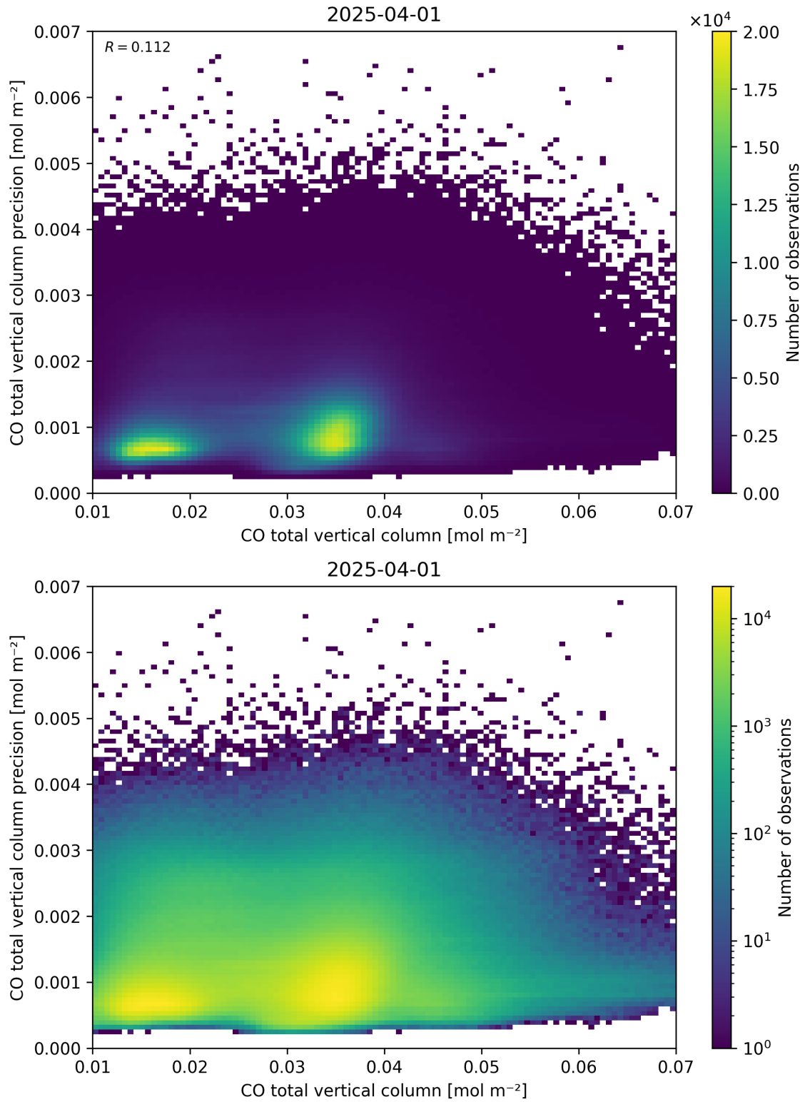
Figure 34: Scatter density plot of “CO total vertical column” against “CO total vertical column precision” for 2025-03-31 to 2025-04-02.
