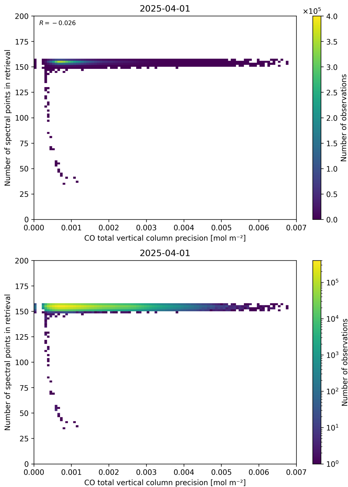
Figure 47: Scatter density plot of “CO total vertical column precision” against “Number of spectral points in retrieval” for 2025-03-31 to 2025-04-02.
