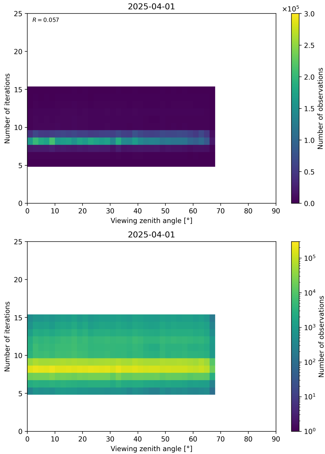
Figure 75: Scatter density plot of “Viewing zenith angle” against “Number of iterations” for 2025-03-31 to 2025-04-02.
