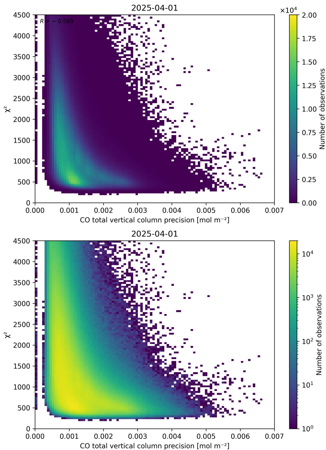
Figure 44: Scatter density plot of “CO total vertical column precision” against “ \chi^2 ” for 2025-03-31 to 2025-04-02.
