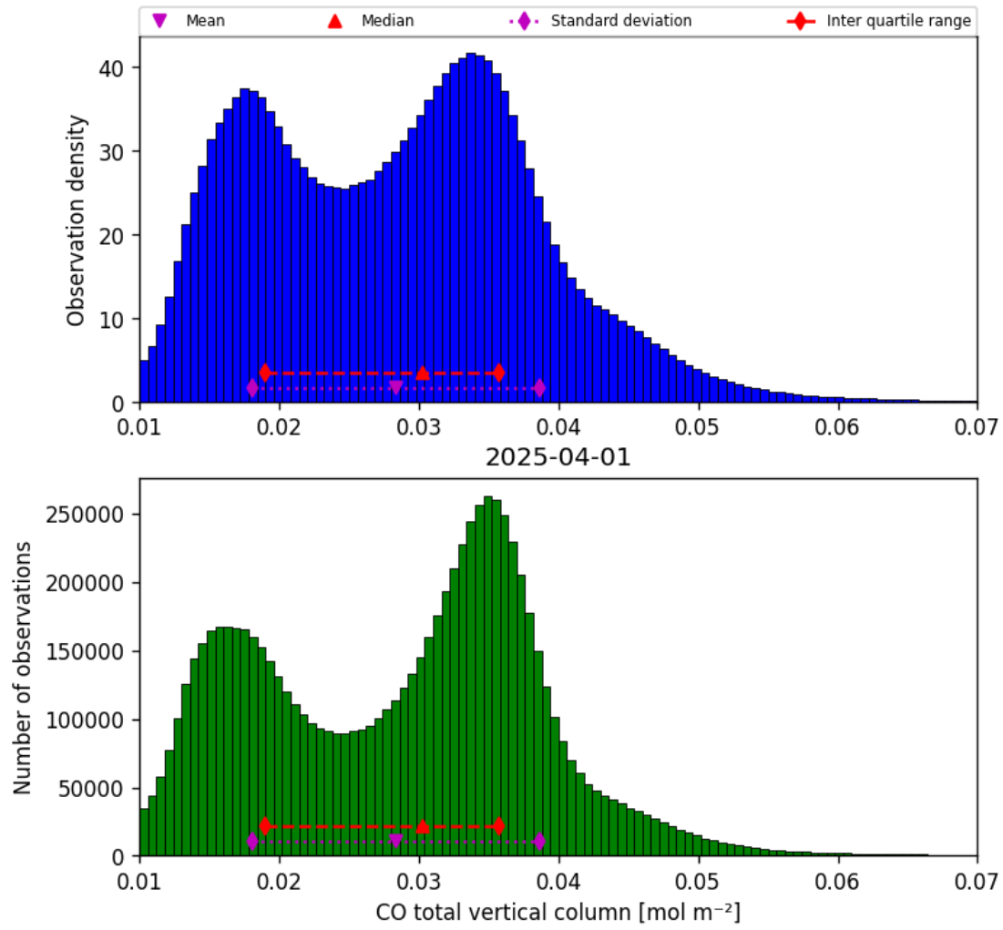
Figure 18: Histogram of “CO total vertical column” for 2025-03-31 to 2025-04-02
