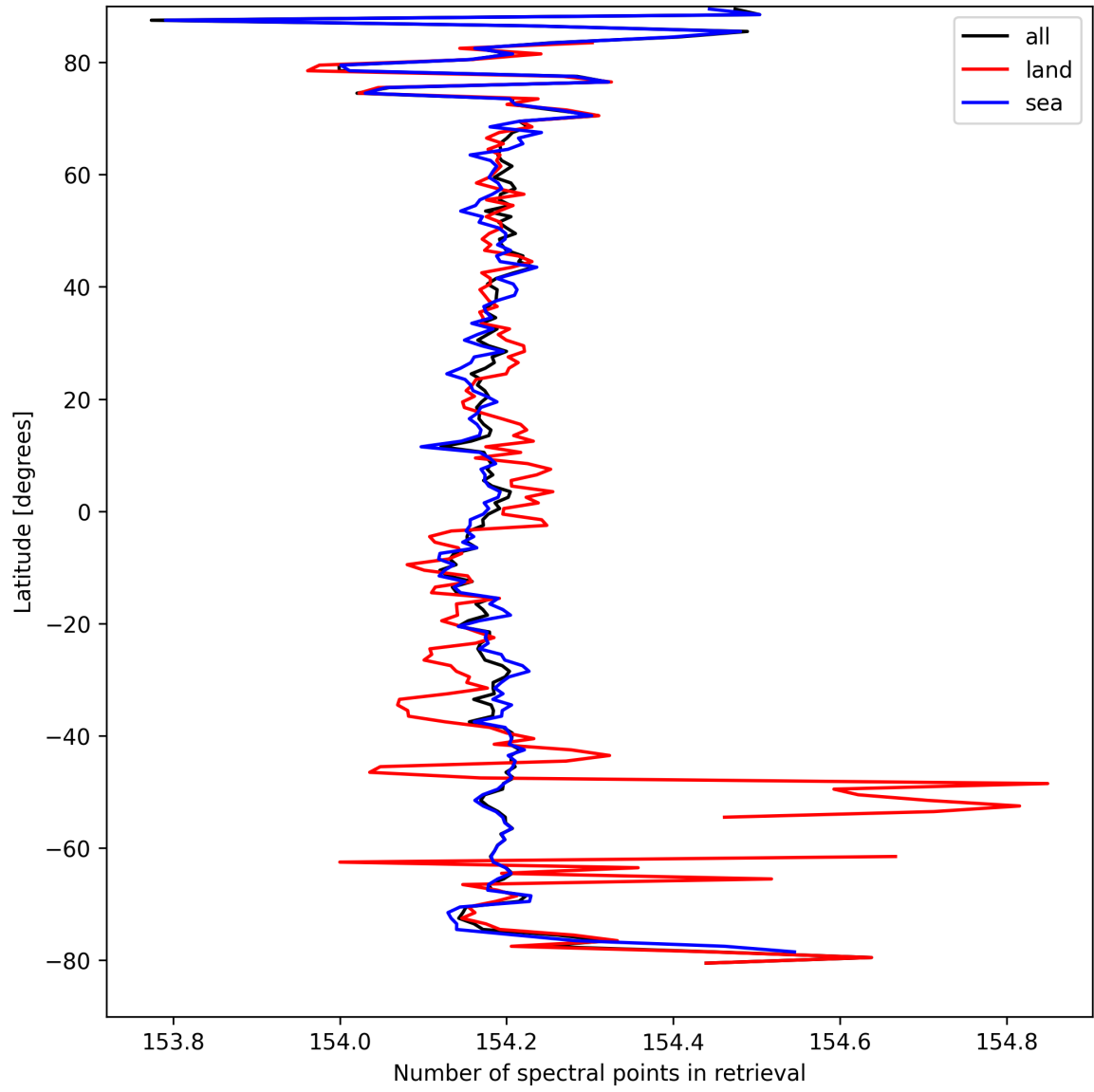
Figure 13: Zonal average of “Number of spectral points in retrieval” for 2025-03-31 to 2025-04-02.
