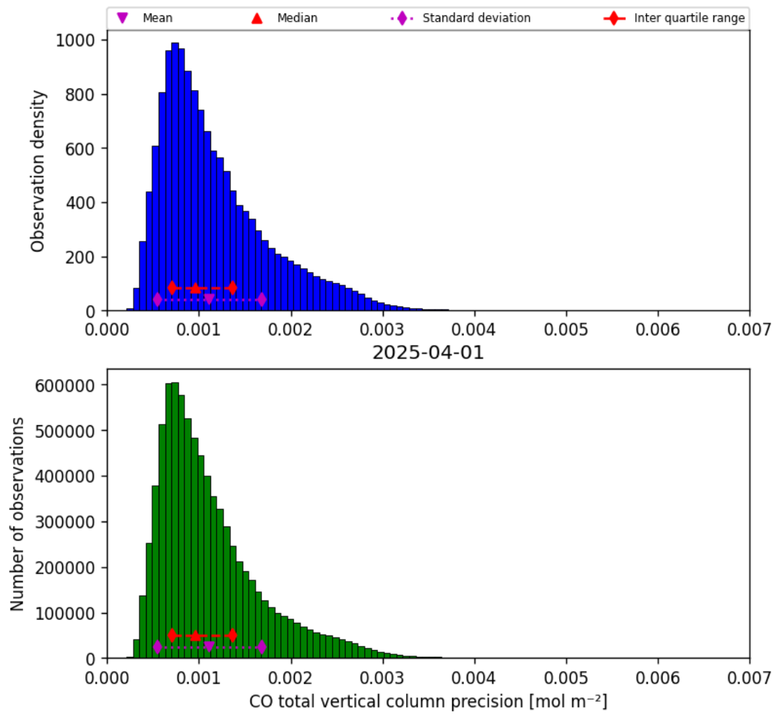
Figure 20: Histogram of “CO total vertical column precision” for 2025-03-31 to 2025-04-02
