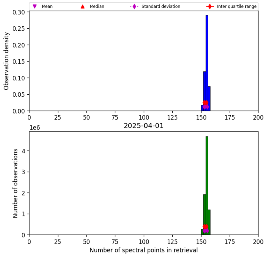
Figure 21: Histogram of “Number of spectral points in retrieval” for 2025-03-31 to 2025-04-02
