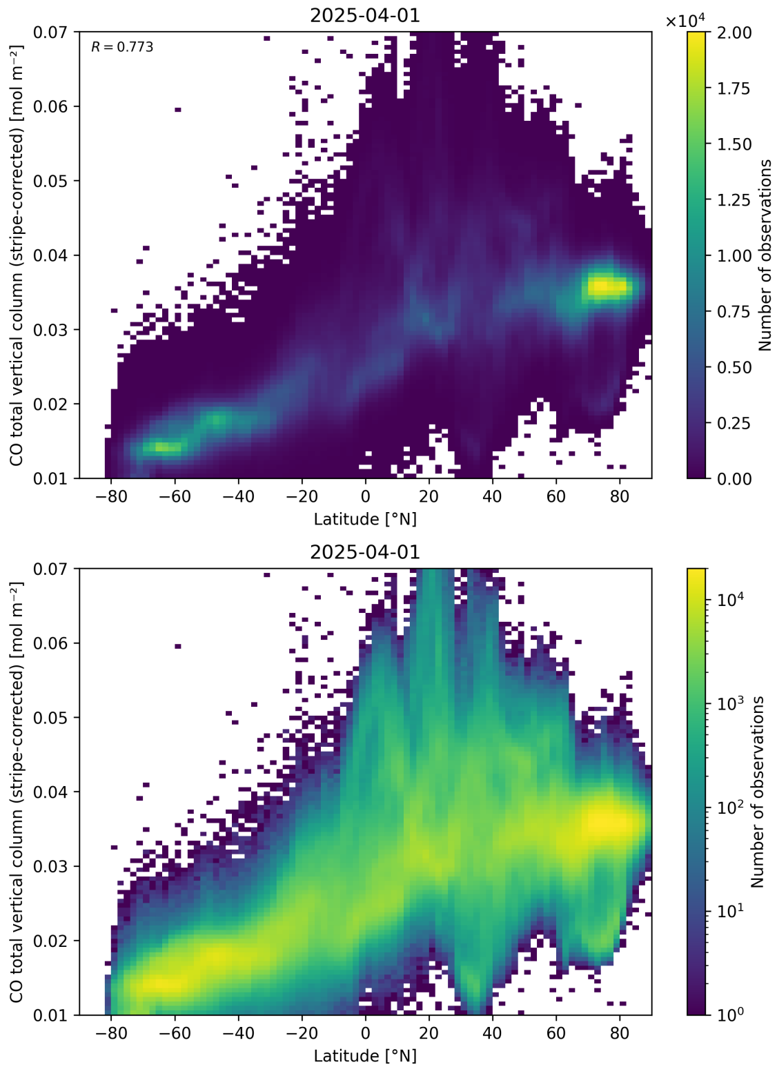
Figure 52: Scatter density plot of “Latitude” against “CO total vertical column (stripe-corrected)” for 2025-03-31 to 2025-04-02.
