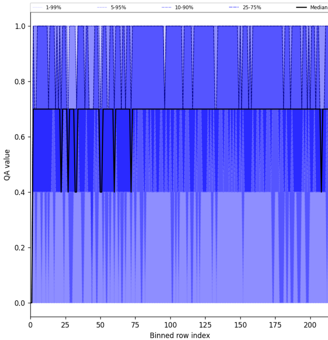
Figure 25: Along track statistics of “QA value” for 2025-03-31 to 2025-04-02
