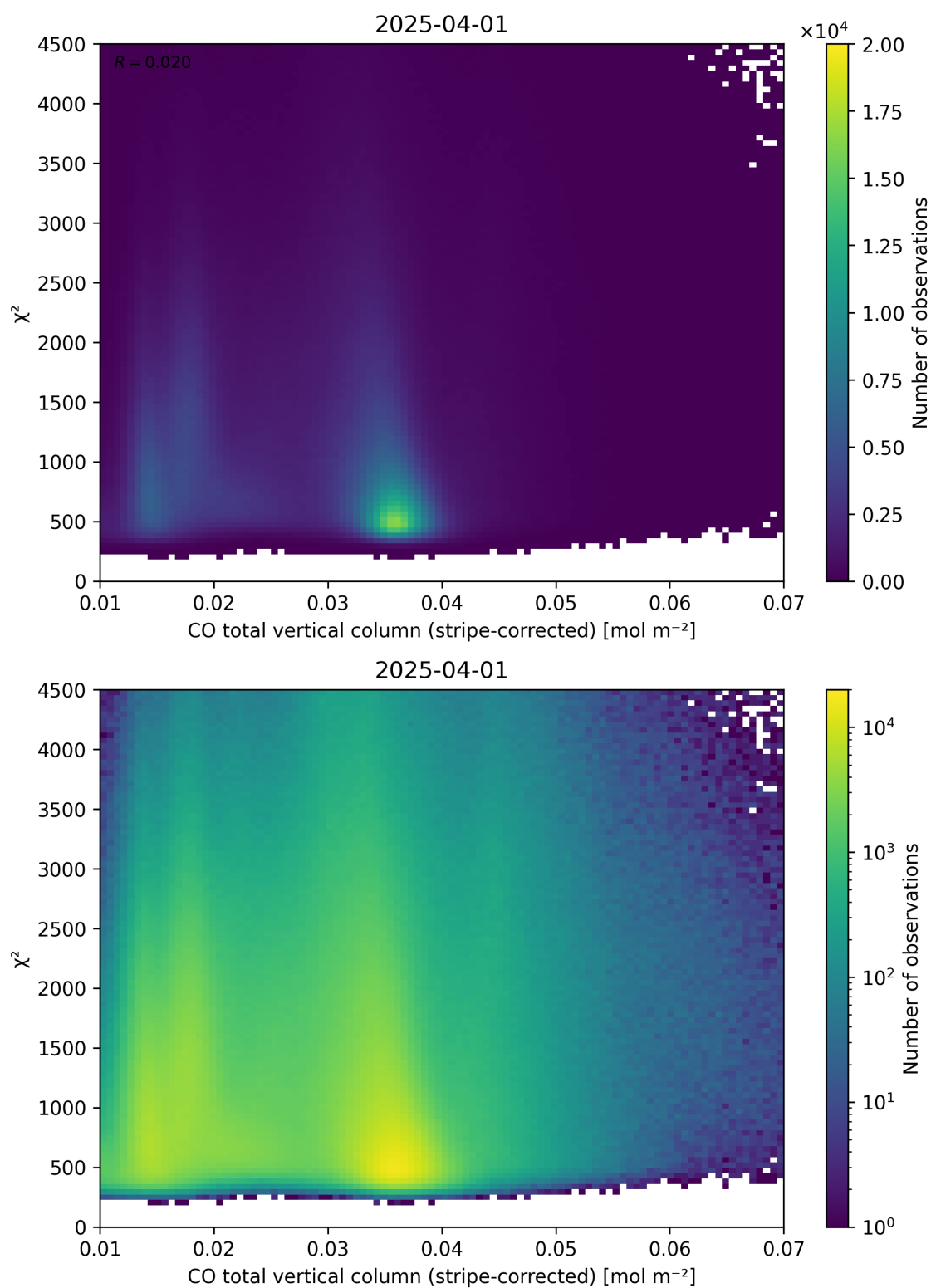
Figure 37: Scatter density plot of “CO total vertical column (stripe-corrected)” against “ \chi^2 ” for 2025-03-31 to 2025-04-02.
