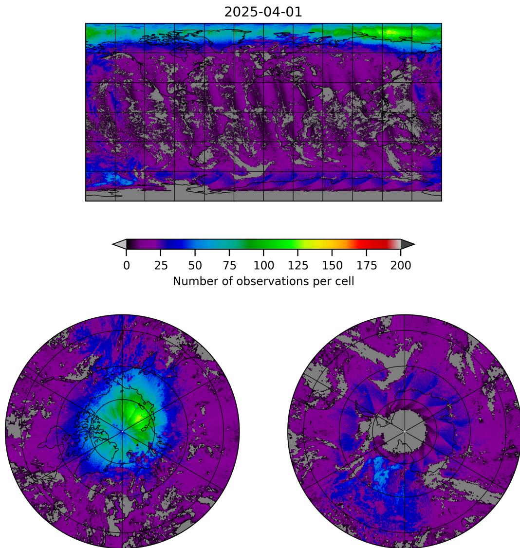
Figure 8: Map of the number of observations for 2025-03-31 to 2025-04-02
