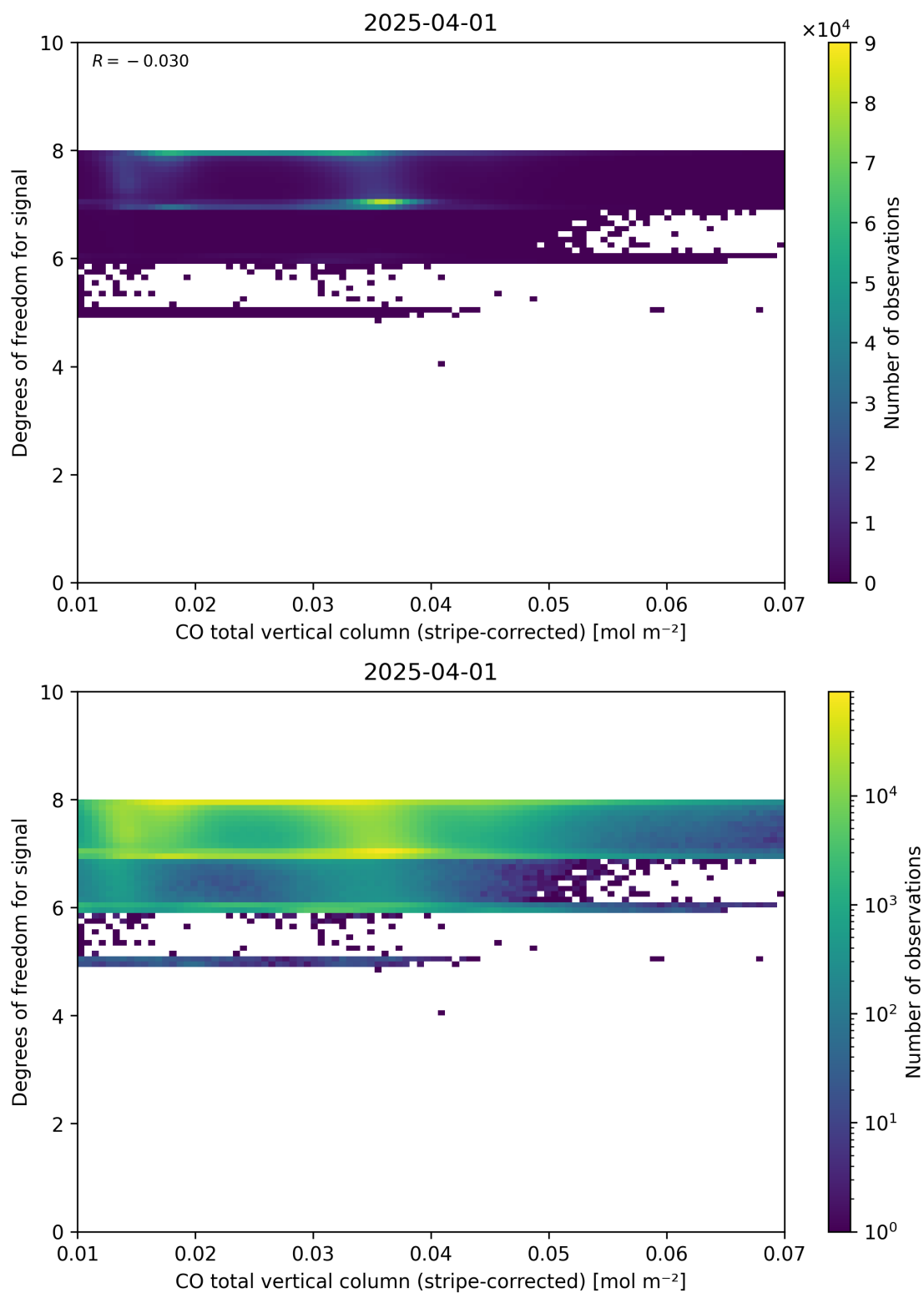
Figure 38: Scatter density plot of “CO total vertical column (stripe-corrected)” against “Degrees of freedom for signal” for 2025-03-31 to 2025-04-02.
