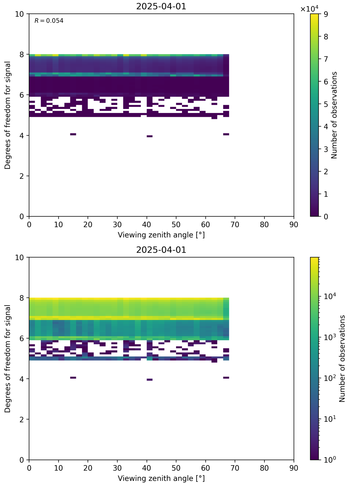
Figure 73: Scatter density plot of “Viewing zenith angle” against “Degrees of freedom for signal” for 2025-03-31 to 2025-04-02.
