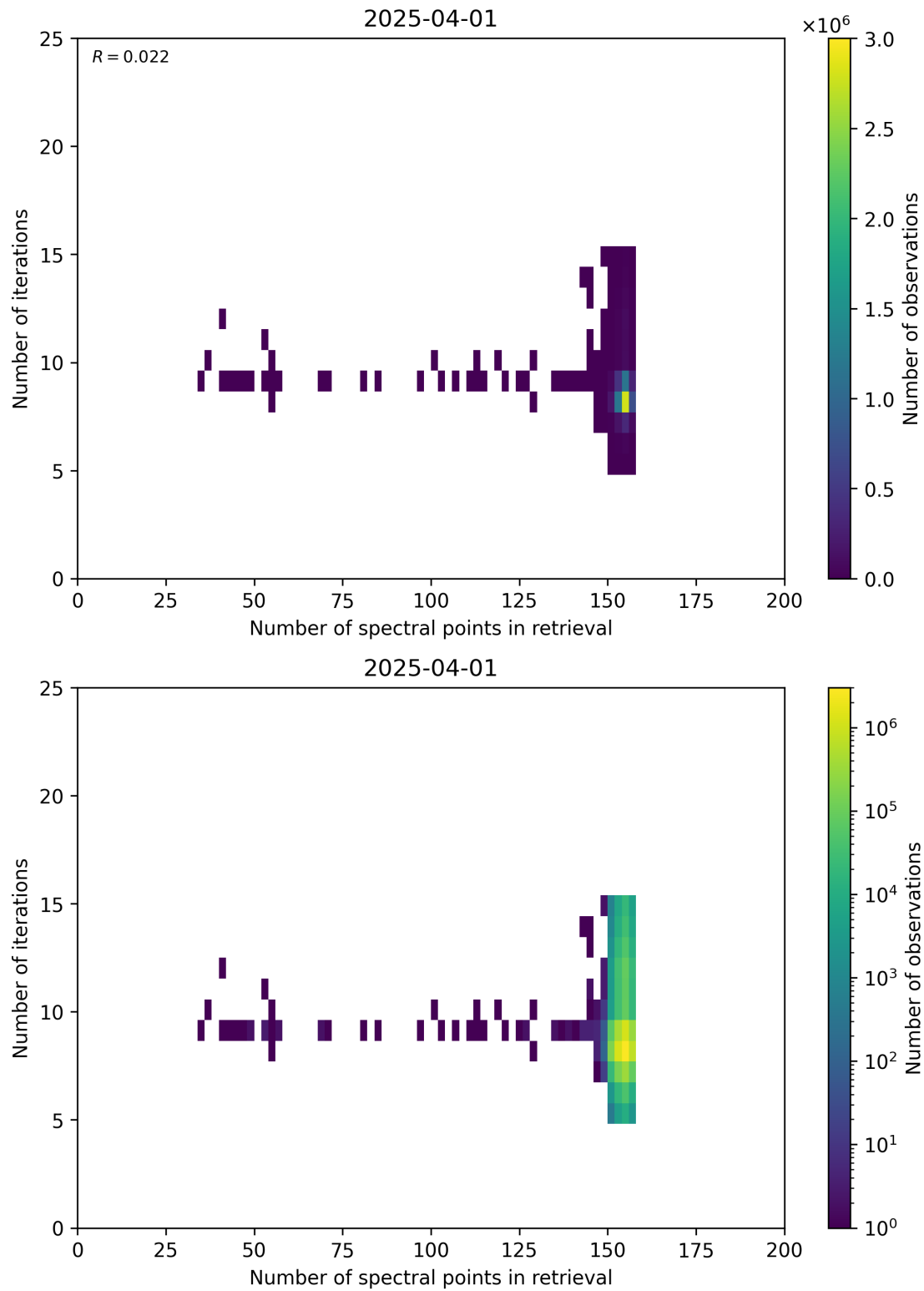
Figure 60: Scatter density plot of “Number of spectral points in retrieval” against “Number of iterations” for 2025-03-31 to 2025-04-02.
