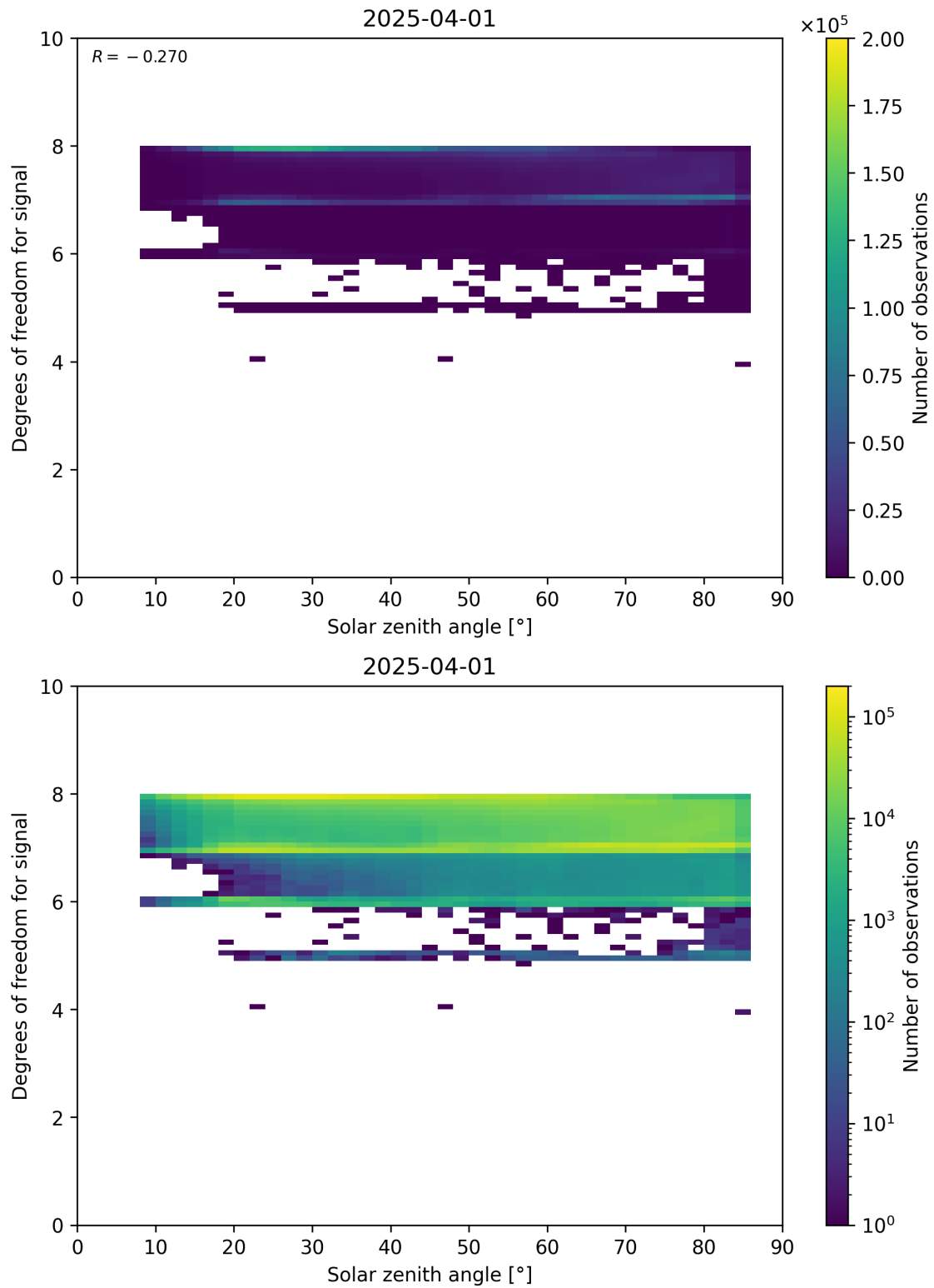
Figure 65: Scatter density plot of “Solar zenith angle” against “Degrees of freedom for signal” for 2025-03-31 to 2025-04-02.
