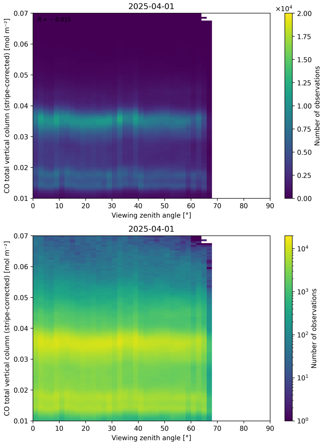
Figure 70: Scatter density plot of “Viewing zenith angle” against “CO total vertical column (stripe-corrected)” for 2025-03-31 to 2025-04-02.
