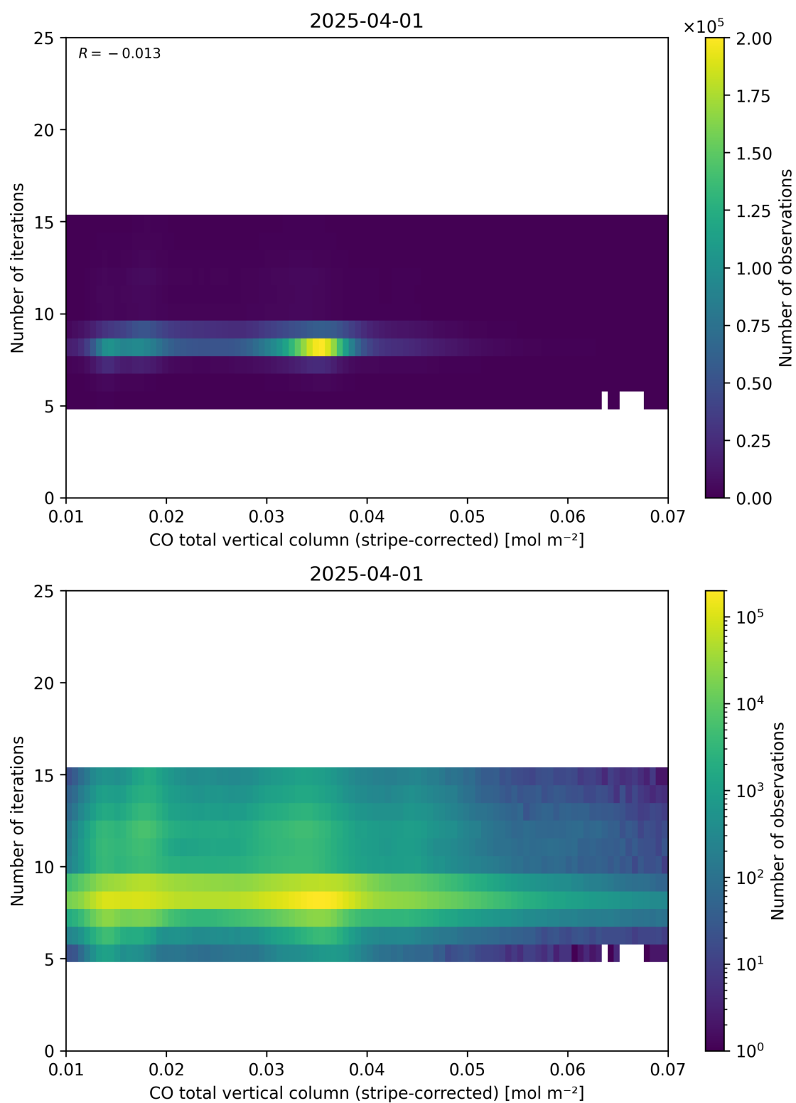
Figure 39: Scatter density plot of “CO total vertical column (stripe-corrected)” against “Number of iterations” for 2025-03-31 to 2025-04-02.
