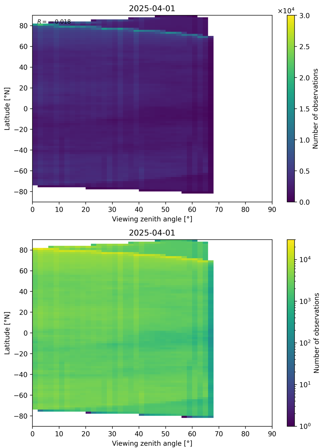
Figure 74: Scatter density plot of “Viewing zenith angle” against “Latitude” for 2025-03-31 to 2025-04-02.
