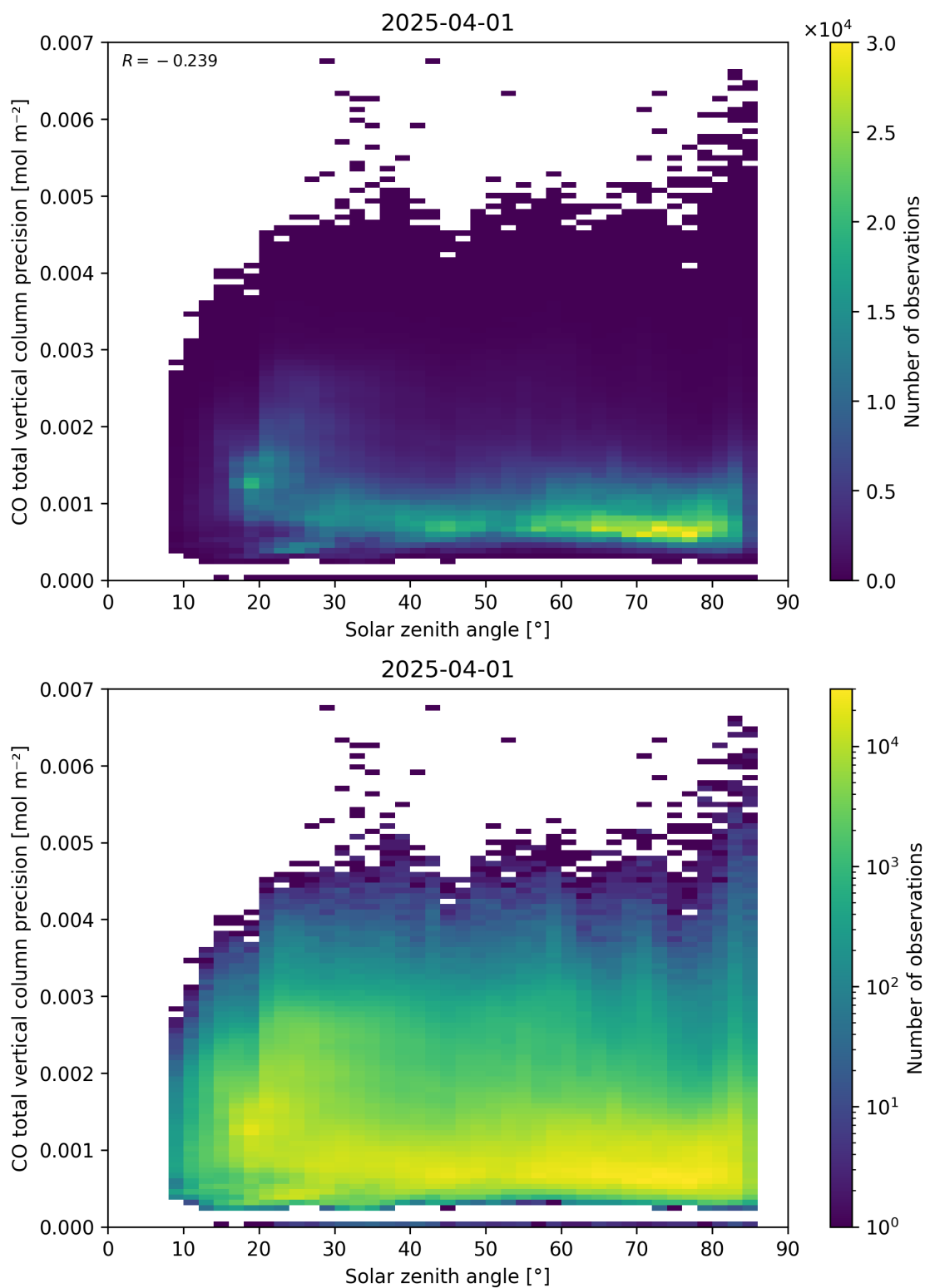
Figure 63: Scatter density plot of “Solar zenith angle” against “CO total vertical column precision” for 2025-03-31 to 2025-04-02.
