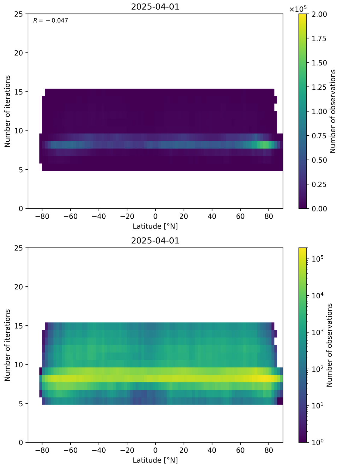
Figure 56: Scatter density plot of “Latitude” against “Number of iterations” for 2025-03-31 to 2025-04-02.
