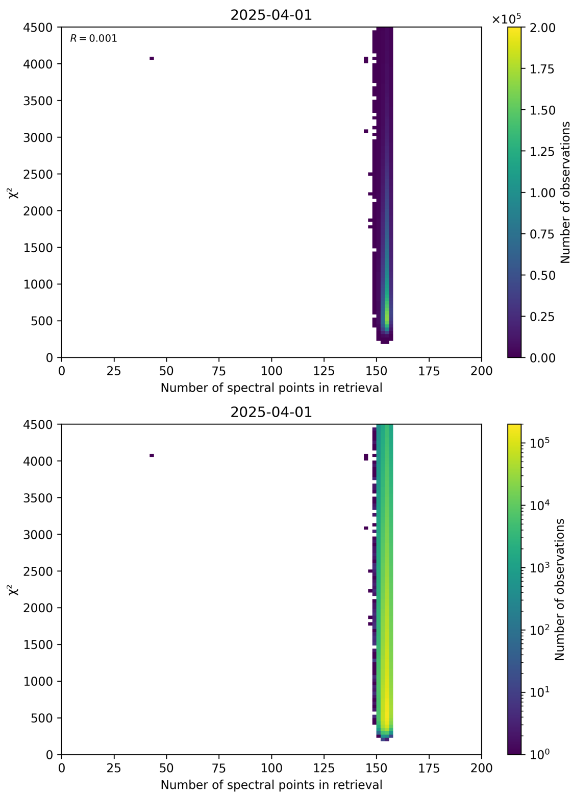
Figure 58: Scatter density plot of “Number of spectral points in retrieval” against “ \chi^2 ” for 2025-03-31 to 2025-04-02.
