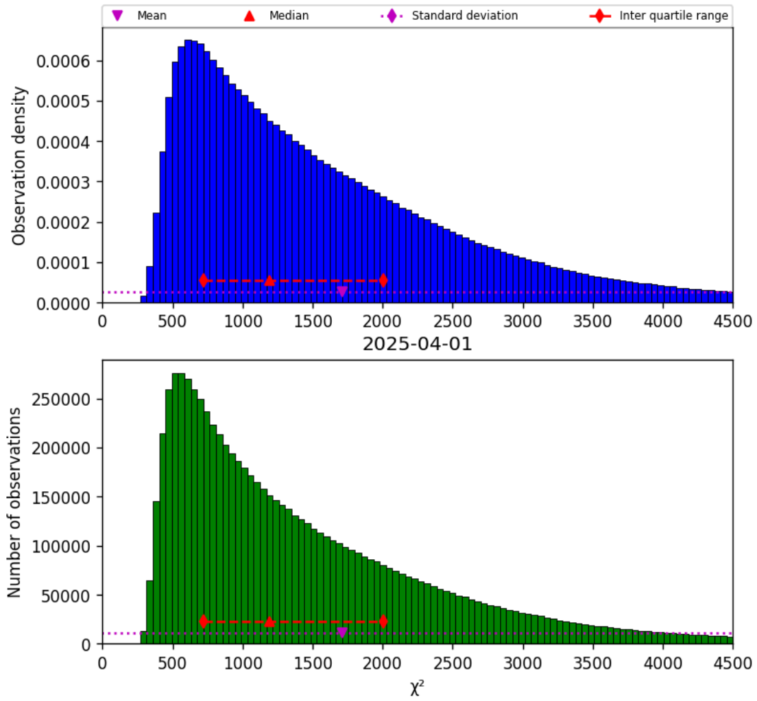
Figure 22: Histogram of “ \chi^2 ” for 2025-03-31 to 2025-04-02
