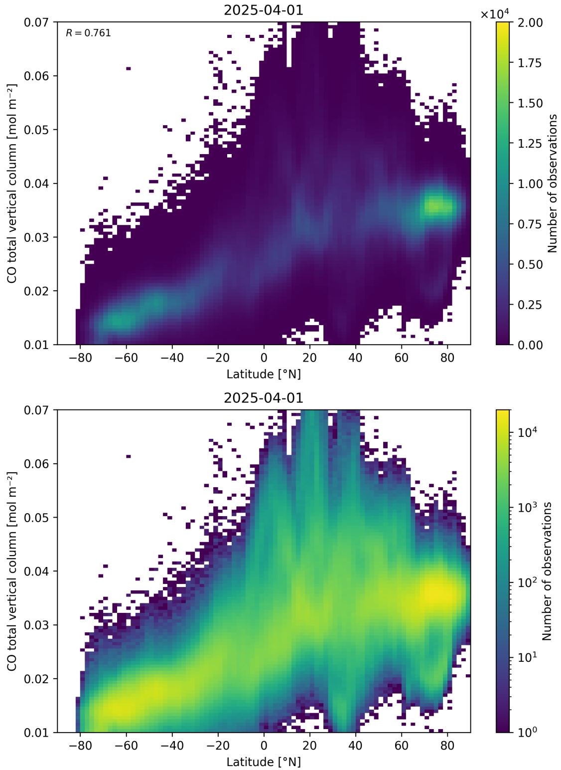
Figure 51: Scatter density plot of “Latitude” against “CO total vertical column” for 2025-03-31 to 2025-04-02.
