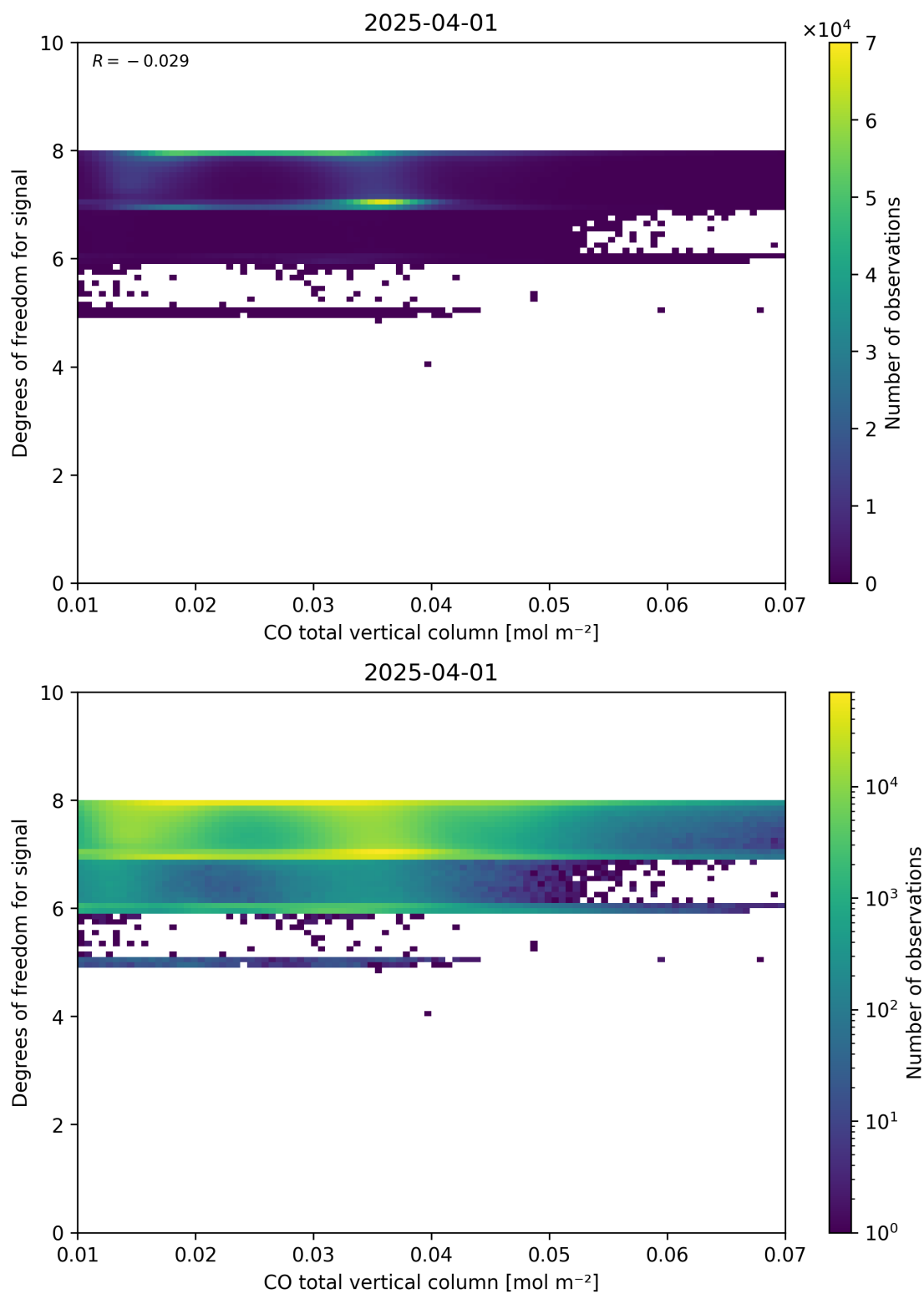
Figure 41: Scatter density plot of “CO total vertical column” against “Degrees of freedom for signal” for 2025-03-31 to 2025-04-02.
