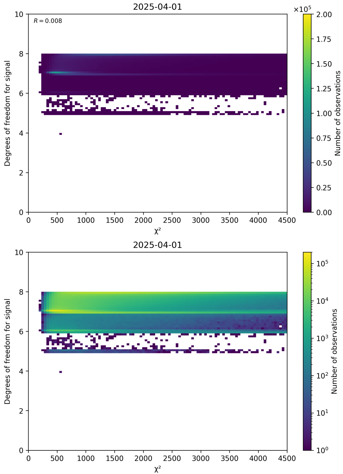
Figure 48: Scatter density plot of “ \chi^2 ” against “Degrees of freedom for signal” for 2025-03-31 to 2025-04-02.
