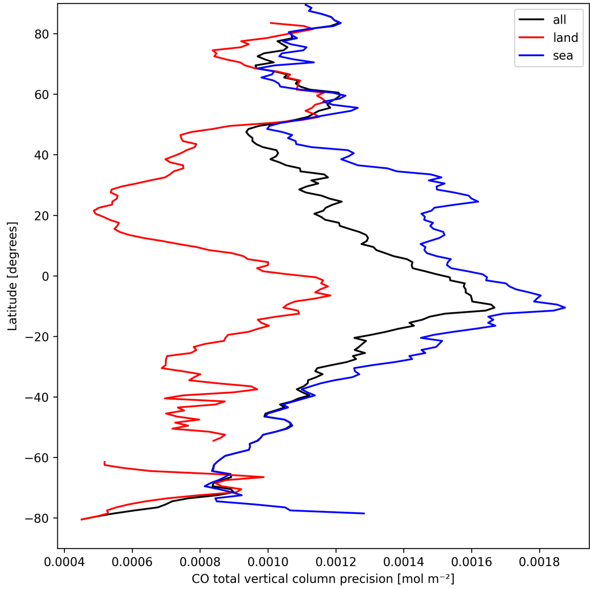
Figure 12: Zonal average of "CO total vertical column precision" for 2025-03-31 to 2025-04-02.
