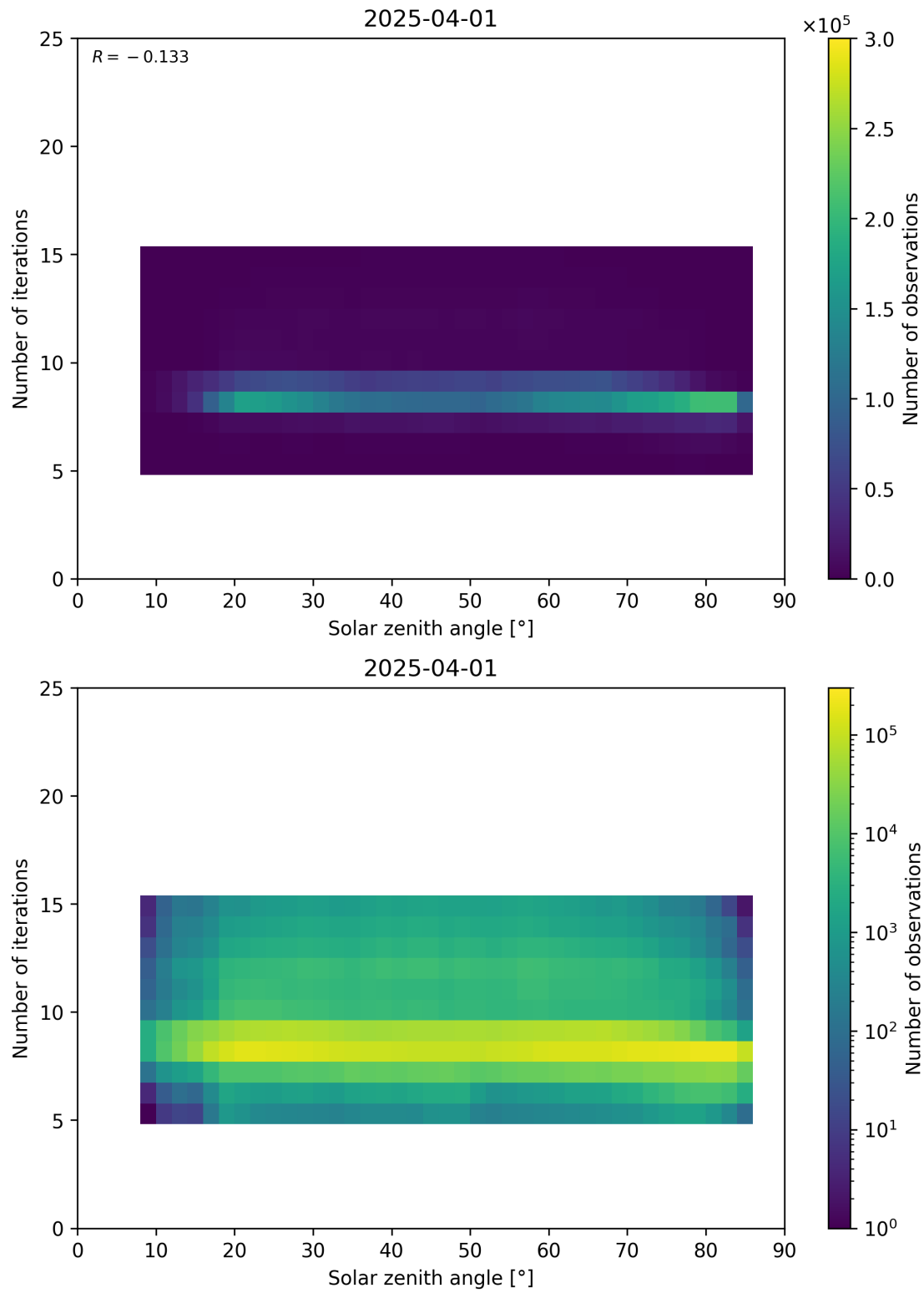
Figure 67: Scatter density plot of “Solar zenith angle” against “Number of iterations” for 2025-03-31 to 2025-04-02.
