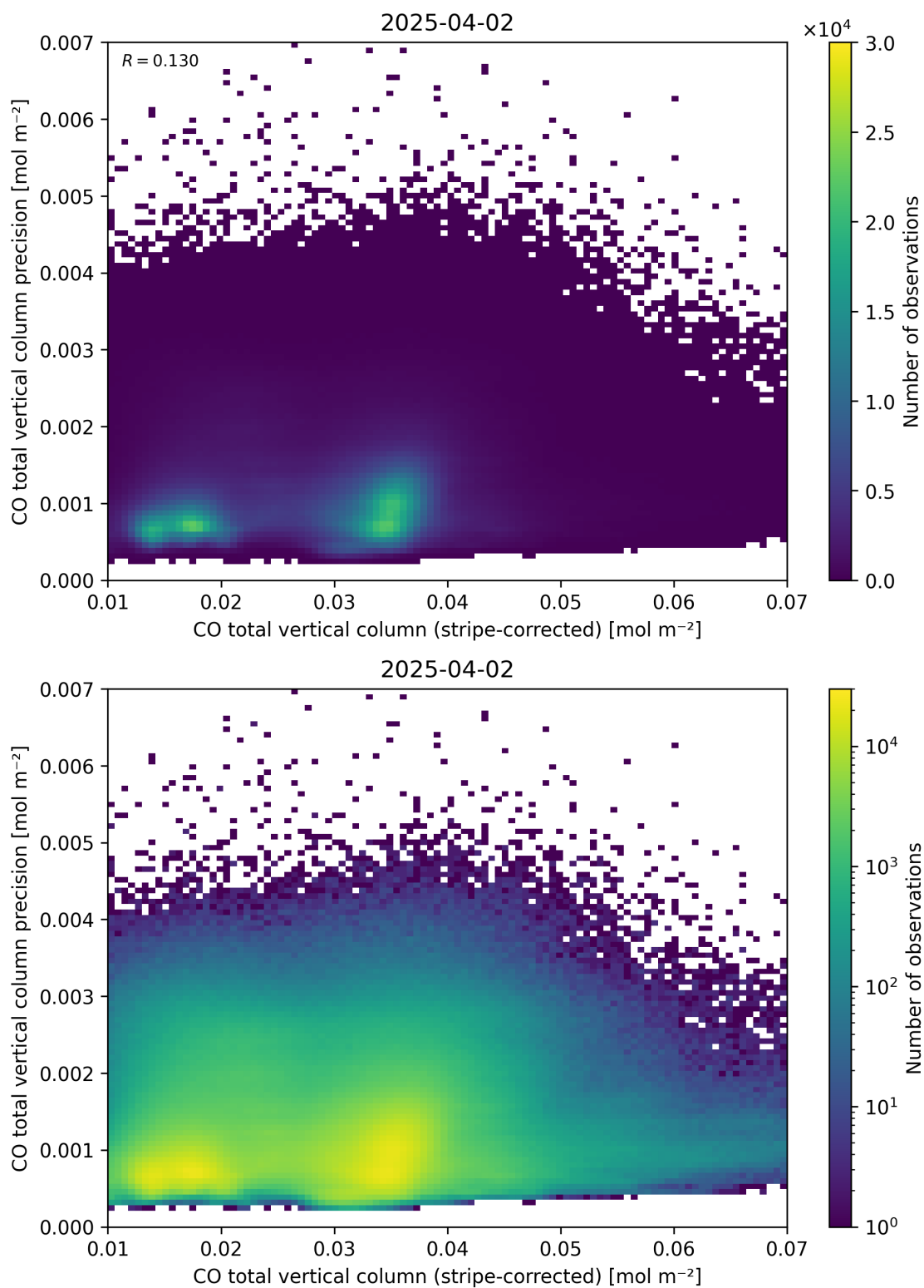
Figure 36: Scatter density plot of “CO total vertical column (stripe-corrected)” against “CO total vertical column precision” for 2025-04-02 to 2025-04-03.
