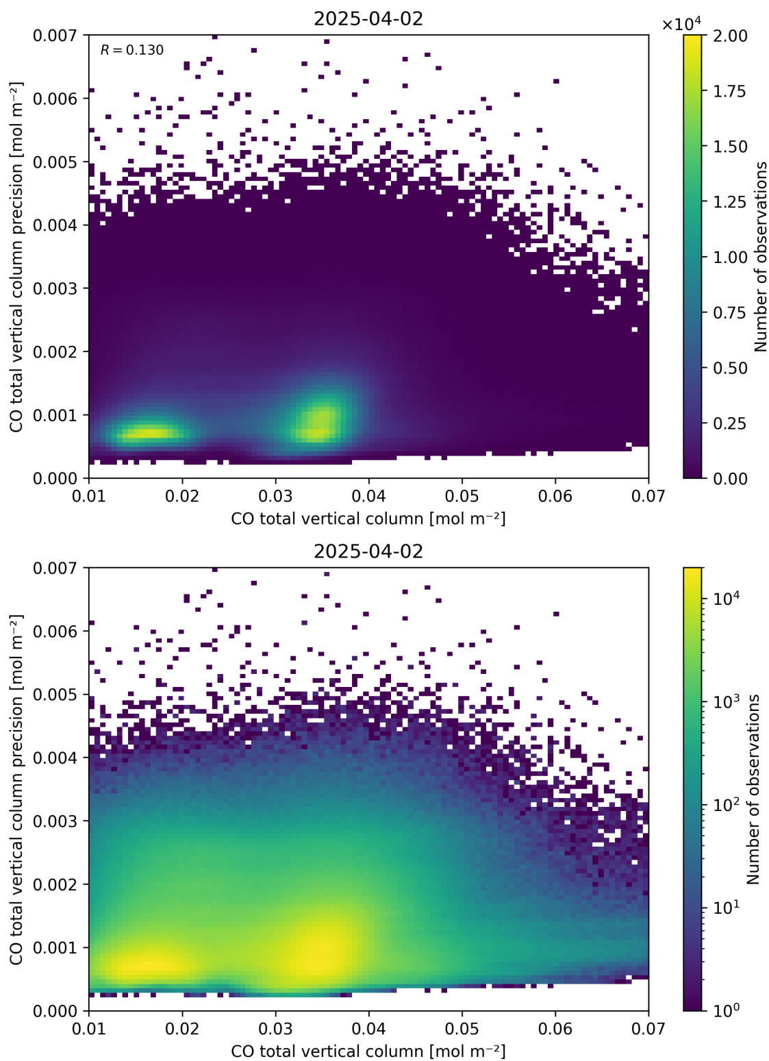
Figure 34: Scatter density plot of “CO total vertical column” against “CO total vertical column precision” for 2025-04-02 to 2025-04-03.
