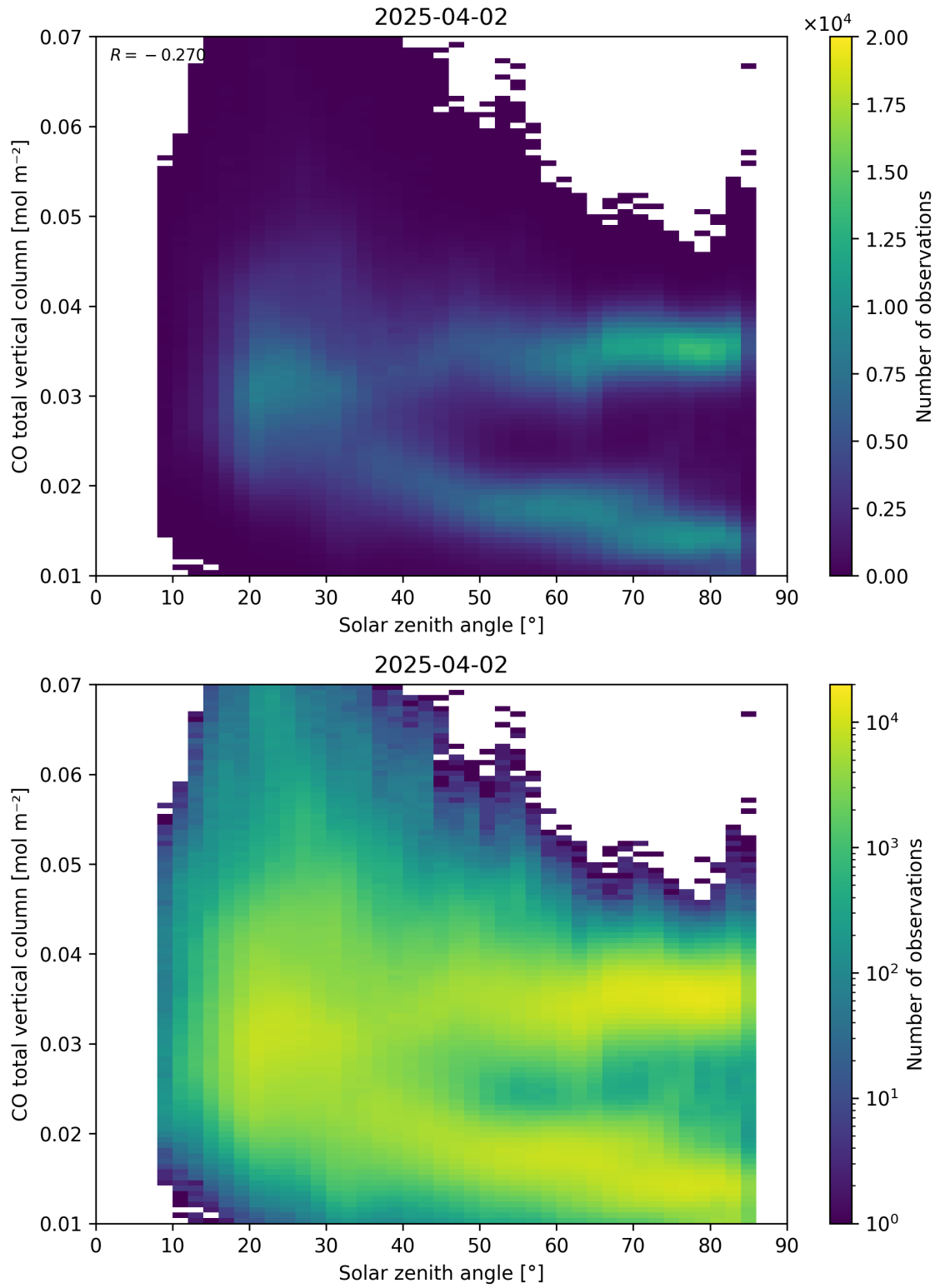
Figure 61: Scatter density plot of “Solar zenith angle” against “CO total vertical column” for 2025-04-02 to 2025-04-03.
