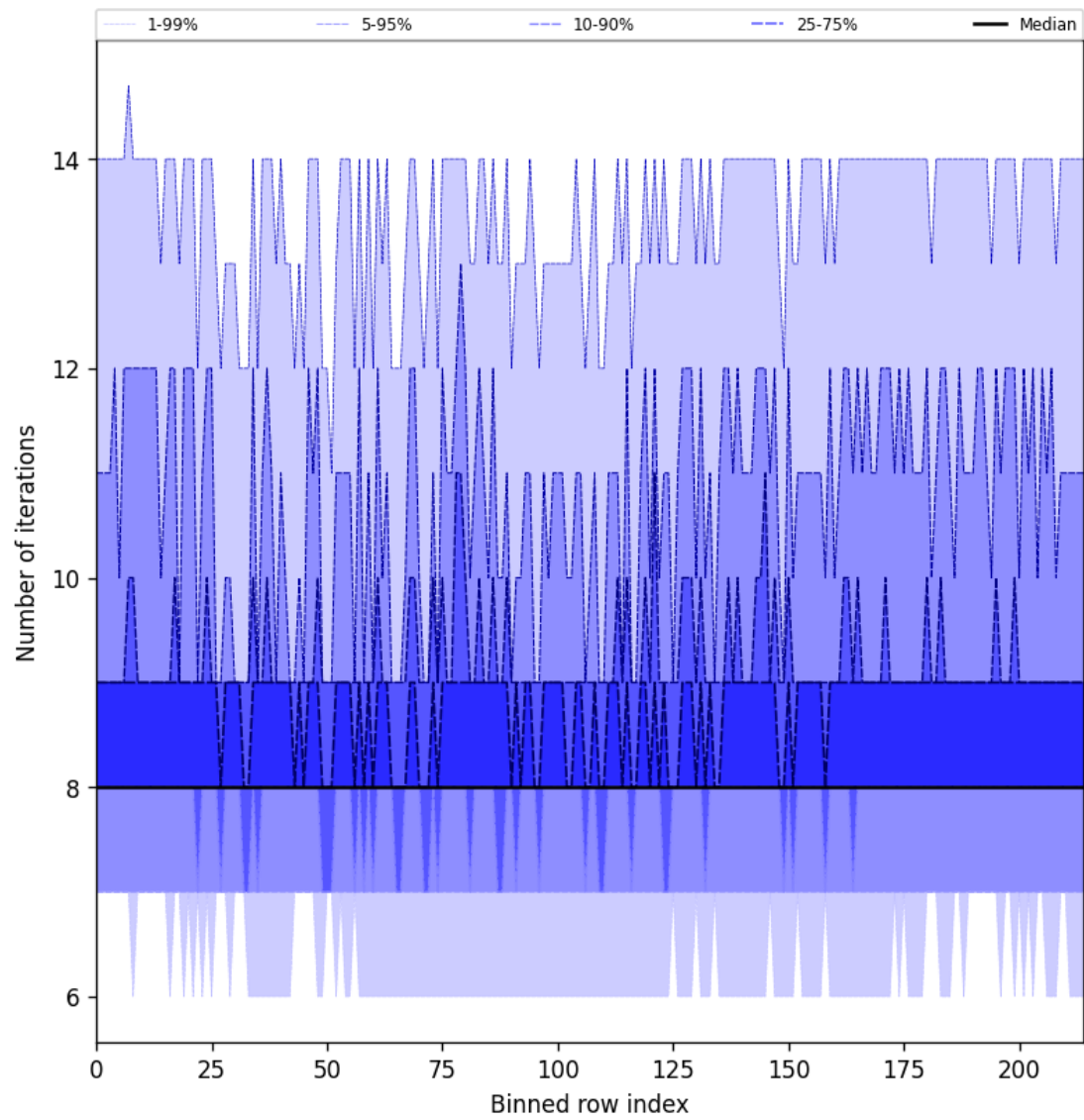
Figure 32: Along track statistics of “Number of iterations” for 2025-04-02 to 2025-04-03
