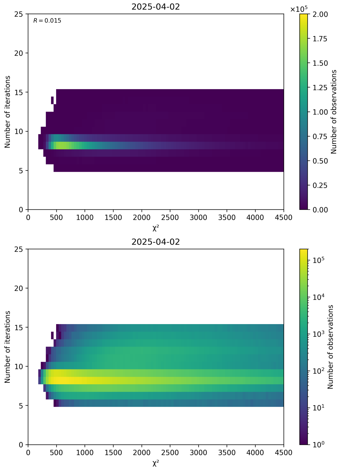
Figure 49: Scatter density plot of “ \chi^2 ” against “Number of iterations” for 2025-04-02 to 2025-04-03.
