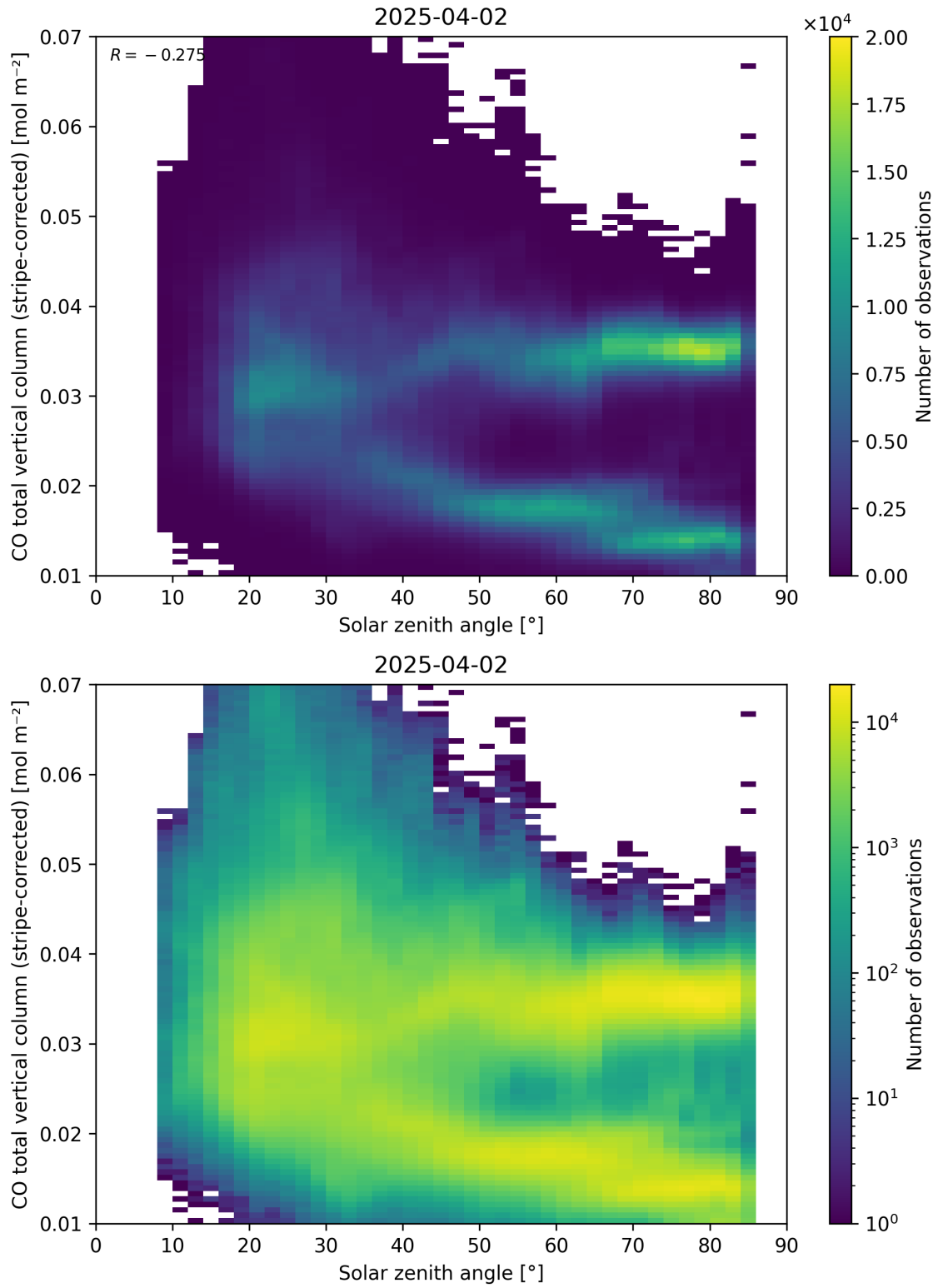
Figure 62: Scatter density plot of “Solar zenith angle” against “CO total vertical column (stripe-corrected)” for 2025-04-02 to 2025-04-03.
