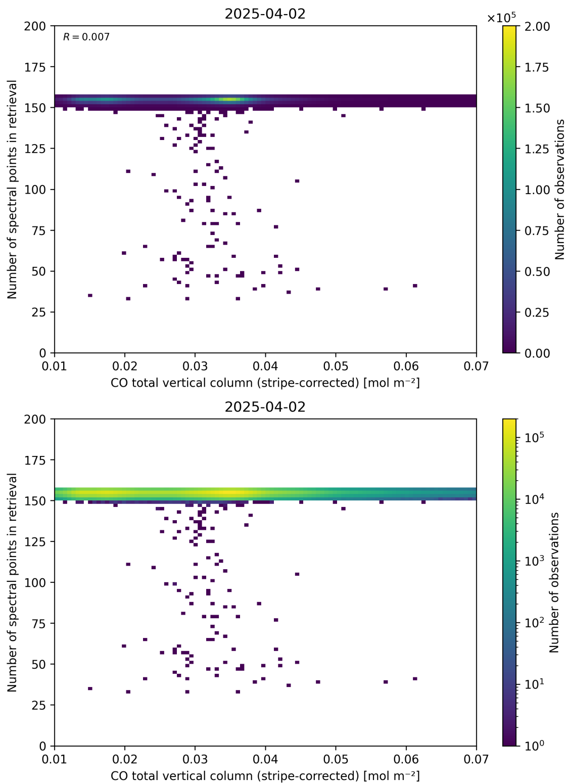
Figure 40: Scatter density plot of “CO total vertical column (stripe-corrected)” against “Number of spectral points in retrieval” for 2025-04-02 to 2025-04-03.
