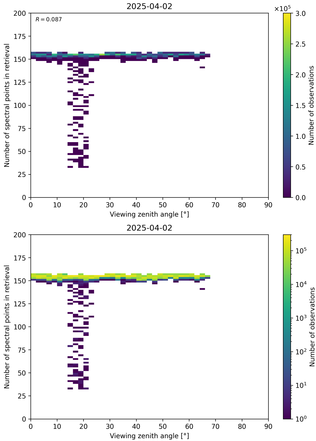
Figure 76: Scatter density plot of “Viewing zenith angle” against “Number of spectral points in retrieval” for 2025-04-02 to 2025-04-03.
