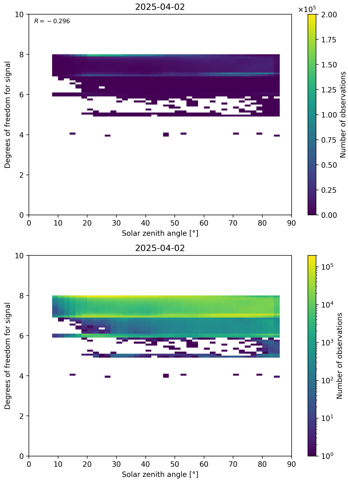
Figure 65: Scatter density plot of “Solar zenith angle” against “Degrees of freedom for signal” for 2025-04-02 to 2025-04-03.
