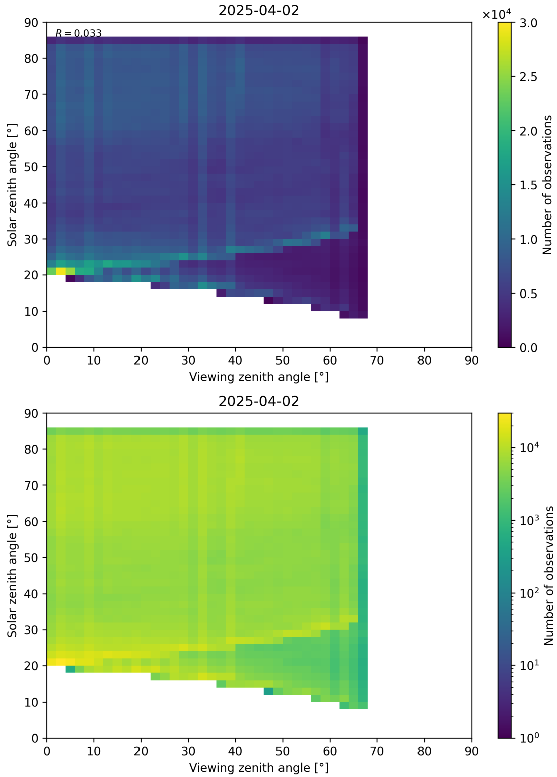
Figure 77: Scatter density plot of “Viewing zenith angle” against “Solar zenith angle” for 2025-04-02 to 2025-04-03.
