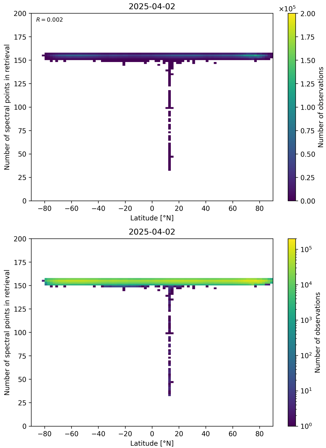
Figure 57: Scatter density plot of “Latitude” against “Number of spectral points in retrieval” for 2025-04-02 to 2025-04-03.
