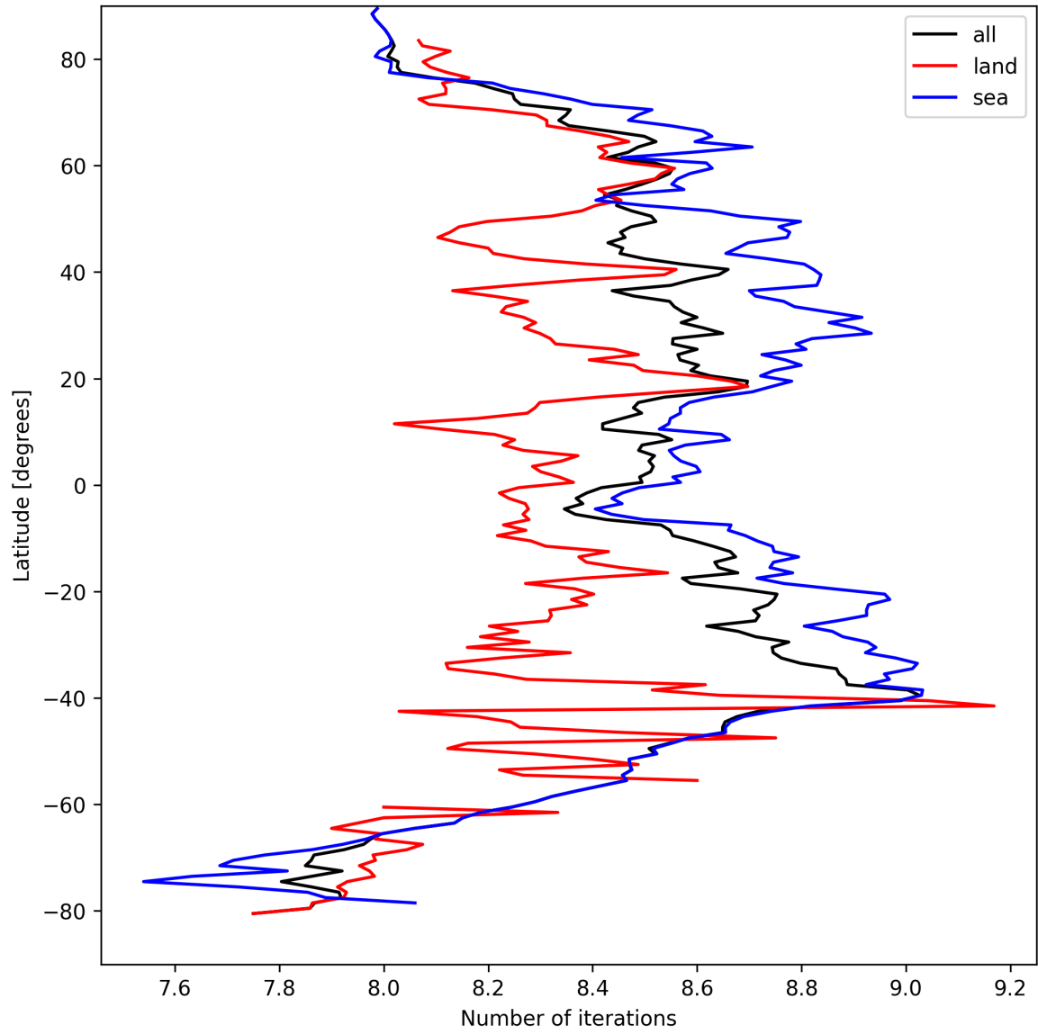
Figure 16: Zonal average of “Number of iterations” for 2025-04-02 to 2025-04-03.
