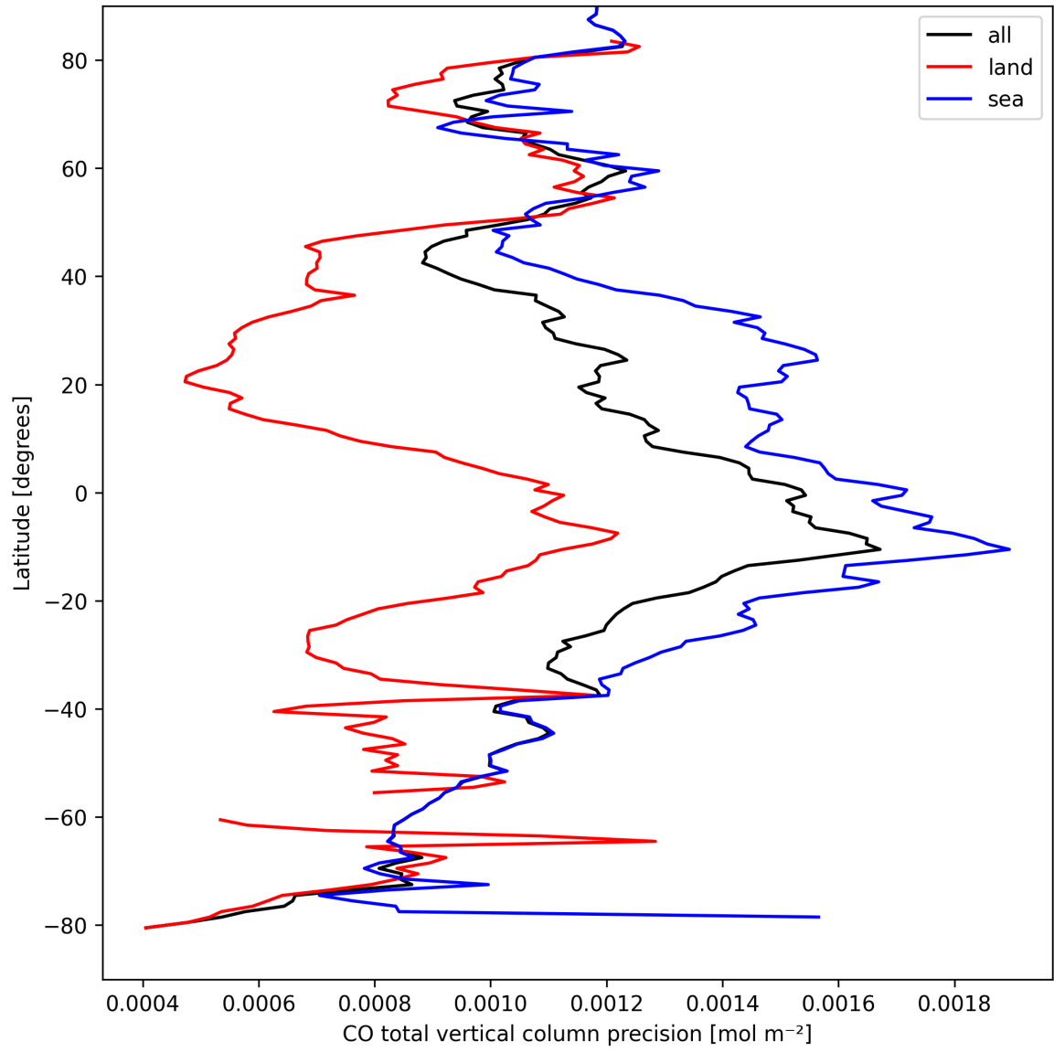
Figure 12: Zonal average of “CO total vertical column precision” for 2025-04-02 to 2025-04-03.
