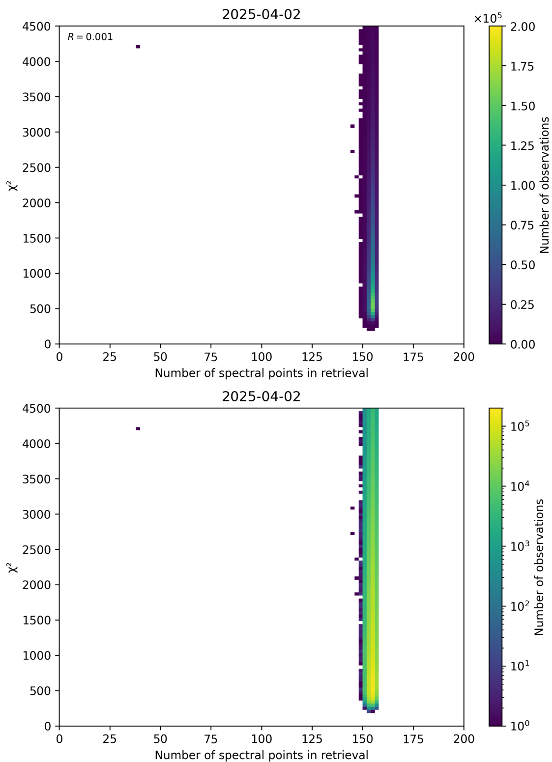
Figure 58: Scatter density plot of “Number of spectral points in retrieval” against “ \chi^2 ” for 2025-04-02 to 2025-04-03.
