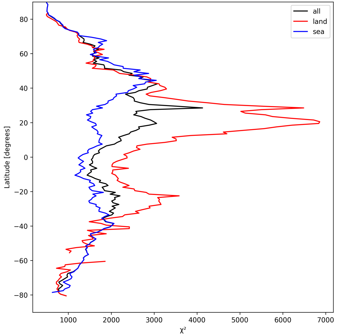
Figure 14: Zonal average of “ \chi^2 ” for 2025-04-02 to 2025-04-03.
