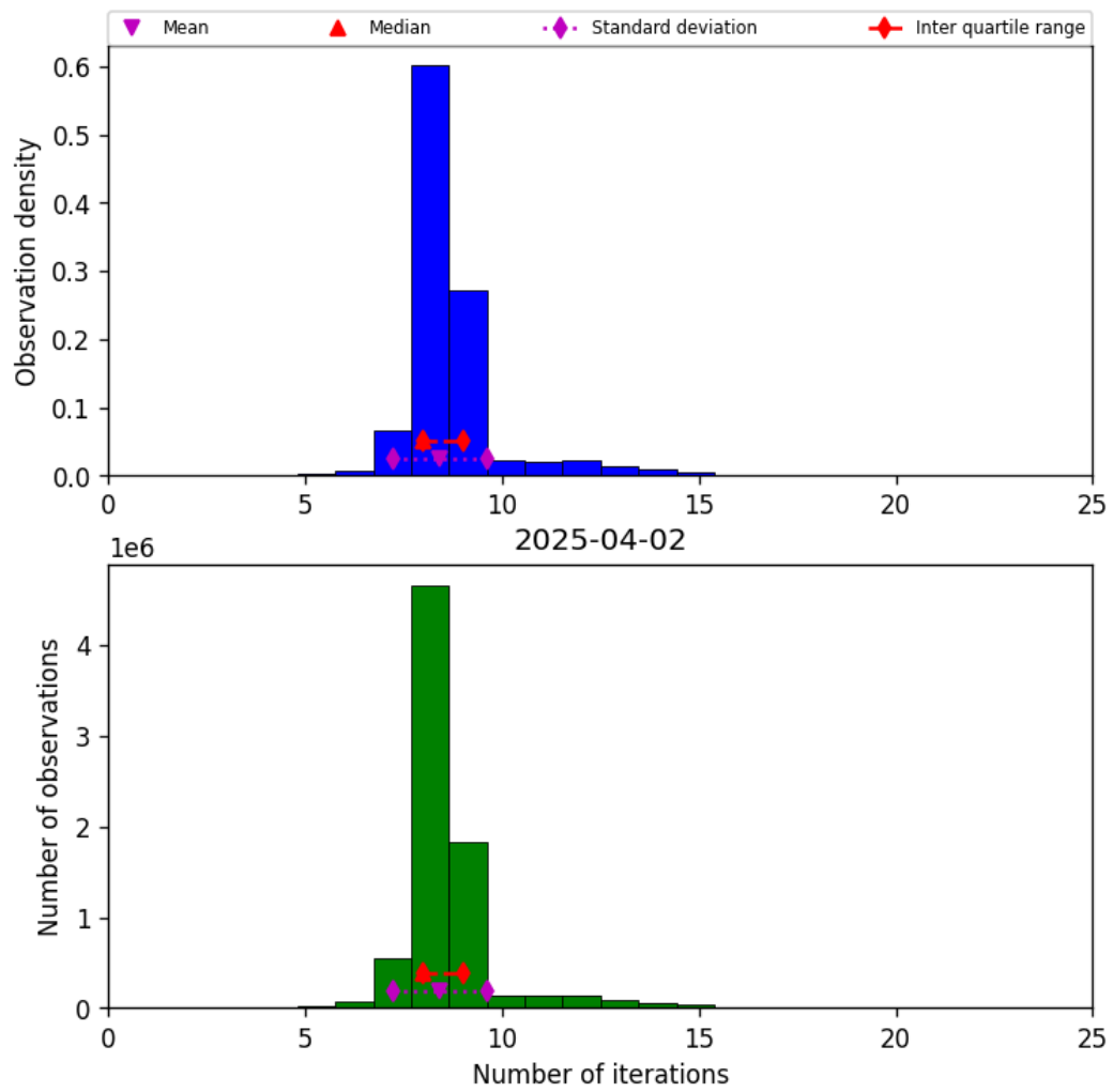
Figure 24: Histogram of “Number of iterations” for 2025-04-02 to 2025-04-03
