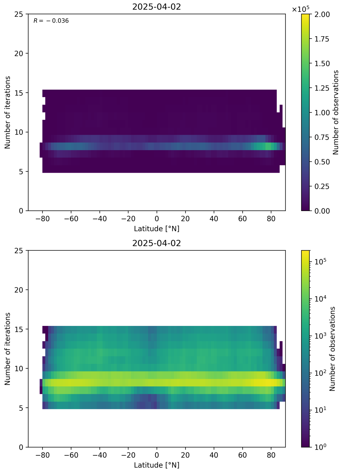
Figure 56: Scatter density plot of “Latitude” against “Number of iterations” for 2025-04-02 to 2025-04-03.
