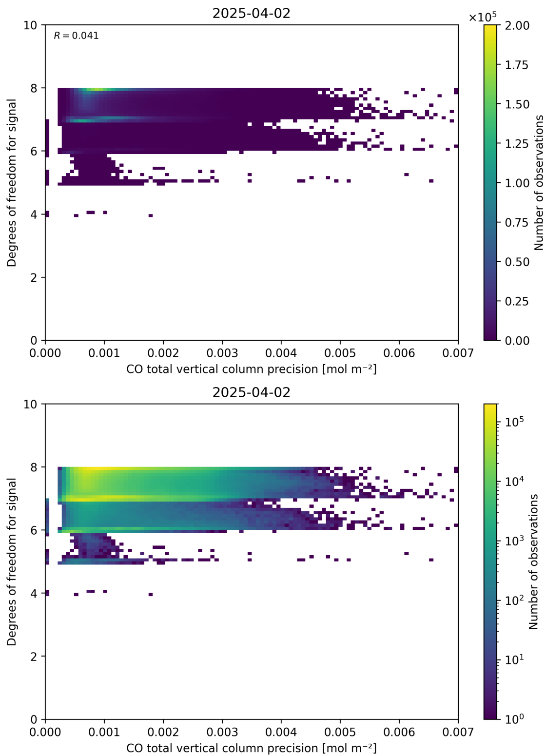
Figure 45: Scatter density plot of “CO total vertical column precision” against “Degrees of freedom for signal” for 2025-04-02 to 2025-04-03.
