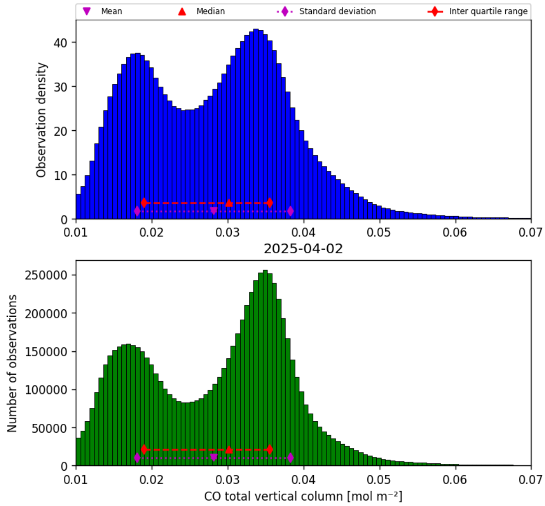
Figure 18: Histogram of “CO total vertical column” for 2025-04-02 to 2025-04-03
