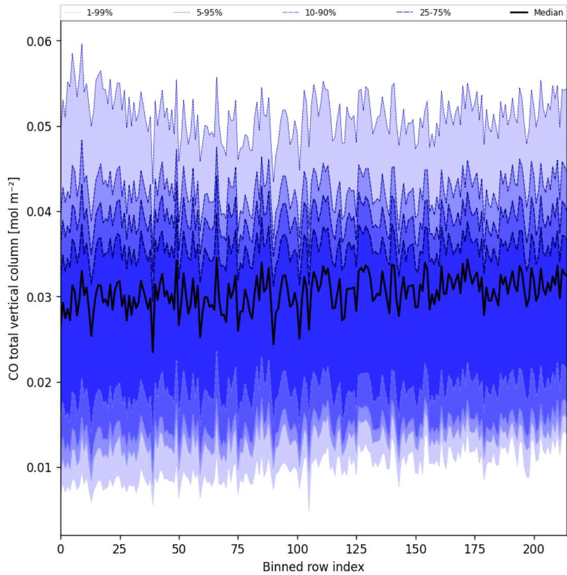
Figure 26: Along track statistics of “CO total vertical column” for 2025-04-02 to 2025-04-03
