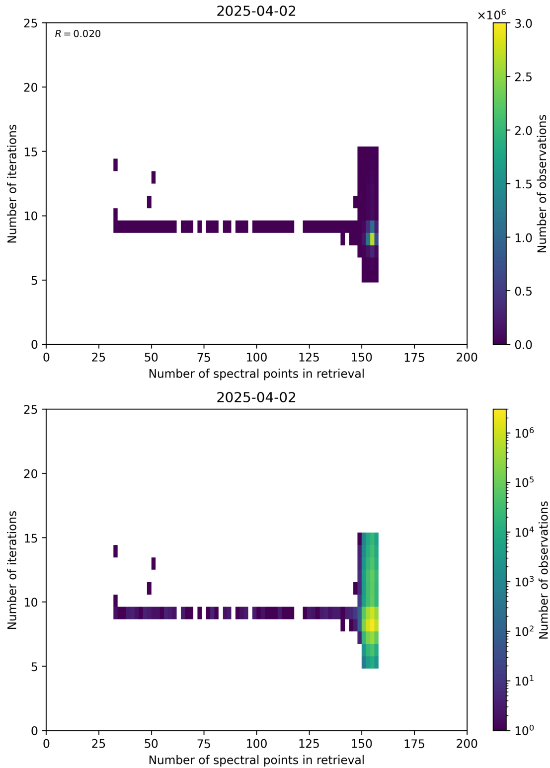
Figure 60: Scatter density plot of “Number of spectral points in retrieval” against “Number of iterations” for 2025-04-02 to 2025-04-03.
