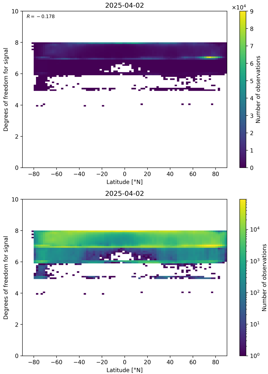
Figure 55: Scatter density plot of “Latitude” against “Degrees of freedom for signal” for 2025-04-02 to 2025-04-03.
