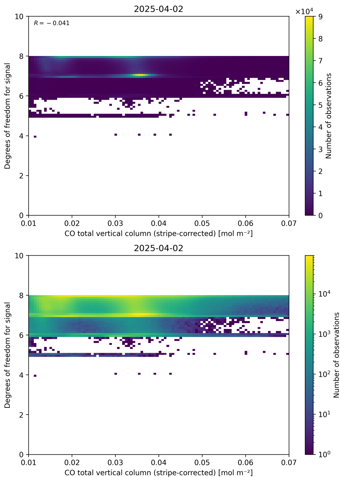
Figure 38: Scatter density plot of “CO total vertical column (stripe-corrected)” against “Degrees of freedom for signal” for 2025-04-02 to 2025-04-03.
