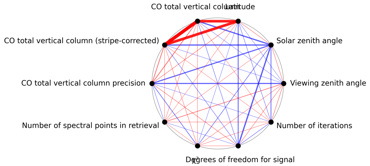
Figure 1: Map of correlation graph for 2025-04-02 to 2025-04-03.
