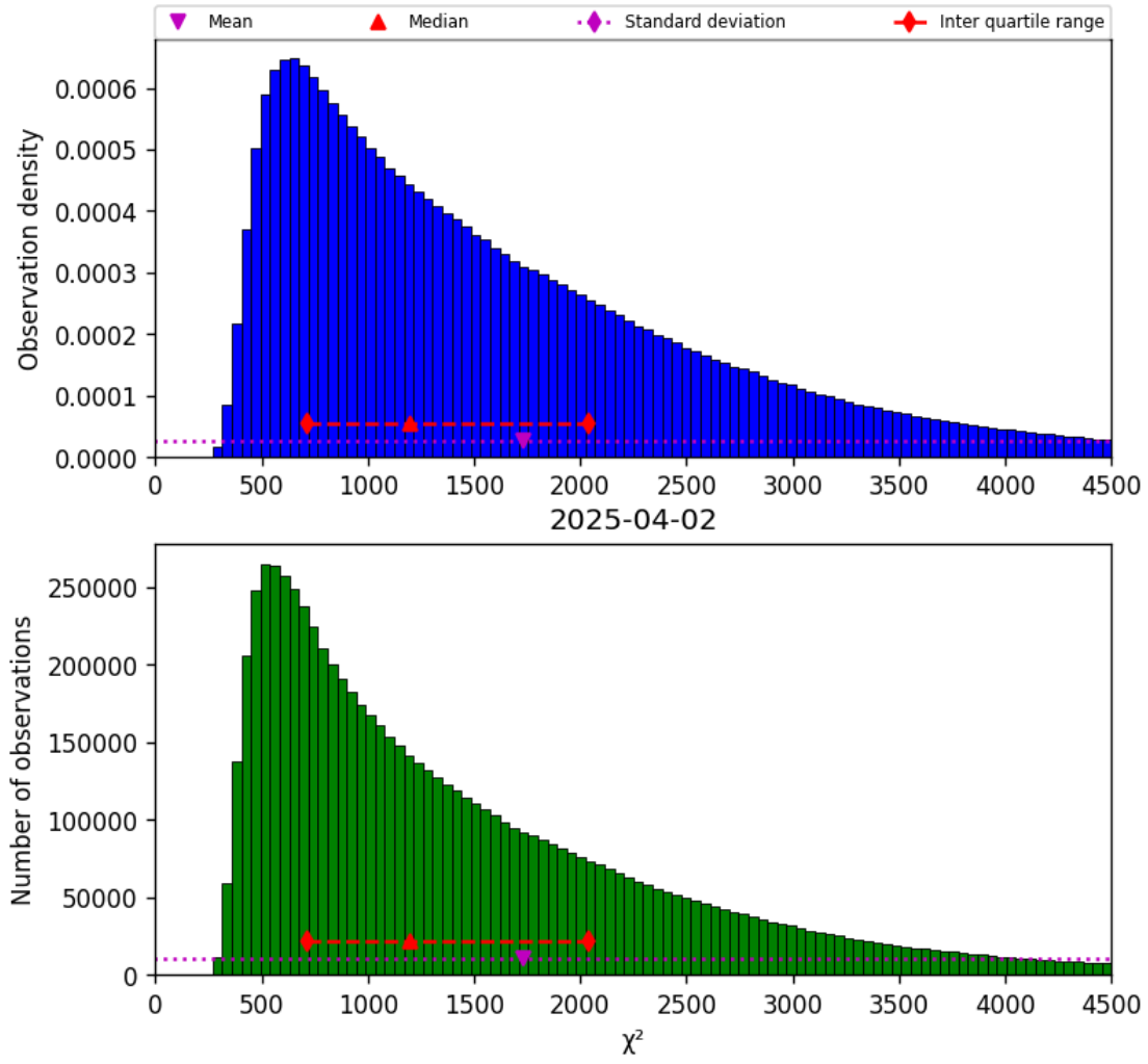
Figure 22: Histogram of “ \chi^2 ” for 2025-04-02 to 2025-04-03
