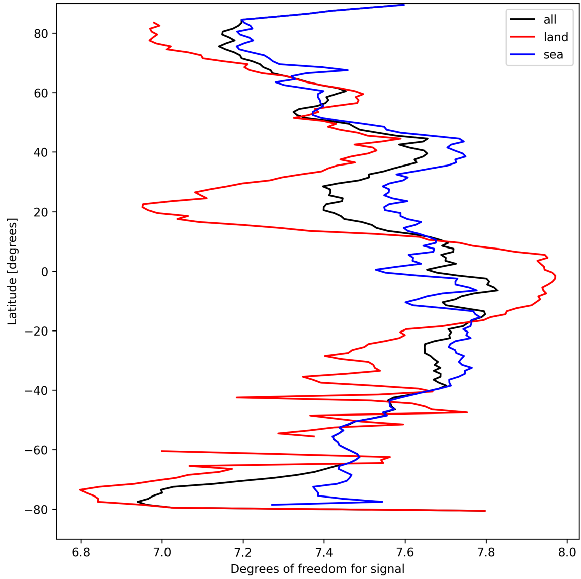
Figure 15: Zonal average of “Degrees of freedom for signal” for 2025-04-02 to 2025-04-03.
