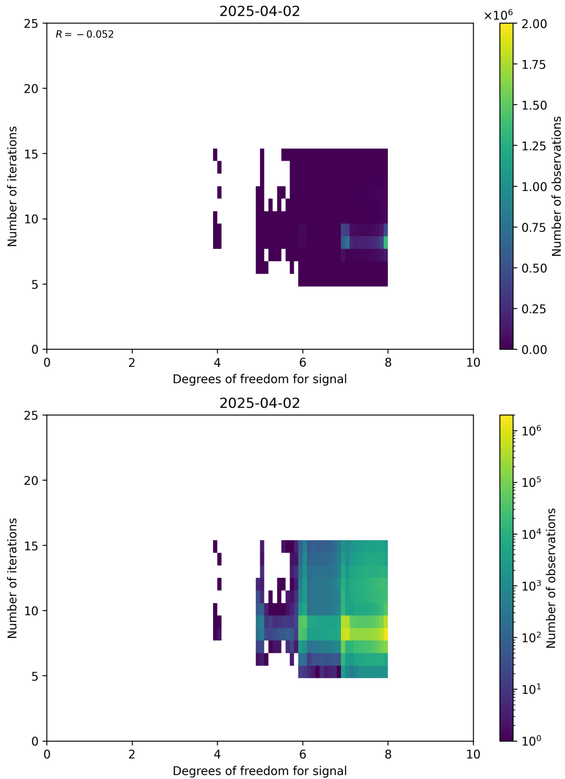
Figure 50: Scatter density plot of “Degrees of freedom for signal” against “Number of iterations” for 2025-04-02 to 2025-04-03.
