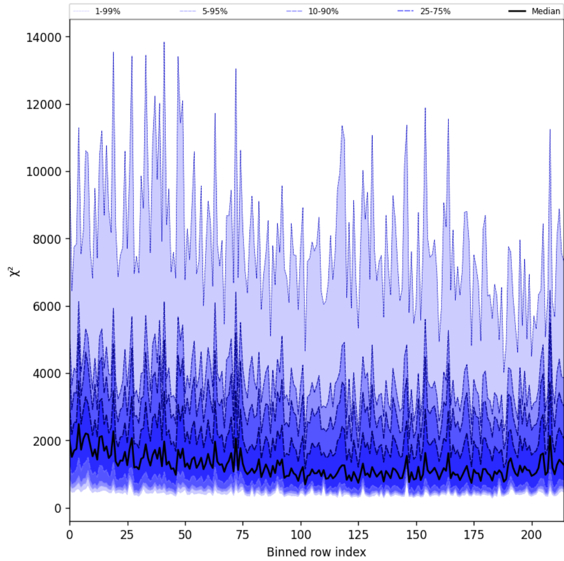
Figure 30: Along track statistics of “ \chi^2 ” for 2025-04-02 to 2025-04-03
