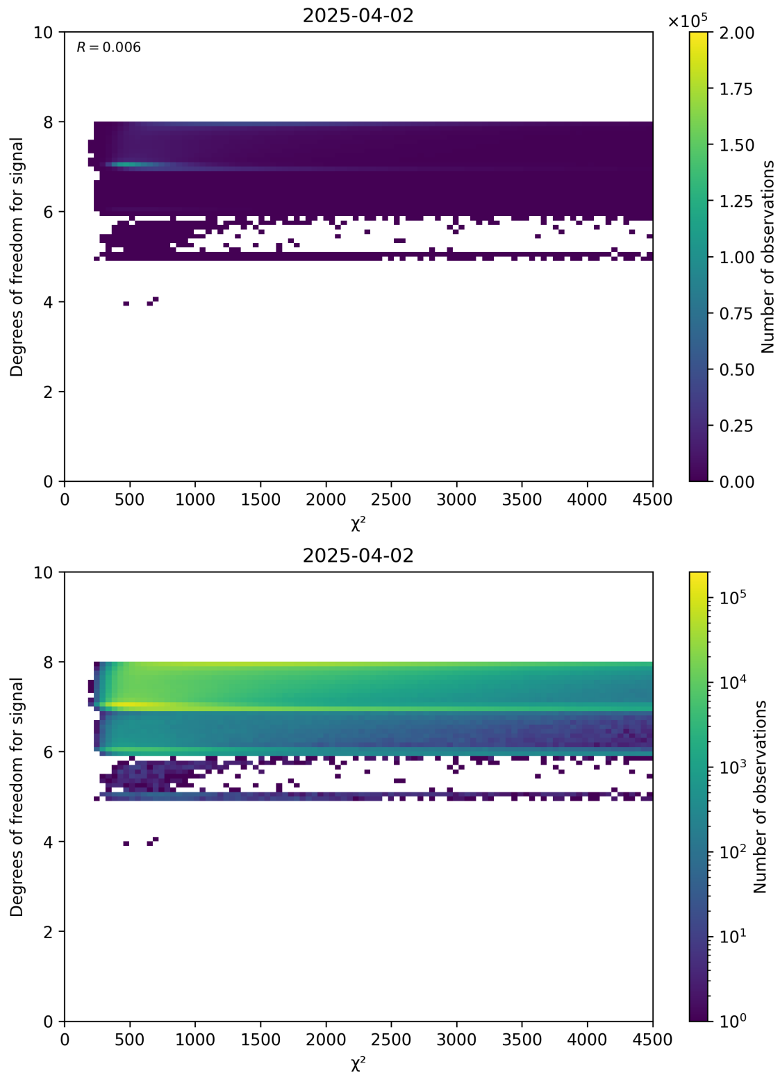
Figure 48: Scatter density plot of “ \chi^2 ” against “Degrees of freedom for signal” for 2025-04-02 to 2025-04-03.
