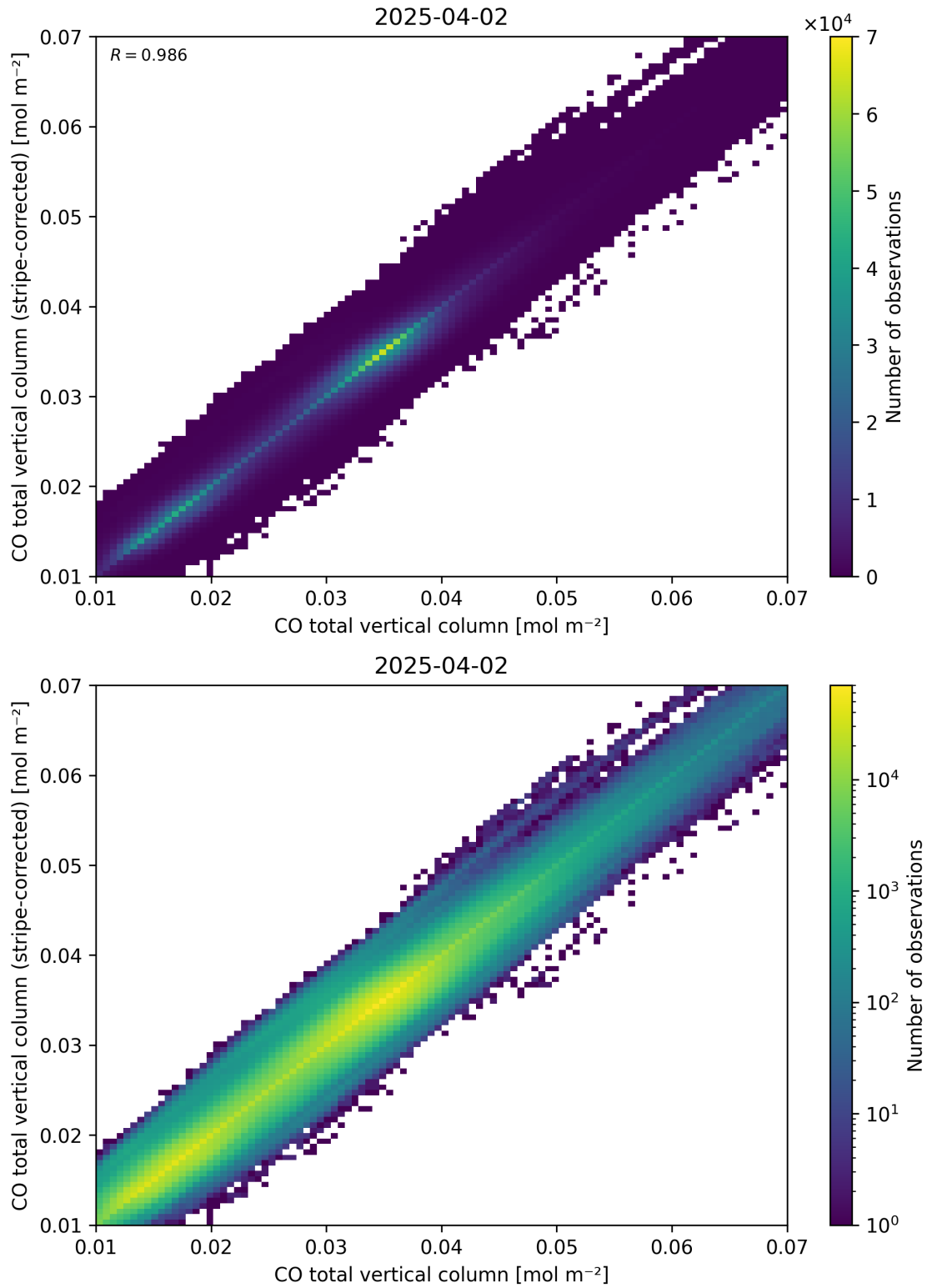
Figure 33: Scatter density plot of “CO total vertical column” against “CO total vertical column (stripe-corrected)” for 2025-04-02 to 2025-04-03.
