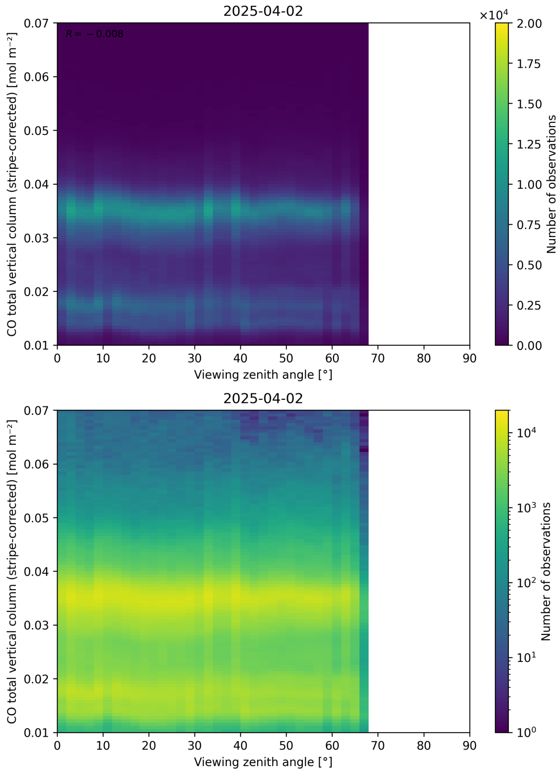
Figure 70: Scatter density plot of “Viewing zenith angle” against “CO total vertical column (stripe-corrected)” for 2025-04-02 to 2025-04-03.
