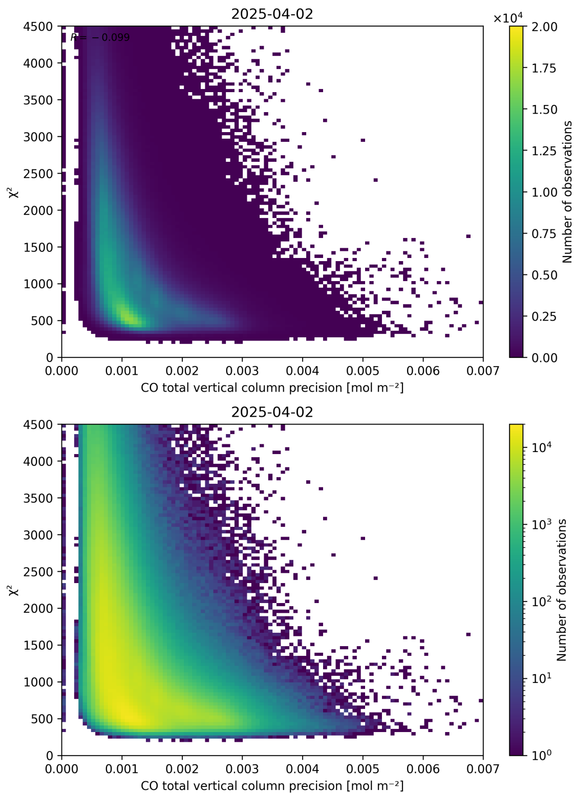
Figure 44: Scatter density plot of “CO total vertical column precision” against “ \chi^2 ” for 2025-04-02 to 2025-04-03.
