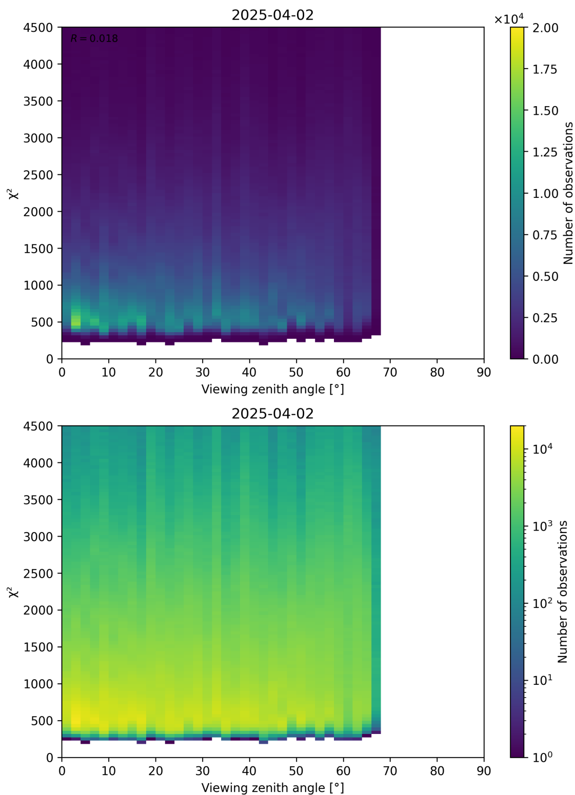
Figure 72: Scatter density plot of “Viewing zenith angle” against “ \chi^2 ” for 2025-04-02 to 2025-04-03.
