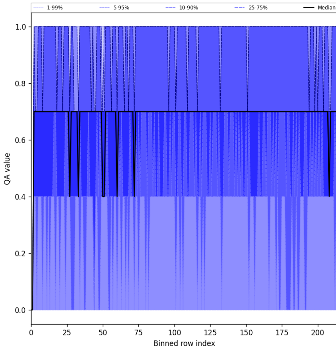
Figure 25: Along track statistics of “QA value” for 2025-04-02 to 2025-04-03
