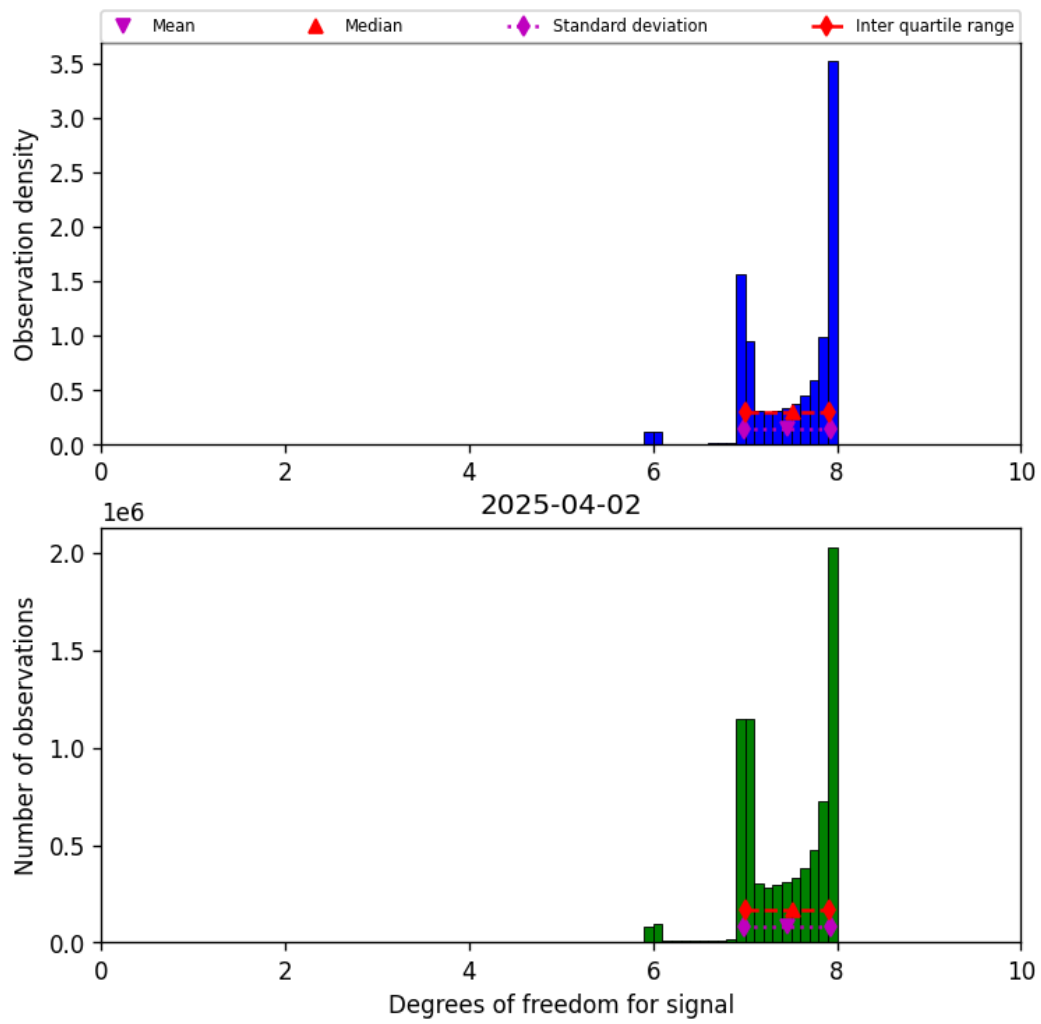
Figure 23: Histogram of “Degrees of freedom for signal” for 2025-04-02 to 2025-04-03
