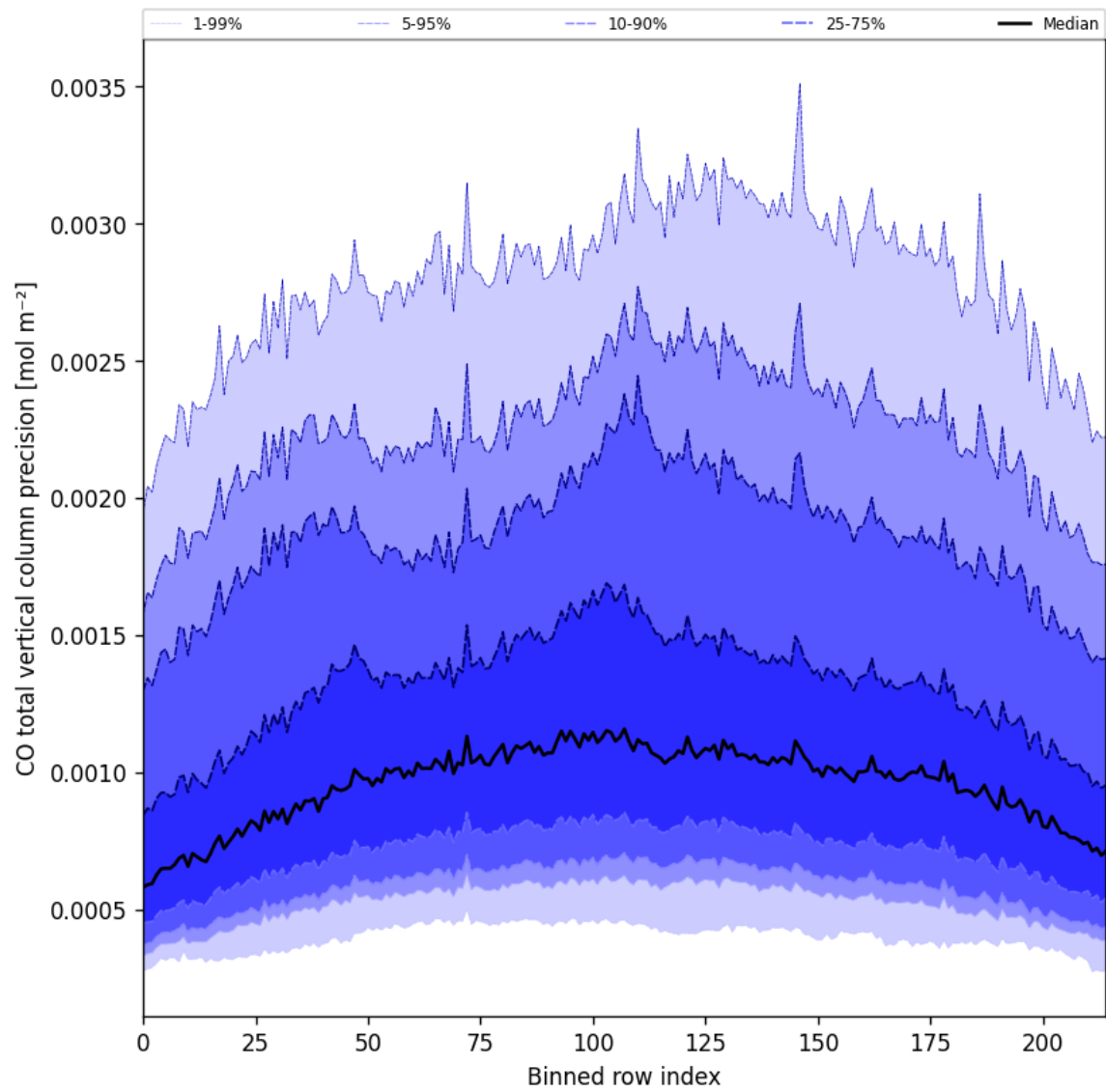
Figure 28: Along track statistics of “CO total vertical column precision” for 2025-04-02 to 2025-04-03
