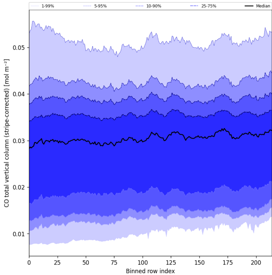
Figure 27: Along track statistics of “CO total vertical column (stripe-corrected)” for 2025-04-02 to 2025-04-03
