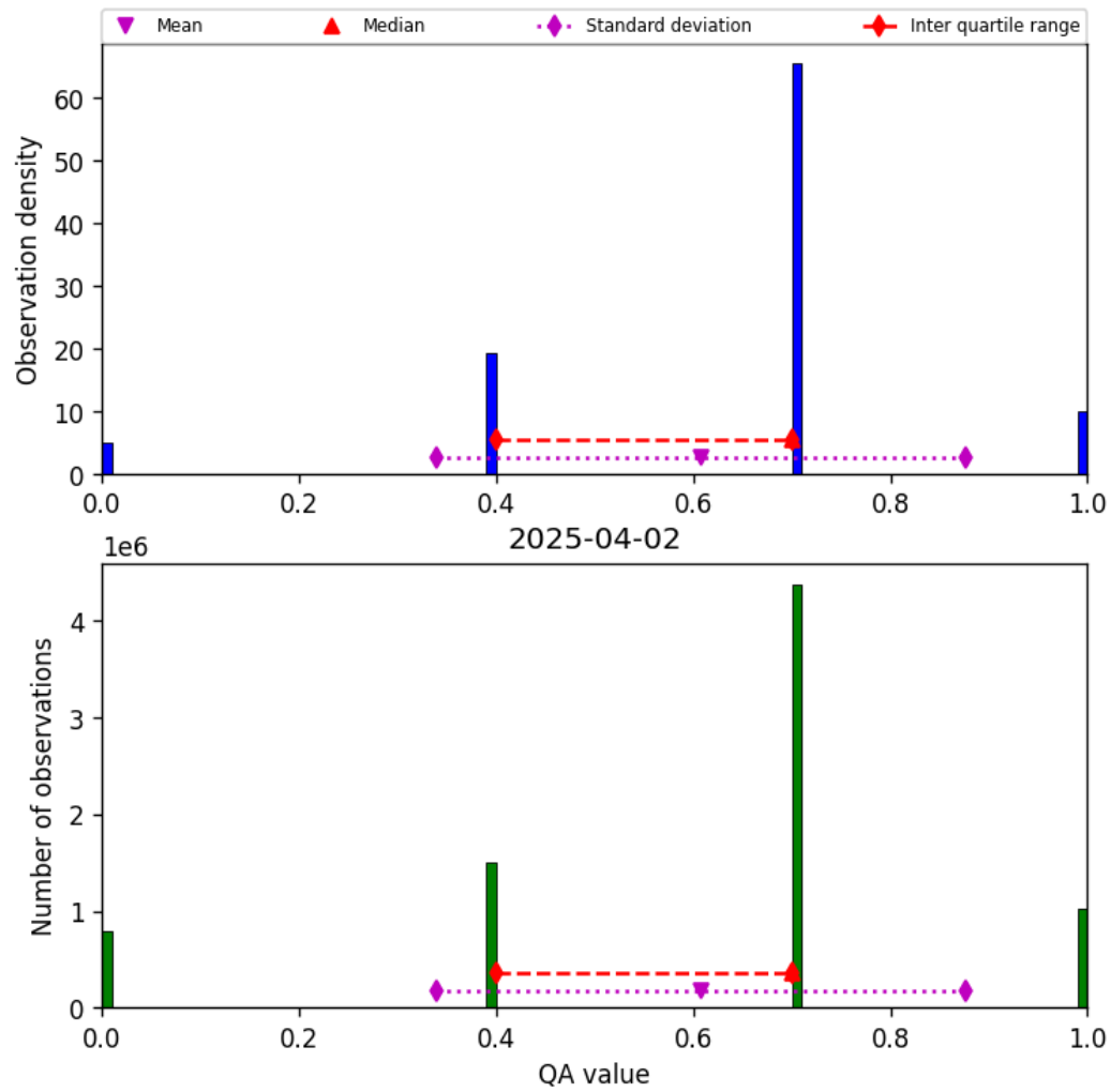
Figure 17: Histogram of “QA value” for 2025-04-02 to 2025-04-03
