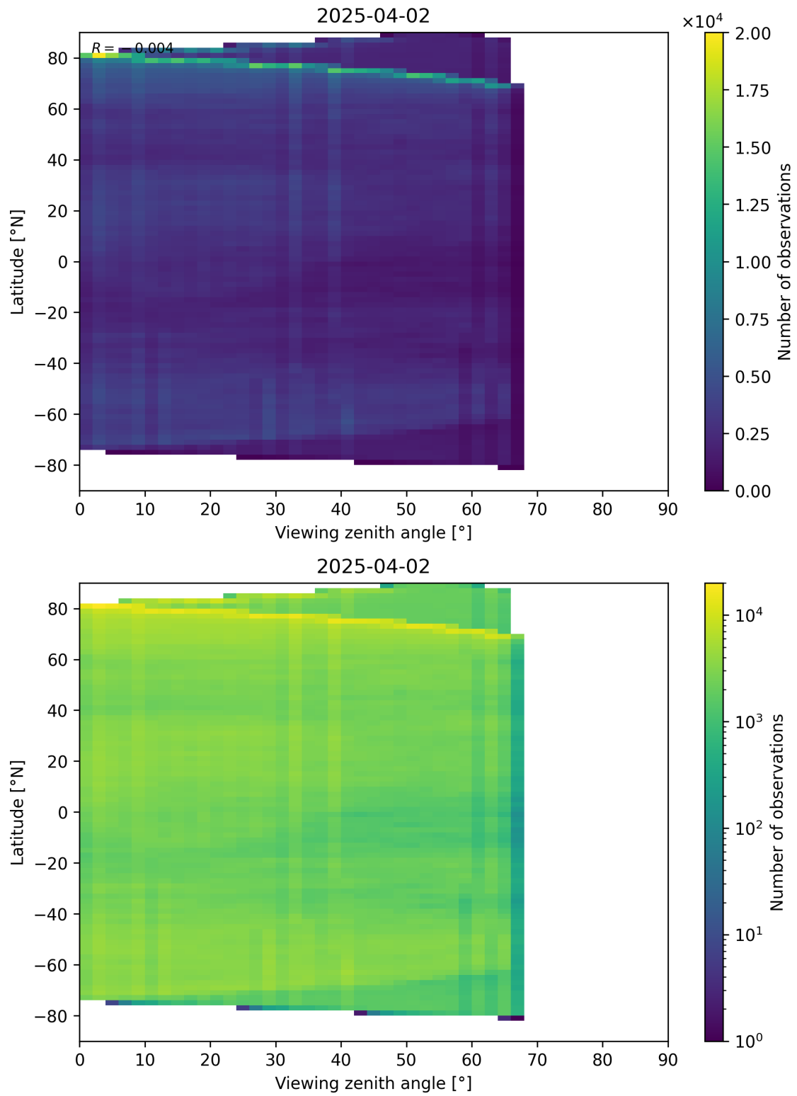
Figure 74: Scatter density plot of “Viewing zenith angle” against “Latitude” for 2025-04-02 to 2025-04-03.
