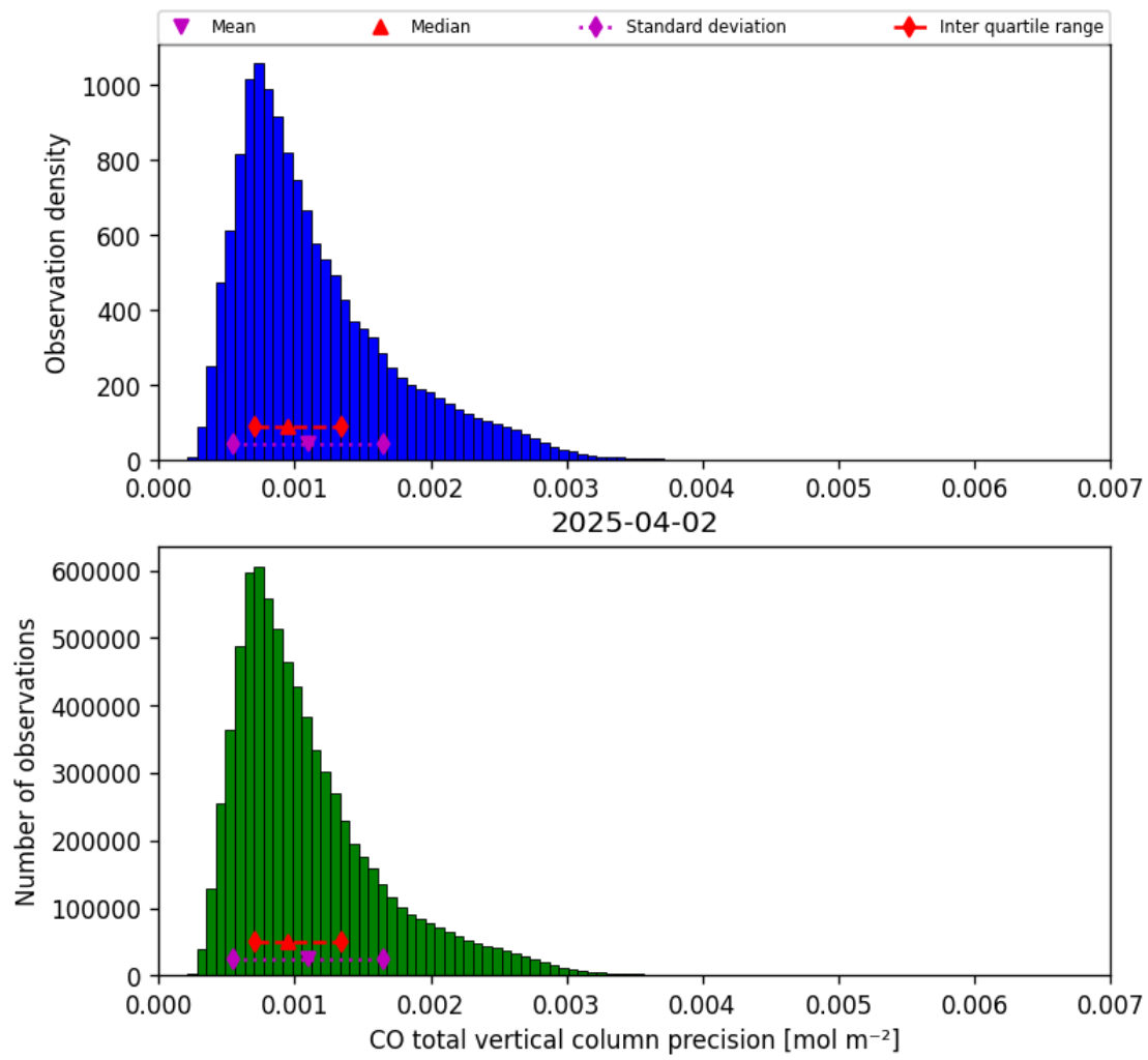
Figure 20: Histogram of “CO total vertical column precision” for 2025-04-02 to 2025-04-03
