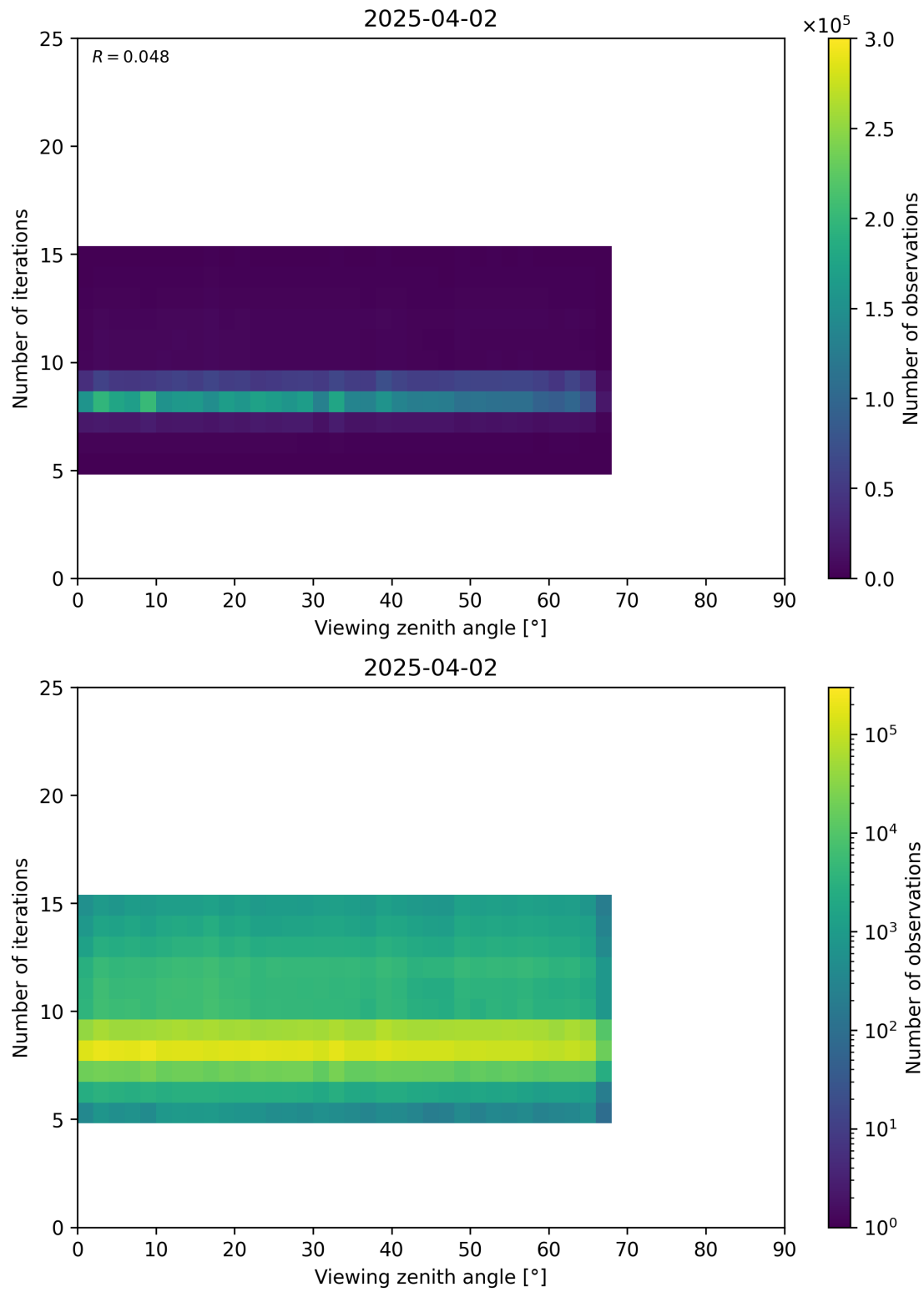
Figure 75: Scatter density plot of “Viewing zenith angle” against “Number of iterations” for 2025-04-02 to 2025-04-03.
