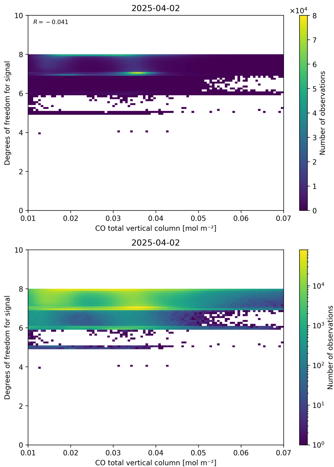
Figure 41: Scatter density plot of “CO total vertical column” against “Degrees of freedom for signal” for 2025-04-02 to 2025-04-03.
