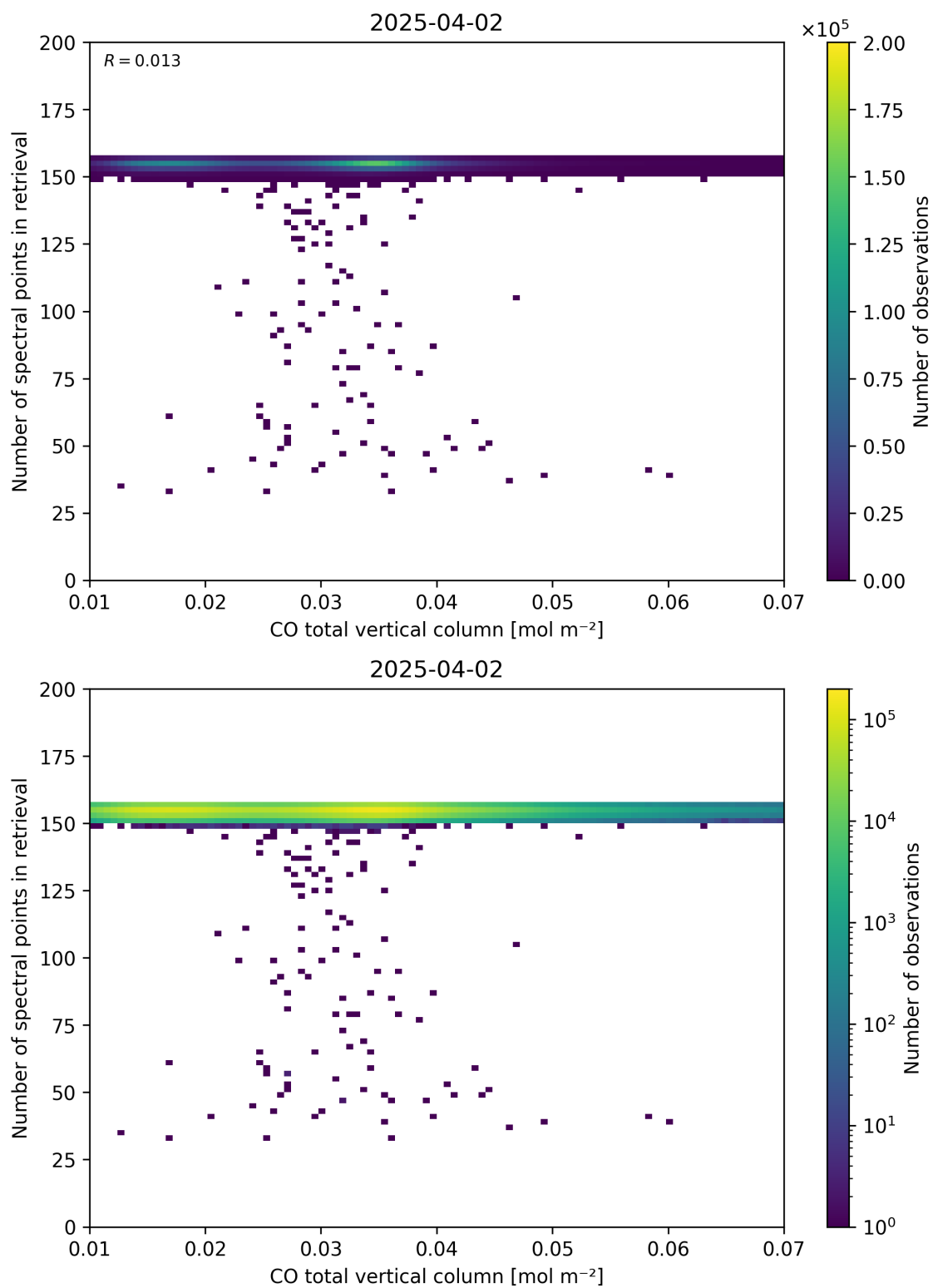
Figure 43: Scatter density plot of “CO total vertical column” against “Number of spectral points in retrieval” for 2025-04-02 to 2025-04-03.
