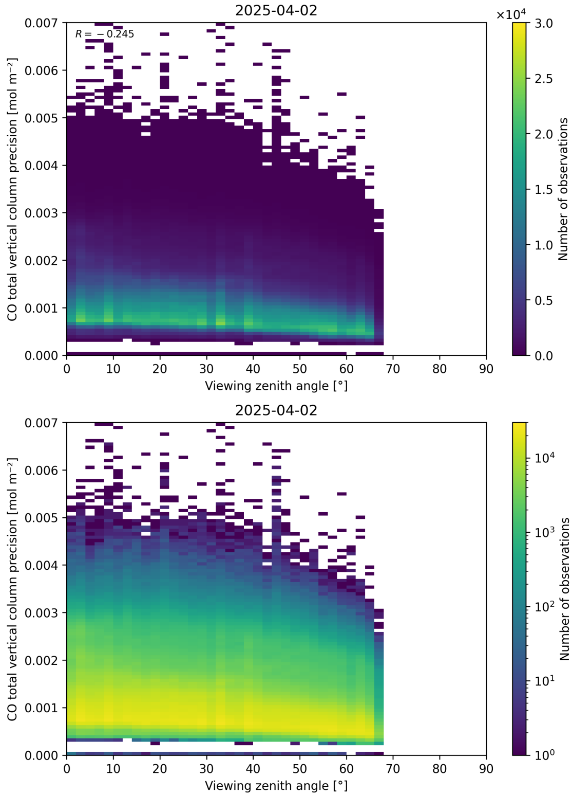
Figure 71: Scatter density plot of “Viewing zenith angle” against “CO total vertical column precision” for 2025-04-02 to 2025-04-03.
