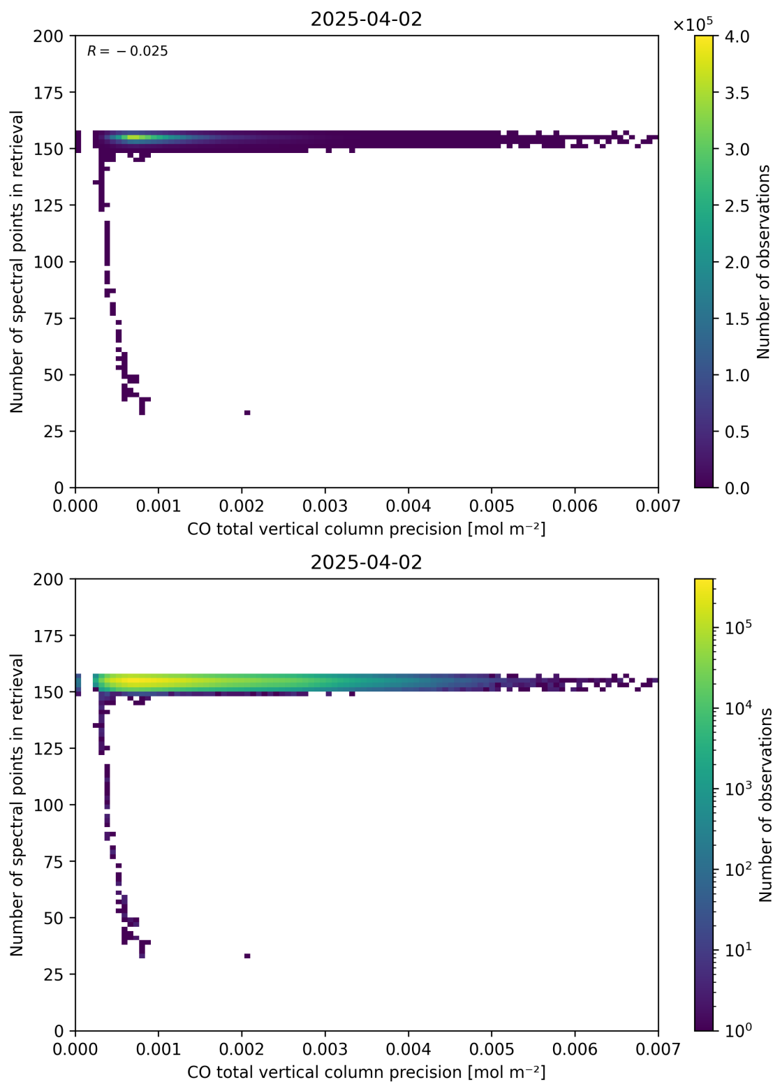
Figure 47: Scatter density plot of “CO total vertical column precision” against “Number of spectral points in retrieval” for 2025-04-02 to 2025-04-03.
