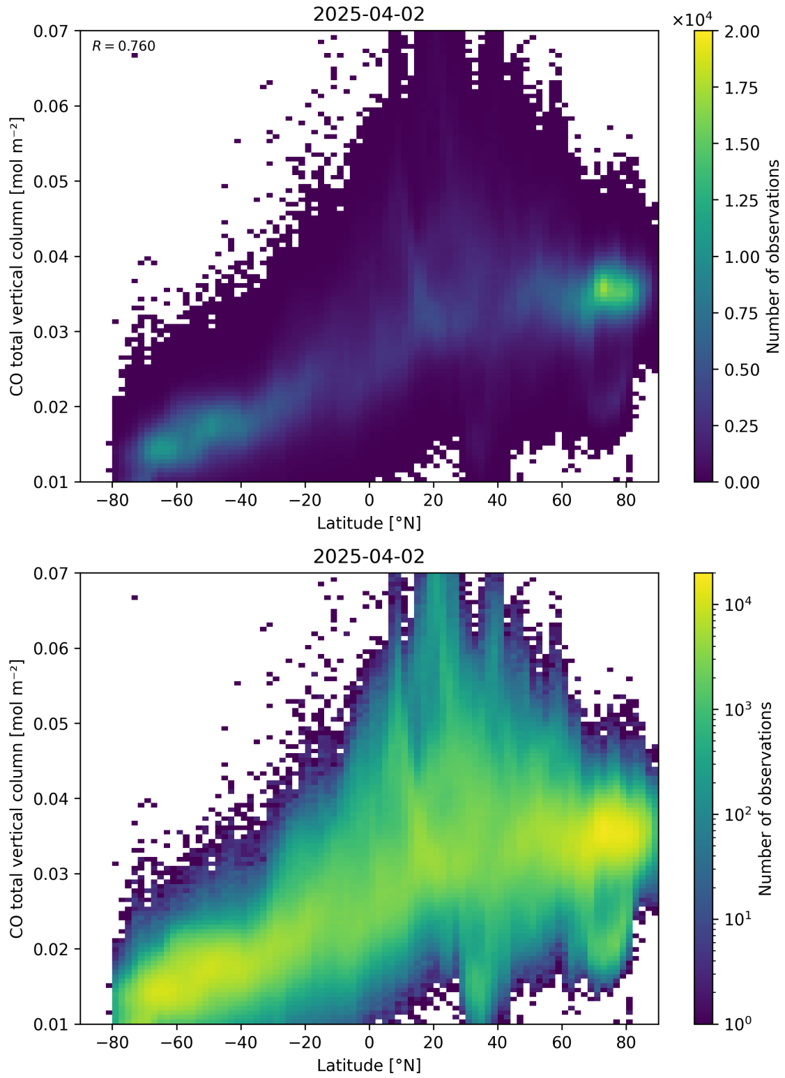
Figure 51: Scatter density plot of “Latitude” against “CO total vertical column” for 2025-04-02 to 2025-04-03.
