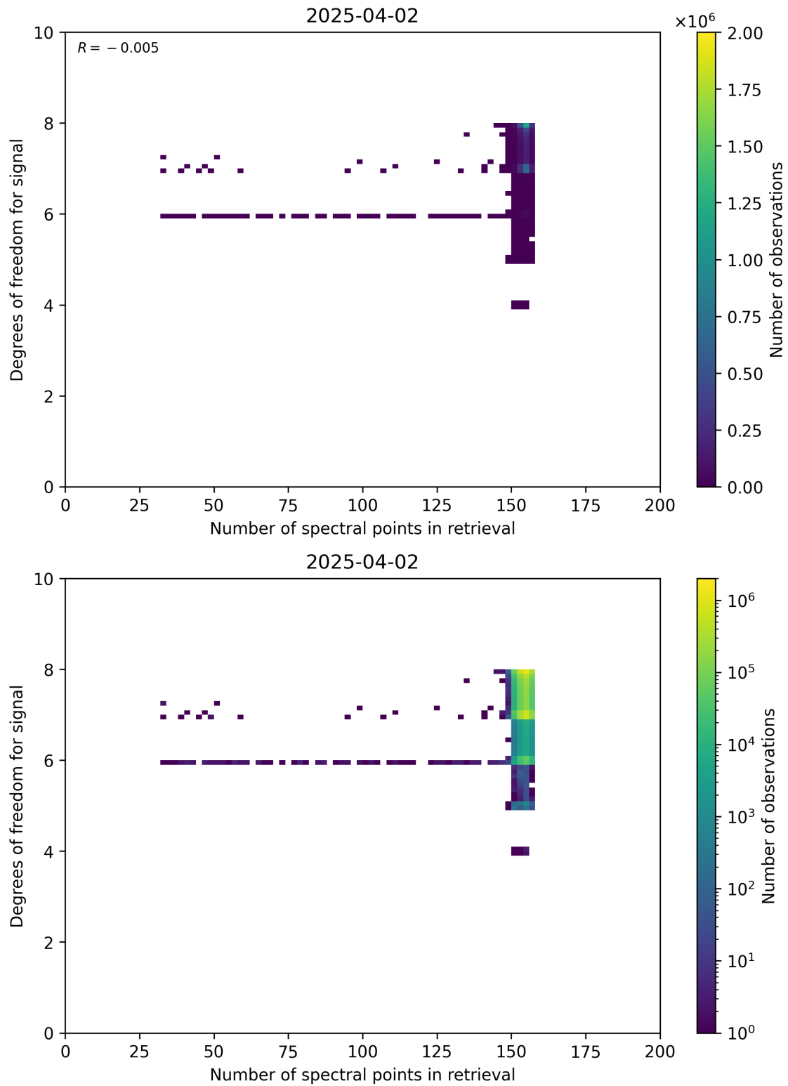
Figure 59: Scatter density plot of “Number of spectral points in retrieval” against “Degrees of freedom for signal” for 2025-04-02 to 2025-04-03.
