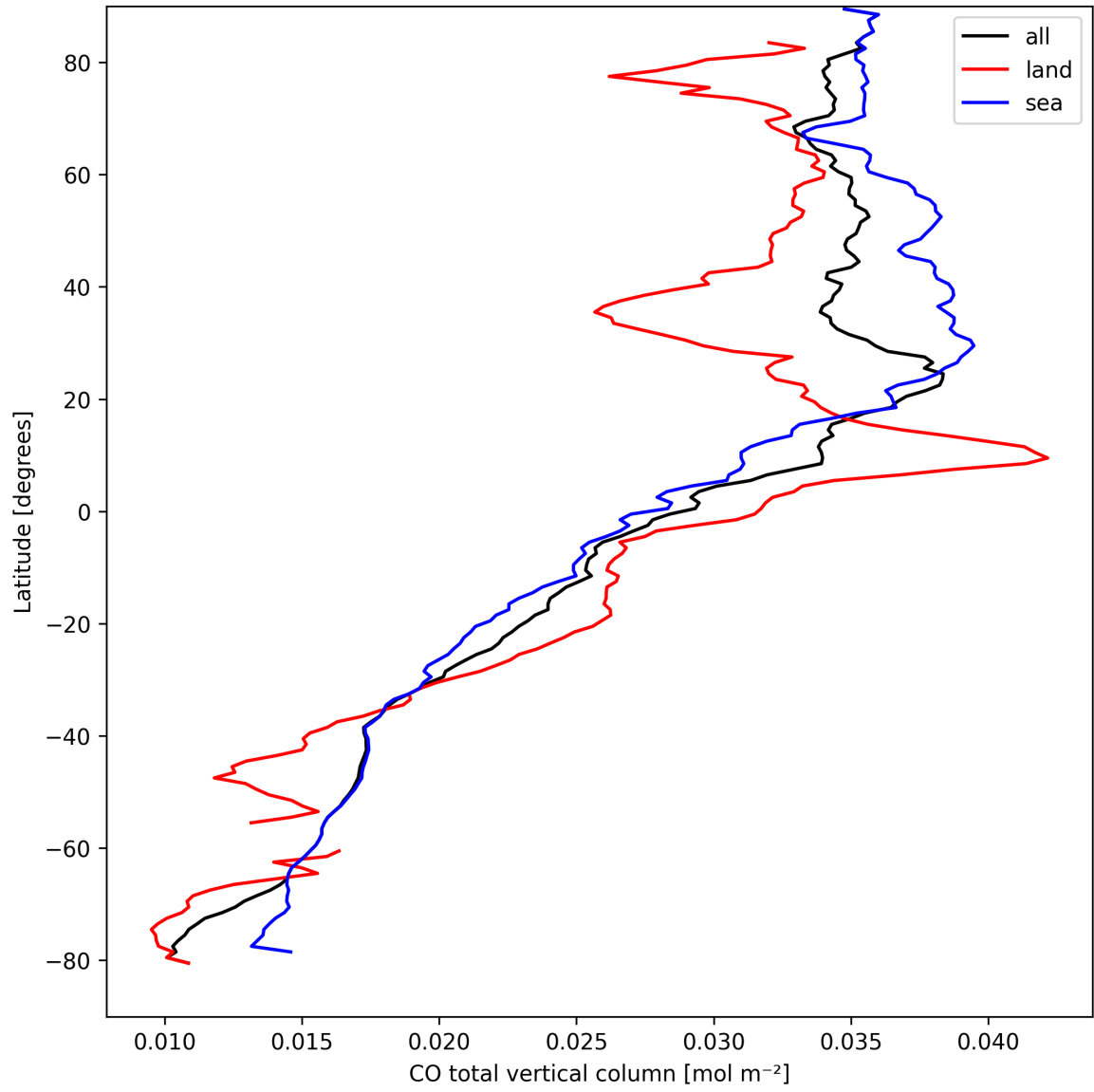
Figure 10: Zonal average of “CO total vertical column” for 2025-04-02 to 2025-04-03.
