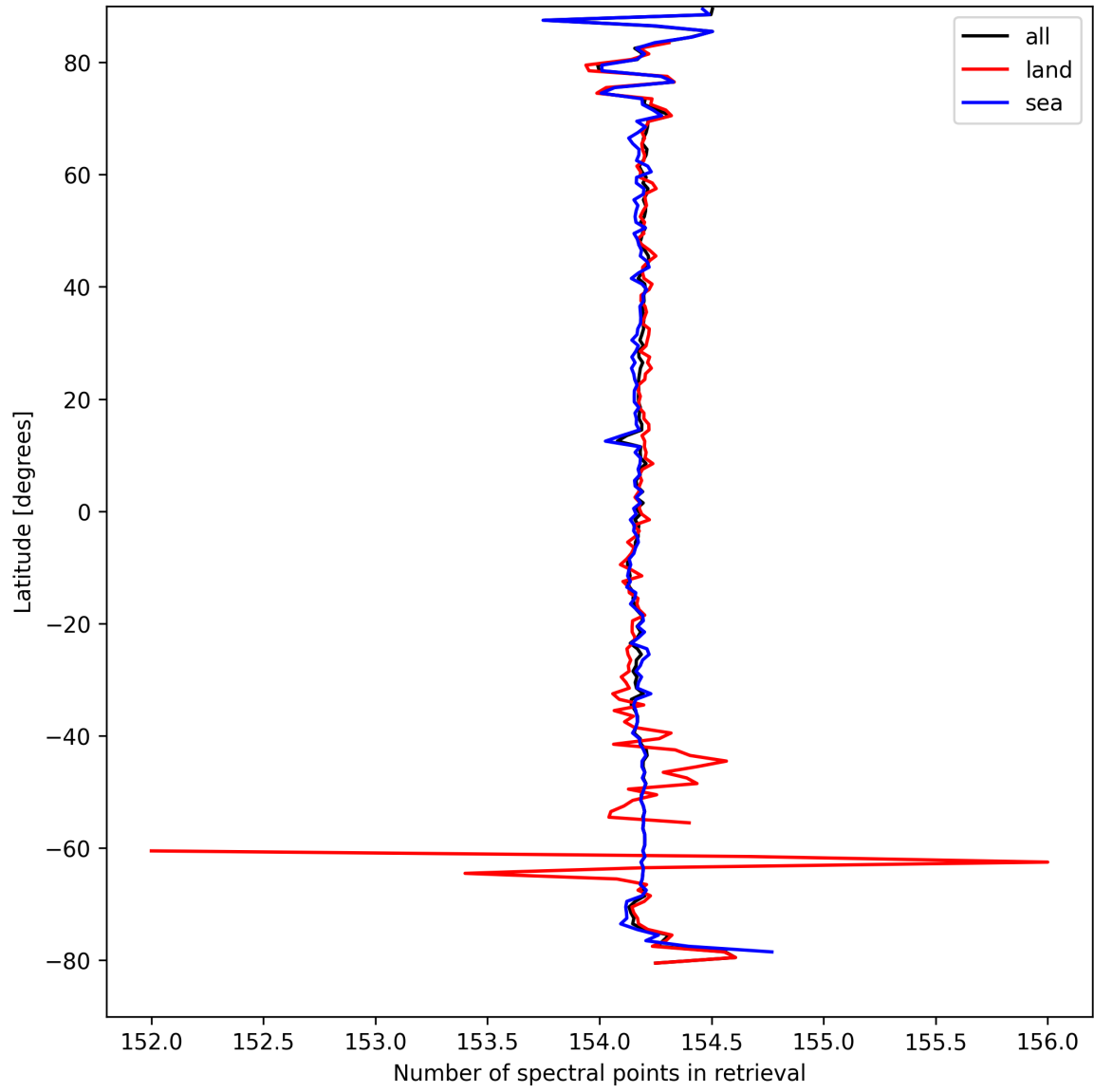
Figure 13: Zonal average of “Number of spectral points in retrieval” for 2025-04-02 to 2025-04-03.
