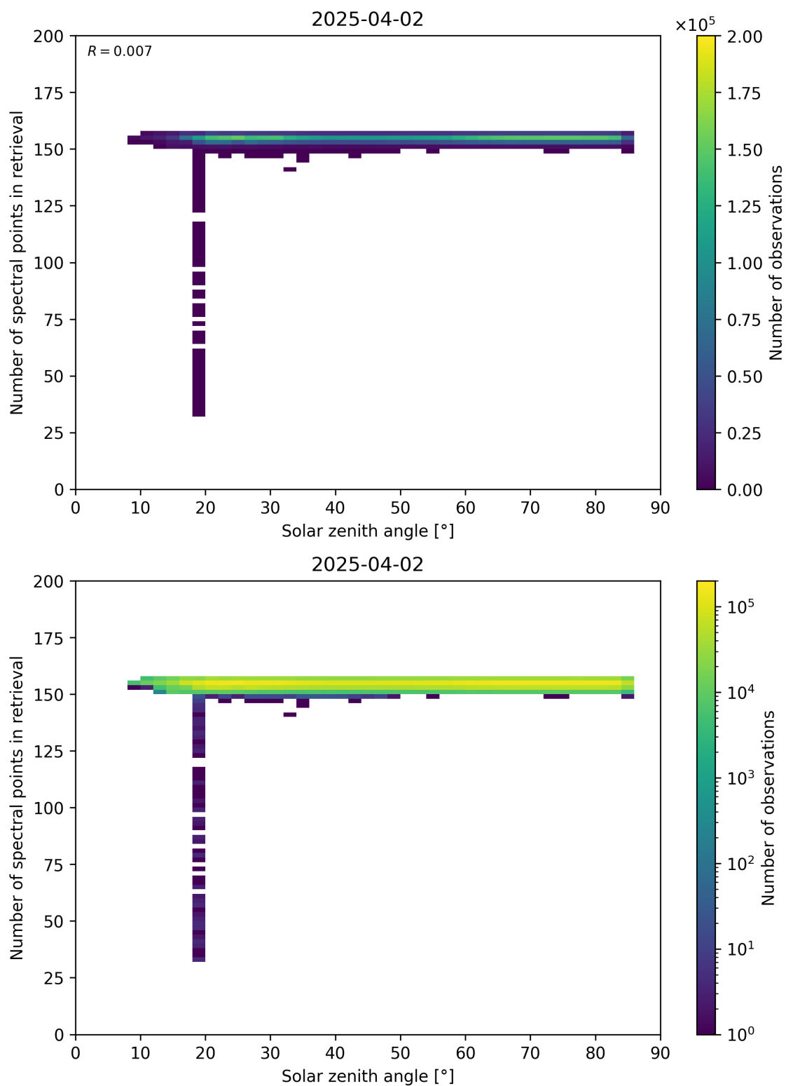
Figure 68: Scatter density plot of “Solar zenith angle” against “Number of spectral points in retrieval” for 2025-04-02 to 2025-04-03.
