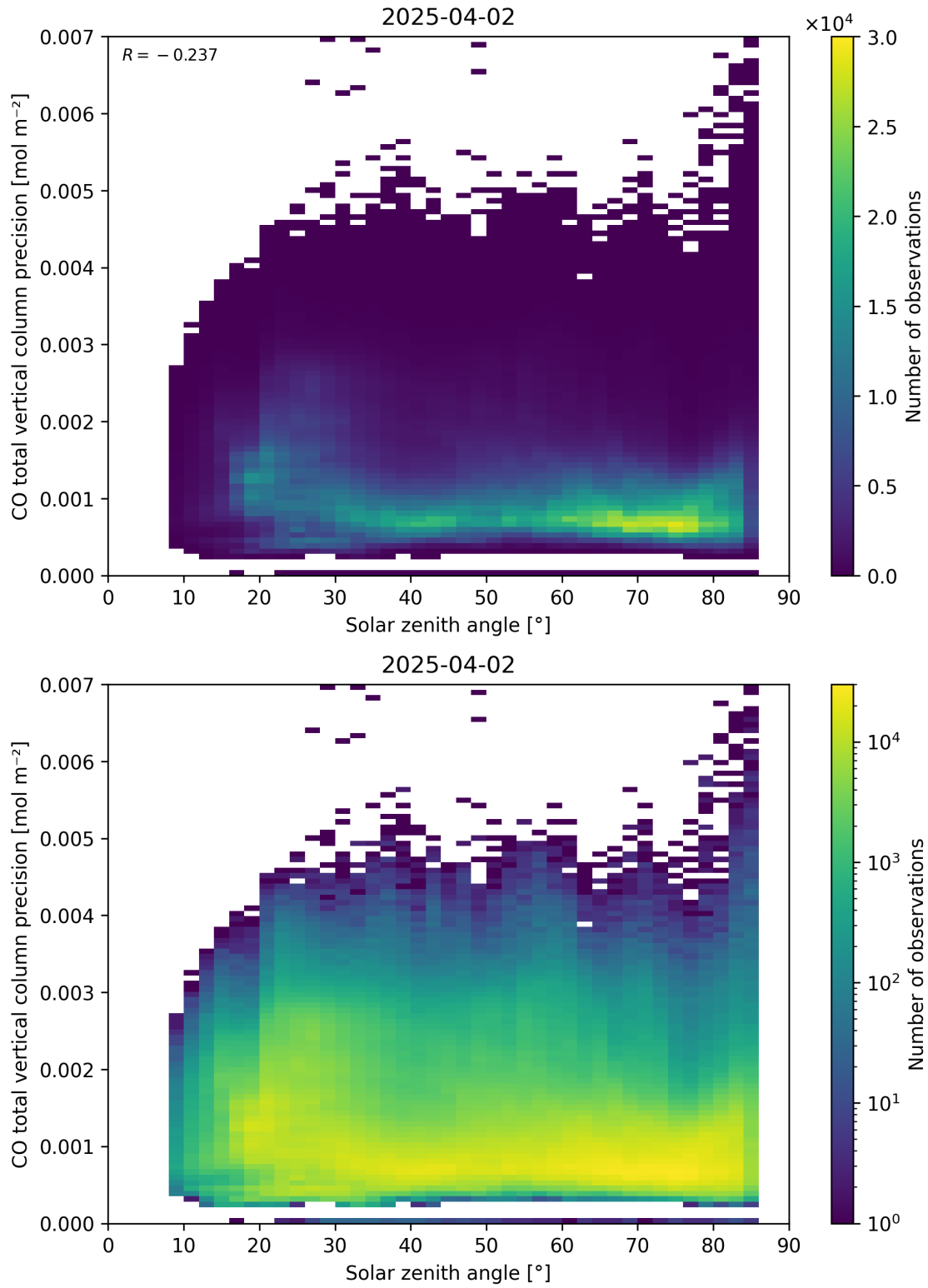
Figure 63: Scatter density plot of “Solar zenith angle” against “CO total vertical column precision” for 2025-04-02 to 2025-04-03.
