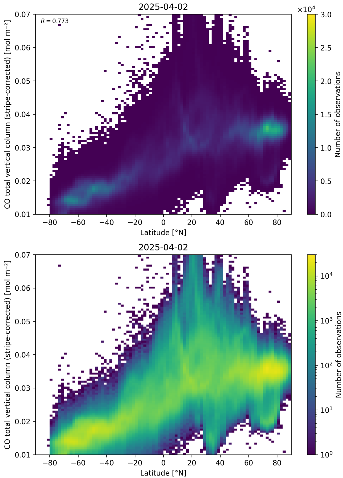
Figure 52: Scatter density plot of “Latitude” against “CO total vertical column (stripe-corrected)” for 2025-04-02 to 2025-04-03.
