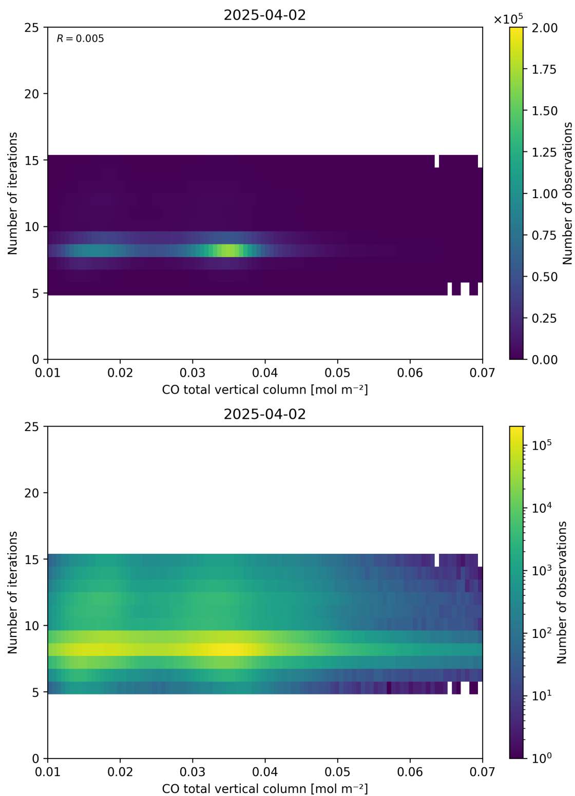
Figure 42: Scatter density plot of “CO total vertical column” against “Number of iterations” for 2025-04-02 to 2025-04-03.
