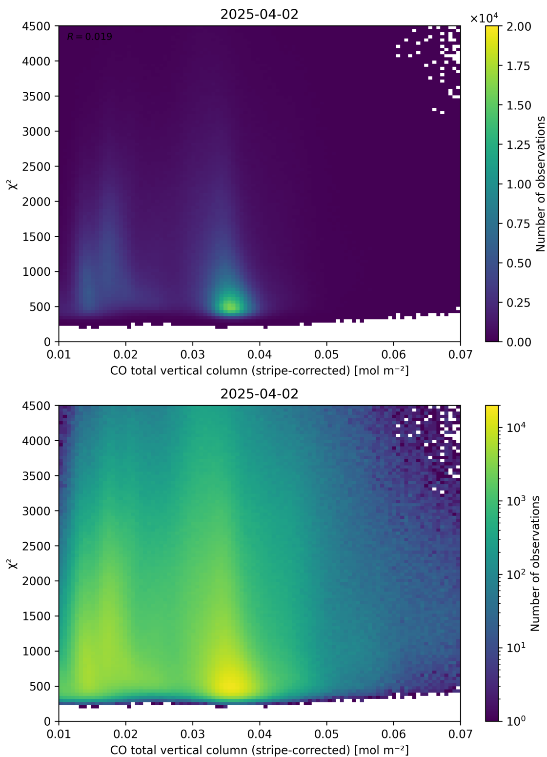
Figure 37: Scatter density plot of “CO total vertical column (stripe-corrected)” against “ \chi^2 ” for 2025-04-02 to 2025-04-03.
