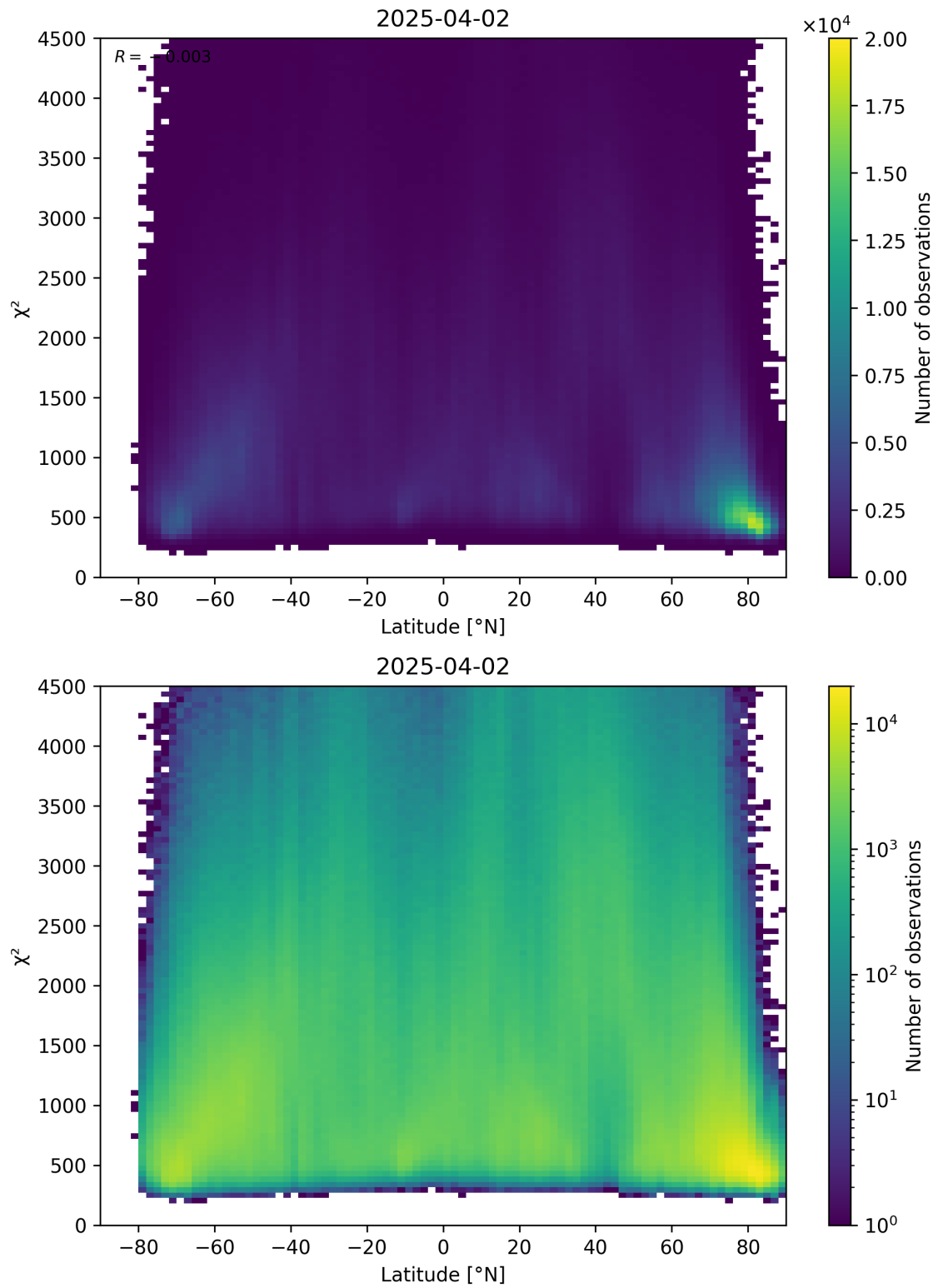
Figure 54: Scatter density plot of “Latitude” against “ \chi^2 ” for 2025-04-02 to 2025-04-03.
