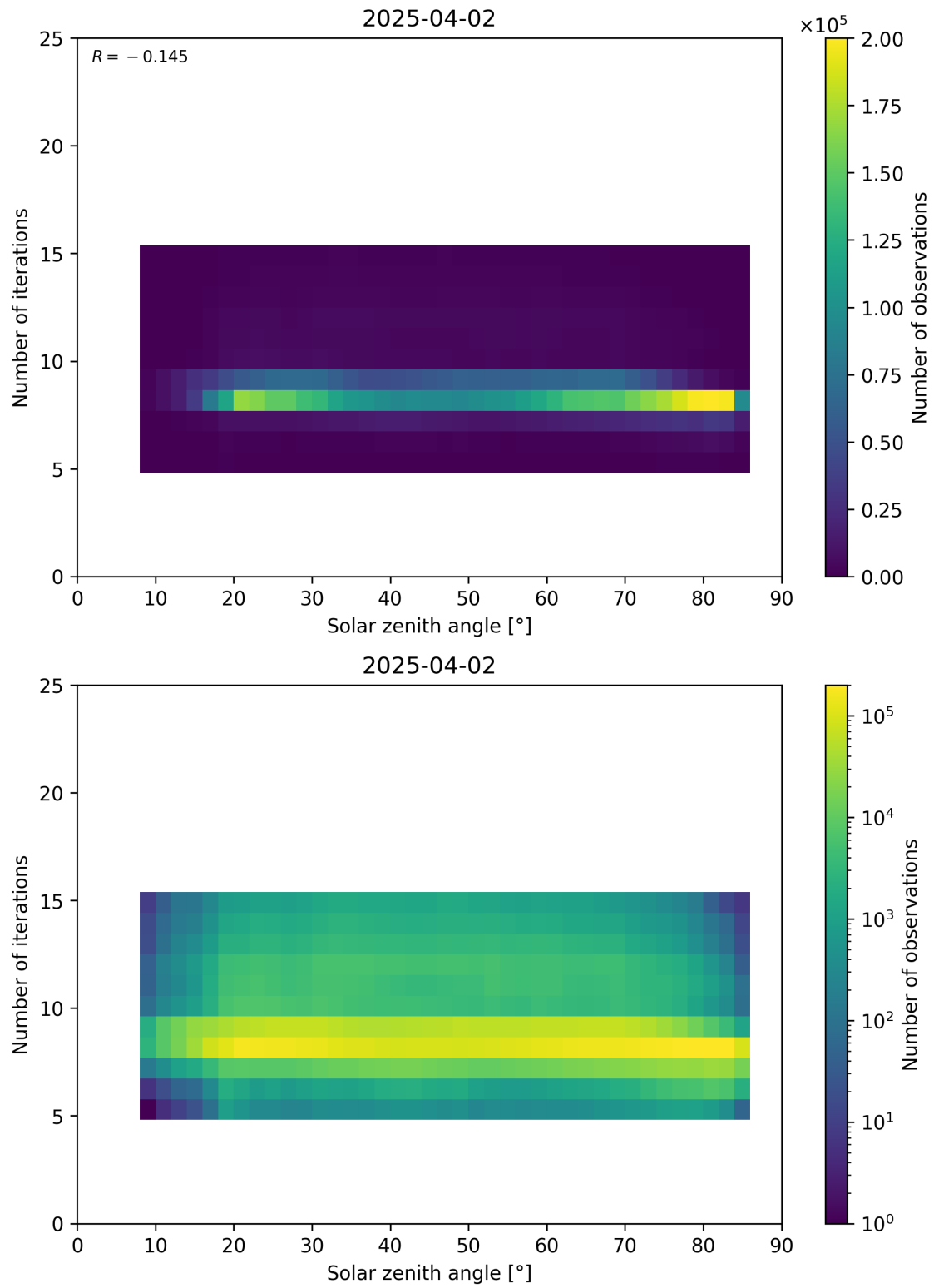
Figure 67: Scatter density plot of “Solar zenith angle” against “Number of iterations” for 2025-04-02 to 2025-04-03.
