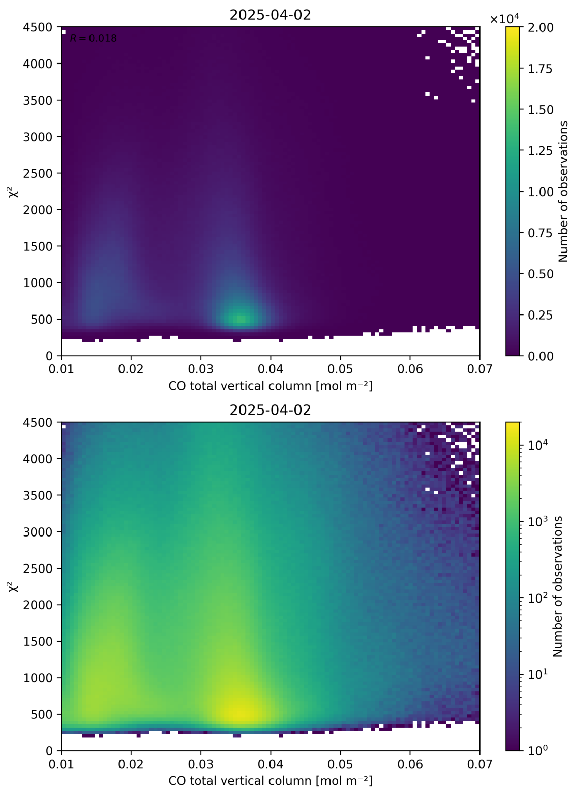
Figure 35: Scatter density plot of “CO total vertical column” against “ \chi^2 ” for 2025-04-02 to 2025-04-03.
