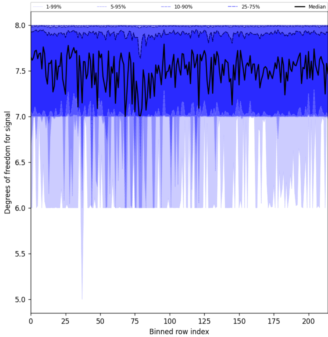
Figure 31: Along track statistics of “Degrees of freedom for signal” for 2025-04-02 to 2025-04-03
