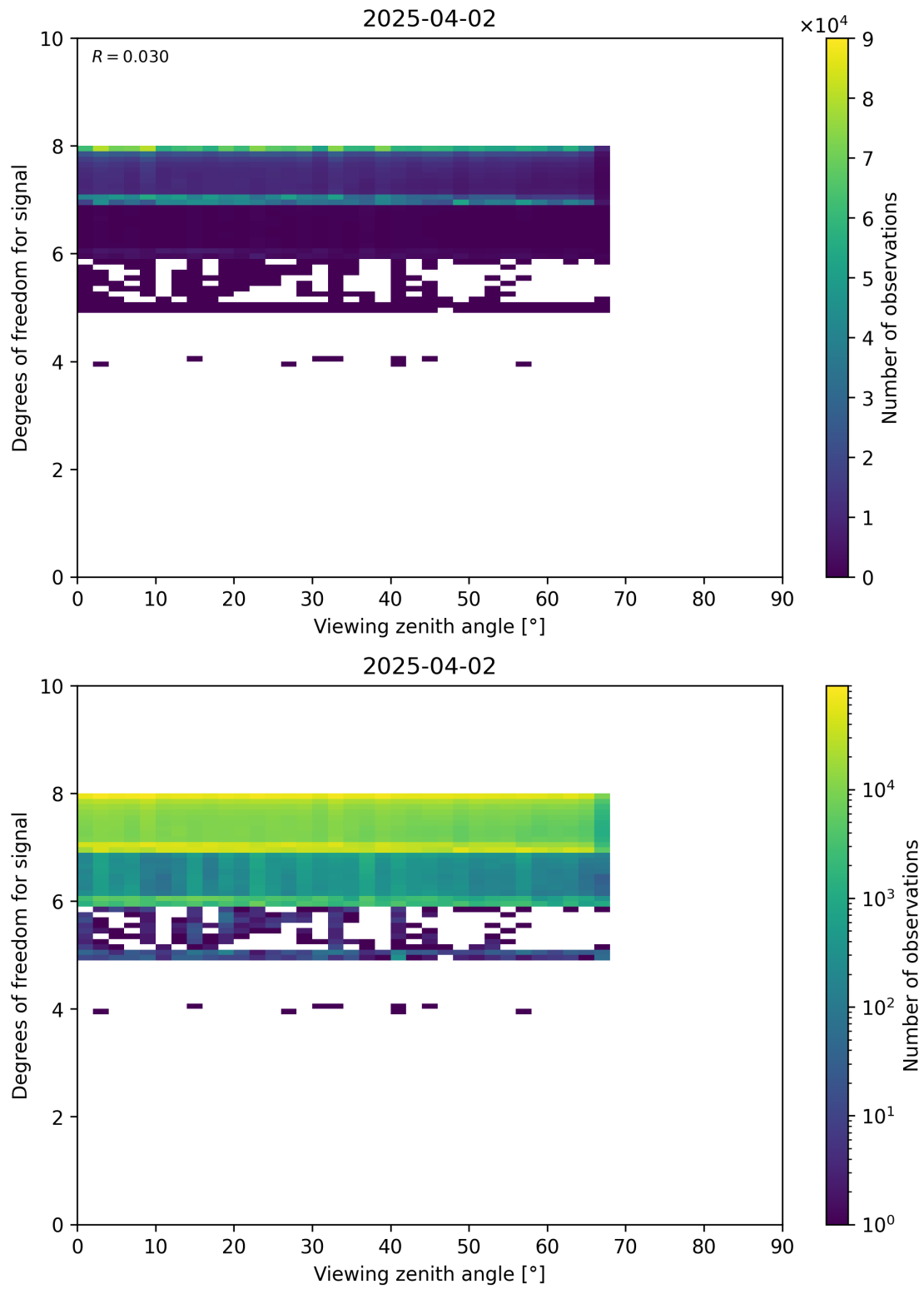
Figure 73: Scatter density plot of “Viewing zenith angle” against “Degrees of freedom for signal” for 2025-04-02 to 2025-04-03.
