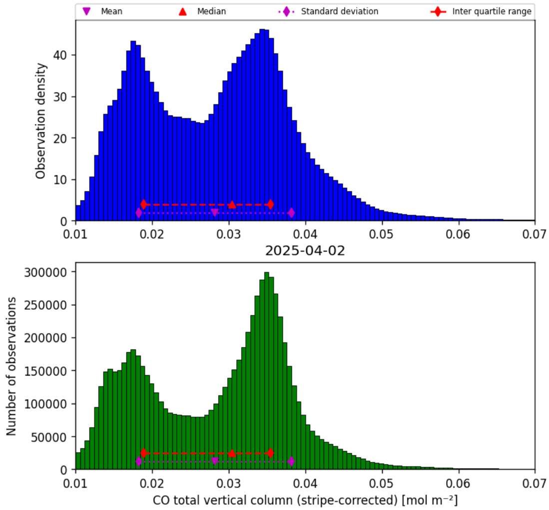
Figure 19: Histogram of “CO total vertical column (stripe-corrected)” for 2025-04-02 to 2025-04-03
