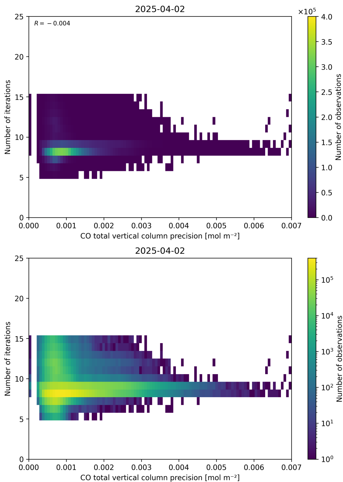
Figure 46: Scatter density plot of “CO total vertical column precision” against “Number of iterations” for 2025-04-02 to 2025-04-03.
