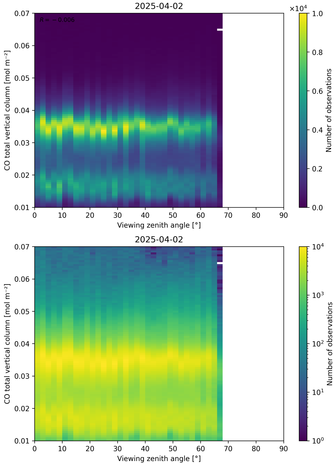
Figure 69: Scatter density plot of “Viewing zenith angle” against “CO total vertical column” for 2025-04-02 to 2025-04-03.
