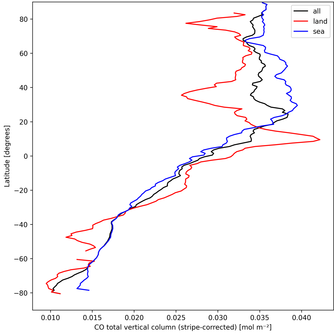
Figure 11: Zonal average of “CO total vertical column (stripe-corrected)” for 2025-04-02 to 2025-04-03.
