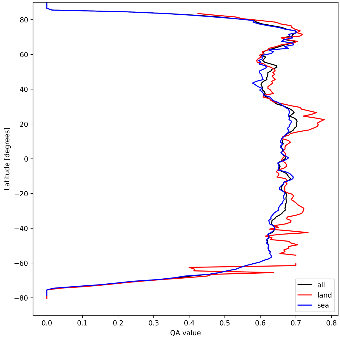
Figure 9: Zonal average of “QA value” for 2025-04-02 to 2025-04-03.
