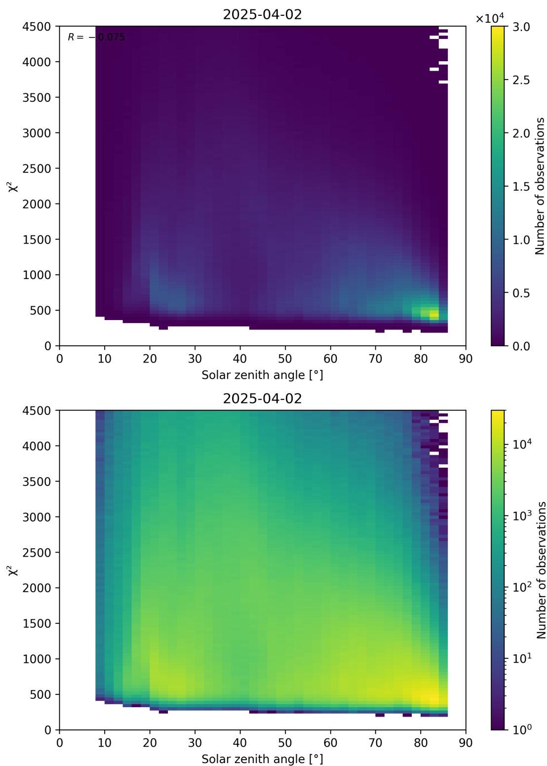
Figure 64: Scatter density plot of “Solar zenith angle” against “ \chi^2 ” for 2025-04-02 to 2025-04-03.
