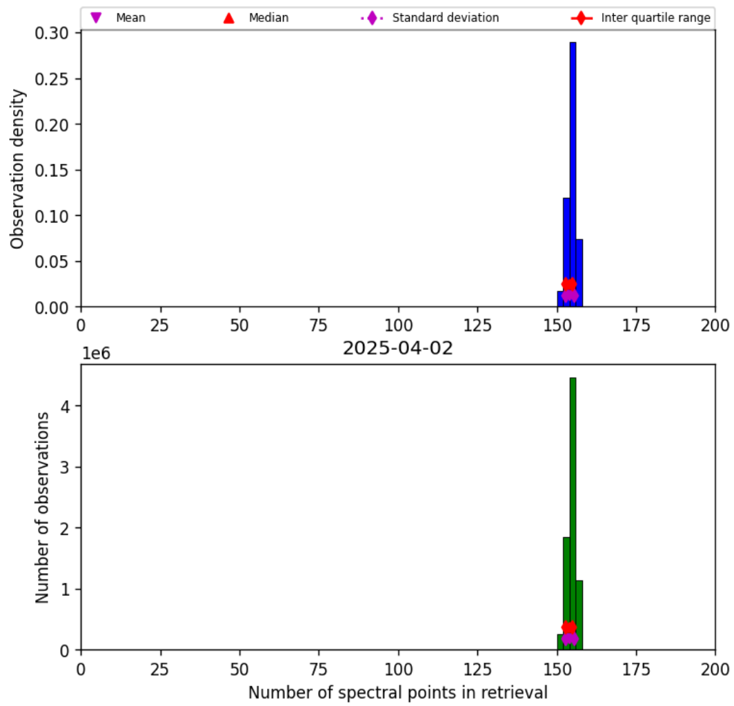
Figure 21: Histogram of “Number of spectral points in retrieval” for 2025-04-02 to 2025-04-03
