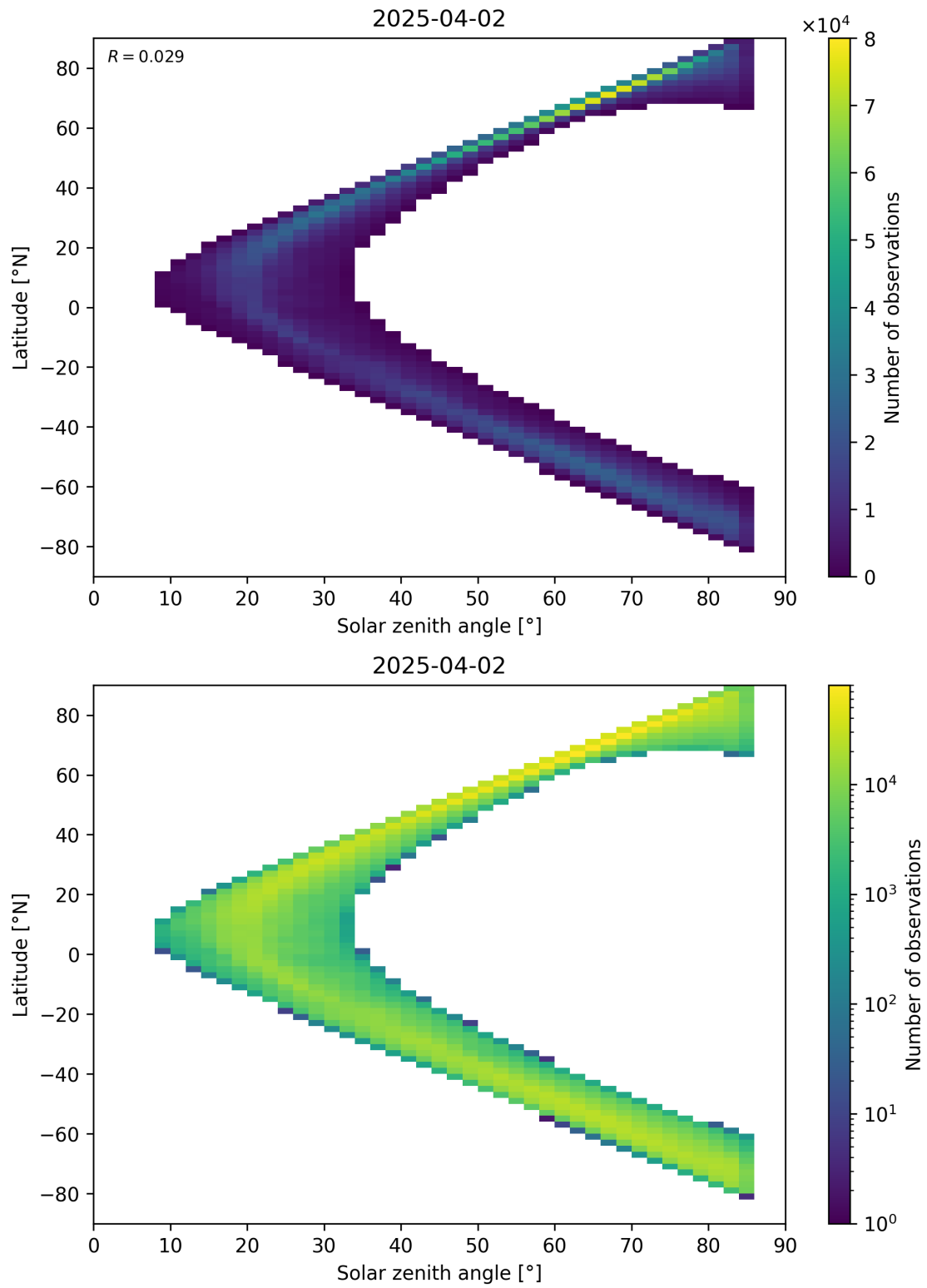
Figure 66: Scatter density plot of “Solar zenith angle” against “Latitude” for 2025-04-02 to 2025-04-03.
