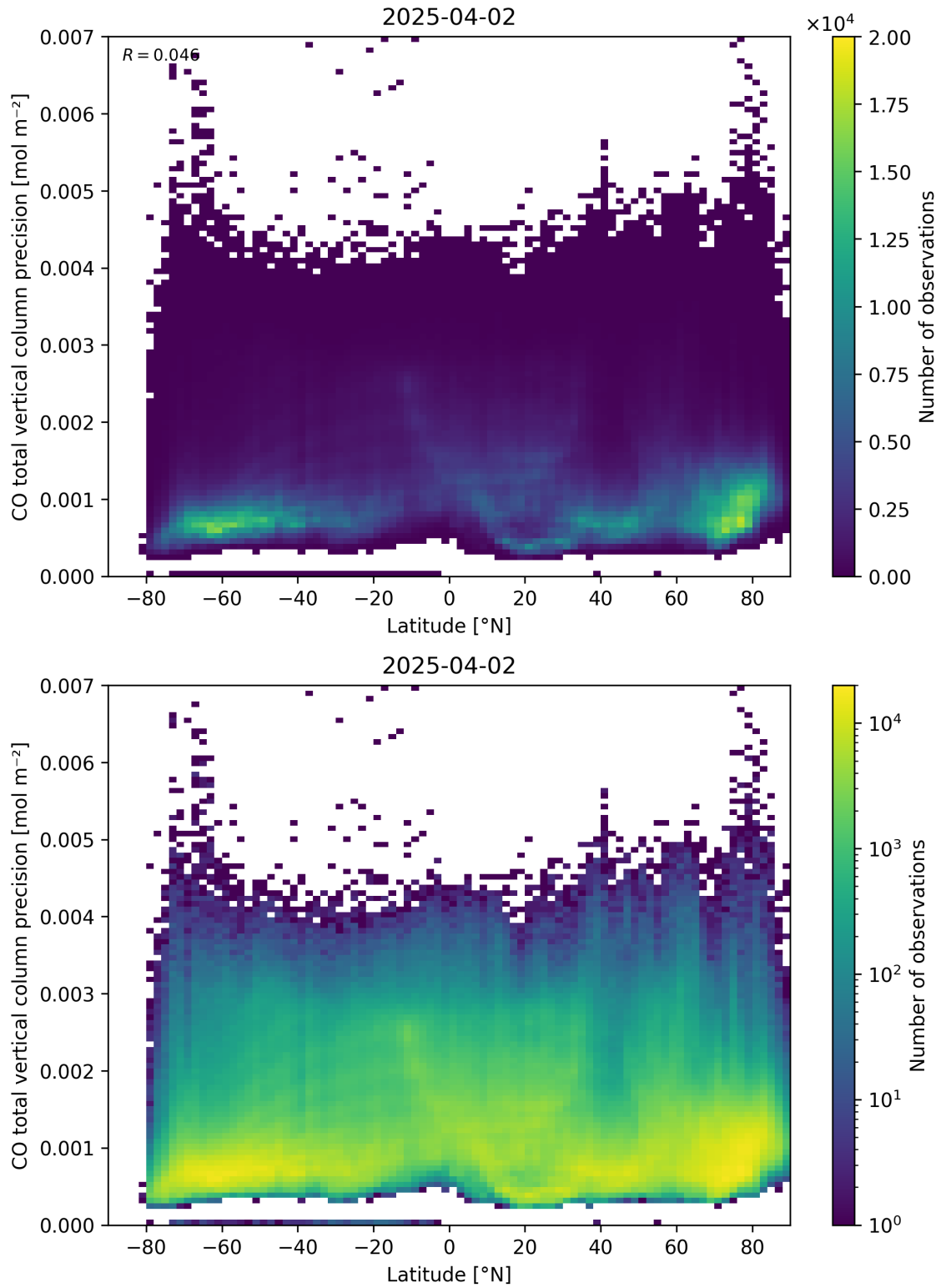
Figure 53: Scatter density plot of “Latitude” against “CO total vertical column precision” for 2025-04-02 to 2025-04-03.
