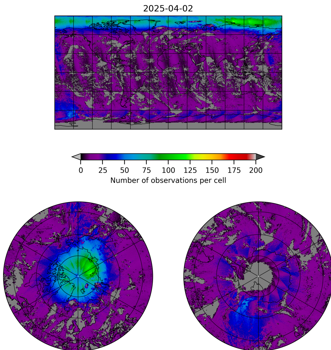
Figure 8: Map of the number of observations for 2025-04-02 to 2025-04-03
