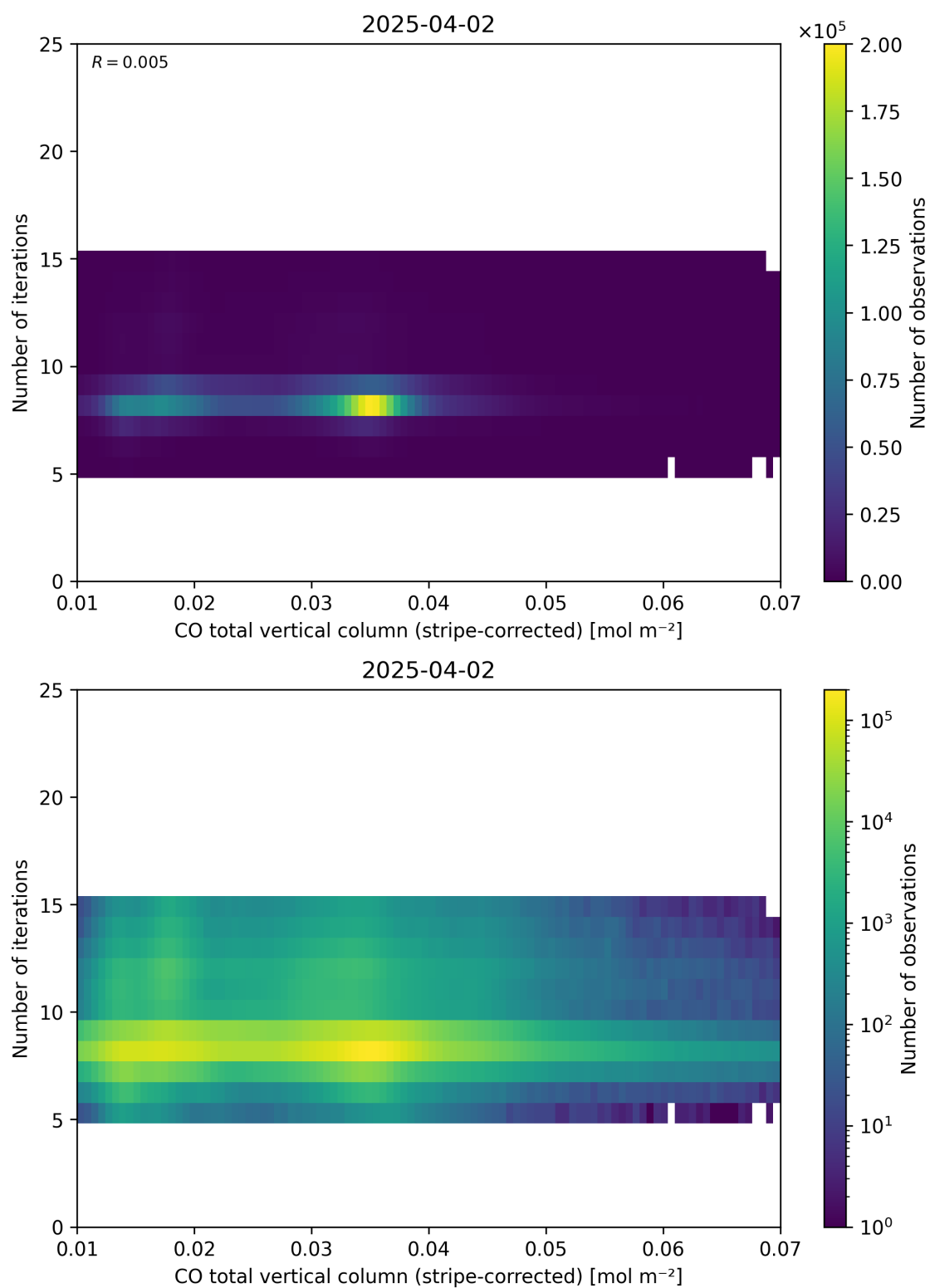
Figure 39: Scatter density plot of “CO total vertical column (stripe-corrected)” against “Number of iterations” for 2025-04-02 to 2025-04-03.
