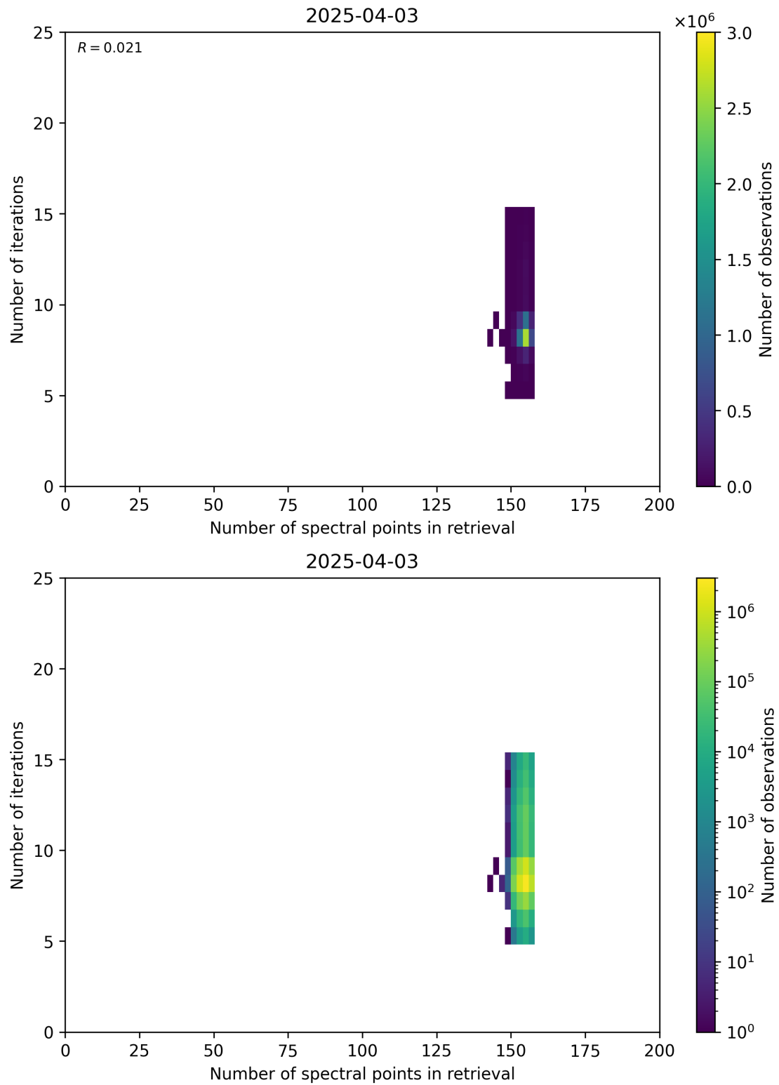
Figure 60: Scatter density plot of “Number of spectral points in retrieval” against “Number of iterations” for 2025-04-03 to 2025-04-04.
