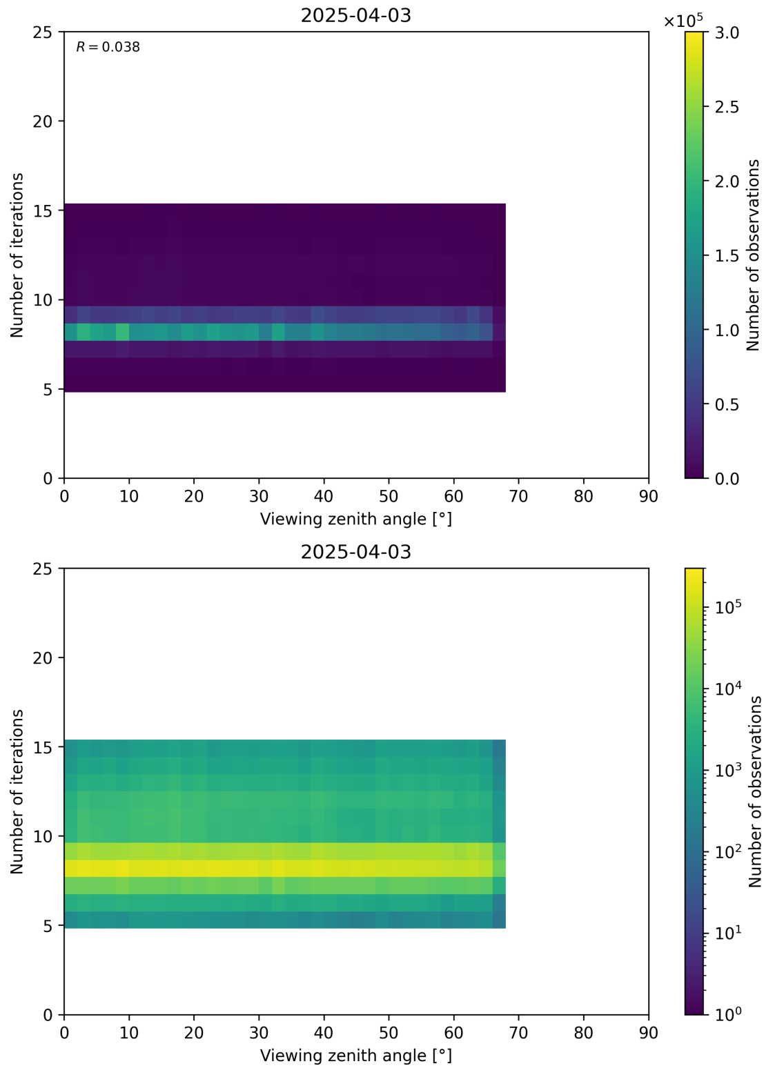
Figure 75: Scatter density plot of “Viewing zenith angle” against “Number of iterations” for 2025-04-03 to 2025-04-04.
