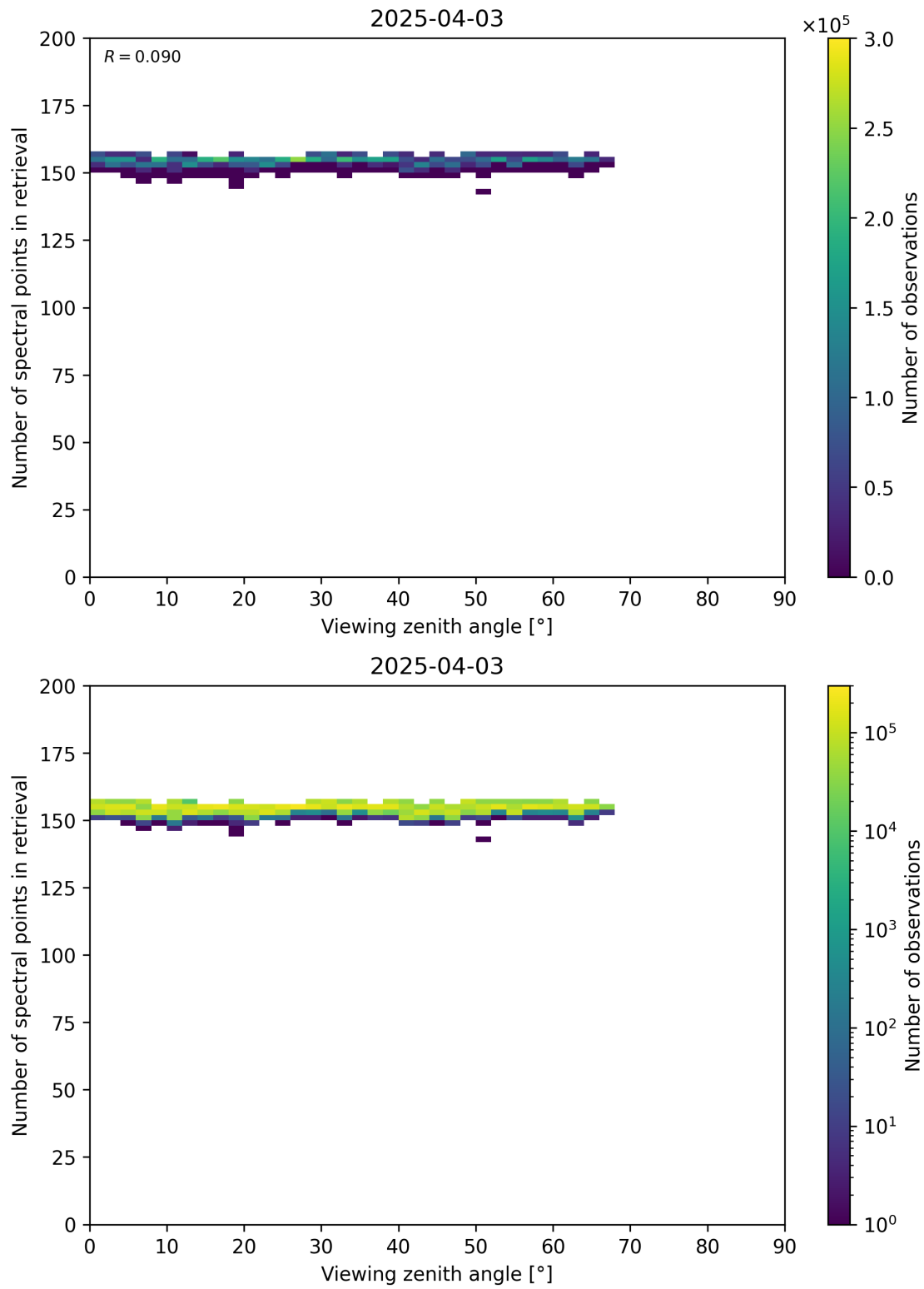
Figure 76: Scatter density plot of “Viewing zenith angle” against “Number of spectral points in retrieval” for 2025-04-03 to 2025-04-04.
