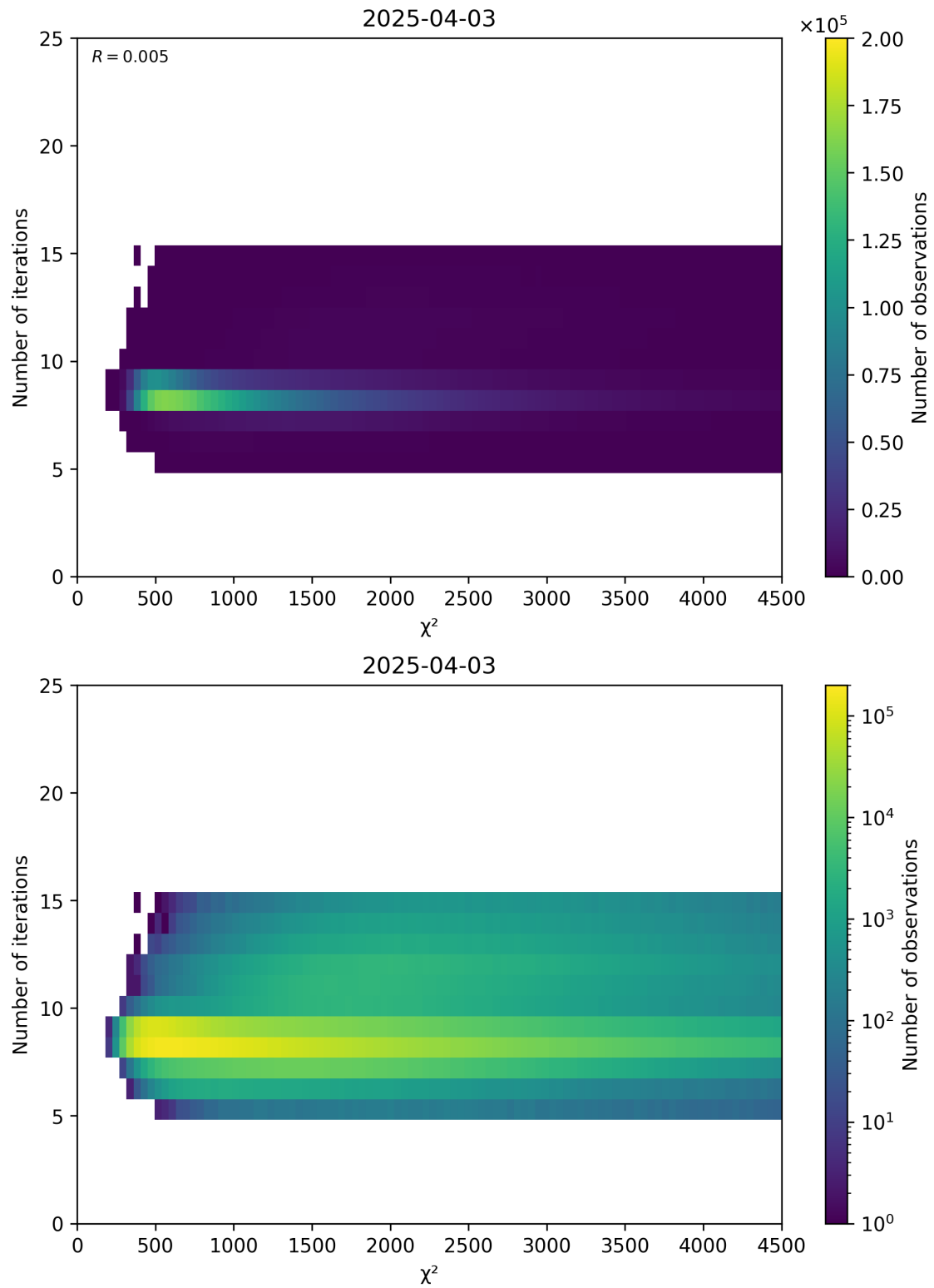
Figure 49: Scatter density plot of “ \chi^2 ” against “Number of iterations” for 2025-04-03 to 2025-04-04.
