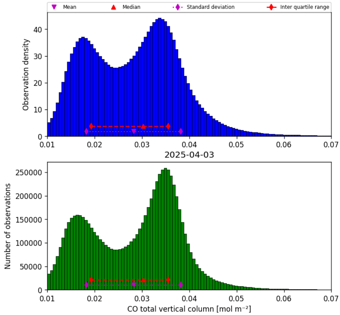
Figure 18: Histogram of “CO total vertical column” for 2025-04-03 to 2025-04-04
