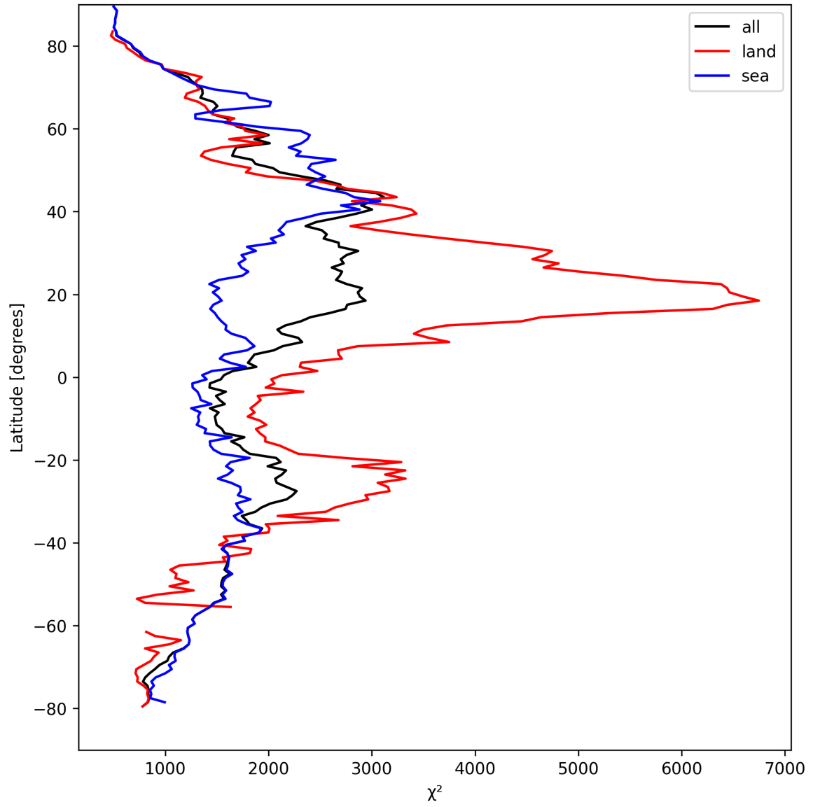
Figure 14: Zonal average of “ \chi^2 ” for 2025-04-03 to 2025-04-04.
