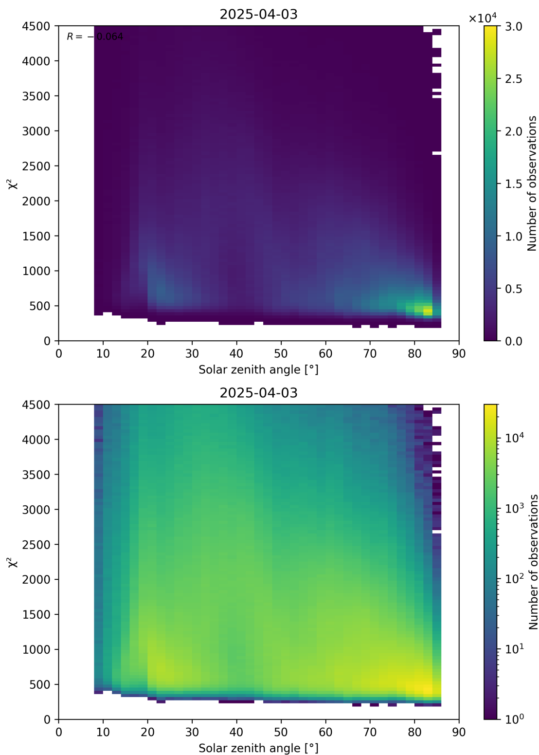
Figure 64: Scatter density plot of “Solar zenith angle” against “ \chi^2 ” for 2025-04-03 to 2025-04-04.
