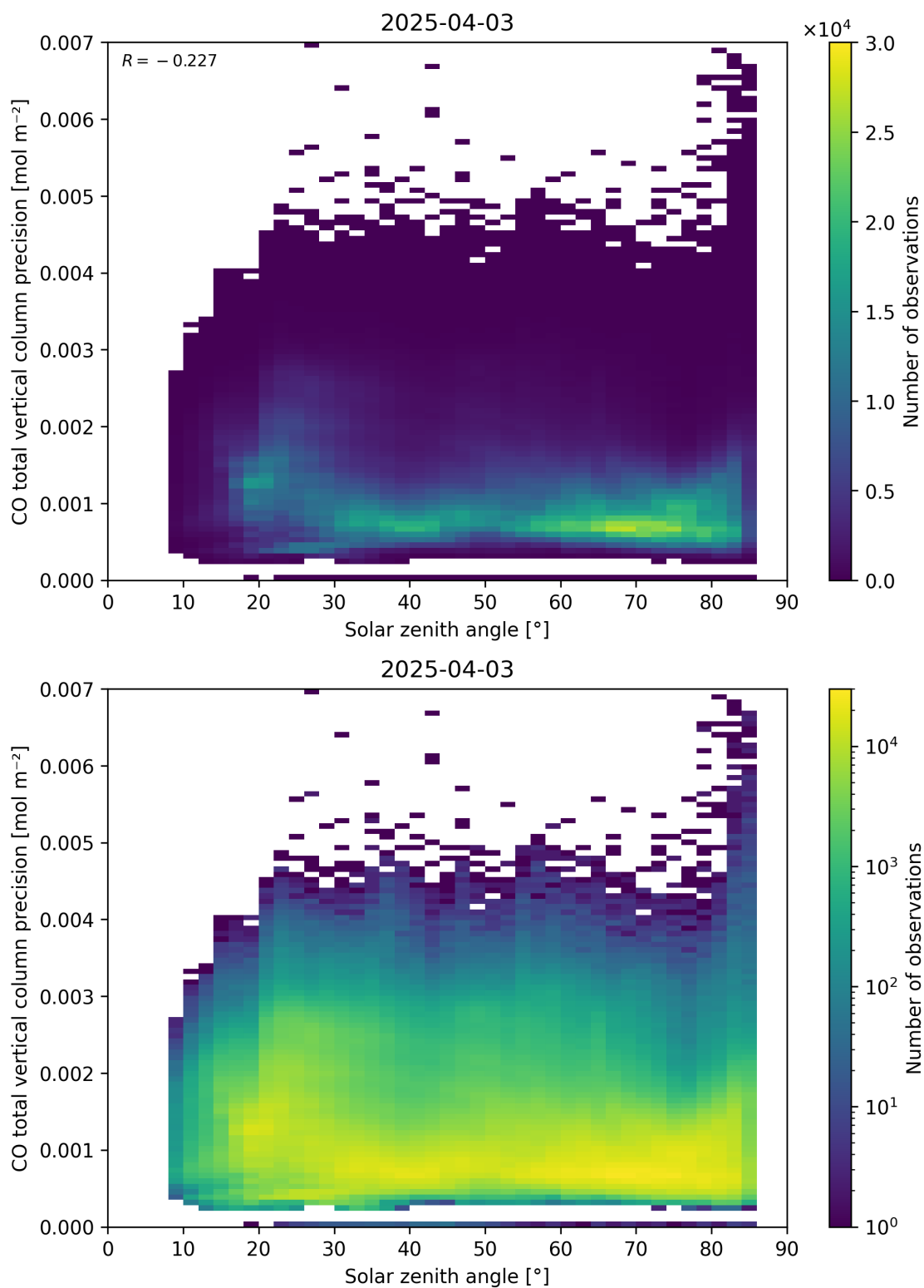
Figure 63: Scatter density plot of “Solar zenith angle” against “CO total vertical column precision” for 2025-04-03 to 2025-04-04.
