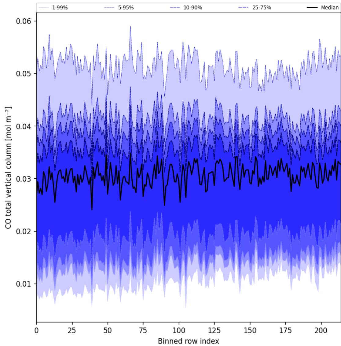
Figure 26: Along track statistics of “CO total vertical column” for 2025-04-03 to 2025-04-04
