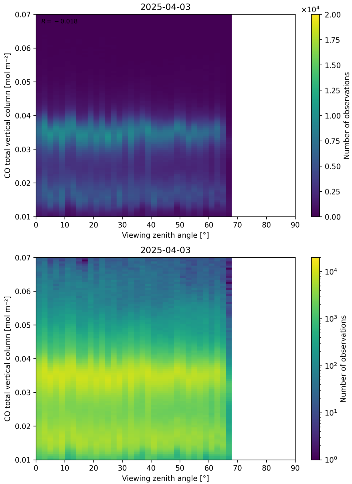
Figure 69: Scatter density plot of “Viewing zenith angle” against “CO total vertical column” for 2025-04-03 to 2025-04-04.
