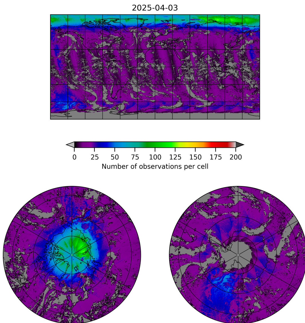
Figure 8: Map of the number of observations for 2025-04-03 to 2025-04-04
