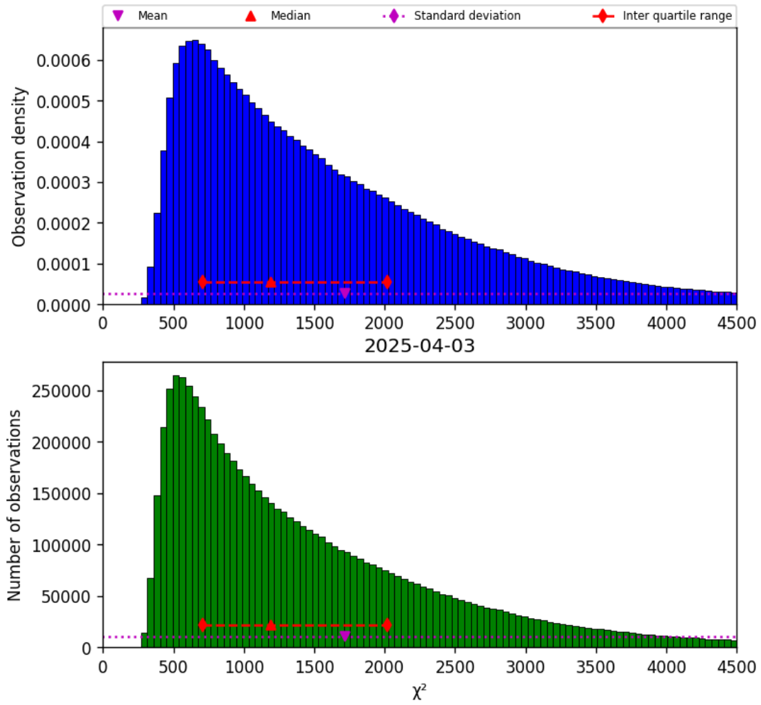
Figure 22: Histogram of “ \chi^2 ” for 2025-04-03 to 2025-04-04
