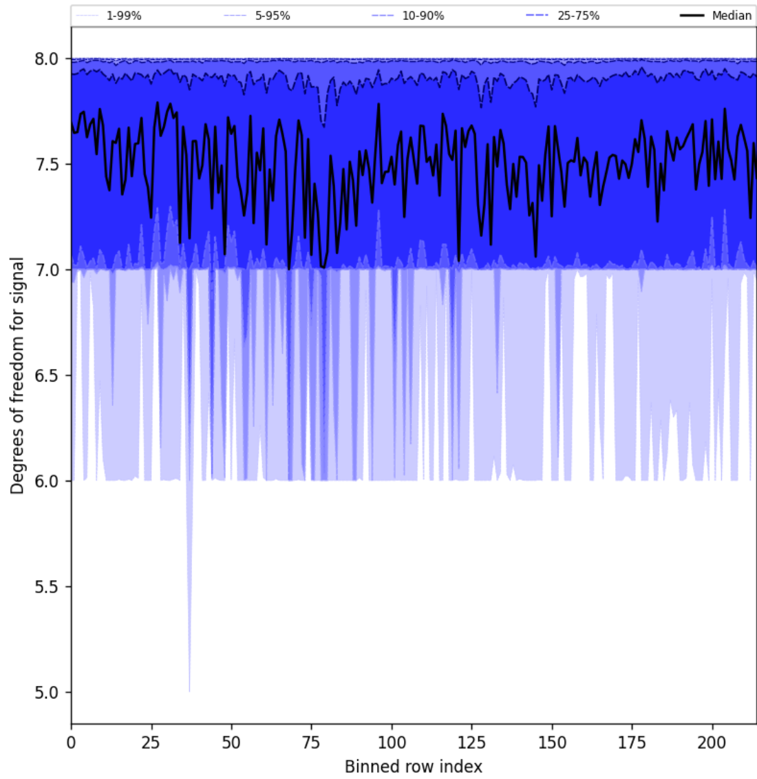
Figure 31: Along track statistics of “Degrees of freedom for signal” for 2025-04-03 to 2025-04-04
