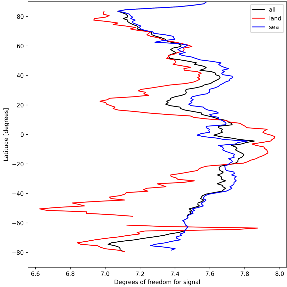
Figure 15: Zonal average of “Degrees of freedom for signal” for 2025-04-03 to 2025-04-04.
