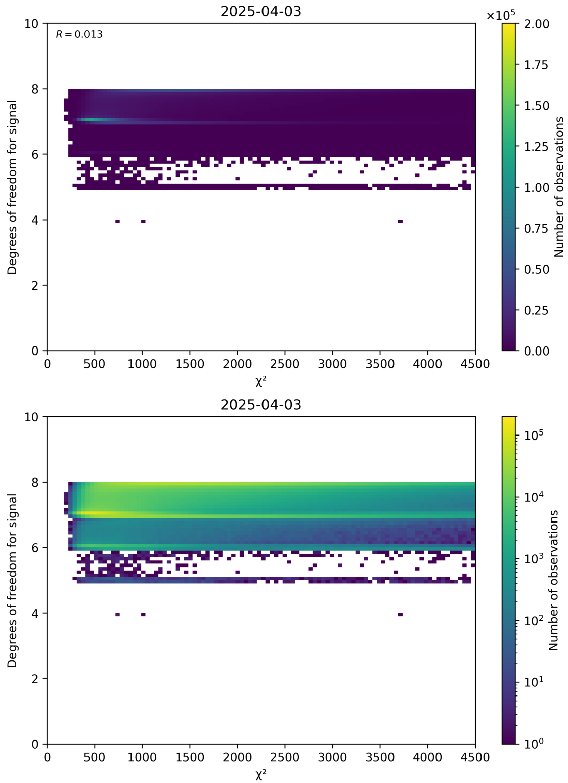
Figure 48: Scatter density plot of " \chi^2 " against "Degrees of freedom for signal" for 2025-04-03 to 2025-04-04.
