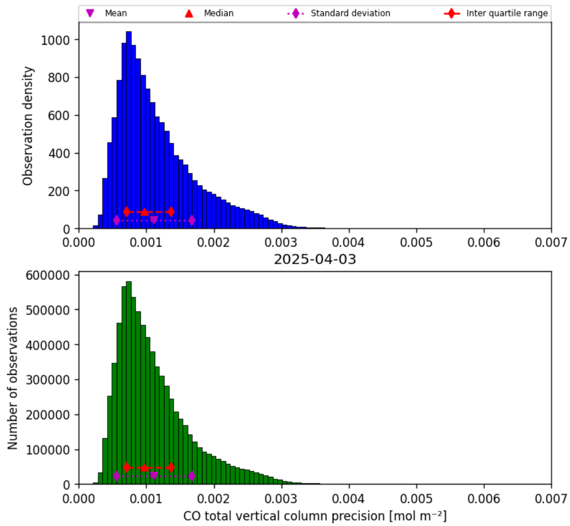
Figure 20: Histogram of “CO total vertical column precision” for 2025-04-03 to 2025-04-04
