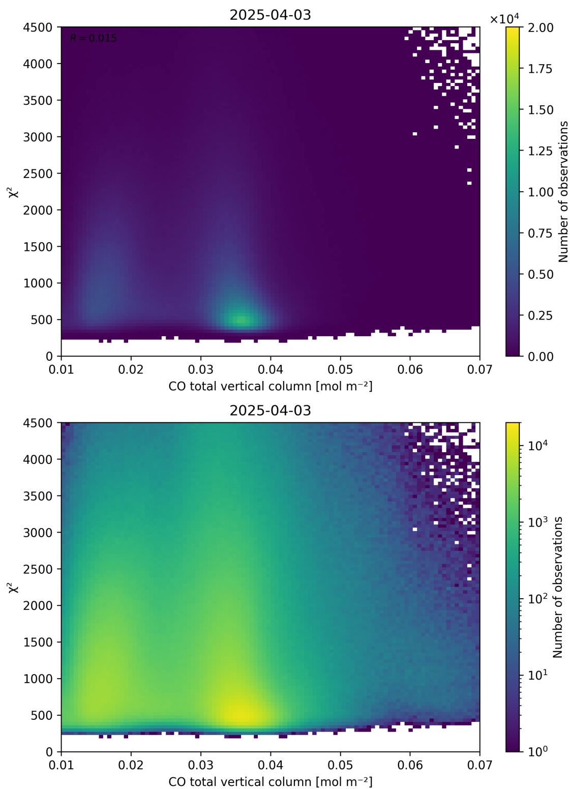
Figure 35: Scatter density plot of “CO total vertical column” against “ \chi^2 ” for 2025-04-03 to 2025-04-04.
