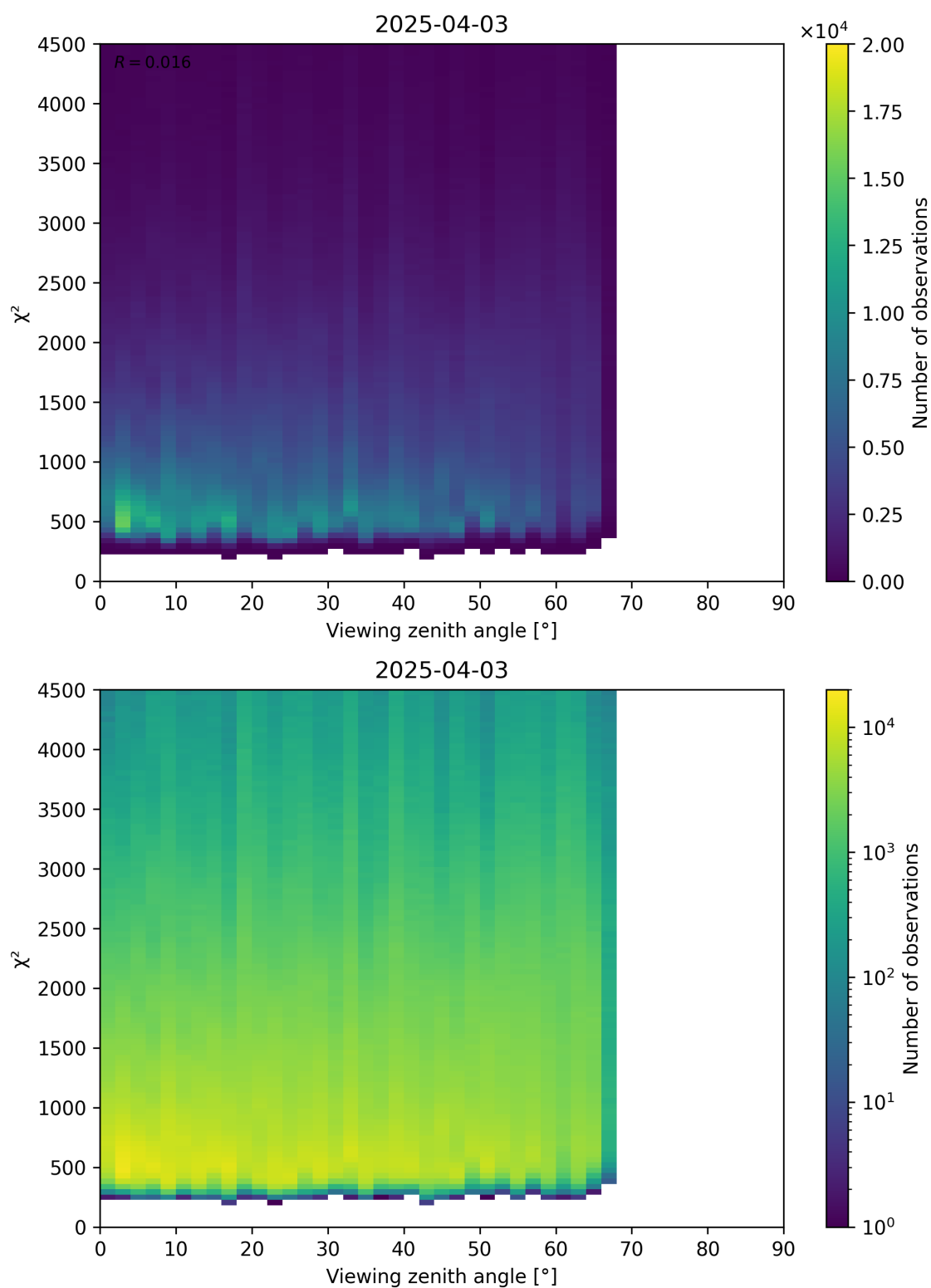
Figure 72: Scatter density plot of “Viewing zenith angle” against “ \chi^2 ” for 2025-04-03 to 2025-04-04.
