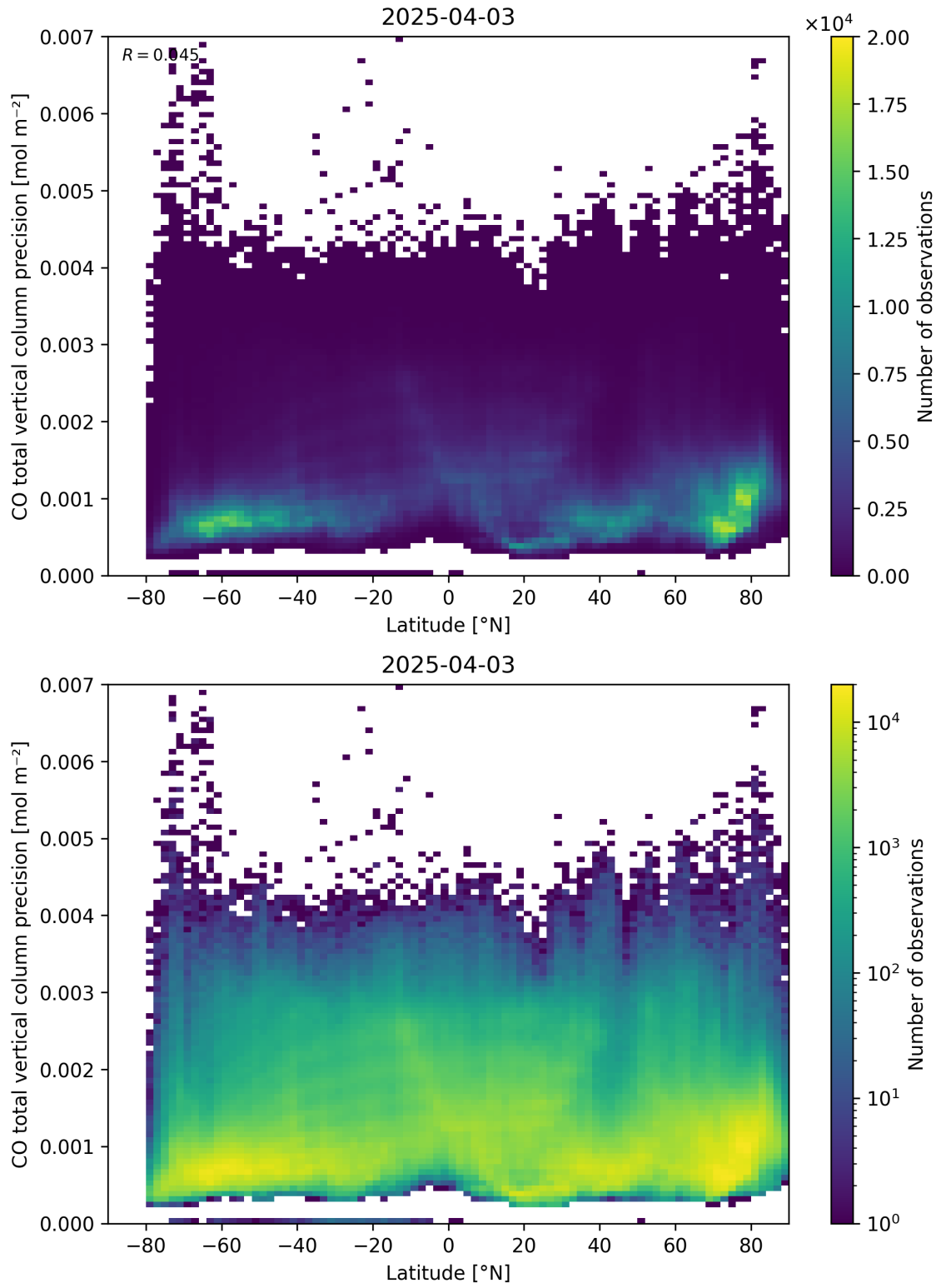
Figure 53: Scatter density plot of “Latitude” against “CO total vertical column precision” for 2025-04-03 to 2025-04-04.
