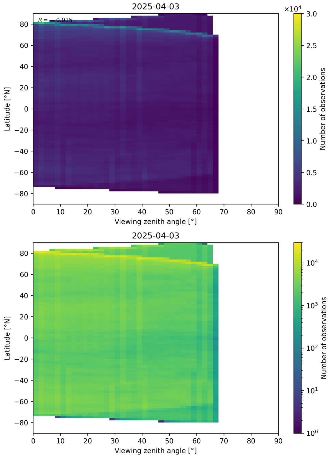
Figure 74: Scatter density plot of “Viewing zenith angle” against “Latitude” for 2025-04-03 to 2025-04-04.
