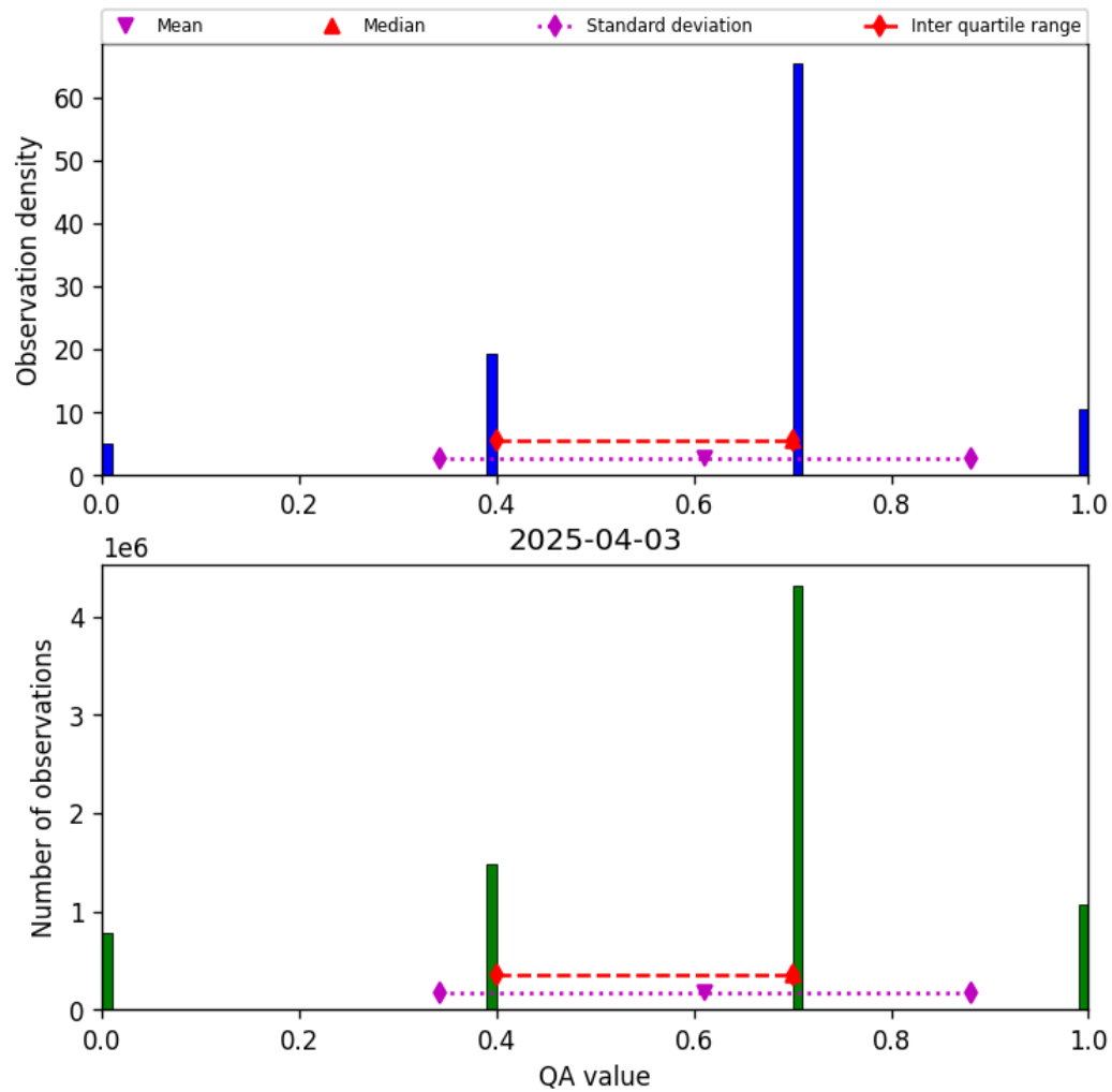
Figure 17: Histogram of “QA value” for 2025-04-03 to 2025-04-04
