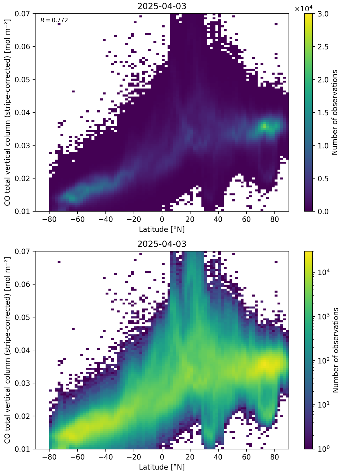
Figure 52: Scatter density plot of “Latitude” against “CO total vertical column (stripe-corrected)” for 2025-04-03 to 2025-04-04.
