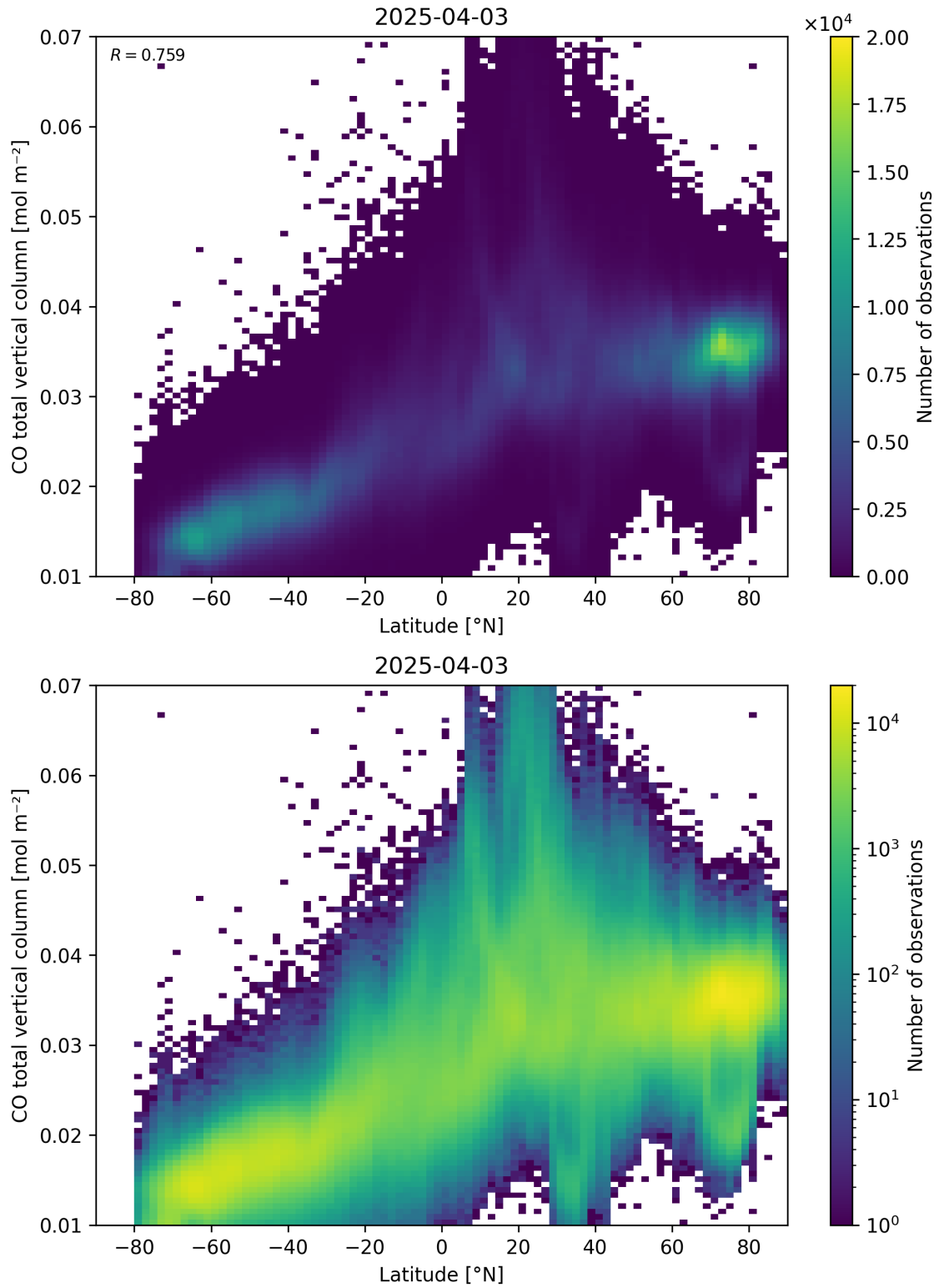
Figure 51: Scatter density plot of “Latitude” against “CO total vertical column” for 2025-04-03 to 2025-04-04.
