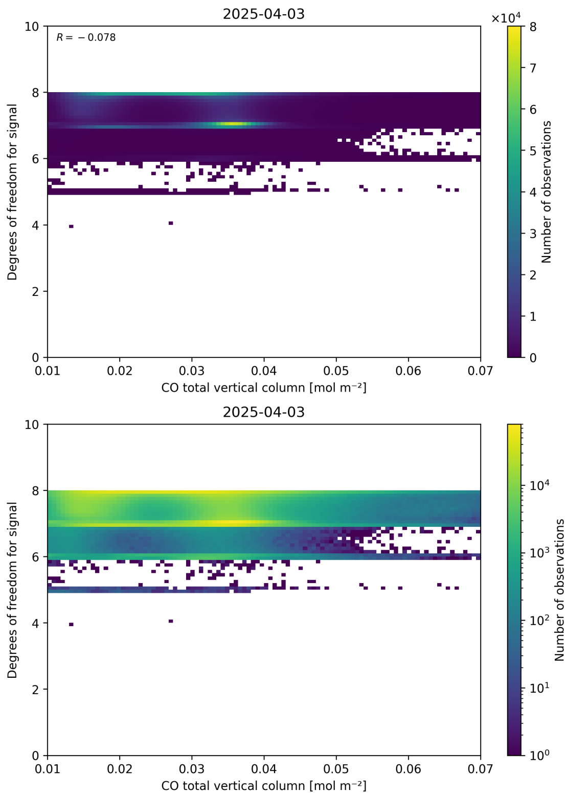
Figure 41: Scatter density plot of “CO total vertical column” against “Degrees of freedom for signal” for 2025-04-03 to 2025-04-04.
