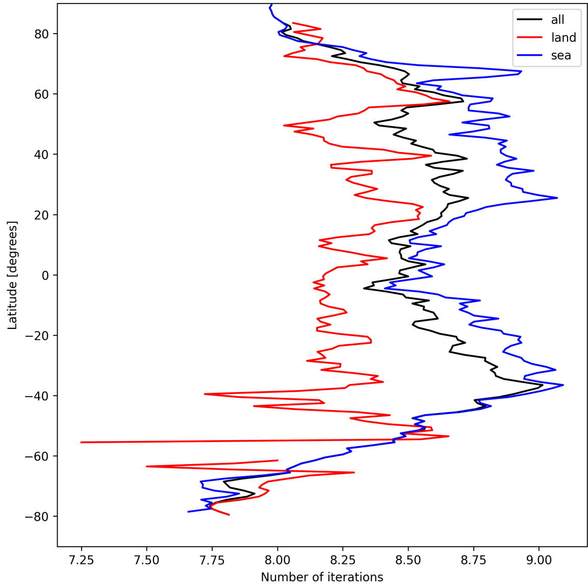
Figure 16: Zonal average of “Number of iterations” for 2025-04-03 to 2025-04-04.
