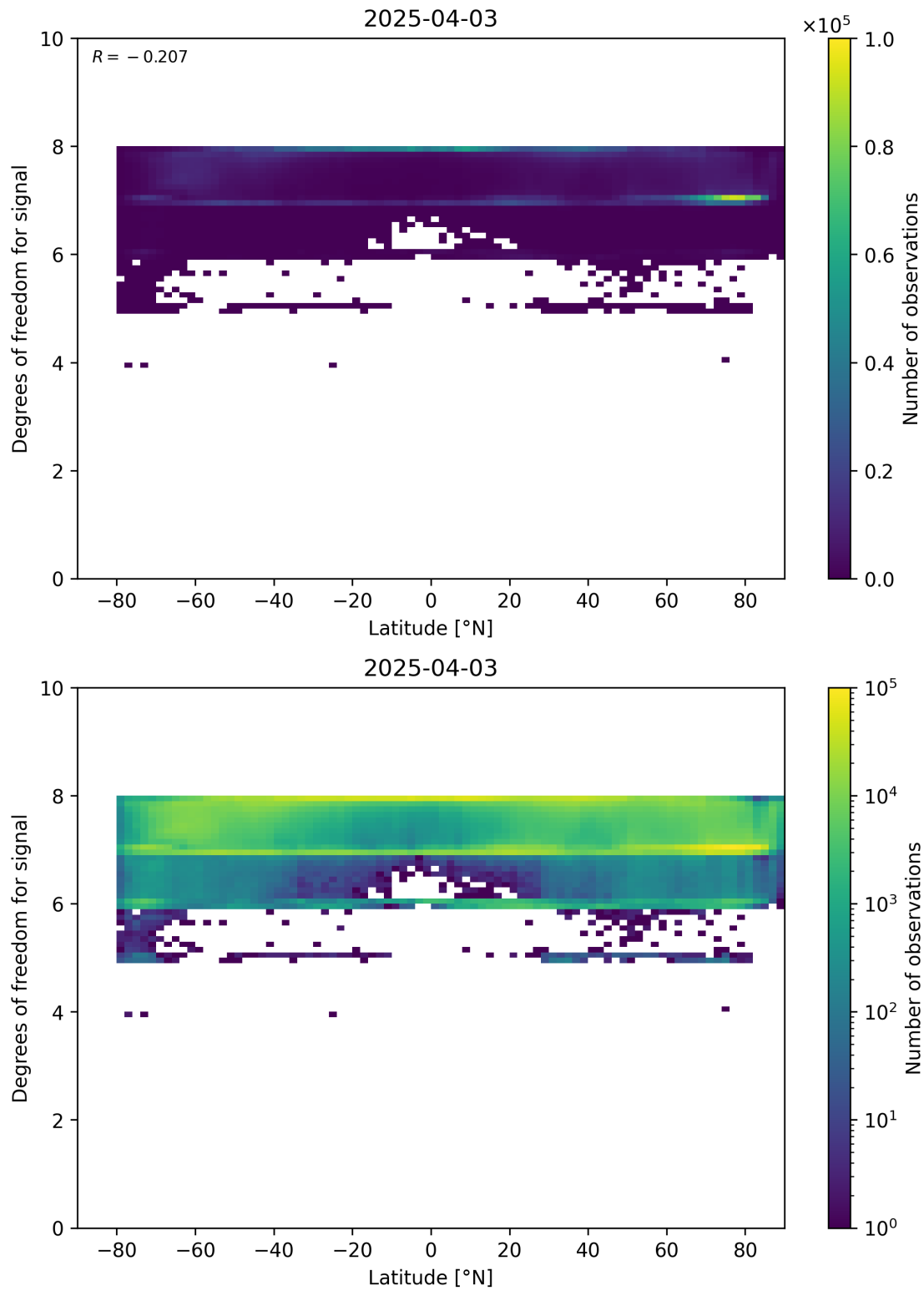
Figure 55: Scatter density plot of “Latitude” against “Degrees of freedom for signal” for 2025-04-03 to 2025-04-04.
