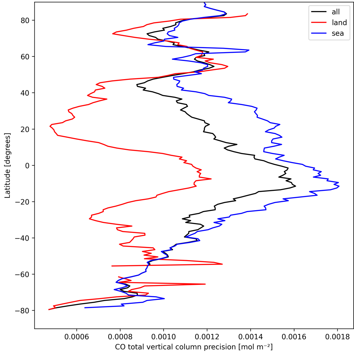
Figure 12: Zonal average of “CO total vertical column precision” for 2025-04-03 to 2025-04-04.
