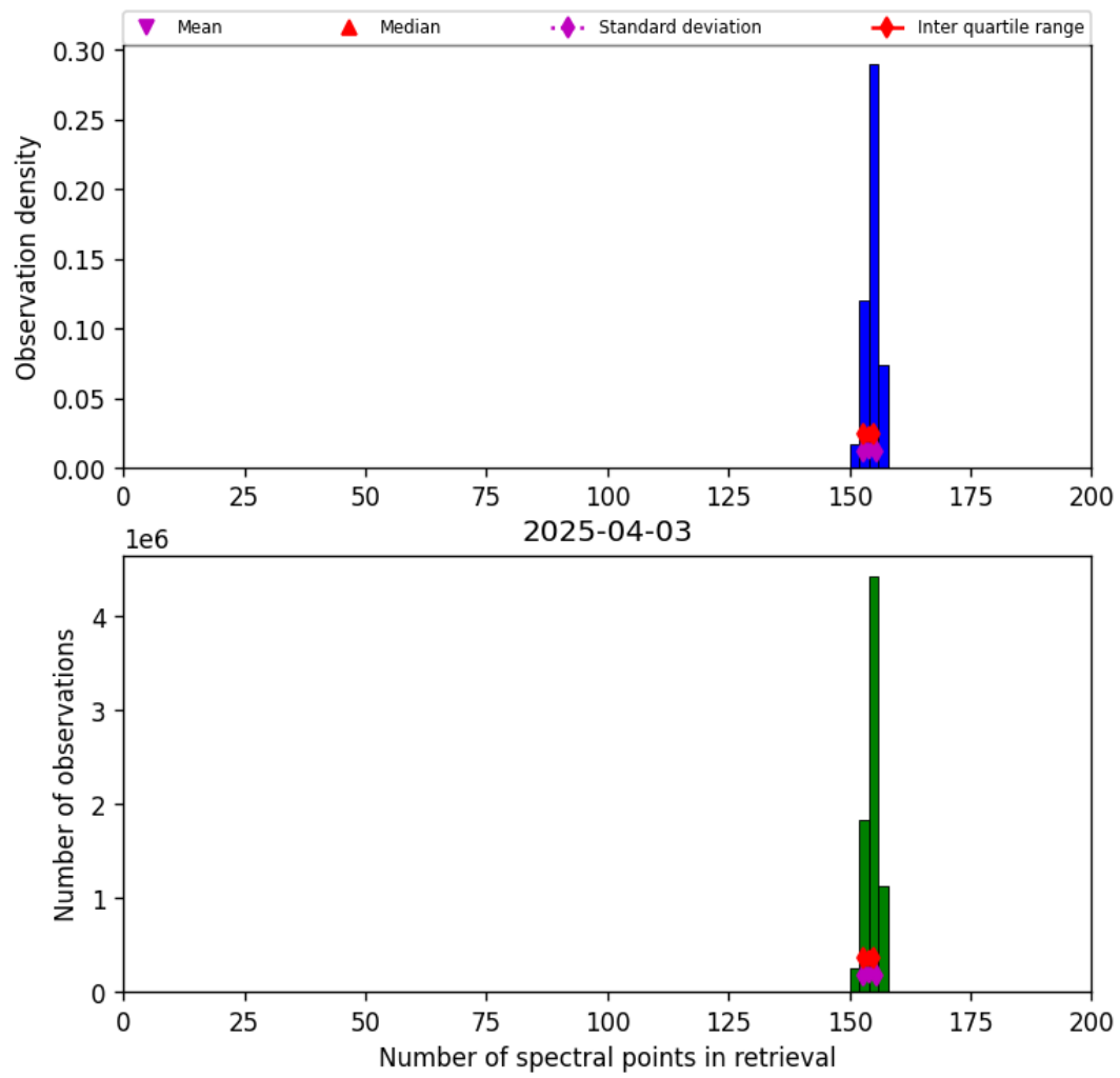
Figure 21: Histogram of “Number of spectral points in retrieval” for 2025-04-03 to 2025-04-04
