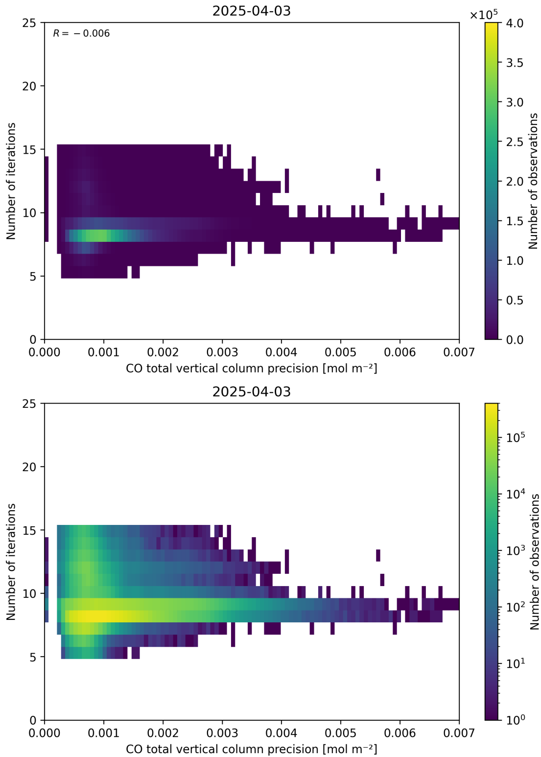
Figure 46: Scatter density plot of “CO total vertical column precision” against “Number of iterations” for 2025-04-03 to 2025-04-04.
