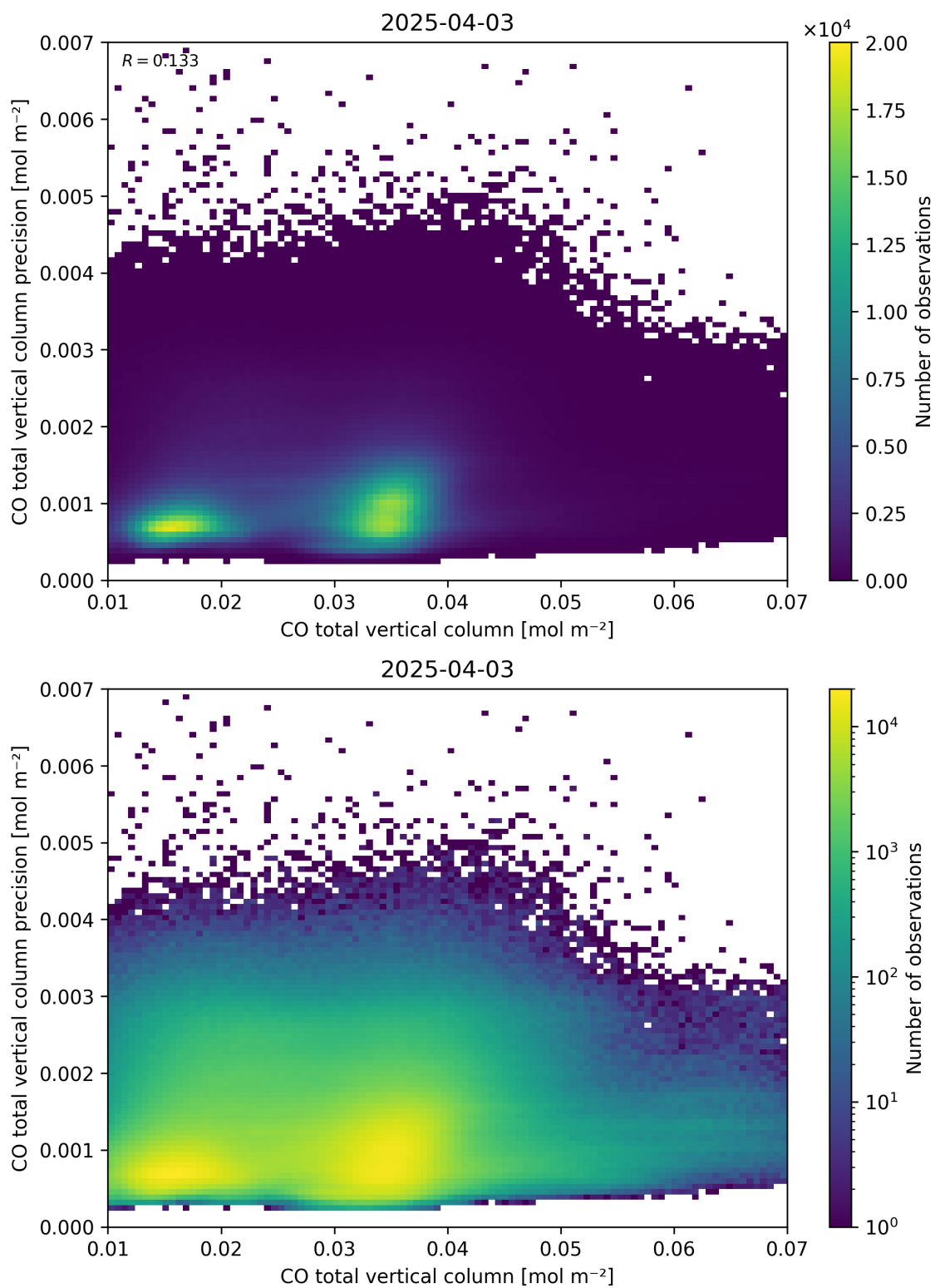
Figure 34: Scatter density plot of “CO total vertical column” against “CO total vertical column precision” for 2025-04-03 to 2025-04-04.
