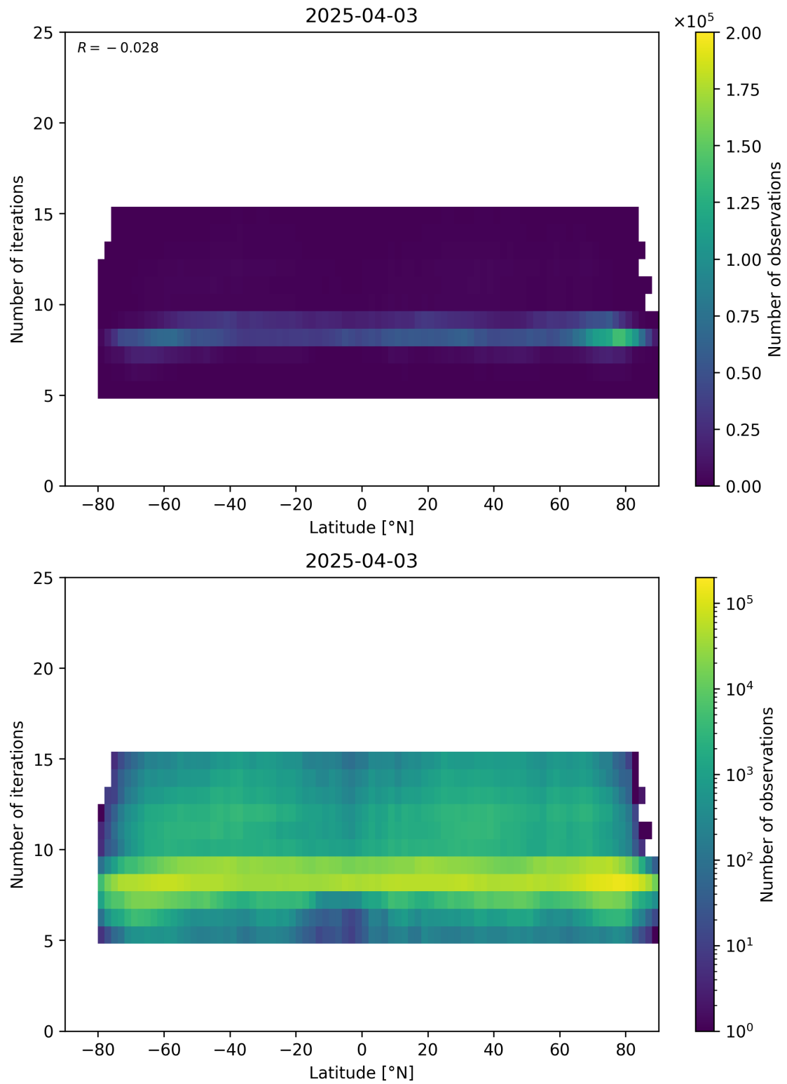
Figure 56: Scatter density plot of “Latitude” against “Number of iterations” for 2025-04-03 to 2025-04-04.
