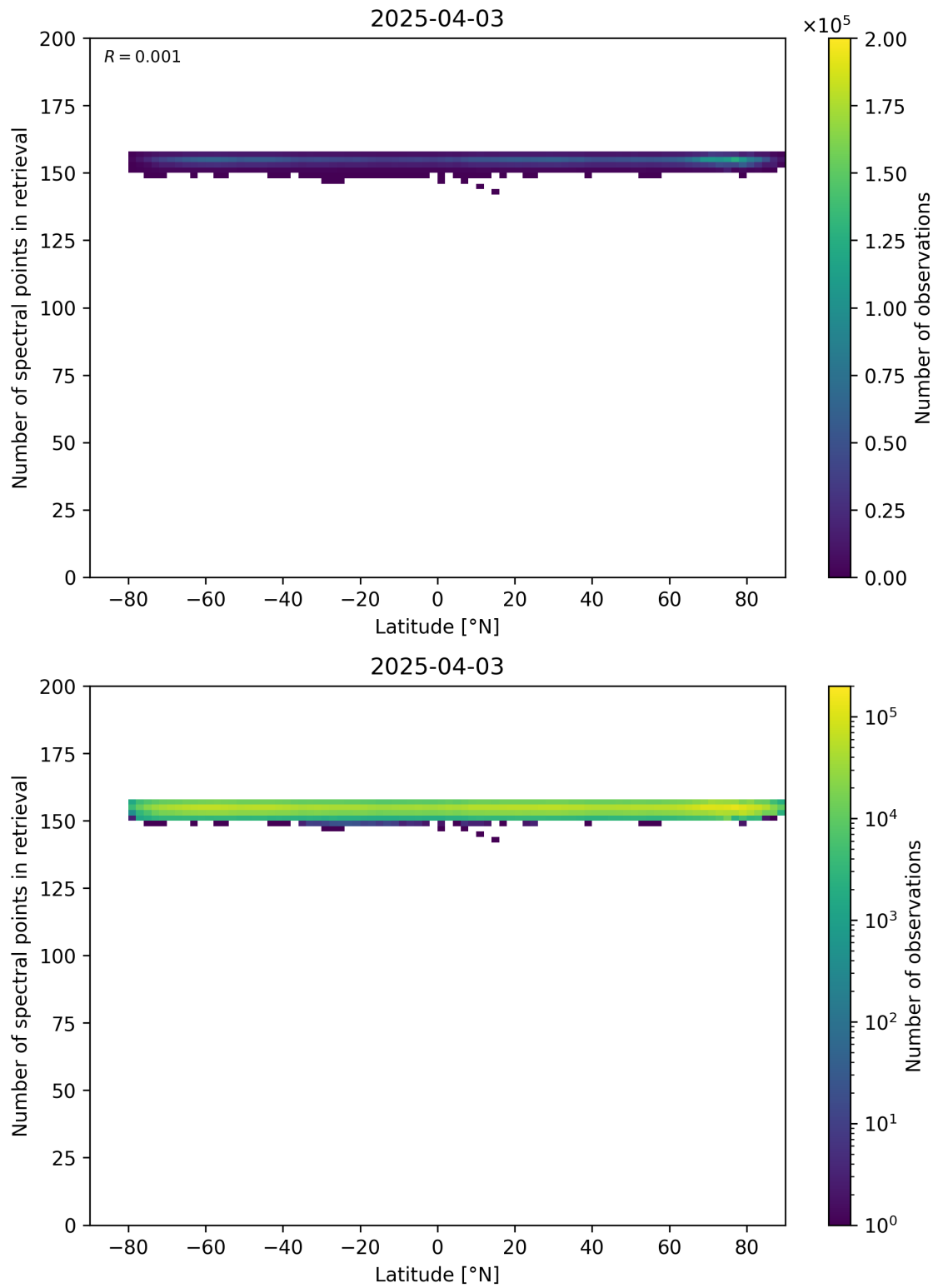
Figure 57: Scatter density plot of “Latitude” against “Number of spectral points in retrieval” for 2025-04-03 to 2025-04-04.
