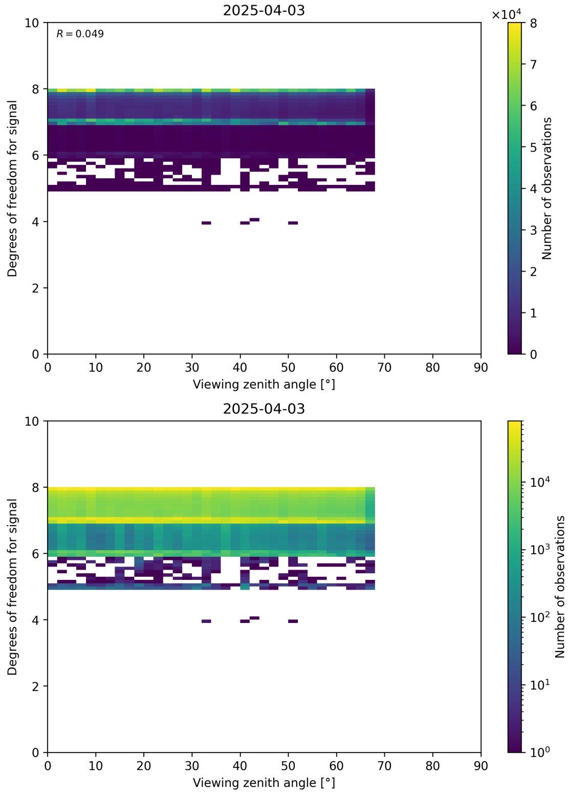
Figure 73: Scatter density plot of “Viewing zenith angle” against “Degrees of freedom for signal” for 2025-04-03 to 2025-04-04.
