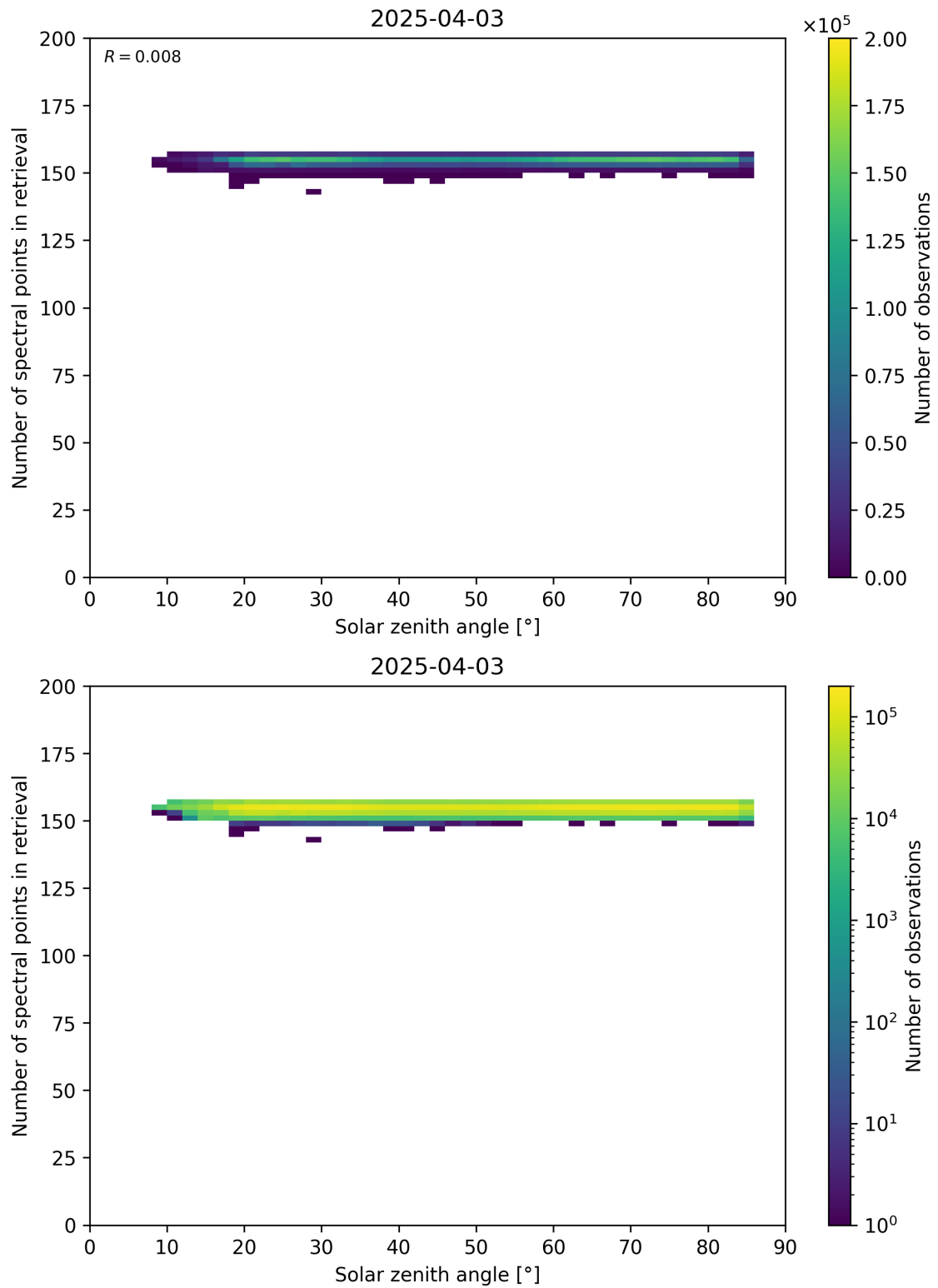
Figure 68: Scatter density plot of “Solar zenith angle” against “Number of spectral points in retrieval” for 2025-04-03 to 2025-04-04.
