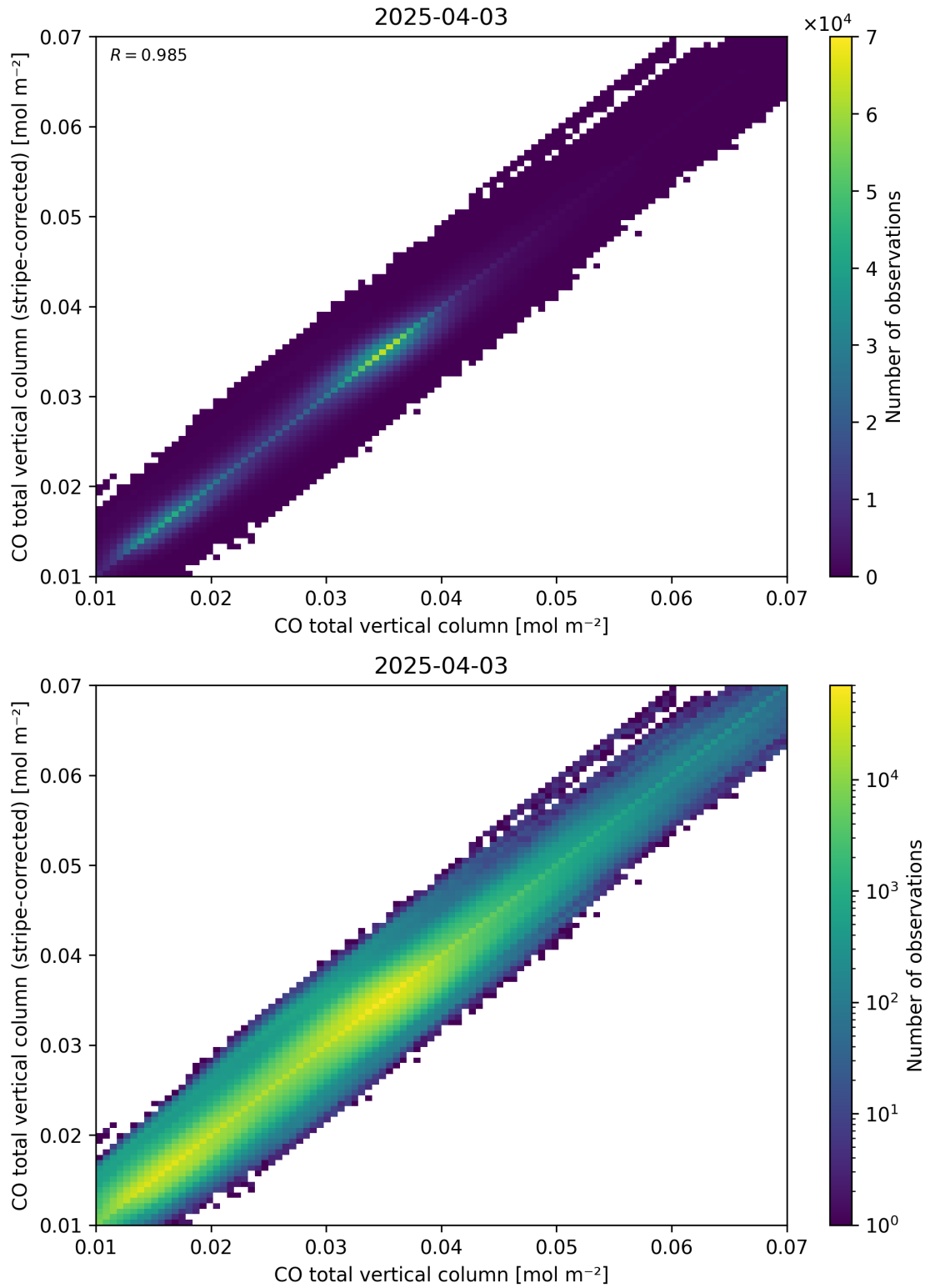
Figure 33: Scatter density plot of “CO total vertical column” against “CO total vertical column (stripe-corrected)” for 2025-04-03 to 2025-04-04.
