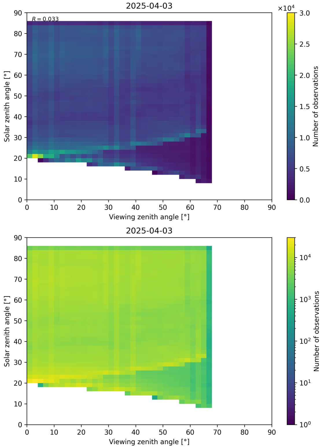
Figure 77: Scatter density plot of “Viewing zenith angle” against “Solar zenith angle” for 2025-04-03 to 2025-04-04.
