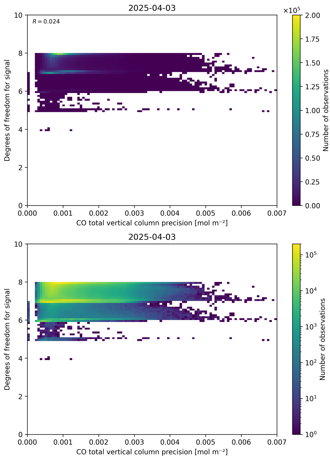
Figure 45: Scatter density plot of “CO total vertical column precision” against “Degrees of freedom for signal” for 2025-04-03 to 2025-04-04.
