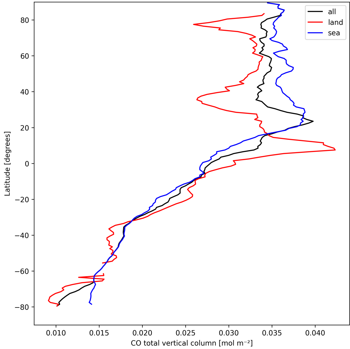
Figure 10: Zonal average of “CO total vertical column” for 2025-04-03 to 2025-04-04.
