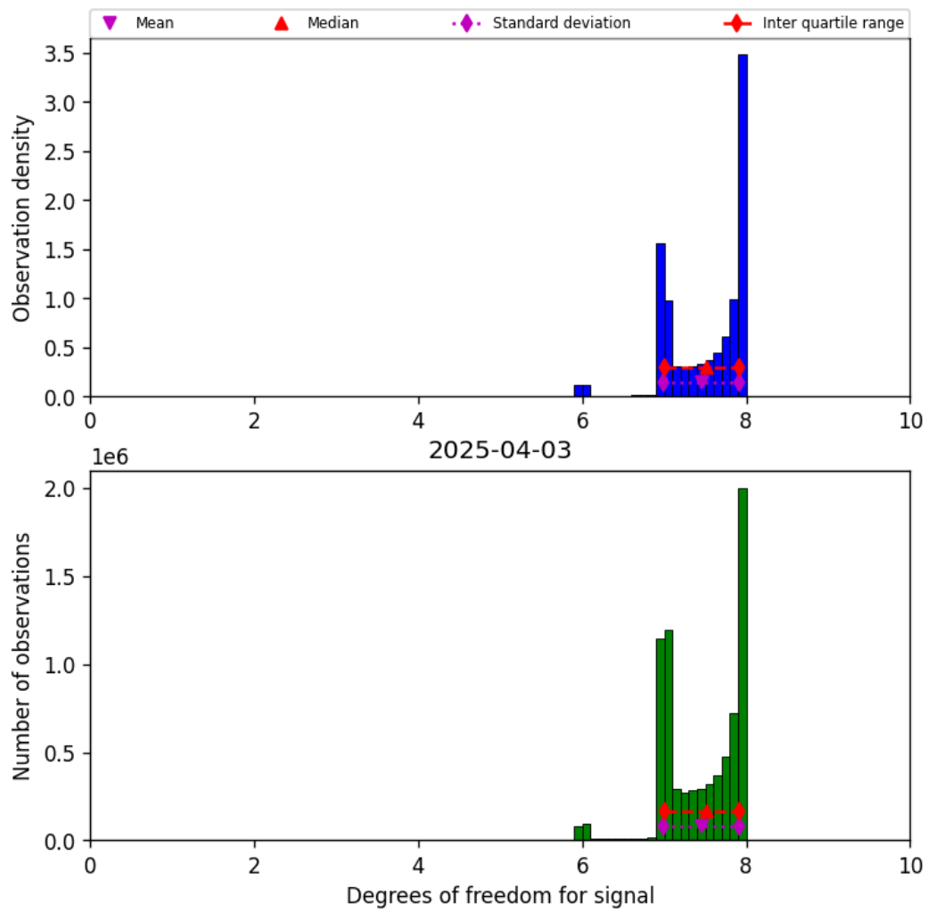
Figure 23: Histogram of “Degrees of freedom for signal” for 2025-04-03 to 2025-04-04
