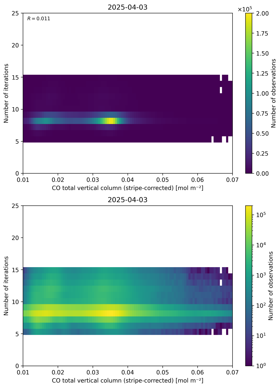
Figure 39: Scatter density plot of “CO total vertical column (stripe-corrected)” against “Number of iterations” for 2025-04-03 to 2025-04-04.
