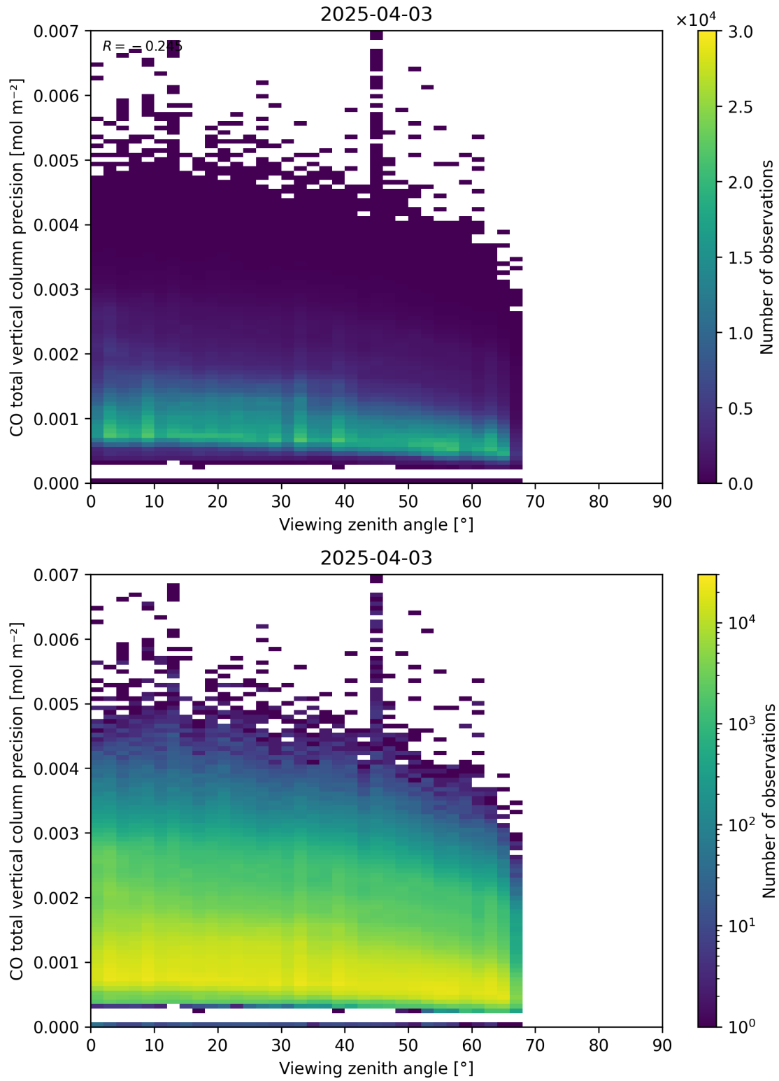
Figure 71: Scatter density plot of “Viewing zenith angle” against “CO total vertical column precision” for 2025-04-03 to 2025-04-04.
