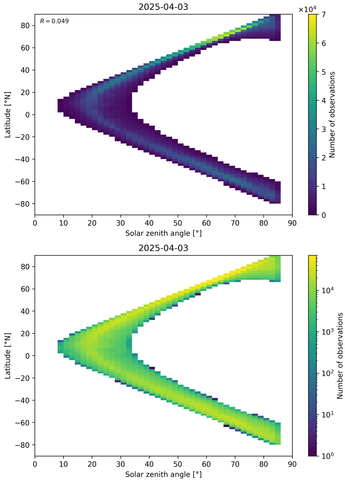
Figure 66: Scatter density plot of “Solar zenith angle” against “Latitude” for 2025-04-03 to 2025-04-04.
