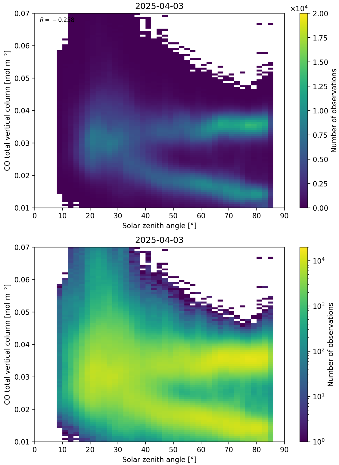
Figure 61: Scatter density plot of “Solar zenith angle” against “CO total vertical column” for 2025-04-03 to 2025-04-04.
