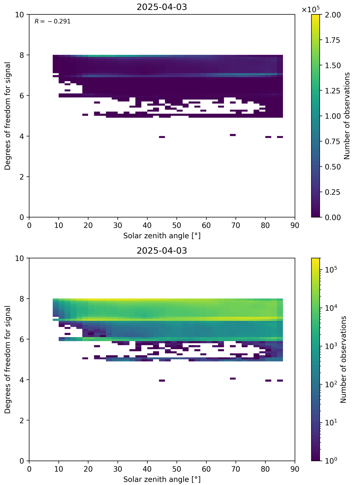
Figure 65: Scatter density plot of “Solar zenith angle” against “Degrees of freedom for signal” for 2025-04-03 to 2025-04-04.
