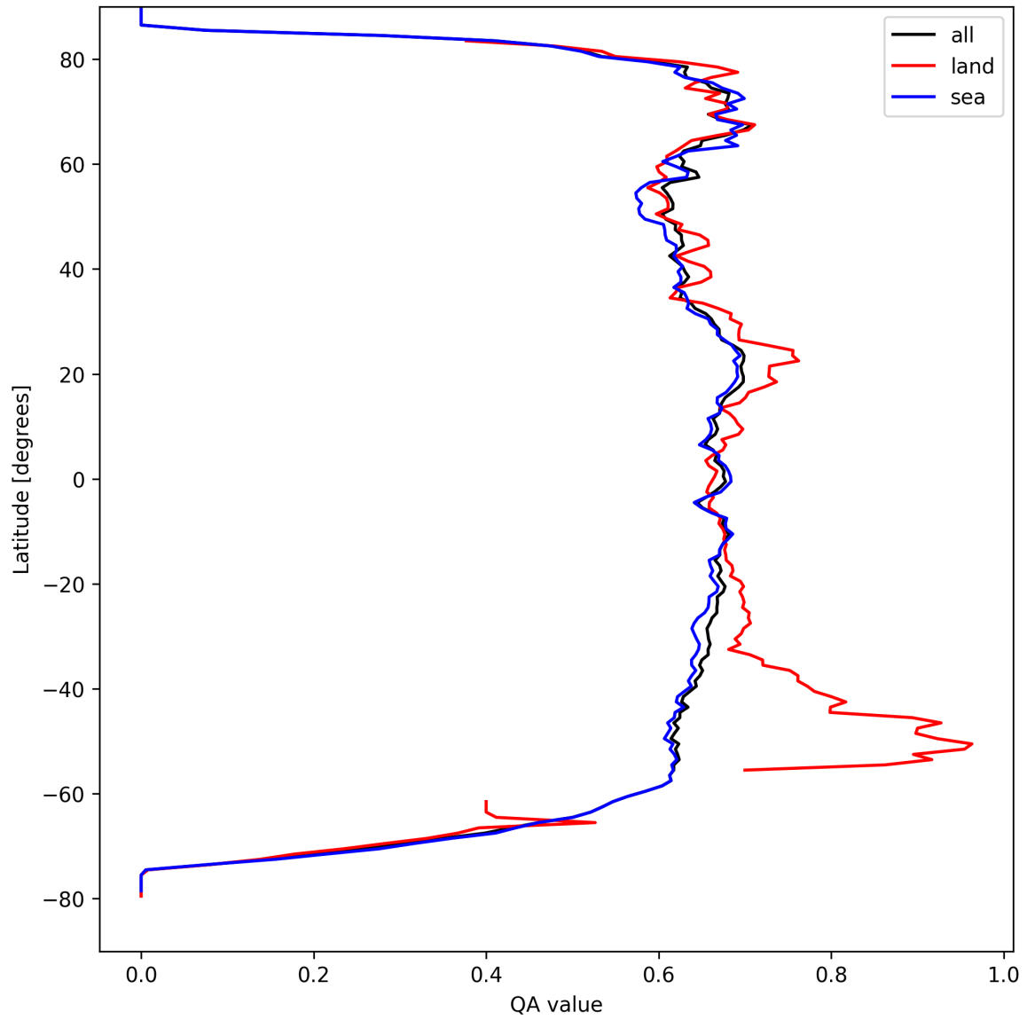
Figure 9: Zonal average of “QA value” for 2025-04-03 to 2025-04-04.
