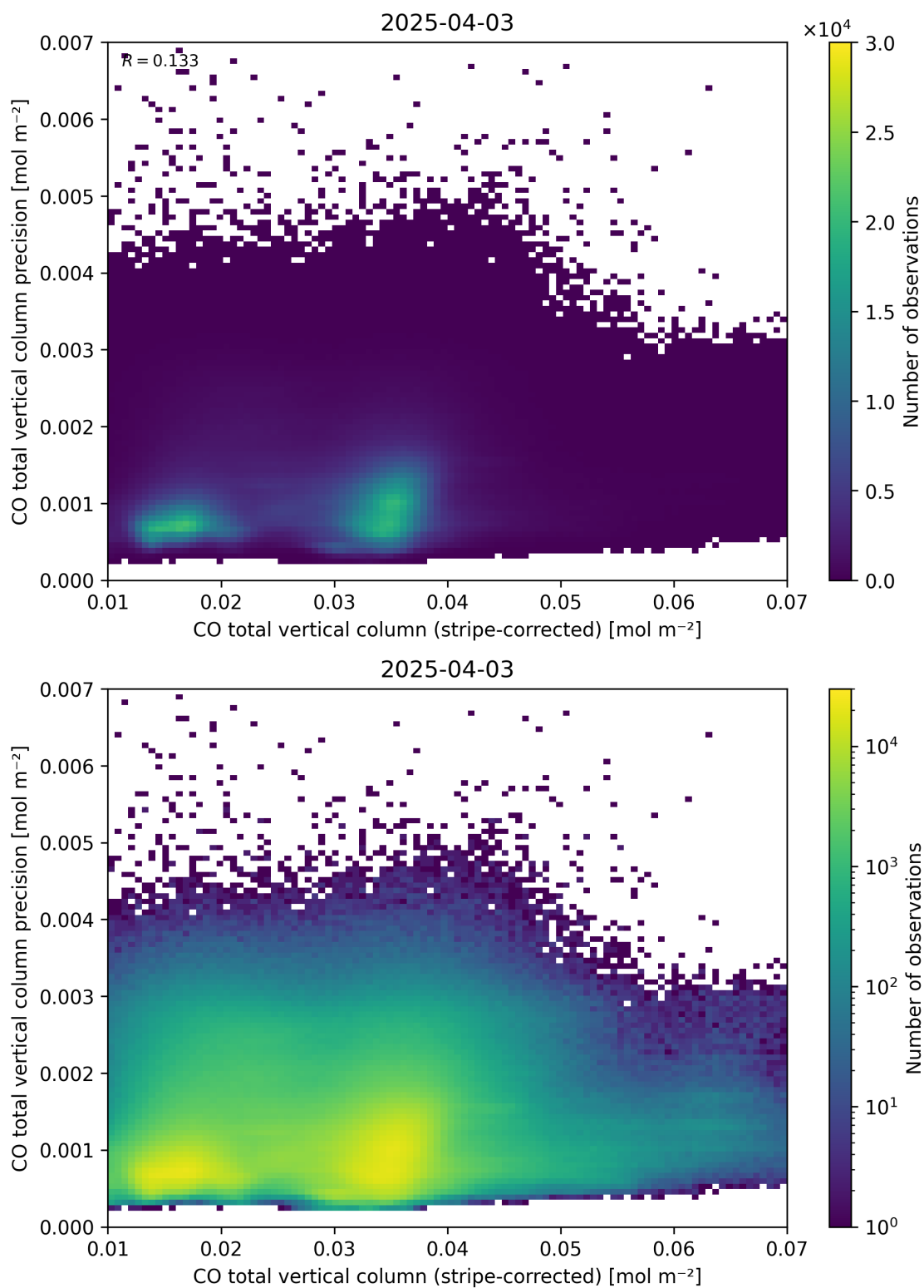
Figure 36: Scatter density plot of “CO total vertical column (stripe-corrected)” against “CO total vertical column precision” for 2025-04-03 to 2025-04-04.
