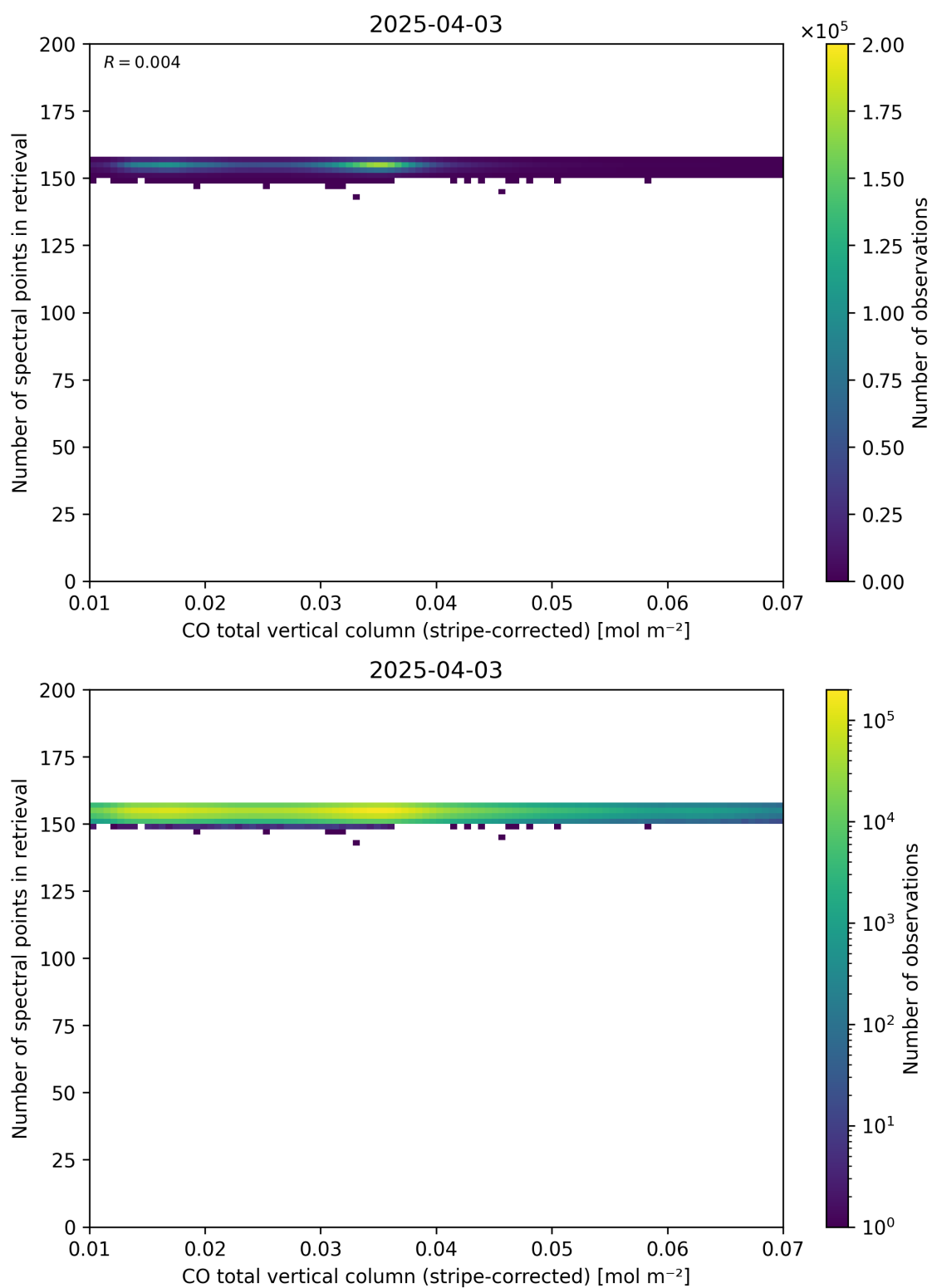
Figure 40: Scatter density plot of “CO total vertical column (stripe-corrected)” against “Number of spectral points in retrieval” for 2025-04-03 to 2025-04-04.
