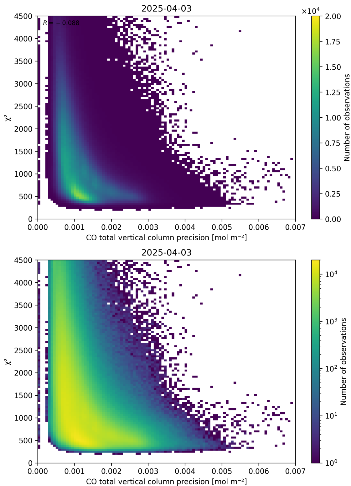
Figure 44: Scatter density plot of “CO total vertical column precision” against “ \chi^2 ” for 2025-04-03 to 2025-04-04.
