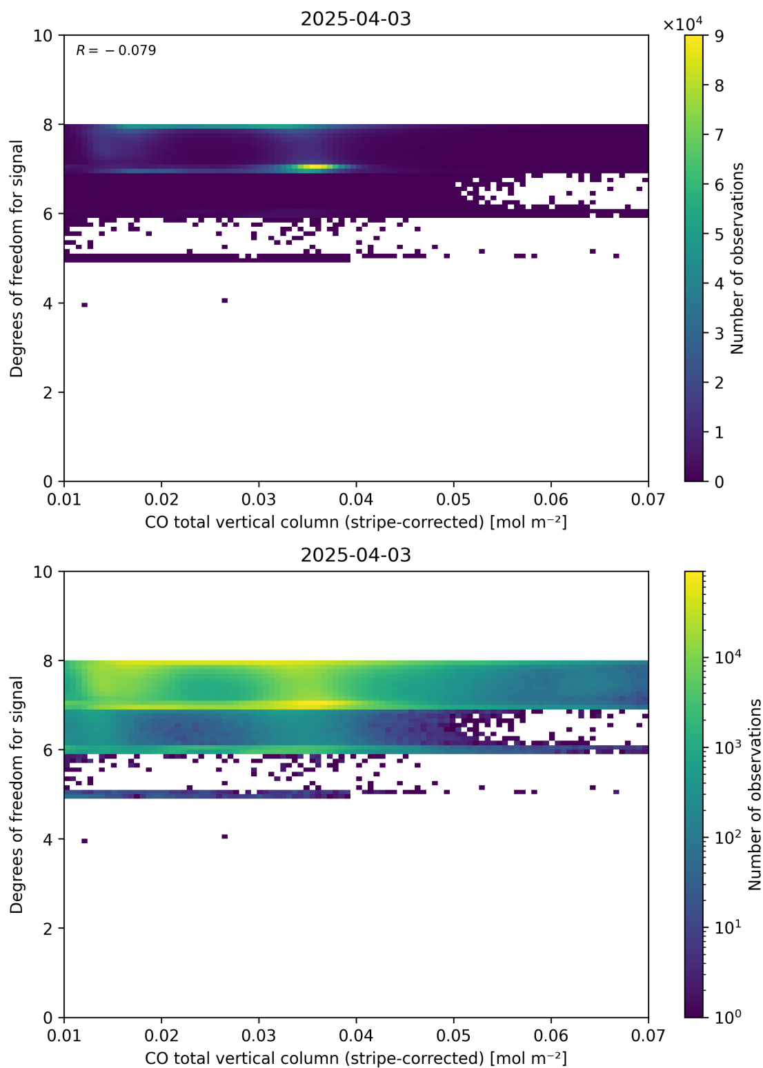
Figure 38: Scatter density plot of “CO total vertical column (stripe-corrected)” against “Degrees of freedom for signal” for 2025-04-03 to 2025-04-04.
