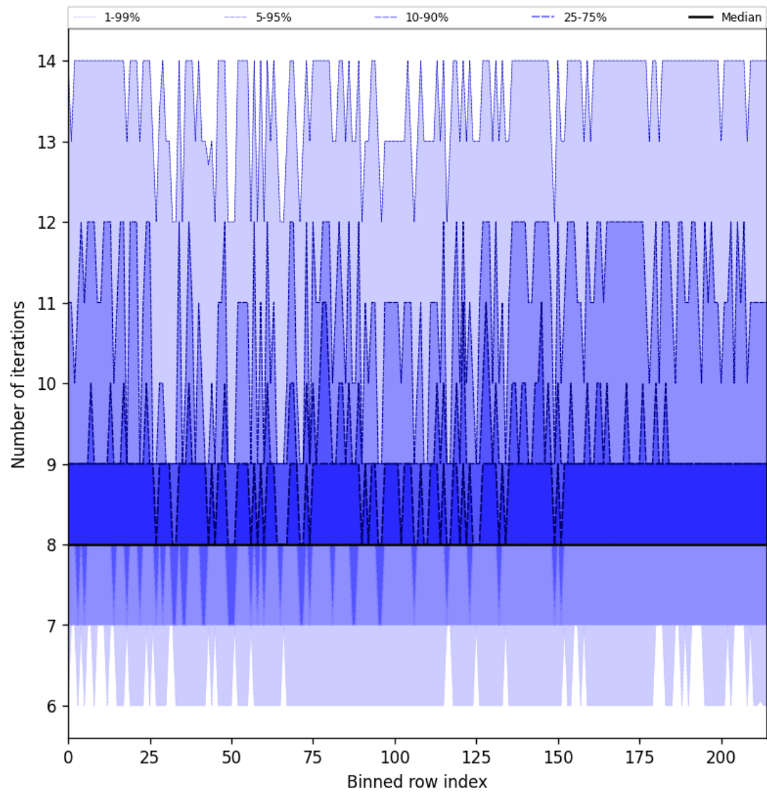
Figure 32: Along track statistics of “Number of iterations” for 2025-04-03 to 2025-04-04
