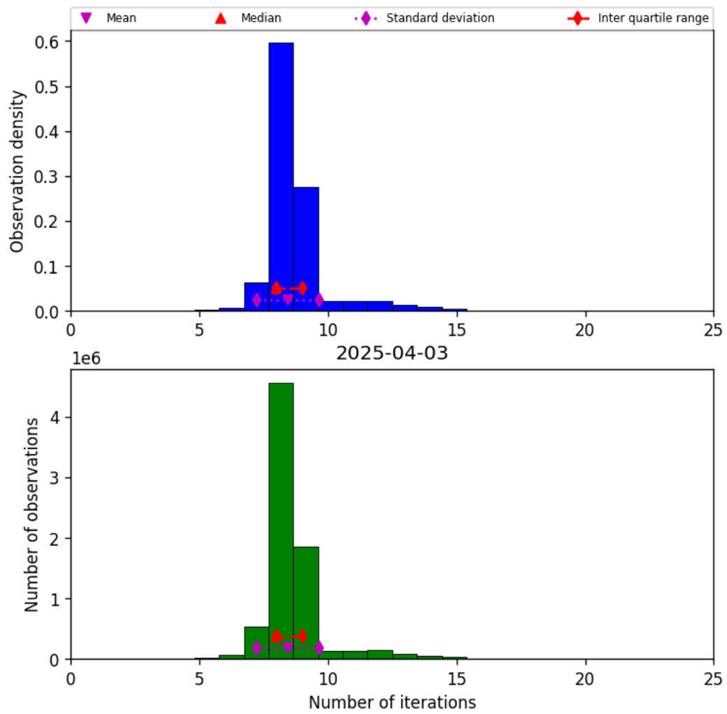
Figure 24: Histogram of “Number of iterations” for 2025-04-03 to 2025-04-04
