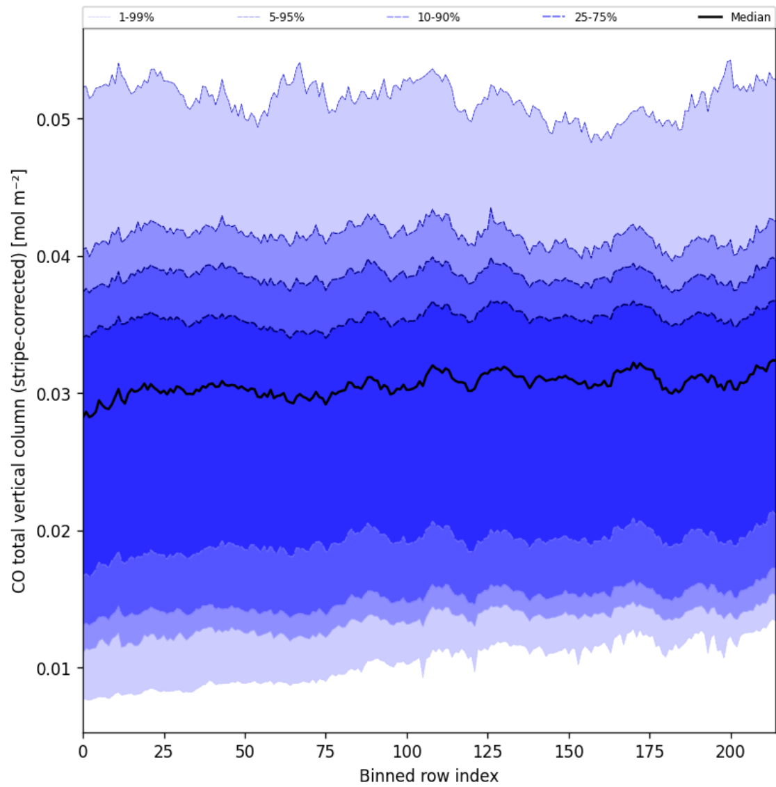
Figure 27: Along track statistics of “CO total vertical column (stripe-corrected)” for 2025-04-03 to 2025-04-04
