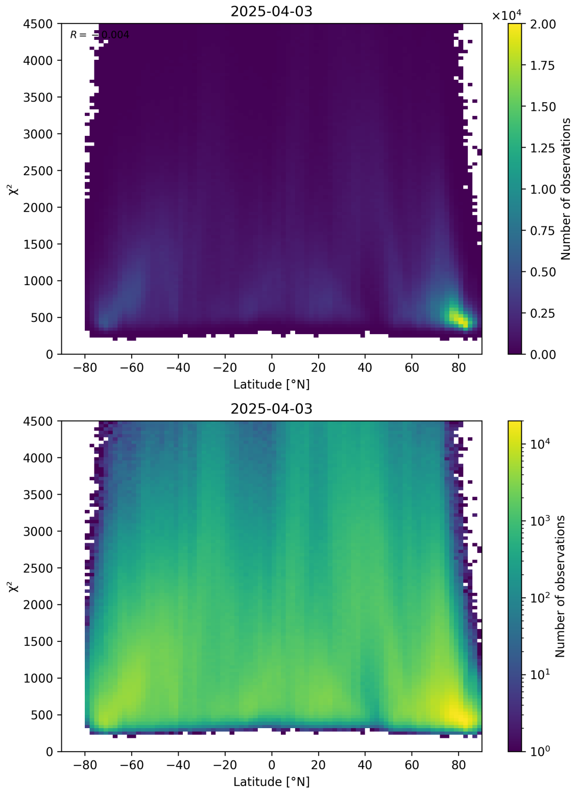
Figure 54: Scatter density plot of “Latitude” against “ \chi^2 ” for 2025-04-03 to 2025-04-04.
