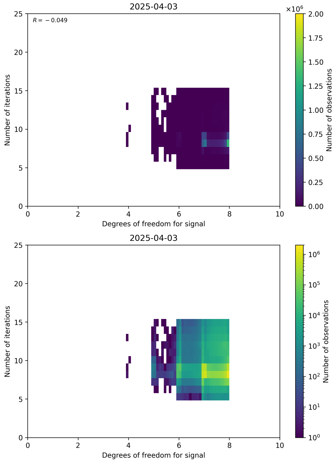
Figure 50: Scatter density plot of “Degrees of freedom for signal” against “Number of iterations” for 2025-04-03 to 2025-04-04.
