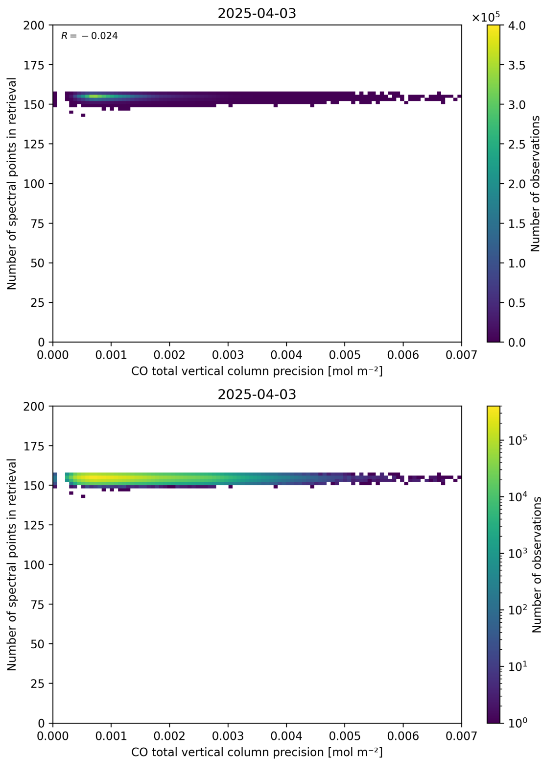
Figure 47: Scatter density plot of “CO total vertical column precision” against “Number of spectral points in retrieval” for 2025-04-03 to 2025-04-04.
