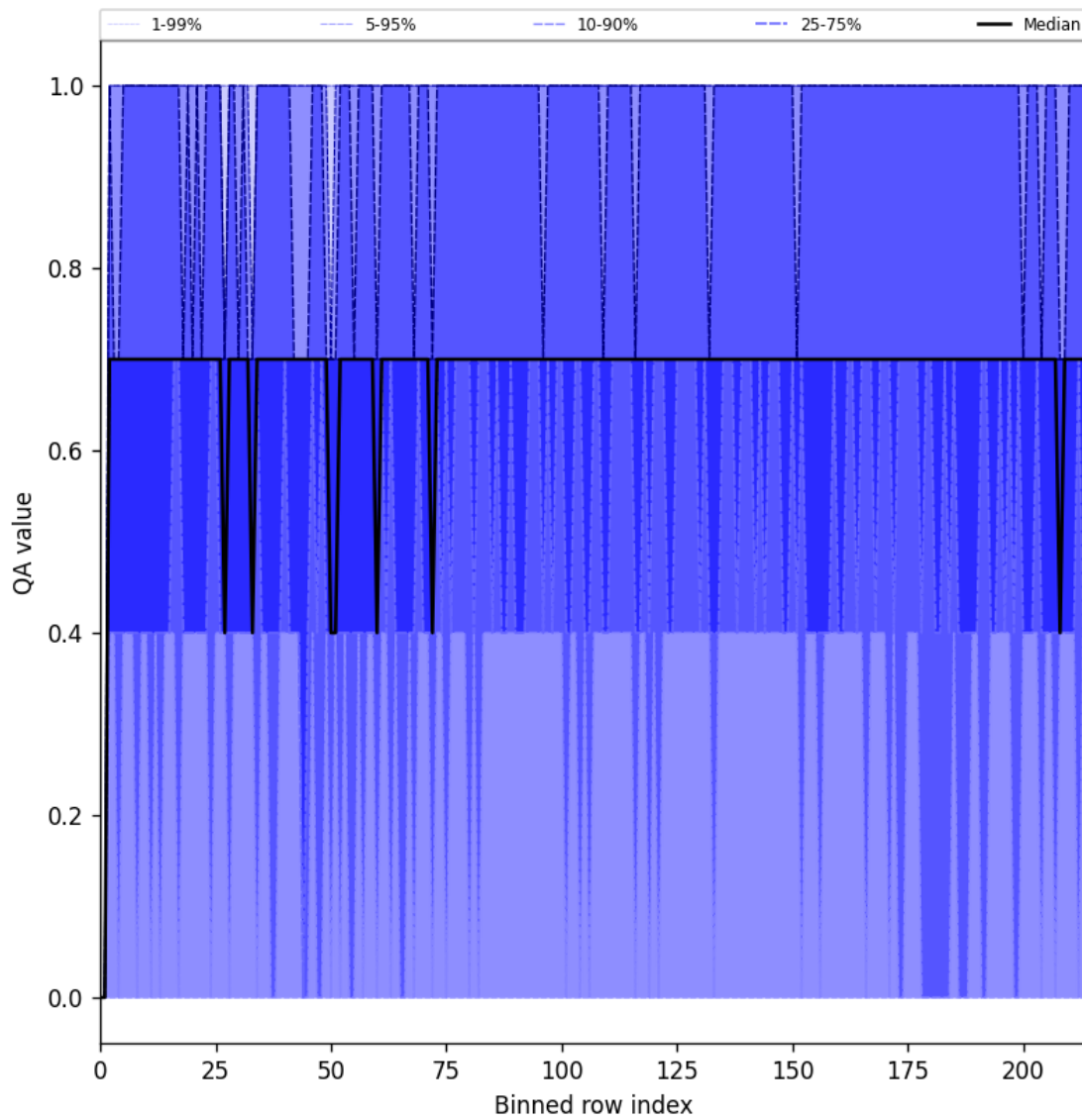
Figure 25: Along track statistics of “QA value” for 2025-04-03 to 2025-04-04
