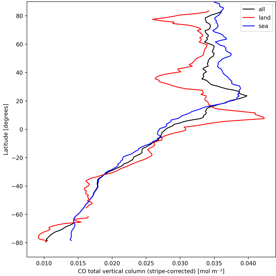
Figure 11: Zonal average of “CO total vertical column (stripe-corrected)” for 2025-04-03 to 2025-04-04.
