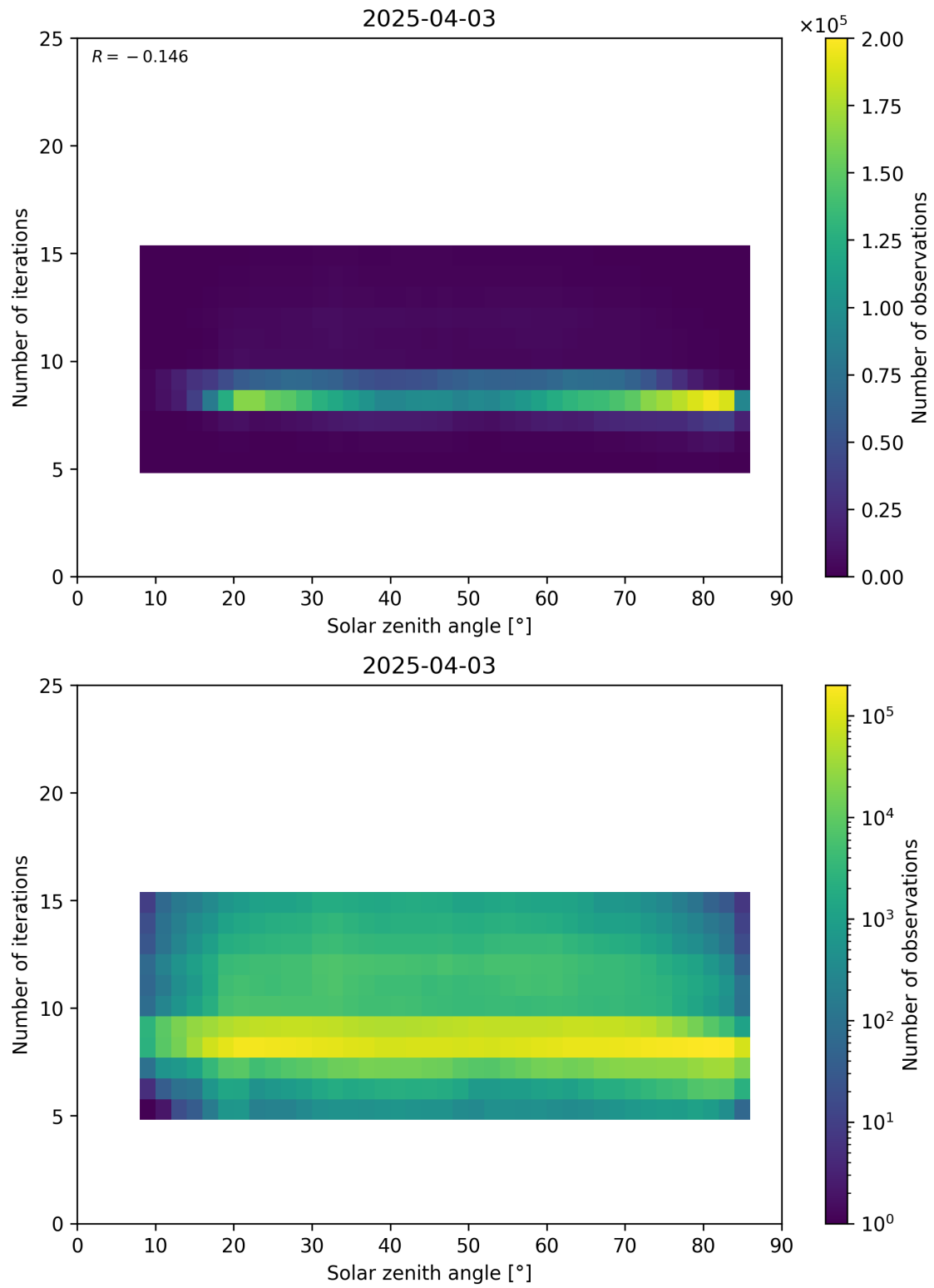
Figure 67: Scatter density plot of “Solar zenith angle” against “Number of iterations” for 2025-04-03 to 2025-04-04.
