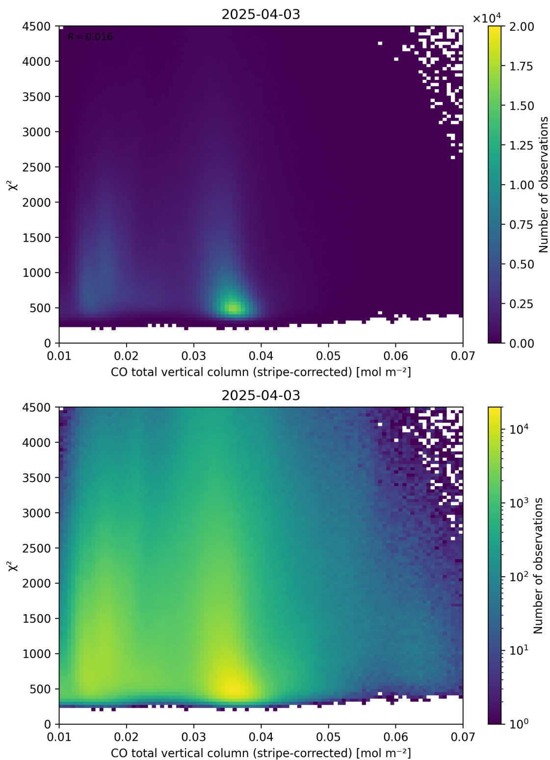
Figure 37: Scatter density plot of “CO total vertical column (stripe-corrected)” against “ \chi^2 ” for 2025-04-03 to 2025-04-04.
