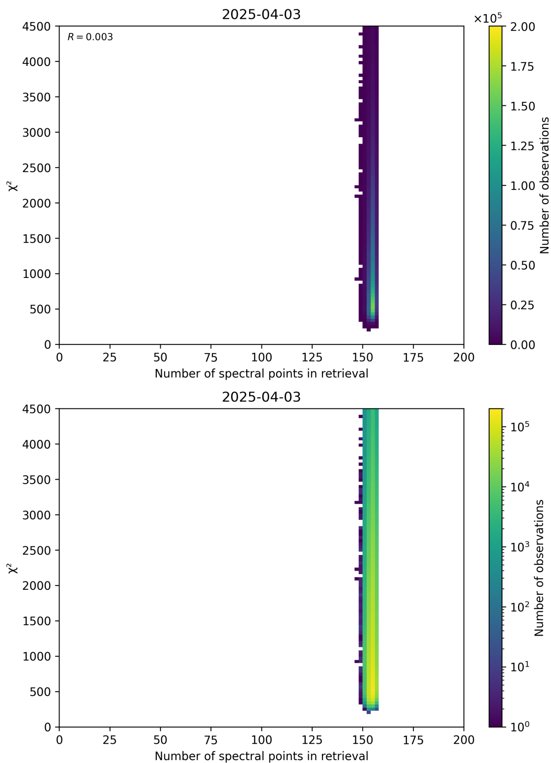
Figure 58: Scatter density plot of “Number of spectral points in retrieval” against “ \chi^2 ” for 2025-04-03 to 2025-04-04.
