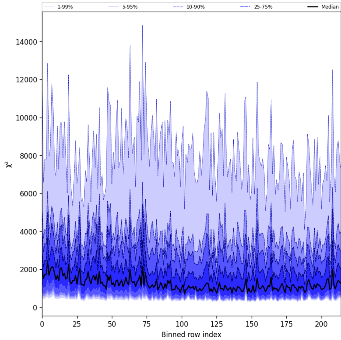
Figure 30: Along track statistics of “ \chi^2 ” for 2025-04-03 to 2025-04-04
