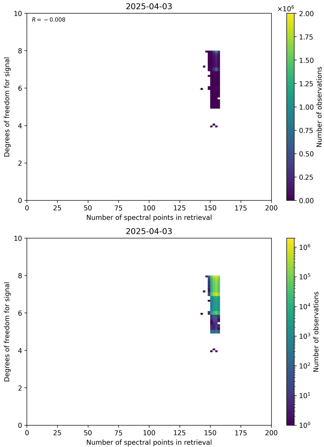
Figure 59: Scatter density plot of “Number of spectral points in retrieval” against “Degrees of freedom for signal” for 2025-04-03 to 2025-04-04.
