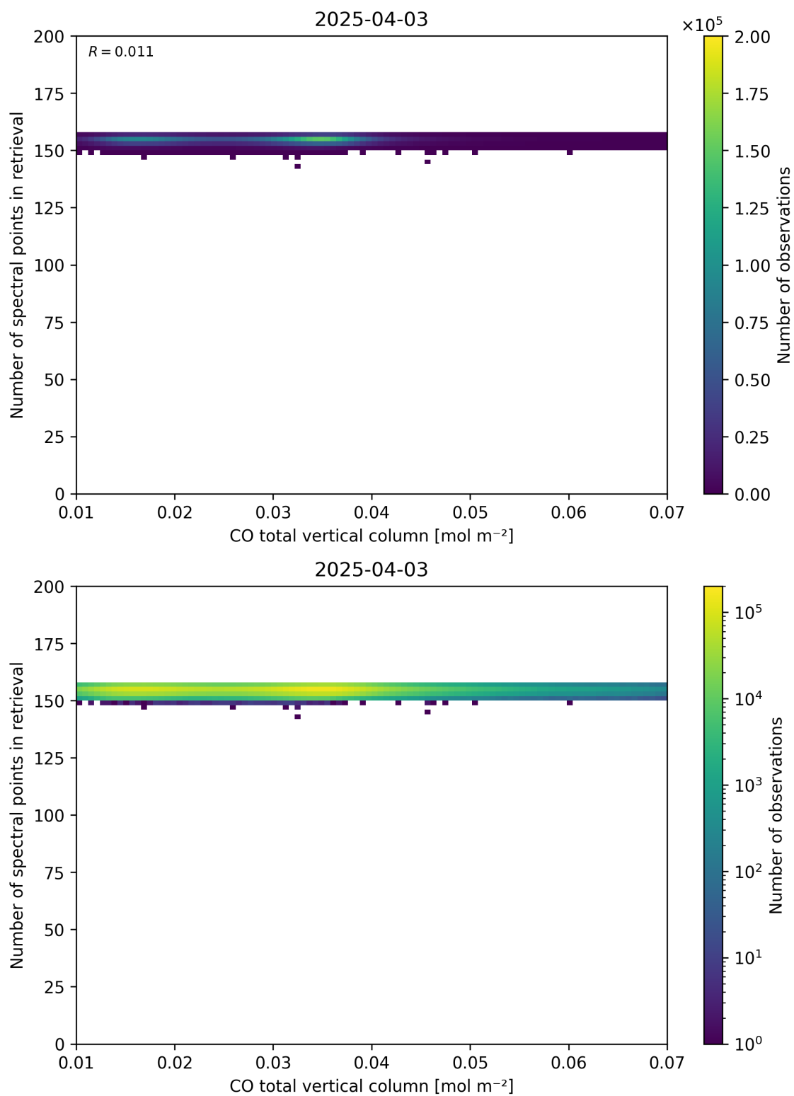
Figure 43: Scatter density plot of “CO total vertical column” against “Number of spectral points in retrieval” for 2025-04-03 to 2025-04-04.
