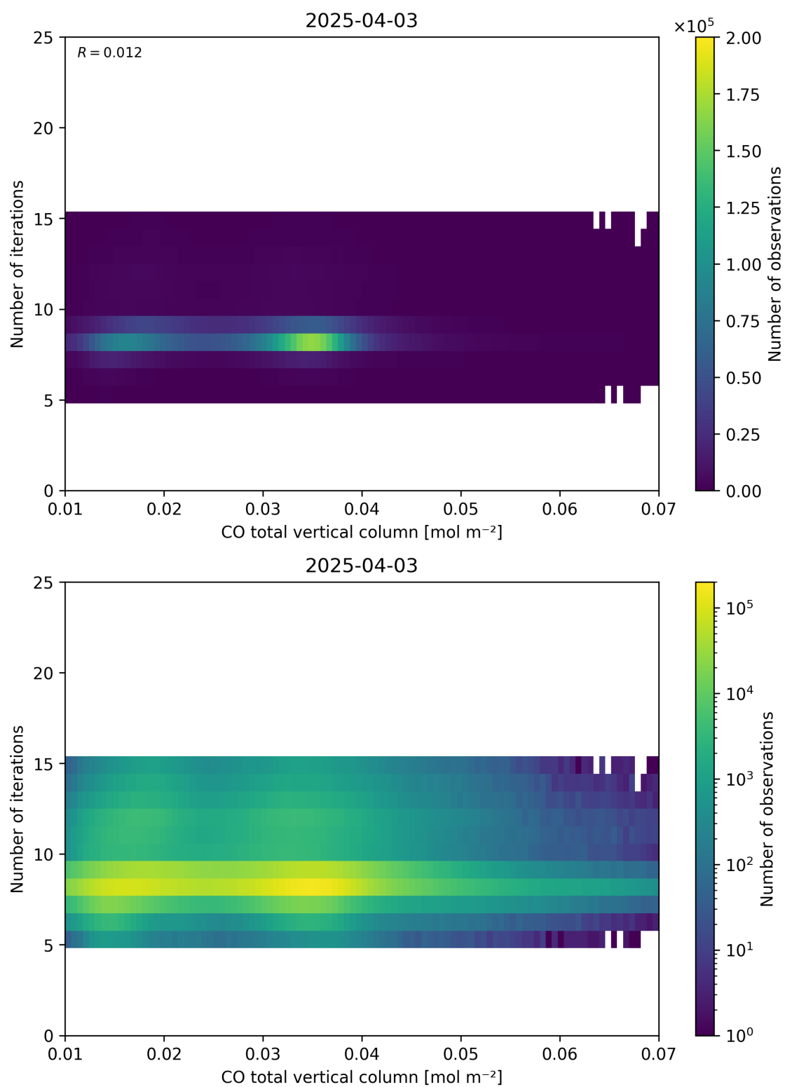
Figure 42: Scatter density plot of “CO total vertical column” against “Number of iterations” for 2025-04-03 to 2025-04-04.
