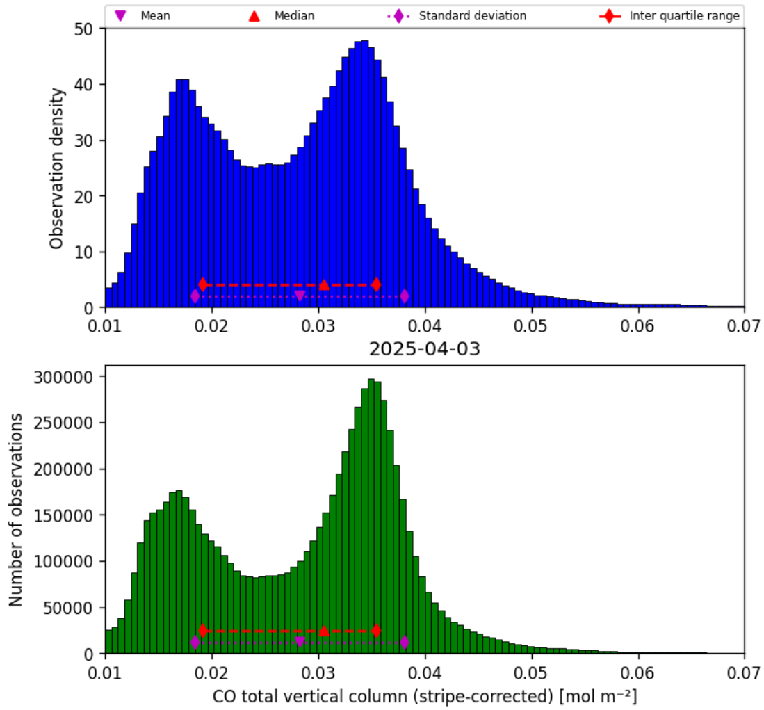
Figure 19: Histogram of “CO total vertical column (stripe-corrected)” for 2025-04-03 to 2025-04-04
