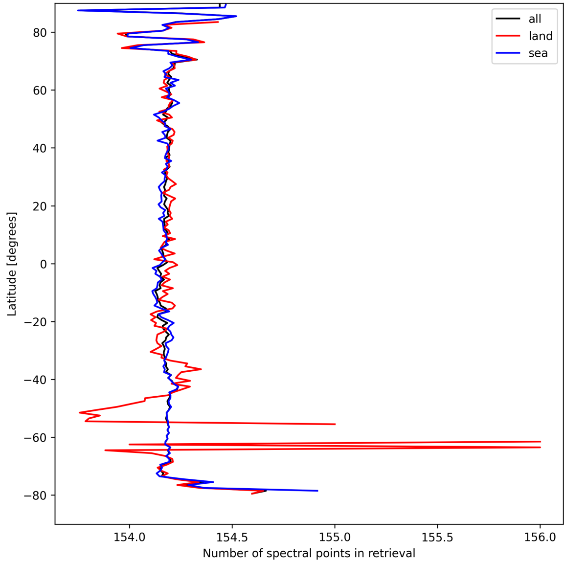
Figure 13: Zonal average of “Number of spectral points in retrieval” for 2025-04-03 to 2025-04-04.
