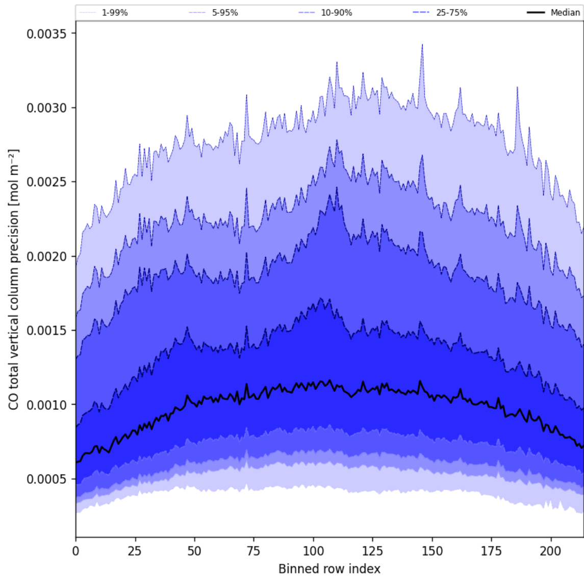
Figure 28: Along track statistics of “CO total vertical column precision” for 2025-04-03 to 2025-04-04
