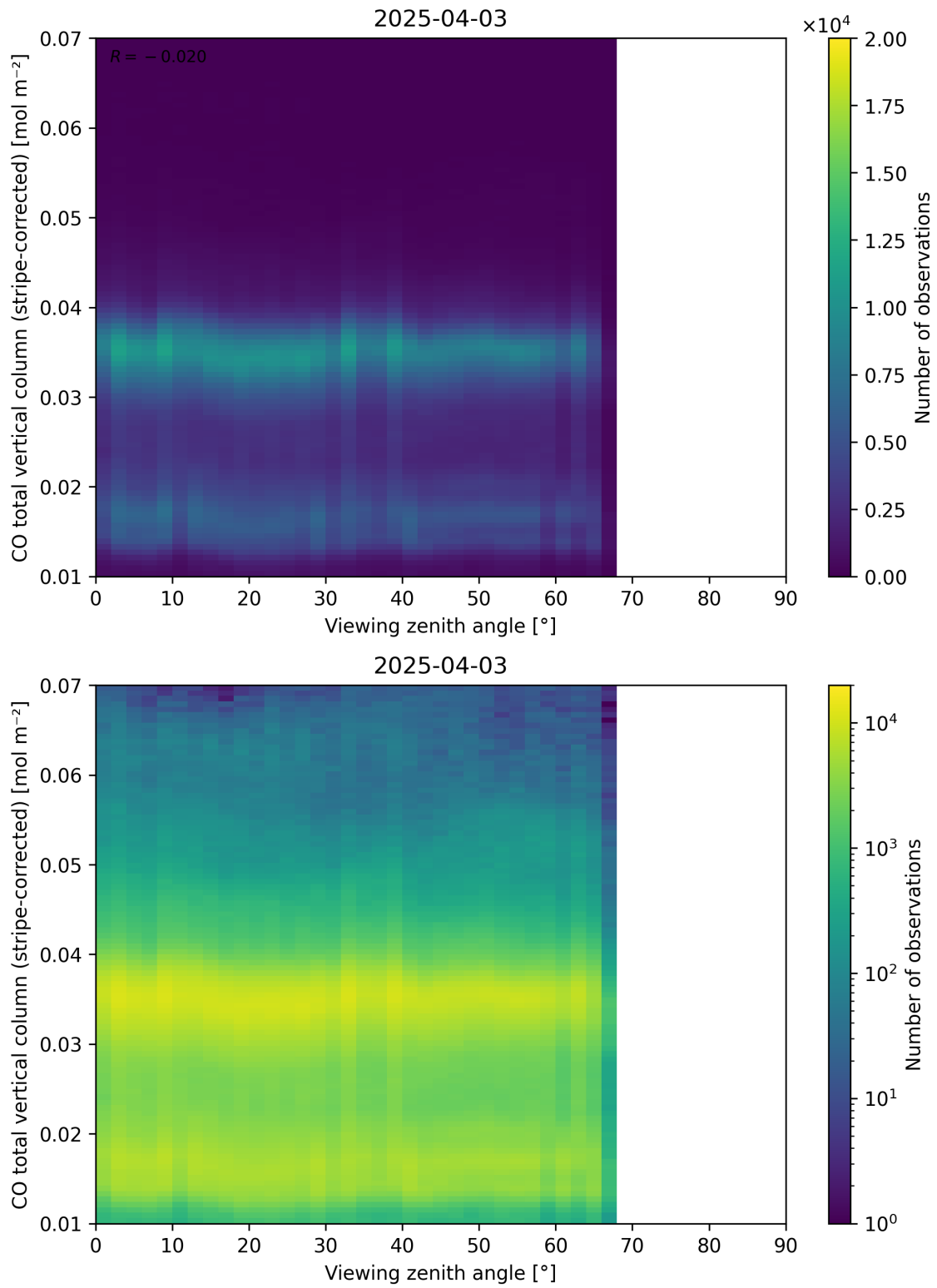
Figure 70: Scatter density plot of “Viewing zenith angle” against “CO total vertical column (stripe-corrected)” for 2025-04-03 to 2025-04-04.
