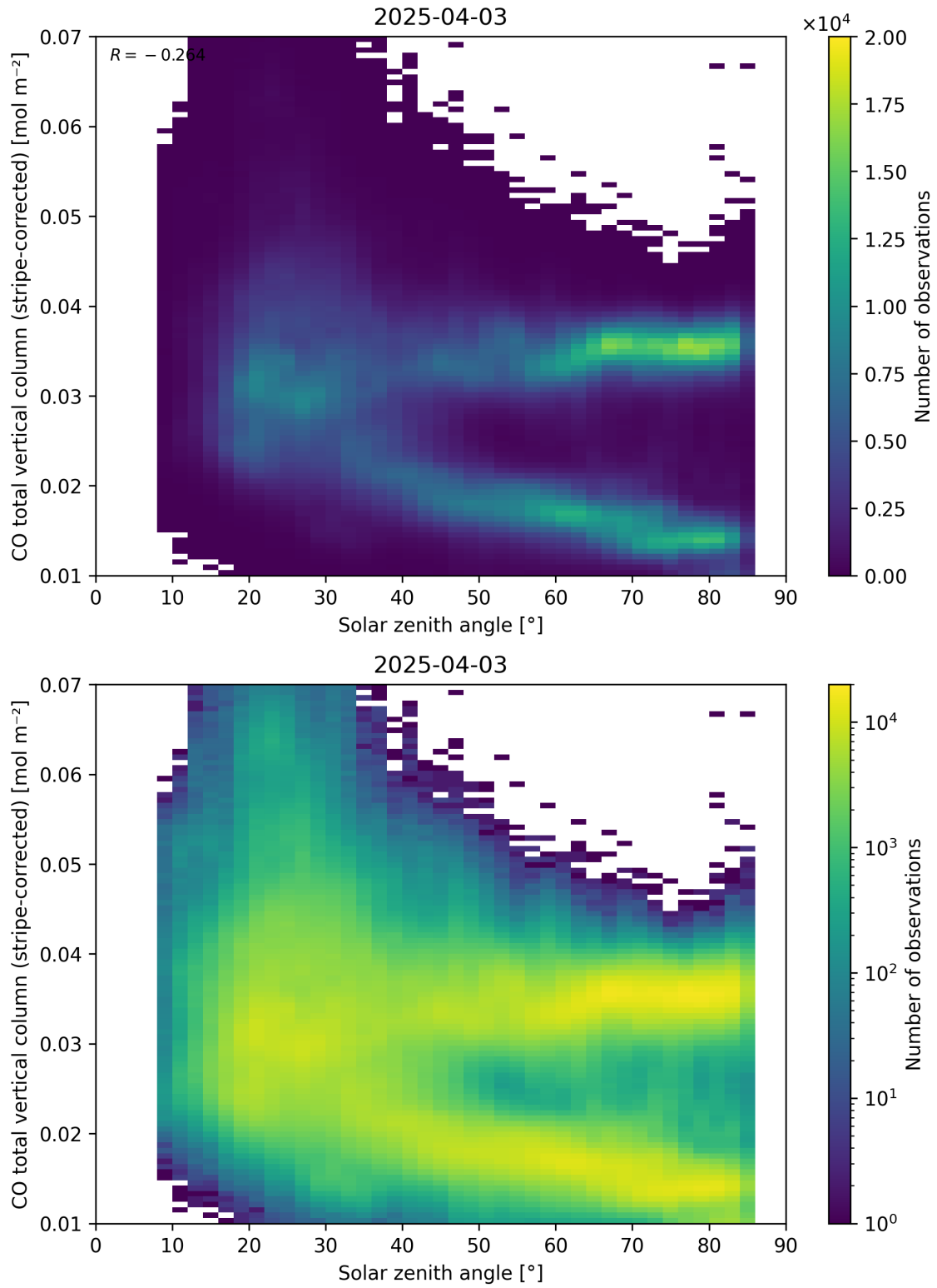
Figure 62: Scatter density plot of “Solar zenith angle” against “CO total vertical column (stripe-corrected)” for 2025-04-03 to 2025-04-04.
