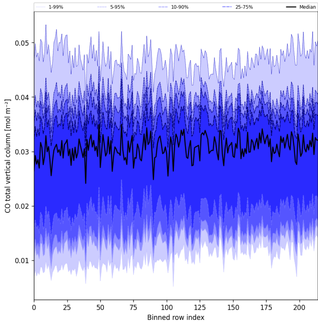
Figure 26: Along track statistics of “CO total vertical column” for 2025-04-04 to 2025-04-06
