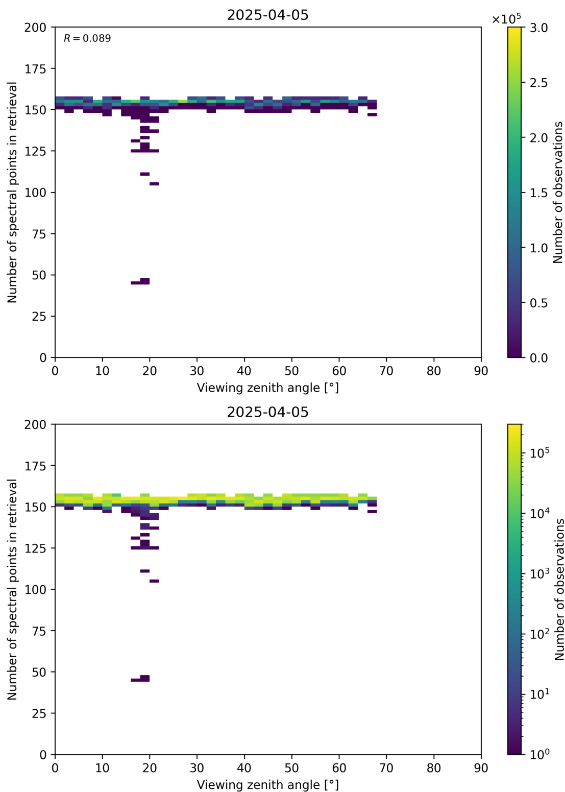
Figure 76: Scatter density plot of “Viewing zenith angle” against “Number of spectral points in retrieval” for 2025-04-04 to 2025-04-06.
