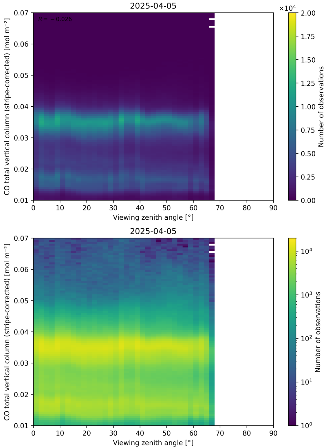
Figure 70: Scatter density plot of “Viewing zenith angle” against “CO total vertical column (stripe-corrected)” for 2025-04-04 to 2025-04-06.
