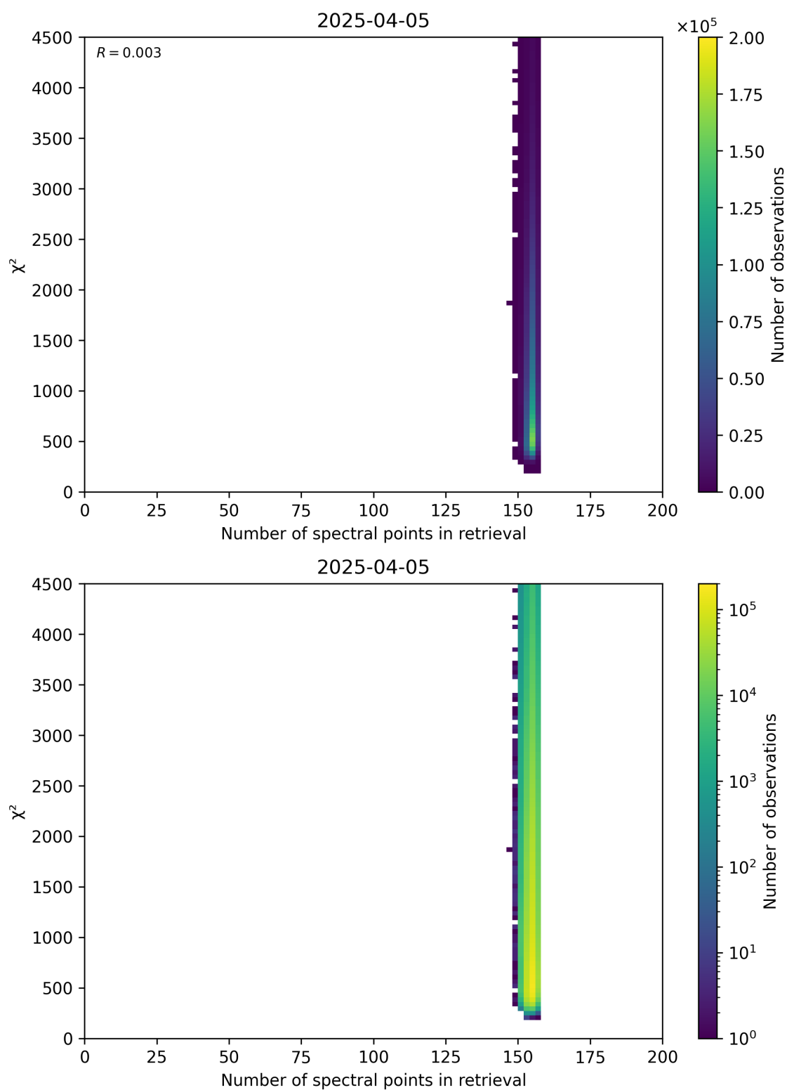
Figure 58: Scatter density plot of “Number of spectral points in retrieval” against “ \chi^2 ” for 2025-04-04 to 2025-04-06.
