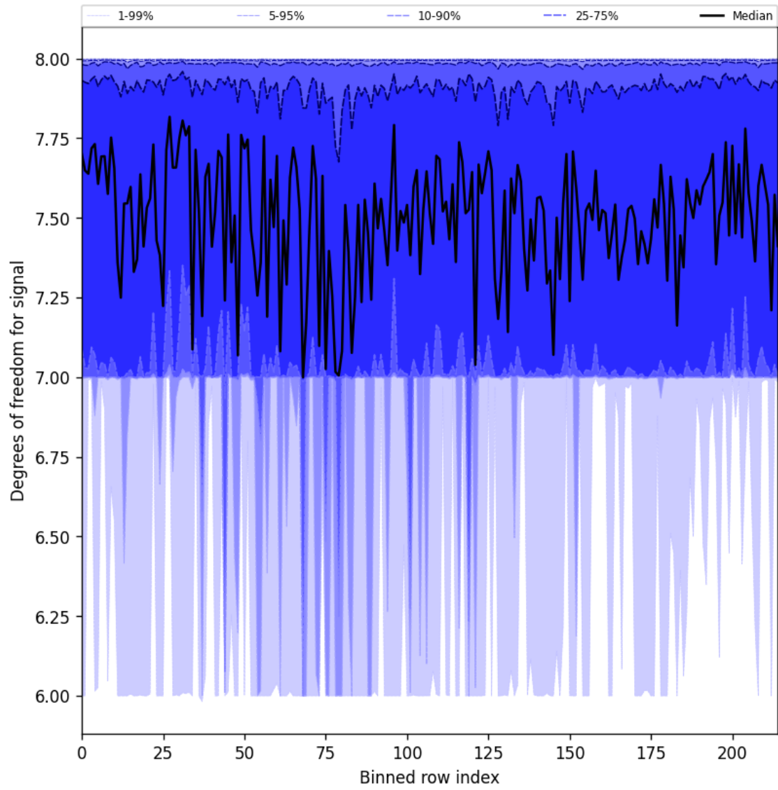
Figure 31: Along track statistics of “Degrees of freedom for signal” for 2025-04-04 to 2025-04-06
