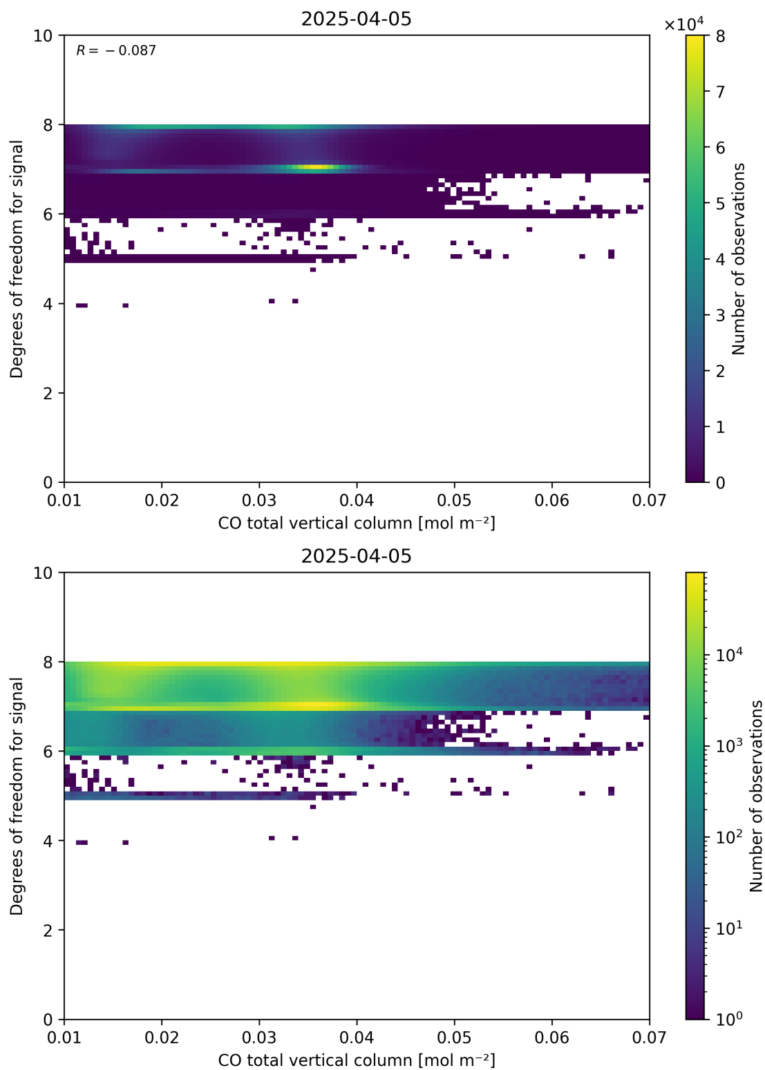
Figure 41: Scatter density plot of “CO total vertical column” against “Degrees of freedom for signal” for 2025-04-04 to 2025-04-06.
