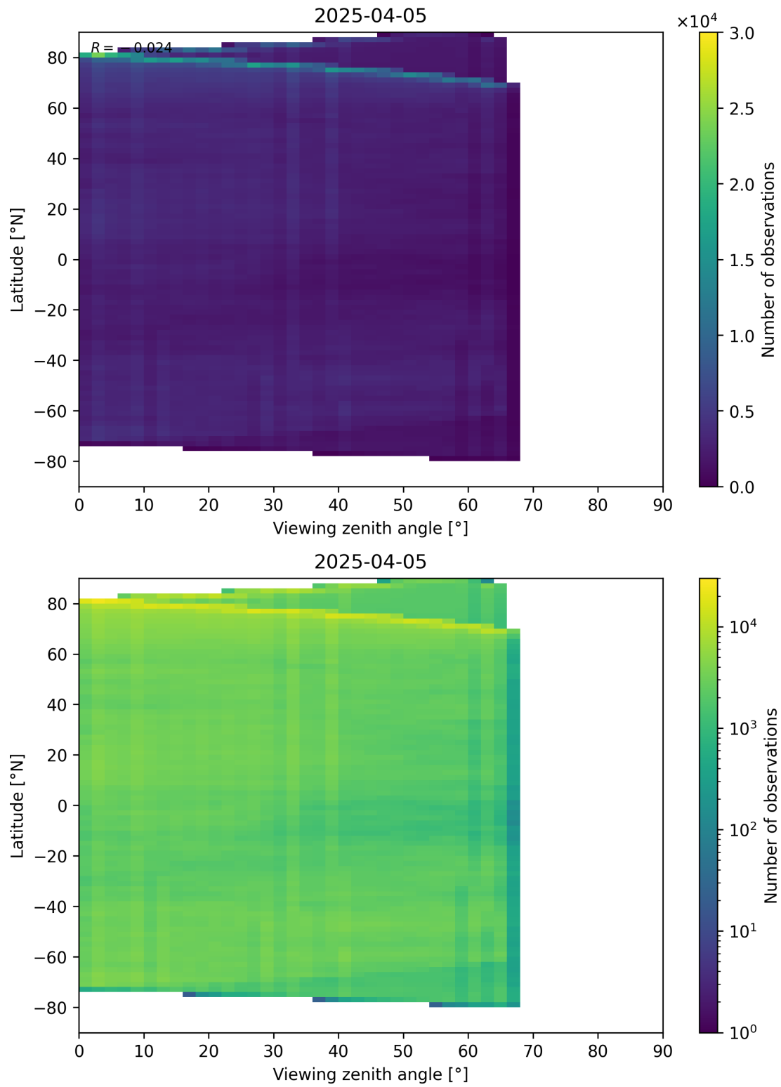
Figure 74: Scatter density plot of “Viewing zenith angle” against “Latitude” for 2025-04-04 to 2025-04-06.
