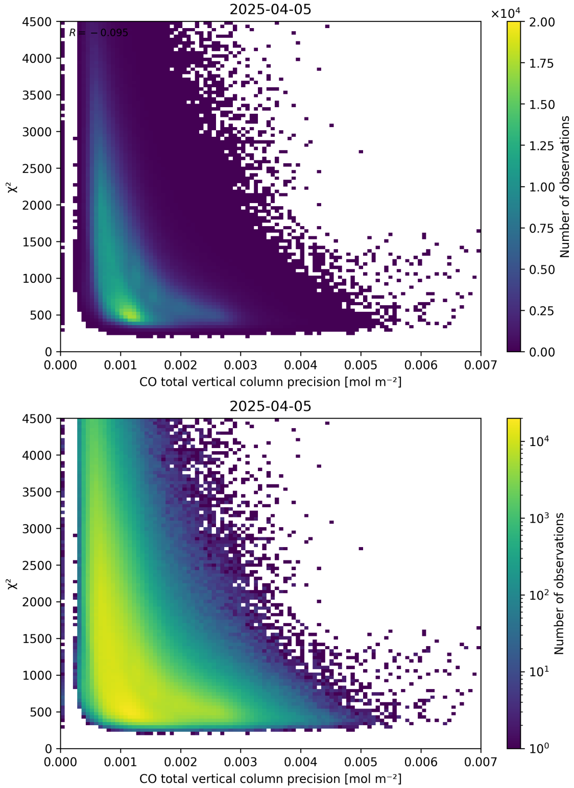
Figure 44: Scatter density plot of “CO total vertical column precision” against “ \chi^2 ” for 2025-04-04 to 2025-04-06.
