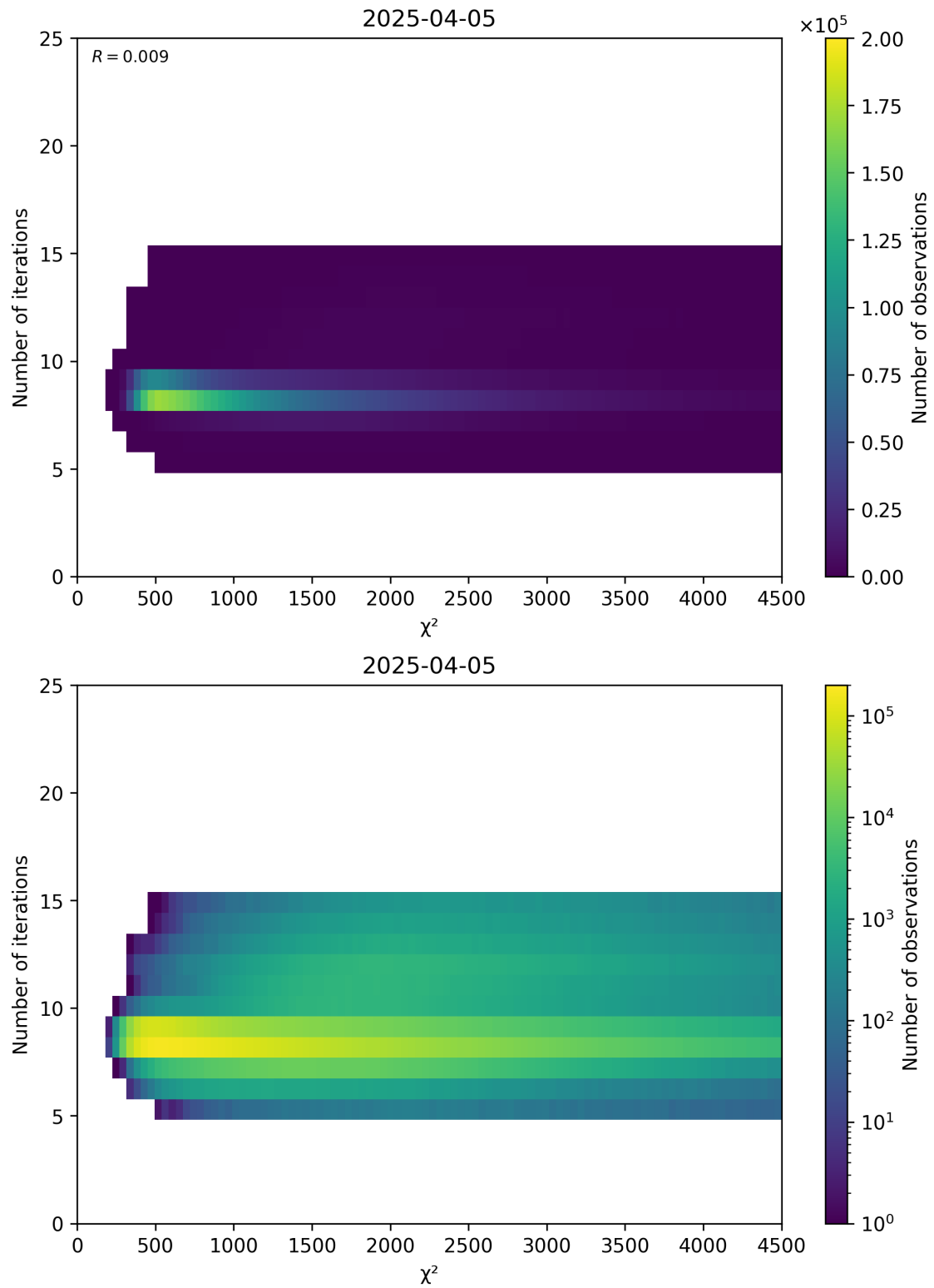
Figure 49: Scatter density plot of “ \chi^2 ” against “Number of iterations” for 2025-04-04 to 2025-04-06.
