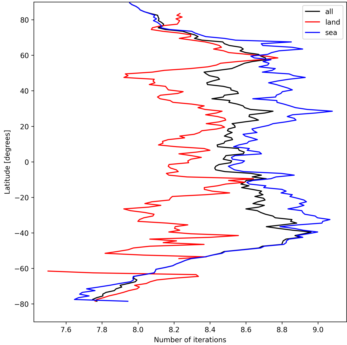
Figure 16: Zonal average of “Number of iterations” for 2025-04-04 to 2025-04-06.
