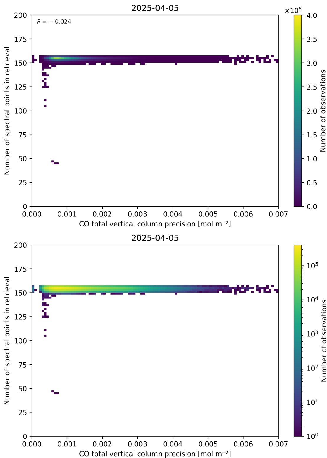
Figure 47: Scatter density plot of “CO total vertical column precision” against “Number of spectral points in retrieval” for 2025-04-04 to 2025-04-06.
