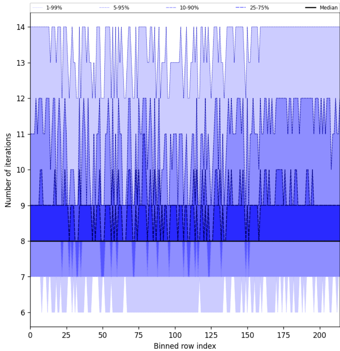
Figure 32: Along track statistics of “Number of iterations” for 2025-04-04 to 2025-04-06
