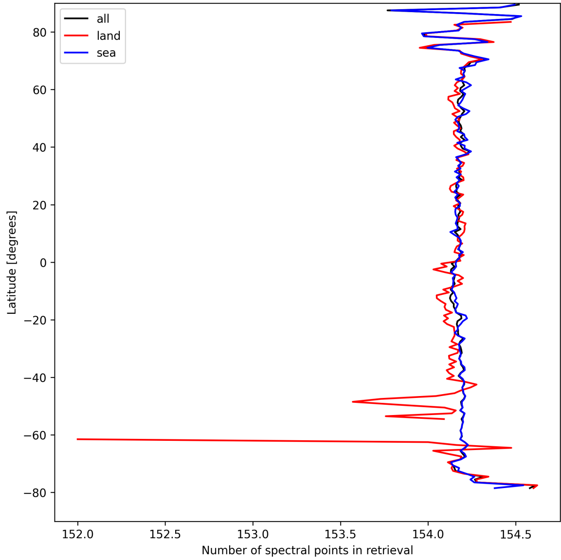
Figure 13: Zonal average of “Number of spectral points in retrieval” for 2025-04-04 to 2025-04-06.
