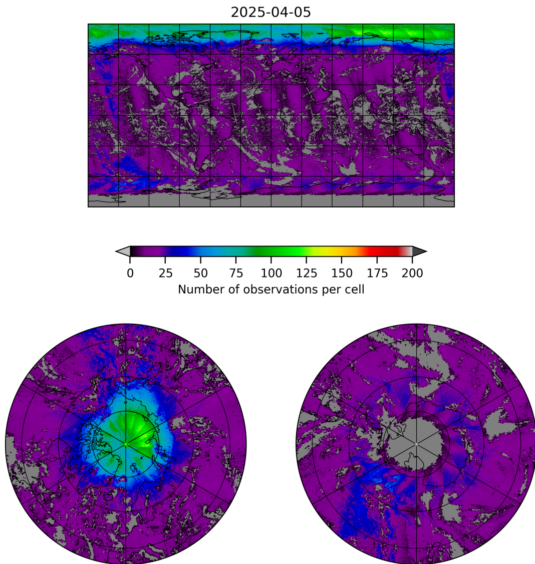
Figure 8: Map of the number of observations for 2025-04-04 to 2025-04-06
