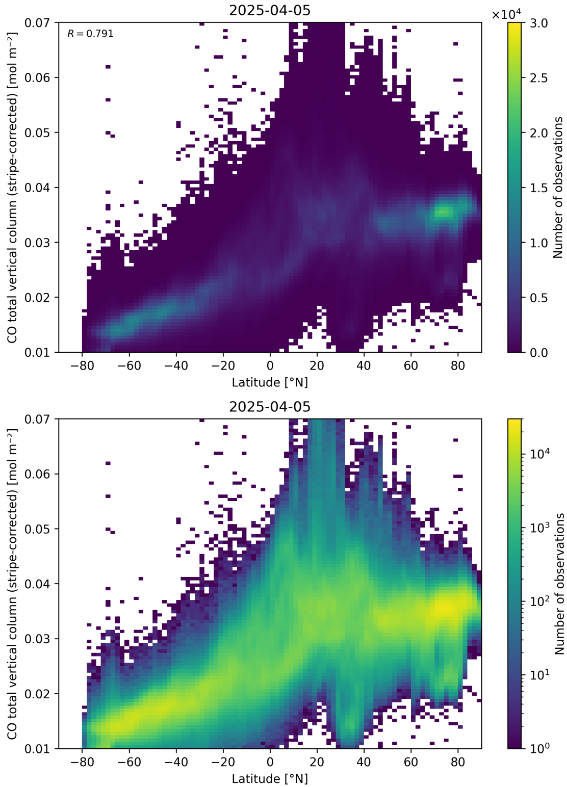
Figure 52: Scatter density plot of “Latitude” against “CO total vertical column (stripe-corrected)” for 2025-04-04 to 2025-04-06.
