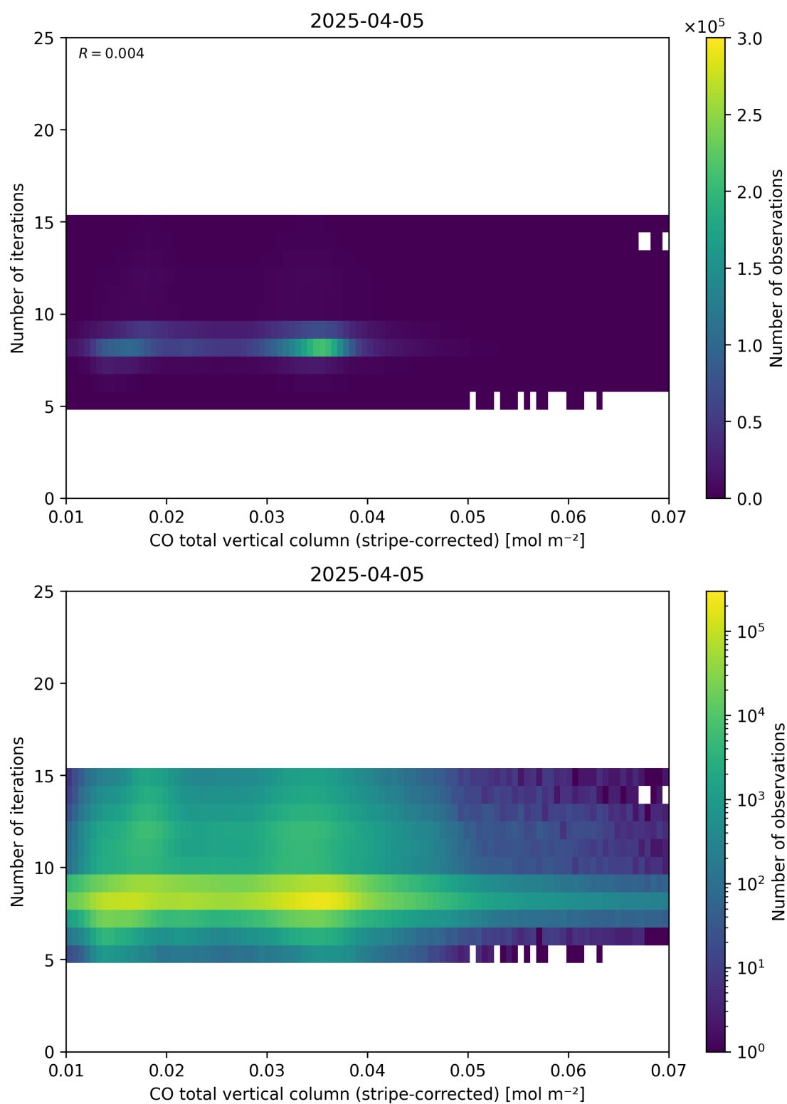
Figure 39: Scatter density plot of “CO total vertical column (stripe-corrected)” against “Number of iterations” for 2025-04-04 to 2025-04-06.
