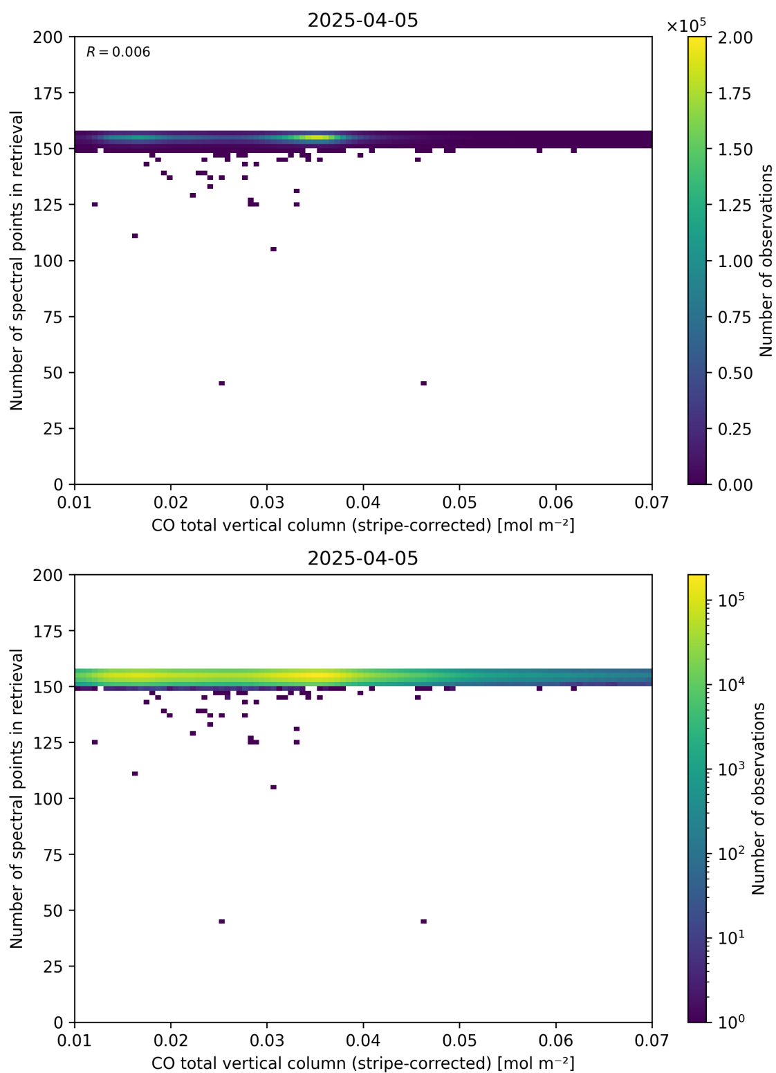
Figure 40: Scatter density plot of “CO total vertical column (stripe-corrected)” against “Number of spectral points in retrieval” for 2025-04-04 to 2025-04-06.
