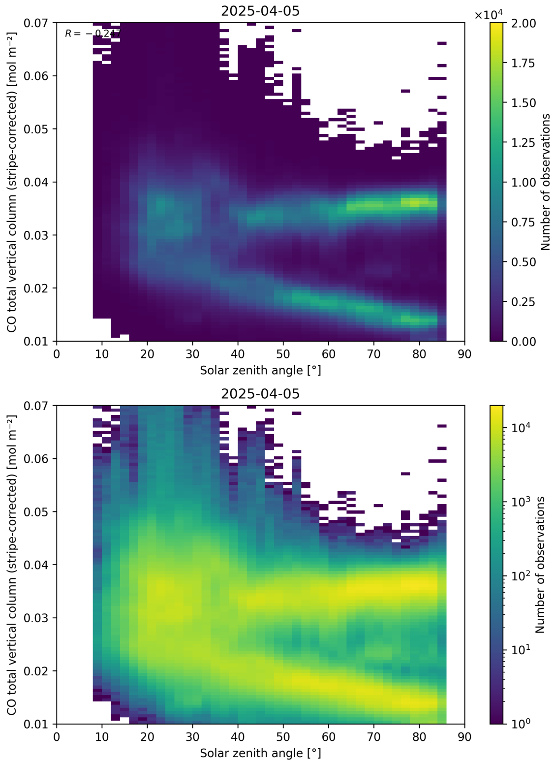
Figure 62: Scatter density plot of “Solar zenith angle” against “CO total vertical column (stripe-corrected)” for 2025-04-04 to 2025-04-06.
