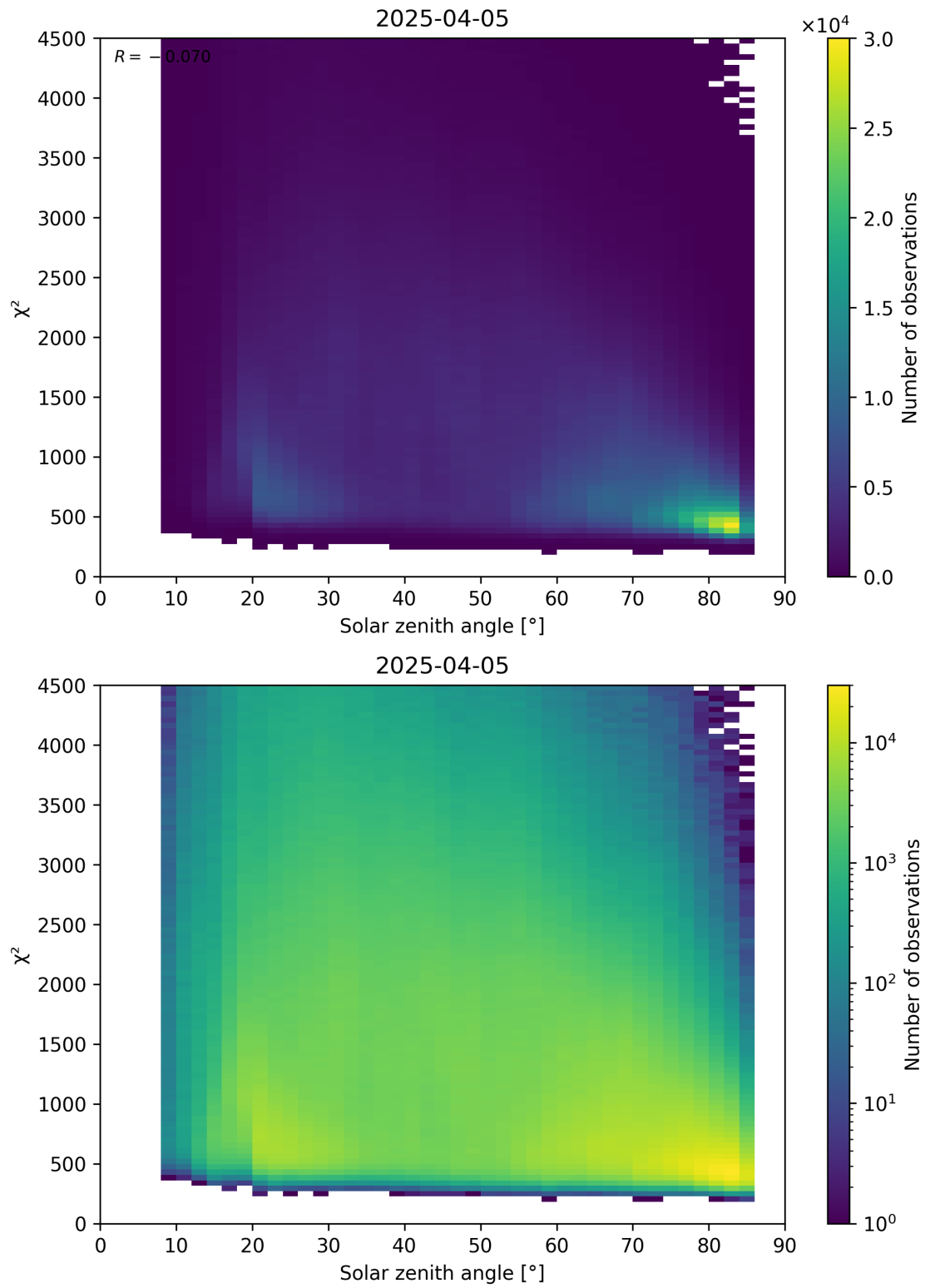
Figure 64: Scatter density plot of “Solar zenith angle” against “ \chi^2 ” for 2025-04-04 to 2025-04-06.
