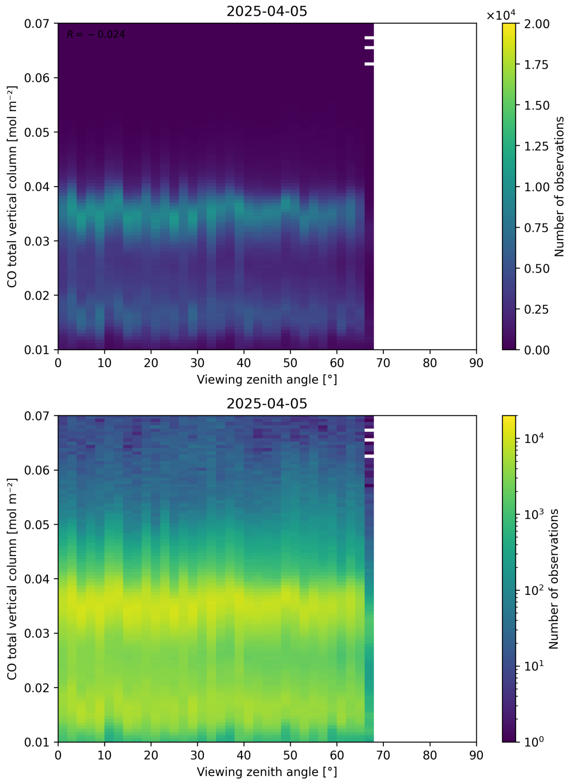
Figure 69: Scatter density plot of “Viewing zenith angle” against “CO total vertical column” for 2025-04-04 to 2025-04-06.
