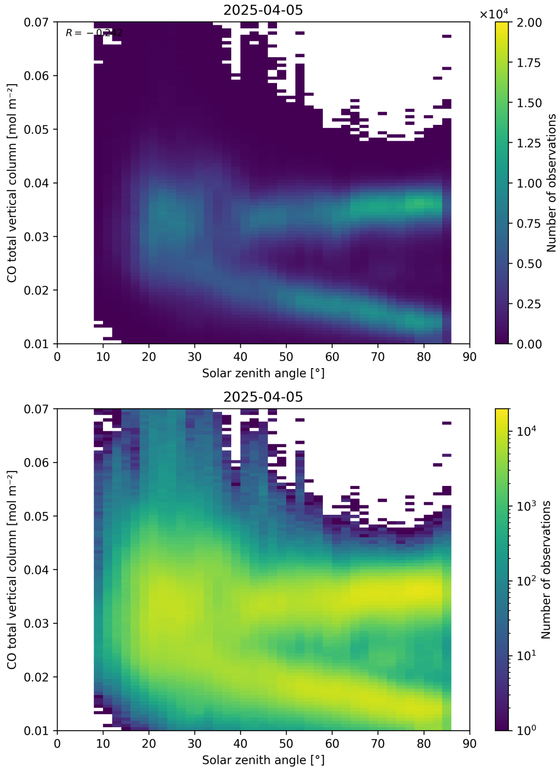
Figure 61: Scatter density plot of “Solar zenith angle” against “CO total vertical column” for 2025-04-04 to 2025-04-06.
