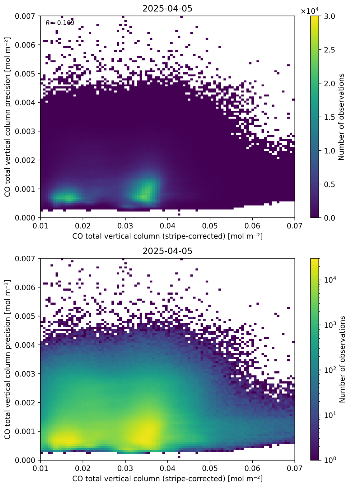
Figure 36: Scatter density plot of “CO total vertical column (stripe-corrected)” against “CO total vertical column precision” for 2025-04-04 to 2025-04-06.
