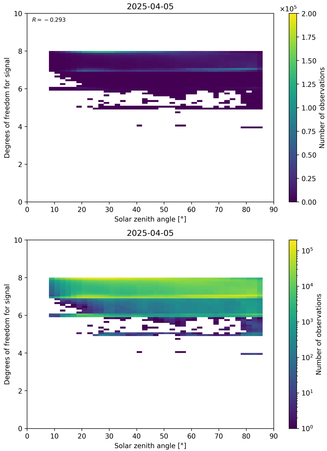
Figure 65: Scatter density plot of “Solar zenith angle” against “Degrees of freedom for signal” for 2025-04-04 to 2025-04-06.
