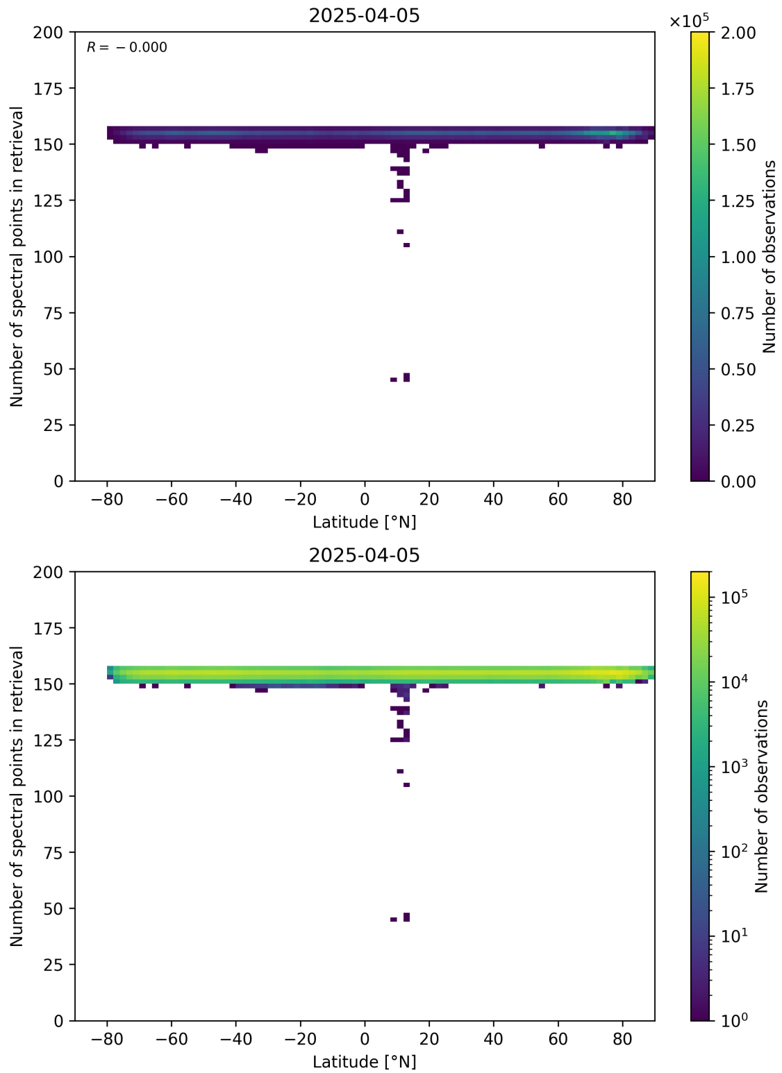
Figure 57: Scatter density plot of “Latitude” against “Number of spectral points in retrieval” for 2025-04-04 to 2025-04-06.
