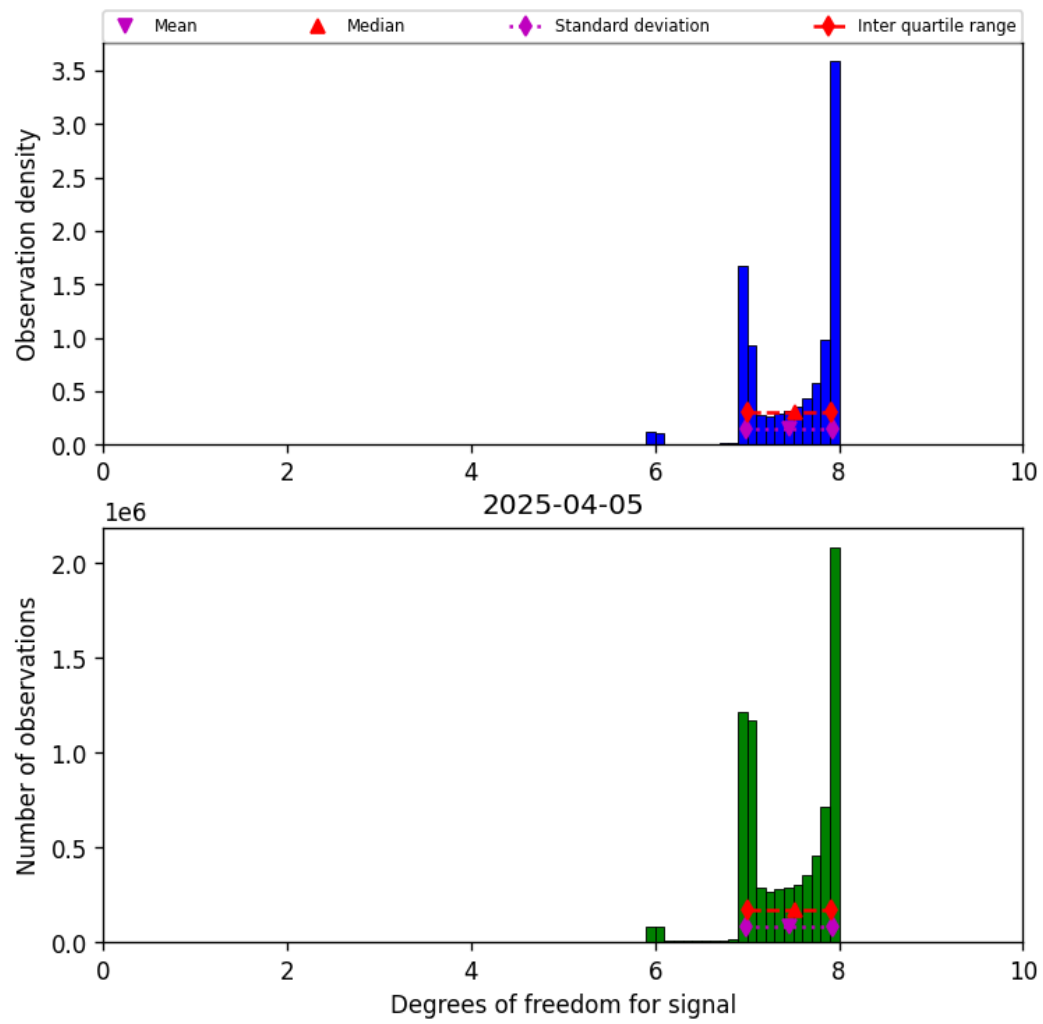
Figure 23: Histogram of “Degrees of freedom for signal” for 2025-04-04 to 2025-04-06
