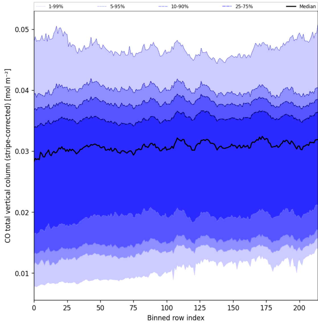
Figure 27: Along track statistics of "CO total vertical column (stripe-corrected)" for 2025-04-04 to 2025-04-06
