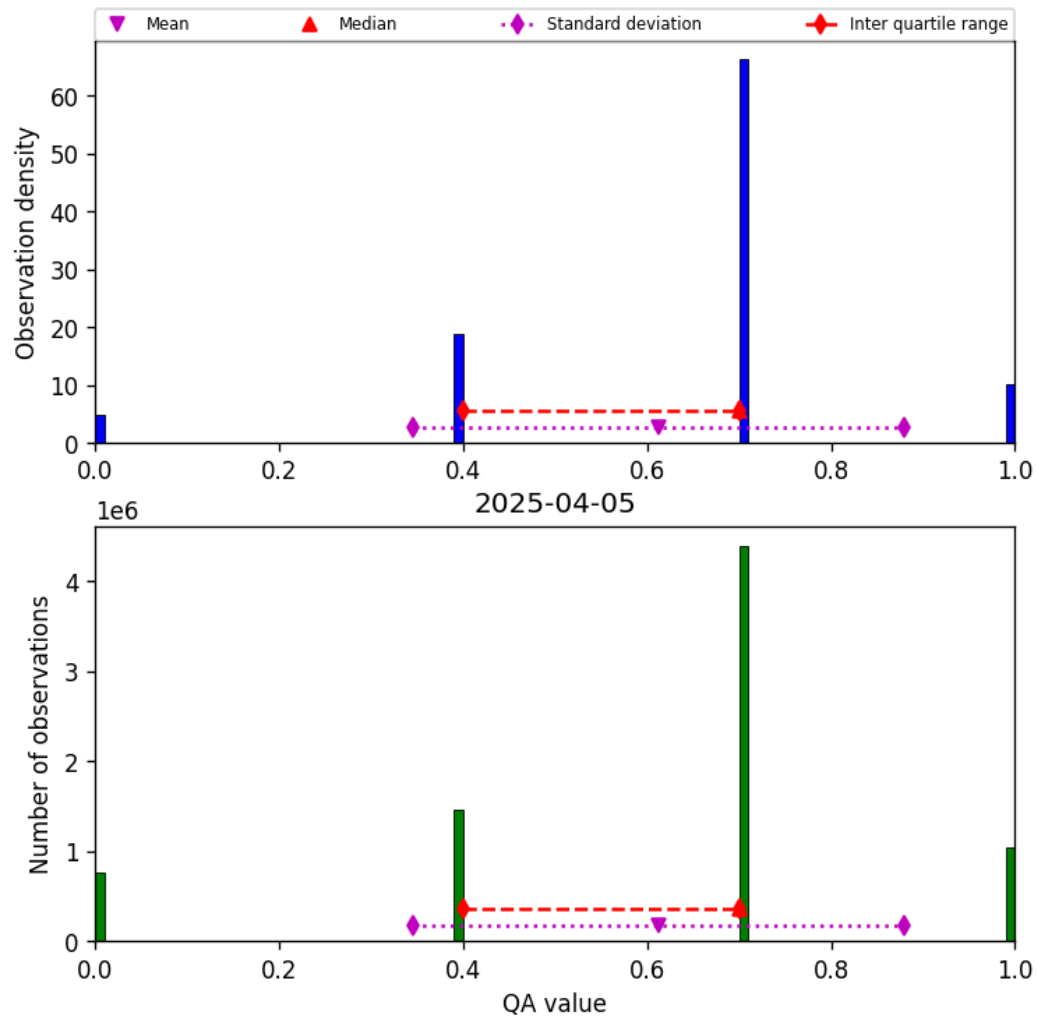
Figure 17: Histogram of “QA value” for 2025-04-04 to 2025-04-06
