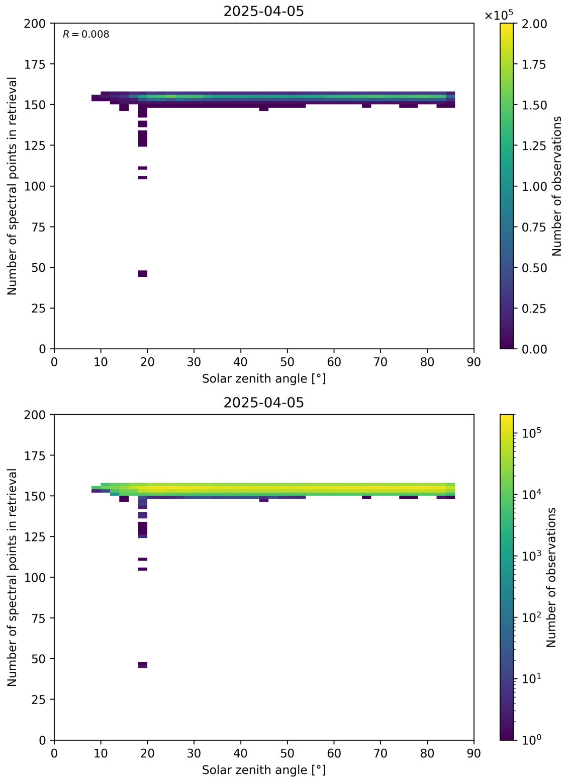
Figure 68: Scatter density plot of “Solar zenith angle” against “Number of spectral points in retrieval” for 2025-04-04 to 2025-04-06.
