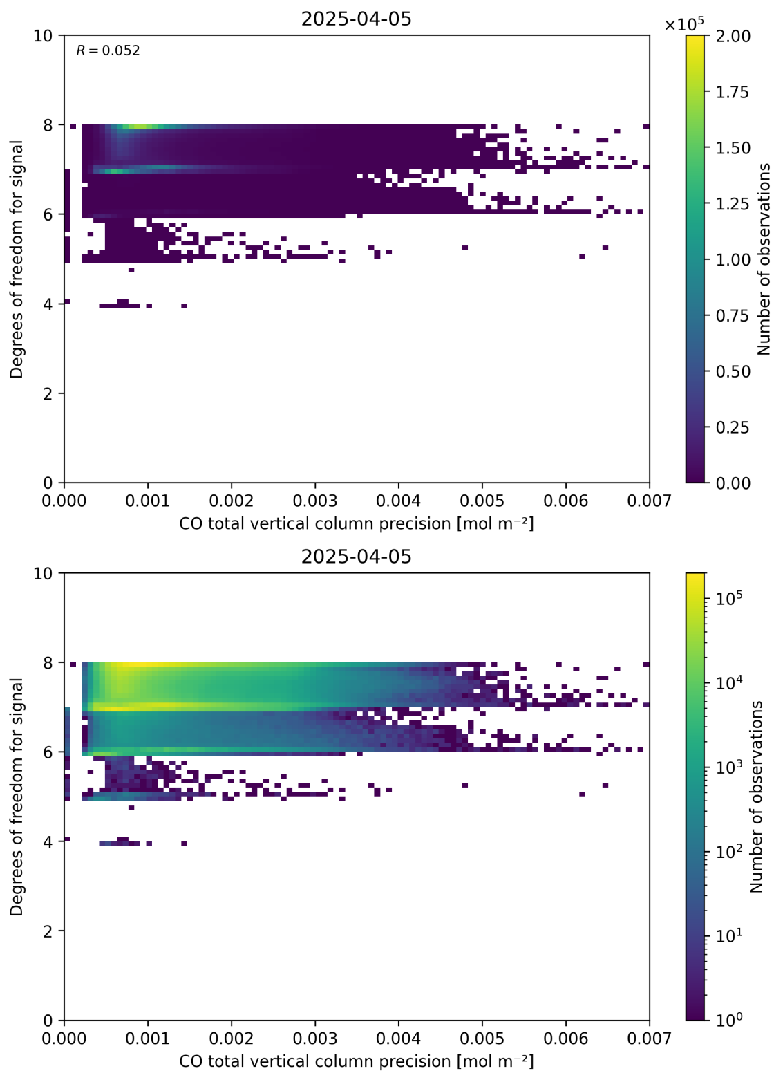
Figure 45: Scatter density plot of “CO total vertical column precision” against “Degrees of freedom for signal” for 2025-04-04 to 2025-04-06.
