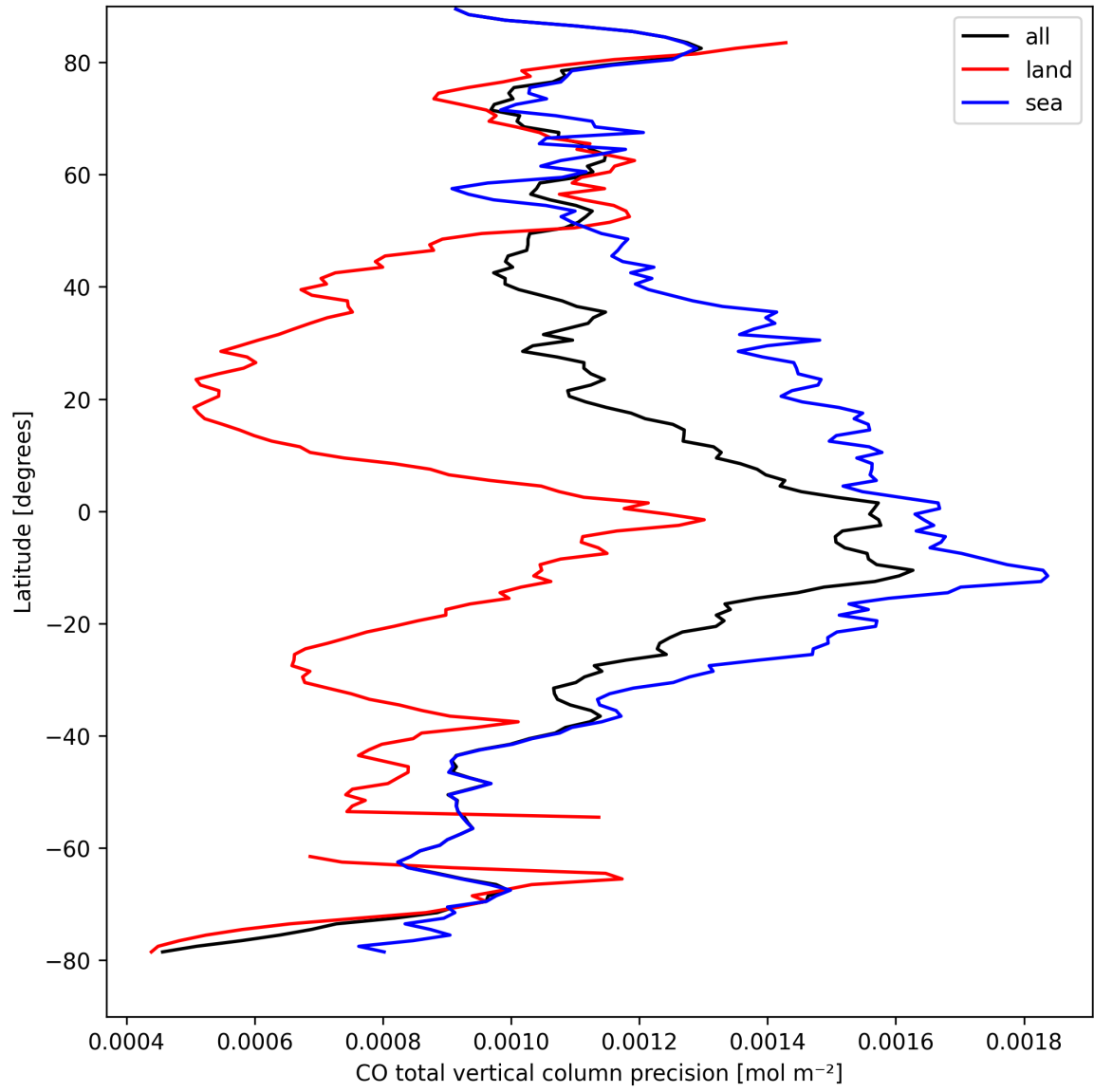
Figure 12: Zonal average of “CO total vertical column precision” for 2025-04-04 to 2025-04-06.
