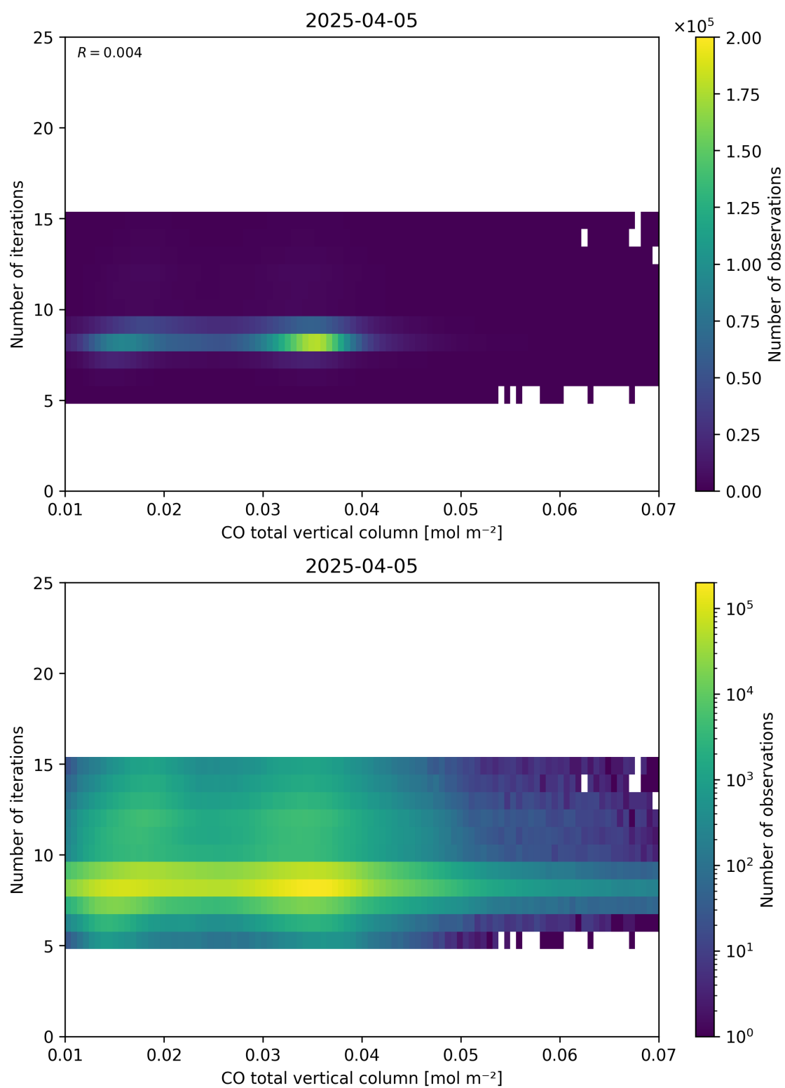
Figure 42: Scatter density plot of “CO total vertical column” against “Number of iterations” for 2025-04-04 to 2025-04-06.
