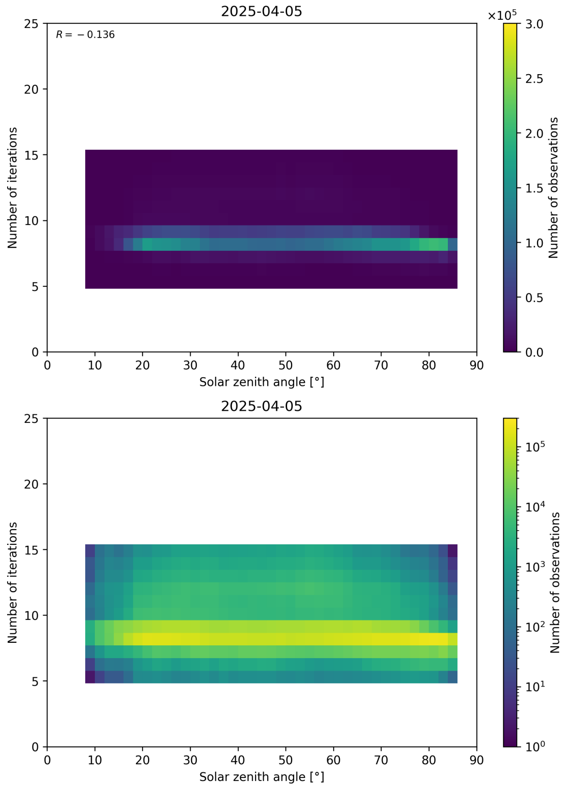
Figure 67: Scatter density plot of “Solar zenith angle” against “Number of iterations” for 2025-04-04 to 2025-04-06.
