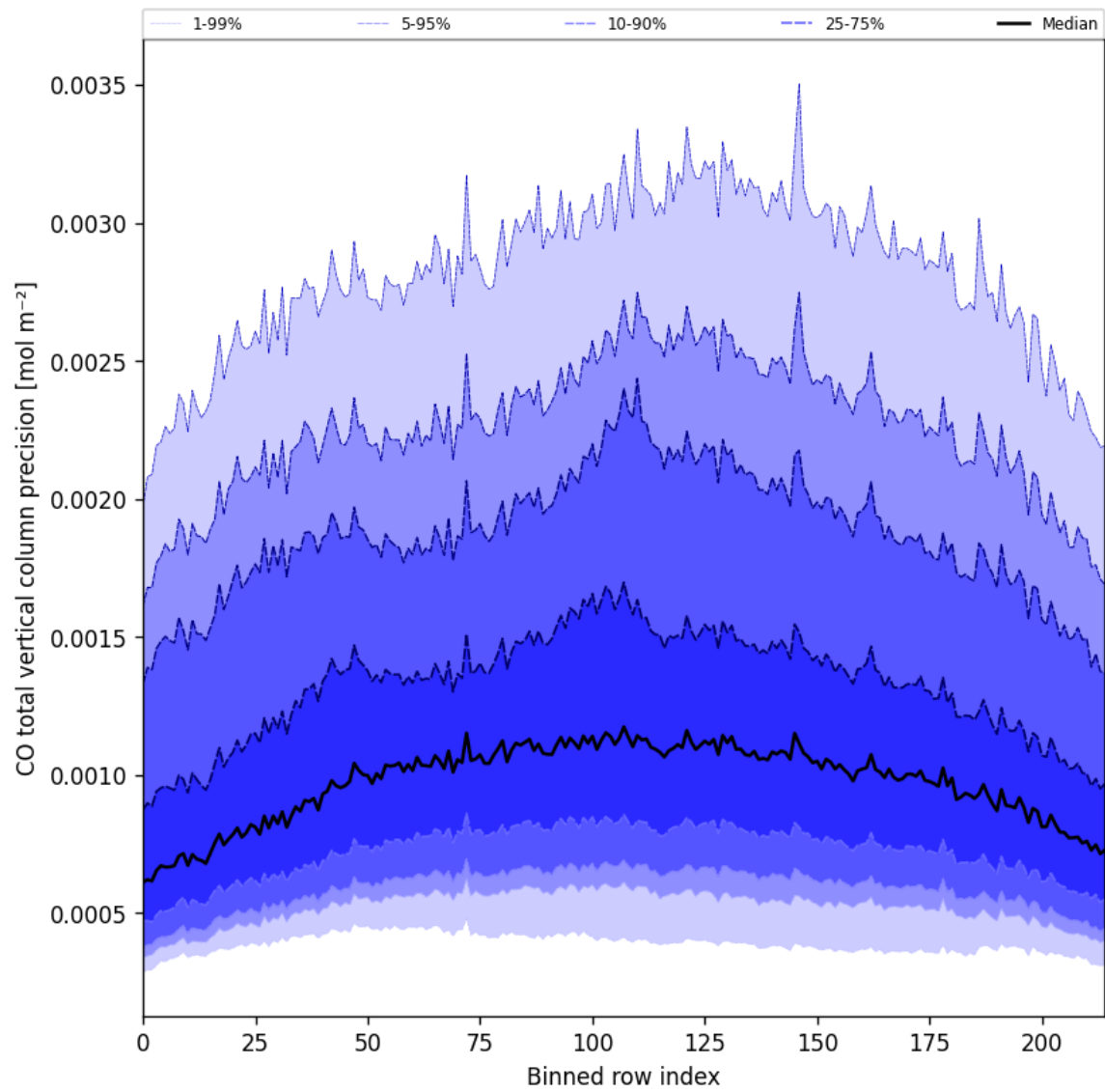
Figure 28: Along track statistics of “CO total vertical column precision” for 2025-04-04 to 2025-04-06
