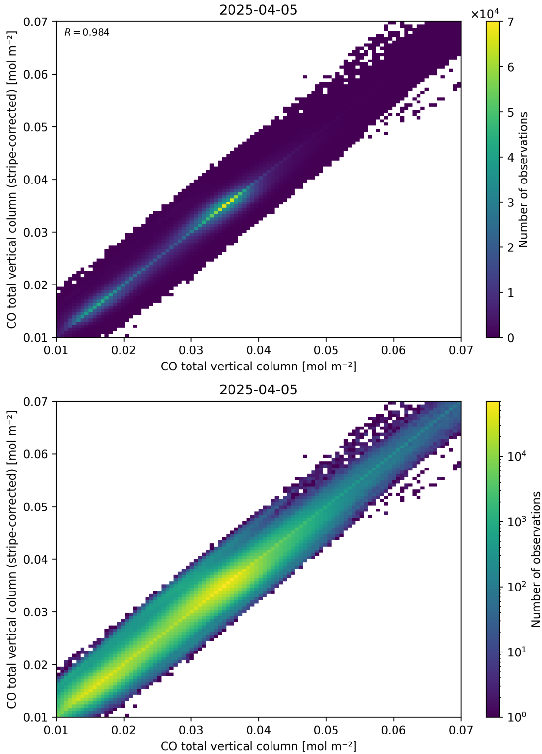
Figure 33: Scatter density plot of “CO total vertical column” against “CO total vertical column (stripe-corrected)” for 2025-04-04 to 2025-04-06.
