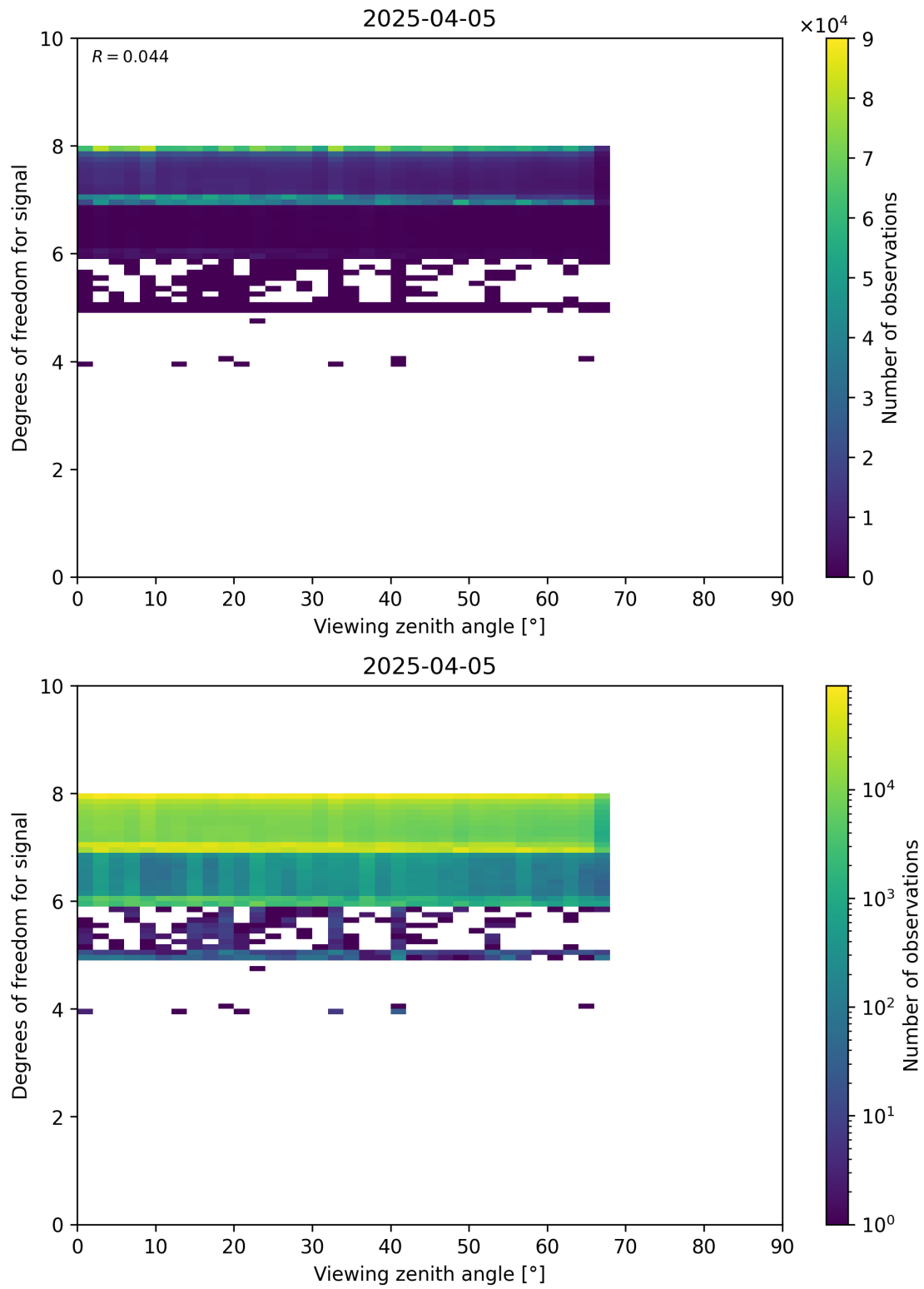
Figure 73: Scatter density plot of “Viewing zenith angle” against “Degrees of freedom for signal” for 2025-04-04 to 2025-04-06.
