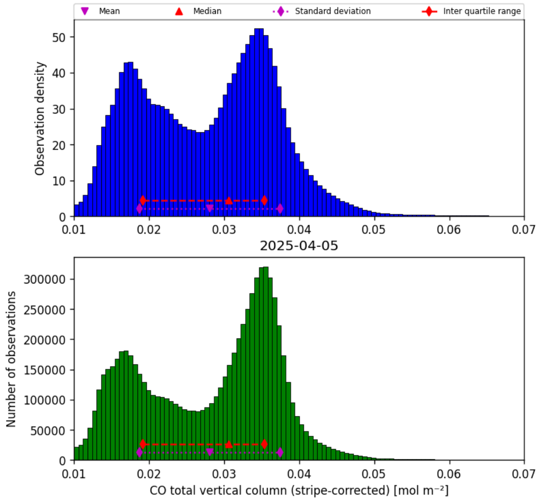
Figure 19: Histogram of “CO total vertical column (stripe-corrected)” for 2025-04-04 to 2025-04-06
