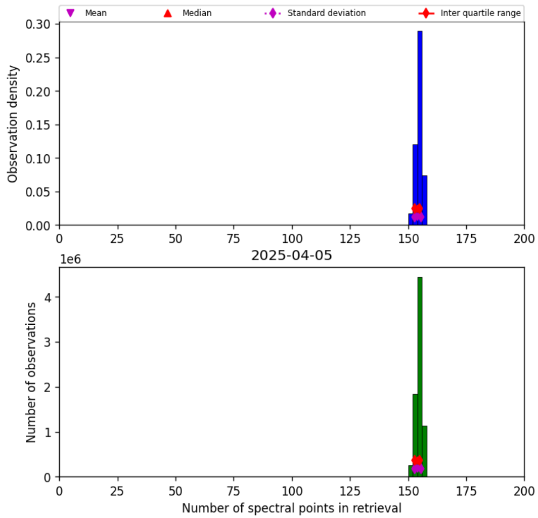
Figure 21: Histogram of “Number of spectral points in retrieval” for 2025-04-04 to 2025-04-06
