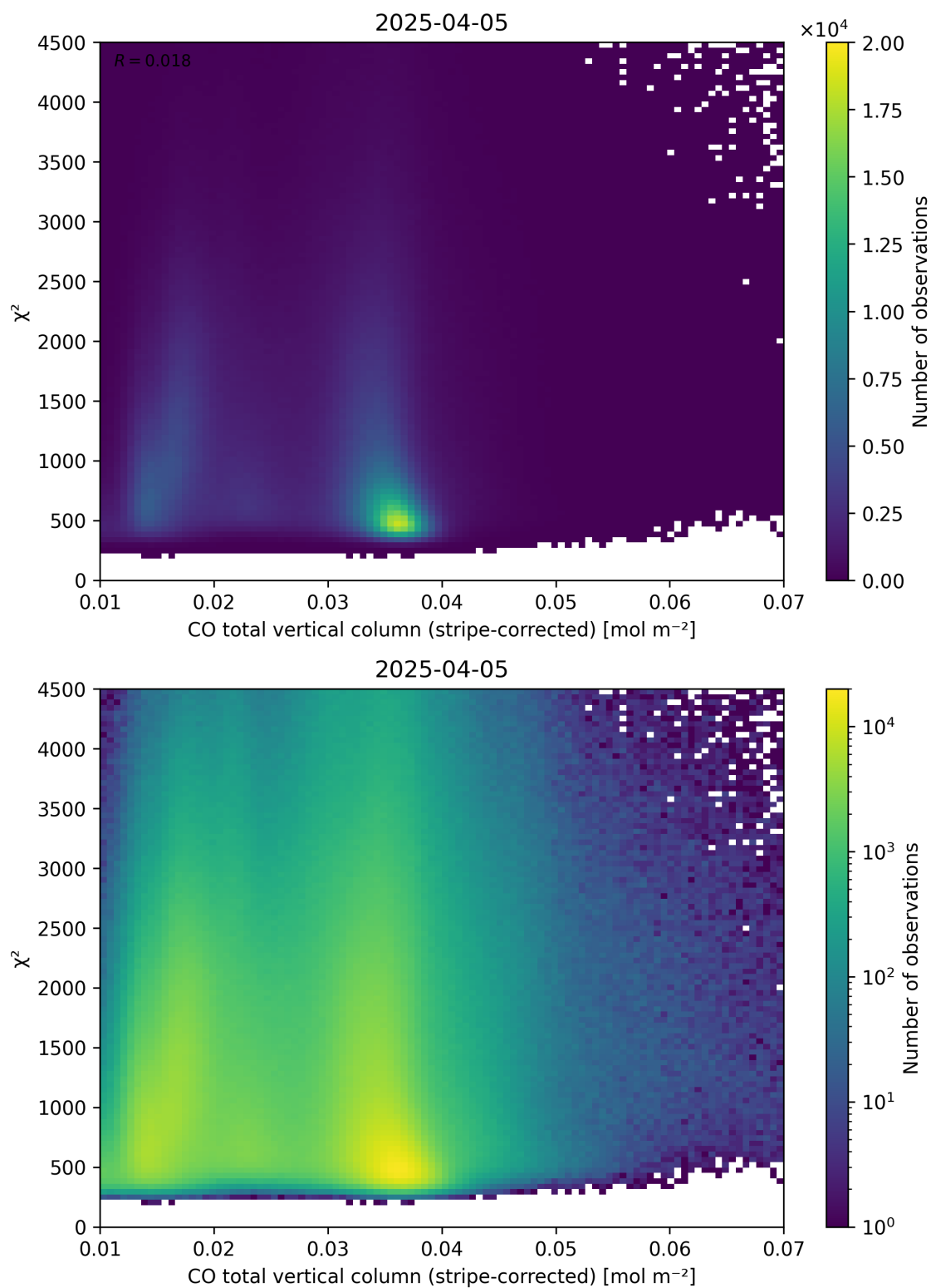
Figure 37: Scatter density plot of “CO total vertical column (stripe-corrected)” against “ \chi^2 ” for 2025-04-04 to 2025-04-06.
