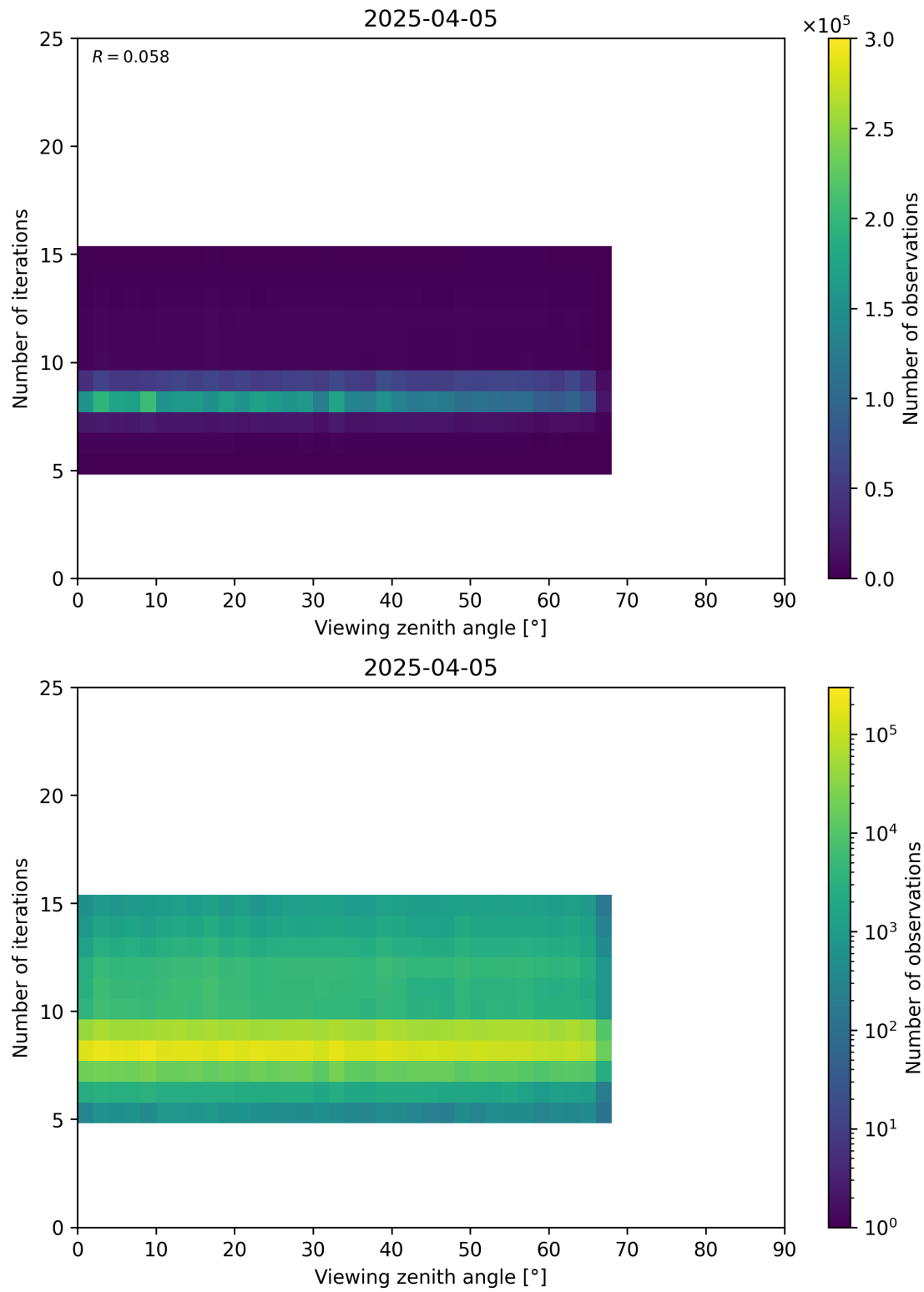
Figure 75: Scatter density plot of “Viewing zenith angle” against “Number of iterations” for 2025-04-04 to 2025-04-06.
