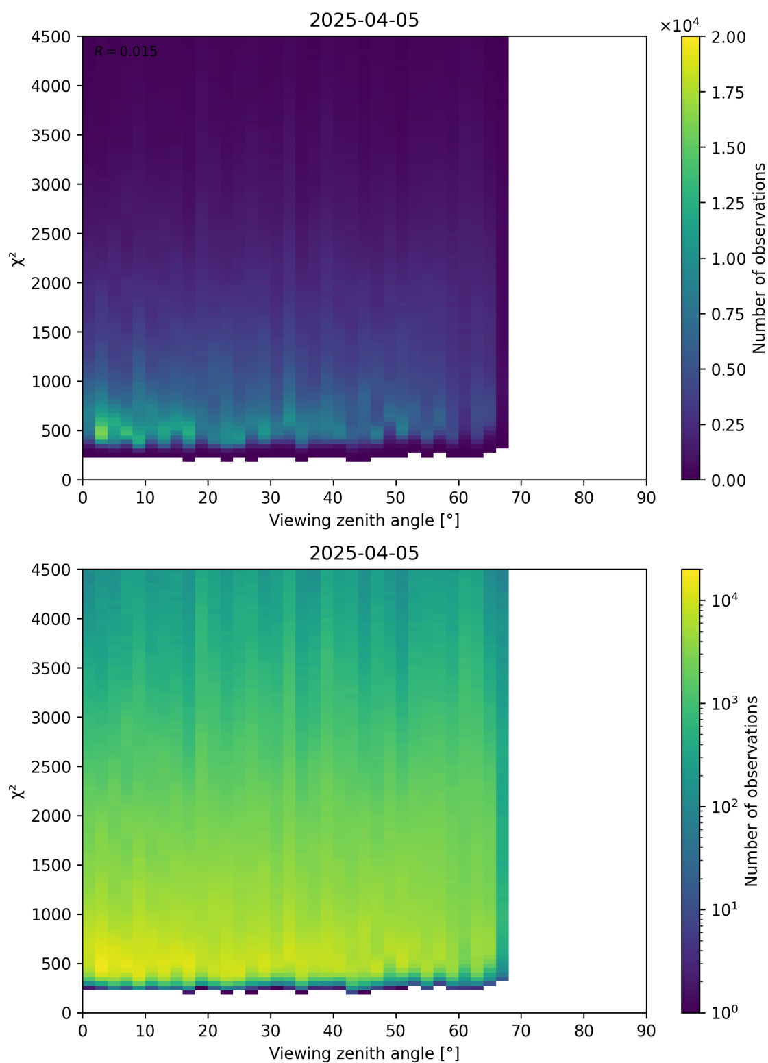
Figure 72: Scatter density plot of “Viewing zenith angle” against “ \chi^2 ” for 2025-04-04 to 2025-04-06.
