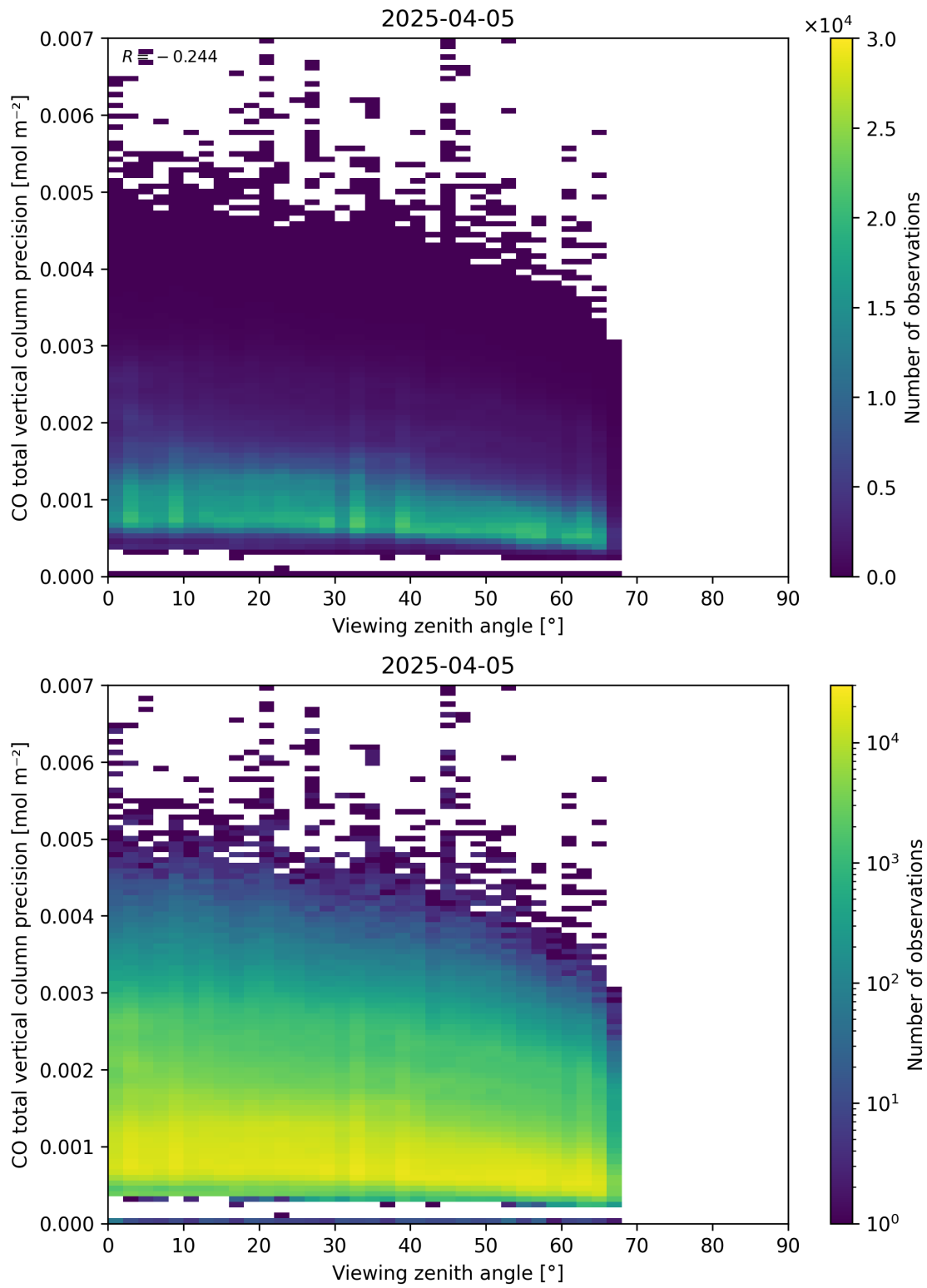
Figure 71: Scatter density plot of “Viewing zenith angle” against “CO total vertical column precision” for 2025-04-04 to 2025-04-06.
