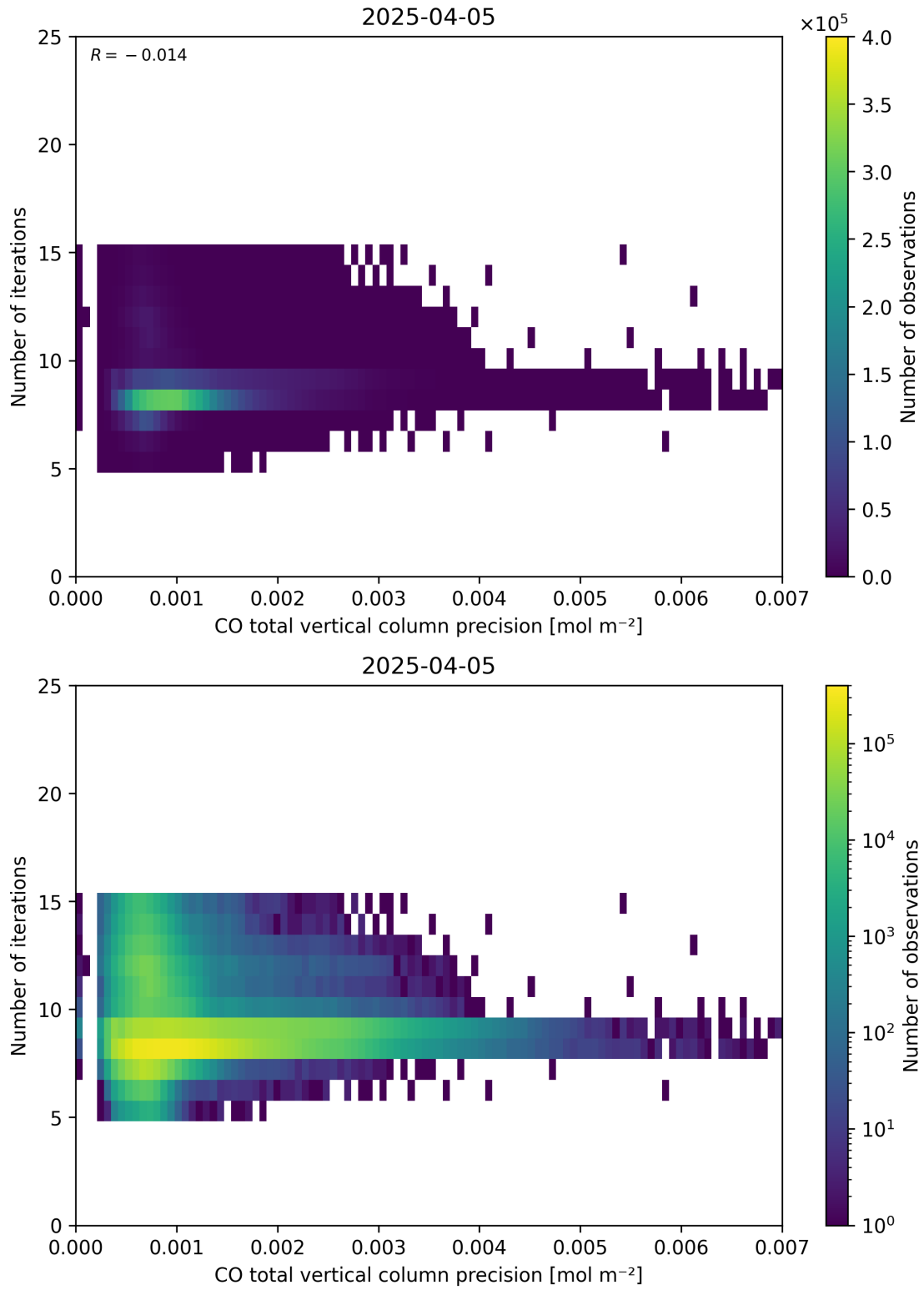
Figure 46: Scatter density plot of “CO total vertical column precision” against “Number of iterations” for 2025-04-04 to 2025-04-06.
