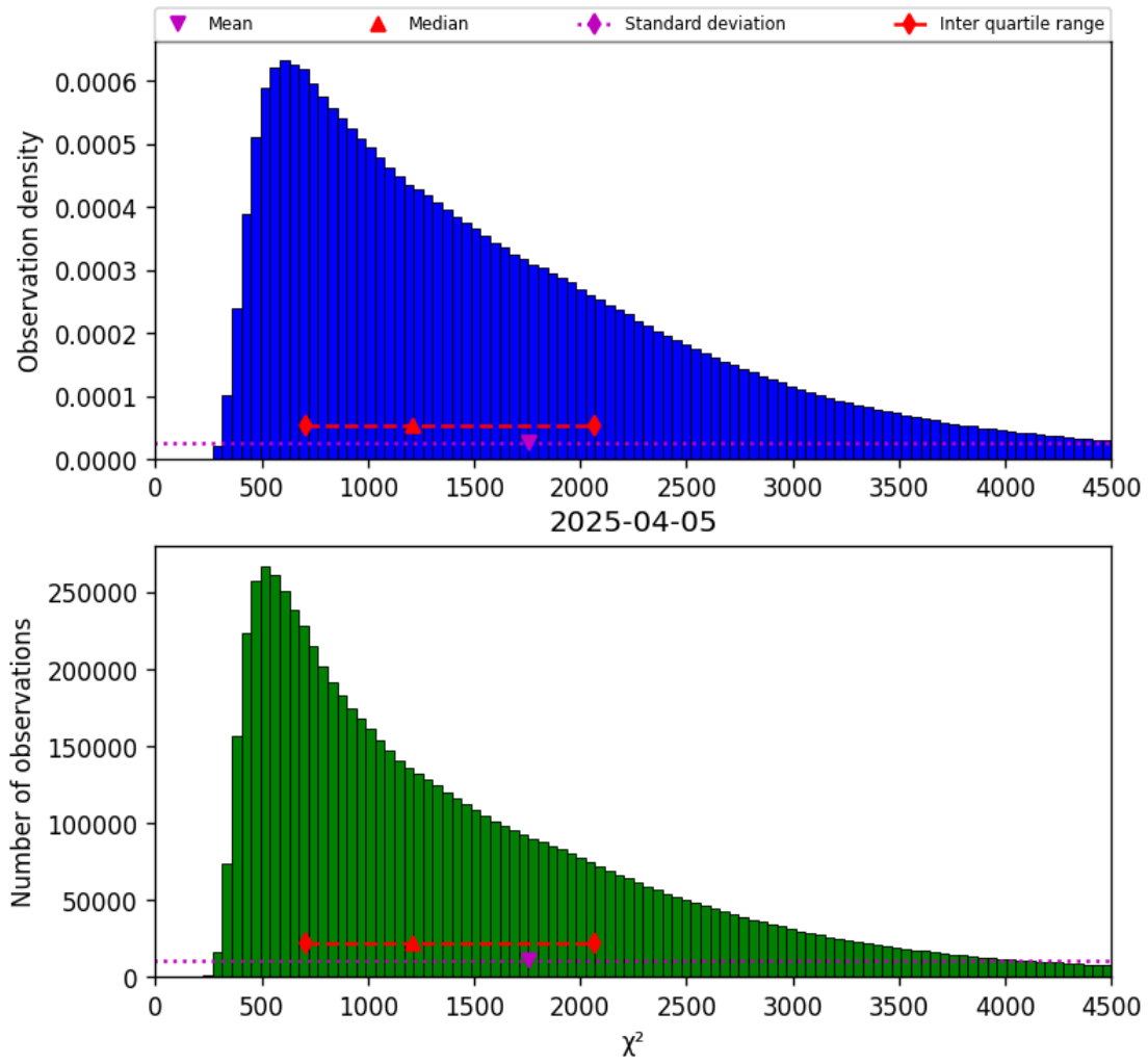
Figure 22: Histogram of “ \chi^2 ” for 2025-04-04 to 2025-04-06
