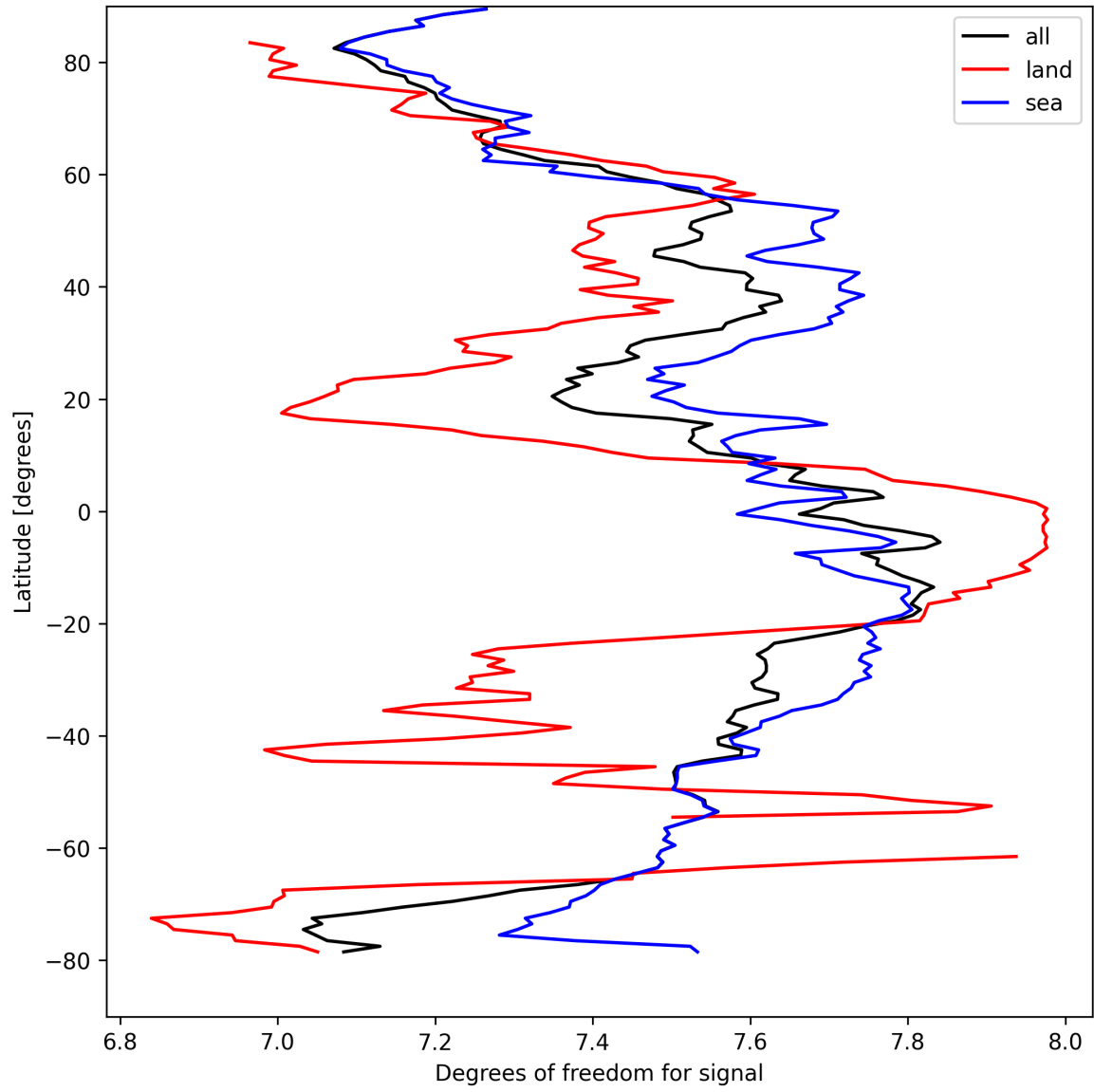
Figure 15: Zonal average of “Degrees of freedom for signal” for 2025-04-04 to 2025-04-06.
