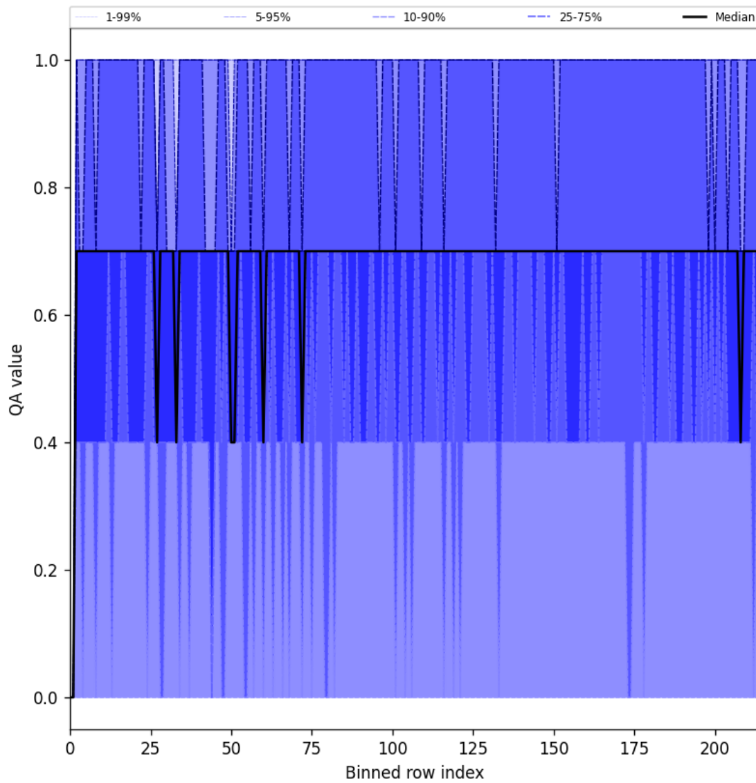
Figure 25: Along track statistics of “QA value” for 2025-04-04 to 2025-04-06
