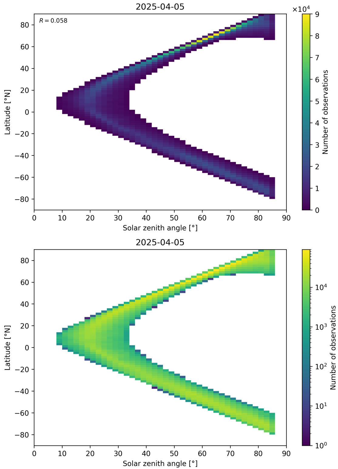
Figure 66: Scatter density plot of “Solar zenith angle” against “Latitude” for 2025-04-04 to 2025-04-06.
