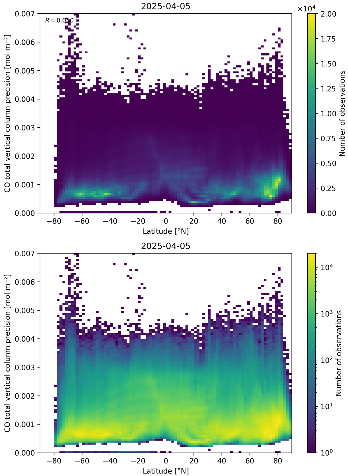
Figure 53: Scatter density plot of “Latitude” against “CO total vertical column precision” for 2025-04-04 to 2025-04-06.
