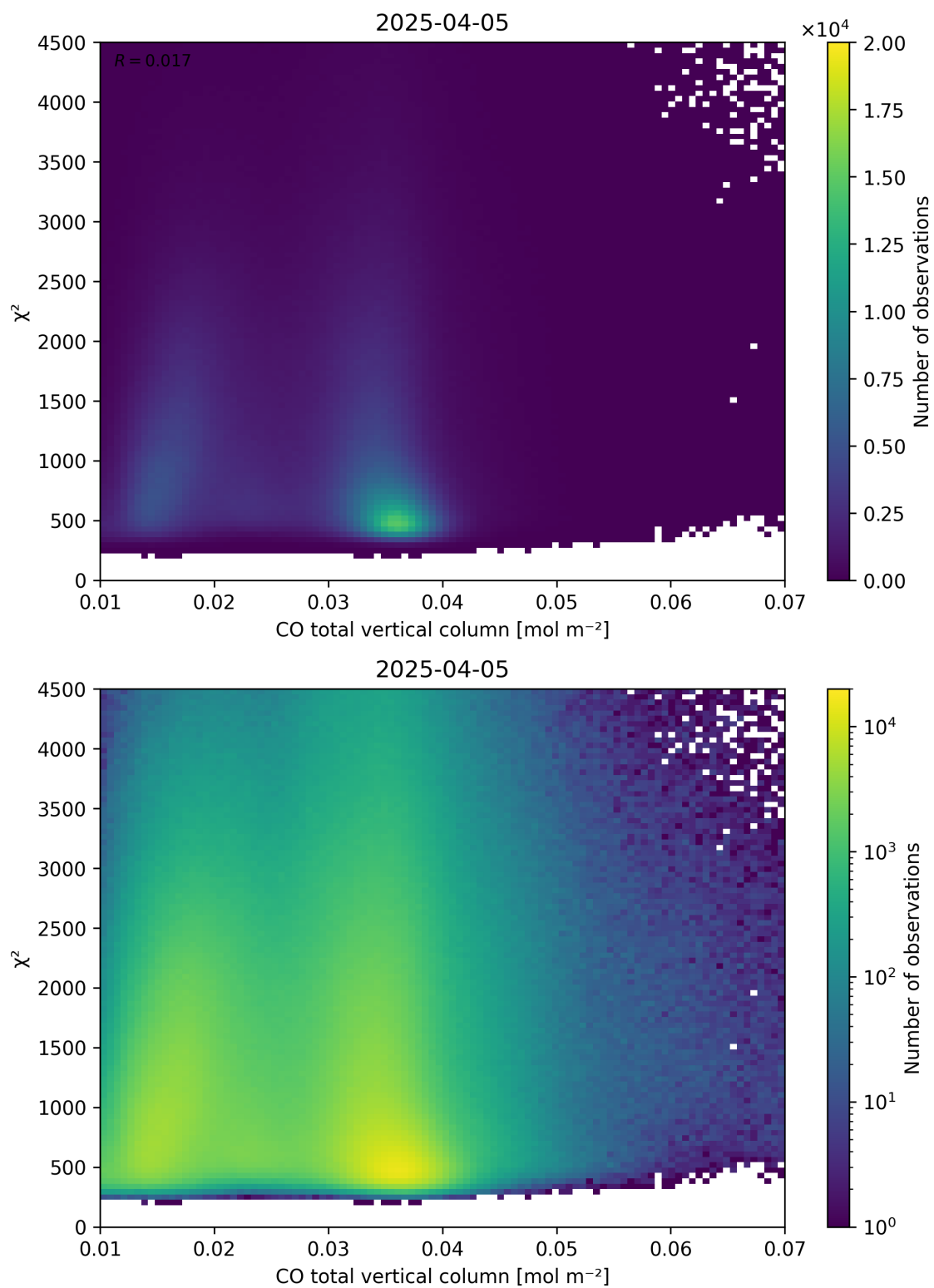
Figure 35: Scatter density plot of “CO total vertical column” against “ \chi^2 ” for 2025-04-04 to 2025-04-06.
