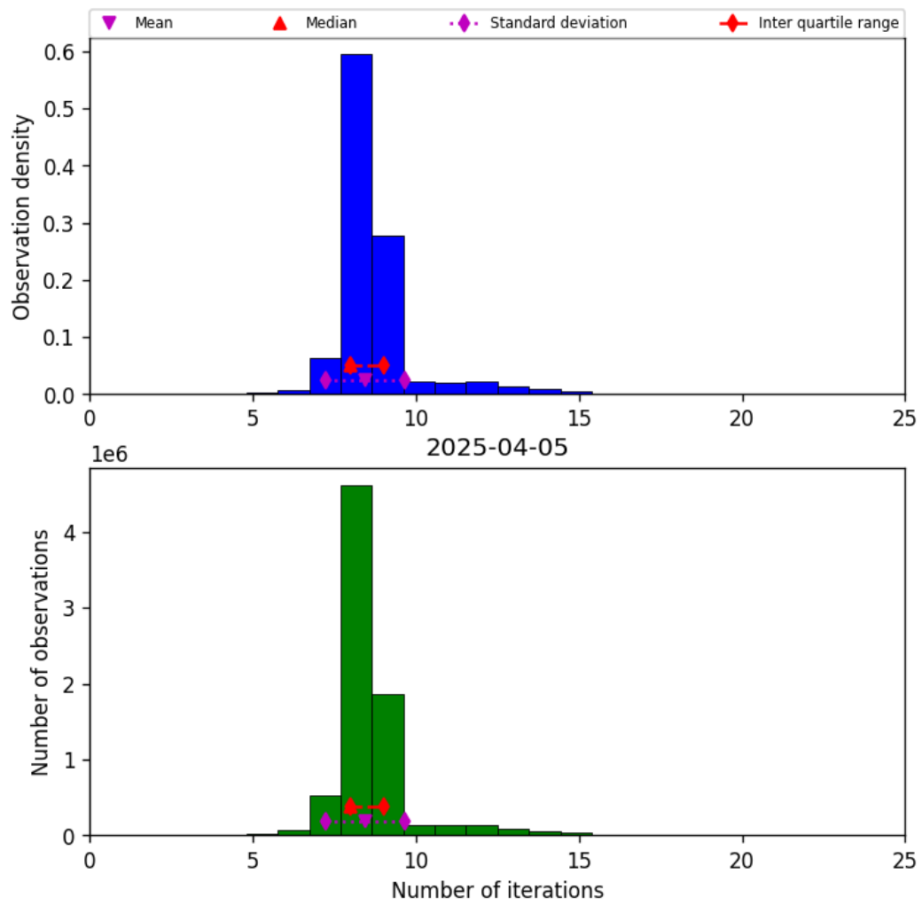
Figure 24: Histogram of “Number of iterations” for 2025-04-04 to 2025-04-06
