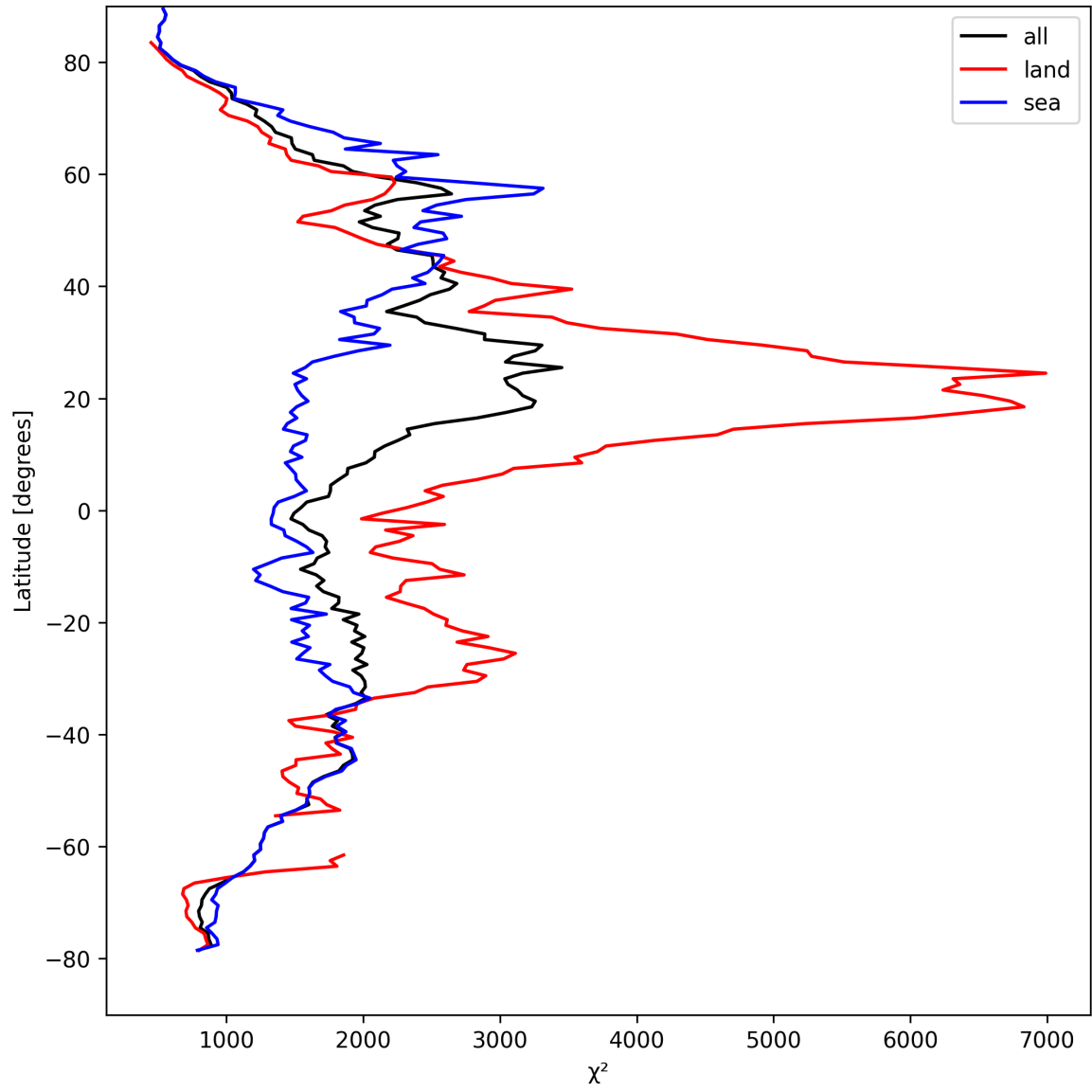
Figure 14: Zonal average of “ \chi^2 ” for 2025-04-04 to 2025-04-06.
