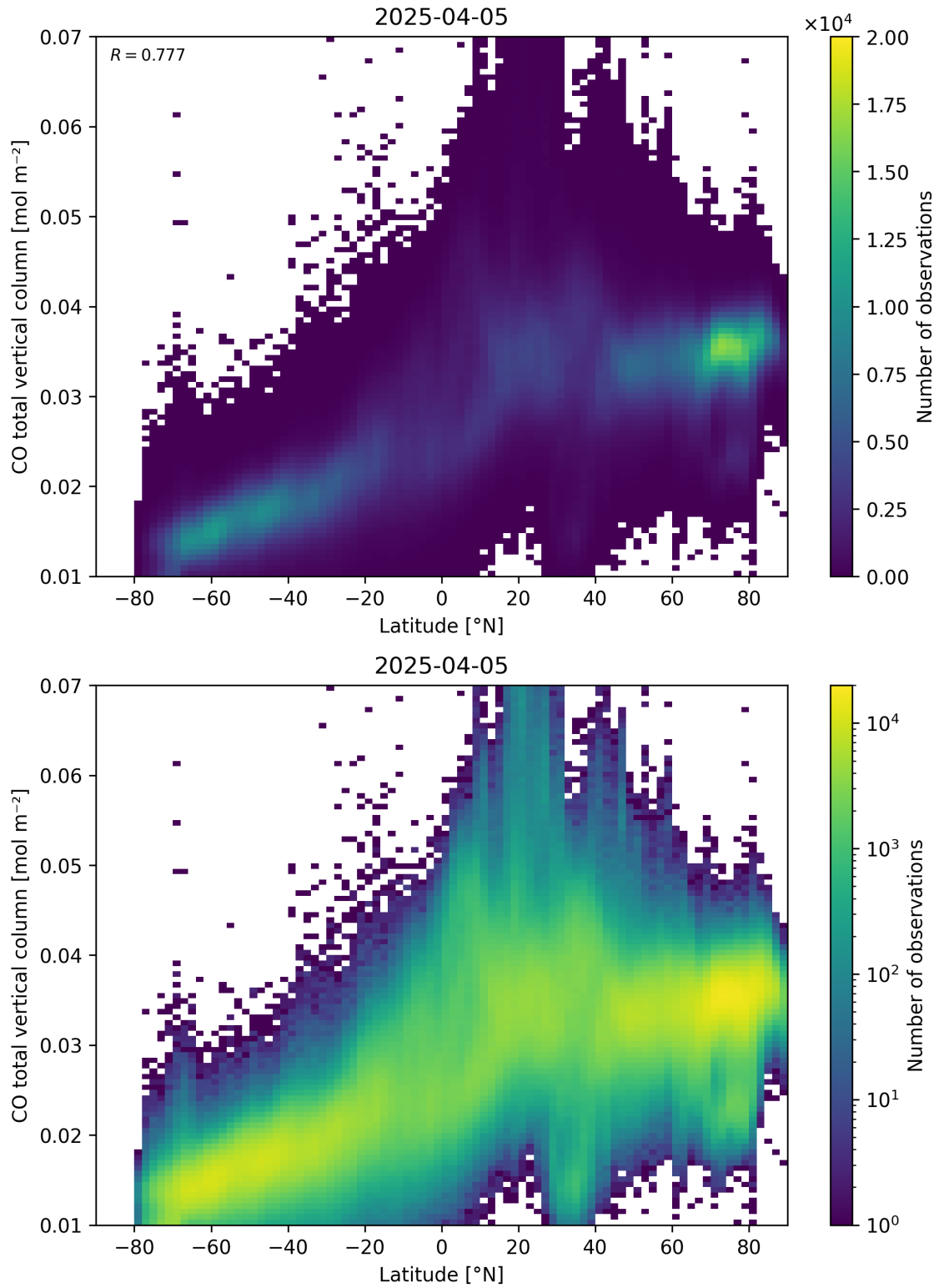
Figure 51: Scatter density plot of “Latitude” against “CO total vertical column” for 2025-04-04 to 2025-04-06.
