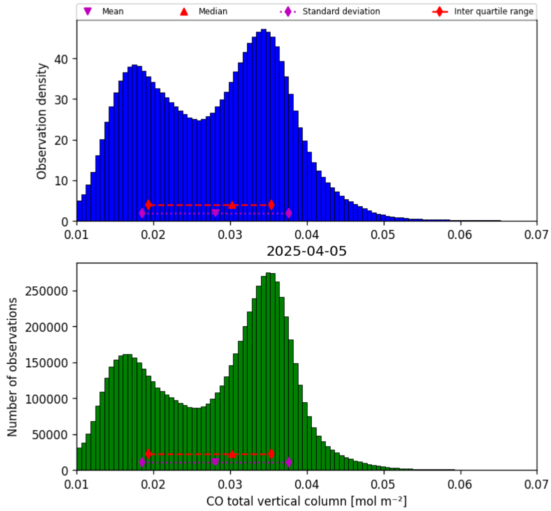
Figure 18: Histogram of “CO total vertical column” for 2025-04-04 to 2025-04-06
