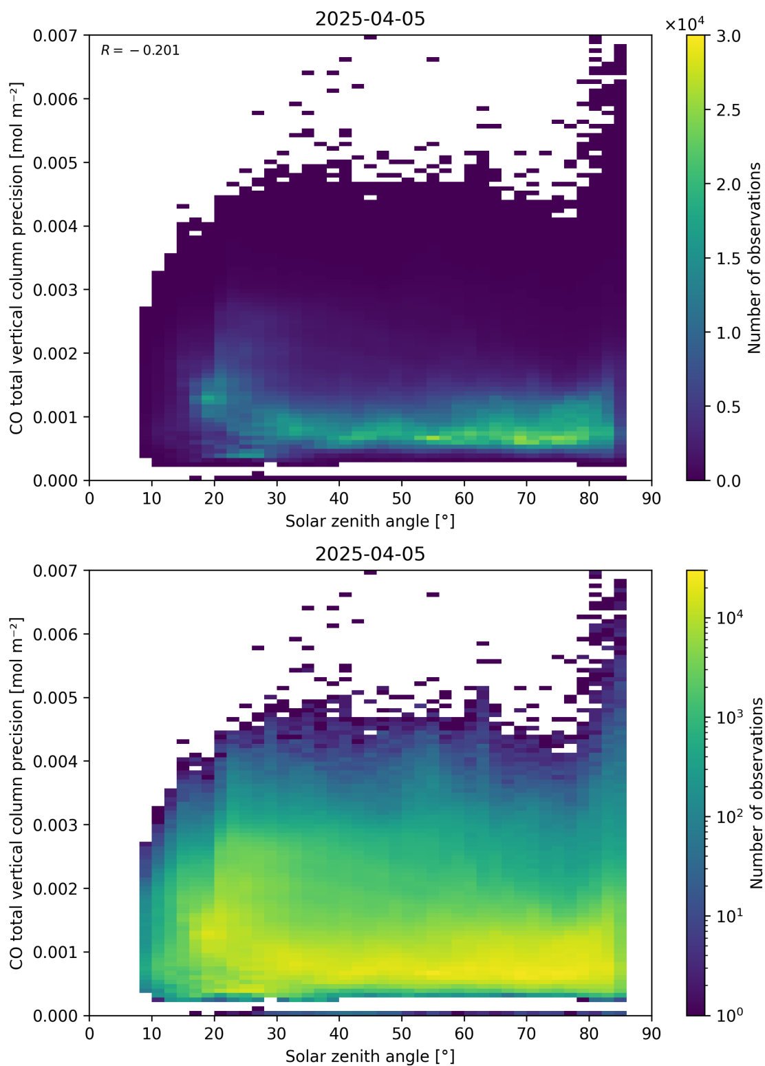
Figure 63: Scatter density plot of “Solar zenith angle” against “CO total vertical column precision” for 2025-04-04 to 2025-04-06.
