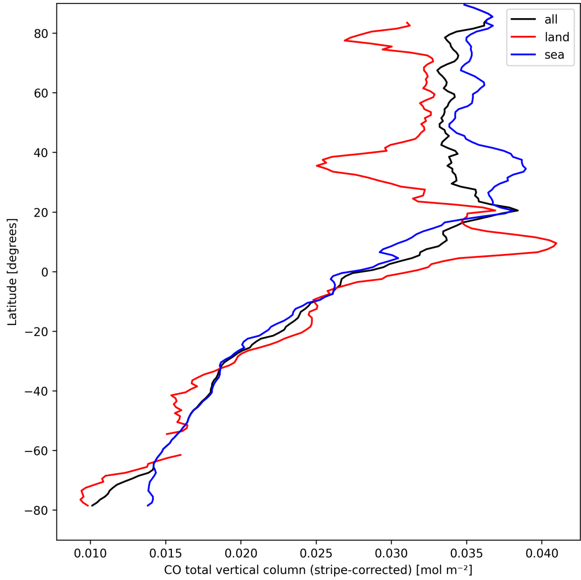
Figure 11: Zonal average of “CO total vertical column (stripe-corrected)” for 2025-04-04 to 2025-04-06.
