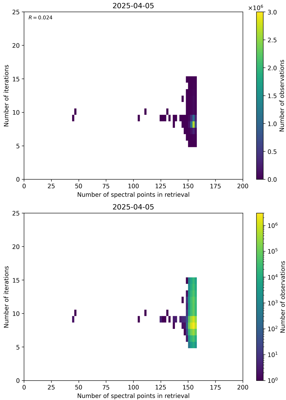
Figure 60: Scatter density plot of “Number of spectral points in retrieval” against “Number of iterations” for 2025-04-04 to 2025-04-06.
