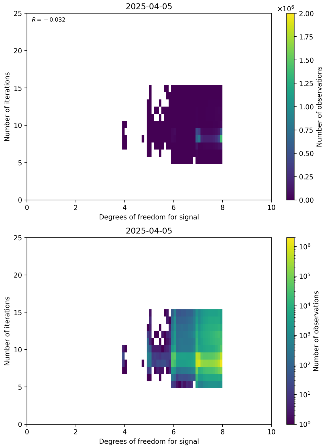
Figure 50: Scatter density plot of “Degrees of freedom for signal” against “Number of iterations” for 2025-04-04 to 2025-04-06.
