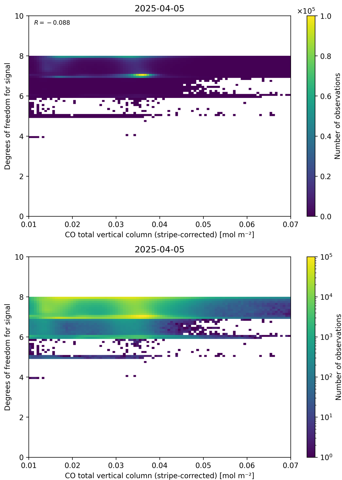
Figure 38: Scatter density plot of “CO total vertical column (stripe-corrected)” against “Degrees of freedom for signal” for 2025-04-04 to 2025-04-06.
