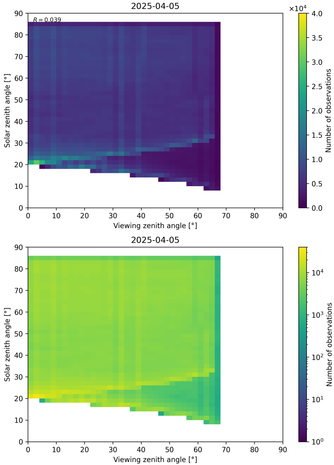
Figure 77: Scatter density plot of “Viewing zenith angle” against “Solar zenith angle” for 2025-04-04 to 2025-04-06.
