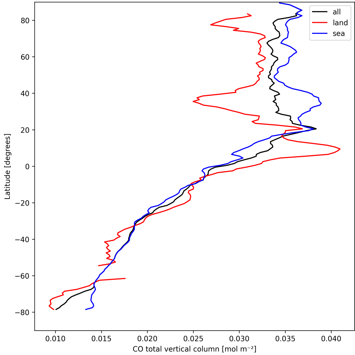
Figure 10: Zonal average of “CO total vertical column” for 2025-04-04 to 2025-04-06.
