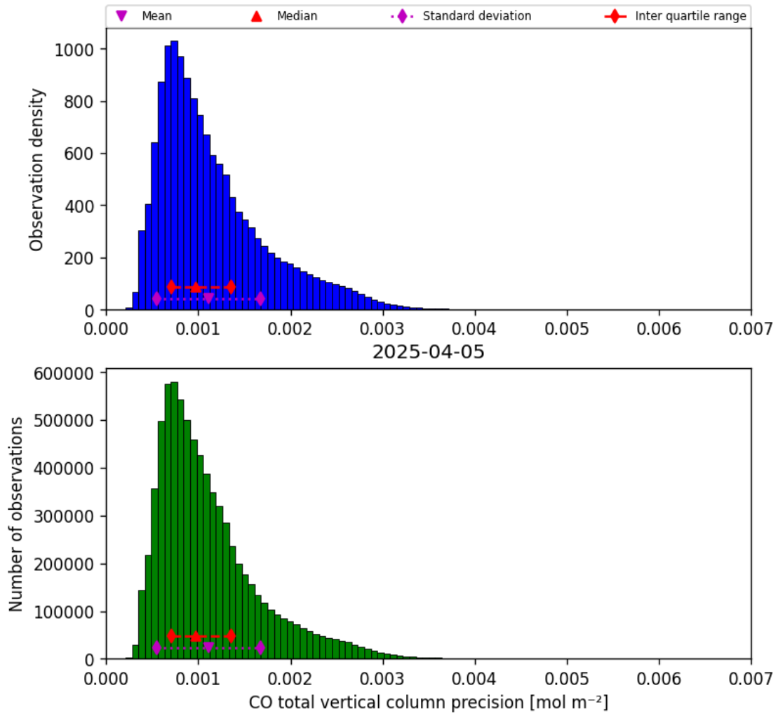
Figure 20: Histogram of “CO total vertical column precision” for 2025-04-04 to 2025-04-06
