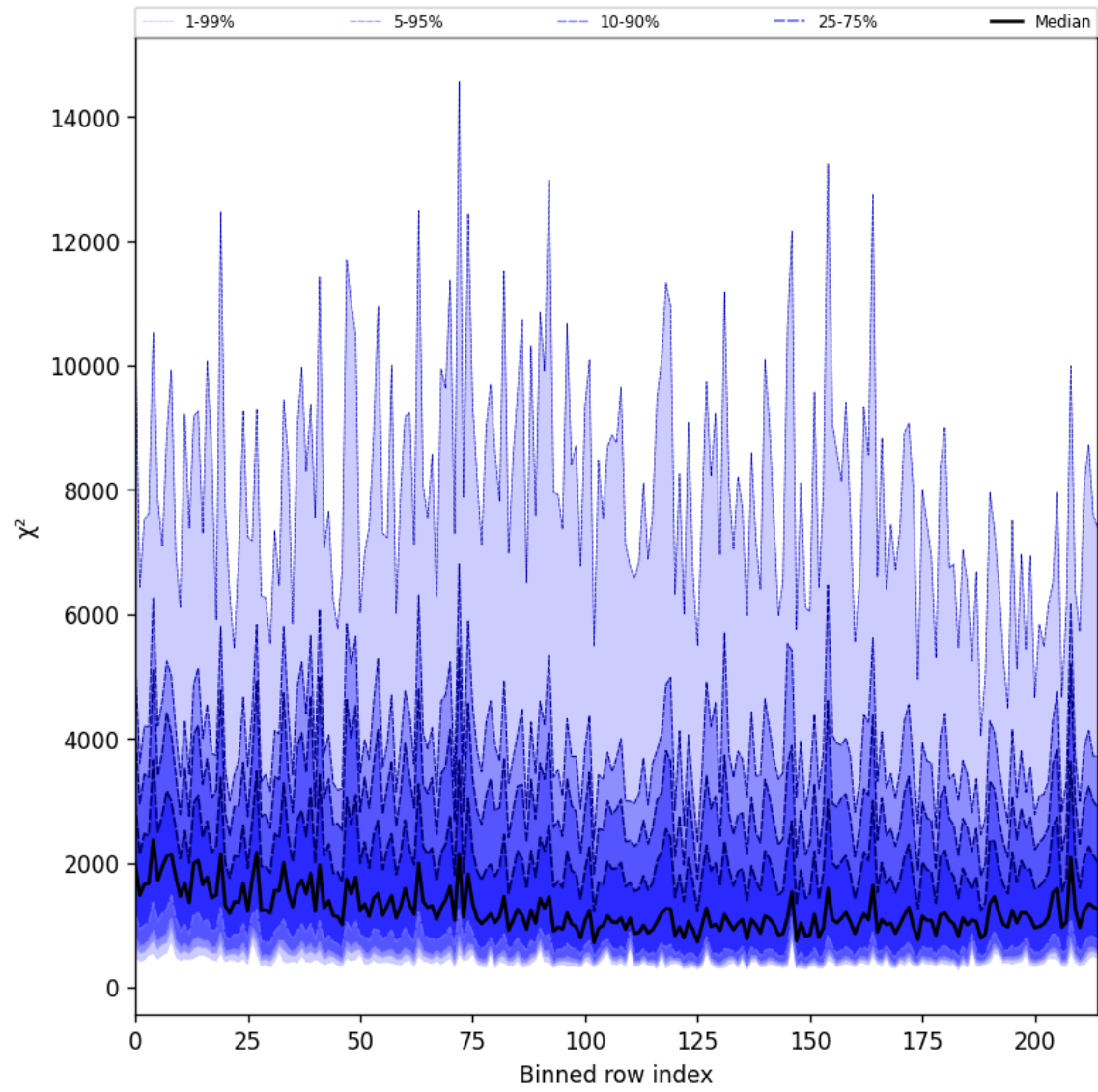
Figure 30: Along track statistics of “ \chi^2 ” for 2025-04-04 to 2025-04-06
