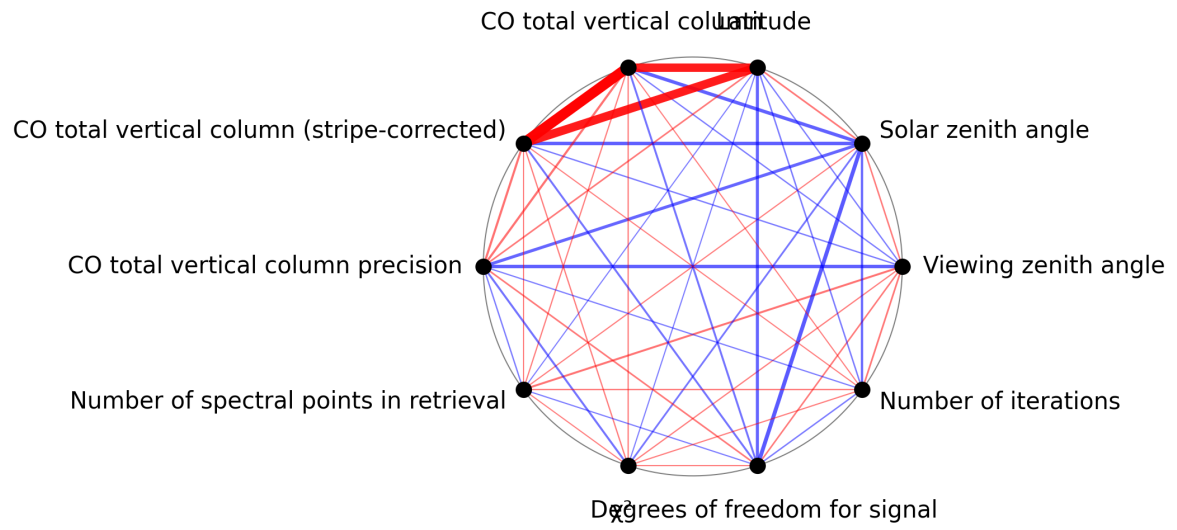
Figure 1: Map of correlation graph for 2025-04-04 to 2025-04-06.
