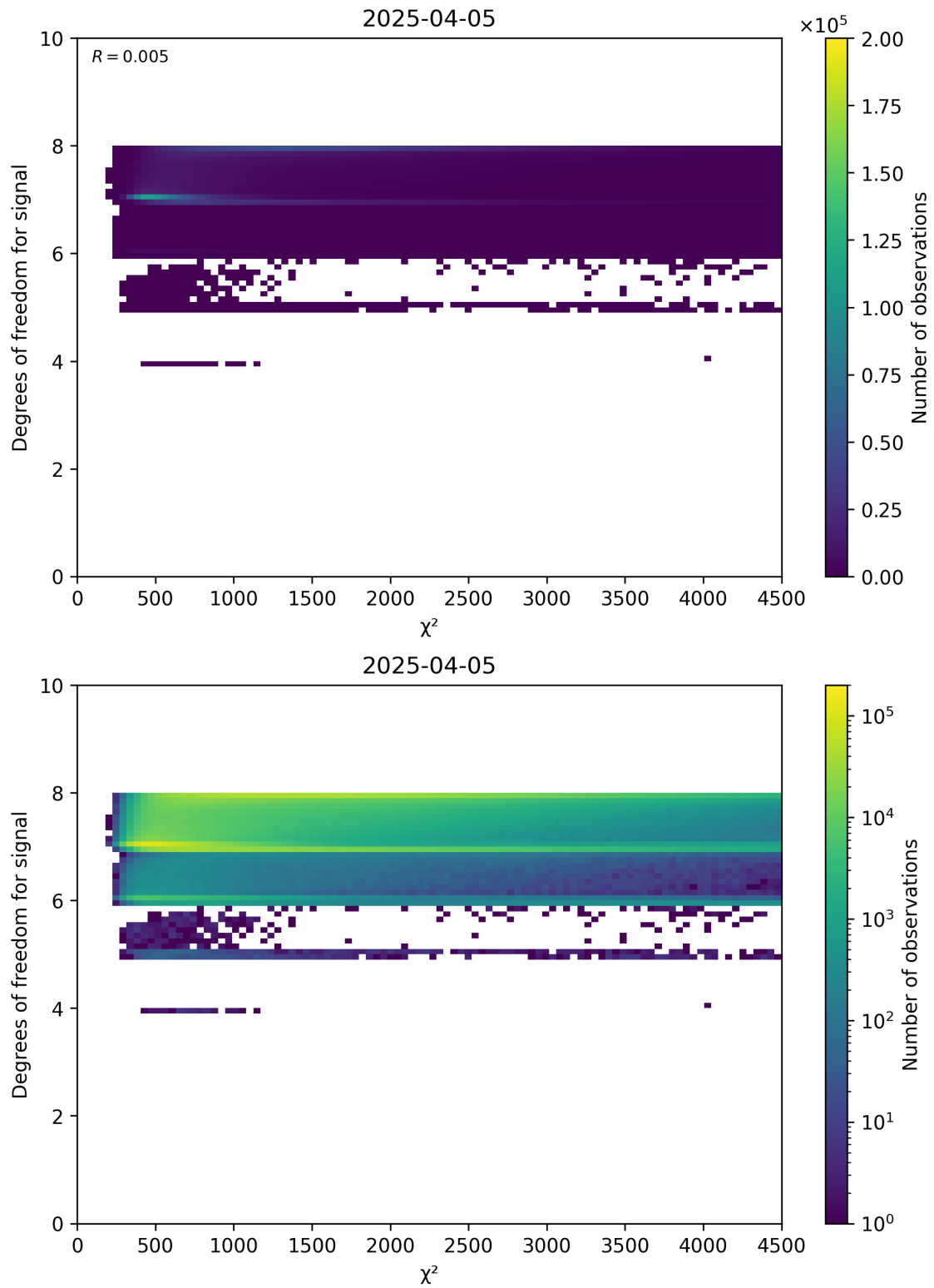
Figure 48: Scatter density plot of “ \chi^2 ” against “Degrees of freedom for signal” for 2025-04-04 to 2025-04-06.
