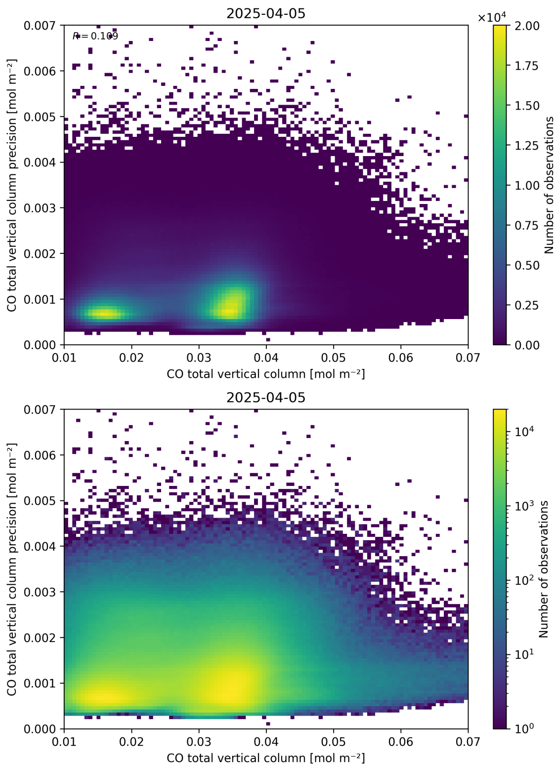
Figure 34: Scatter density plot of “CO total vertical column” against “CO total vertical column precision” for 2025-04-04 to 2025-04-06.
