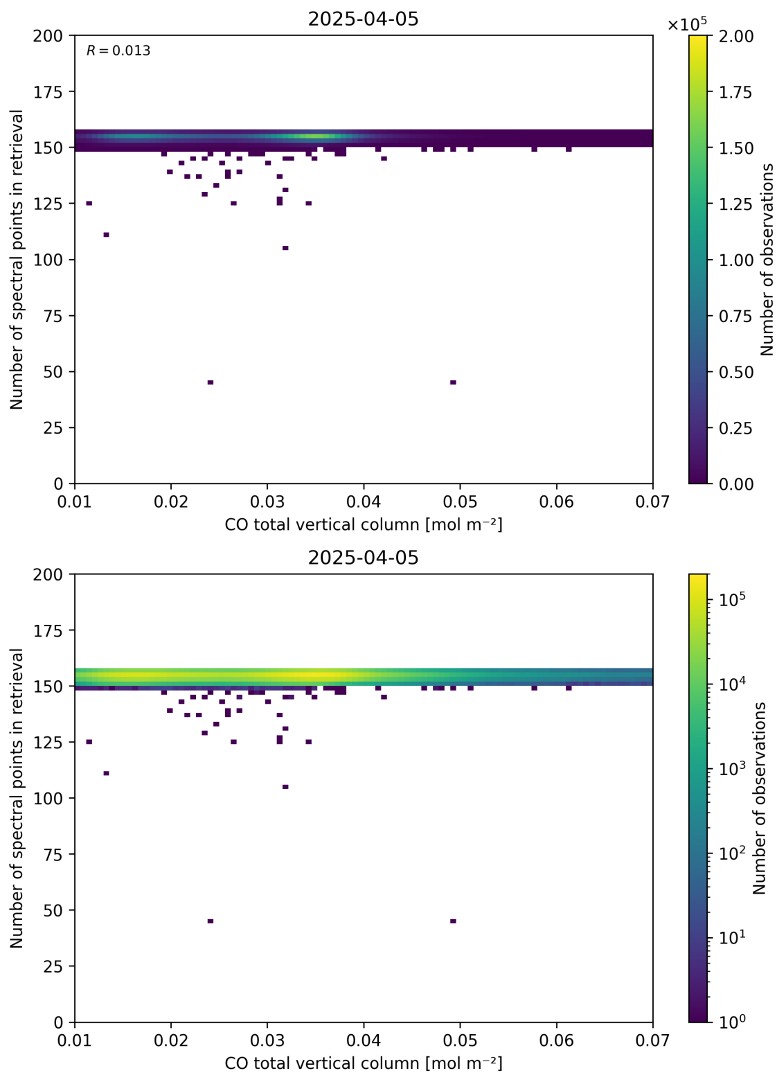
Figure 43: Scatter density plot of “CO total vertical column” against “Number of spectral points in retrieval” for 2025-04-04 to 2025-04-06.
