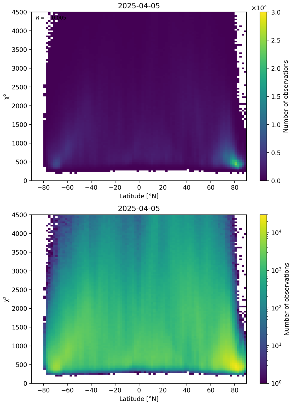
Figure 54: Scatter density plot of “Latitude” against “ \chi^2 ” for 2025-04-04 to 2025-04-06.
