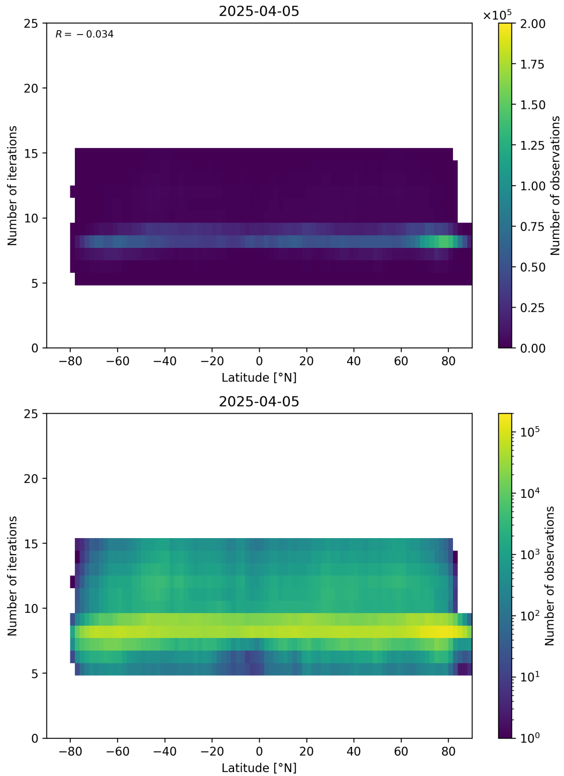
Figure 56: Scatter density plot of “Latitude” against “Number of iterations” for 2025-04-04 to 2025-04-06.
