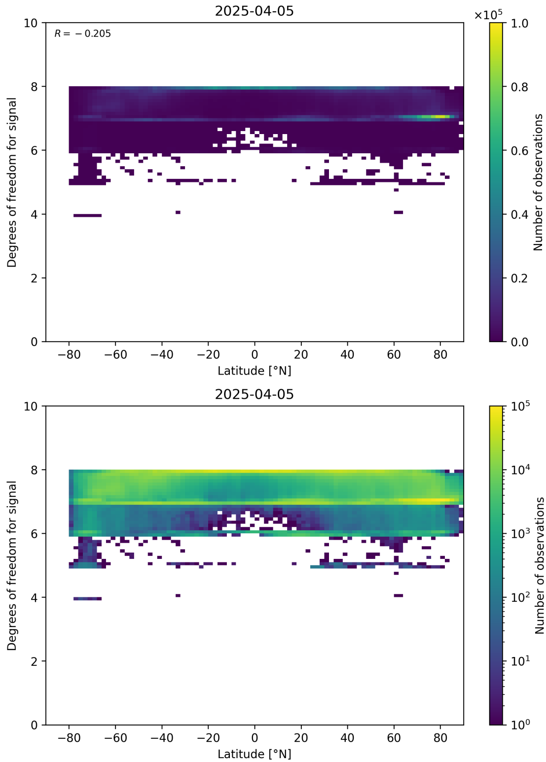
Figure 55: Scatter density plot of “Latitude” against “Degrees of freedom for signal” for 2025-04-04 to 2025-04-06.
