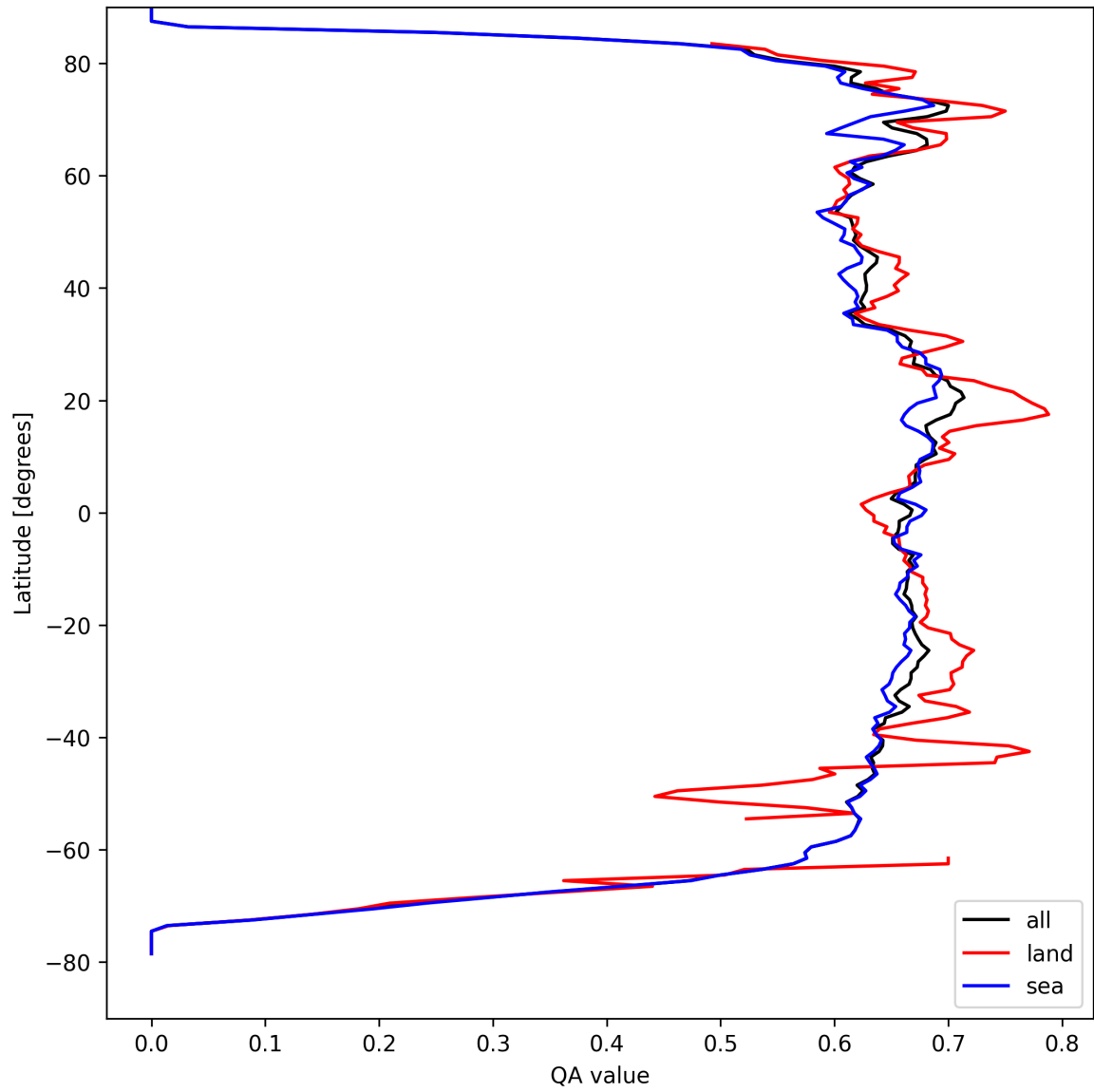
Figure 9: Zonal average of “QA value” for 2025-04-04 to 2025-04-06.
