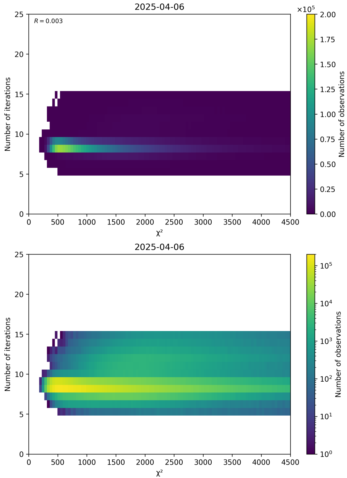
Figure 49: Scatter density plot of “ \chi^2 ” against “Number of iterations” for 2025-04-05 to 2025-04-07.
