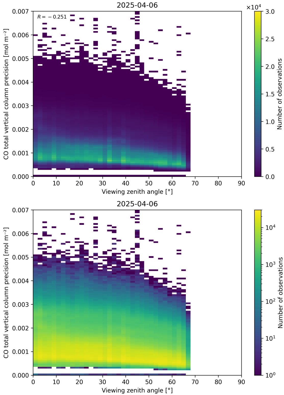
Figure 71: Scatter density plot of “Viewing zenith angle” against “CO total vertical column precision” for 2025-04-05 to 2025-04-07.
