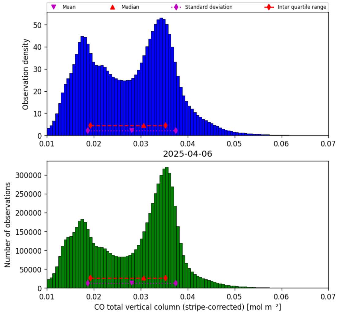
Figure 19: Histogram of “CO total vertical column (stripe-corrected)” for 2025-04-05 to 2025-04-07
