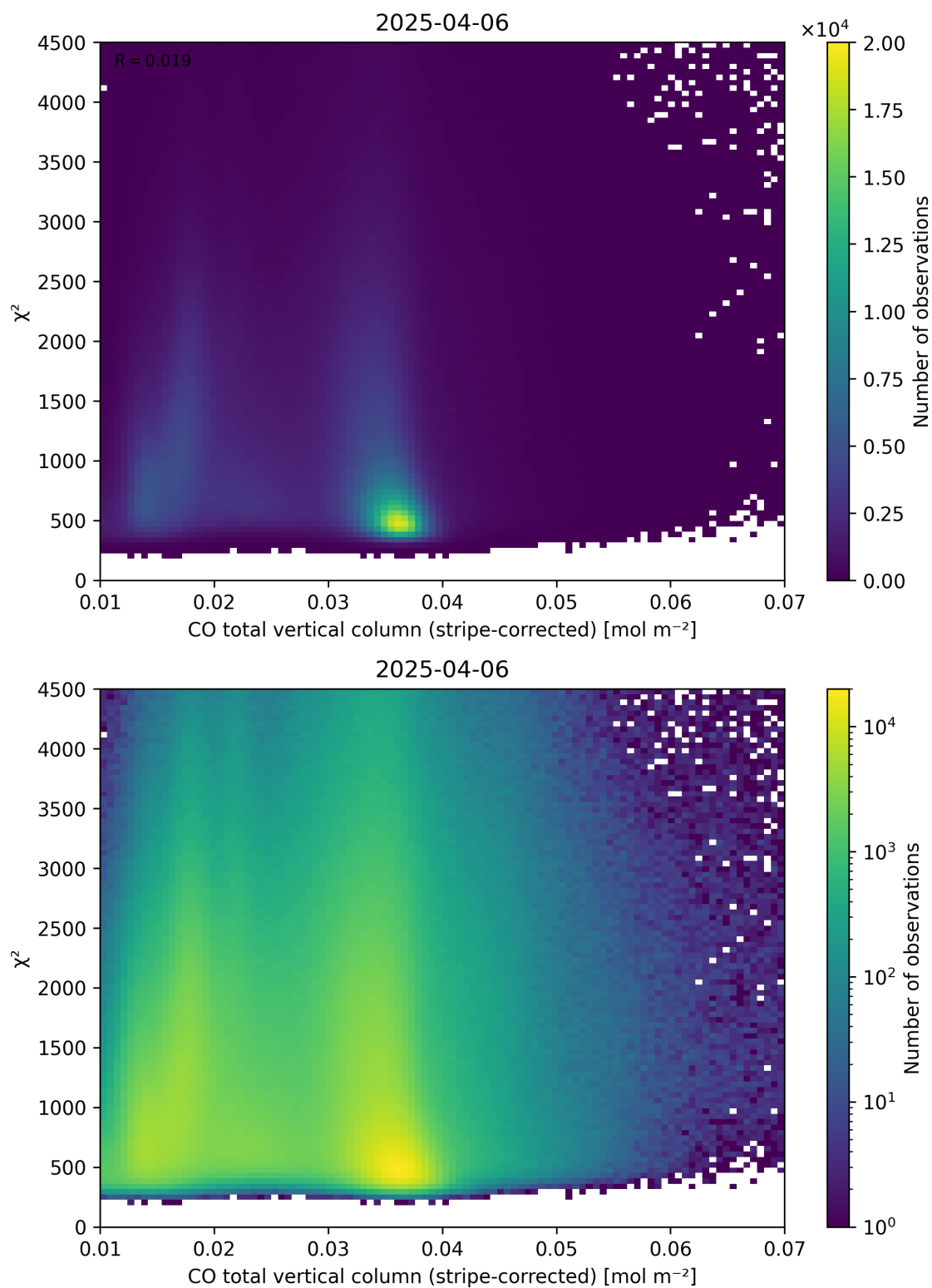
Figure 37: Scatter density plot of “CO total vertical column (stripe-corrected)” against “ \chi^2 ” for 2025-04-05 to 2025-04-07.
