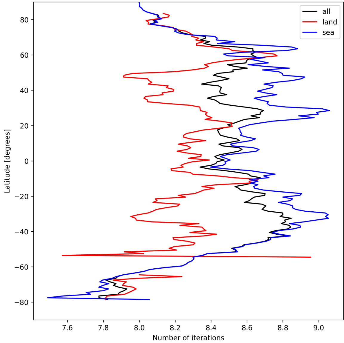
Figure 16: Zonal average of “Number of iterations” for 2025-04-05 to 2025-04-07.
