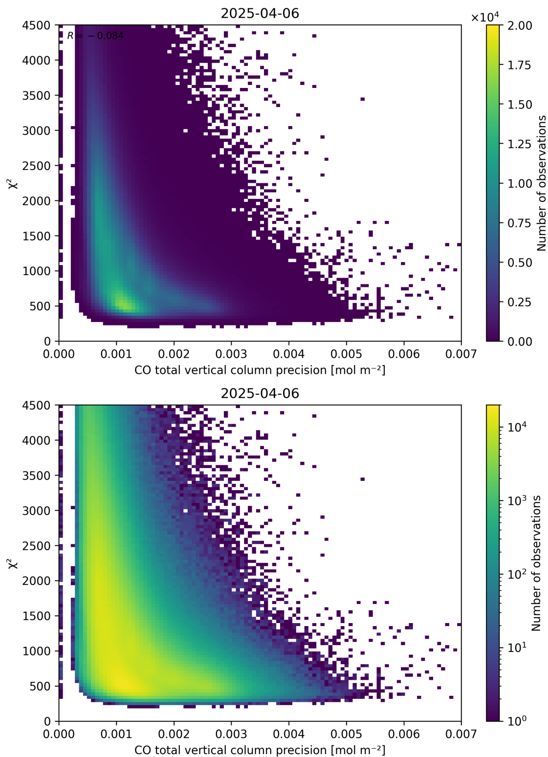
Figure 44: Scatter density plot of “CO total vertical column precision” against “ \chi^2 ” for 2025-04-05 to 2025-04-07.
