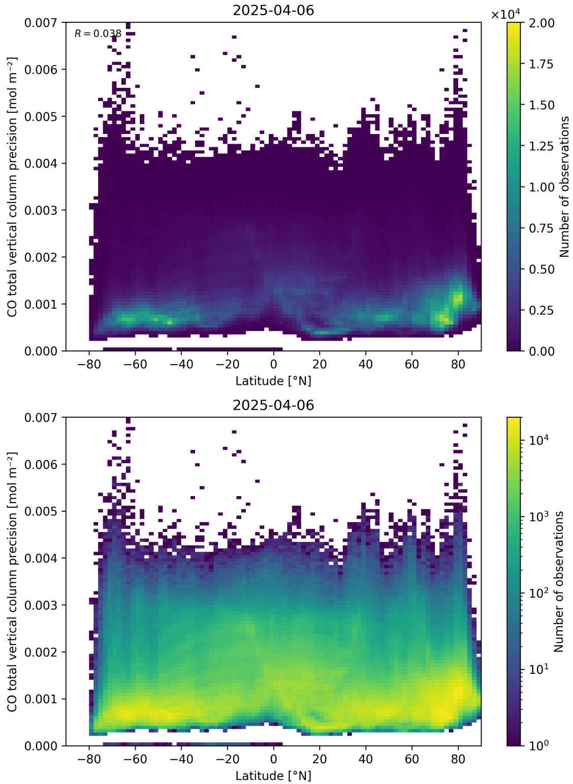
Figure 53: Scatter density plot of “Latitude” against “CO total vertical column precision” for 2025-04-05 to 2025-04-07.
