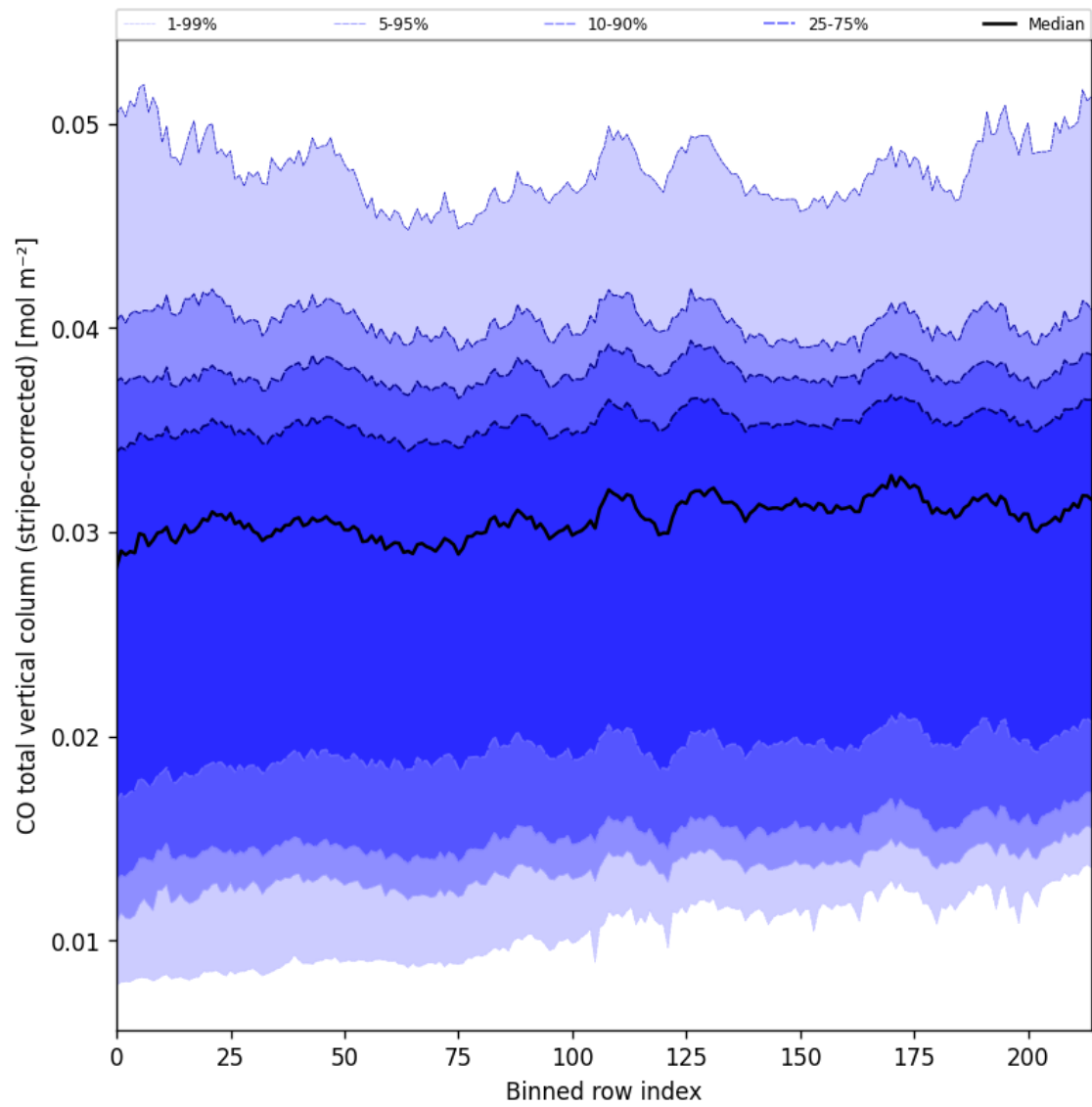
Figure 27: Along track statistics of “CO total vertical column (stripe-corrected)” for 2025-04-05 to 2025-04-07
