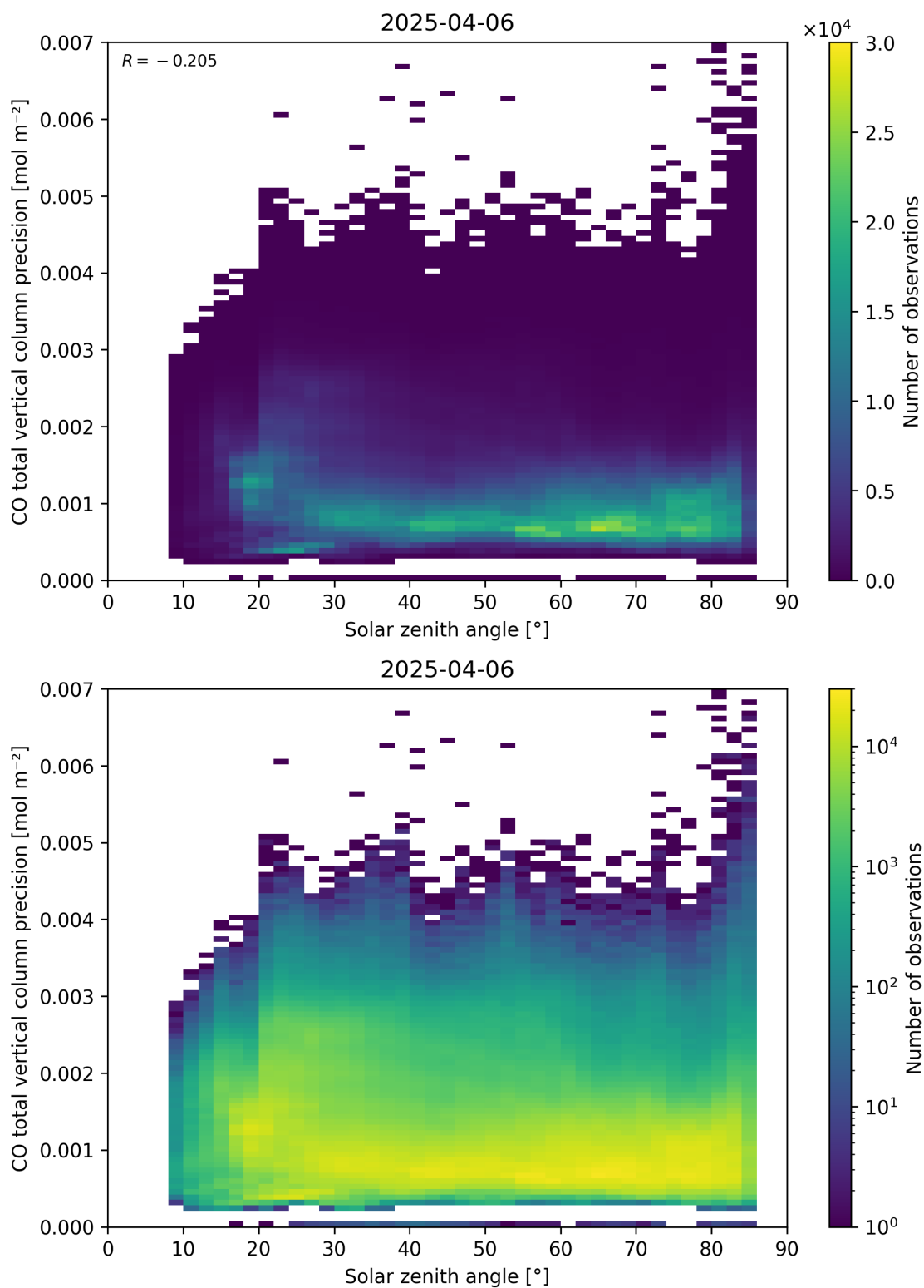
Figure 63: Scatter density plot of “Solar zenith angle” against “CO total vertical column precision” for 2025-04-05 to 2025-04-07.
