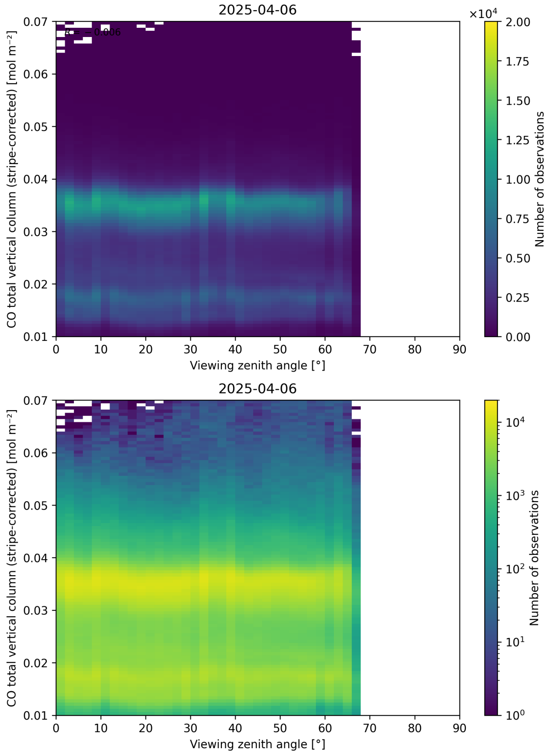
Figure 70: Scatter density plot of “Viewing zenith angle” against “CO total vertical column (stripe-corrected)” for 2025-04-05 to 2025-04-07.
