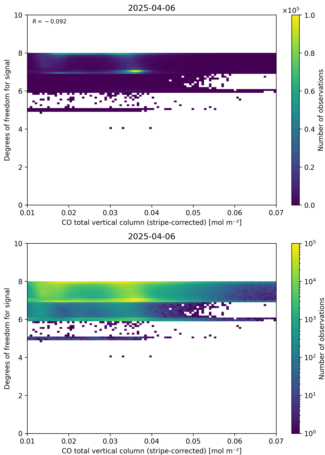
Figure 38: Scatter density plot of “CO total vertical column (stripe-corrected)” against “Degrees of freedom for signal” for 2025-04-05 to 2025-04-07.
