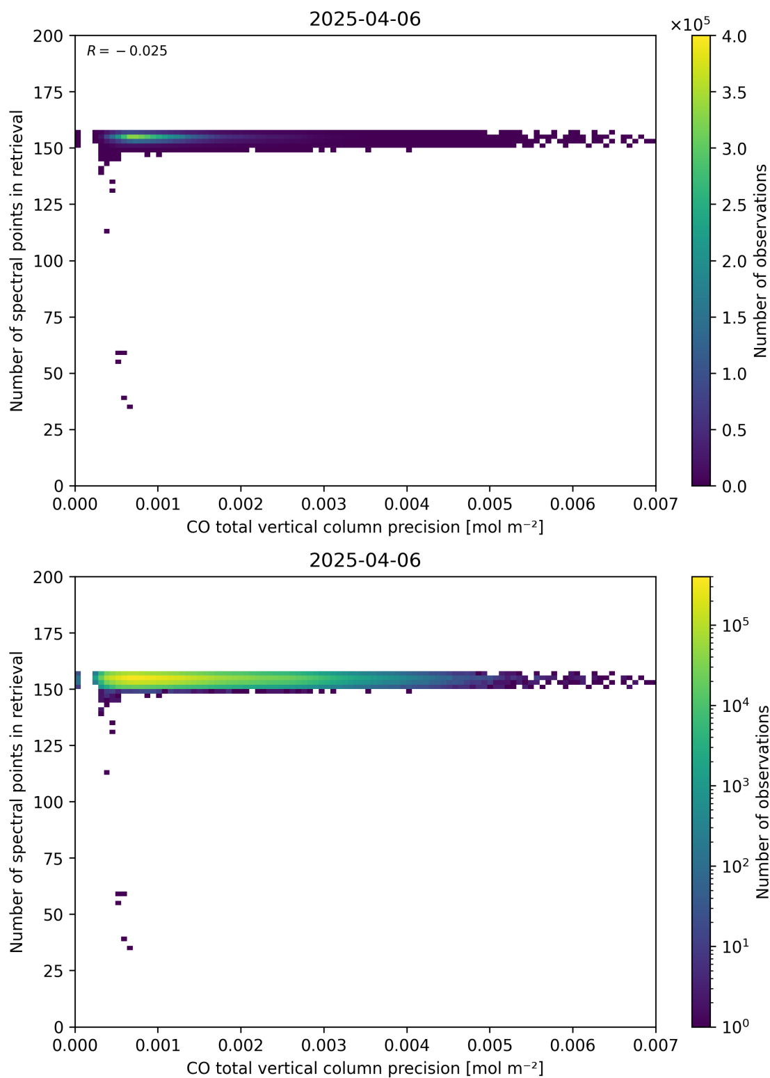
Figure 47: Scatter density plot of “CO total vertical column precision” against “Number of spectral points in retrieval” for 2025-04-05 to 2025-04-07.
