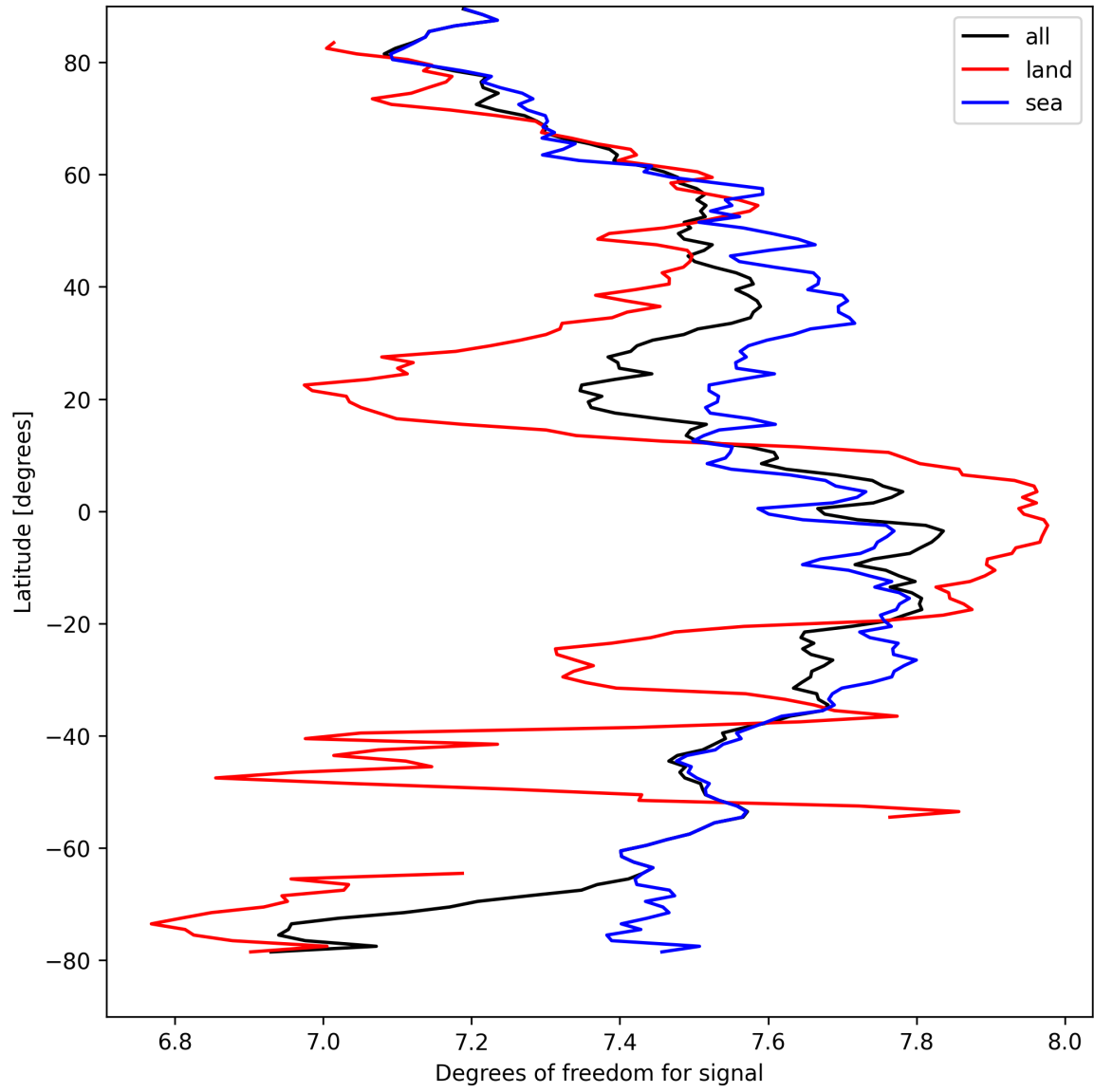
Figure 15: Zonal average of “Degrees of freedom for signal” for 2025-04-05 to 2025-04-07.
