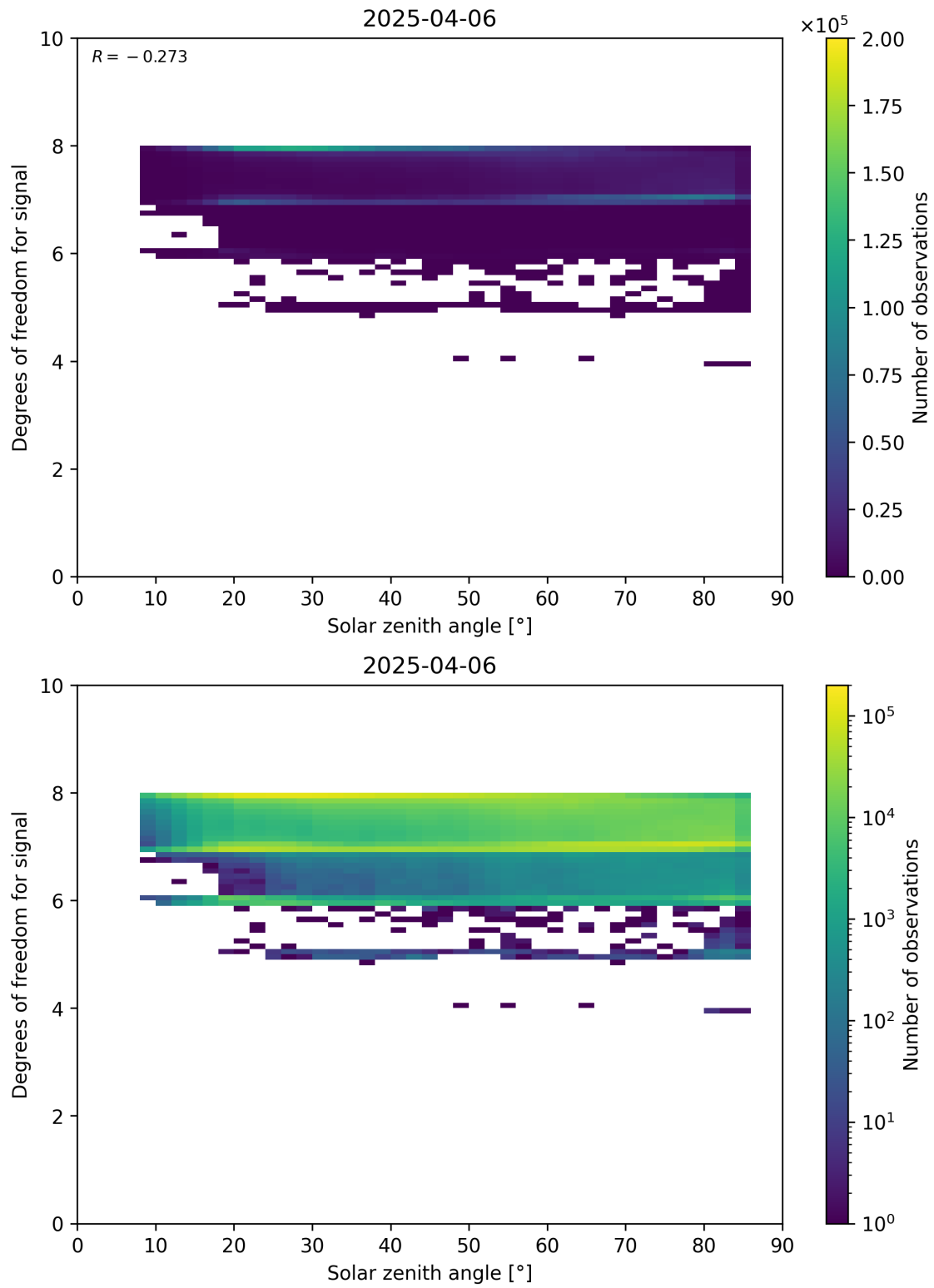
Figure 65: Scatter density plot of “Solar zenith angle” against “Degrees of freedom for signal” for 2025-04-05 to 2025-04-07.
