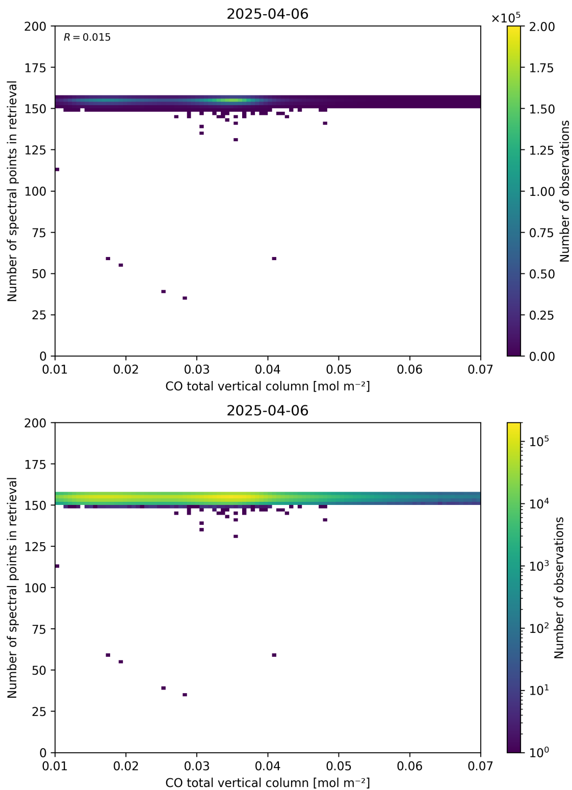
Figure 43: Scatter density plot of “CO total vertical column” against “Number of spectral points in retrieval” for 2025-04-05 to 2025-04-07.
