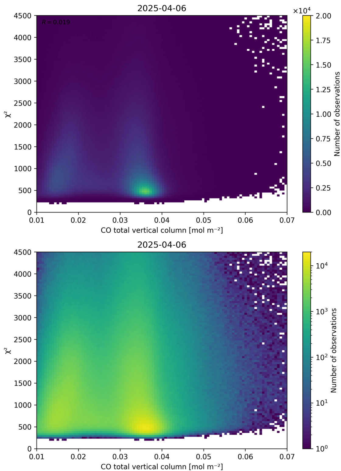
Figure 35: Scatter density plot of “CO total vertical column” against “ \chi^2 ” for 2025-04-05 to 2025-04-07.
