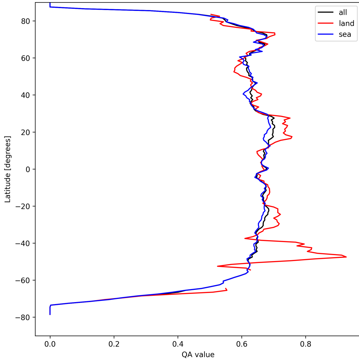
Figure 9: Zonal average of “QA value” for 2025-04-05 to 2025-04-07.
