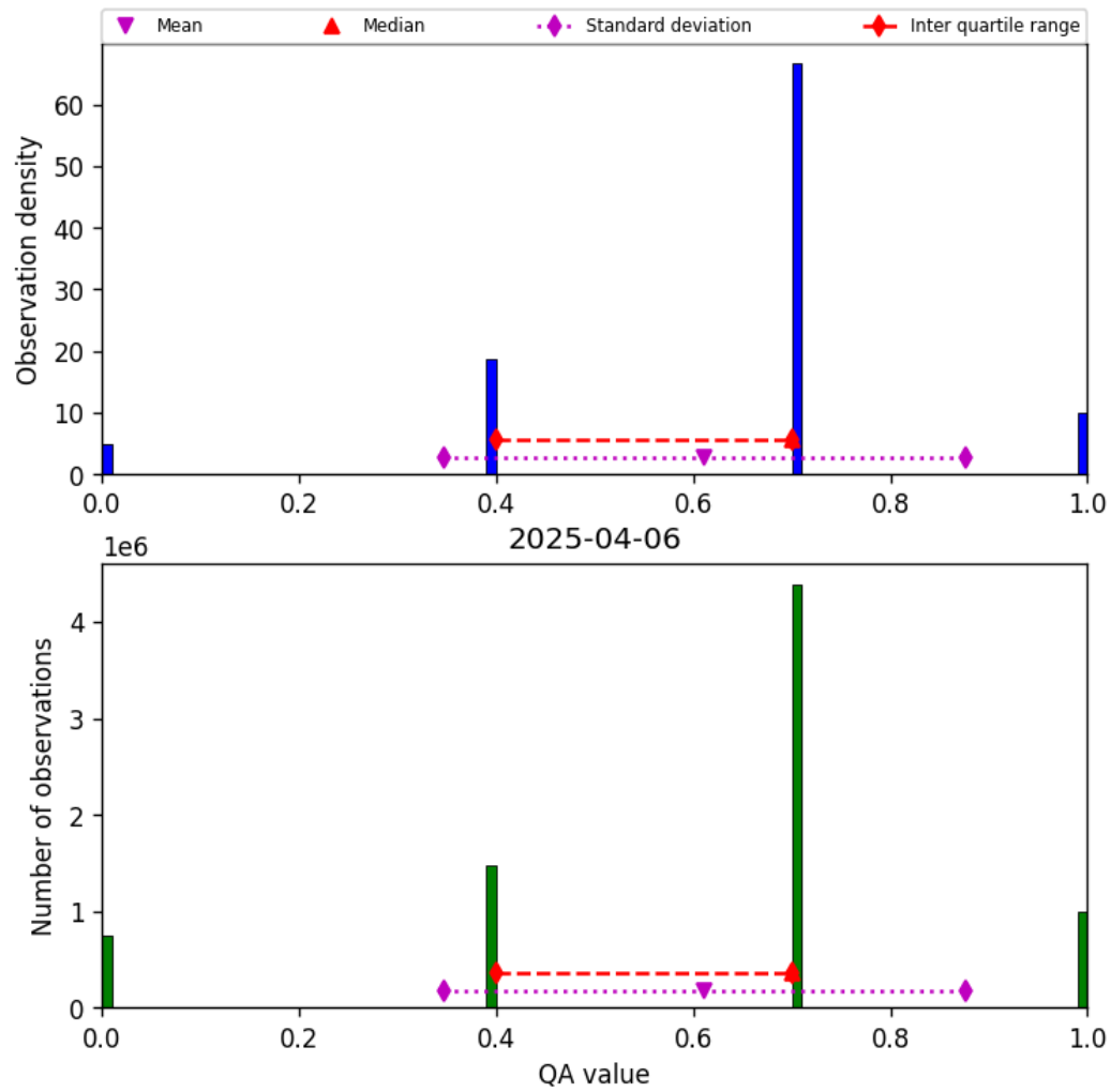
Figure 17: Histogram of “QA value” for 2025-04-05 to 2025-04-07
