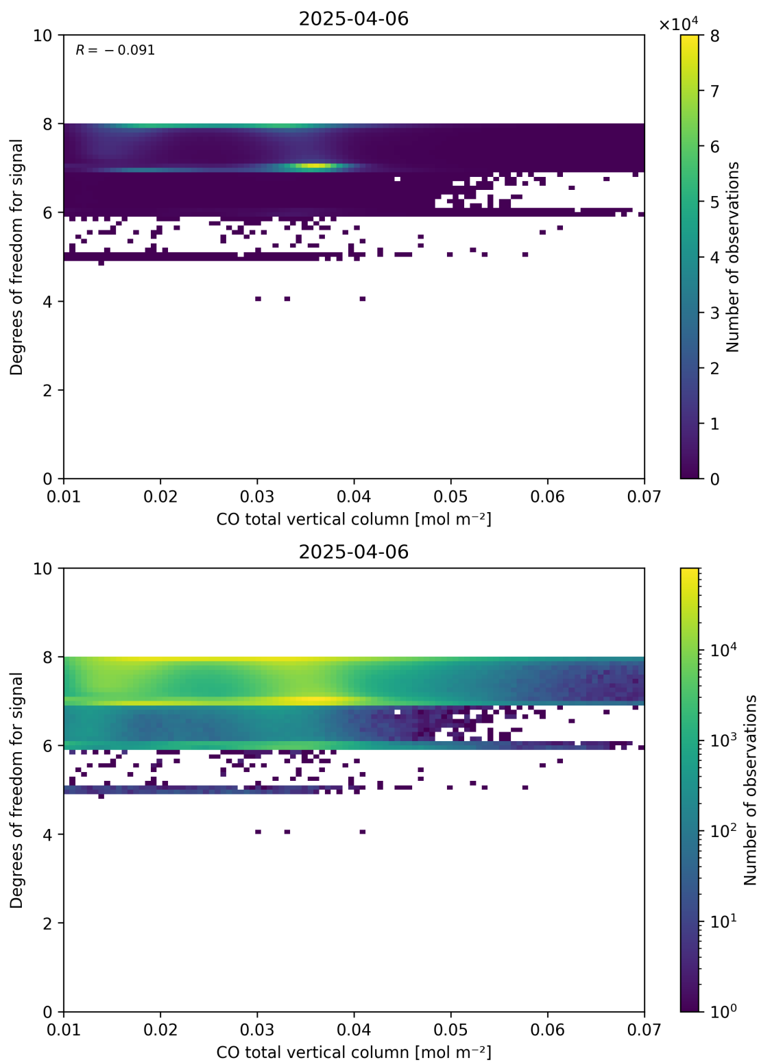
Figure 41: Scatter density plot of “CO total vertical column” against “Degrees of freedom for signal” for 2025-04-05 to 2025-04-07.
