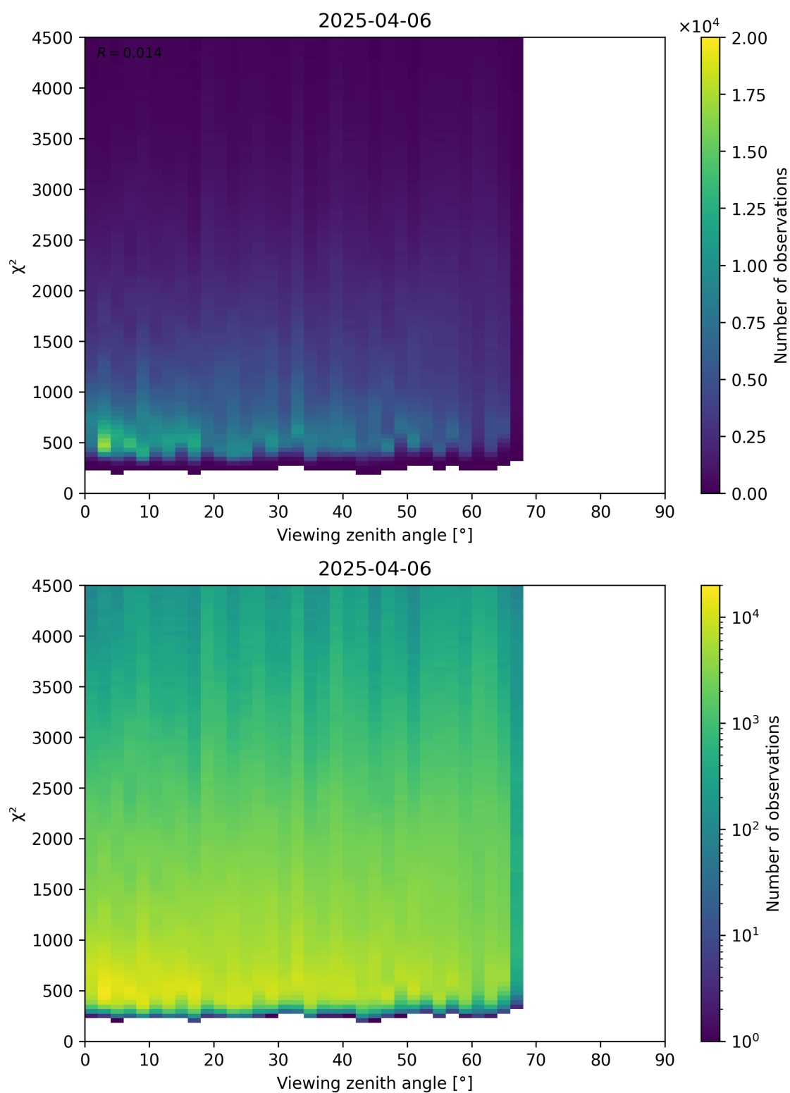
Figure 72: Scatter density plot of “Viewing zenith angle” against “ \chi^2 ” for 2025-04-05 to 2025-04-07.
