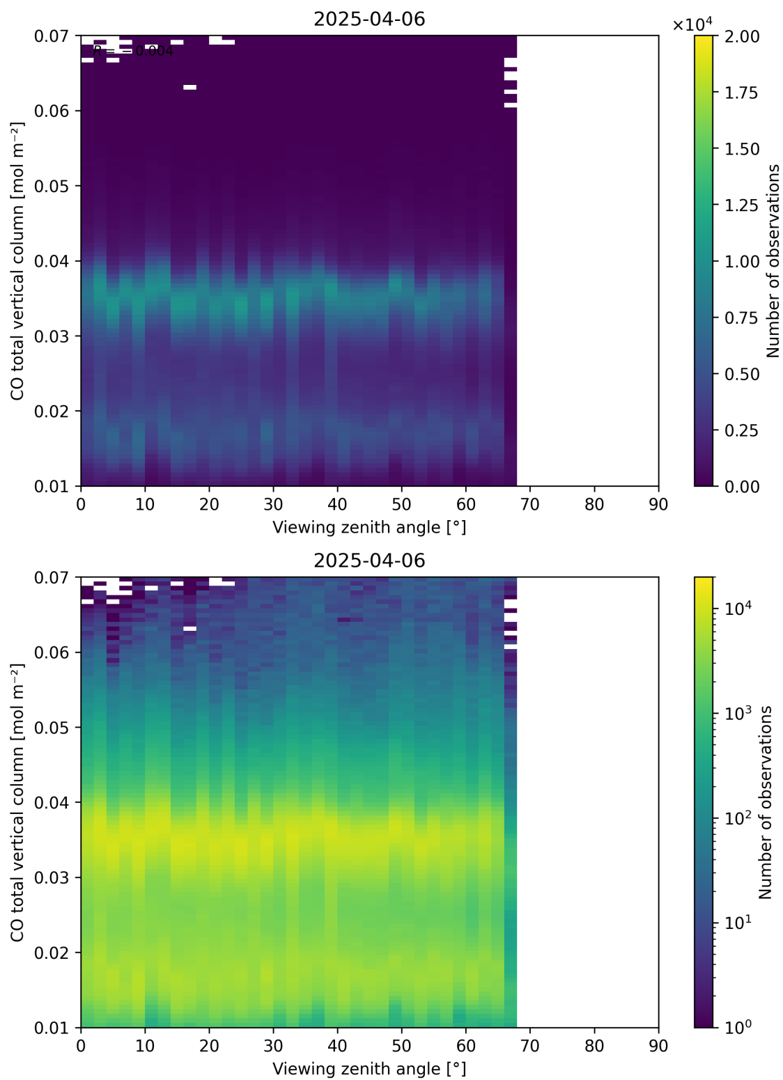
Figure 69: Scatter density plot of “Viewing zenith angle” against “CO total vertical column” for 2025-04-05 to 2025-04-07.
