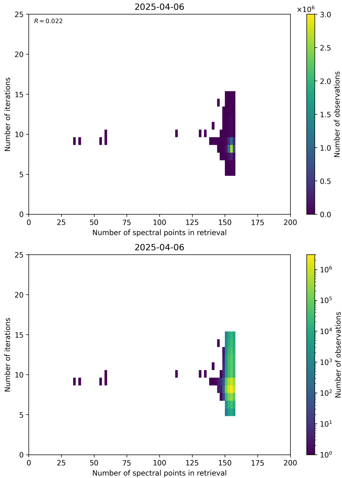
Figure 60: Scatter density plot of “Number of spectral points in retrieval” against “Number of iterations” for 2025-04-05 to 2025-04-07.
