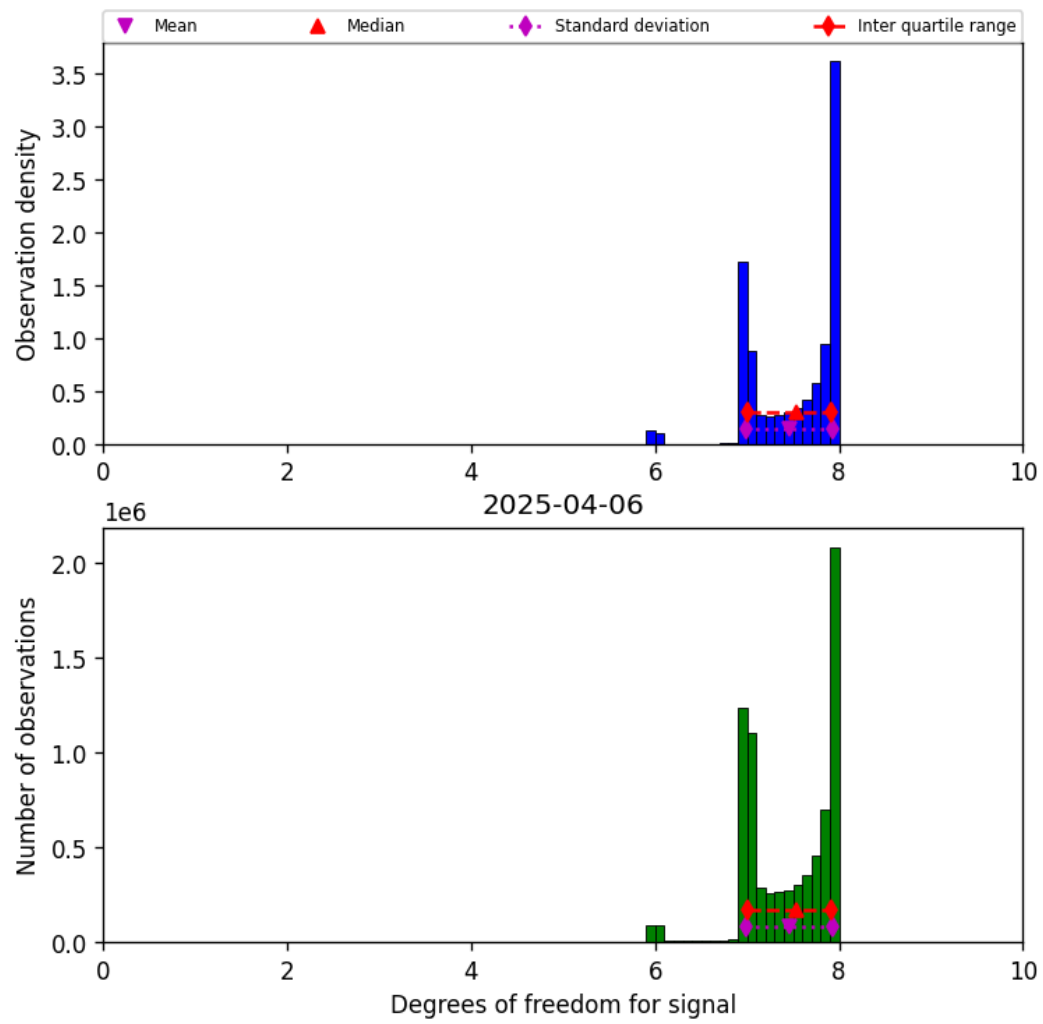
Figure 23: Histogram of “Degrees of freedom for signal” for 2025-04-05 to 2025-04-07
