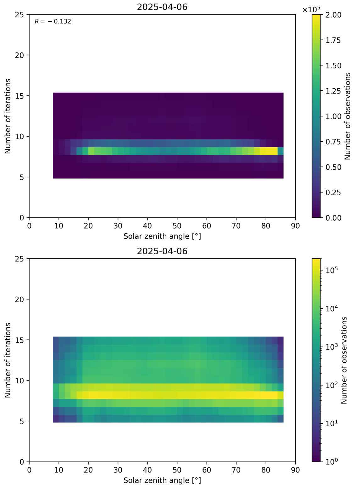
Figure 67: Scatter density plot of “Solar zenith angle” against “Number of iterations” for 2025-04-05 to 2025-04-07.
