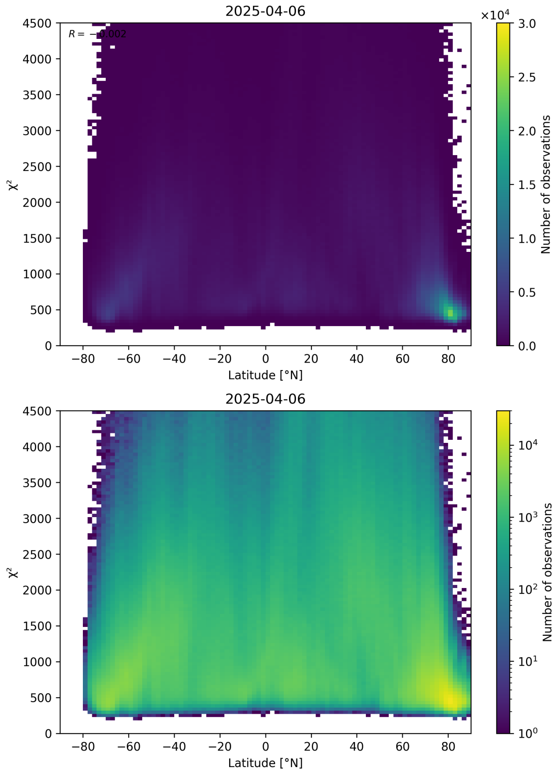
Figure 54: Scatter density plot of “Latitude” against “ \chi^2 ” for 2025-04-05 to 2025-04-07.
