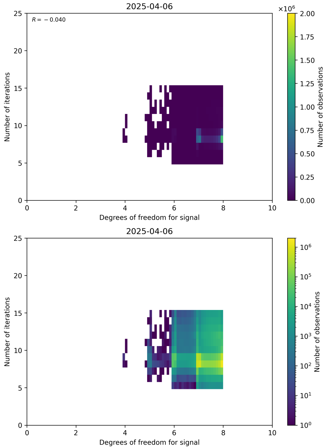
Figure 50: Scatter density plot of “Degrees of freedom for signal” against “Number of iterations” for 2025-04-05 to 2025-04-07.
