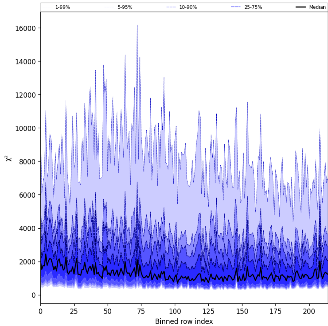
Figure 30: Along track statistics of “ \chi^2 ” for 2025-04-05 to 2025-04-07
