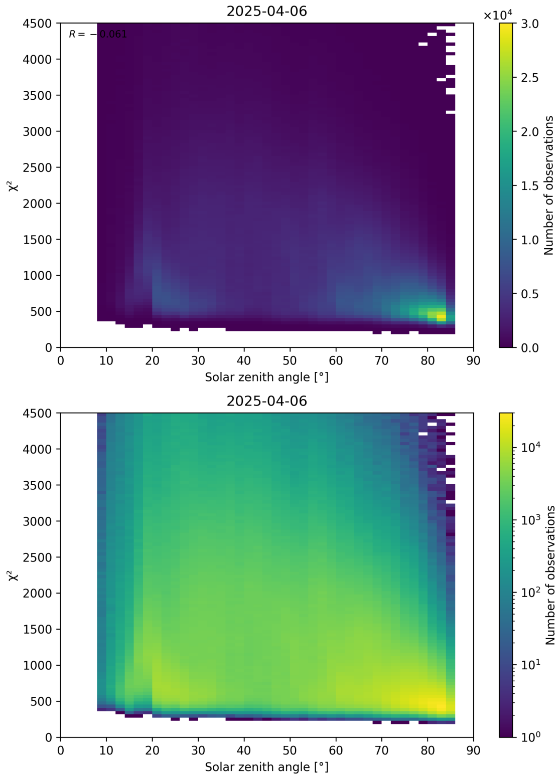
Figure 64: Scatter density plot of “Solar zenith angle” against “ \chi^2 ” for 2025-04-05 to 2025-04-07.
