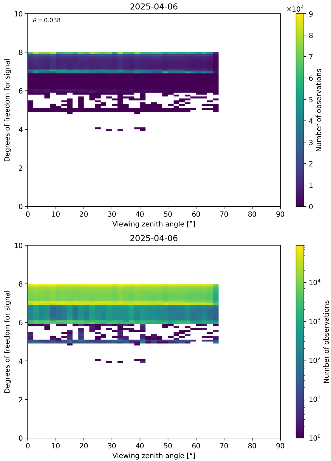
Figure 73: Scatter density plot of “Viewing zenith angle” against “Degrees of freedom for signal” for 2025-04-05 to 2025-04-07.
