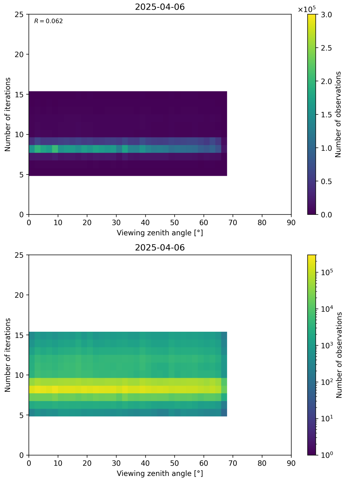
Figure 75: Scatter density plot of “Viewing zenith angle” against “Number of iterations” for 2025-04-05 to 2025-04-07.
