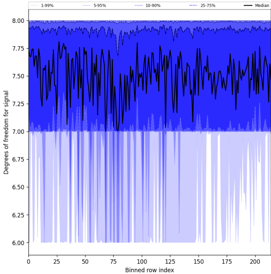
Figure 31: Along track statistics of “Degrees of freedom for signal” for 2025-04-05 to 2025-04-07
