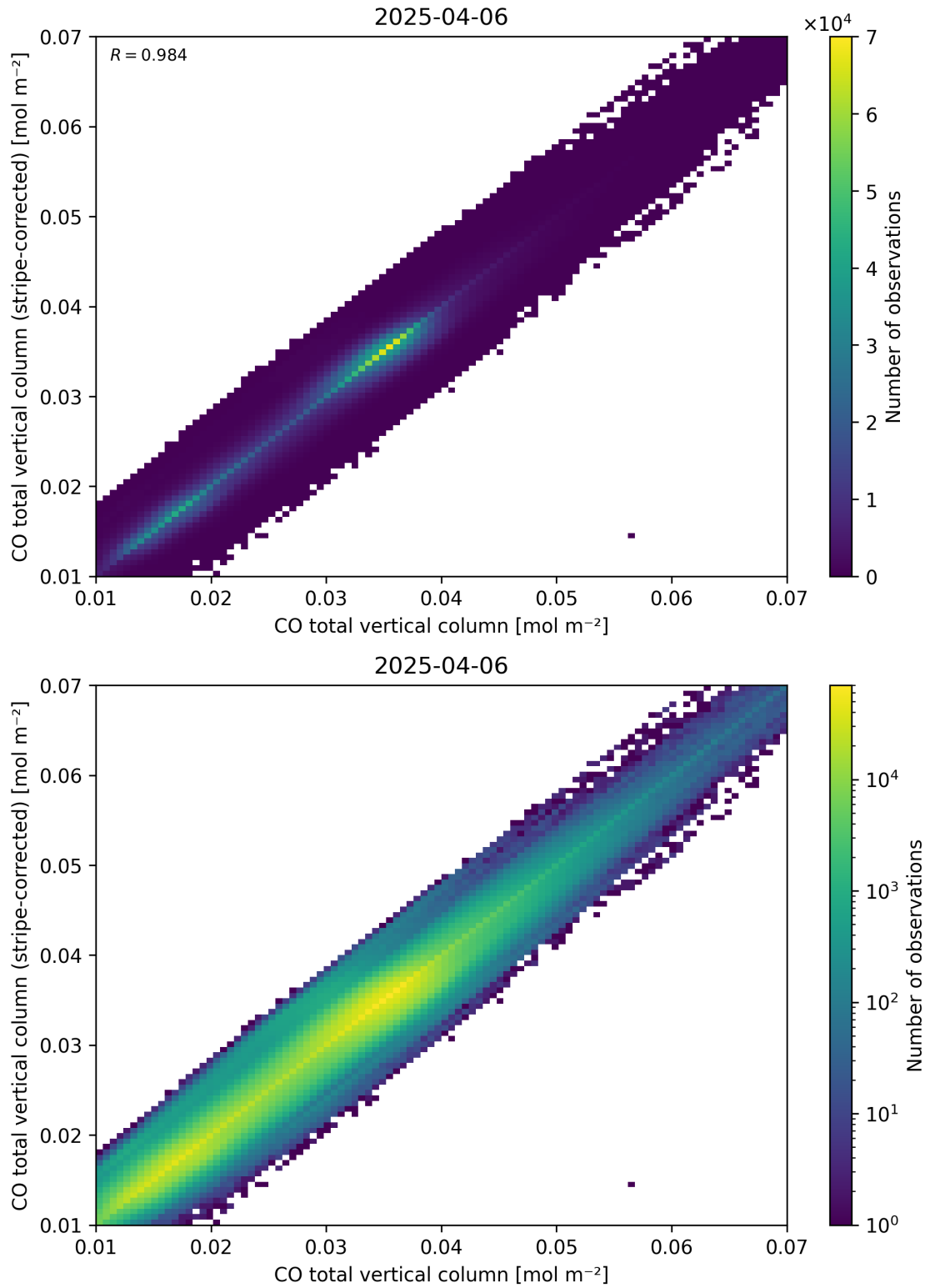
Figure 33: Scatter density plot of “CO total vertical column” against “CO total vertical column (stripe-corrected)” for 2025-04-05 to 2025-04-07.
