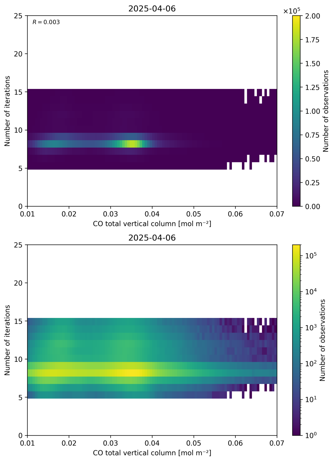
Figure 42: Scatter density plot of “CO total vertical column” against “Number of iterations” for 2025-04-05 to 2025-04-07.
