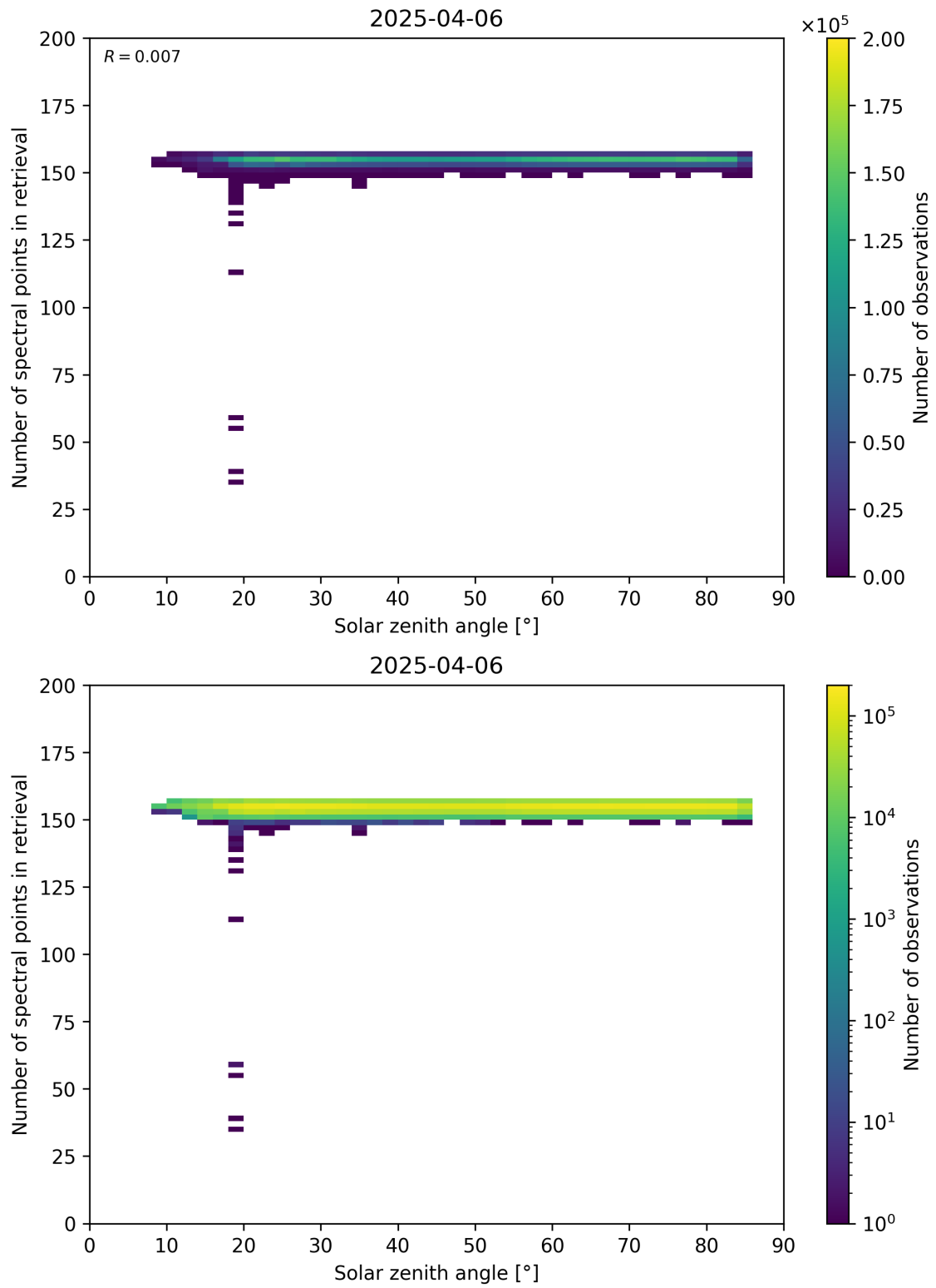
Figure 68: Scatter density plot of “Solar zenith angle” against “Number of spectral points in retrieval” for 2025-04-05 to 2025-04-07.
