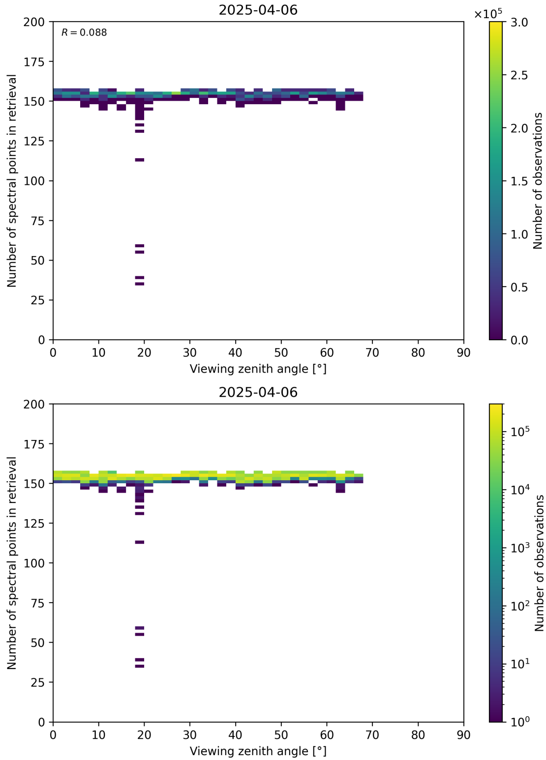
Figure 76: Scatter density plot of “Viewing zenith angle” against “Number of spectral points in retrieval” for 2025-04-05 to 2025-04-07.
