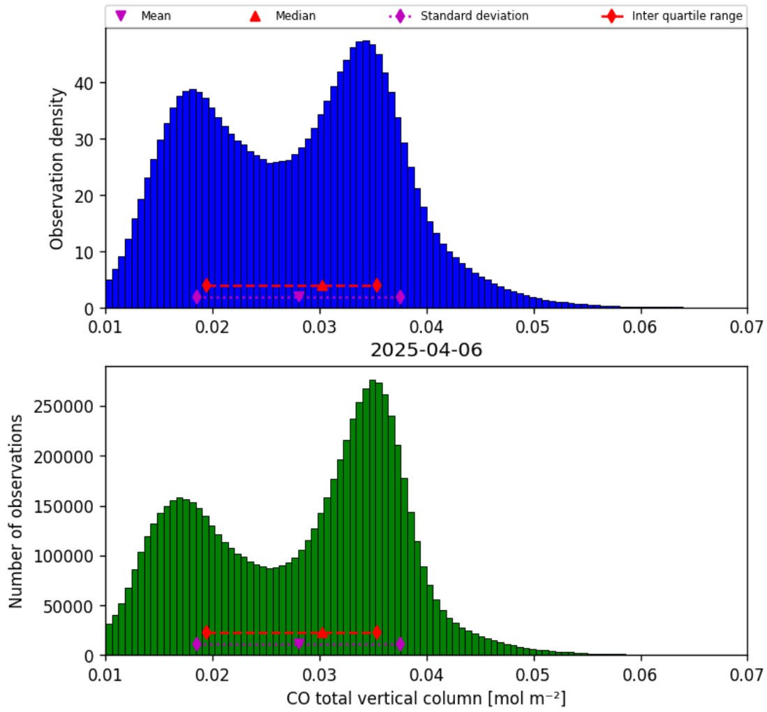
Figure 18: Histogram of “CO total vertical column” for 2025-04-05 to 2025-04-07
