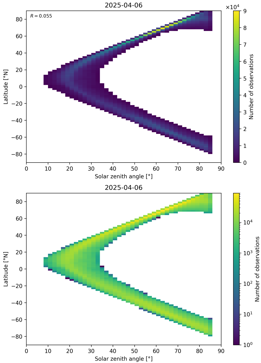
Figure 66: Scatter density plot of “Solar zenith angle” against “Latitude” for 2025-04-05 to 2025-04-07.
