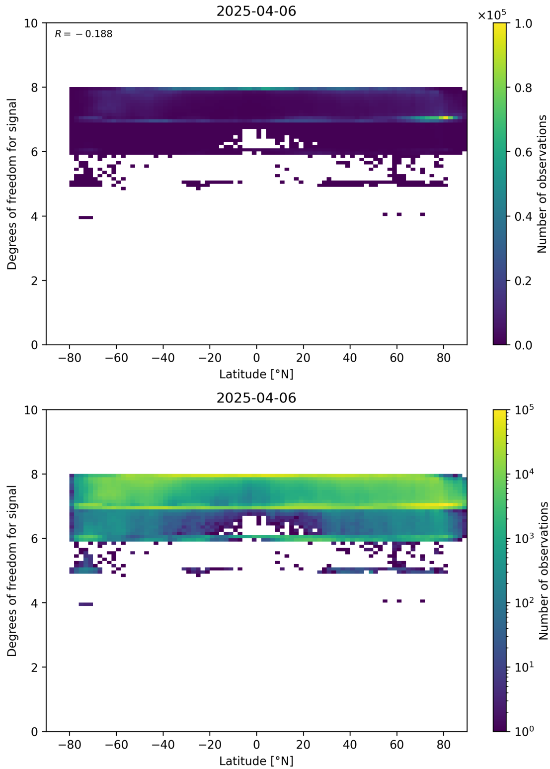
Figure 55: Scatter density plot of “Latitude” against “Degrees of freedom for signal” for 2025-04-05 to 2025-04-07.
