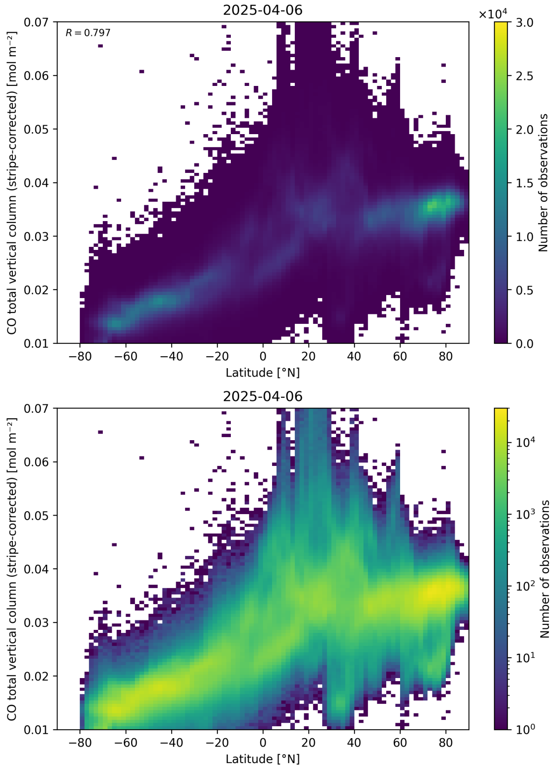
Figure 52: Scatter density plot of “Latitude” against “CO total vertical column (stripe-corrected)” for 2025-04-05 to 2025-04-07.
