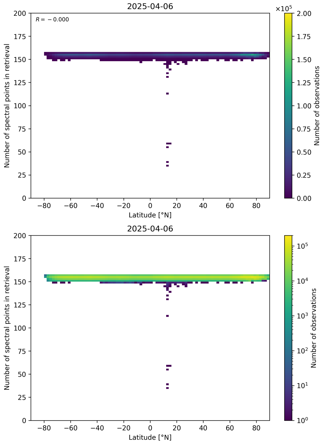
Figure 57: Scatter density plot of “Latitude” against “Number of spectral points in retrieval” for 2025-04-05 to 2025-04-07.
