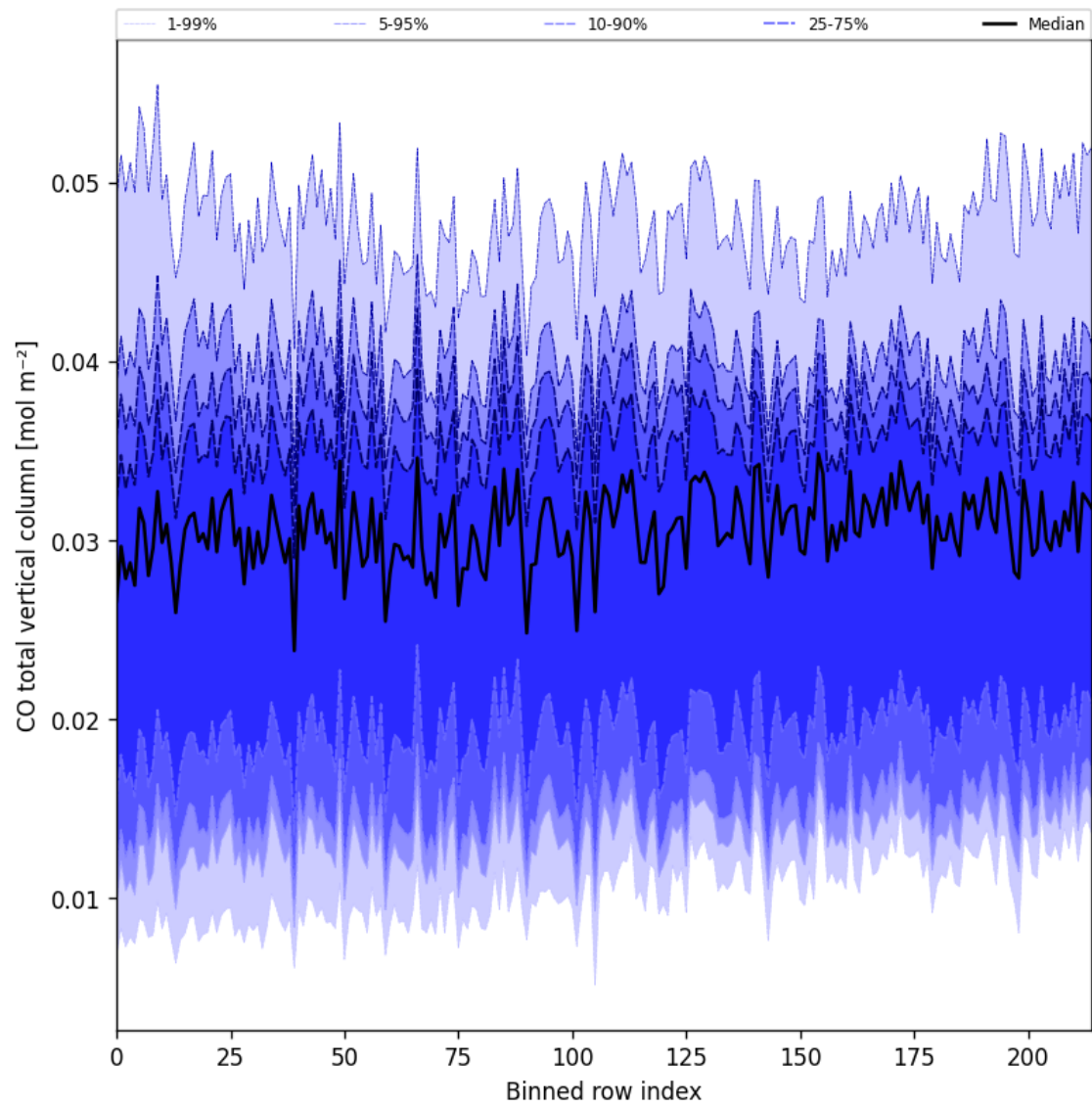
Figure 26: Along track statistics of “CO total vertical column” for 2025-04-05 to 2025-04-07
