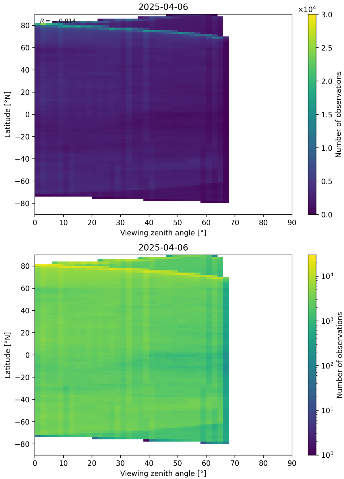
Figure 74: Scatter density plot of “Viewing zenith angle” against “Latitude” for 2025-04-05 to 2025-04-07.
