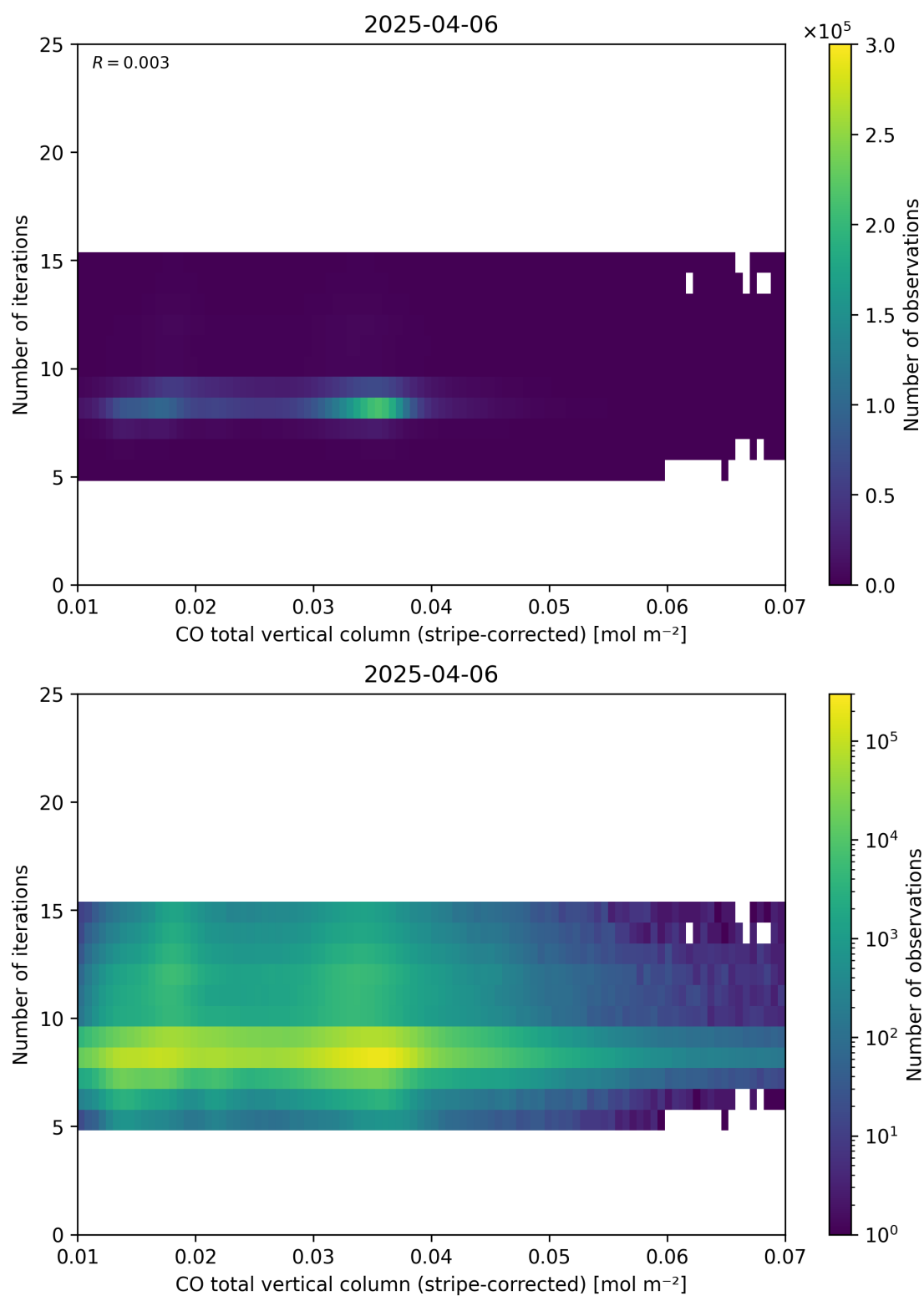
Figure 39: Scatter density plot of “CO total vertical column (stripe-corrected)” against “Number of iterations” for 2025-04-05 to 2025-04-07.
