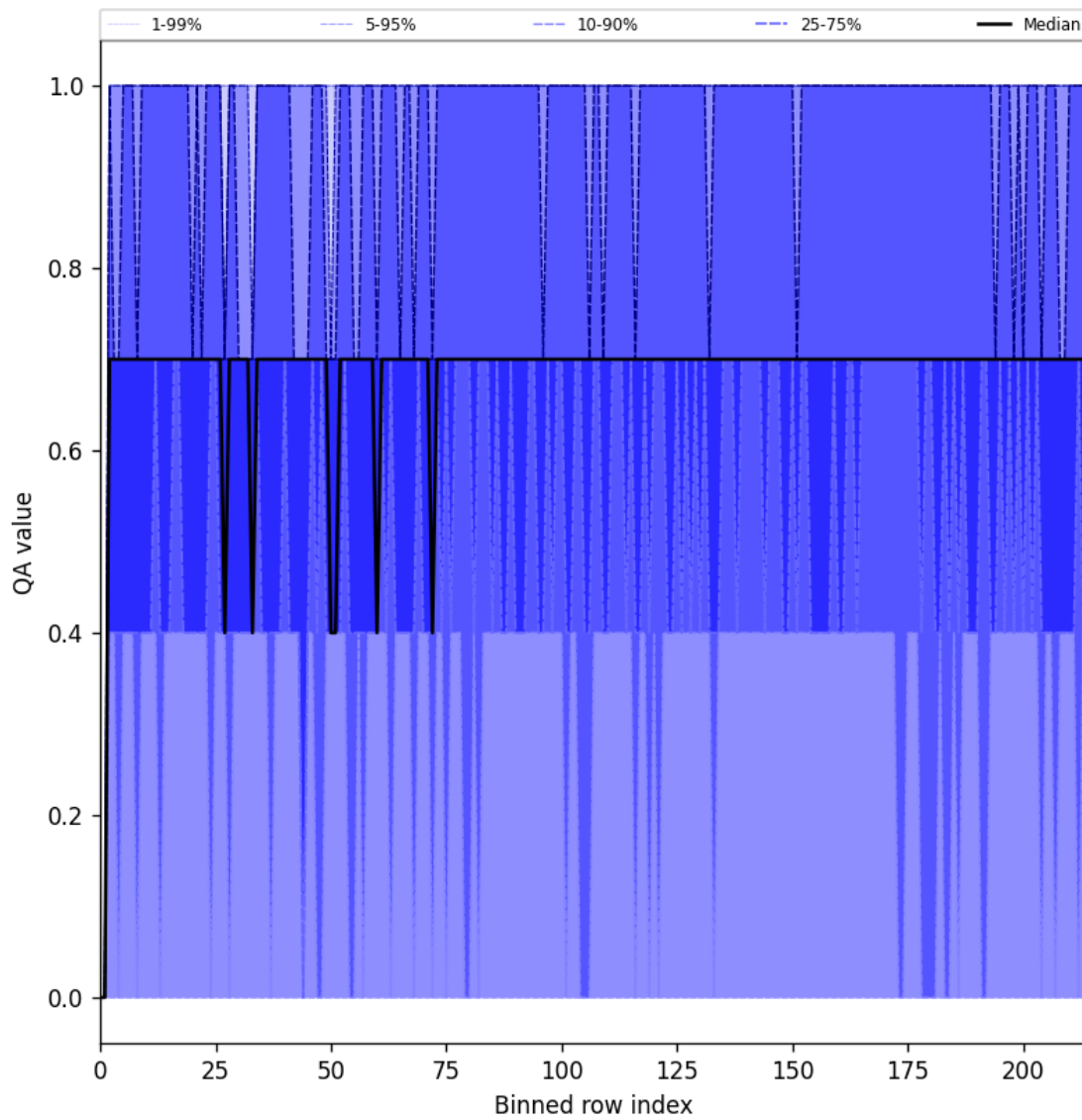
Figure 25: Along track statistics of "QA value" for 2025-04-05 to 2025-04-07
