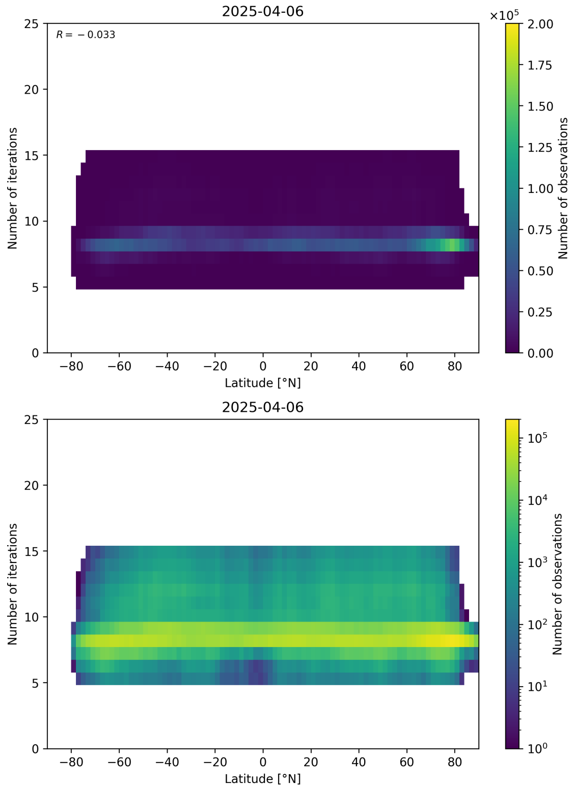
Figure 56: Scatter density plot of “Latitude” against “Number of iterations” for 2025-04-05 to 2025-04-07.
