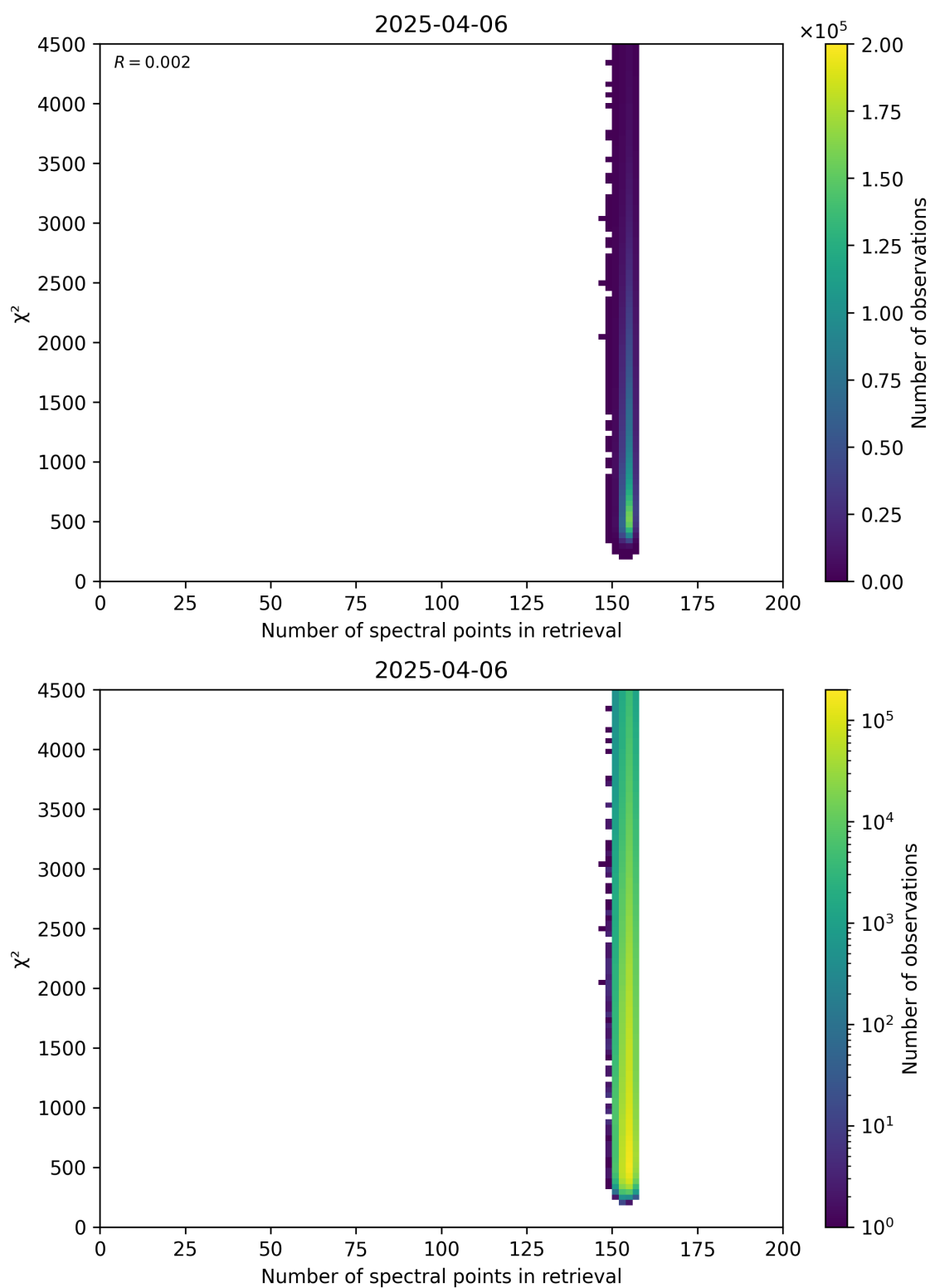
Figure 58: Scatter density plot of “Number of spectral points in retrieval” against “ \chi^2 ” for 2025-04-05 to 2025-04-07.
