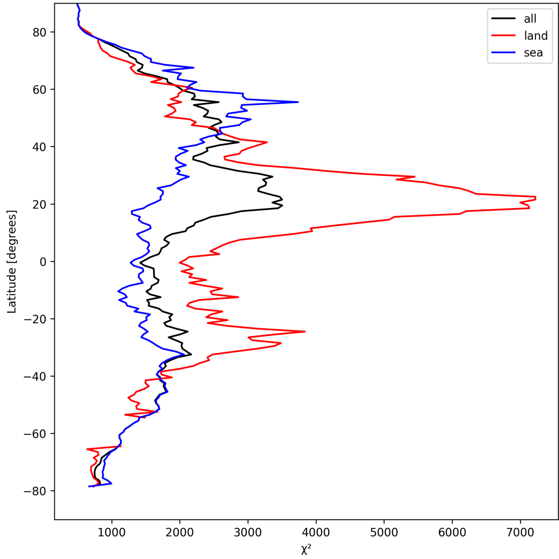
Figure 14: Zonal average of “ \chi^2 ” for 2025-04-05 to 2025-04-07.
