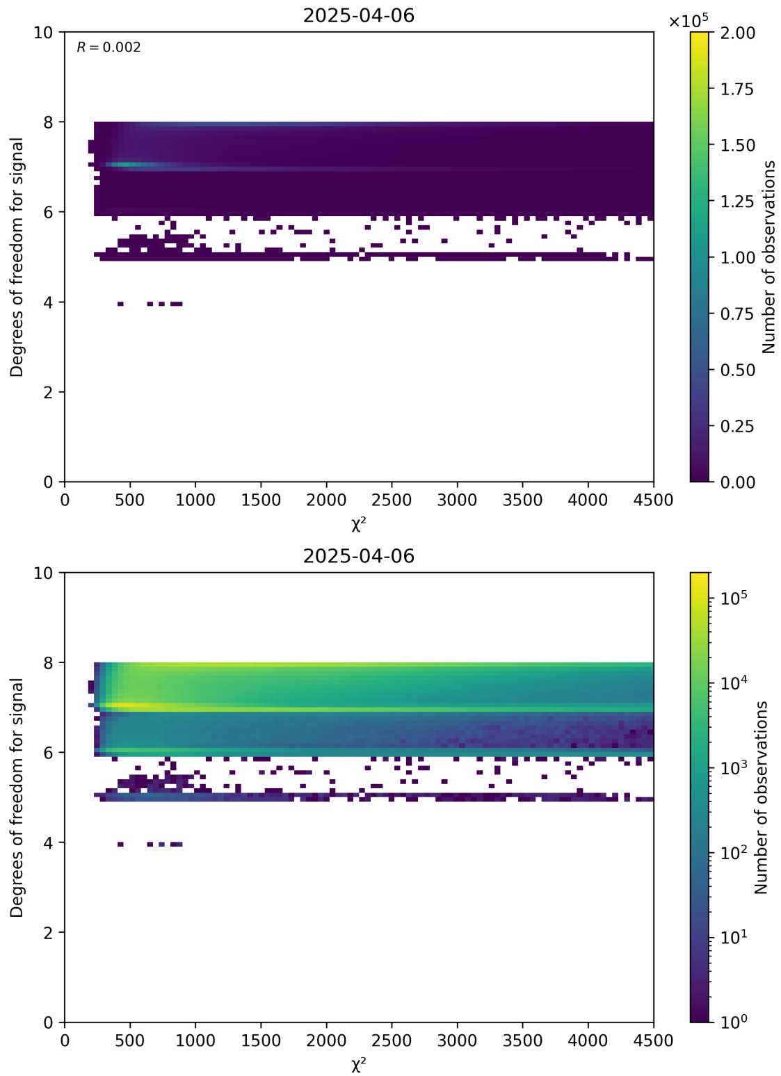
Figure 48: Scatter density plot of “ \chi^2 ” against “Degrees of freedom for signal” for 2025-04-05 to 2025-04-07.
