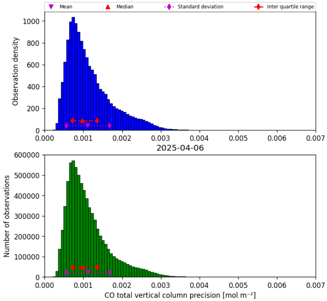
Figure 20: Histogram of “CO total vertical column precision” for 2025-04-05 to 2025-04-07
