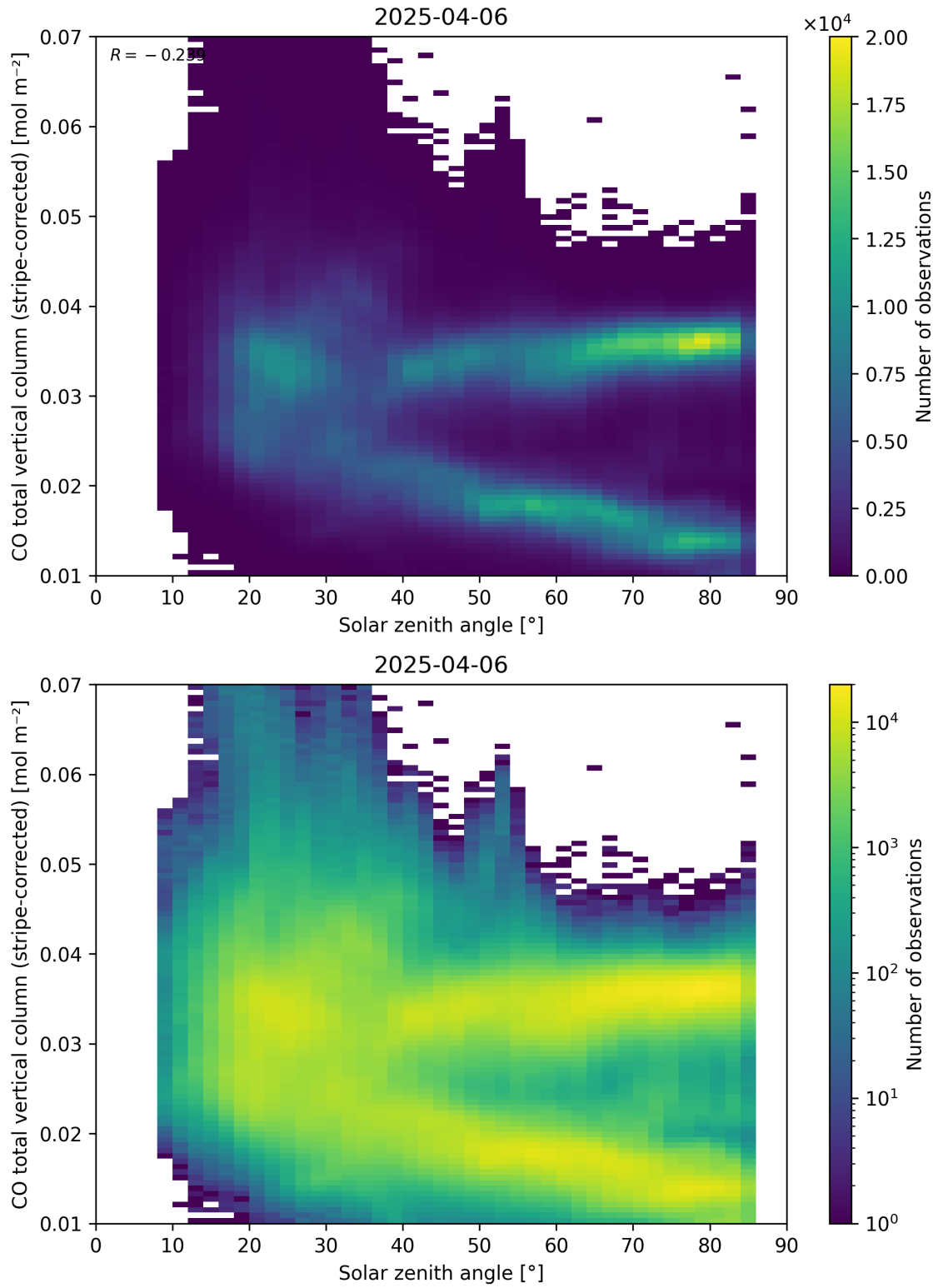
Figure 62: Scatter density plot of “Solar zenith angle” against “CO total vertical column (stripe-corrected)” for 2025-04-05 to 2025-04-07.
