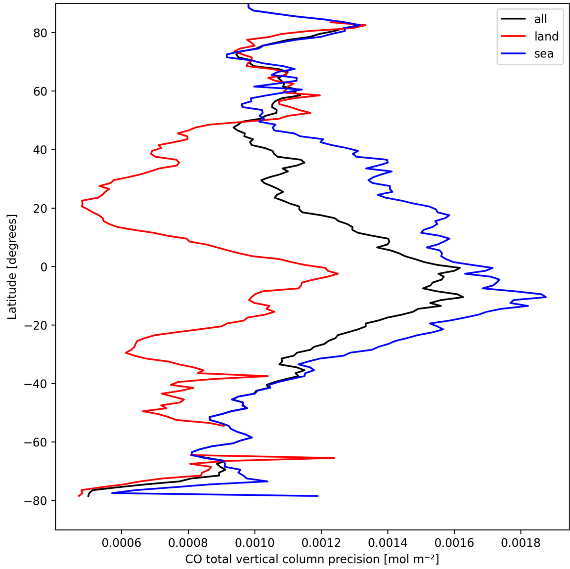
Figure 12: Zonal average of “CO total vertical column precision” for 2025-04-05 to 2025-04-07.
