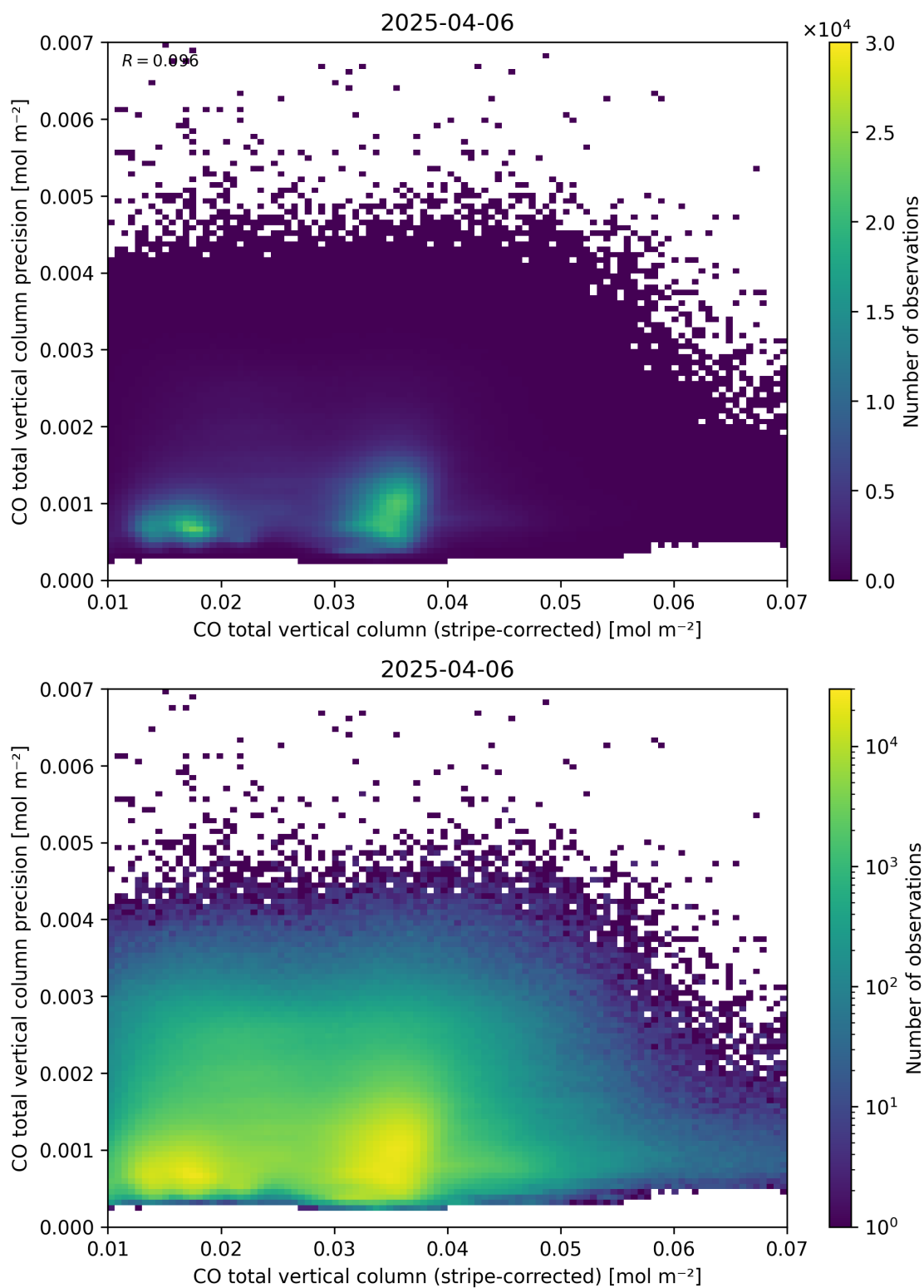
Figure 36: Scatter density plot of “CO total vertical column (stripe-corrected)” against “CO total vertical column precision” for 2025-04-05 to 2025-04-07.
