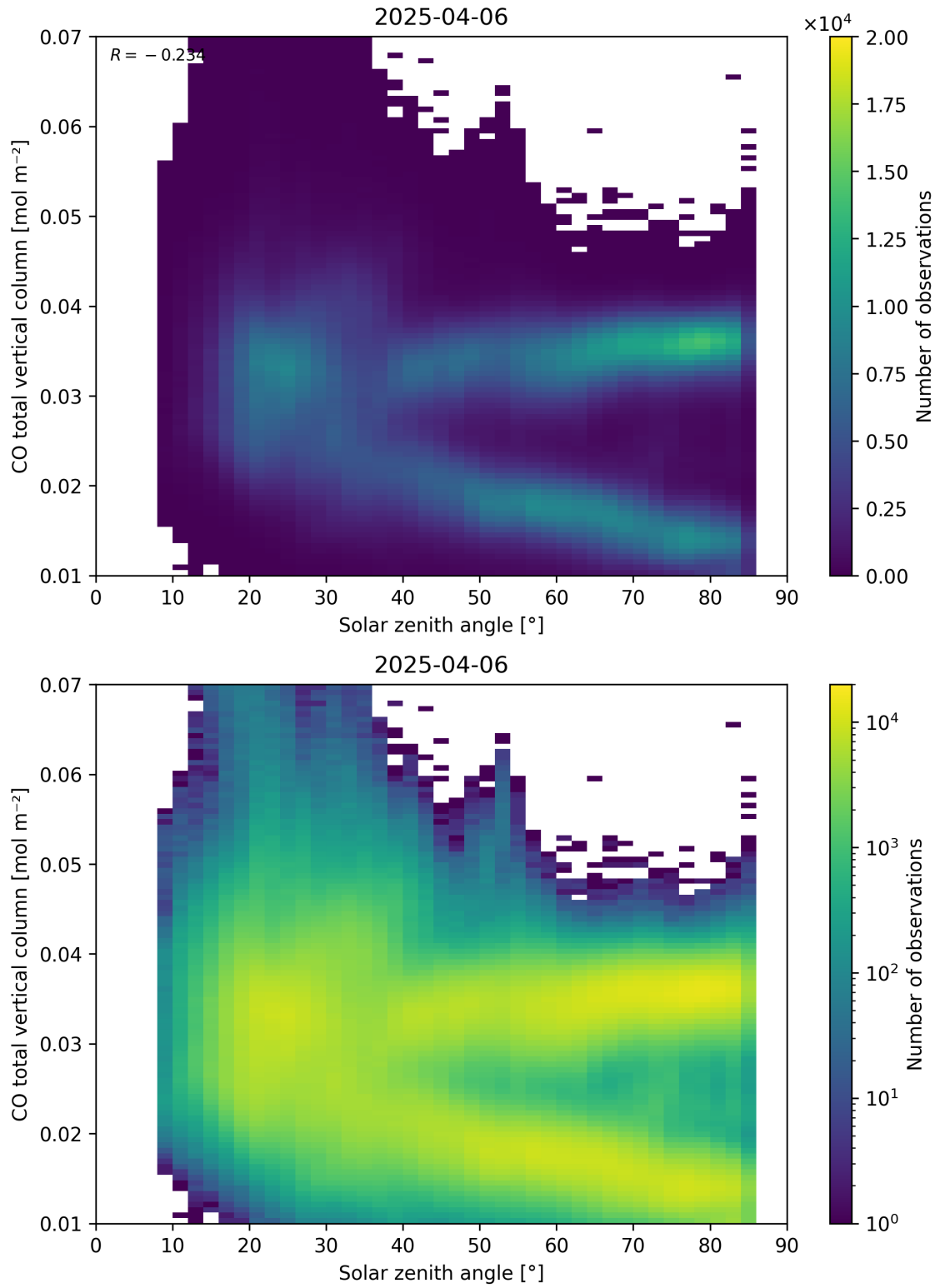
Figure 61: Scatter density plot of “Solar zenith angle” against “CO total vertical column” for 2025-04-05 to 2025-04-07.
