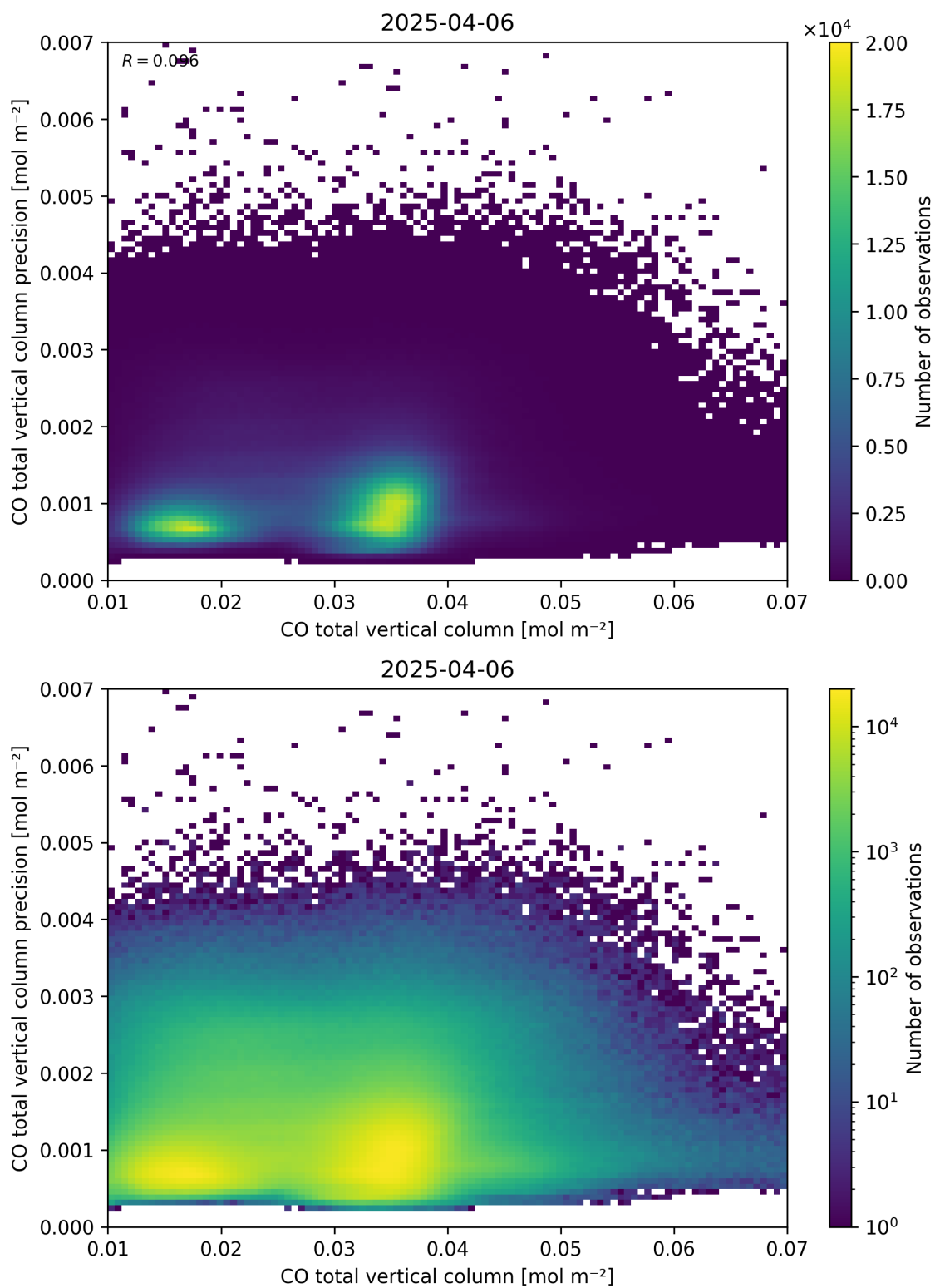
Figure 34: Scatter density plot of “CO total vertical column” against “CO total vertical column precision” for 2025-04-05 to 2025-04-07.
