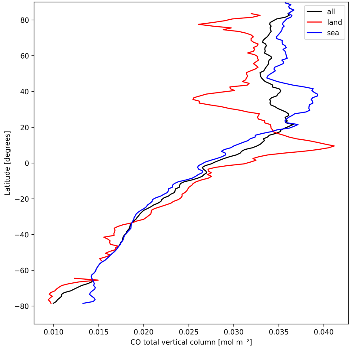
Figure 10: Zonal average of “CO total vertical column” for 2025-04-05 to 2025-04-07.
