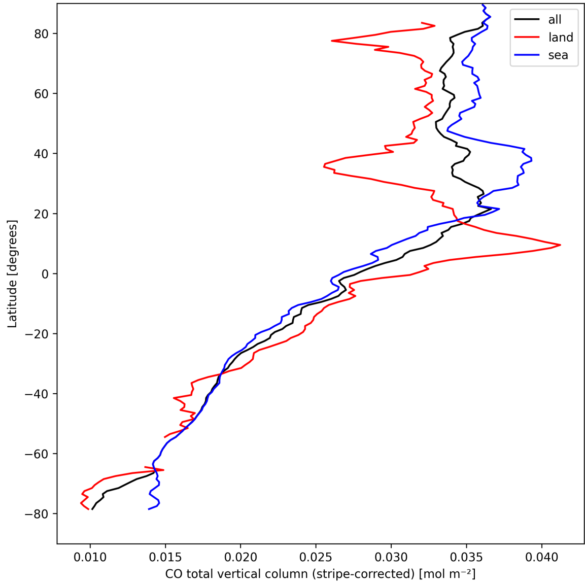
Figure 11: Zonal average of “CO total vertical column (stripe-corrected)” for 2025-04-05 to 2025-04-07.
