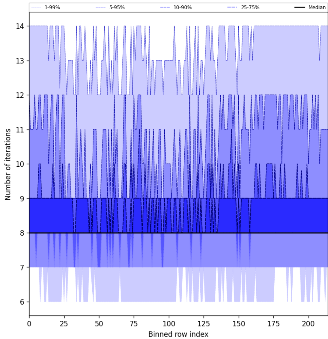
Figure 32: Along track statistics of “Number of iterations” for 2025-04-05 to 2025-04-07
