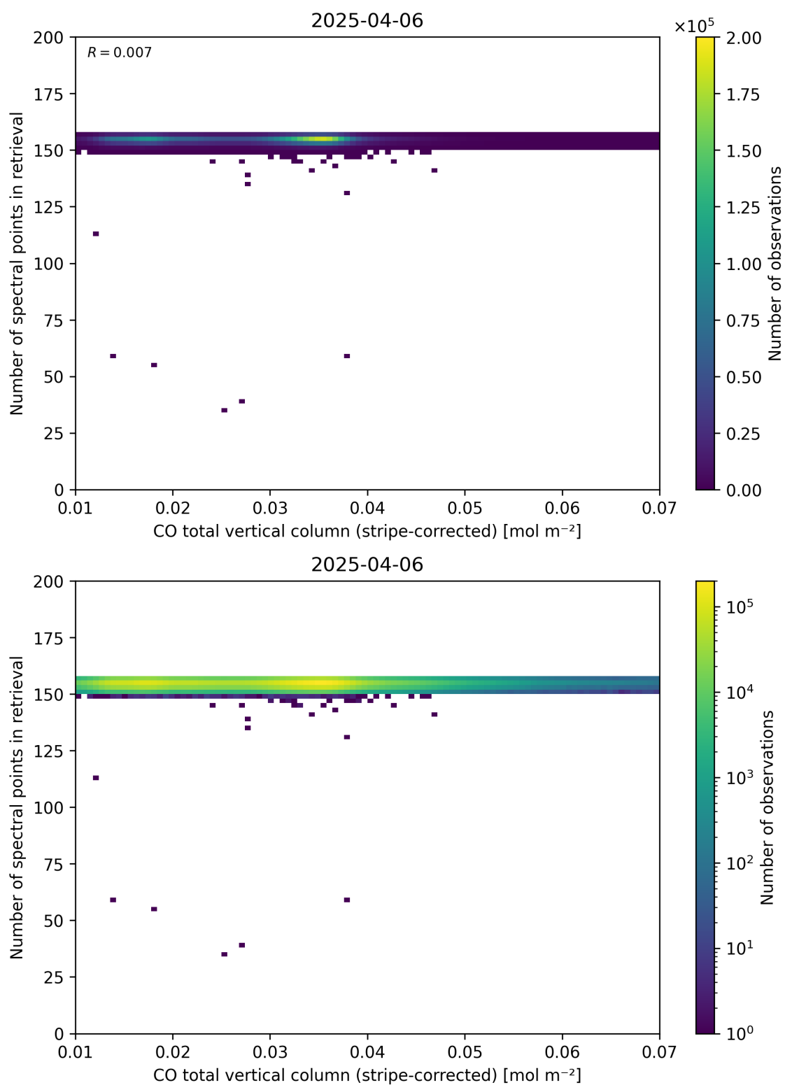
Figure 40: Scatter density plot of “CO total vertical column (stripe-corrected)” against “Number of spectral points in retrieval” for 2025-04-05 to 2025-04-07.
