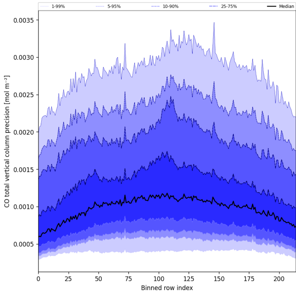
Figure 28: Along track statistics of “CO total vertical column precision” for 2025-04-05 to 2025-04-07
