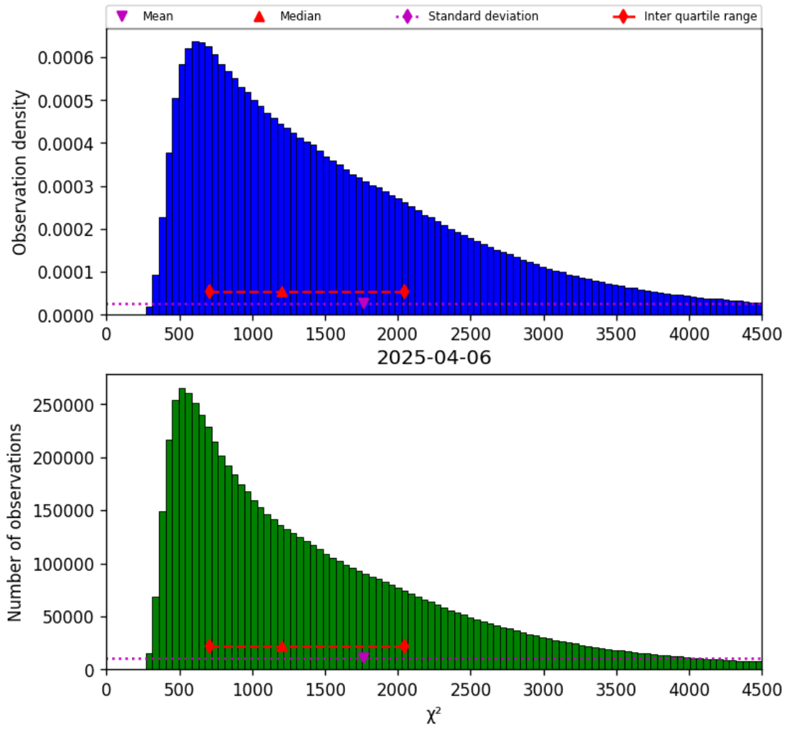
Figure 22: Histogram of “ \chi^2 ” for 2025-04-05 to 2025-04-07
