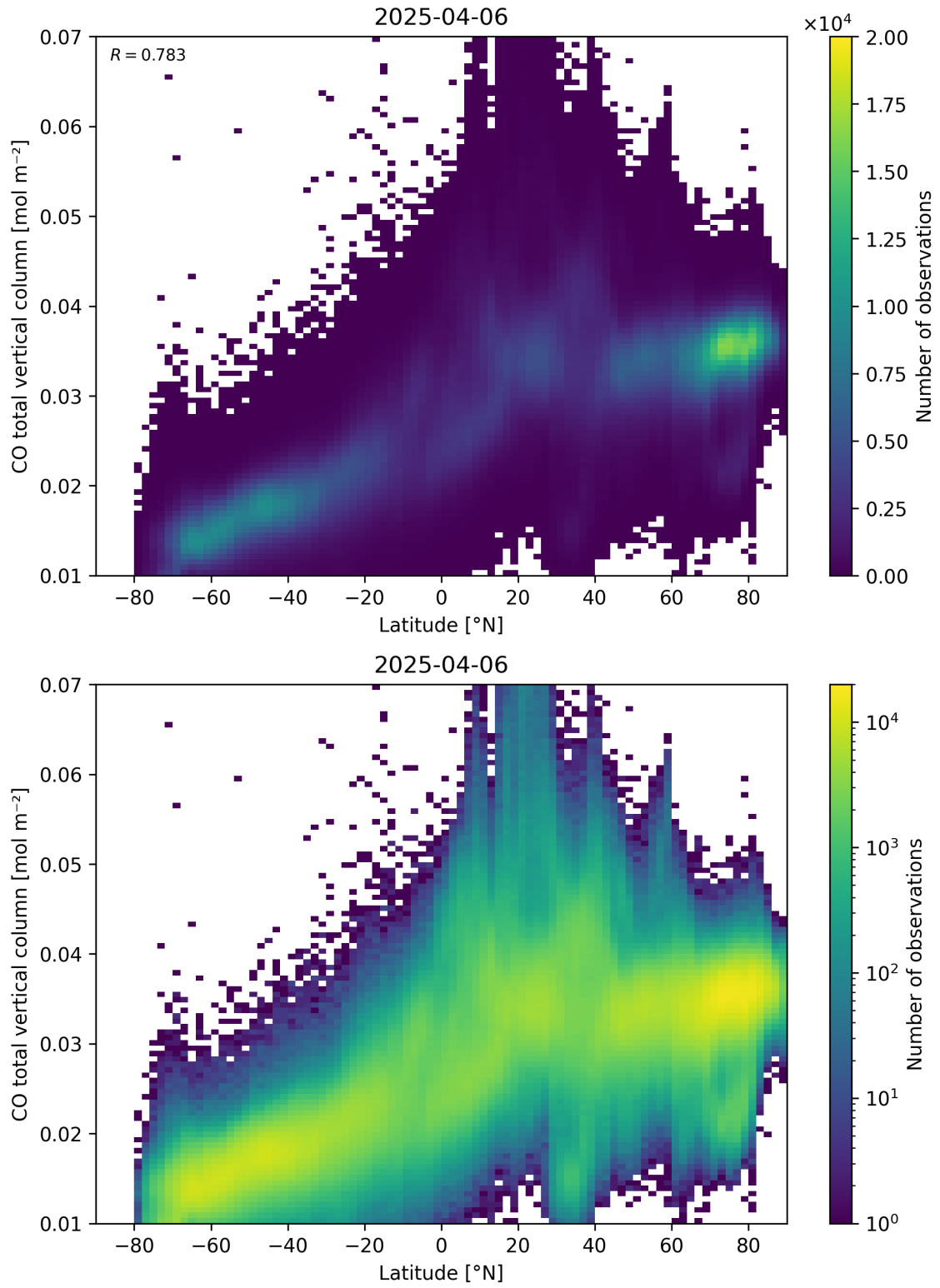
Figure 51: Scatter density plot of “Latitude” against “CO total vertical column” for 2025-04-05 to 2025-04-07.
