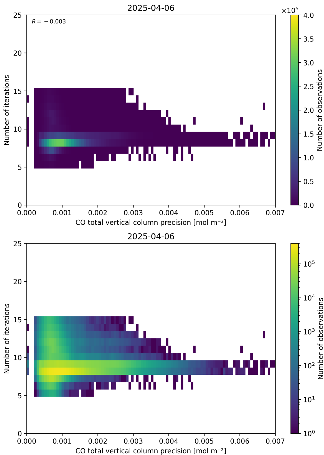
Figure 46: Scatter density plot of “CO total vertical column precision” against “Number of iterations” for 2025-04-05 to 2025-04-07.
