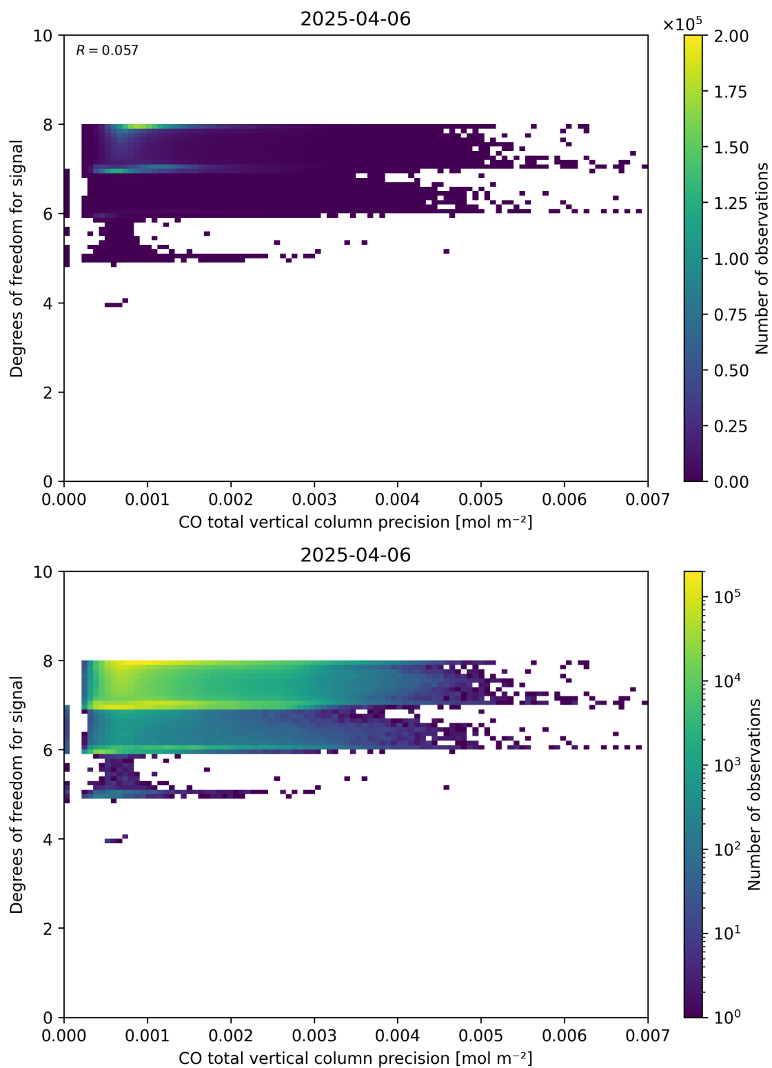
Figure 45: Scatter density plot of “CO total vertical column precision” against “Degrees of freedom for signal” for 2025-04-05 to 2025-04-07.
