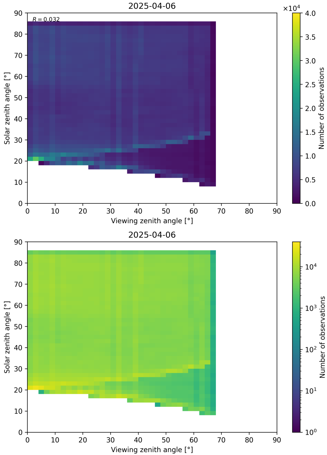
Figure 77: Scatter density plot of “Viewing zenith angle” against “Solar zenith angle” for 2025-04-05 to 2025-04-07.
