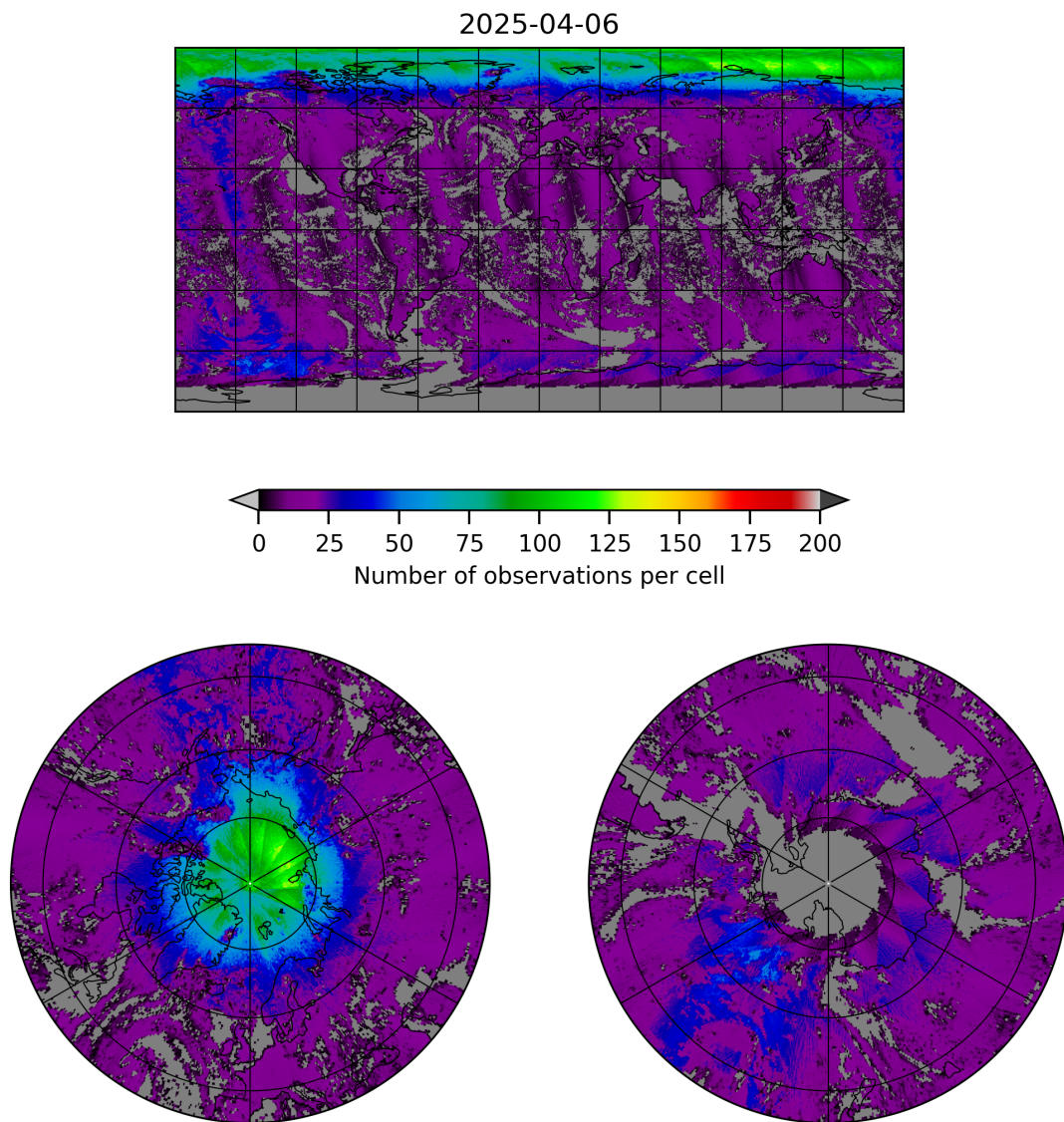
Figure 8: Map of the number of observations for 2025-04-05 to 2025-04-07
