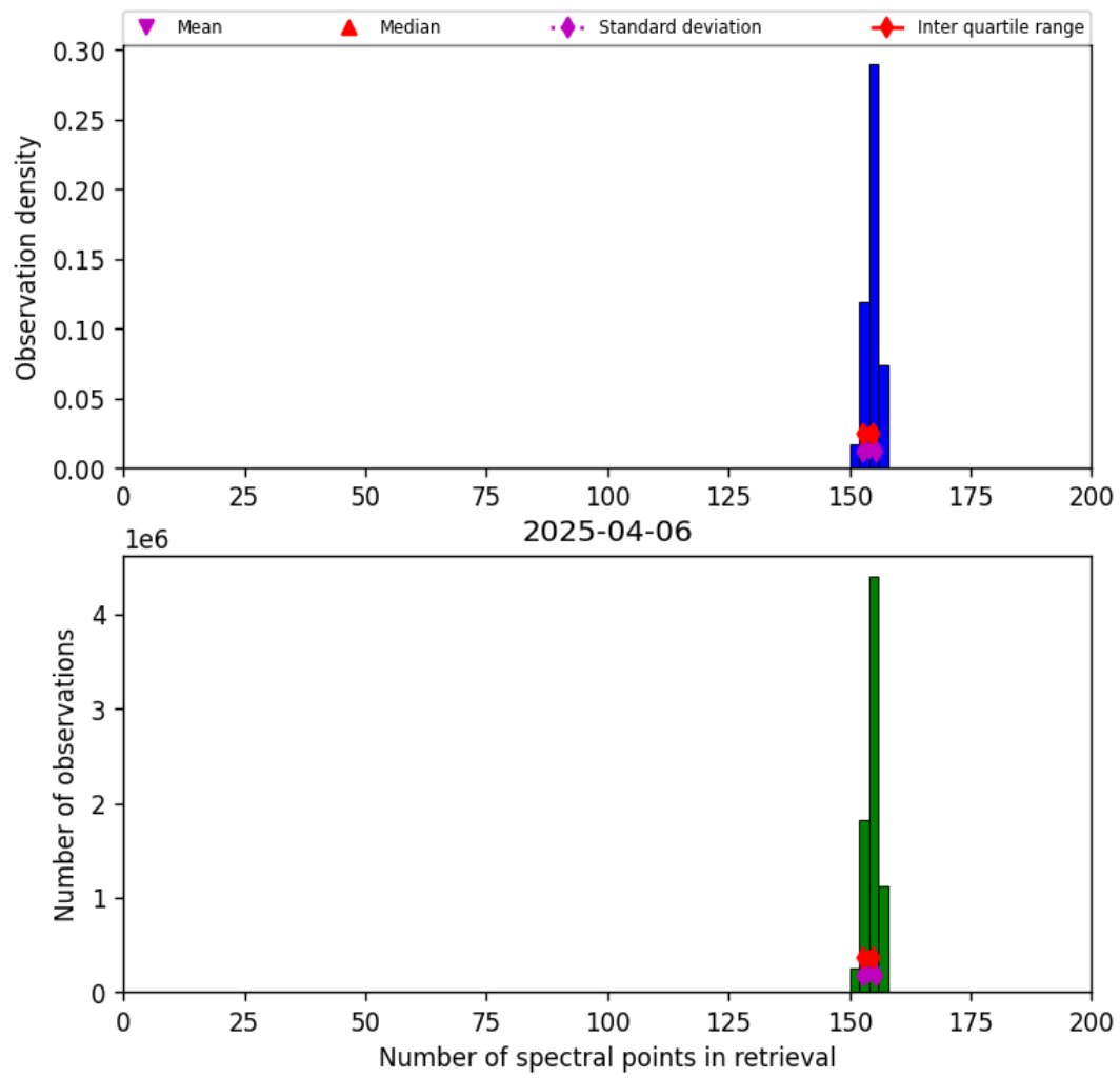
Figure 21: Histogram of “Number of spectral points in retrieval” for 2025-04-05 to 2025-04-07
