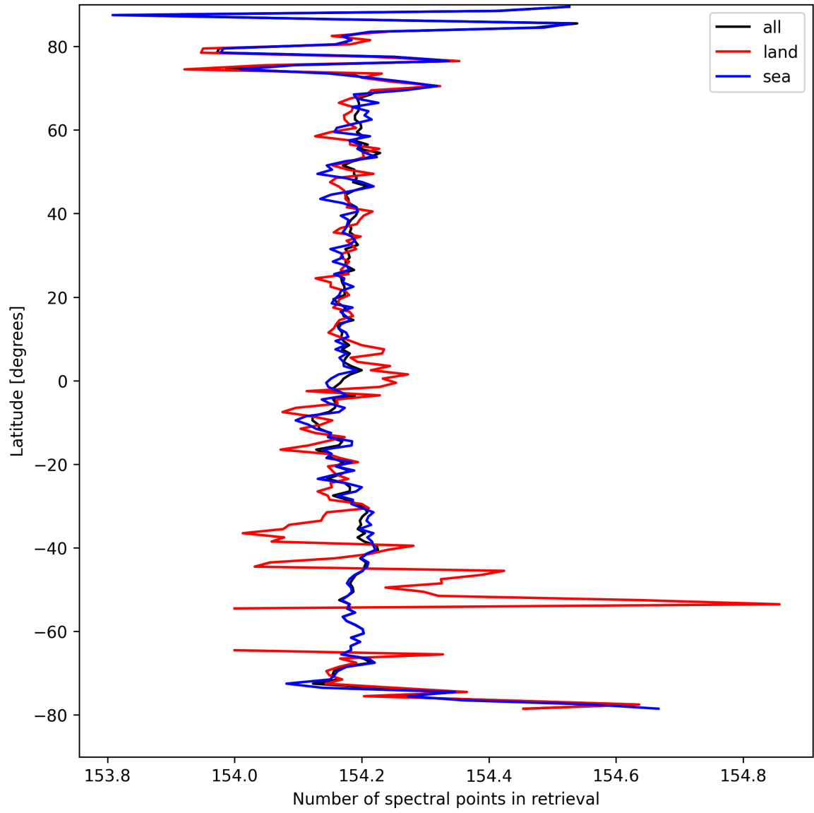
Figure 13: Zonal average of “Number of spectral points in retrieval” for 2025-04-05 to 2025-04-07.
