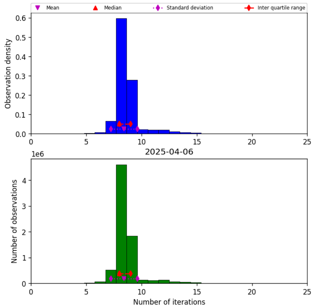
Figure 24: Histogram of “Number of iterations” for 2025-04-05 to 2025-04-07
