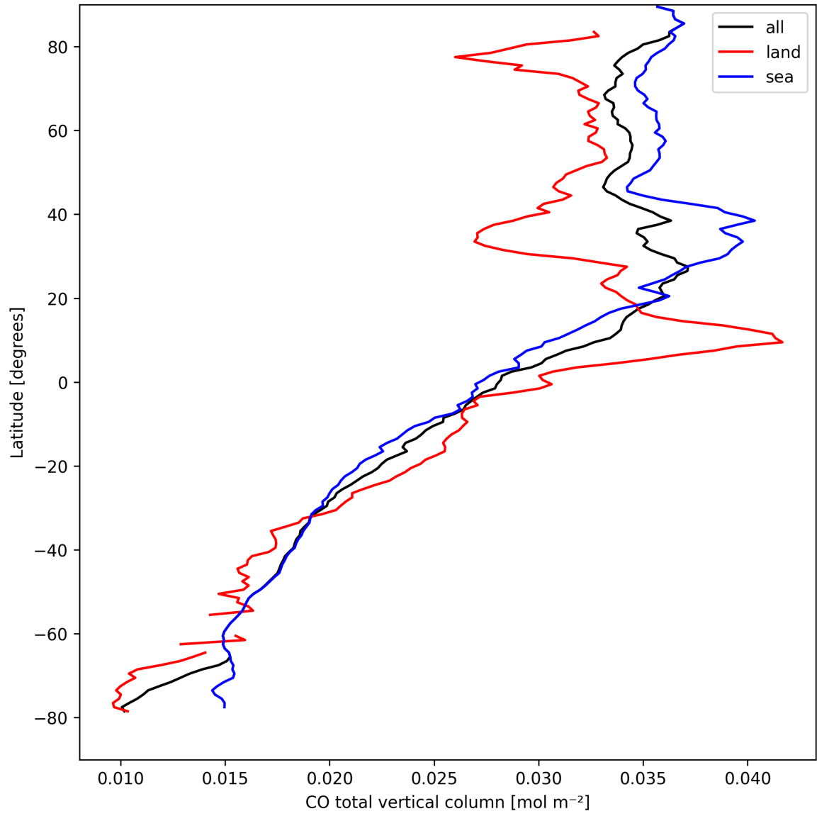
Figure 10: Zonal average of “CO total vertical column” for 2025-04-06 to 2025-04-08.
