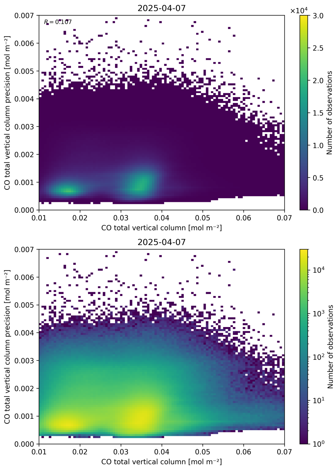
Figure 34: Scatter density plot of “CO total vertical column” against “CO total vertical column precision” for 2025-04-06 to 2025-04-08.
