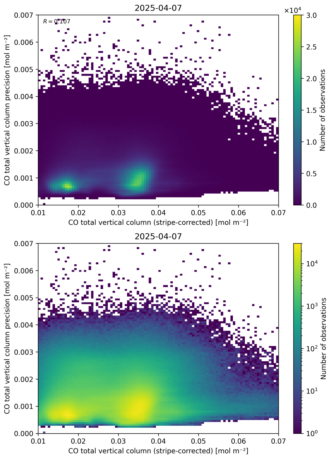
Figure 36: Scatter density plot of “CO total vertical column (stripe-corrected)” against “CO total vertical column precision” for 2025-04-06 to 2025-04-08.
