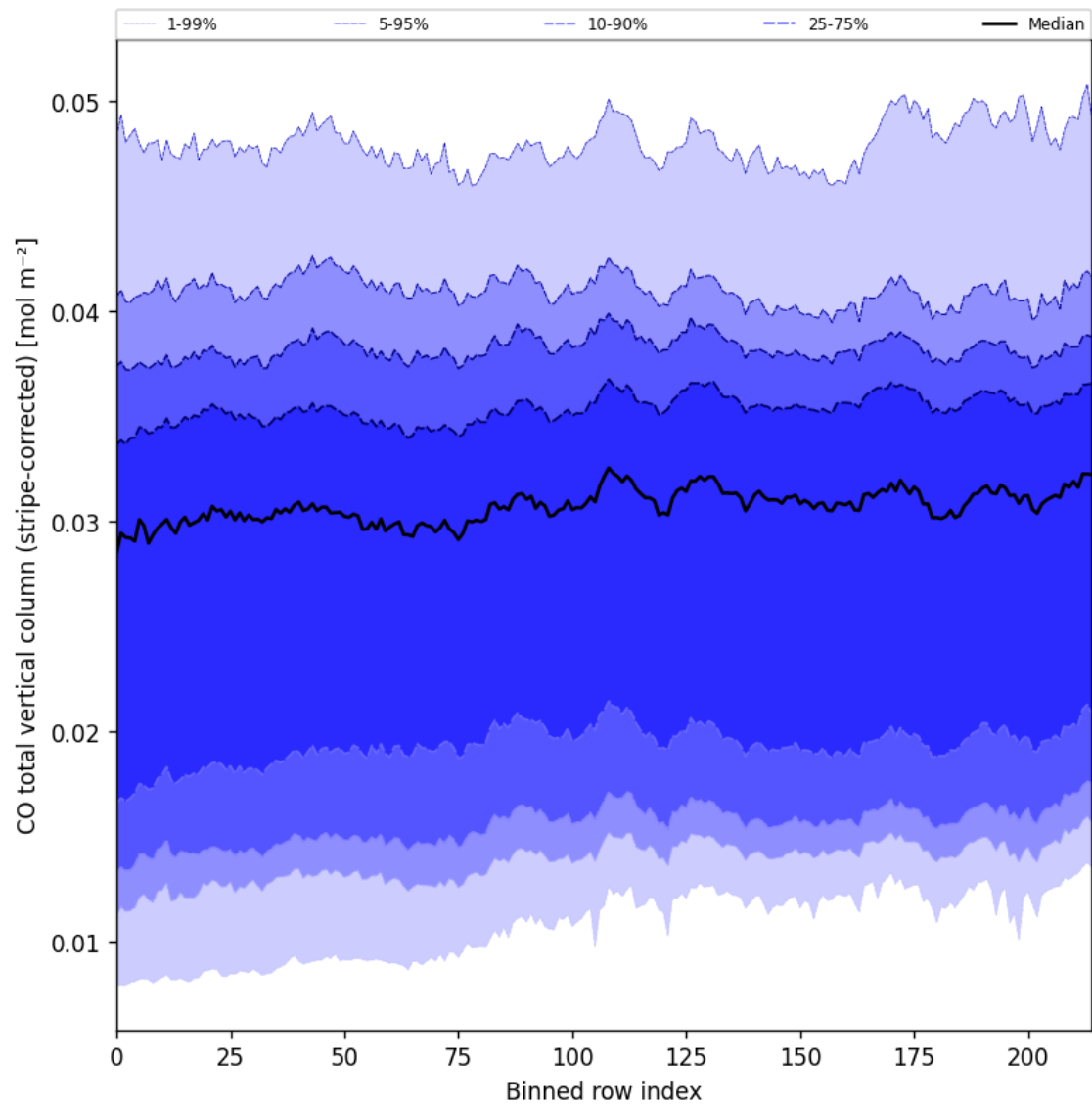
Figure 27: Along track statistics of “CO total vertical column (stripe-corrected)” for 2025-04-06 to 2025-04-08
