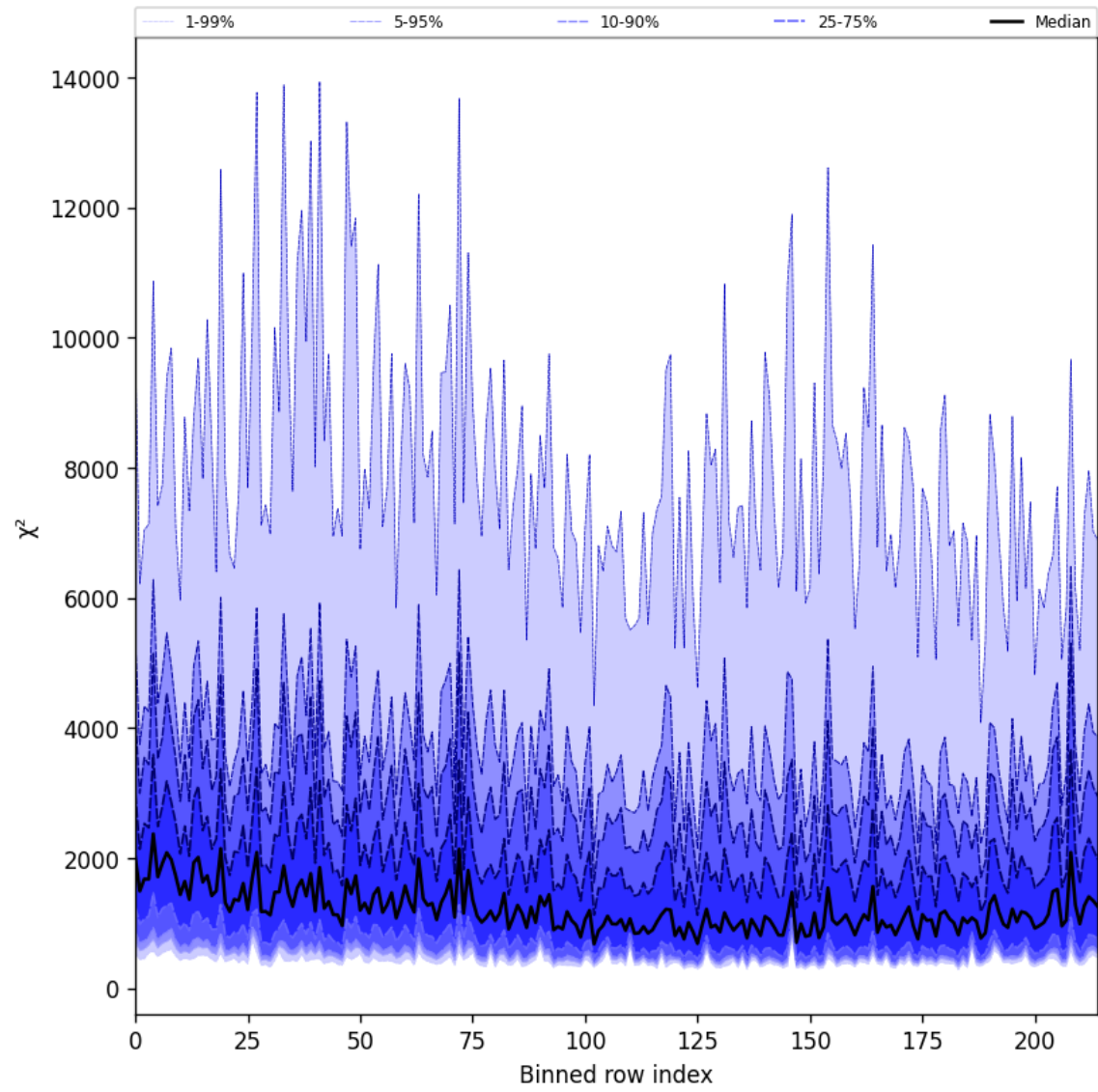
Figure 30: Along track statistics of “ \chi^2 ” for 2025-04-06 to 2025-04-08
