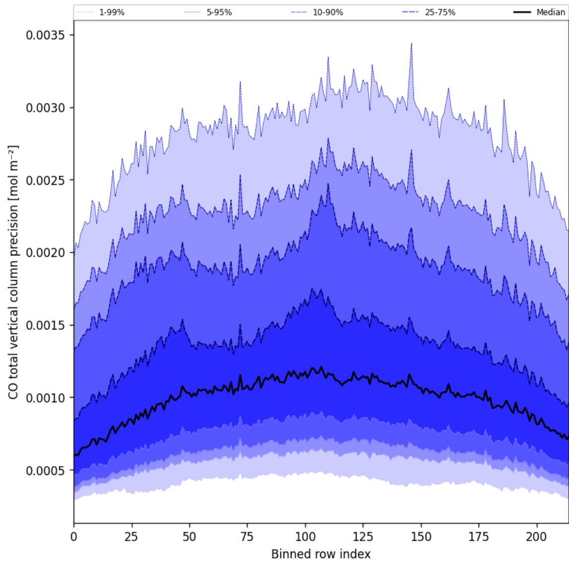
Figure 28: Along track statistics of “CO total vertical column precision” for 2025-04-06 to 2025-04-08
