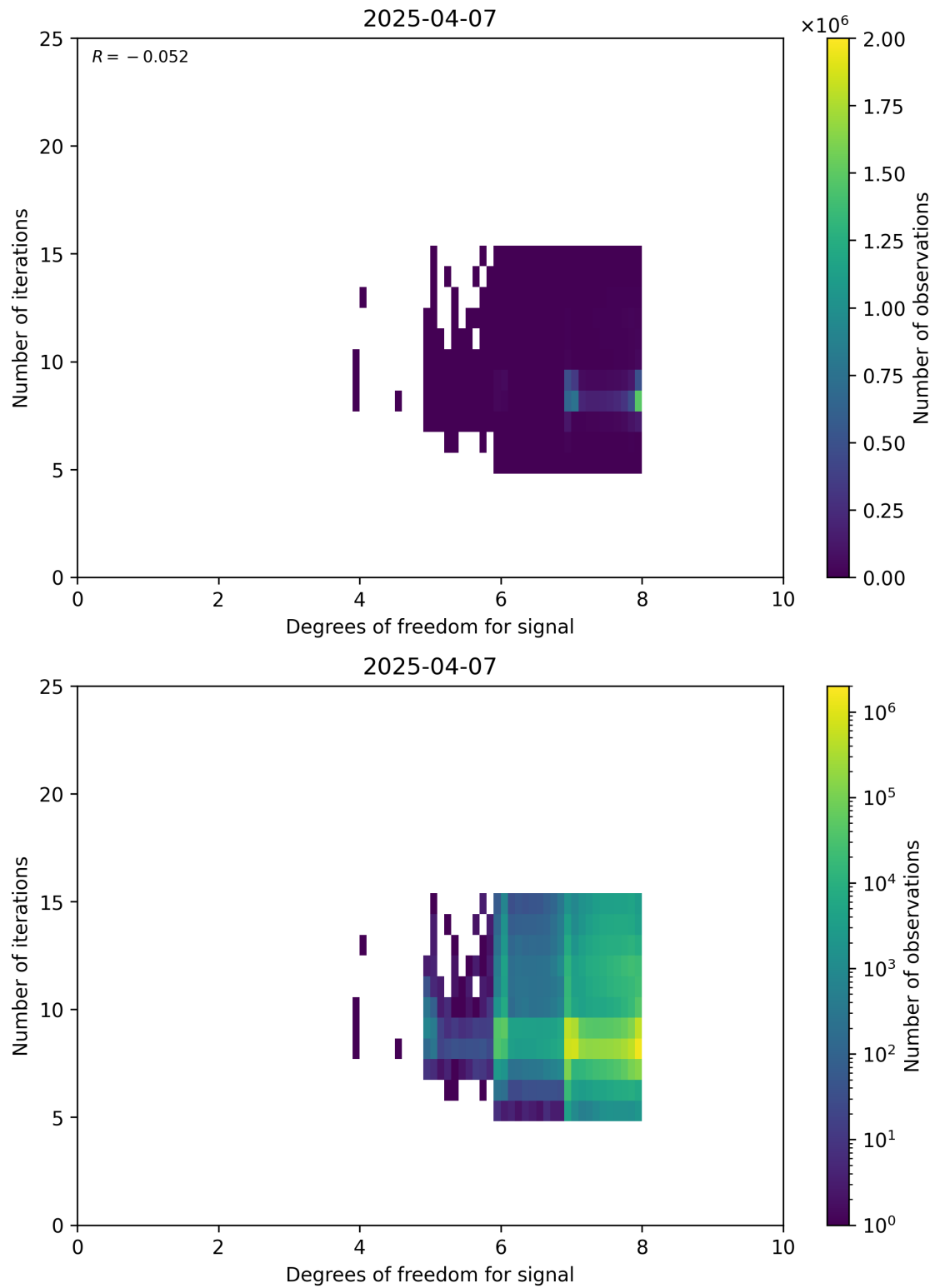
Figure 50: Scatter density plot of “Degrees of freedom for signal” against “Number of iterations” for 2025-04-06 to 2025-04-08.
