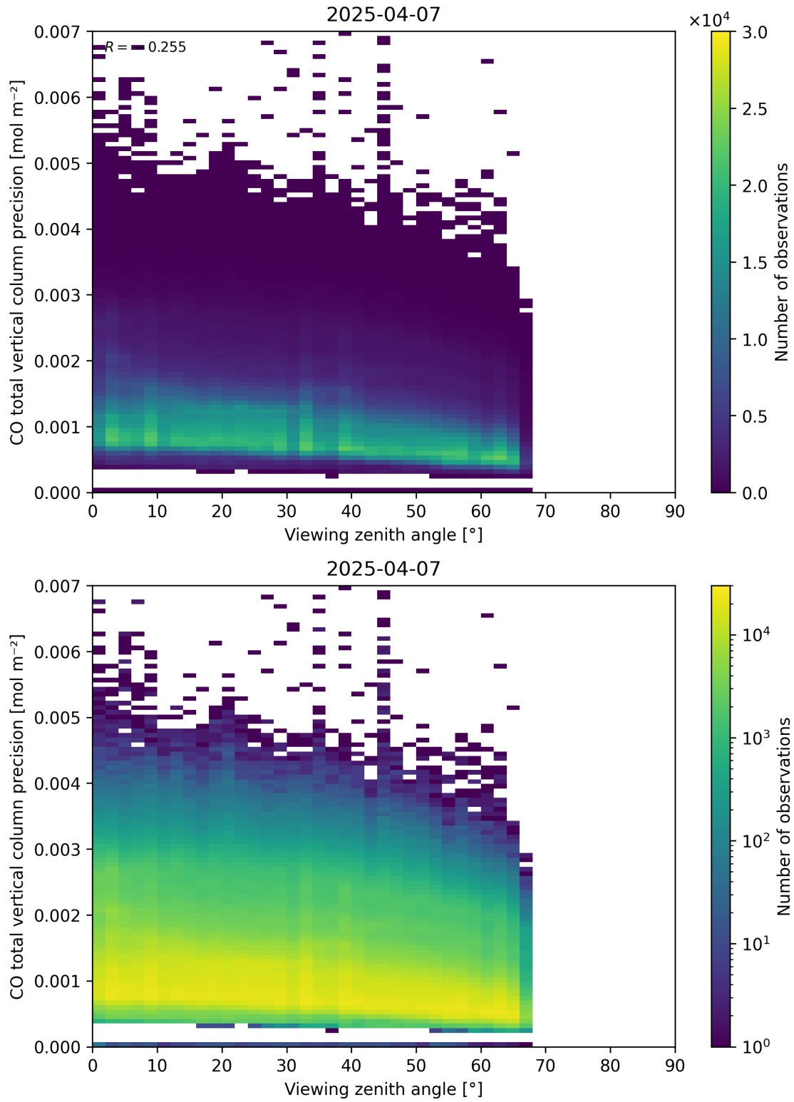
Figure 71: Scatter density plot of “Viewing zenith angle” against “CO total vertical column precision” for 2025-04-06 to 2025-04-08.
