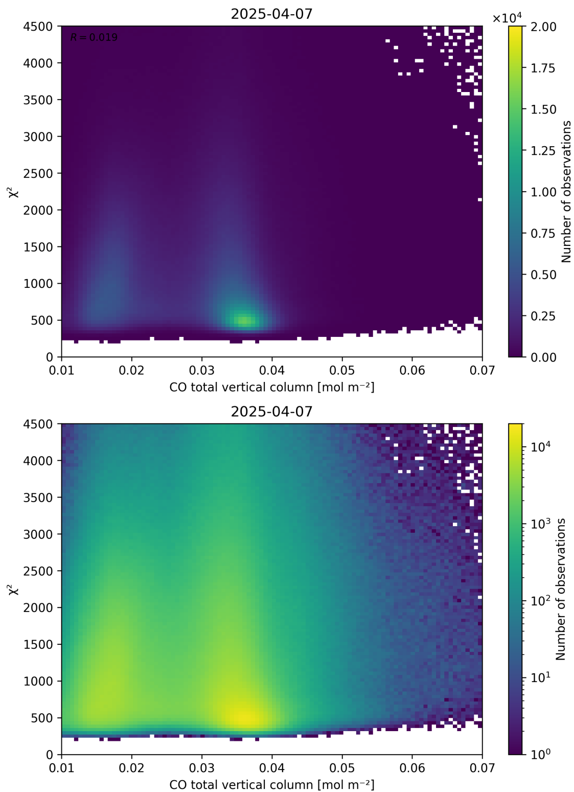
Figure 35: Scatter density plot of “CO total vertical column” against “ \chi^2 ” for 2025-04-06 to 2025-04-08.
