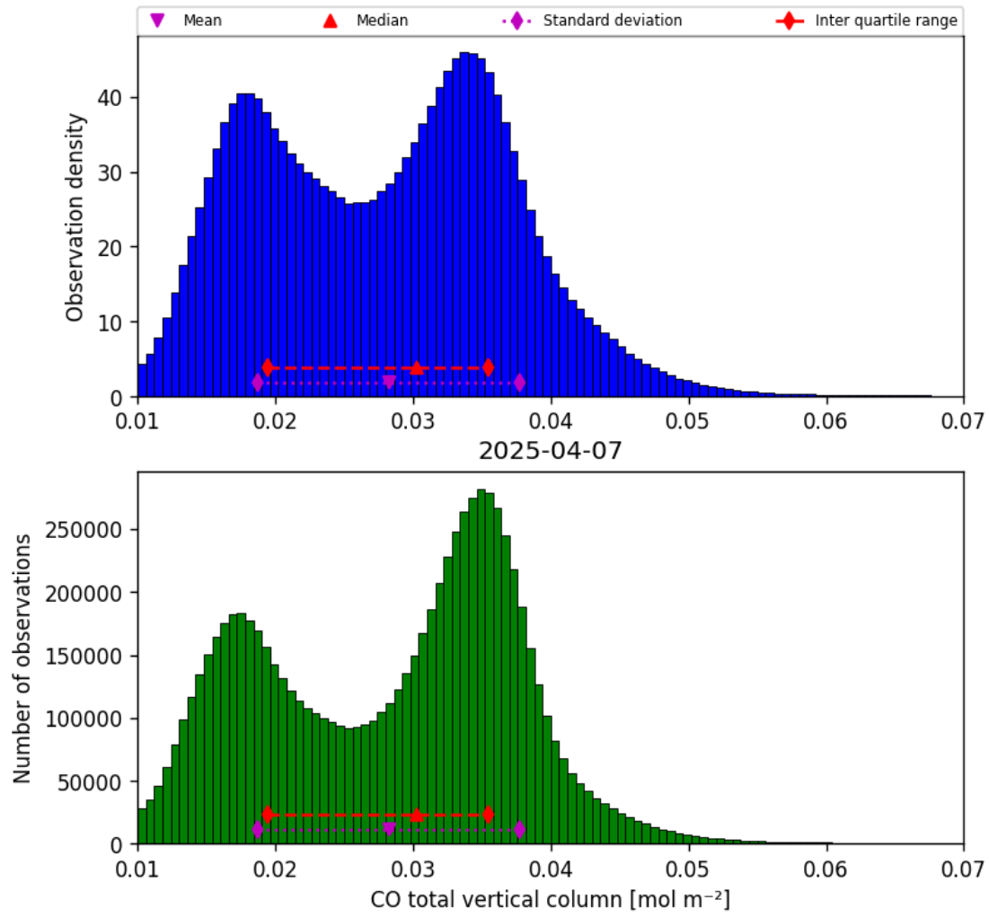
Figure 18: Histogram of “CO total vertical column” for 2025-04-06 to 2025-04-08
