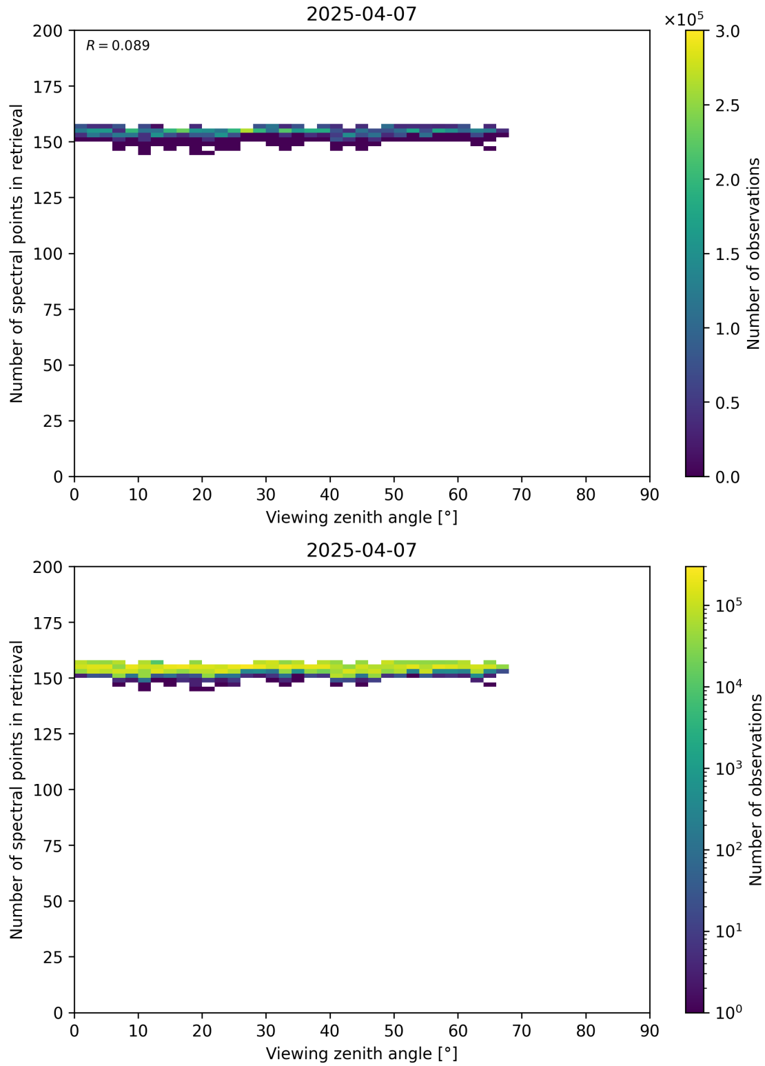
Figure 76: Scatter density plot of “Viewing zenith angle” against “Number of spectral points in retrieval” for 2025-04-06 to 2025-04-08.
