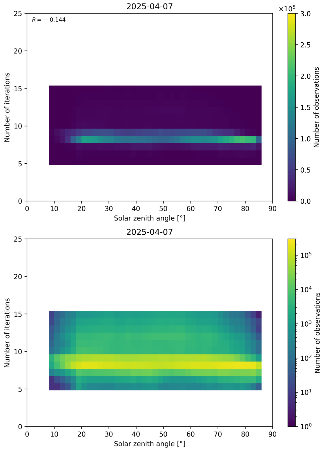
Figure 67: Scatter density plot of “Solar zenith angle” against “Number of iterations” for 2025-04-06 to 2025-04-08.
