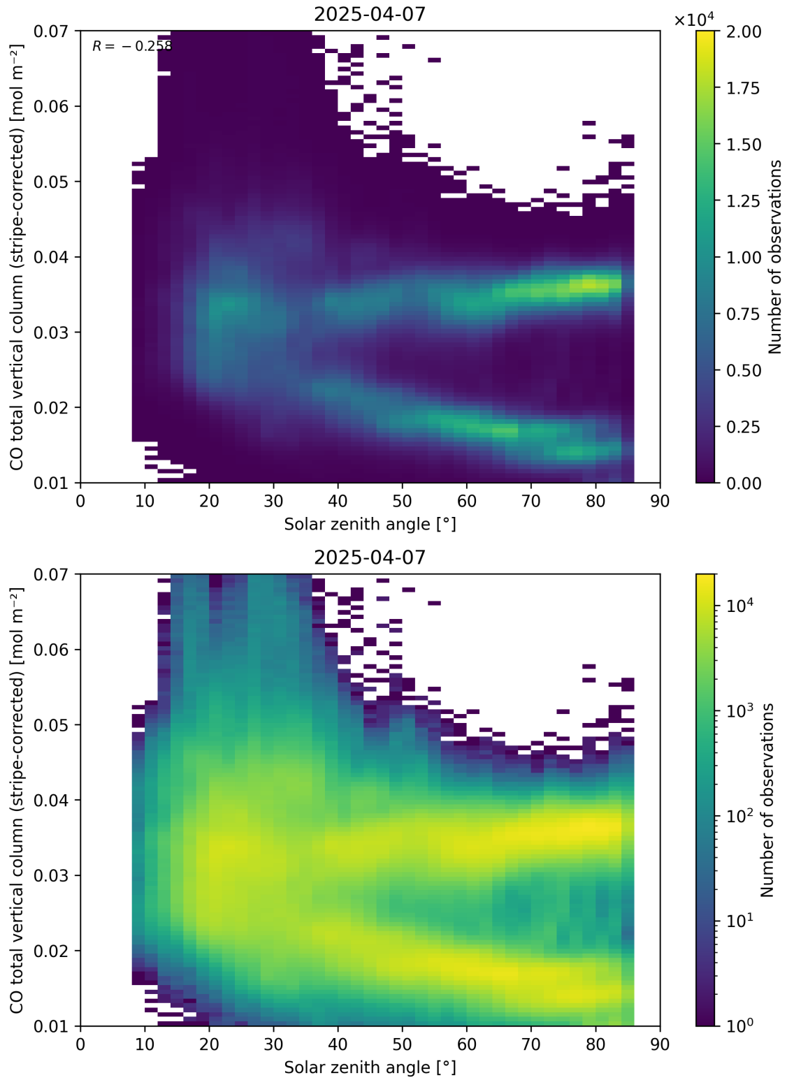
Figure 62: Scatter density plot of “Solar zenith angle” against “CO total vertical column (stripe-corrected)” for 2025-04-06 to 2025-04-08.
