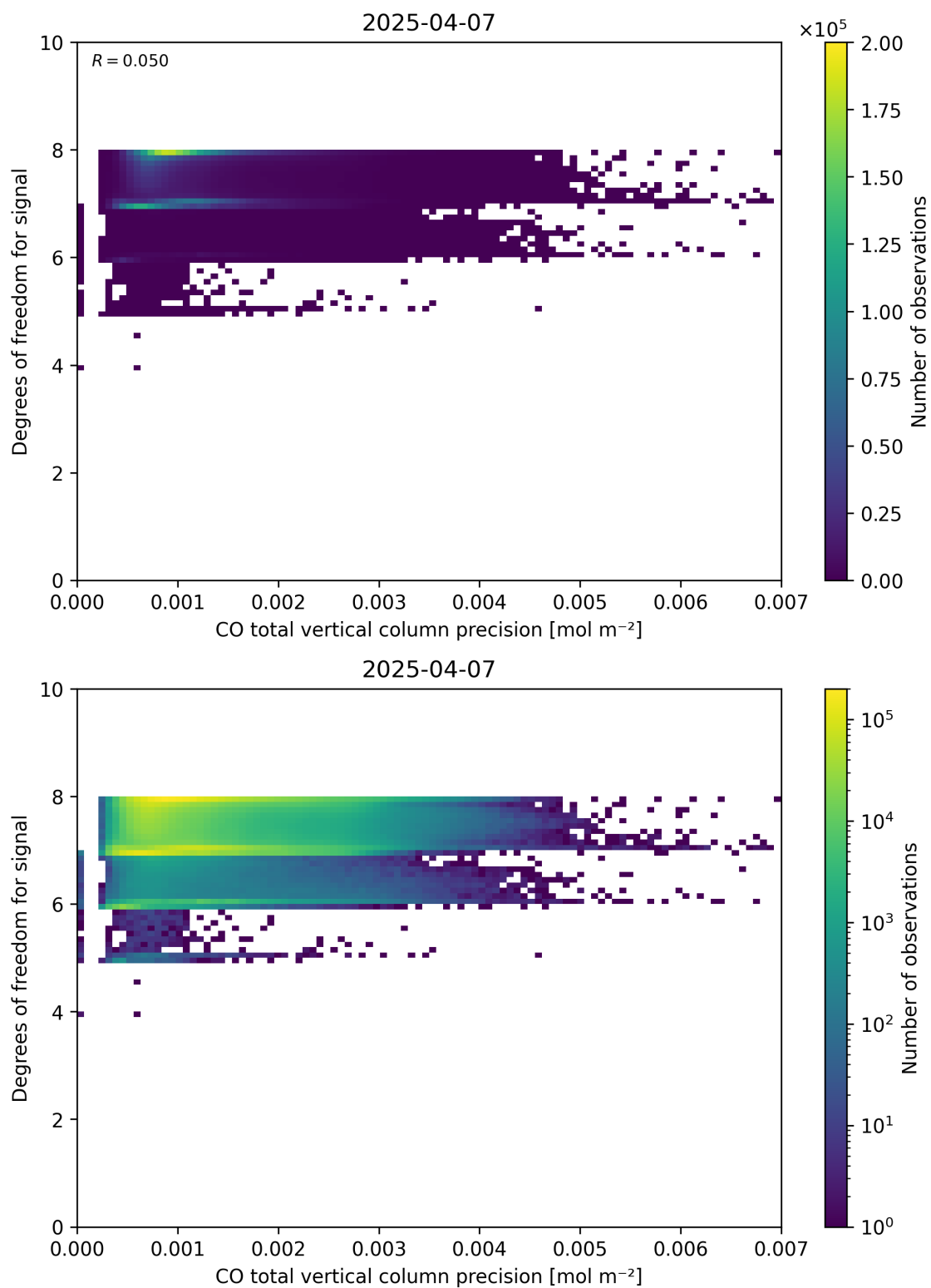
Figure 45: Scatter density plot of “CO total vertical column precision” against “Degrees of freedom for signal” for 2025-04-06 to 2025-04-08.
