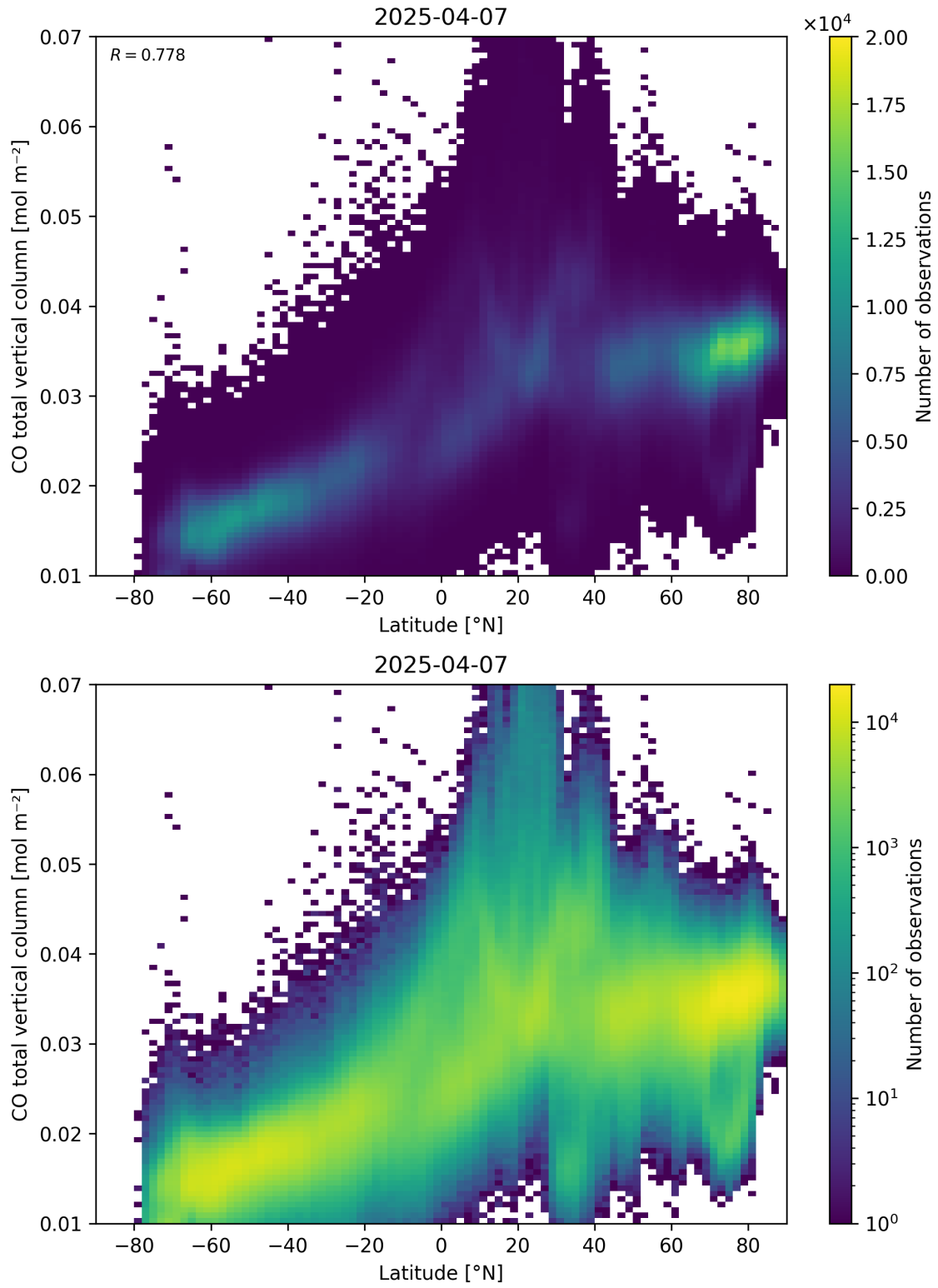
Figure 51: Scatter density plot of “Latitude” against “CO total vertical column” for 2025-04-06 to 2025-04-08.
