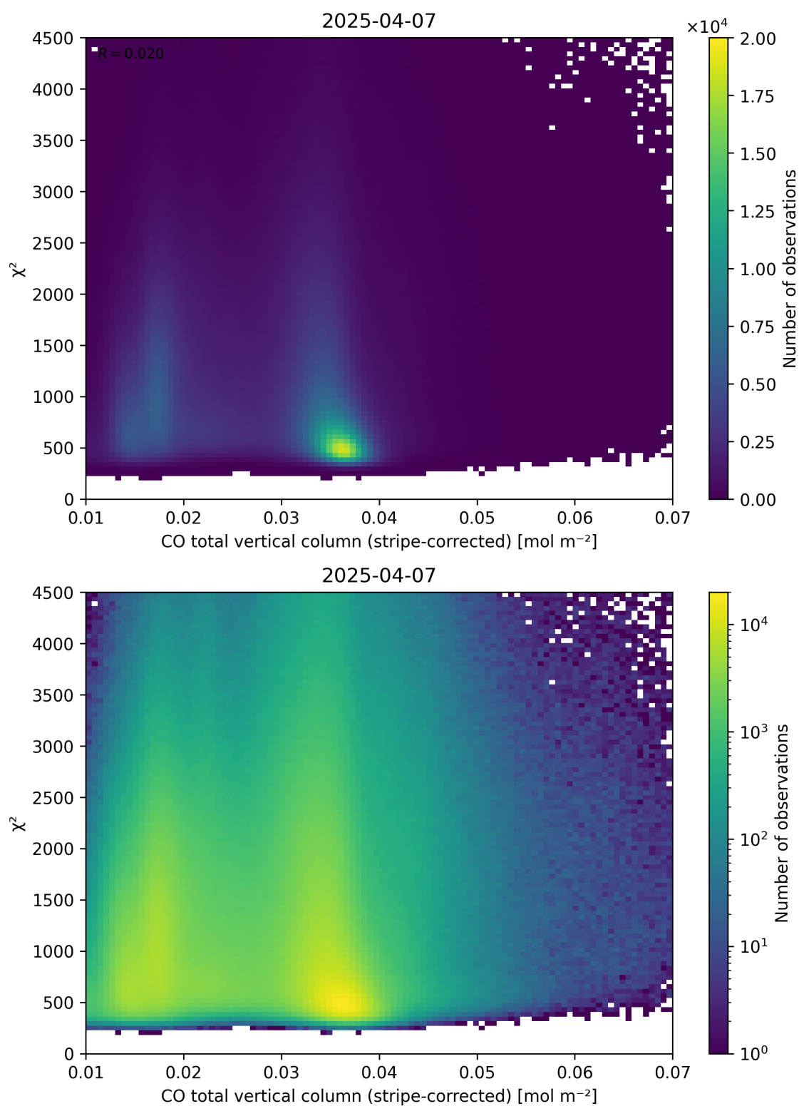
Figure 37: Scatter density plot of “CO total vertical column (stripe-corrected)” against “ \chi^2 ” for 2025-04-06 to 2025-04-08.
