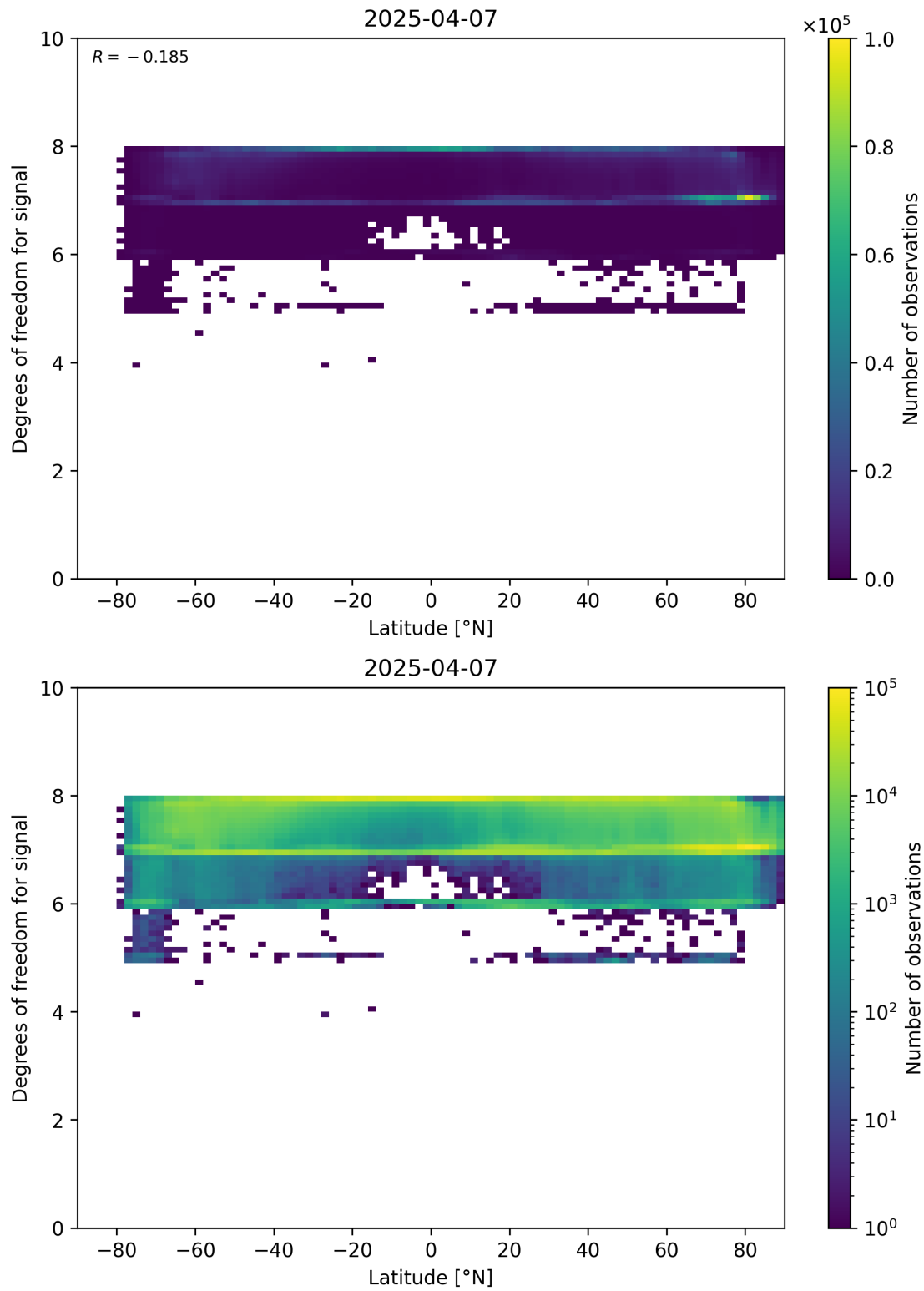
Figure 55: Scatter density plot of “Latitude” against “Degrees of freedom for signal” for 2025-04-06 to 2025-04-08.
