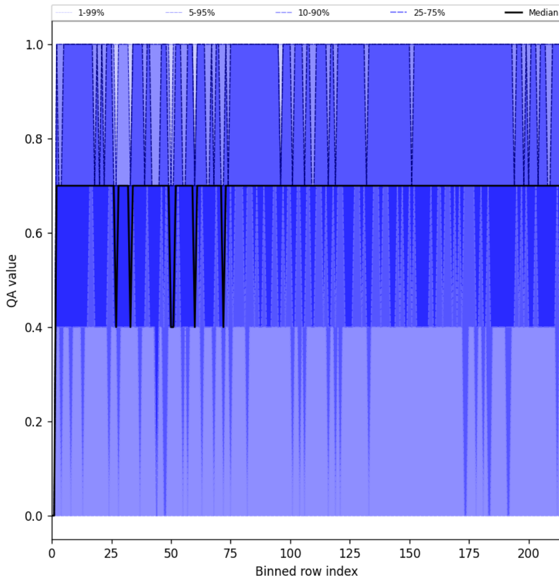
Figure 25: Along track statistics of “QA value” for 2025-04-06 to 2025-04-08
