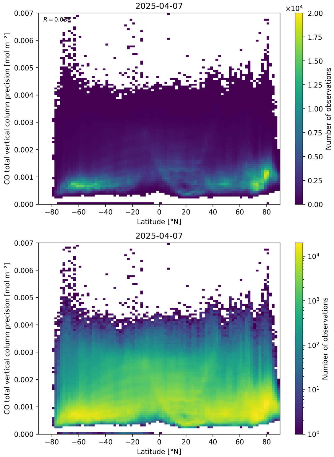
Figure 53: Scatter density plot of “Latitude” against “CO total vertical column precision” for 2025-04-06 to 2025-04-08.
