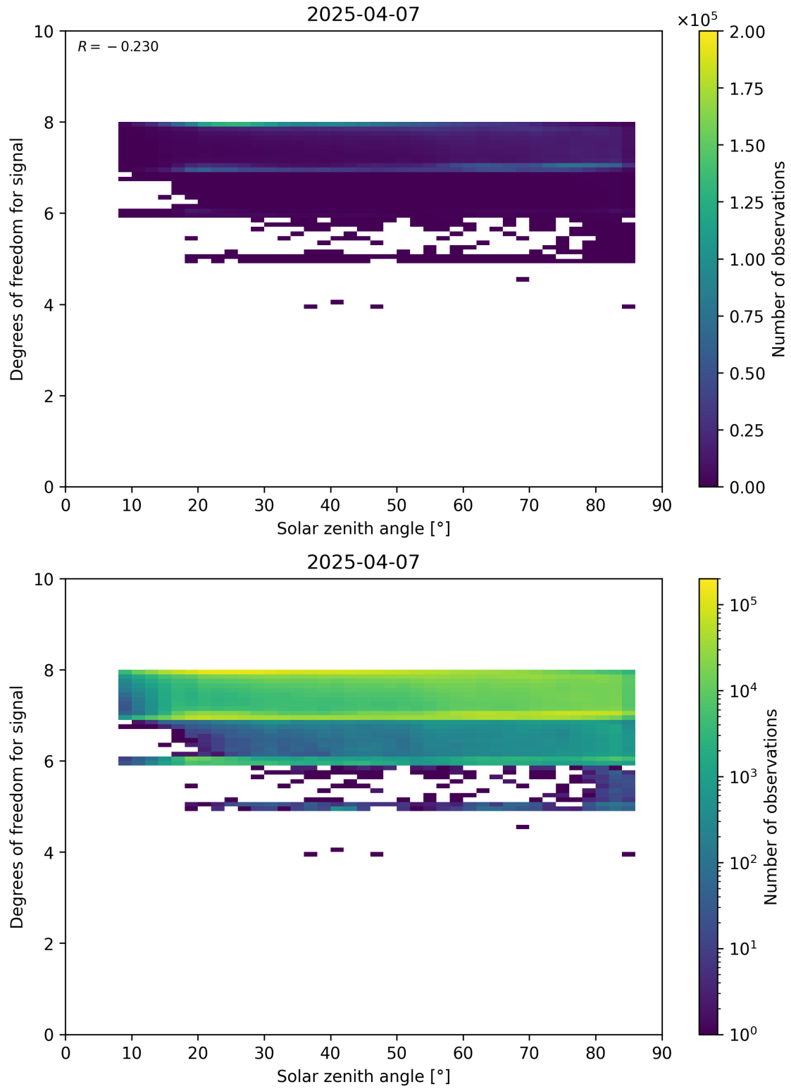
Figure 65: Scatter density plot of “Solar zenith angle” against “Degrees of freedom for signal” for 2025-04-06 to 2025-04-08.
