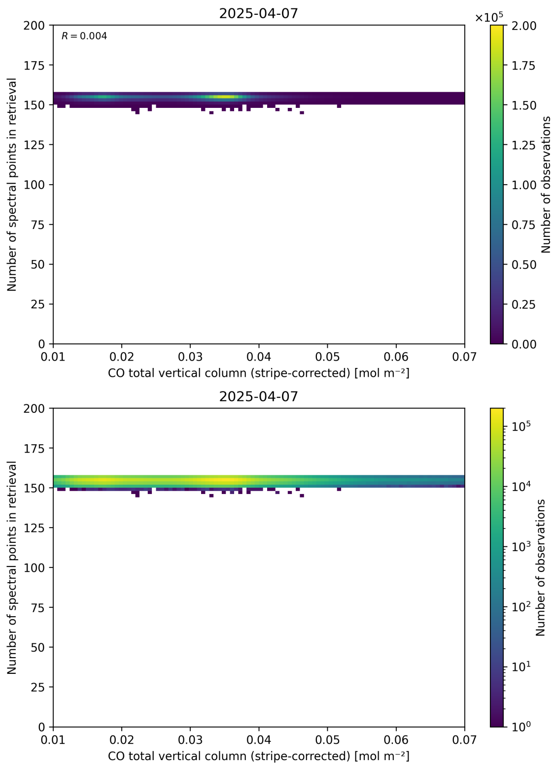
Figure 40: Scatter density plot of “CO total vertical column (stripe-corrected)” against “Number of spectral points in retrieval” for 2025-04-06 to 2025-04-08.
