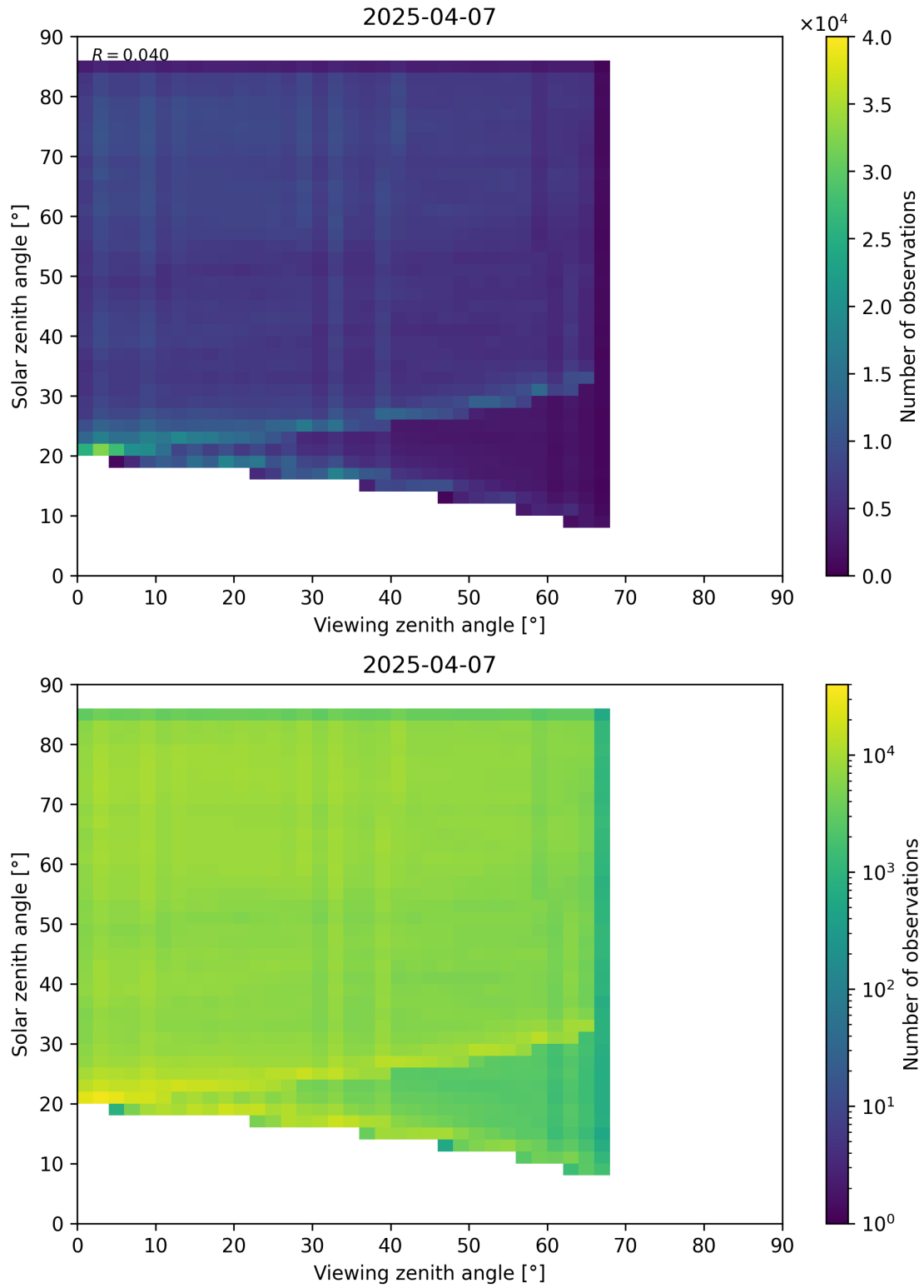
Figure 77: Scatter density plot of “Viewing zenith angle” against “Solar zenith angle” for 2025-04-06 to 2025-04-08.
