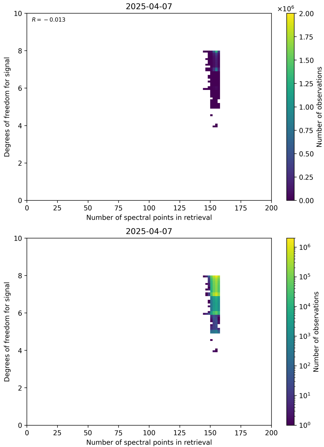
Figure 59: Scatter density plot of “Number of spectral points in retrieval” against “Degrees of freedom for signal” for 2025-04-06 to 2025-04-08.
