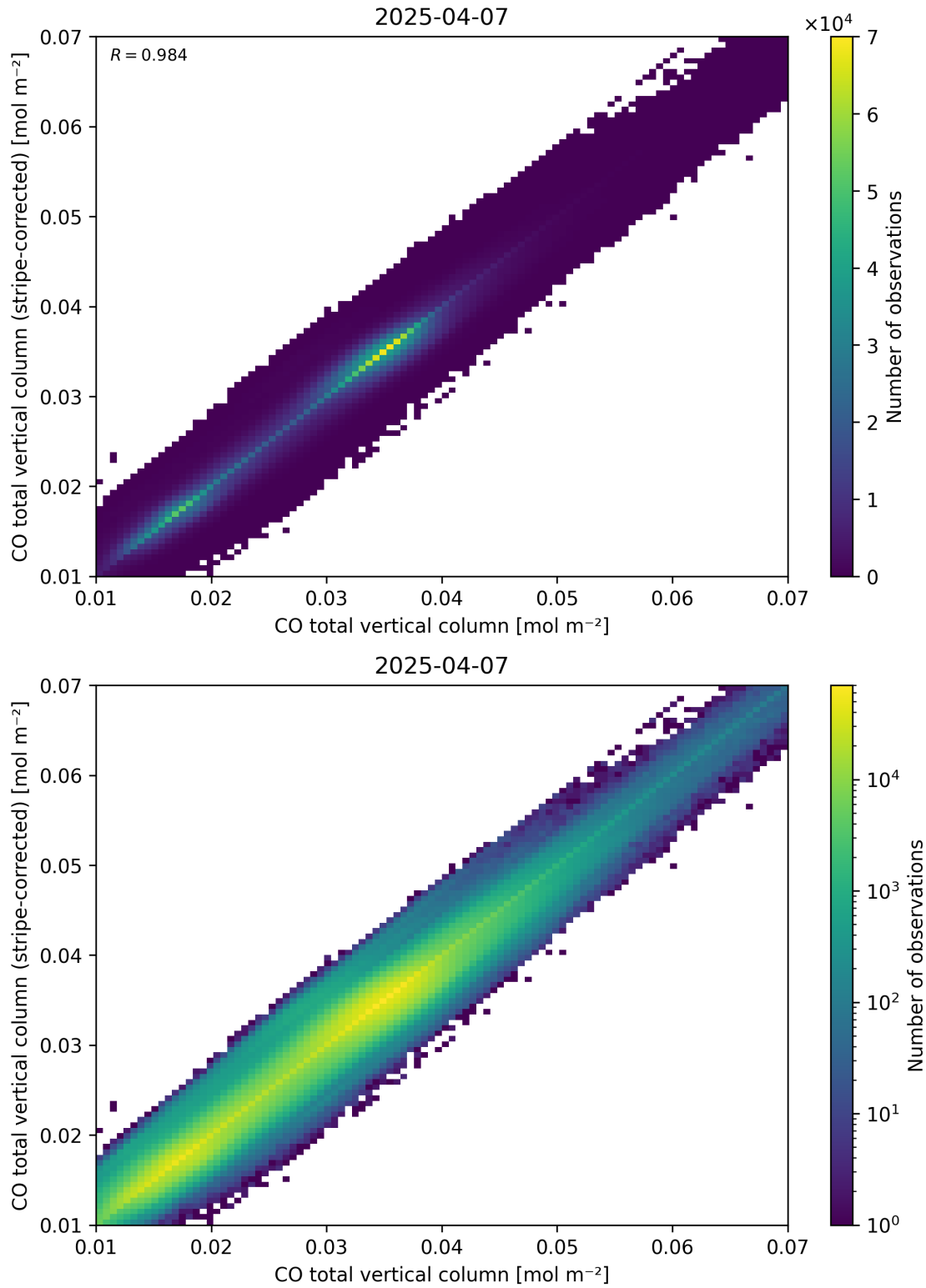
Figure 33: Scatter density plot of “CO total vertical column” against “CO total vertical column (stripe-corrected)” for 2025-04-06 to 2025-04-08.
