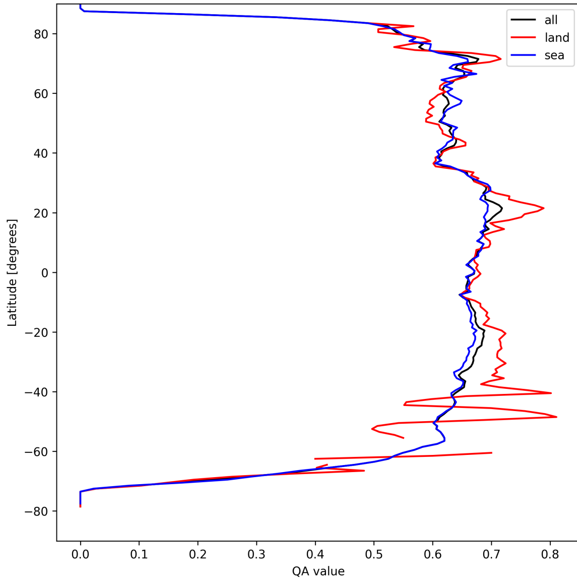
Figure 9: Zonal average of “QA value” for 2025-04-06 to 2025-04-08.
