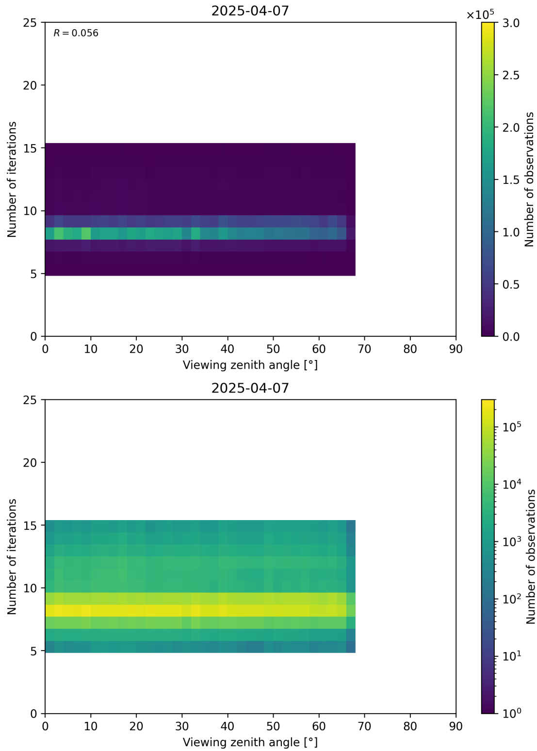
Figure 75: Scatter density plot of “Viewing zenith angle” against “Number of iterations” for 2025-04-06 to 2025-04-08.
