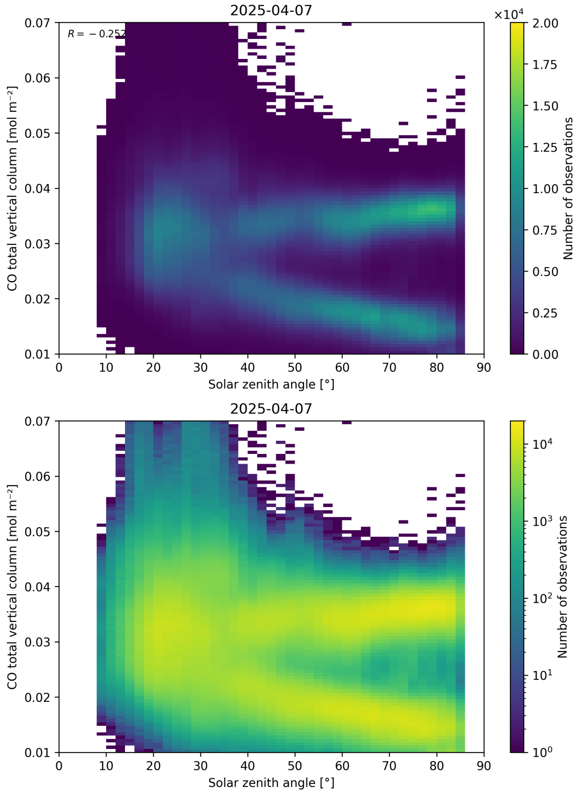
Figure 61: Scatter density plot of “Solar zenith angle” against “CO total vertical column” for 2025-04-06 to 2025-04-08.
