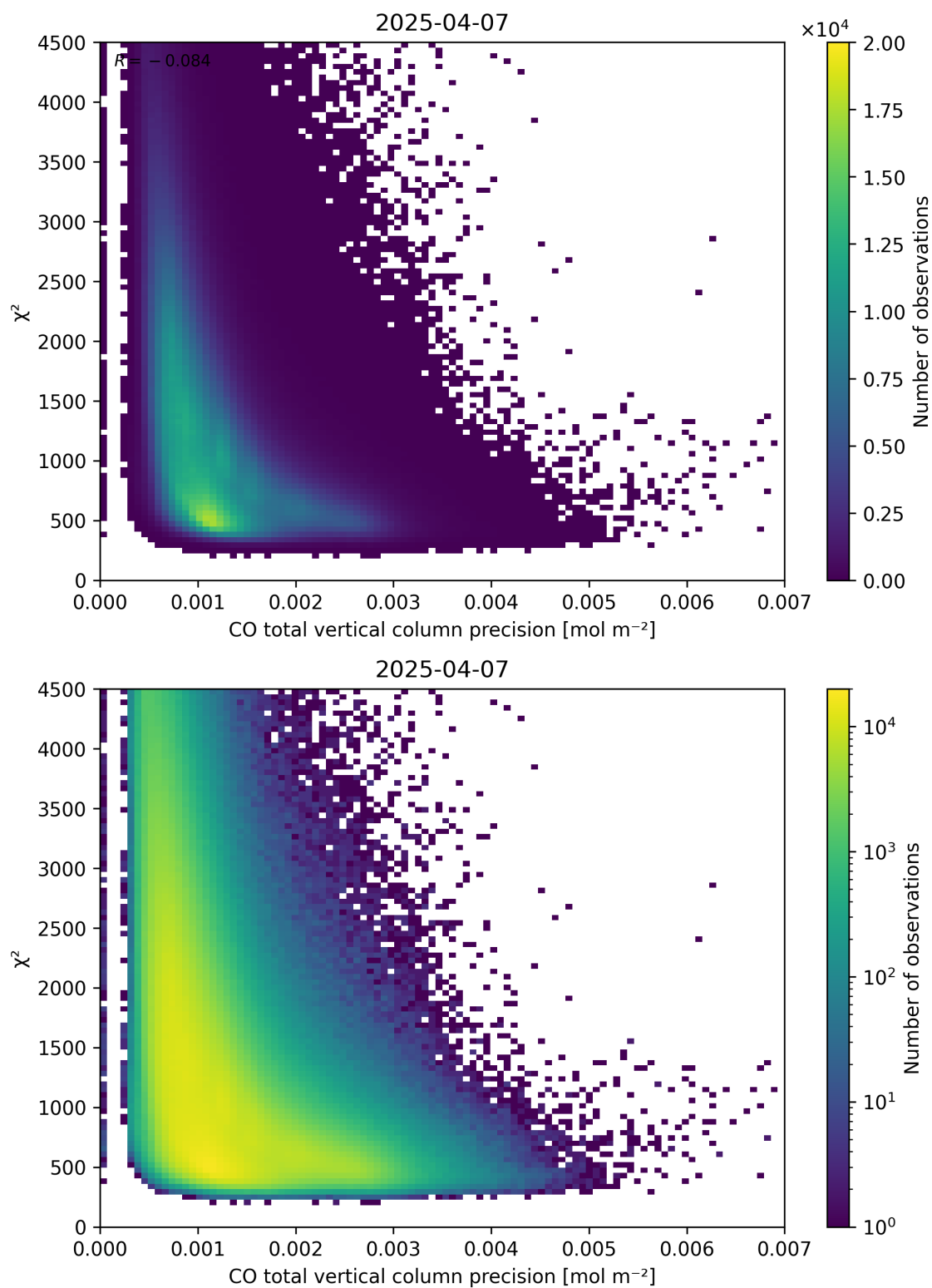
Figure 44: Scatter density plot of “CO total vertical column precision” against “ \chi^2 ” for 2025-04-06 to 2025-04-08.
