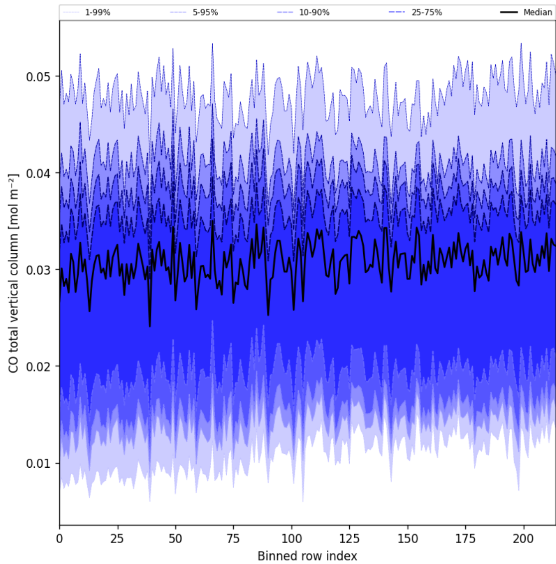
Figure 26: Along track statistics of “CO total vertical column” for 2025-04-06 to 2025-04-08
