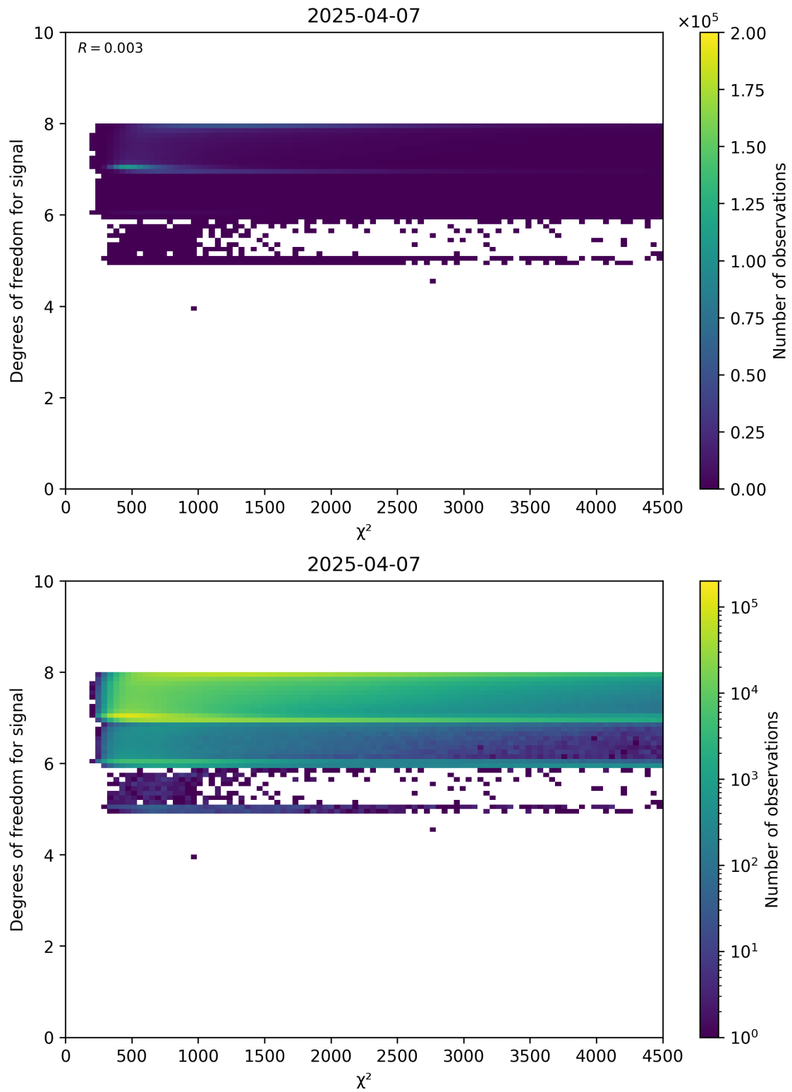
Figure 48: Scatter density plot of “ \chi^2 ” against “Degrees of freedom for signal” for 2025-04-06 to 2025-04-08.
