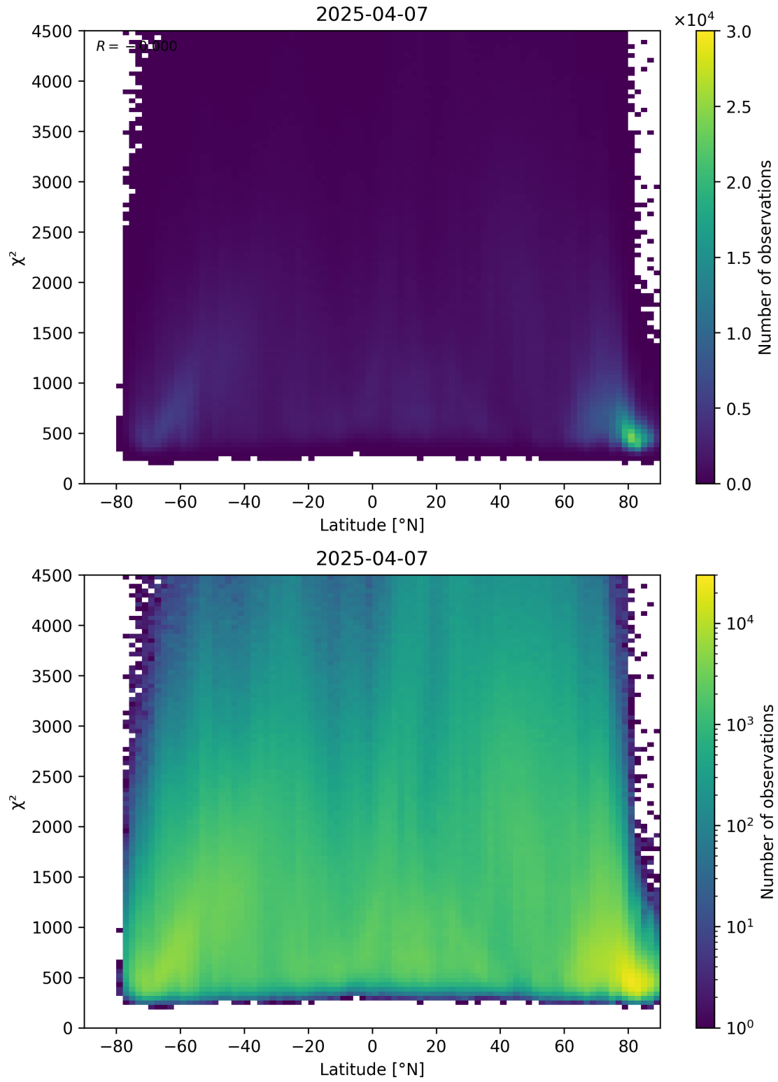
Figure 54: Scatter density plot of “Latitude” against “ \chi^2 ” for 2025-04-06 to 2025-04-08.
