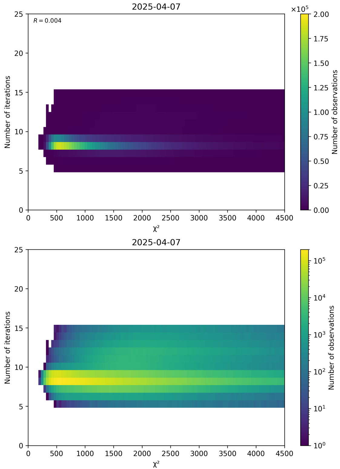
Figure 49: Scatter density plot of “ \chi^2 ” against “Number of iterations” for 2025-04-06 to 2025-04-08.
