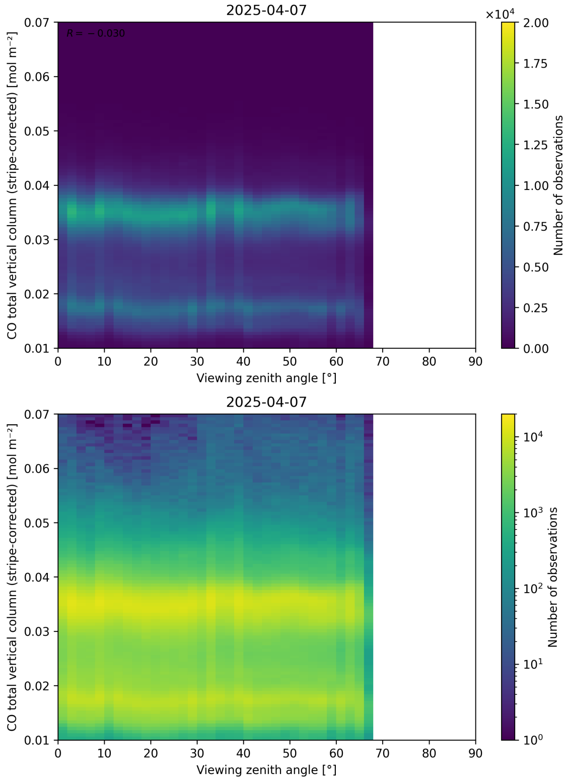
Figure 70: Scatter density plot of “Viewing zenith angle” against “CO total vertical column (stripe-corrected)” for 2025-04-06 to 2025-04-08.
