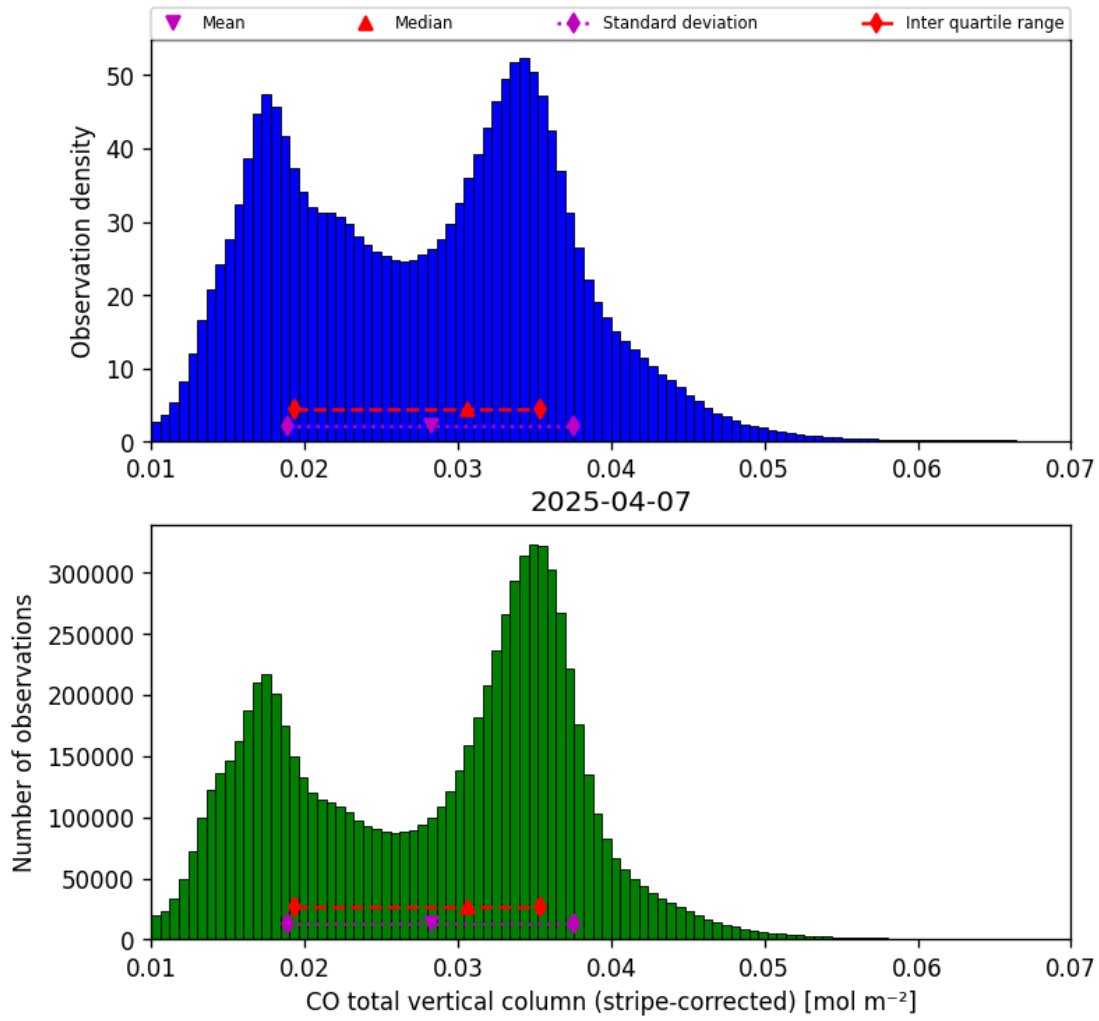
Figure 19: Histogram of “CO total vertical column (stripe-corrected)” for 2025-04-06 to 2025-04-08
