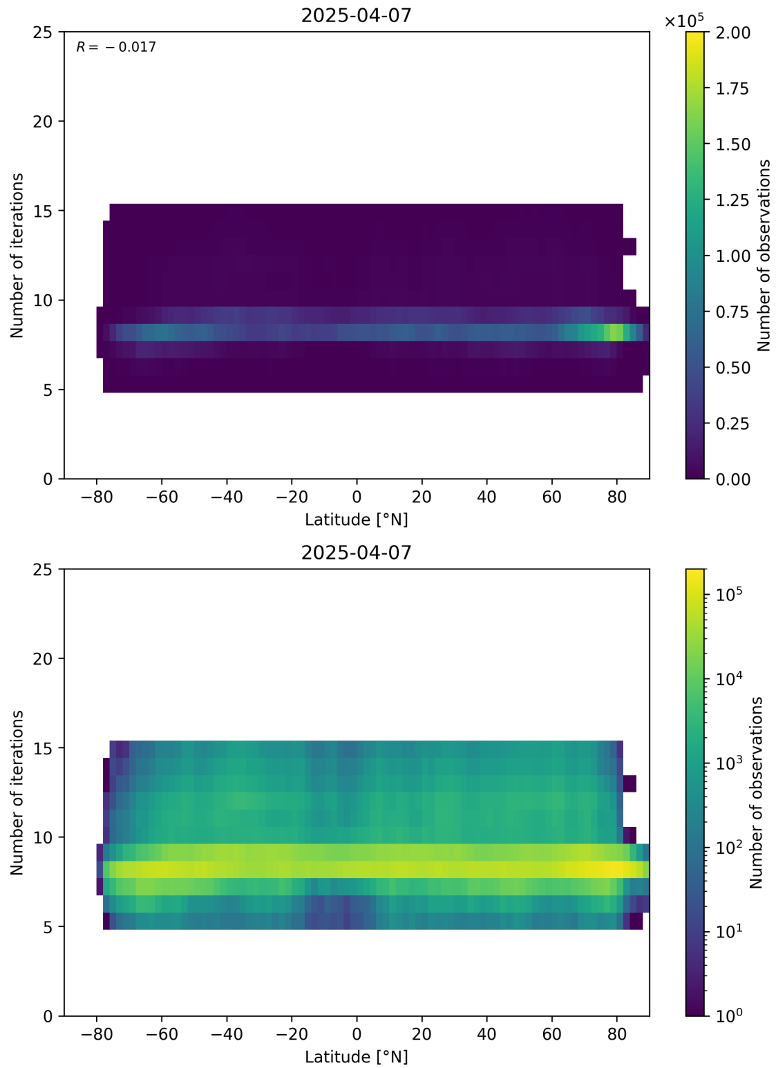
Figure 56: Scatter density plot of “Latitude” against “Number of iterations” for 2025-04-06 to 2025-04-08.
