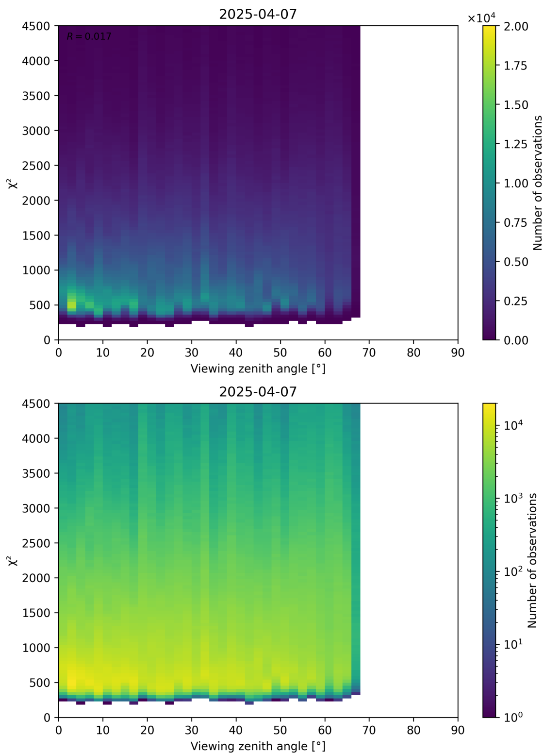
Figure 72: Scatter density plot of “Viewing zenith angle” against “ \chi^2 ” for 2025-04-06 to 2025-04-08.
