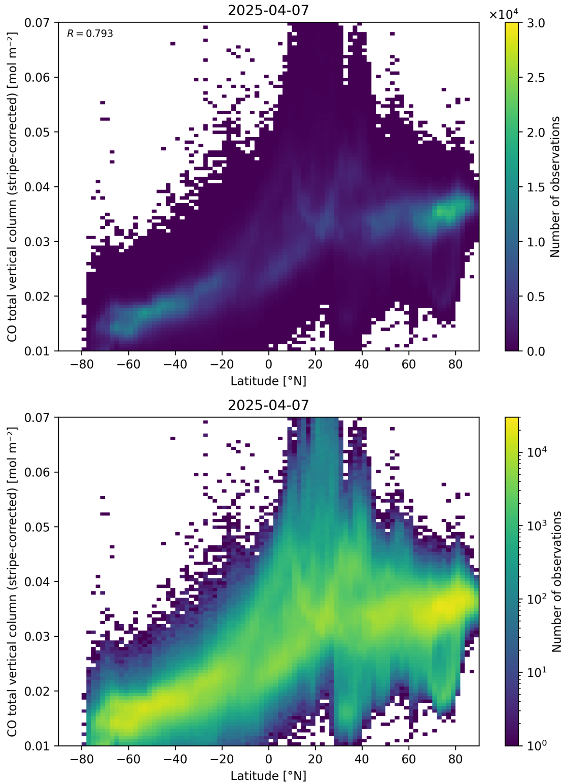
Figure 52: Scatter density plot of “Latitude” against “CO total vertical column (stripe-corrected)” for 2025-04-06 to 2025-04-08.
