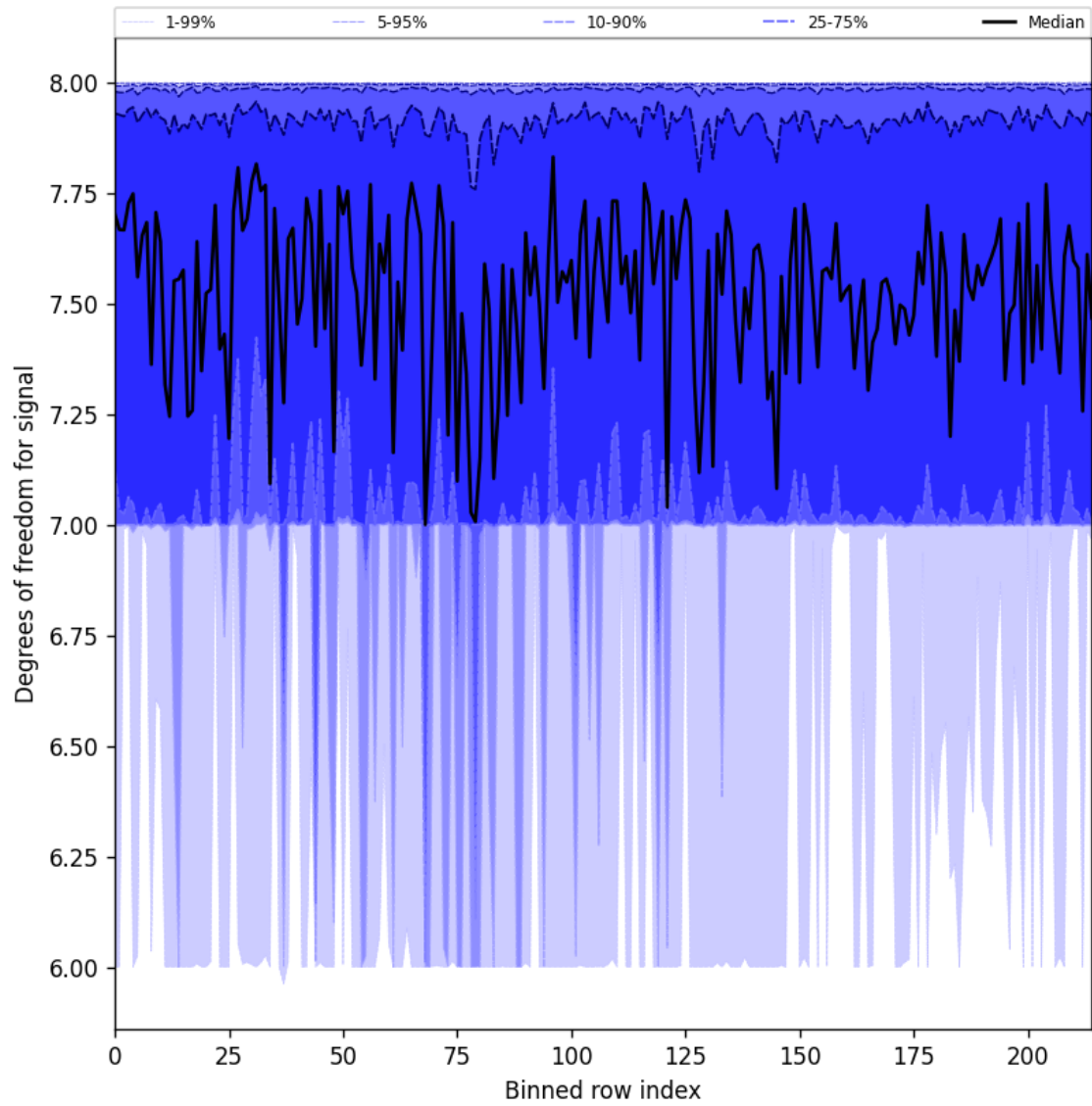
Figure 31: Along track statistics of “Degrees of freedom for signal” for 2025-04-06 to 2025-04-08
