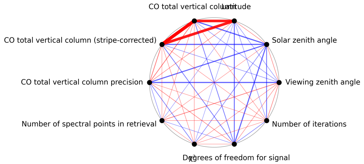
Figure 1: Map of correlation graph for 2025-04-06 to 2025-04-08.
