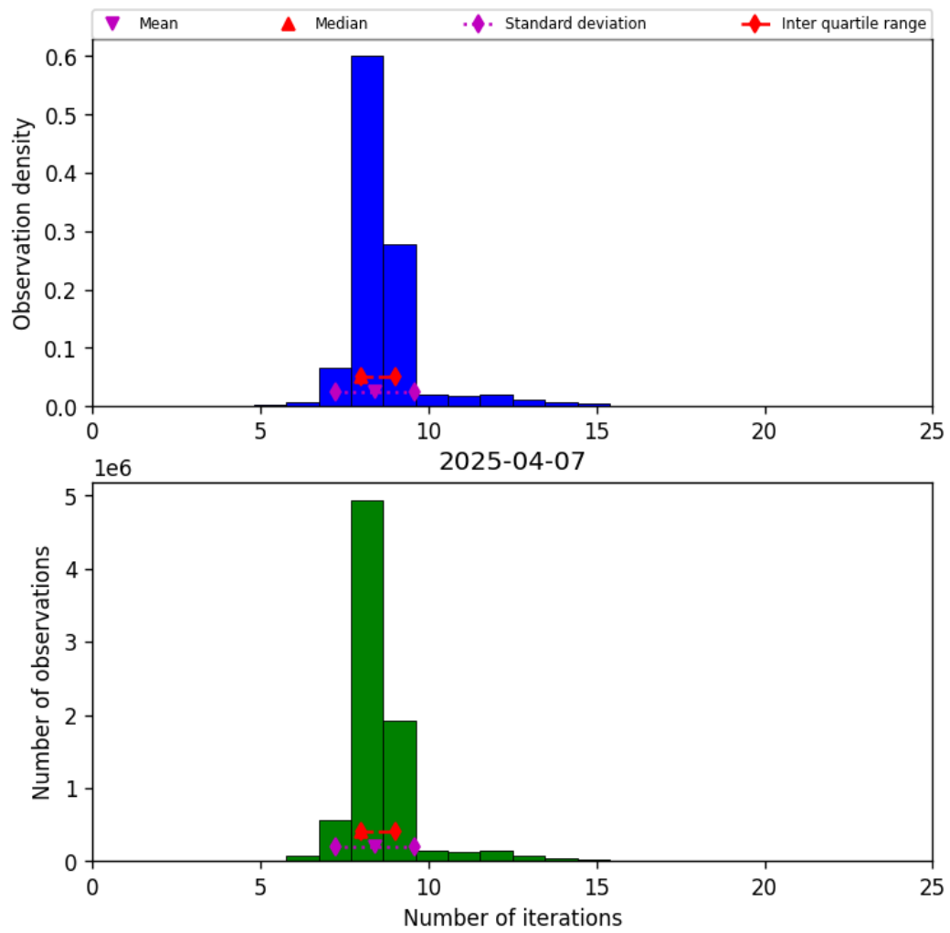
Figure 24: Histogram of “Number of iterations” for 2025-04-06 to 2025-04-08
