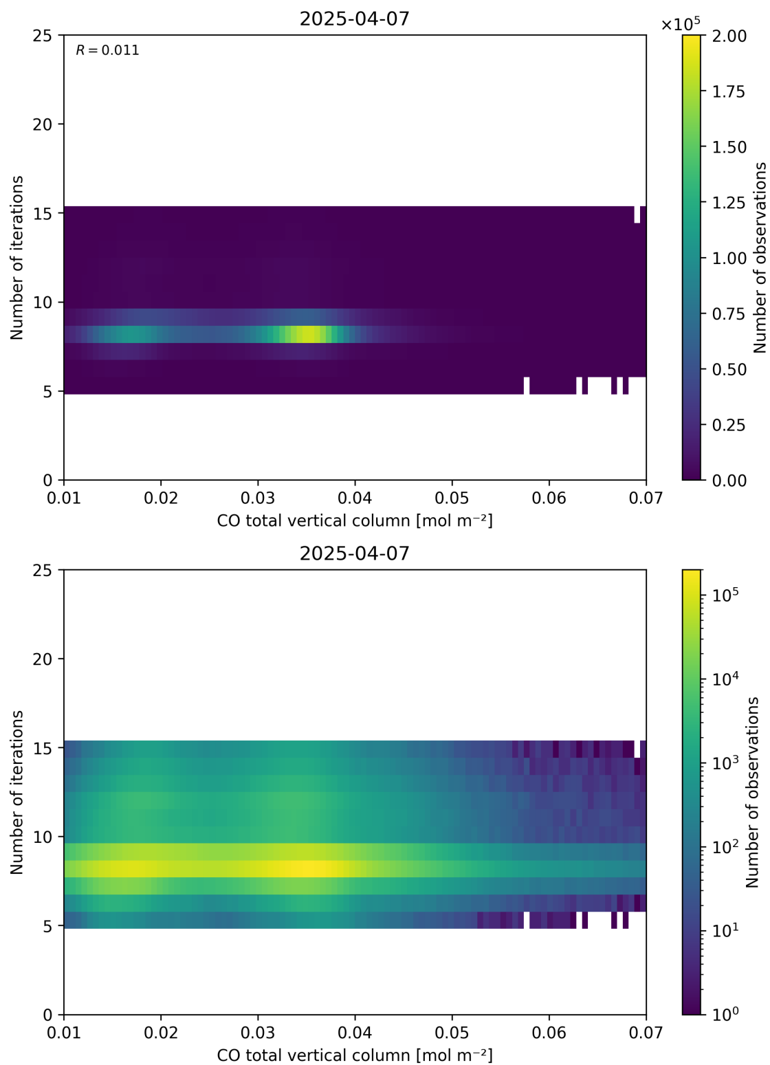
Figure 42: Scatter density plot of “CO total vertical column” against “Number of iterations” for 2025-04-06 to 2025-04-08.
