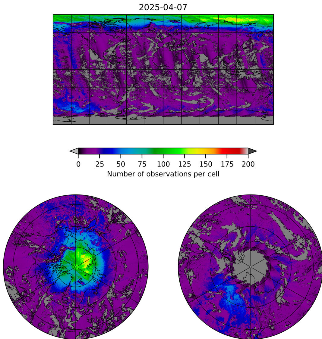
Figure 8: Map of the number of observations for 2025-04-06 to 2025-04-08
