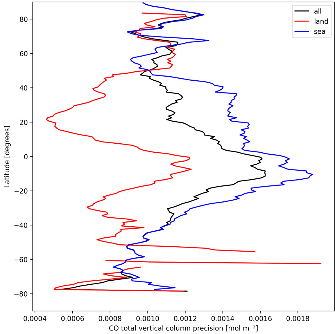
Figure 12: Zonal average of “CO total vertical column precision” for 2025-04-06 to 2025-04-08.
