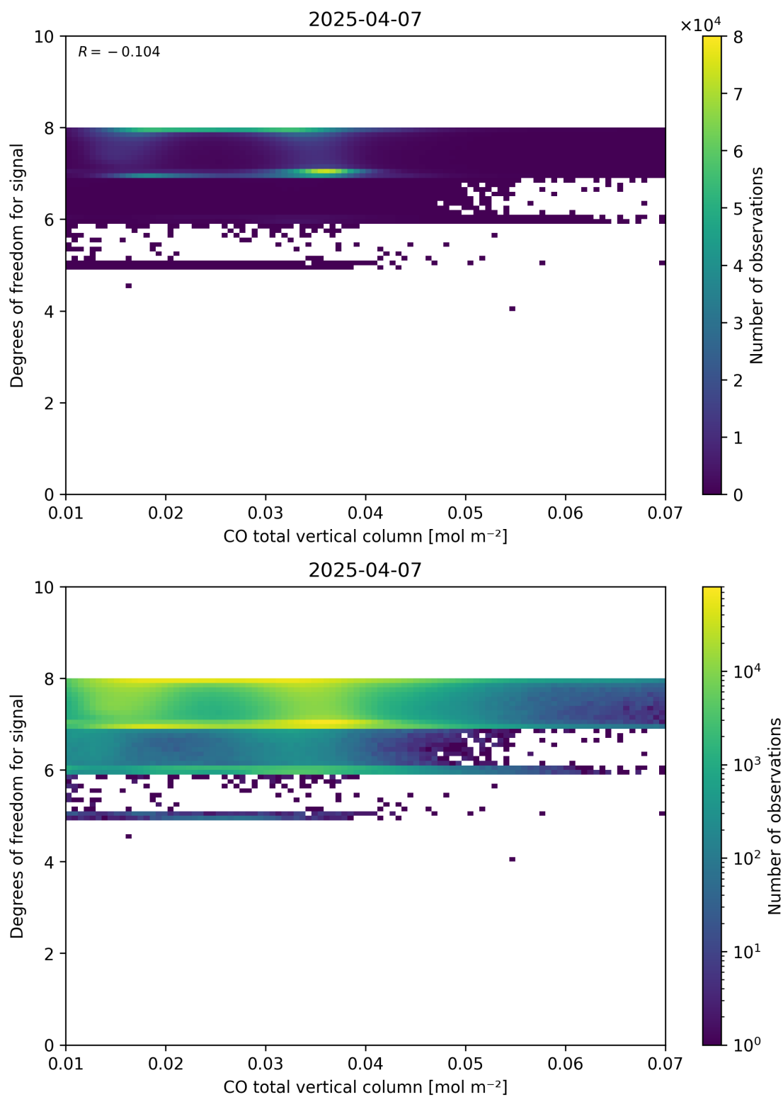
Figure 41: Scatter density plot of “CO total vertical column” against “Degrees of freedom for signal” for 2025-04-06 to 2025-04-08.
