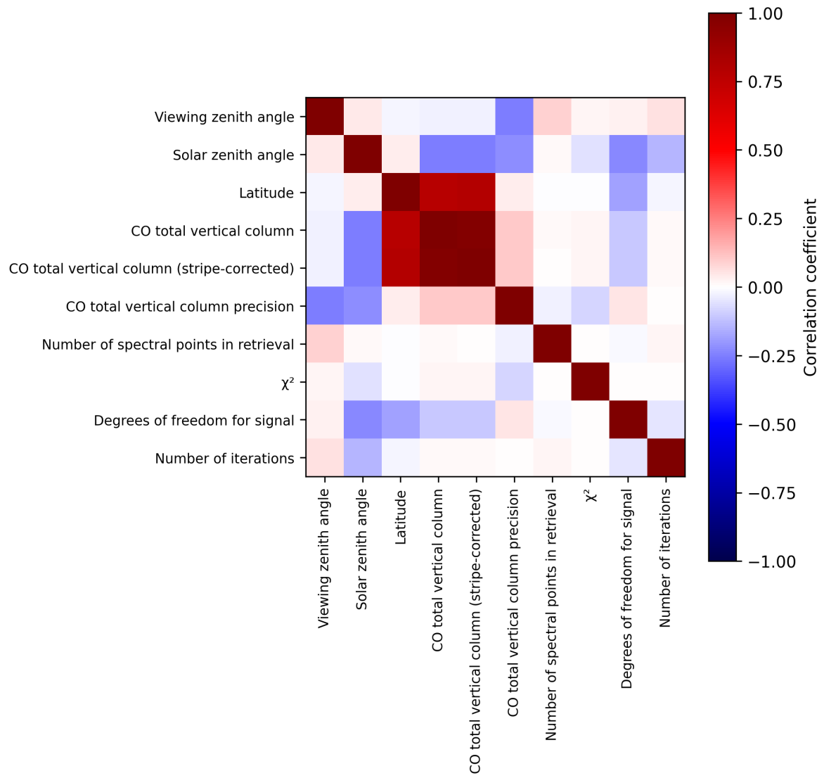
Figure 2: Map of correlation matrix for 2025-04-06 to 2025-04-08.
