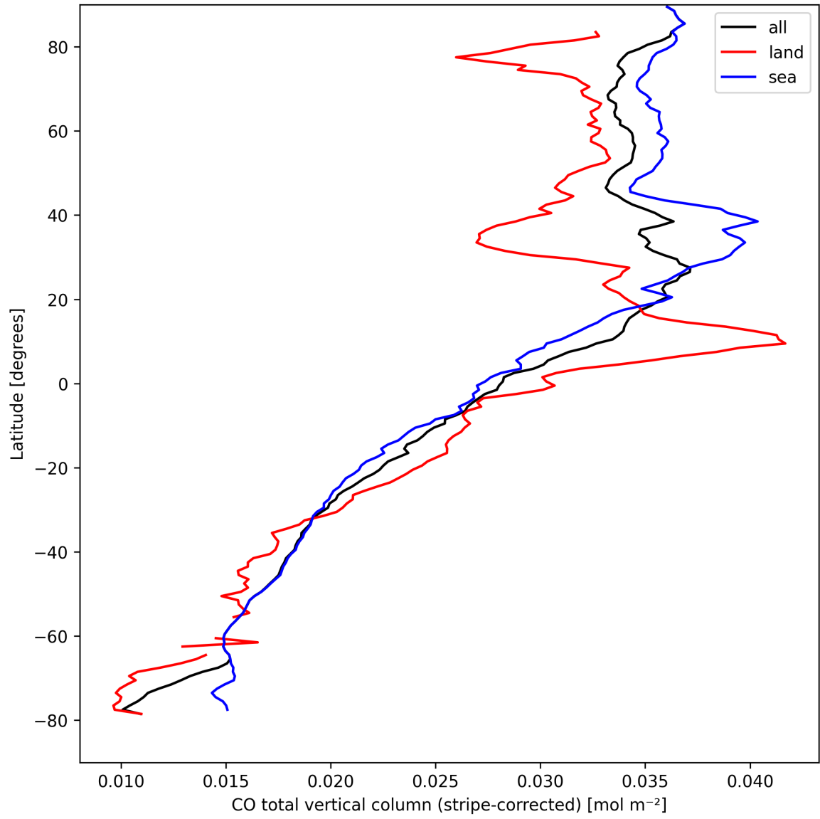
Figure 11: Zonal average of “CO total vertical column (stripe-corrected)” for 2025-04-06 to 2025-04-08.
