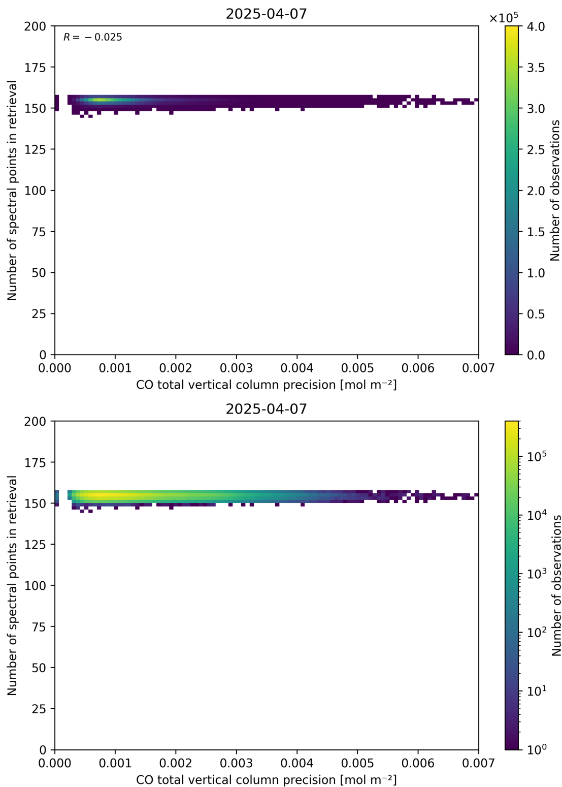
Figure 47: Scatter density plot of “CO total vertical column precision” against “Number of spectral points in retrieval” for 2025-04-06 to 2025-04-08.
