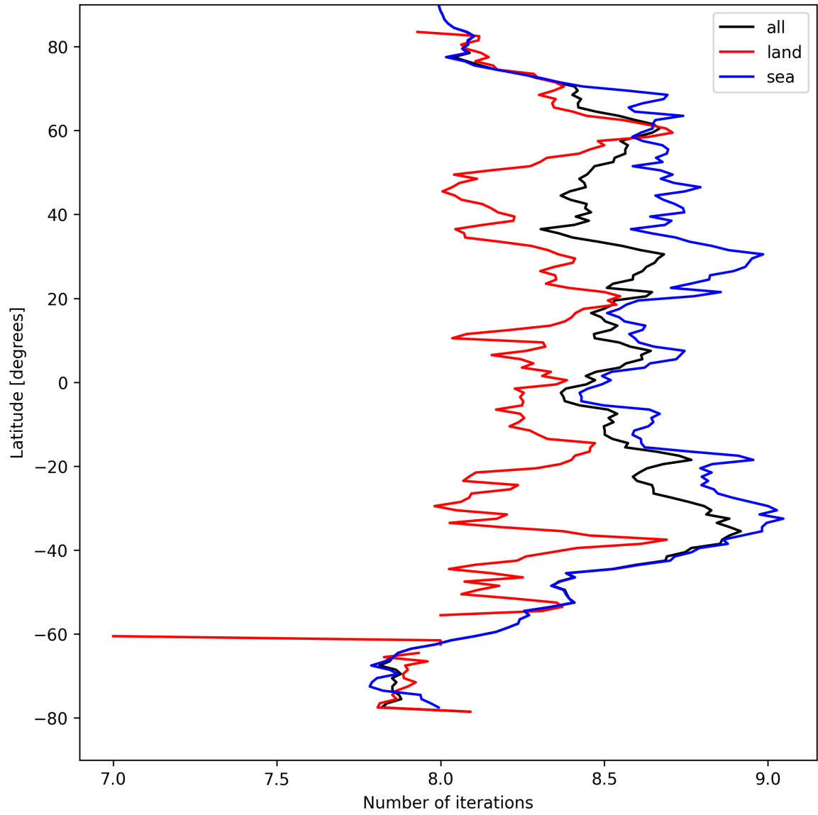
Figure 16: Zonal average of “Number of iterations” for 2025-04-06 to 2025-04-08.
