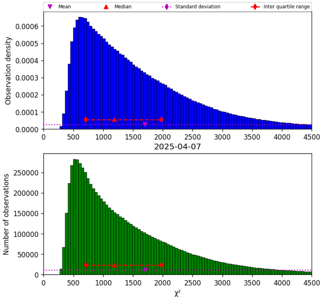
Figure 22: Histogram of “ \chi^2 ” for 2025-04-06 to 2025-04-08
