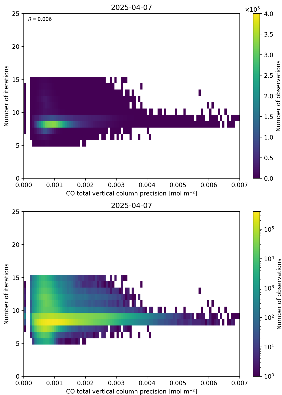
Figure 46: Scatter density plot of “CO total vertical column precision” against “Number of iterations” for 2025-04-06 to 2025-04-08.
