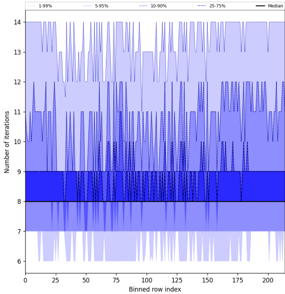
Figure 32: Along track statistics of “Number of iterations” for 2025-04-06 to 2025-04-08
