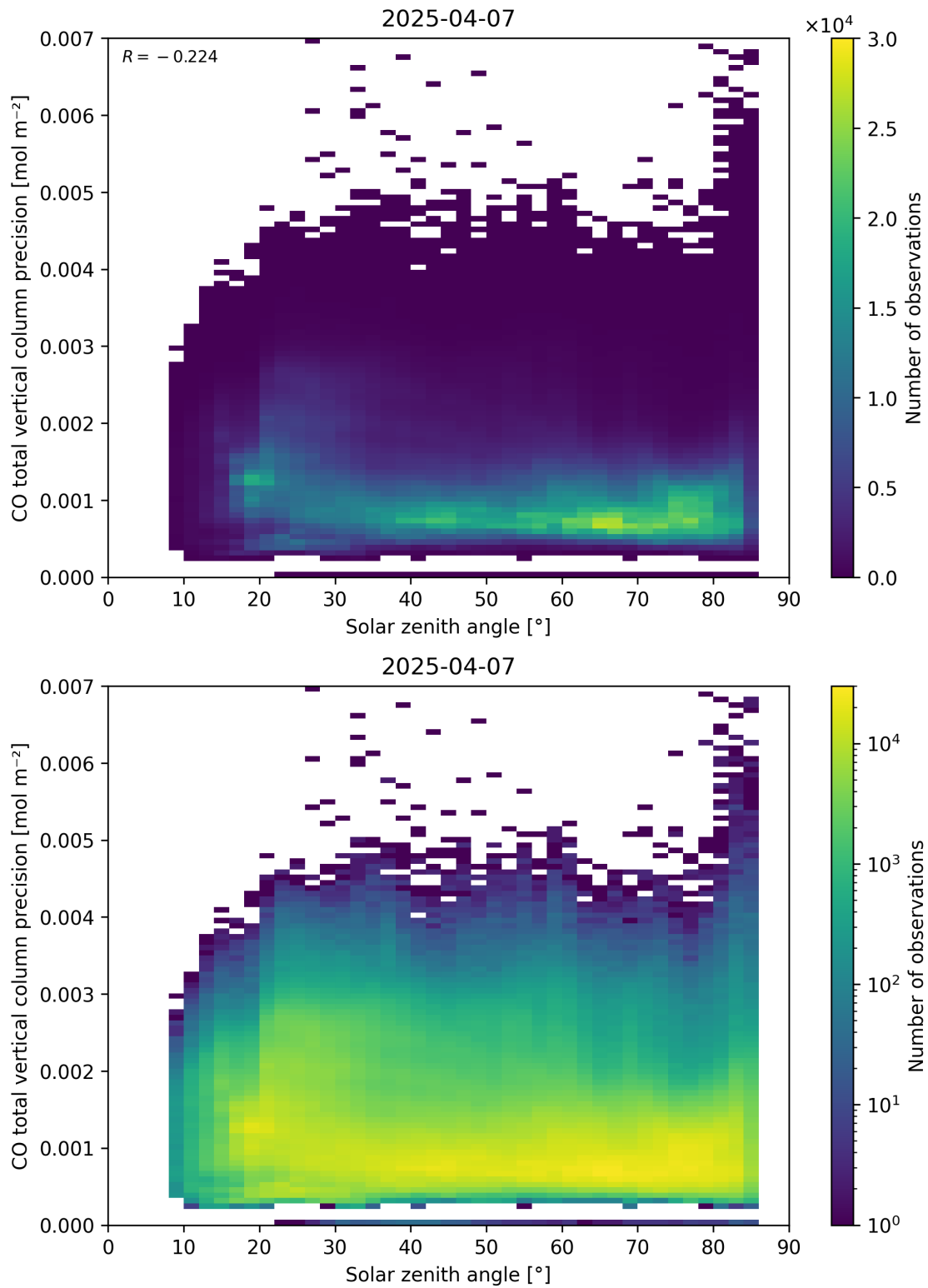
Figure 63: Scatter density plot of “Solar zenith angle” against “CO total vertical column precision” for 2025-04-06 to 2025-04-08.
