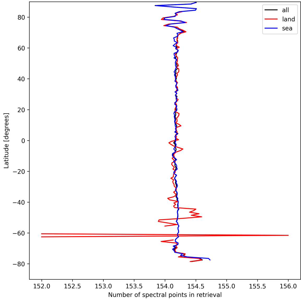
Figure 13: Zonal average of “Number of spectral points in retrieval” for 2025-04-06 to 2025-04-08.
