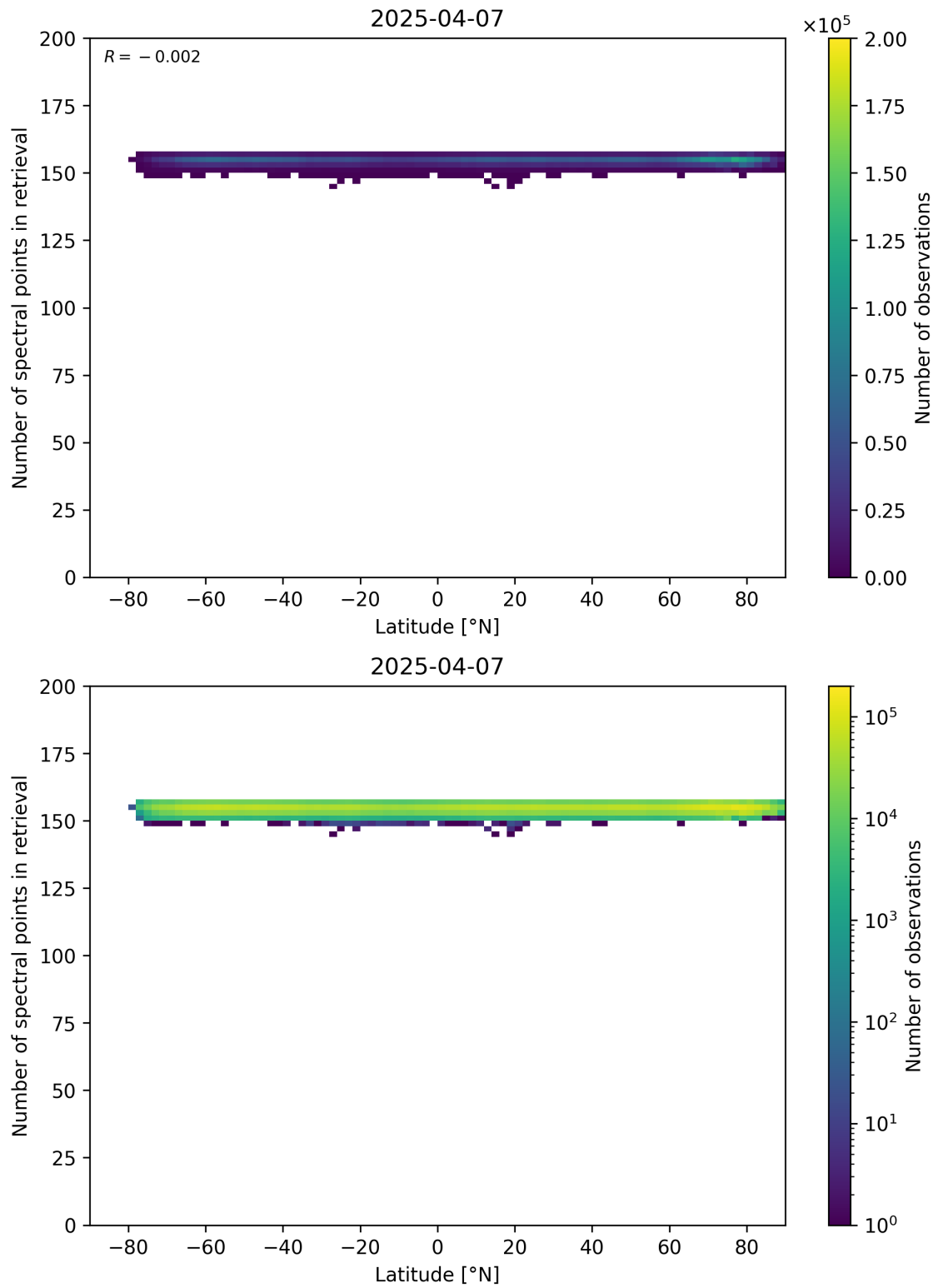
Figure 57: Scatter density plot of “Latitude” against “Number of spectral points in retrieval” for 2025-04-06 to 2025-04-08.
