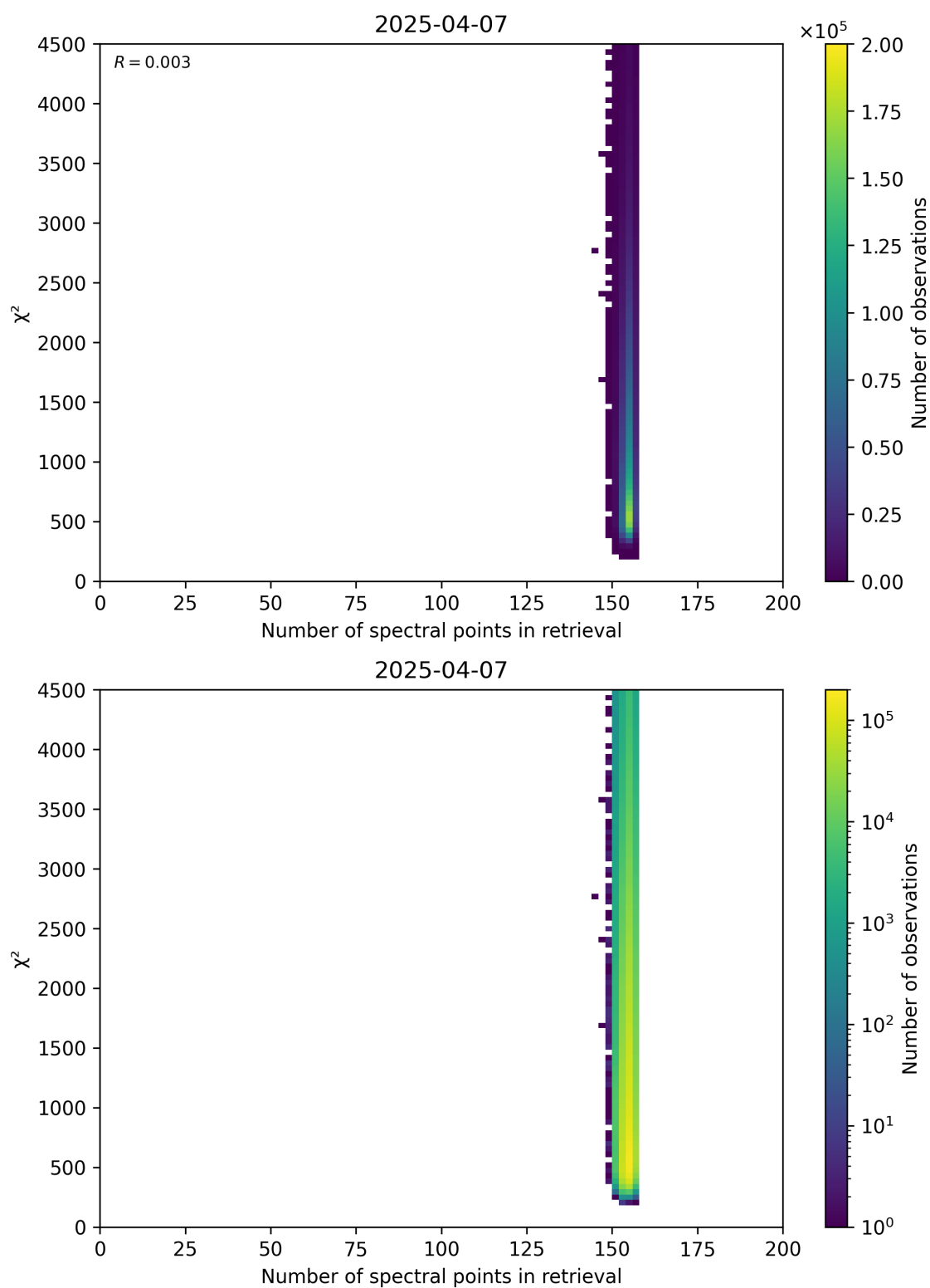
Figure 58: Scatter density plot of “Number of spectral points in retrieval” against “ \chi^2 ” for 2025-04-06 to 2025-04-08.
