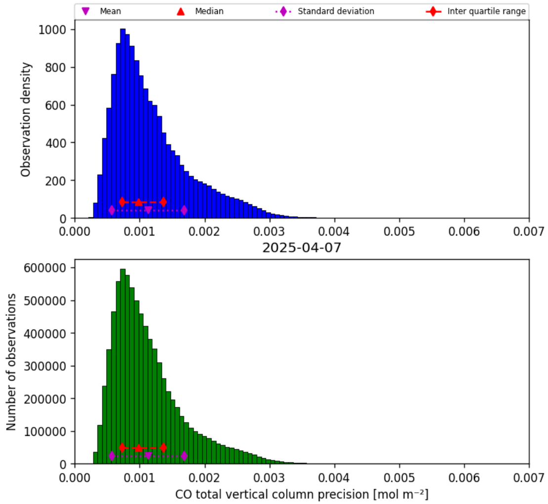
Figure 20: Histogram of “CO total vertical column precision” for 2025-04-06 to 2025-04-08
