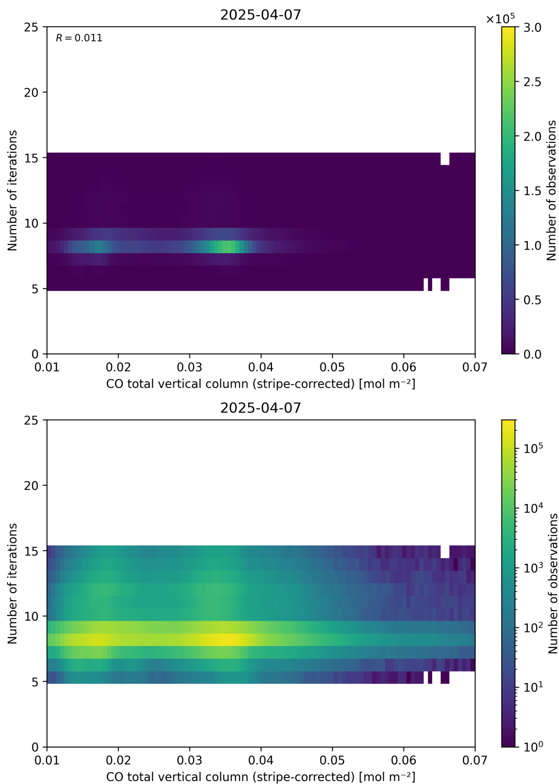
Figure 39: Scatter density plot of “CO total vertical column (stripe-corrected)” against “Number of iterations” for 2025-04-06 to 2025-04-08.
