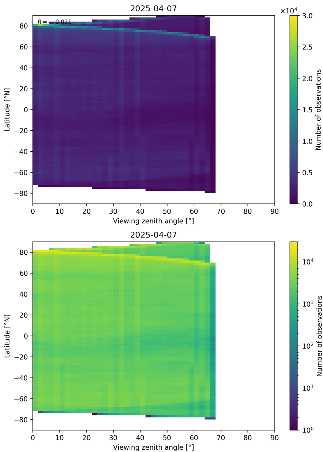
Figure 74: Scatter density plot of “Viewing zenith angle” against “Latitude” for 2025-04-06 to 2025-04-08.
