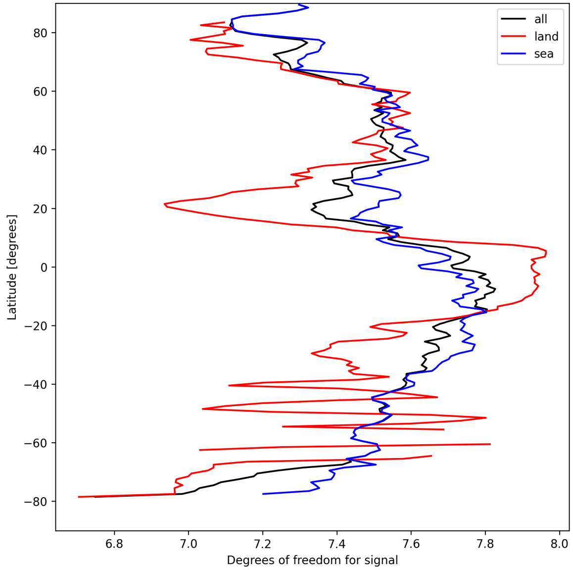
Figure 15: Zonal average of “Degrees of freedom for signal” for 2025-04-06 to 2025-04-08.
