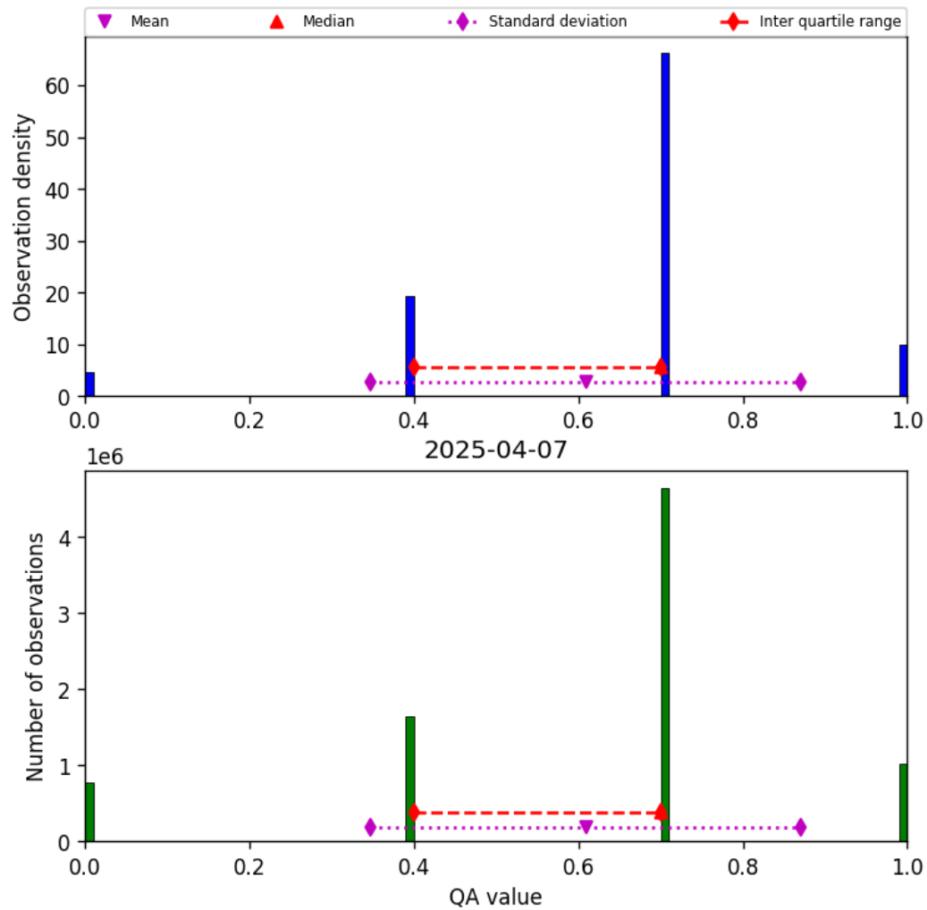
Figure 17: Histogram of “QA value” for 2025-04-06 to 2025-04-08
