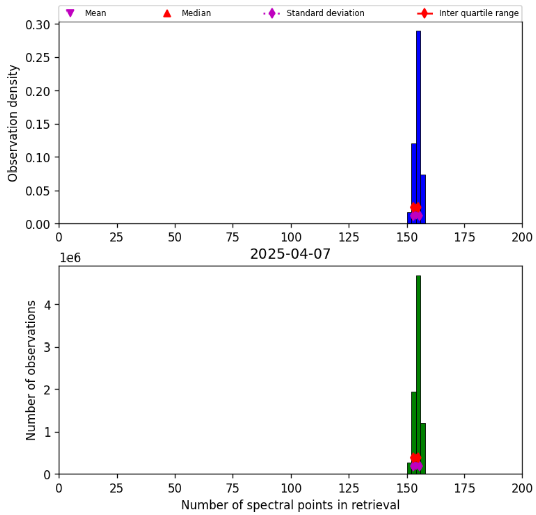
Figure 21: Histogram of “Number of spectral points in retrieval” for 2025-04-06 to 2025-04-08
