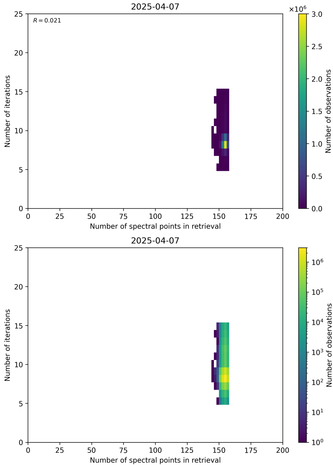
Figure 60: Scatter density plot of “Number of spectral points in retrieval” against “Number of iterations” for 2025-04-06 to 2025-04-08.
