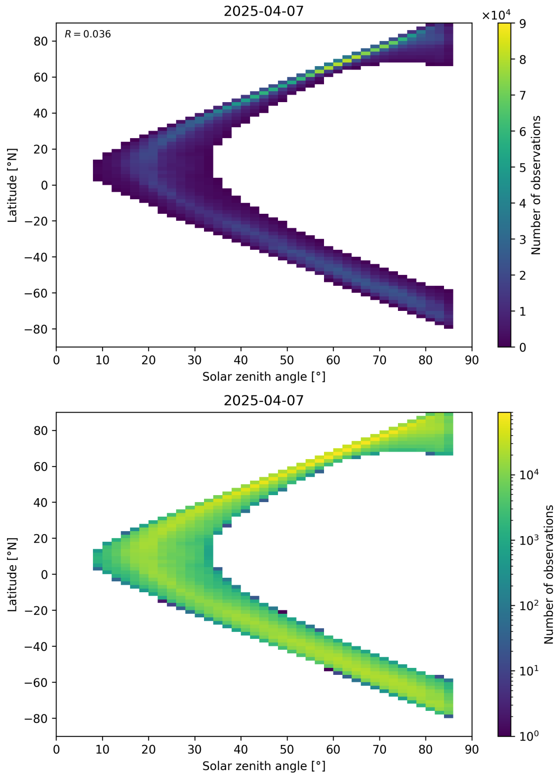
Figure 66: Scatter density plot of “Solar zenith angle” against “Latitude” for 2025-04-06 to 2025-04-08.
