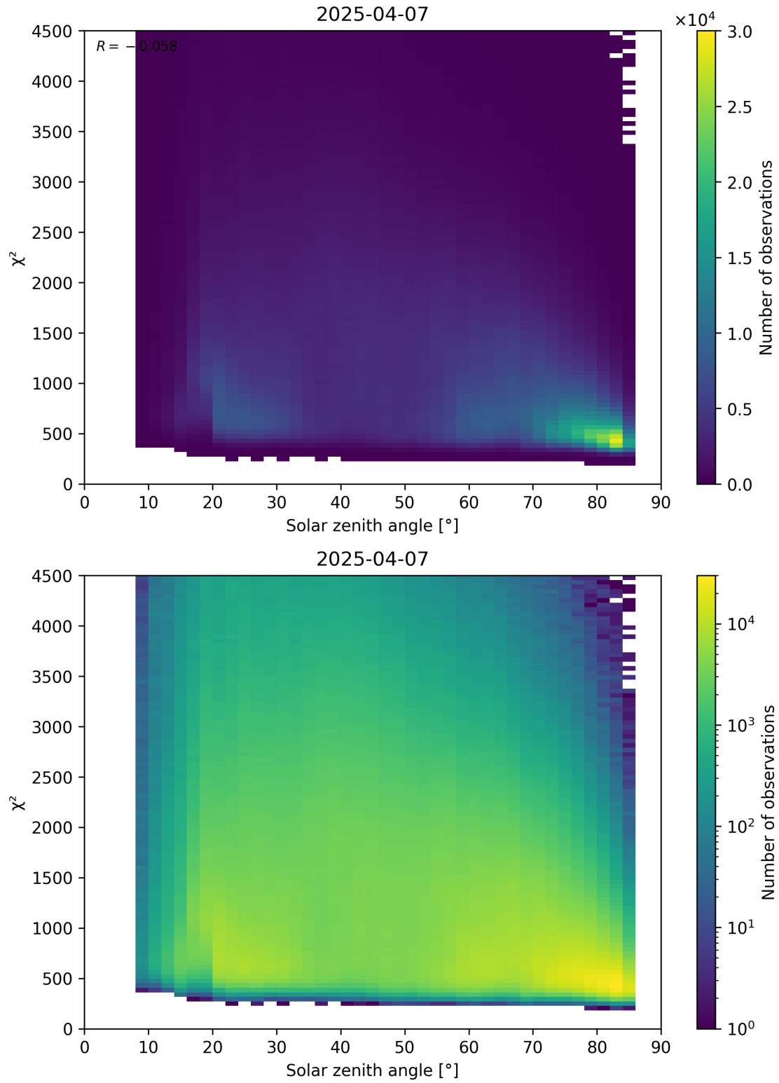
Figure 64: Scatter density plot of “Solar zenith angle” against “ \chi^2 ” for 2025-04-06 to 2025-04-08.
