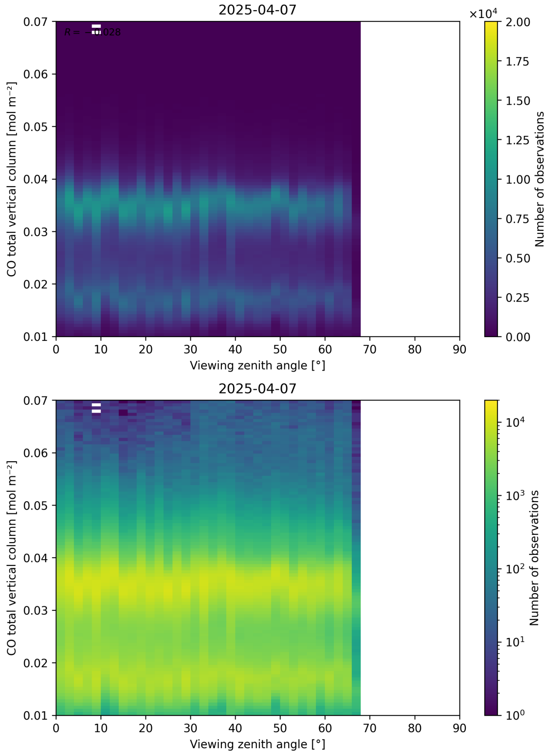
Figure 69: Scatter density plot of “Viewing zenith angle” against “CO total vertical column” for 2025-04-06 to 2025-04-08.
