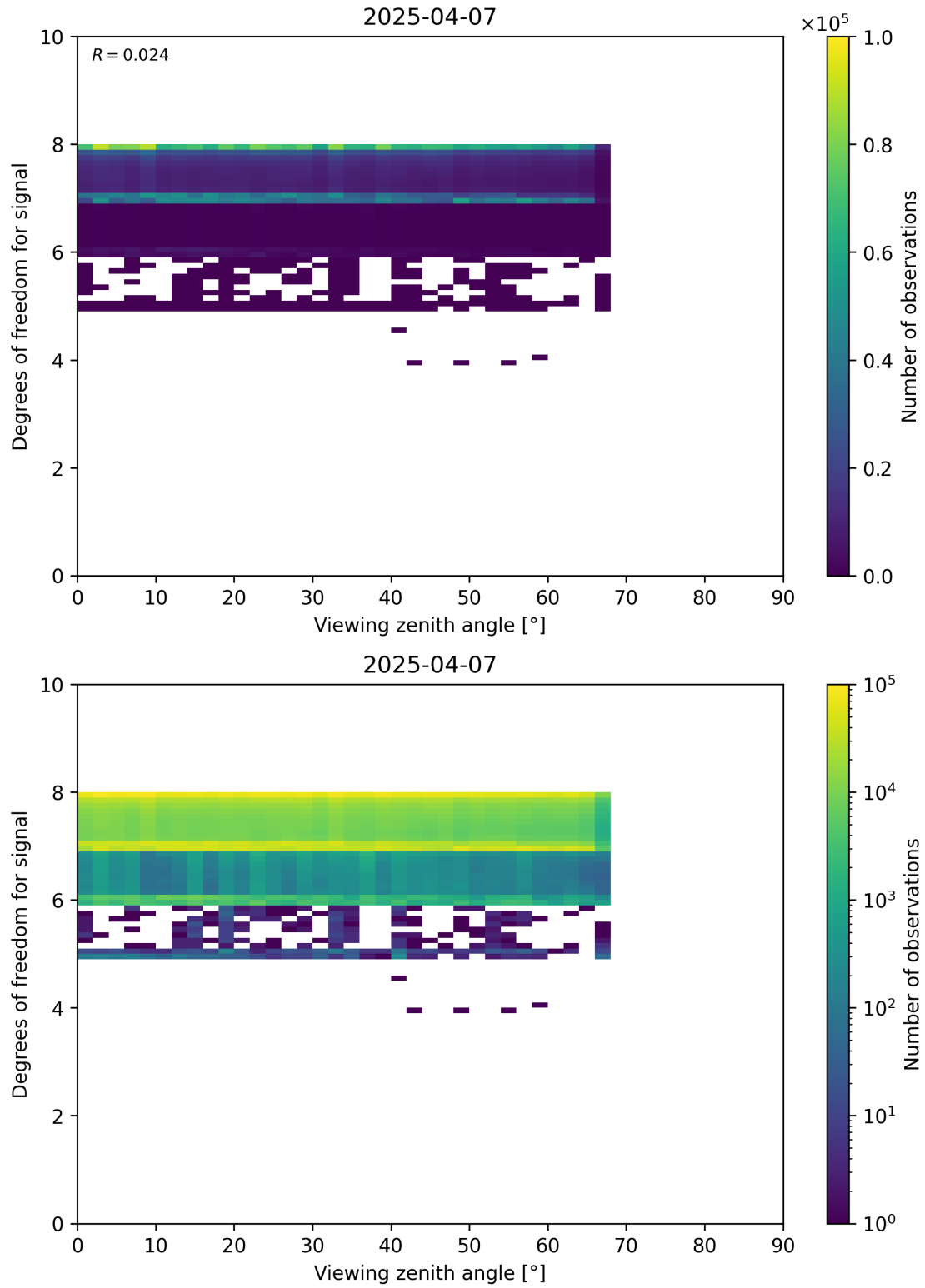
Figure 73: Scatter density plot of “Viewing zenith angle” against “Degrees of freedom for signal” for 2025-04-06 to 2025-04-08.
