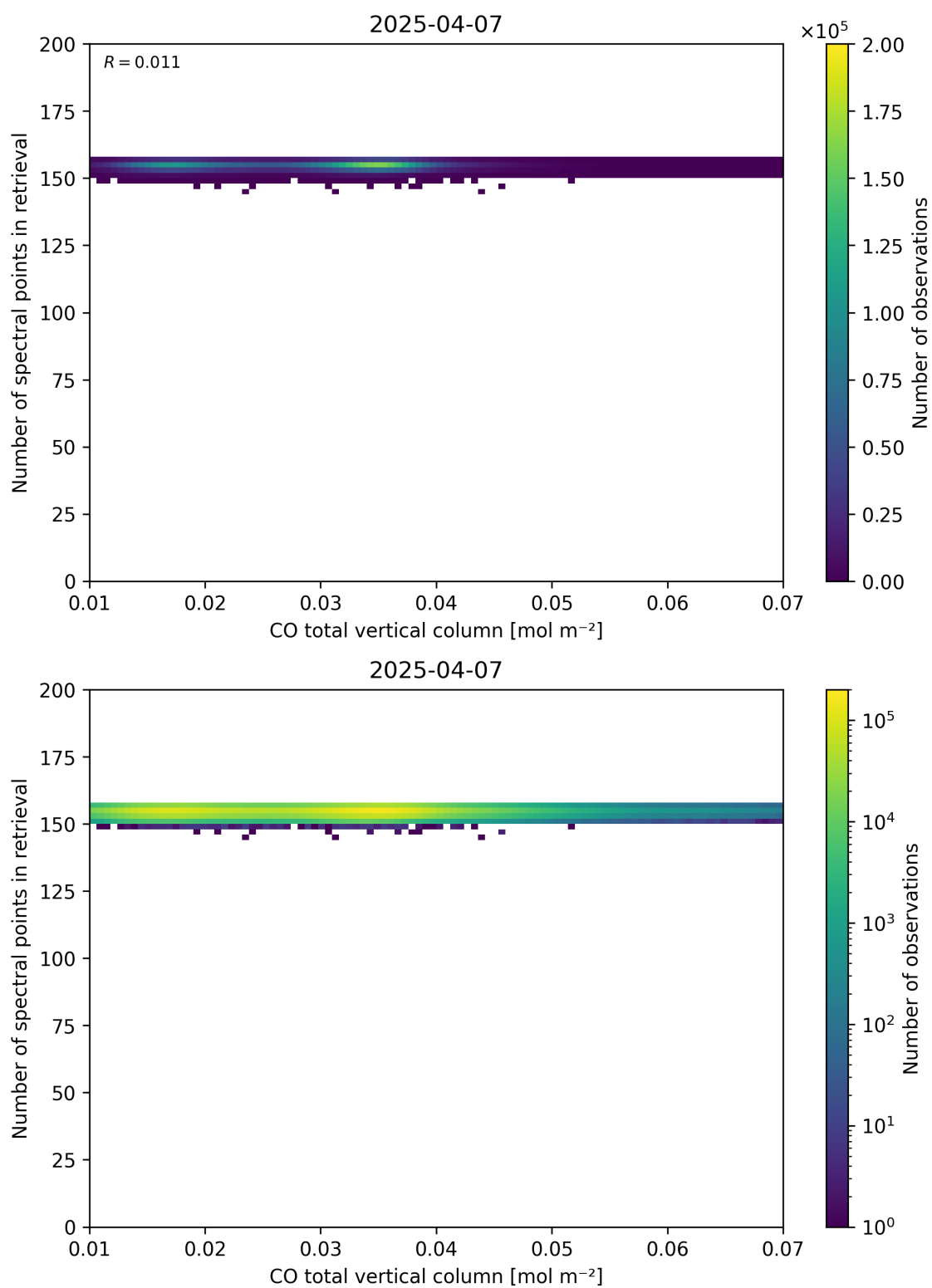
Figure 43: Scatter density plot of “CO total vertical column” against “Number of spectral points in retrieval” for 2025-04-06 to 2025-04-08.
