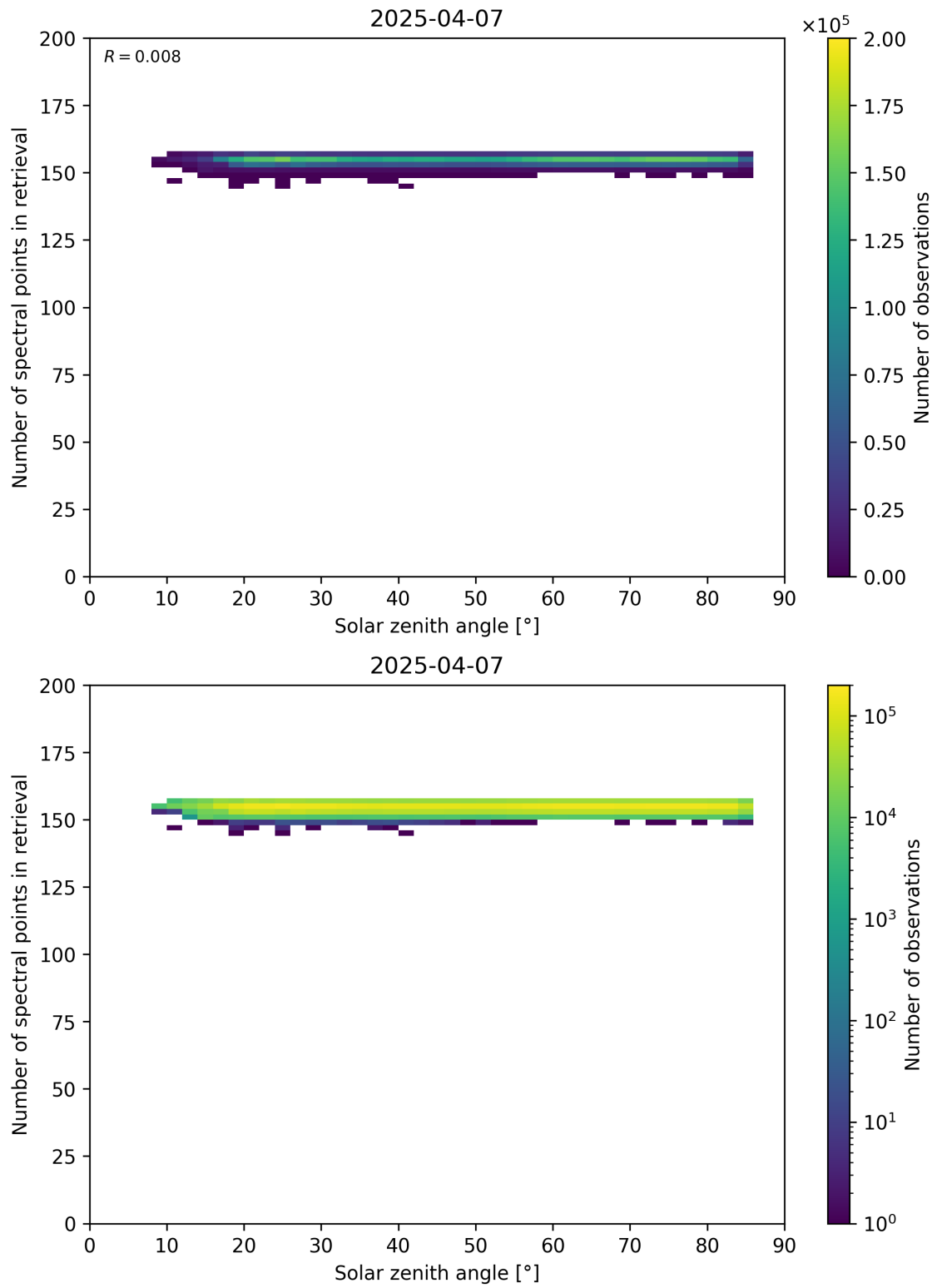
Figure 68: Scatter density plot of “Solar zenith angle” against “Number of spectral points in retrieval” for 2025-04-06 to 2025-04-08.
