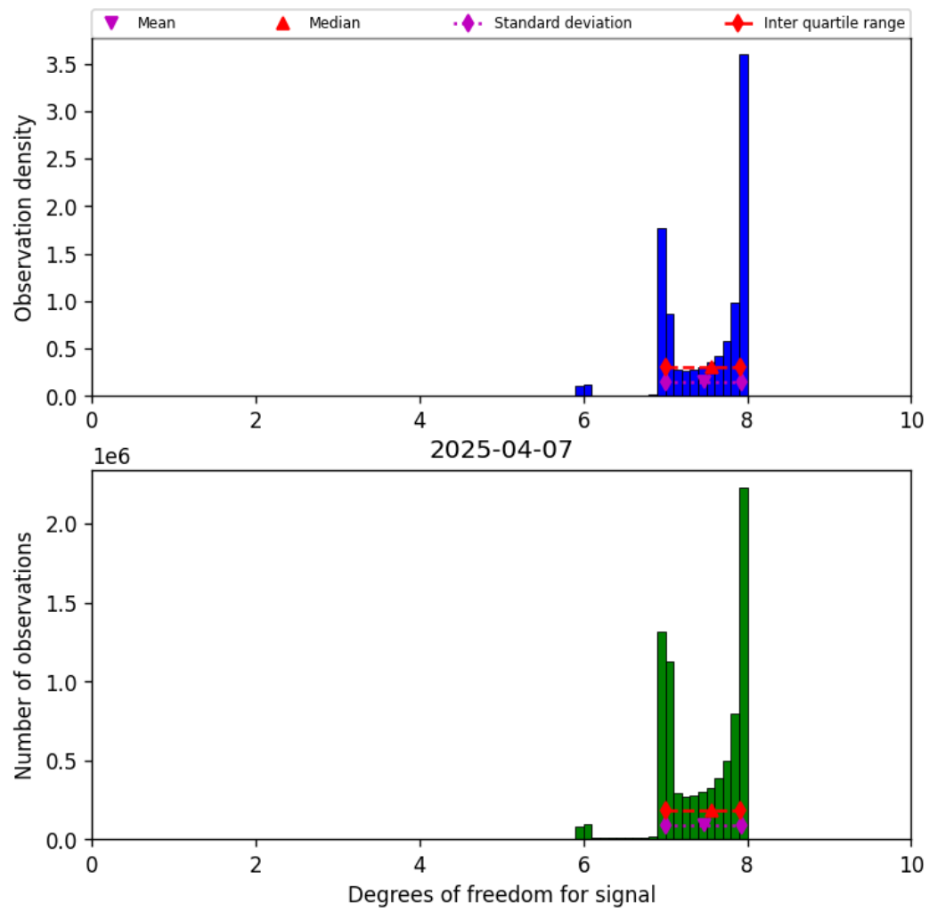
Figure 23: Histogram of “Degrees of freedom for signal” for 2025-04-06 to 2025-04-08
