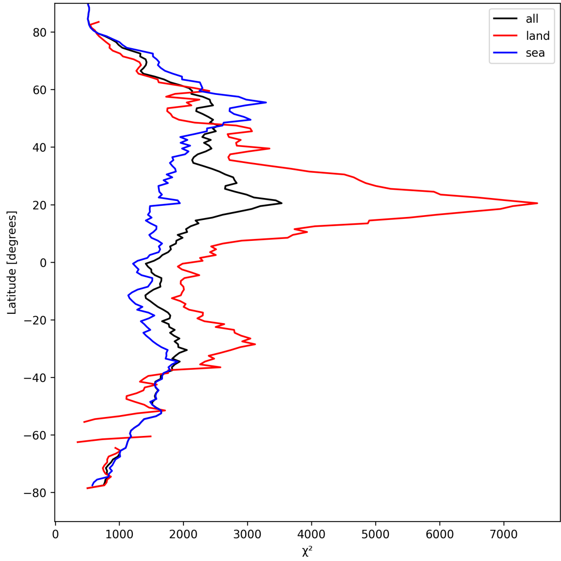
Figure 14: Zonal average of “ \chi^2 ” for 2025-04-06 to 2025-04-08.
