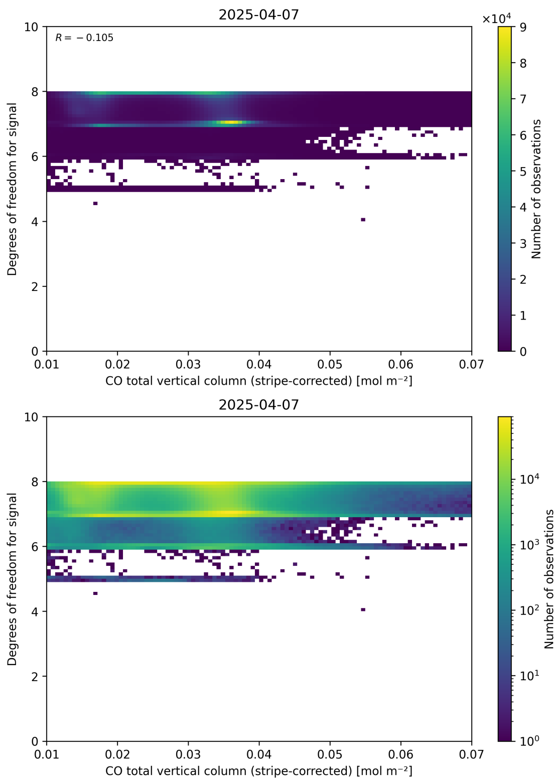
Figure 38: Scatter density plot of “CO total vertical column (stripe-corrected)” against “Degrees of freedom for signal” for 2025-04-06 to 2025-04-08.
