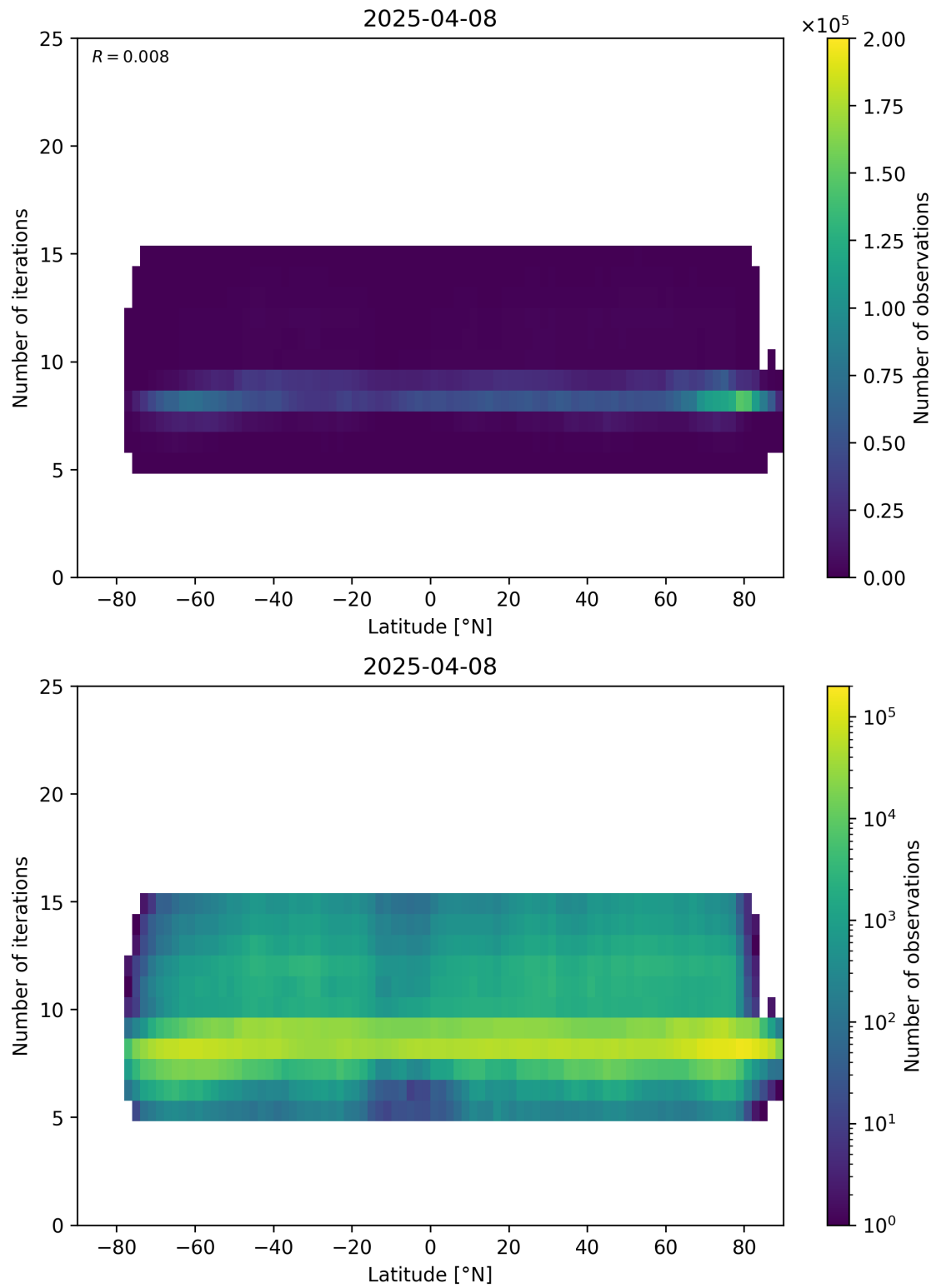
Figure 56: Scatter density plot of “Latitude” against “Number of iterations” for 2025-04-08 to 2025-04-09.
