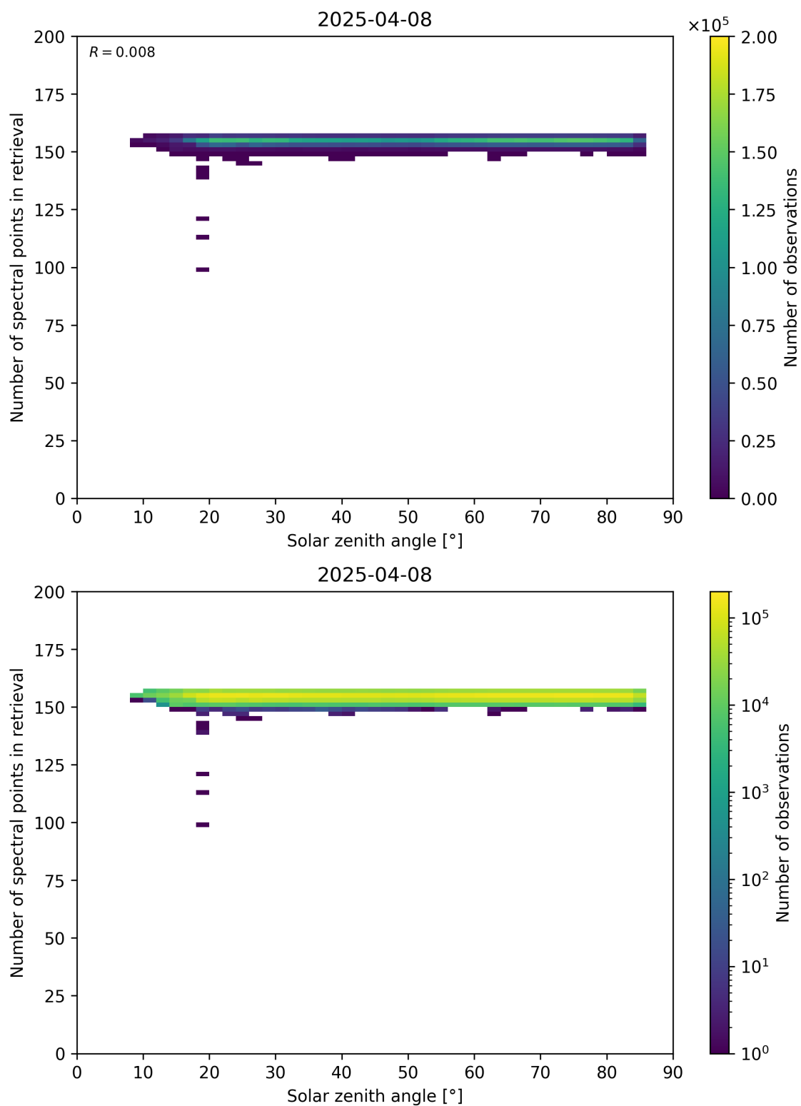
Figure 68: Scatter density plot of “Solar zenith angle” against “Number of spectral points in retrieval” for 2025-04-08 to 2025-04-09.
