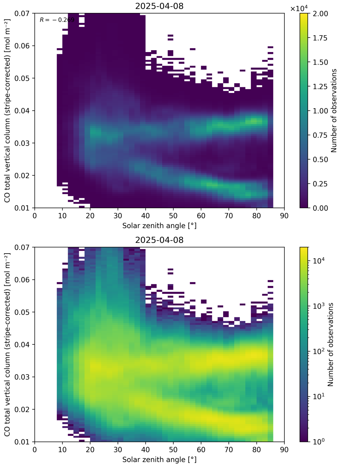
Figure 62: Scatter density plot of “Solar zenith angle” against “CO total vertical column (stripe-corrected)” for 2025-04-08 to 2025-04-09.
