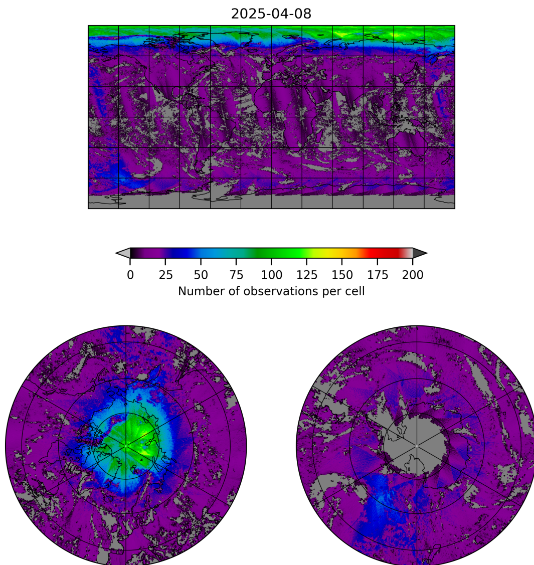
Figure 8: Map of the number of observations for 2025-04-08 to 2025-04-09
