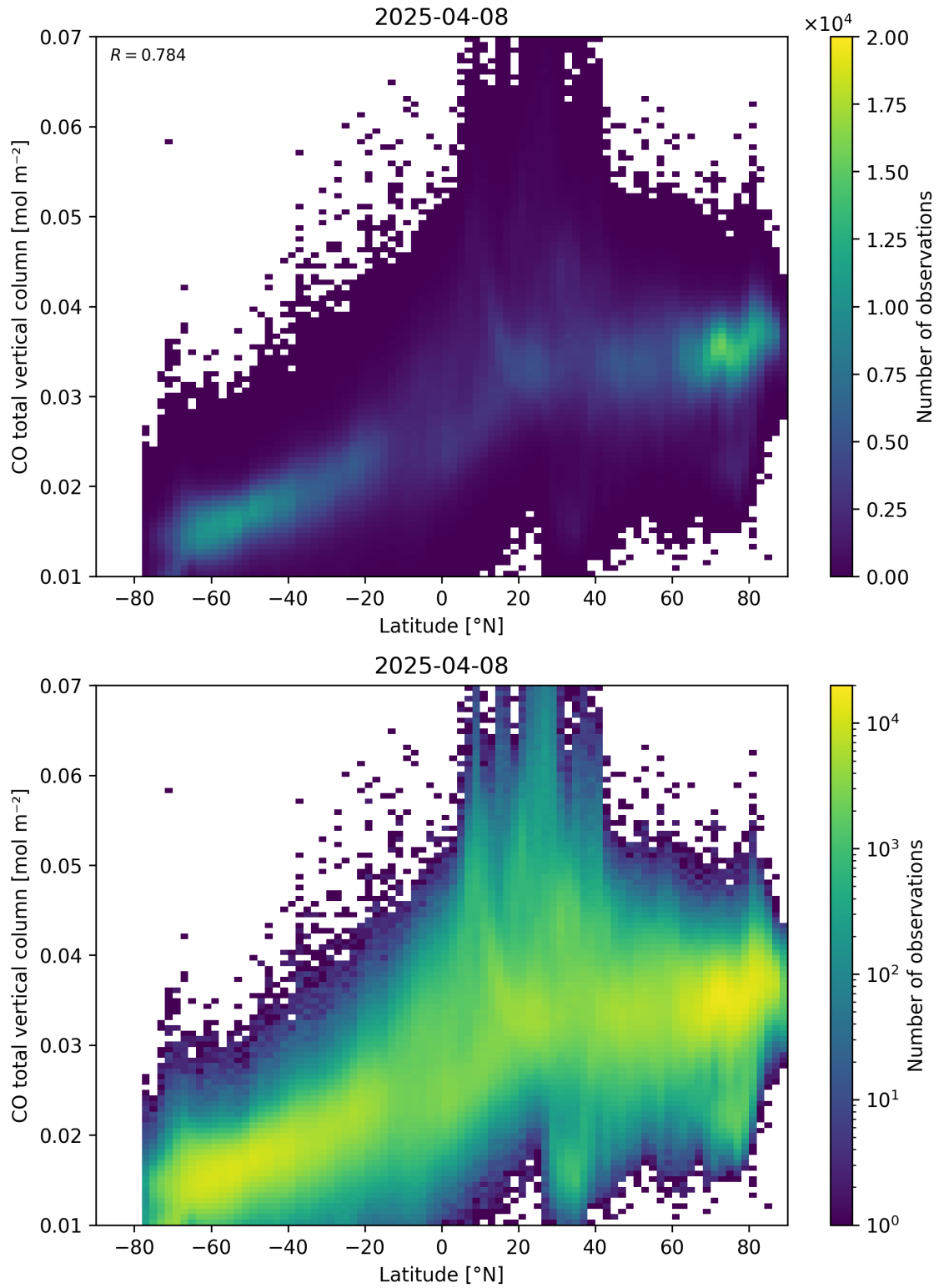
Figure 51: Scatter density plot of “Latitude” against “CO total vertical column” for 2025-04-08 to 2025-04-09.
