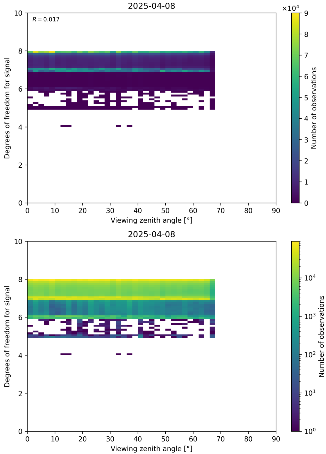
Figure 73: Scatter density plot of “Viewing zenith angle” against “Degrees of freedom for signal” for 2025-04-08 to 2025-04-09.
