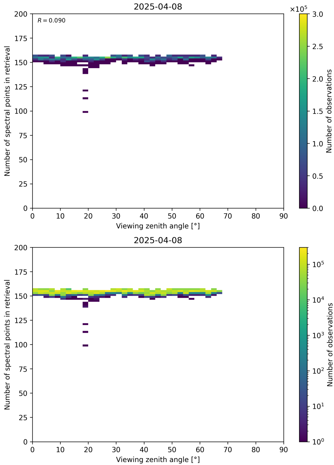
Figure 76: Scatter density plot of “Viewing zenith angle” against “Number of spectral points in retrieval” for 2025-04-08 to 2025-04-09.
