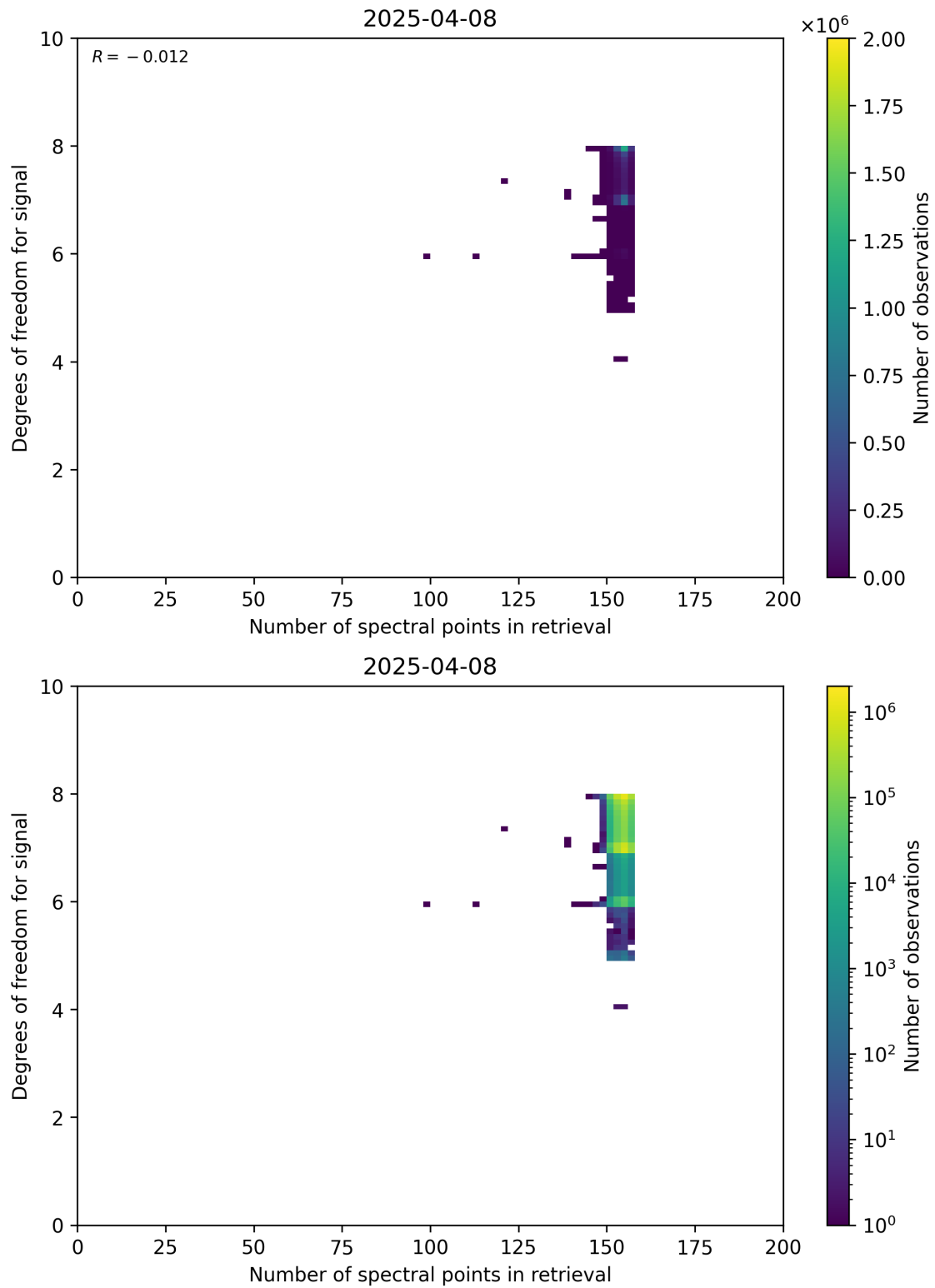
Figure 59: Scatter density plot of “Number of spectral points in retrieval” against “Degrees of freedom for signal” for 2025-04-08 to 2025-04-09.
