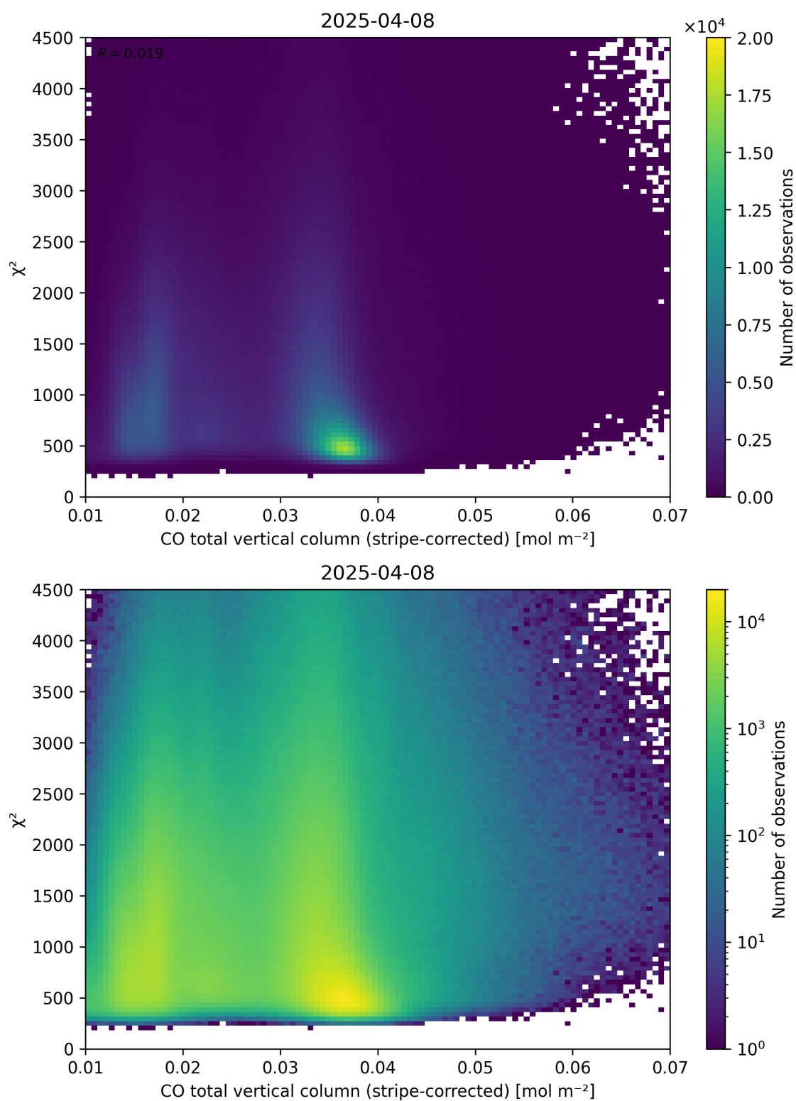
Figure 37: Scatter density plot of “CO total vertical column (stripe-corrected)” against “ \chi^2 ” for 2025-04-08 to 2025-04-09.
