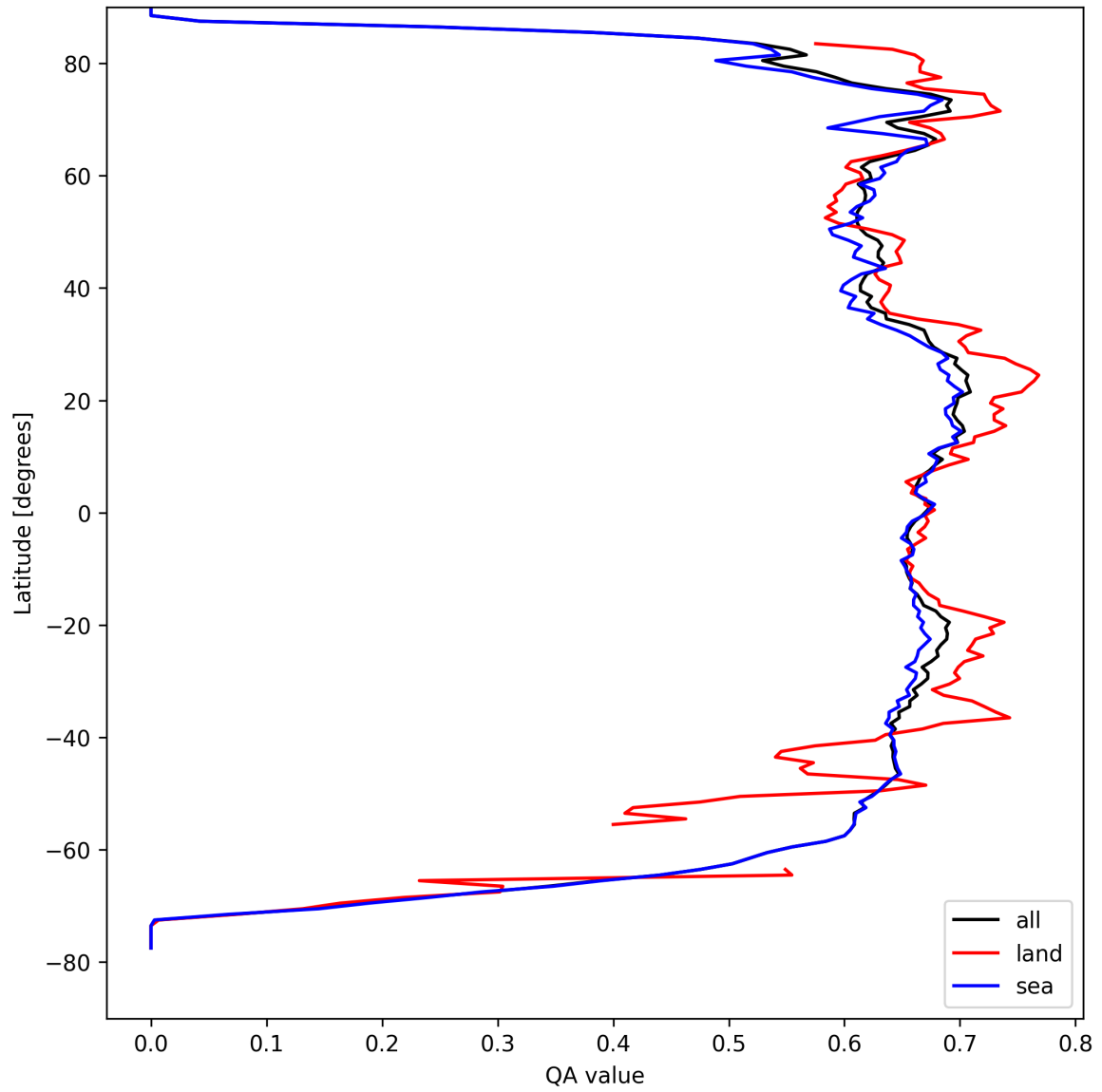
Figure 9: Zonal average of “QA value” for 2025-04-08 to 2025-04-09.
