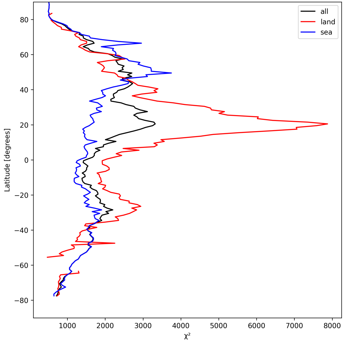
Figure 14: Zonal average of “ \chi^2 ” for 2025-04-08 to 2025-04-09.
