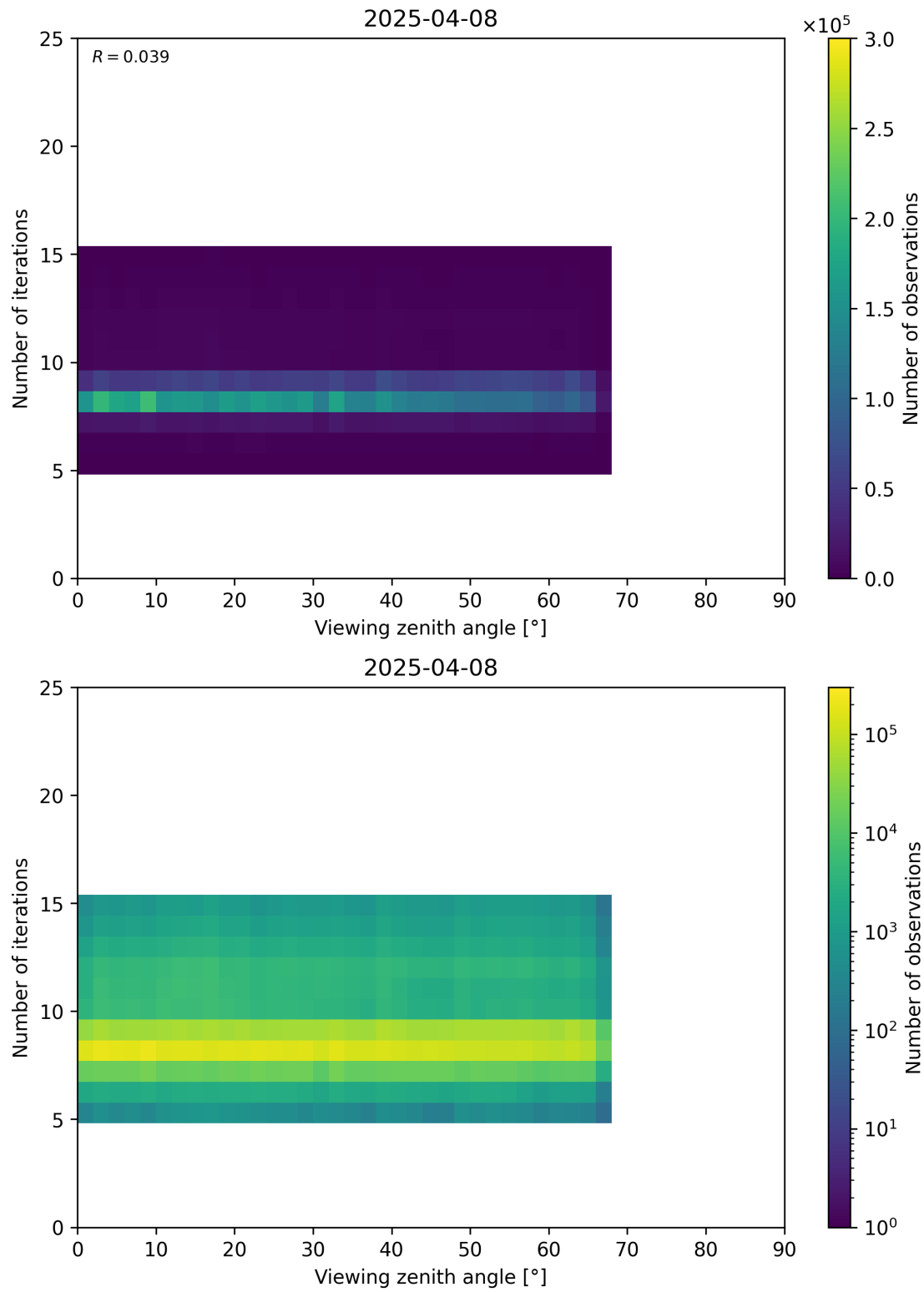
Figure 75: Scatter density plot of “Viewing zenith angle” against “Number of iterations” for 2025-04-08 to 2025-04-09.
