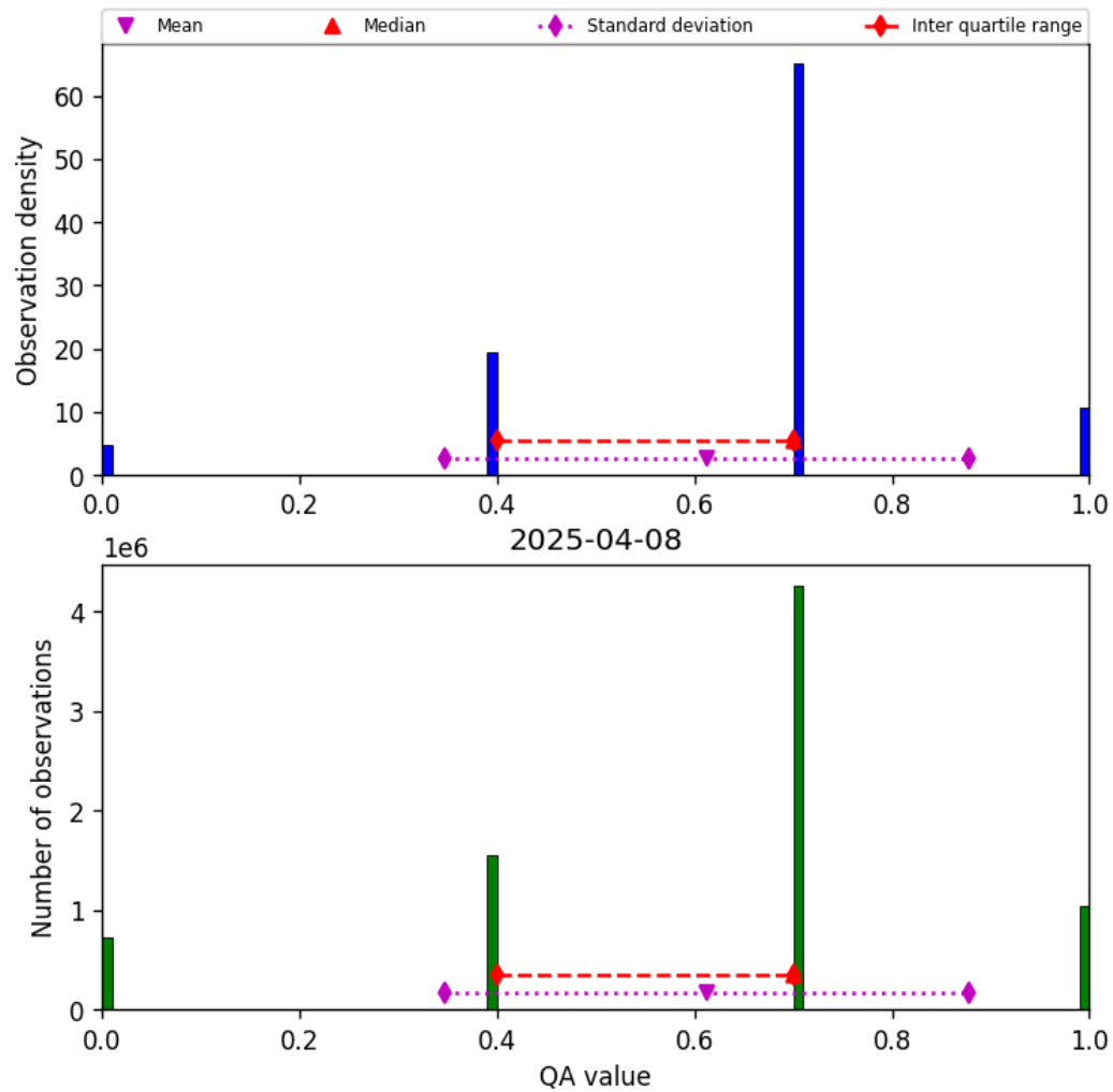
Figure 17: Histogram of “QA value” for 2025-04-08 to 2025-04-09
