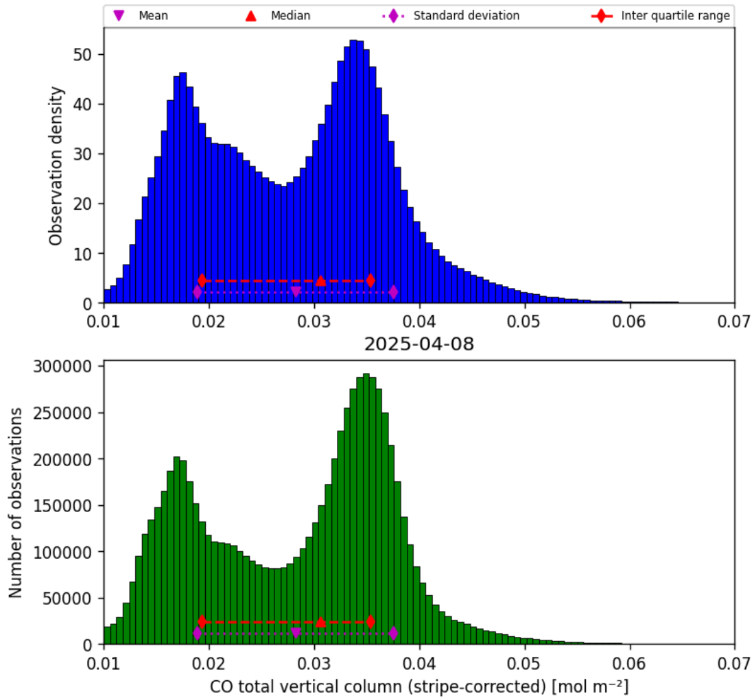
Figure 19: Histogram of “CO total vertical column (stripe-corrected)” for 2025-04-08 to 2025-04-09
