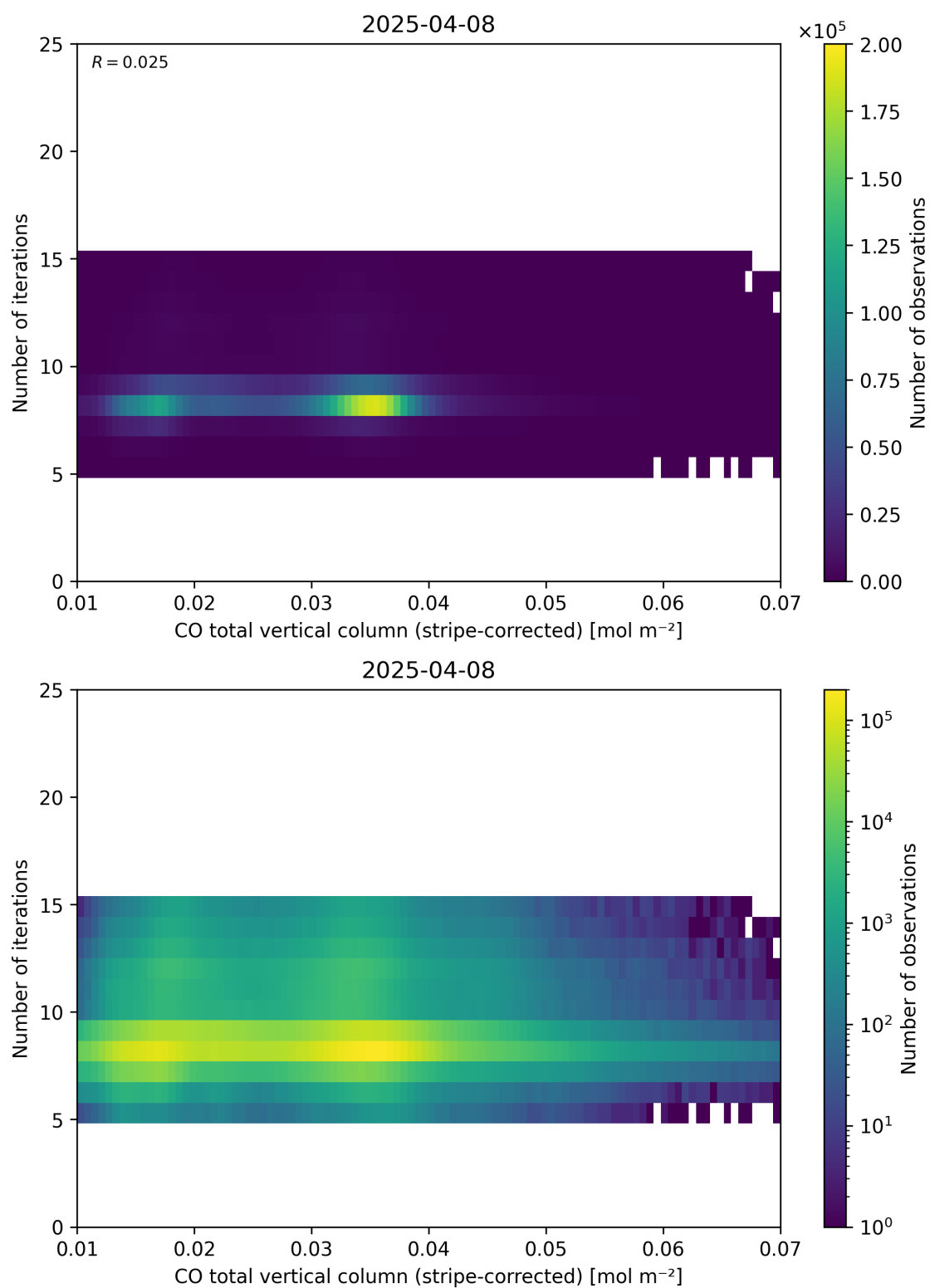
Figure 39: Scatter density plot of “CO total vertical column (stripe-corrected)” against “Number of iterations” for 2025-04-08 to 2025-04-09.
