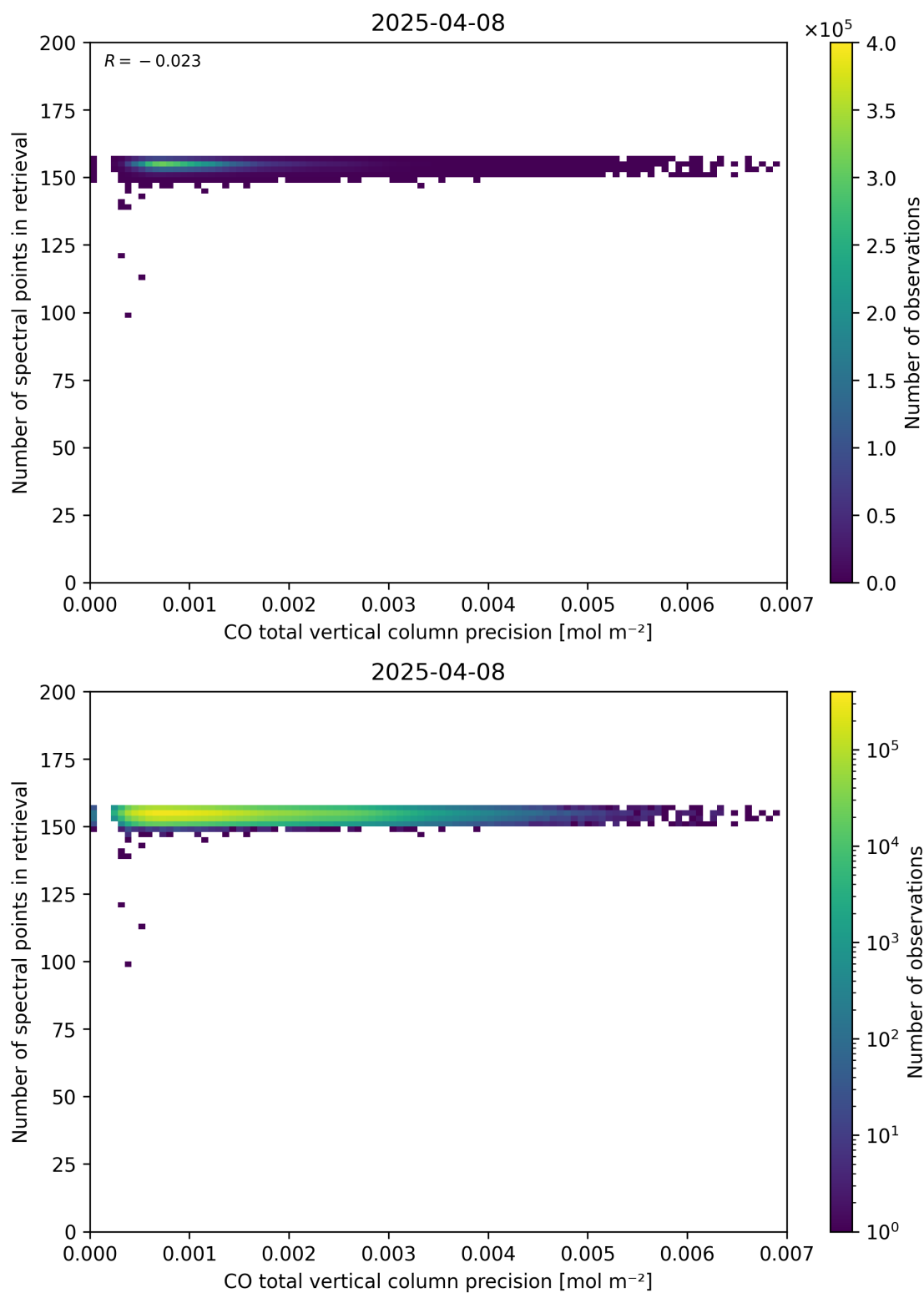
Figure 47: Scatter density plot of “CO total vertical column precision” against “Number of spectral points in retrieval” for 2025-04-08 to 2025-04-09.
