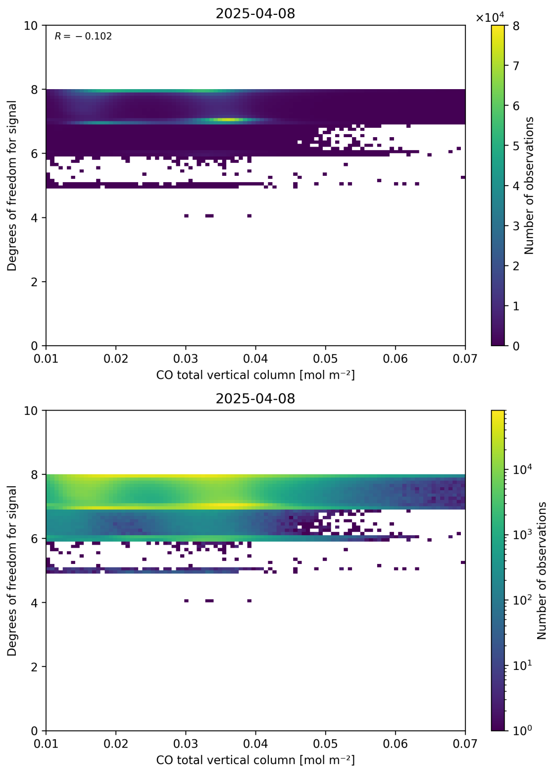
Figure 41: Scatter density plot of “CO total vertical column” against “Degrees of freedom for signal” for 2025-04-08 to 2025-04-09.
