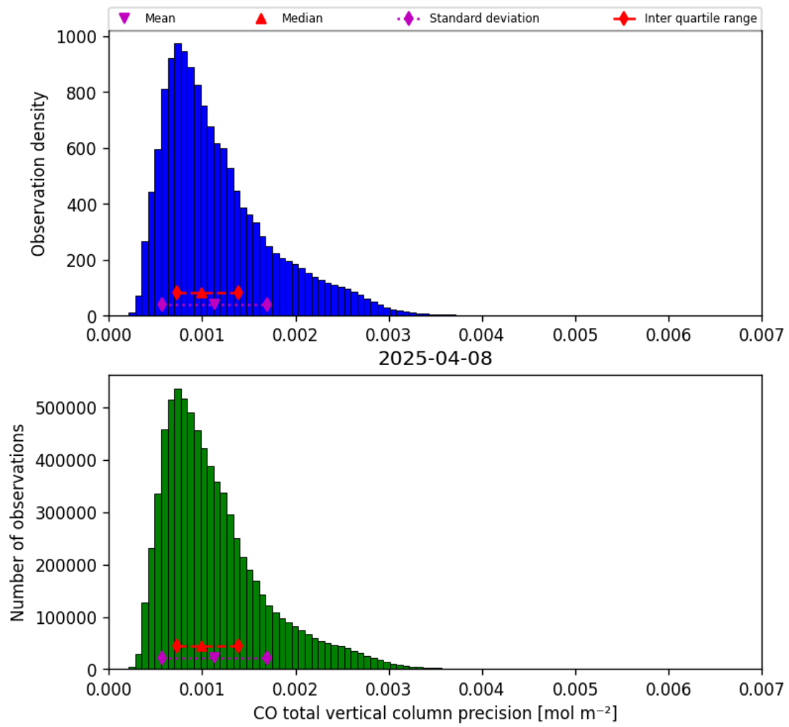
Figure 20: Histogram of “CO total vertical column precision” for 2025-04-08 to 2025-04-09
