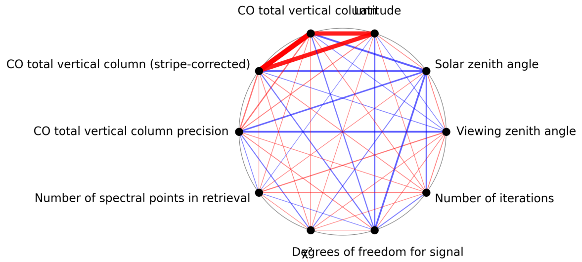
Figure 1: Map of correlation graph for 2025-04-08 to 2025-04-09.
