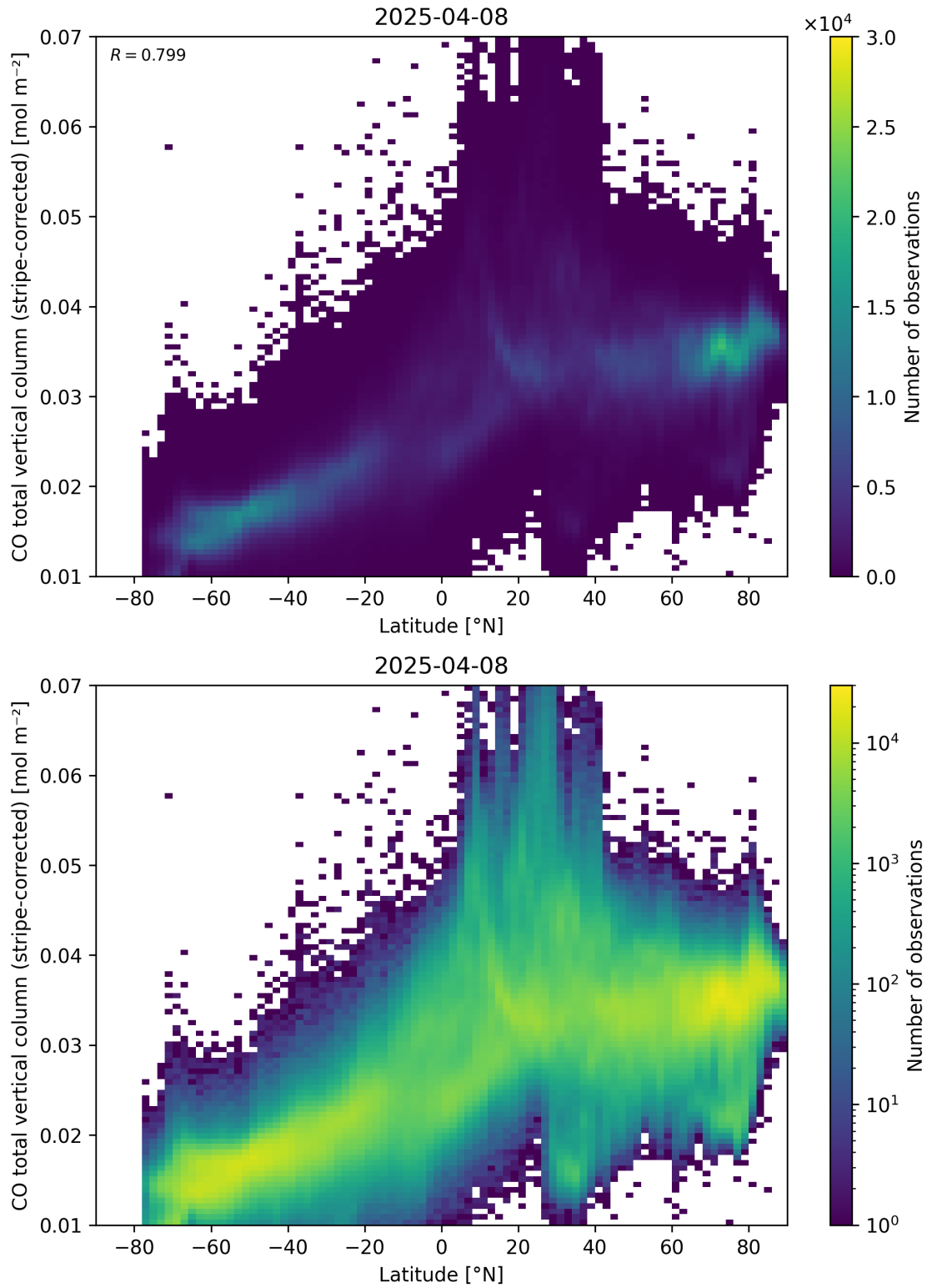
Figure 52: Scatter density plot of “Latitude” against “CO total vertical column (stripe-corrected)” for 2025-04-08 to 2025-04-09.
