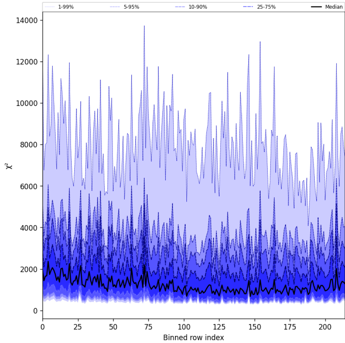
Figure 30: Along track statistics of “ \chi^2 ” for 2025-04-08 to 2025-04-09
