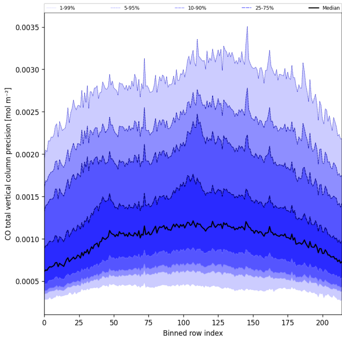
Figure 28: Along track statistics of “CO total vertical column precision” for 2025-04-08 to 2025-04-09
