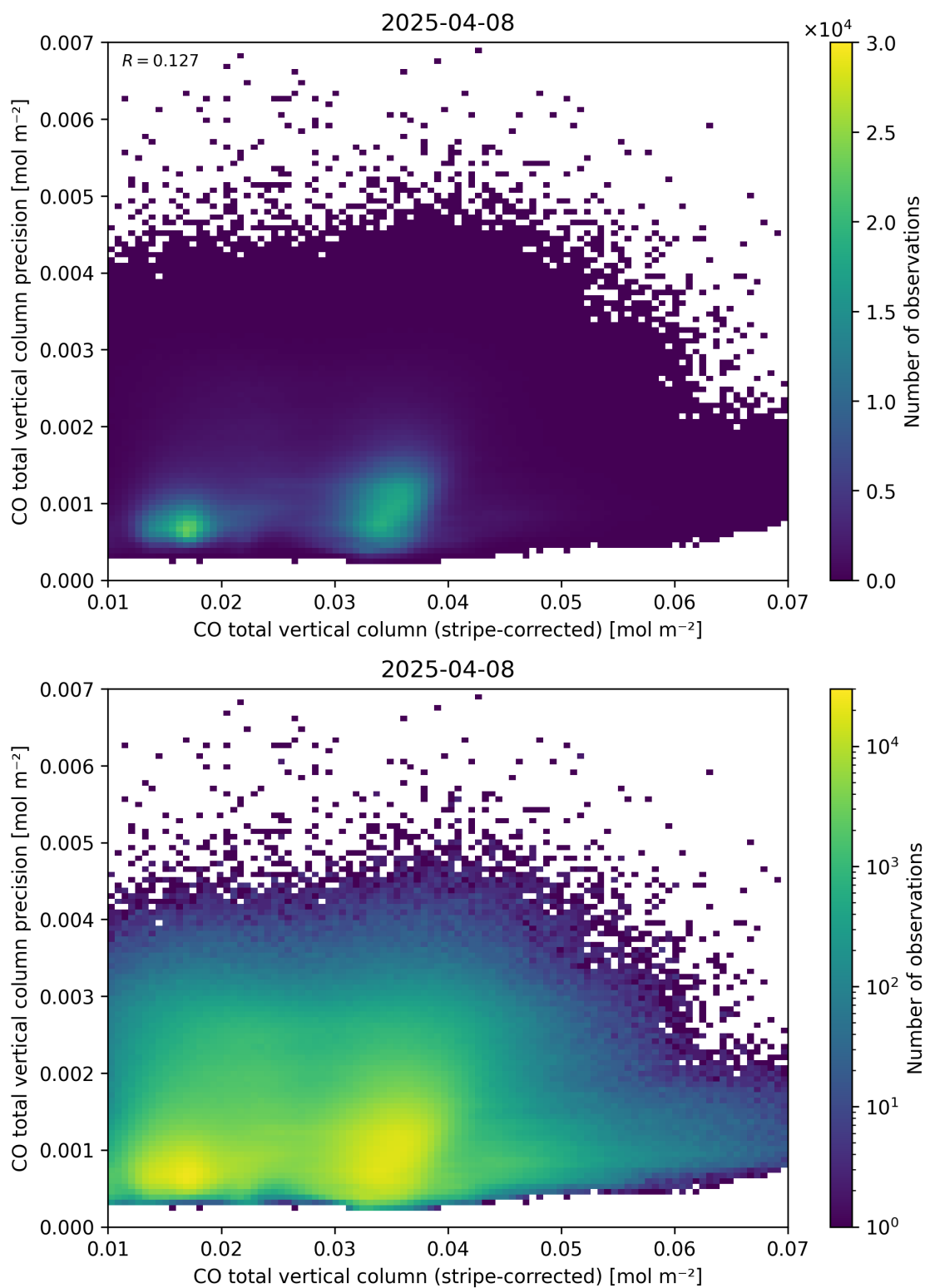
Figure 36: Scatter density plot of “CO total vertical column (stripe-corrected)” against “CO total vertical column precision” for 2025-04-08 to 2025-04-09.
