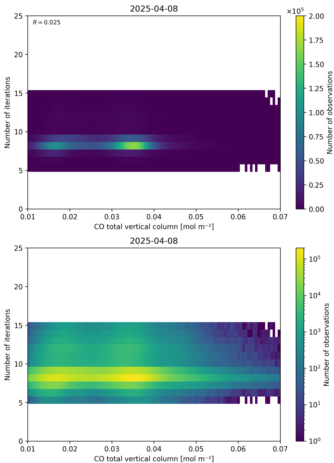
Figure 42: Scatter density plot of “CO total vertical column” against “Number of iterations” for 2025-04-08 to 2025-04-09.
