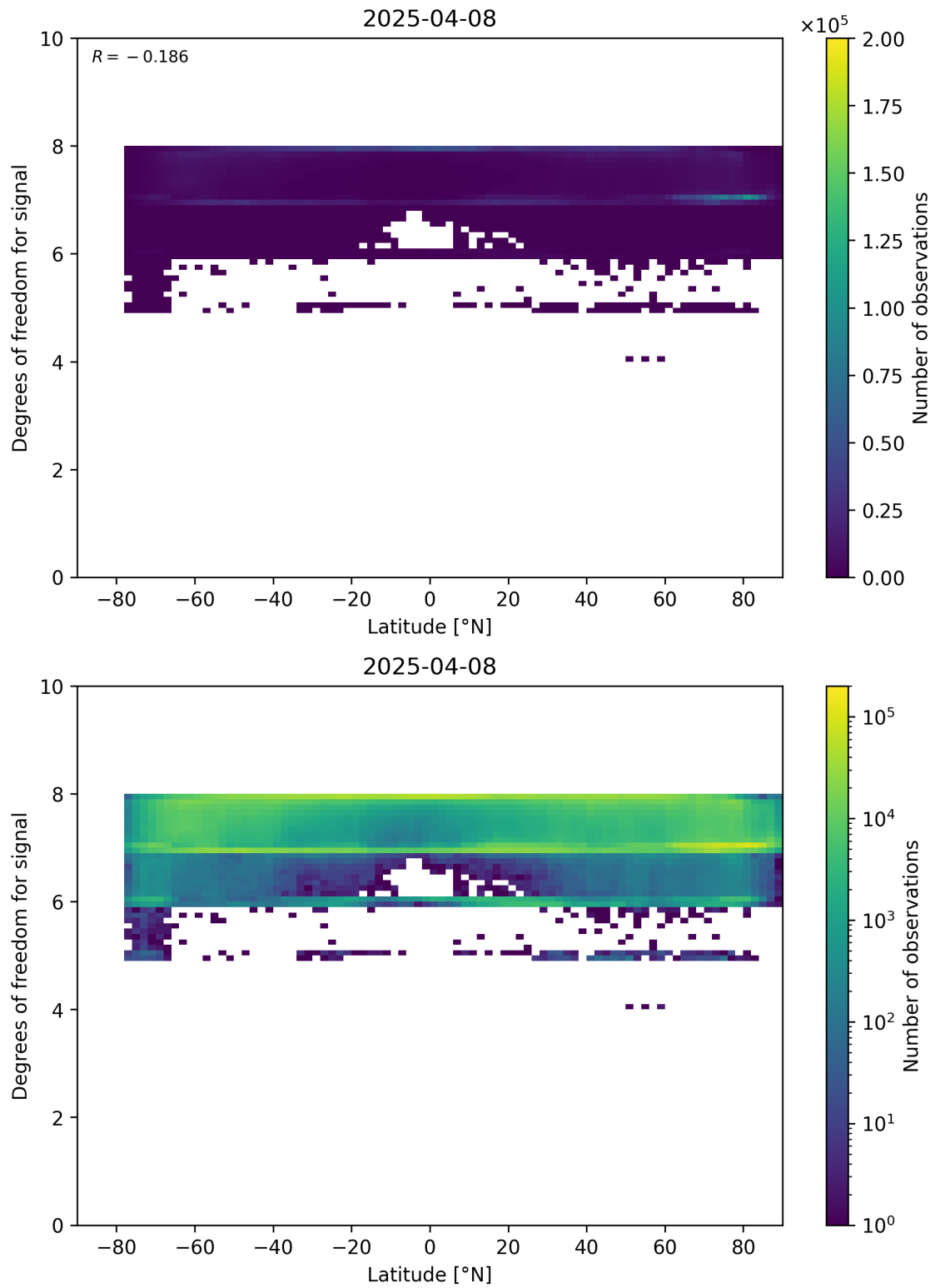
Figure 55: Scatter density plot of “Latitude” against “Degrees of freedom for signal” for 2025-04-08 to 2025-04-09.
