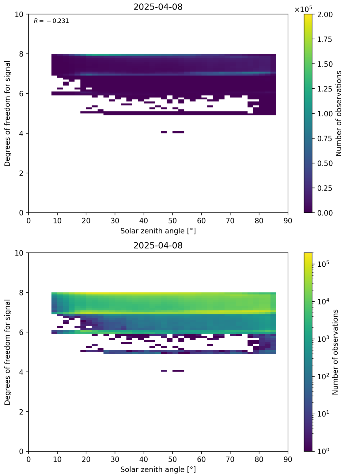
Figure 65: Scatter density plot of “Solar zenith angle” against “Degrees of freedom for signal” for 2025-04-08 to 2025-04-09.
