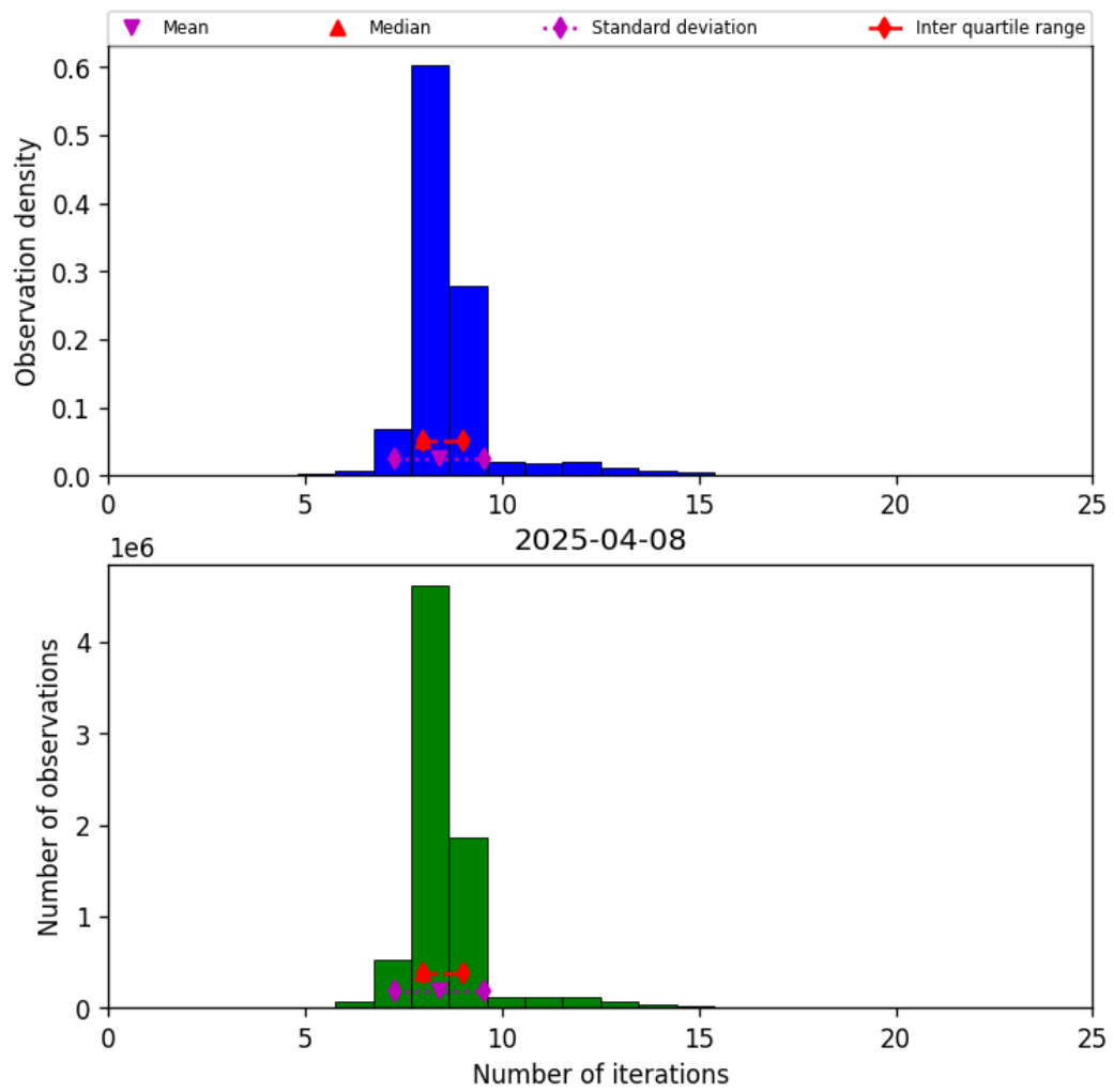
Figure 24: Histogram of “Number of iterations” for 2025-04-08 to 2025-04-09
