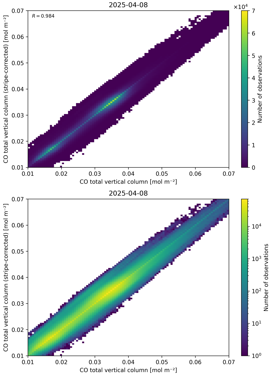
Figure 33: Scatter density plot of “CO total vertical column” against “CO total vertical column (stripe-corrected)” for 2025-04-08 to 2025-04-09.
