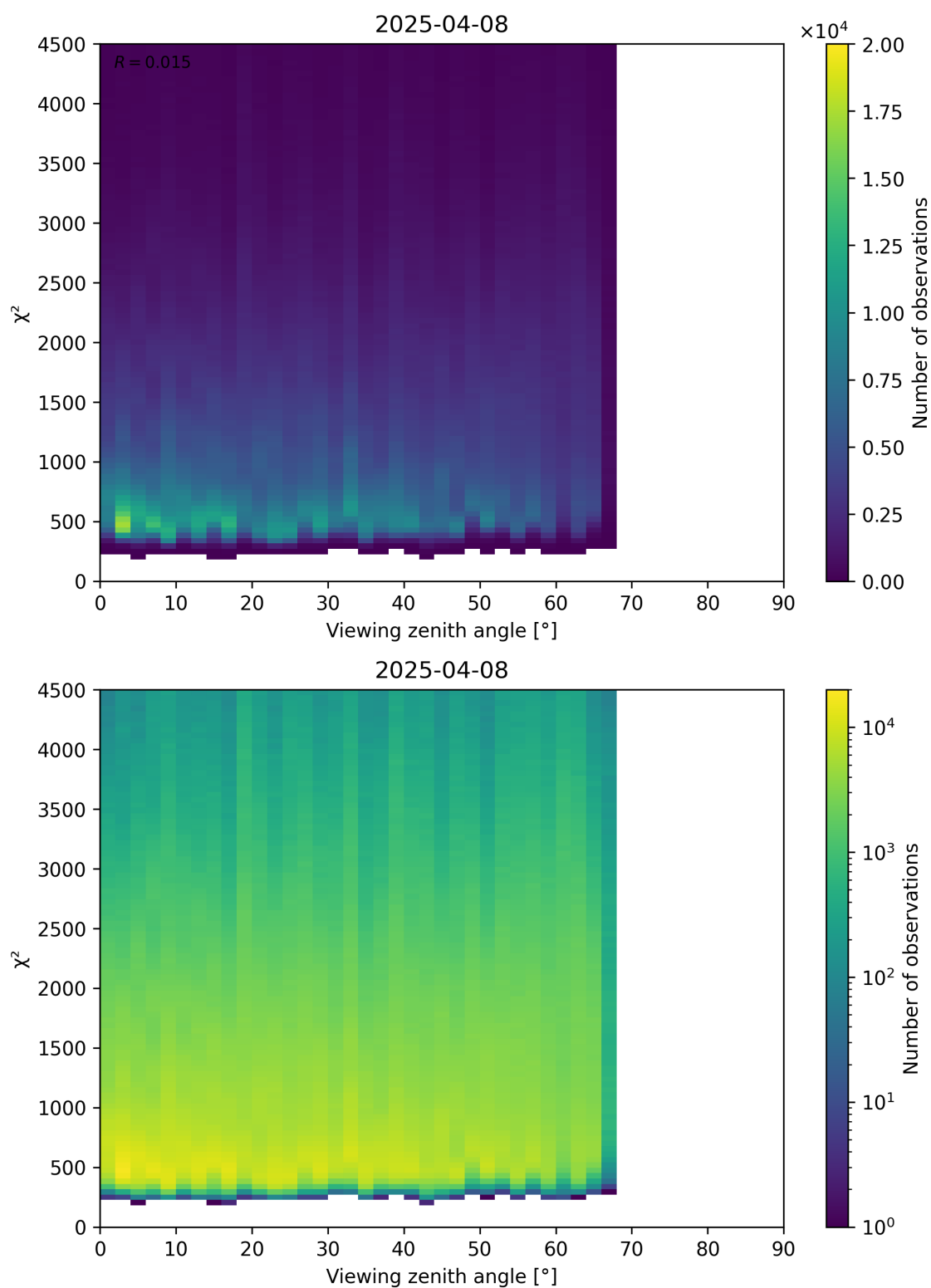
Figure 72: Scatter density plot of “Viewing zenith angle” against “ \chi^2 ” for 2025-04-08 to 2025-04-09.
