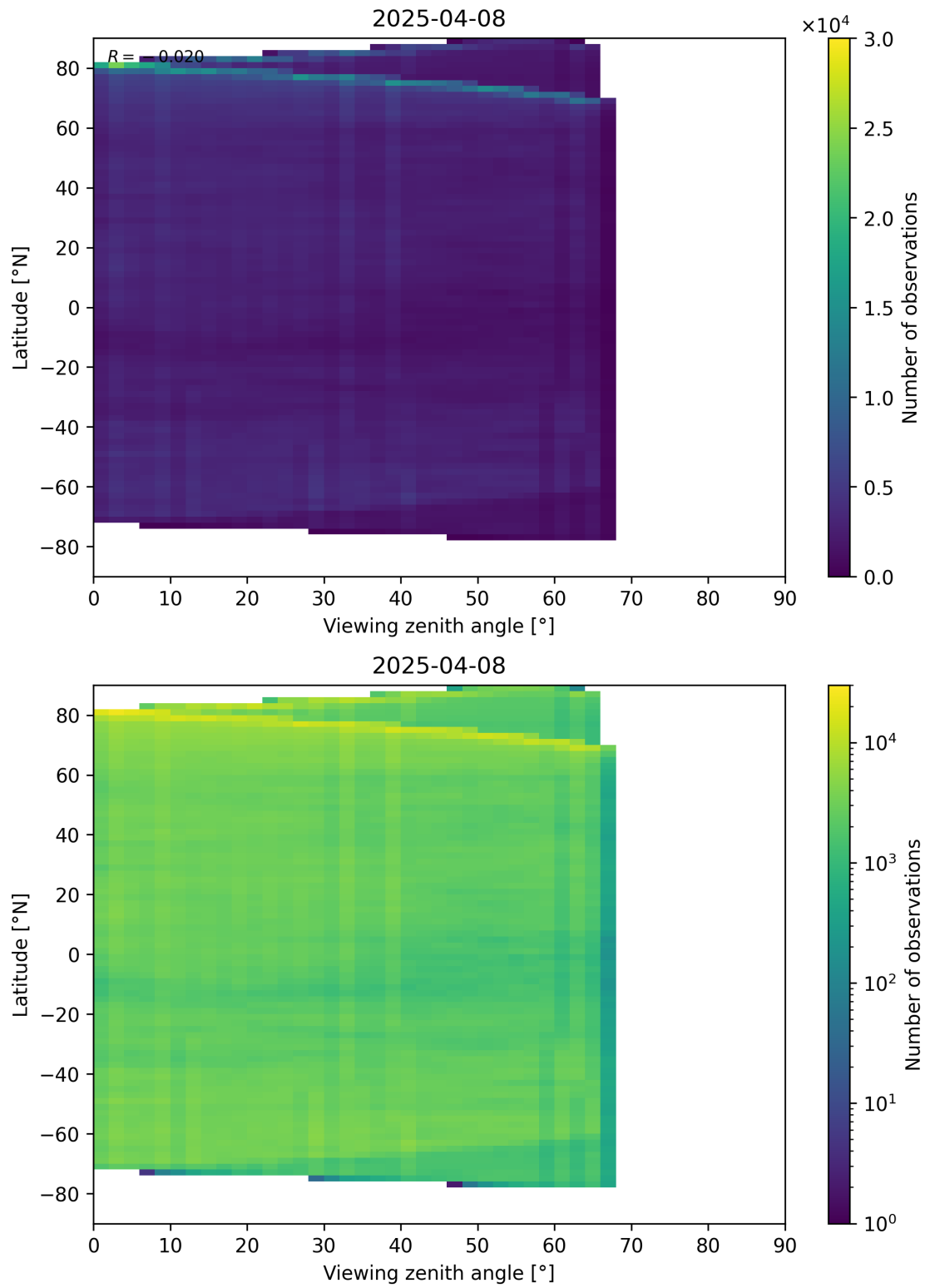
Figure 74: Scatter density plot of “Viewing zenith angle” against “Latitude” for 2025-04-08 to 2025-04-09.
