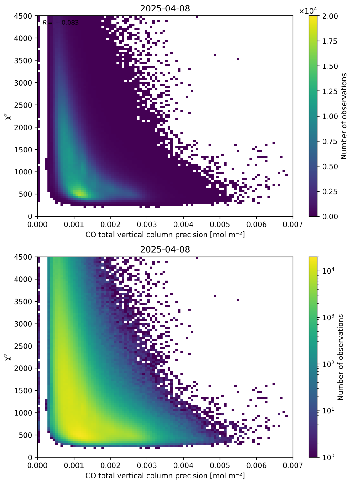
Figure 44: Scatter density plot of “CO total vertical column precision” against “ \chi^2 ” for 2025-04-08 to 2025-04-09.
