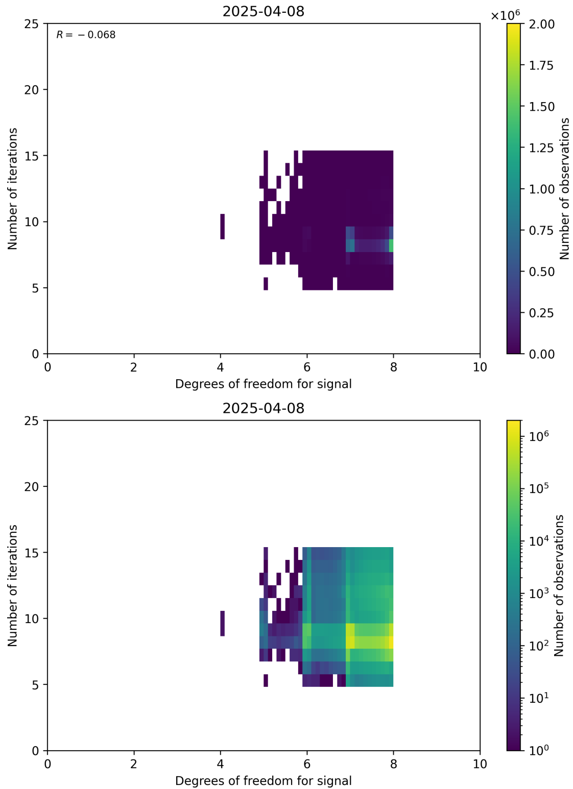
Figure 50: Scatter density plot of “Degrees of freedom for signal” against “Number of iterations” for 2025-04-08 to 2025-04-09.
