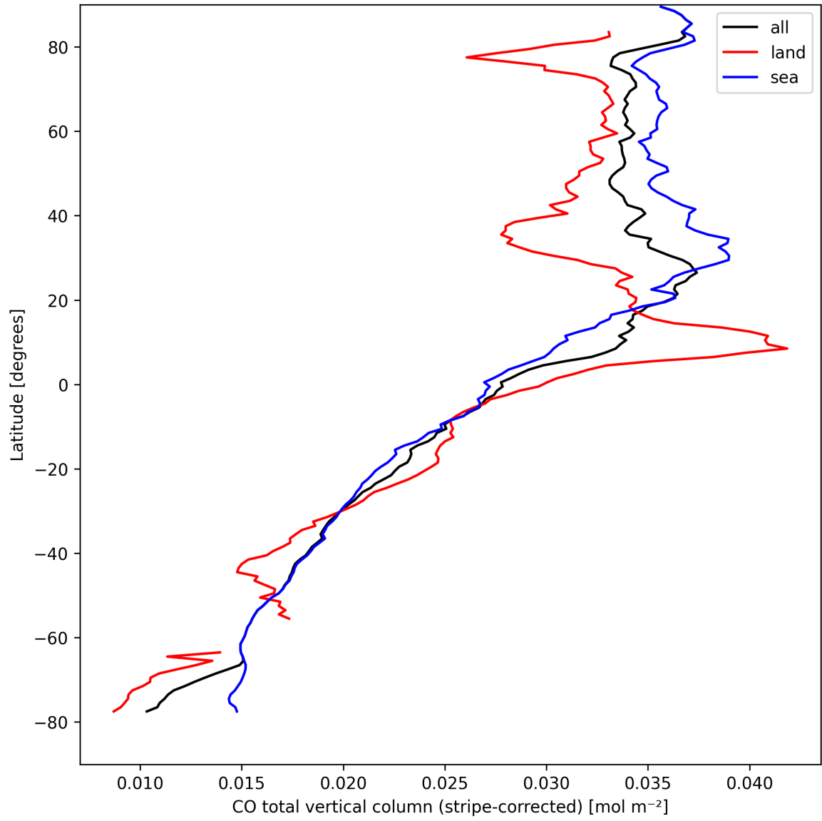
Figure 11: Zonal average of “CO total vertical column (stripe-corrected)” for 2025-04-08 to 2025-04-09.
