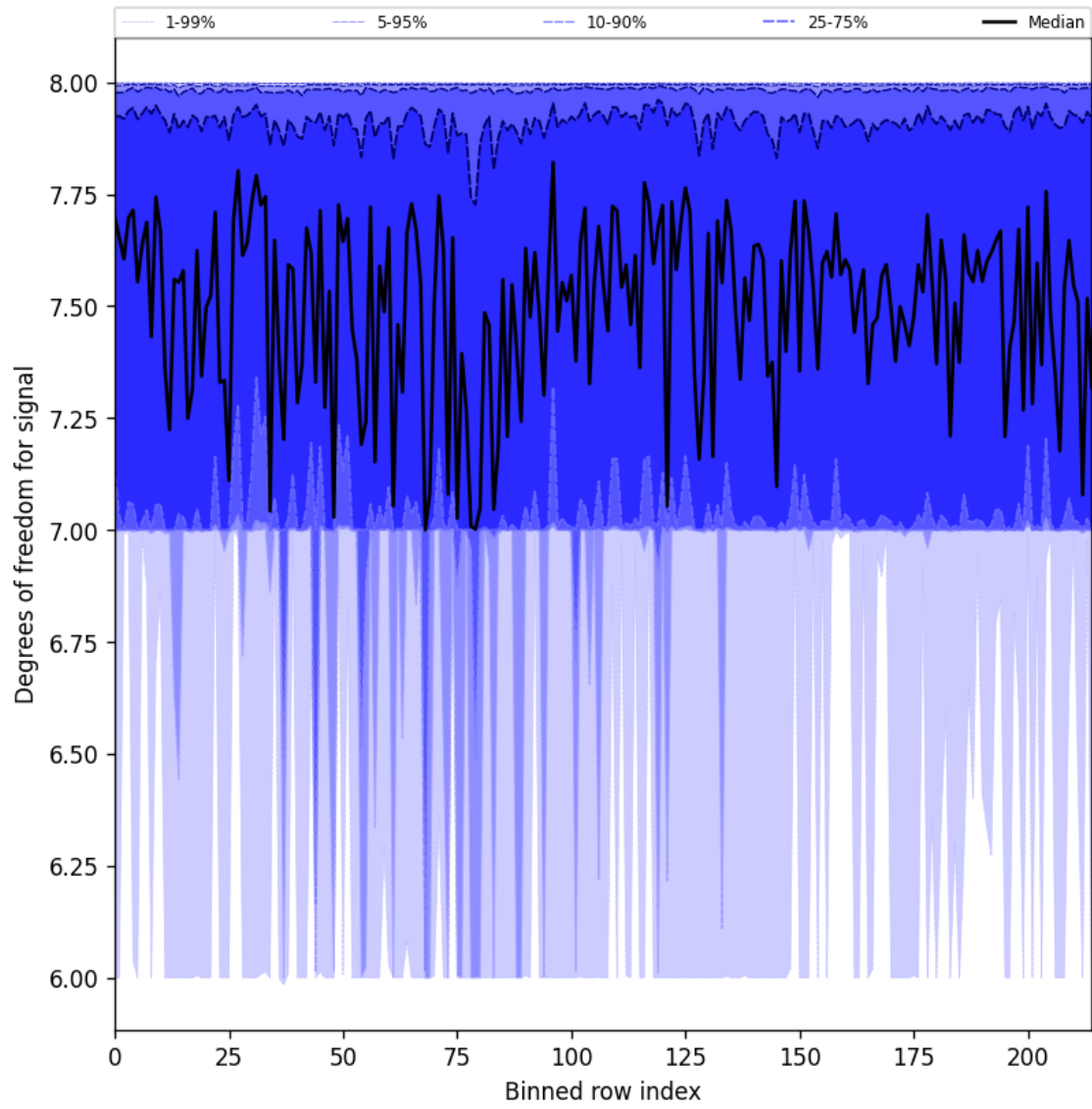
Figure 31: Along track statistics of “Degrees of freedom for signal” for 2025-04-08 to 2025-04-09
