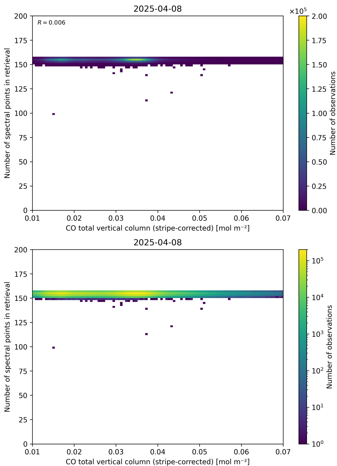
Figure 40: Scatter density plot of “CO total vertical column (stripe-corrected)” against “Number of spectral points in retrieval” for 2025-04-08 to 2025-04-09.
