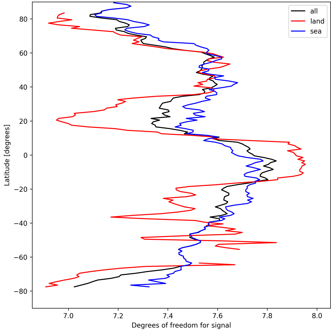
Figure 15: Zonal average of “Degrees of freedom for signal” for 2025-04-08 to 2025-04-09.
