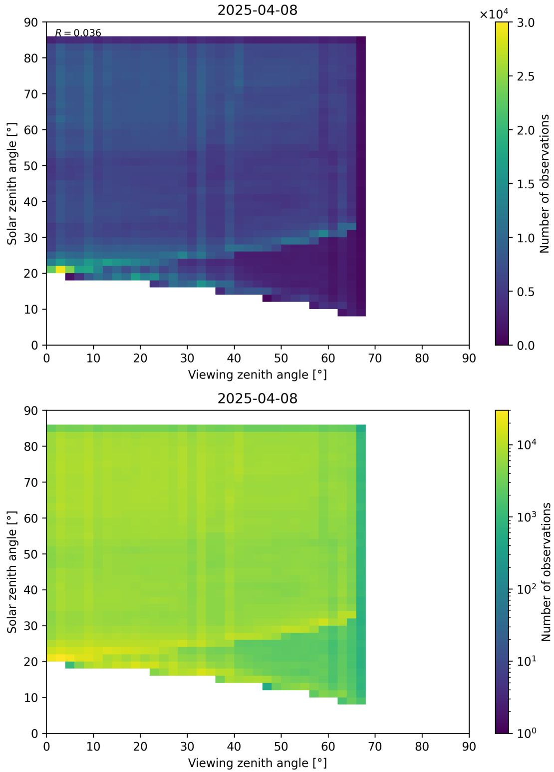
Figure 77: Scatter density plot of “Viewing zenith angle” against “Solar zenith angle” for 2025-04-08 to 2025-04-09.
