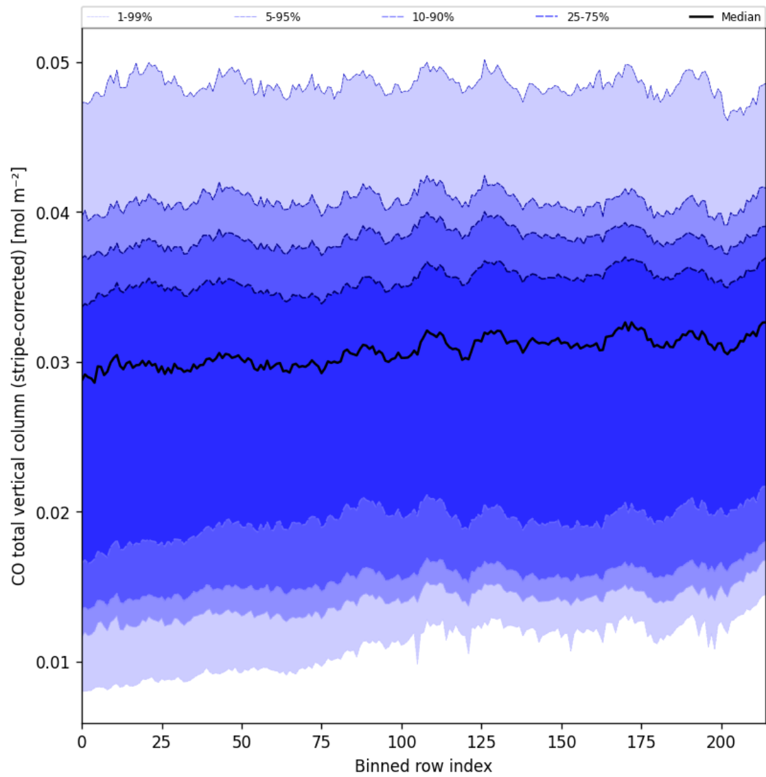
Figure 27: Along track statistics of “CO total vertical column (stripe-corrected)” for 2025-04-08 to 2025-04-09
