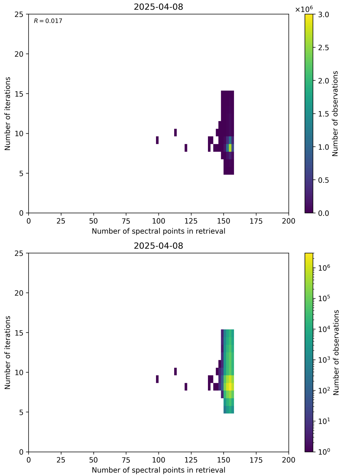
Figure 60: Scatter density plot of “Number of spectral points in retrieval” against “Number of iterations” for 2025-04-08 to 2025-04-09.
