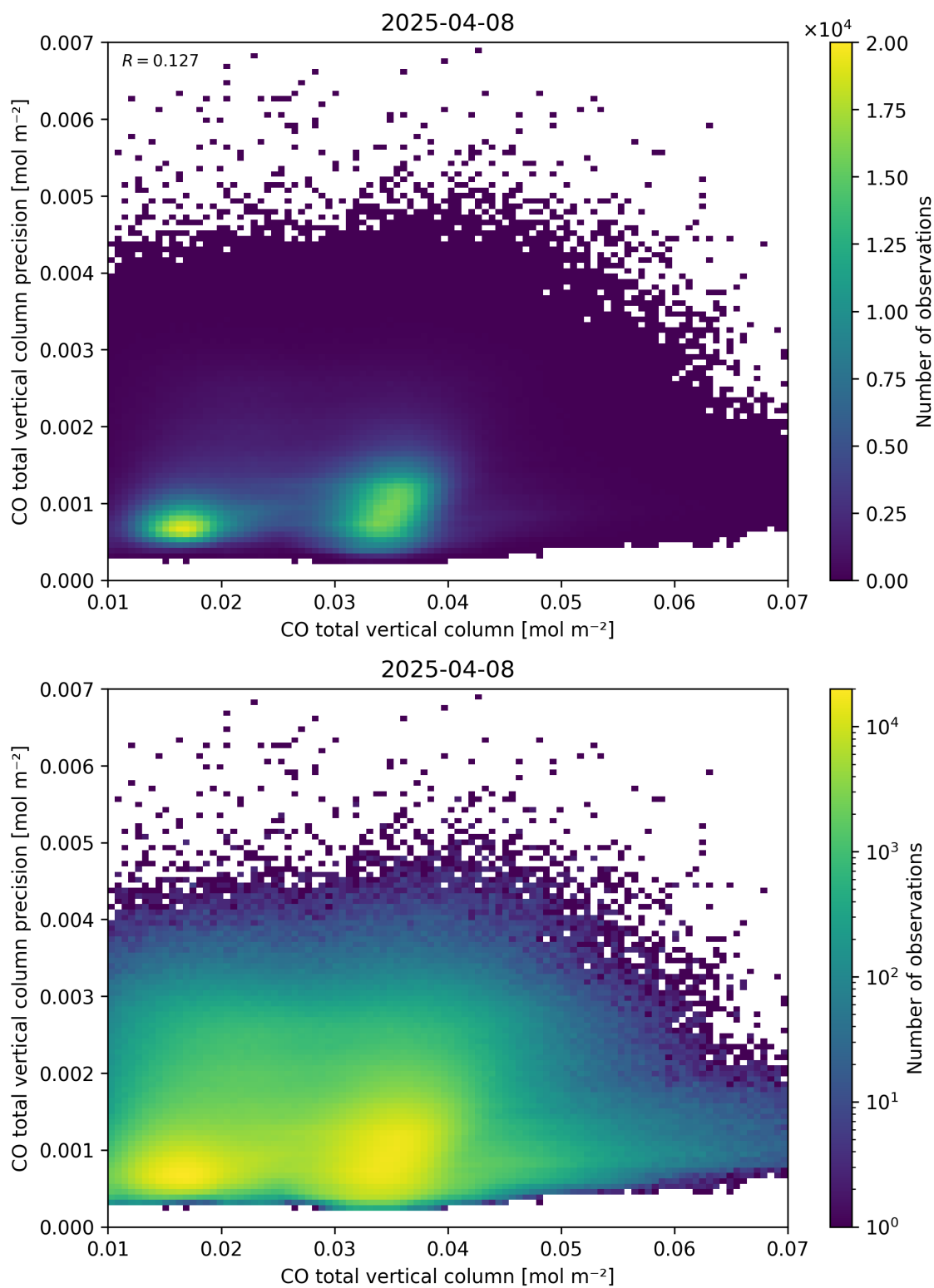
Figure 34: Scatter density plot of “CO total vertical column” against “CO total vertical column precision” for 2025-04-08 to 2025-04-09.
