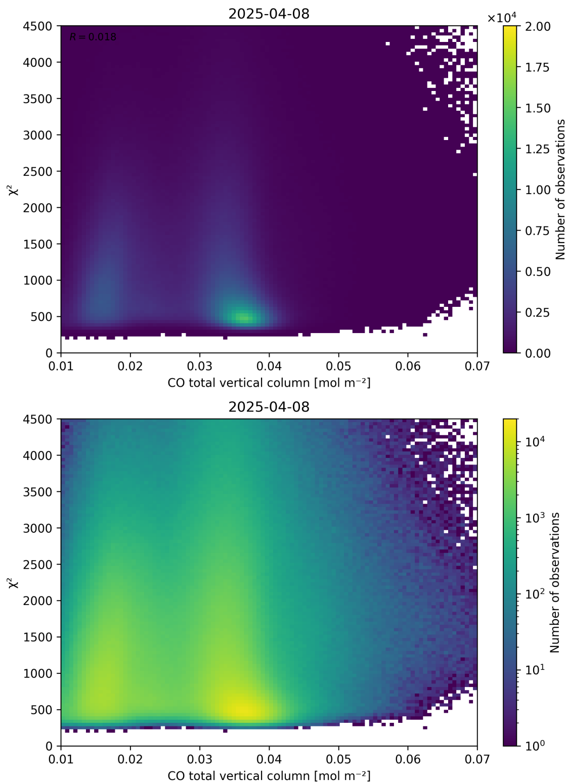
Figure 35: Scatter density plot of “CO total vertical column” against “ \chi^2 ” for 2025-04-08 to 2025-04-09.
