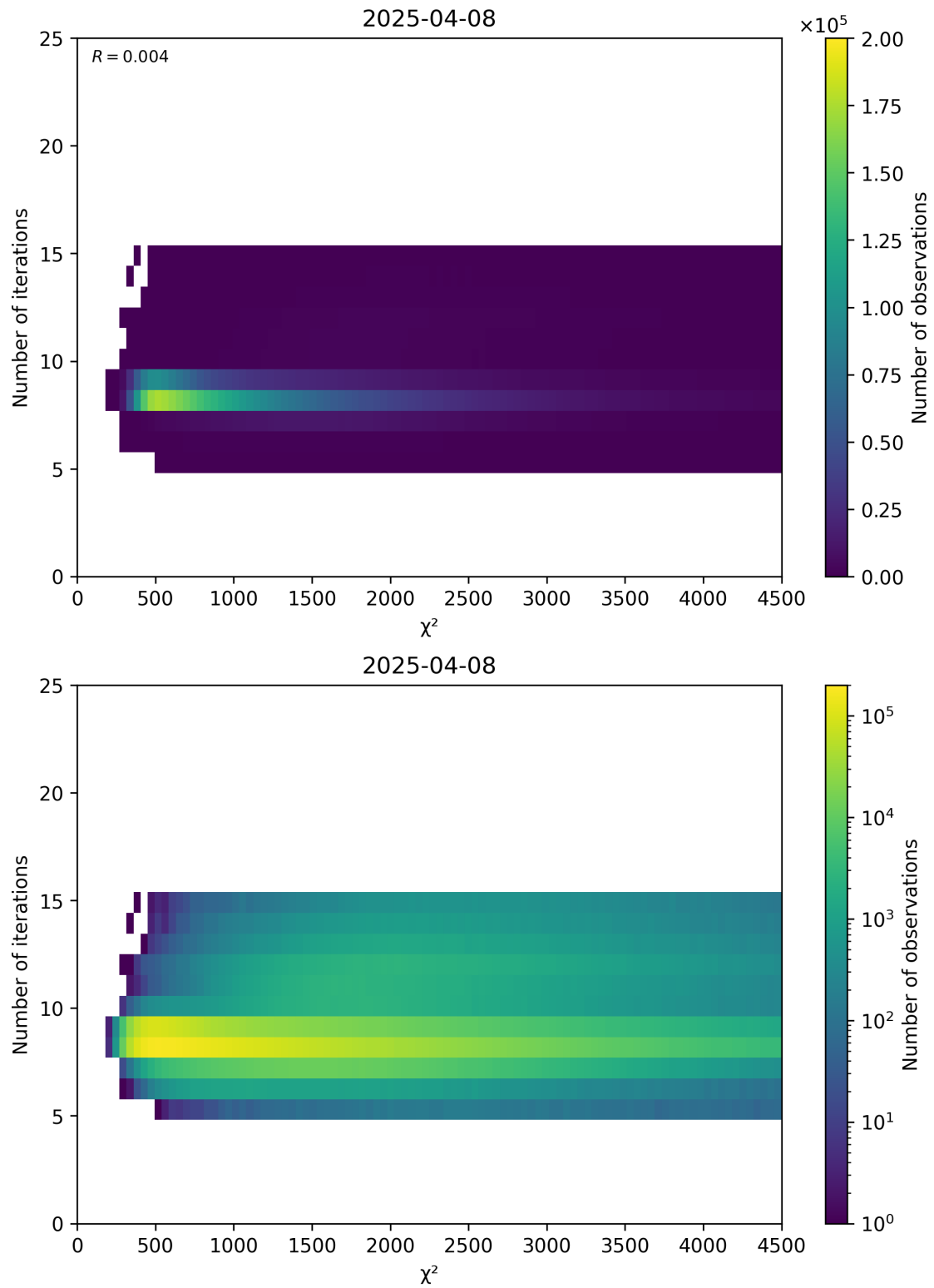
Figure 49: Scatter density plot of “ \chi^2 ” against “Number of iterations” for 2025-04-08 to 2025-04-09.
