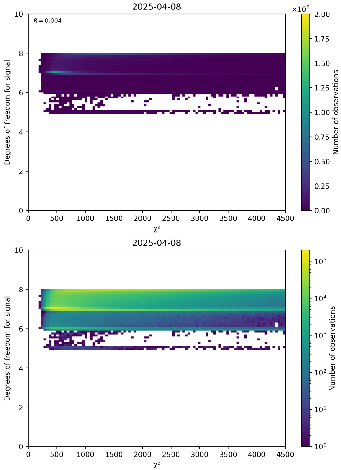
Figure 48: Scatter density plot of “ \chi^2 ” against “Degrees of freedom for signal” for 2025-04-08 to 2025-04-09.
