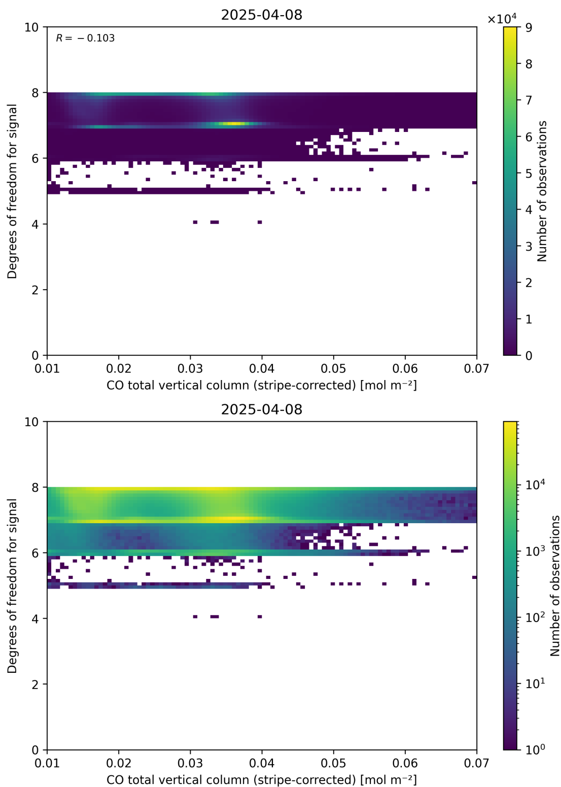
Figure 38: Scatter density plot of “CO total vertical column (stripe-corrected)” against “Degrees of freedom for signal” for 2025-04-08 to 2025-04-09.
