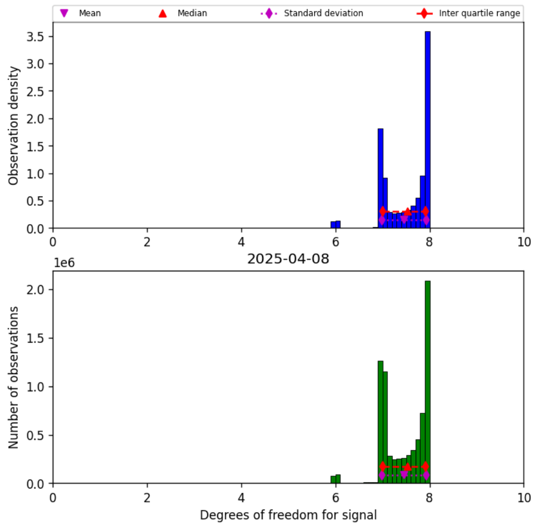
Figure 23: Histogram of “Degrees of freedom for signal” for 2025-04-08 to 2025-04-09
