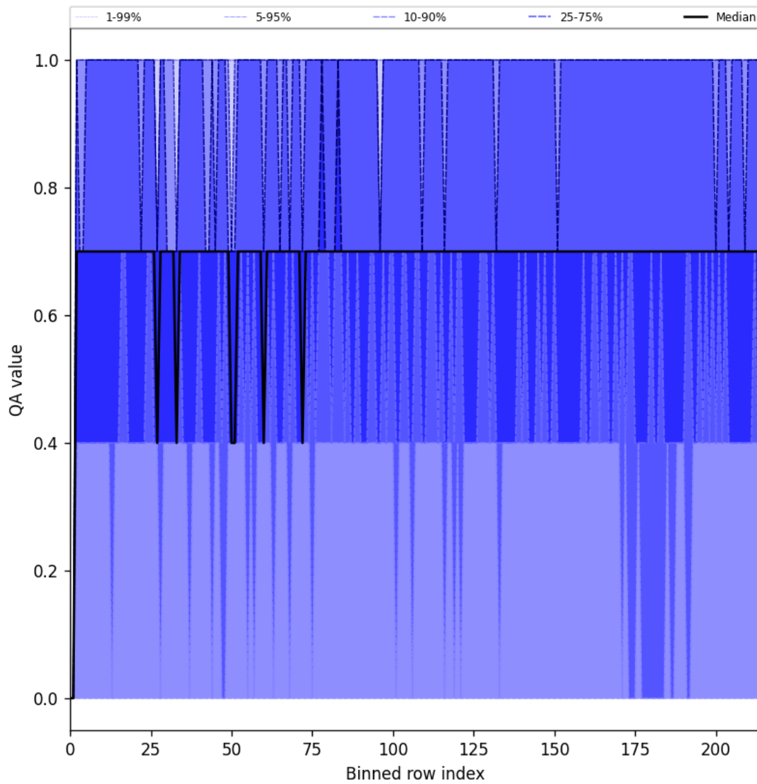
Figure 25: Along track statistics of “QA value” for 2025-04-08 to 2025-04-09
