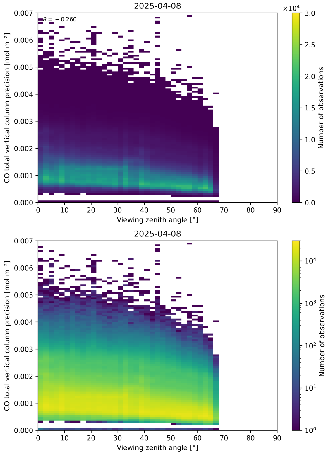
Figure 71: Scatter density plot of “Viewing zenith angle” against “CO total vertical column precision” for 2025-04-08 to 2025-04-09.
