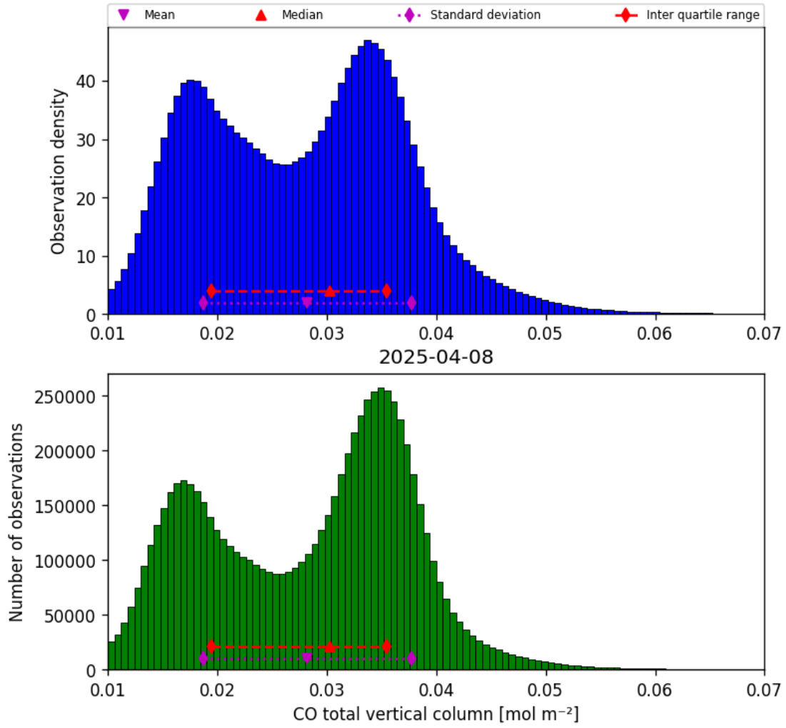
Figure 18: Histogram of “CO total vertical column” for 2025-04-08 to 2025-04-09
