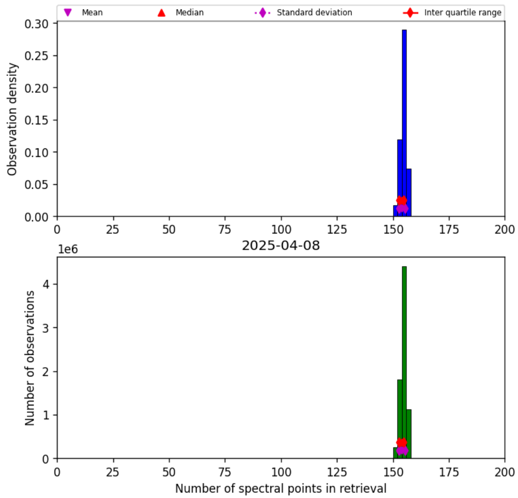
Figure 21: Histogram of “Number of spectral points in retrieval” for 2025-04-08 to 2025-04-09
