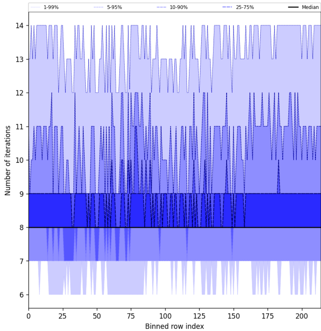
Figure 32: Along track statistics of “Number of iterations” for 2025-04-08 to 2025-04-09
