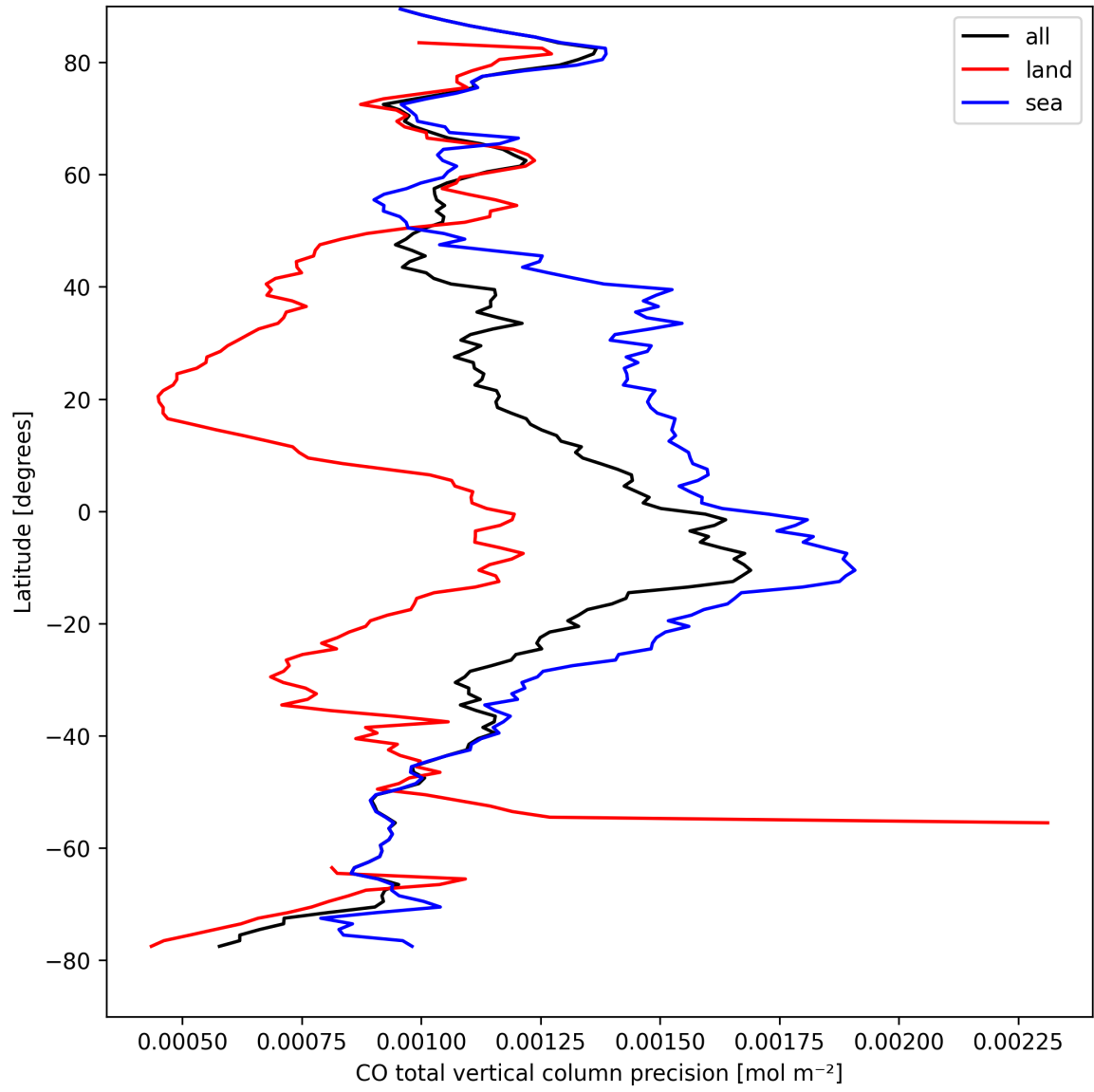
Figure 12: Zonal average of “CO total vertical column precision” for 2025-04-08 to 2025-04-09.
