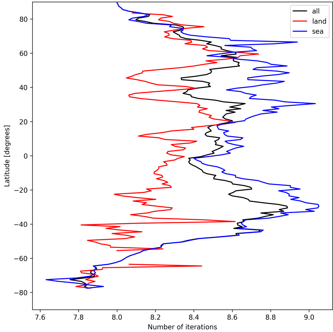
Figure 16: Zonal average of “Number of iterations” for 2025-04-08 to 2025-04-09.
