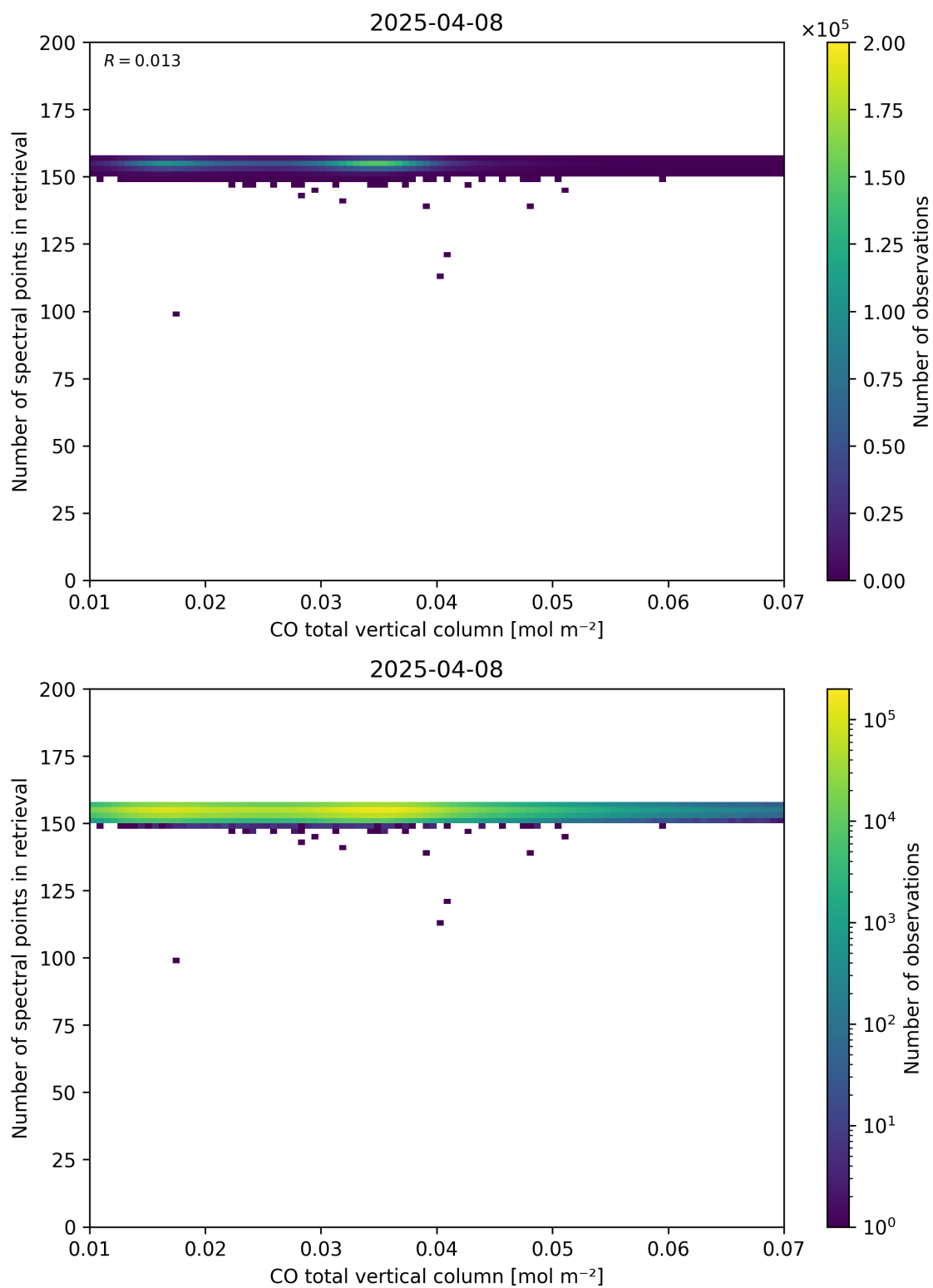
Figure 43: Scatter density plot of “CO total vertical column” against “Number of spectral points in retrieval” for 2025-04-08 to 2025-04-09.
