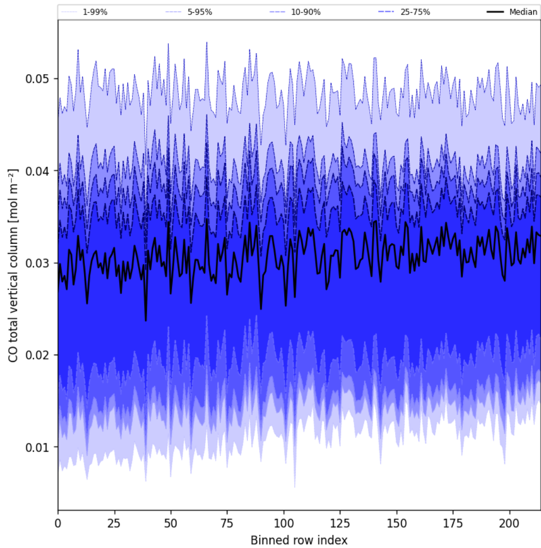
Figure 26: Along track statistics of “CO total vertical column” for 2025-04-08 to 2025-04-09
