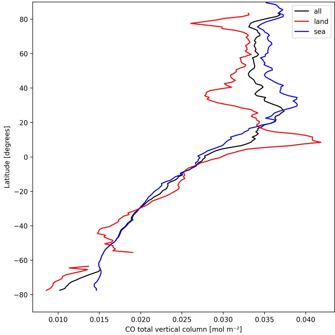
Figure 10: Zonal average of “CO total vertical column” for 2025-04-08 to 2025-04-09.
