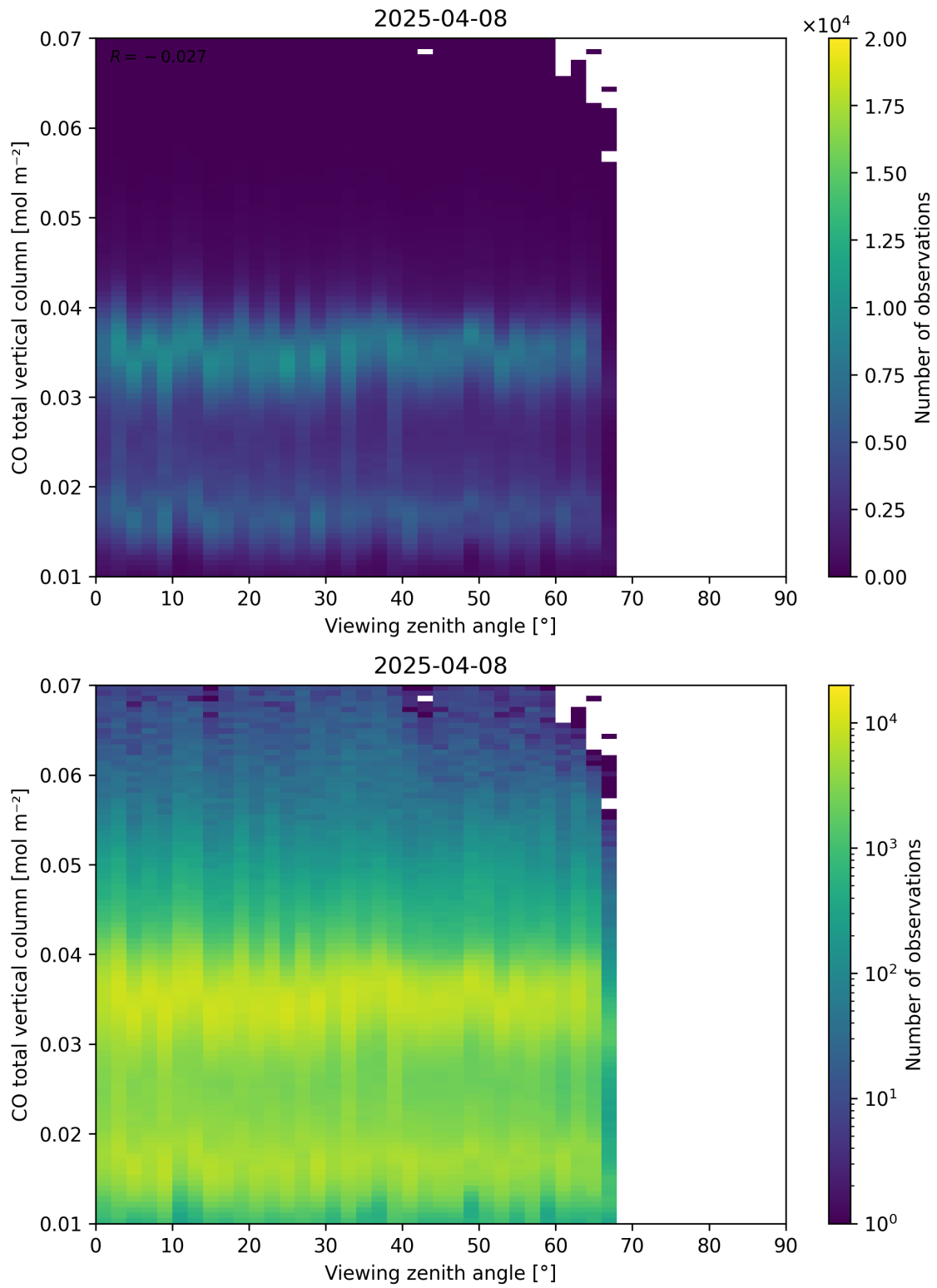
Figure 69: Scatter density plot of “Viewing zenith angle” against “CO total vertical column” for 2025-04-08 to 2025-04-09.
