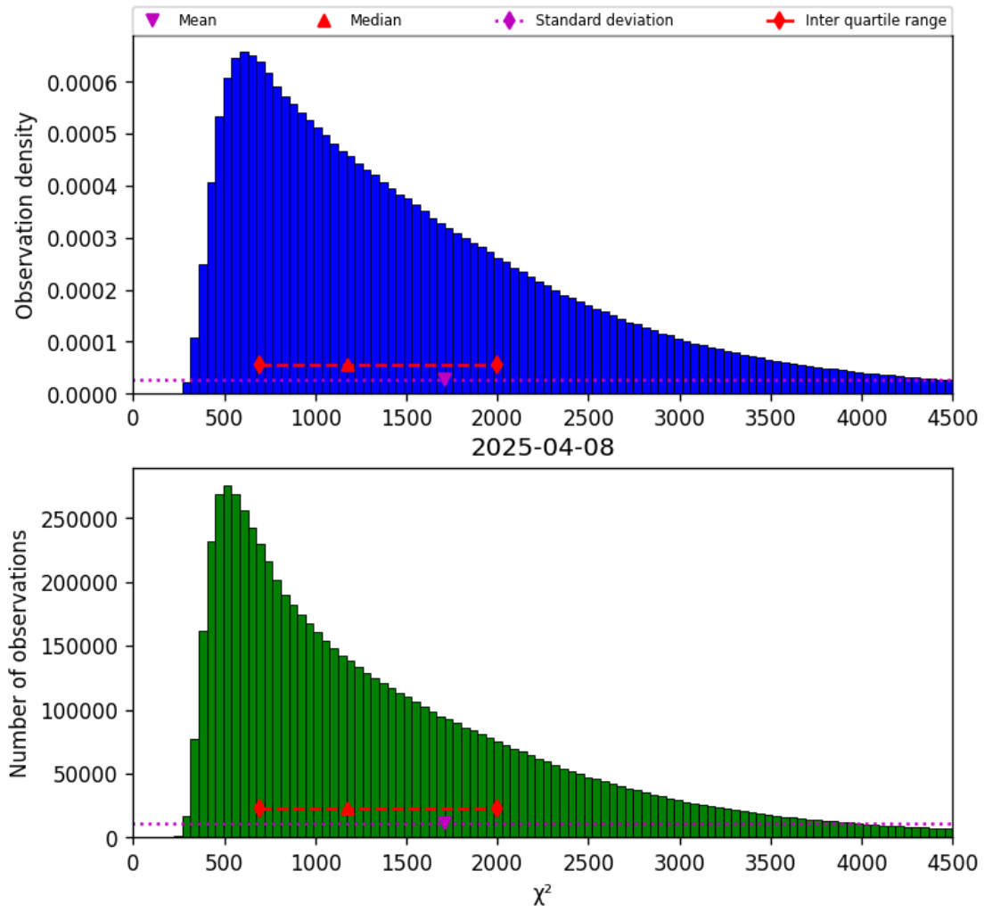
Figure 22: Histogram of “ \chi^2 ” for 2025-04-08 to 2025-04-09
