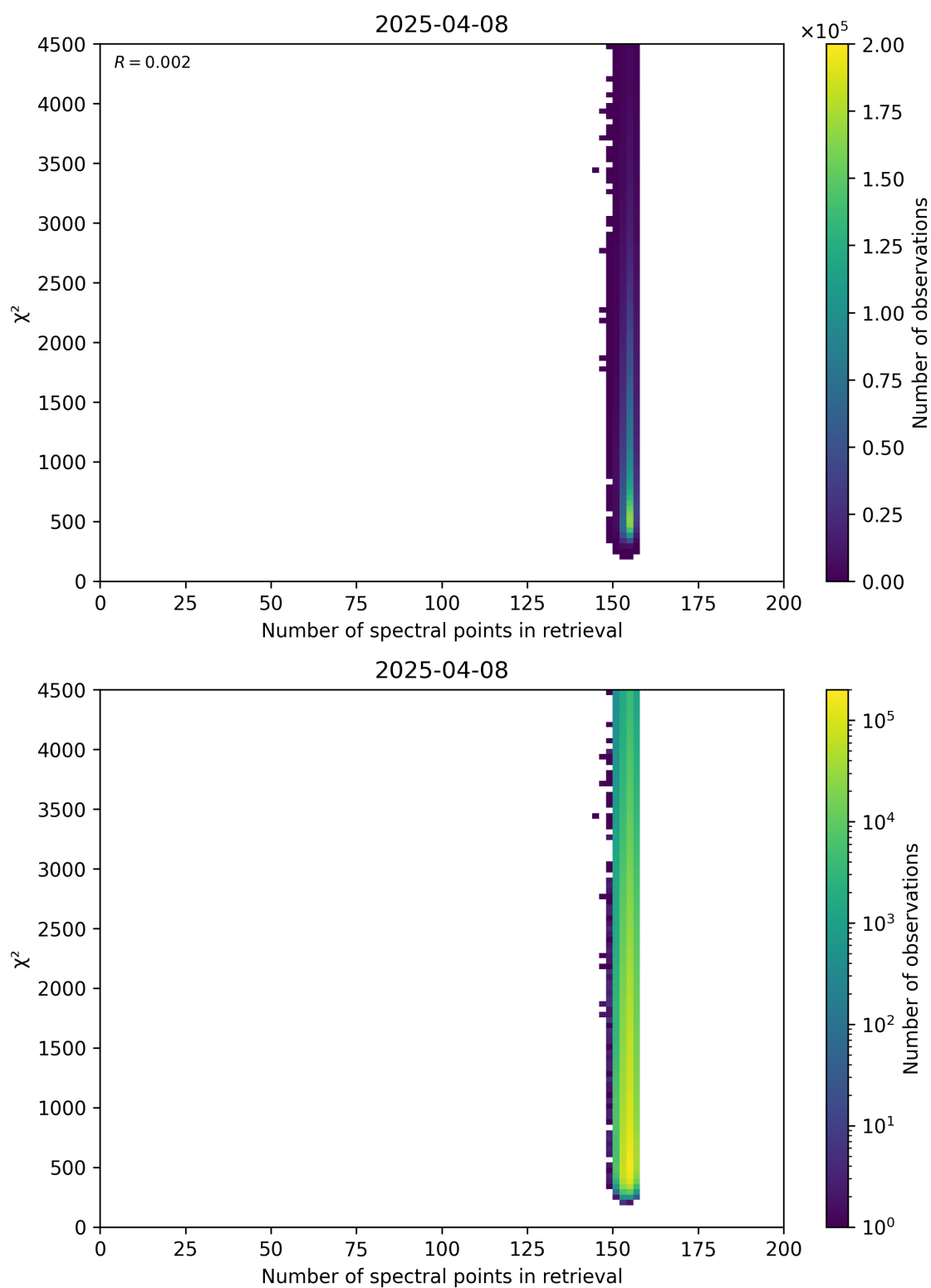
Figure 58: Scatter density plot of “Number of spectral points in retrieval” against “ \chi^2 ” for 2025-04-08 to 2025-04-09.
