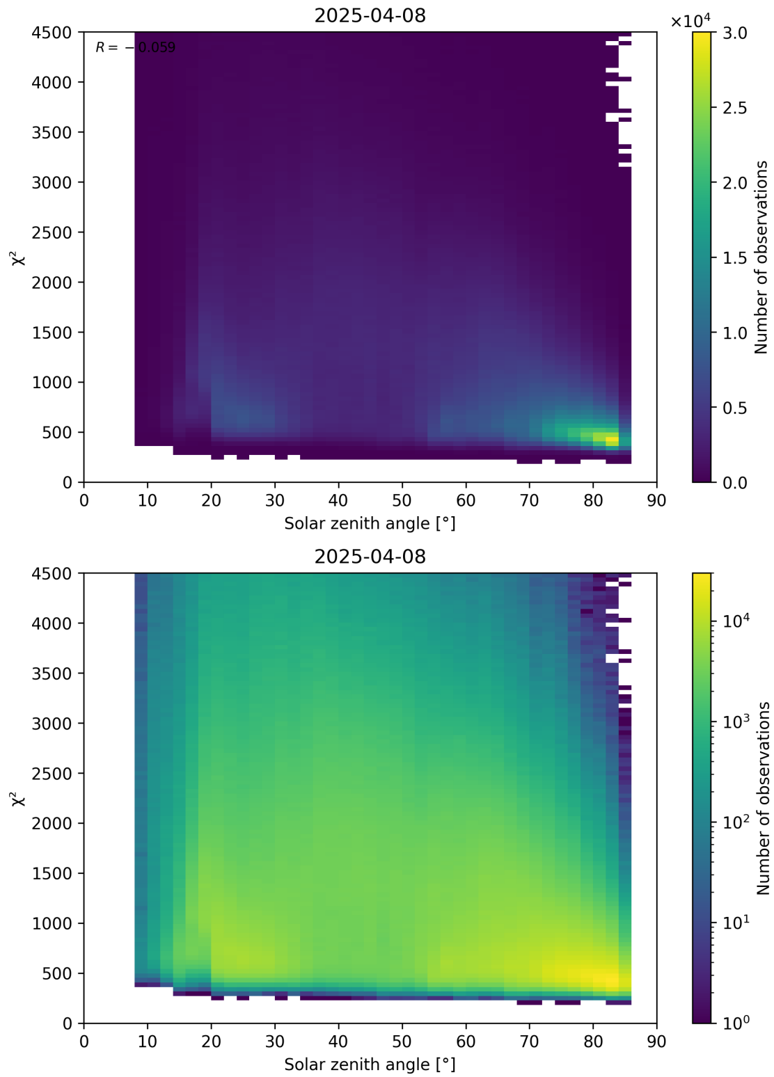
Figure 64: Scatter density plot of “Solar zenith angle” against “ \chi^2 ” for 2025-04-08 to 2025-04-09.
