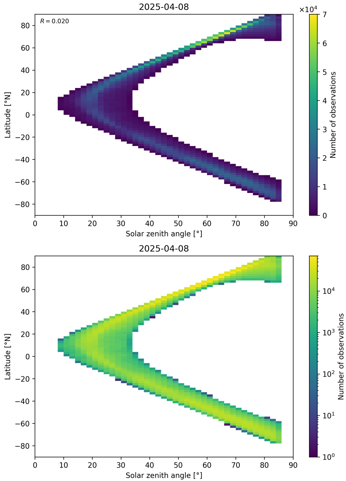
Figure 66: Scatter density plot of “Solar zenith angle” against “Latitude” for 2025-04-08 to 2025-04-09.
