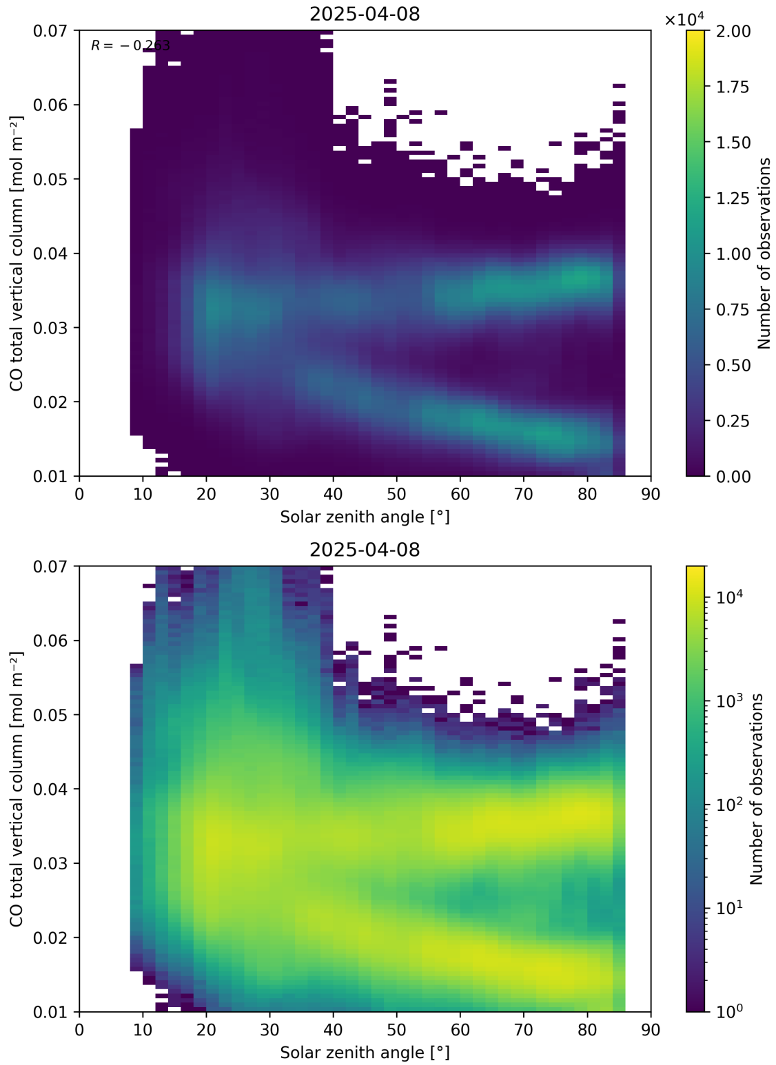
Figure 61: Scatter density plot of “Solar zenith angle” against “CO total vertical column” for 2025-04-08 to 2025-04-09.
