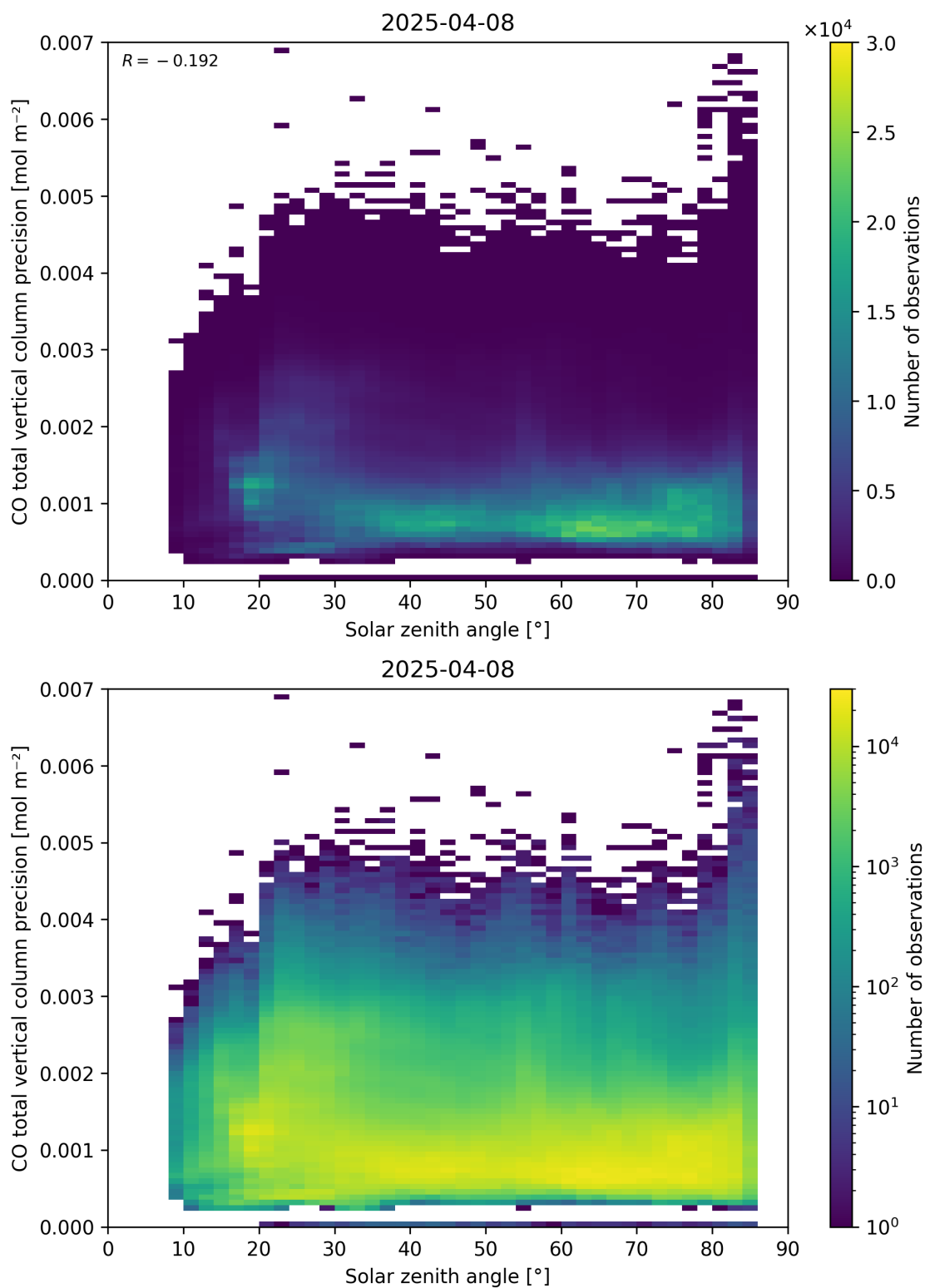
Figure 63: Scatter density plot of “Solar zenith angle” against “CO total vertical column precision” for 2025-04-08 to 2025-04-09.
