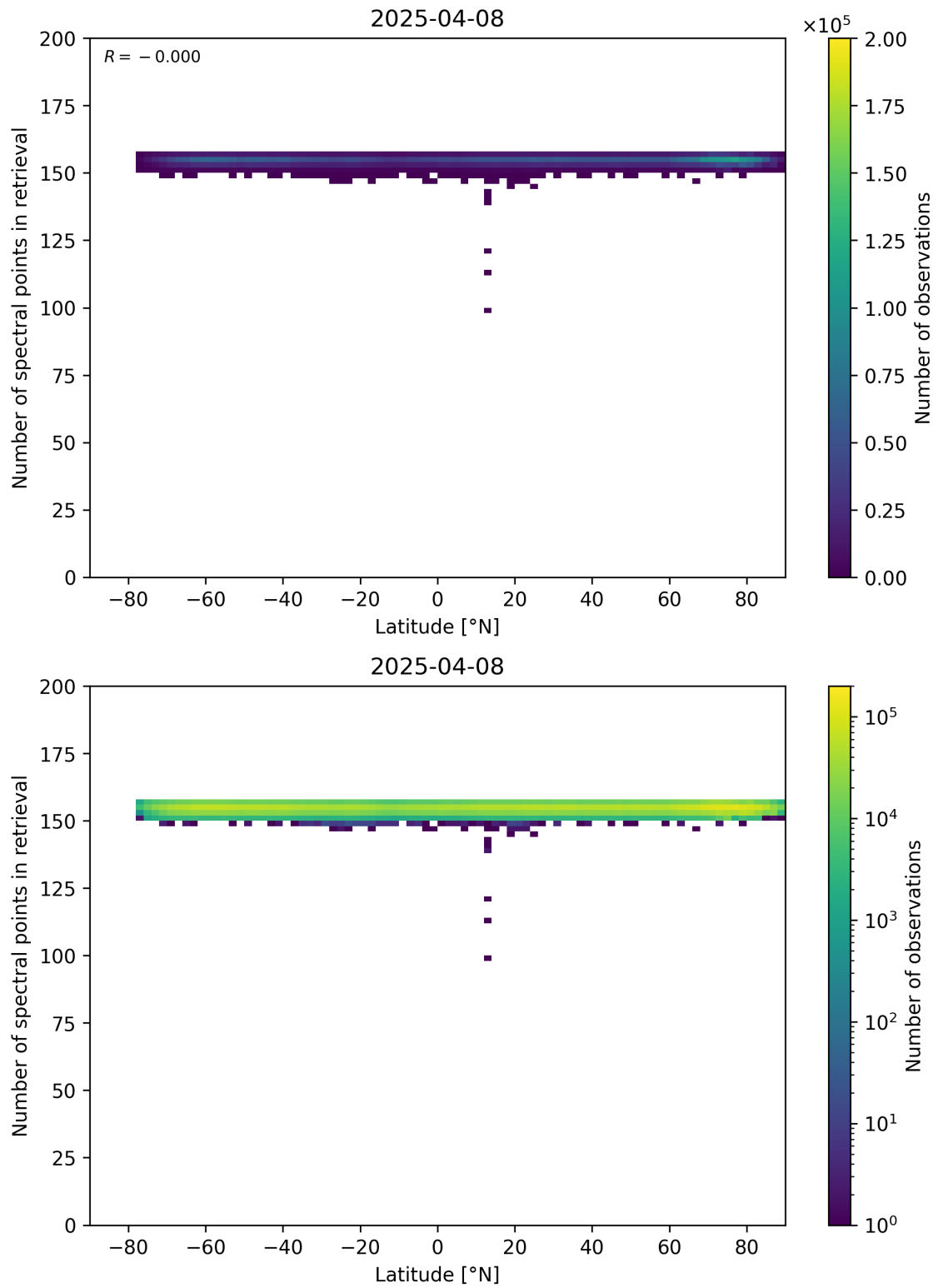
Figure 57: Scatter density plot of “Latitude” against “Number of spectral points in retrieval” for 2025-04-08 to 2025-04-09.
