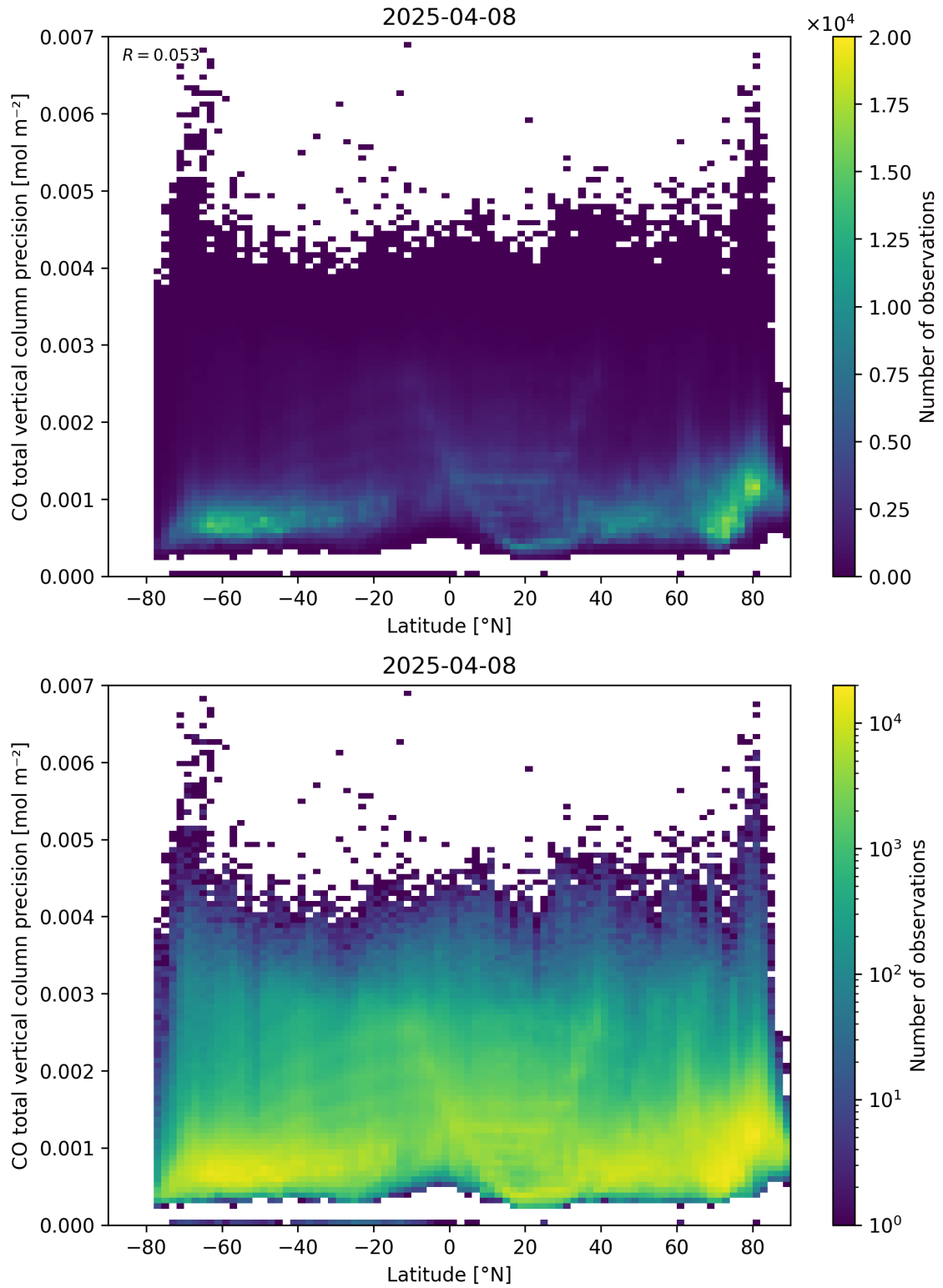
Figure 53: Scatter density plot of “Latitude” against “CO total vertical column precision” for 2025-04-08 to 2025-04-09.
