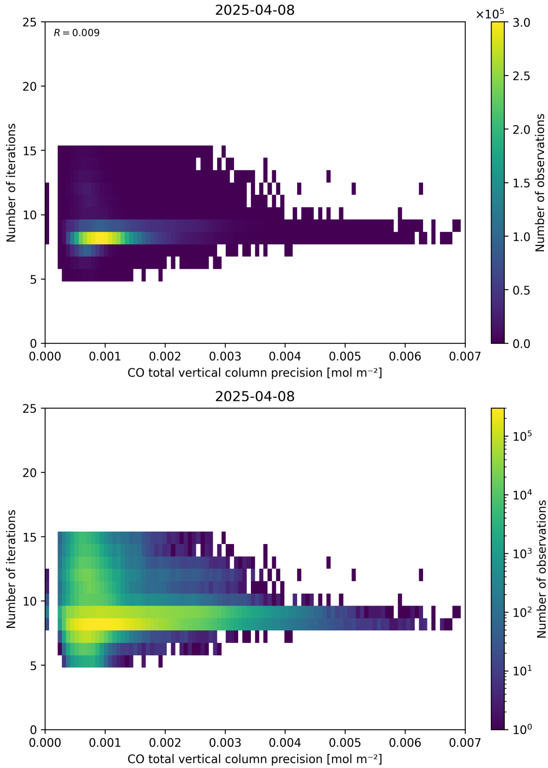
Figure 46: Scatter density plot of “CO total vertical column precision” against “Number of iterations” for 2025-04-08 to 2025-04-09.
