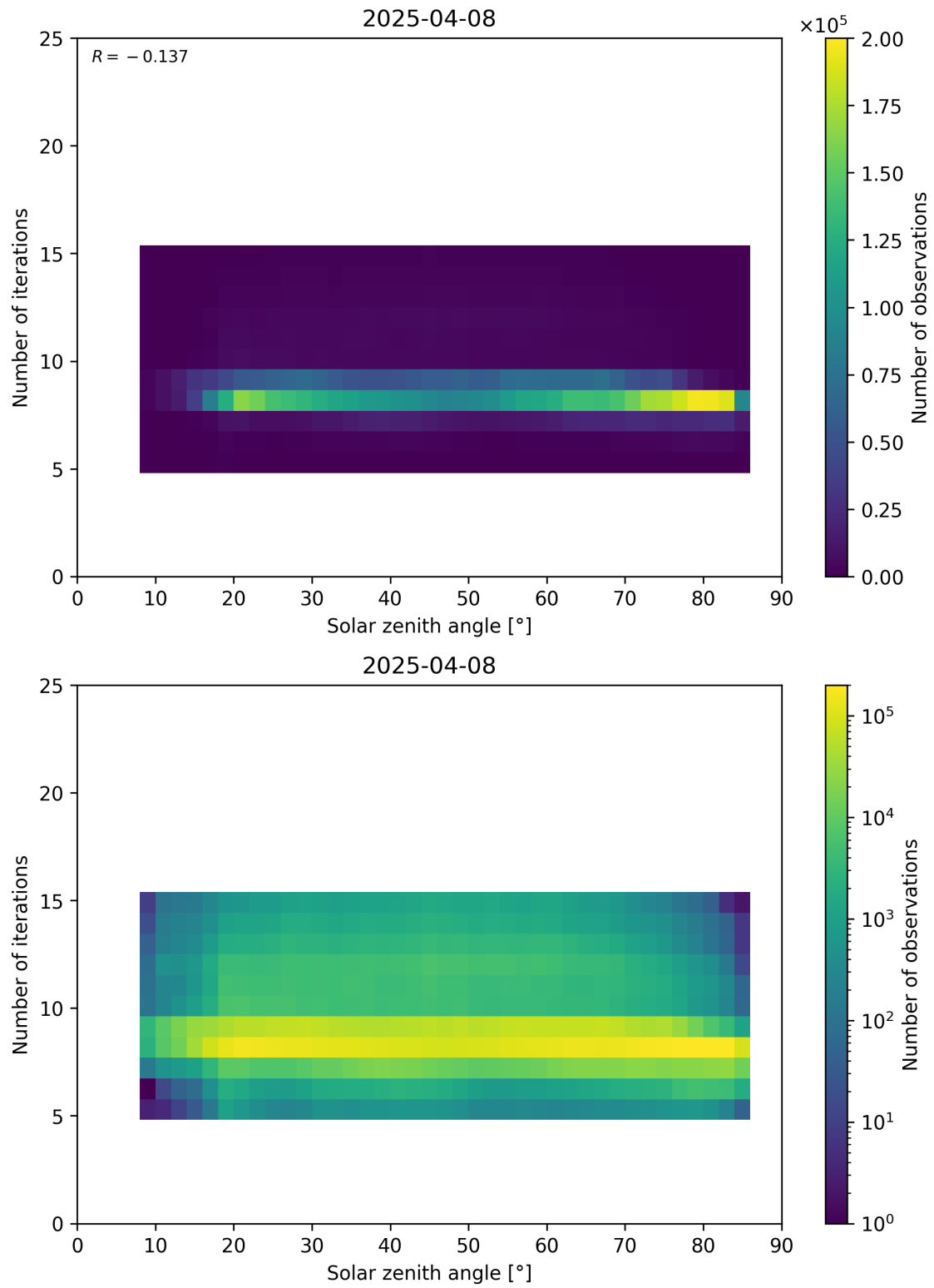
Figure 67: Scatter density plot of “Solar zenith angle” against “Number of iterations” for 2025-04-08 to 2025-04-09.
