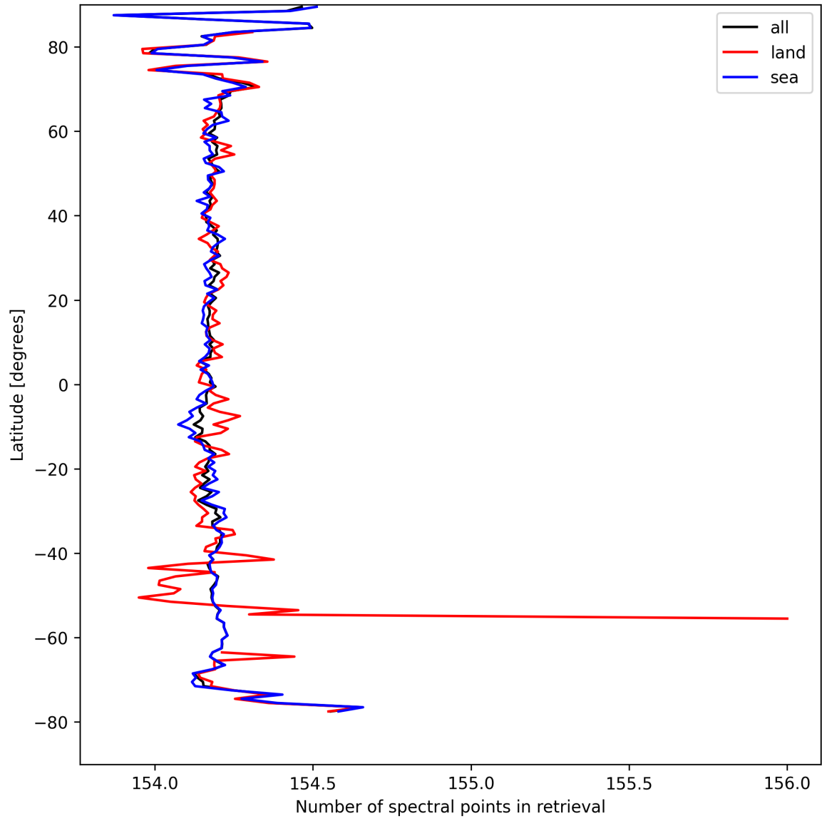
Figure 13: Zonal average of “Number of spectral points in retrieval” for 2025-04-08 to 2025-04-09.
