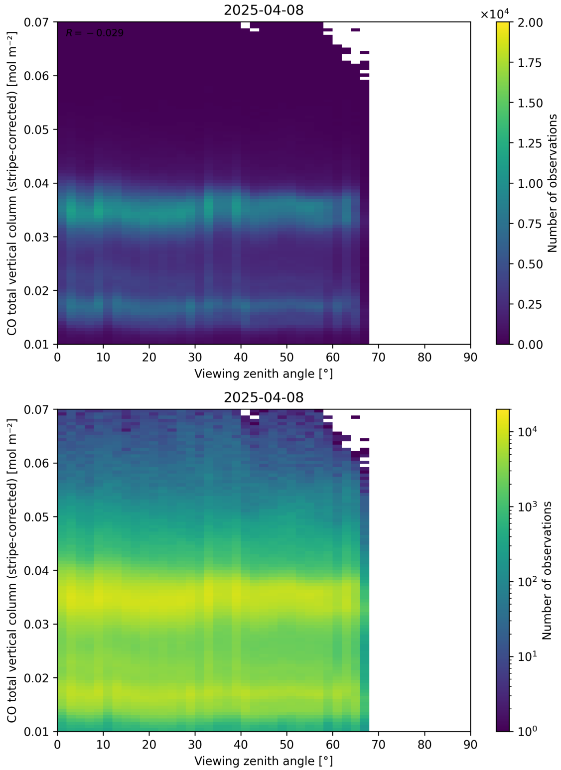
Figure 70: Scatter density plot of “Viewing zenith angle” against “CO total vertical column (stripe-corrected)” for 2025-04-08 to 2025-04-09.
