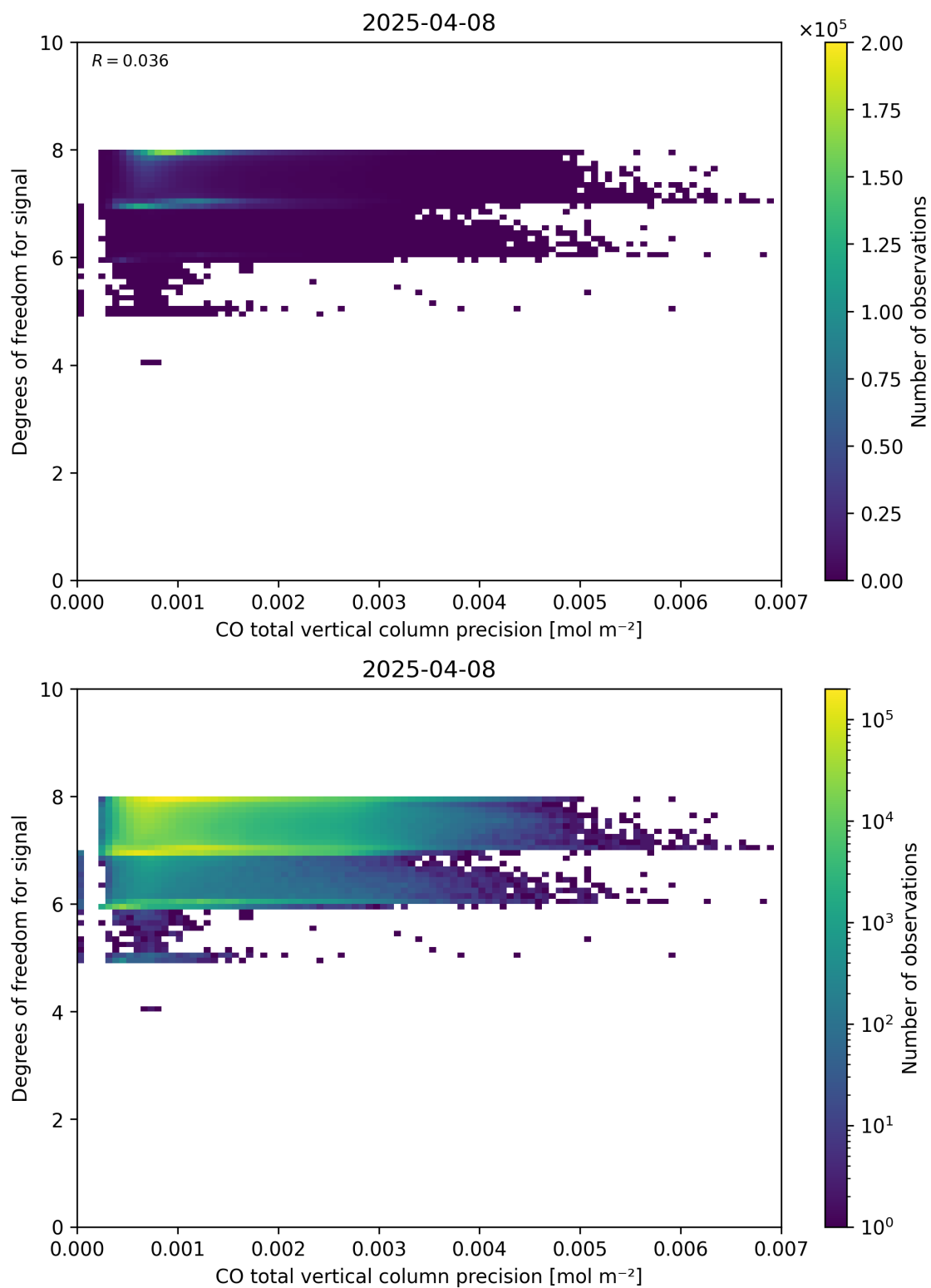
Figure 45: Scatter density plot of “CO total vertical column precision” against “Degrees of freedom for signal” for 2025-04-08 to 2025-04-09.
