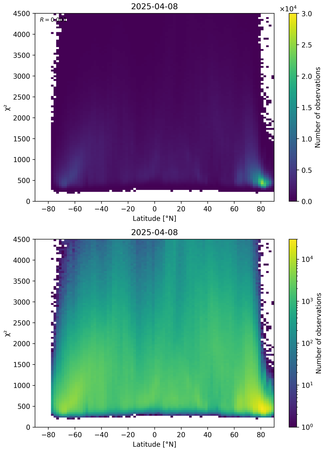
Figure 54: Scatter density plot of “Latitude” against “ \chi^2 ” for 2025-04-08 to 2025-04-09.
