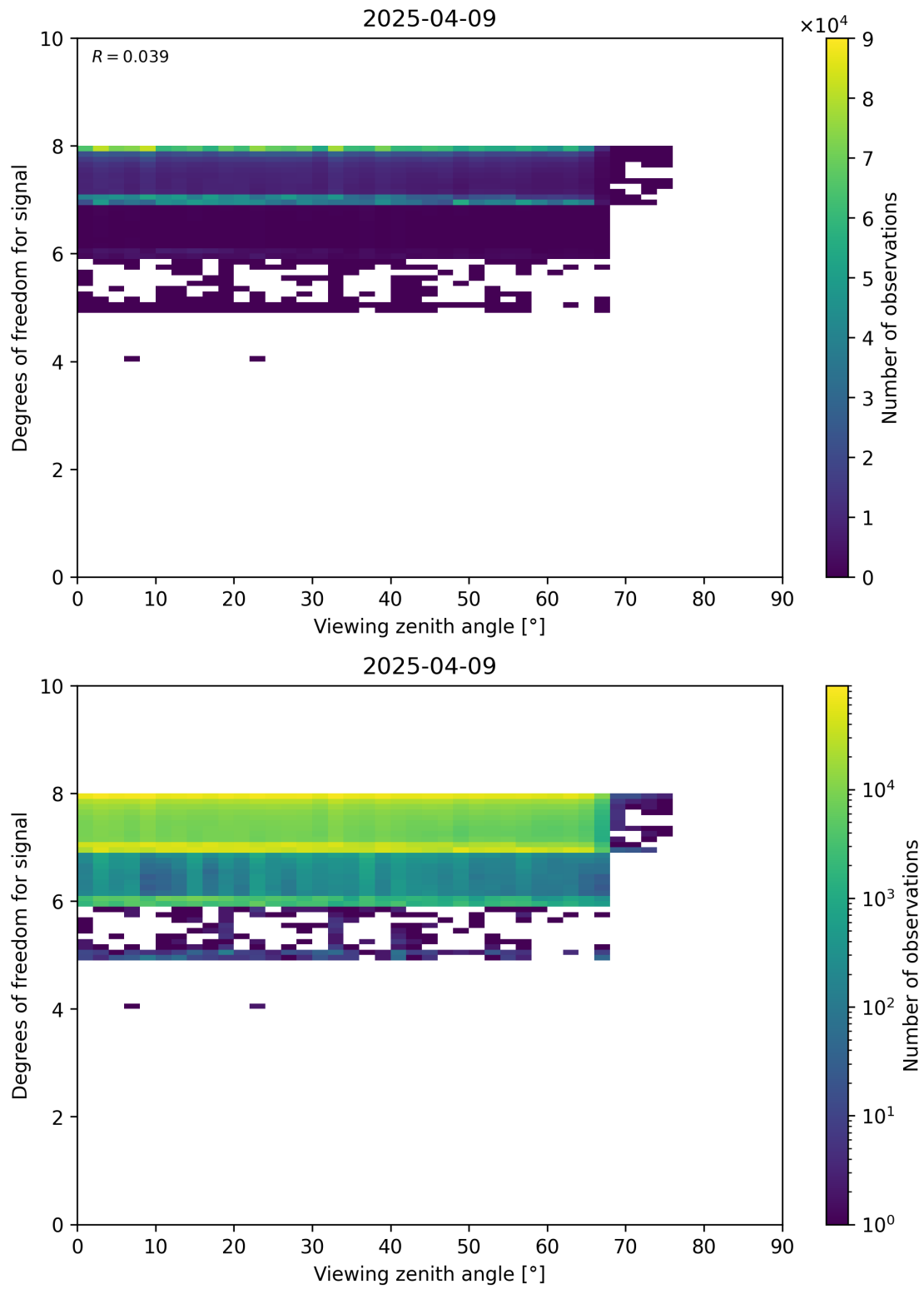
Figure 73: Scatter density plot of “Viewing zenith angle” against “Degrees of freedom for signal” for 2025-04-08 to 2025-04-10.
