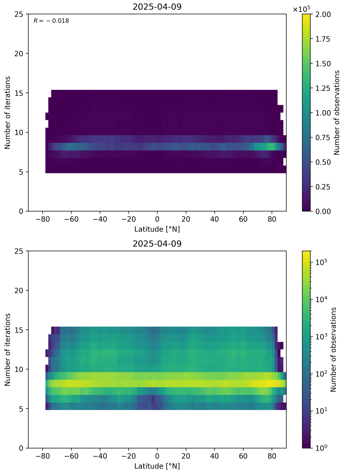
Figure 56: Scatter density plot of “Latitude” against “Number of iterations” for 2025-04-08 to 2025-04-10.
