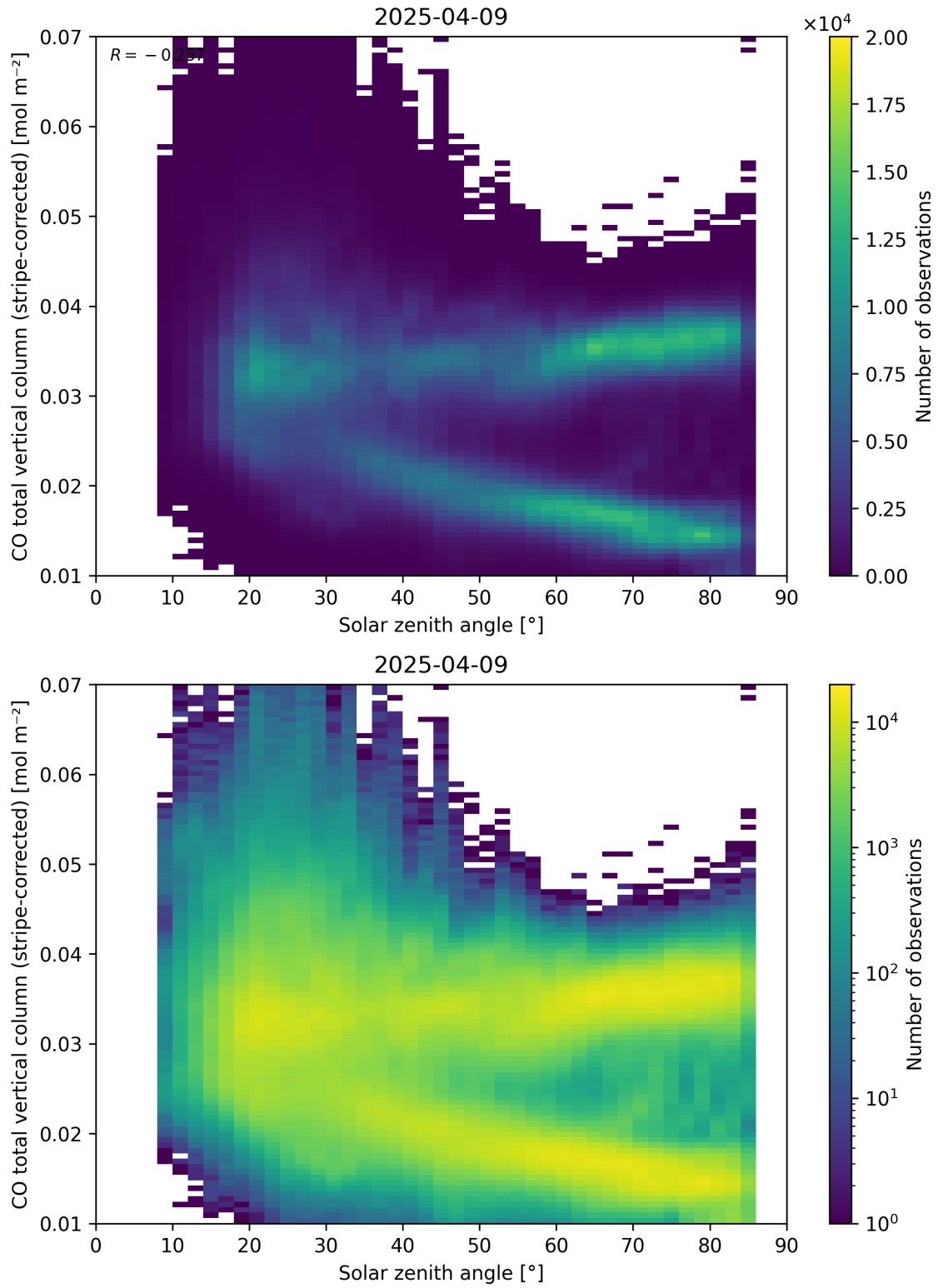
Figure 62: Scatter density plot of “Solar zenith angle” against “CO total vertical column (stripe-corrected)” for 2025-04-08 to 2025-04-10.
