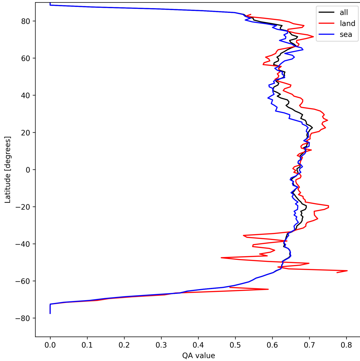
Figure 9: Zonal average of “QA value” for 2025-04-08 to 2025-04-10.
