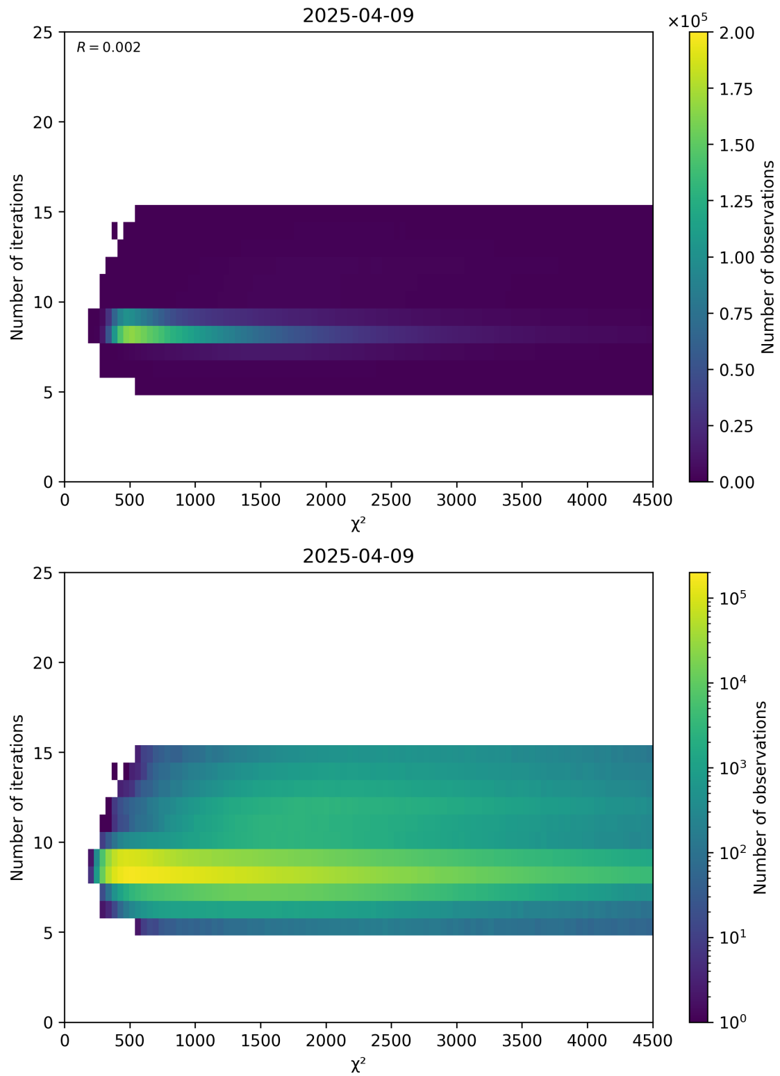
Figure 49: Scatter density plot of “ \chi^2 ” against “Number of iterations” for 2025-04-08 to 2025-04-10.
