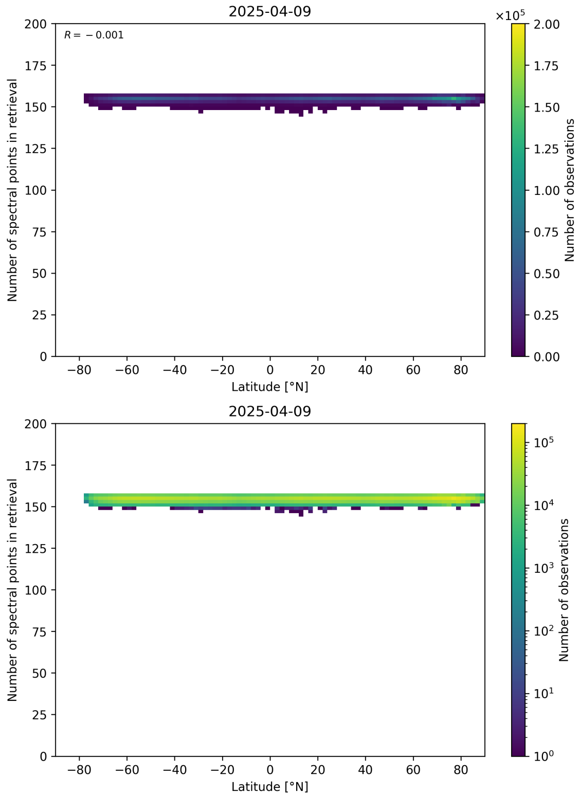
Figure 57: Scatter density plot of “Latitude” against “Number of spectral points in retrieval” for 2025-04-08 to 2025-04-10.
