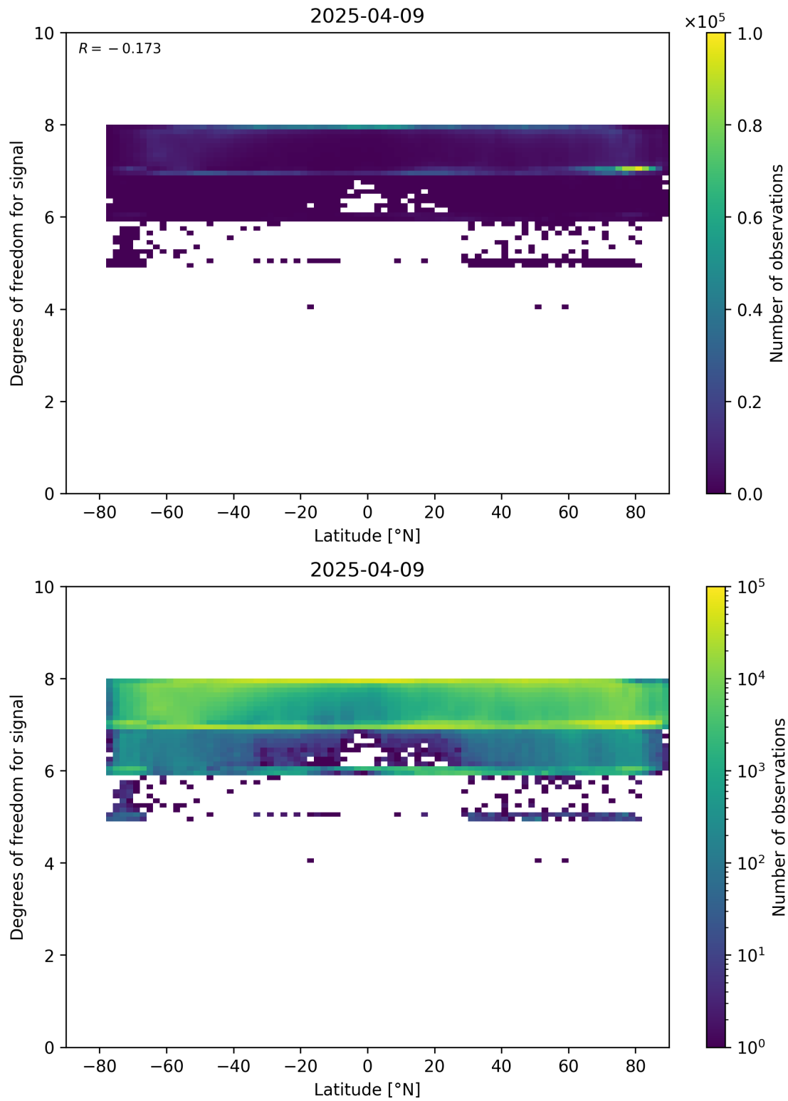
Figure 55: Scatter density plot of “Latitude” against “Degrees of freedom for signal” for 2025-04-08 to 2025-04-10.
