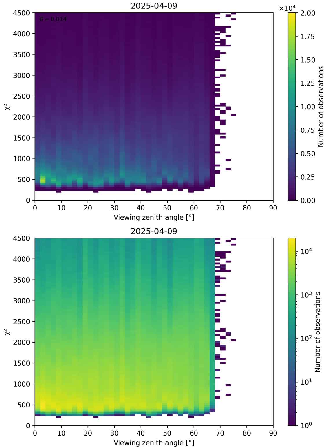
Figure 72: Scatter density plot of “Viewing zenith angle” against “ \chi^2 ” for 2025-04-08 to 2025-04-10.
