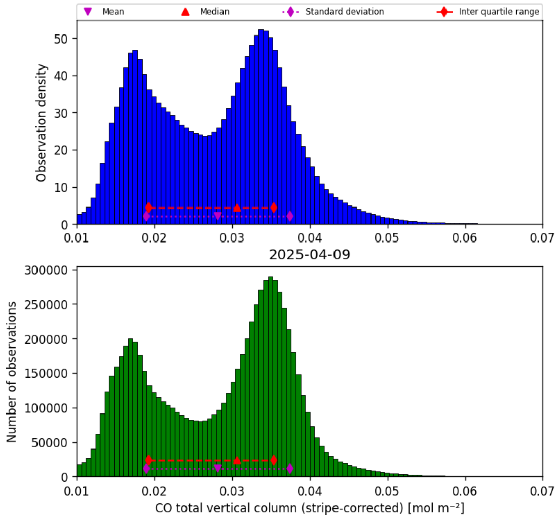
Figure 19: Histogram of “CO total vertical column (stripe-corrected)” for 2025-04-08 to 2025-04-10
