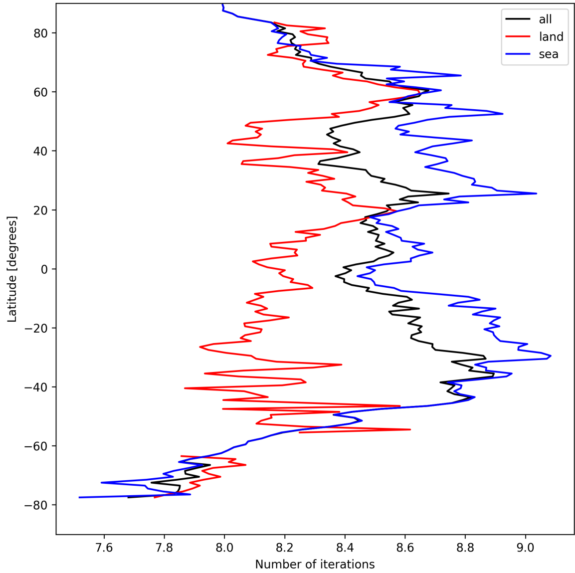
Figure 16: Zonal average of “Number of iterations” for 2025-04-08 to 2025-04-10.
