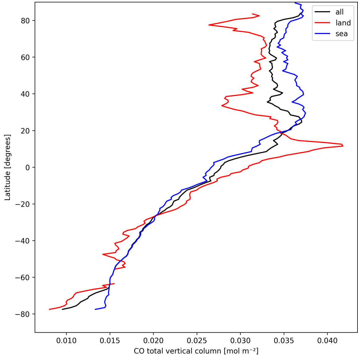
Figure 10: Zonal average of “CO total vertical column” for 2025-04-08 to 2025-04-10.
