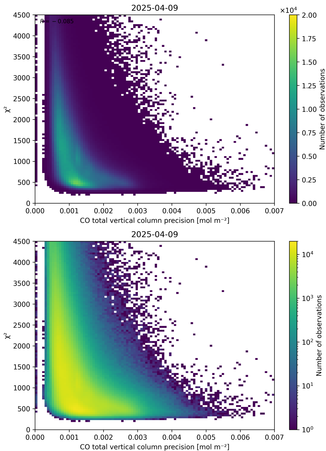
Figure 44: Scatter density plot of “CO total vertical column precision” against “ \chi^2 ” for 2025-04-08 to 2025-04-10.
