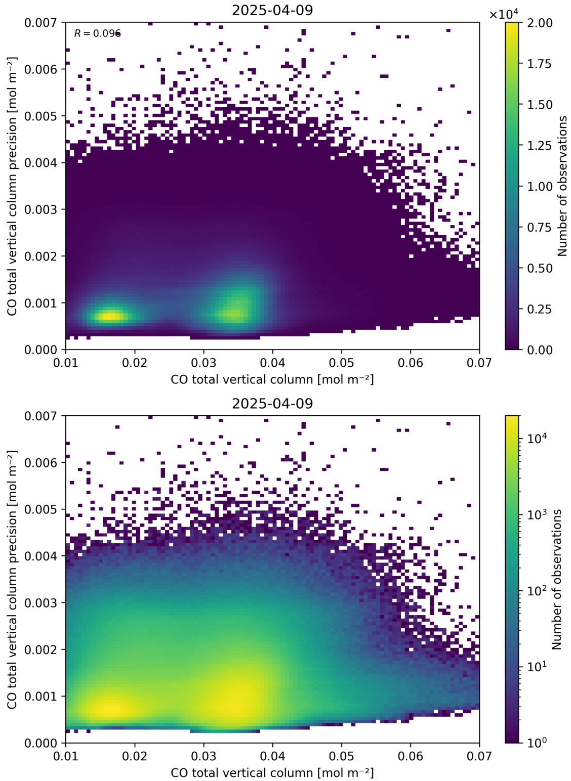
Figure 34: Scatter density plot of “CO total vertical column” against “CO total vertical column precision” for 2025-04-08 to 2025-04-10.
