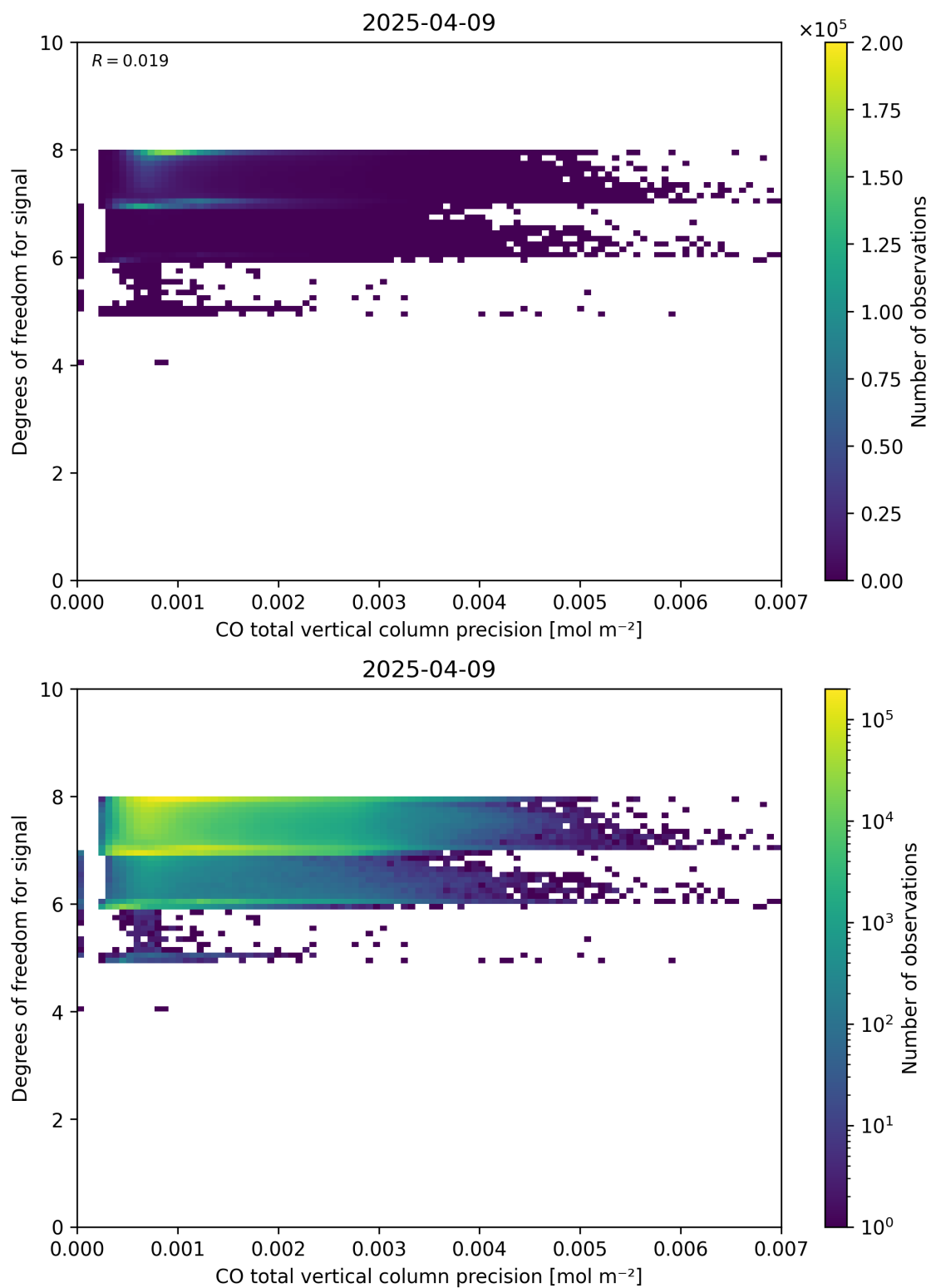
Figure 45: Scatter density plot of “CO total vertical column precision” against “Degrees of freedom for signal” for 2025-04-08 to 2025-04-10.
