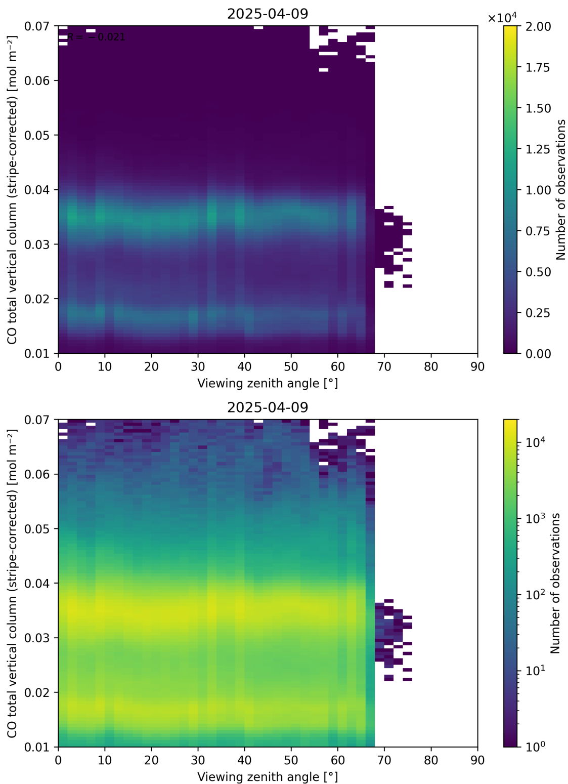
Figure 70: Scatter density plot of “Viewing zenith angle” against “CO total vertical column (stripe-corrected)” for 2025-04-08 to 2025-04-10.
