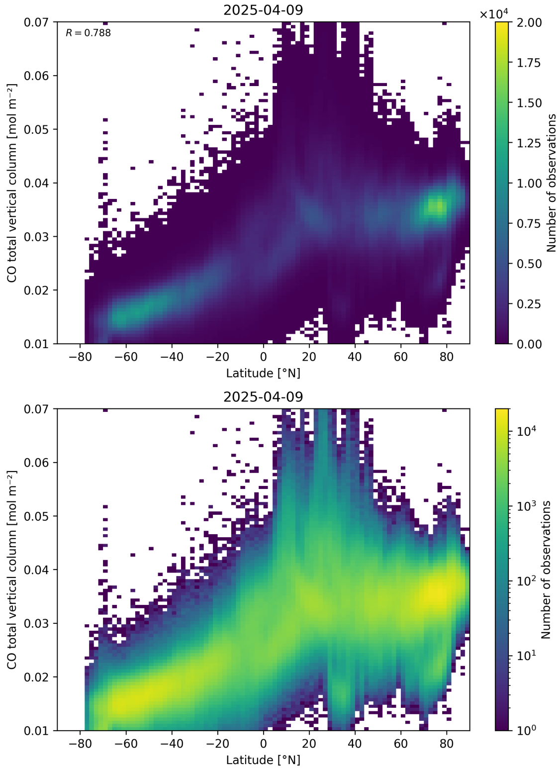
Figure 51: Scatter density plot of “Latitude” against “CO total vertical column” for 2025-04-08 to 2025-04-10.
