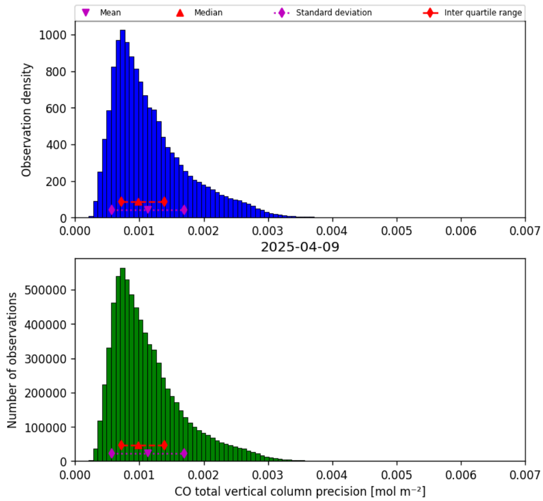
Figure 20: Histogram of “CO total vertical column precision” for 2025-04-08 to 2025-04-10
