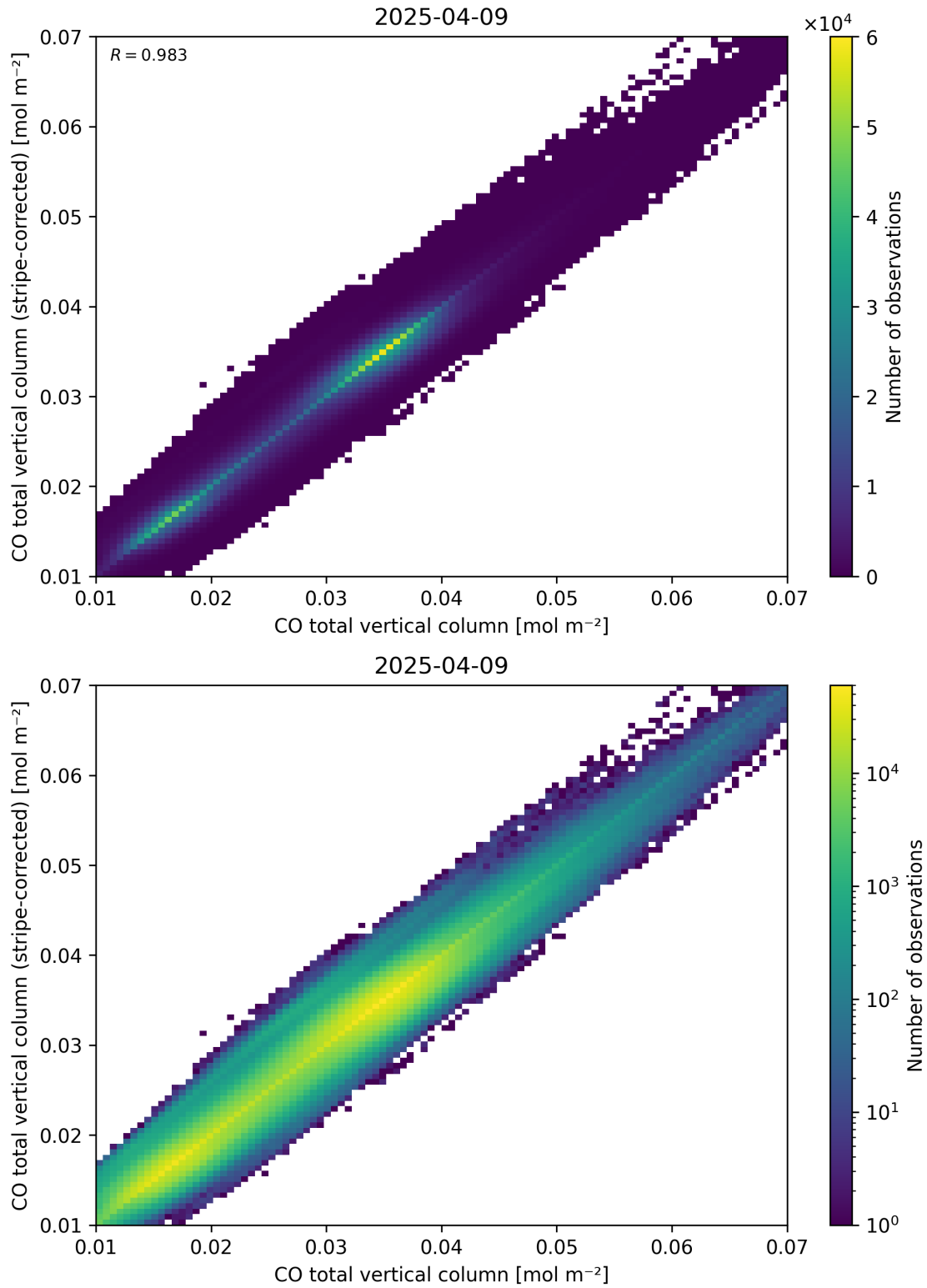
Figure 33: Scatter density plot of “CO total vertical column” against “CO total vertical column (stripe-corrected)” for 2025-04-08 to 2025-04-10.
