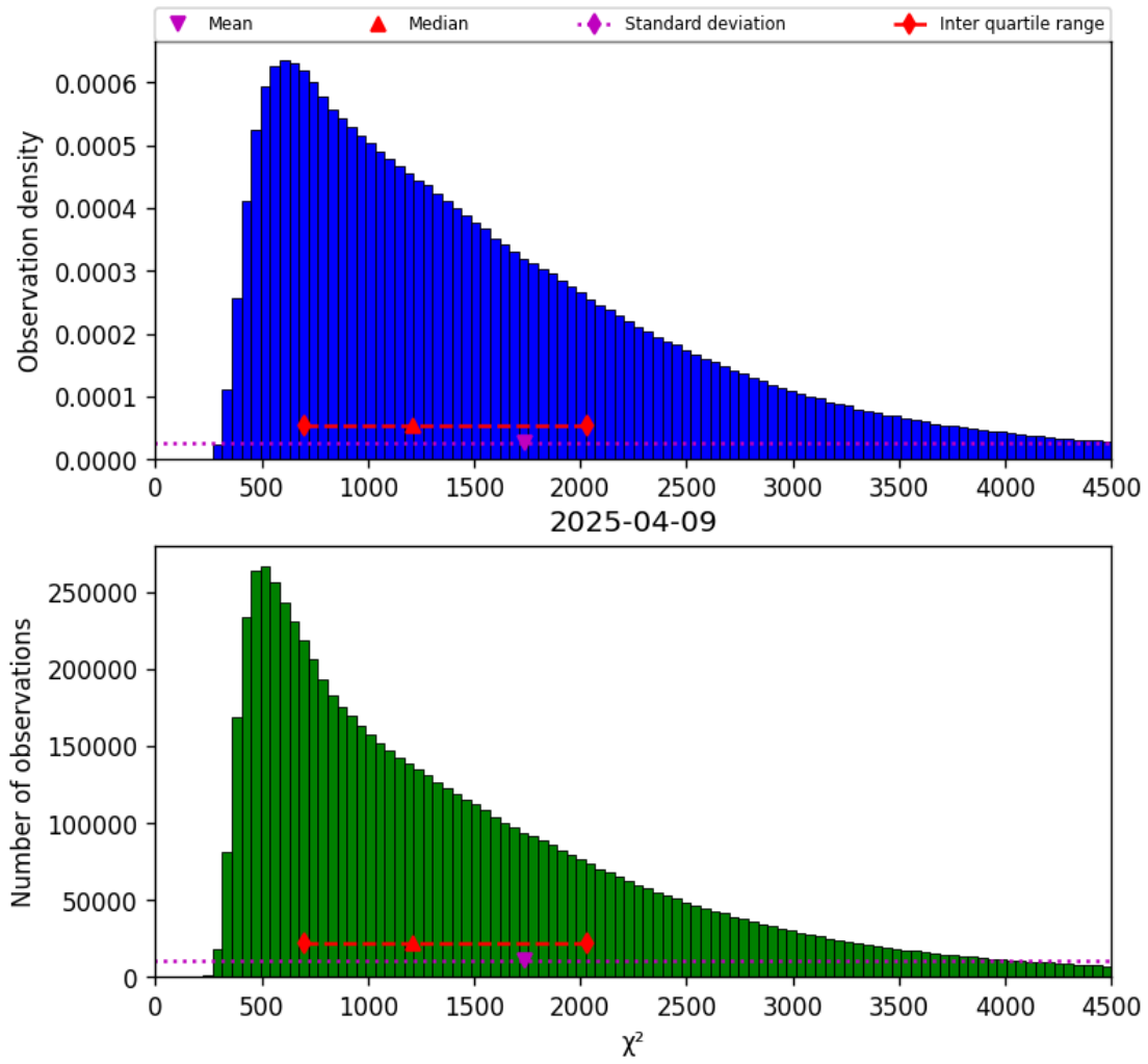
Figure 22: Histogram of “ \chi^2 ” for 2025-04-08 to 2025-04-10
