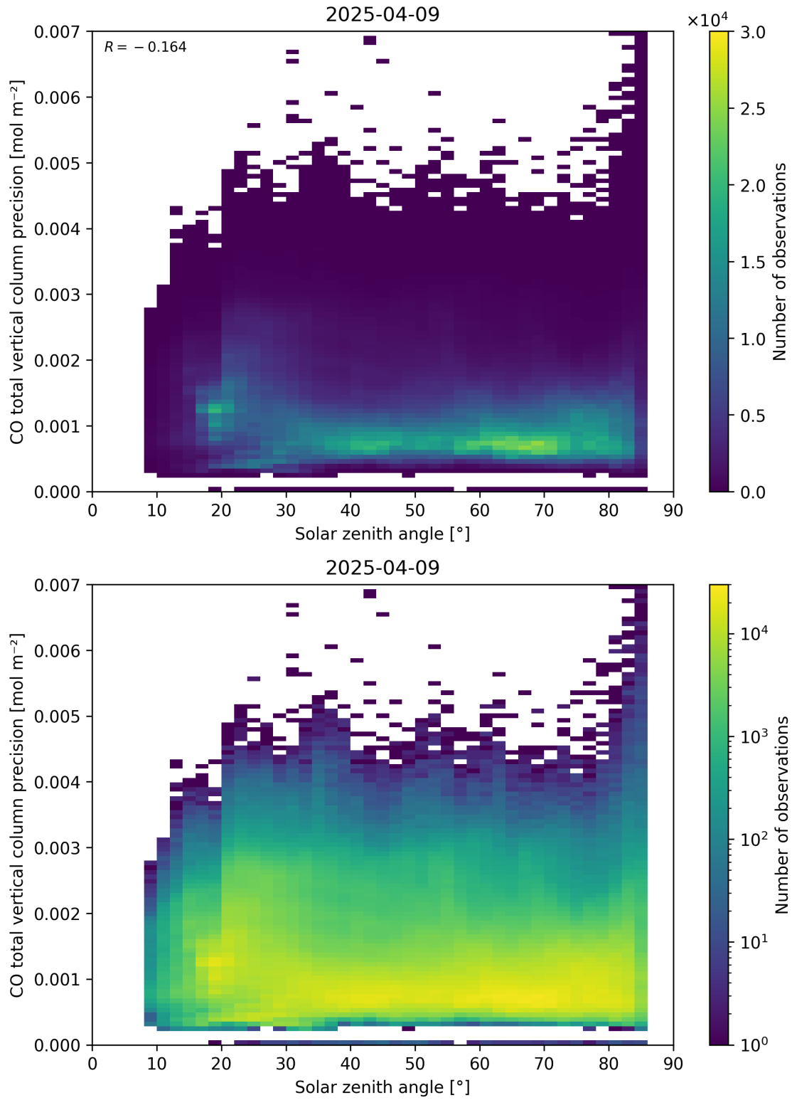
Figure 63: Scatter density plot of “Solar zenith angle” against “CO total vertical column precision” for 2025-04-08 to 2025-04-10.
