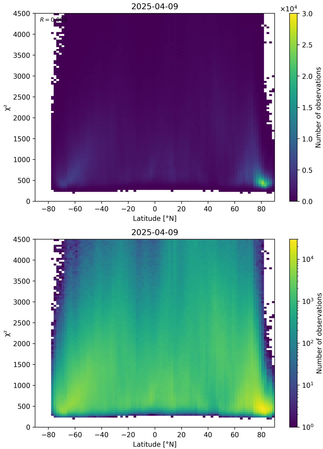
Figure 54: Scatter density plot of “Latitude” against “ \chi^2 ” for 2025-04-08 to 2025-04-10.
