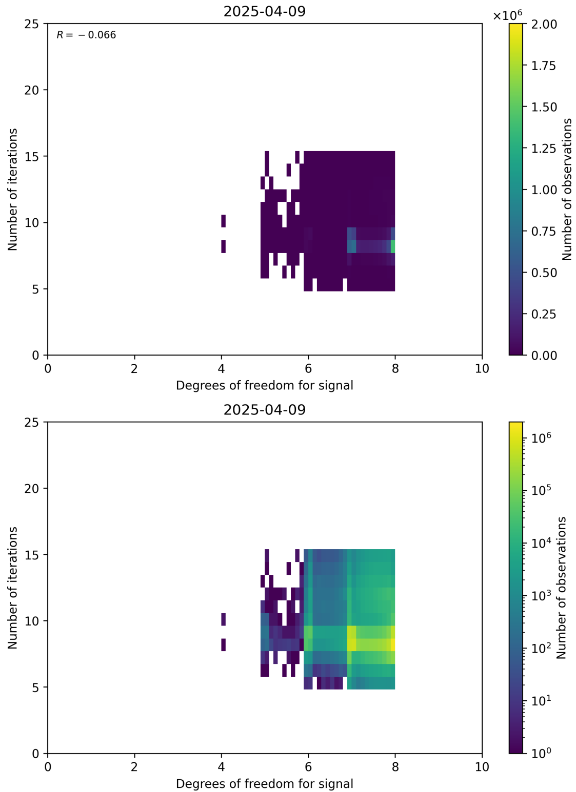
Figure 50: Scatter density plot of “Degrees of freedom for signal” against “Number of iterations” for 2025-04-08 to 2025-04-10.
