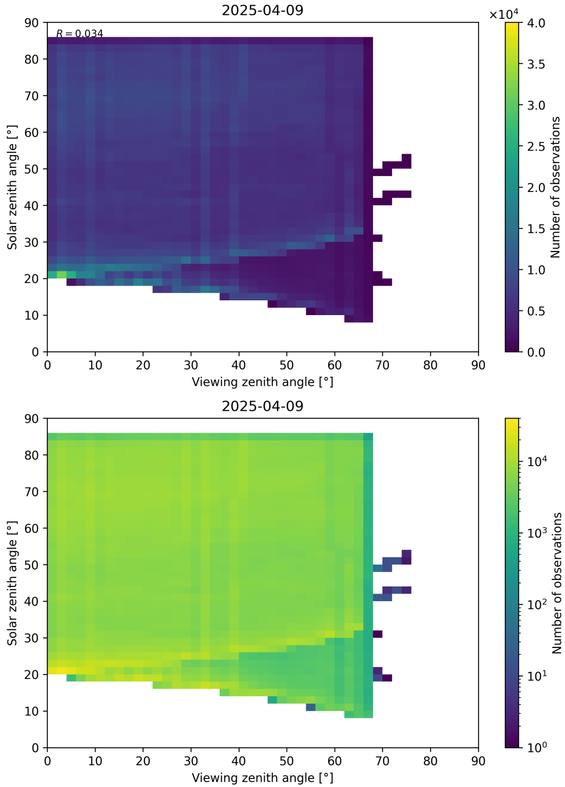
Figure 77: Scatter density plot of “Viewing zenith angle” against “Solar zenith angle” for 2025-04-08 to 2025-04-10.
