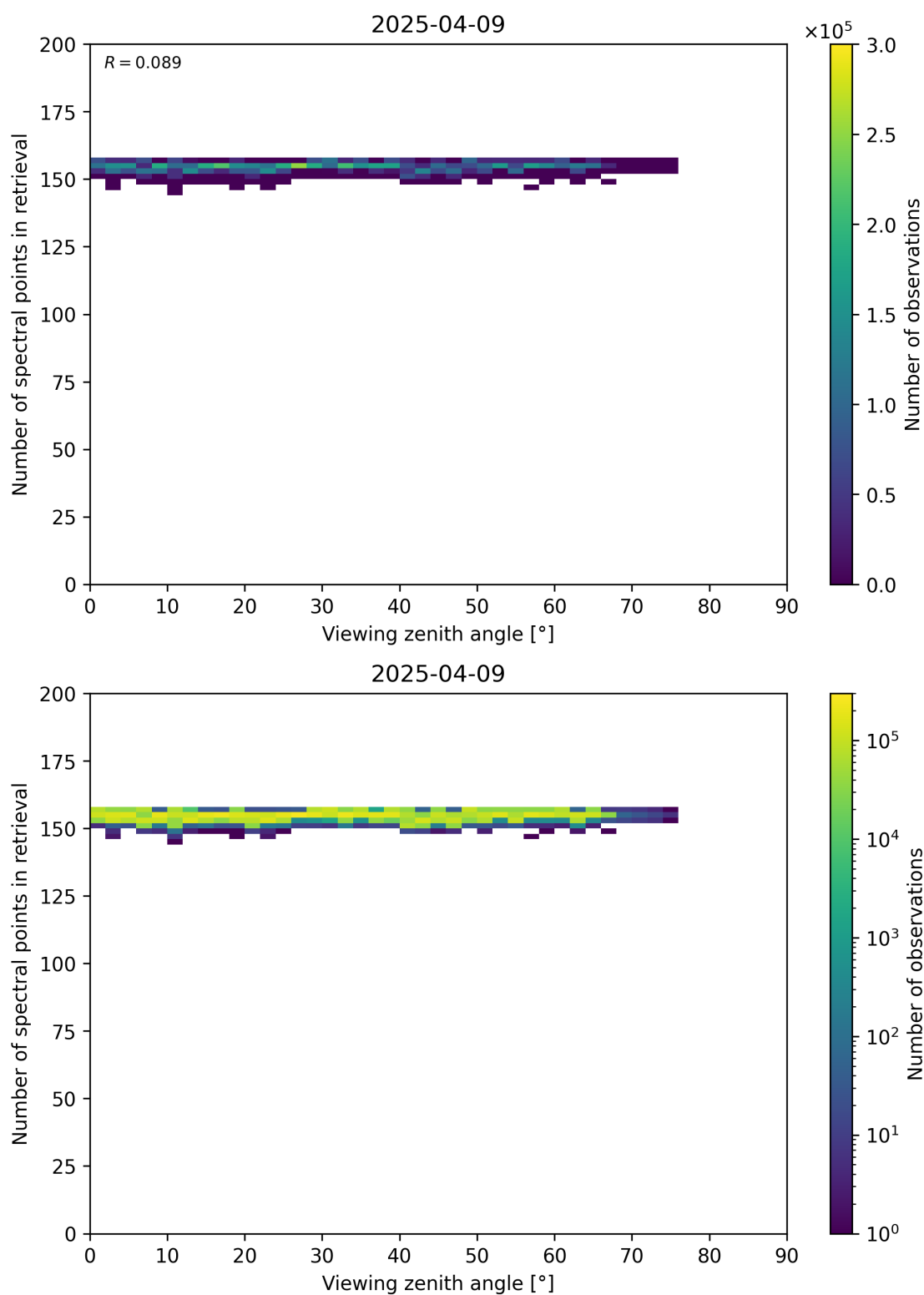
Figure 76: Scatter density plot of “Viewing zenith angle” against “Number of spectral points in retrieval” for 2025-04-08 to 2025-04-10.
