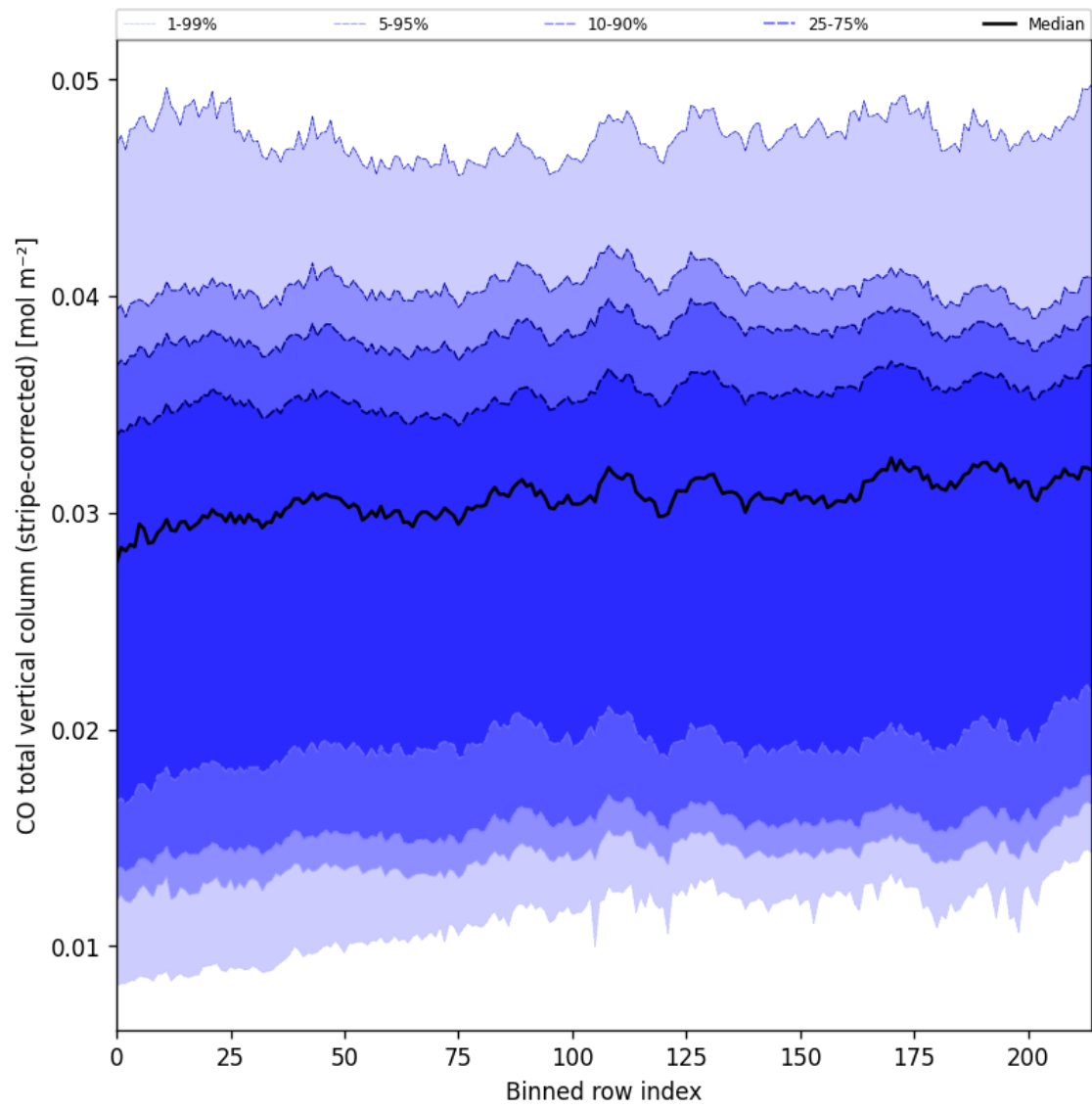
Figure 27: Along track statistics of “CO total vertical column (stripe-corrected)” for 2025-04-08 to 2025-04-10
