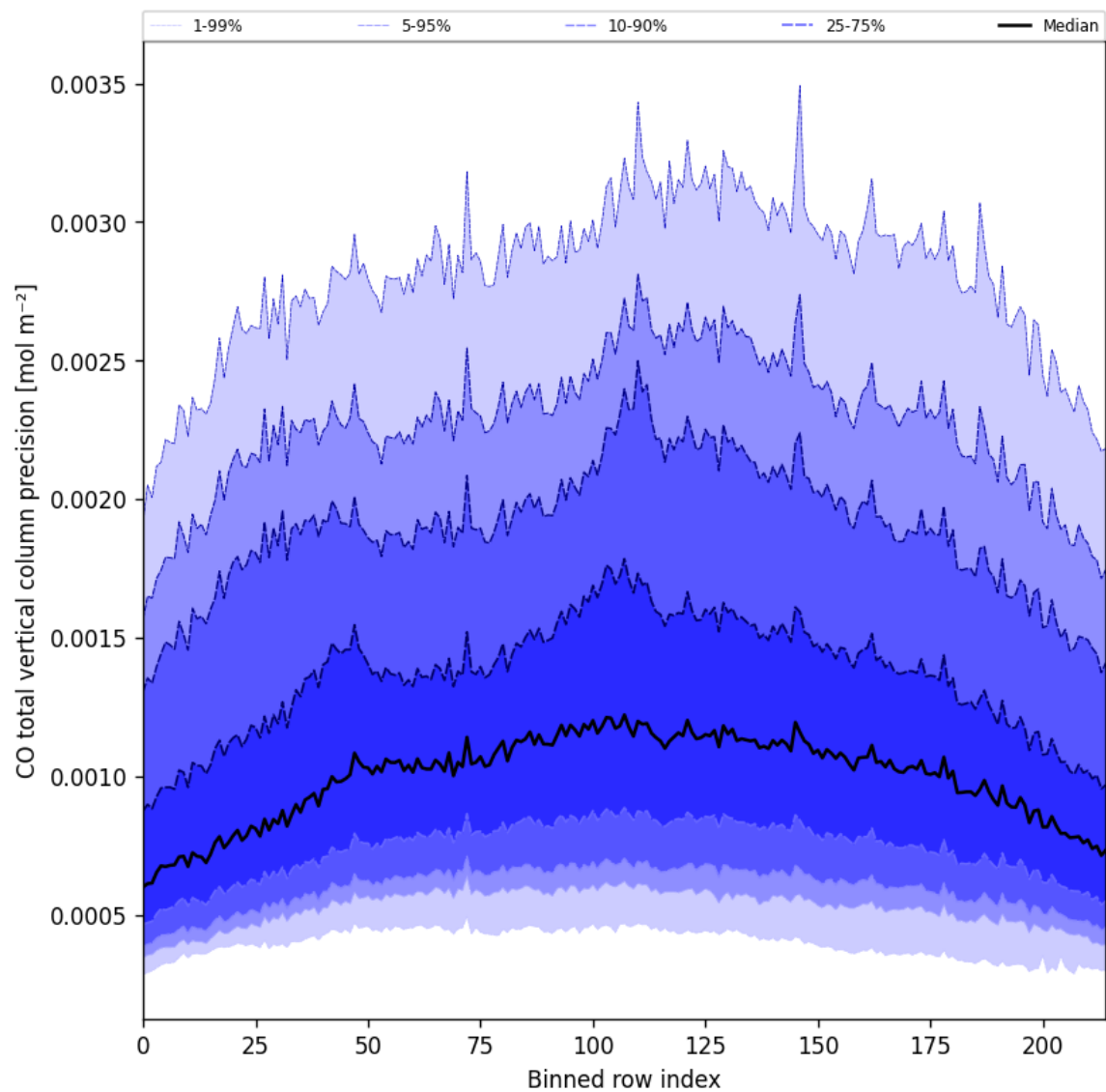
Figure 28: Along track statistics of “CO total vertical column precision” for 2025-04-08 to 2025-04-10
