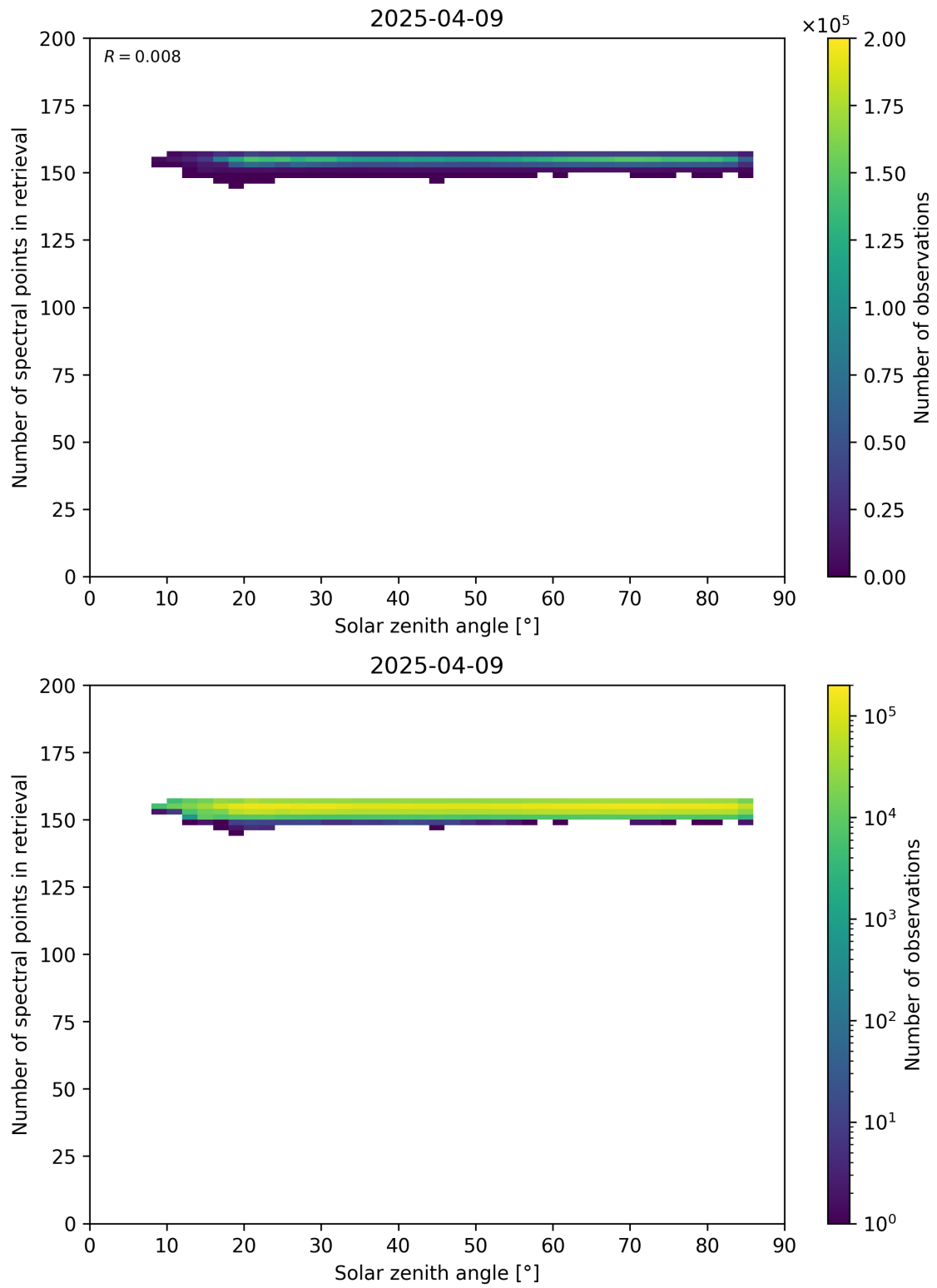
Figure 68: Scatter density plot of “Solar zenith angle” against “Number of spectral points in retrieval” for 2025-04-08 to 2025-04-10.
