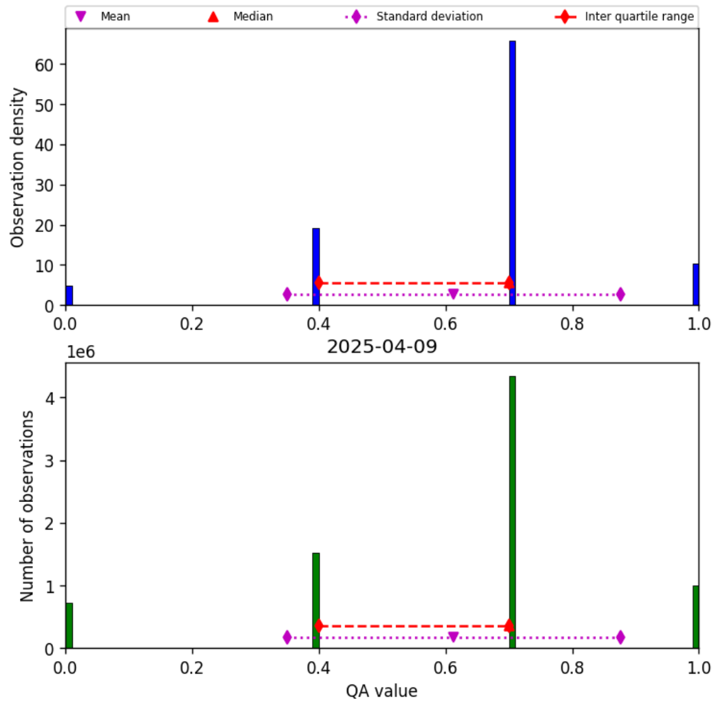
Figure 17: Histogram of “QA value” for 2025-04-08 to 2025-04-10
