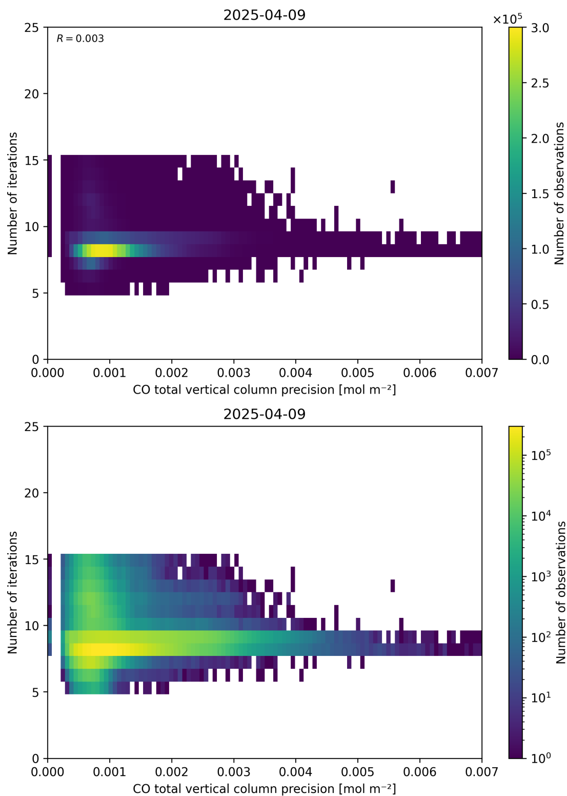
Figure 46: Scatter density plot of “CO total vertical column precision” against “Number of iterations” for 2025-04-08 to 2025-04-10.
