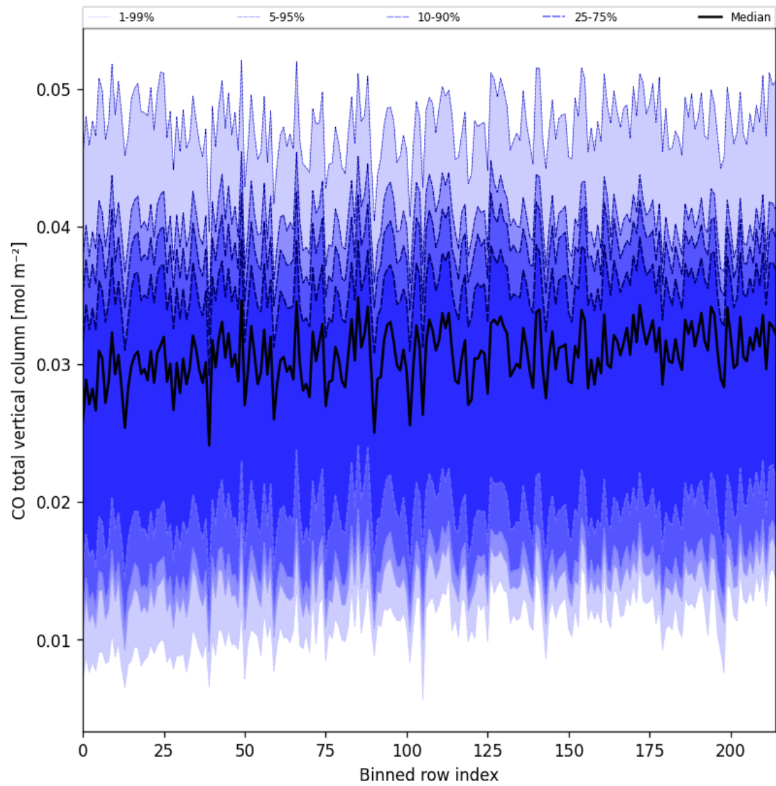
Figure 26: Along track statistics of “CO total vertical column” for 2025-04-08 to 2025-04-10
