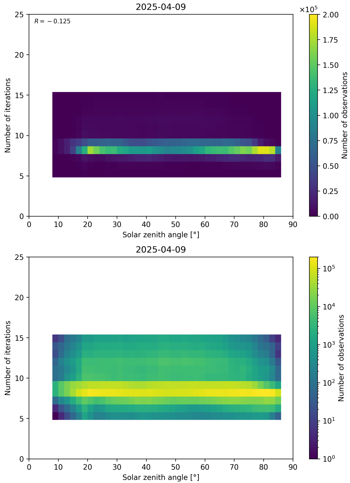
Figure 67: Scatter density plot of “Solar zenith angle” against “Number of iterations” for 2025-04-08 to 2025-04-10.
