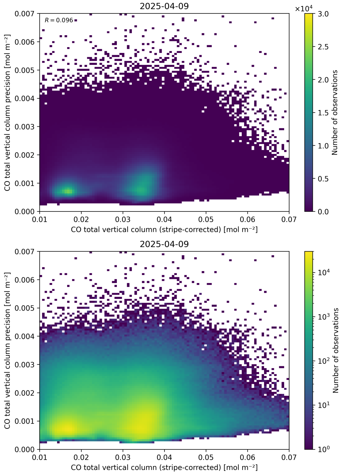
Figure 36: Scatter density plot of “CO total vertical column (stripe-corrected)” against “CO total vertical column precision” for 2025-04-08 to 2025-04-10.
