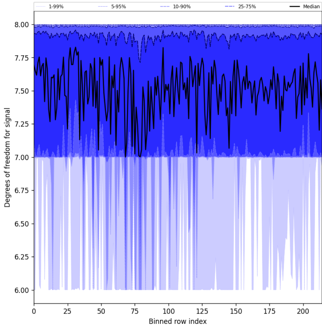
Figure 31: Along track statistics of “Degrees of freedom for signal” for 2025-04-08 to 2025-04-10
