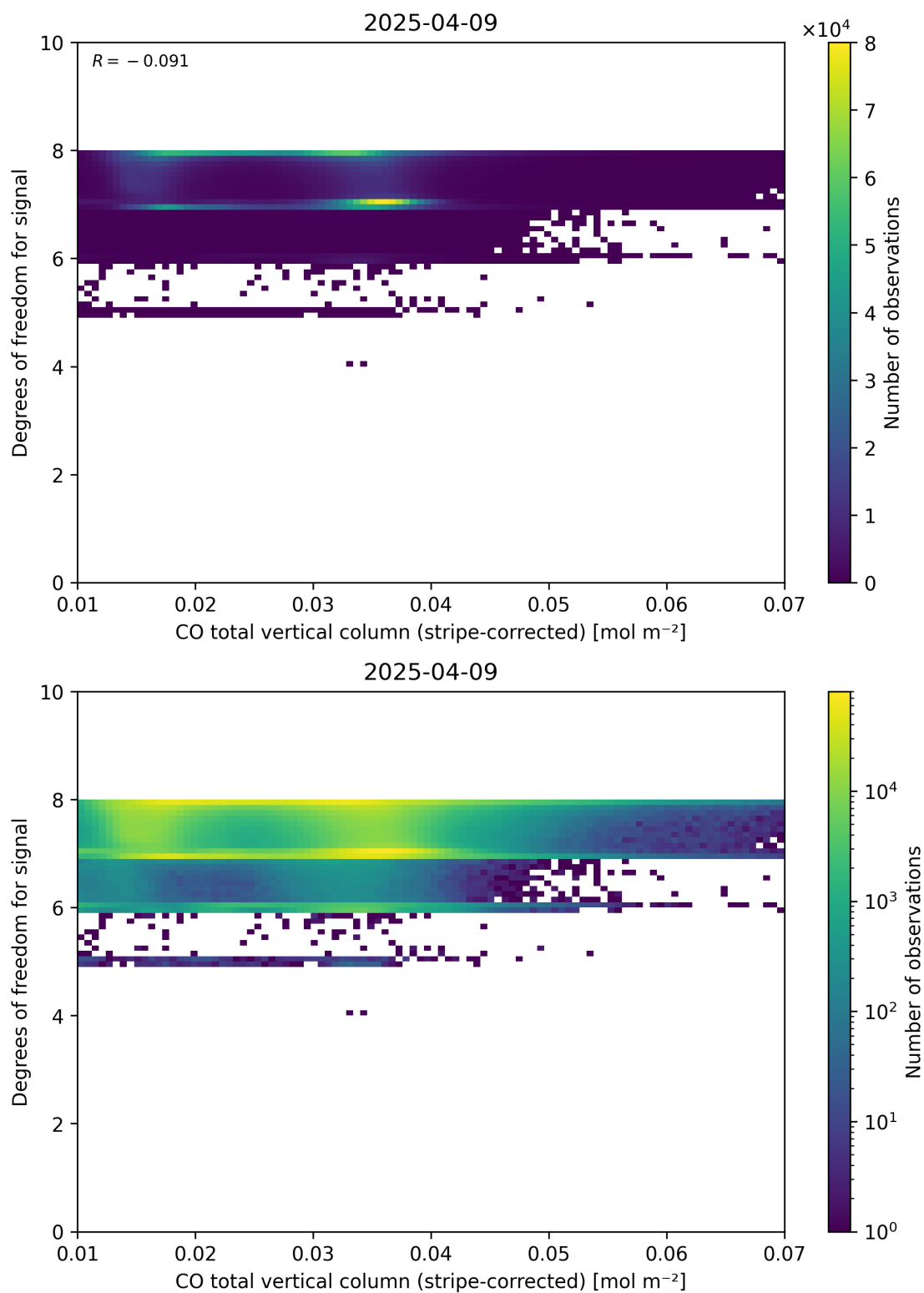
Figure 38: Scatter density plot of “CO total vertical column (stripe-corrected)” against “Degrees of freedom for signal” for 2025-04-08 to 2025-04-10.
