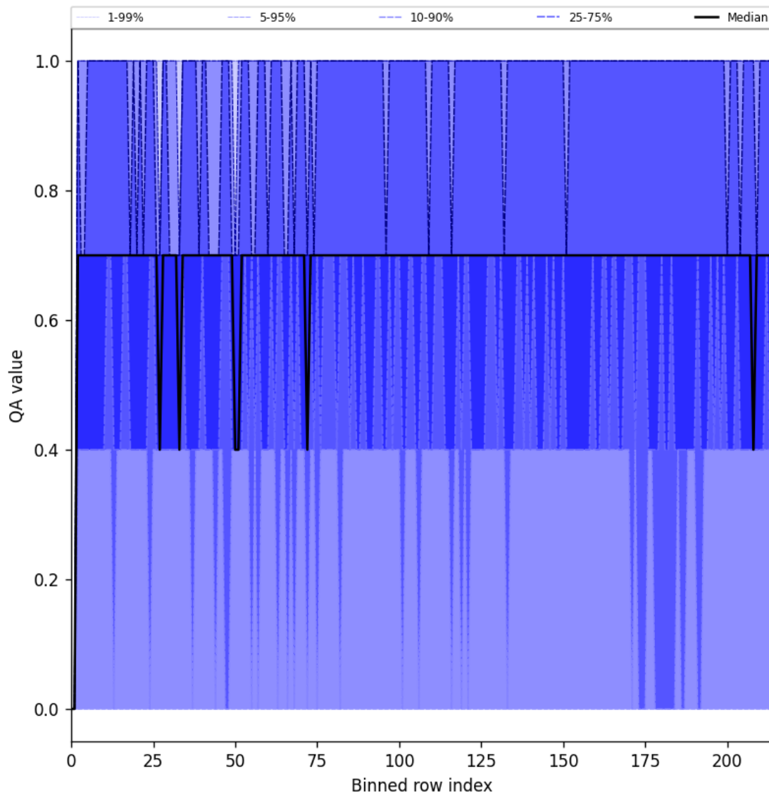
Figure 25: Along track statistics of “QA value” for 2025-04-08 to 2025-04-10
