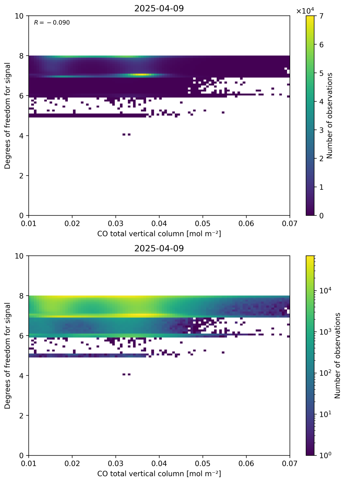
Figure 41: Scatter density plot of “CO total vertical column” against “Degrees of freedom for signal” for 2025-04-08 to 2025-04-10.
