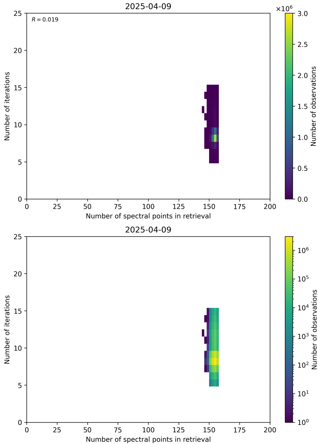
Figure 60: Scatter density plot of “Number of spectral points in retrieval” against “Number of iterations” for 2025-04-08 to 2025-04-10.
