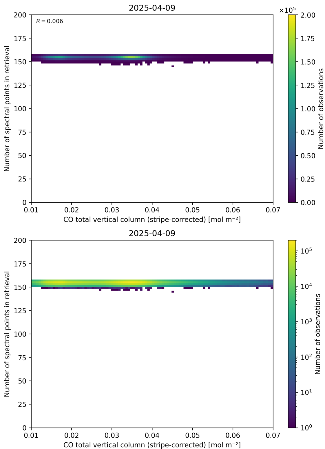
Figure 40: Scatter density plot of “CO total vertical column (stripe-corrected)” against “Number of spectral points in retrieval” for 2025-04-08 to 2025-04-10.
