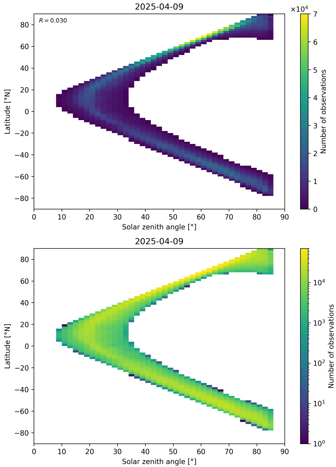
Figure 66: Scatter density plot of “Solar zenith angle” against “Latitude” for 2025-04-08 to 2025-04-10.
