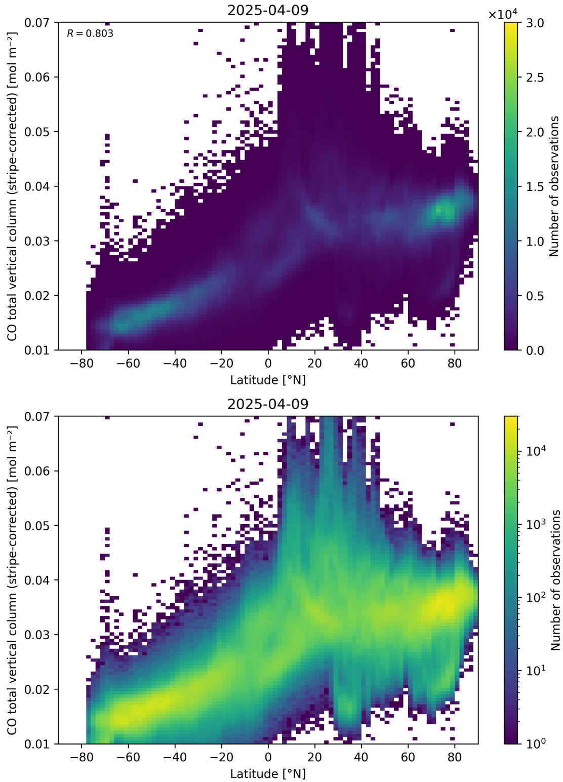
Figure 52: Scatter density plot of “Latitude” against “CO total vertical column (stripe-corrected)” for 2025-04-08 to 2025-04-10.
