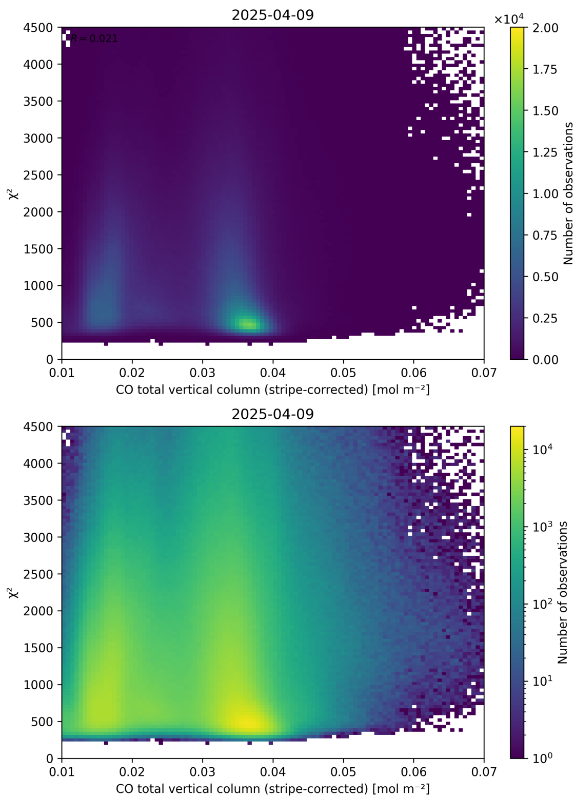
Figure 37: Scatter density plot of “CO total vertical column (stripe-corrected)” against “ \chi^2 ” for 2025-04-08 to 2025-04-10.
