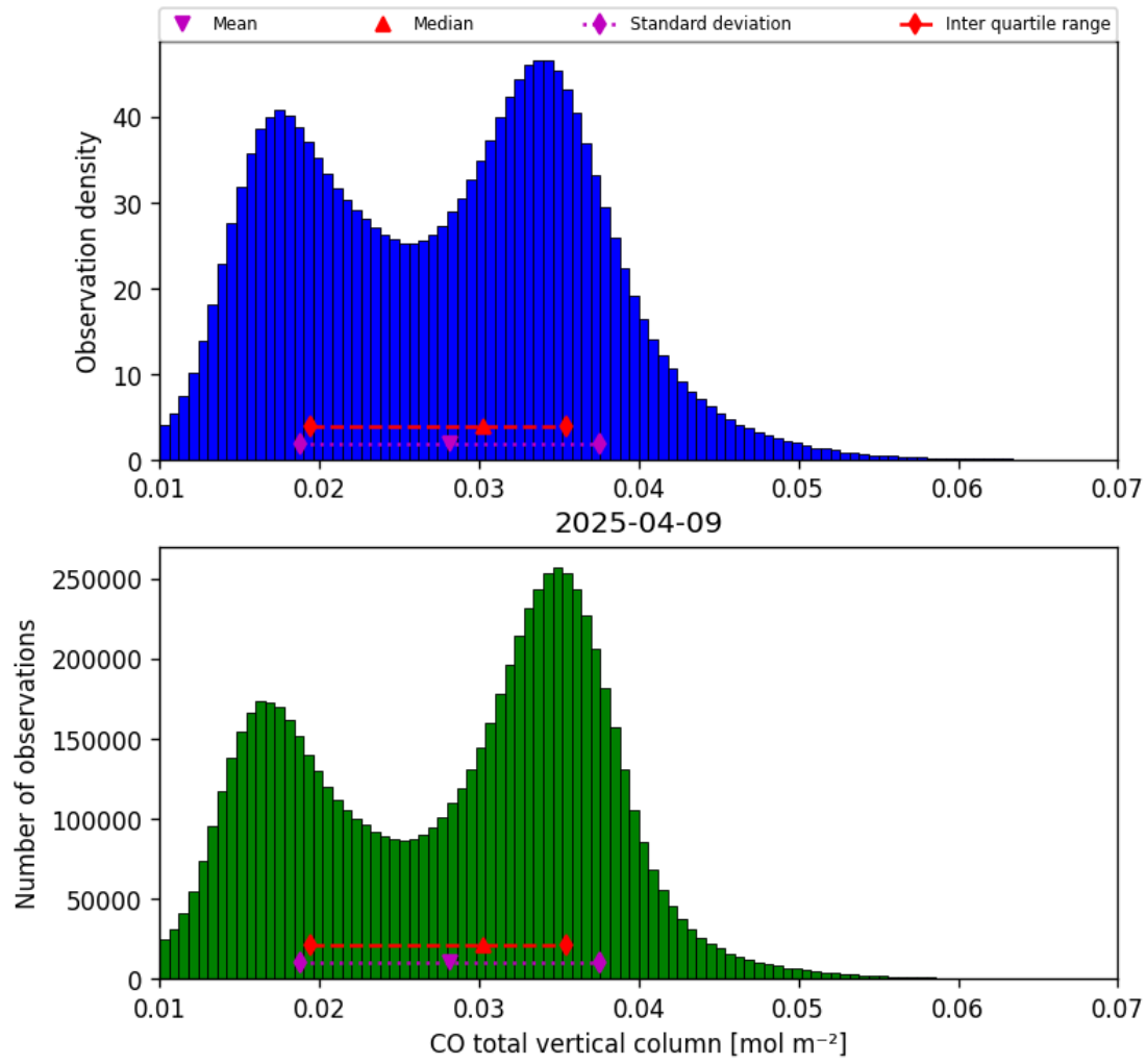
Figure 18: Histogram of “CO total vertical column” for 2025-04-08 to 2025-04-10
