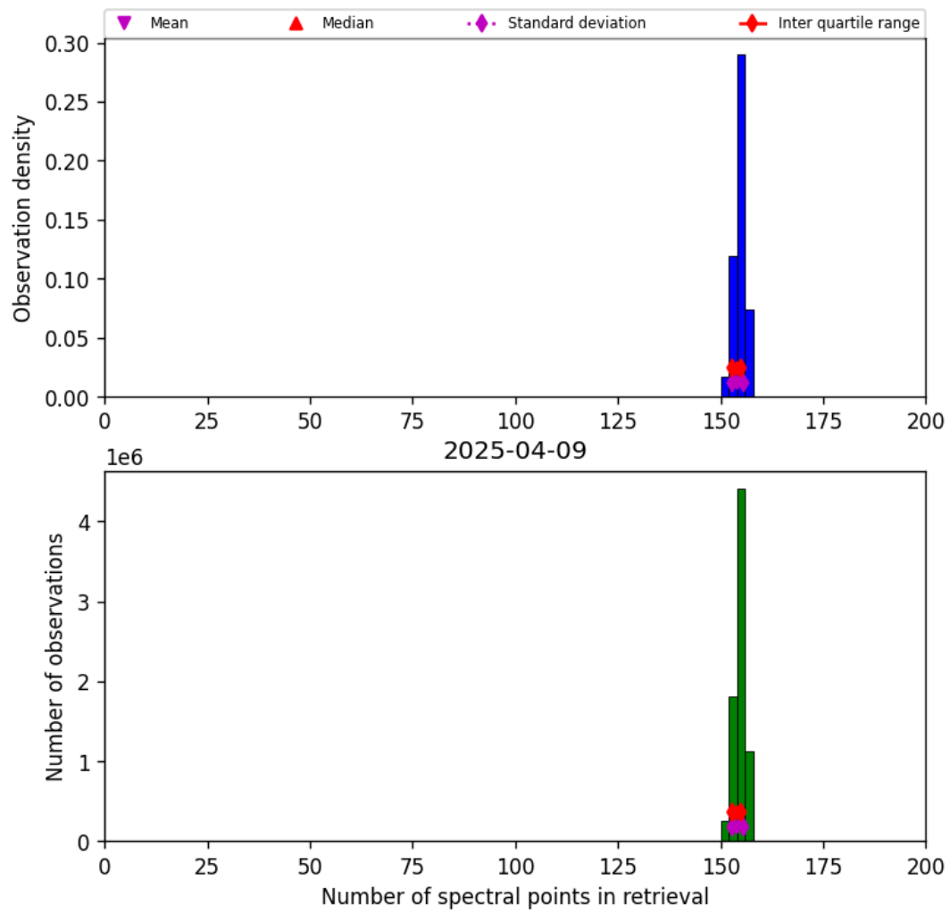
Figure 21: Histogram of “Number of spectral points in retrieval” for 2025-04-08 to 2025-04-10
