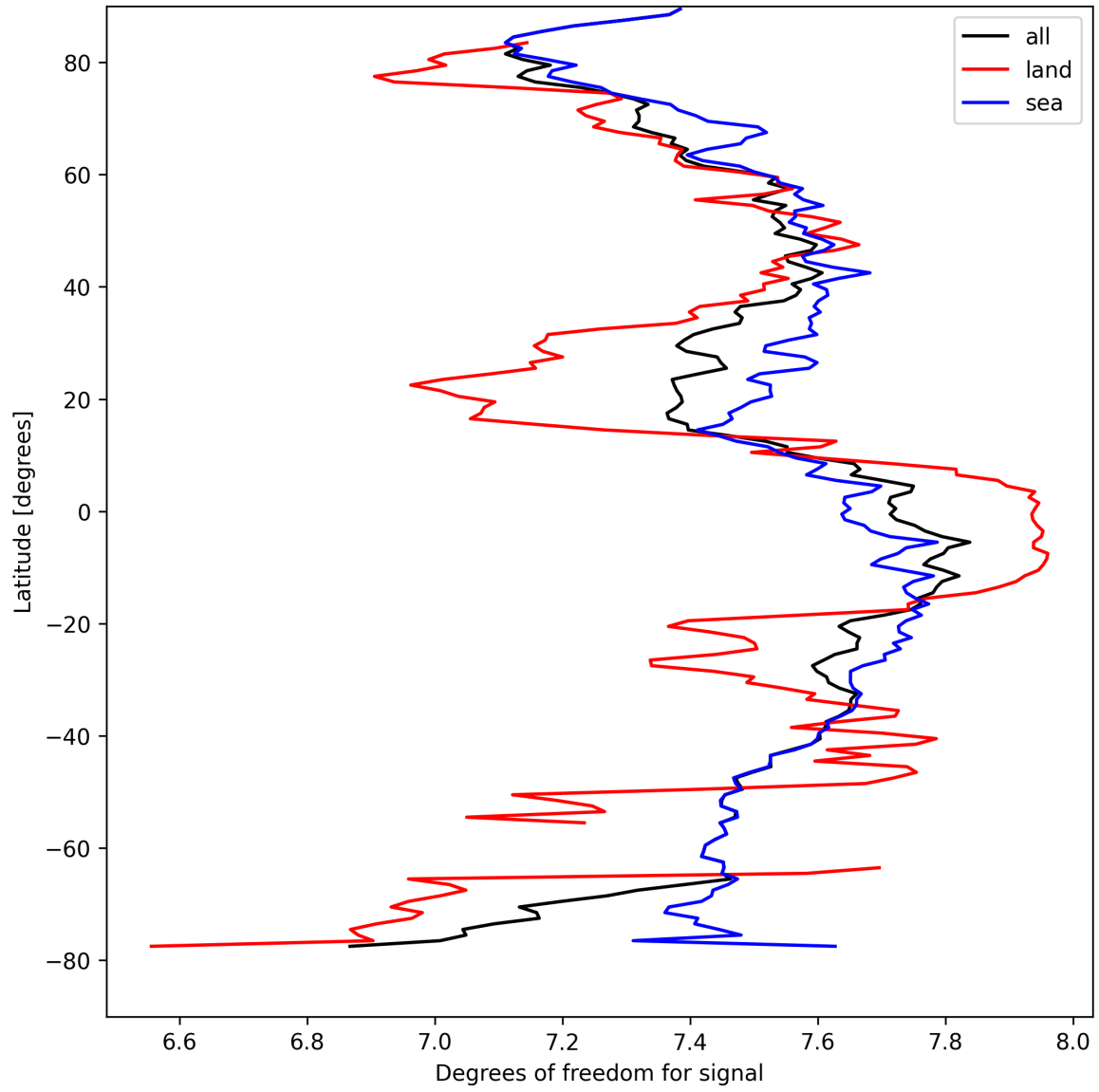
Figure 15: Zonal average of “Degrees of freedom for signal” for 2025-04-08 to 2025-04-10.
