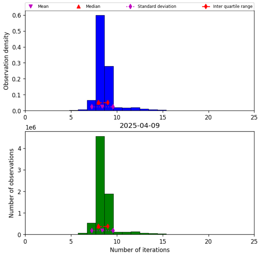
Figure 24: Histogram of “Number of iterations” for 2025-04-08 to 2025-04-10
