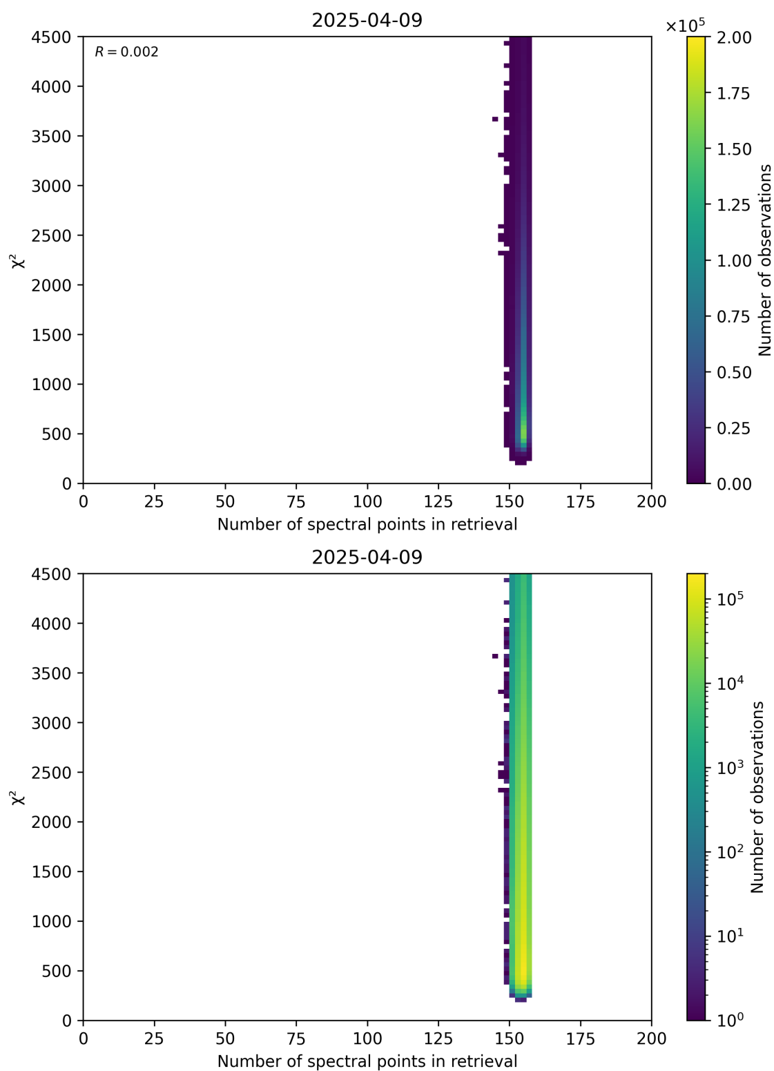
Figure 58: Scatter density plot of “Number of spectral points in retrieval” against “ \chi^2 ” for 2025-04-08 to 2025-04-10.
