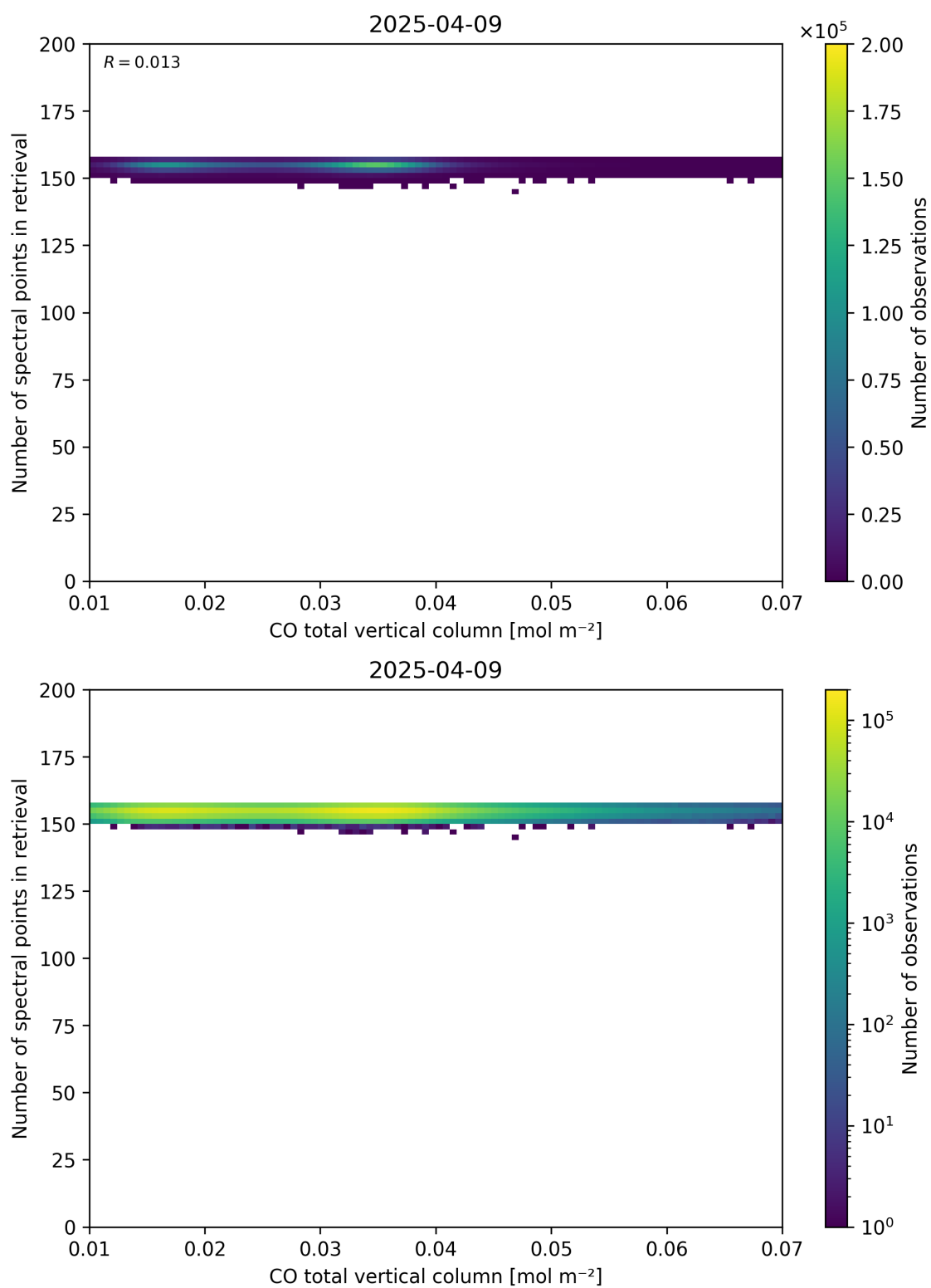
Figure 43: Scatter density plot of “CO total vertical column” against “Number of spectral points in retrieval” for 2025-04-08 to 2025-04-10.
