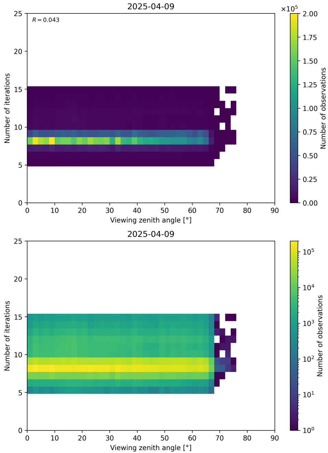
Figure 75: Scatter density plot of “Viewing zenith angle” against “Number of iterations” for 2025-04-08 to 2025-04-10.
