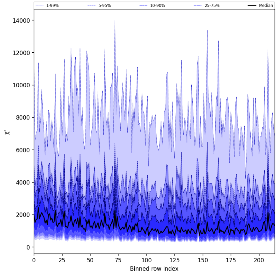
Figure 30: Along track statistics of “ \chi^2 ” for 2025-04-08 to 2025-04-10
