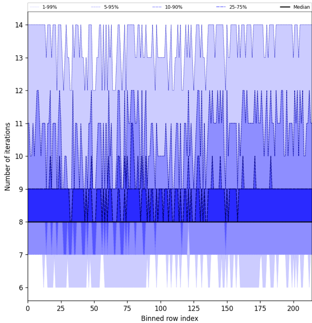
Figure 32: Along track statistics of “Number of iterations” for 2025-04-08 to 2025-04-10
