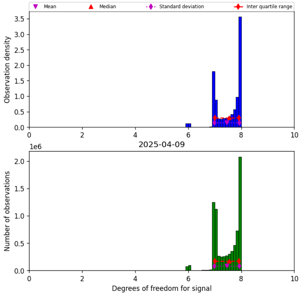
Figure 23: Histogram of “Degrees of freedom for signal” for 2025-04-08 to 2025-04-10
