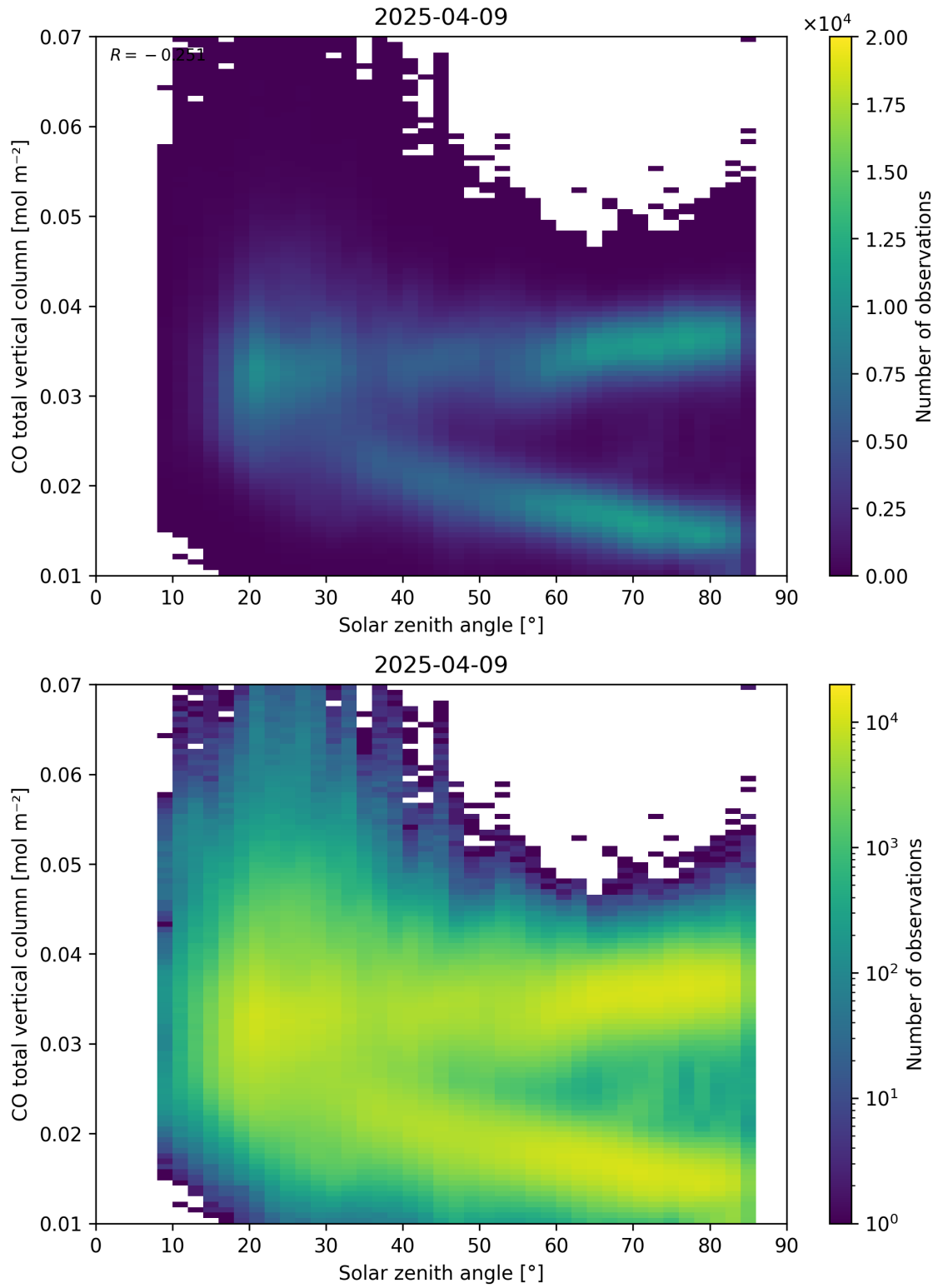
Figure 61: Scatter density plot of “Solar zenith angle” against “CO total vertical column” for 2025-04-08 to 2025-04-10.
