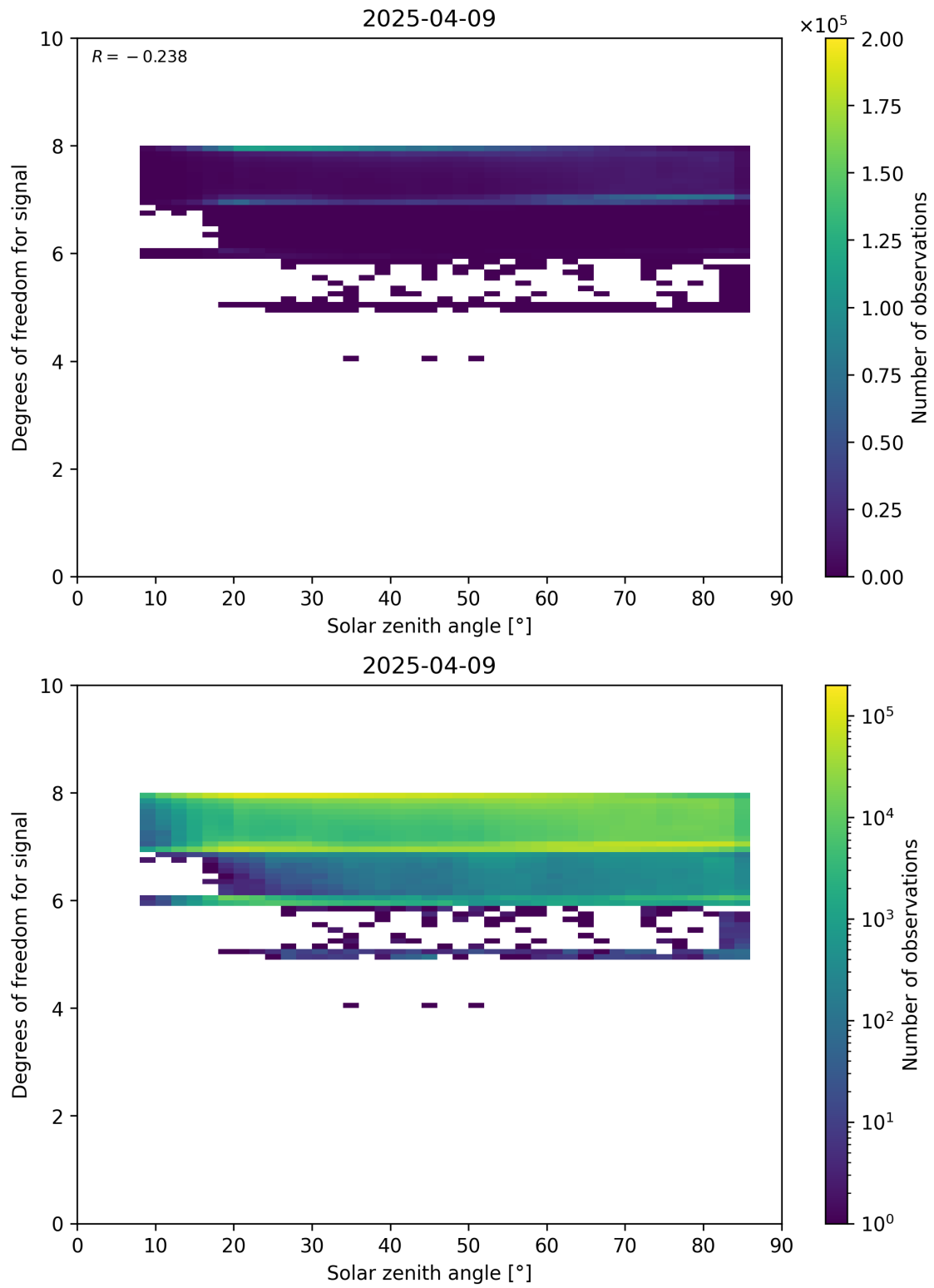
Figure 65: Scatter density plot of “Solar zenith angle” against “Degrees of freedom for signal” for 2025-04-08 to 2025-04-10.
