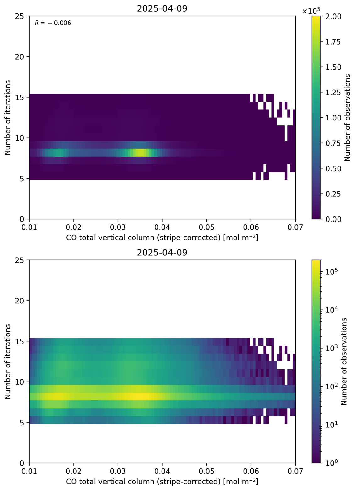
Figure 39: Scatter density plot of “CO total vertical column (stripe-corrected)” against “Number of iterations” for 2025-04-08 to 2025-04-10.
