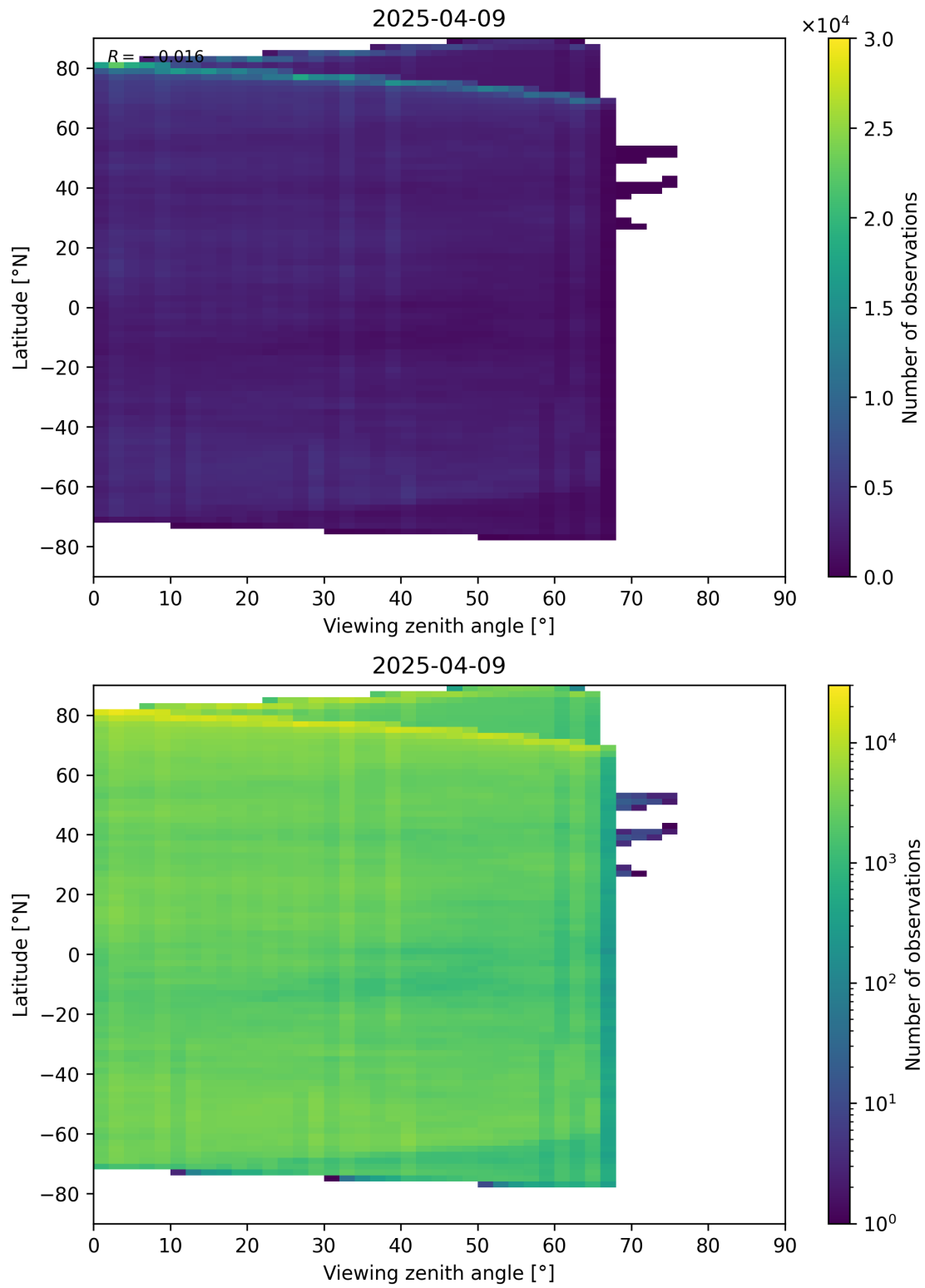
Figure 74: Scatter density plot of “Viewing zenith angle” against “Latitude” for 2025-04-08 to 2025-04-10.
