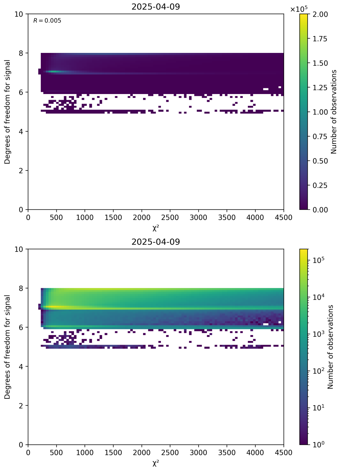
Figure 48: Scatter density plot of “ \chi^2 ” against “Degrees of freedom for signal” for 2025-04-08 to 2025-04-10.
