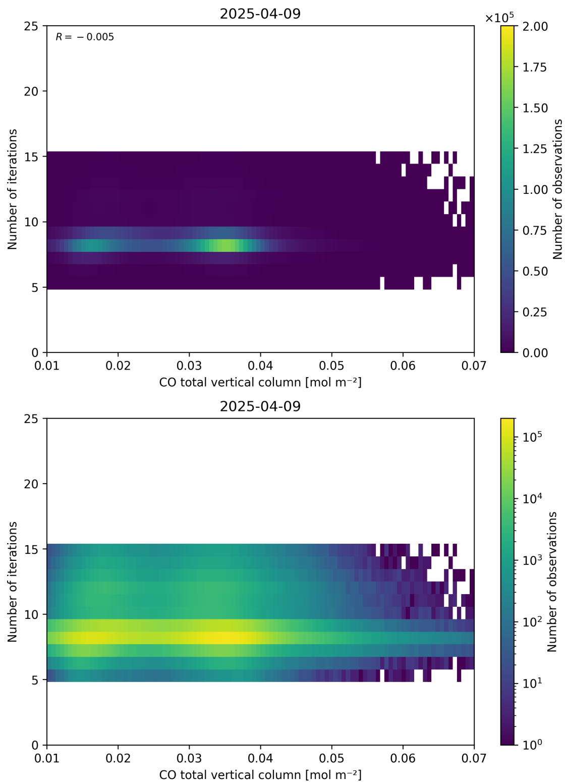
Figure 42: Scatter density plot of “CO total vertical column” against “Number of iterations” for 2025-04-08 to 2025-04-10.
