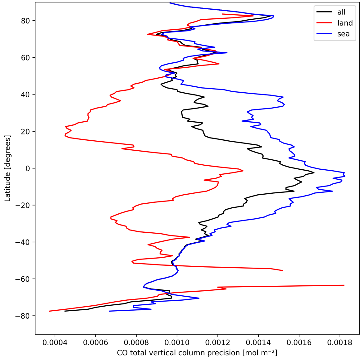
Figure 12: Zonal average of “CO total vertical column precision” for 2025-04-08 to 2025-04-10.
