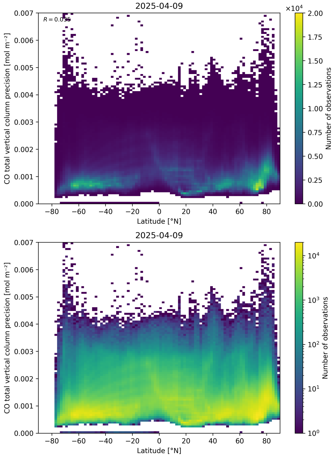
Figure 53: Scatter density plot of “Latitude” against “CO total vertical column precision” for 2025-04-08 to 2025-04-10.
