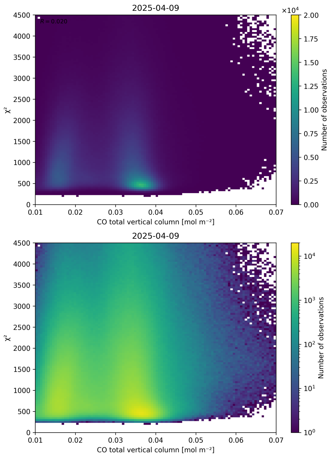
Figure 35: Scatter density plot of “CO total vertical column” against “ \chi^2 ” for 2025-04-08 to 2025-04-10.
