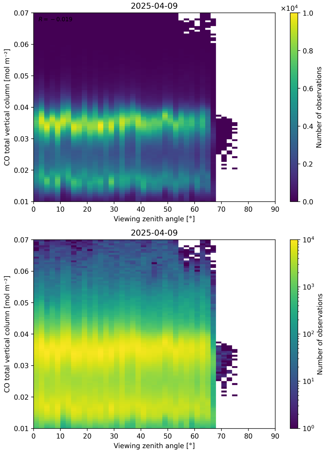
Figure 69: Scatter density plot of “Viewing zenith angle” against “CO total vertical column” for 2025-04-08 to 2025-04-10.
