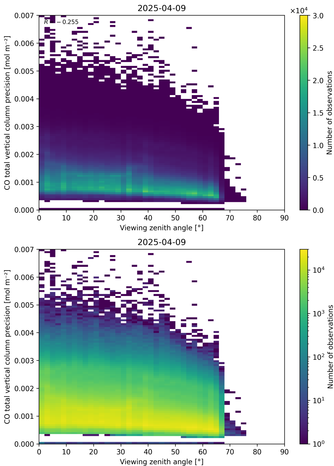
Figure 71: Scatter density plot of “Viewing zenith angle” against “CO total vertical column precision” for 2025-04-08 to 2025-04-10.
