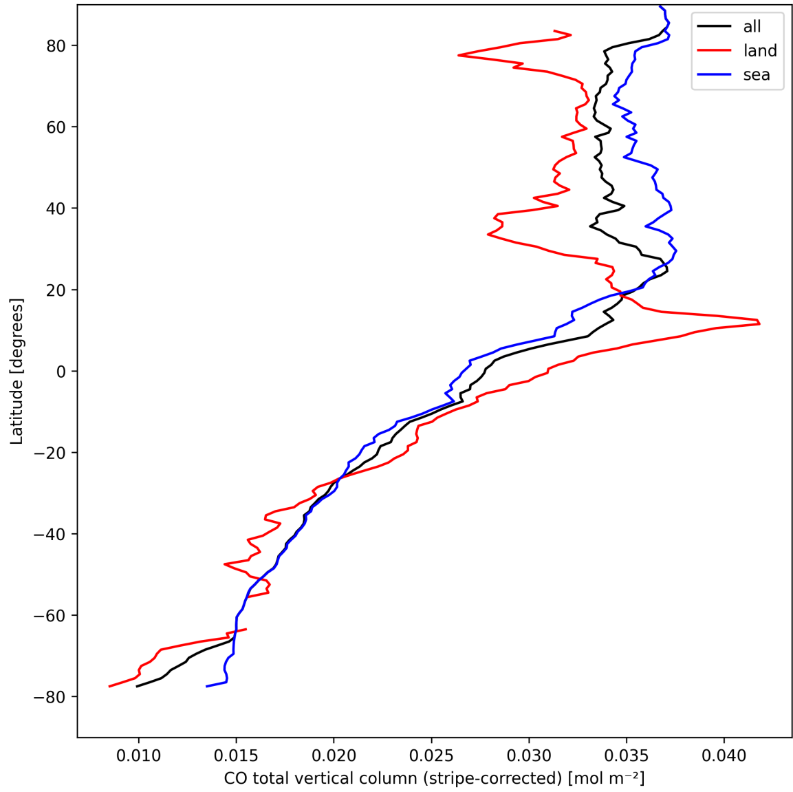
Figure 11: Zonal average of “CO total vertical column (stripe-corrected)” for 2025-04-08 to 2025-04-10.
