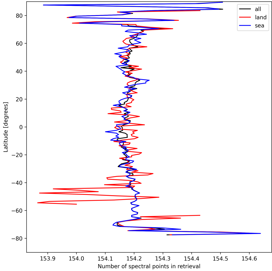
Figure 13: Zonal average of “Number of spectral points in retrieval” for 2025-04-08 to 2025-04-10.
