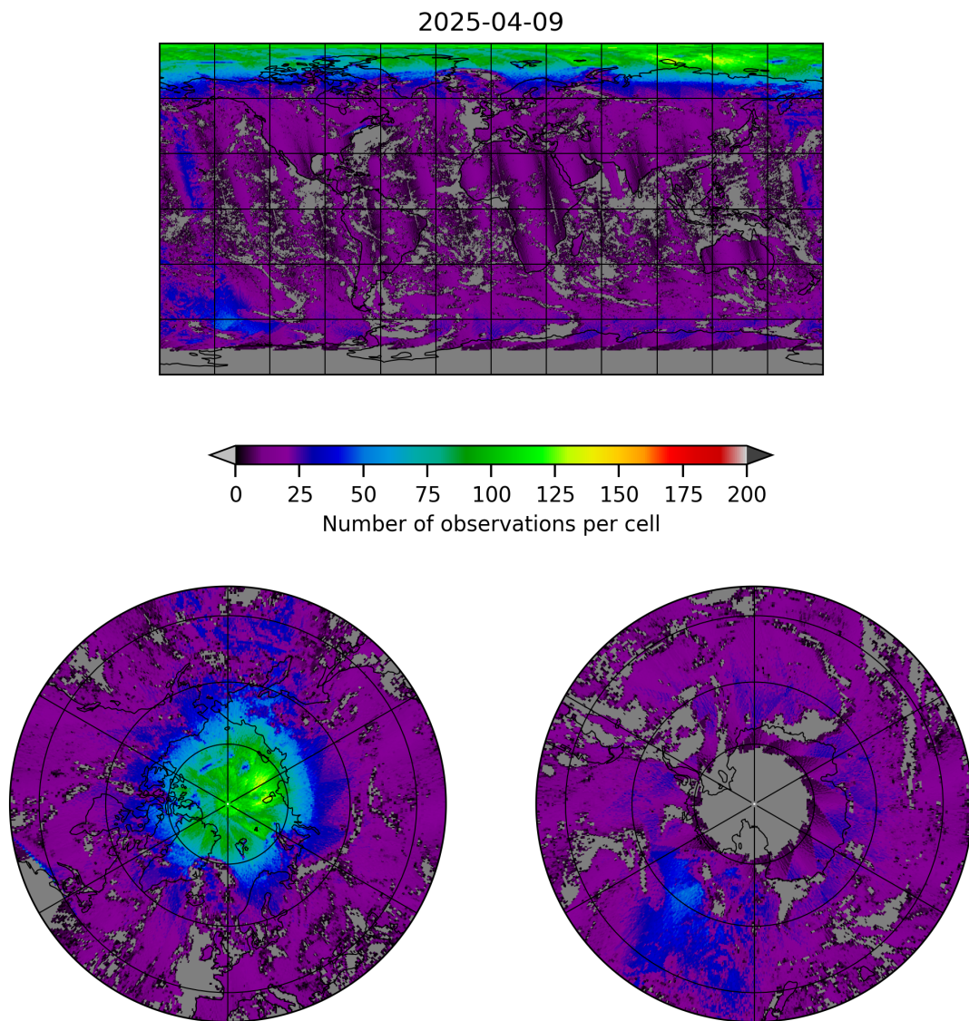
Figure 8: Map of the number of observations for 2025-04-08 to 2025-04-10
