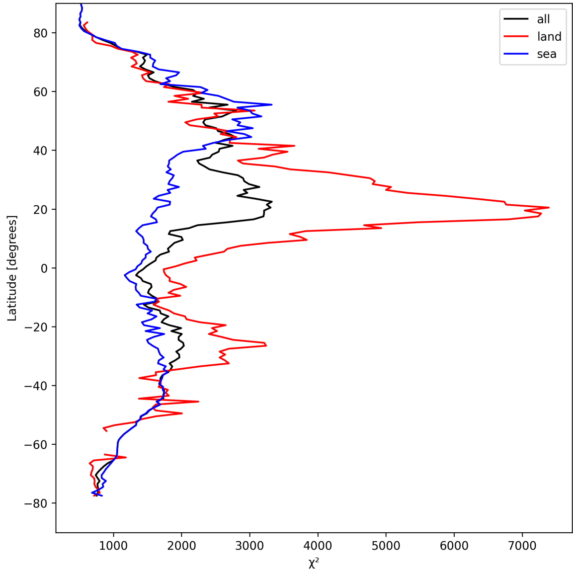
Figure 14: Zonal average of “ \chi^2 ” for 2025-04-08 to 2025-04-10.
