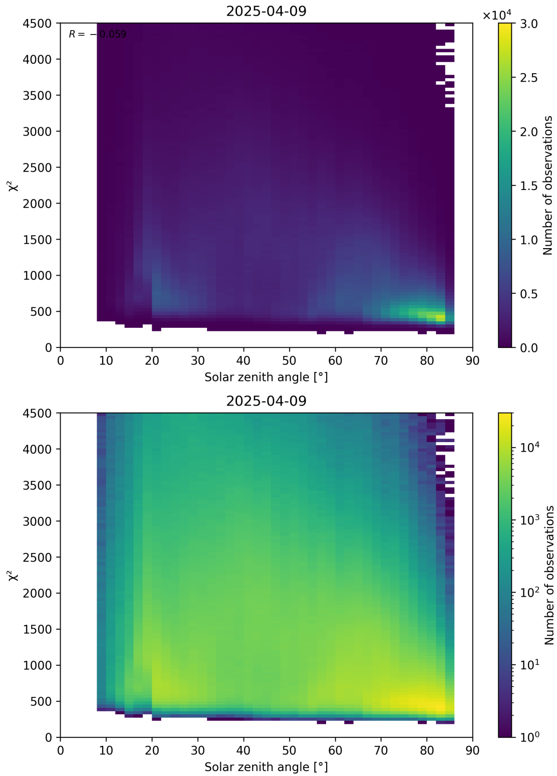
Figure 64: Scatter density plot of “Solar zenith angle” against “ \chi^2 ” for 2025-04-08 to 2025-04-10.
