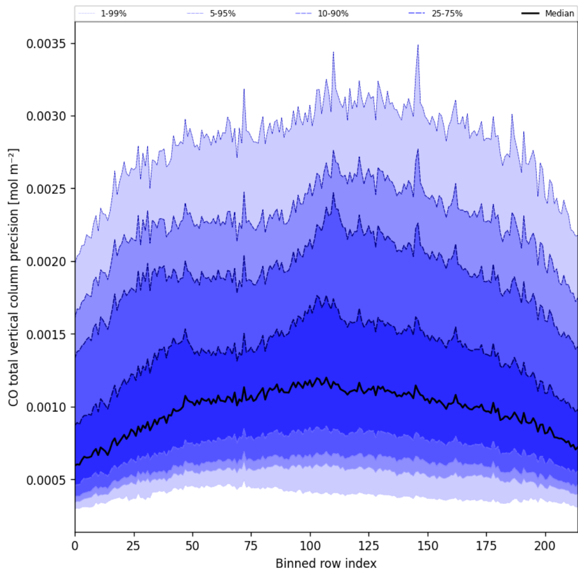
Figure 28: Along track statistics of “CO total vertical column precision” for 2025-04-09 to 2025-04-11
