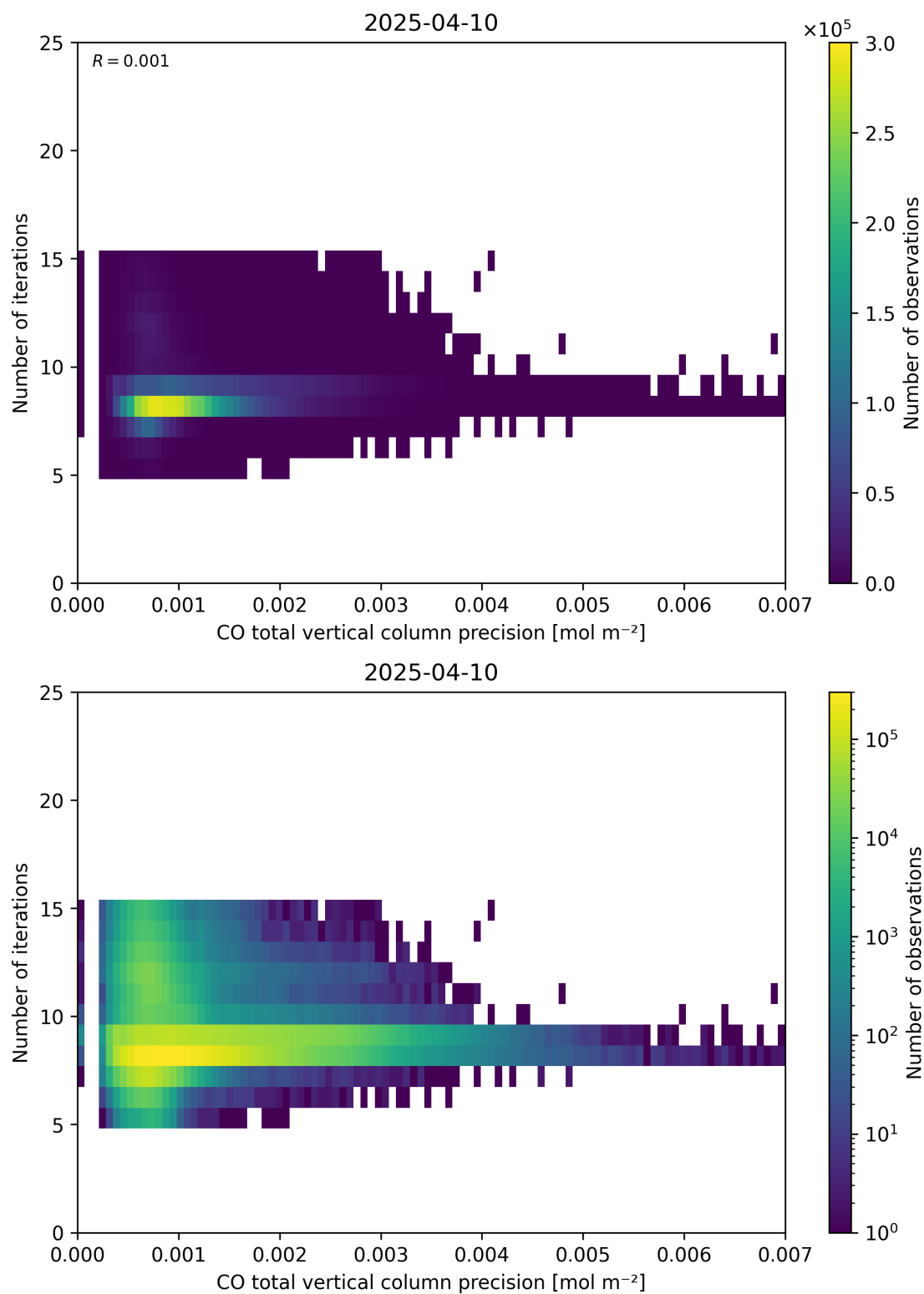
Figure 46: Scatter density plot of “CO total vertical column precision” against “Number of iterations” for 2025-04-09 to 2025-04-11.
