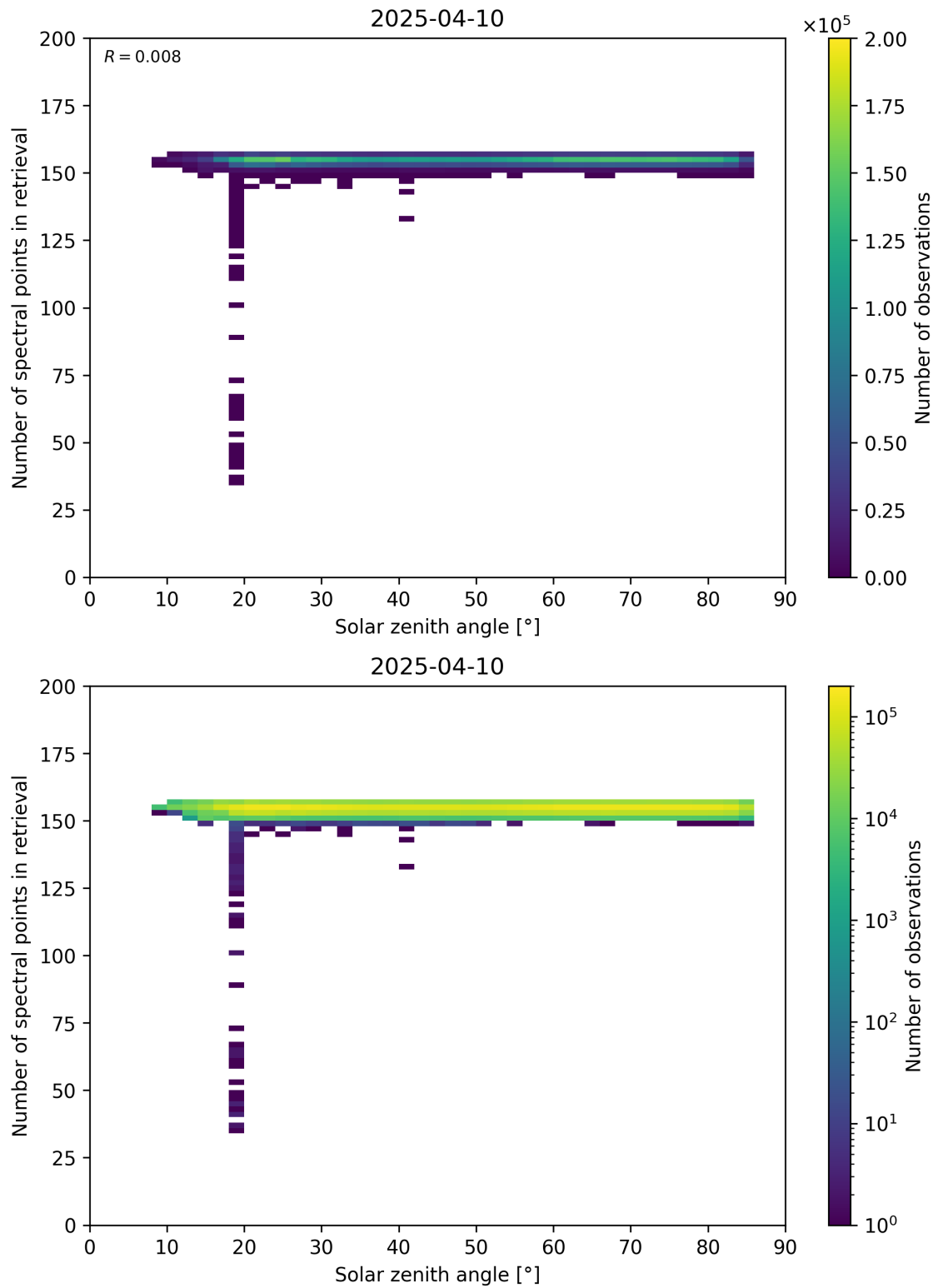
Figure 68: Scatter density plot of “Solar zenith angle” against “Number of spectral points in retrieval” for 2025-04-09 to 2025-04-11.
