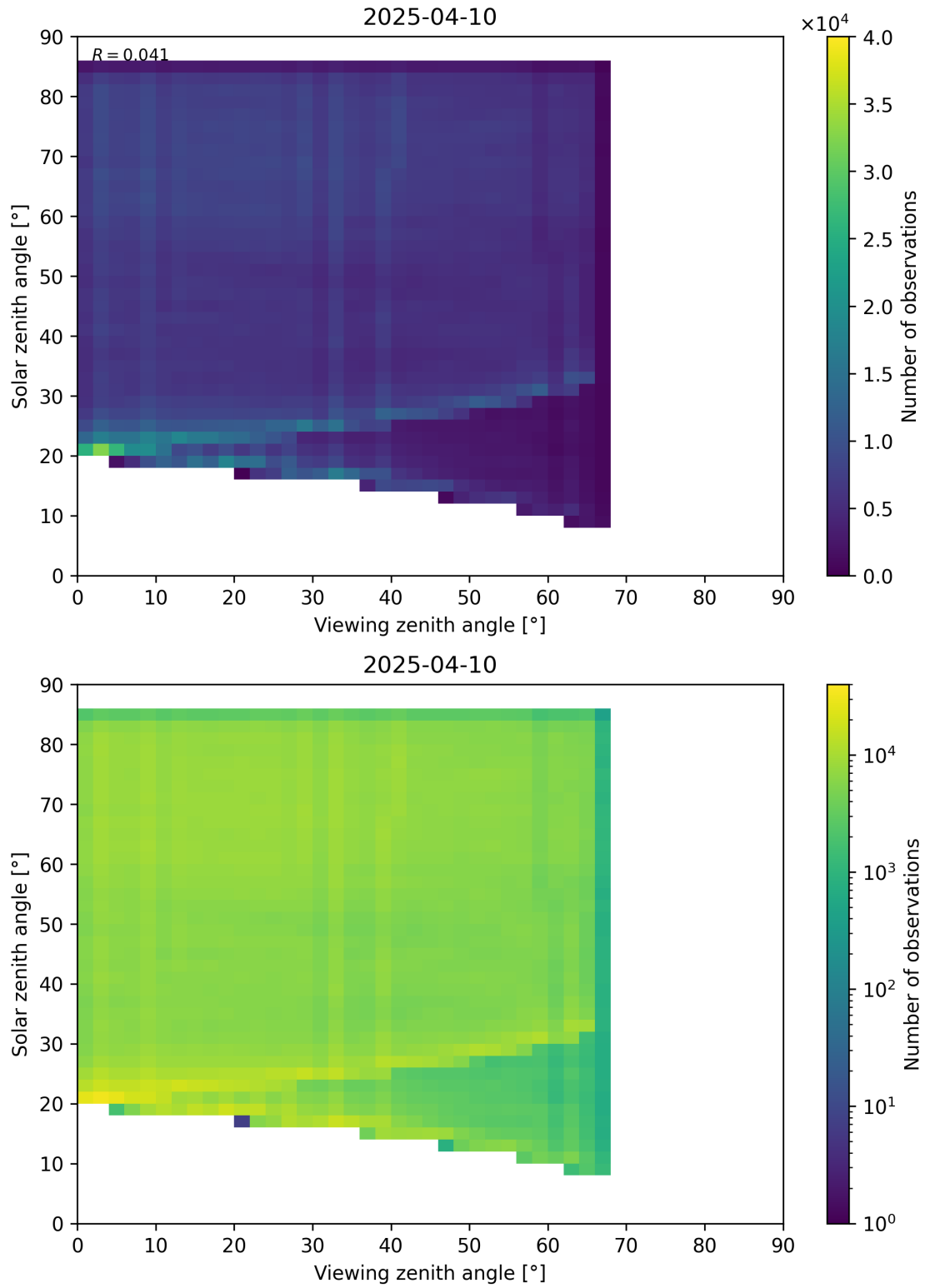
Figure 77: Scatter density plot of “Viewing zenith angle” against “Solar zenith angle” for 2025-04-09 to 2025-04-11.
