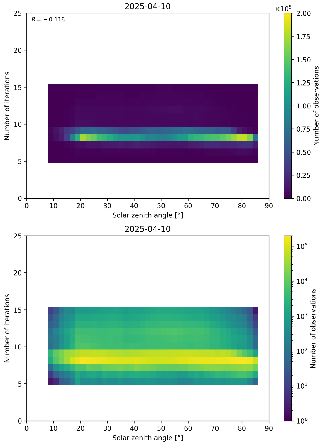
Figure 67: Scatter density plot of “Solar zenith angle” against “Number of iterations” for 2025-04-09 to 2025-04-11.
