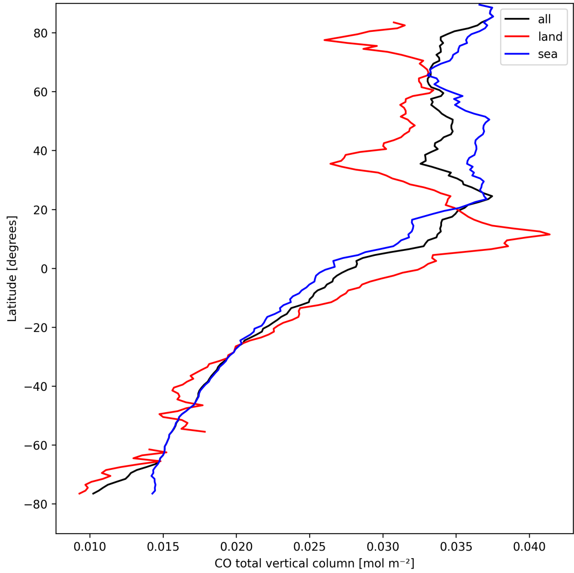
Figure 10: Zonal average of “CO total vertical column” for 2025-04-09 to 2025-04-11.
