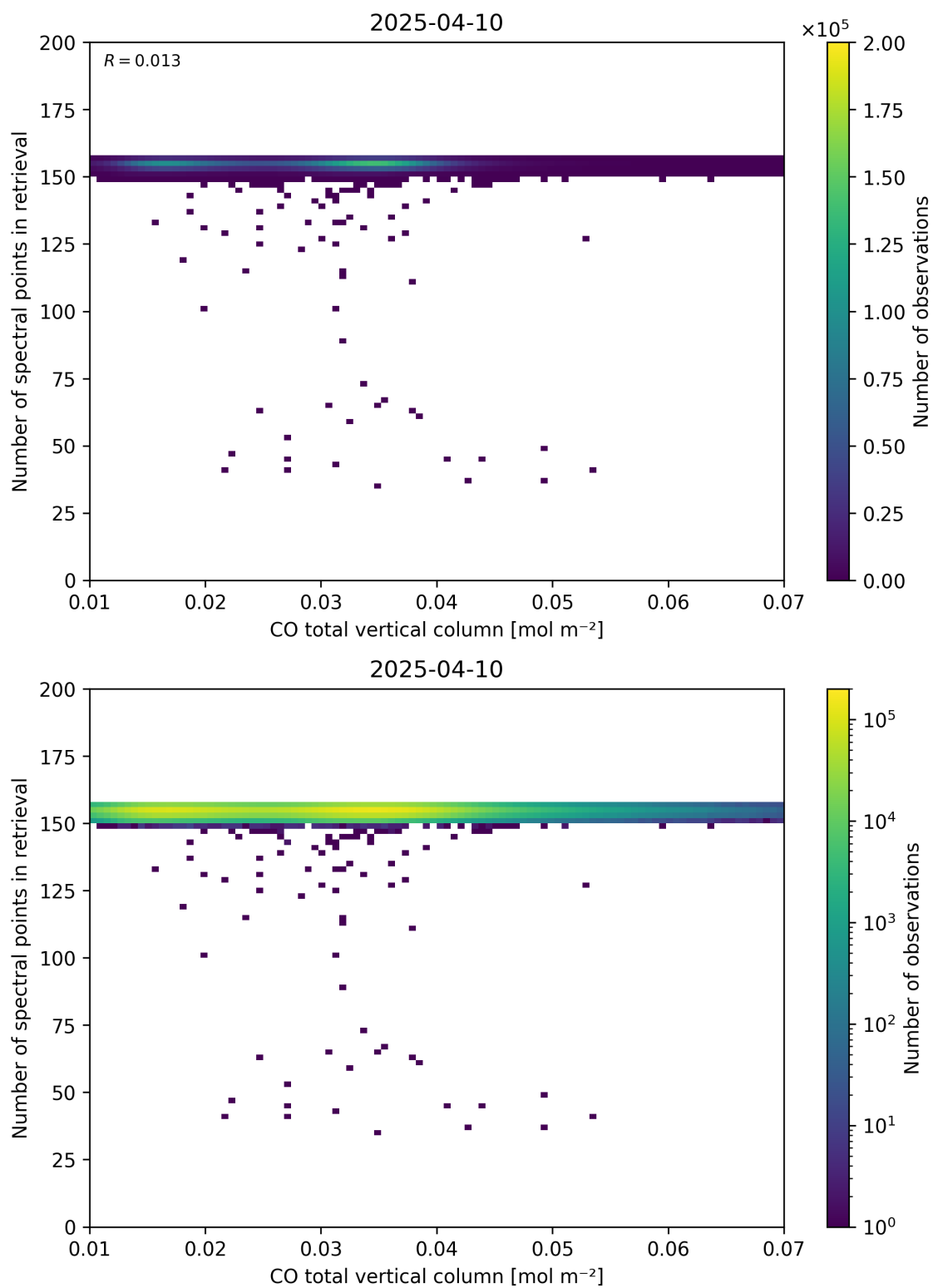
Figure 43: Scatter density plot of “CO total vertical column” against “Number of spectral points in retrieval” for 2025-04-09 to 2025-04-11.
