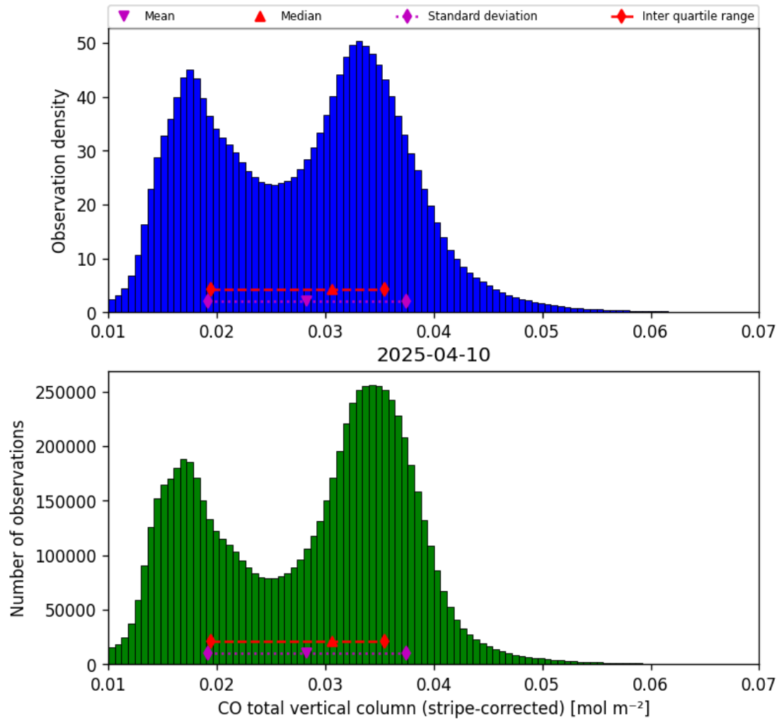
Figure 19: Histogram of “CO total vertical column (stripe-corrected)” for 2025-04-09 to 2025-04-11
