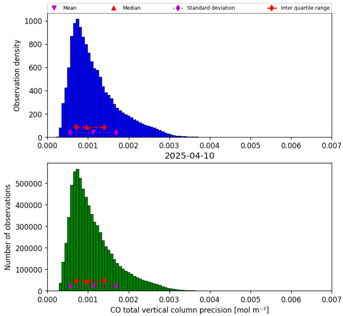
Figure 20: Histogram of “CO total vertical column precision” for 2025-04-09 to 2025-04-11
