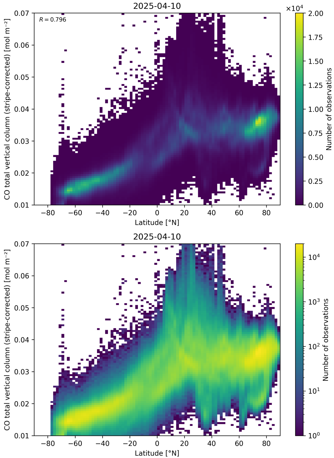
Figure 52: Scatter density plot of “Latitude” against “CO total vertical column (stripe-corrected)” for 2025-04-09 to 2025-04-11.
