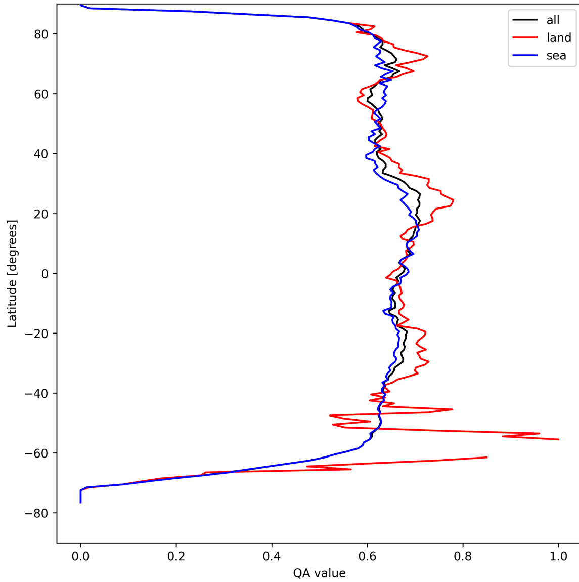
Figure 9: Zonal average of “QA value” for 2025-04-09 to 2025-04-11.
