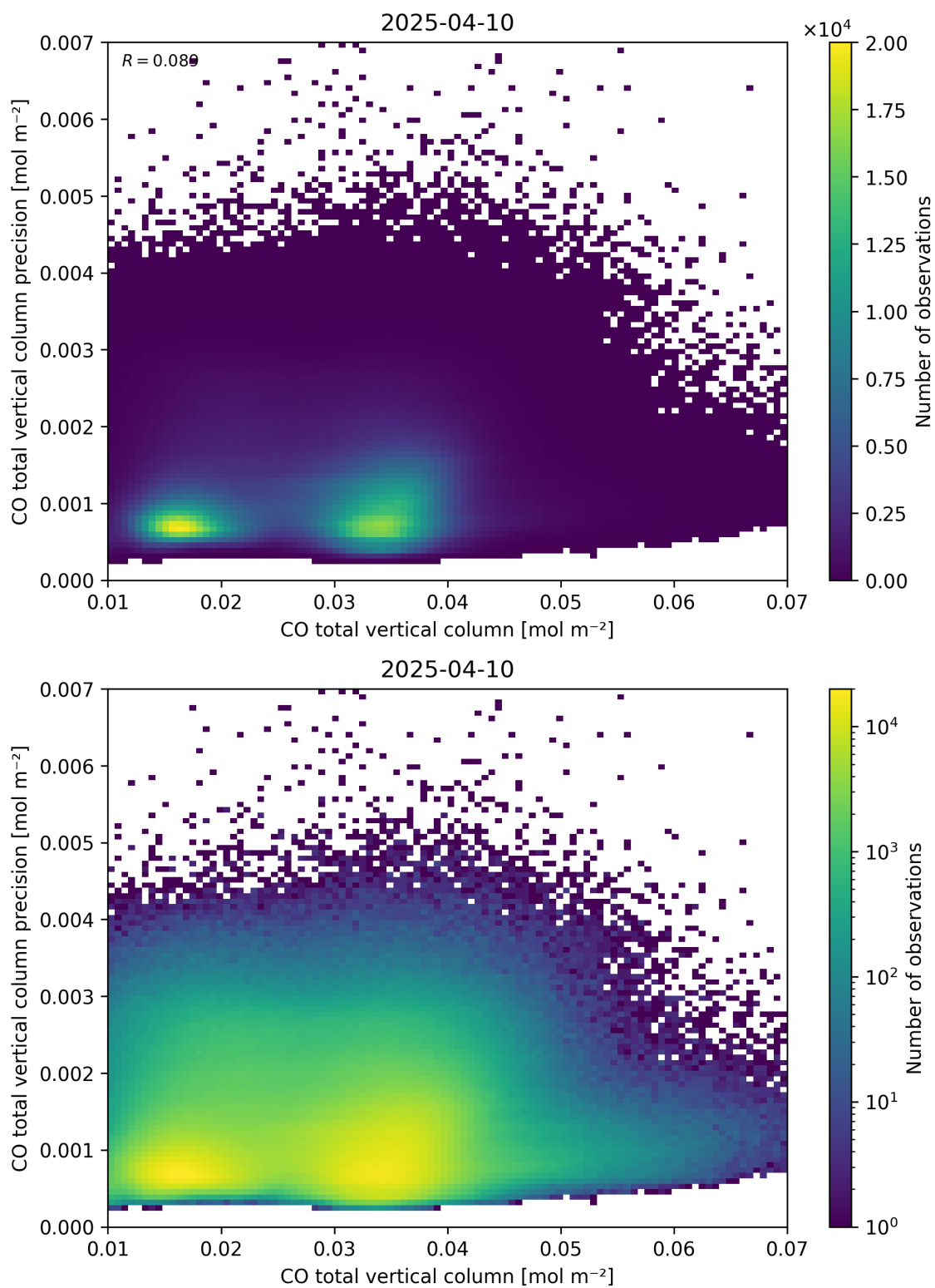
Figure 34: Scatter density plot of “CO total vertical column” against “CO total vertical column precision” for 2025-04-09 to 2025-04-11.
