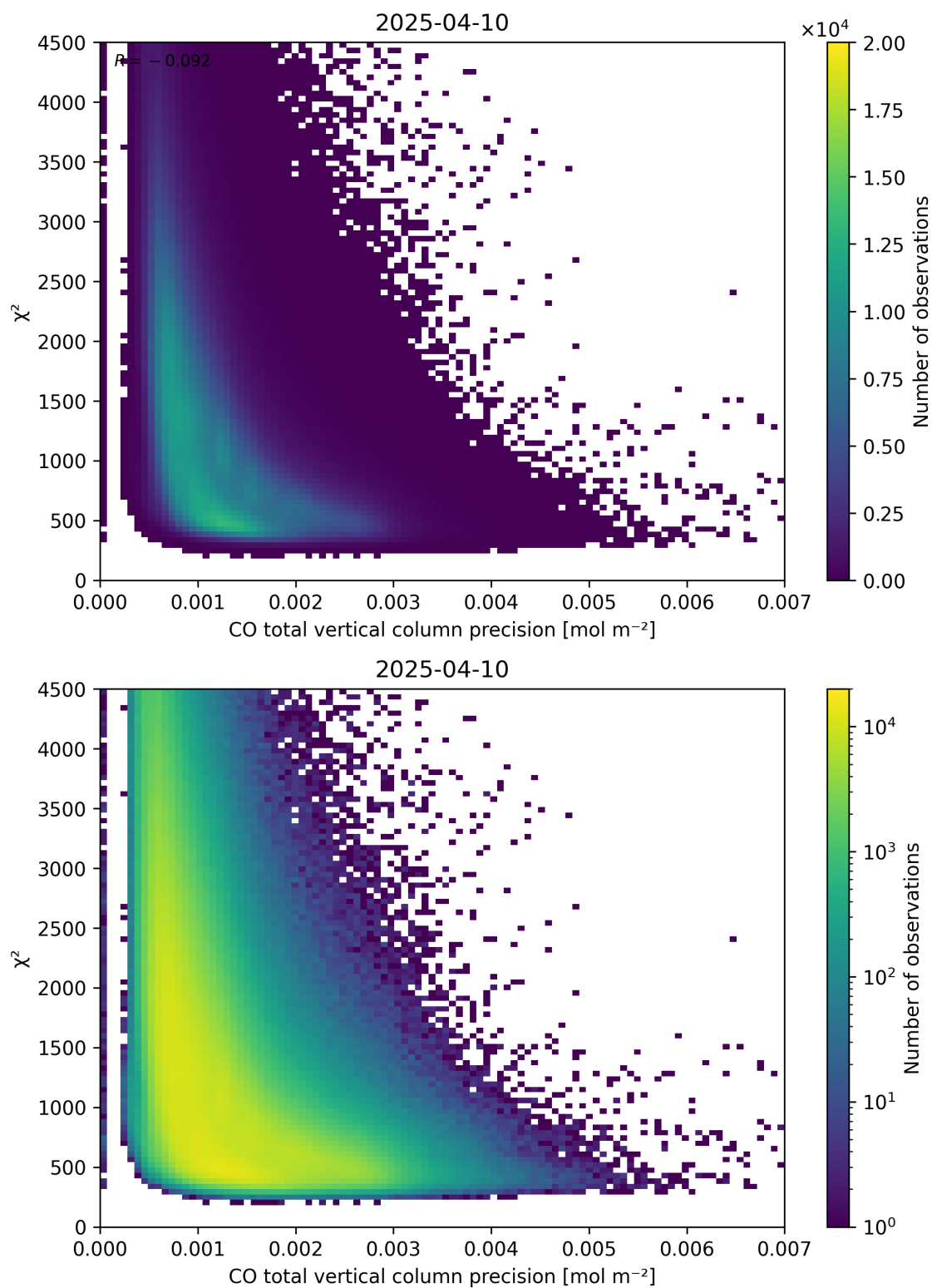
Figure 44: Scatter density plot of “CO total vertical column precision” against “ \chi^2 ” for 2025-04-09 to 2025-04-11.
