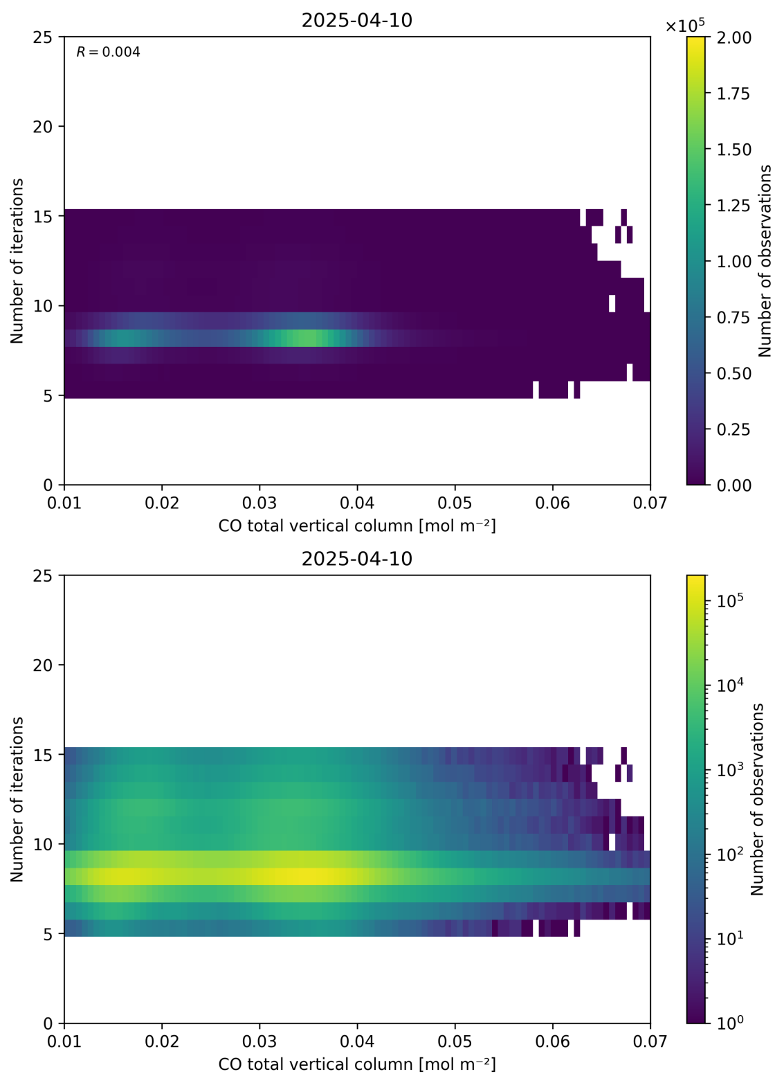
Figure 42: Scatter density plot of “CO total vertical column” against “Number of iterations” for 2025-04-09 to 2025-04-11.
