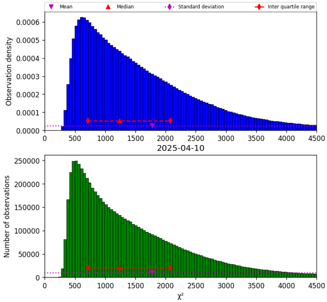
Figure 22: Histogram of “ \chi^2 ” for 2025-04-09 to 2025-04-11
