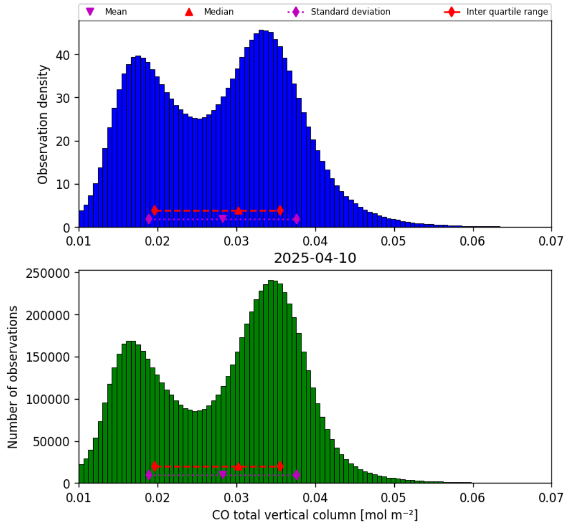
Figure 18: Histogram of “CO total vertical column” for 2025-04-09 to 2025-04-11
