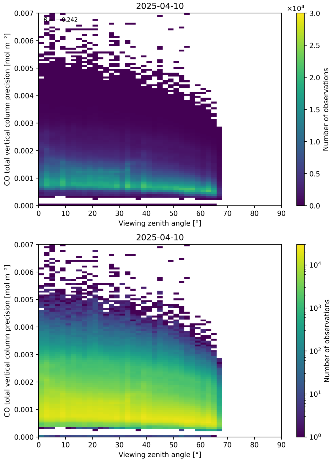
Figure 71: Scatter density plot of “Viewing zenith angle” against “CO total vertical column precision” for 2025-04-09 to 2025-04-11.
