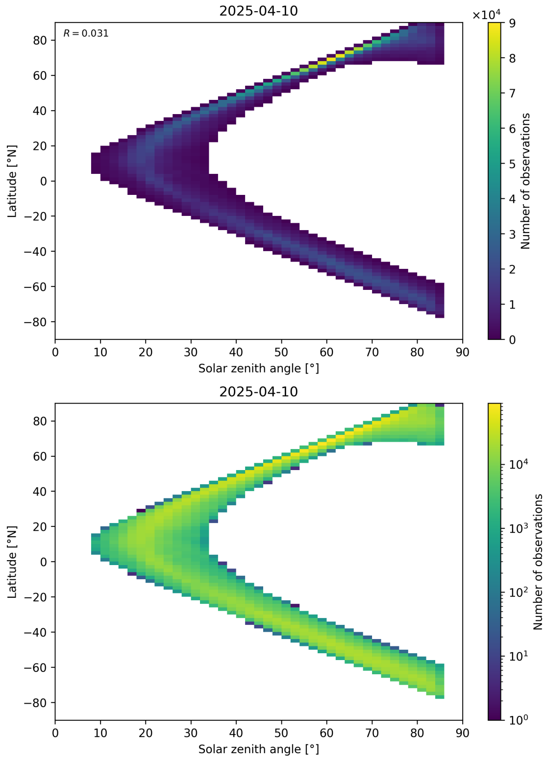
Figure 66: Scatter density plot of “Solar zenith angle” against “Latitude” for 2025-04-09 to 2025-04-11.
