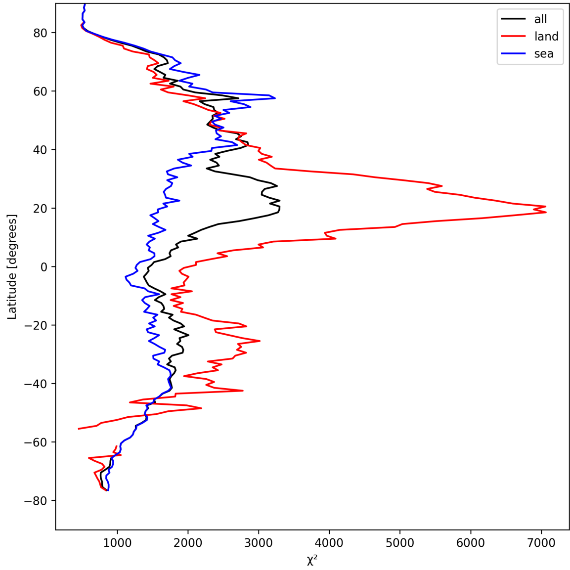
Figure 14: Zonal average of “ \chi^2 ” for 2025-04-09 to 2025-04-11.
