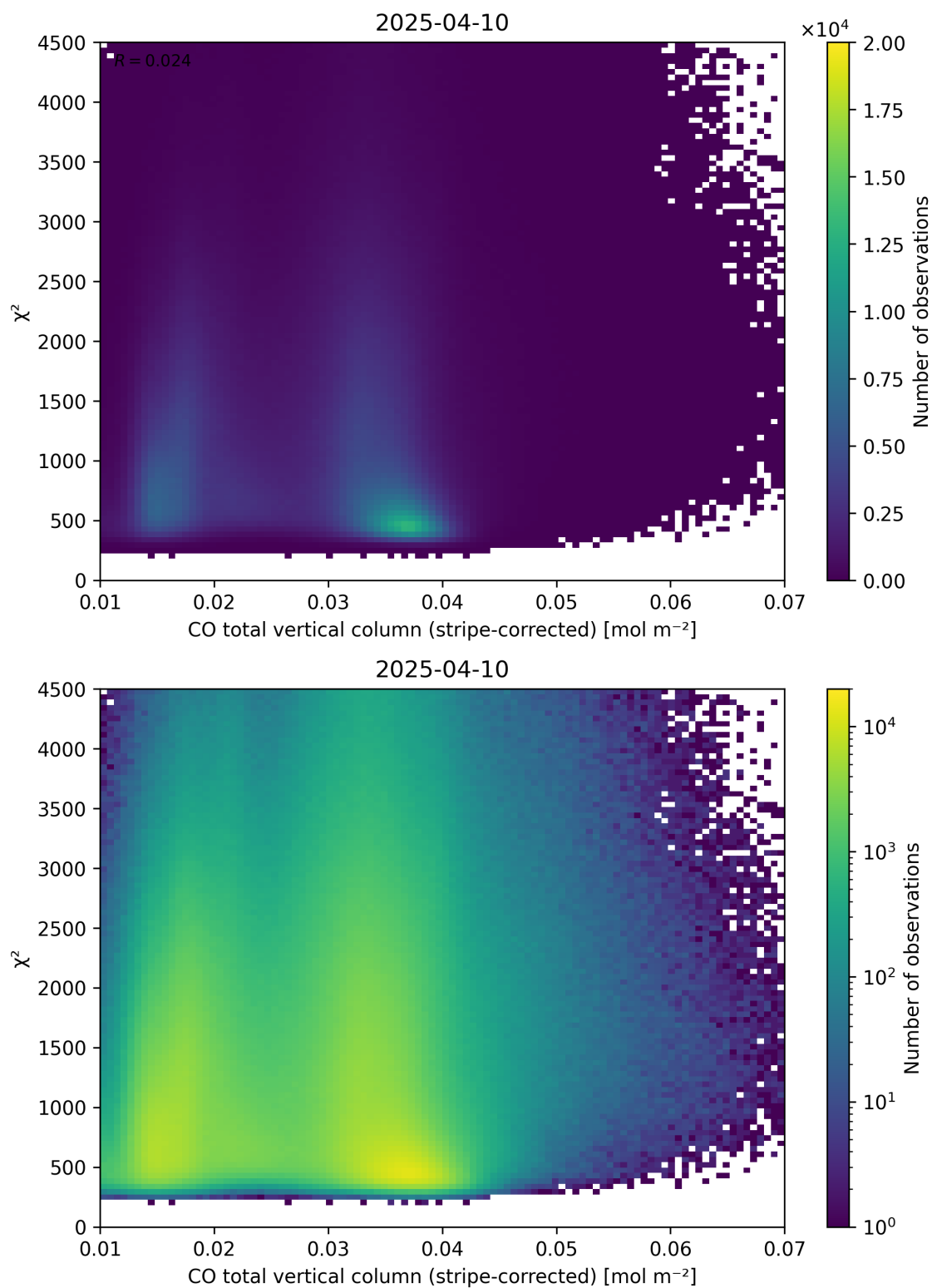
Figure 37: Scatter density plot of “CO total vertical column (stripe-corrected)” against “ \chi^2 ” for 2025-04-09 to 2025-04-11.
