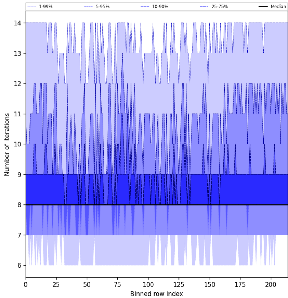
Figure 32: Along track statistics of “Number of iterations” for 2025-04-09 to 2025-04-11
