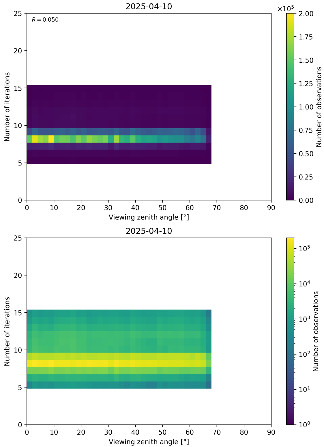
Figure 75: Scatter density plot of “Viewing zenith angle” against “Number of iterations” for 2025-04-09 to 2025-04-11.
