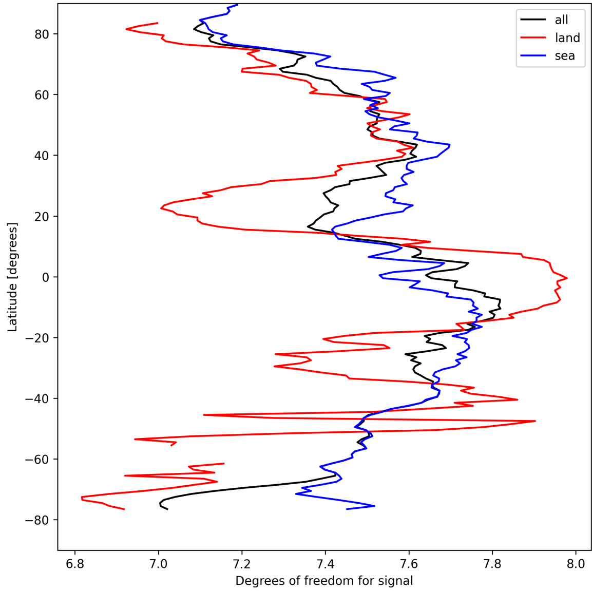
Figure 15: Zonal average of “Degrees of freedom for signal” for 2025-04-09 to 2025-04-11.
