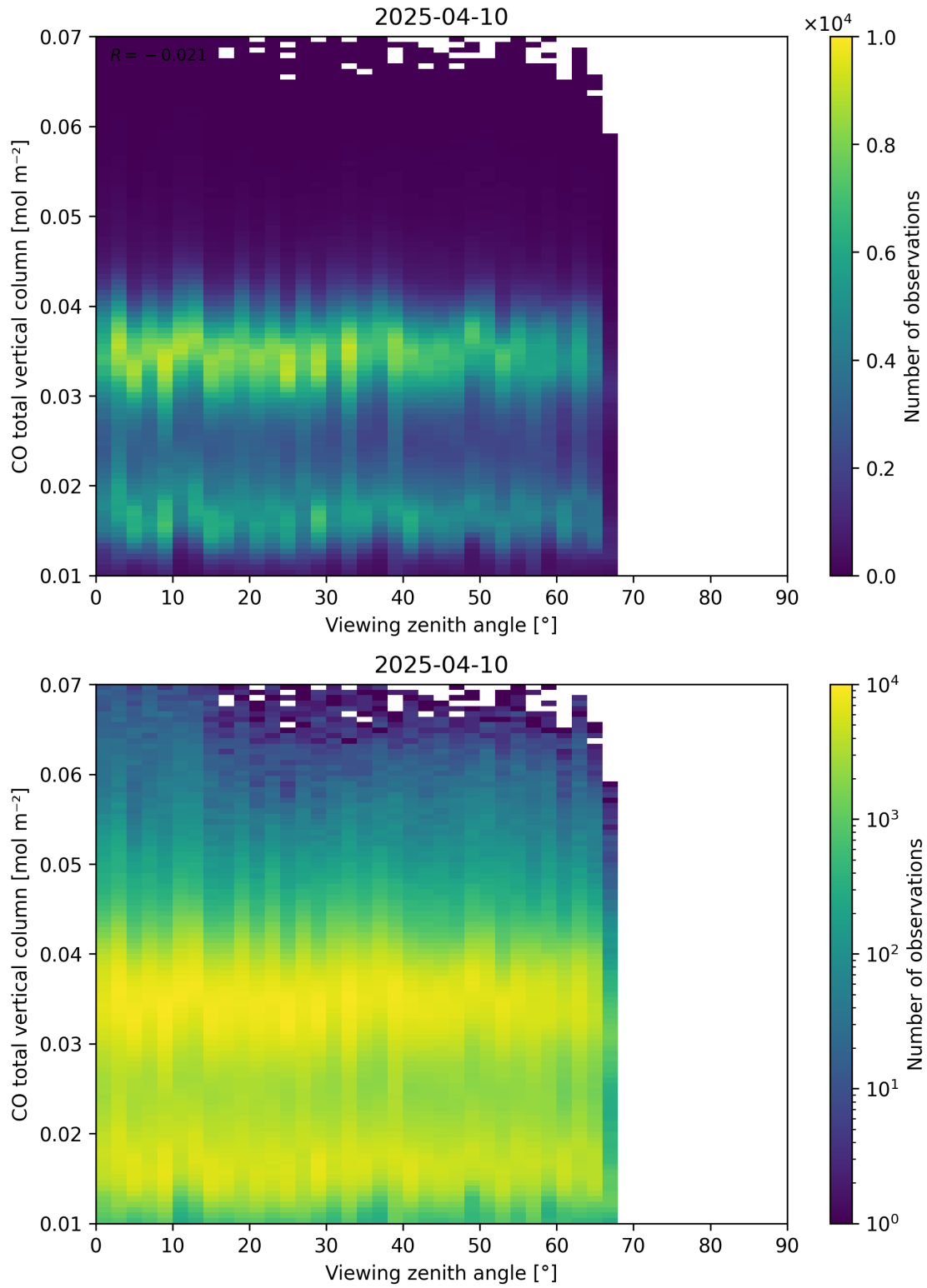
Figure 69: Scatter density plot of “Viewing zenith angle” against “CO total vertical column” for 2025-04-09 to 2025-04-11.
