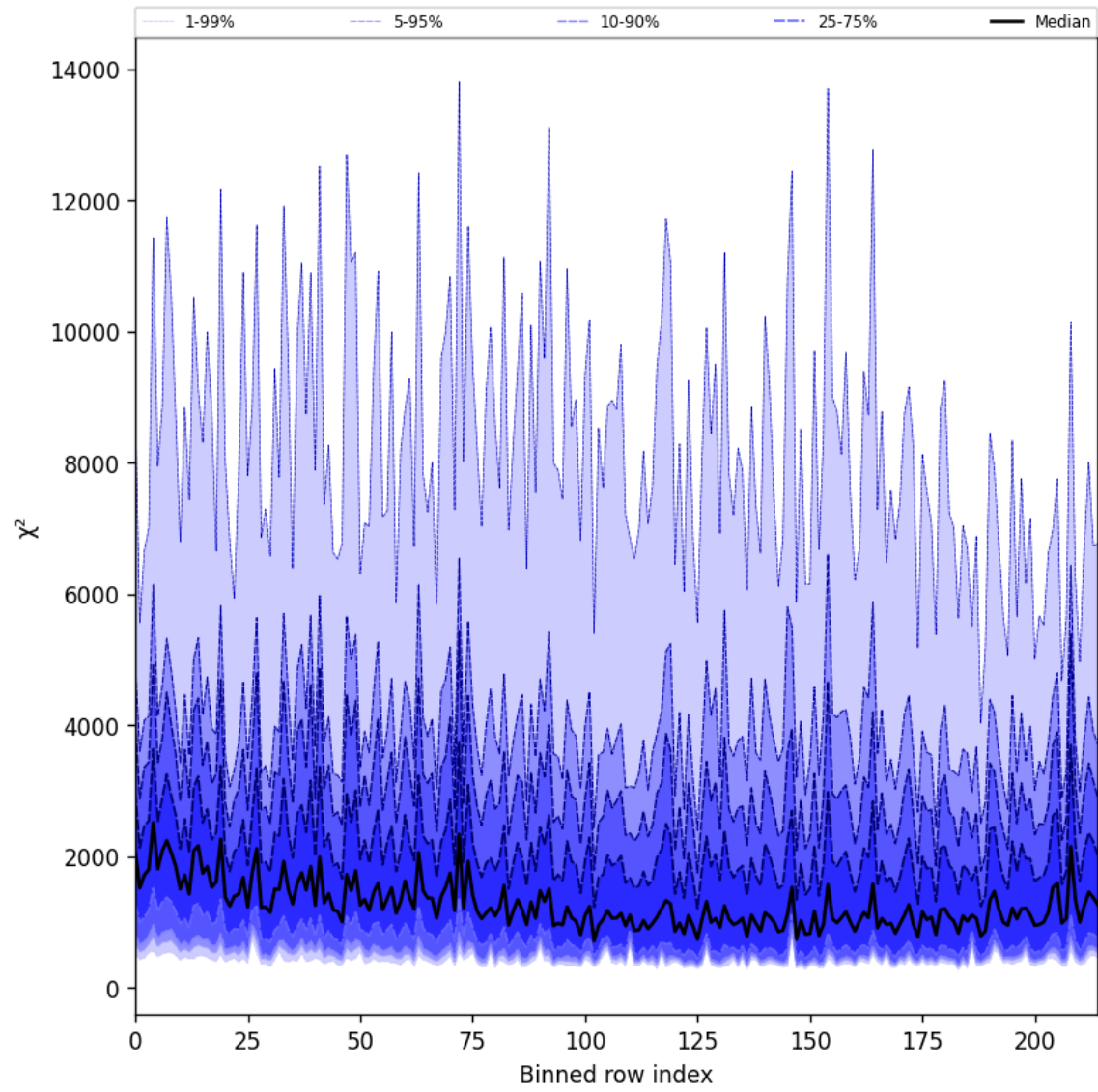
Figure 30: Along track statistics of “ \chi^2 ” for 2025-04-09 to 2025-04-11
