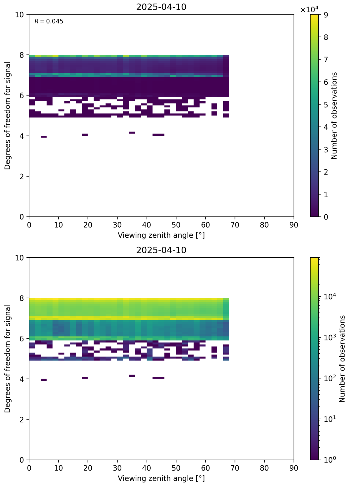
Figure 73: Scatter density plot of “Viewing zenith angle” against “Degrees of freedom for signal” for 2025-04-09 to 2025-04-11.
