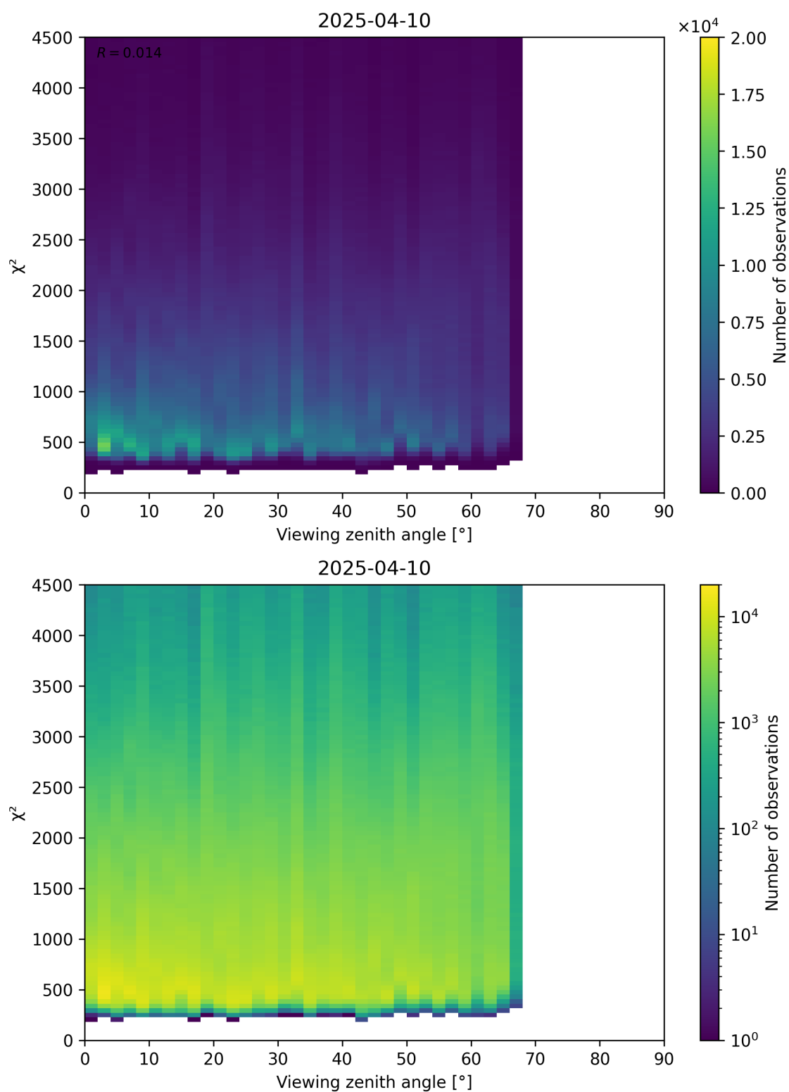
Figure 72: Scatter density plot of “Viewing zenith angle” against “ \chi^2 ” for 2025-04-09 to 2025-04-11.
