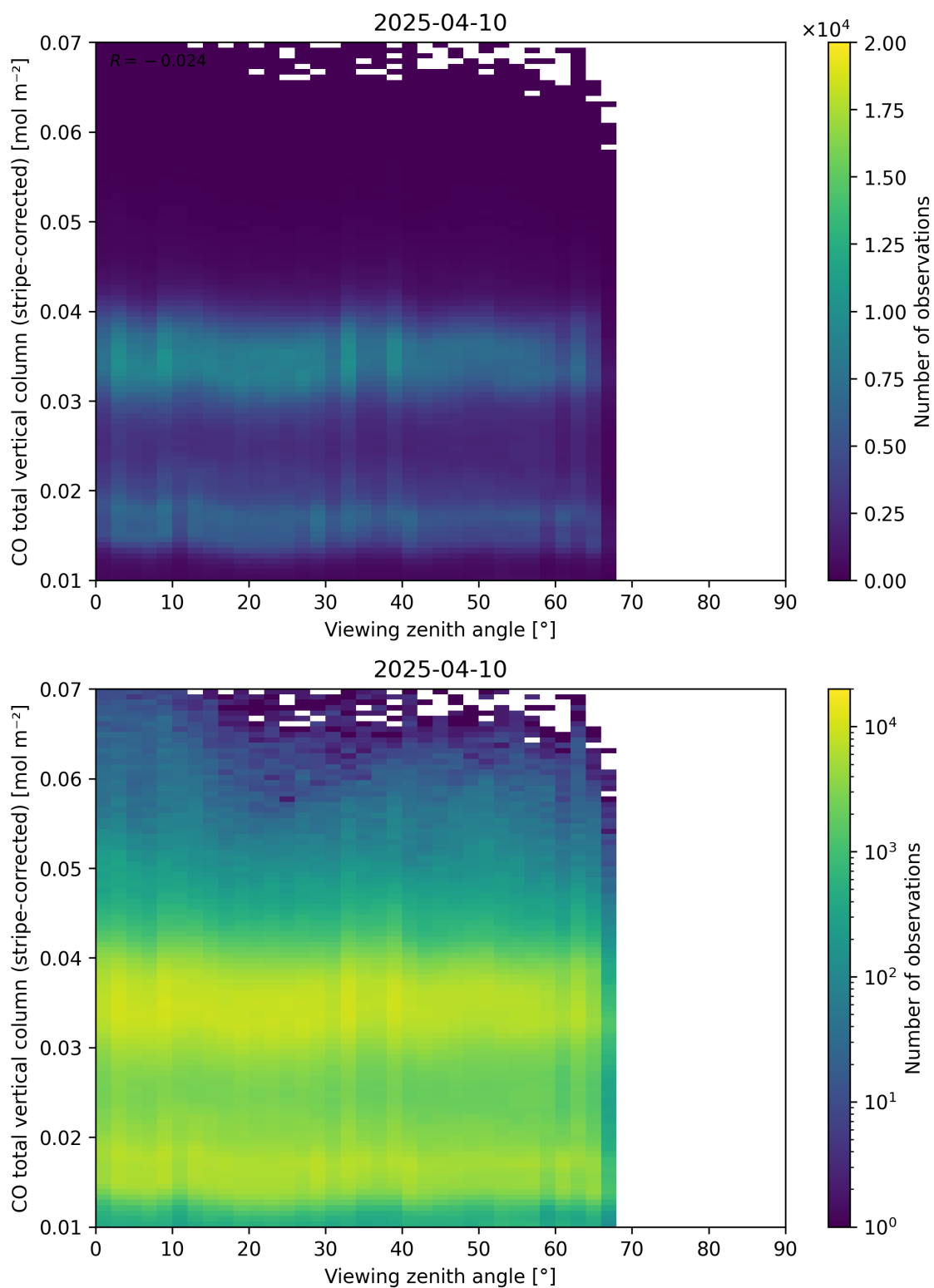
Figure 70: Scatter density plot of “Viewing zenith angle” against “CO total vertical column (stripe-corrected)” for 2025-04-09 to 2025-04-11.
