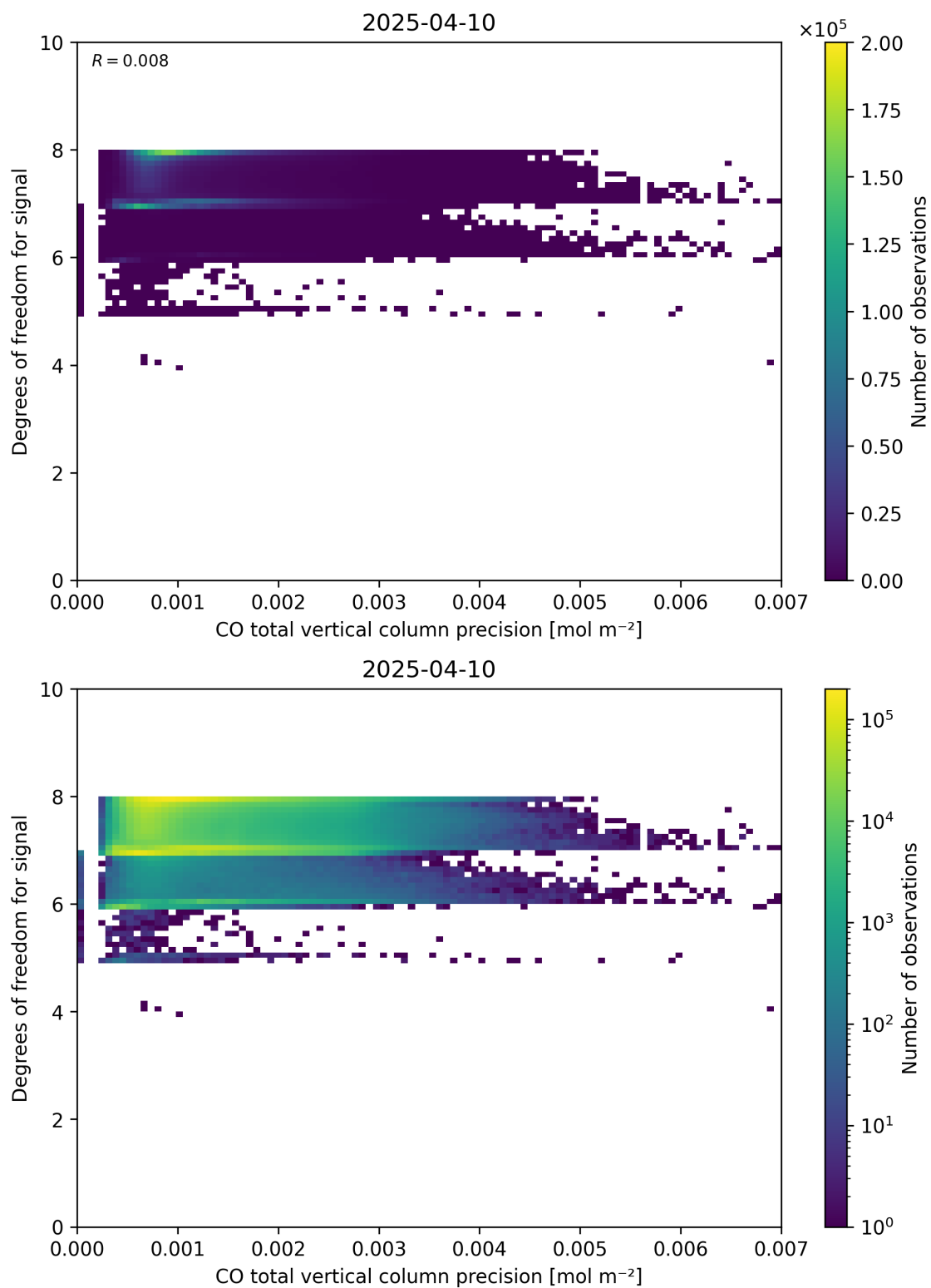
Figure 45: Scatter density plot of “CO total vertical column precision” against “Degrees of freedom for signal” for 2025-04-09 to 2025-04-11.
