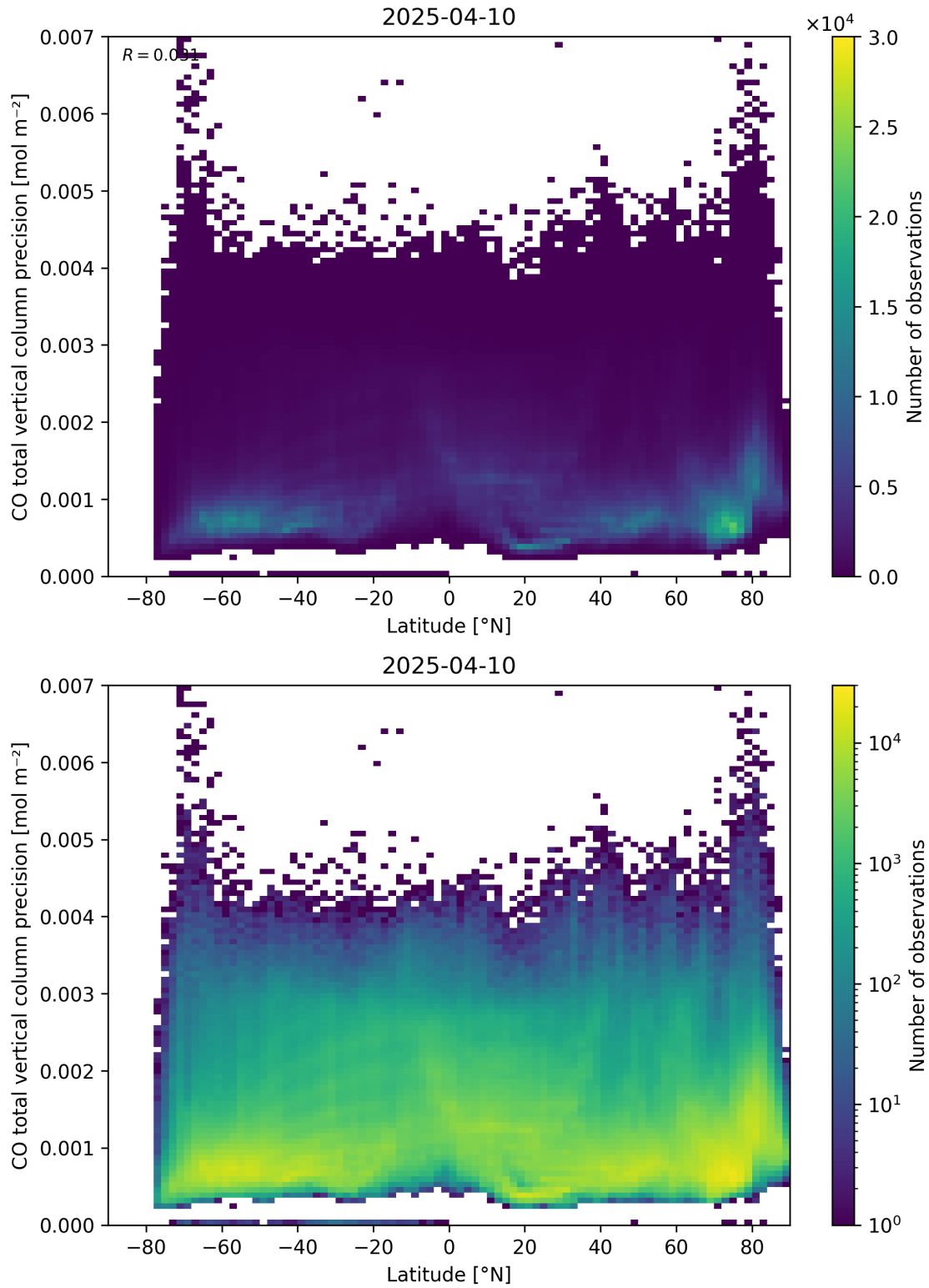
Figure 53: Scatter density plot of “Latitude” against “CO total vertical column precision” for 2025-04-09 to 2025-04-11.
