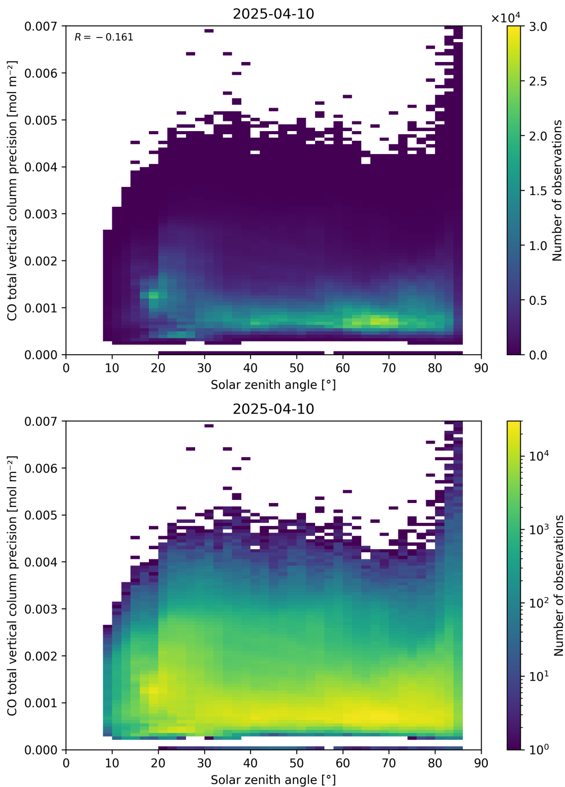
Figure 63: Scatter density plot of “Solar zenith angle” against “CO total vertical column precision” for 2025-04-09 to 2025-04-11.
