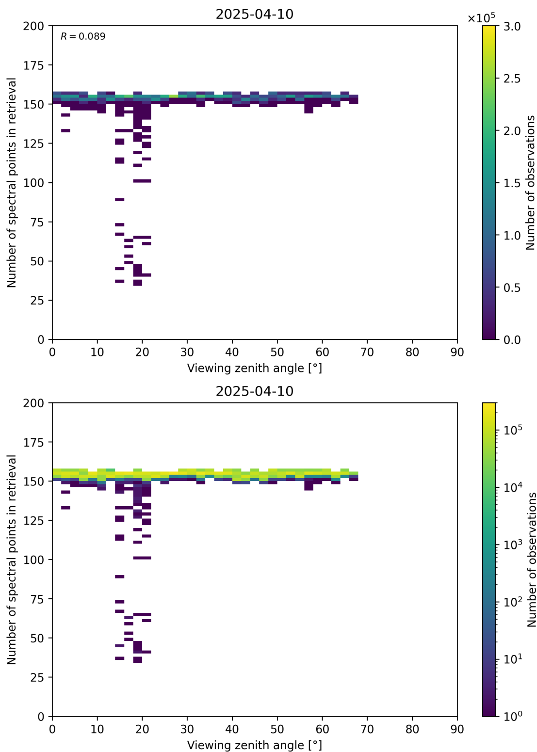
Figure 76: Scatter density plot of “Viewing zenith angle” against “Number of spectral points in retrieval” for 2025-04-09 to 2025-04-11.
