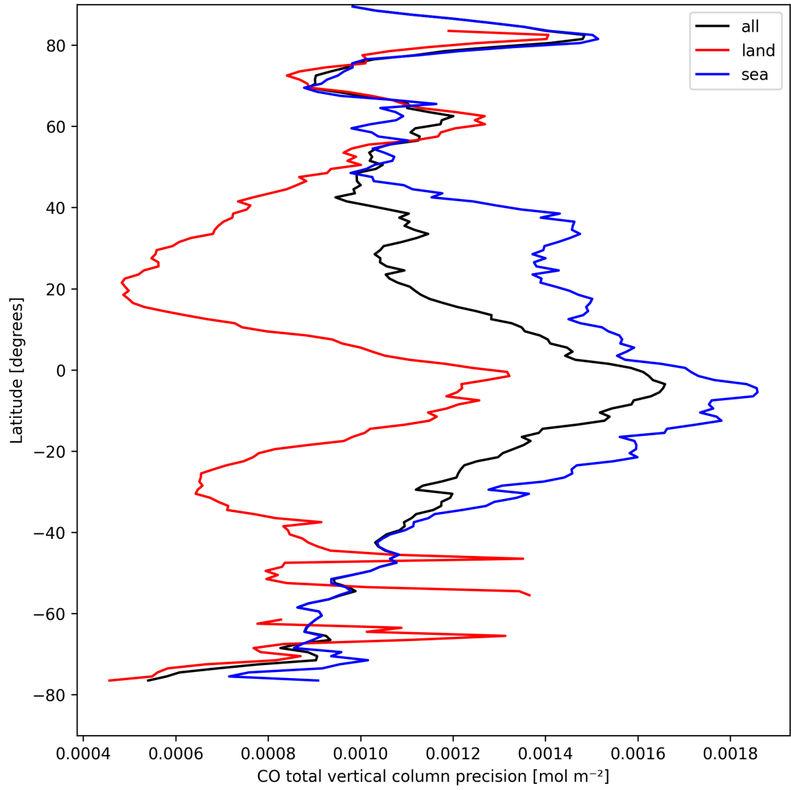
Figure 12: Zonal average of “CO total vertical column precision” for 2025-04-09 to 2025-04-11.
