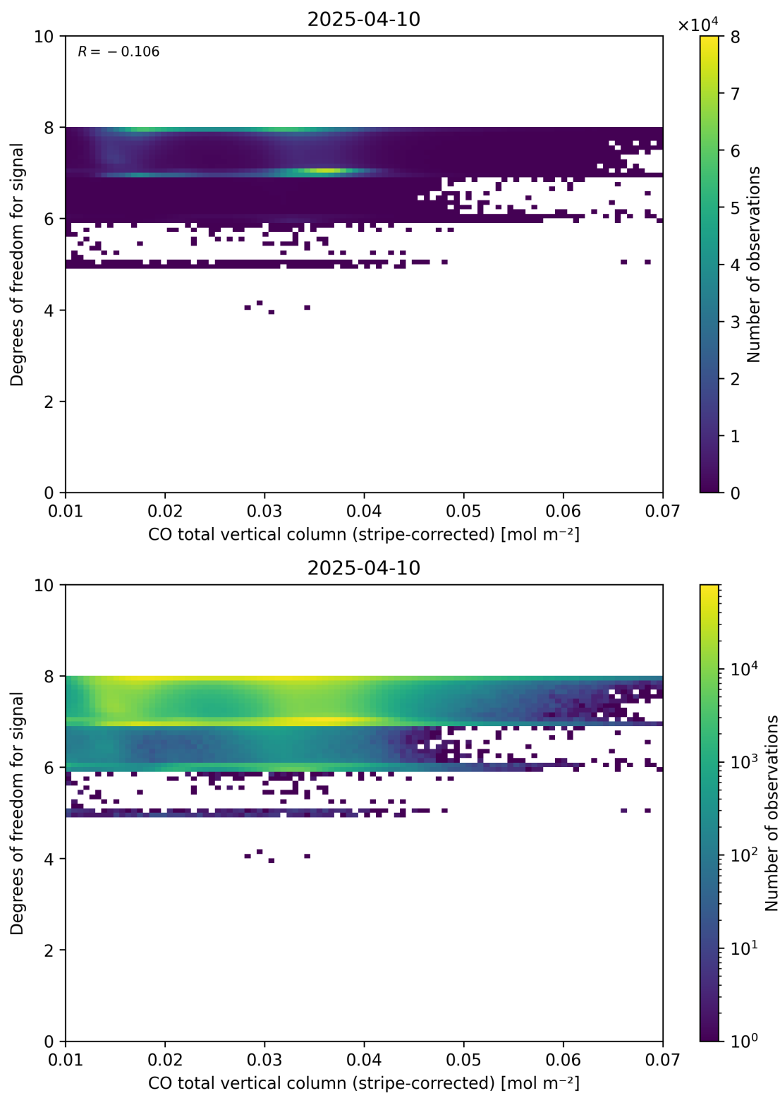
Figure 38: Scatter density plot of “CO total vertical column (stripe-corrected)” against “Degrees of freedom for signal” for 2025-04-09 to 2025-04-11.
