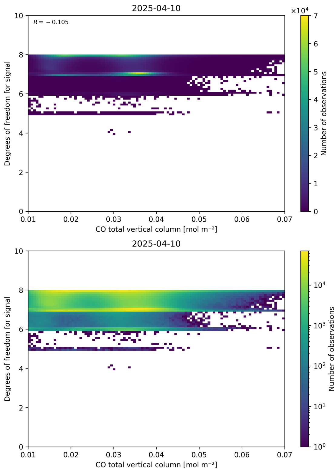
Figure 41: Scatter density plot of “CO total vertical column” against “Degrees of freedom for signal” for 2025-04-09 to 2025-04-11.
