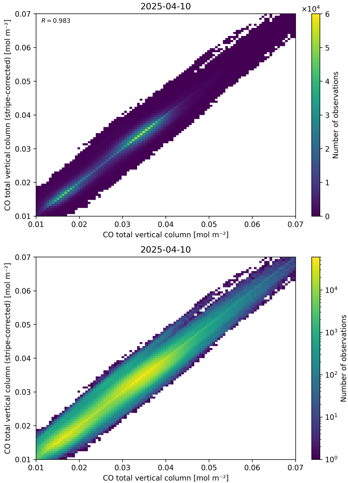
Figure 33: Scatter density plot of “CO total vertical column” against “CO total vertical column (stripe-corrected)” for 2025-04-09 to 2025-04-11.
