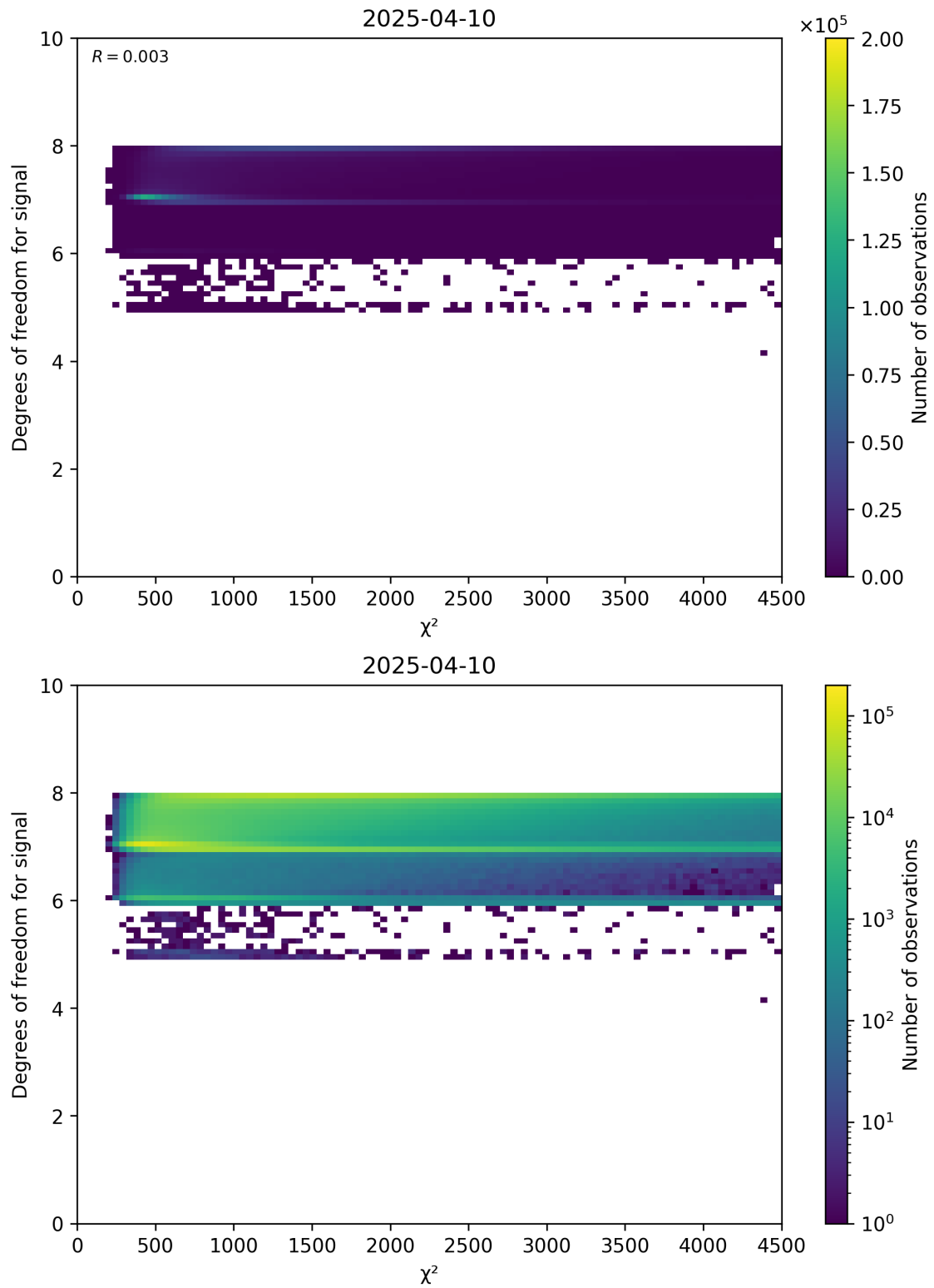
Figure 48: Scatter density plot of “ \chi^2 ” against “Degrees of freedom for signal” for 2025-04-09 to 2025-04-11.
