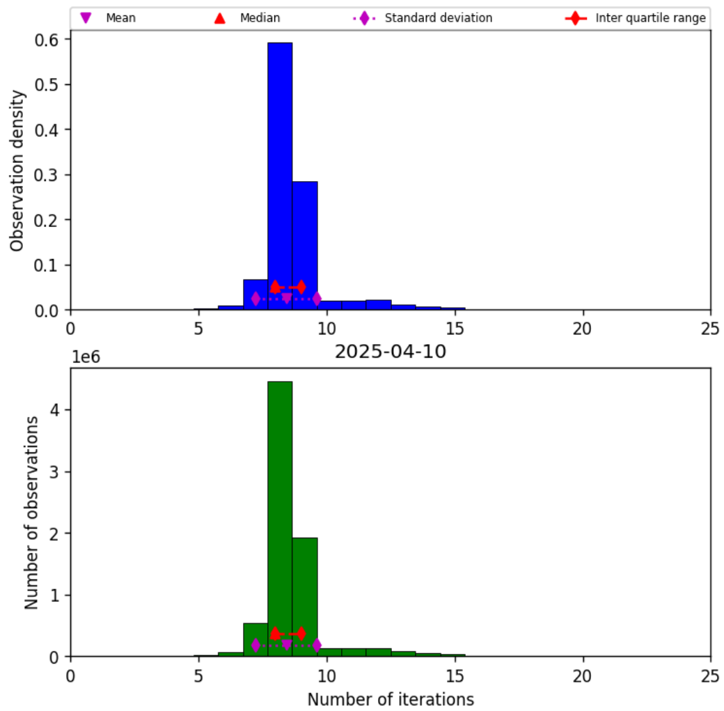
Figure 24: Histogram of “Number of iterations” for 2025-04-09 to 2025-04-11
