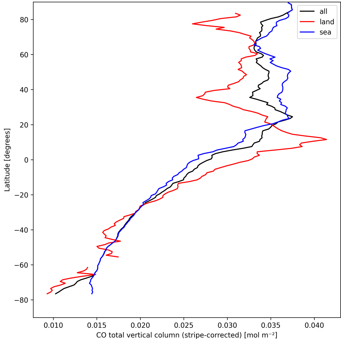
Figure 11: Zonal average of “CO total vertical column (stripe-corrected)” for 2025-04-09 to 2025-04-11.
