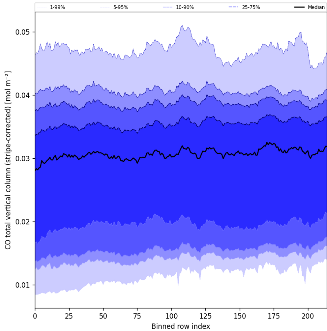
Figure 27: Along track statistics of “CO total vertical column (stripe-corrected)” for 2025-04-09 to 2025-04-11
