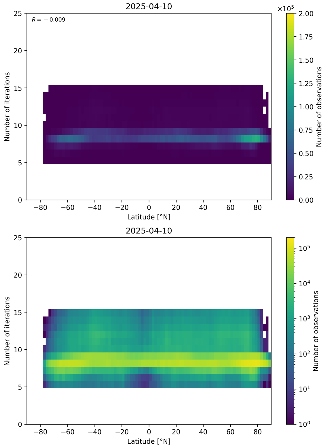
Figure 56: Scatter density plot of “Latitude” against “Number of iterations” for 2025-04-09 to 2025-04-11.
