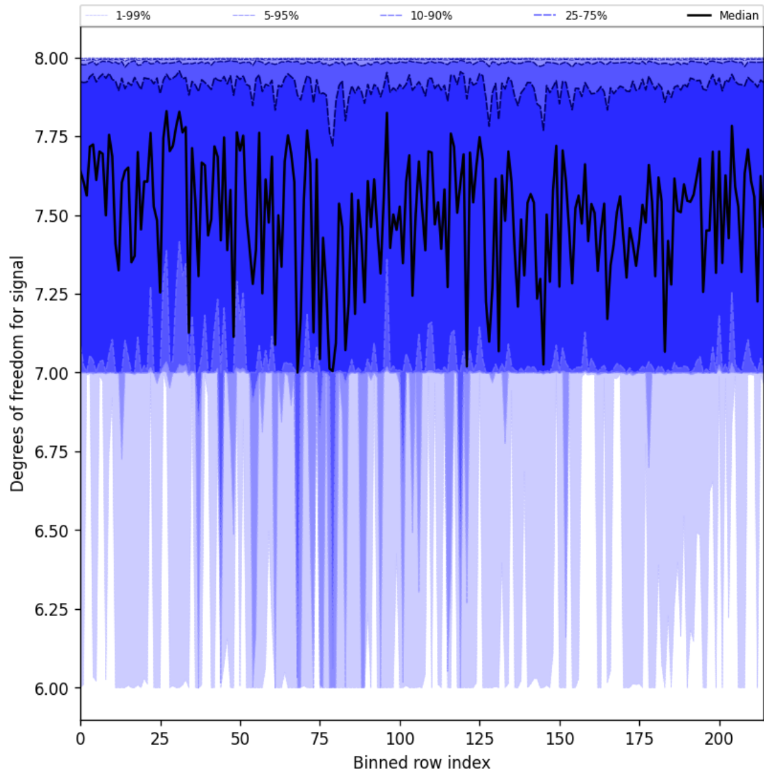
Figure 31: Along track statistics of “Degrees of freedom for signal” for 2025-04-09 to 2025-04-11
