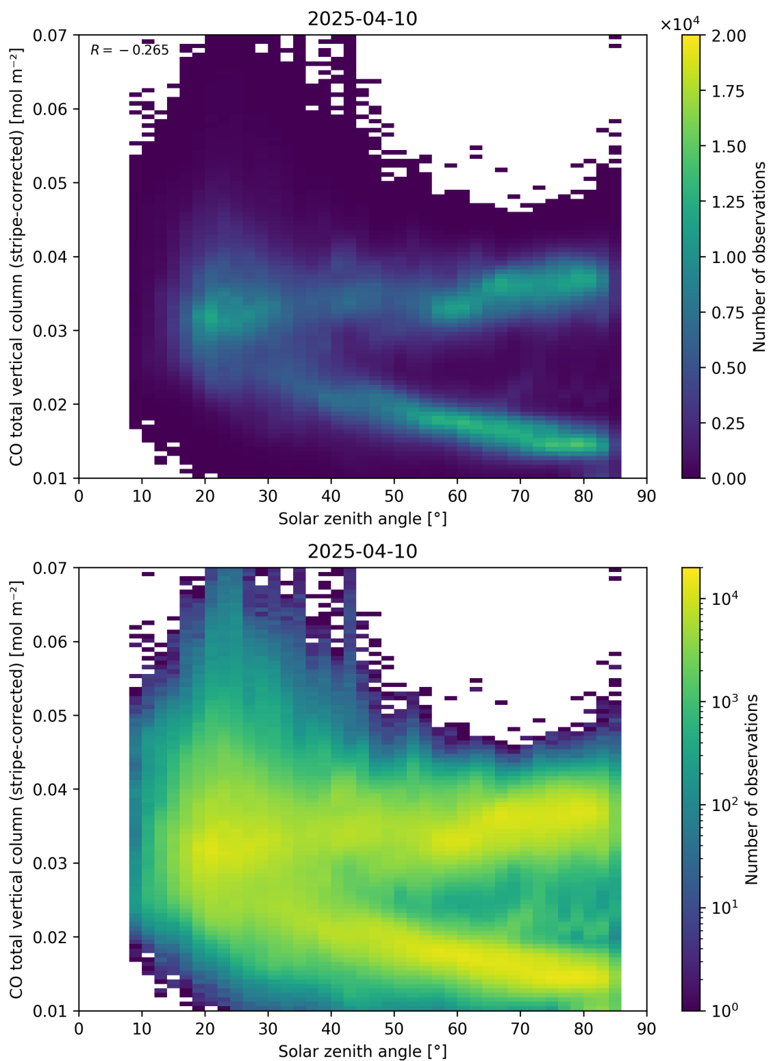
Figure 62: Scatter density plot of “Solar zenith angle” against “CO total vertical column (stripe-corrected)” for 2025-04-09 to 2025-04-11.
