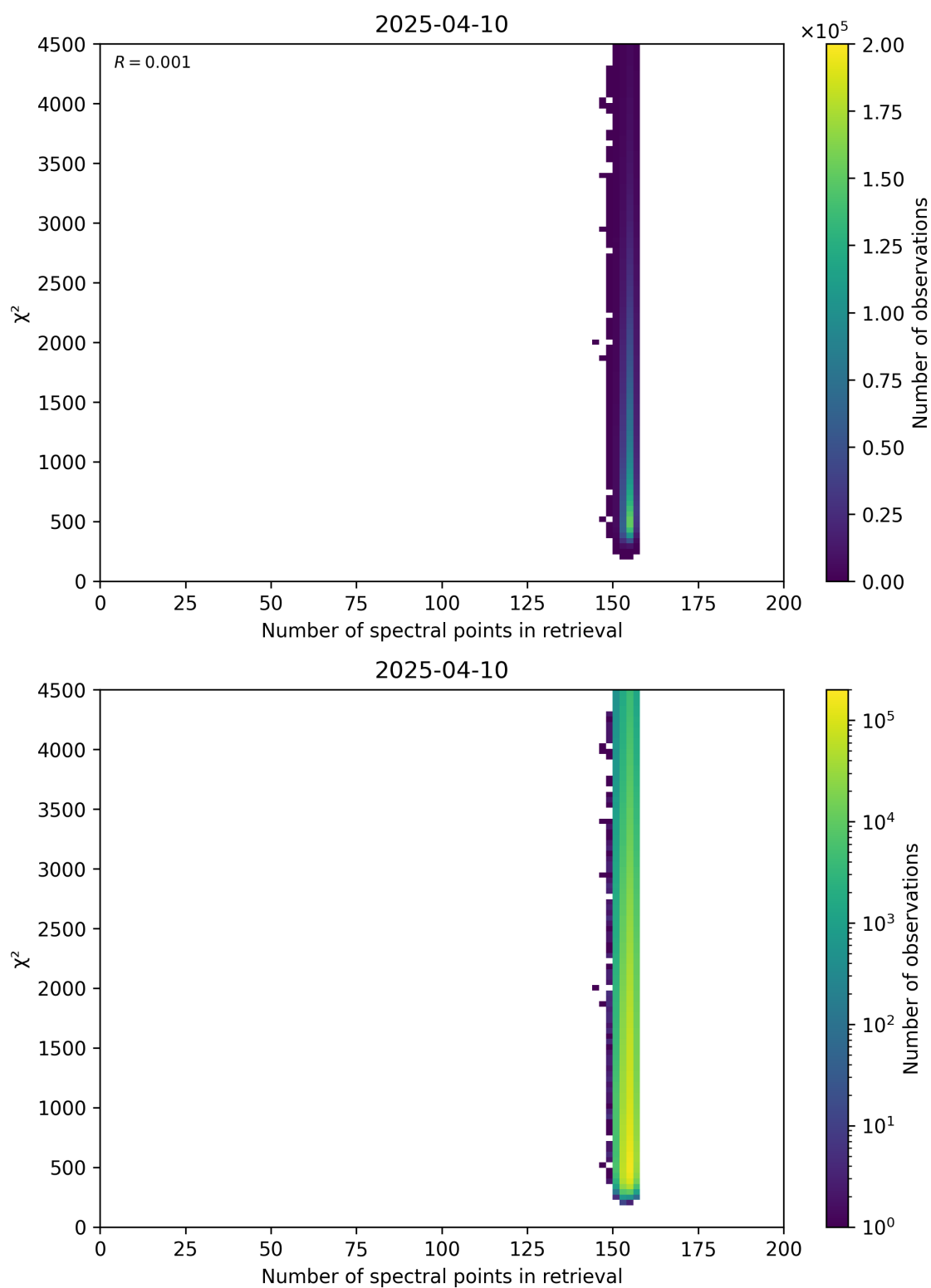
Figure 58: Scatter density plot of “Number of spectral points in retrieval” against “ \chi^2 ” for 2025-04-09 to 2025-04-11.
