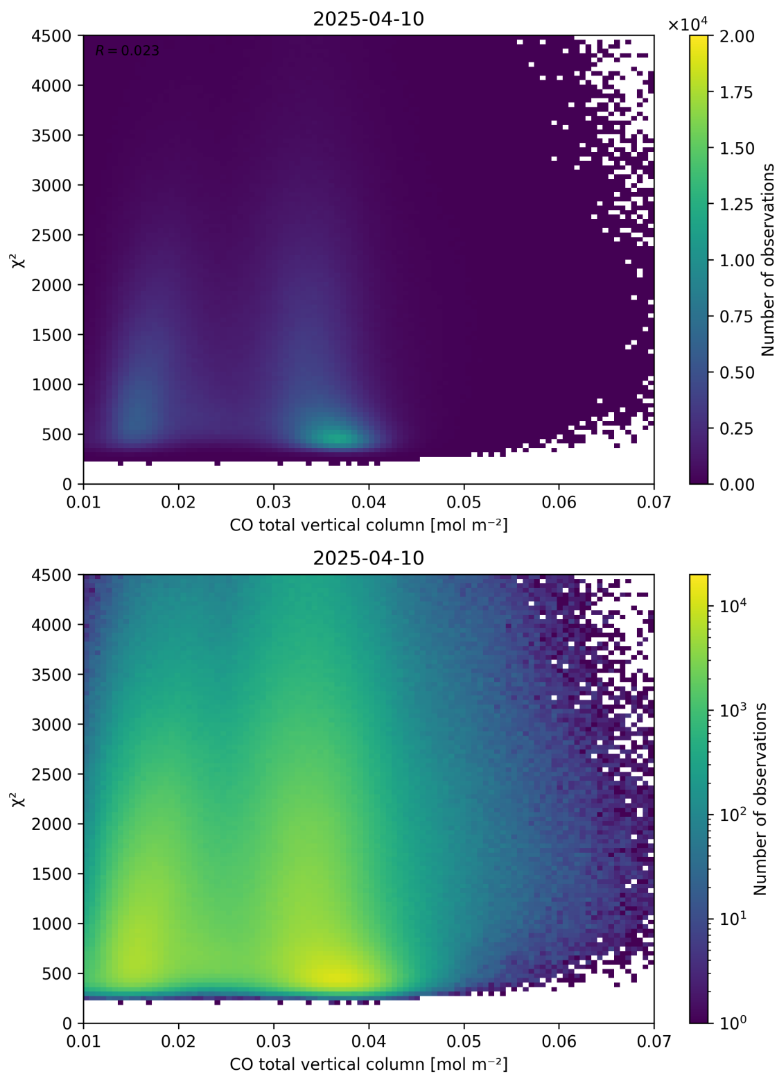
Figure 35: Scatter density plot of “CO total vertical column” against “ \chi^2 ” for 2025-04-09 to 2025-04-11.
