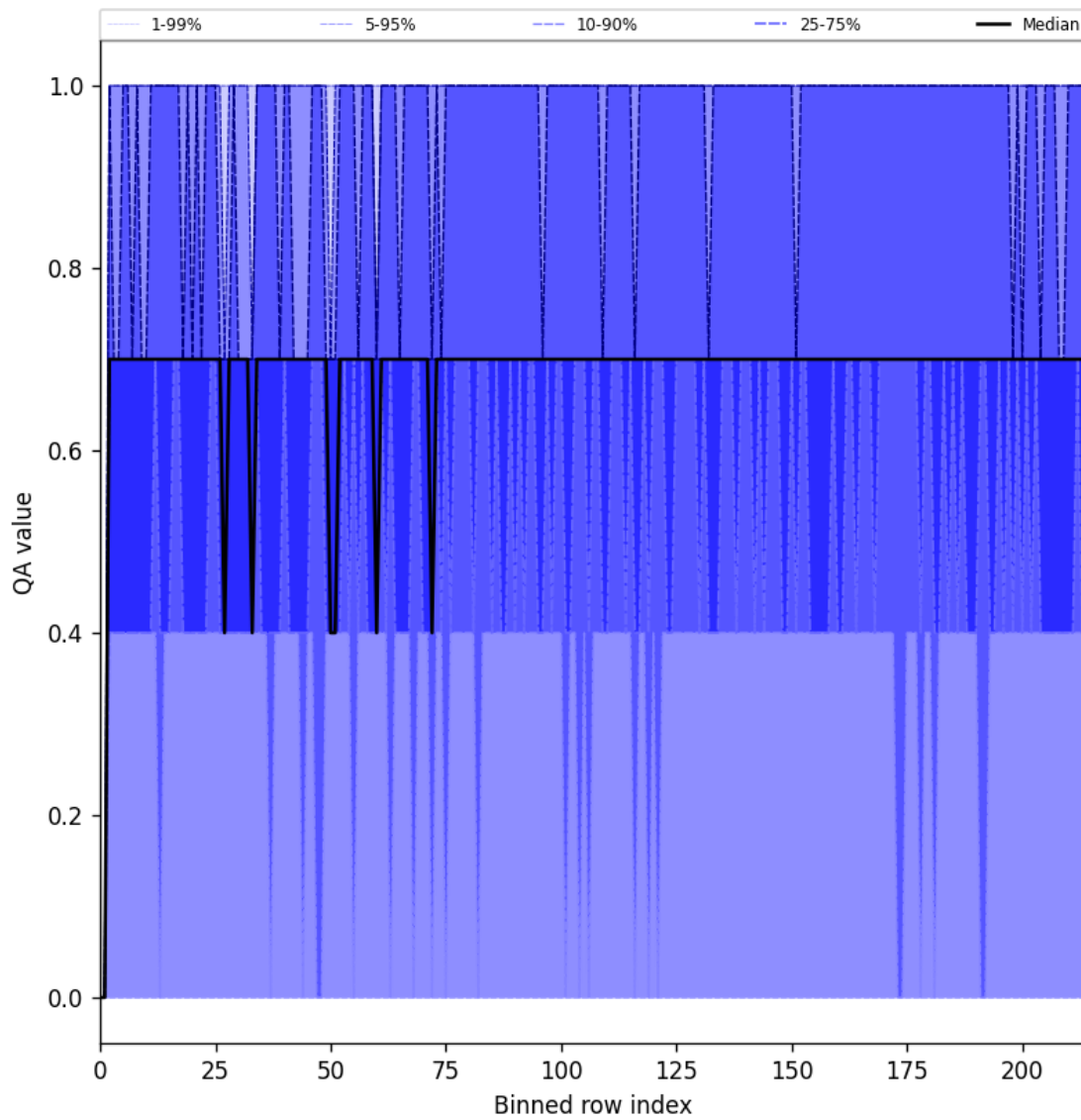
Figure 25: Along track statistics of “QA value” for 2025-04-09 to 2025-04-11
