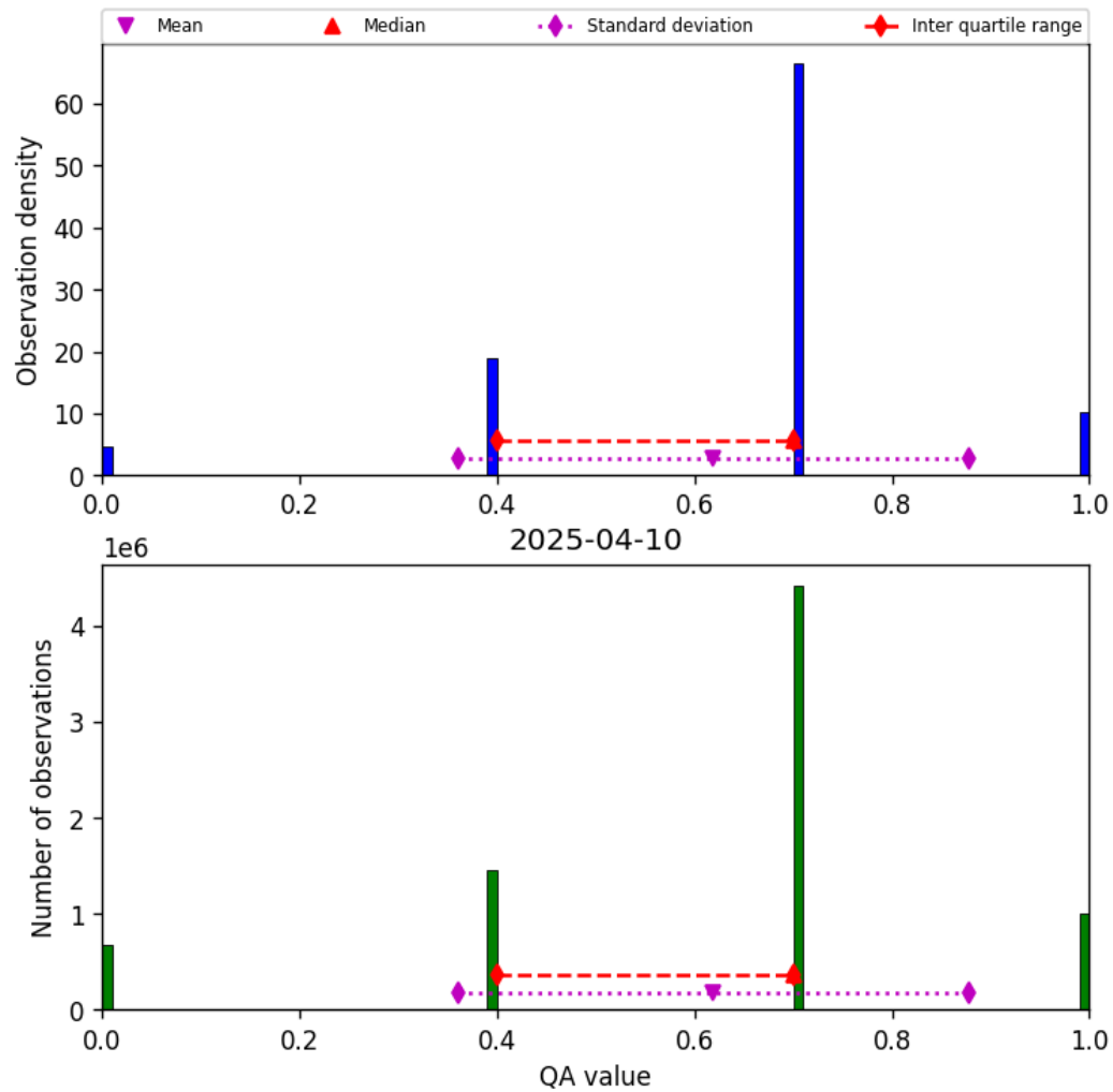
Figure 17: Histogram of “QA value” for 2025-04-09 to 2025-04-11
