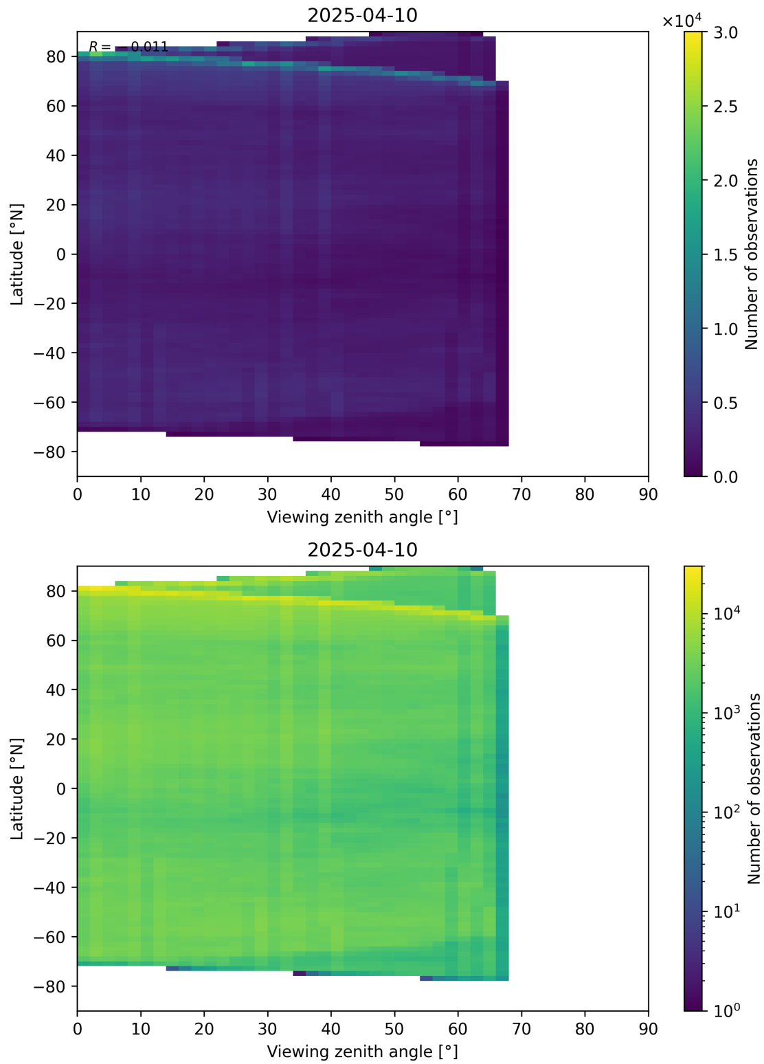
Figure 74: Scatter density plot of “Viewing zenith angle” against “Latitude” for 2025-04-09 to 2025-04-11.
