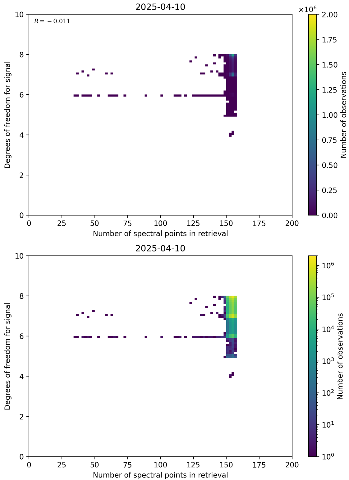
Figure 59: Scatter density plot of “Number of spectral points in retrieval” against “Degrees of freedom for signal” for 2025-04-09 to 2025-04-11.
