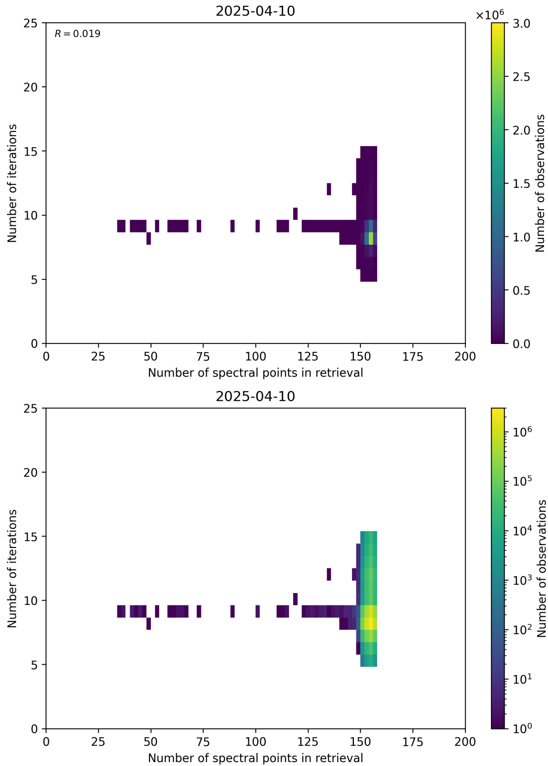
Figure 60: Scatter density plot of “Number of spectral points in retrieval” against “Number of iterations” for 2025-04-09 to 2025-04-11.
