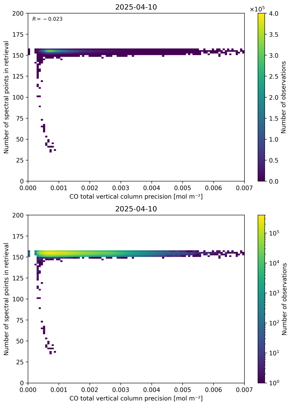
Figure 47: Scatter density plot of “CO total vertical column precision” against “Number of spectral points in retrieval” for 2025-04-09 to 2025-04-11.
