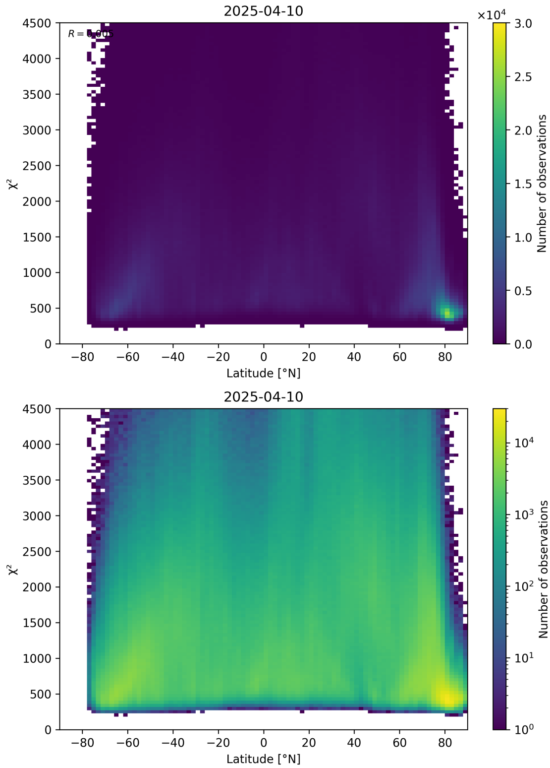
Figure 54: Scatter density plot of “Latitude” against “ \chi^2 ” for 2025-04-09 to 2025-04-11.
