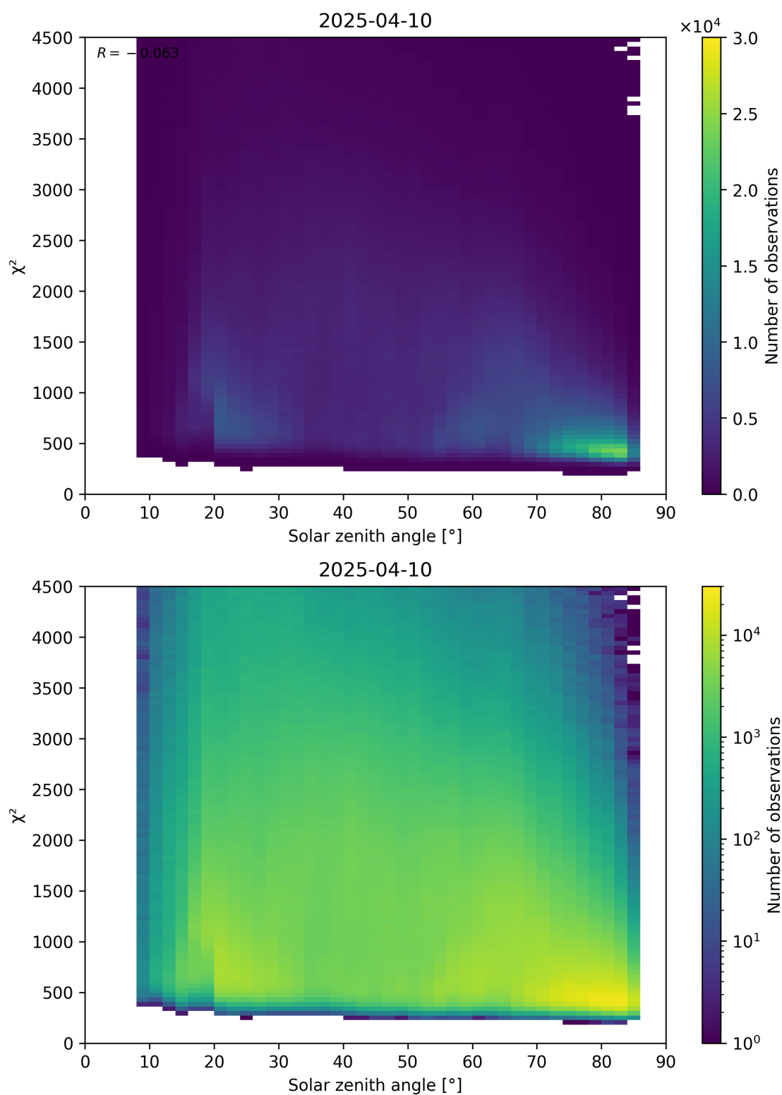
Figure 64: Scatter density plot of “Solar zenith angle” against “ \chi^2 ” for 2025-04-09 to 2025-04-11.
