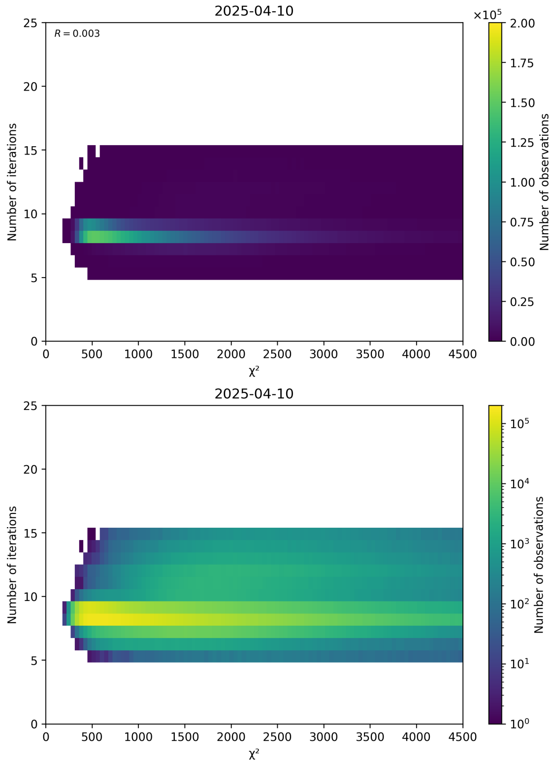
Figure 49: Scatter density plot of “ \chi^2 ” against “Number of iterations” for 2025-04-09 to 2025-04-11.
