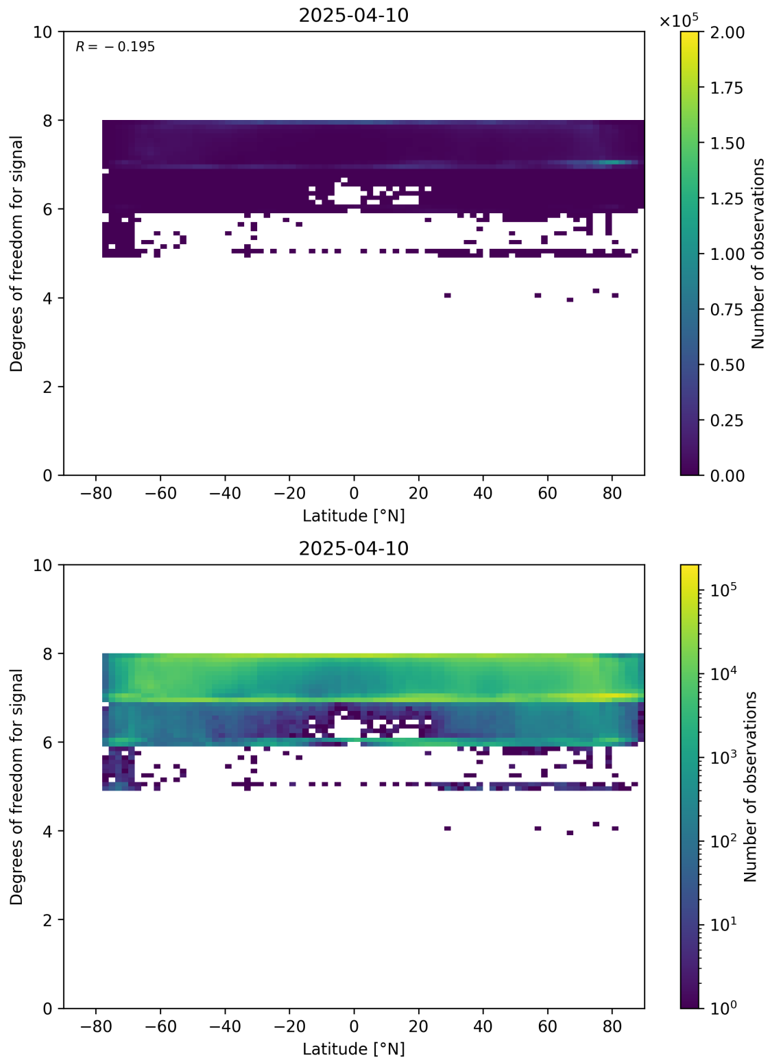
Figure 55: Scatter density plot of “Latitude” against “Degrees of freedom for signal” for 2025-04-09 to 2025-04-11.
