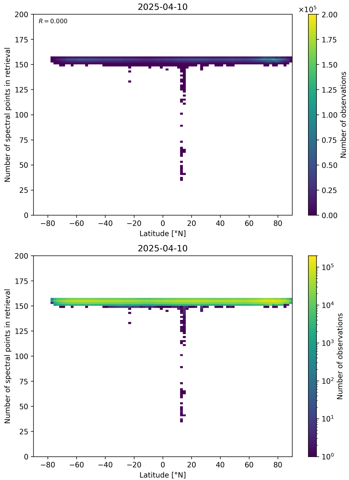
Figure 57: Scatter density plot of “Latitude” against “Number of spectral points in retrieval” for 2025-04-09 to 2025-04-11.
