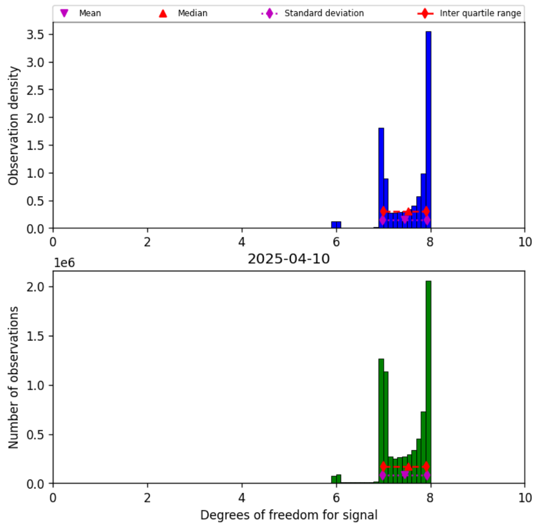
Figure 23: Histogram of “Degrees of freedom for signal” for 2025-04-09 to 2025-04-11
