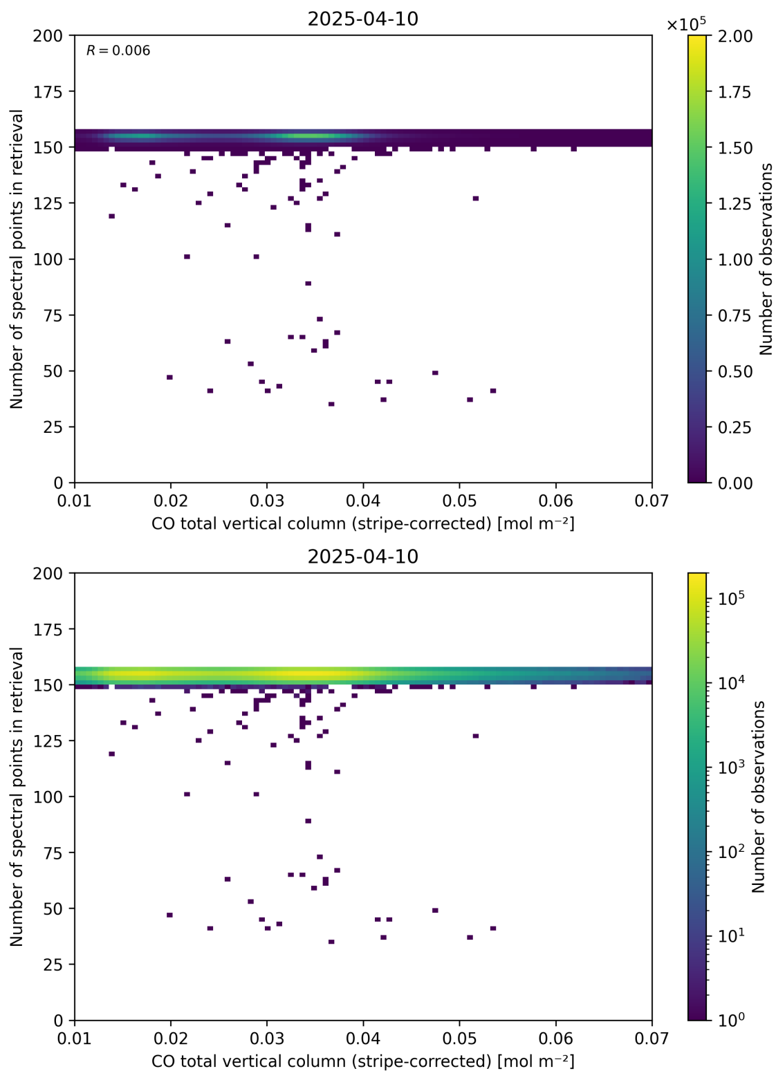
Figure 40: Scatter density plot of “CO total vertical column (stripe-corrected)” against “Number of spectral points in retrieval” for 2025-04-09 to 2025-04-11.
