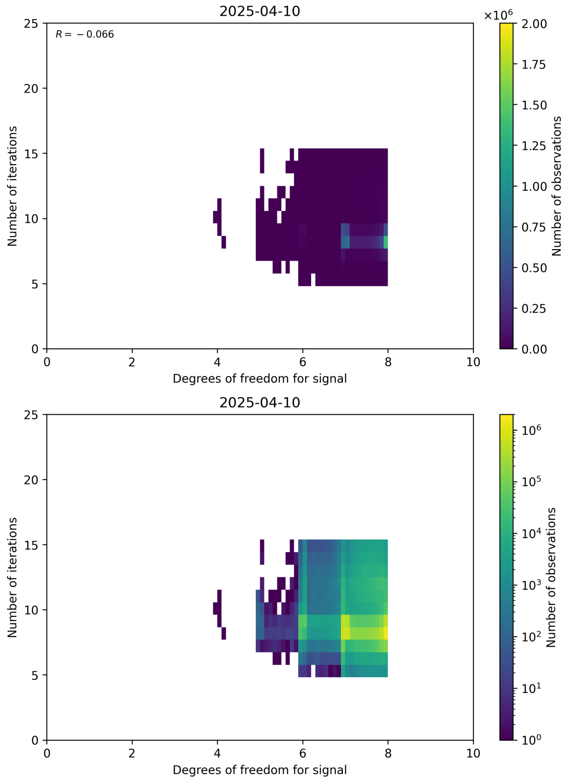
Figure 50: Scatter density plot of “Degrees of freedom for signal” against “Number of iterations” for 2025-04-09 to 2025-04-11.
