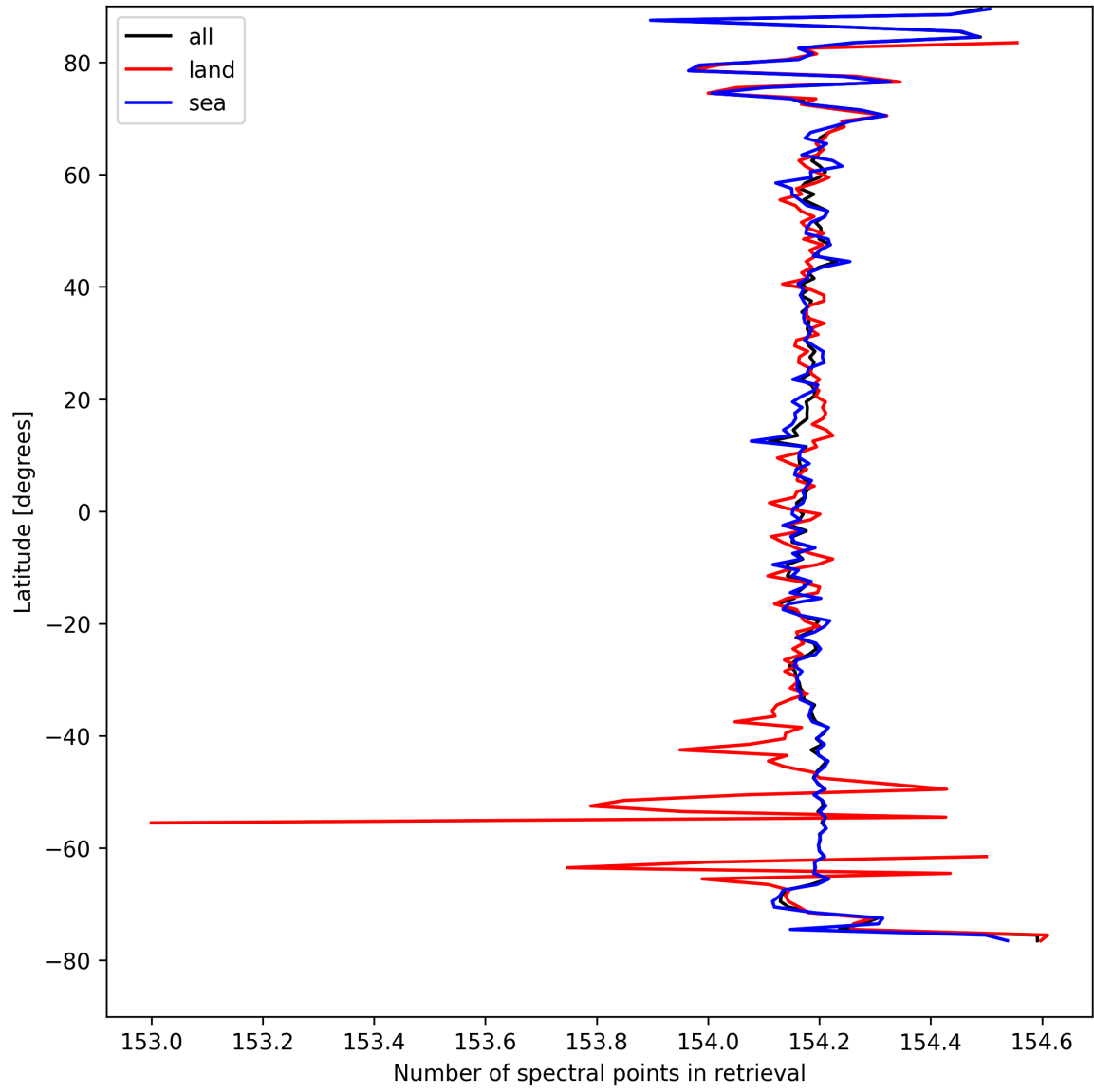
Figure 13: Zonal average of “Number of spectral points in retrieval” for 2025-04-09 to 2025-04-11.
