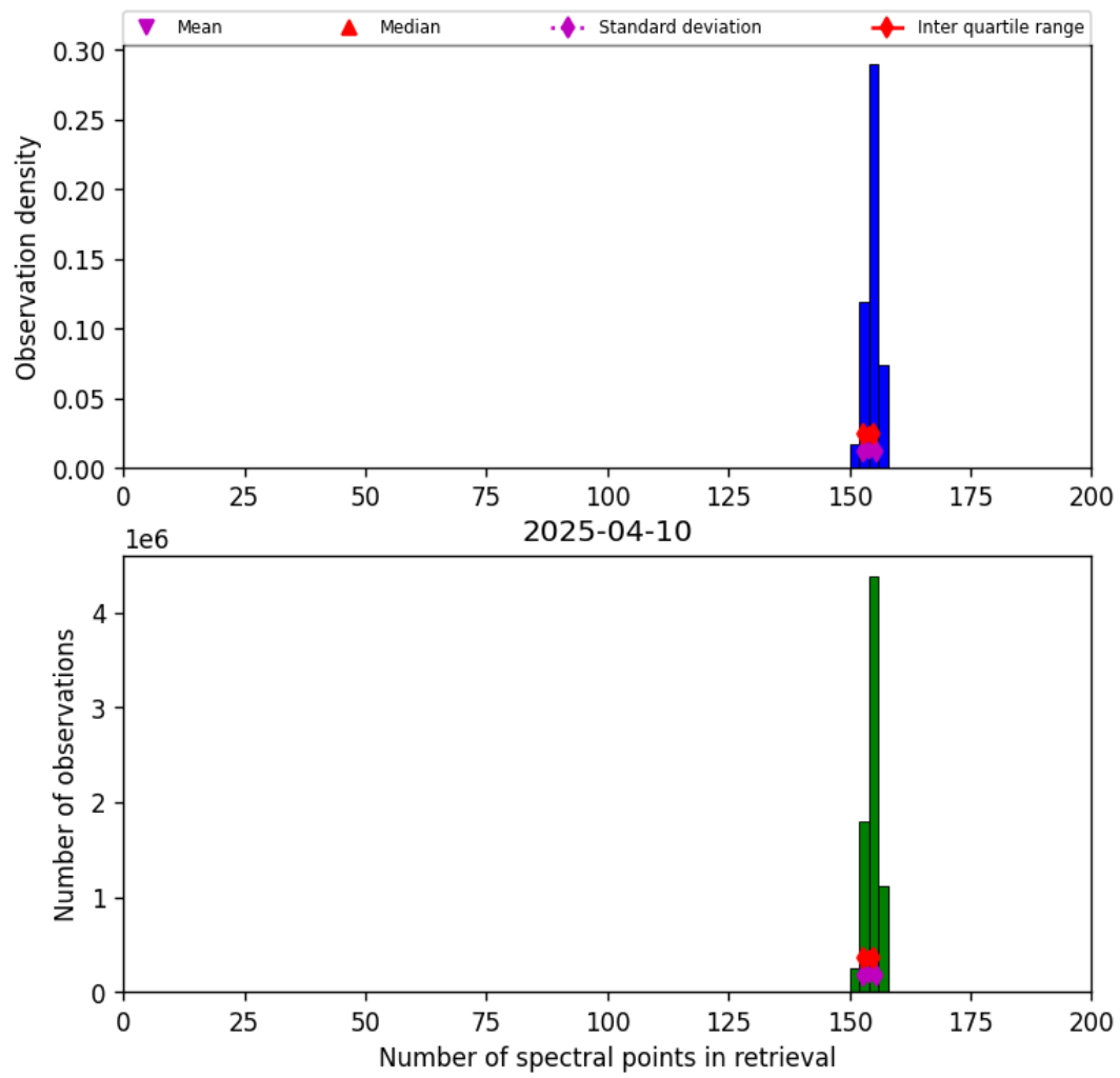
Figure 21: Histogram of “Number of spectral points in retrieval” for 2025-04-09 to 2025-04-11
