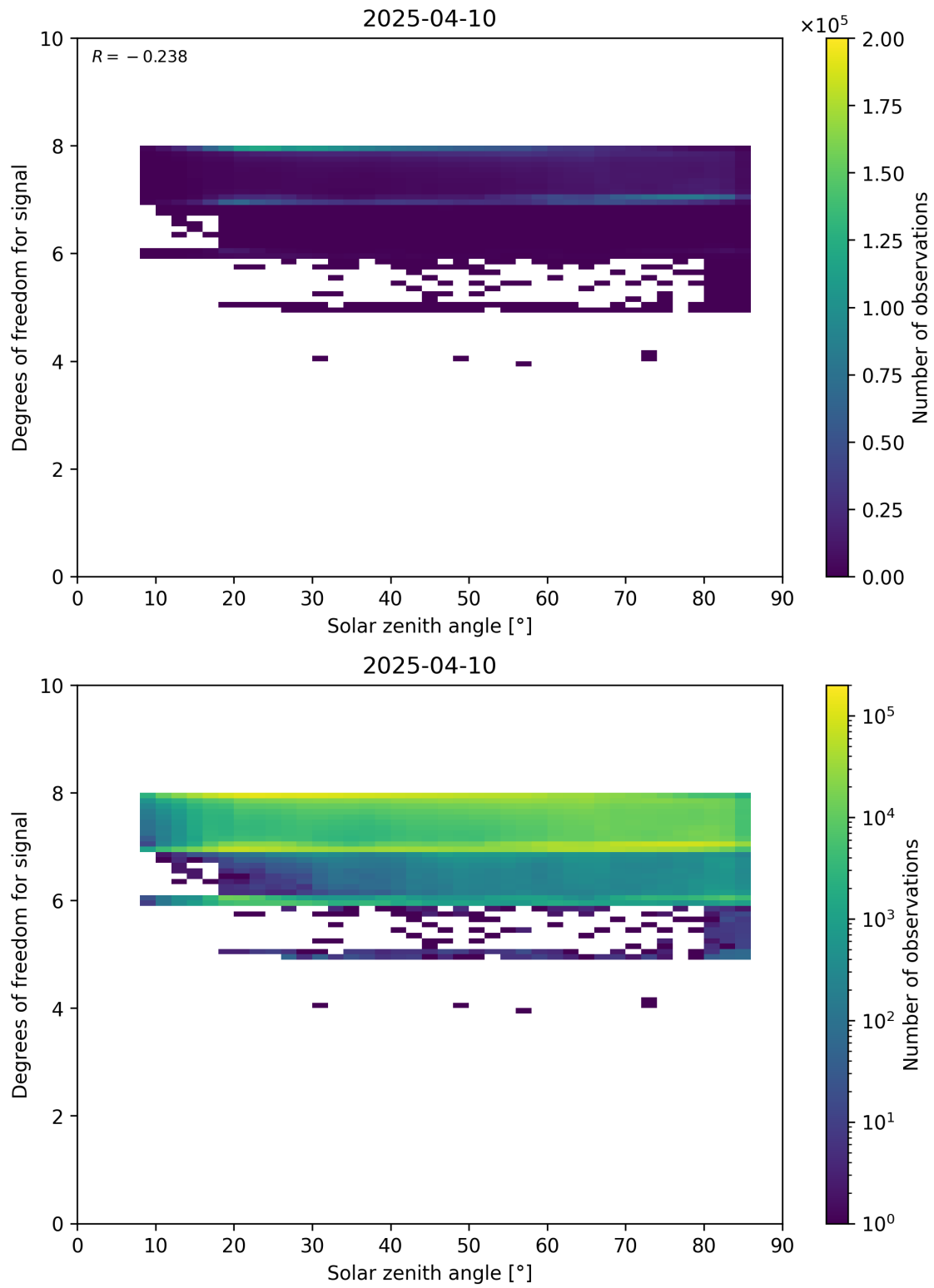
Figure 65: Scatter density plot of “Solar zenith angle” against “Degrees of freedom for signal” for 2025-04-09 to 2025-04-11.
