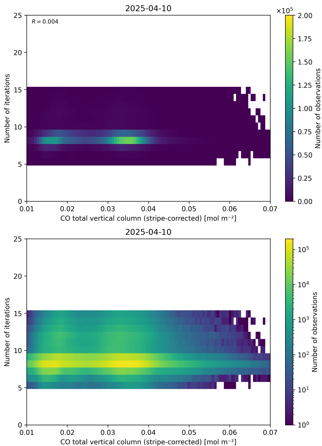
Figure 39: Scatter density plot of “CO total vertical column (stripe-corrected)” against “Number of iterations” for 2025-04-09 to 2025-04-11.
