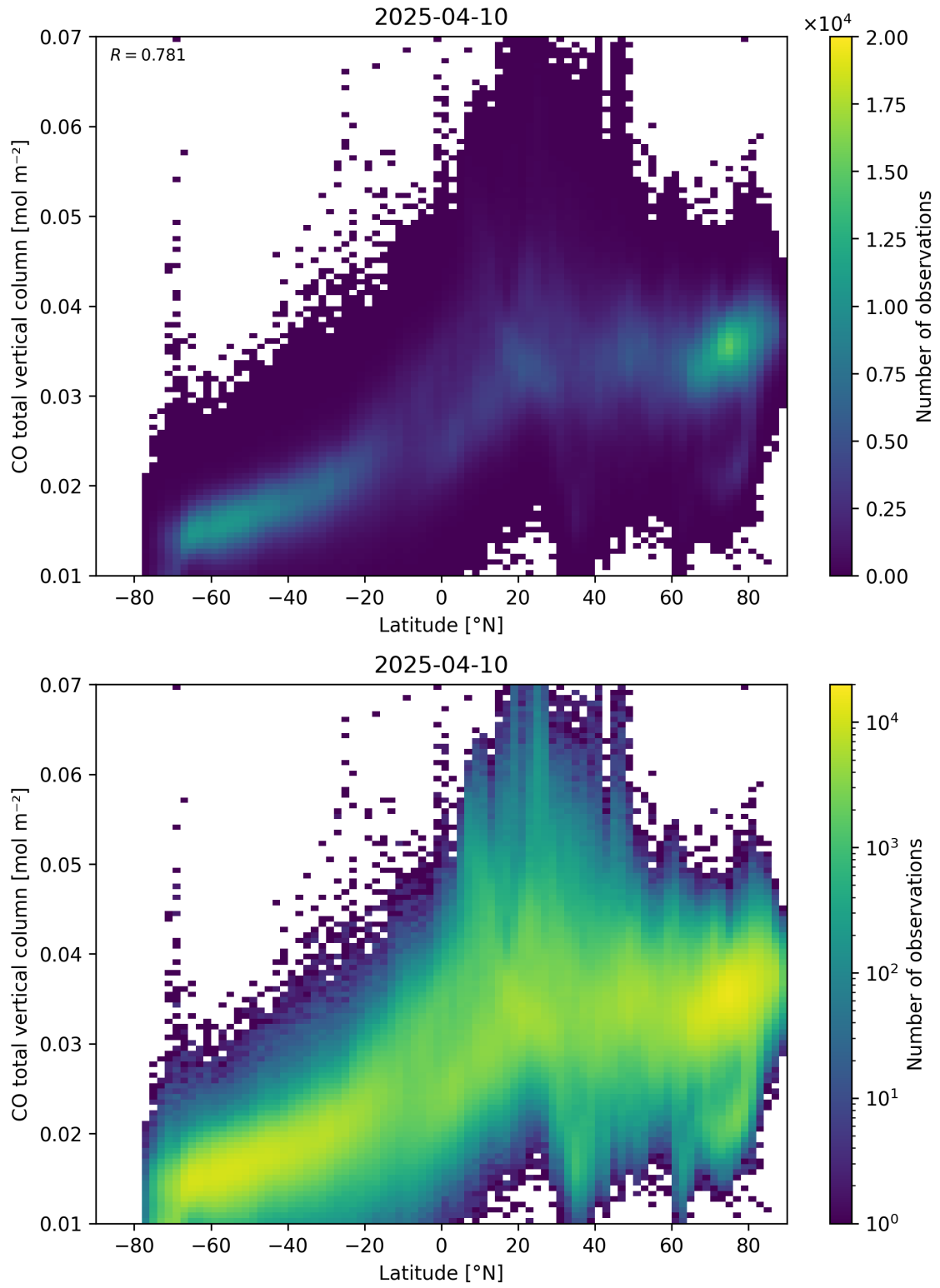
Figure 51: Scatter density plot of “Latitude” against “CO total vertical column” for 2025-04-09 to 2025-04-11.
