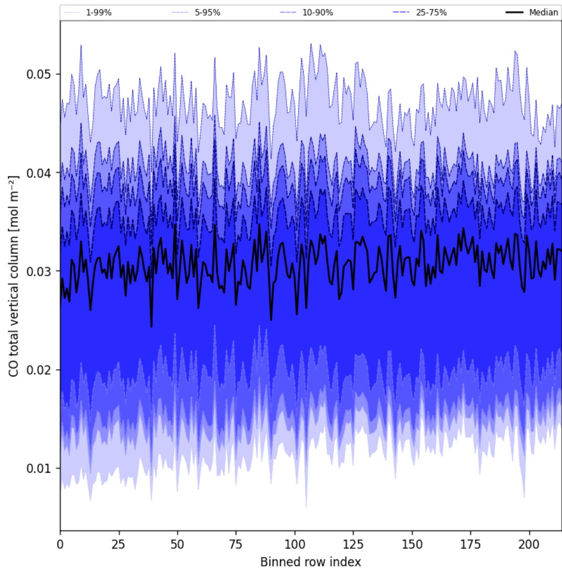
Figure 26: Along track statistics of “CO total vertical column” for 2025-04-09 to 2025-04-11
