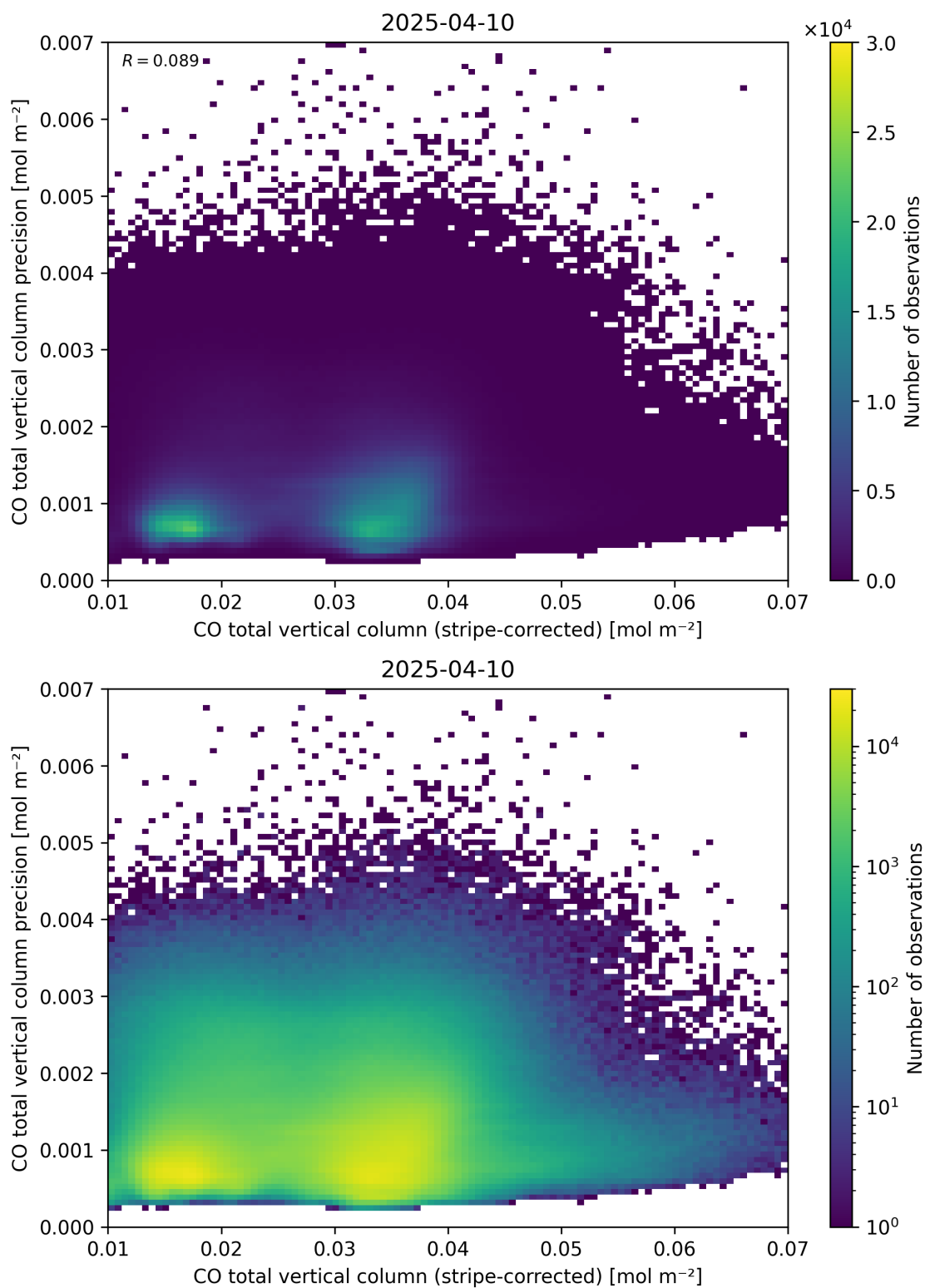
Figure 36: Scatter density plot of “CO total vertical column (stripe-corrected)” against “CO total vertical column precision” for 2025-04-09 to 2025-04-11.
