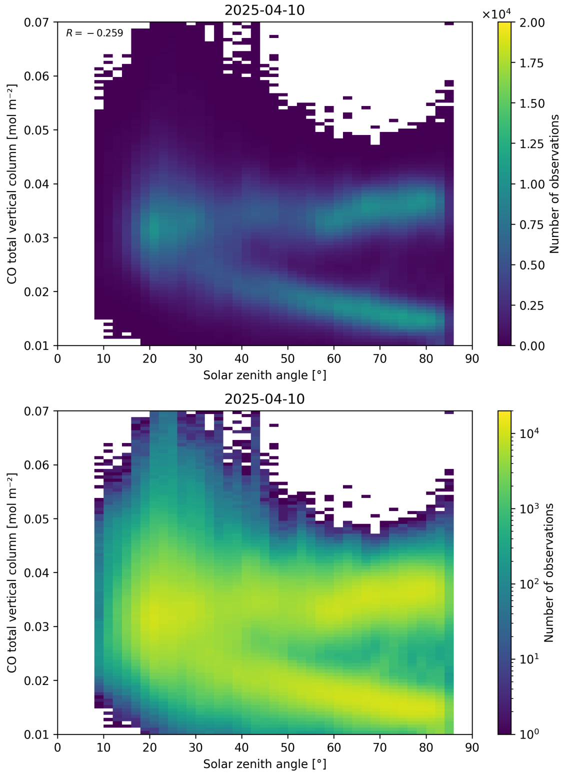
Figure 61: Scatter density plot of “Solar zenith angle” against “CO total vertical column” for 2025-04-09 to 2025-04-11.
