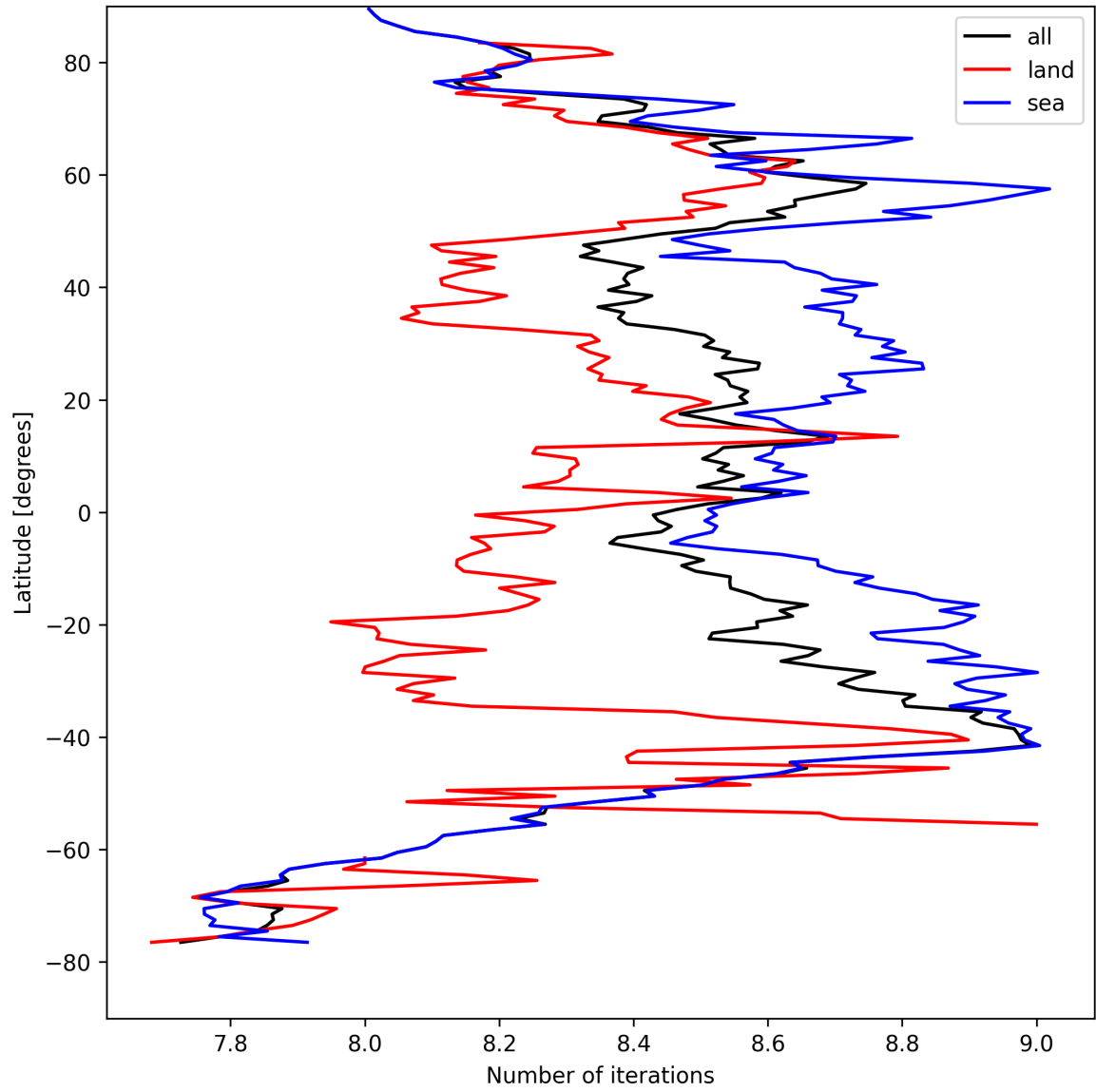
Figure 16: Zonal average of “Number of iterations” for 2025-04-09 to 2025-04-11.
