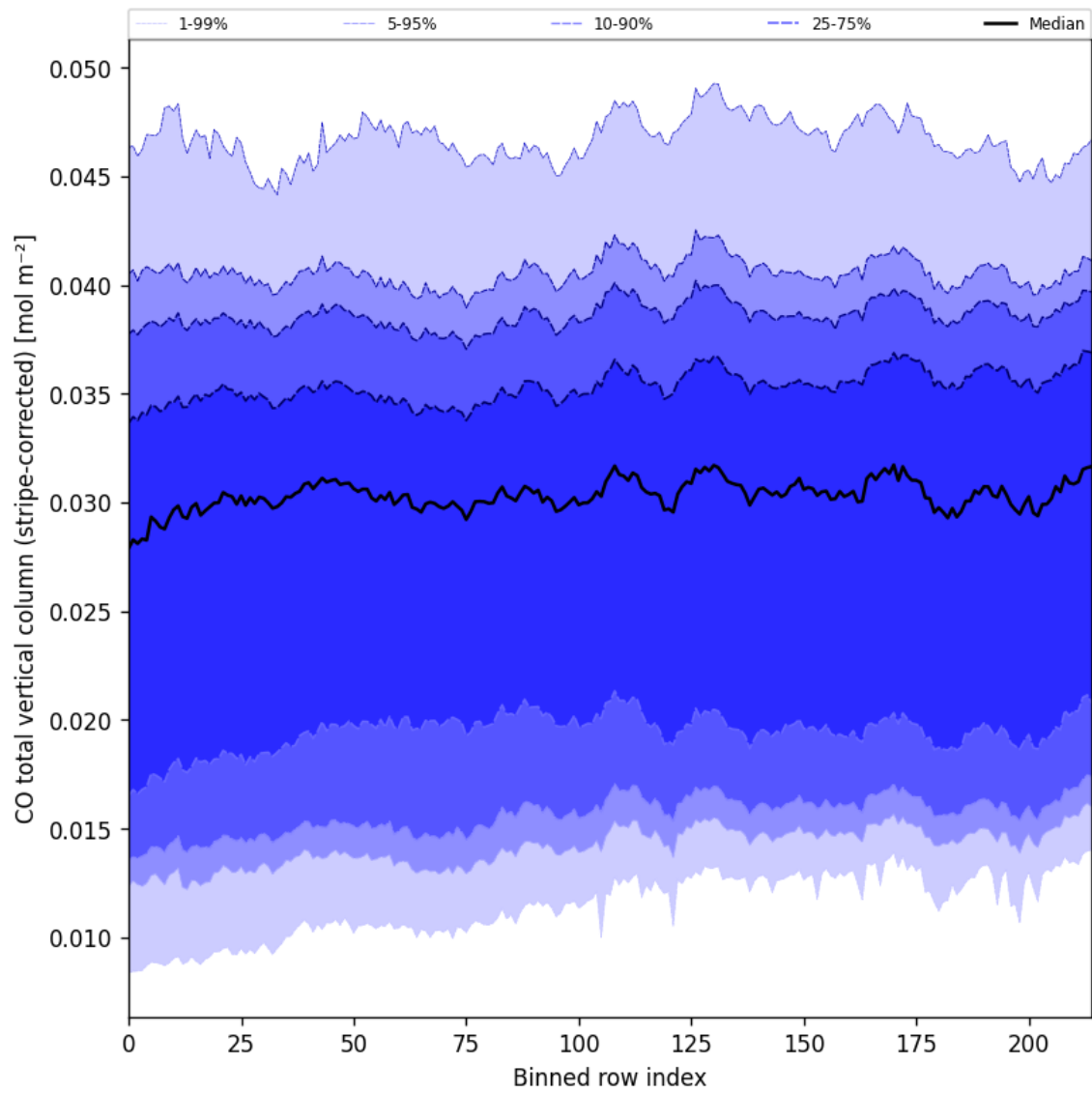
Figure 27: Along track statistics of “CO total vertical column (stripe-corrected)” for 2025-04-10 to 2025-04-12
