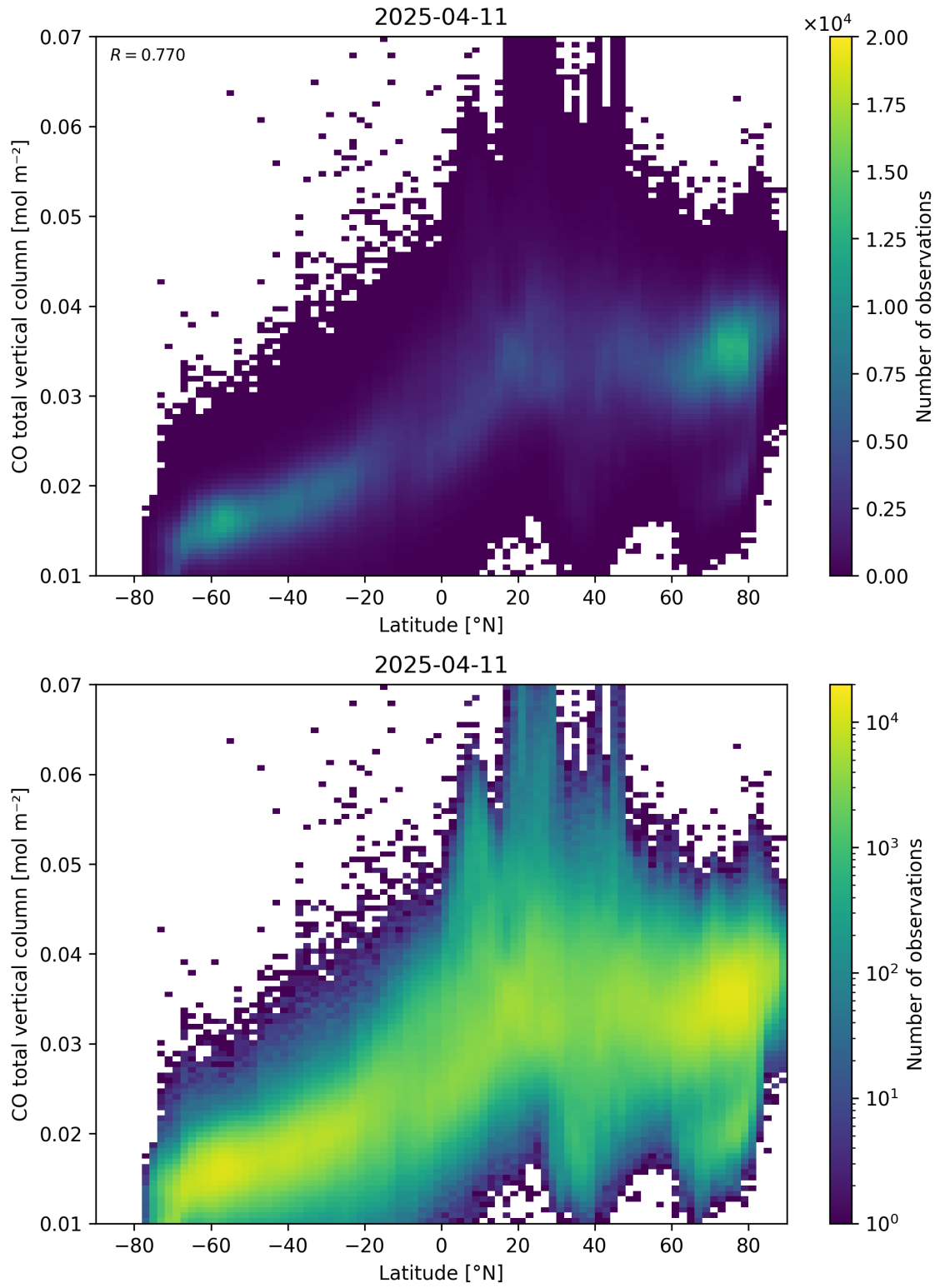
Figure 51: Scatter density plot of “Latitude” against “CO total vertical column” for 2025-04-10 to 2025-04-12.
