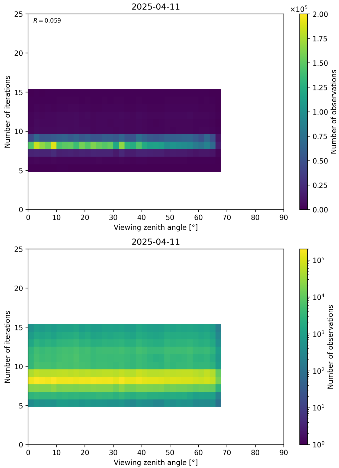
Figure 75: Scatter density plot of “Viewing zenith angle” against “Number of iterations” for 2025-04-10 to 2025-04-12.
