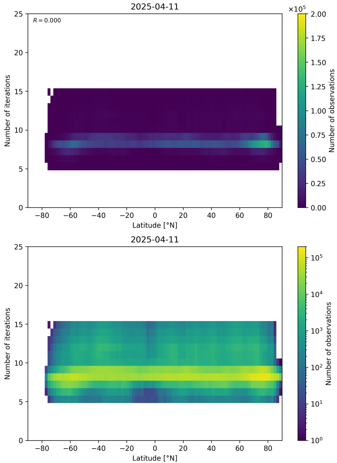
Figure 56: Scatter density plot of “Latitude” against “Number of iterations” for 2025-04-10 to 2025-04-12.
