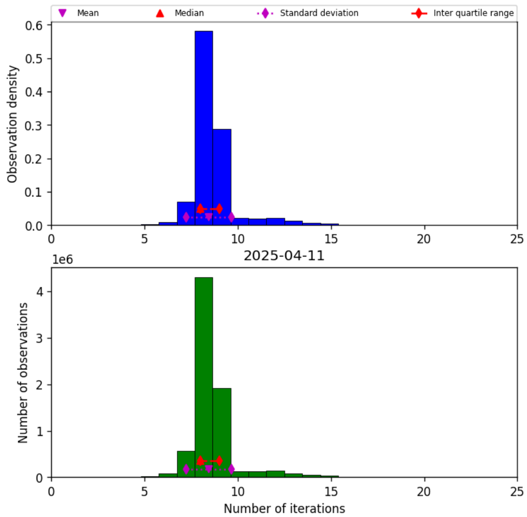
Figure 24: Histogram of “Number of iterations” for 2025-04-10 to 2025-04-12
