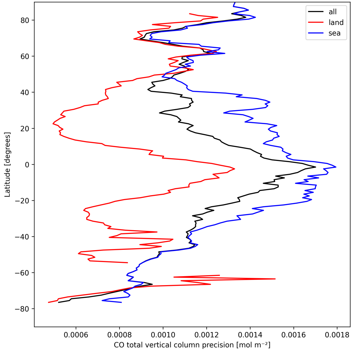
Figure 12: Zonal average of "CO total vertical column precision" for 2025-04-10 to 2025-04-12.
