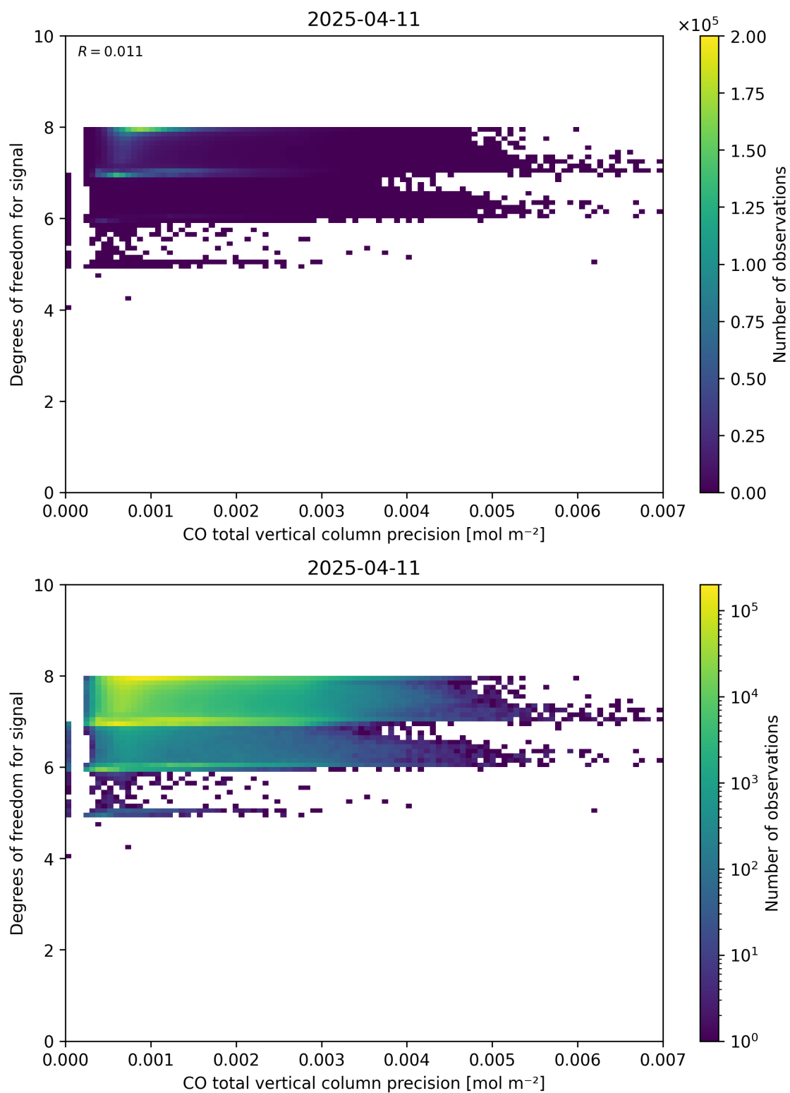
Figure 45: Scatter density plot of “CO total vertical column precision” against “Degrees of freedom for signal” for 2025-04-10 to 2025-04-12.
