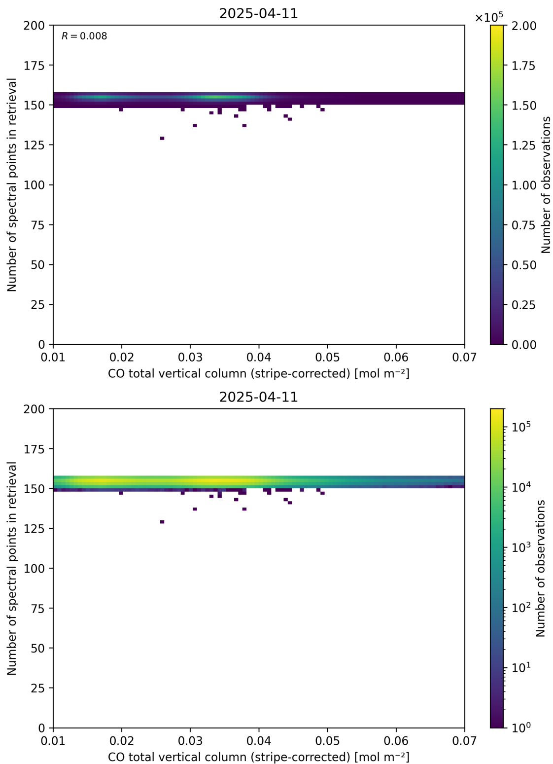
Figure 40: Scatter density plot of “CO total vertical column (stripe-corrected)” against “Number of spectral points in retrieval” for 2025-04-10 to 2025-04-12.
