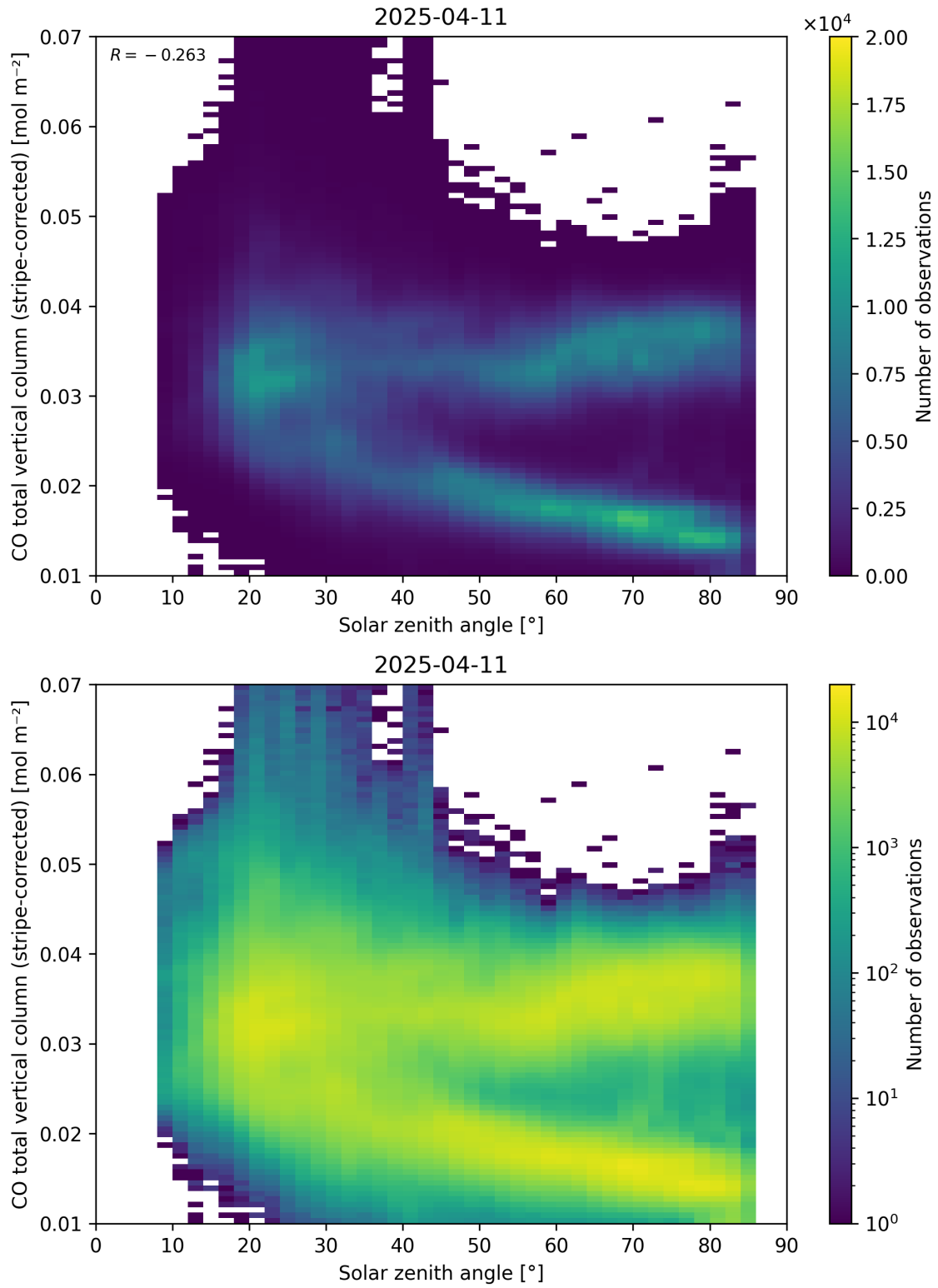
Figure 62: Scatter density plot of “Solar zenith angle” against “CO total vertical column (stripe-corrected)” for 2025-04-10 to 2025-04-12.
