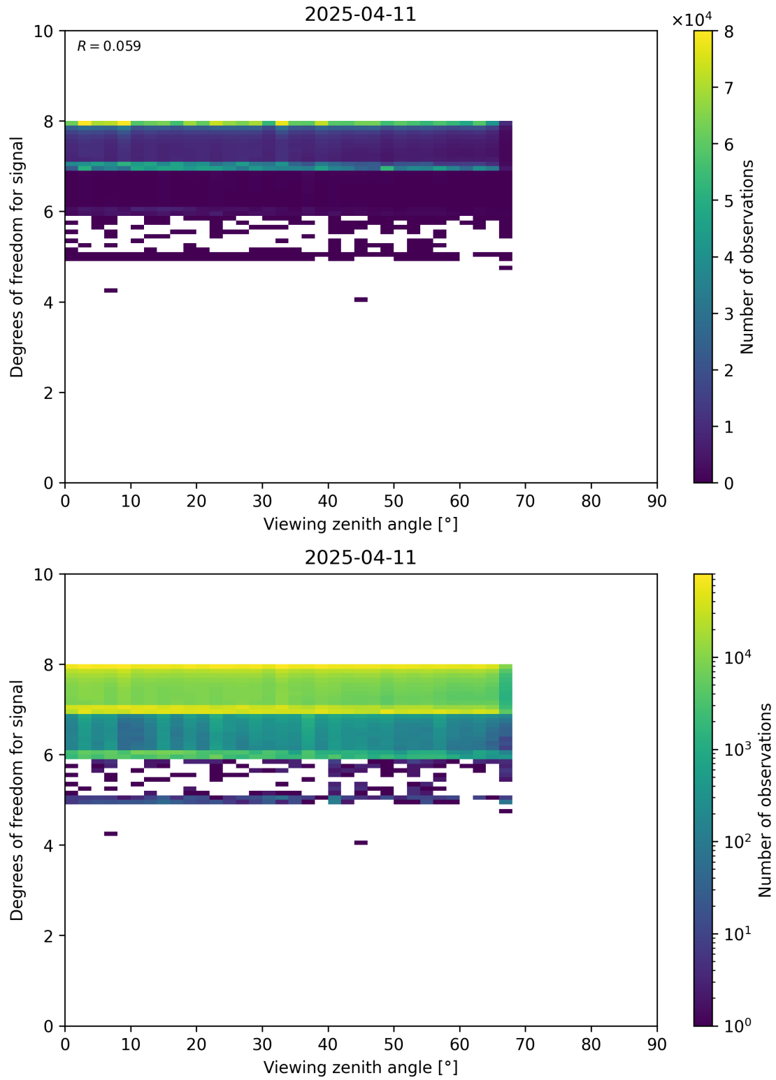
Figure 73: Scatter density plot of “Viewing zenith angle” against “Degrees of freedom for signal” for 2025-04-10 to 2025-04-12.
