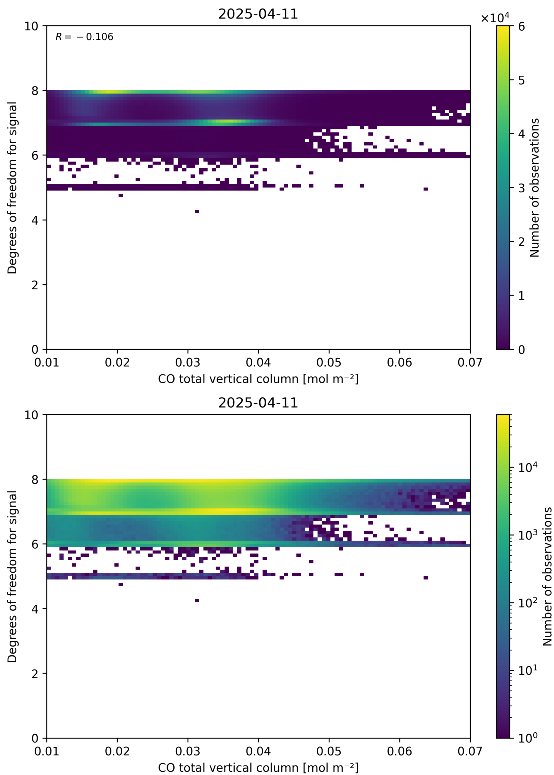
Figure 41: Scatter density plot of “CO total vertical column” against “Degrees of freedom for signal” for 2025-04-10 to 2025-04-12.
