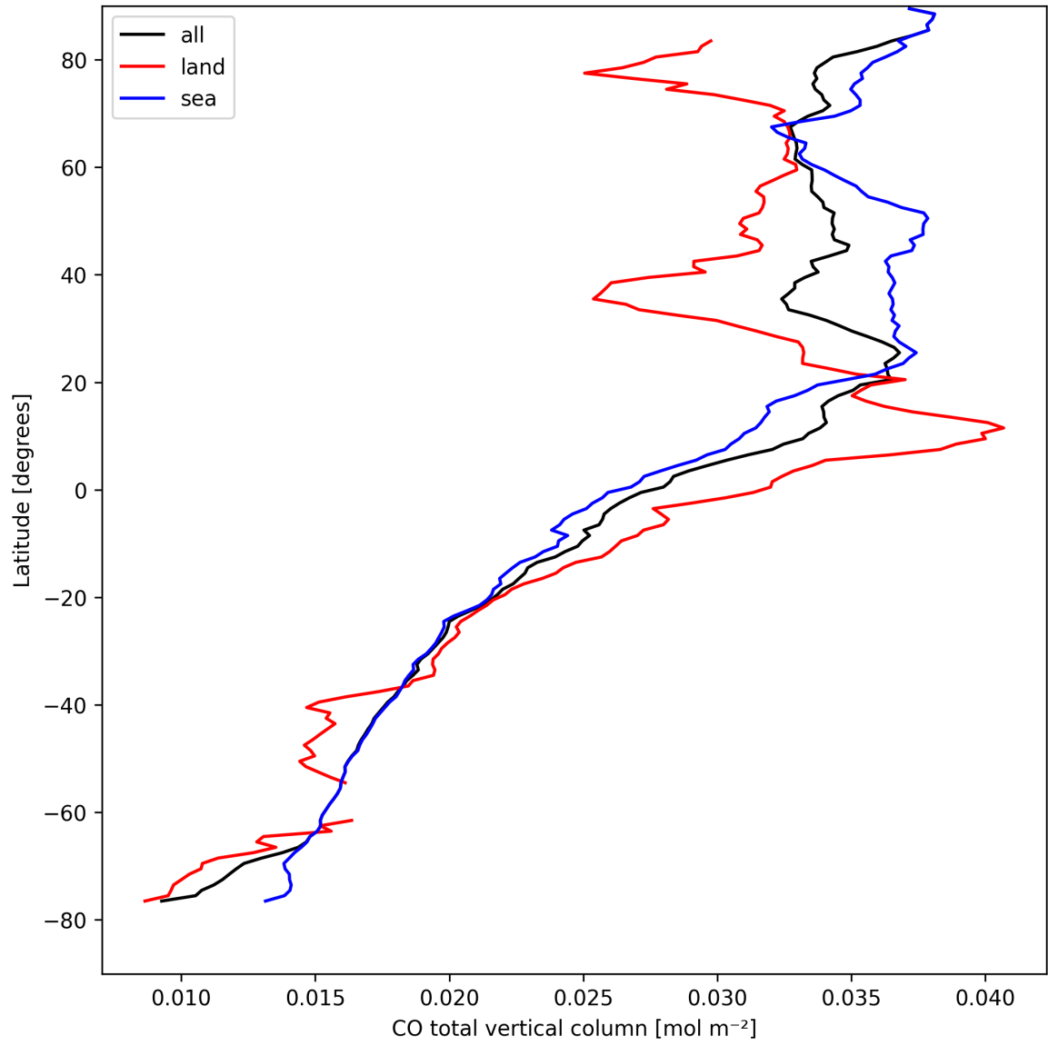
Figure 10: Zonal average of “CO total vertical column” for 2025-04-10 to 2025-04-12.
