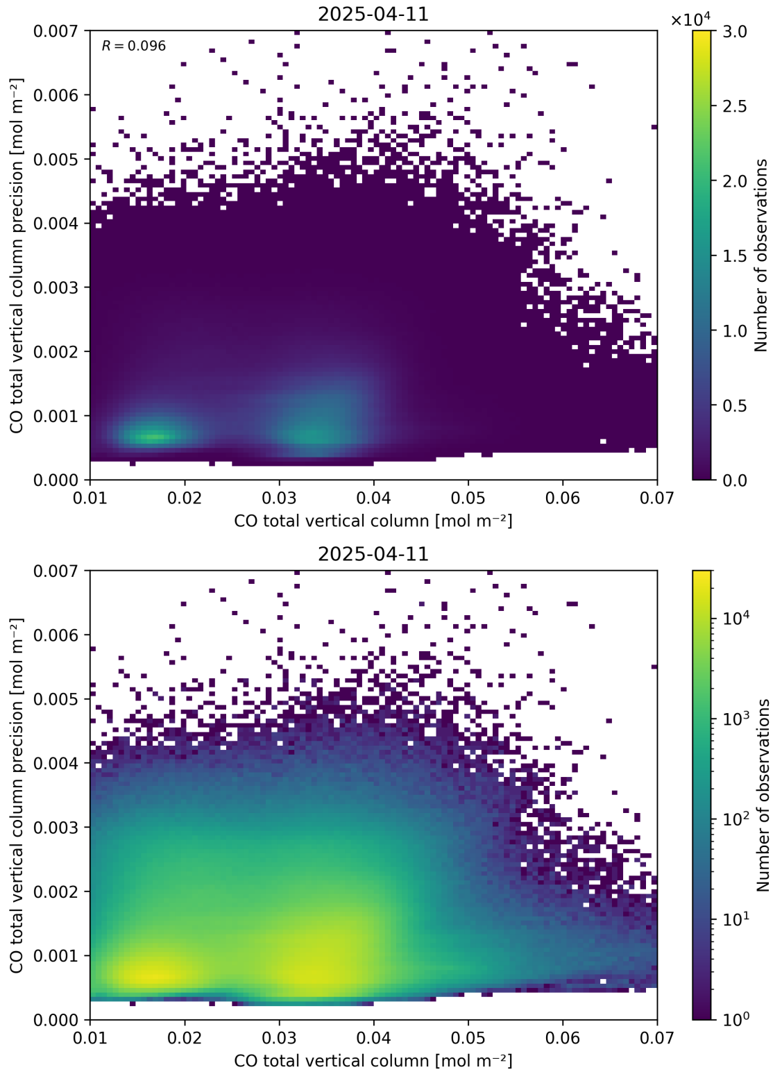
Figure 34: Scatter density plot of “CO total vertical column” against “CO total vertical column precision” for 2025-04-10 to 2025-04-12.
