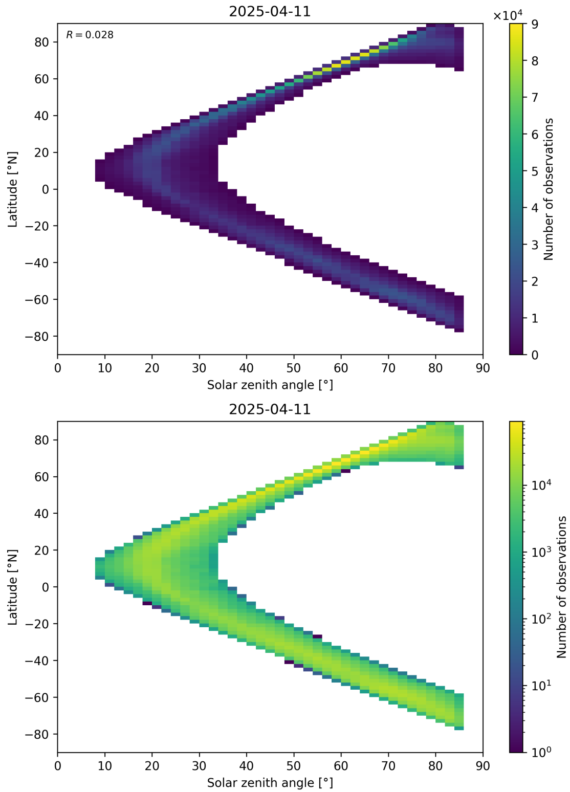
Figure 66: Scatter density plot of “Solar zenith angle” against “Latitude” for 2025-04-10 to 2025-04-12.
