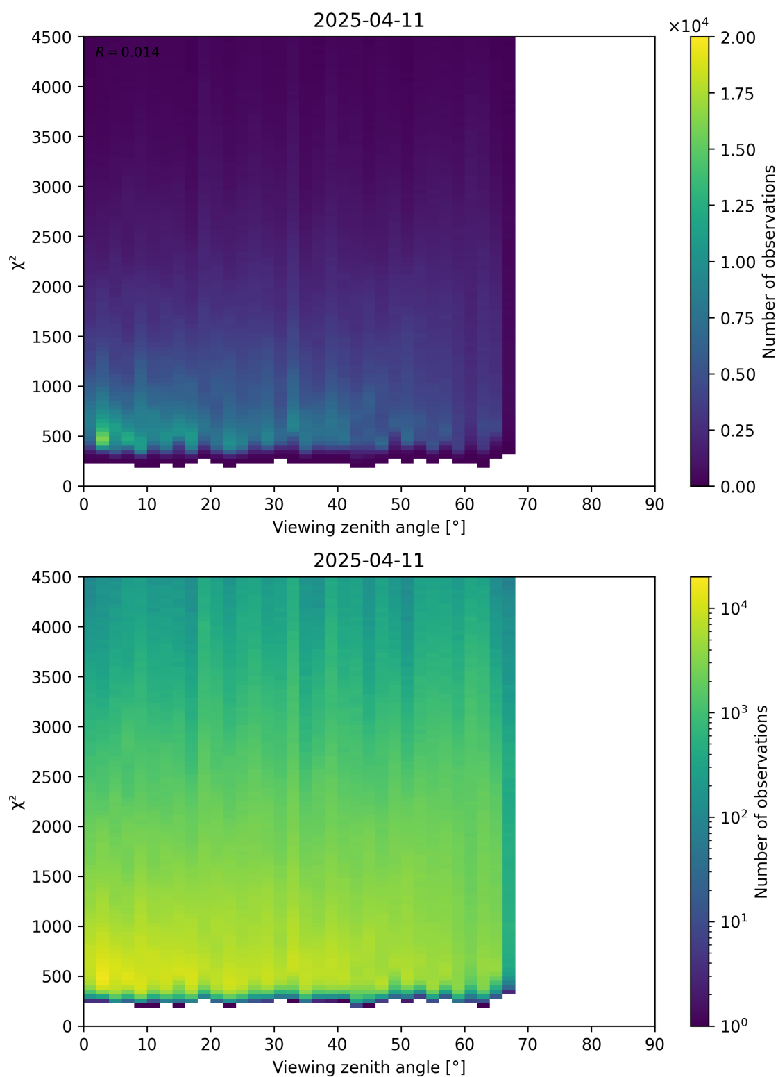
Figure 72: Scatter density plot of “Viewing zenith angle” against “ \chi^2 ” for 2025-04-10 to 2025-04-12.
