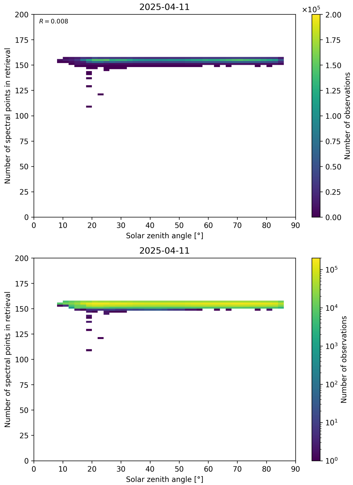
Figure 68: Scatter density plot of “Solar zenith angle” against “Number of spectral points in retrieval” for 2025-04-10 to 2025-04-12.
