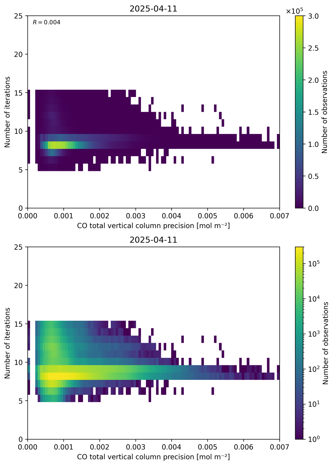
Figure 46: Scatter density plot of “CO total vertical column precision” against “Number of iterations” for 2025-04-10 to 2025-04-12.
