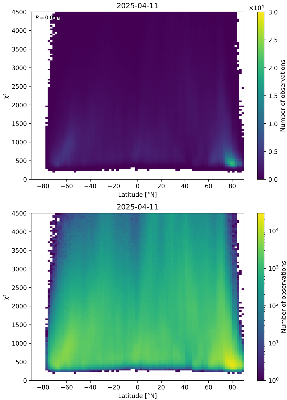
Figure 54: Scatter density plot of “Latitude” against “ \chi^2 ” for 2025-04-10 to 2025-04-12.
