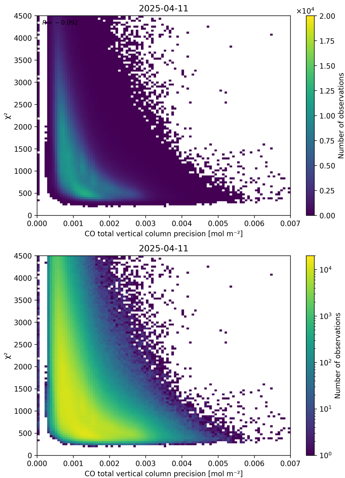
Figure 44: Scatter density plot of “CO total vertical column precision” against “ \chi^2 ” for 2025-04-10 to 2025-04-12.
