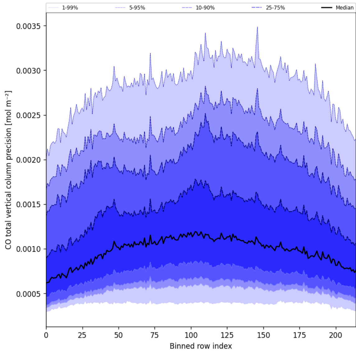
Figure 28: Along track statistics of “CO total vertical column precision” for 2025-04-10 to 2025-04-12
