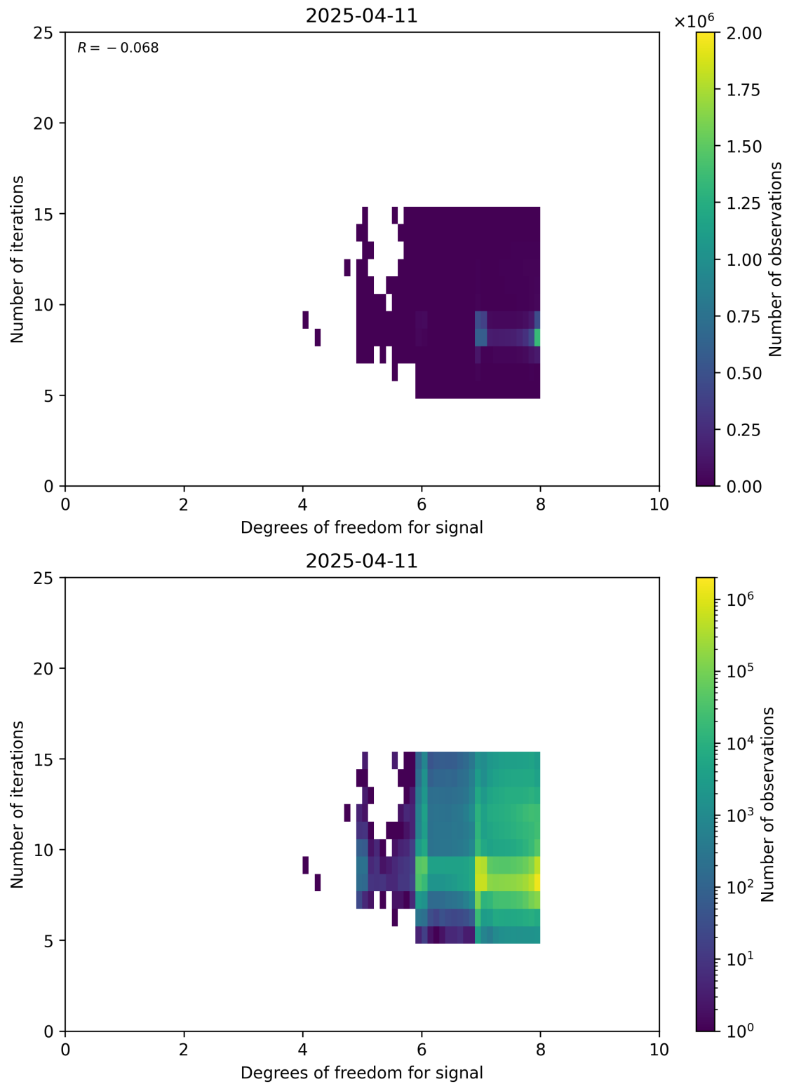
Figure 50: Scatter density plot of “Degrees of freedom for signal” against “Number of iterations” for 2025-04-10 to 2025-04-12.
