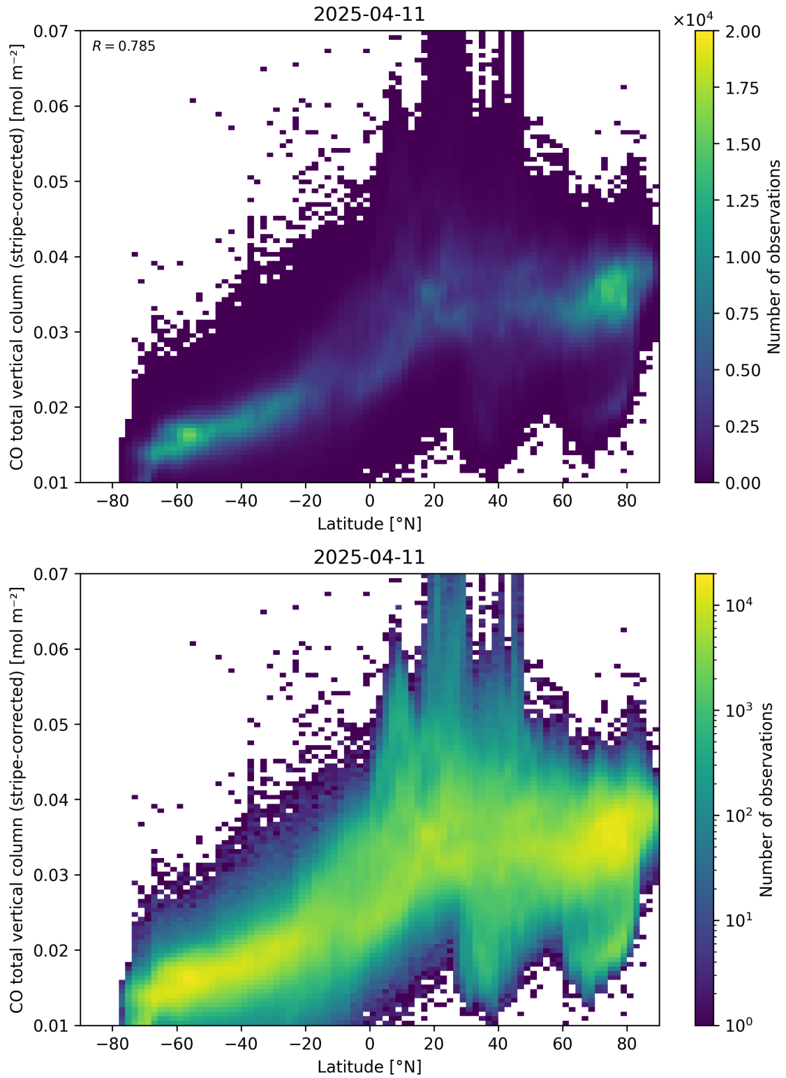
Figure 52: Scatter density plot of “Latitude” against “CO total vertical column (stripe-corrected)” for 2025-04-10 to 2025-04-12.
