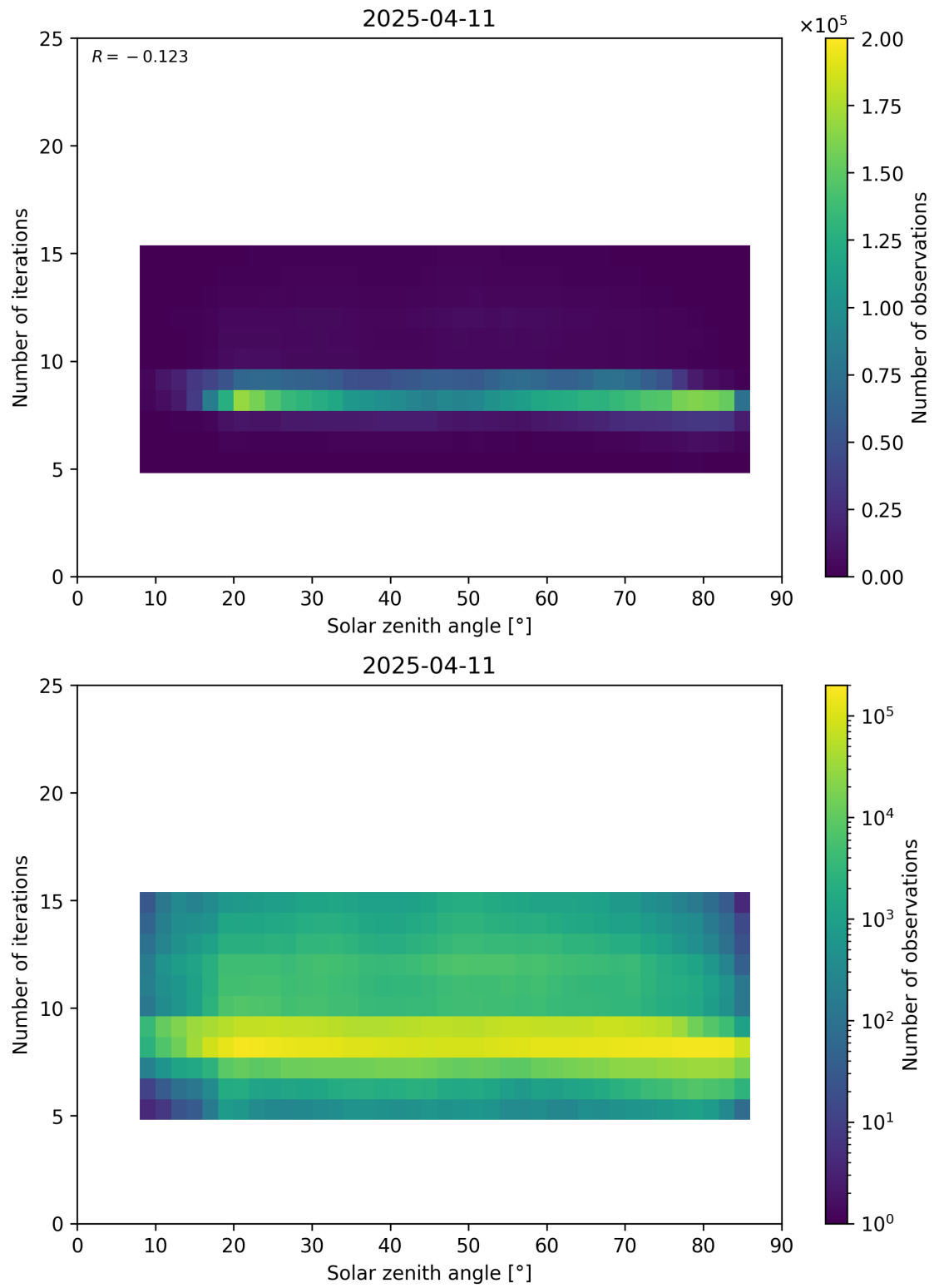
Figure 67: Scatter density plot of “Solar zenith angle” against “Number of iterations” for 2025-04-10 to 2025-04-12.
