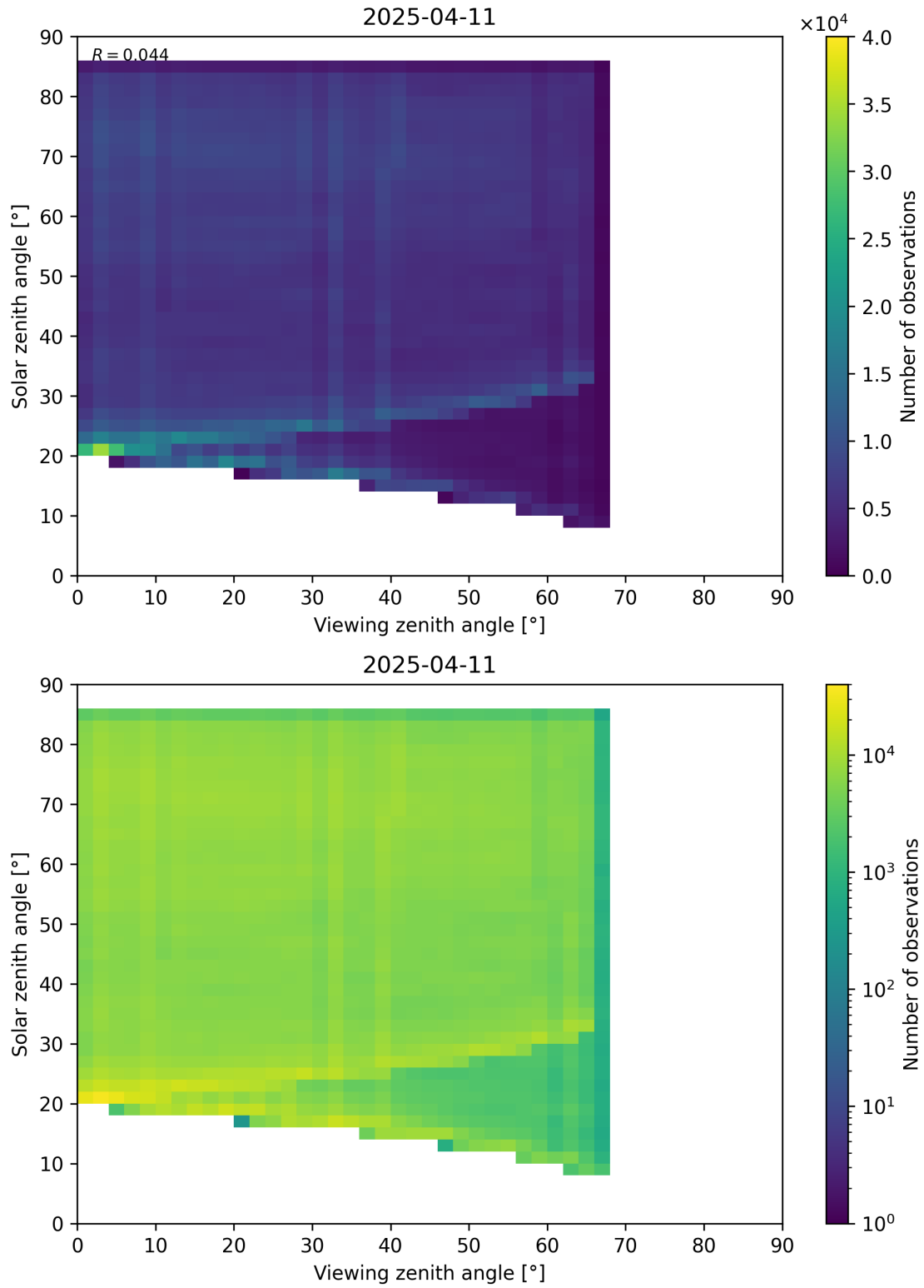
Figure 77: Scatter density plot of “Viewing zenith angle” against “Solar zenith angle” for 2025-04-10 to 2025-04-12.
