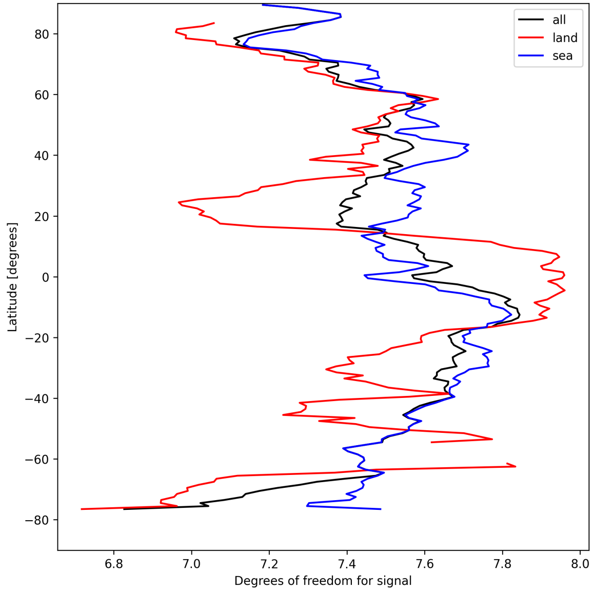
Figure 15: Zonal average of “Degrees of freedom for signal” for 2025-04-10 to 2025-04-12.
