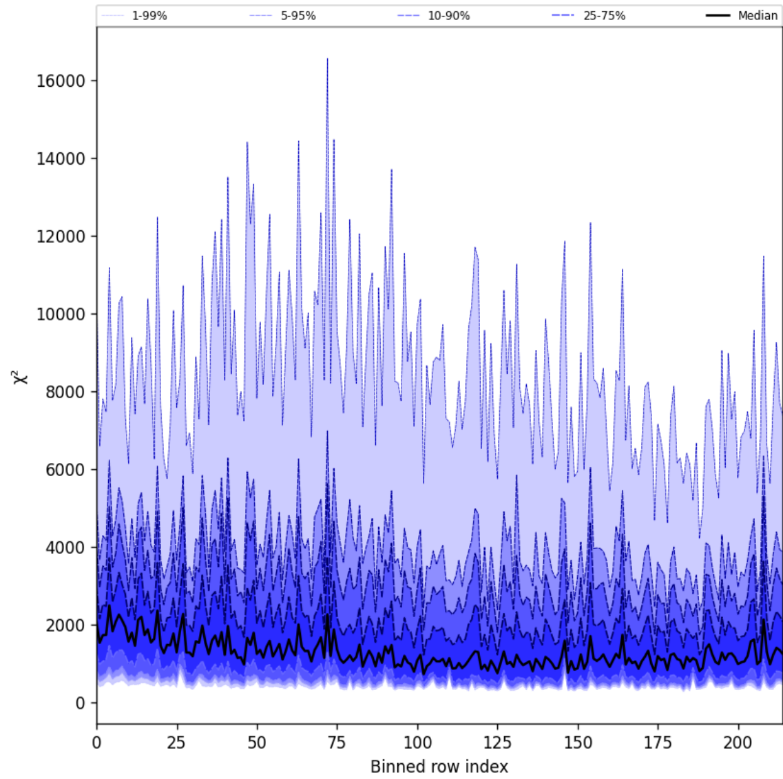
Figure 30: Along track statistics of “ \chi^2 ” for 2025-04-10 to 2025-04-12
