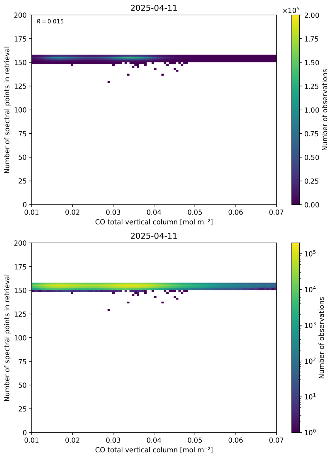
Figure 43: Scatter density plot of “CO total vertical column” against “Number of spectral points in retrieval” for 2025-04-10 to 2025-04-12.
