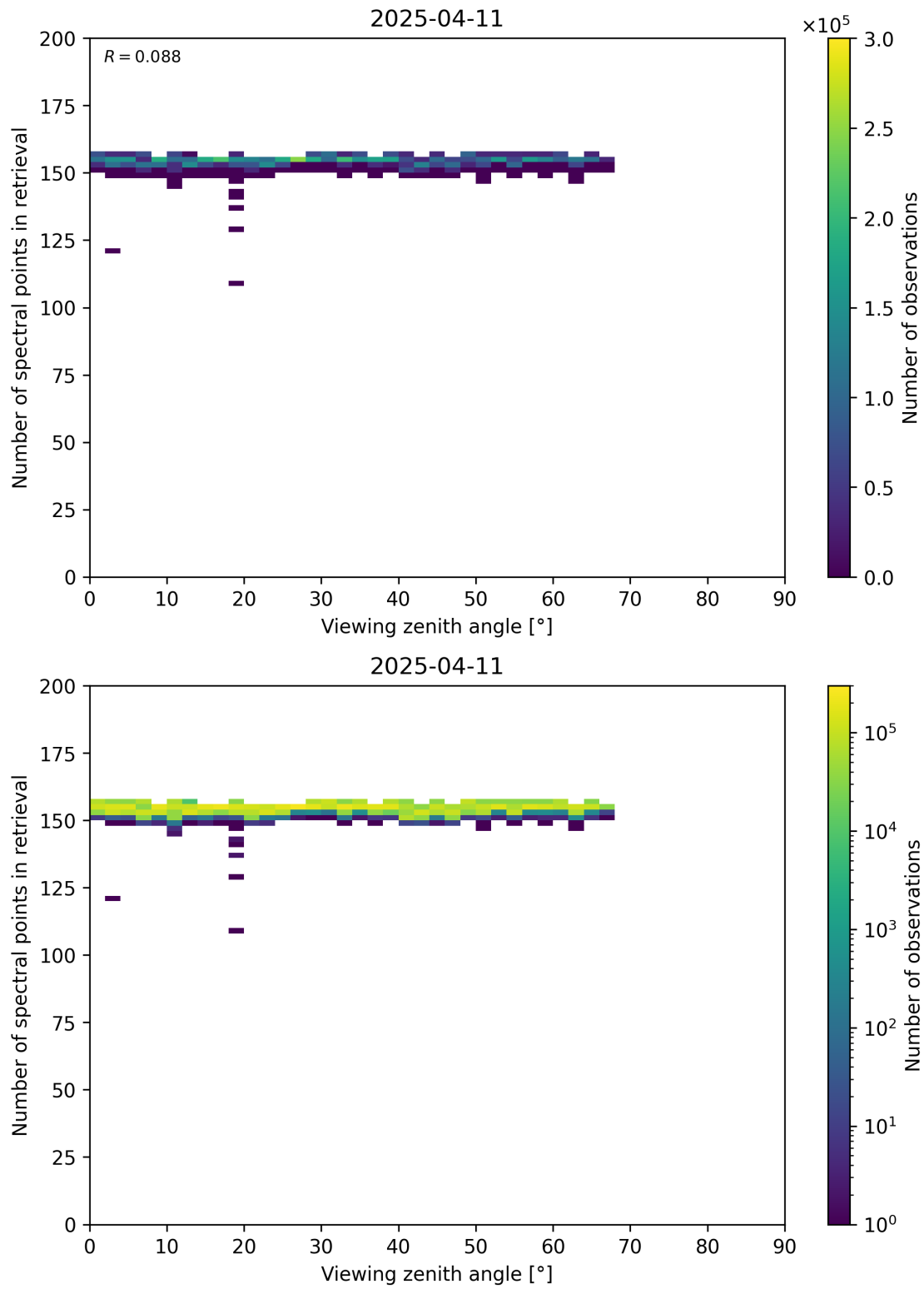
Figure 76: Scatter density plot of “Viewing zenith angle” against “Number of spectral points in retrieval” for 2025-04-10 to 2025-04-12.
