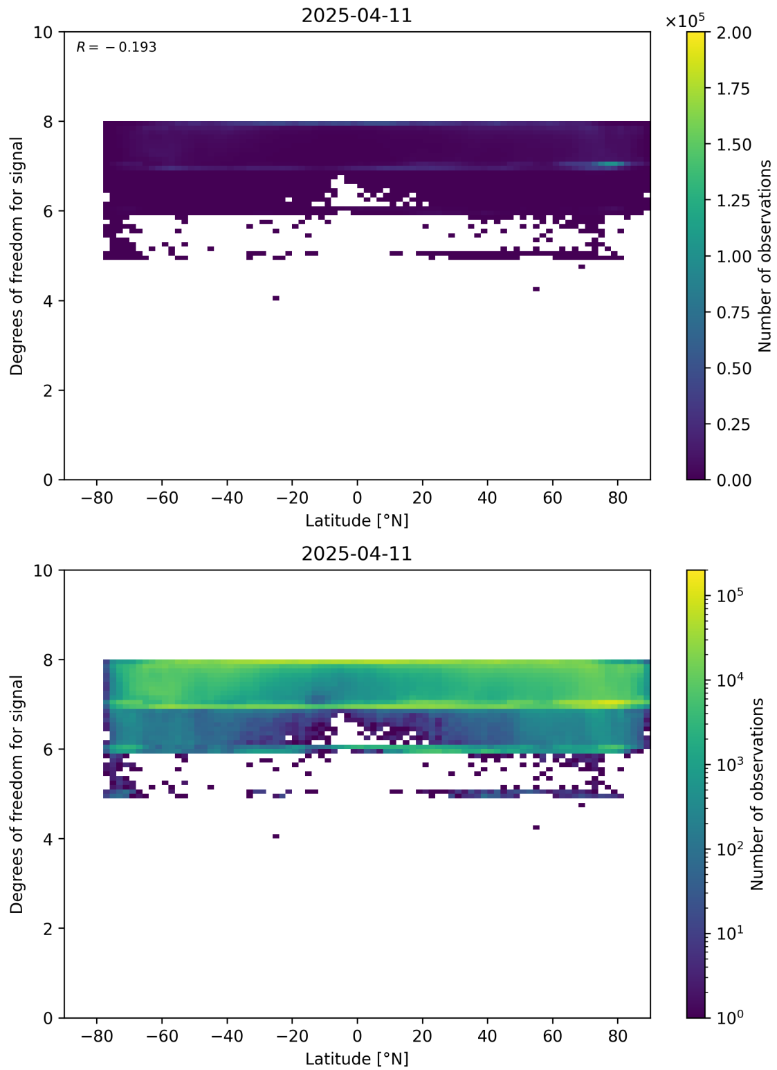
Figure 55: Scatter density plot of “Latitude” against “Degrees of freedom for signal” for 2025-04-10 to 2025-04-12.
