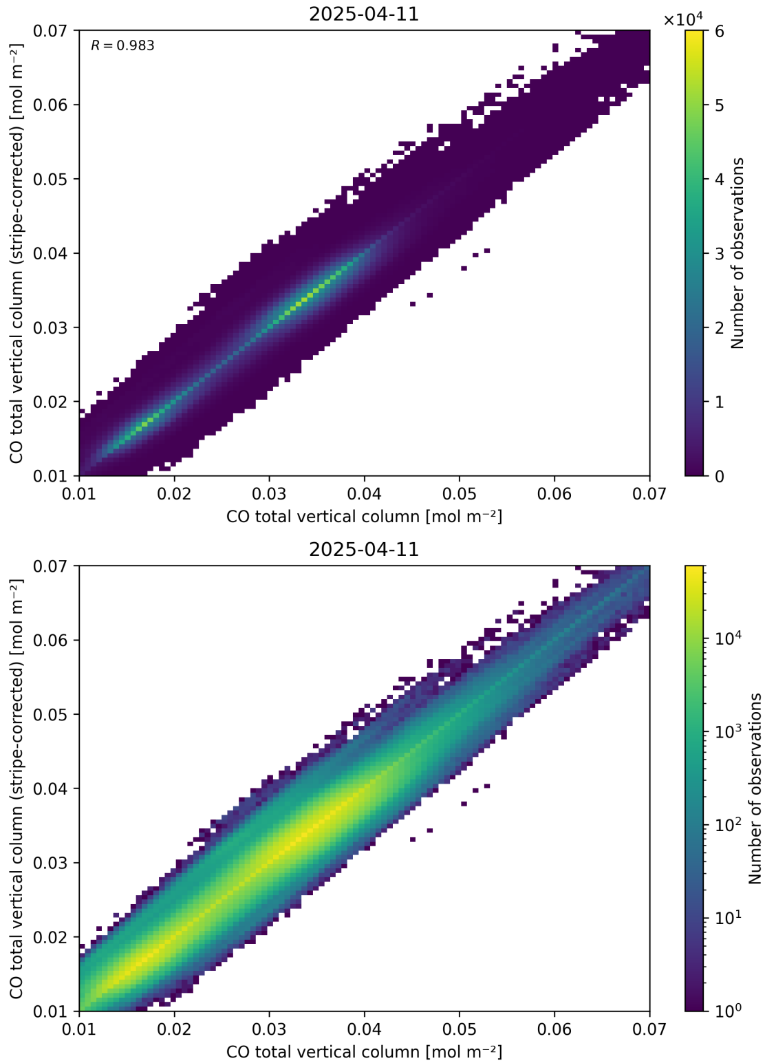
Figure 33: Scatter density plot of “CO total vertical column” against “CO total vertical column (stripe-corrected)” for 2025-04-10 to 2025-04-12.
