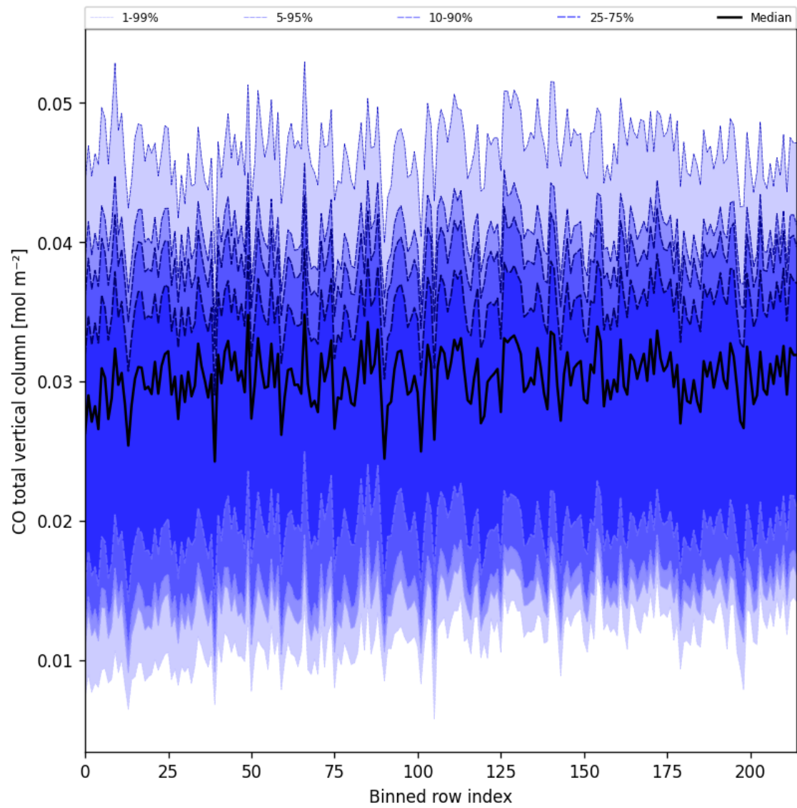
Figure 26: Along track statistics of “CO total vertical column” for 2025-04-10 to 2025-04-12
