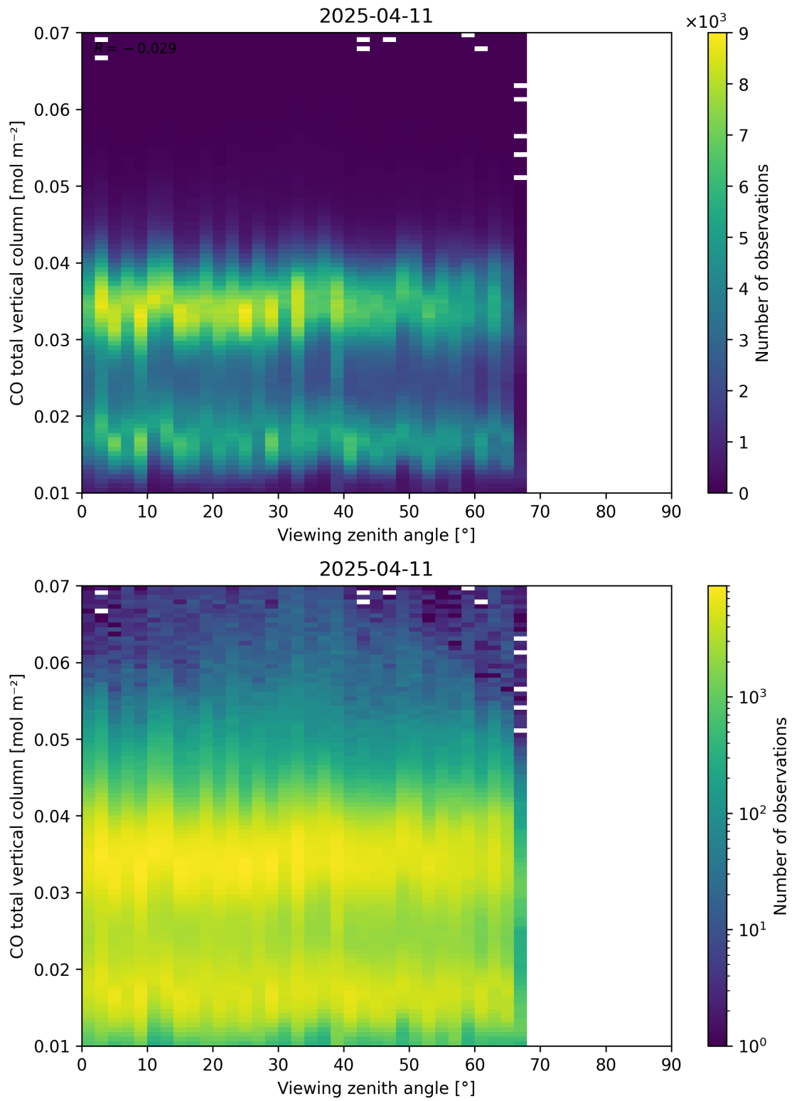
Figure 69: Scatter density plot of “Viewing zenith angle” against “CO total vertical column” for 2025-04-10 to 2025-04-12.
