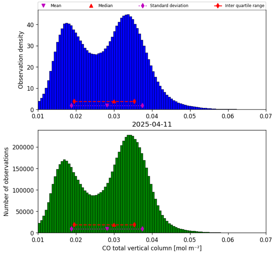
Figure 18: Histogram of “CO total vertical column” for 2025-04-10 to 2025-04-12
