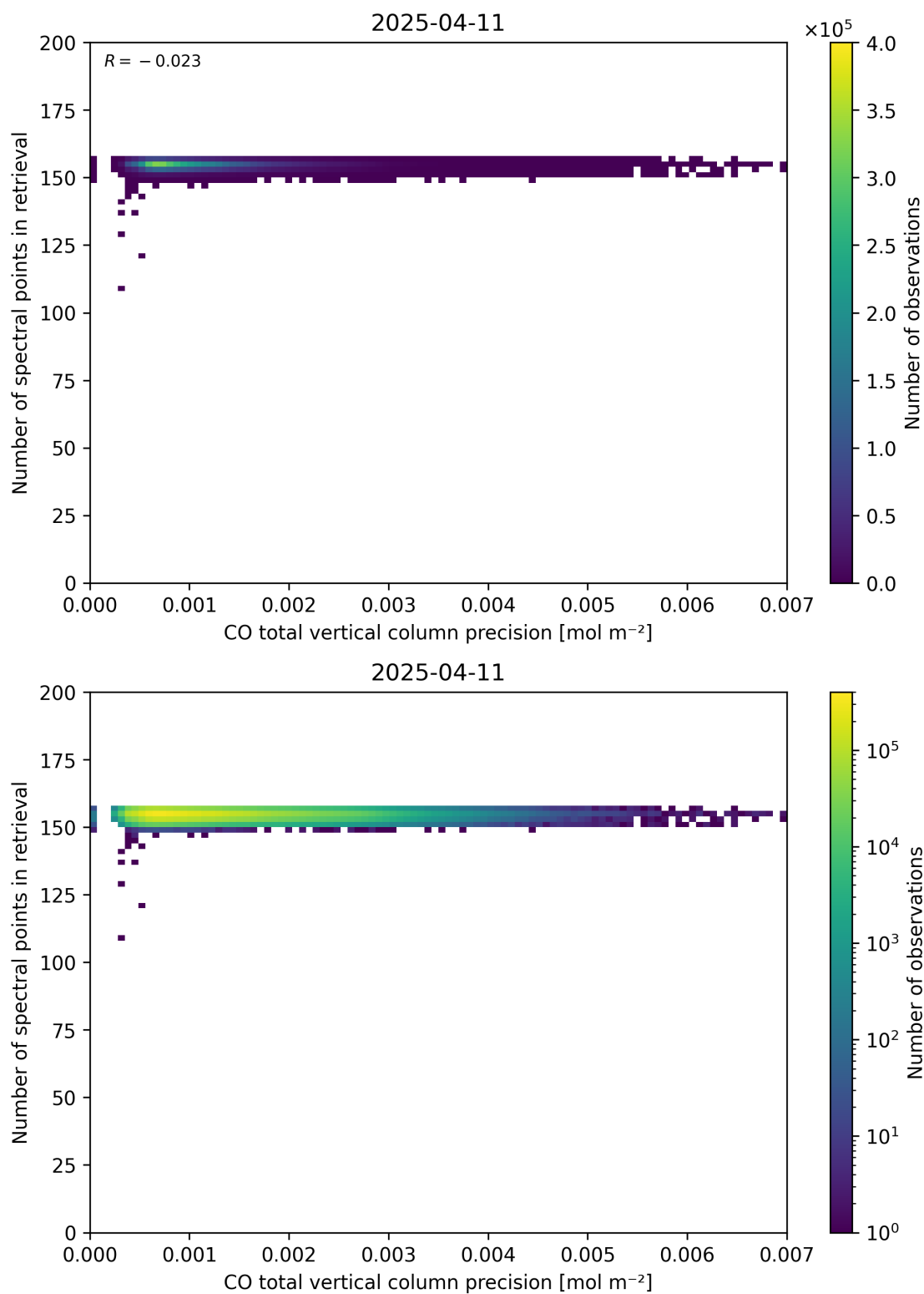
Figure 47: Scatter density plot of “CO total vertical column precision” against “Number of spectral points in retrieval” for 2025-04-10 to 2025-04-12.
