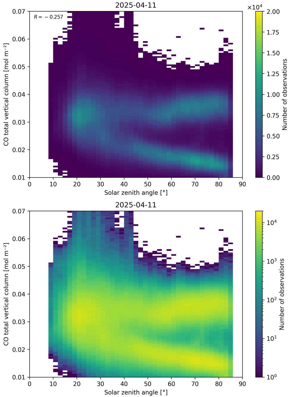
Figure 61: Scatter density plot of “Solar zenith angle” against “CO total vertical column” for 2025-04-10 to 2025-04-12.
