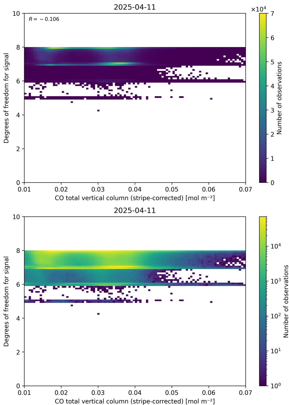
Figure 38: Scatter density plot of “CO total vertical column (stripe-corrected)” against “Degrees of freedom for signal” for 2025-04-10 to 2025-04-12.
