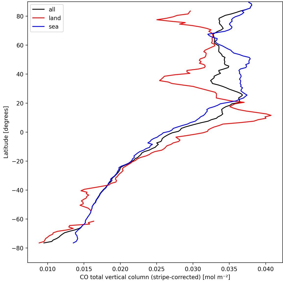
Figure 11: Zonal average of “CO total vertical column (stripe-corrected)” for 2025-04-10 to 2025-04-12.
