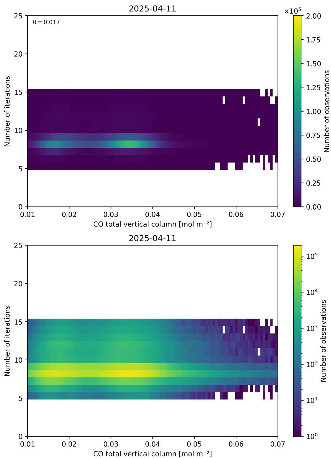
Figure 42: Scatter density plot of “CO total vertical column” against “Number of iterations” for 2025-04-10 to 2025-04-12.
