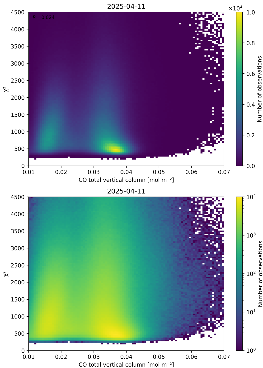
Figure 35: Scatter density plot of “CO total vertical column” against “ \chi^2 ” for 2025-04-10 to 2025-04-12.
