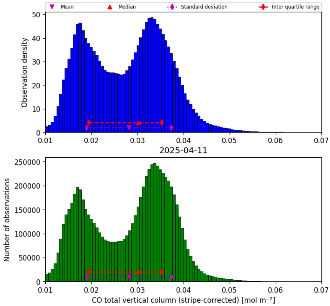
Figure 19: Histogram of “CO total vertical column (stripe-corrected)” for 2025-04-10 to 2025-04-12
