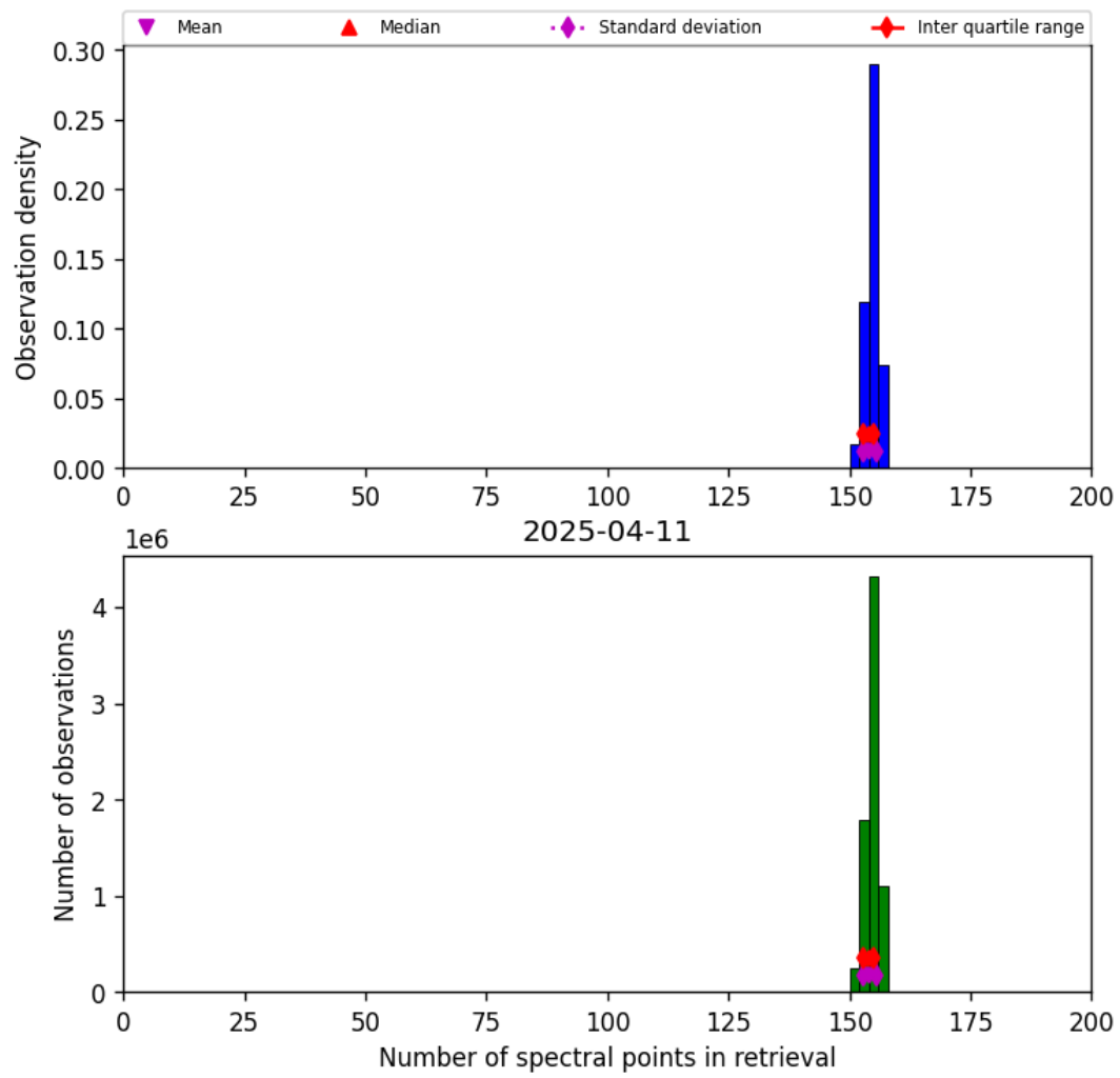
Figure 21: Histogram of “Number of spectral points in retrieval” for 2025-04-10 to 2025-04-12
