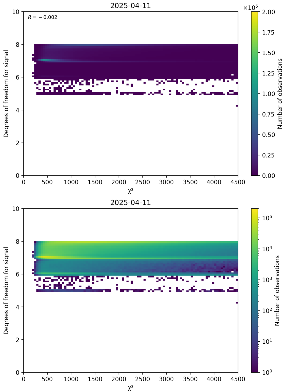
Figure 48: Scatter density plot of “ \chi^2 ” against “Degrees of freedom for signal” for 2025-04-10 to 2025-04-12.
