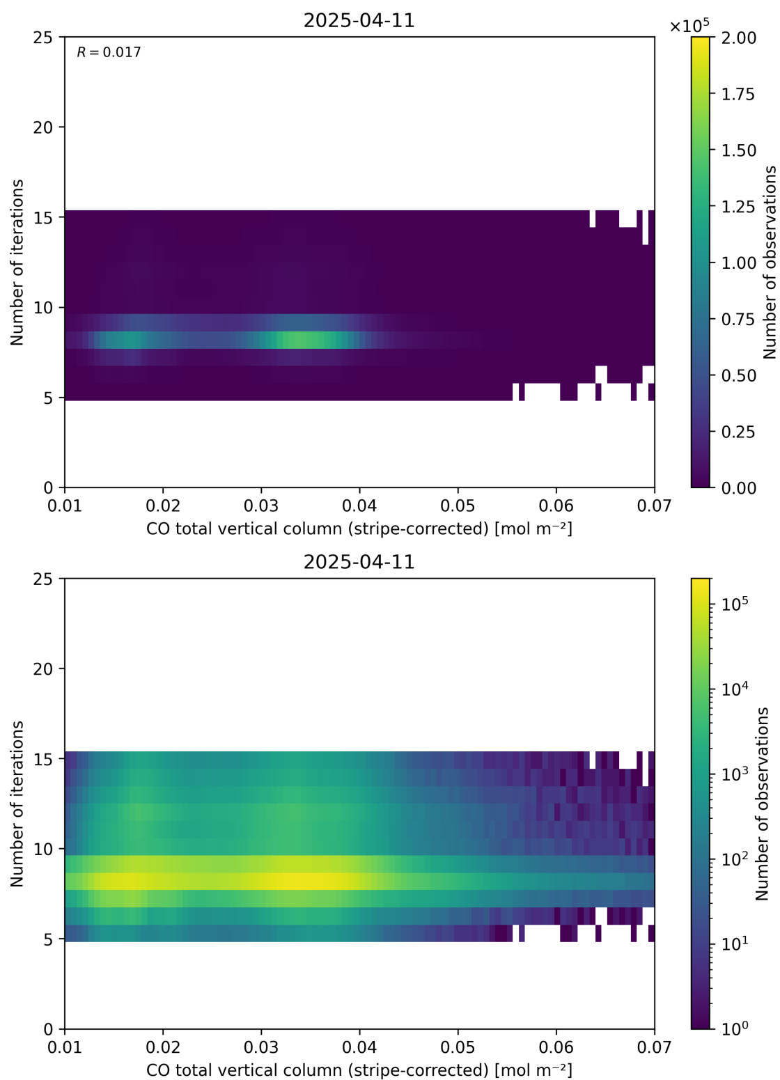
Figure 39: Scatter density plot of “CO total vertical column (stripe-corrected)” against “Number of iterations” for 2025-04-10 to 2025-04-12.
