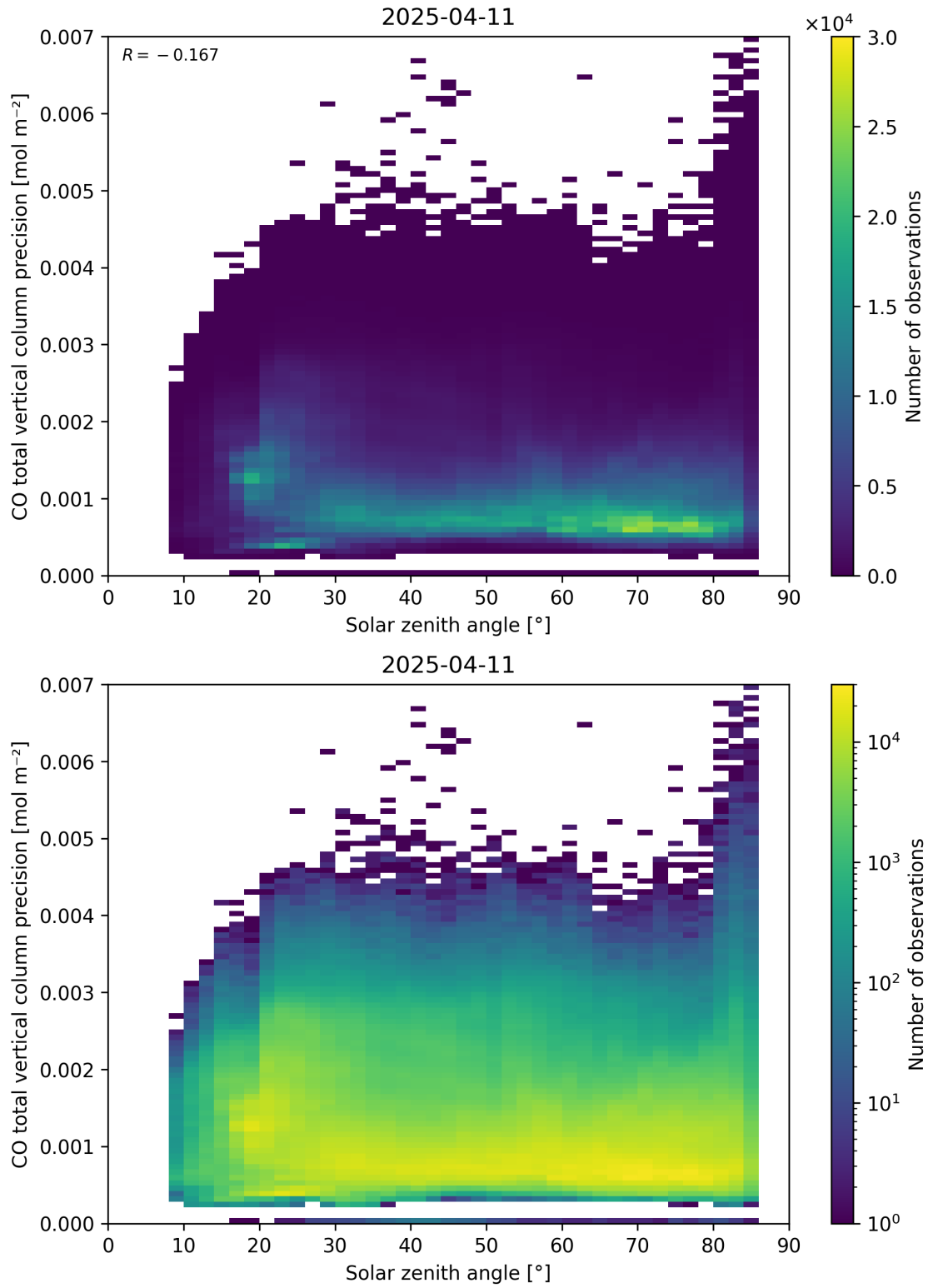
Figure 63: Scatter density plot of “Solar zenith angle” against “CO total vertical column precision” for 2025-04-10 to 2025-04-12.
