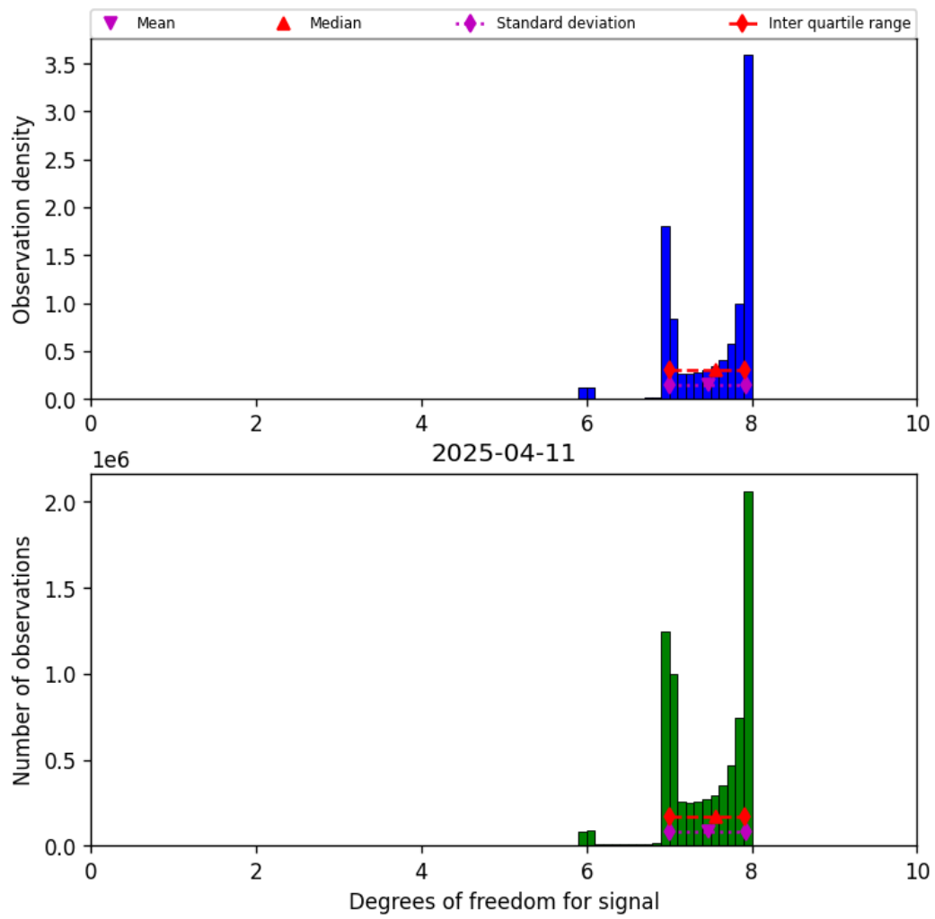
Figure 23: Histogram of “Degrees of freedom for signal” for 2025-04-10 to 2025-04-12
