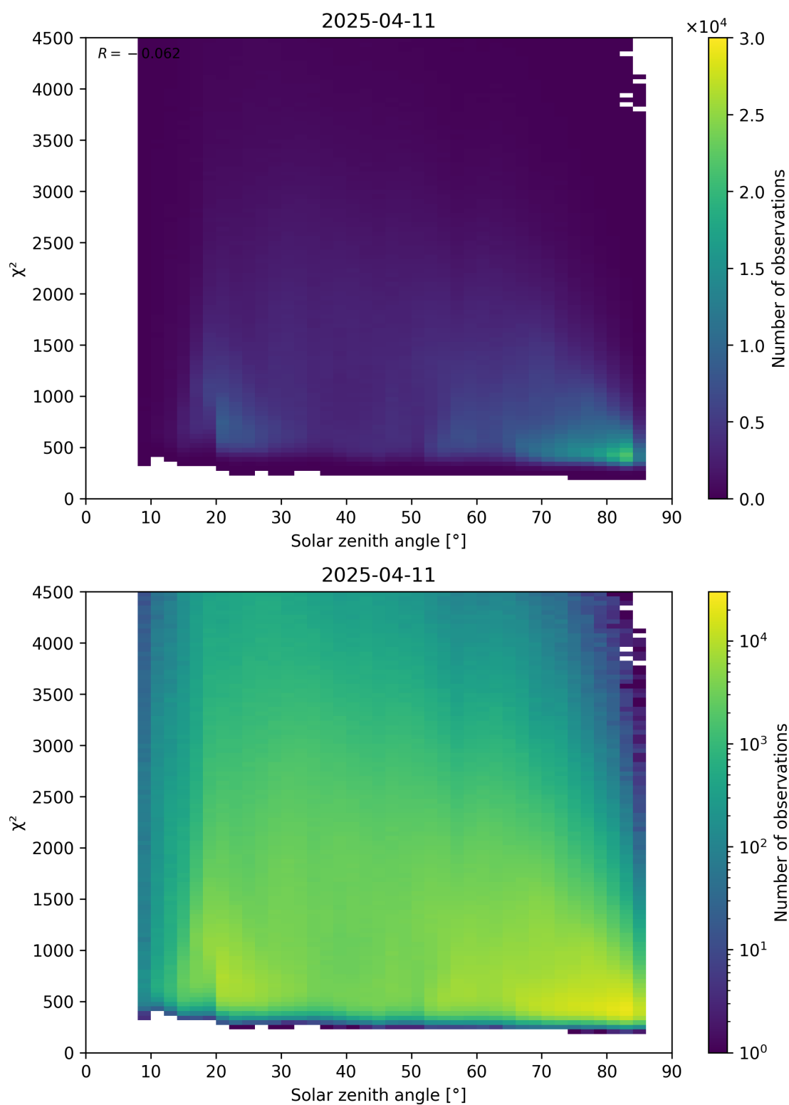
Figure 64: Scatter density plot of “Solar zenith angle” against “ \chi^2 ” for 2025-04-10 to 2025-04-12.
