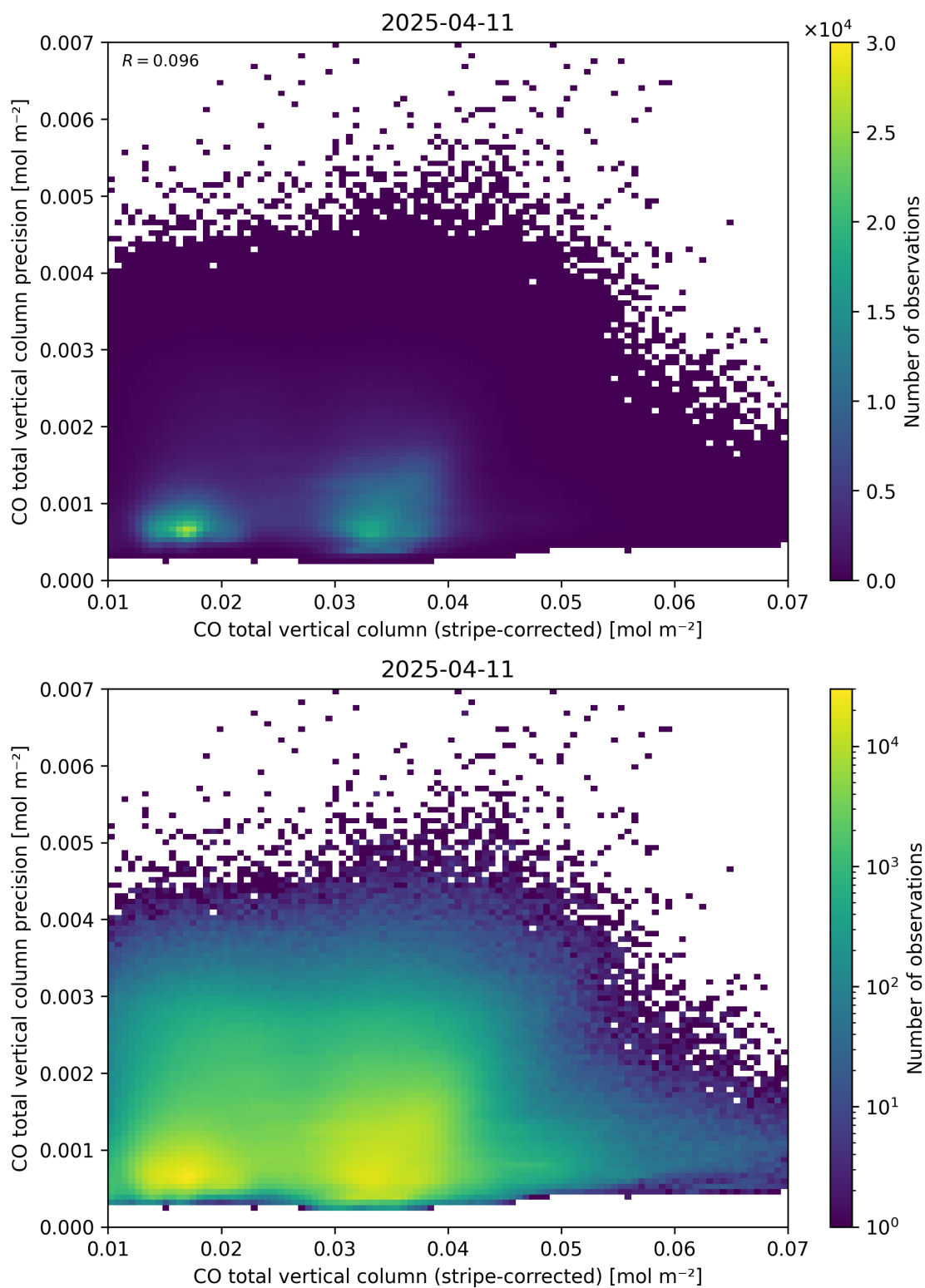
Figure 36: Scatter density plot of “CO total vertical column (stripe-corrected)” against “CO total vertical column precision” for 2025-04-10 to 2025-04-12.
