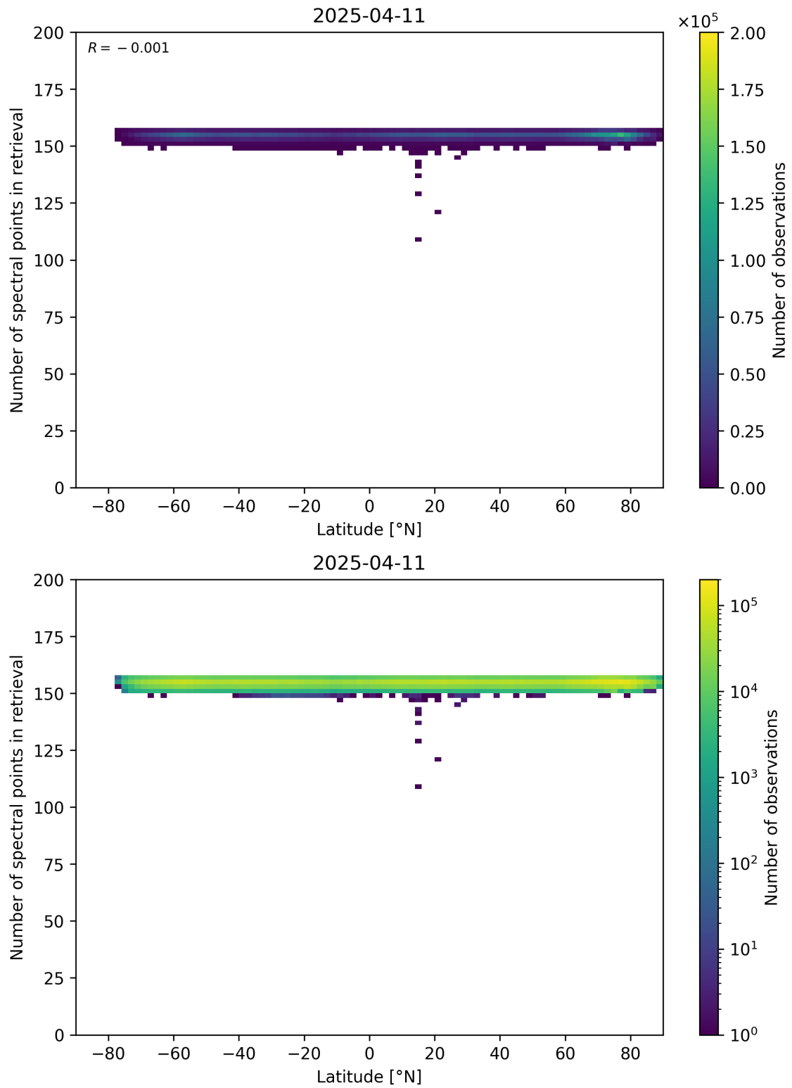
Figure 57: Scatter density plot of “Latitude” against “Number of spectral points in retrieval” for 2025-04-10 to 2025-04-12.
