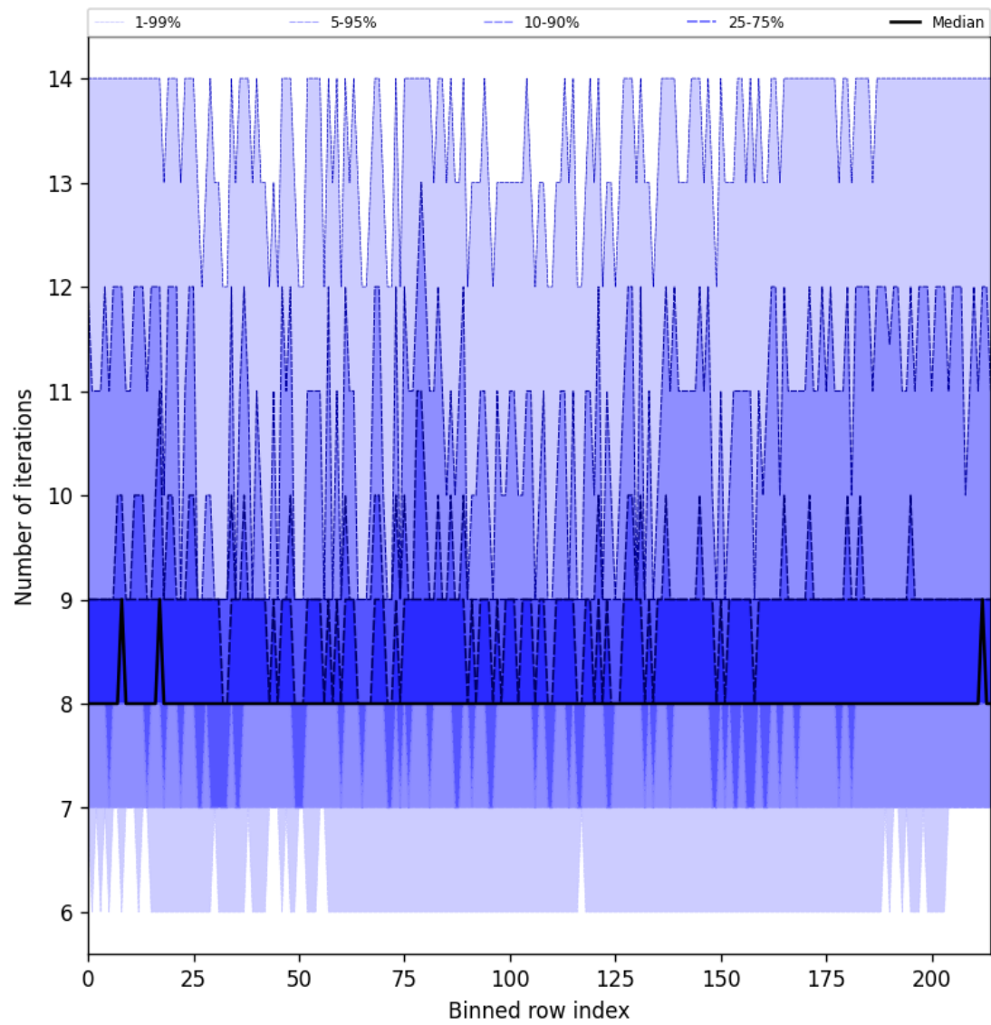
Figure 32: Along track statistics of “Number of iterations” for 2025-04-10 to 2025-04-12
