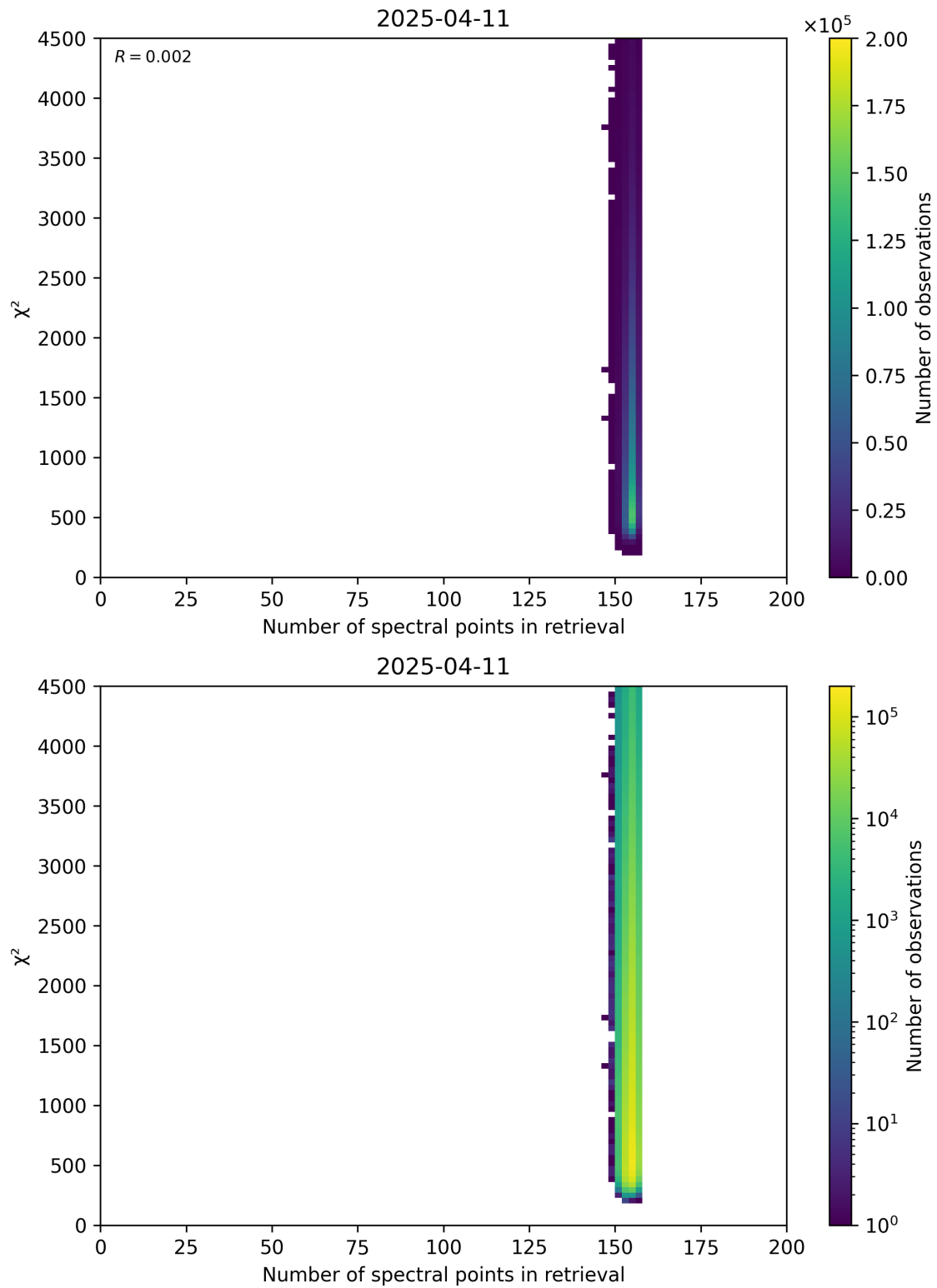
Figure 58: Scatter density plot of “Number of spectral points in retrieval” against “ \chi^2 ” for 2025-04-10 to 2025-04-12.
