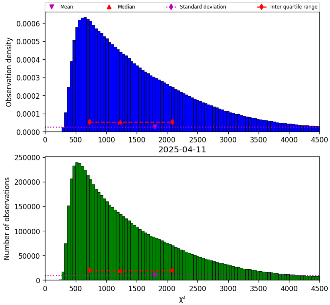
Figure 22: Histogram of “ \chi^2 ” for 2025-04-10 to 2025-04-12
