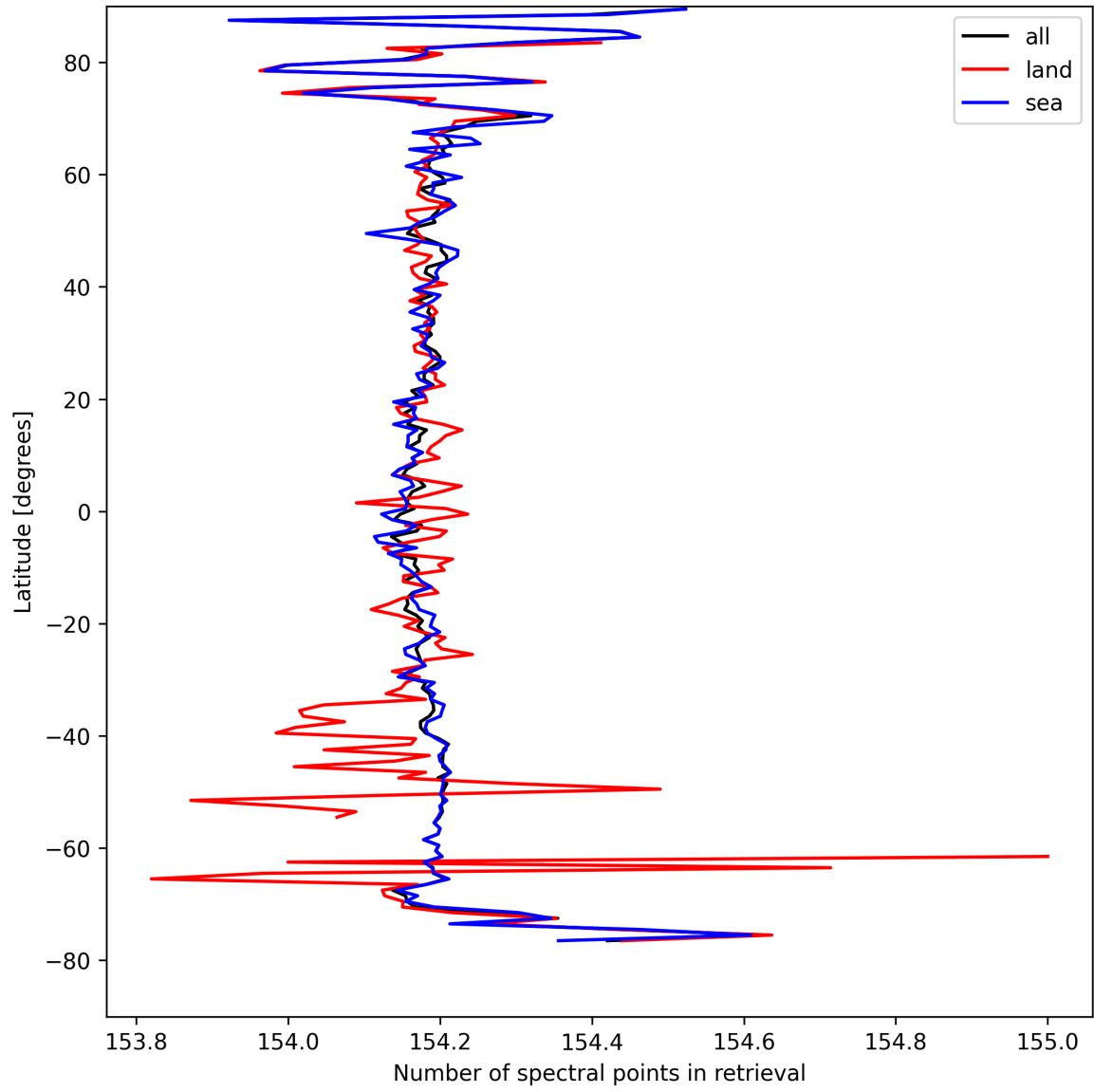
Figure 13: Zonal average of “Number of spectral points in retrieval” for 2025-04-10 to 2025-04-12.
