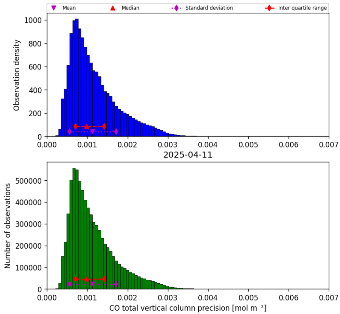
Figure 20: Histogram of “CO total vertical column precision” for 2025-04-10 to 2025-04-12
