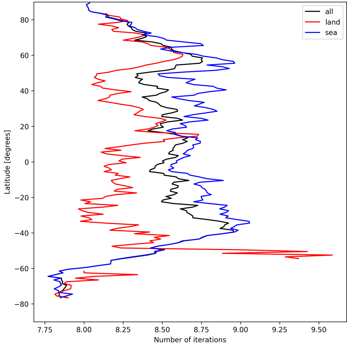
Figure 16: Zonal average of “Number of iterations” for 2025-04-10 to 2025-04-12.
