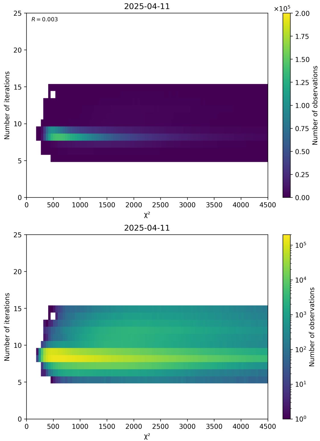
Figure 49: Scatter density plot of “ \chi^2 ” against “Number of iterations” for 2025-04-10 to 2025-04-12.
