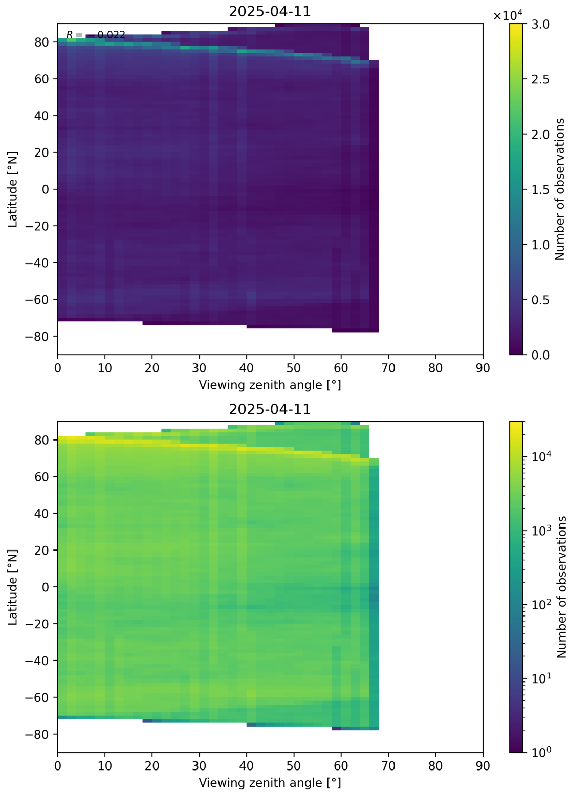
Figure 74: Scatter density plot of “Viewing zenith angle” against “Latitude” for 2025-04-10 to 2025-04-12.
