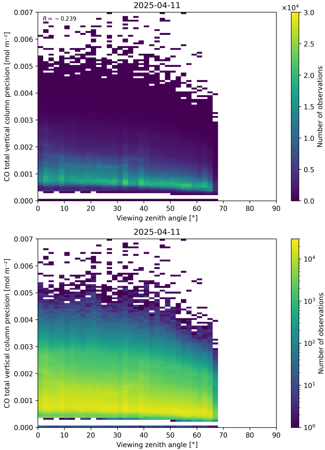
Figure 71: Scatter density plot of “Viewing zenith angle” against “CO total vertical column precision” for 2025-04-10 to 2025-04-12.
