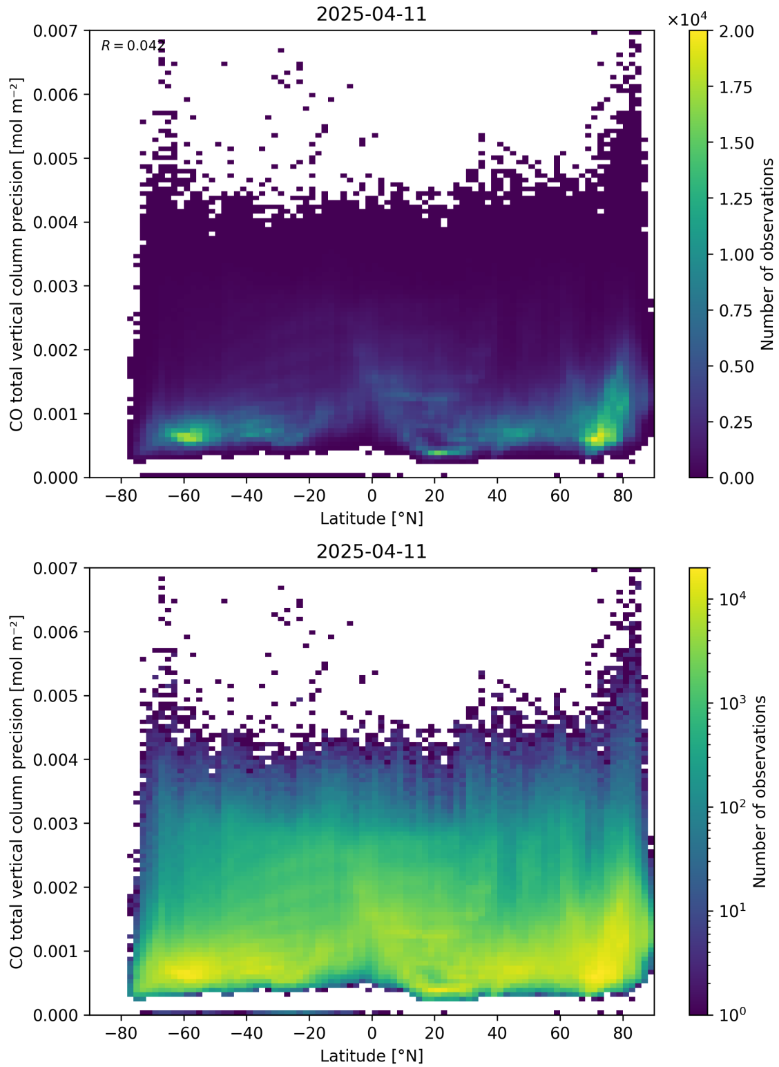
Figure 53: Scatter density plot of “Latitude” against “CO total vertical column precision” for 2025-04-10 to 2025-04-12.
