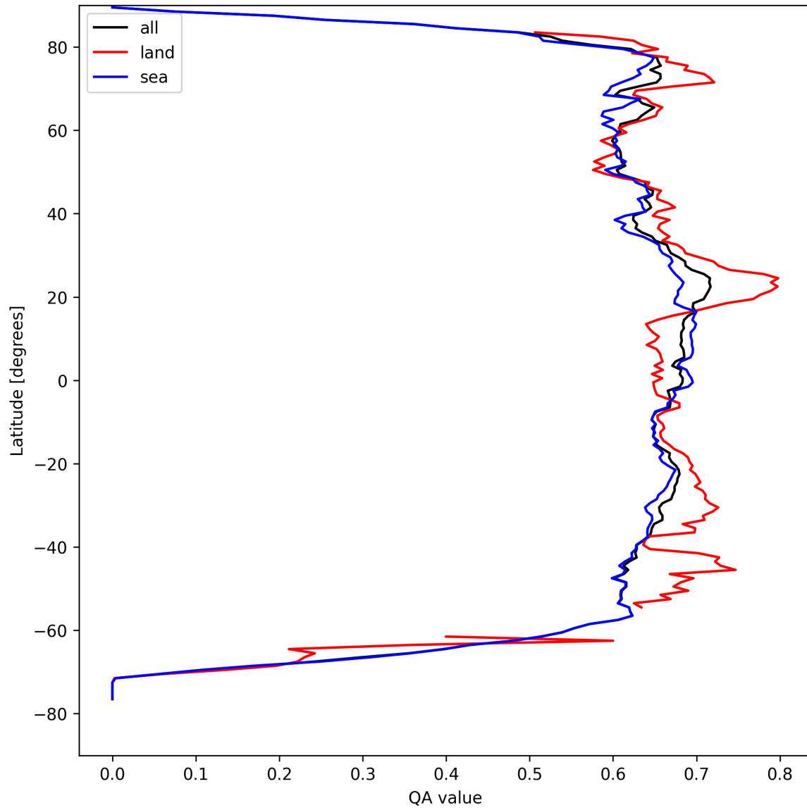
Figure 9: Zonal average of “QA value” for 2025-04-10 to 2025-04-12.
