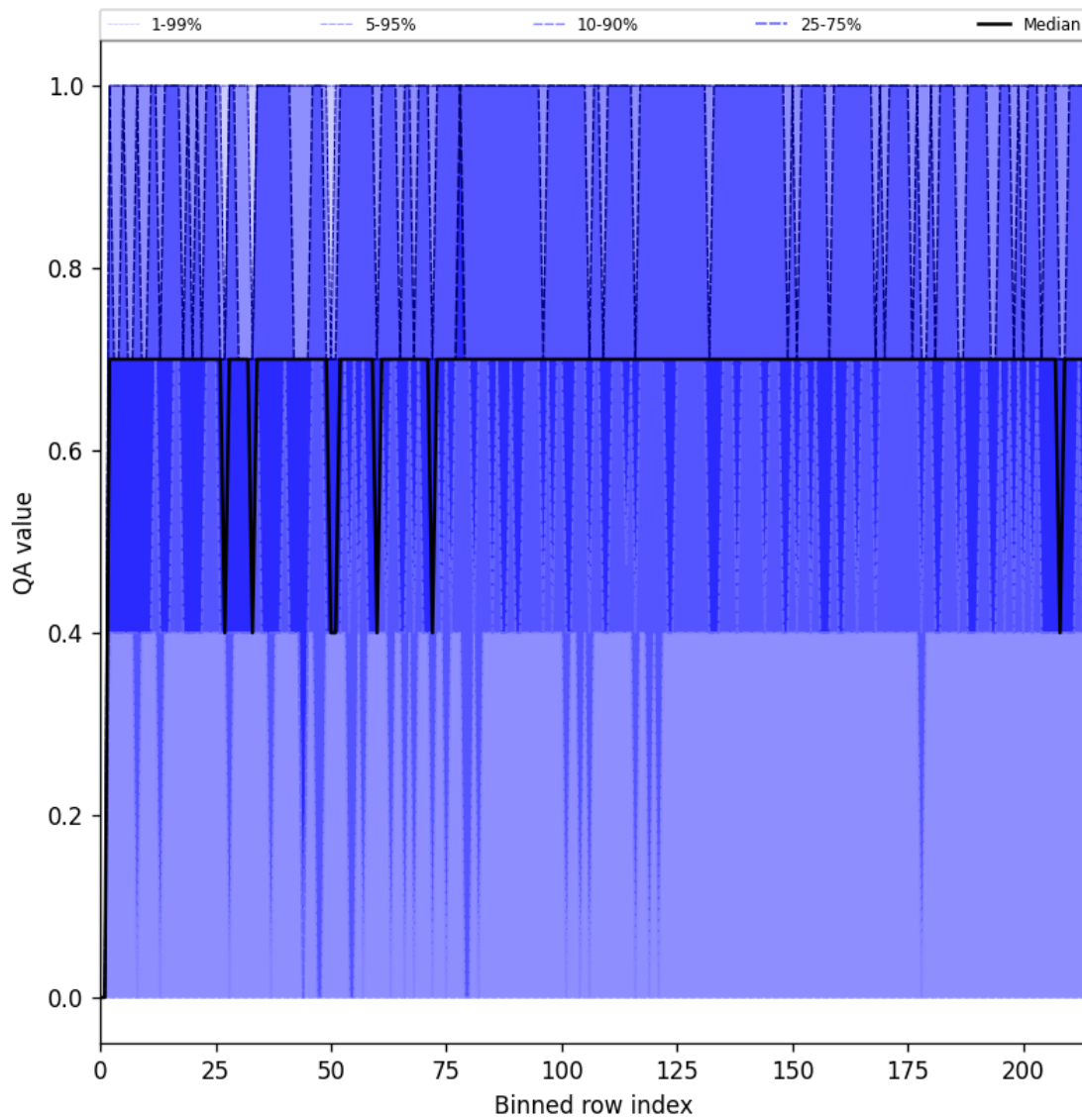
Figure 25: Along track statistics of “QA value” for 2025-04-10 to 2025-04-12
