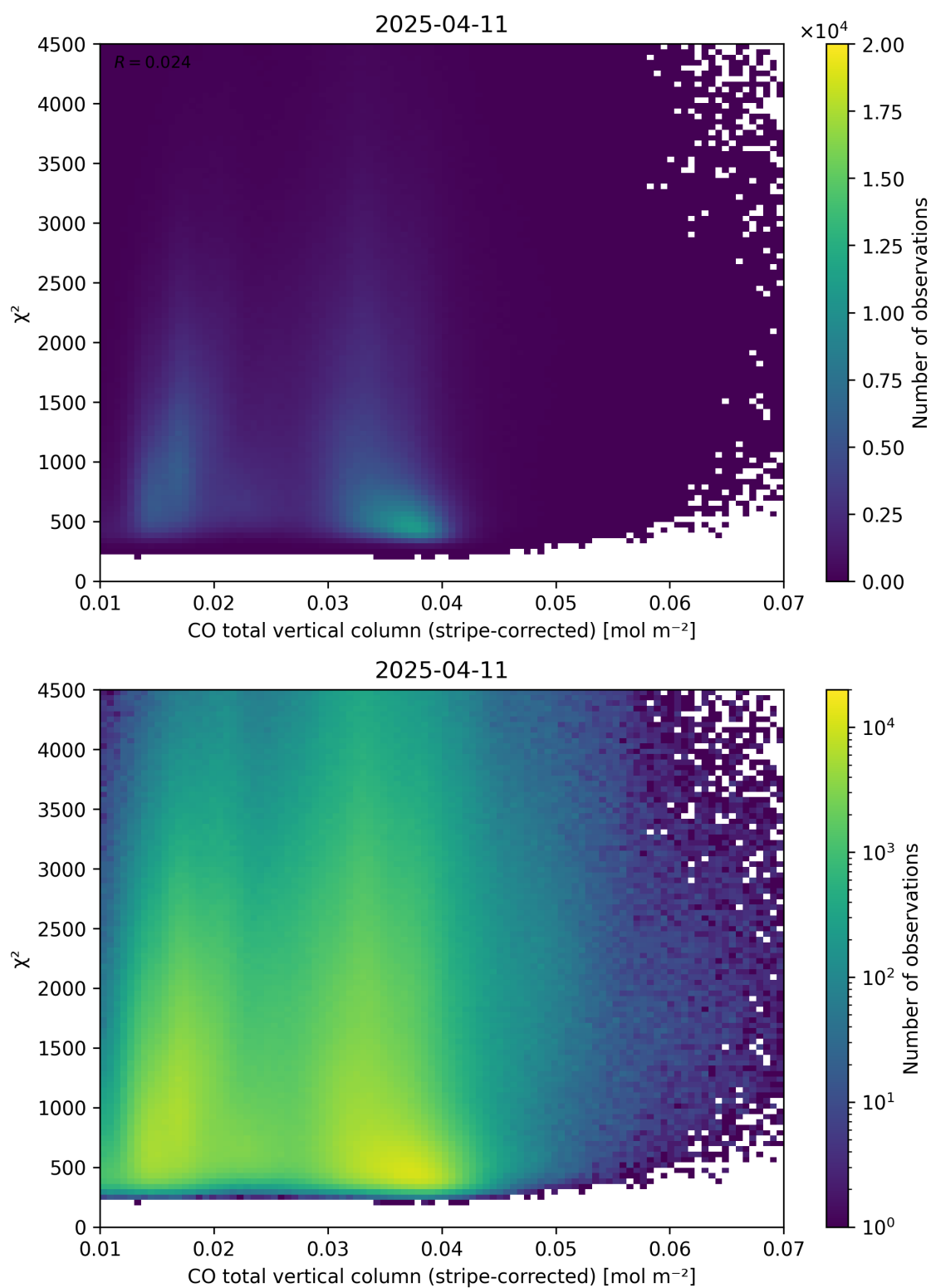
Figure 37: Scatter density plot of “CO total vertical column (stripe-corrected)” against “ \chi^2 ” for 2025-04-10 to 2025-04-12.
