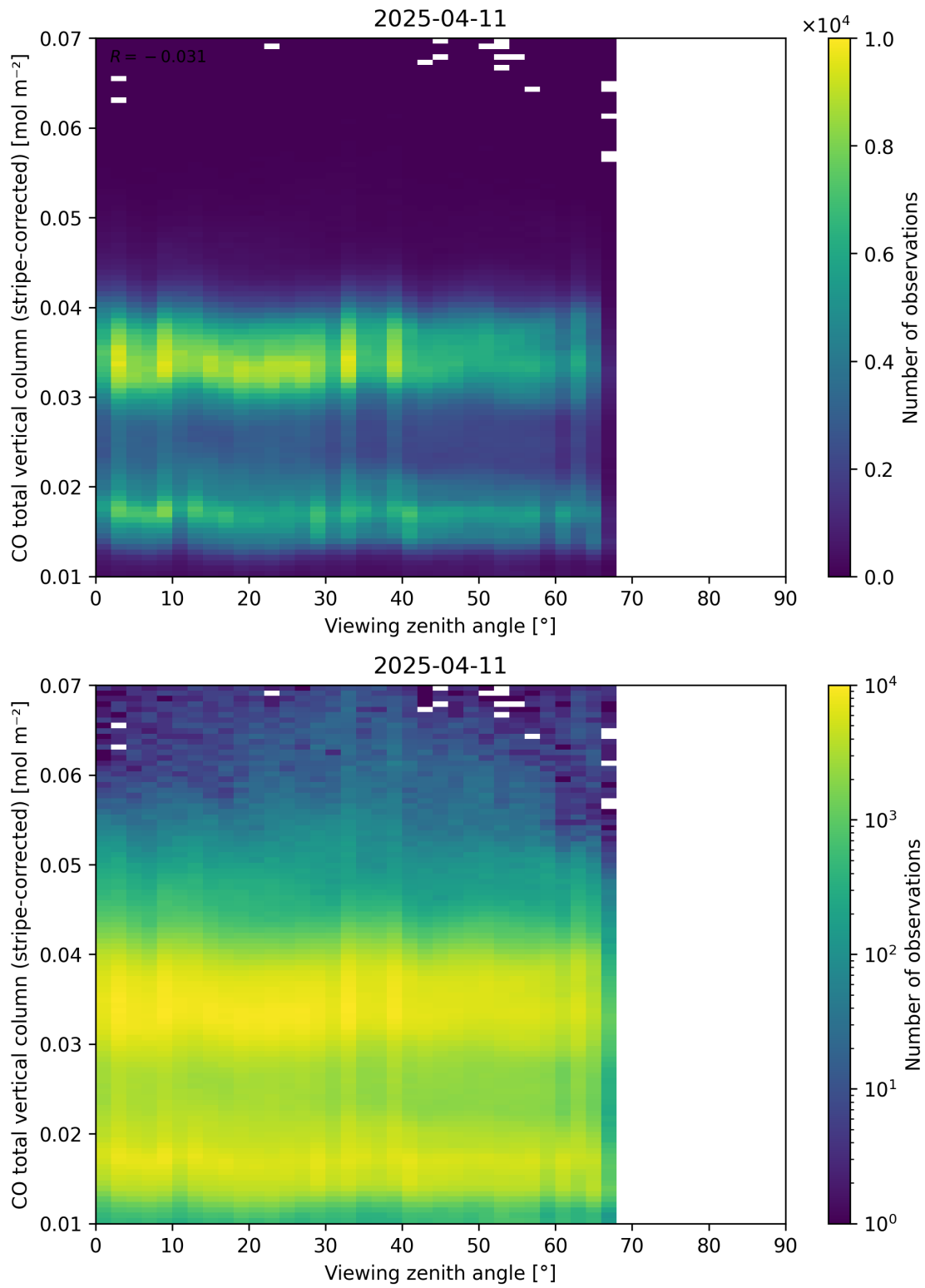
Figure 70: Scatter density plot of “Viewing zenith angle” against “CO total vertical column (stripe-corrected)” for 2025-04-10 to 2025-04-12.
