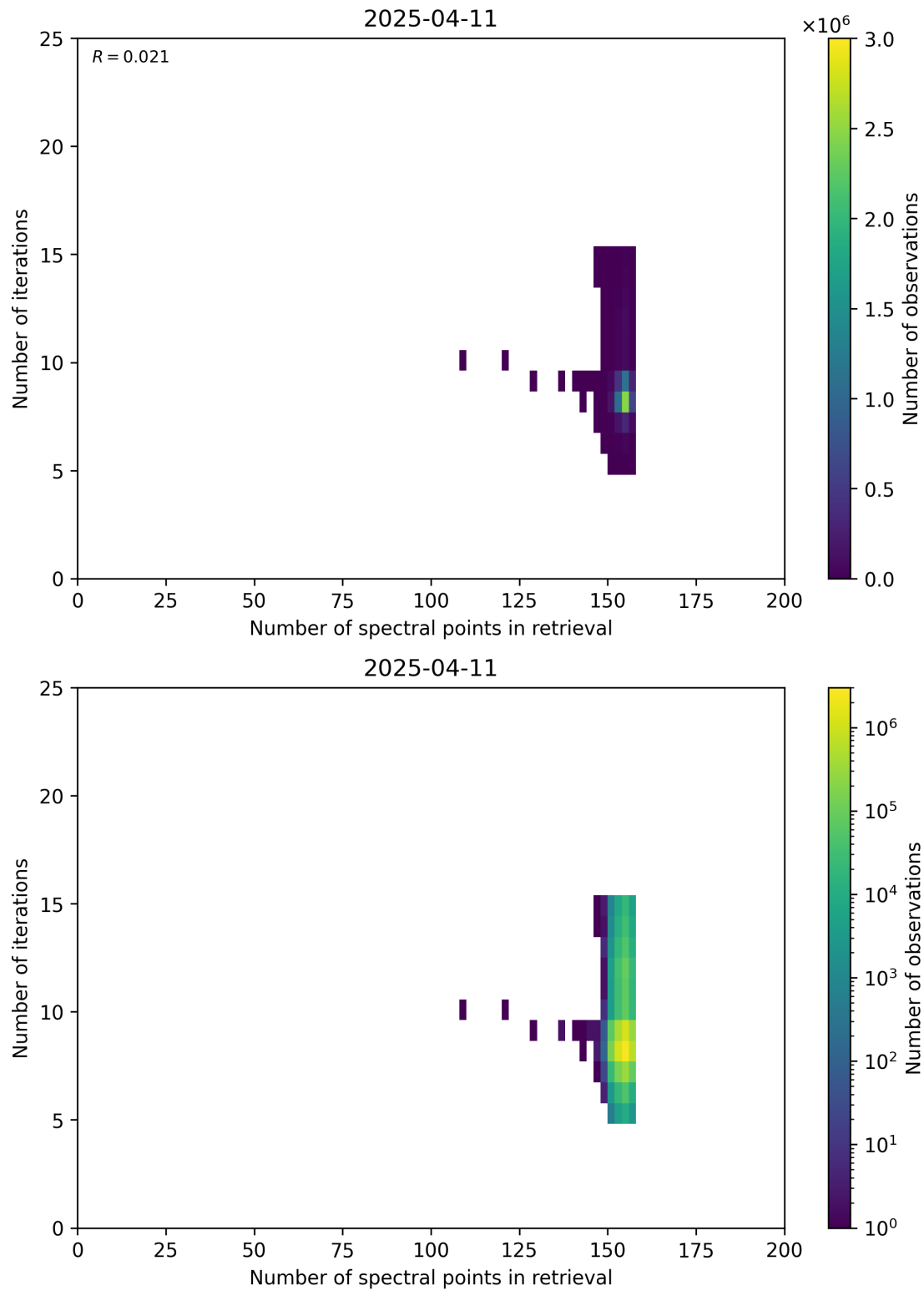
Figure 60: Scatter density plot of “Number of spectral points in retrieval” against “Number of iterations” for 2025-04-10 to 2025-04-12.
