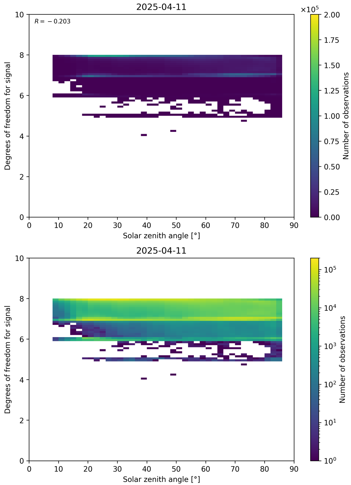
Figure 65: Scatter density plot of “Solar zenith angle” against “Degrees of freedom for signal” for 2025-04-10 to 2025-04-12.
