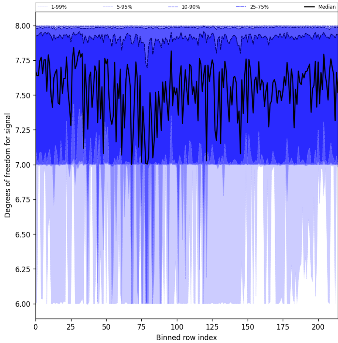
Figure 31: Along track statistics of “Degrees of freedom for signal” for 2025-04-10 to 2025-04-12
