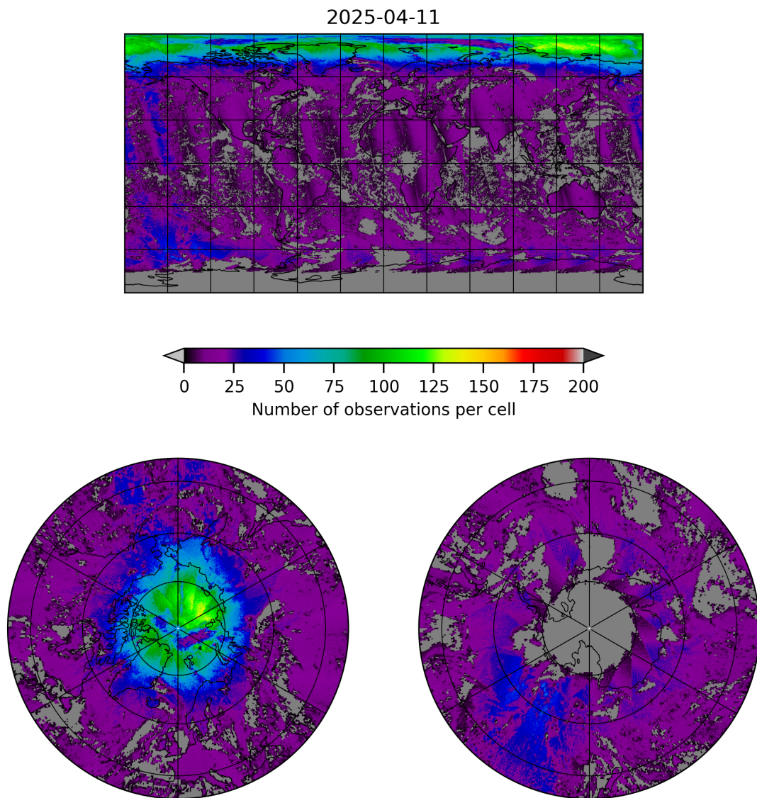
Figure 8: Map of the number of observations for 2025-04-10 to 2025-04-12
