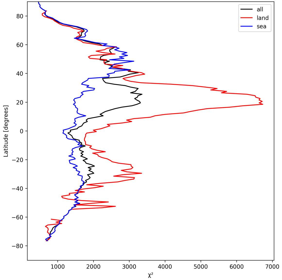
Figure 14: Zonal average of “ \chi^2 ” for 2025-04-10 to 2025-04-12.
