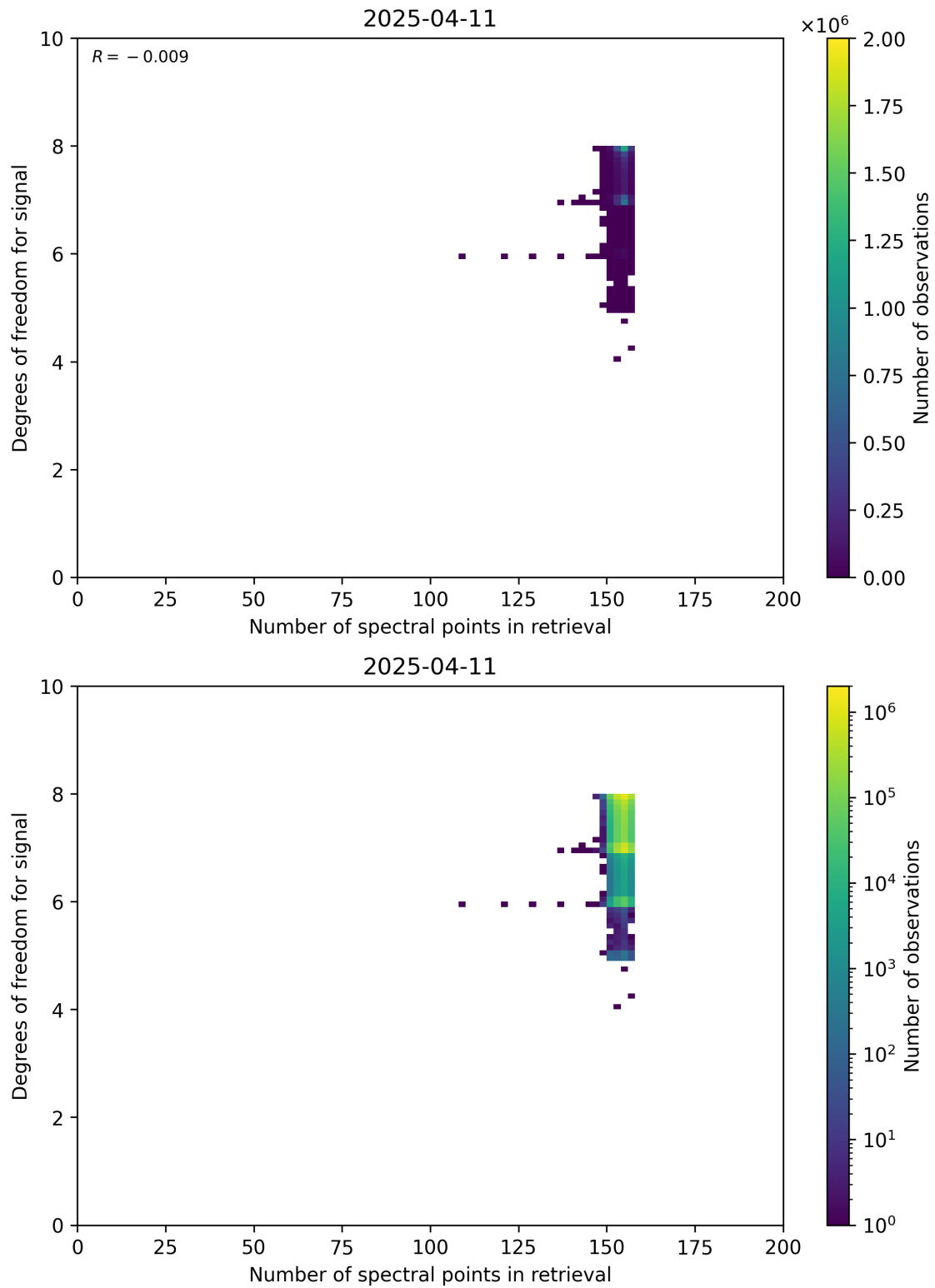
Figure 59: Scatter density plot of “Number of spectral points in retrieval” against “Degrees of freedom for signal” for 2025-04-10 to 2025-04-12.
