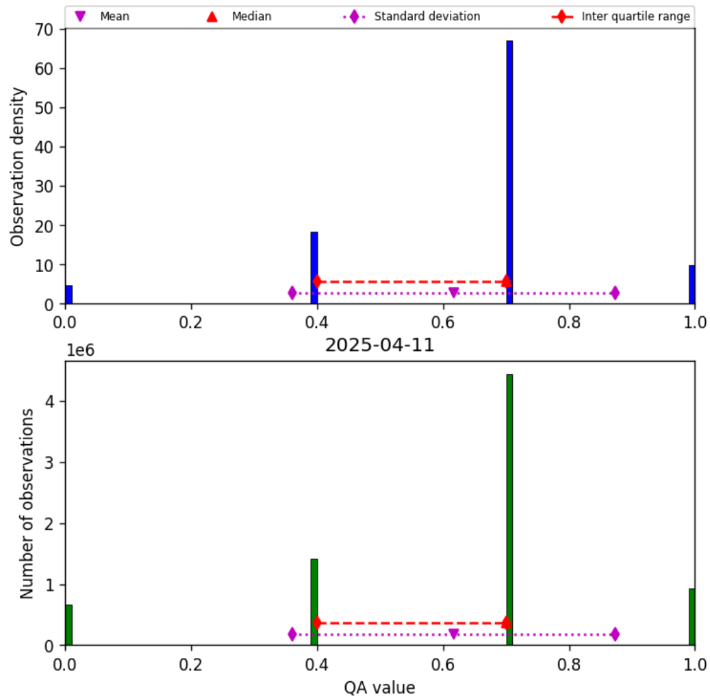
Figure 17: Histogram of “QA value” for 2025-04-10 to 2025-04-12
