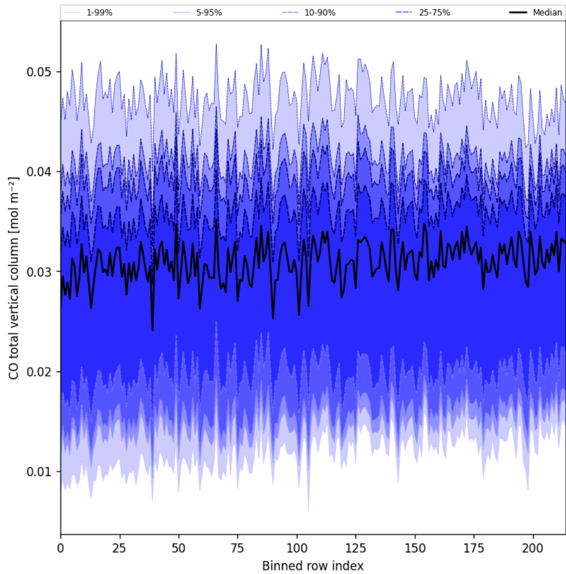
Figure 26: Along track statistics of “CO total vertical column” for 2025-04-11 to 2025-04-13
