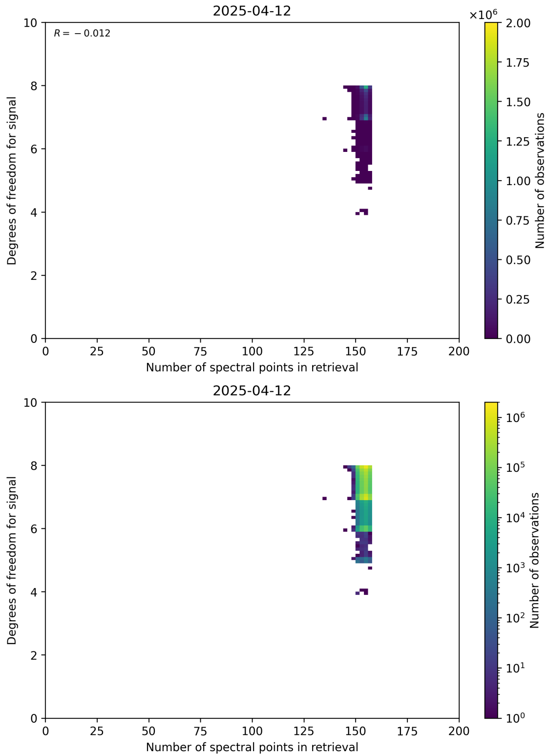
Figure 59: Scatter density plot of “Number of spectral points in retrieval” against “Degrees of freedom for signal” for 2025-04-11 to 2025-04-13.
