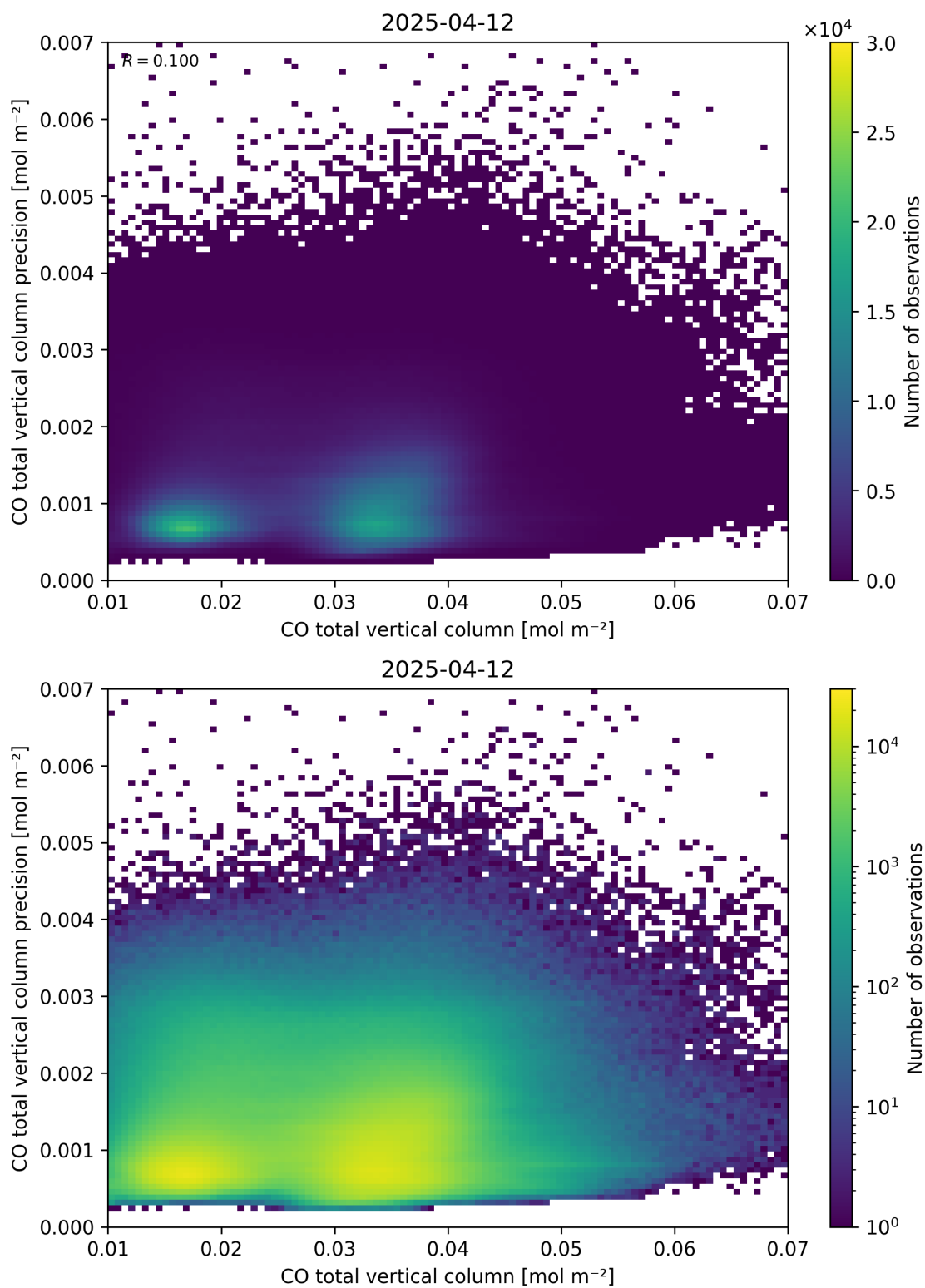
Figure 34: Scatter density plot of “CO total vertical column” against “CO total vertical column precision” for 2025-04-11 to 2025-04-13.
