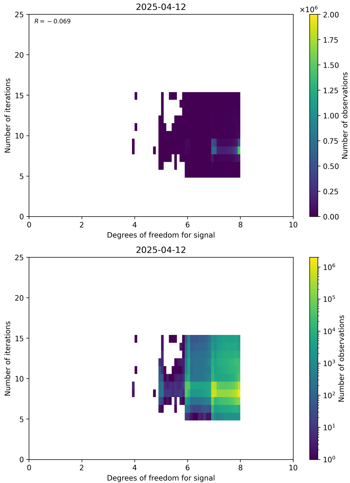
Figure 50: Scatter density plot of “Degrees of freedom for signal” against “Number of iterations” for 2025-04-11 to 2025-04-13.
