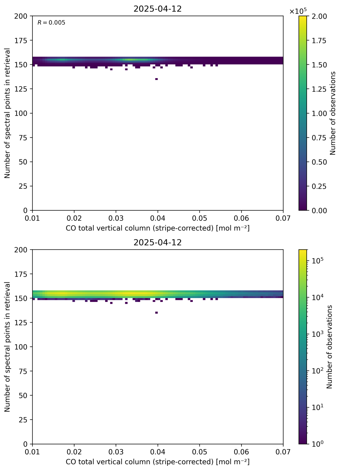
Figure 40: Scatter density plot of “CO total vertical column (stripe-corrected)” against “Number of spectral points in retrieval” for 2025-04-11 to 2025-04-13.
