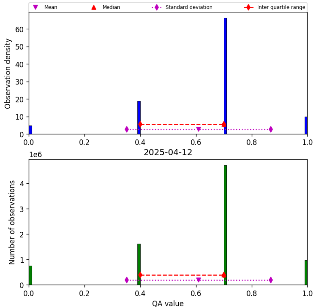
Figure 17: Histogram of “QA value” for 2025-04-11 to 2025-04-13
