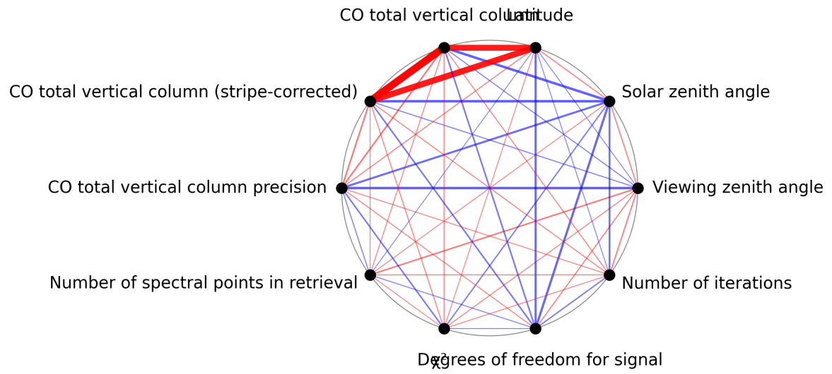
Figure 1: Map of correlation graph for 2025-04-11 to 2025-04-13.
