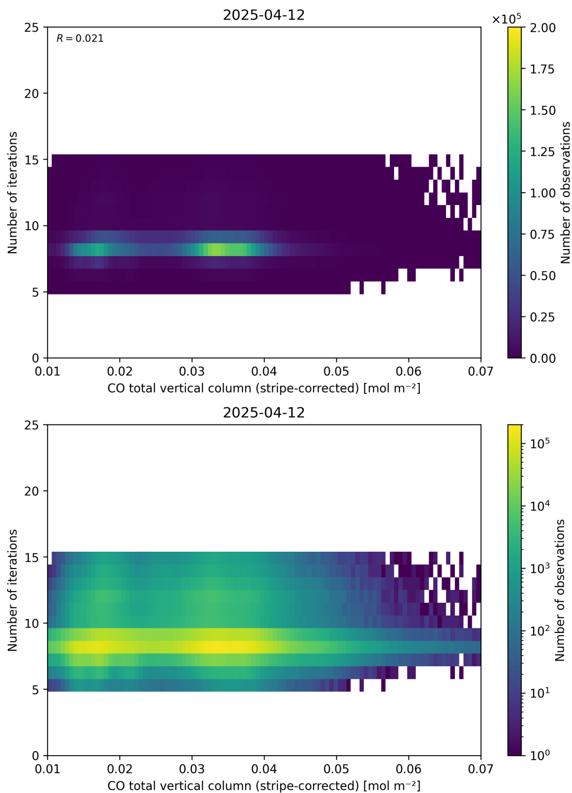
Figure 39: Scatter density plot of “CO total vertical column (stripe-corrected)” against “Number of iterations” for 2025-04-11 to 2025-04-13.
