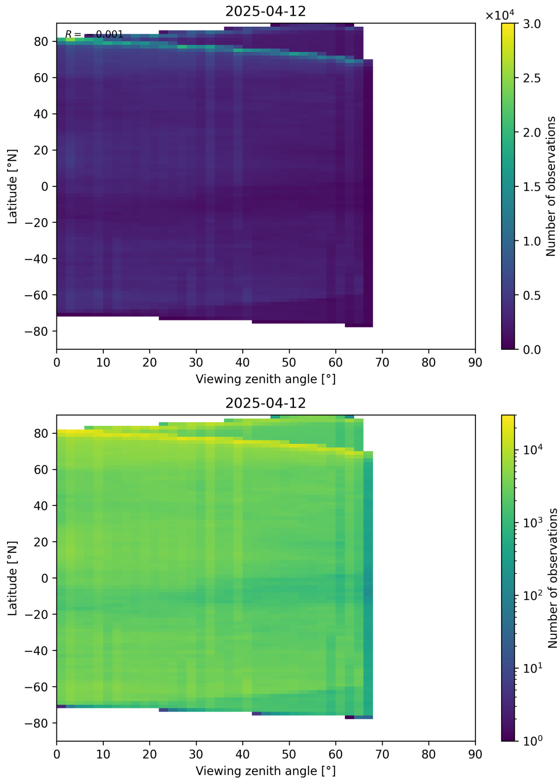
Figure 74: Scatter density plot of “Viewing zenith angle” against “Latitude” for 2025-04-11 to 2025-04-13.
