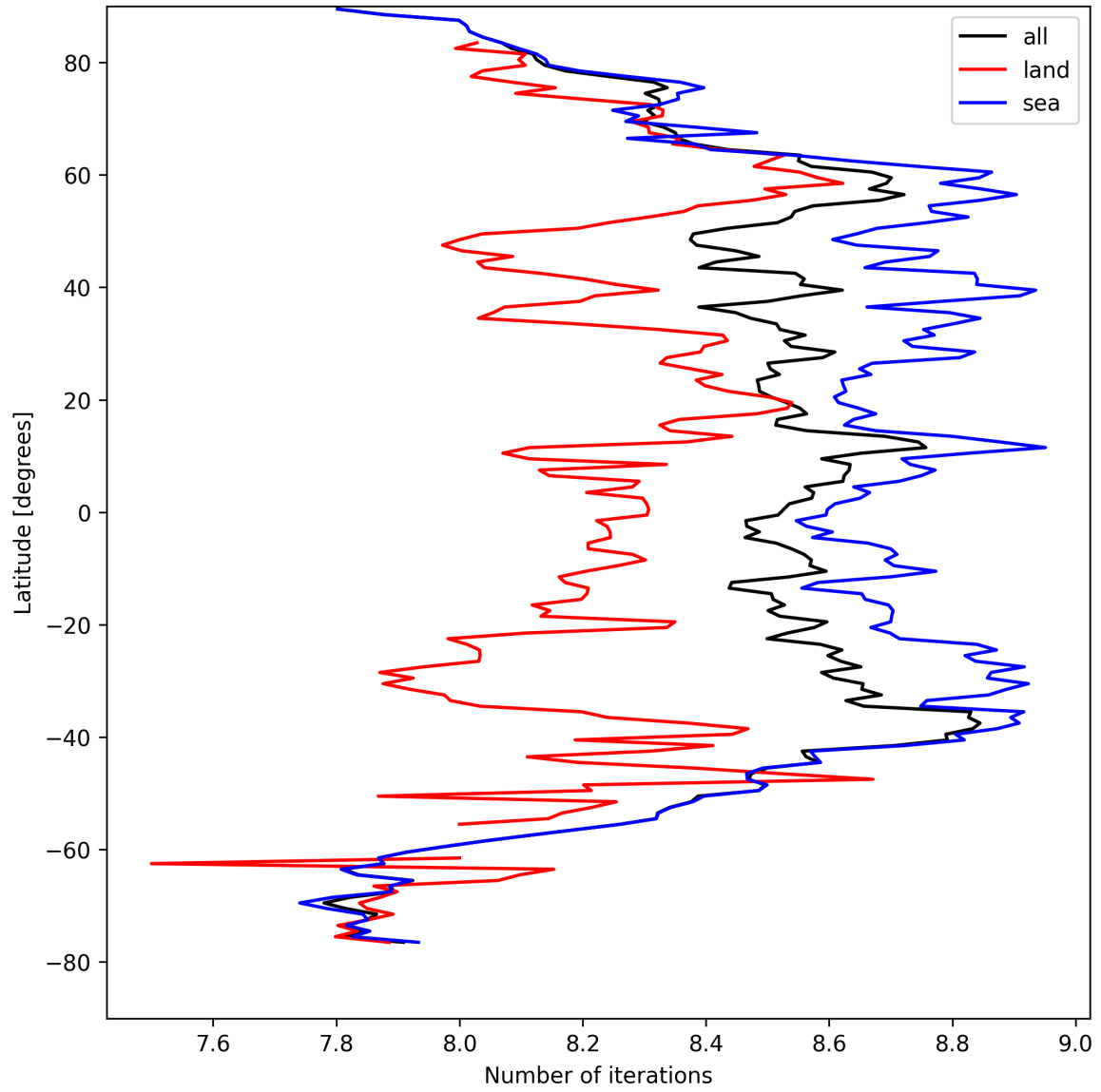
Figure 16: Zonal average of “Number of iterations” for 2025-04-11 to 2025-04-13.
