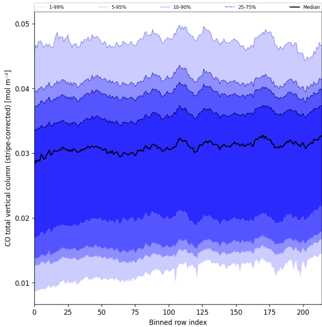
Figure 27: Along track statistics of “CO total vertical column (stripe-corrected)” for 2025-04-11 to 2025-04-13
