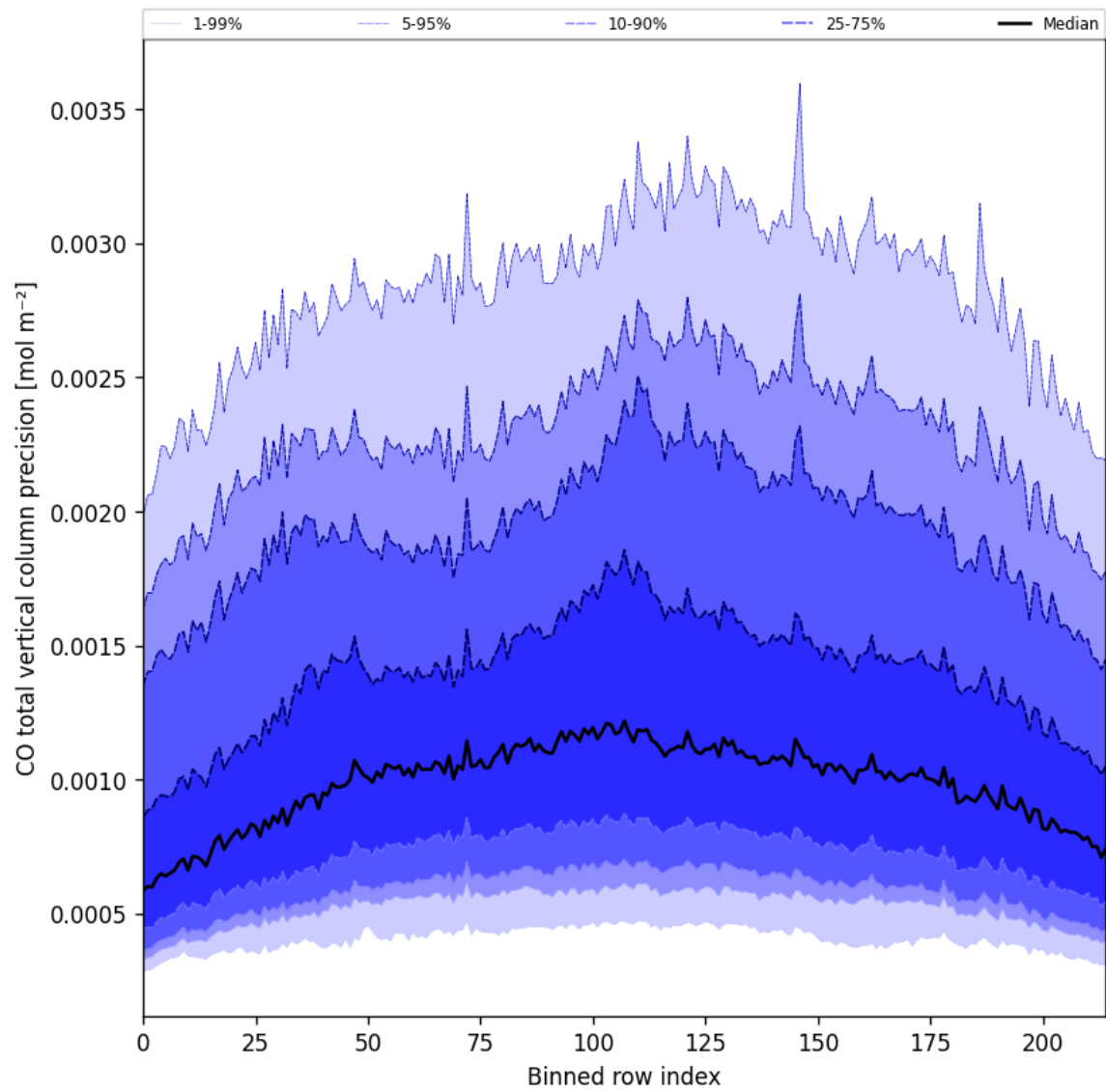
Figure 28: Along track statistics of “CO total vertical column precision” for 2025-04-11 to 2025-04-13
