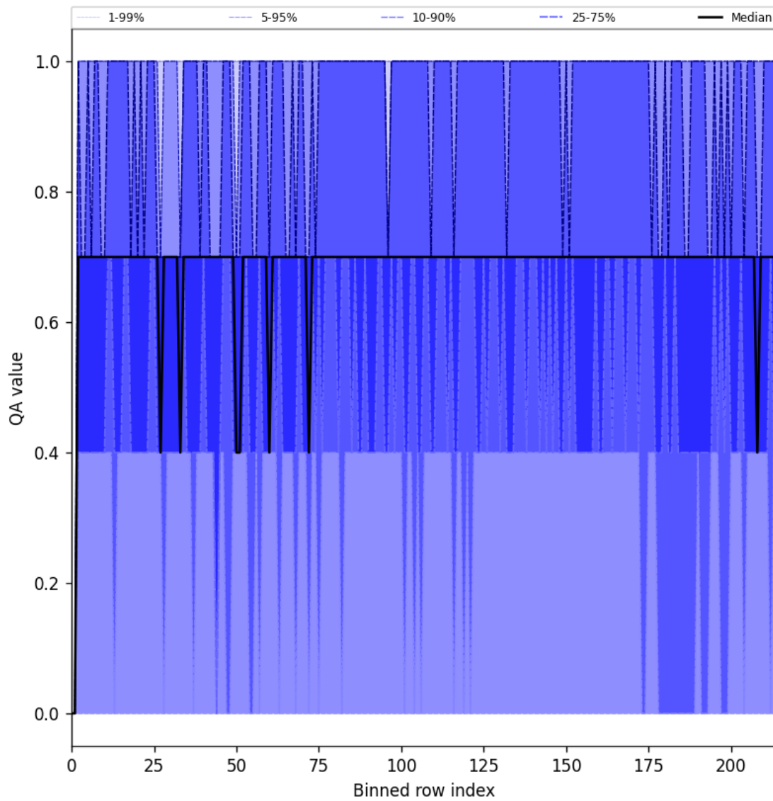
Figure 25: Along track statistics of “QA value” for 2025-04-11 to 2025-04-13
