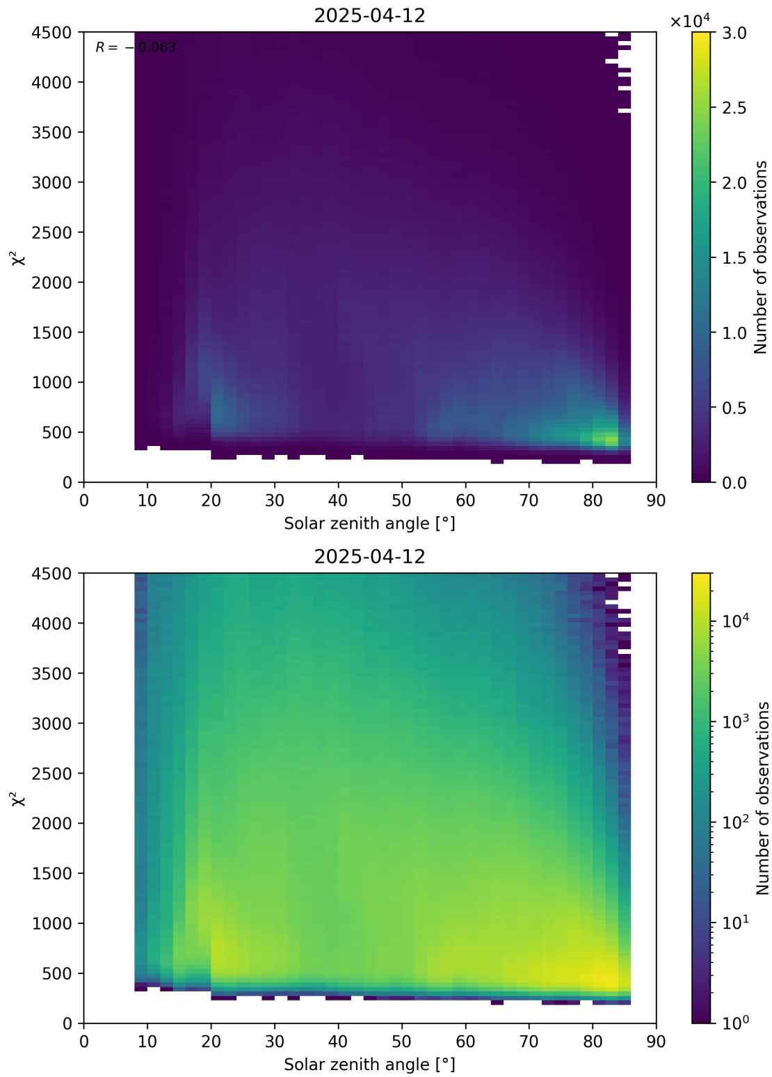
Figure 64: Scatter density plot of “Solar zenith angle” against “ \chi^2 ” for 2025-04-11 to 2025-04-13.
