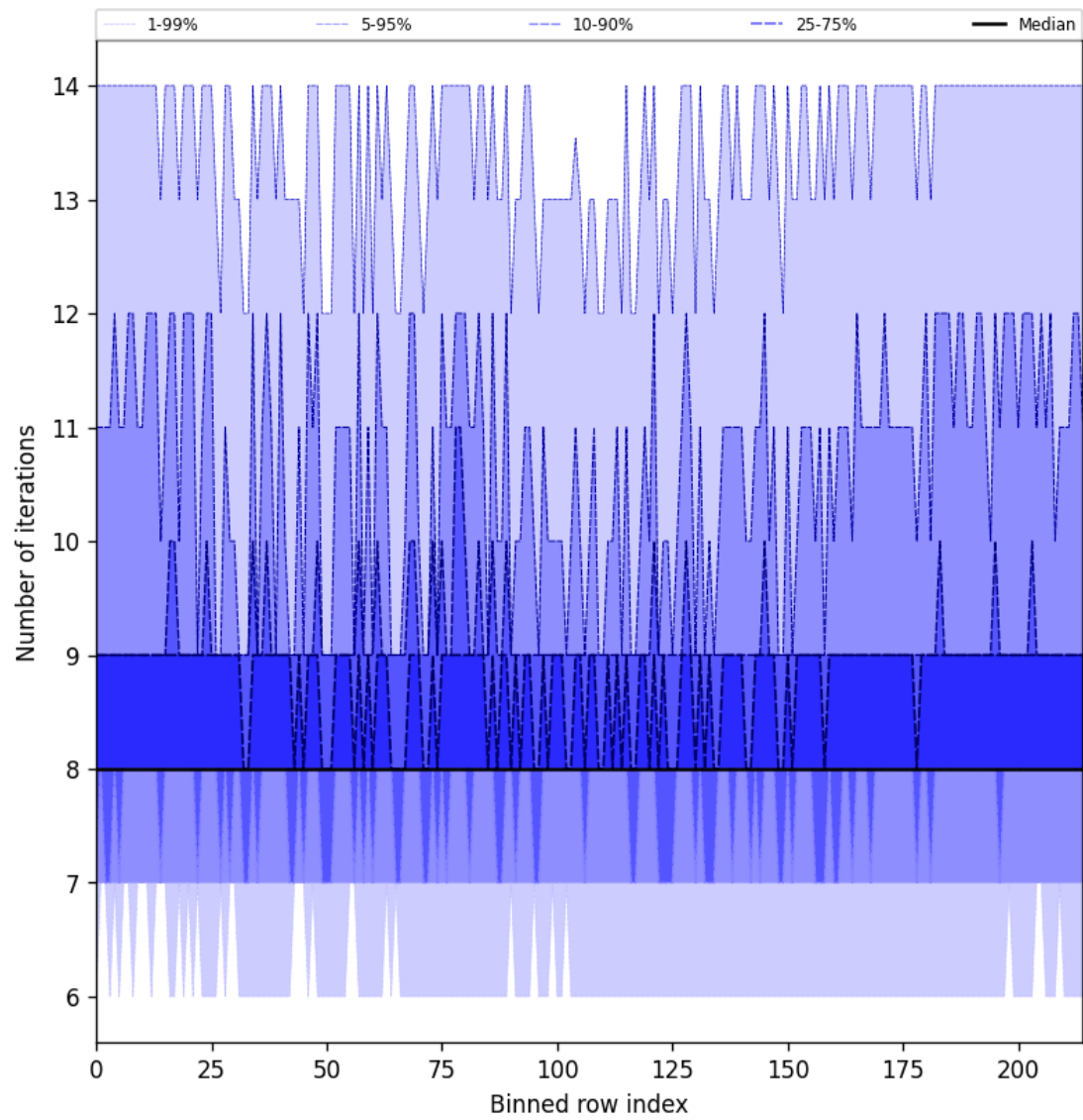
Figure 32: Along track statistics of “Number of iterations” for 2025-04-11 to 2025-04-13
