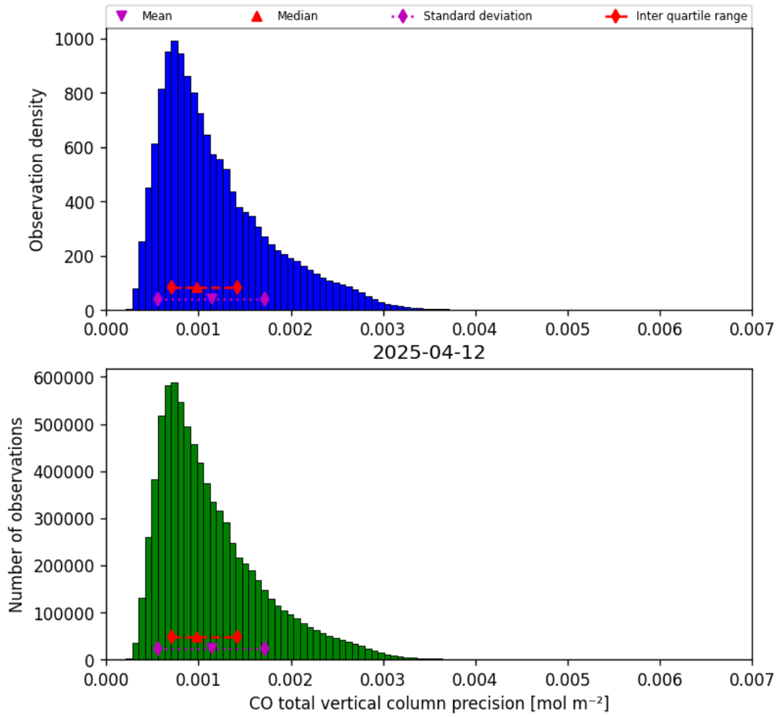
Figure 20: Histogram of “CO total vertical column precision” for 2025-04-11 to 2025-04-13
