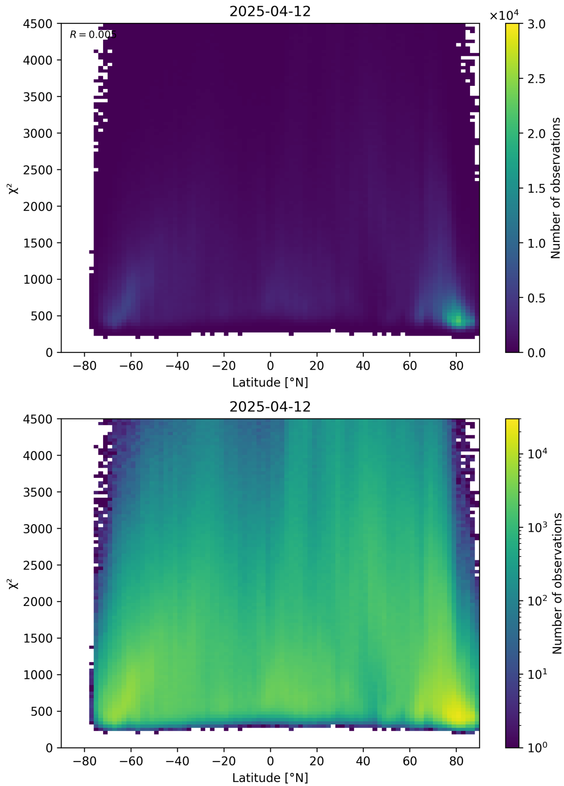
Figure 54: Scatter density plot of “Latitude” against “ \chi^2 ” for 2025-04-11 to 2025-04-13.
