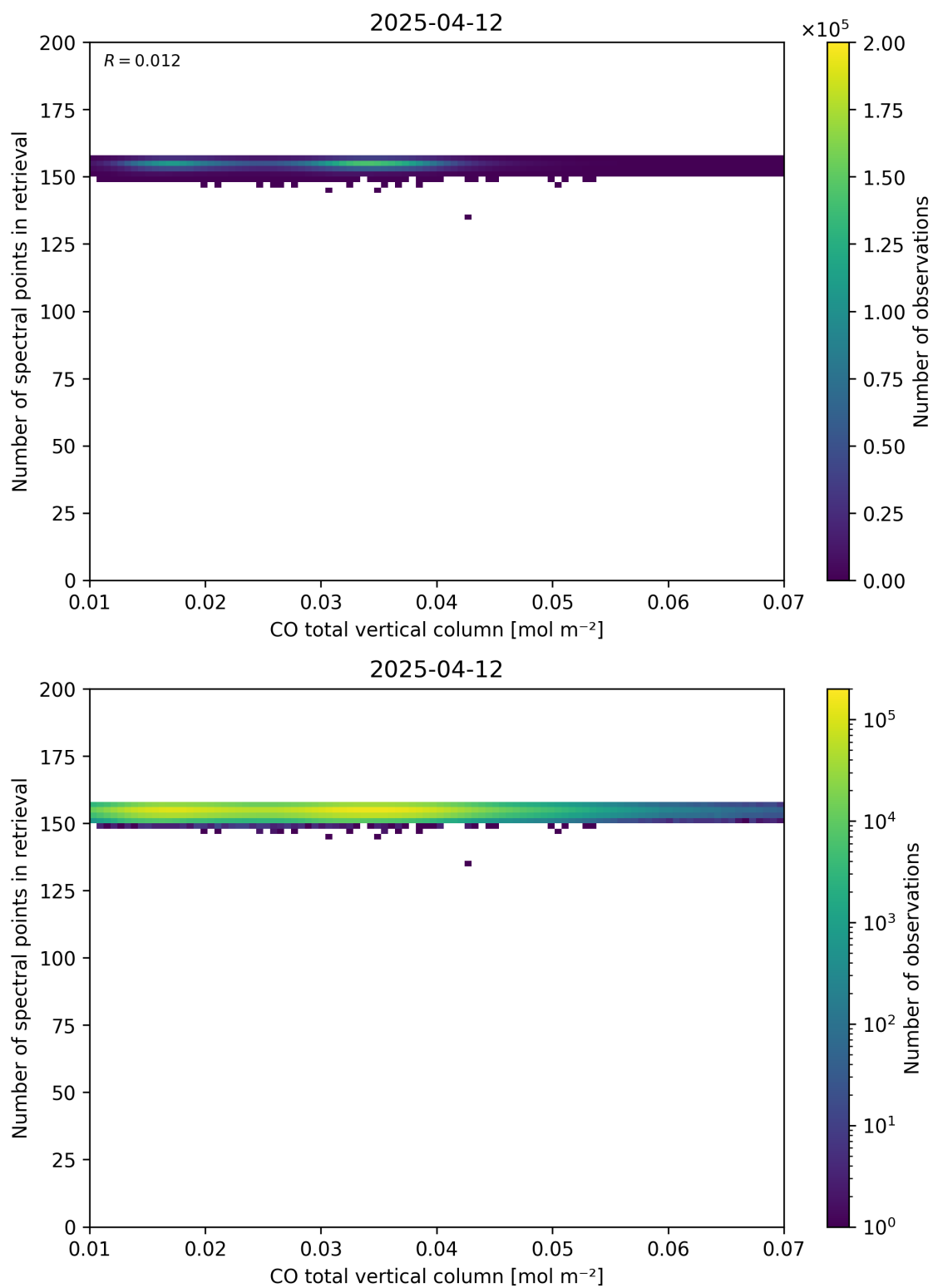
Figure 43: Scatter density plot of “CO total vertical column” against “Number of spectral points in retrieval” for 2025-04-11 to 2025-04-13.
