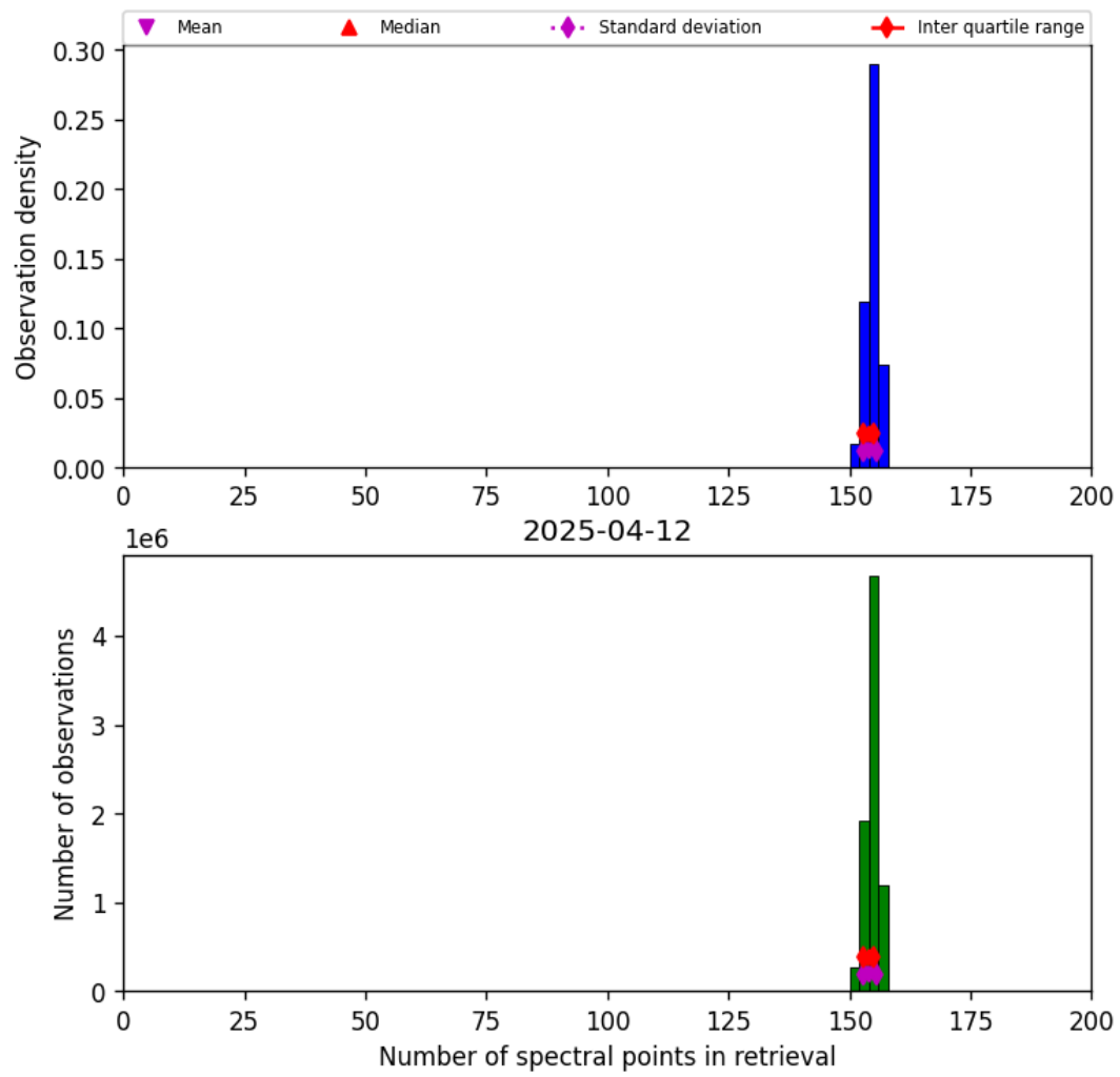
Figure 21: Histogram of “Number of spectral points in retrieval” for 2025-04-11 to 2025-04-13
