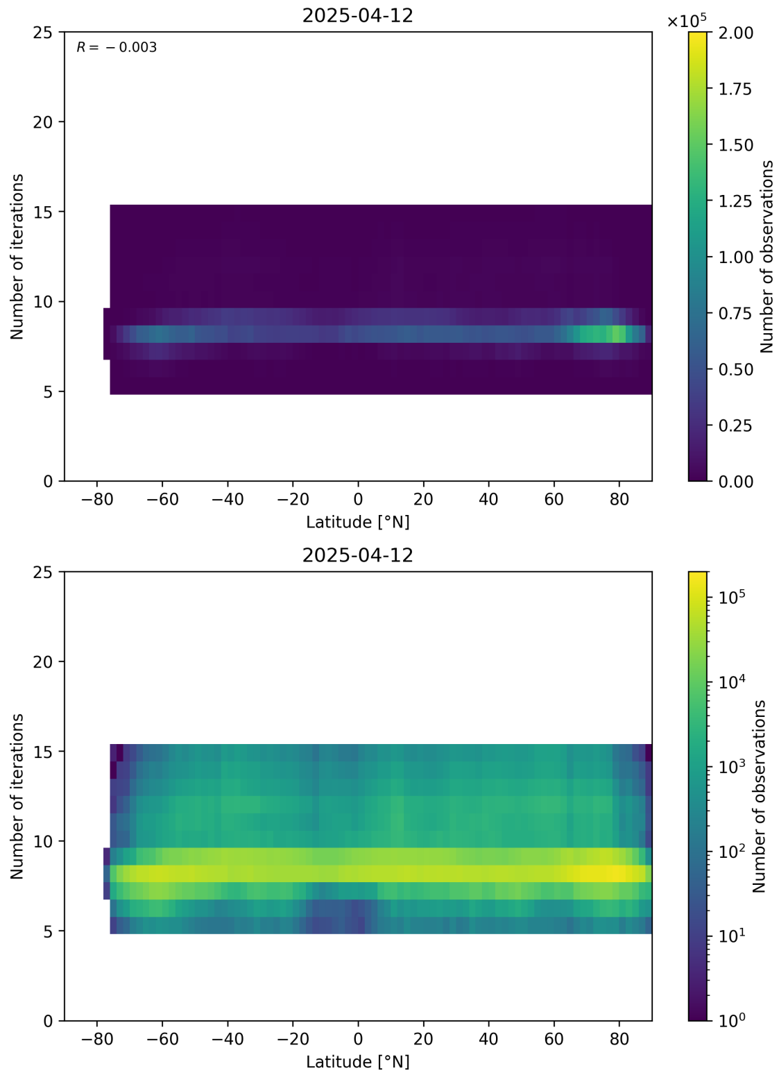
Figure 56: Scatter density plot of “Latitude” against “Number of iterations” for 2025-04-11 to 2025-04-13.
