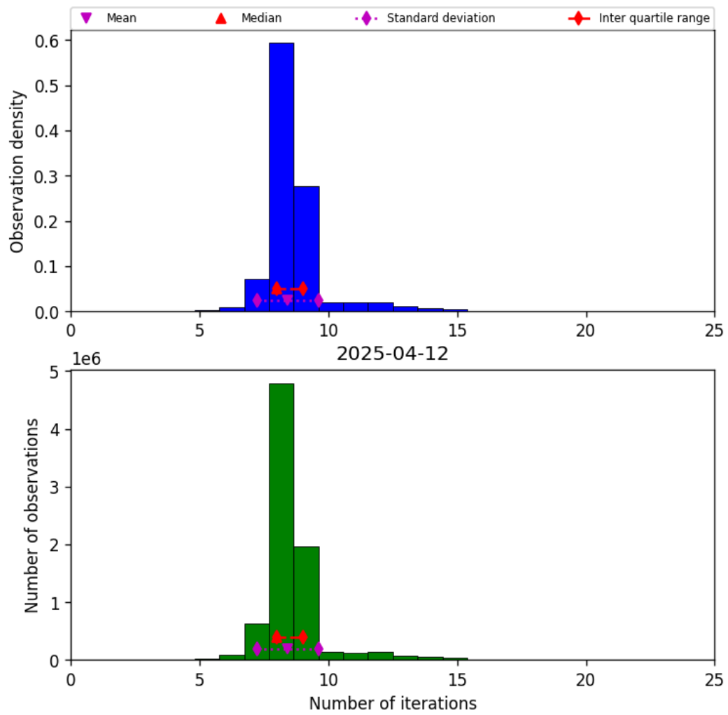
Figure 24: Histogram of “Number of iterations” for 2025-04-11 to 2025-04-13
