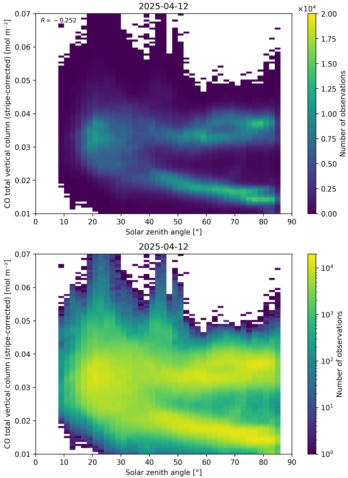
Figure 62: Scatter density plot of “Solar zenith angle” against “CO total vertical column (stripe-corrected)” for 2025-04-11 to 2025-04-13.
