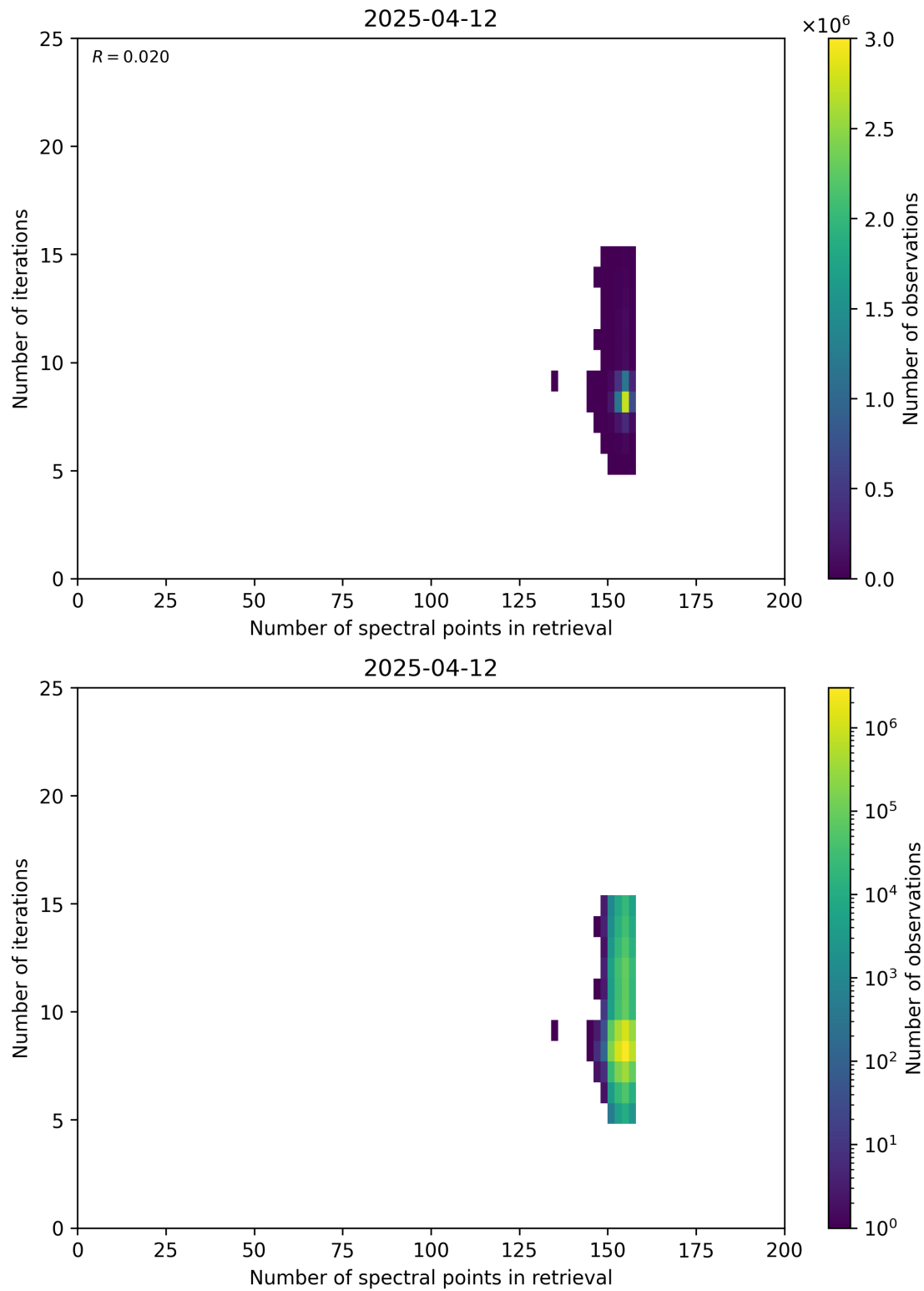
Figure 60: Scatter density plot of “Number of spectral points in retrieval” against “Number of iterations” for 2025-04-11 to 2025-04-13.
