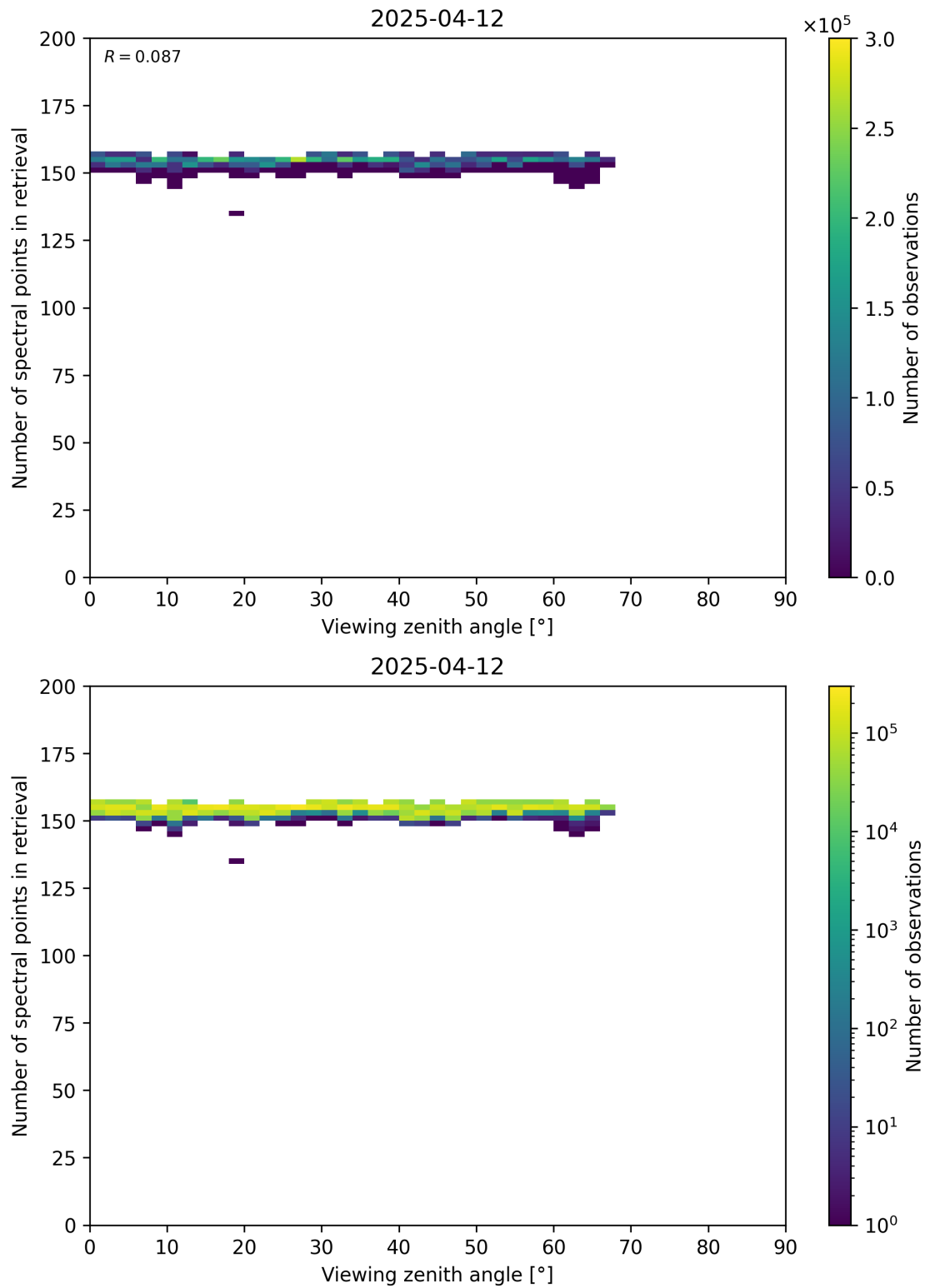
Figure 76: Scatter density plot of “Viewing zenith angle” against “Number of spectral points in retrieval” for 2025-04-11 to 2025-04-13.
