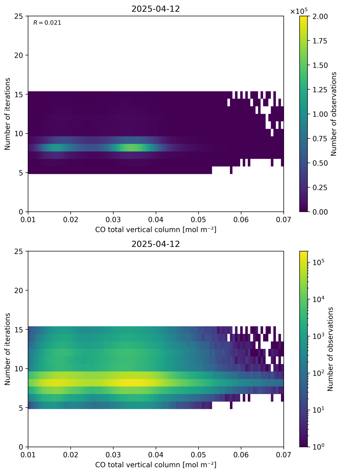
Figure 42: Scatter density plot of “CO total vertical column” against “Number of iterations” for 2025-04-11 to 2025-04-13.
