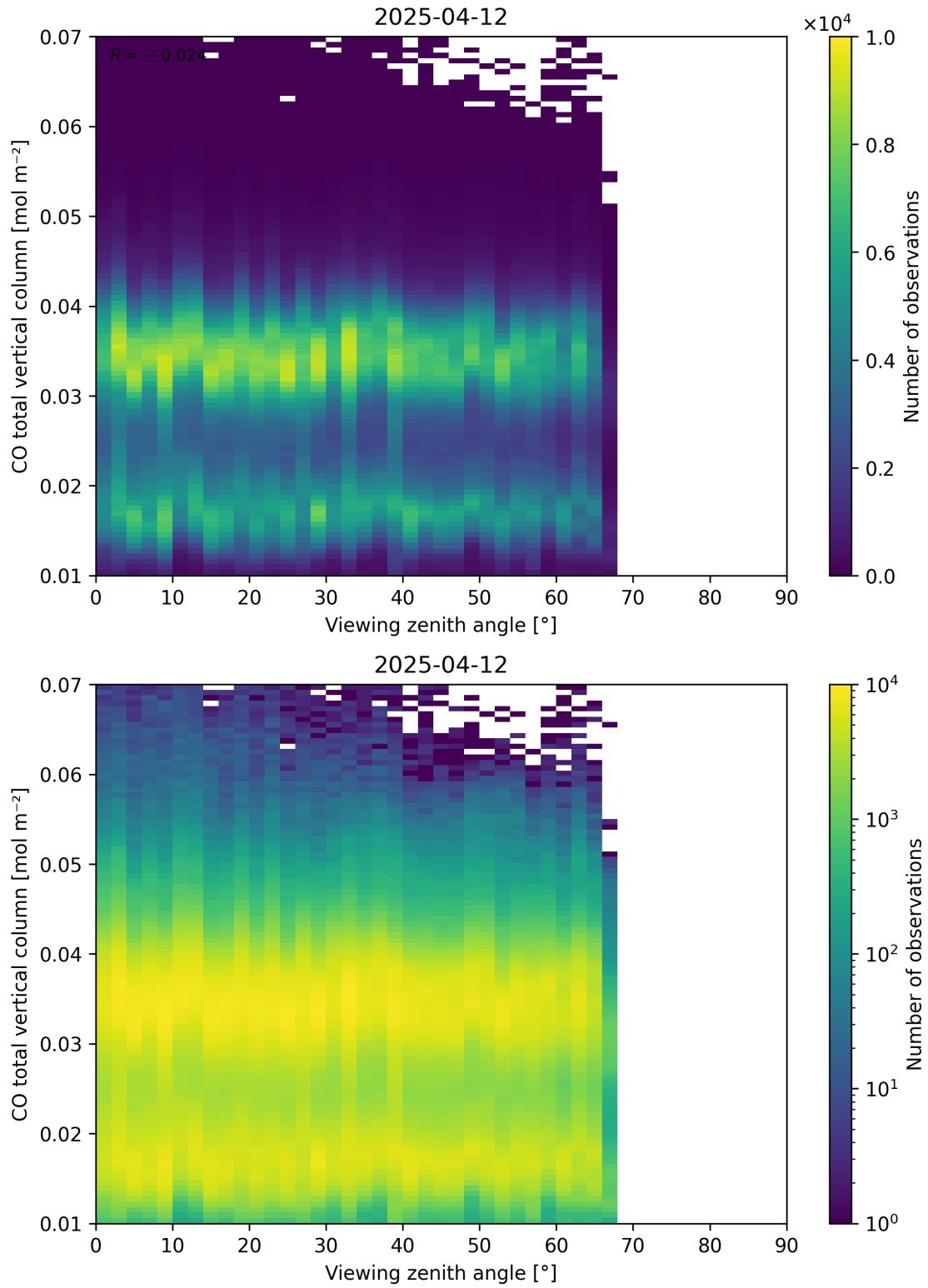
Figure 69: Scatter density plot of “Viewing zenith angle” against “CO total vertical column” for 2025-04-11 to 2025-04-13.
