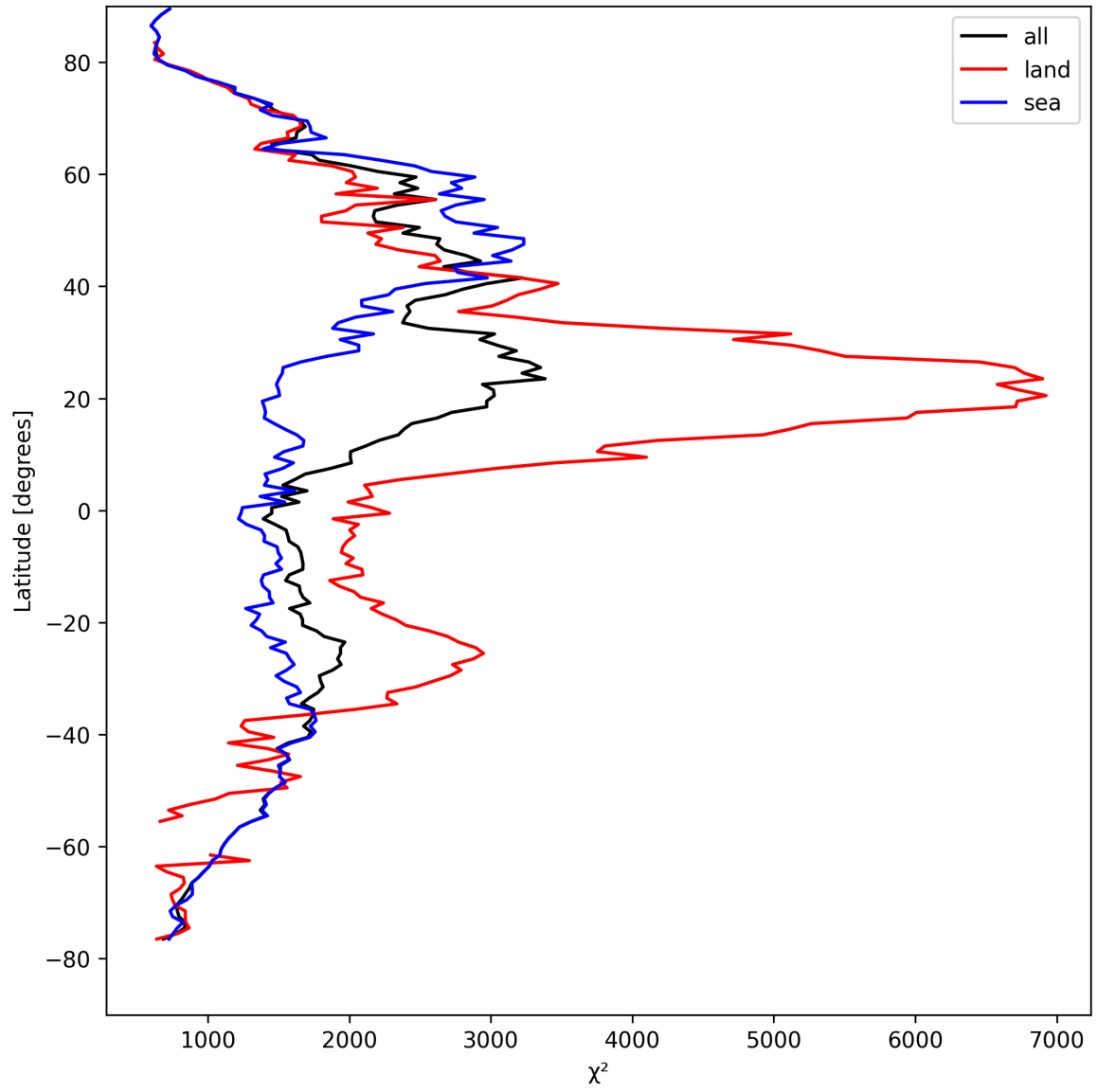
Figure 14: Zonal average of “ \chi^2 ” for 2025-04-11 to 2025-04-13.
