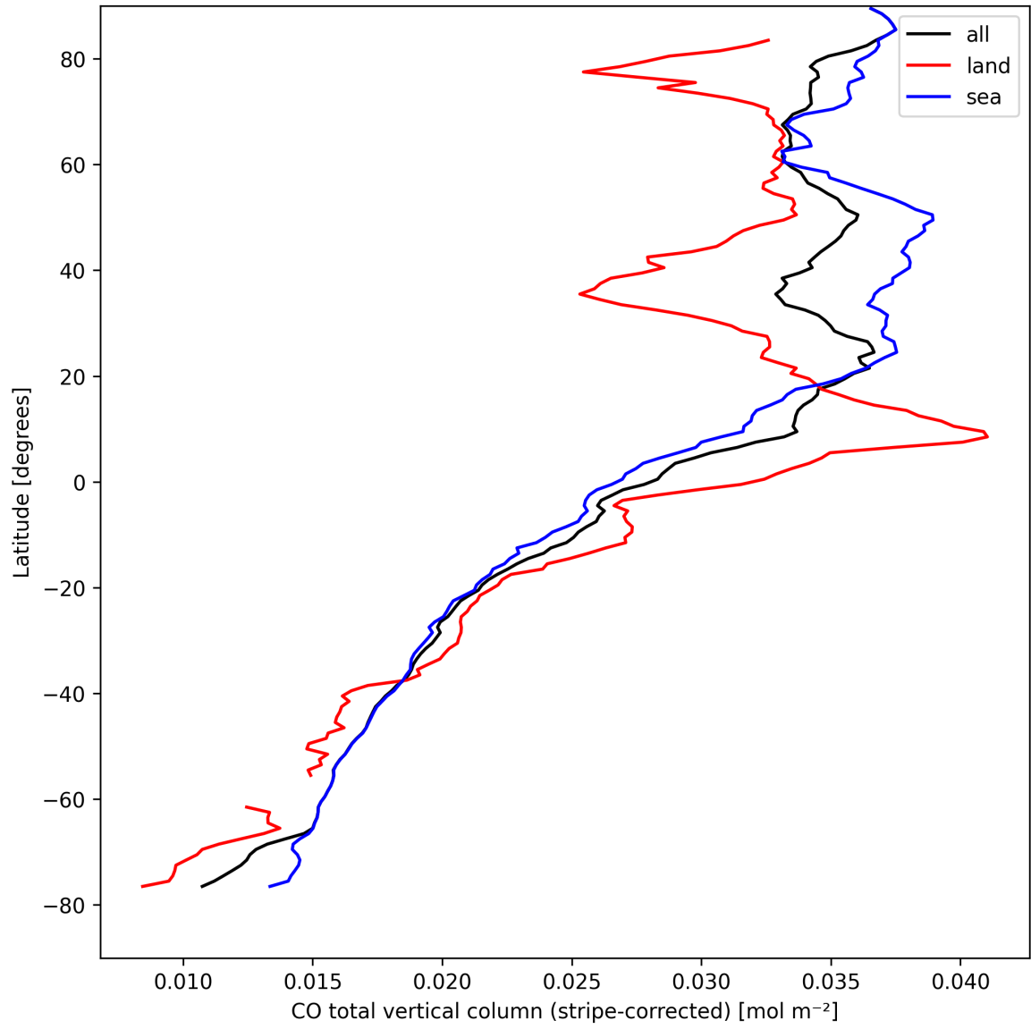
Figure 11: Zonal average of “CO total vertical column (stripe-corrected)” for 2025-04-11 to 2025-04-13.
