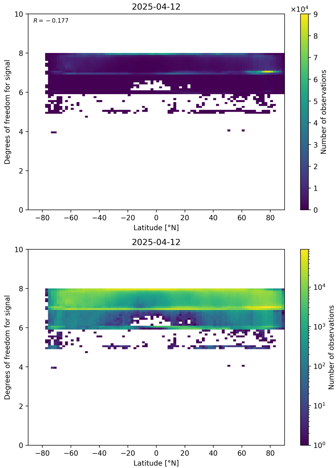
Figure 55: Scatter density plot of “Latitude” against “Degrees of freedom for signal” for 2025-04-11 to 2025-04-13.
