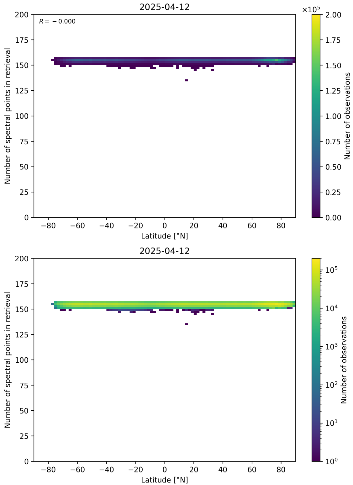
Figure 57: Scatter density plot of “Latitude” against “Number of spectral points in retrieval” for 2025-04-11 to 2025-04-13.
