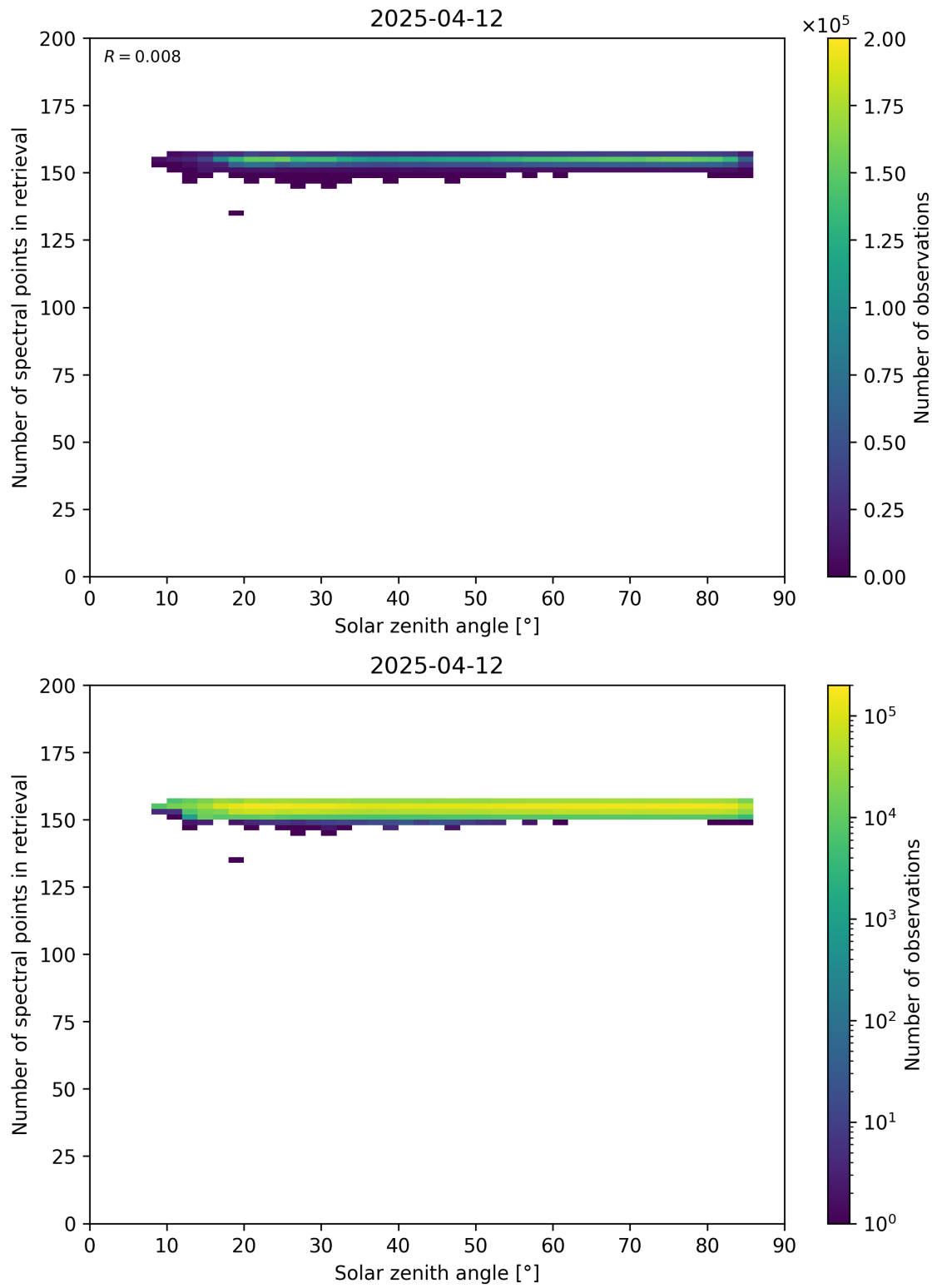
Figure 68: Scatter density plot of “Solar zenith angle” against “Number of spectral points in retrieval” for 2025-04-11 to 2025-04-13.
