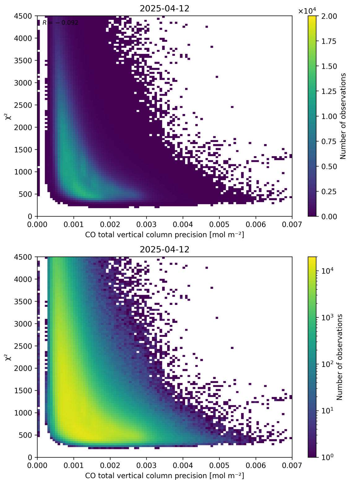
Figure 44: Scatter density plot of “CO total vertical column precision” against “ \chi^2 ” for 2025-04-11 to 2025-04-13.
