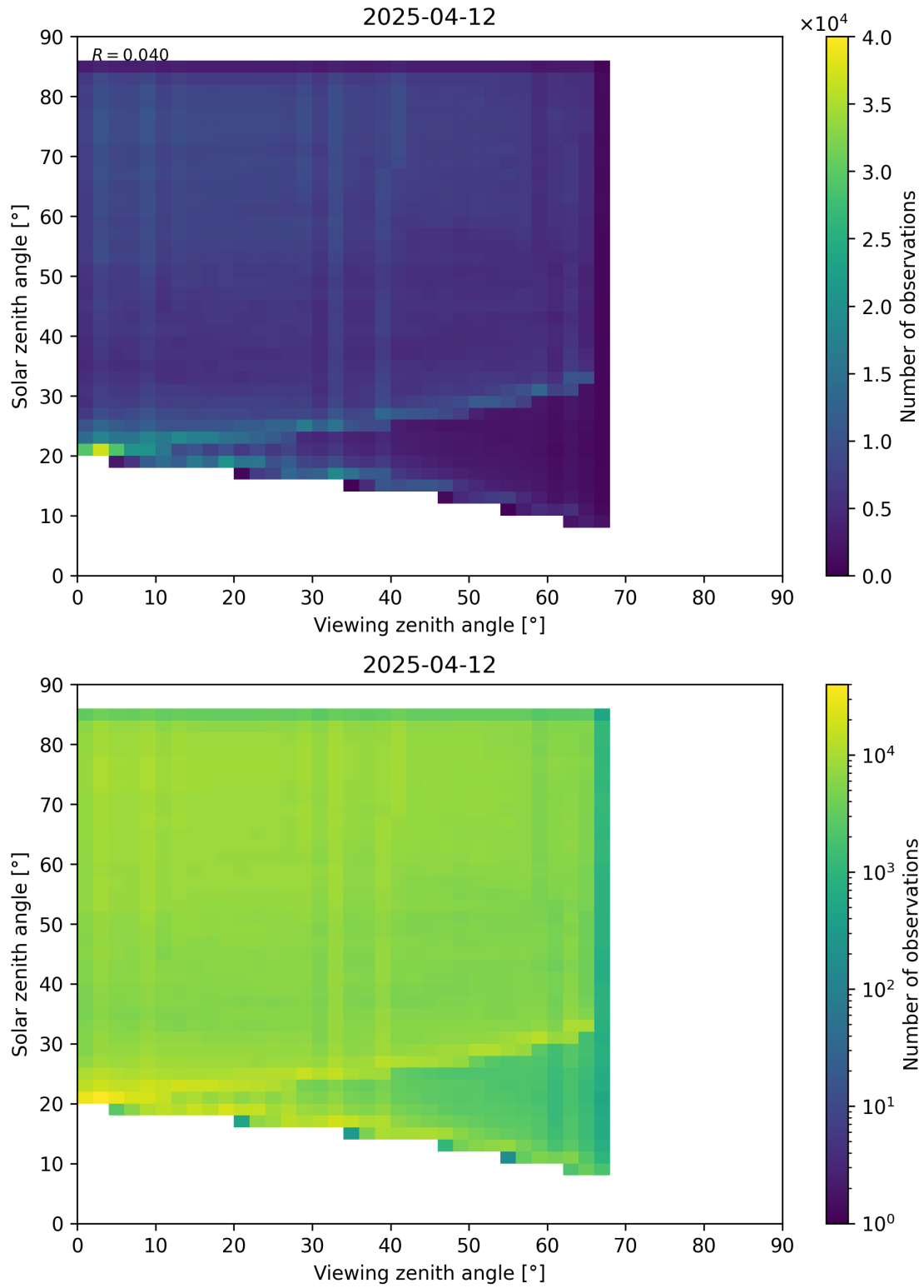
Figure 77: Scatter density plot of “Viewing zenith angle” against “Solar zenith angle” for 2025-04-11 to 2025-04-13.
