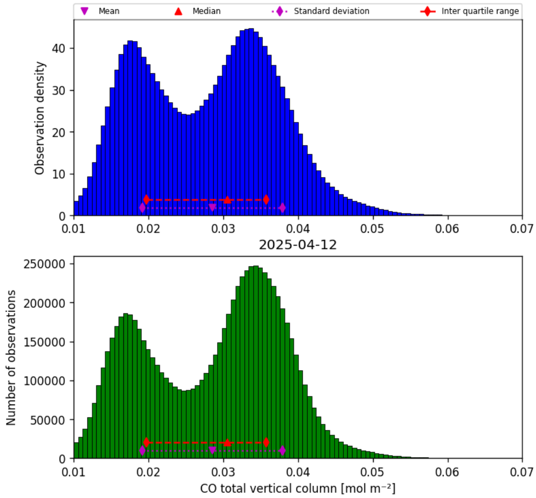
Figure 18: Histogram of “CO total vertical column” for 2025-04-11 to 2025-04-13
