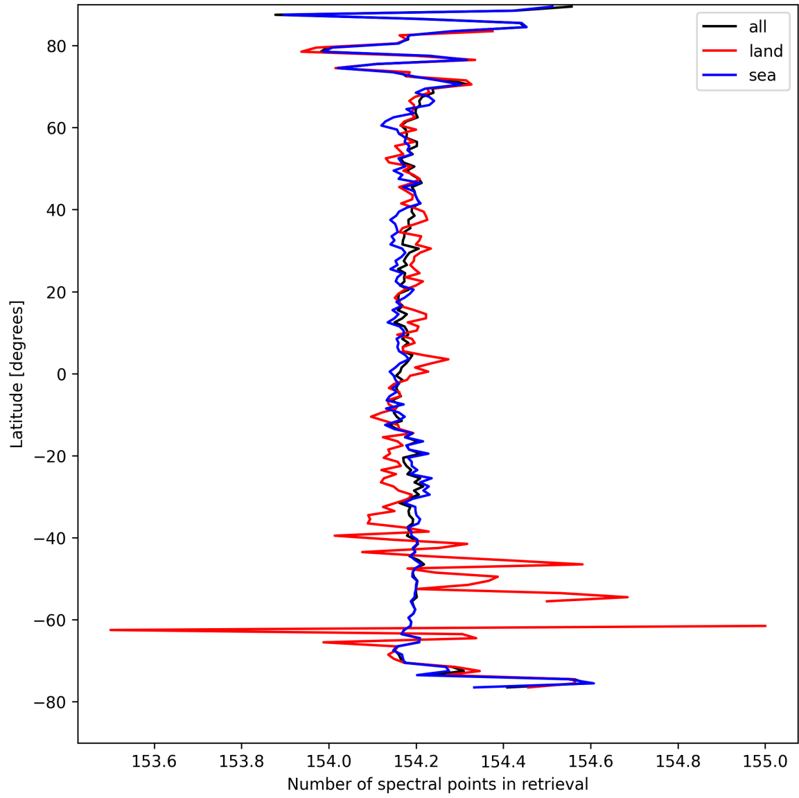
Figure 13: Zonal average of “Number of spectral points in retrieval” for 2025-04-11 to 2025-04-13.
