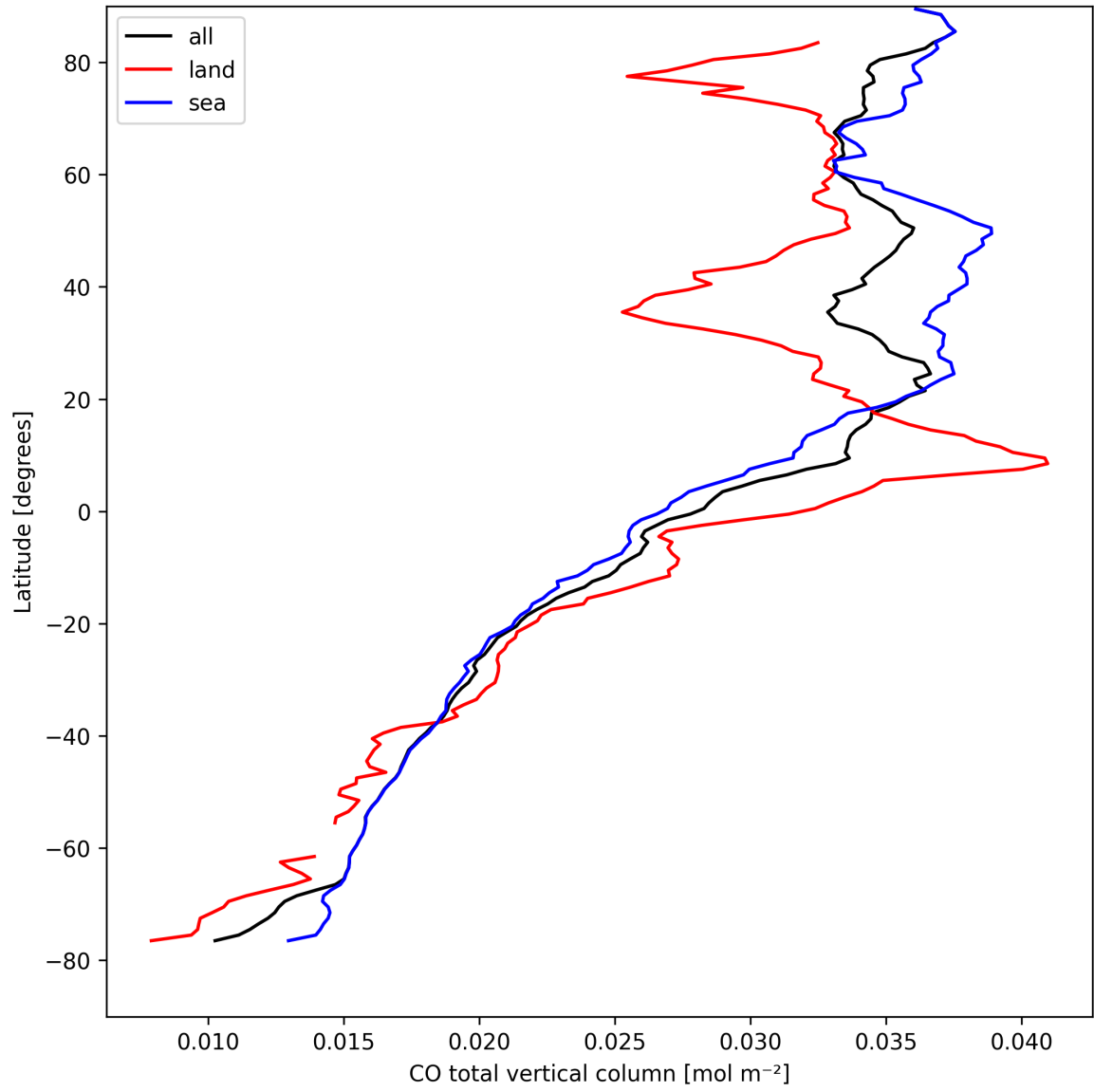
Figure 10: Zonal average of “CO total vertical column” for 2025-04-11 to 2025-04-13.
