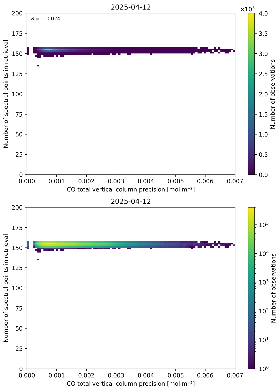
Figure 47: Scatter density plot of “CO total vertical column precision” against “Number of spectral points in retrieval” for 2025-04-11 to 2025-04-13.
