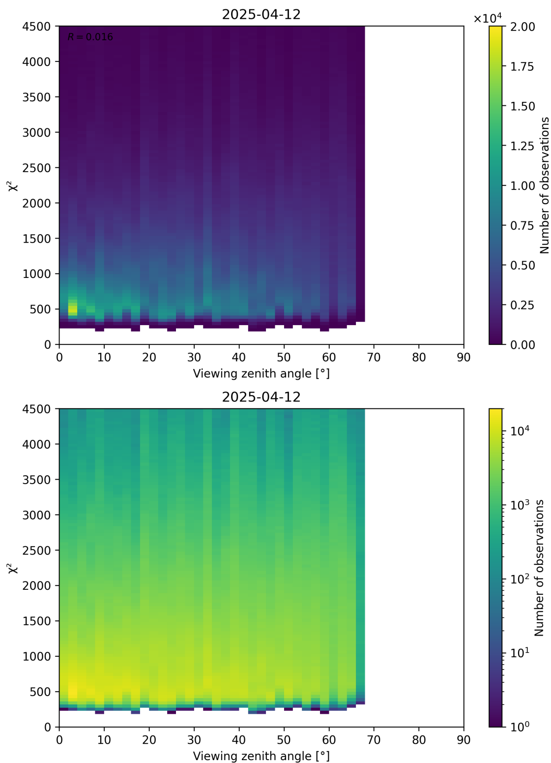
Figure 72: Scatter density plot of “Viewing zenith angle” against “ \chi^2 ” for 2025-04-11 to 2025-04-13.
