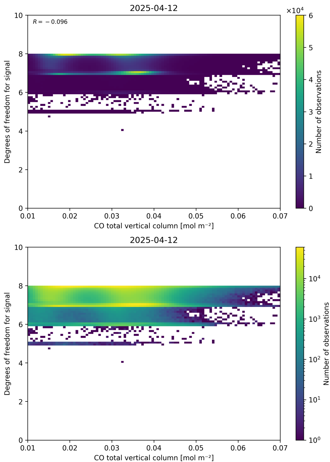
Figure 41: Scatter density plot of “CO total vertical column” against “Degrees of freedom for signal” for 2025-04-11 to 2025-04-13.
