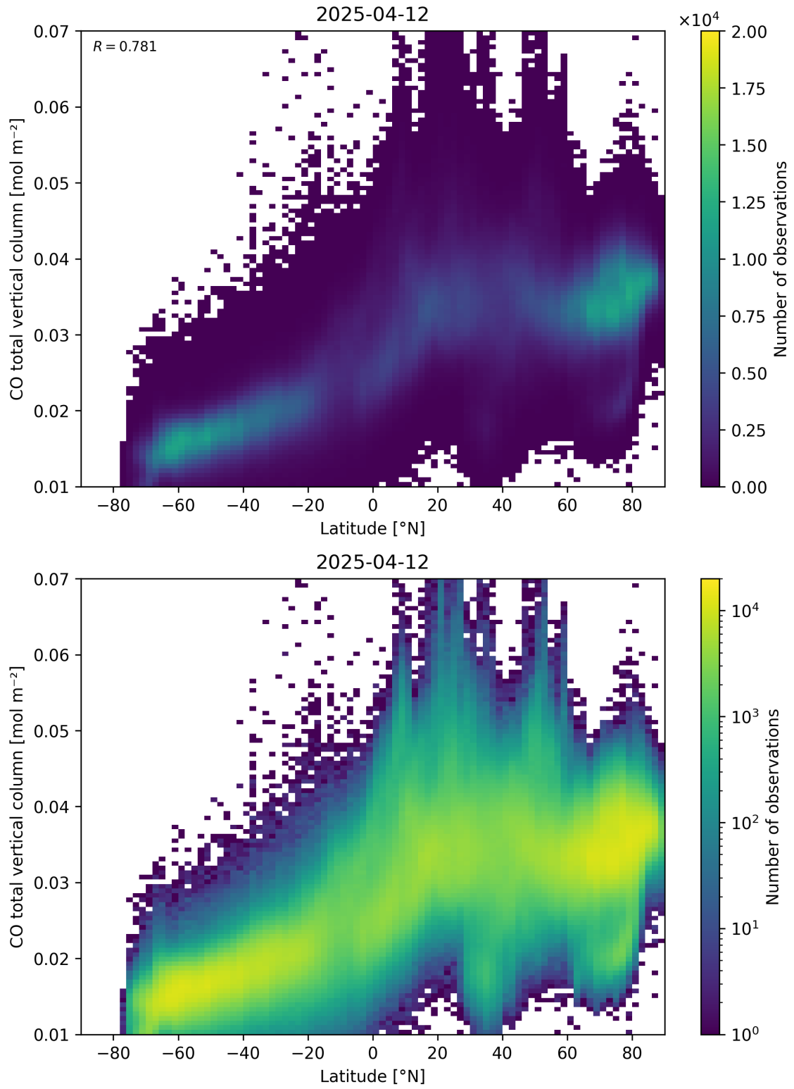
Figure 51: Scatter density plot of “Latitude” against “CO total vertical column” for 2025-04-11 to 2025-04-13.
