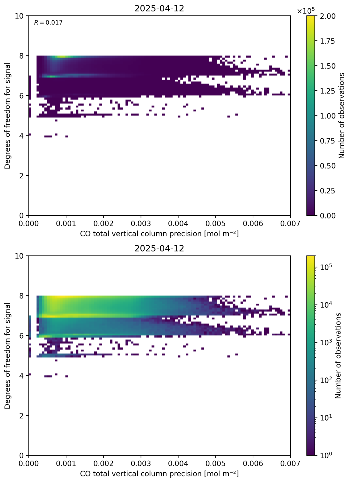
Figure 45: Scatter density plot of “CO total vertical column precision” against “Degrees of freedom for signal” for 2025-04-11 to 2025-04-13.
