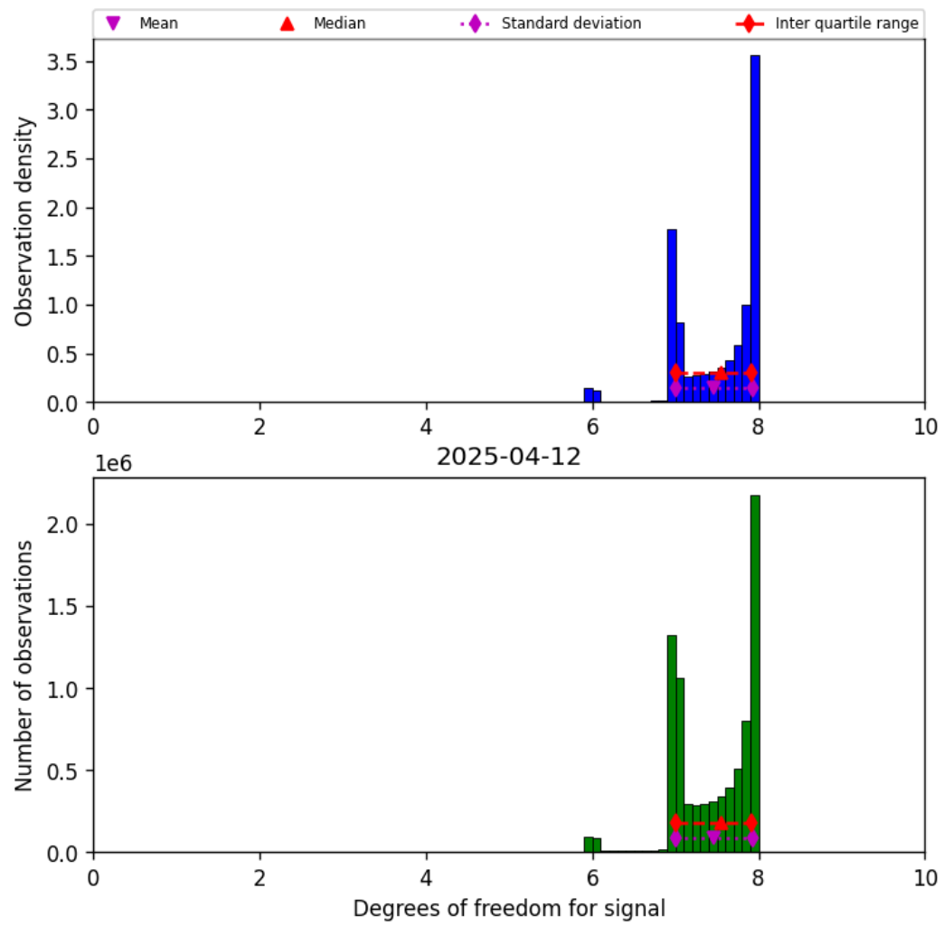
Figure 23: Histogram of “Degrees of freedom for signal” for 2025-04-11 to 2025-04-13
