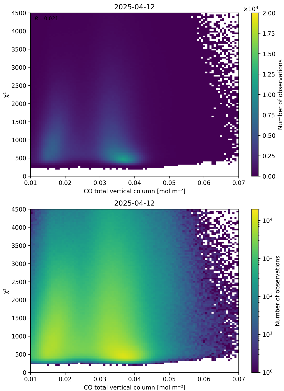
Figure 35: Scatter density plot of “CO total vertical column” against “ \chi^2 ” for 2025-04-11 to 2025-04-13.
