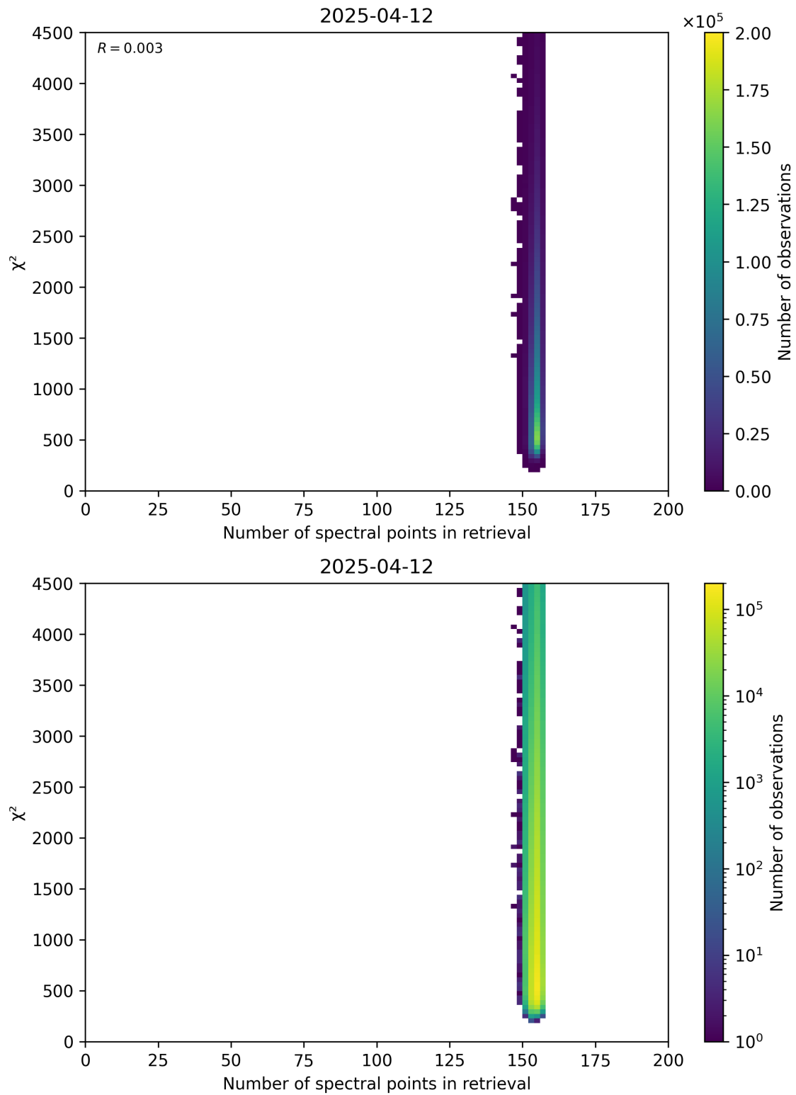
Figure 58: Scatter density plot of “Number of spectral points in retrieval” against “ \chi^2 ” for 2025-04-11 to 2025-04-13.
