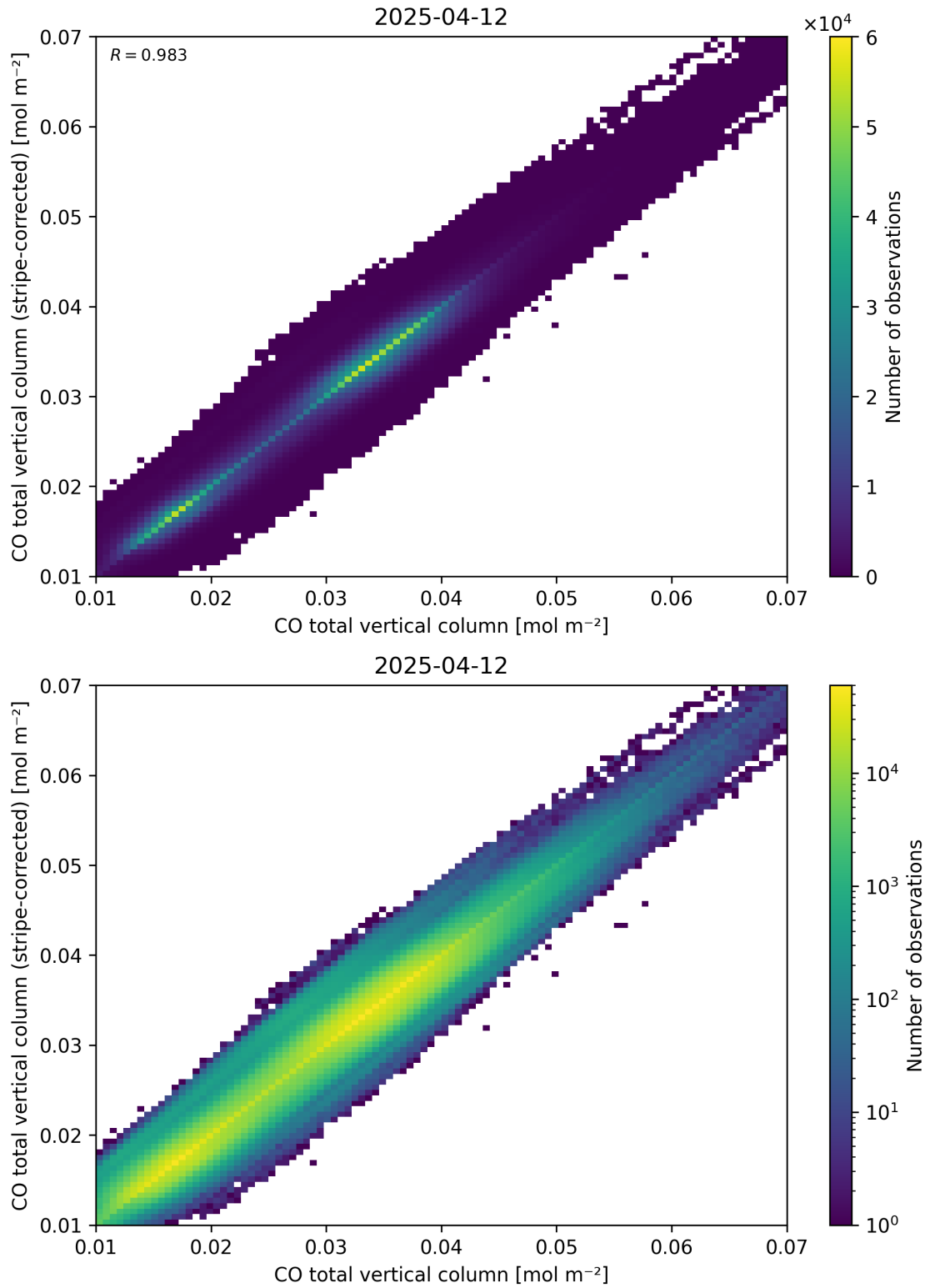
Figure 33: Scatter density plot of “CO total vertical column” against “CO total vertical column (stripe-corrected)” for 2025-04-11 to 2025-04-13.
