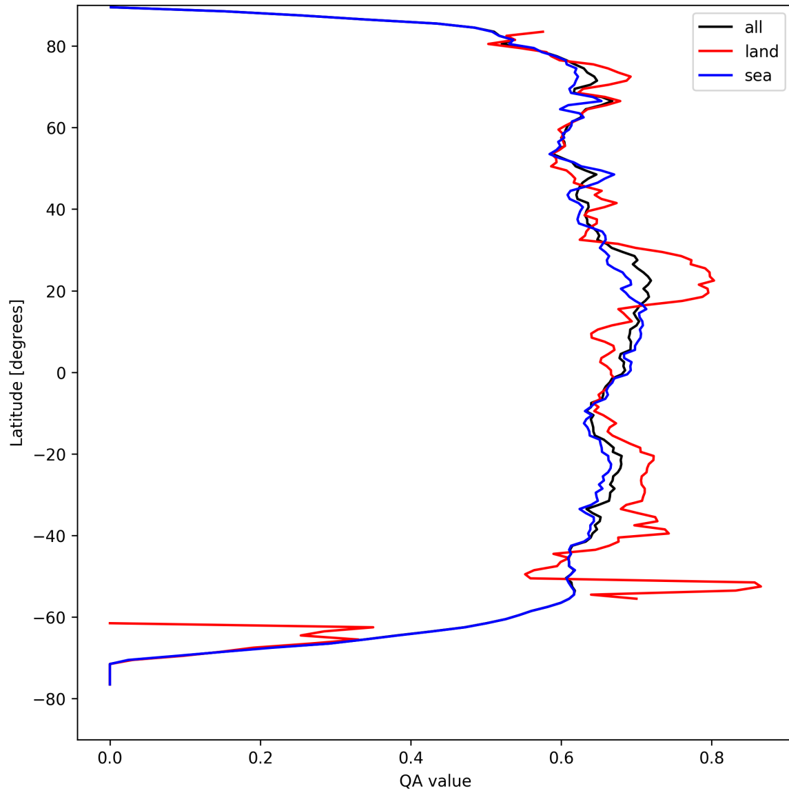
Figure 9: Zonal average of “QA value” for 2025-04-11 to 2025-04-13.
