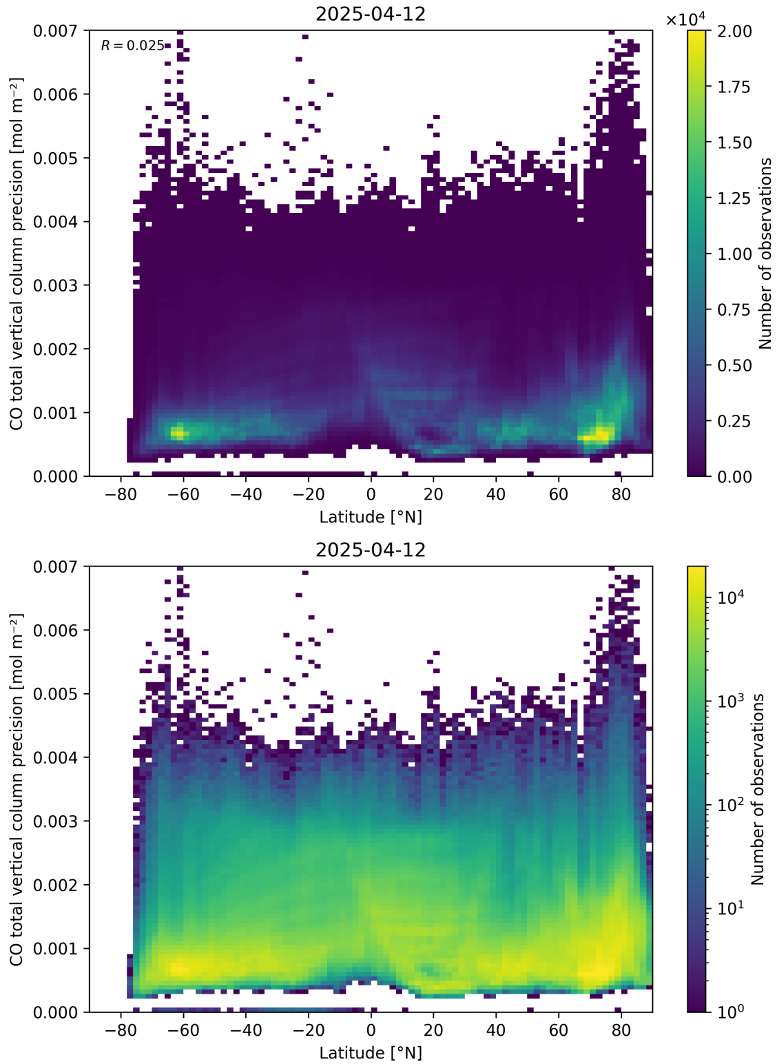
Figure 53: Scatter density plot of “Latitude” against “CO total vertical column precision” for 2025-04-11 to 2025-04-13.
