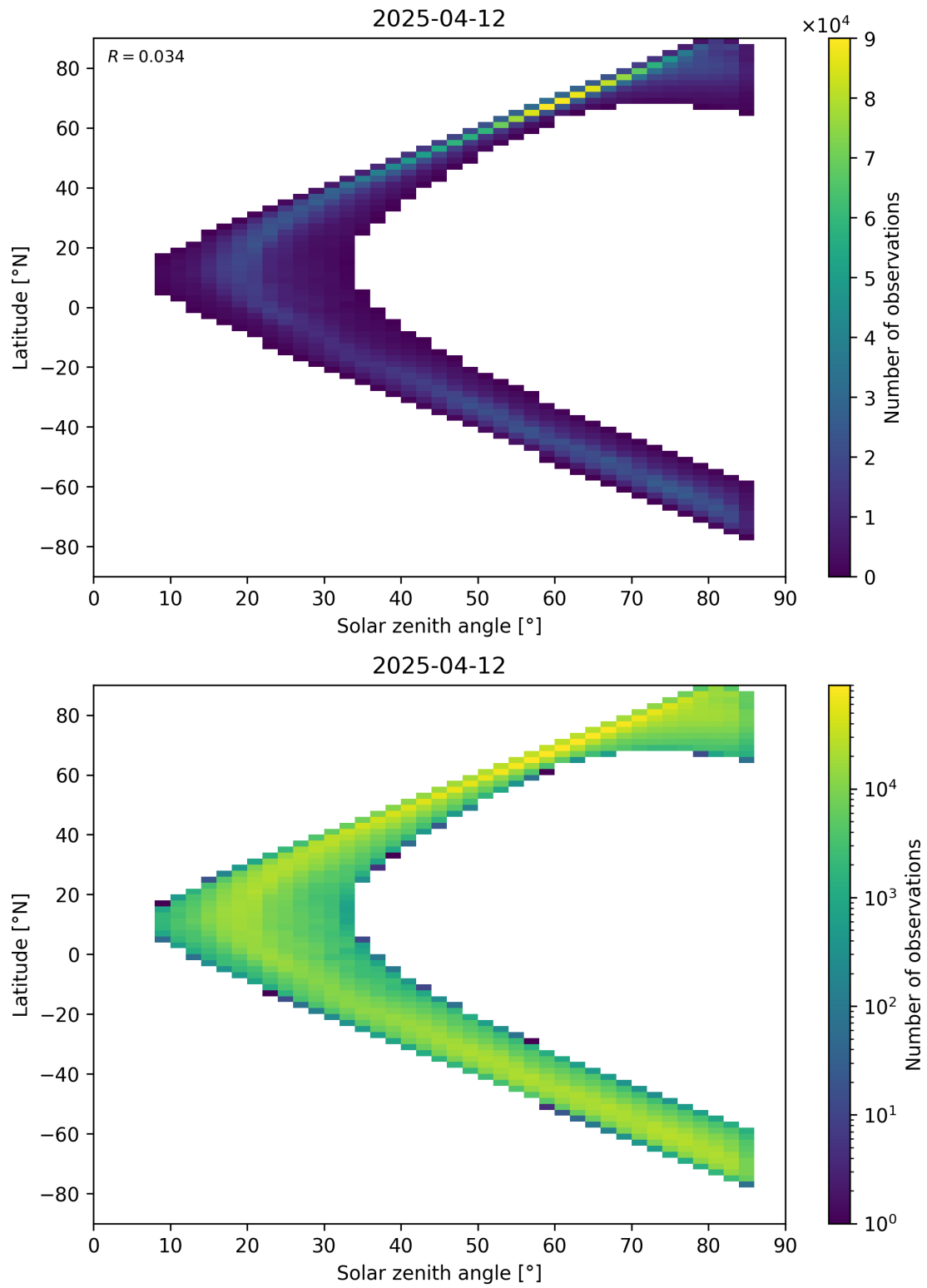
Figure 66: Scatter density plot of “Solar zenith angle” against “Latitude” for 2025-04-11 to 2025-04-13.
