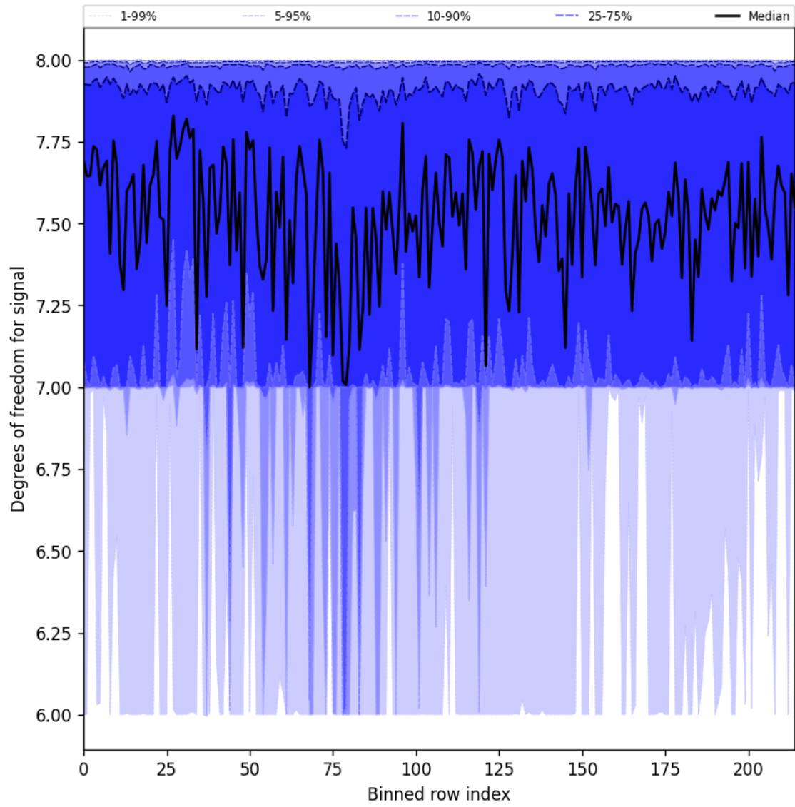
Figure 31: Along track statistics of “Degrees of freedom for signal” for 2025-04-11 to 2025-04-13
