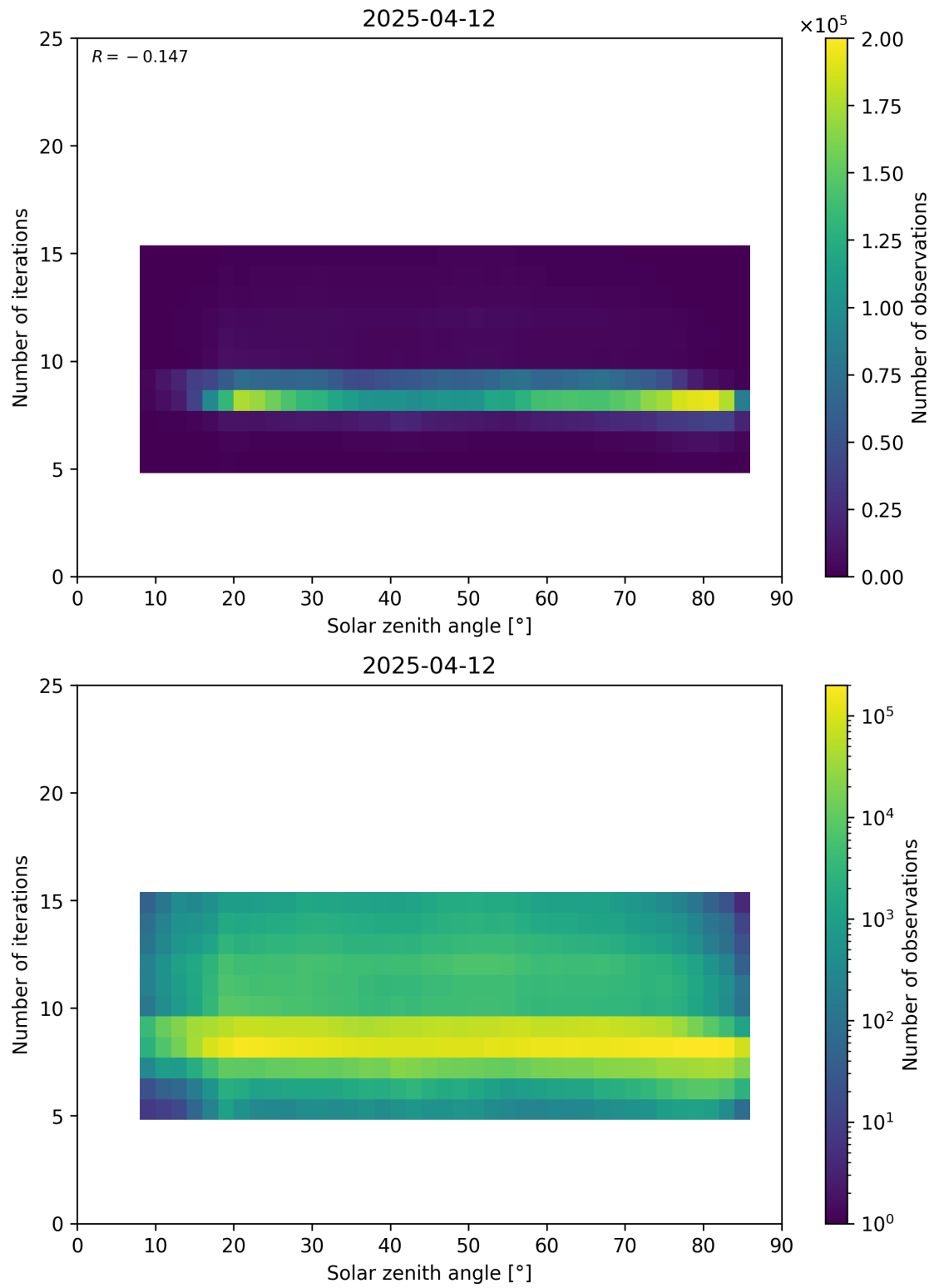
Figure 67: Scatter density plot of “Solar zenith angle” against “Number of iterations” for 2025-04-11 to 2025-04-13.
