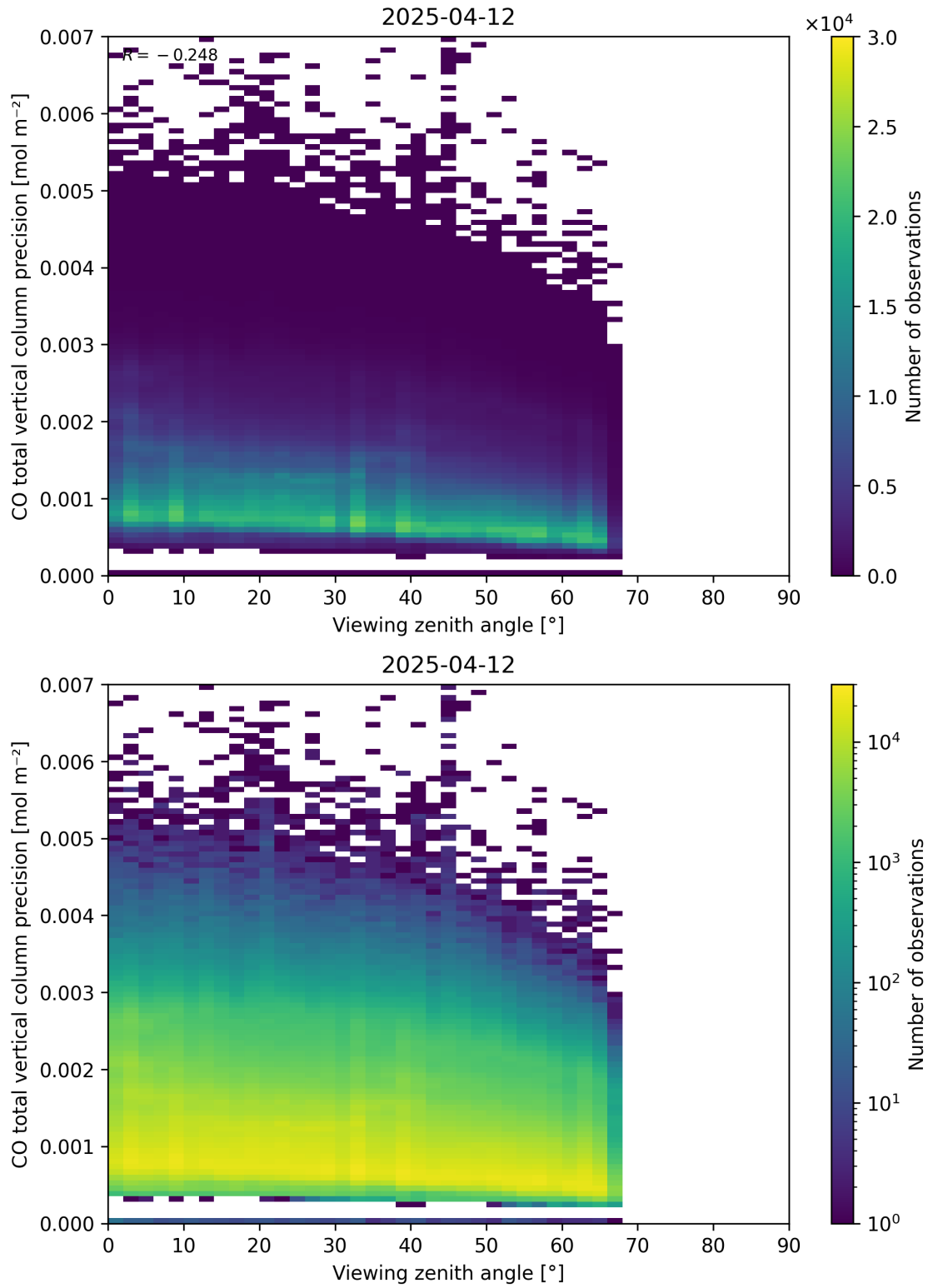
Figure 71: Scatter density plot of “Viewing zenith angle” against “CO total vertical column precision” for 2025-04-11 to 2025-04-13.
