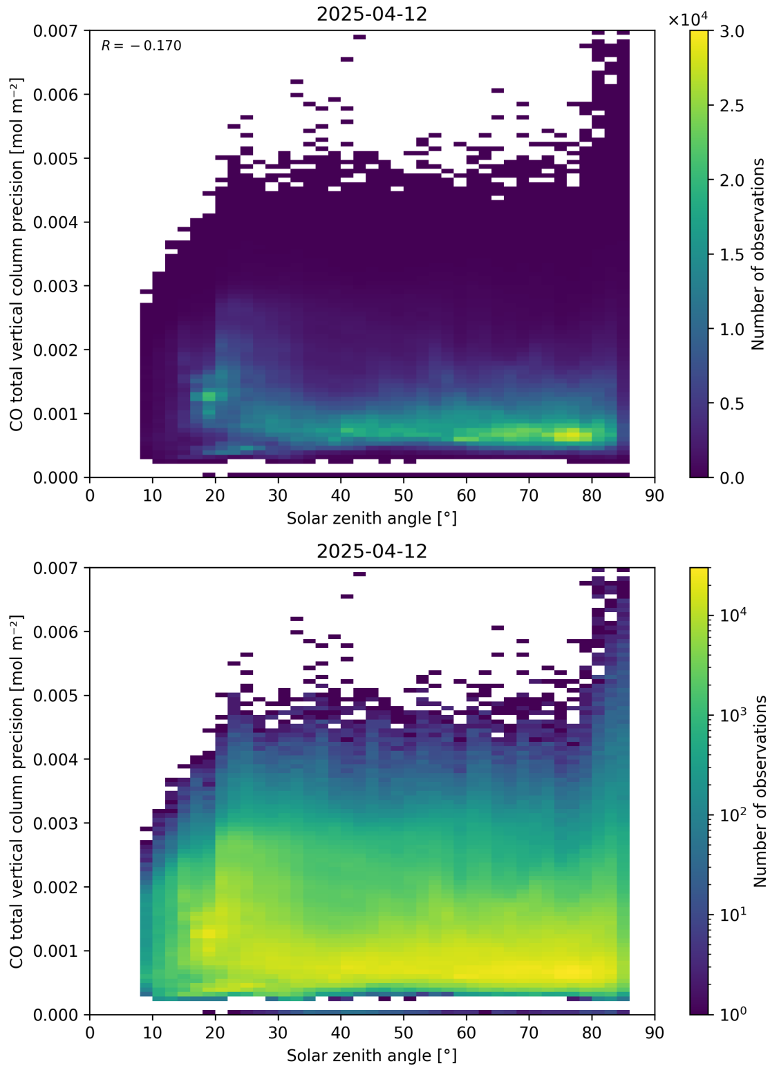
Figure 63: Scatter density plot of “Solar zenith angle” against “CO total vertical column precision” for 2025-04-11 to 2025-04-13.
