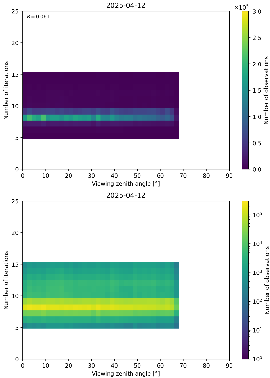
Figure 75: Scatter density plot of “Viewing zenith angle” against “Number of iterations” for 2025-04-11 to 2025-04-13.
