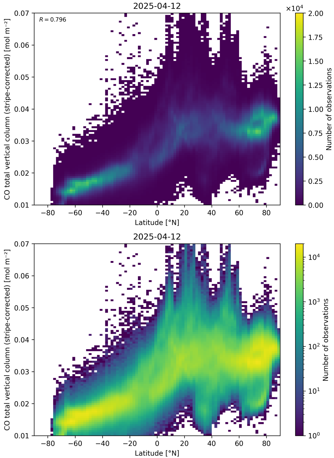
Figure 52: Scatter density plot of “Latitude” against “CO total vertical column (stripe-corrected)” for 2025-04-11 to 2025-04-13.
