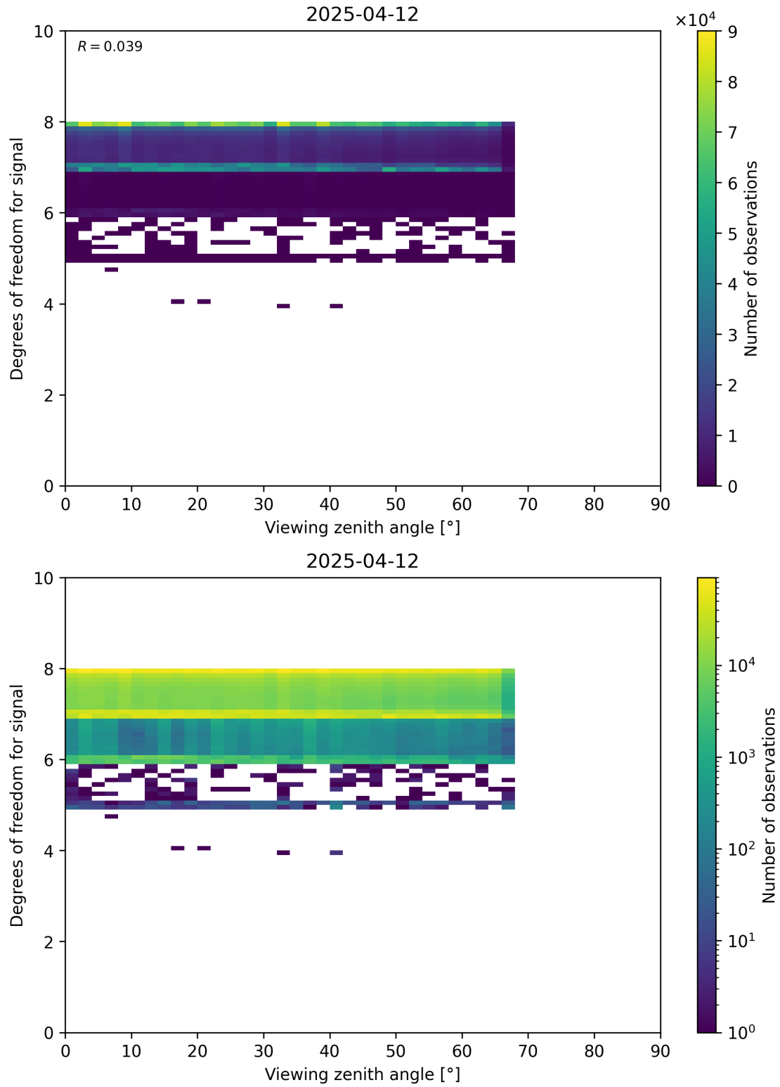
Figure 73: Scatter density plot of “Viewing zenith angle” against “Degrees of freedom for signal” for 2025-04-11 to 2025-04-13.
