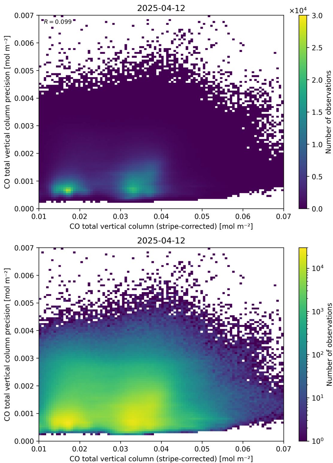
Figure 36: Scatter density plot of “CO total vertical column (stripe-corrected)” against “CO total vertical column precision” for 2025-04-11 to 2025-04-13.
