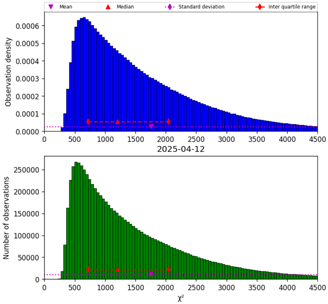
Figure 22: Histogram of “ \chi^2 ” for 2025-04-11 to 2025-04-13
