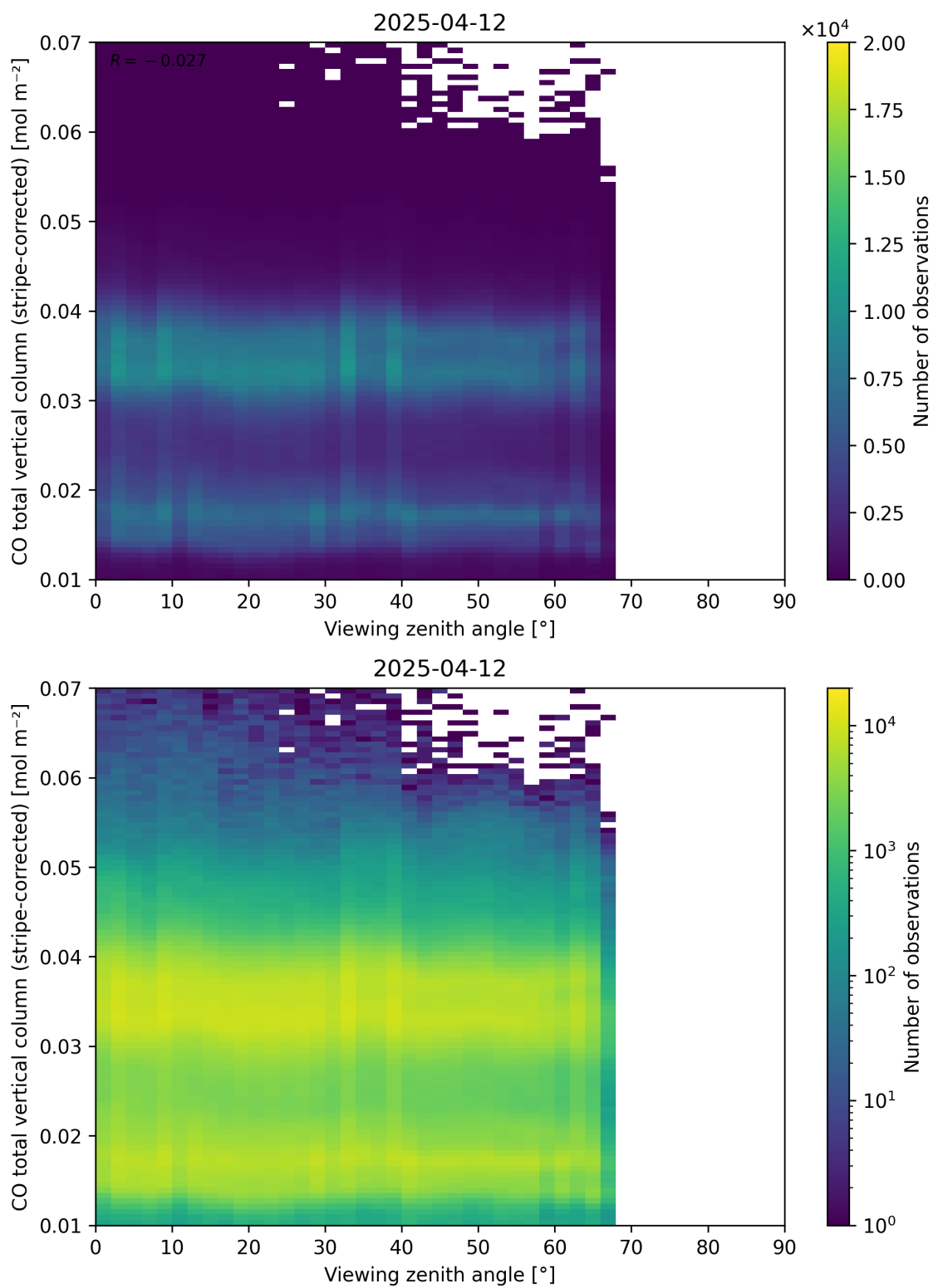
Figure 70: Scatter density plot of “Viewing zenith angle” against “CO total vertical column (stripe-corrected)” for 2025-04-11 to 2025-04-13.
