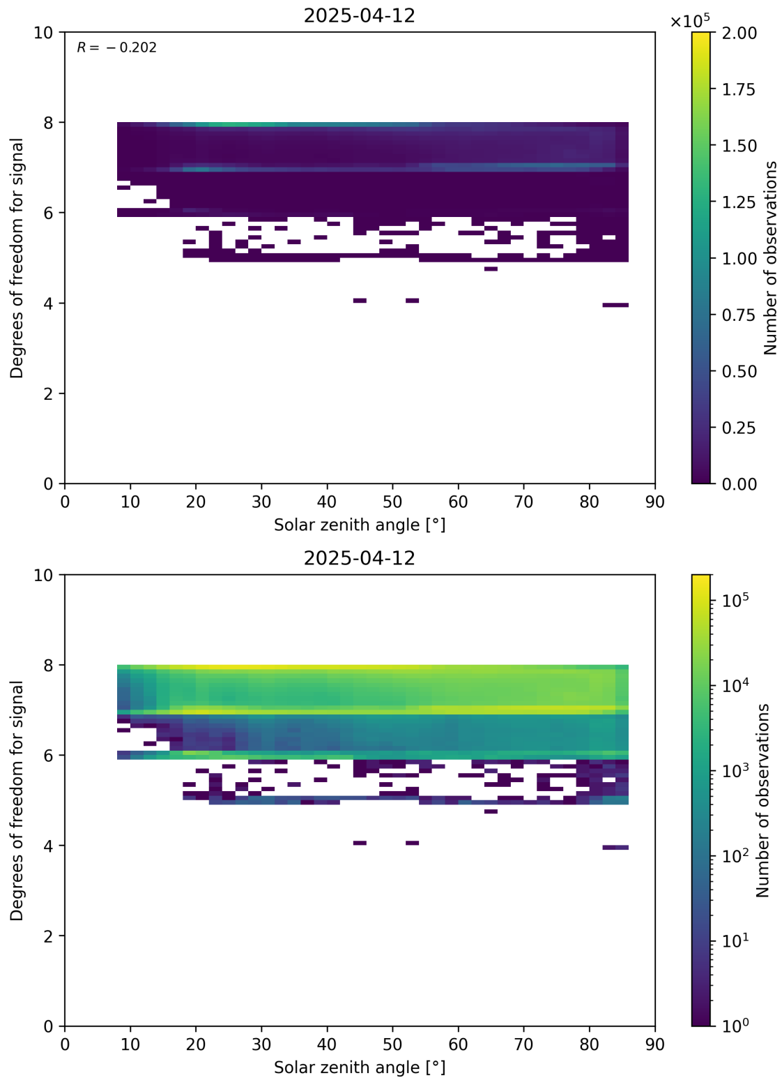
Figure 65: Scatter density plot of “Solar zenith angle” against “Degrees of freedom for signal” for 2025-04-11 to 2025-04-13.
