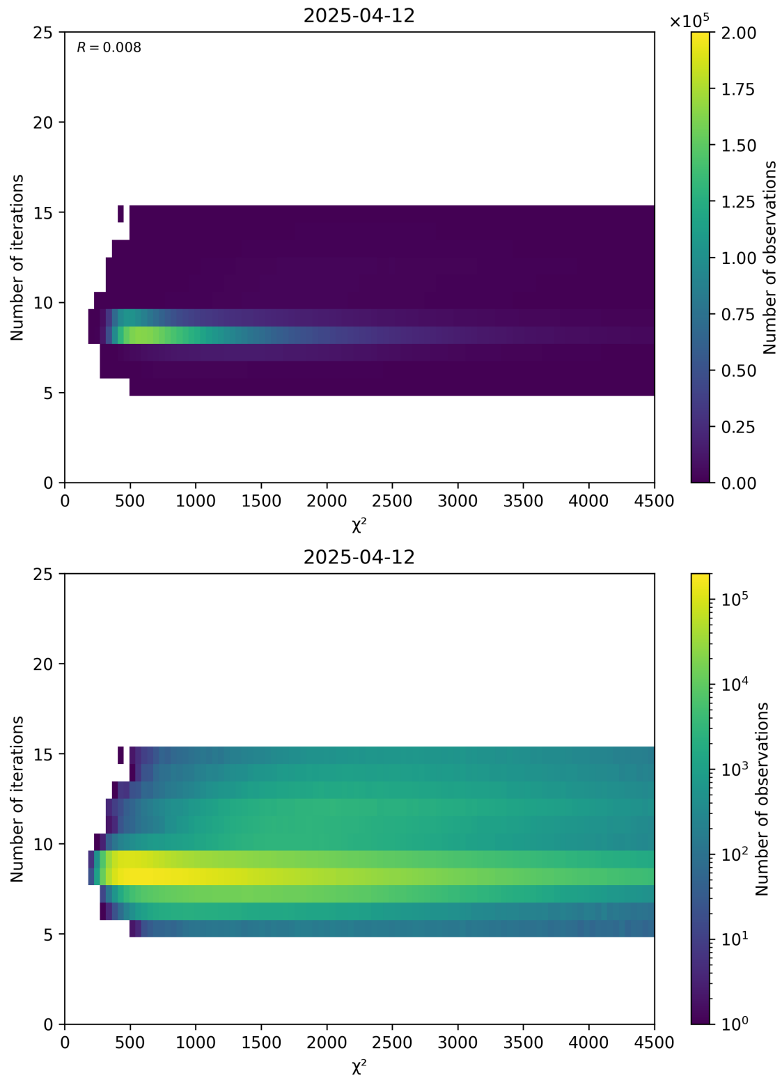
Figure 49: Scatter density plot of “ \chi^2 ” against “Number of iterations” for 2025-04-11 to 2025-04-13.
