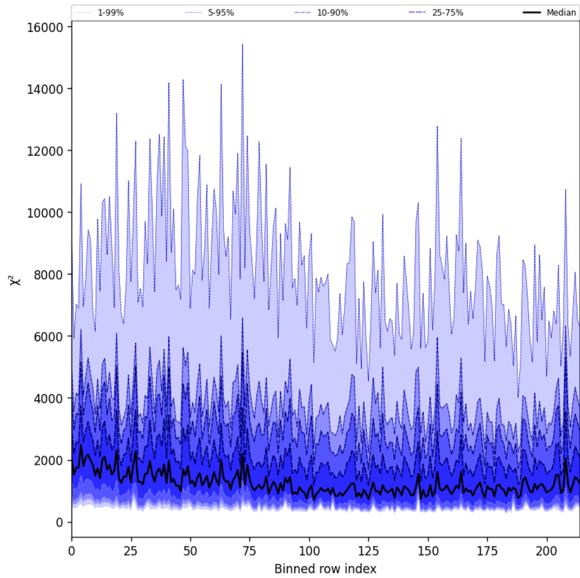
Figure 30: Along track statistics of “ \chi^2 ” for 2025-04-11 to 2025-04-13
