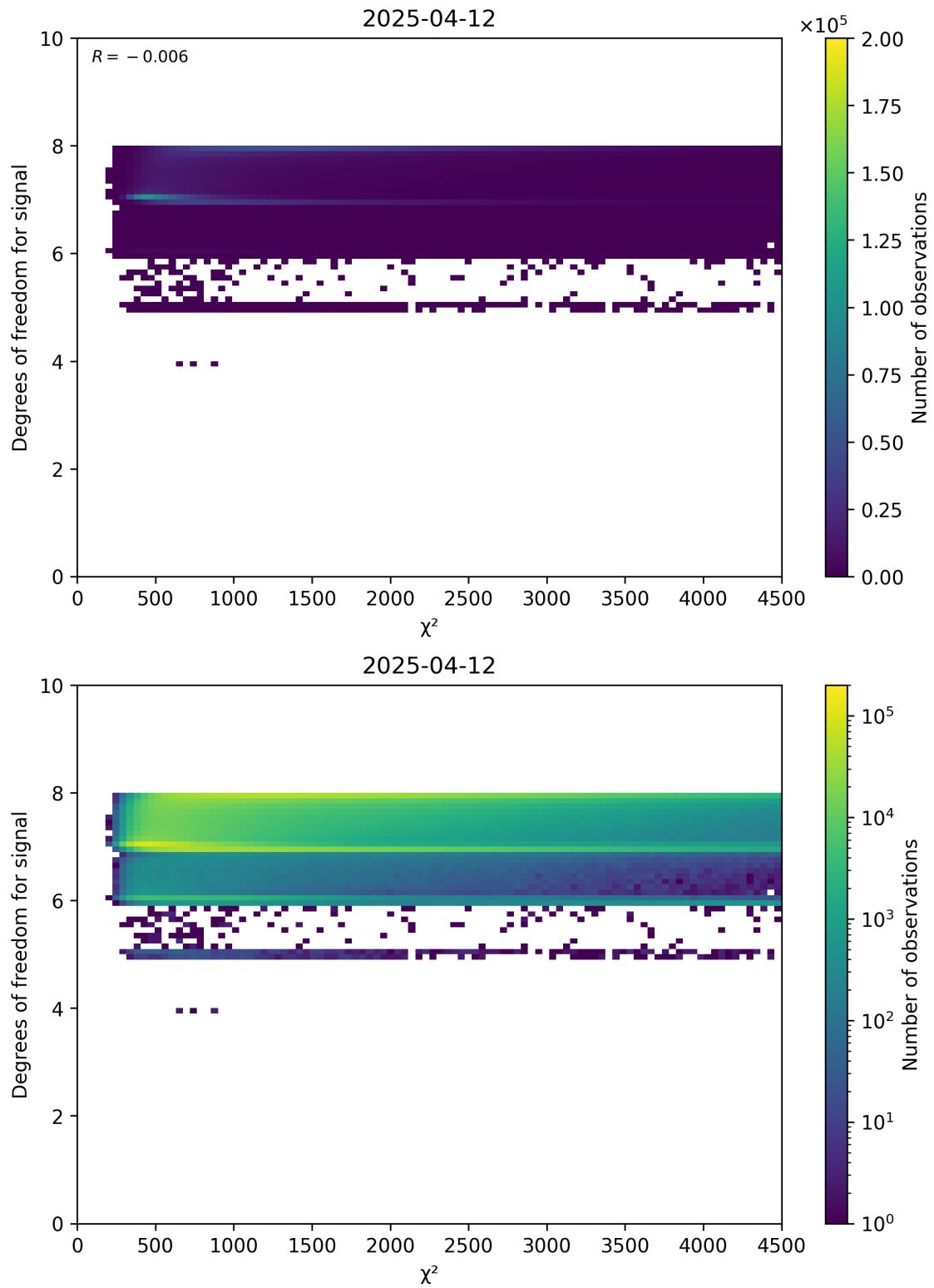
Figure 48: Scatter density plot of “ \chi^2 ” against “Degrees of freedom for signal” for 2025-04-11 to 2025-04-13.
