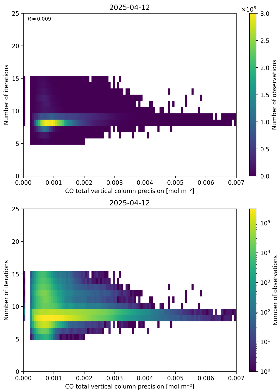
Figure 46: Scatter density plot of “CO total vertical column precision” against “Number of iterations” for 2025-04-11 to 2025-04-13.
