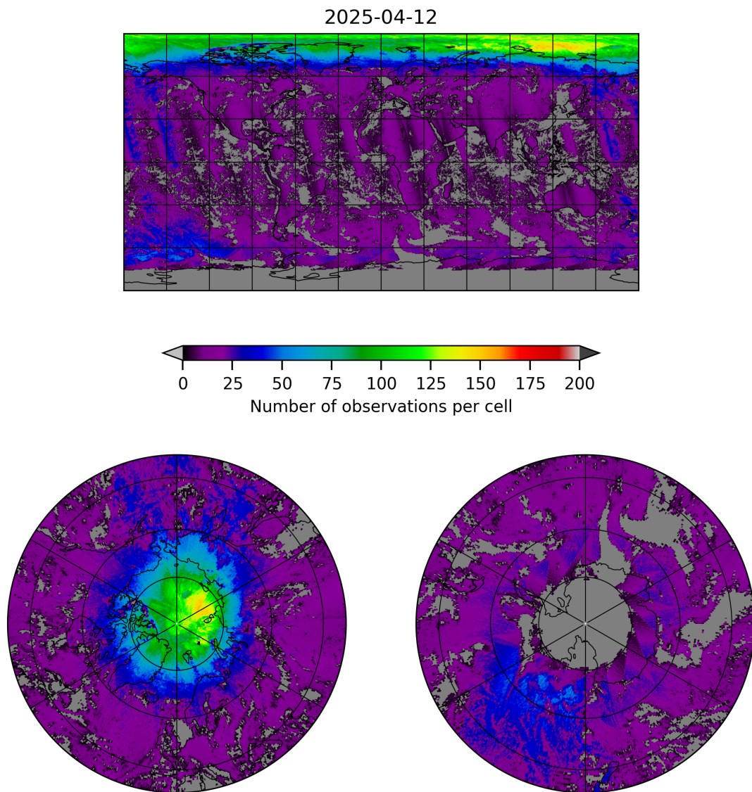
Figure 8: Map of the number of observations for 2025-04-11 to 2025-04-13
