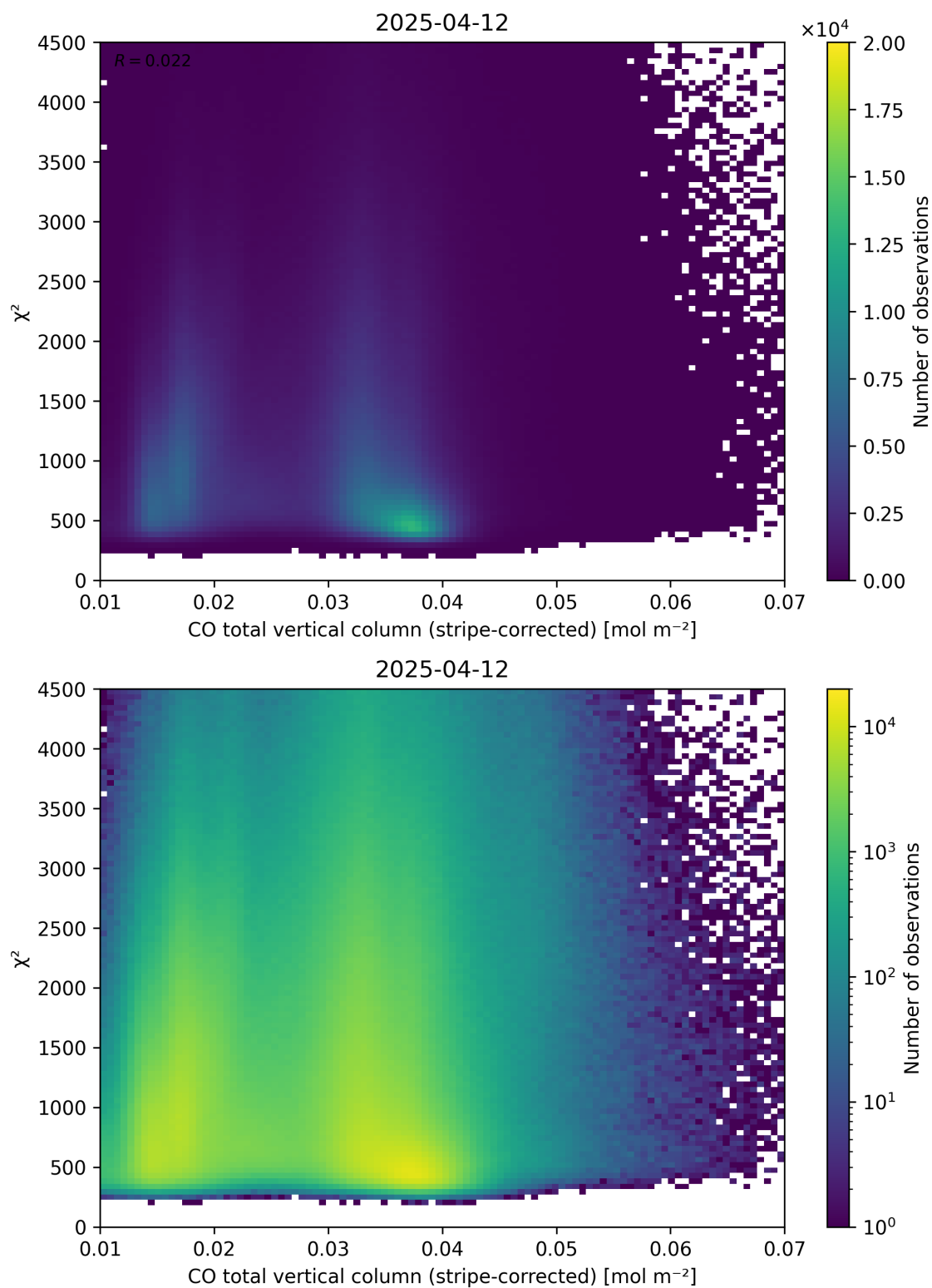
Figure 37: Scatter density plot of “CO total vertical column (stripe-corrected)” against “ \chi^2 ” for 2025-04-11 to 2025-04-13.
