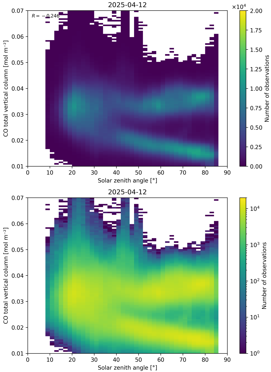
Figure 61: Scatter density plot of “Solar zenith angle” against “CO total vertical column” for 2025-04-11 to 2025-04-13.
