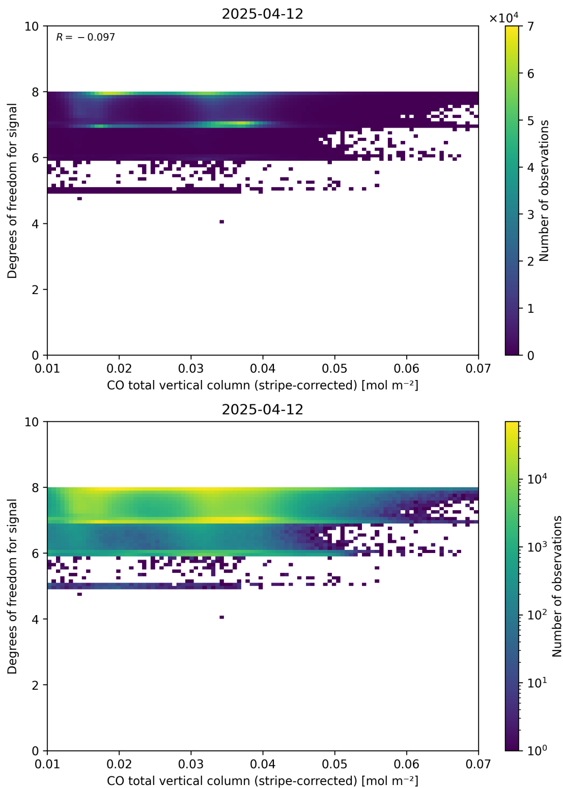
Figure 38: Scatter density plot of “CO total vertical column (stripe-corrected)” against “Degrees of freedom for signal” for 2025-04-11 to 2025-04-13.
