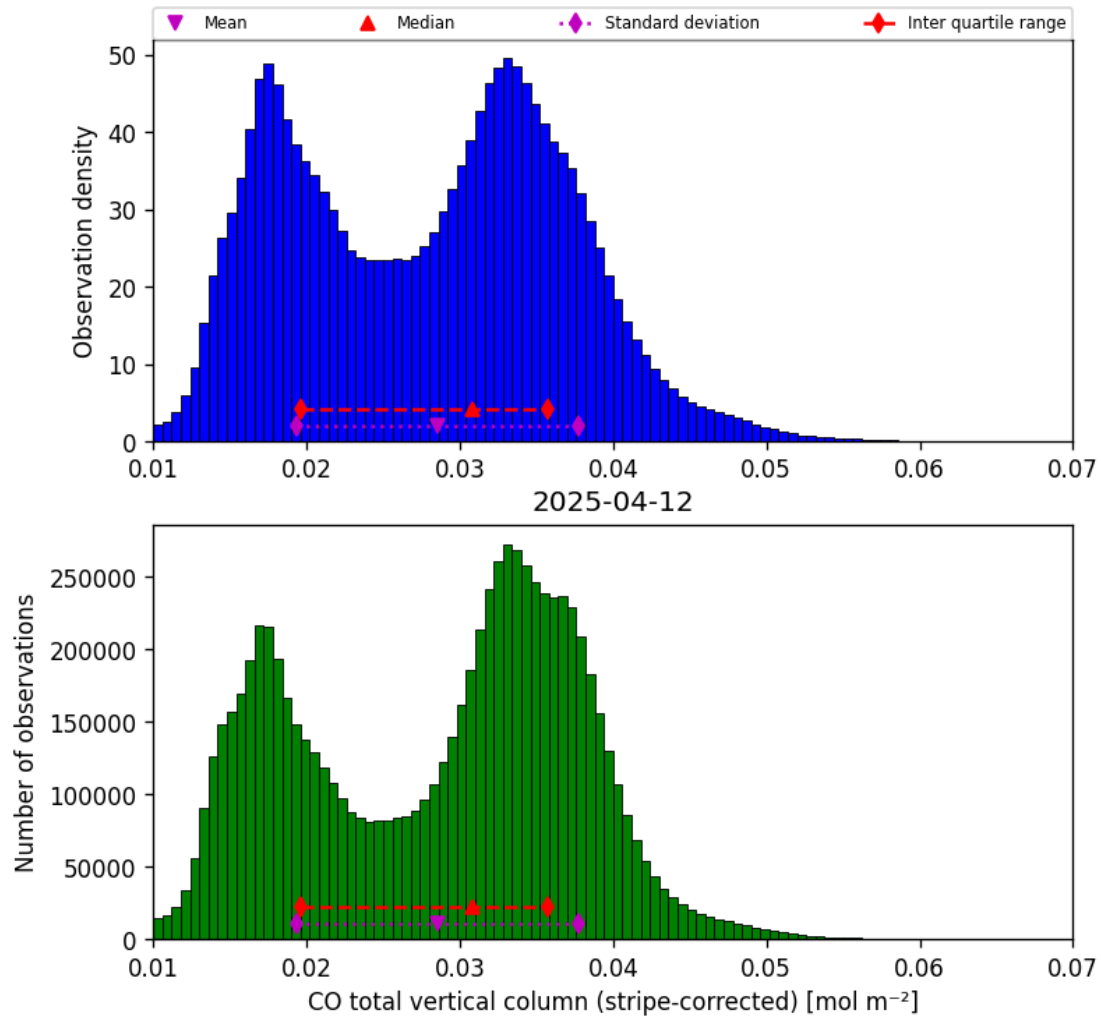
Figure 19: Histogram of “CO total vertical column (stripe-corrected)” for 2025-04-11 to 2025-04-13
