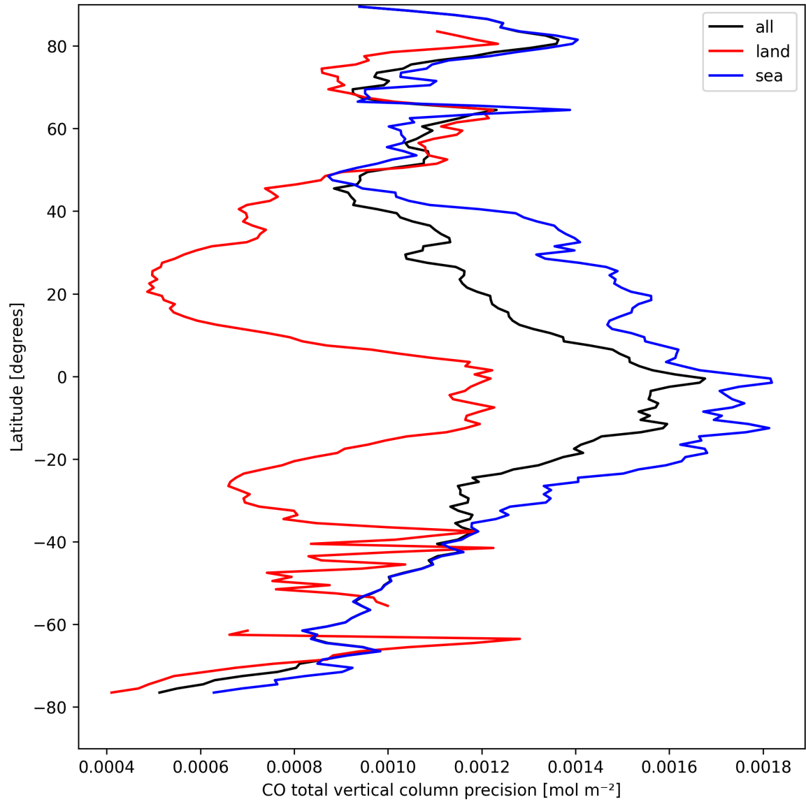
Figure 12: Zonal average of “CO total vertical column precision” for 2025-04-11 to 2025-04-13.
