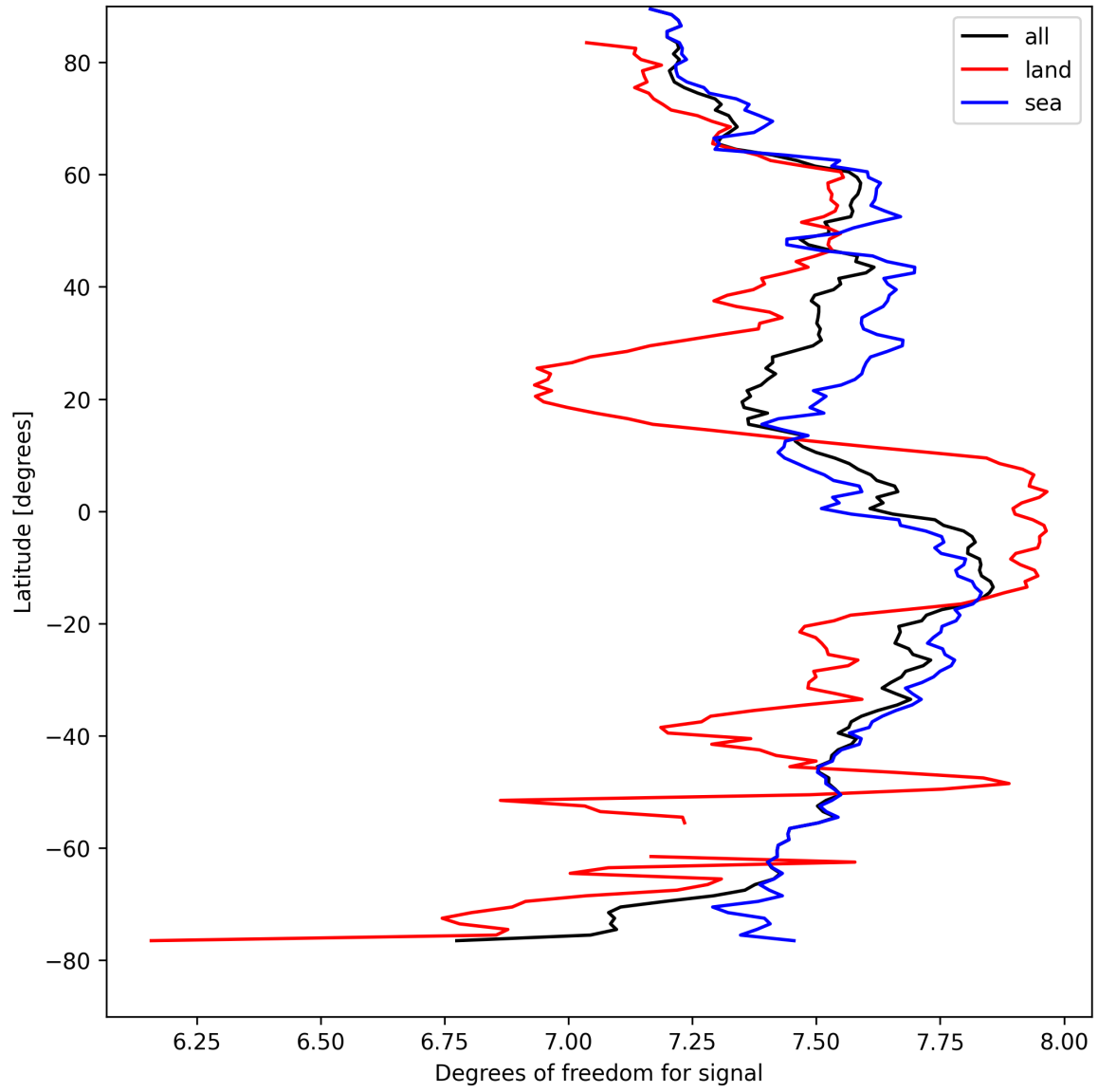
Figure 15: Zonal average of “Degrees of freedom for signal” for 2025-04-11 to 2025-04-13.
