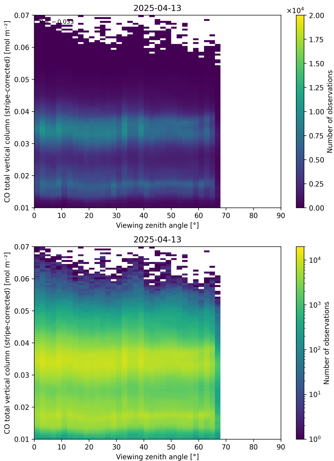
Figure 70: Scatter density plot of “Viewing zenith angle” against “CO total vertical column (stripe-corrected)” for 2025-04-13 to 2025-04-14.
