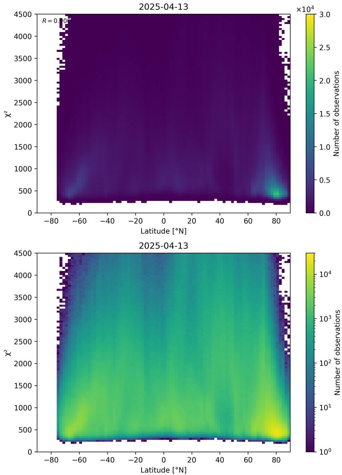
Figure 54: Scatter density plot of “Latitude” against “ \chi^2 ” for 2025-04-13 to 2025-04-14.
