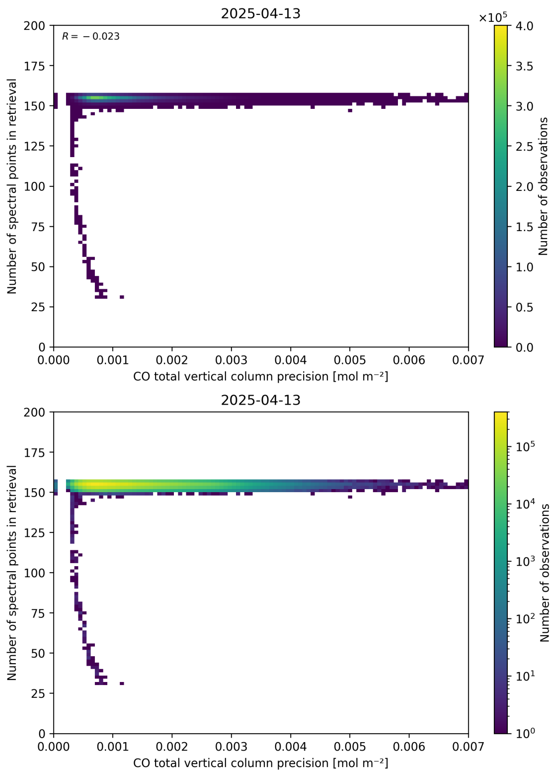
Figure 47: Scatter density plot of “CO total vertical column precision” against “Number of spectral points in retrieval” for 2025-04-13 to 2025-04-14.
