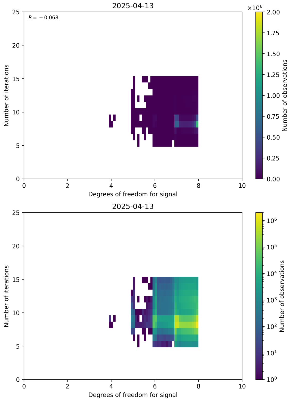
Figure 50: Scatter density plot of “Degrees of freedom for signal” against “Number of iterations” for 2025-04-13 to 2025-04-14.
