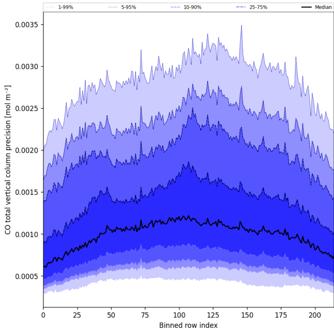
Figure 28: Along track statistics of “CO total vertical column precision” for 2025-04-13 to 2025-04-14
