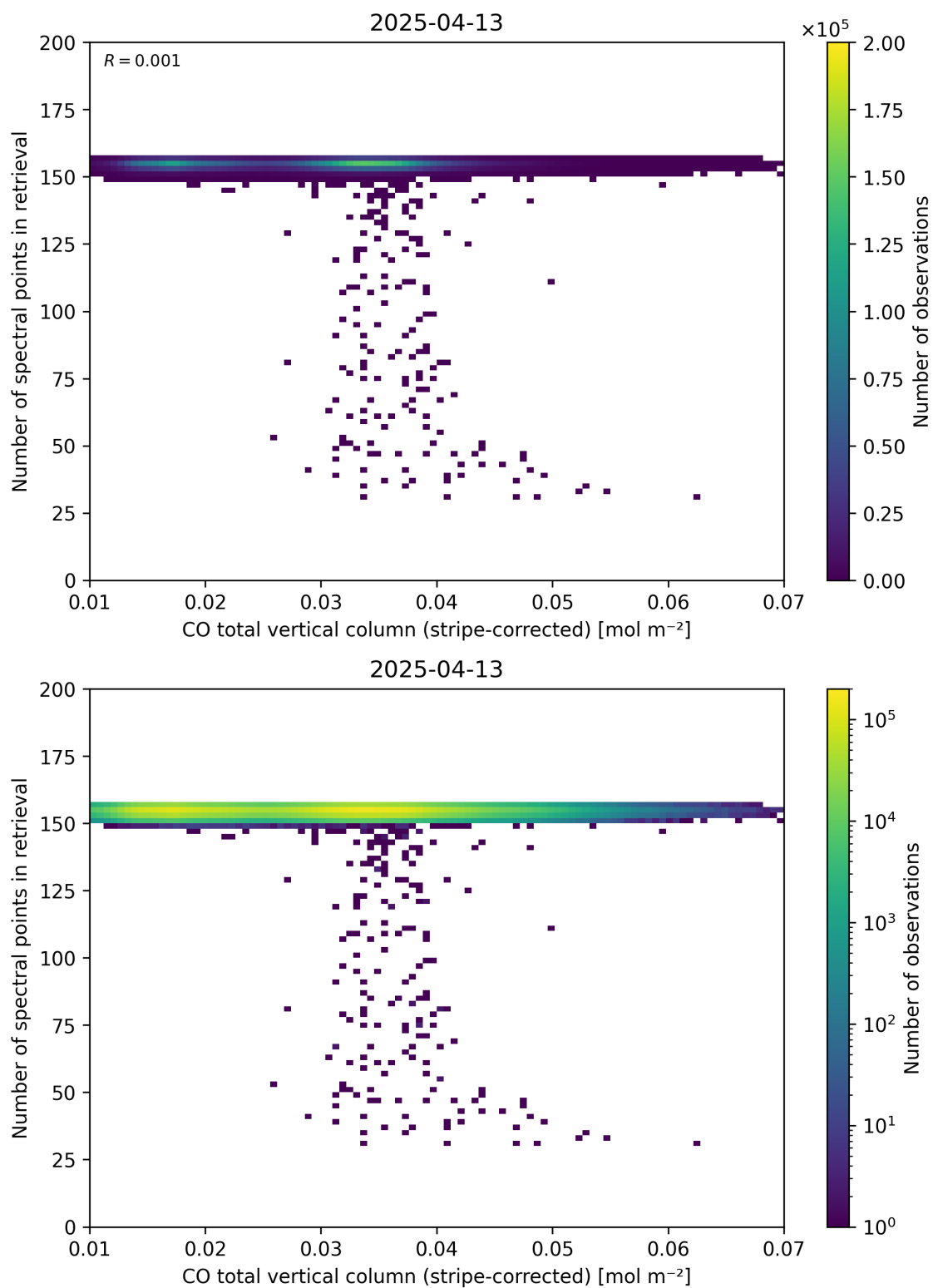
Figure 40: Scatter density plot of “CO total vertical column (stripe-corrected)” against “Number of spectral points in retrieval” for 2025-04-13 to 2025-04-14.
