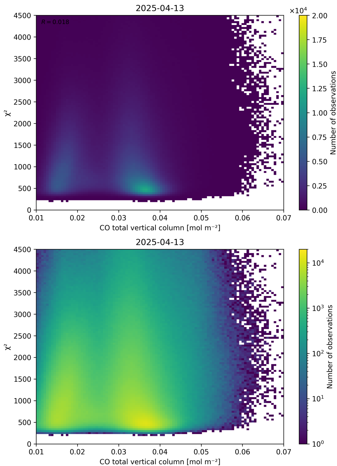
Figure 35: Scatter density plot of “CO total vertical column” against “ \chi^2 ” for 2025-04-13 to 2025-04-14.
