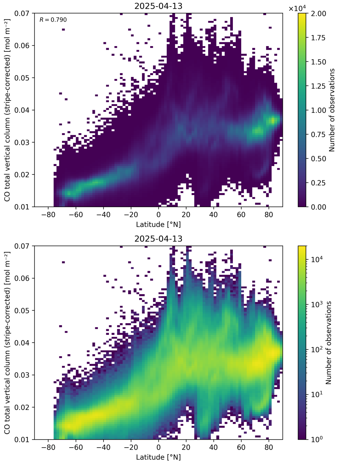
Figure 52: Scatter density plot of “Latitude” against “CO total vertical column (stripe-corrected)” for 2025-04-13 to 2025-04-14.
