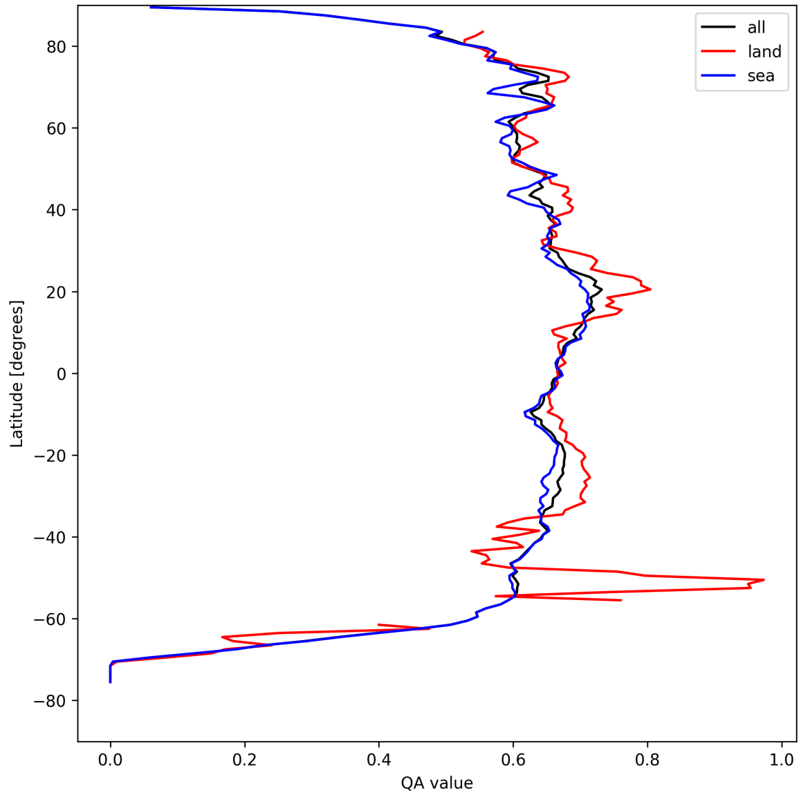
Figure 9: Zonal average of “QA value” for 2025-04-13 to 2025-04-14.
