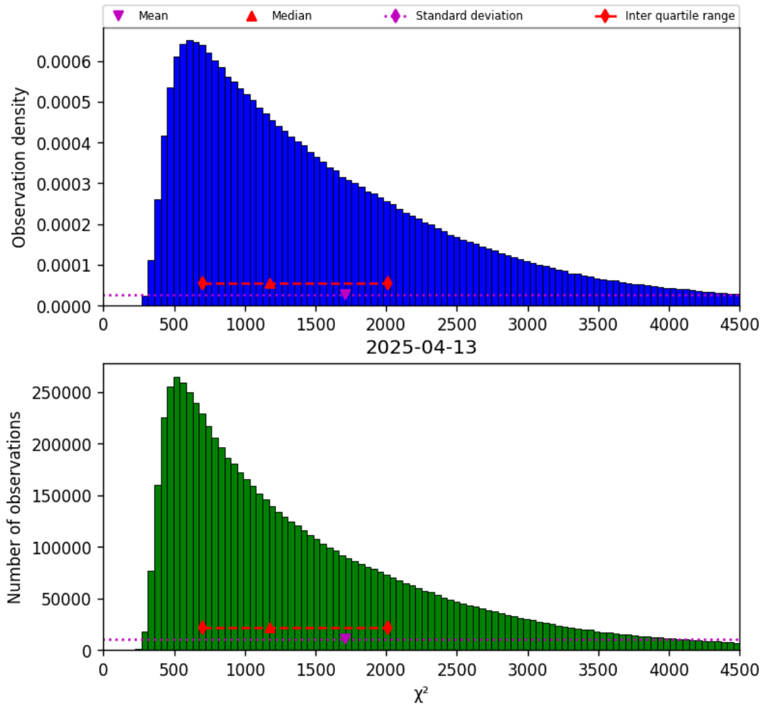
Figure 22: Histogram of “ \chi^2 ” for 2025-04-13 to 2025-04-14
