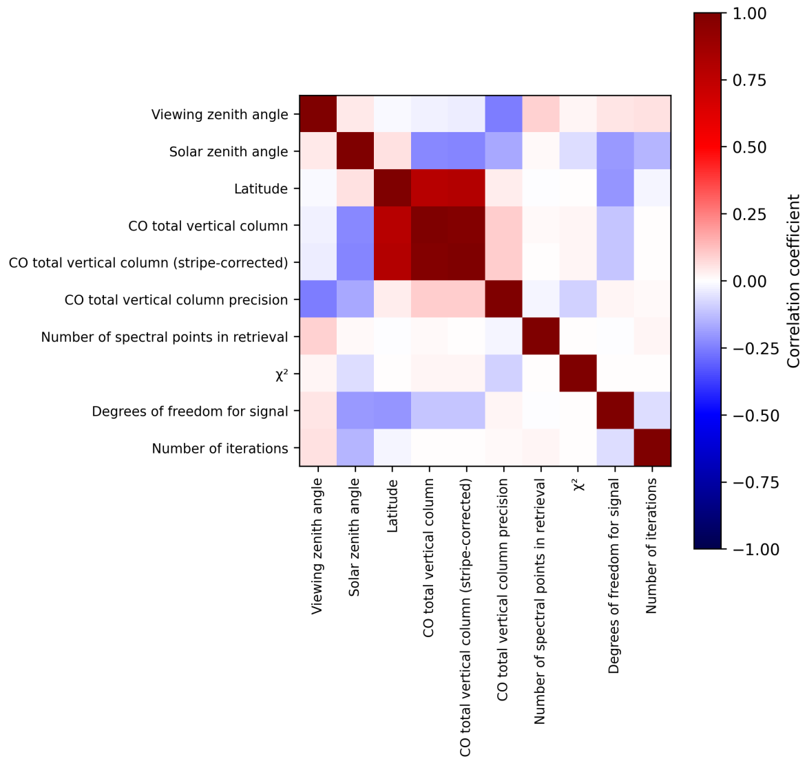
Figure 2: Map of correlation matrix for 2025-04-13 to 2025-04-14.
