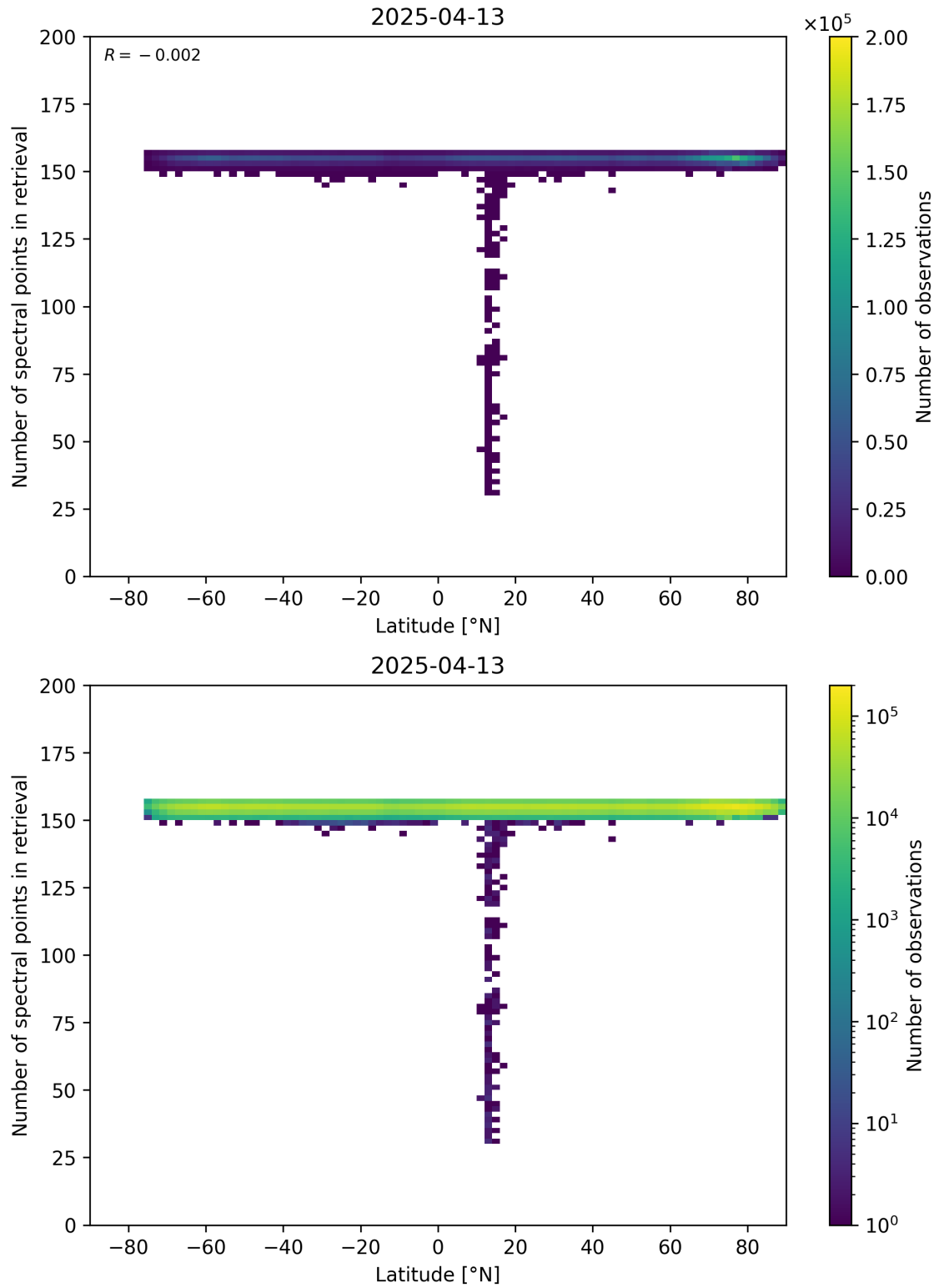
Figure 57: Scatter density plot of “Latitude” against “Number of spectral points in retrieval” for 2025-04-13 to 2025-04-14.
