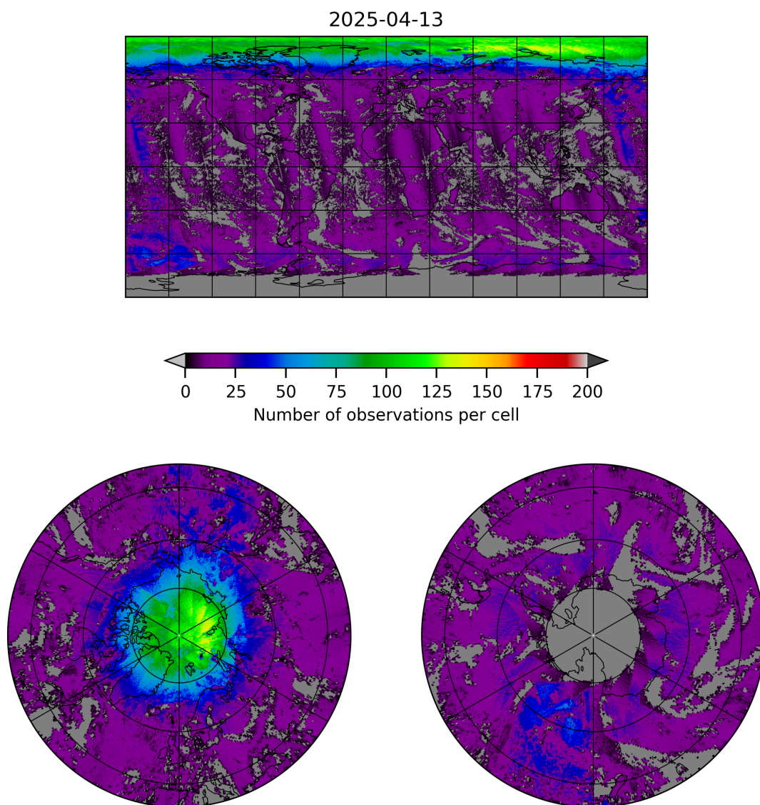
Figure 8: Map of the number of observations for 2025-04-13 to 2025-04-14
