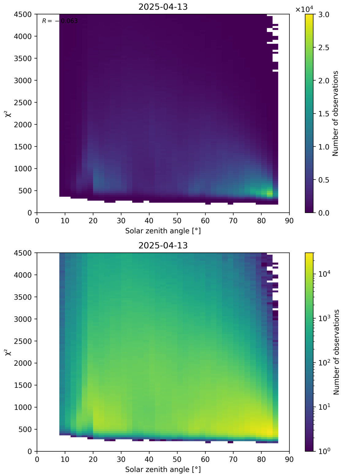
Figure 64: Scatter density plot of “Solar zenith angle” against “ \chi^2 ” for 2025-04-13 to 2025-04-14.
