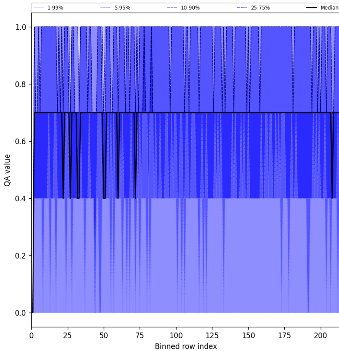
Figure 25: Along track statistics of “QA value” for 2025-04-13 to 2025-04-14
