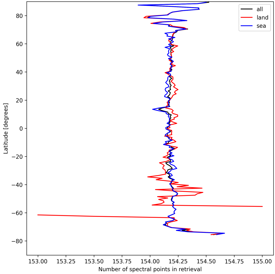
Figure 13: Zonal average of “Number of spectral points in retrieval” for 2025-04-13 to 2025-04-14.
