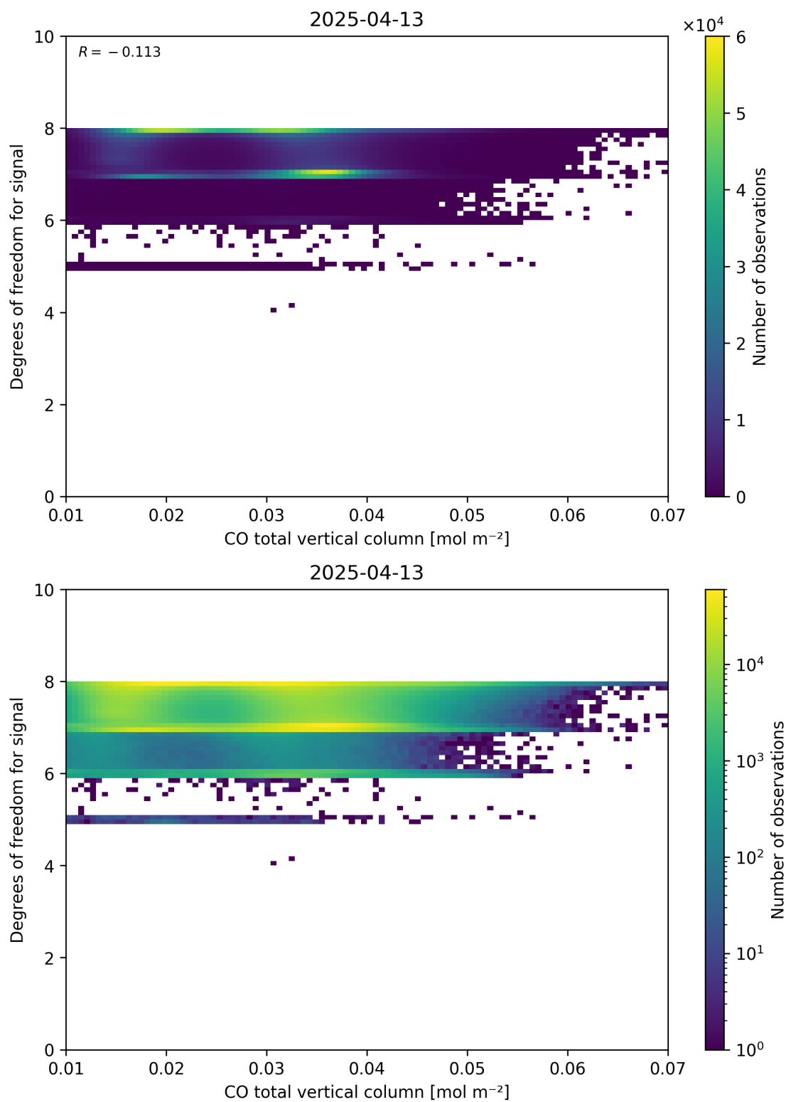
Figure 41: Scatter density plot of “CO total vertical column” against “Degrees of freedom for signal” for 2025-04-13 to 2025-04-14.
