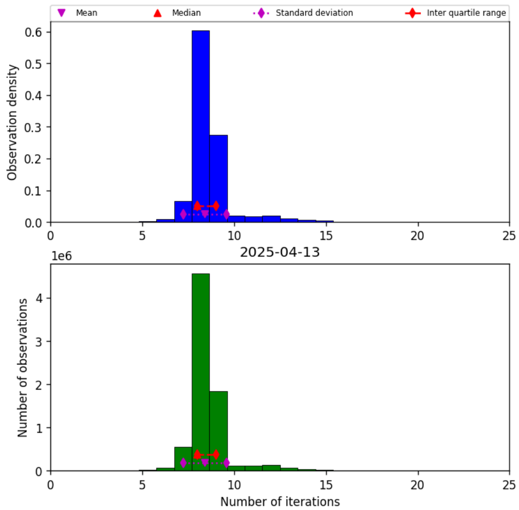
Figure 24: Histogram of “Number of iterations” for 2025-04-13 to 2025-04-14
