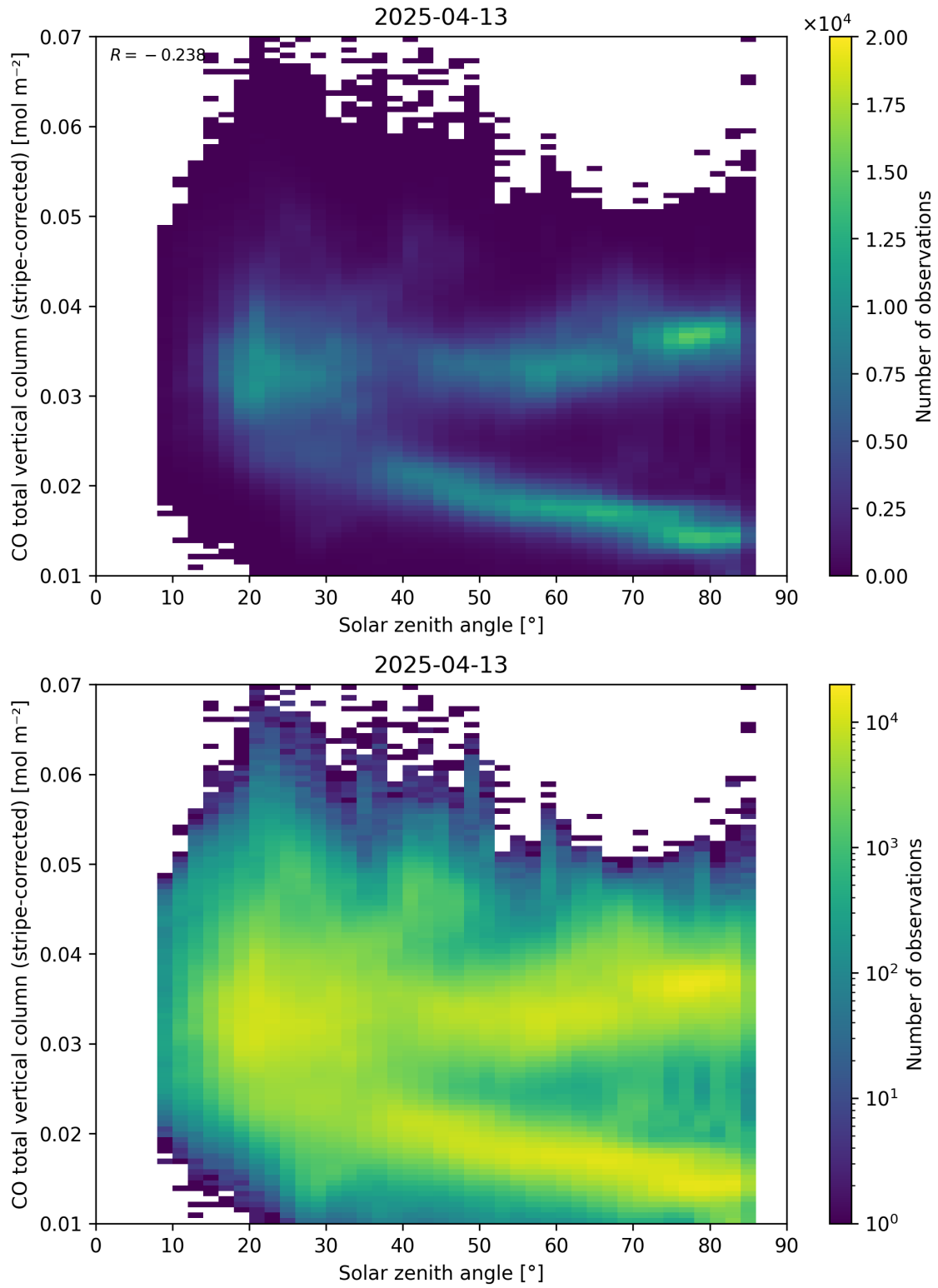
Figure 62: Scatter density plot of “Solar zenith angle” against “CO total vertical column (stripe-corrected)” for 2025-04-13 to 2025-04-14.
