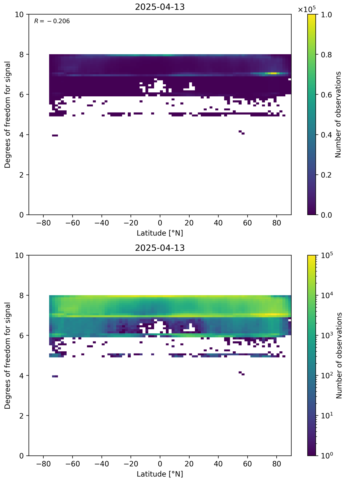
Figure 55: Scatter density plot of “Latitude” against “Degrees of freedom for signal” for 2025-04-13 to 2025-04-14.
