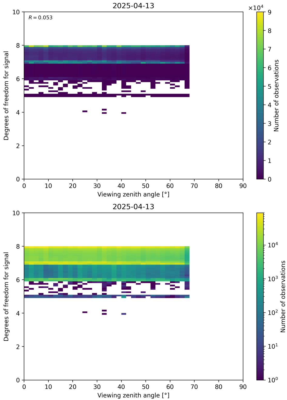
Figure 73: Scatter density plot of “Viewing zenith angle” against “Degrees of freedom for signal” for 2025-04-13 to 2025-04-14.
