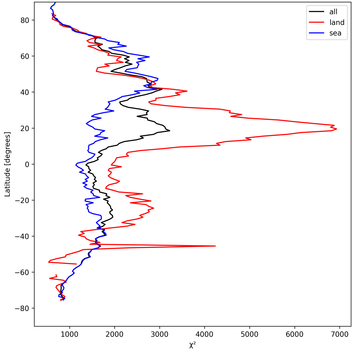
Figure 14: Zonal average of “ \chi^2 ” for 2025-04-13 to 2025-04-14.
