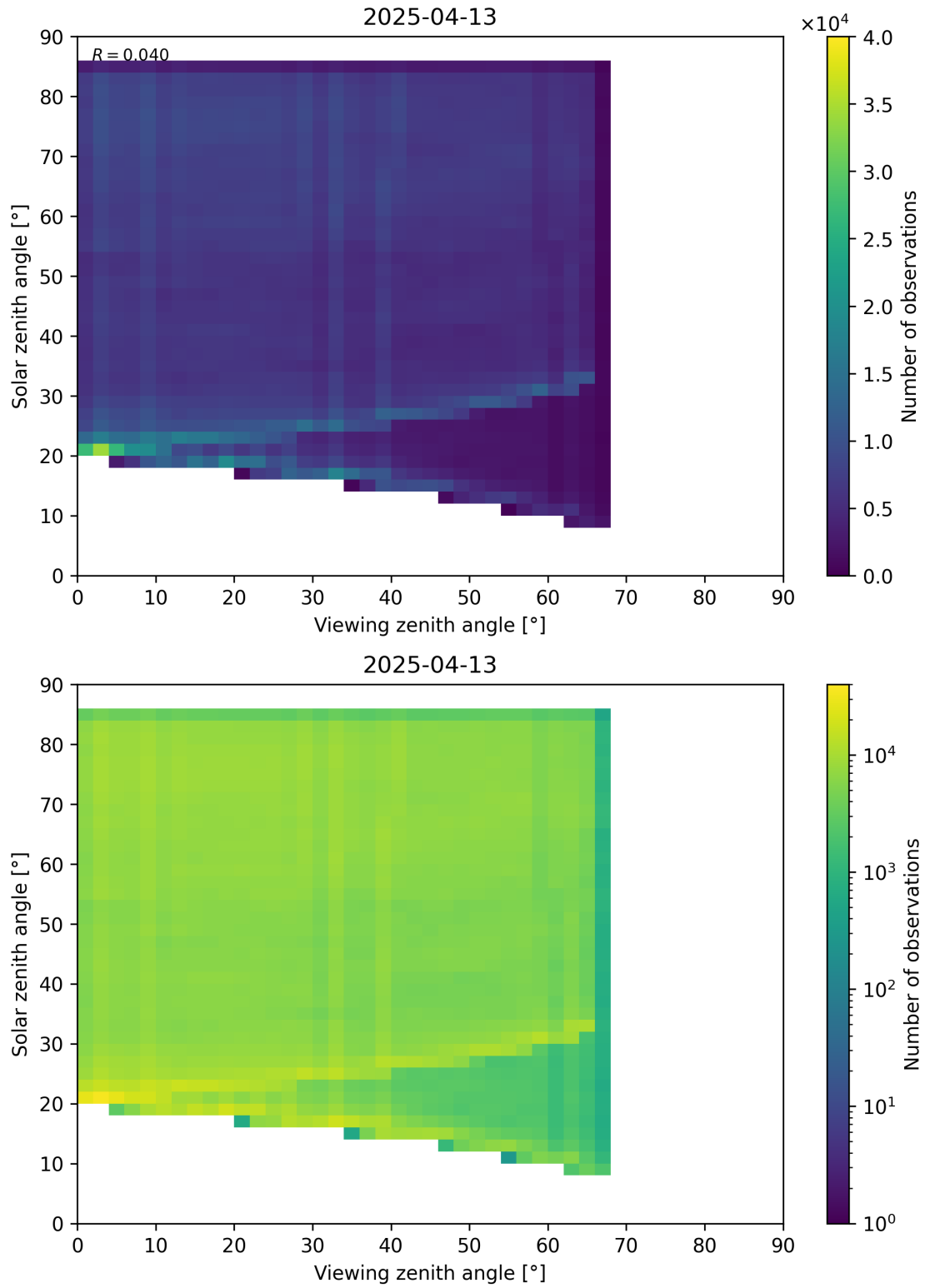
Figure 77: Scatter density plot of “Viewing zenith angle” against “Solar zenith angle” for 2025-04-13 to 2025-04-14.
