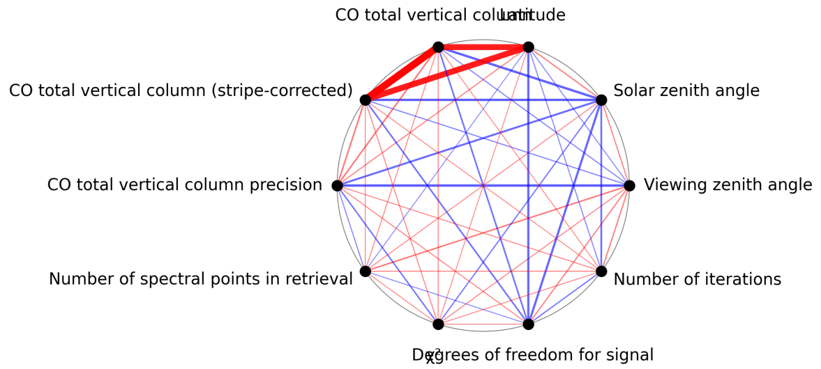
Figure 1: Map of correlation graph for 2025-04-13 to 2025-04-14.
