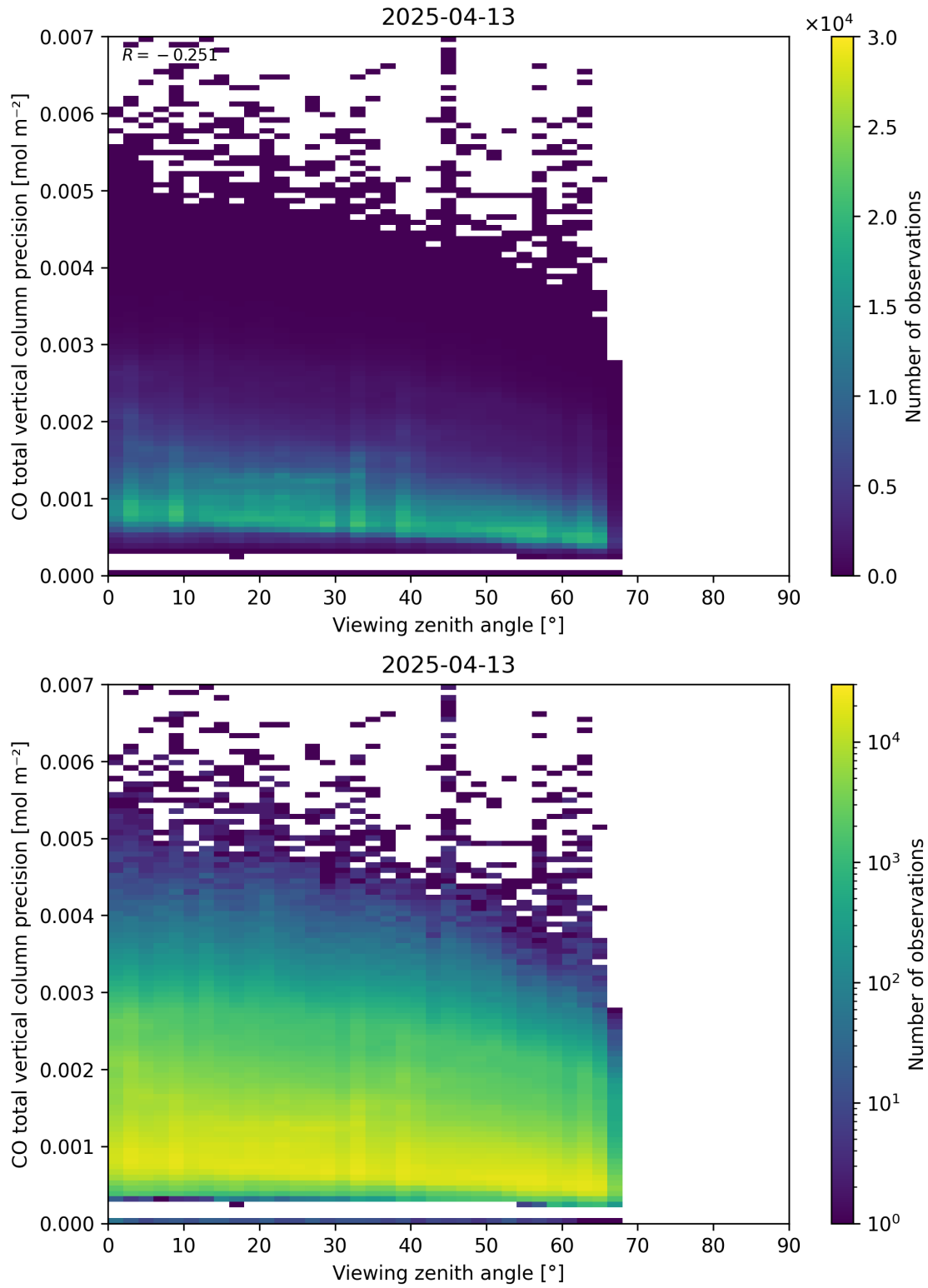
Figure 71: Scatter density plot of “Viewing zenith angle” against “CO total vertical column precision” for 2025-04-13 to 2025-04-14.
