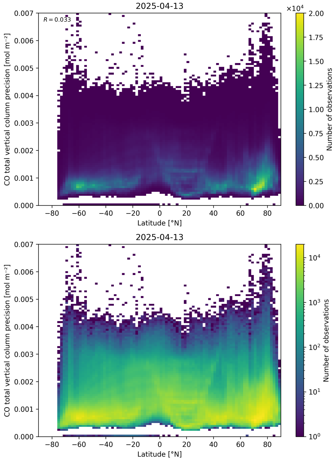
Figure 53: Scatter density plot of “Latitude” against “CO total vertical column precision” for 2025-04-13 to 2025-04-14.
