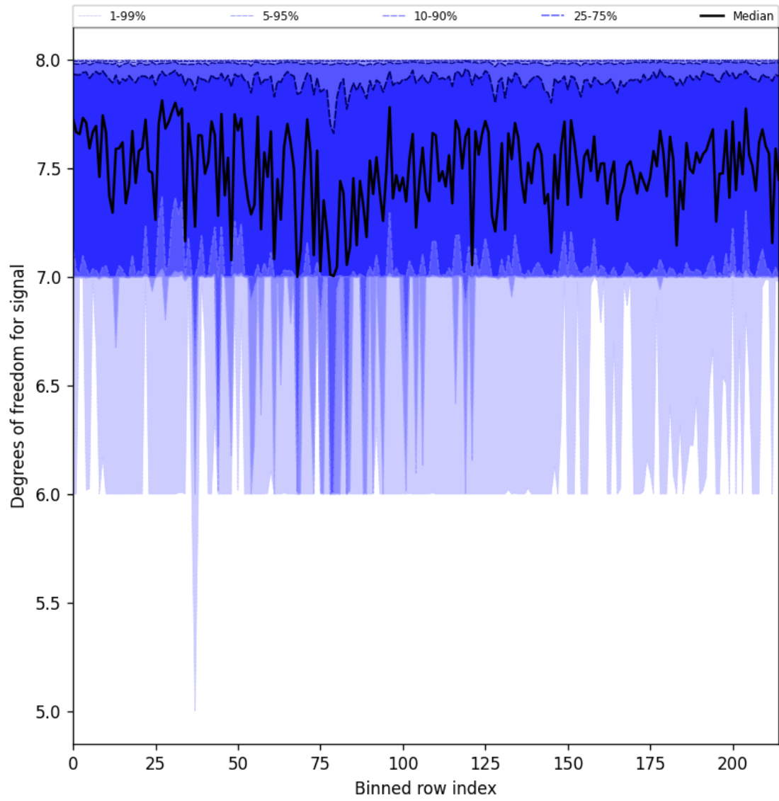
Figure 31: Along track statistics of “Degrees of freedom for signal” for 2025-04-13 to 2025-04-14
