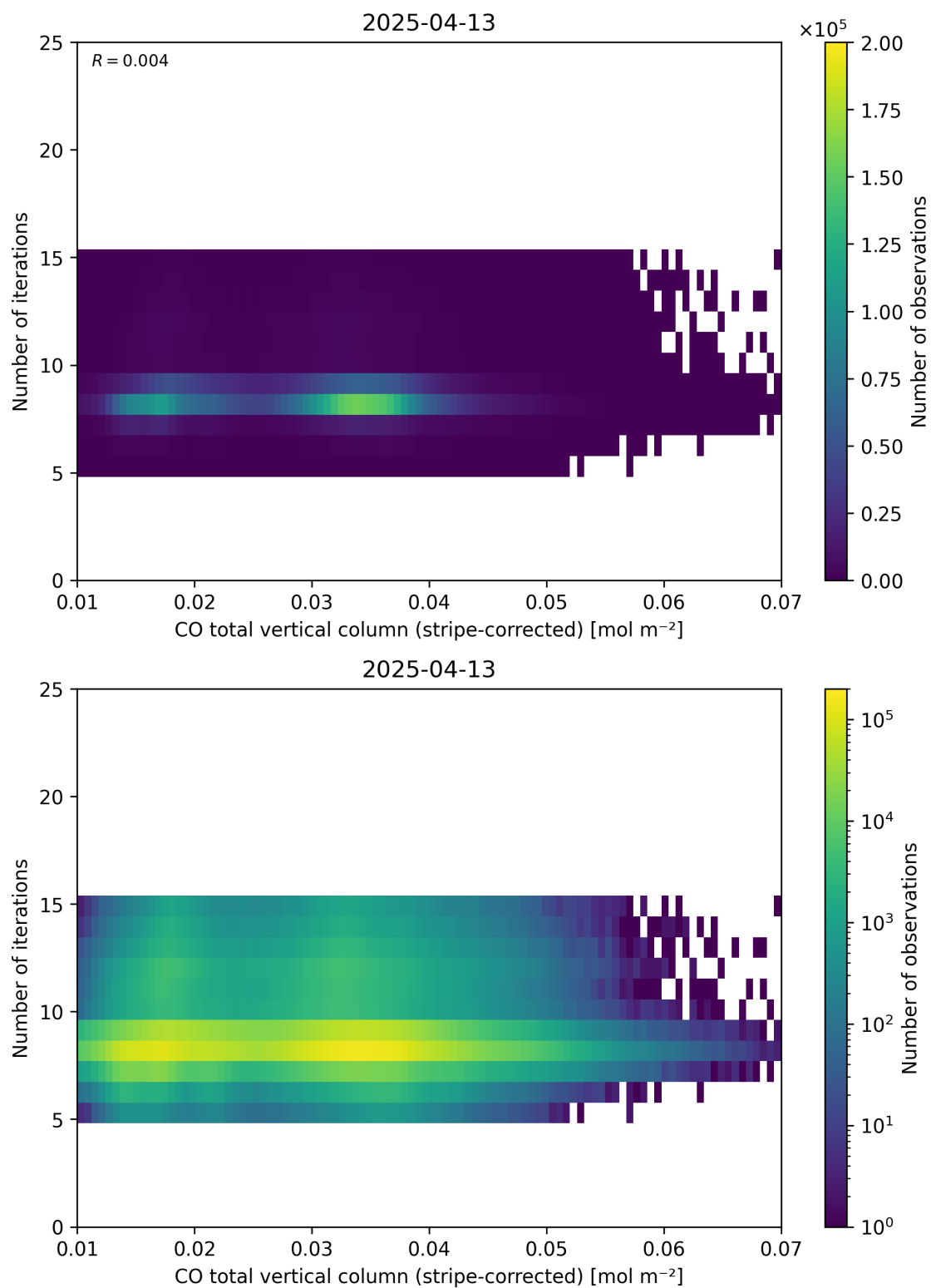
Figure 39: Scatter density plot of “CO total vertical column (stripe-corrected)” against “Number of iterations” for 2025-04-13 to 2025-04-14.
