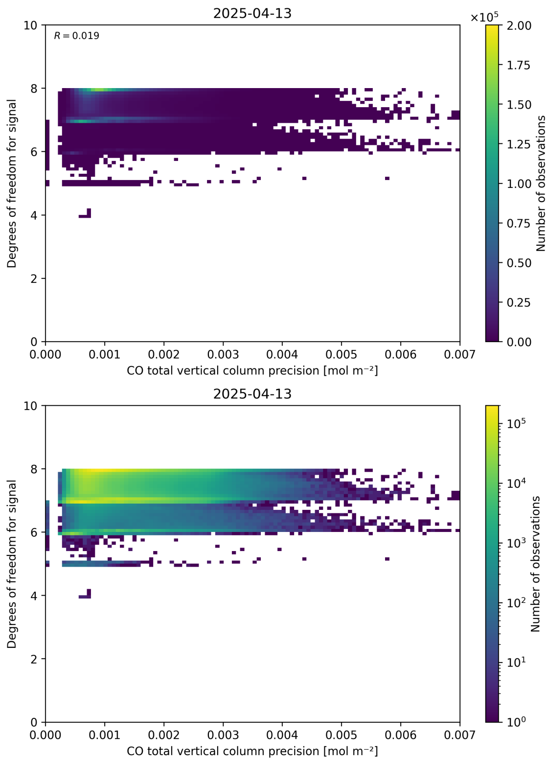
Figure 45: Scatter density plot of “CO total vertical column precision” against “Degrees of freedom for signal” for 2025-04-13 to 2025-04-14.
