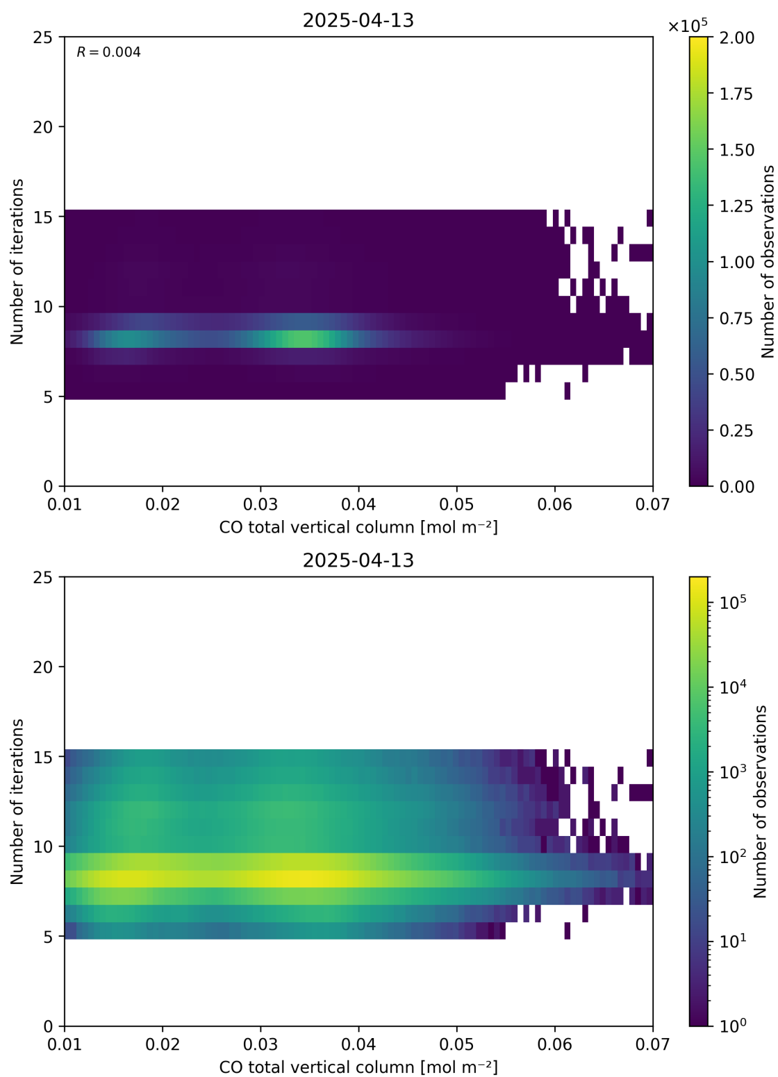
Figure 42: Scatter density plot of “CO total vertical column” against “Number of iterations” for 2025-04-13 to 2025-04-14.
