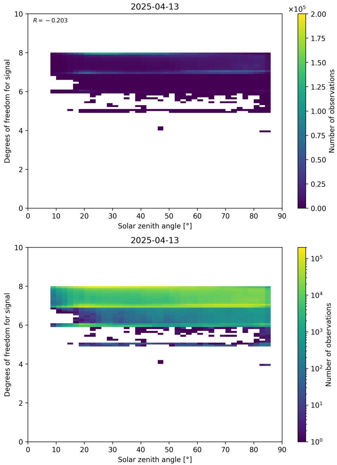
Figure 65: Scatter density plot of “Solar zenith angle” against “Degrees of freedom for signal” for 2025-04-13 to 2025-04-14.
