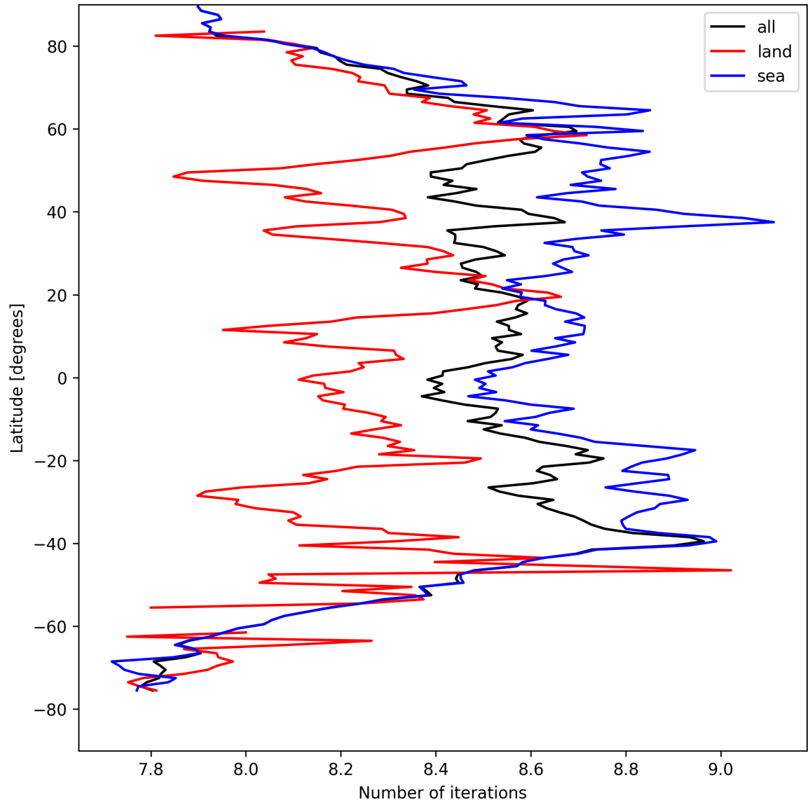
Figure 16: Zonal average of “Number of iterations” for 2025-04-13 to 2025-04-14.
