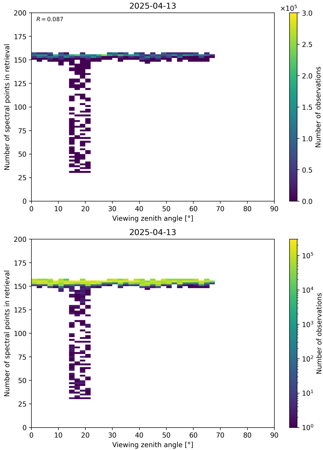
Figure 76: Scatter density plot of “Viewing zenith angle” against “Number of spectral points in retrieval” for 2025-04-13 to 2025-04-14.
