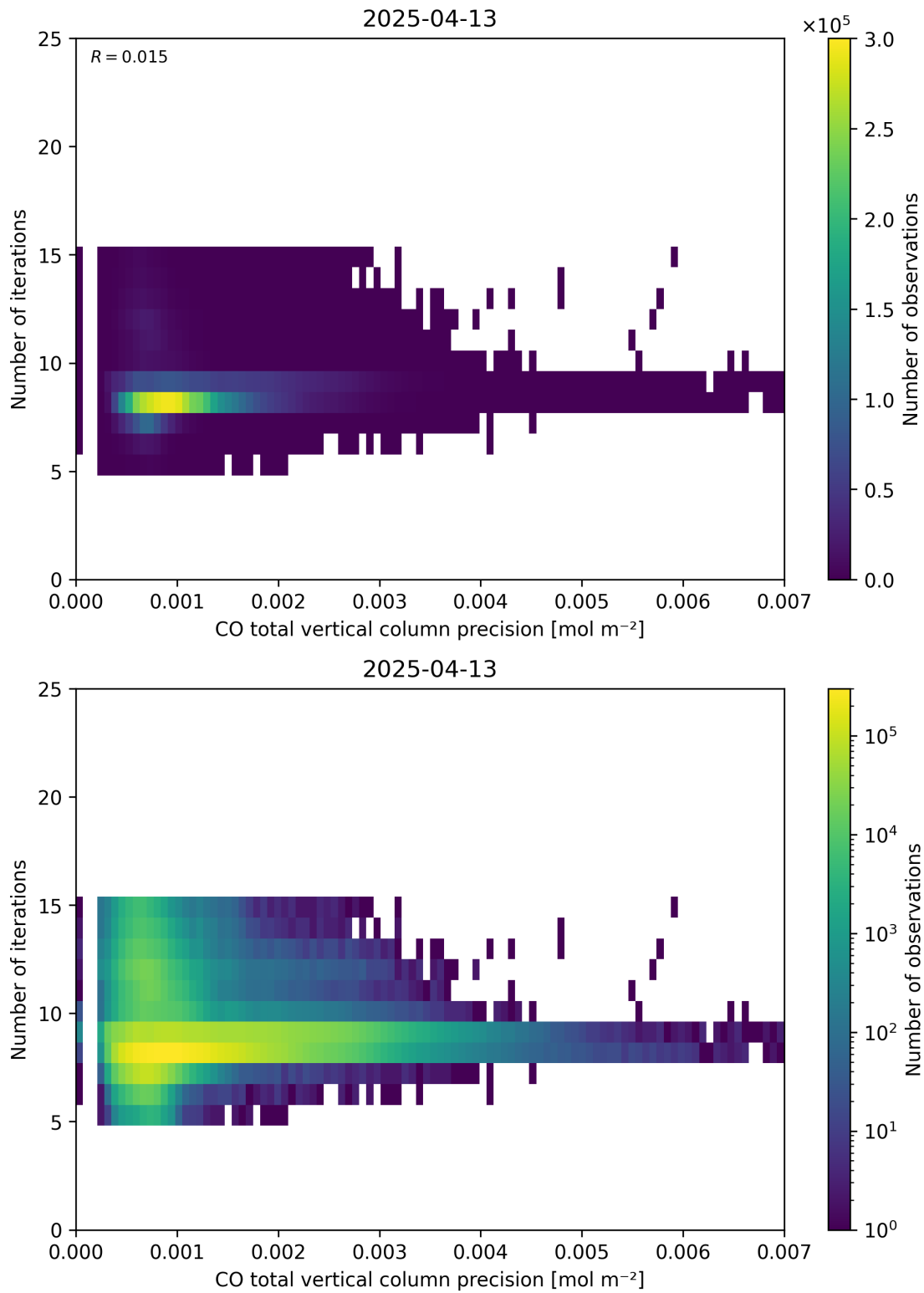
Figure 46: Scatter density plot of “CO total vertical column precision” against “Number of iterations” for 2025-04-13 to 2025-04-14.
