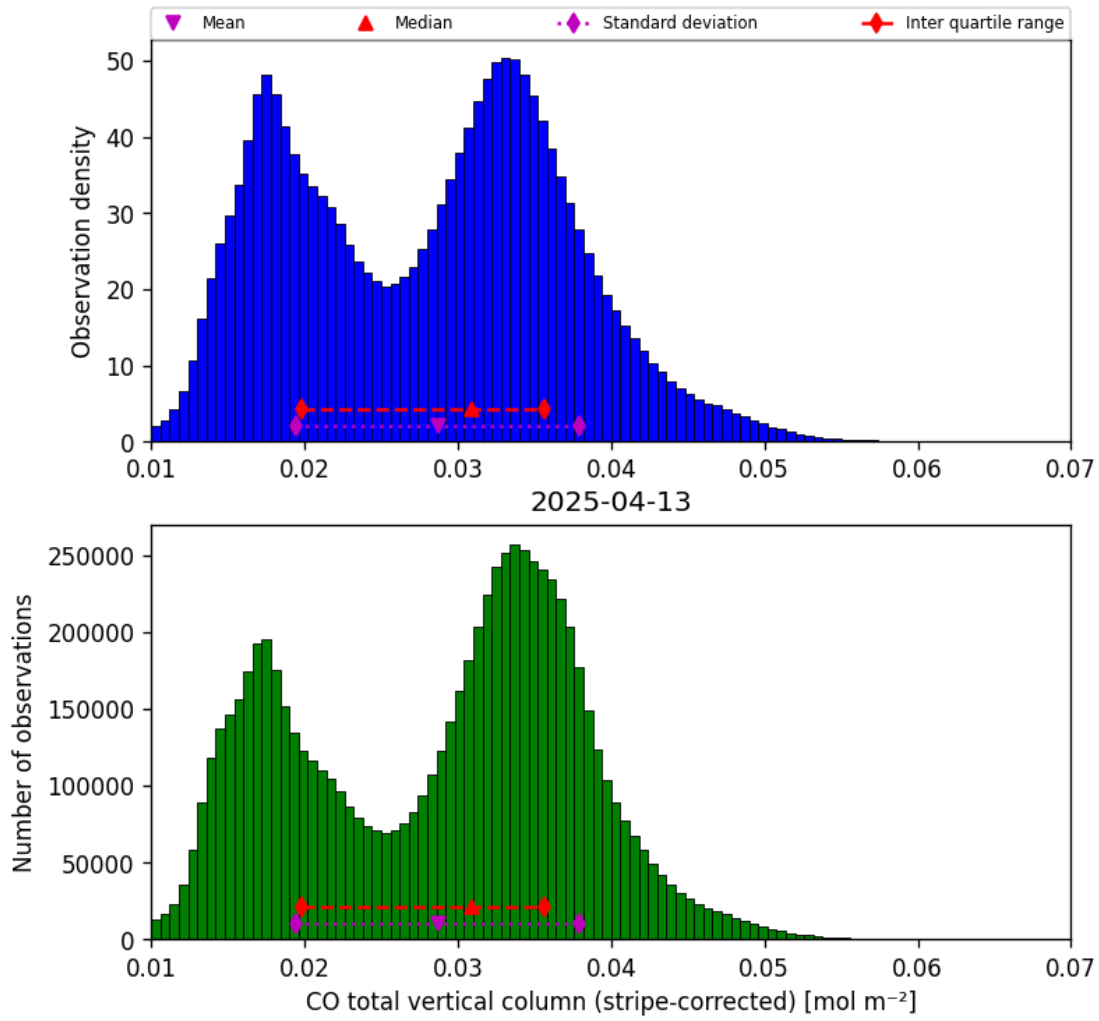
Figure 19: Histogram of “CO total vertical column (stripe-corrected)” for 2025-04-13 to 2025-04-14
