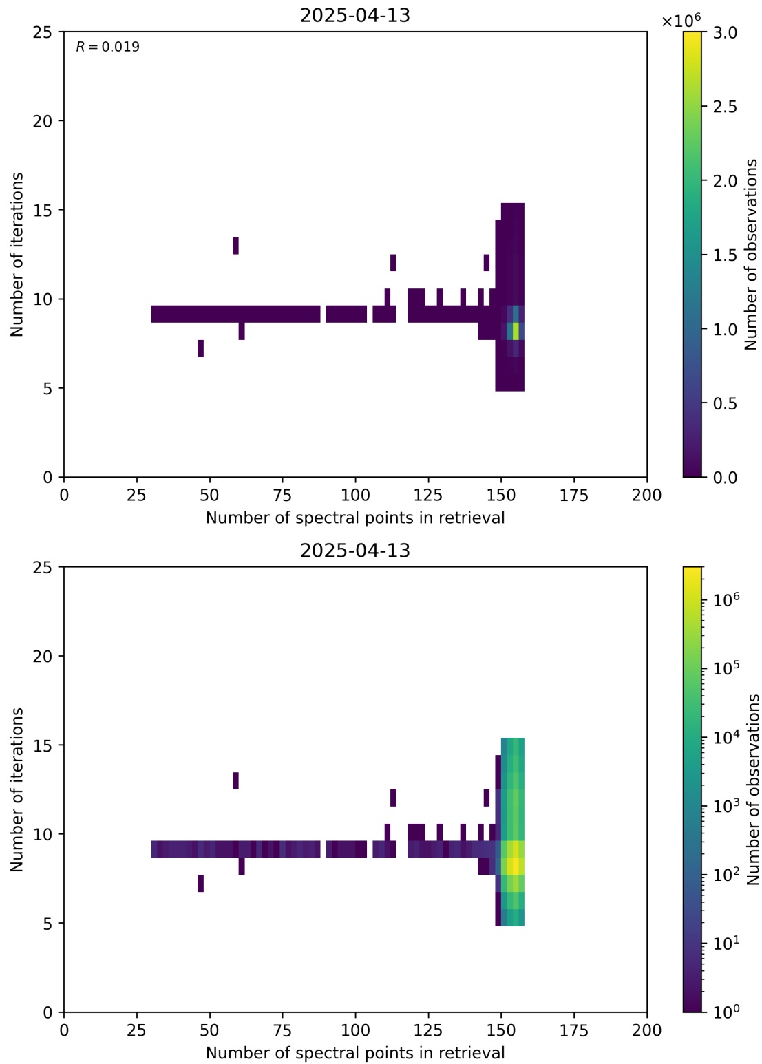
Figure 60: Scatter density plot of “Number of spectral points in retrieval” against “Number of iterations” for 2025-04-13 to 2025-04-14.
