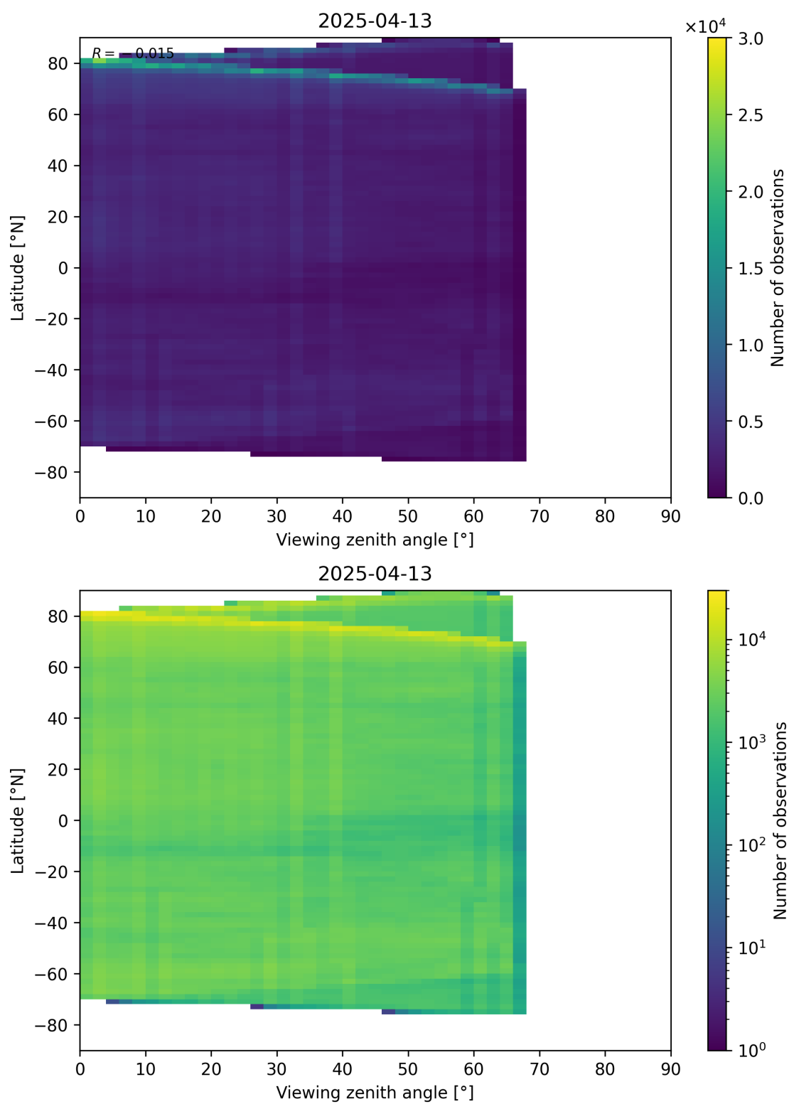
Figure 74: Scatter density plot of “Viewing zenith angle” against “Latitude” for 2025-04-13 to 2025-04-14.
