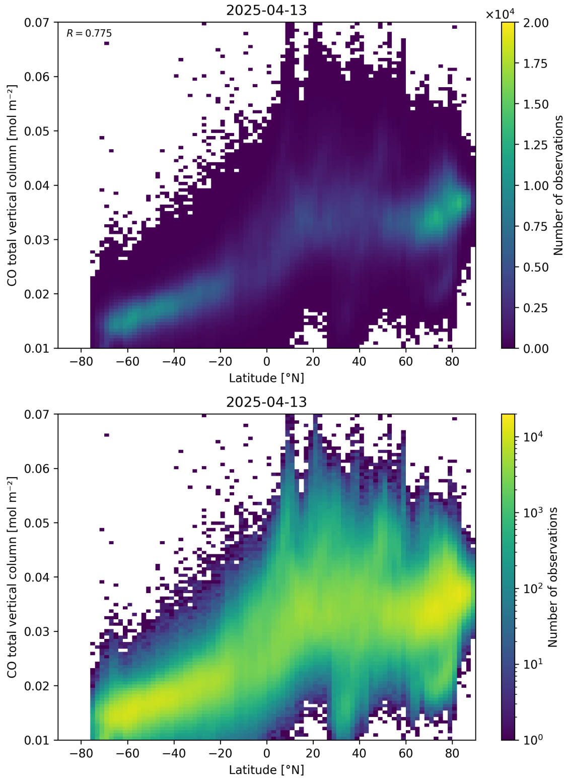
Figure 51: Scatter density plot of “Latitude” against “CO total vertical column” for 2025-04-13 to 2025-04-14.
