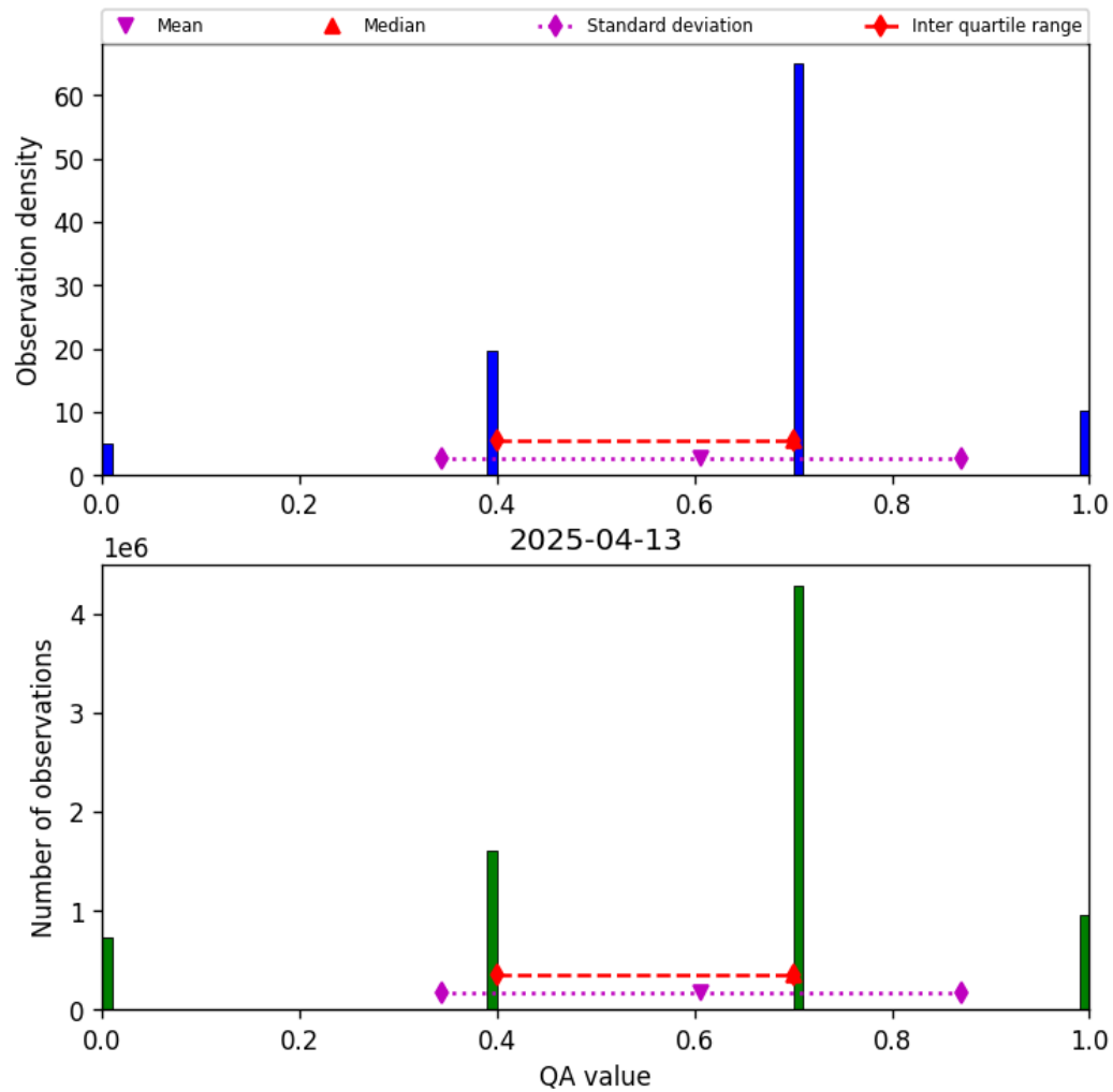
Figure 17: Histogram of “QA value” for 2025-04-13 to 2025-04-14
