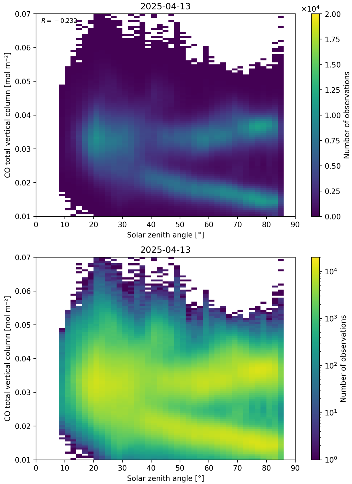
Figure 61: Scatter density plot of “Solar zenith angle” against “CO total vertical column” for 2025-04-13 to 2025-04-14.
