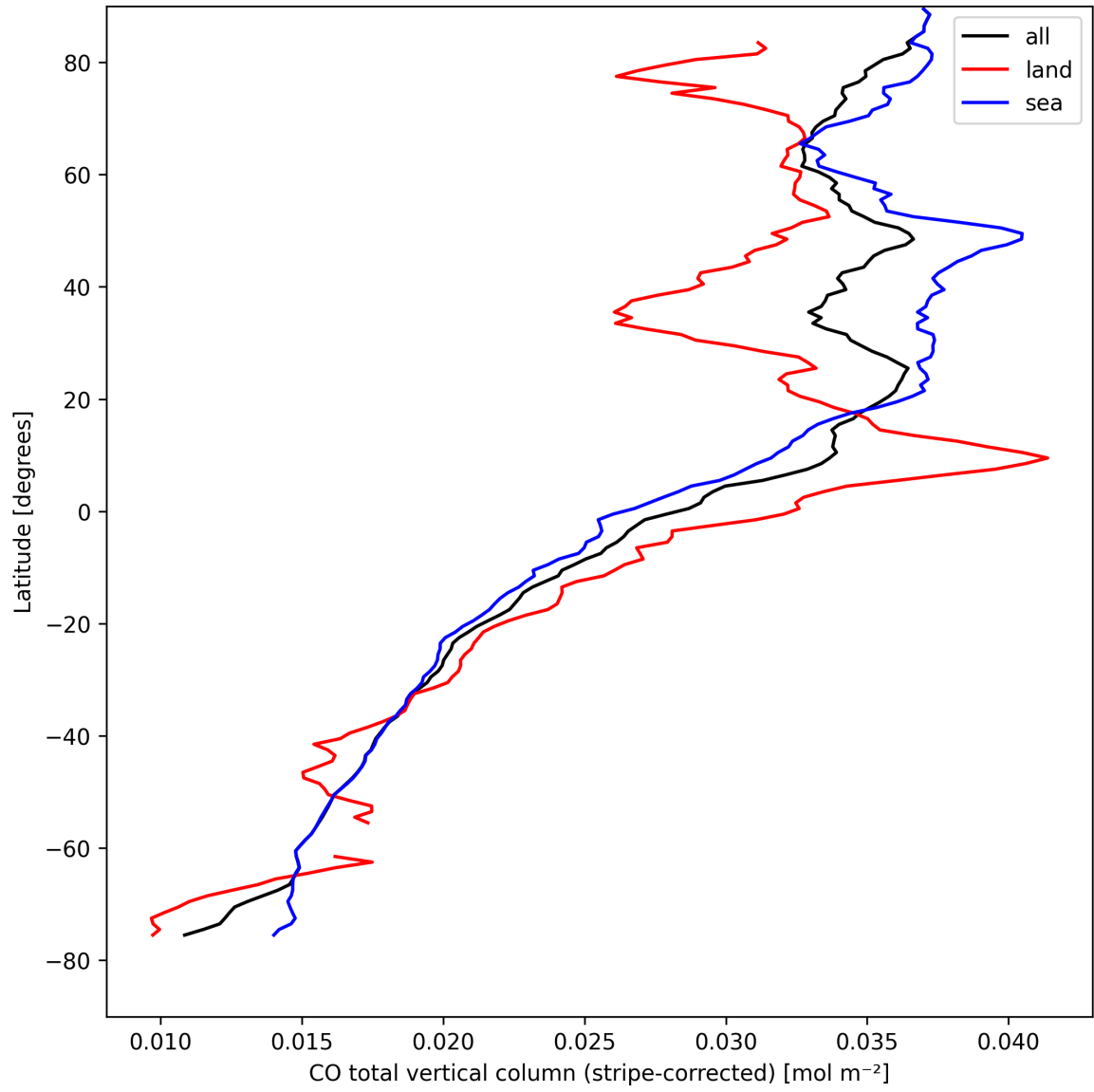
Figure 11: Zonal average of “CO total vertical column (stripe-corrected)” for 2025-04-13 to 2025-04-14.
