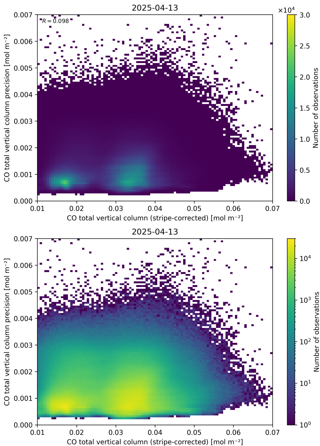
Figure 36: Scatter density plot of “CO total vertical column (stripe-corrected)” against “CO total vertical column precision” for 2025-04-13 to 2025-04-14.
