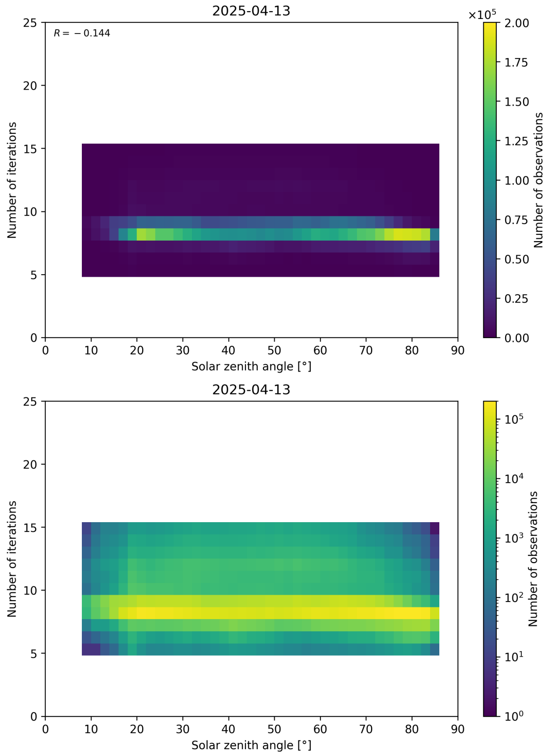
Figure 67: Scatter density plot of “Solar zenith angle” against “Number of iterations” for 2025-04-13 to 2025-04-14.
