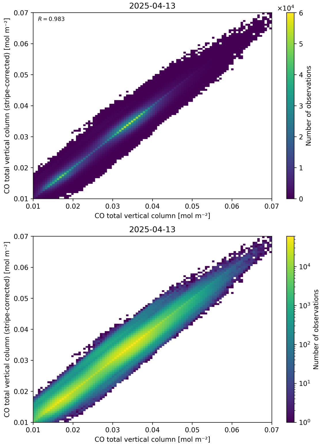
Figure 33: Scatter density plot of “CO total vertical column” against “CO total vertical column (stripe-corrected)” for 2025-04-13 to 2025-04-14.
