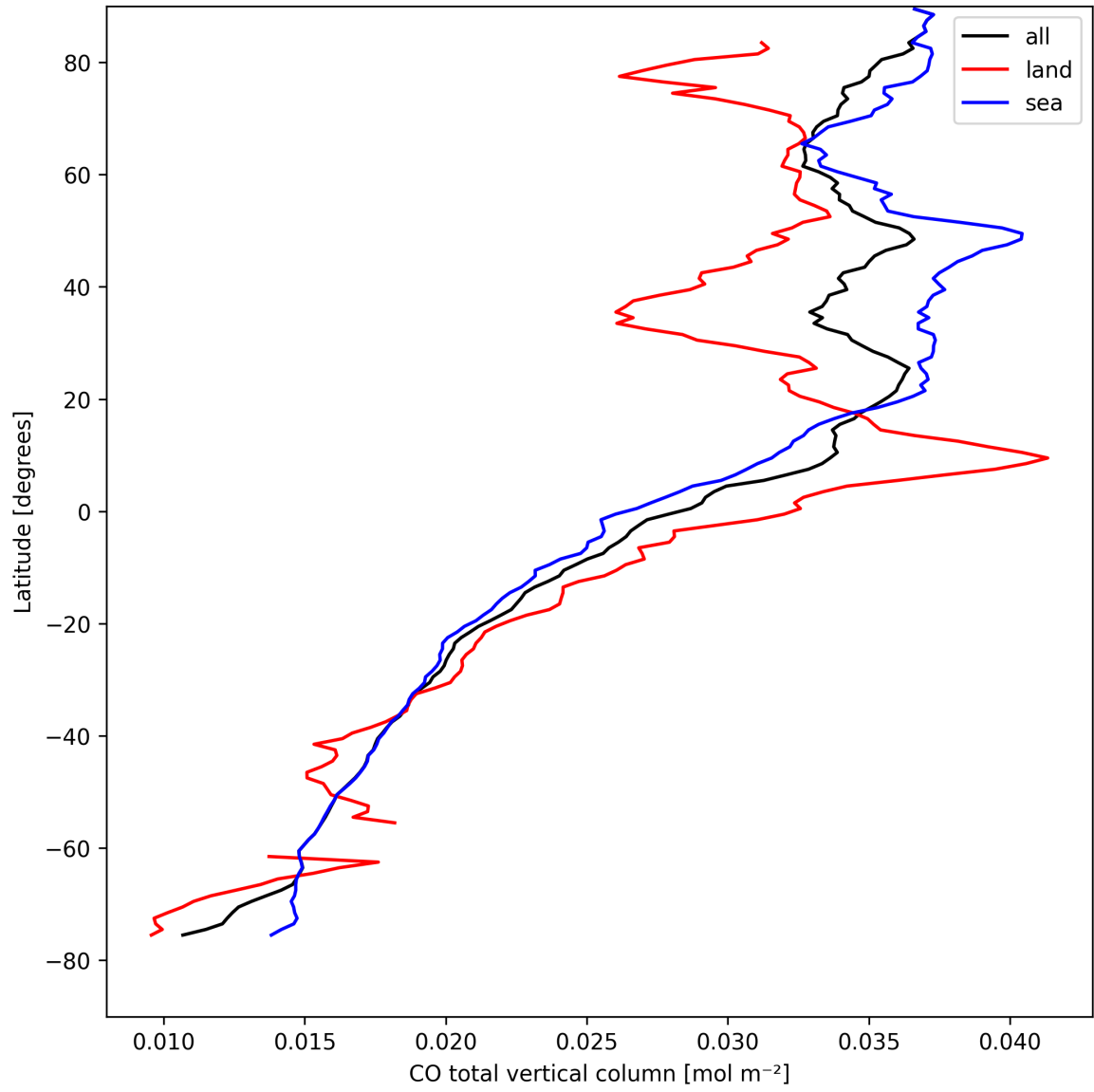
Figure 10: Zonal average of “CO total vertical column” for 2025-04-13 to 2025-04-14.
