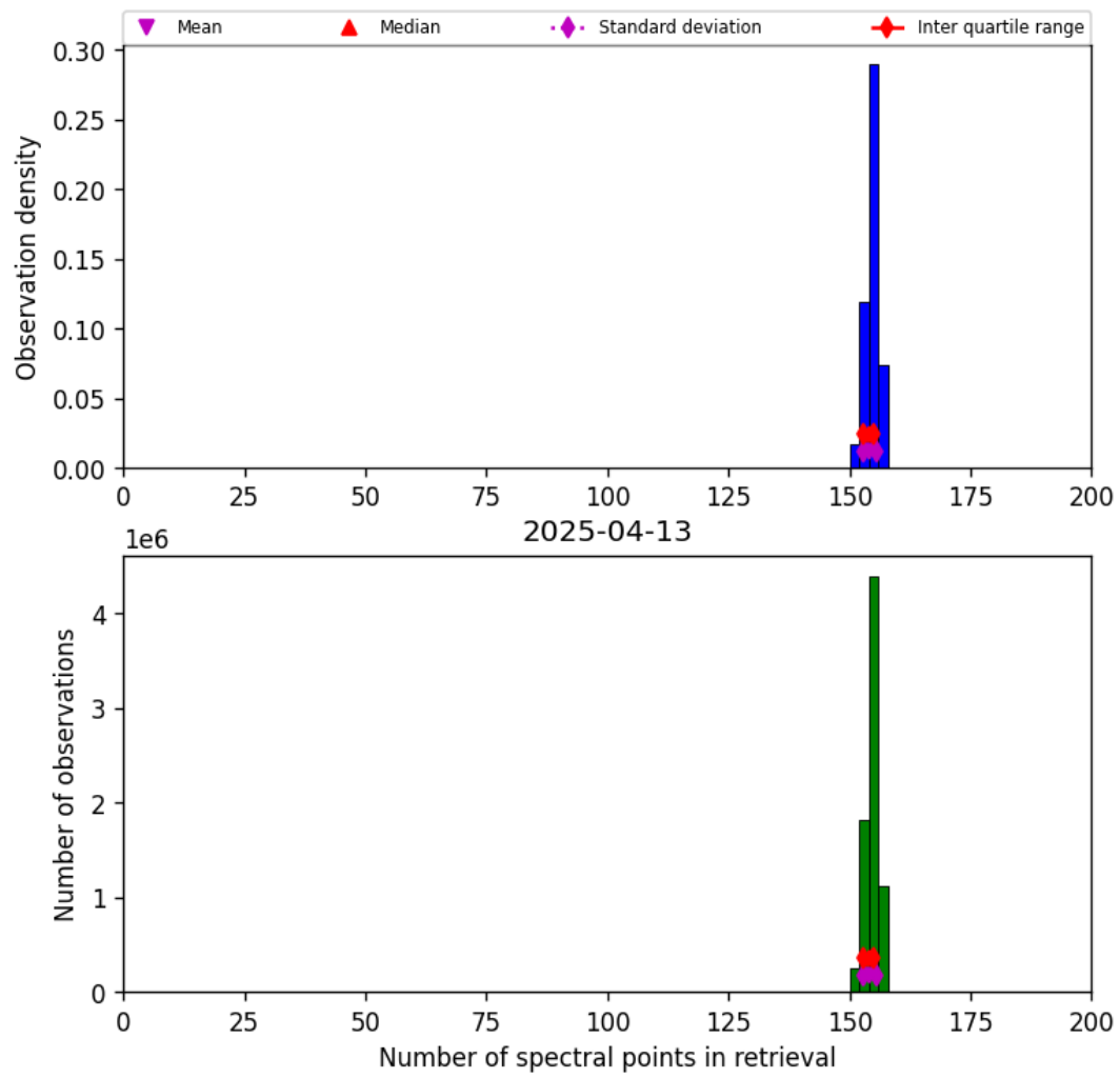
Figure 21: Histogram of “Number of spectral points in retrieval” for 2025-04-13 to 2025-04-14
