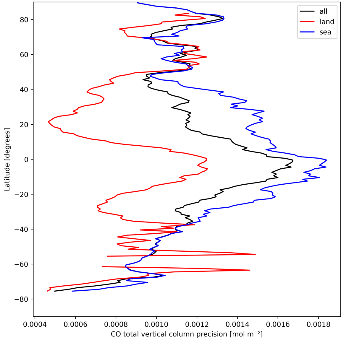
Figure 12: Zonal average of "CO total vertical column precision" for 2025-04-13 to 2025-04-14.
