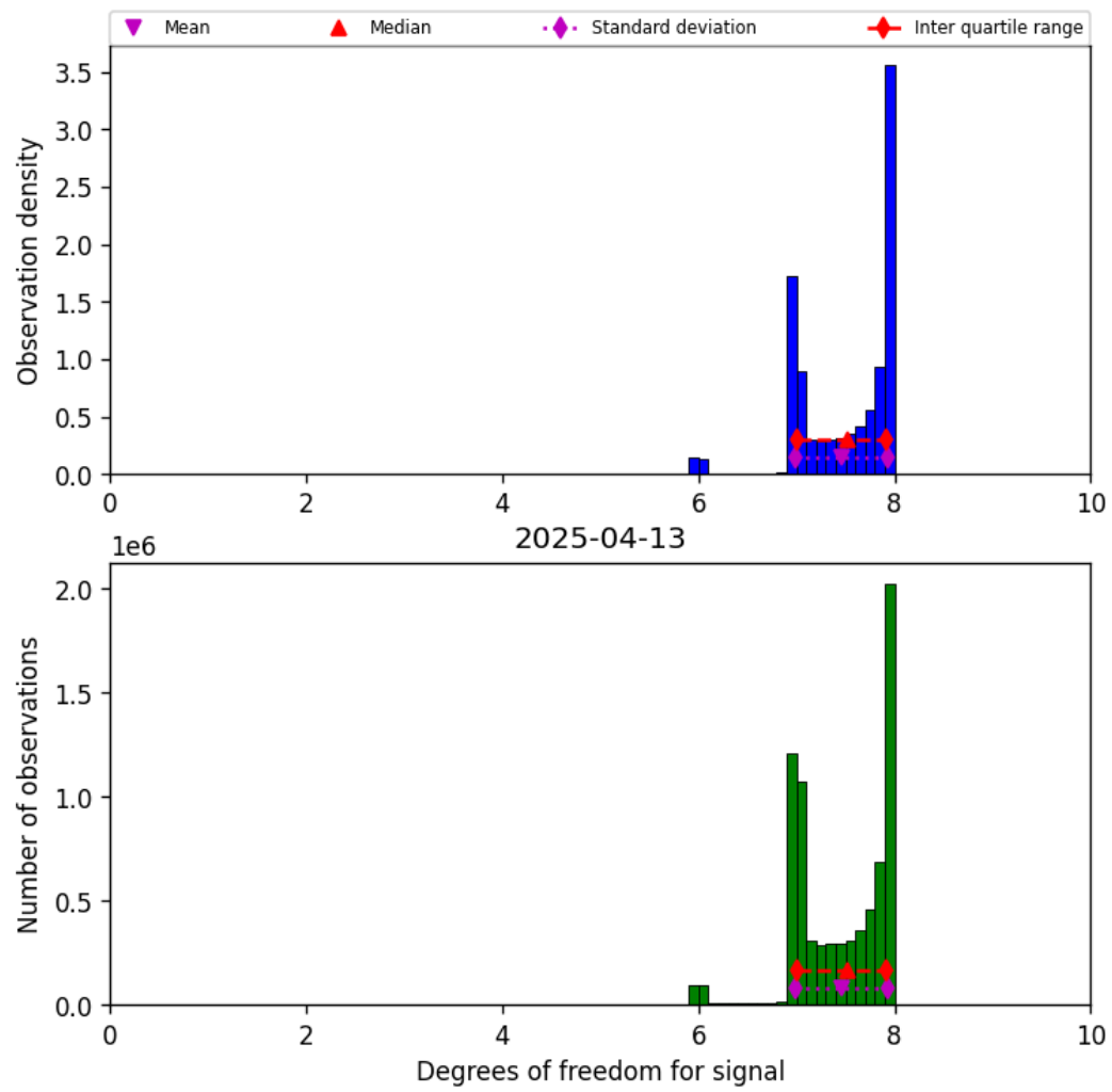
Figure 23: Histogram of “Degrees of freedom for signal” for 2025-04-13 to 2025-04-14
