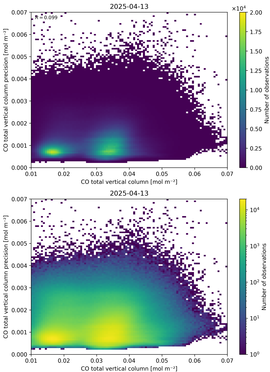
Figure 34: Scatter density plot of “CO total vertical column” against “CO total vertical column precision” for 2025-04-13 to 2025-04-14.
