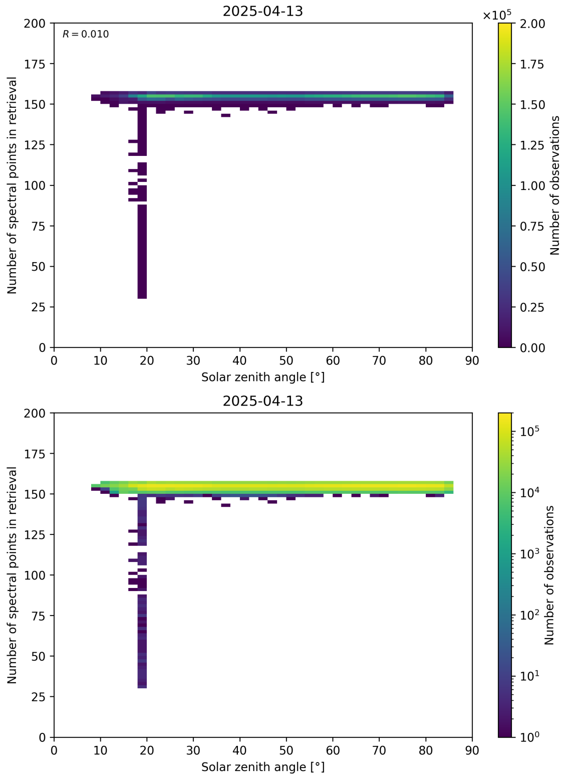
Figure 68: Scatter density plot of “Solar zenith angle” against “Number of spectral points in retrieval” for 2025-04-13 to 2025-04-14.
