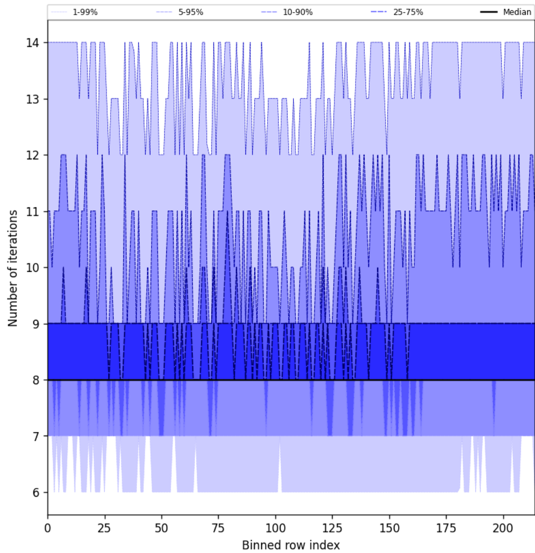
Figure 32: Along track statistics of “Number of iterations” for 2025-04-13 to 2025-04-14
