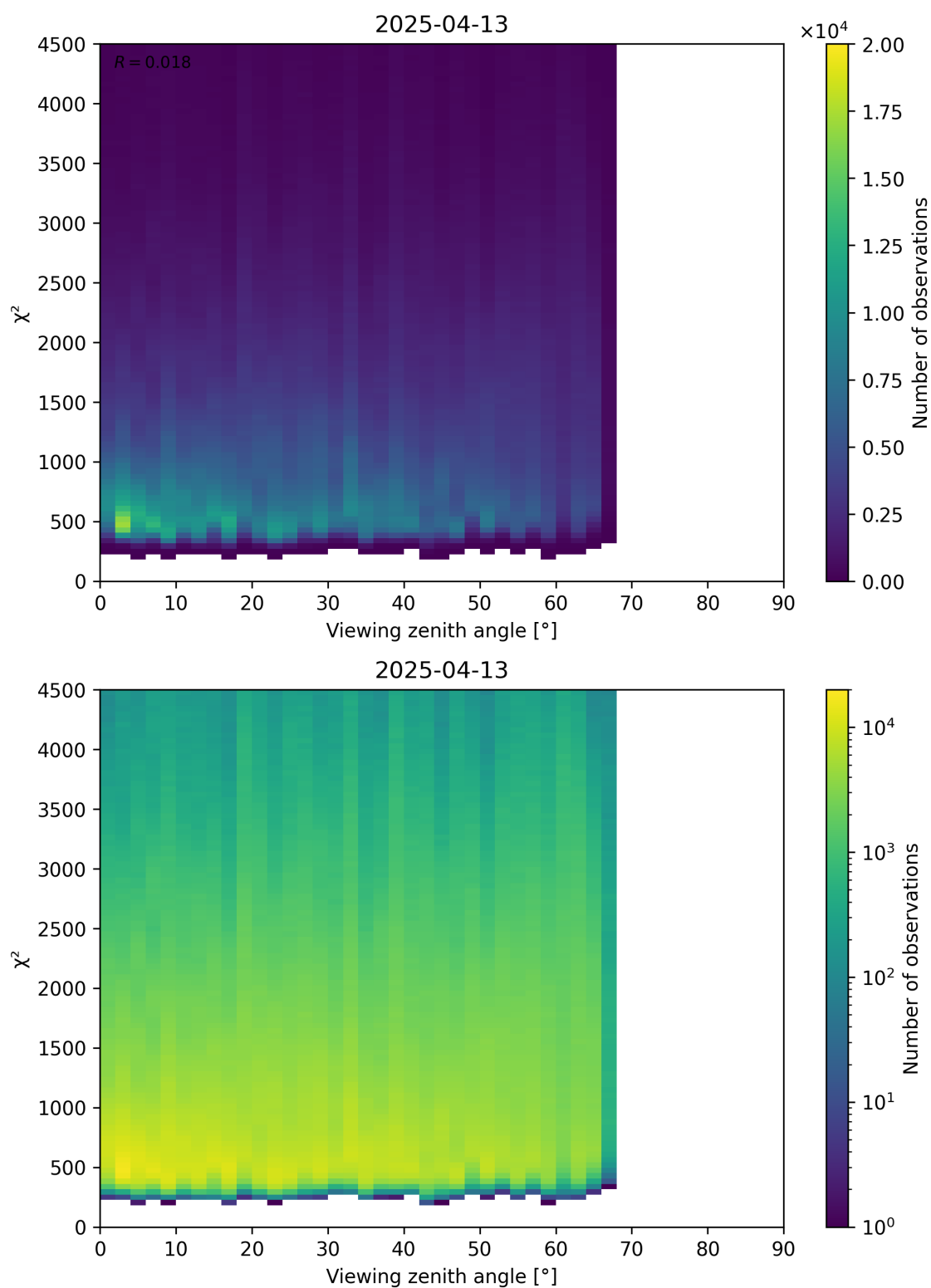
Figure 72: Scatter density plot of “Viewing zenith angle” against “ \chi^2 ” for 2025-04-13 to 2025-04-14.
