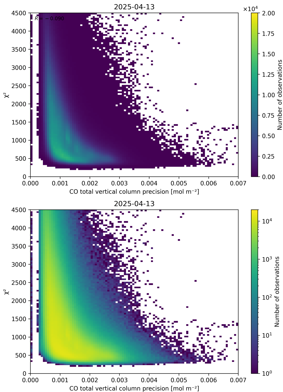
Figure 44: Scatter density plot of “CO total vertical column precision” against “ \chi^2 ” for 2025-04-13 to 2025-04-14.
