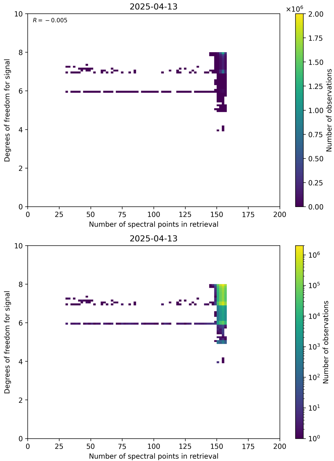
Figure 59: Scatter density plot of “Number of spectral points in retrieval” against “Degrees of freedom for signal” for 2025-04-13 to 2025-04-14.
