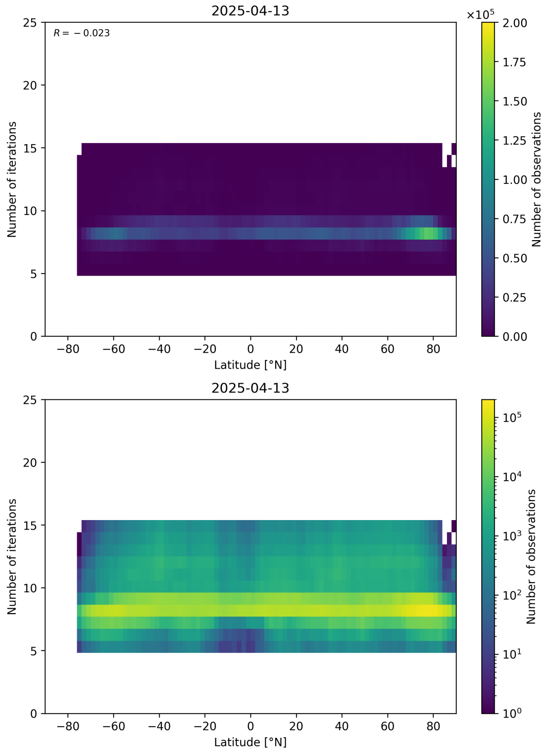
Figure 56: Scatter density plot of “Latitude” against “Number of iterations” for 2025-04-13 to 2025-04-14.
