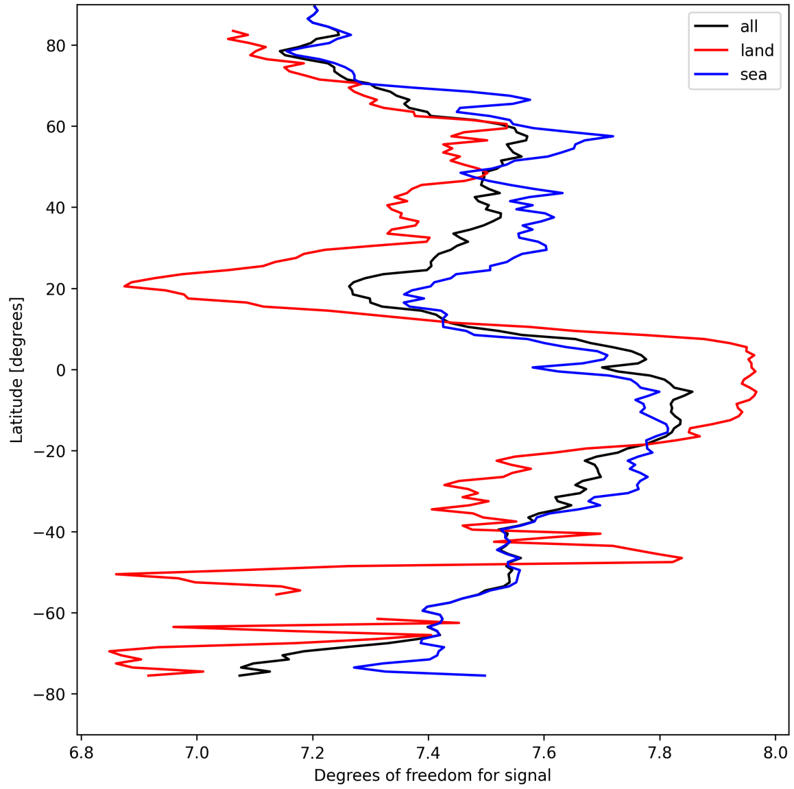
Figure 15: Zonal average of “Degrees of freedom for signal” for 2025-04-13 to 2025-04-14.
