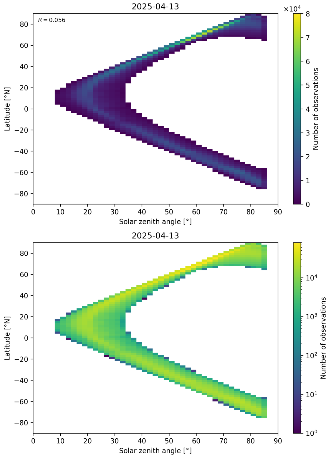
Figure 66: Scatter density plot of “Solar zenith angle” against “Latitude” for 2025-04-13 to 2025-04-14.
