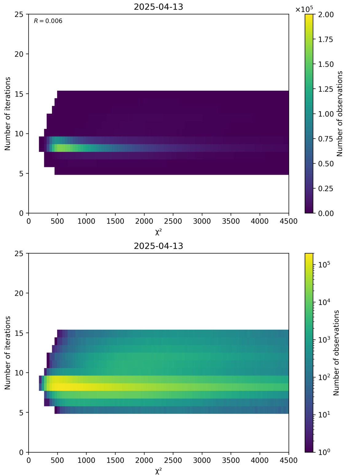
Figure 49: Scatter density plot of “ \chi^2 ” against “Number of iterations” for 2025-04-13 to 2025-04-14.
