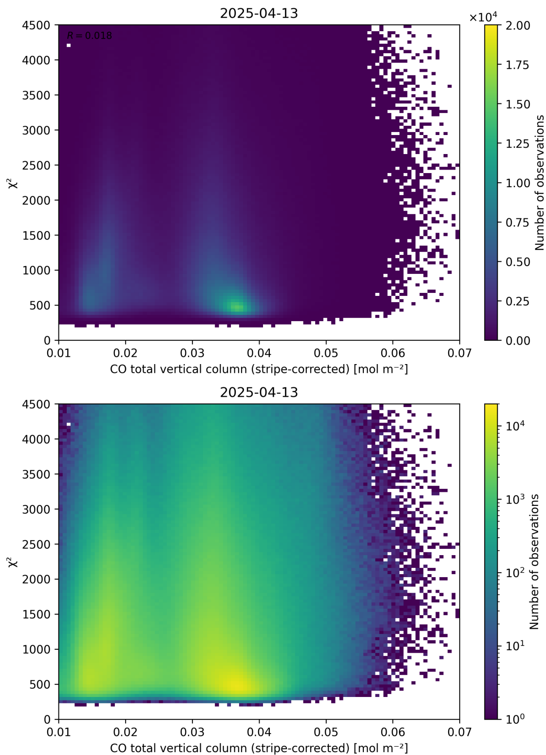
Figure 37: Scatter density plot of “CO total vertical column (stripe-corrected)” against “ \chi^2 ” for 2025-04-13 to 2025-04-14.
