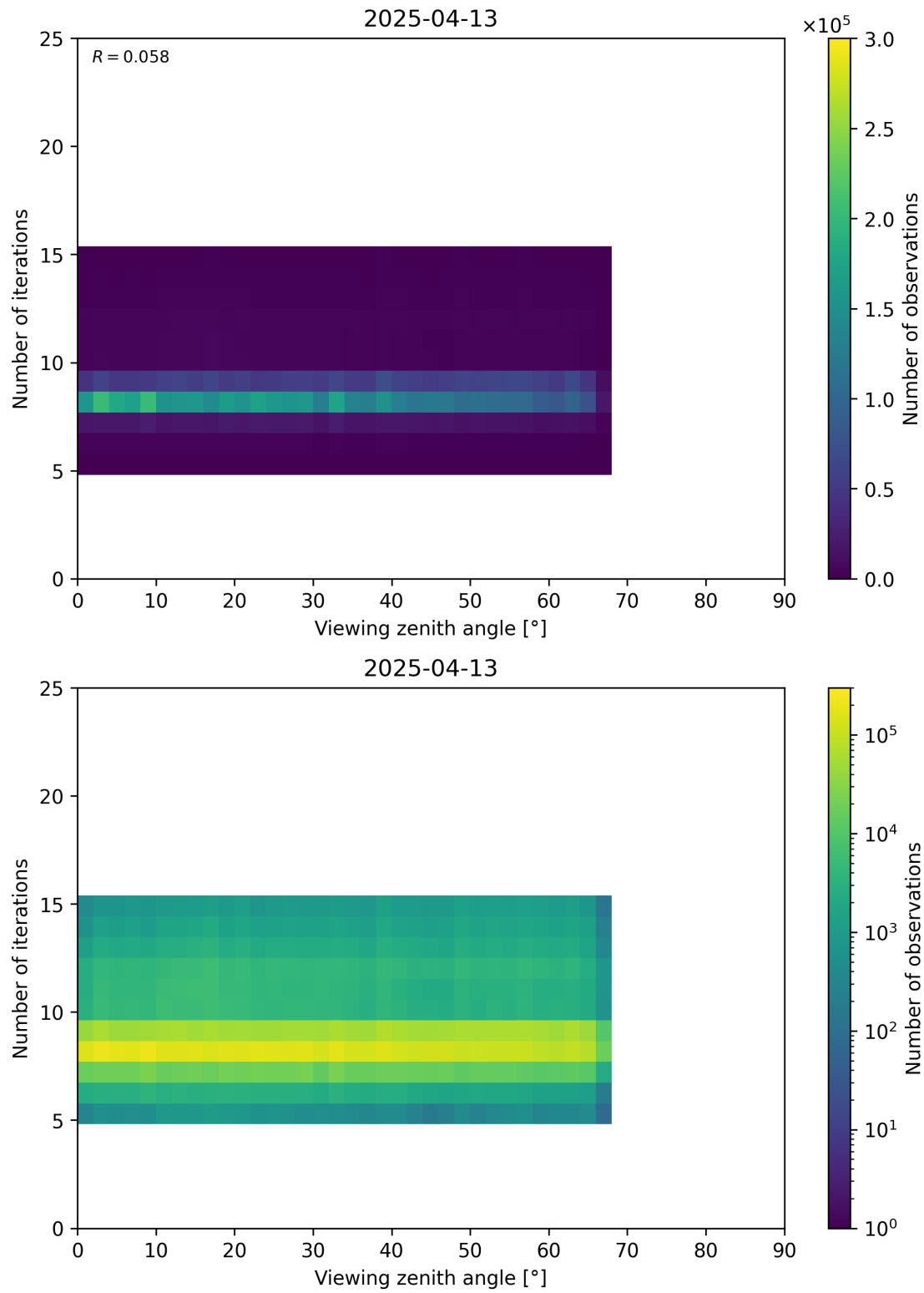
Figure 75: Scatter density plot of “Viewing zenith angle” against “Number of iterations” for 2025-04-13 to 2025-04-14.
