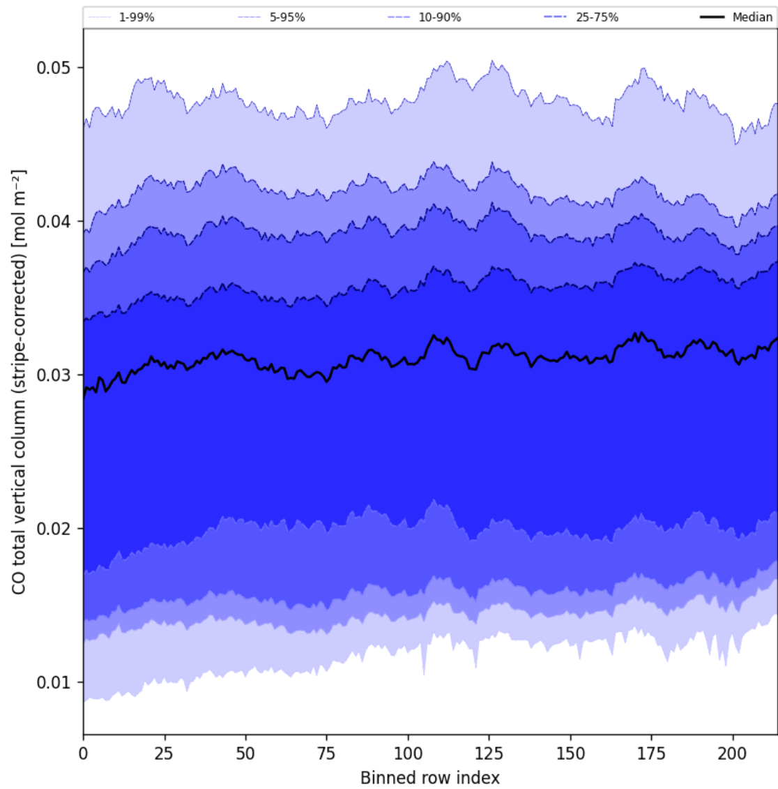
Figure 27: Along track statistics of “CO total vertical column (stripe-corrected)” for 2025-04-13 to 2025-04-14
