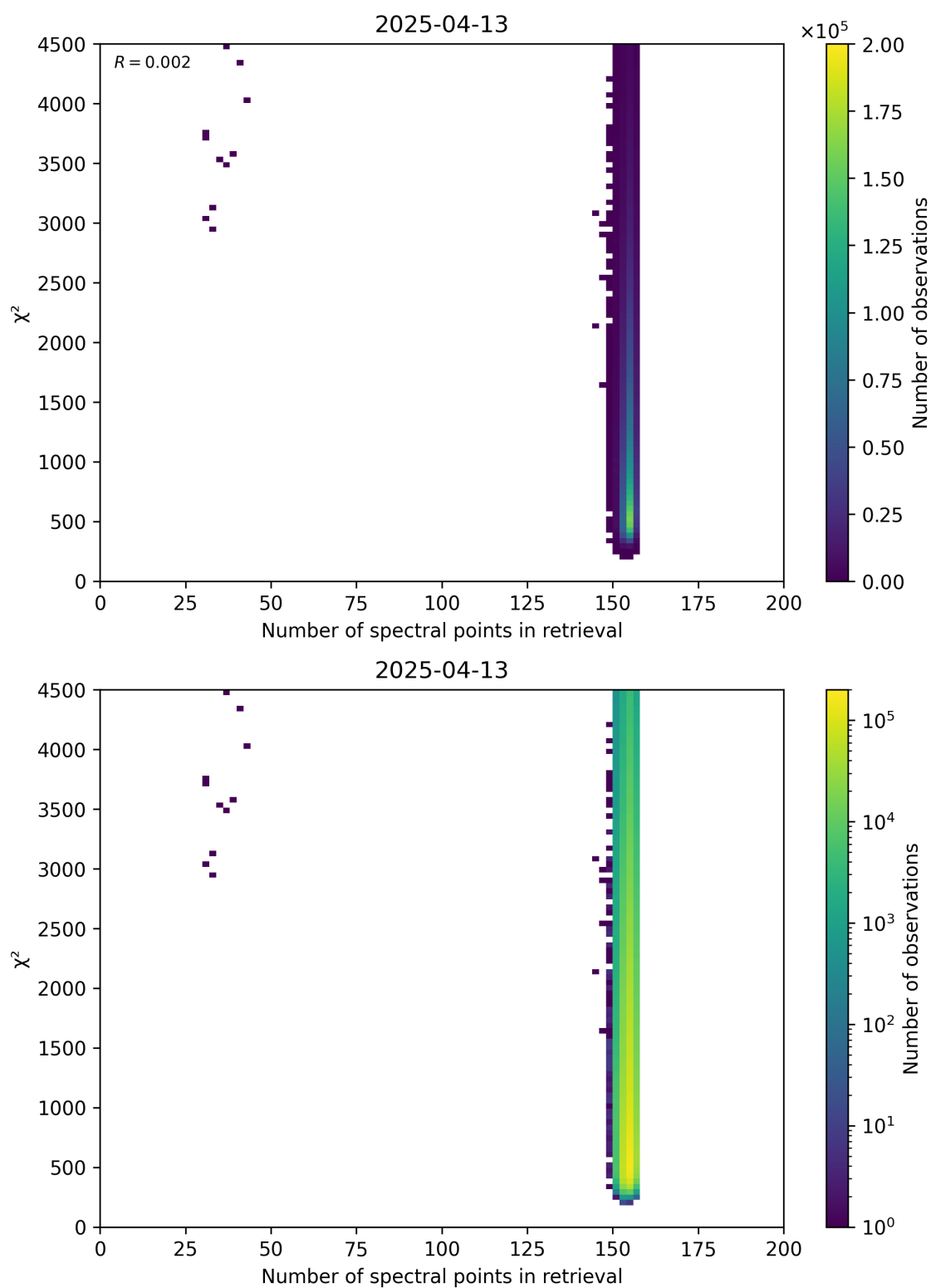
Figure 58: Scatter density plot of “Number of spectral points in retrieval” against “ \chi^2 ” for 2025-04-13 to 2025-04-14.
