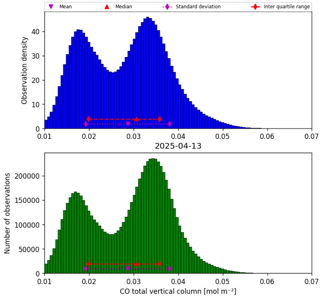
Figure 18: Histogram of “CO total vertical column” for 2025-04-13 to 2025-04-14
