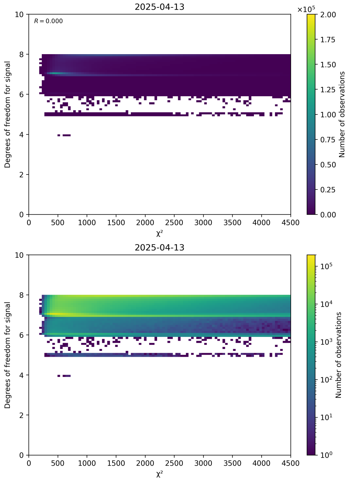
Figure 48: Scatter density plot of " \chi^2 " against "Degrees of freedom for signal" for 2025-04-13 to 2025-04-14.
