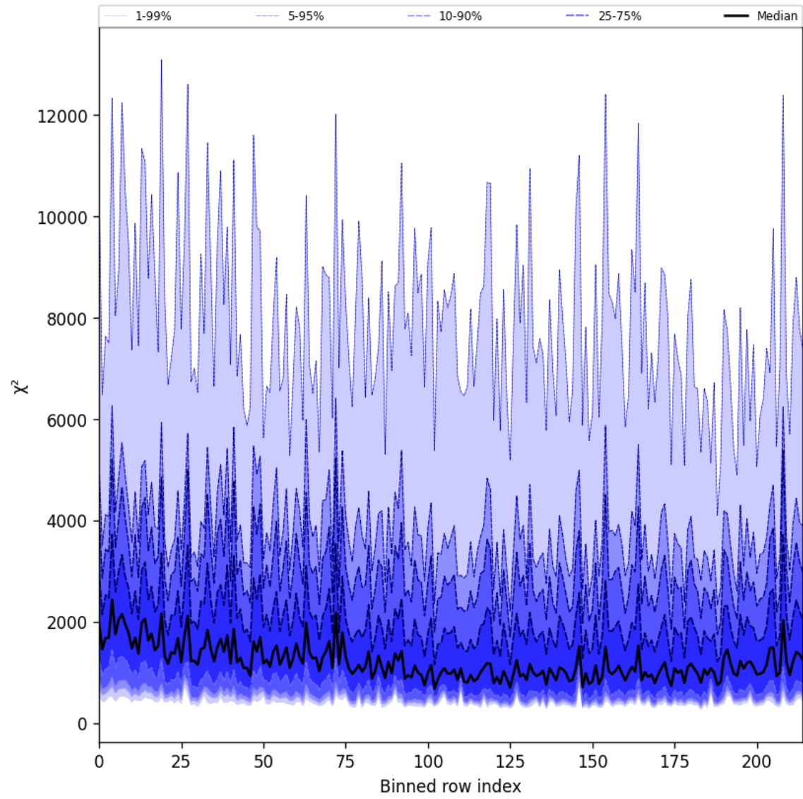
Figure 30: Along track statistics of “ \chi^2 ” for 2025-04-13 to 2025-04-14
