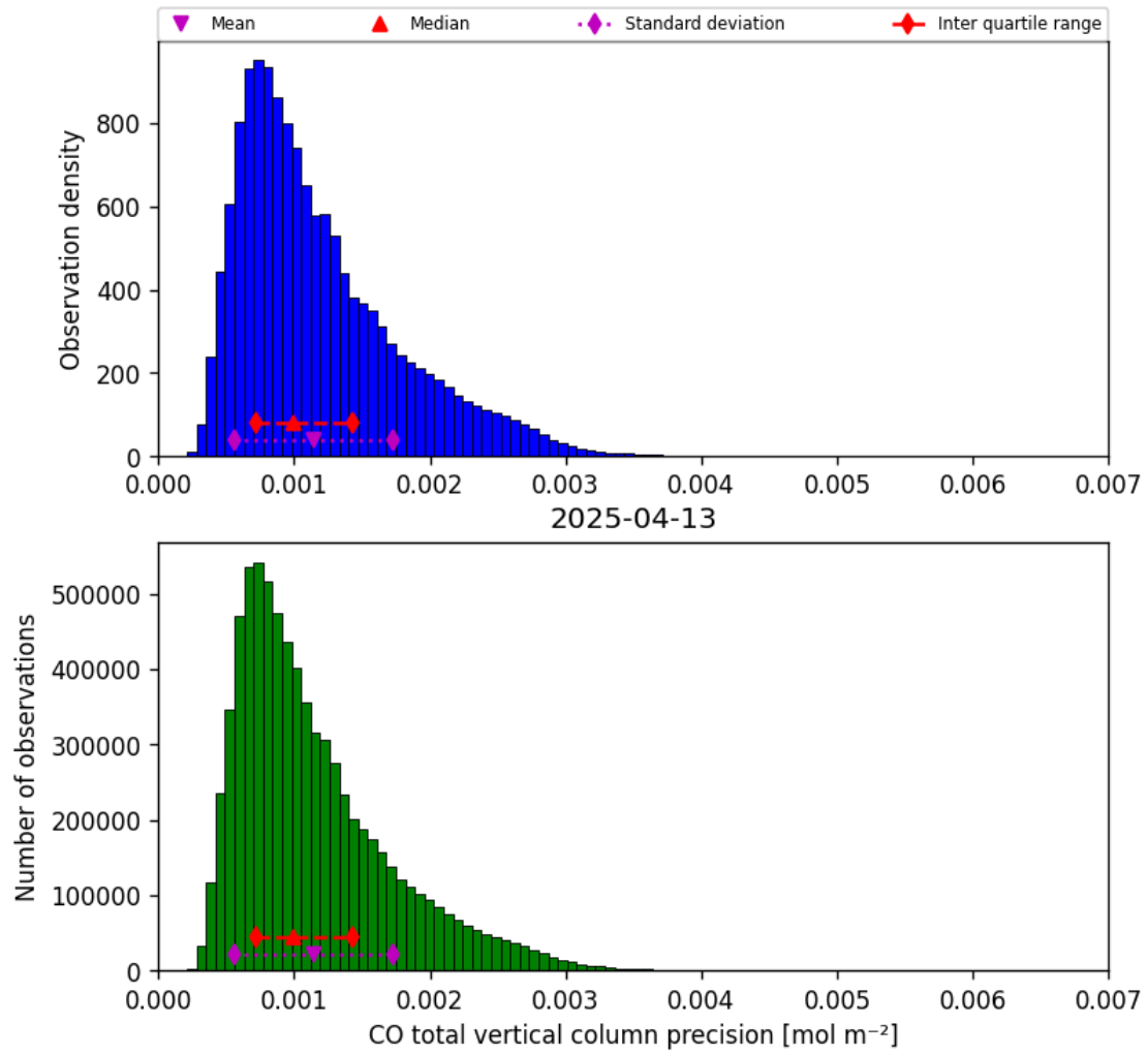
Figure 20: Histogram of “CO total vertical column precision” for 2025-04-13 to 2025-04-14
