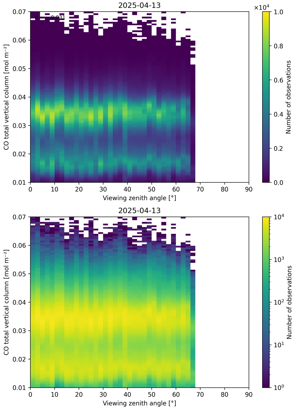
Figure 69: Scatter density plot of “Viewing zenith angle” against “CO total vertical column” for 2025-04-13 to 2025-04-14.
