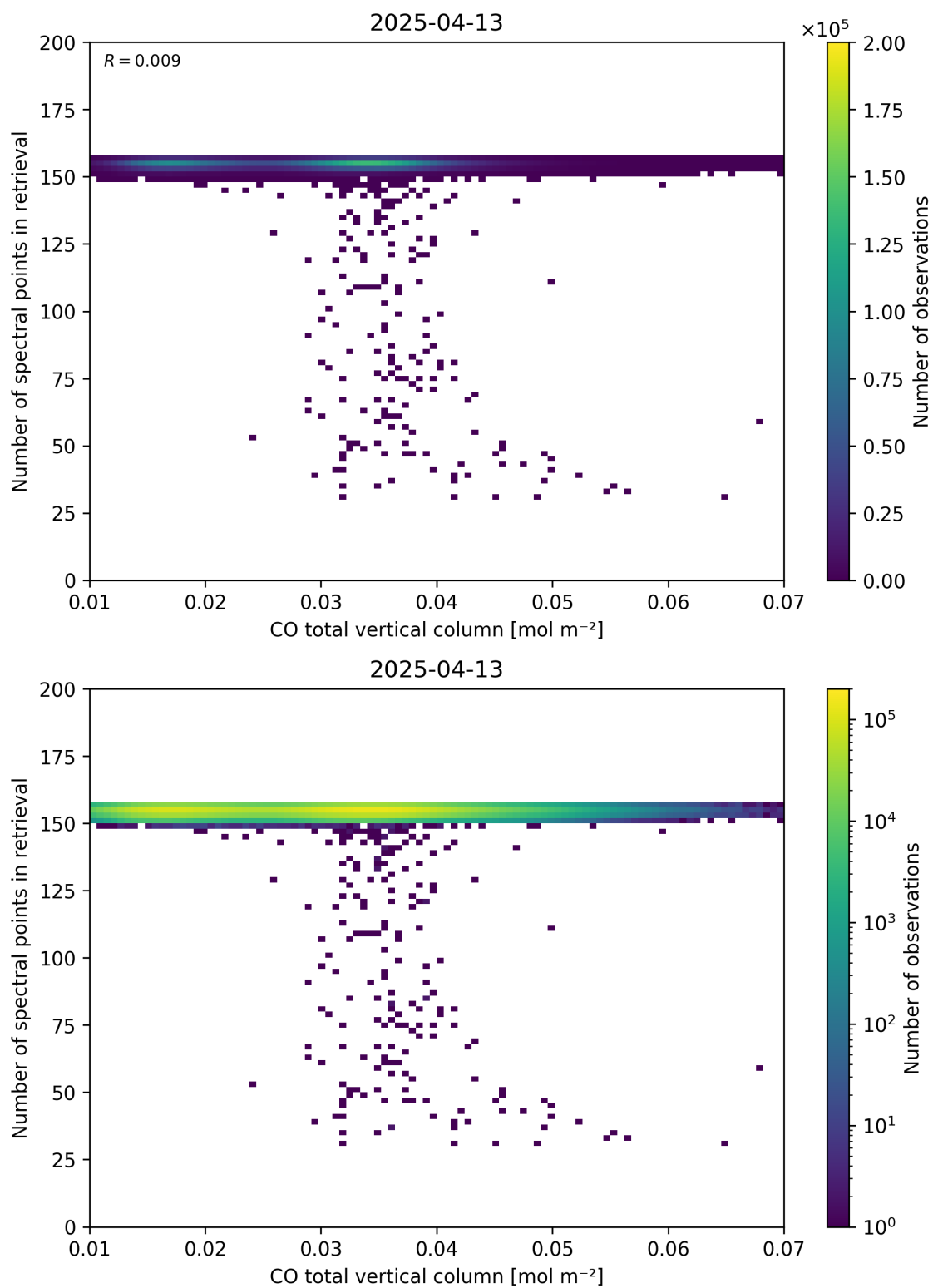
Figure 43: Scatter density plot of “CO total vertical column” against “Number of spectral points in retrieval” for 2025-04-13 to 2025-04-14.
