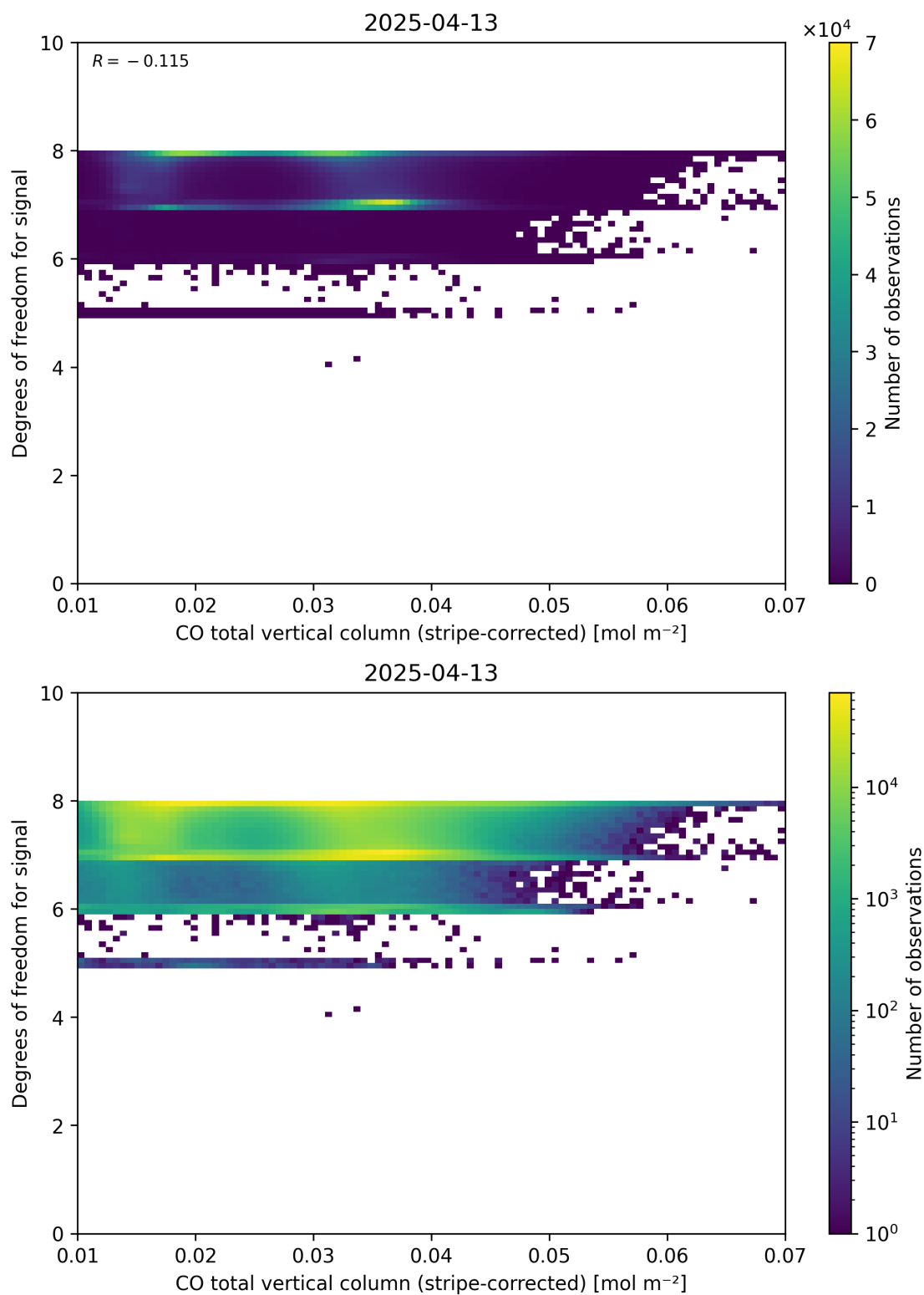
Figure 38: Scatter density plot of “CO total vertical column (stripe-corrected)” against “Degrees of freedom for signal” for 2025-04-13 to 2025-04-14.
