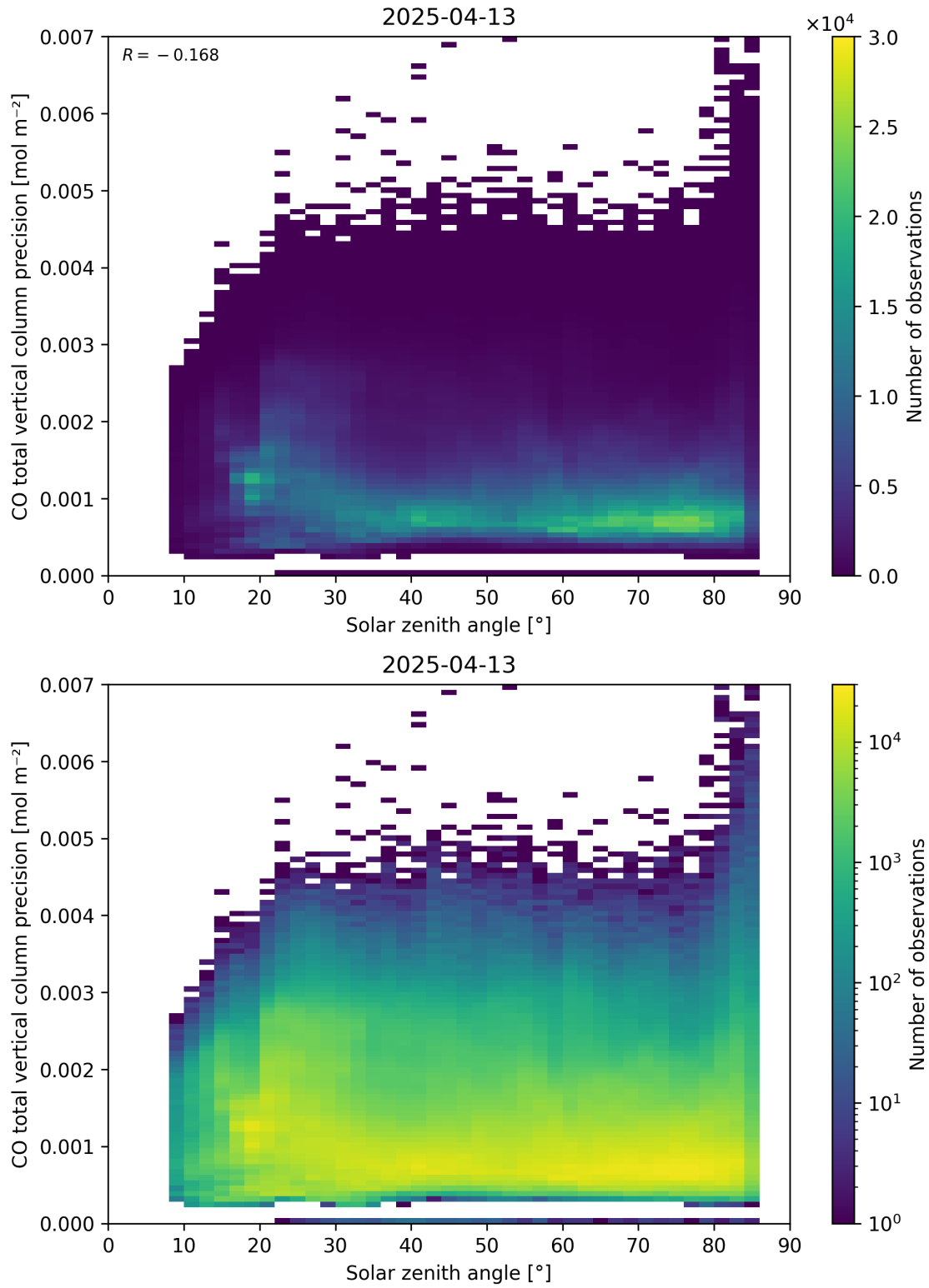
Figure 63: Scatter density plot of “Solar zenith angle” against “CO total vertical column precision” for 2025-04-13 to 2025-04-14.
