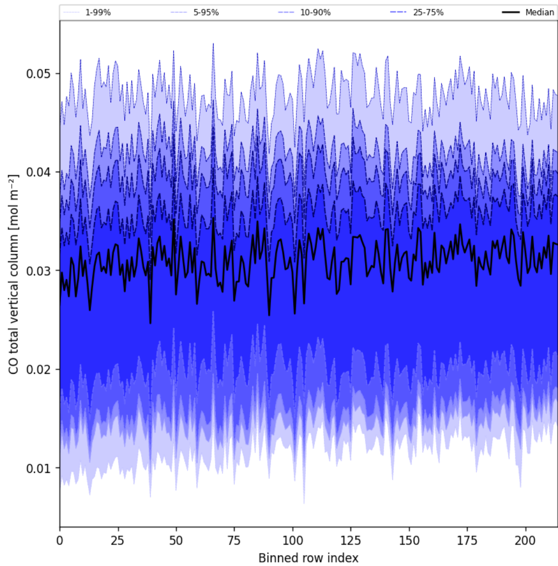
Figure 26: Along track statistics of “CO total vertical column” for 2025-04-13 to 2025-04-14
