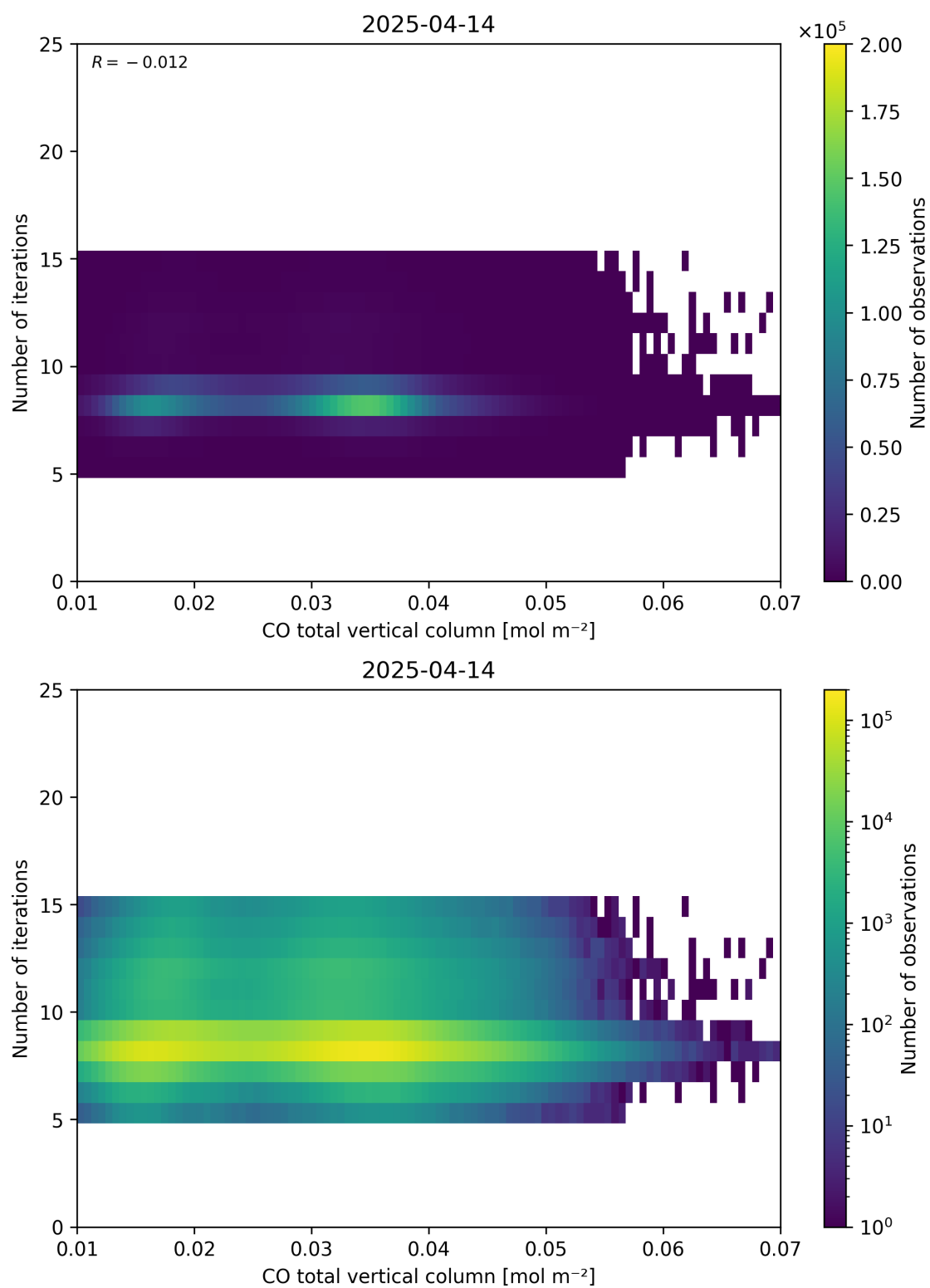
Figure 42: Scatter density plot of “CO total vertical column” against “Number of iterations” for 2025-04-13 to 2025-04-15.
