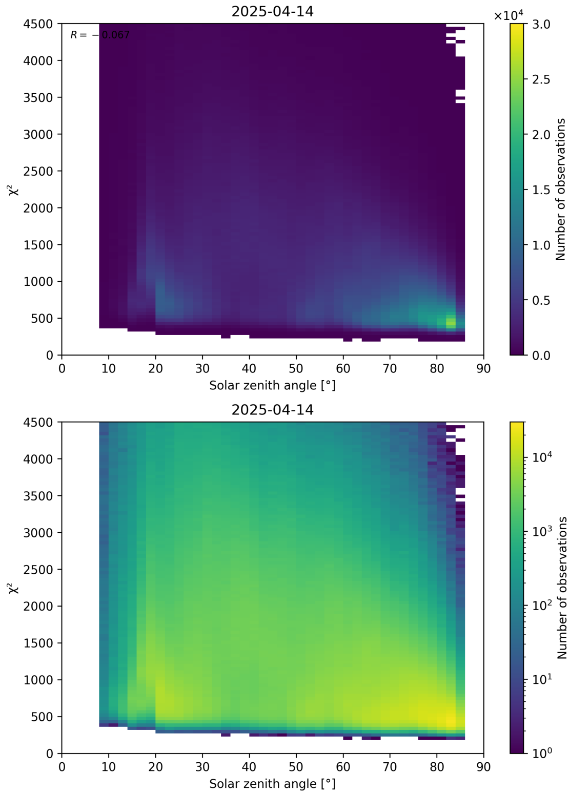
Figure 64: Scatter density plot of “Solar zenith angle” against “ \chi^2 ” for 2025-04-13 to 2025-04-15.
