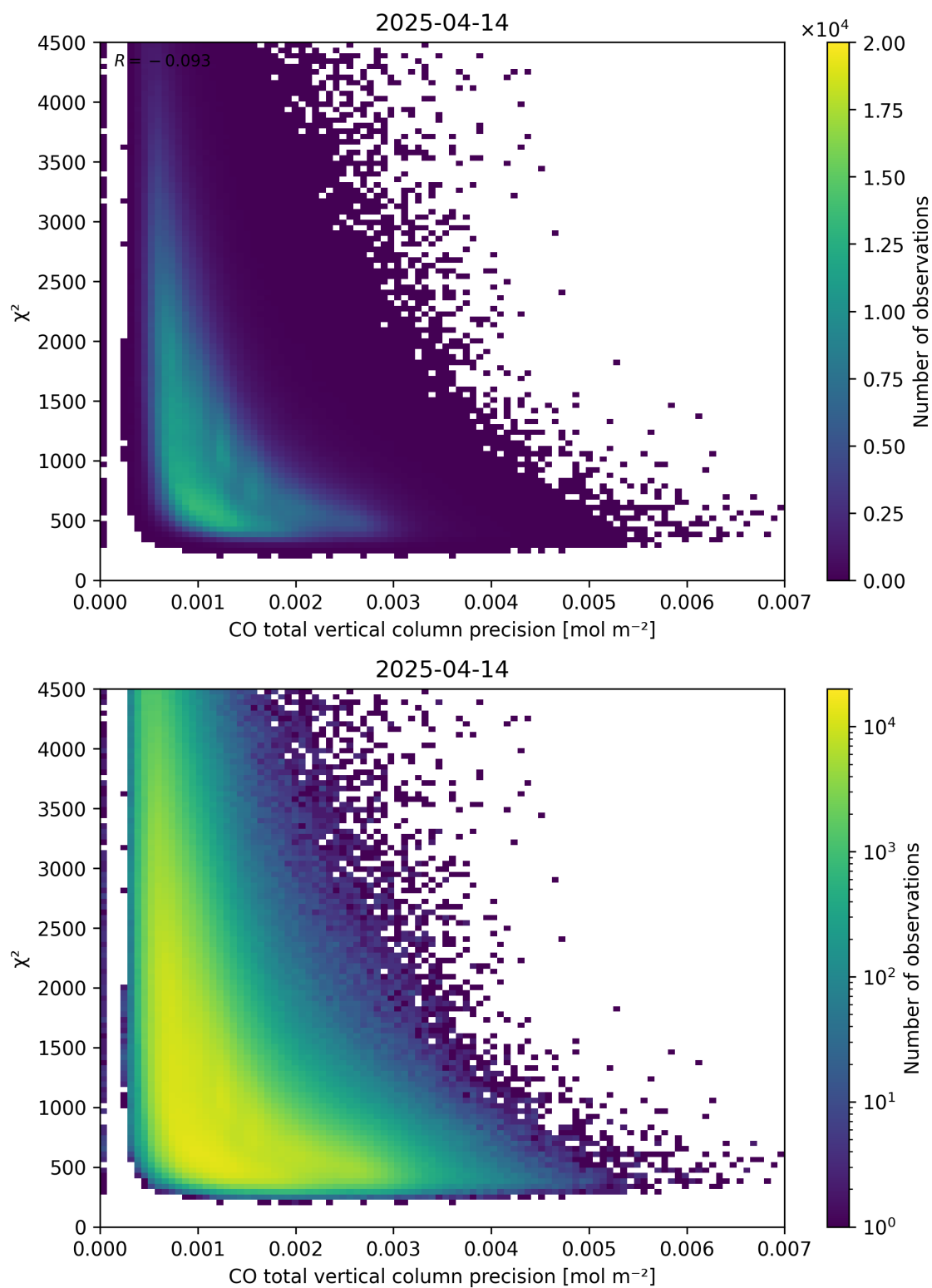
Figure 44: Scatter density plot of “CO total vertical column precision” against “ \chi^2 ” for 2025-04-13 to 2025-04-15.
