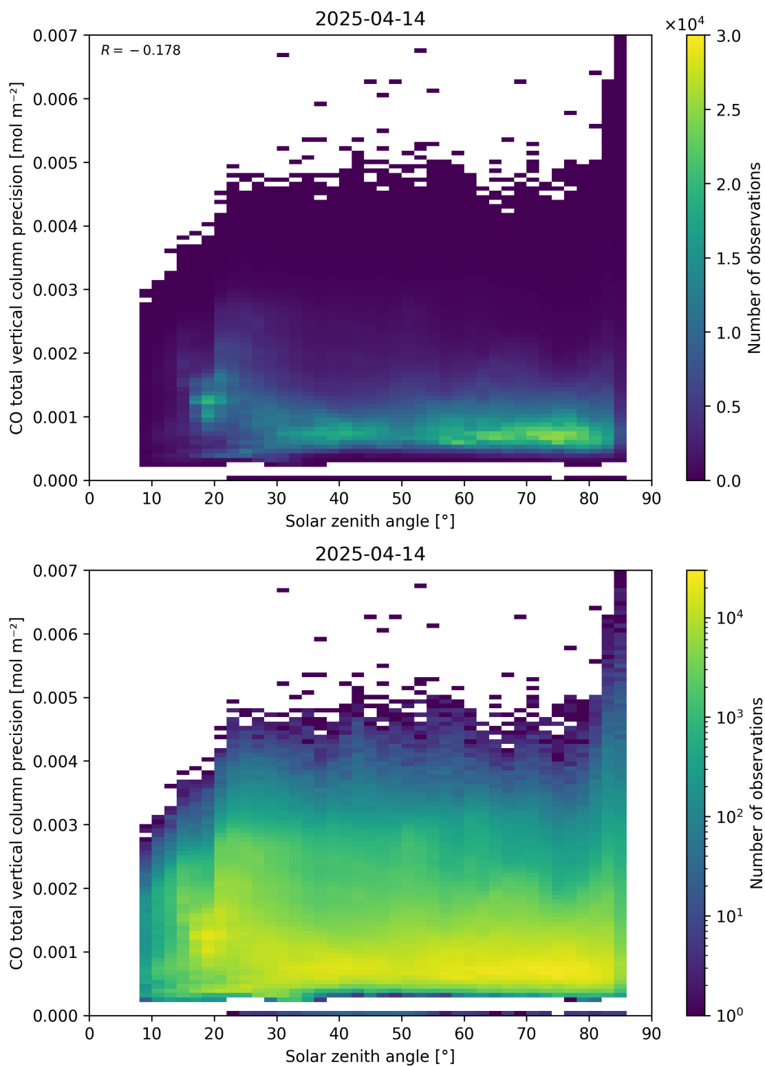
Figure 63: Scatter density plot of “Solar zenith angle” against “CO total vertical column precision” for 2025-04-13 to 2025-04-15.
