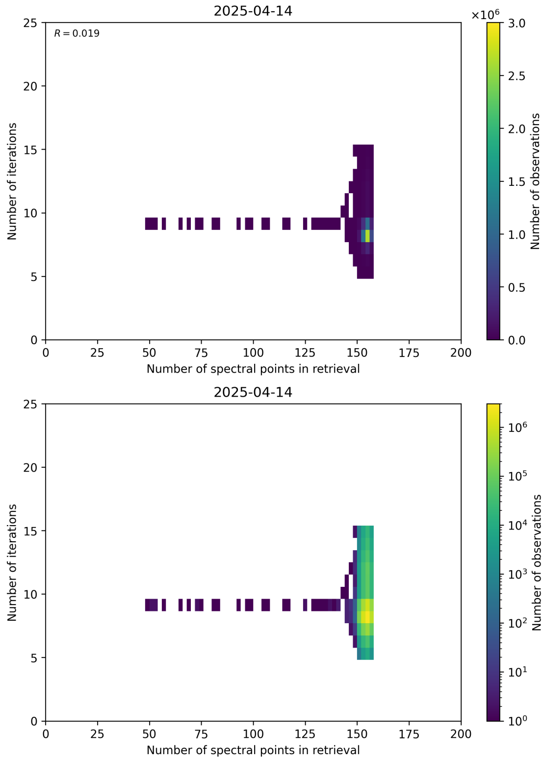
Figure 60: Scatter density plot of “Number of spectral points in retrieval” against “Number of iterations” for 2025-04-13 to 2025-04-15.
