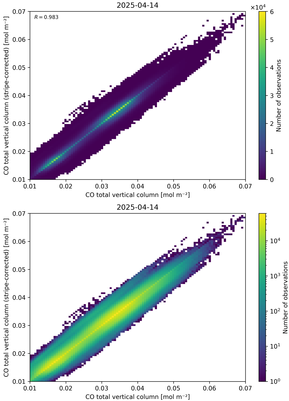
Figure 33: Scatter density plot of “CO total vertical column” against “CO total vertical column (stripe-corrected)” for 2025-04-13 to 2025-04-15.
