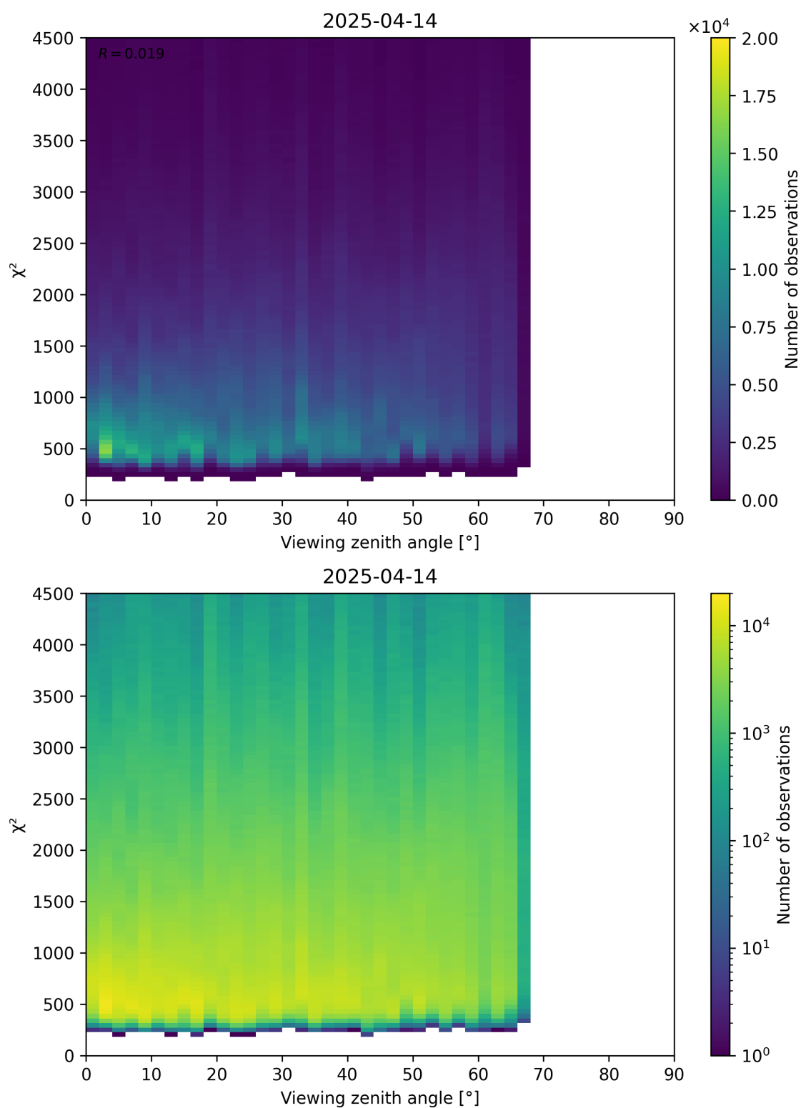
Figure 72: Scatter density plot of “Viewing zenith angle” against “ \chi^2 ” for 2025-04-13 to 2025-04-15.
