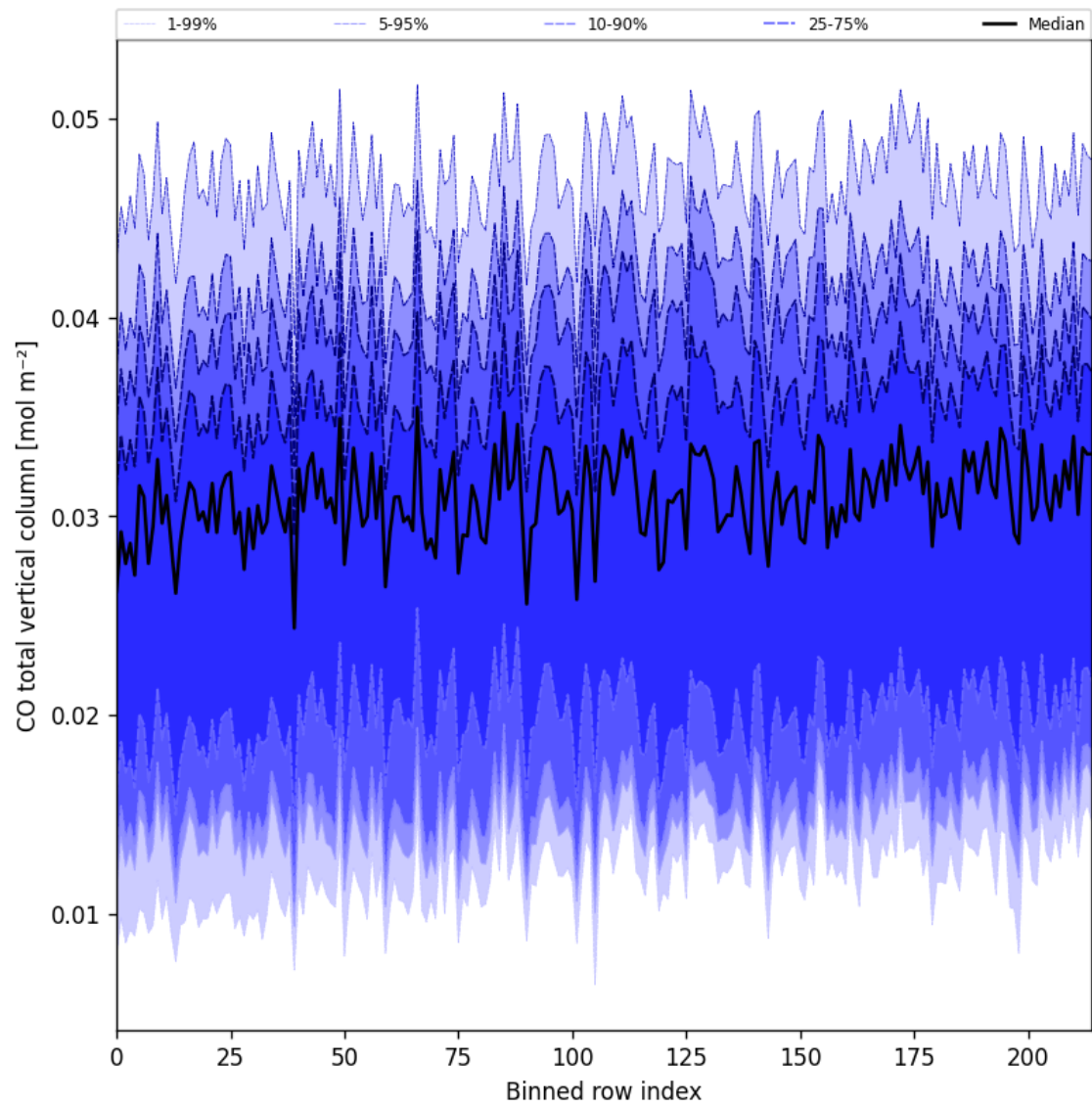
Figure 26: Along track statistics of "CO total vertical column" for 2025-04-13 to 2025-04-15
