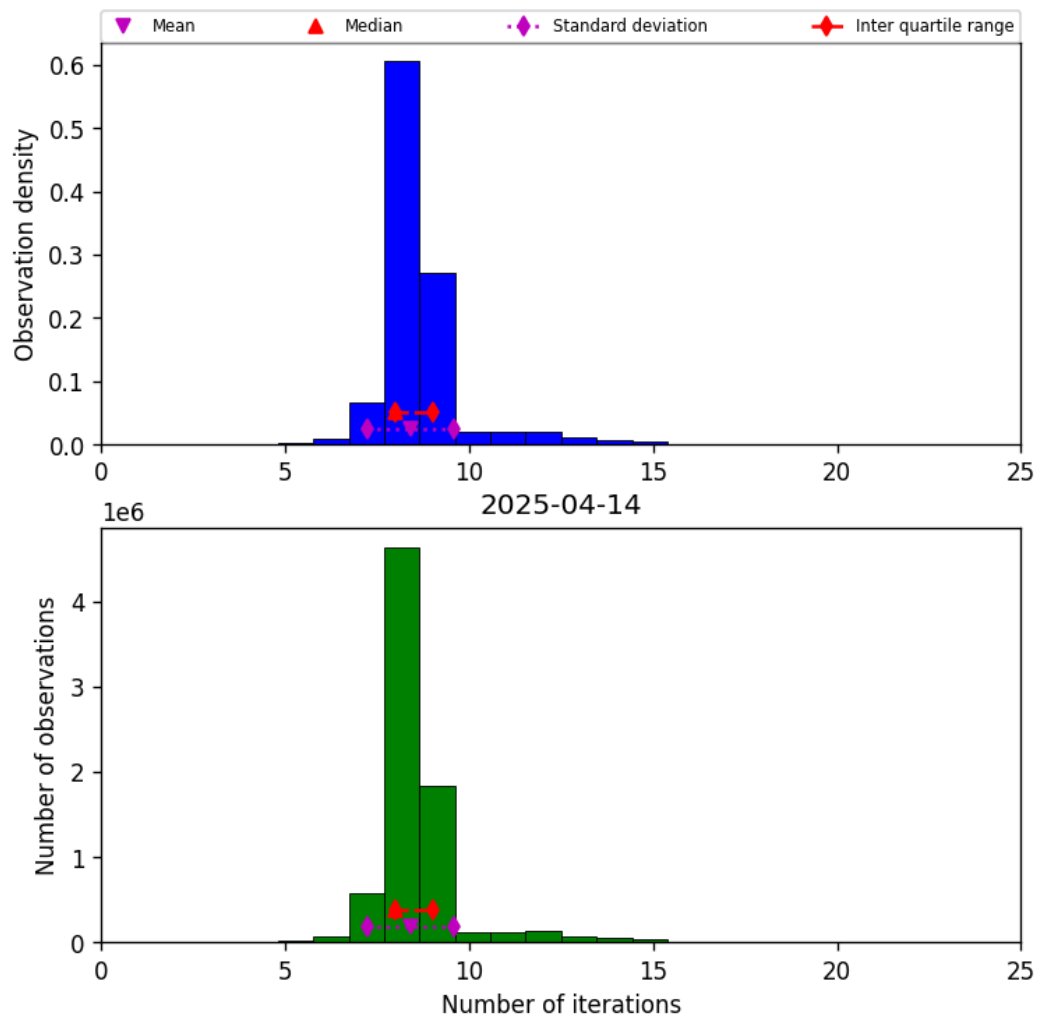
Figure 24: Histogram of “Number of iterations” for 2025-04-13 to 2025-04-15
