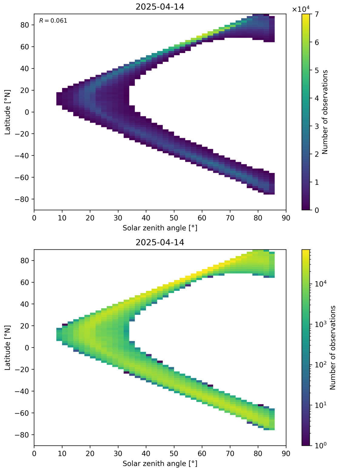
Figure 66: Scatter density plot of “Solar zenith angle” against “Latitude” for 2025-04-13 to 2025-04-15.
