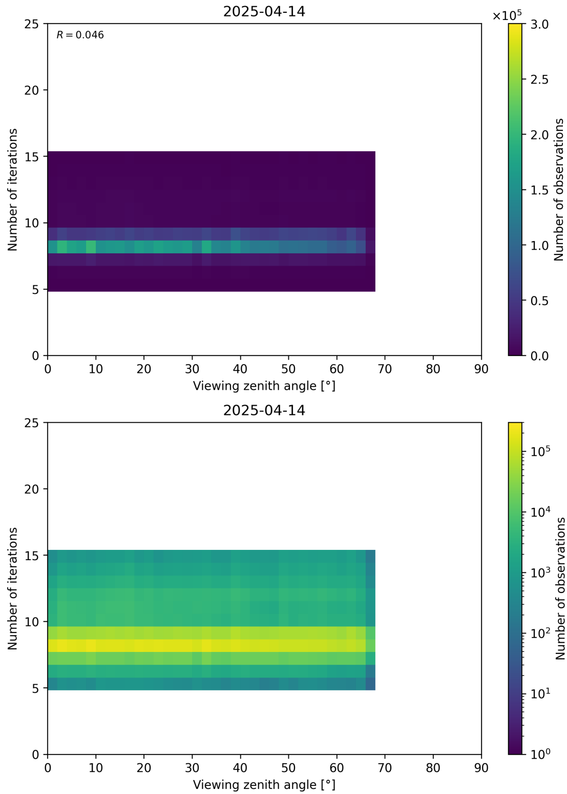
Figure 75: Scatter density plot of “Viewing zenith angle” against “Number of iterations” for 2025-04-13 to 2025-04-15.
