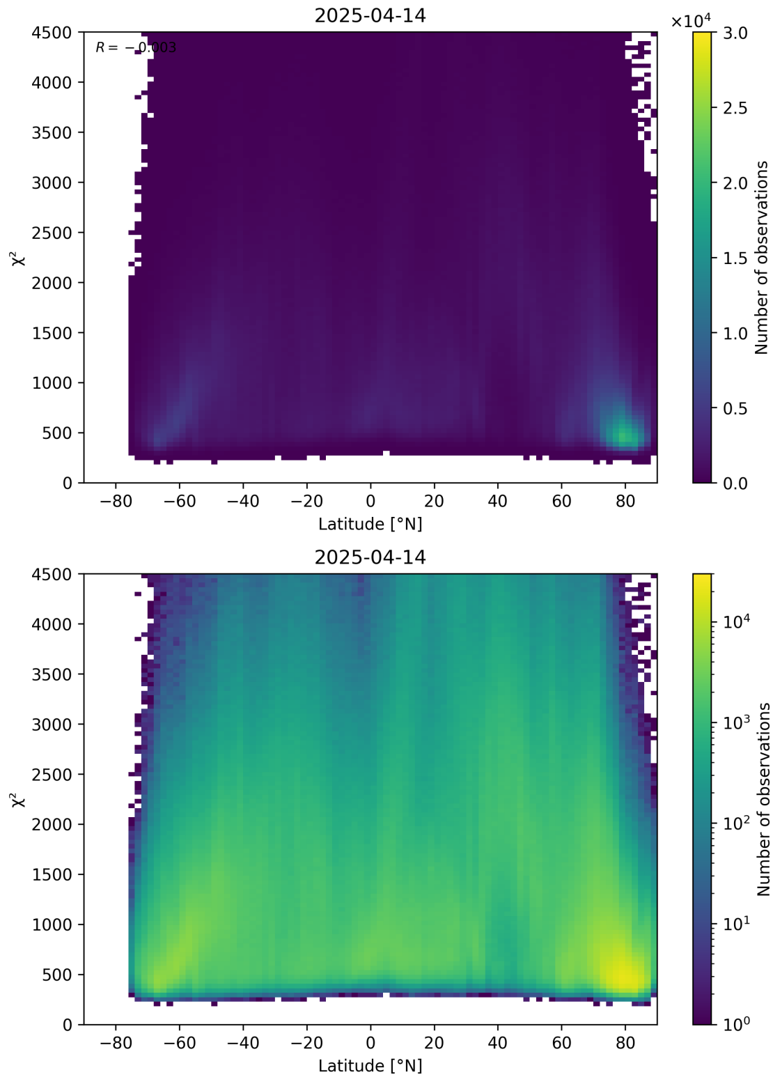
Figure 54: Scatter density plot of “Latitude” against “ \chi^2 ” for 2025-04-13 to 2025-04-15.
