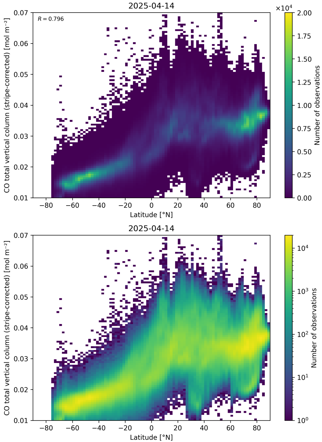
Figure 52: Scatter density plot of “Latitude” against “CO total vertical column (stripe-corrected)” for 2025-04-13 to 2025-04-15.
