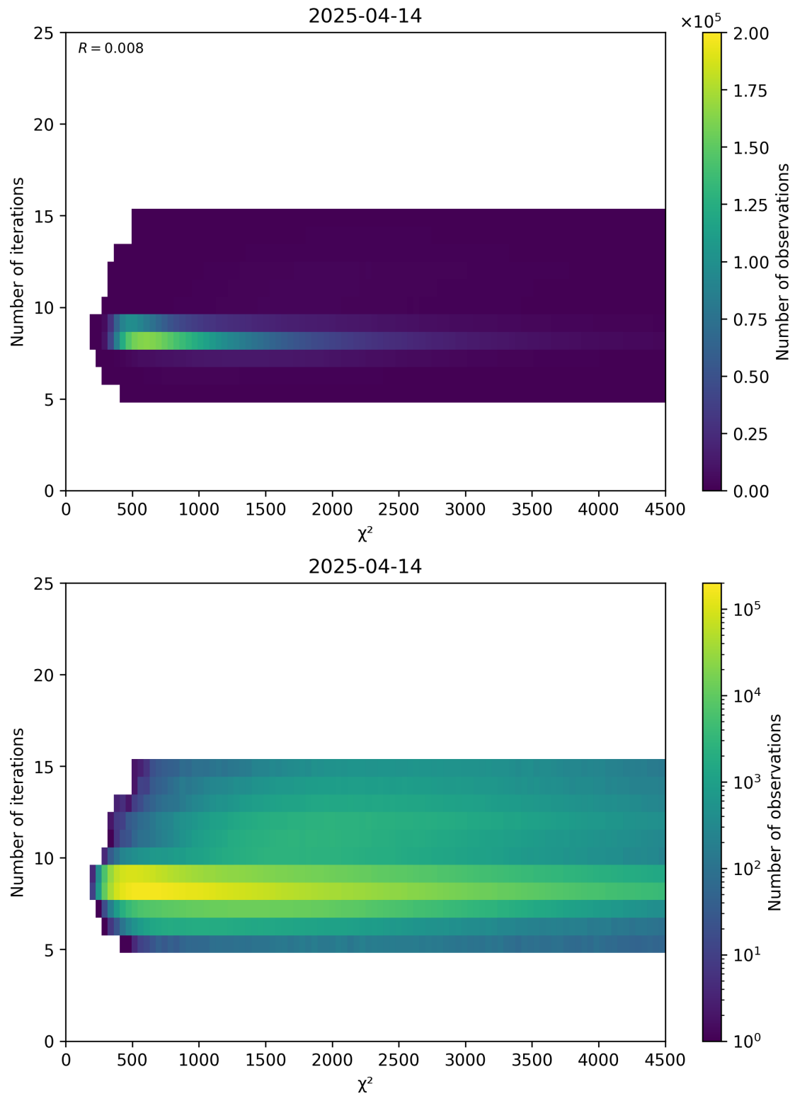
Figure 49: Scatter density plot of “ \chi^2 ” against “Number of iterations” for 2025-04-13 to 2025-04-15.
