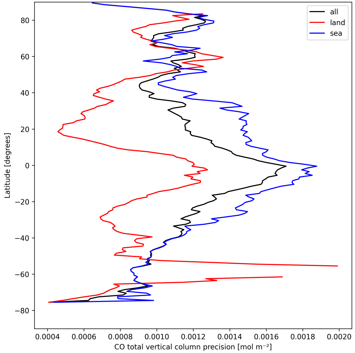
Figure 12: Zonal average of “CO total vertical column precision” for 2025-04-13 to 2025-04-15.
