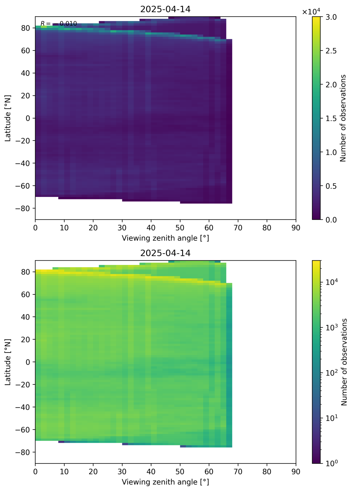
Figure 74: Scatter density plot of “Viewing zenith angle” against “Latitude” for 2025-04-13 to 2025-04-15.
