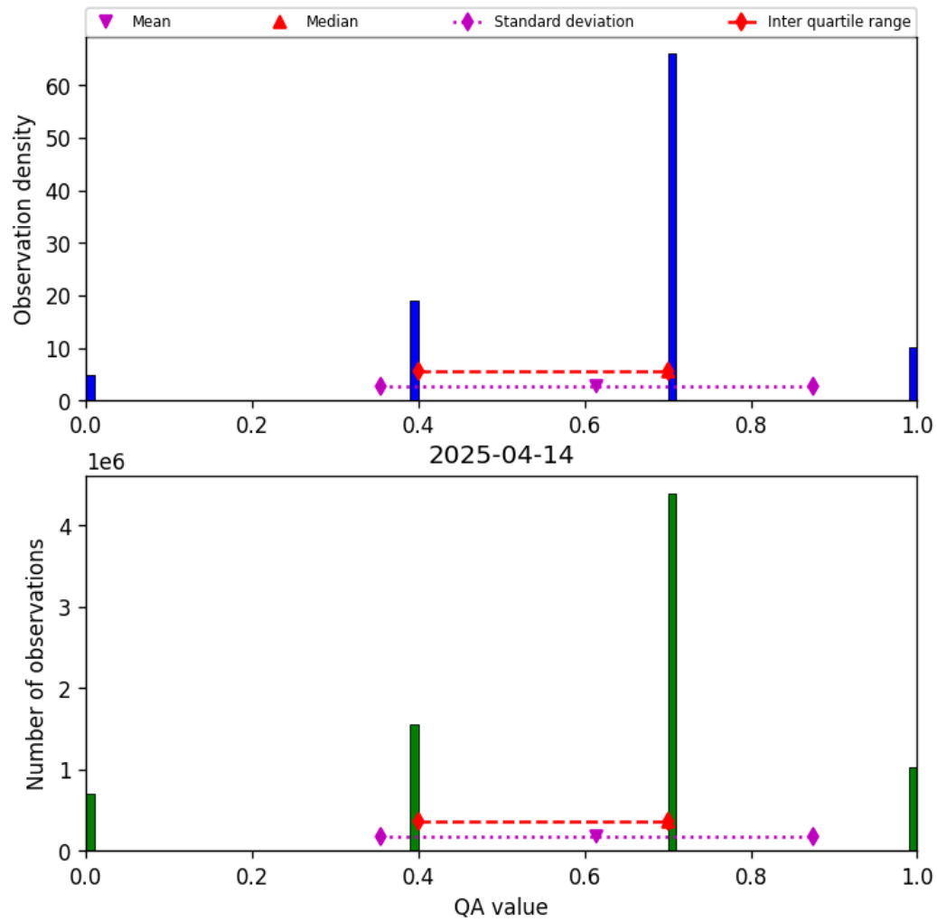
Figure 17: Histogram of “QA value” for 2025-04-13 to 2025-04-15
