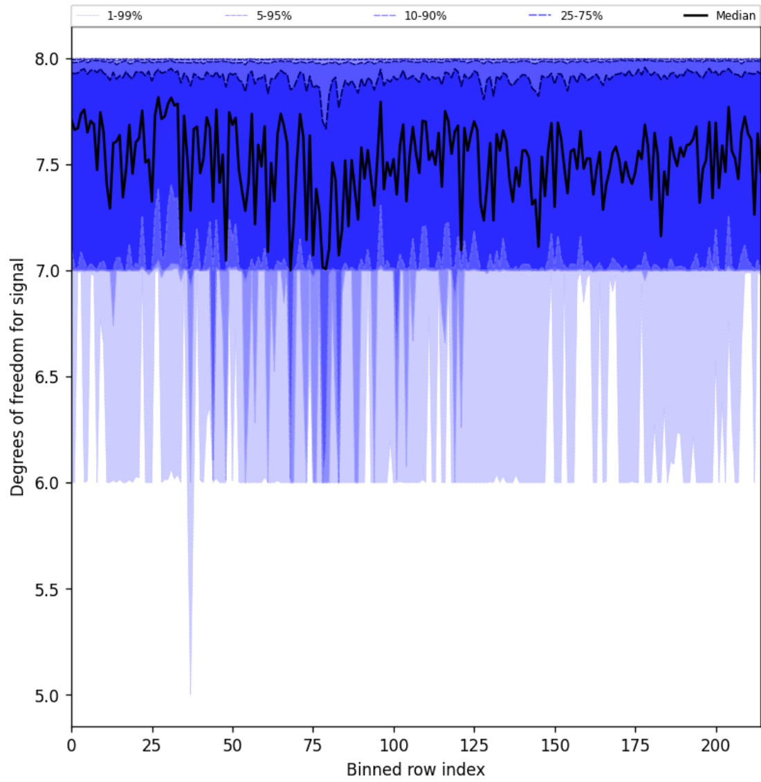
Figure 31: Along track statistics of “Degrees of freedom for signal” for 2025-04-13 to 2025-04-15
