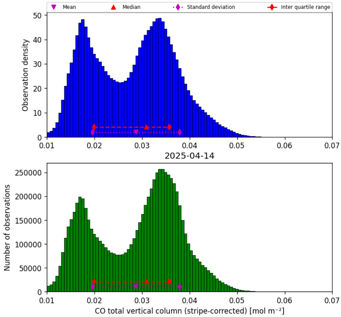
Figure 19: Histogram of “CO total vertical column (stripe-corrected)” for 2025-04-13 to 2025-04-15
