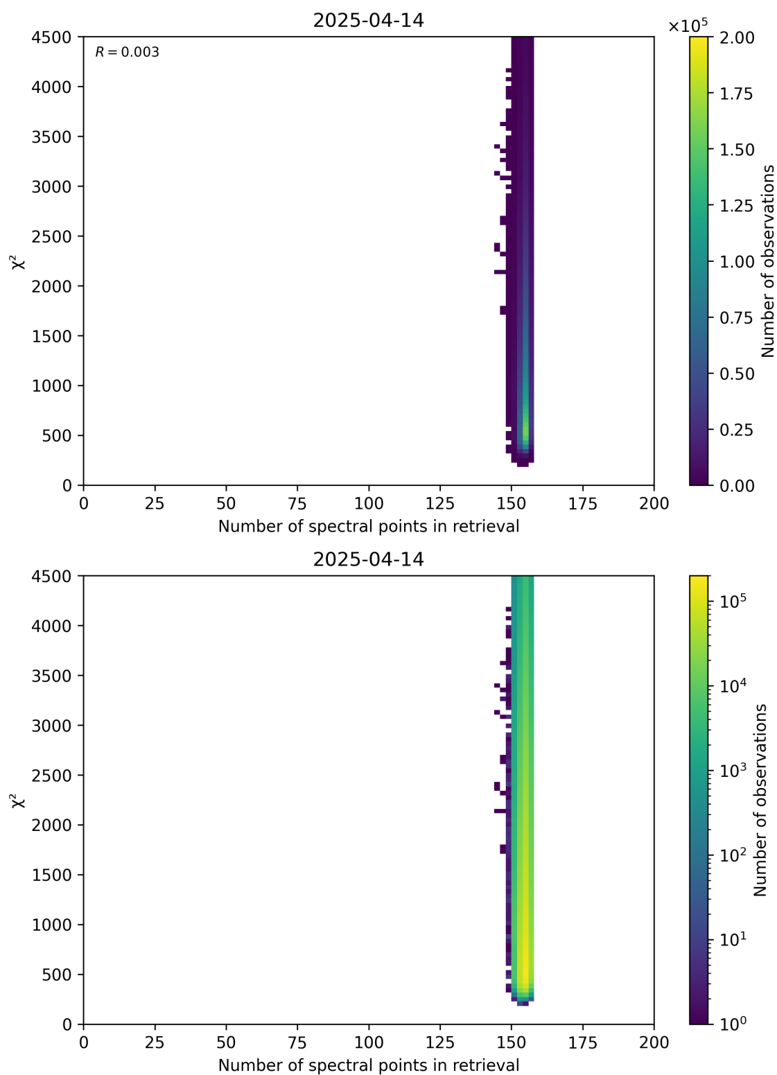
Figure 58: Scatter density plot of “Number of spectral points in retrieval” against “ \chi^2 ” for 2025-04-13 to 2025-04-15.
