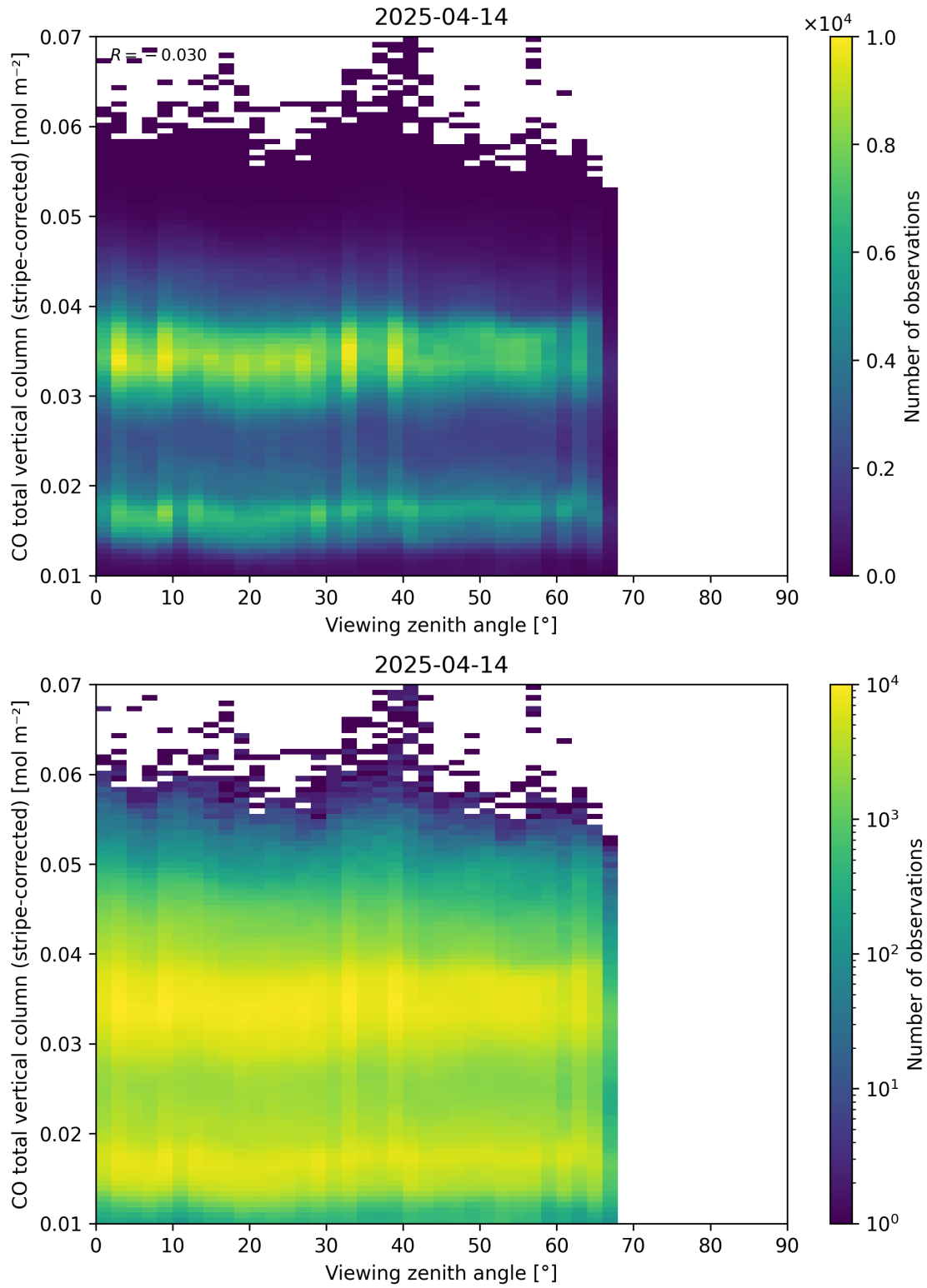
Figure 70: Scatter density plot of “Viewing zenith angle” against “CO total vertical column (stripe-corrected)” for 2025-04-13 to 2025-04-15.
