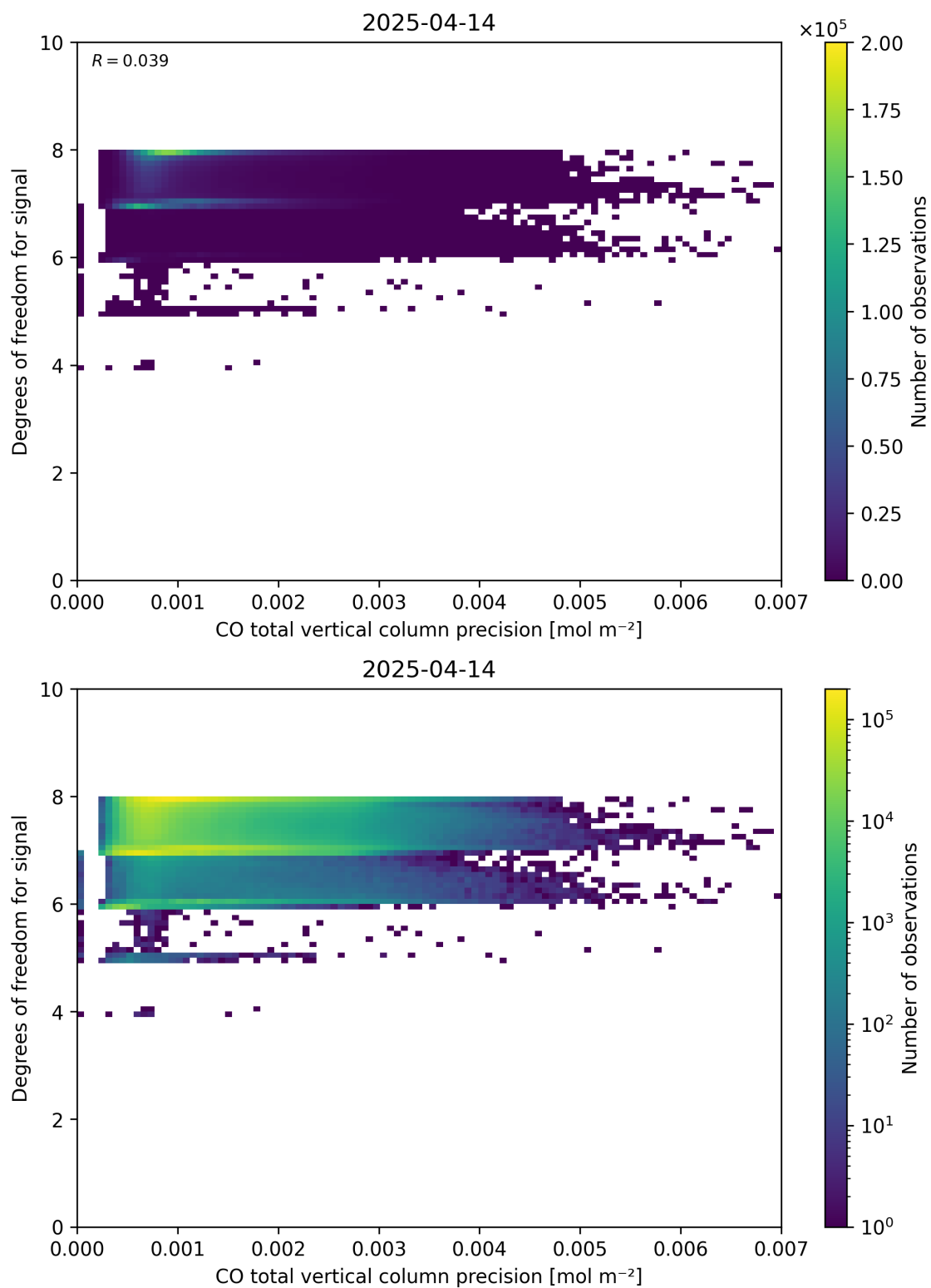
Figure 45: Scatter density plot of “CO total vertical column precision” against “Degrees of freedom for signal” for 2025-04-13 to 2025-04-15.
