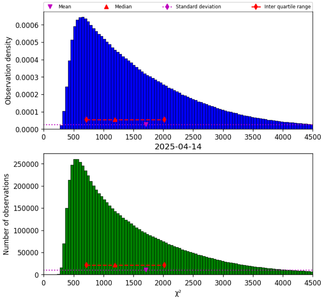
Figure 22: Histogram of “ \chi^2 ” for 2025-04-13 to 2025-04-15
