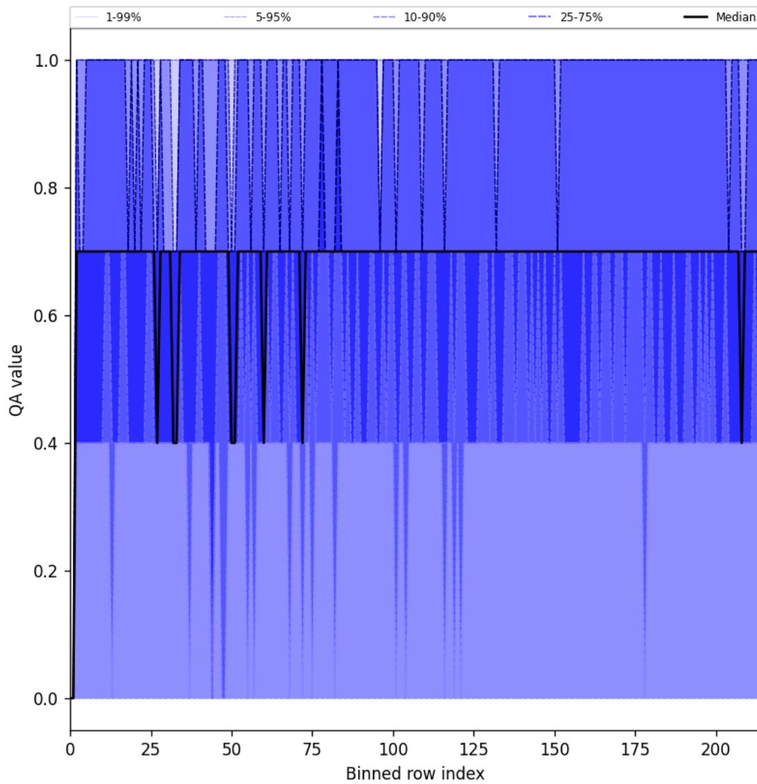
Figure 25: Along track statistics of “QA value” for 2025-04-13 to 2025-04-15
