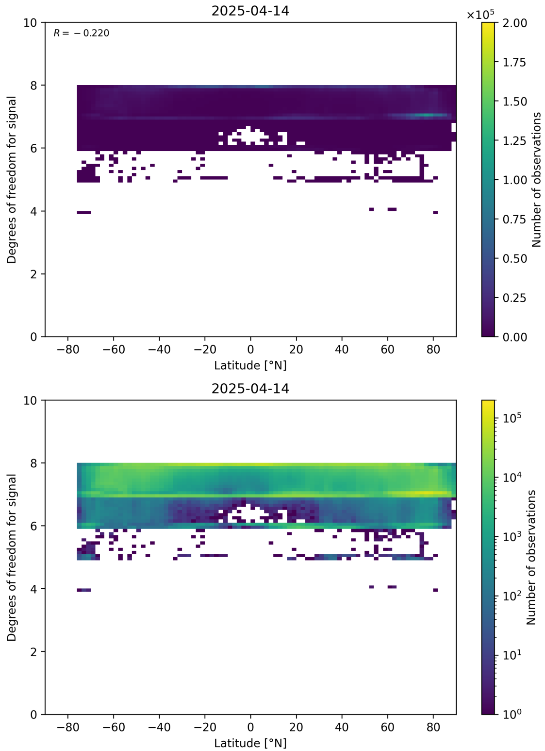
Figure 55: Scatter density plot of “Latitude” against “Degrees of freedom for signal” for 2025-04-13 to 2025-04-15.
