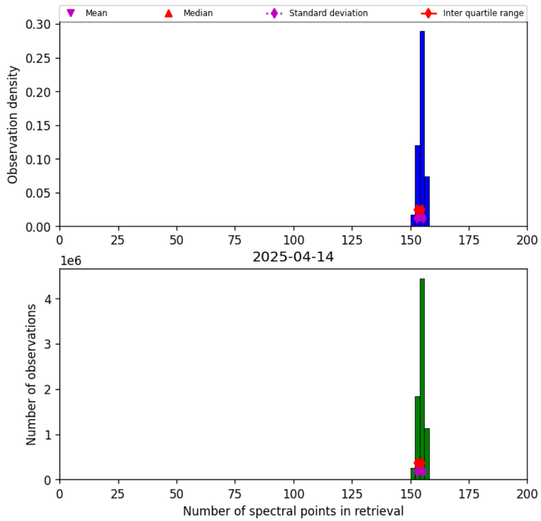
Figure 21: Histogram of “Number of spectral points in retrieval” for 2025-04-13 to 2025-04-15
