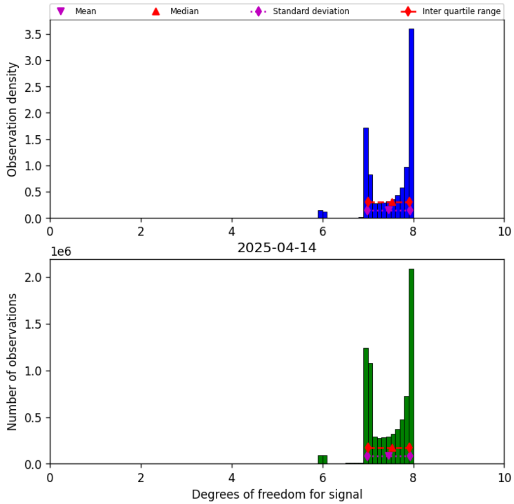
Figure 23: Histogram of “Degrees of freedom for signal” for 2025-04-13 to 2025-04-15
