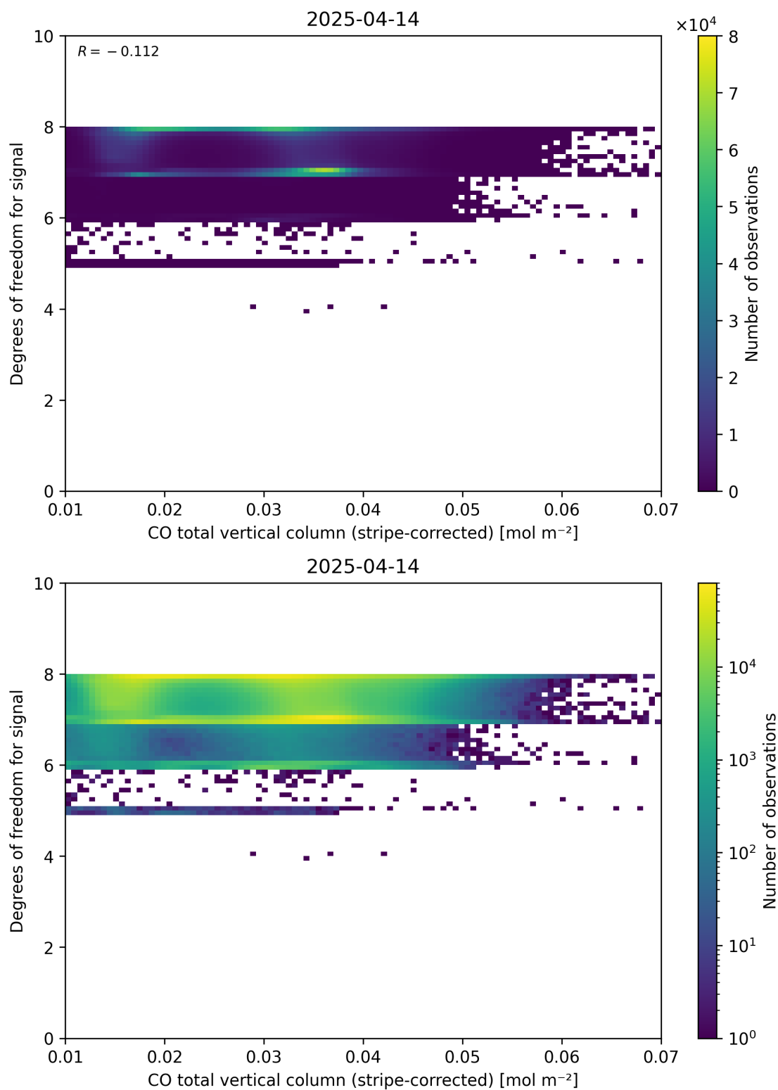
Figure 38: Scatter density plot of “CO total vertical column (stripe-corrected)” against “Degrees of freedom for signal” for 2025-04-13 to 2025-04-15.
