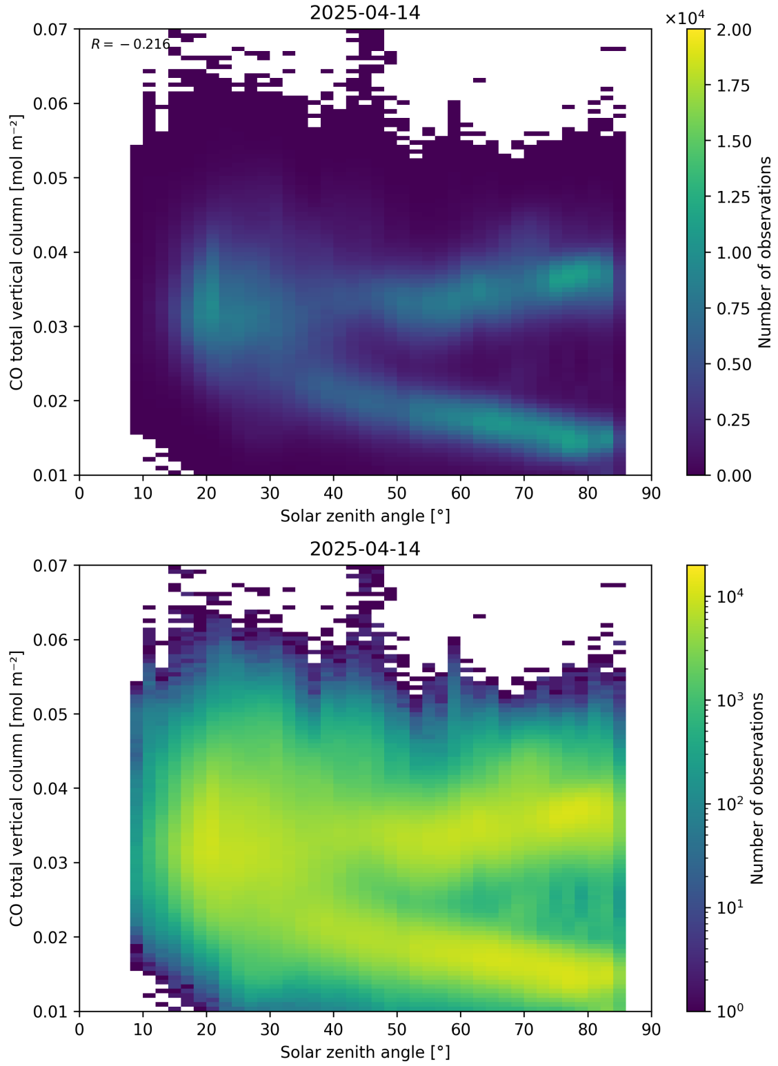
Figure 61: Scatter density plot of “Solar zenith angle” against “CO total vertical column” for 2025-04-13 to 2025-04-15.
