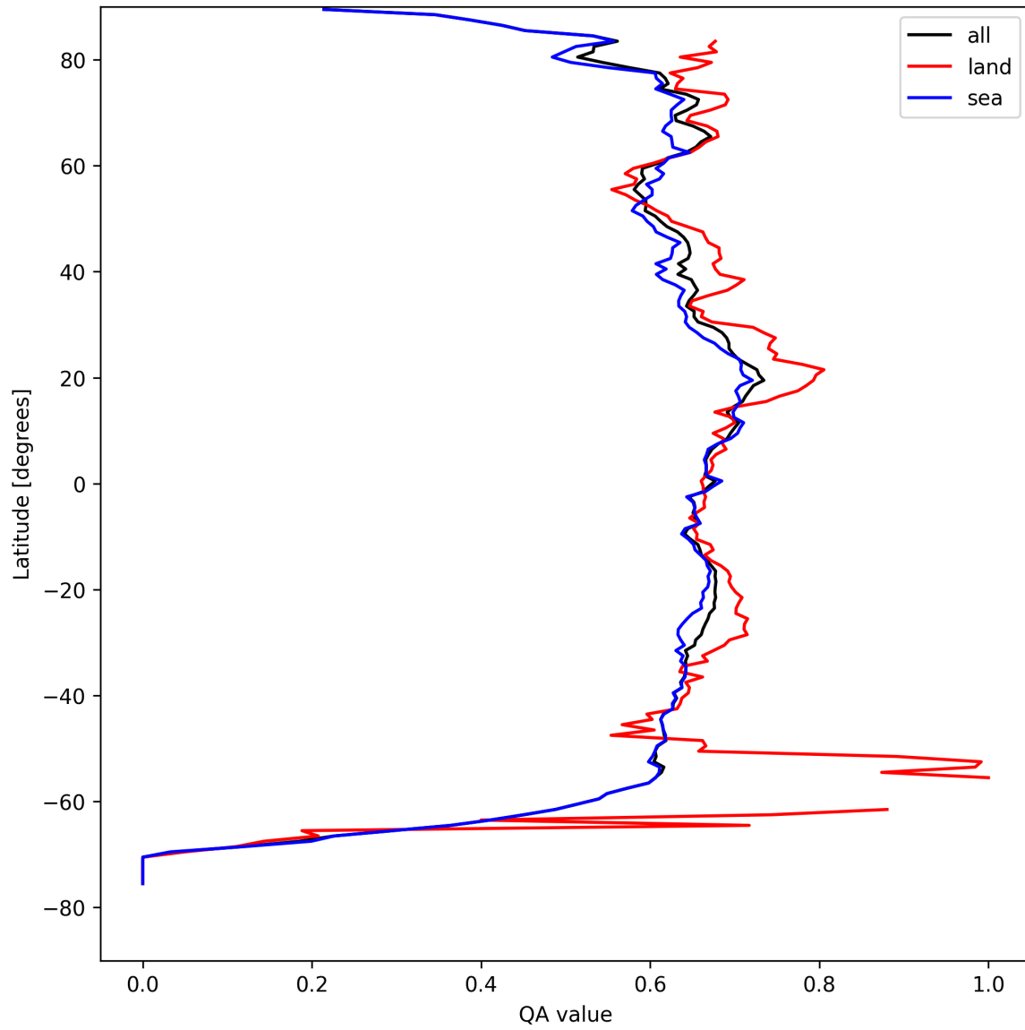
Figure 9: Zonal average of “QA value” for 2025-04-13 to 2025-04-15.
