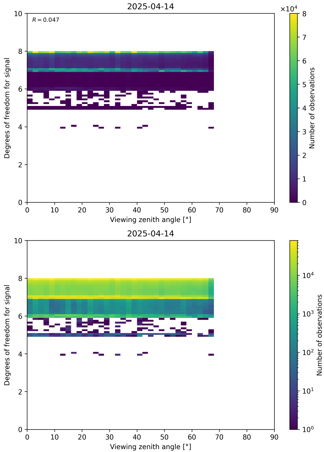
Figure 73: Scatter density plot of “Viewing zenith angle” against “Degrees of freedom for signal” for 2025-04-13 to 2025-04-15.
