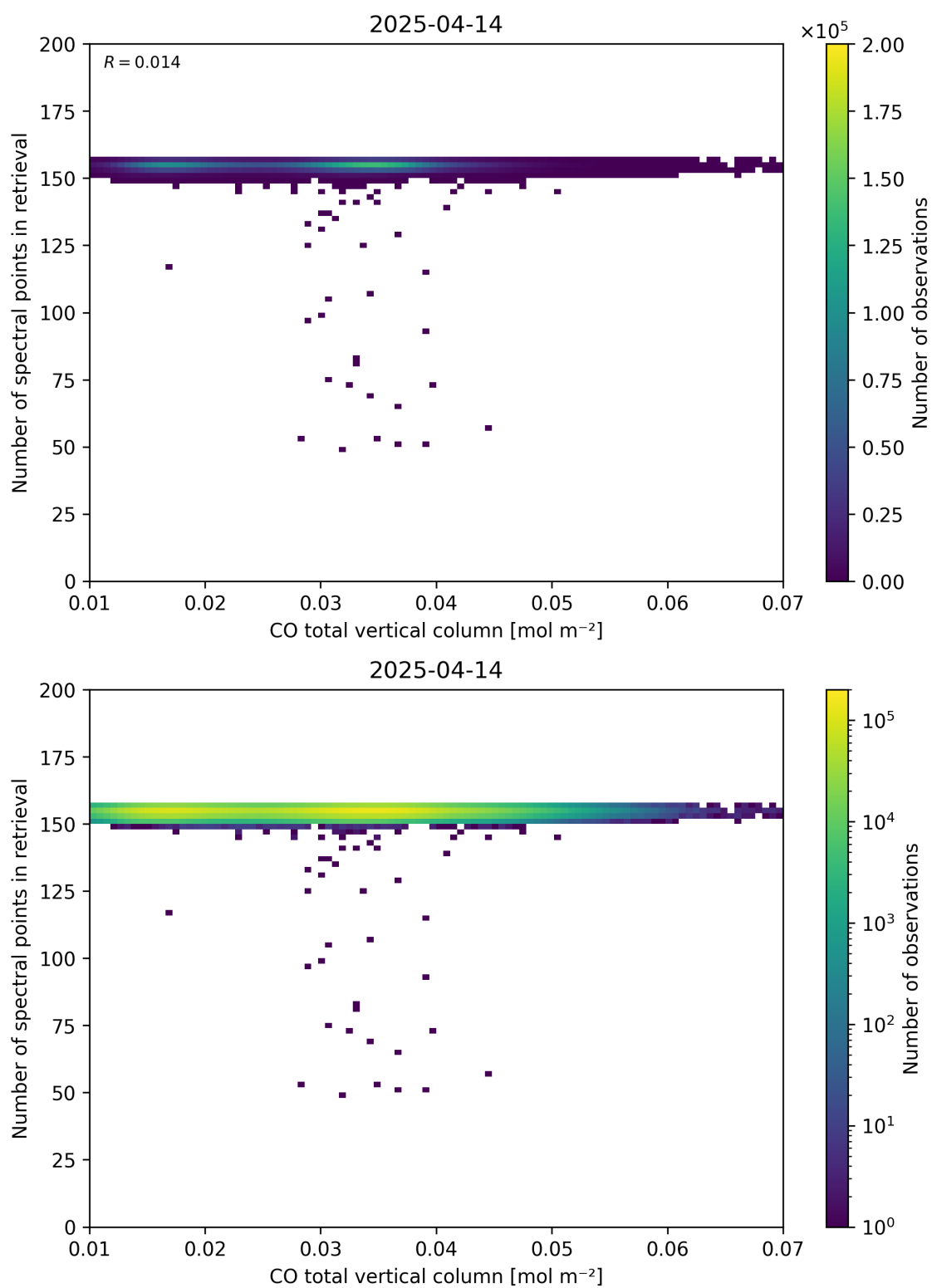
Figure 43: Scatter density plot of “CO total vertical column” against “Number of spectral points in retrieval” for 2025-04-13 to 2025-04-15.
