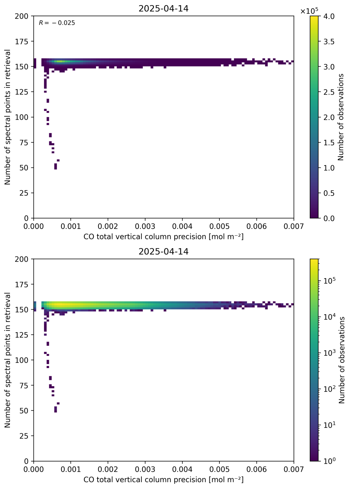
Figure 47: Scatter density plot of “CO total vertical column precision” against “Number of spectral points in retrieval” for 2025-04-13 to 2025-04-15.
