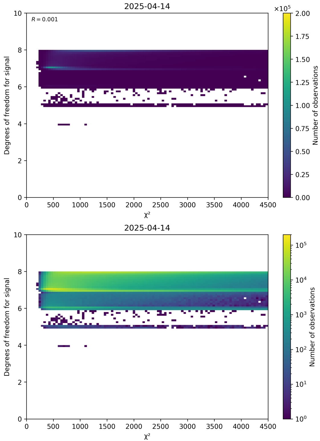
Figure 48: Scatter density plot of " \chi^2 " against "Degrees of freedom for signal" for 2025-04-13 to 2025-04-15.
