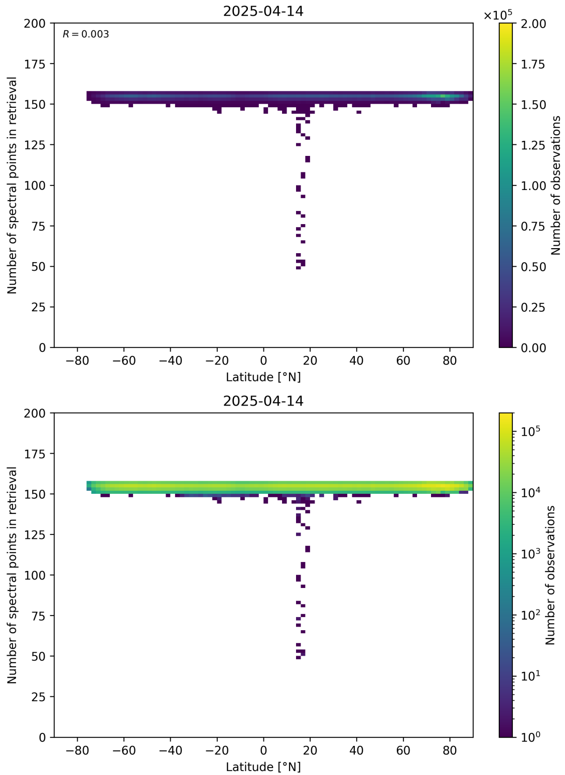
Figure 57: Scatter density plot of “Latitude” against “Number of spectral points in retrieval” for 2025-04-13 to 2025-04-15.
