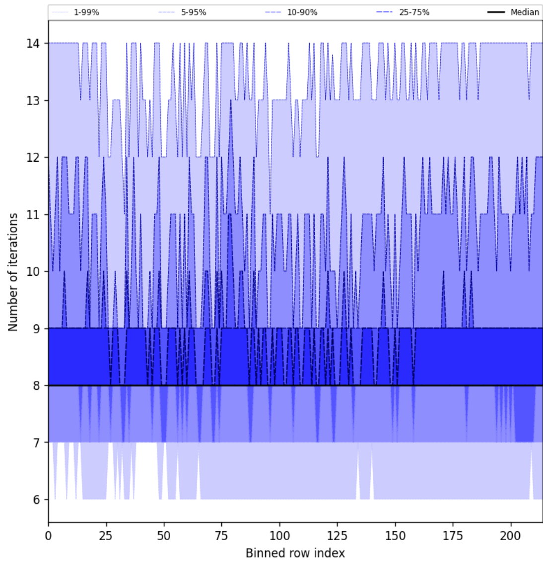
Figure 32: Along track statistics of “Number of iterations” for 2025-04-13 to 2025-04-15
