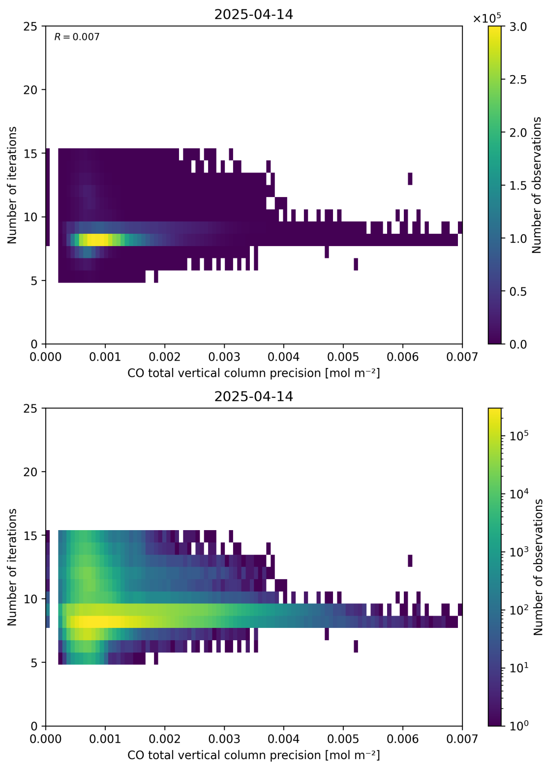
Figure 46: Scatter density plot of “CO total vertical column precision” against “Number of iterations” for 2025-04-13 to 2025-04-15.
