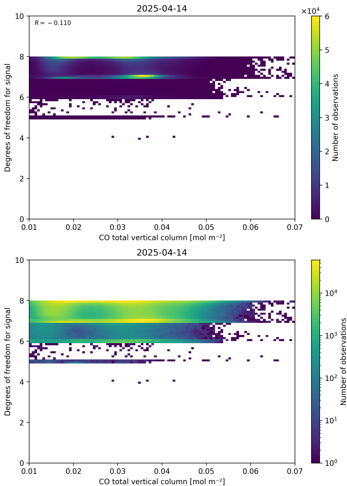
Figure 41: Scatter density plot of “CO total vertical column” against “Degrees of freedom for signal” for 2025-04-13 to 2025-04-15.
