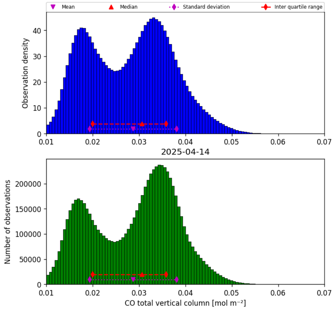
Figure 18: Histogram of “CO total vertical column” for 2025-04-13 to 2025-04-15
