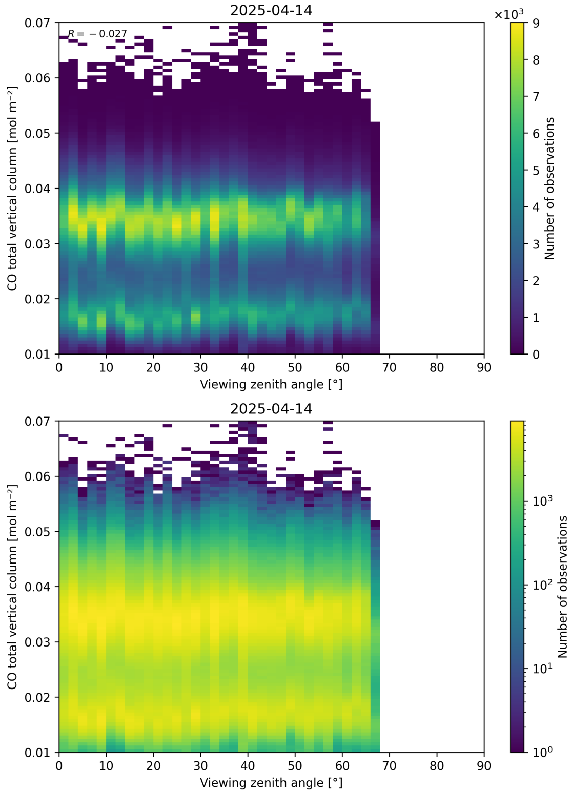
Figure 69: Scatter density plot of “Viewing zenith angle” against “CO total vertical column” for 2025-04-13 to 2025-04-15.
