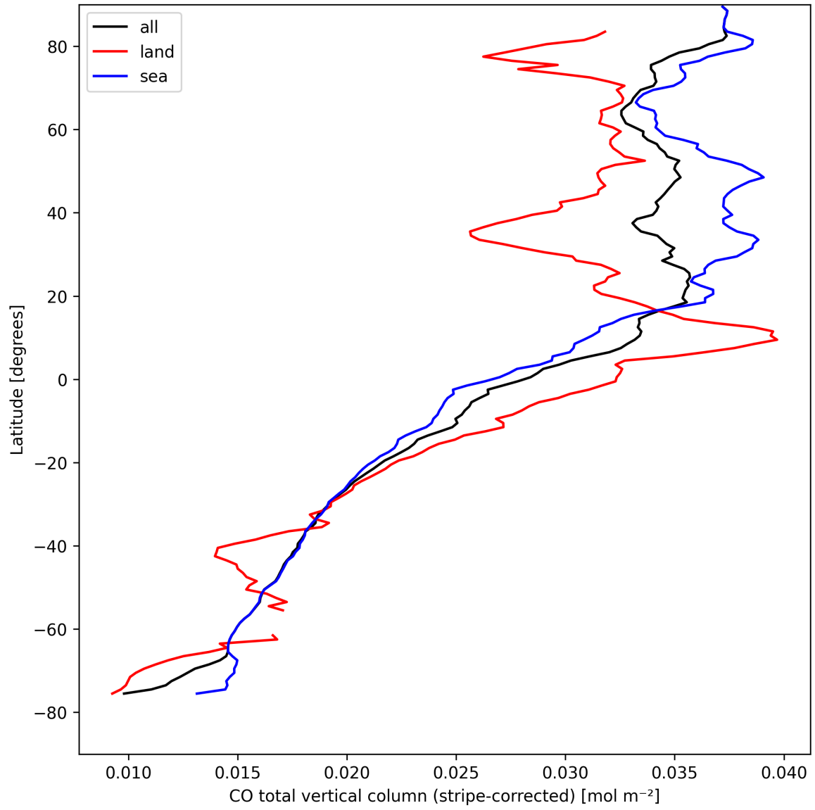
Figure 11: Zonal average of “CO total vertical column (stripe-corrected)” for 2025-04-13 to 2025-04-15.
