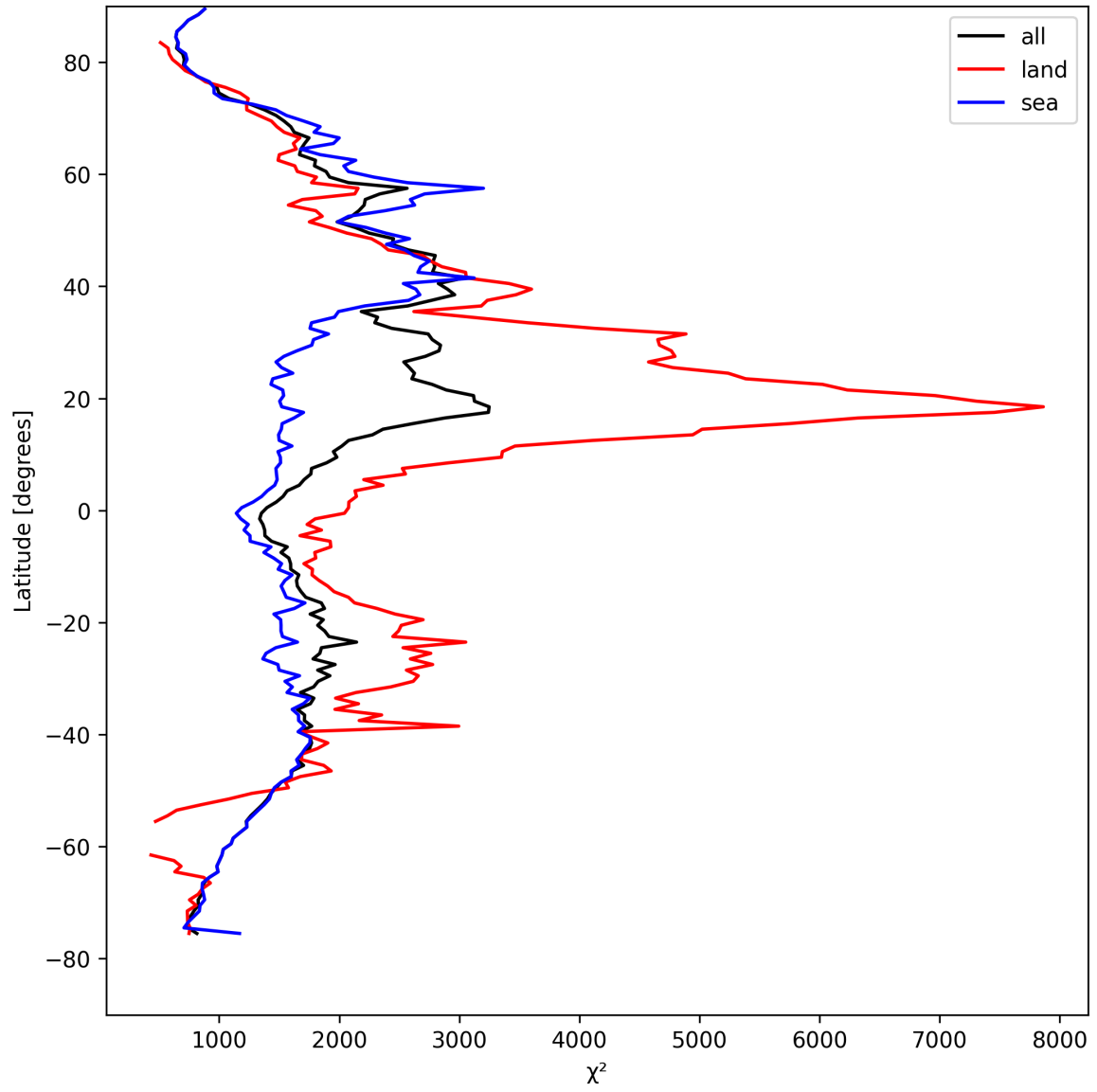
Figure 14: Zonal average of “ \chi^2 ” for 2025-04-13 to 2025-04-15.
