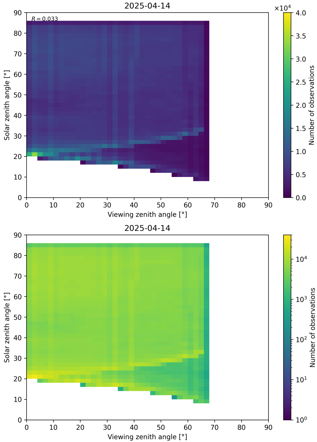
Figure 77: Scatter density plot of “Viewing zenith angle” against “Solar zenith angle” for 2025-04-13 to 2025-04-15.
