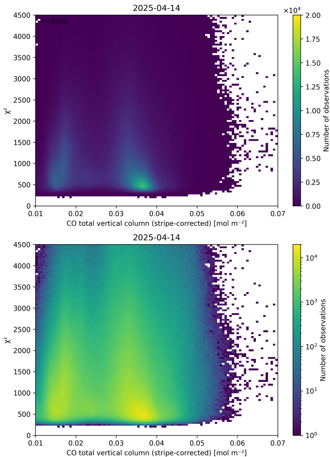
Figure 37: Scatter density plot of “CO total vertical column (stripe-corrected)” against “ \chi^2 ” for 2025-04-13 to 2025-04-15.
