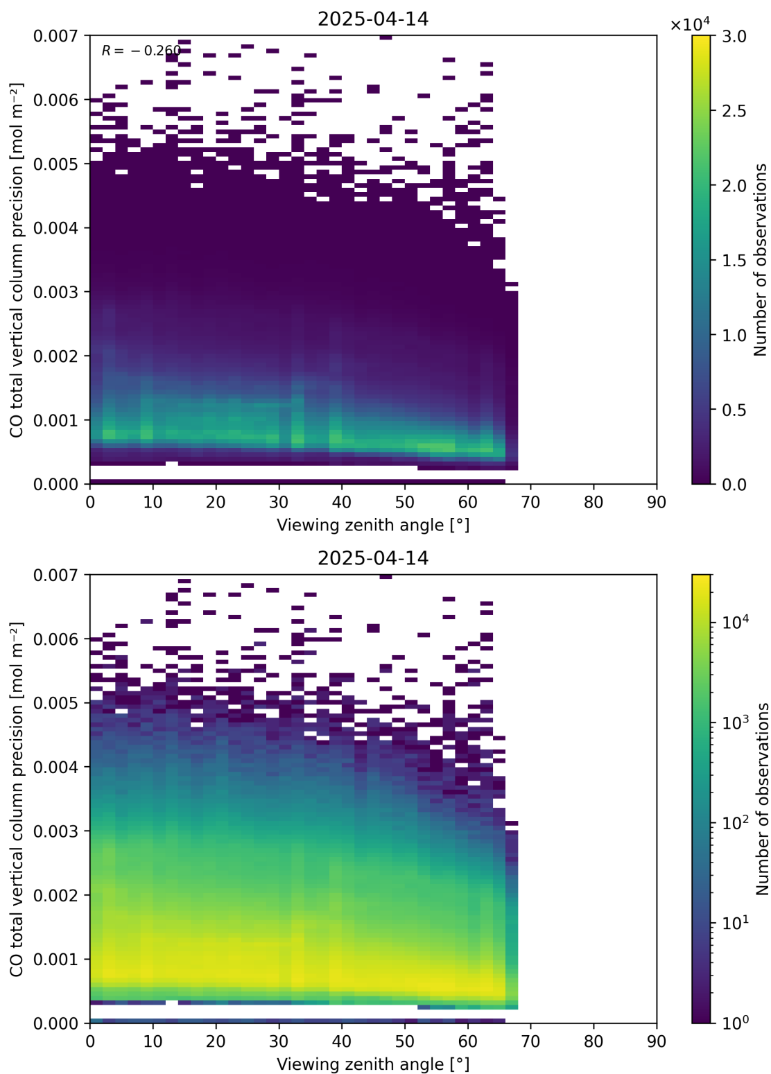
Figure 71: Scatter density plot of “Viewing zenith angle” against “CO total vertical column precision” for 2025-04-13 to 2025-04-15.
