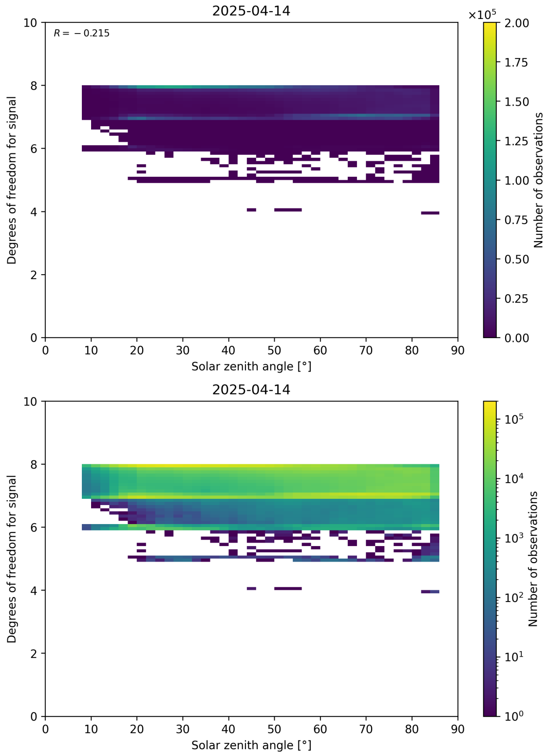
Figure 65: Scatter density plot of “Solar zenith angle” against “Degrees of freedom for signal” for 2025-04-13 to 2025-04-15.
