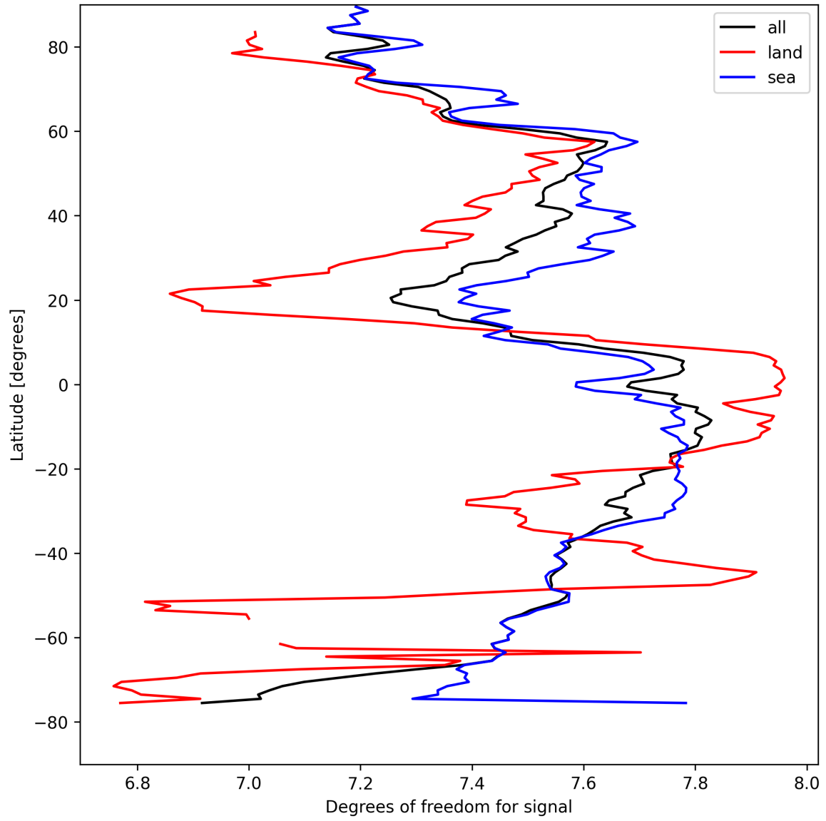
Figure 15: Zonal average of “Degrees of freedom for signal” for 2025-04-13 to 2025-04-15.
