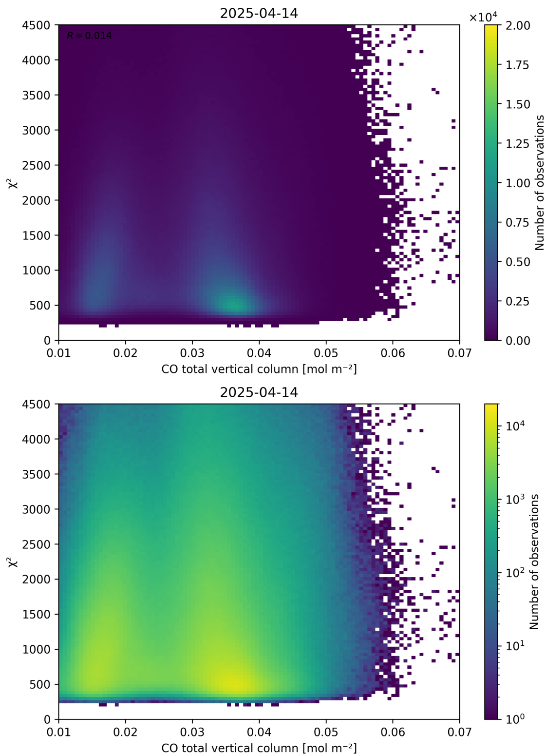
Figure 35: Scatter density plot of “CO total vertical column” against “ \chi^2 ” for 2025-04-13 to 2025-04-15.
