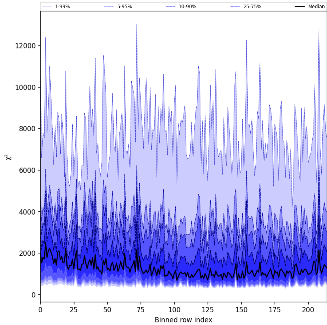
Figure 30: Along track statistics of “ \chi^2 ” for 2025-04-13 to 2025-04-15
