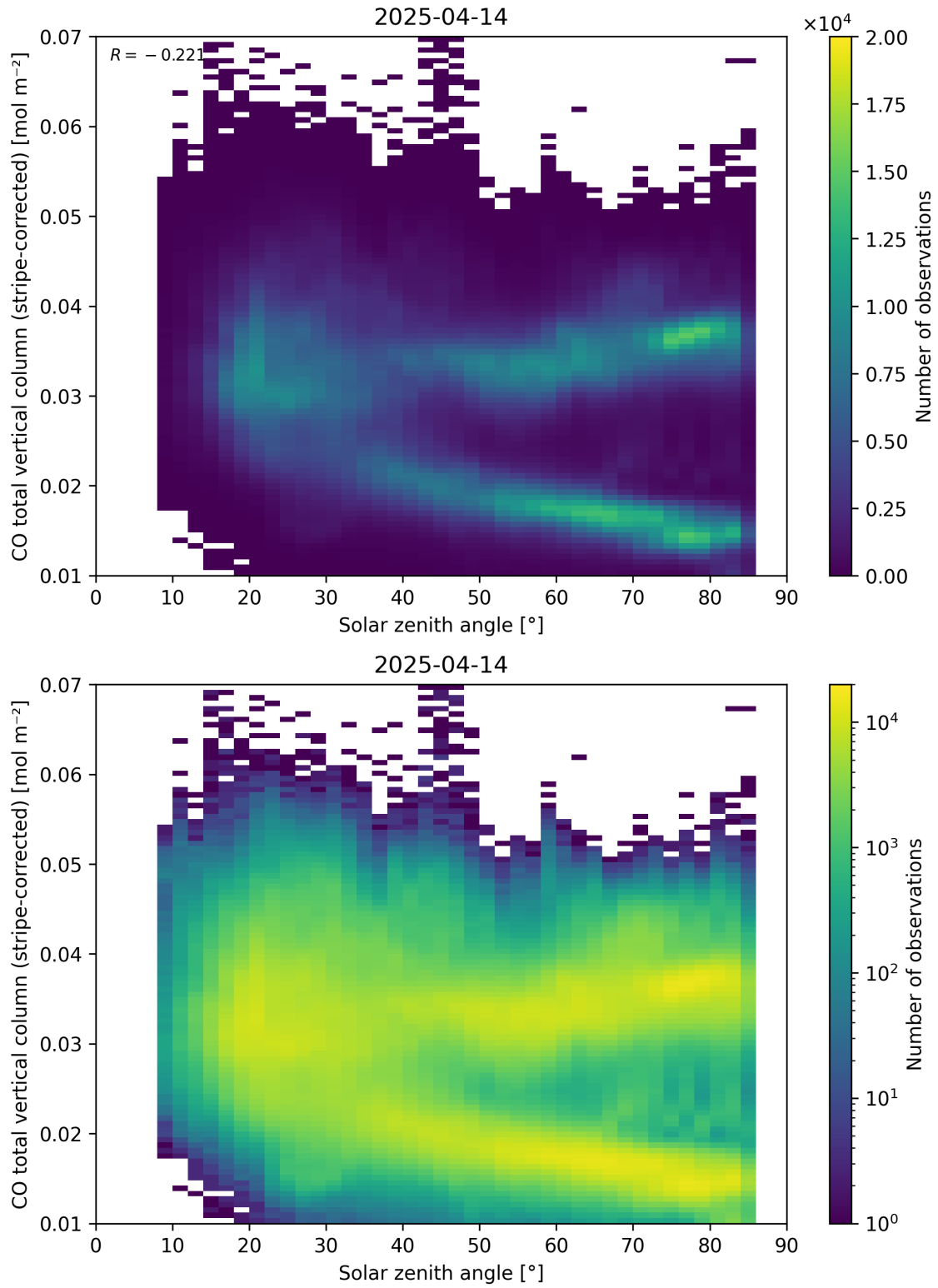
Figure 62: Scatter density plot of “Solar zenith angle” against “CO total vertical column (stripe-corrected)” for 2025-04-13 to 2025-04-15.
