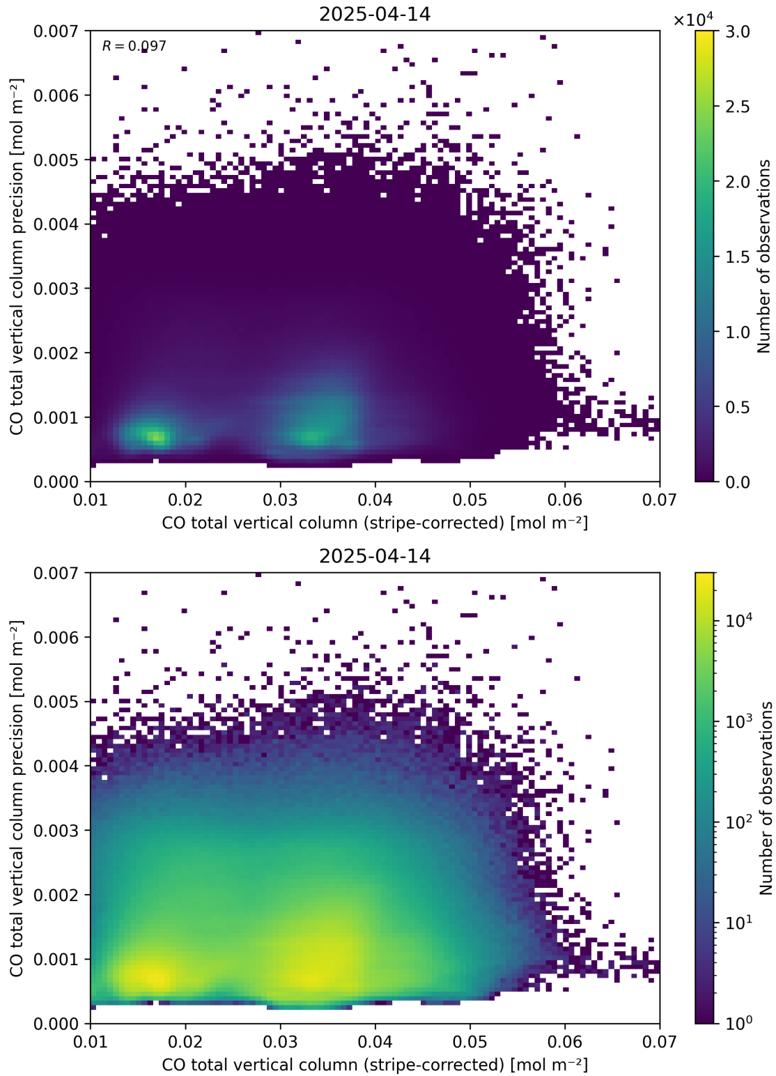
Figure 36: Scatter density plot of “CO total vertical column (stripe-corrected)” against “CO total vertical column precision” for 2025-04-13 to 2025-04-15.
