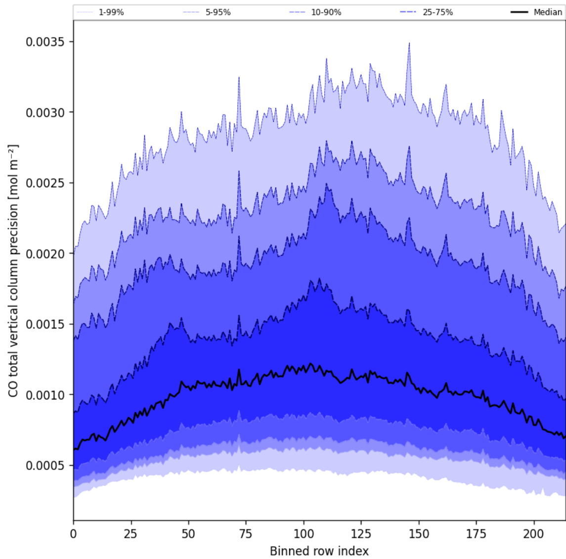
Figure 28: Along track statistics of “CO total vertical column precision” for 2025-04-13 to 2025-04-15
