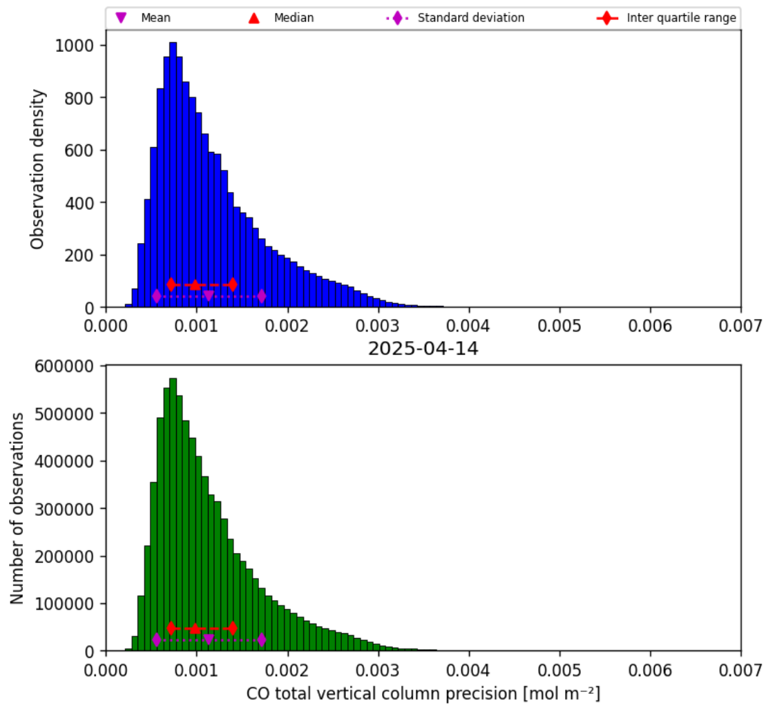
Figure 20: Histogram of “CO total vertical column precision” for 2025-04-13 to 2025-04-15
