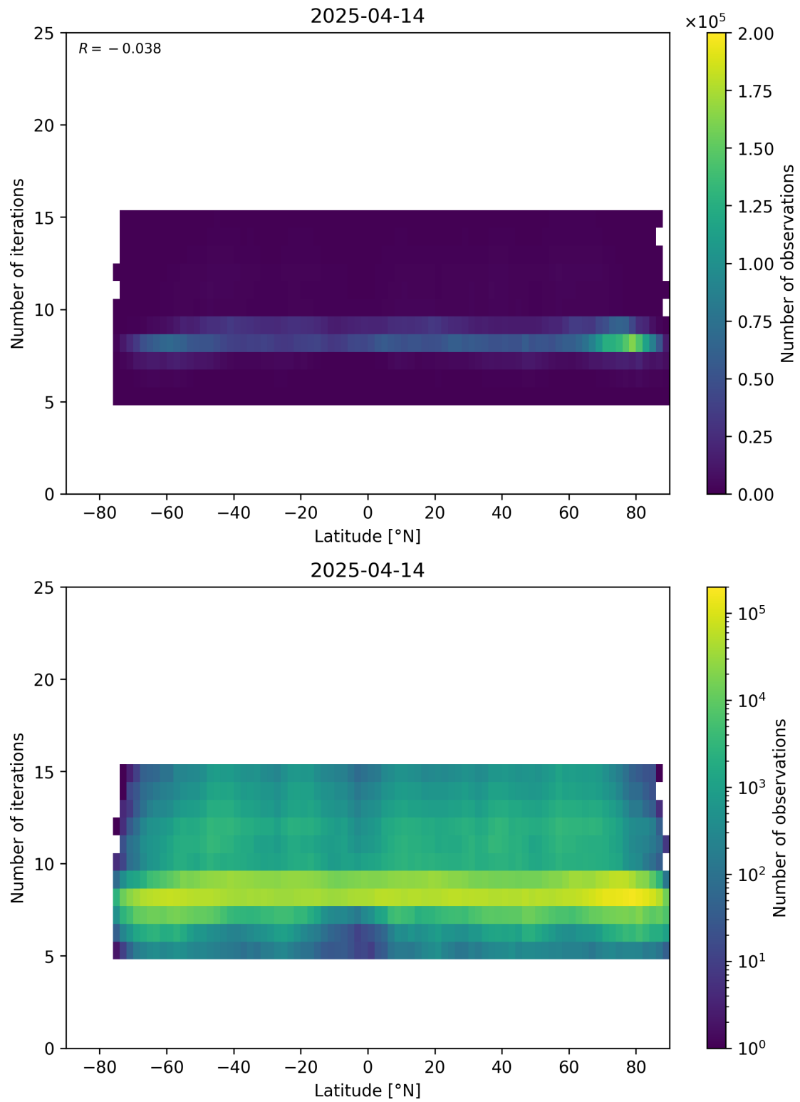
Figure 56: Scatter density plot of “Latitude” against “Number of iterations” for 2025-04-13 to 2025-04-15.
