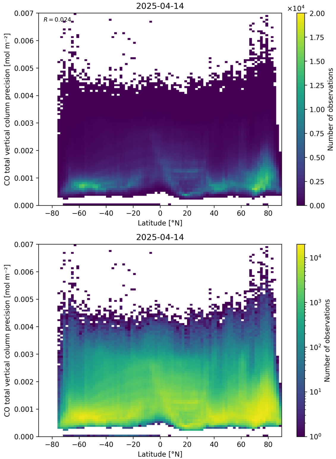
Figure 53: Scatter density plot of “Latitude” against “CO total vertical column precision” for 2025-04-13 to 2025-04-15.
