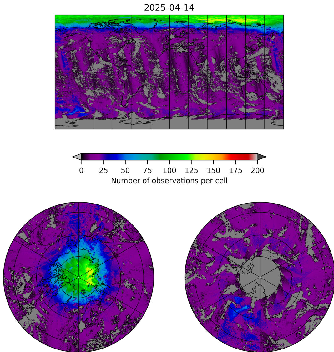
Figure 8: Map of the number of observations for 2025-04-13 to 2025-04-15
