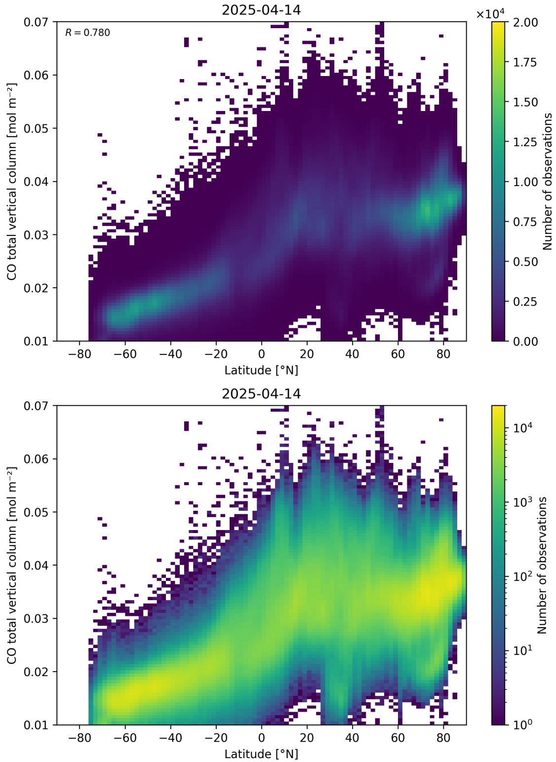
Figure 51: Scatter density plot of “Latitude” against “CO total vertical column” for 2025-04-13 to 2025-04-15.
