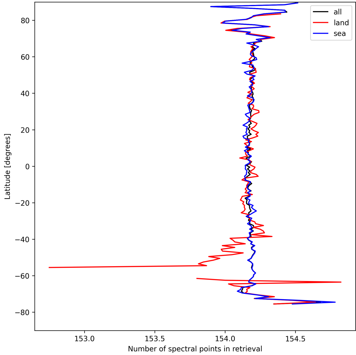
Figure 13: Zonal average of “Number of spectral points in retrieval” for 2025-04-13 to 2025-04-15.
