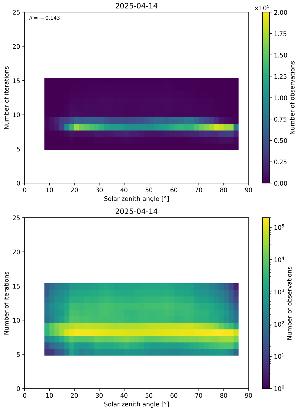
Figure 67: Scatter density plot of “Solar zenith angle” against “Number of iterations” for 2025-04-13 to 2025-04-15.
