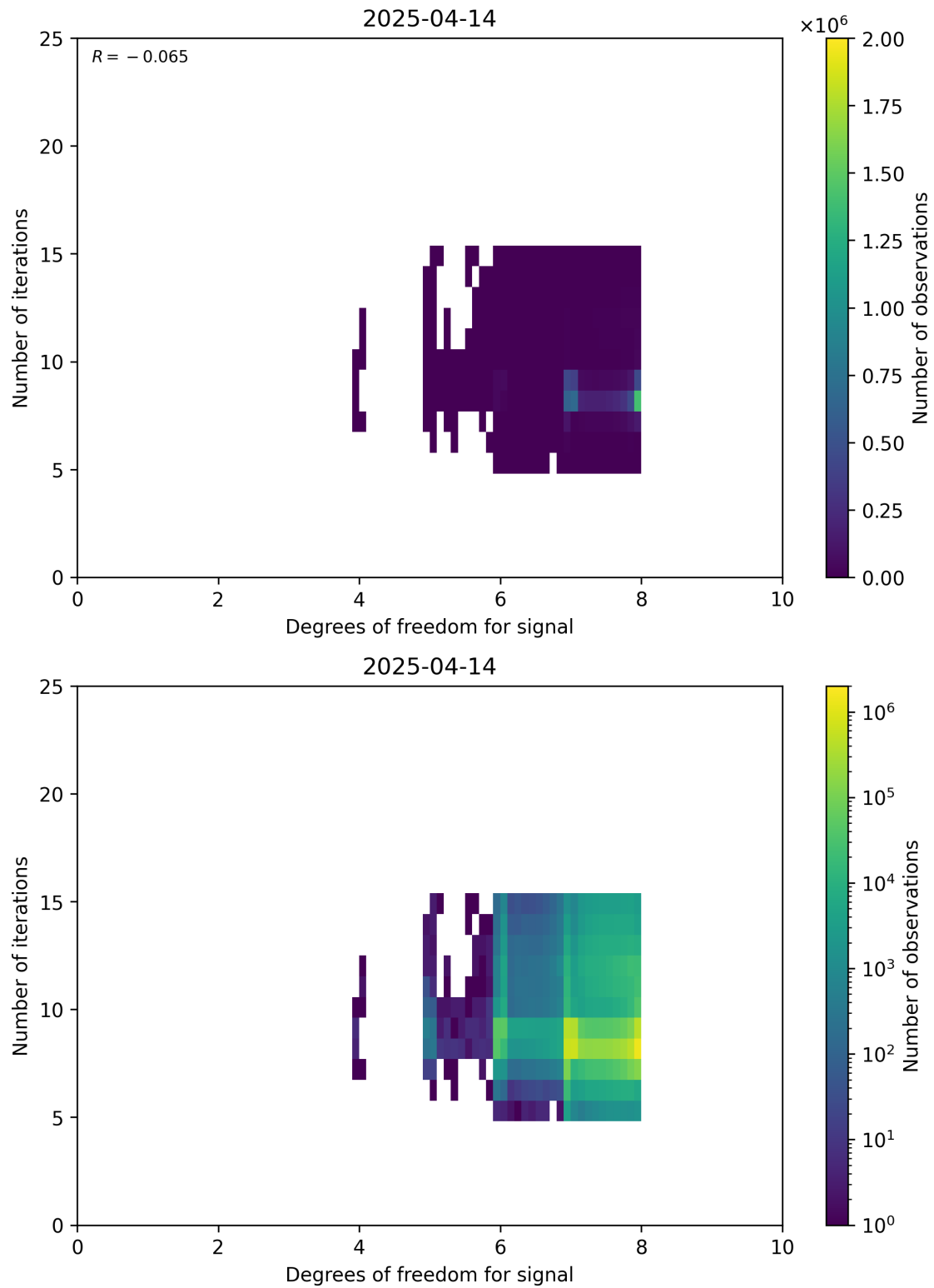
Figure 50: Scatter density plot of “Degrees of freedom for signal” against “Number of iterations” for 2025-04-13 to 2025-04-15.
