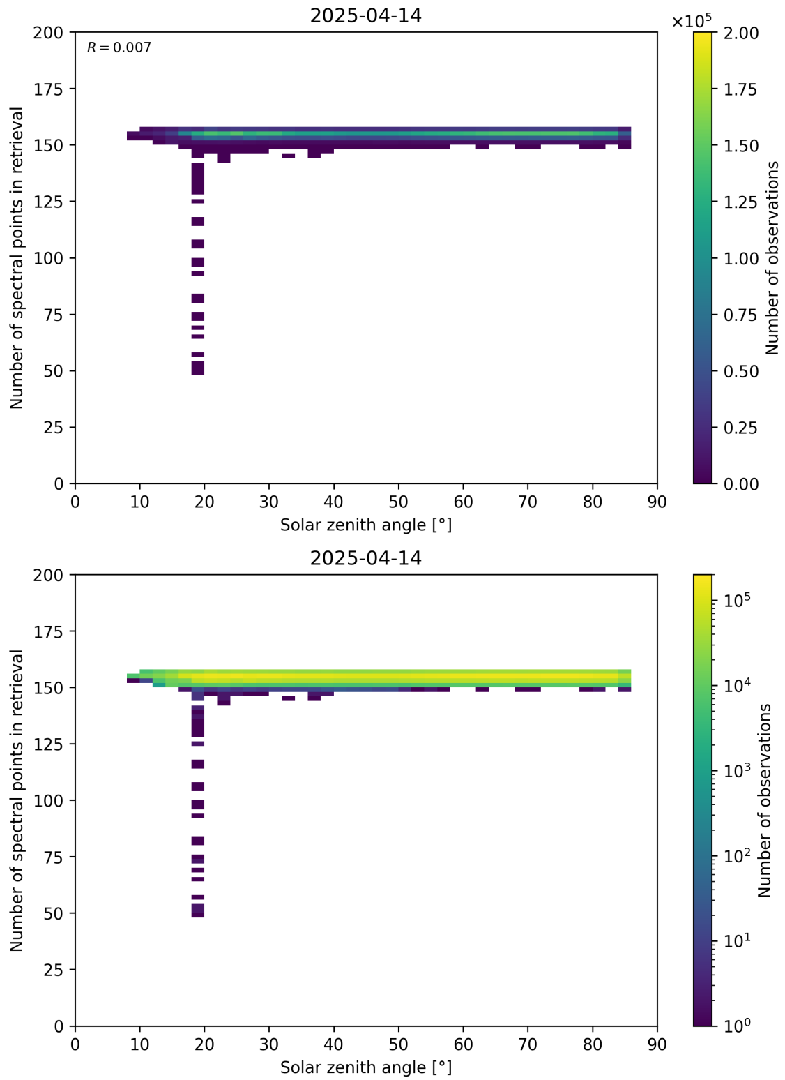
Figure 68: Scatter density plot of “Solar zenith angle” against “Number of spectral points in retrieval” for 2025-04-13 to 2025-04-15.
