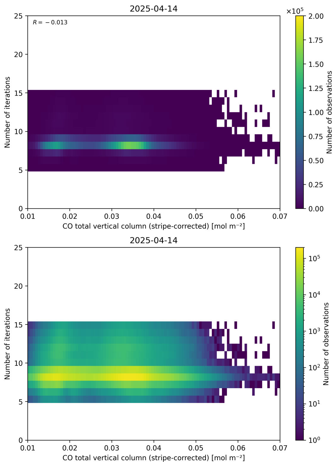
Figure 39: Scatter density plot of “CO total vertical column (stripe-corrected)” against “Number of iterations” for 2025-04-13 to 2025-04-15.
