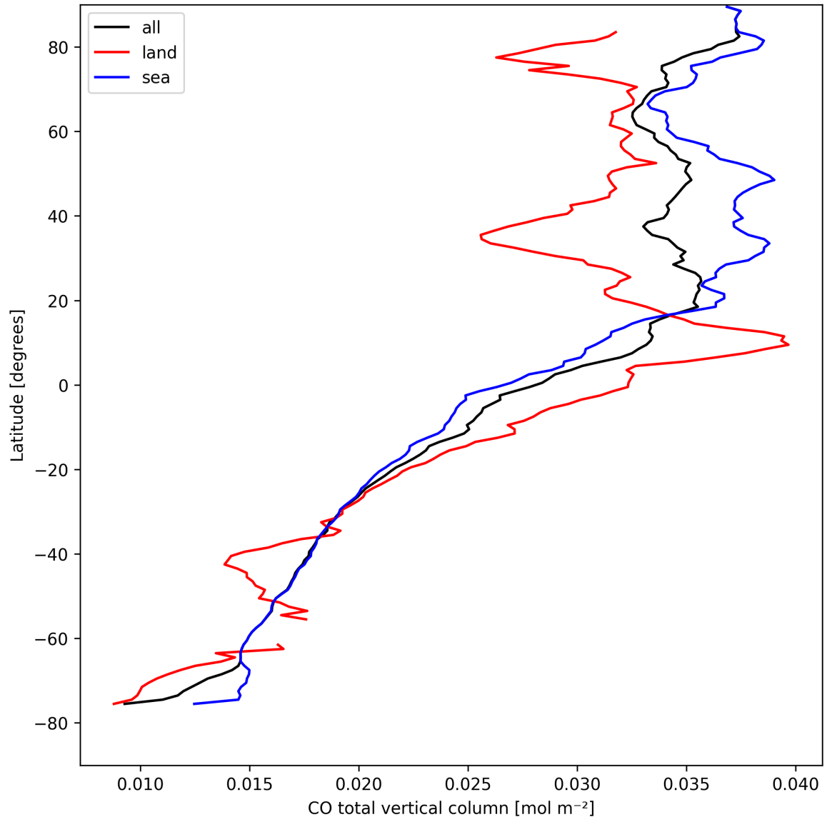
Figure 10: Zonal average of “CO total vertical column” for 2025-04-13 to 2025-04-15.
