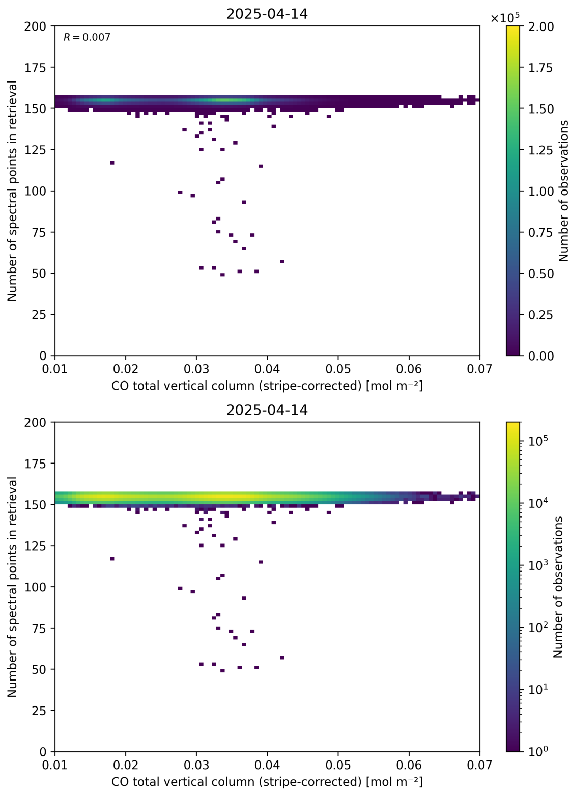
Figure 40: Scatter density plot of “CO total vertical column (stripe-corrected)” against “Number of spectral points in retrieval” for 2025-04-13 to 2025-04-15.
