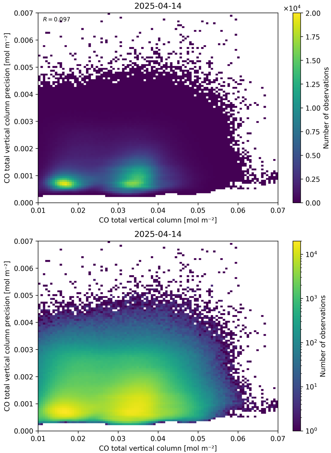
Figure 34: Scatter density plot of “CO total vertical column” against “CO total vertical column precision” for 2025-04-13 to 2025-04-15.
