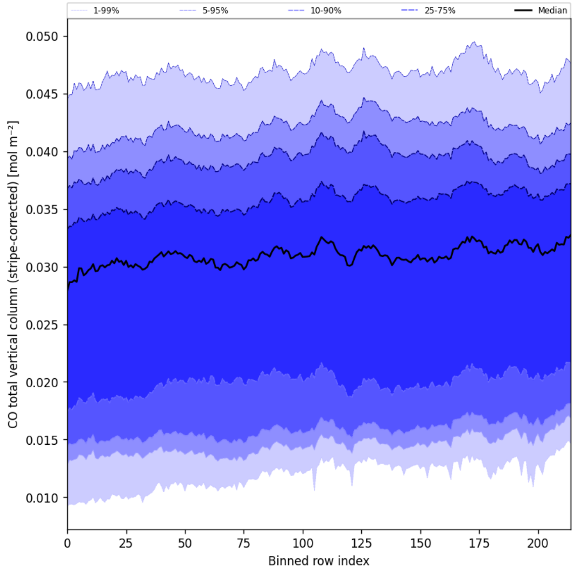
Figure 27: Along track statistics of “CO total vertical column (stripe-corrected)” for 2025-04-13 to 2025-04-15
