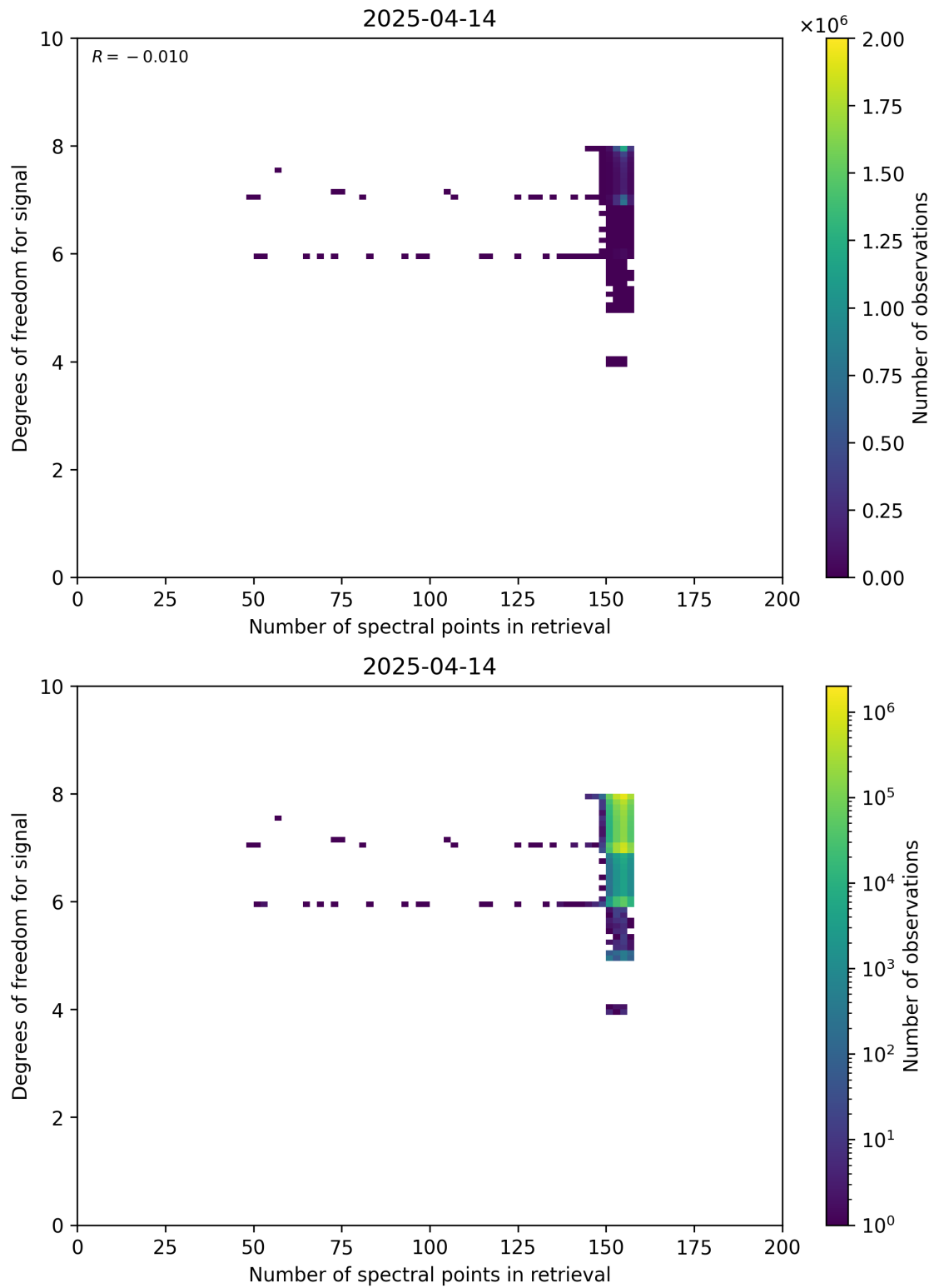
Figure 59: Scatter density plot of “Number of spectral points in retrieval” against “Degrees of freedom for signal” for 2025-04-13 to 2025-04-15.
