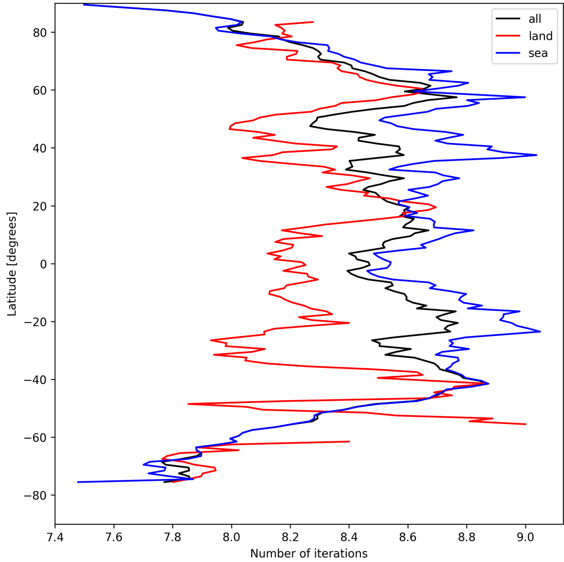
Figure 16: Zonal average of “Number of iterations” for 2025-04-13 to 2025-04-15.
