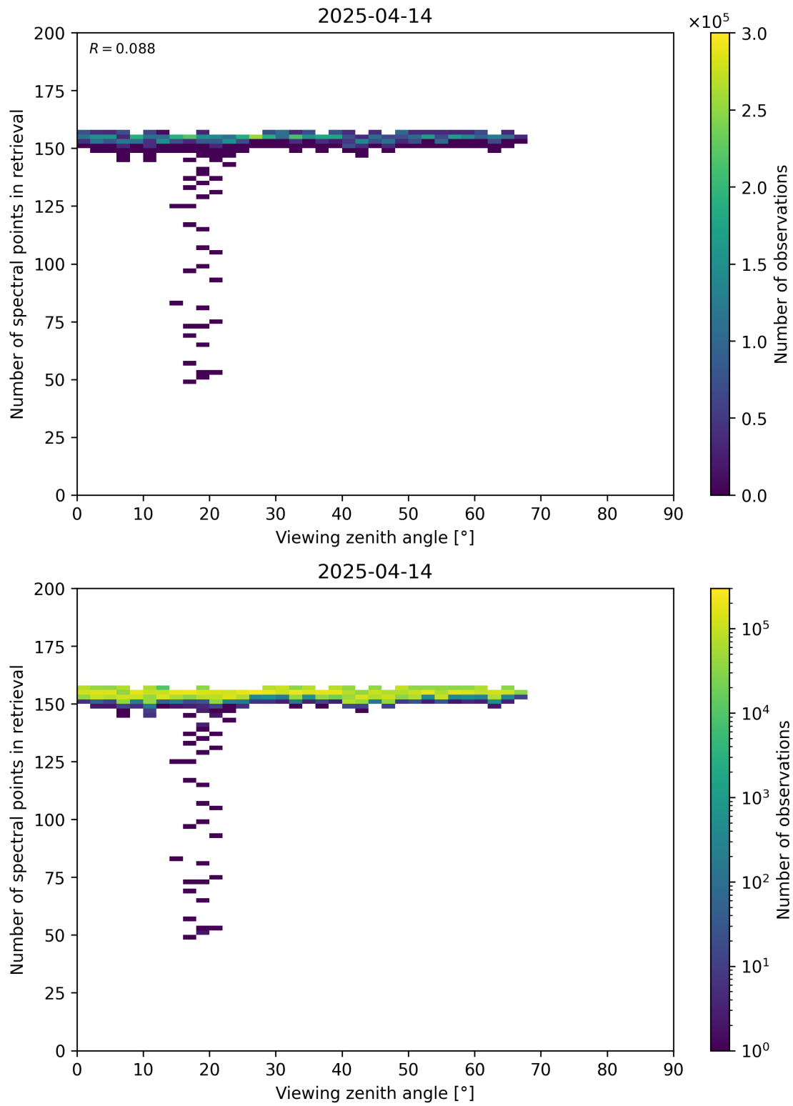
Figure 76: Scatter density plot of “Viewing zenith angle” against “Number of spectral points in retrieval” for 2025-04-13 to 2025-04-15.
