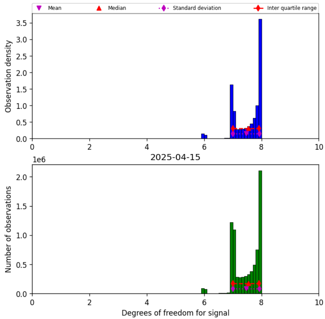
Figure 23: Histogram of “Degrees of freedom for signal” for 2025-04-14 to 2025-04-16
