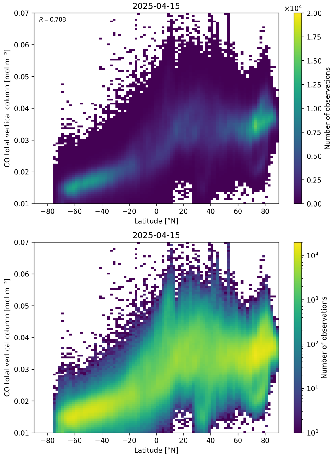
Figure 51: Scatter density plot of “Latitude” against “CO total vertical column” for 2025-04-14 to 2025-04-16.
