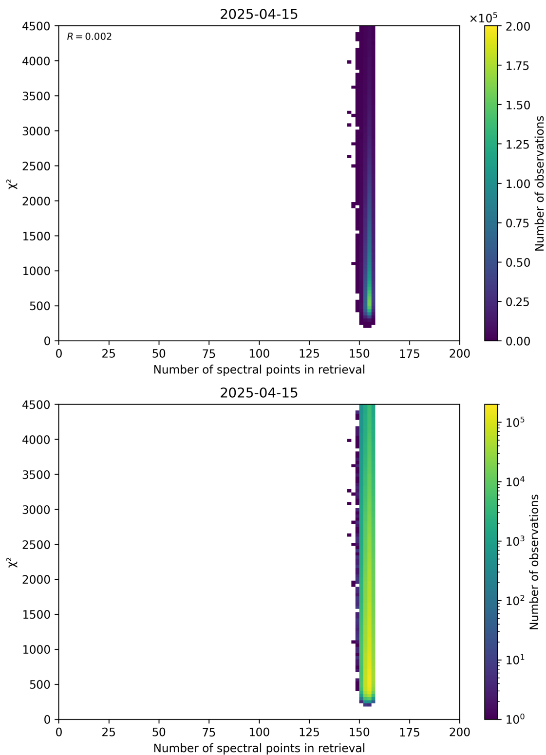
Figure 58: Scatter density plot of “Number of spectral points in retrieval” against “ \chi^2 ” for 2025-04-14 to 2025-04-16.
