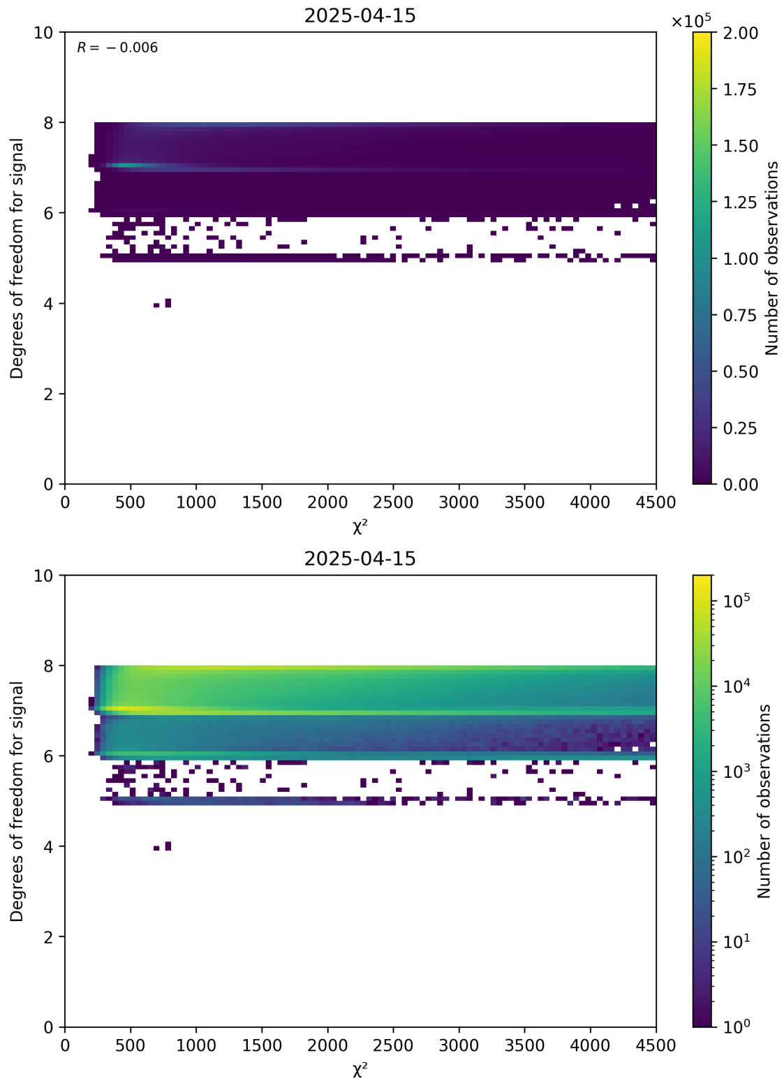
Figure 48: Scatter density plot of “ \chi^2 ” against “Degrees of freedom for signal” for 2025-04-14 to 2025-04-16.
