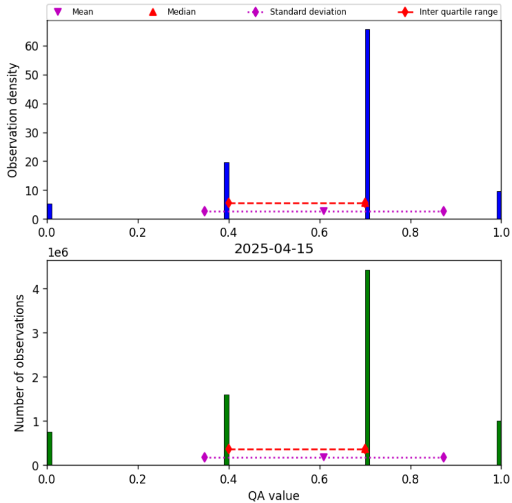
Figure 17: Histogram of “QA value” for 2025-04-14 to 2025-04-16
