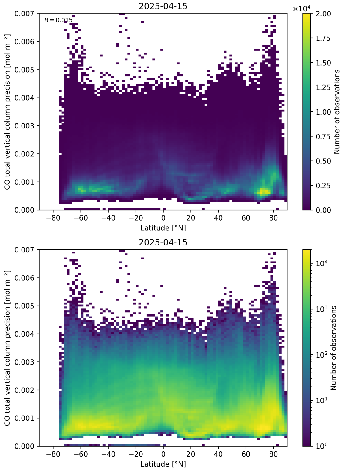
Figure 53: Scatter density plot of “Latitude” against “CO total vertical column precision” for 2025-04-14 to 2025-04-16.
