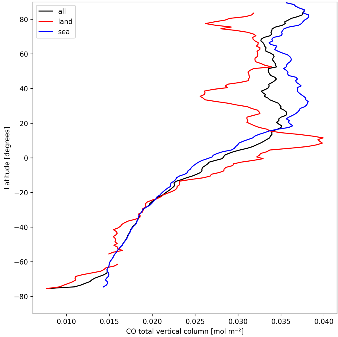
Figure 10: Zonal average of “CO total vertical column” for 2025-04-14 to 2025-04-16.
