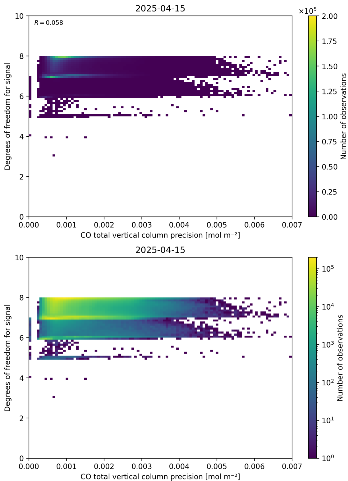
Figure 45: Scatter density plot of “CO total vertical column precision” against “Degrees of freedom for signal” for 2025-04-14 to 2025-04-16.
