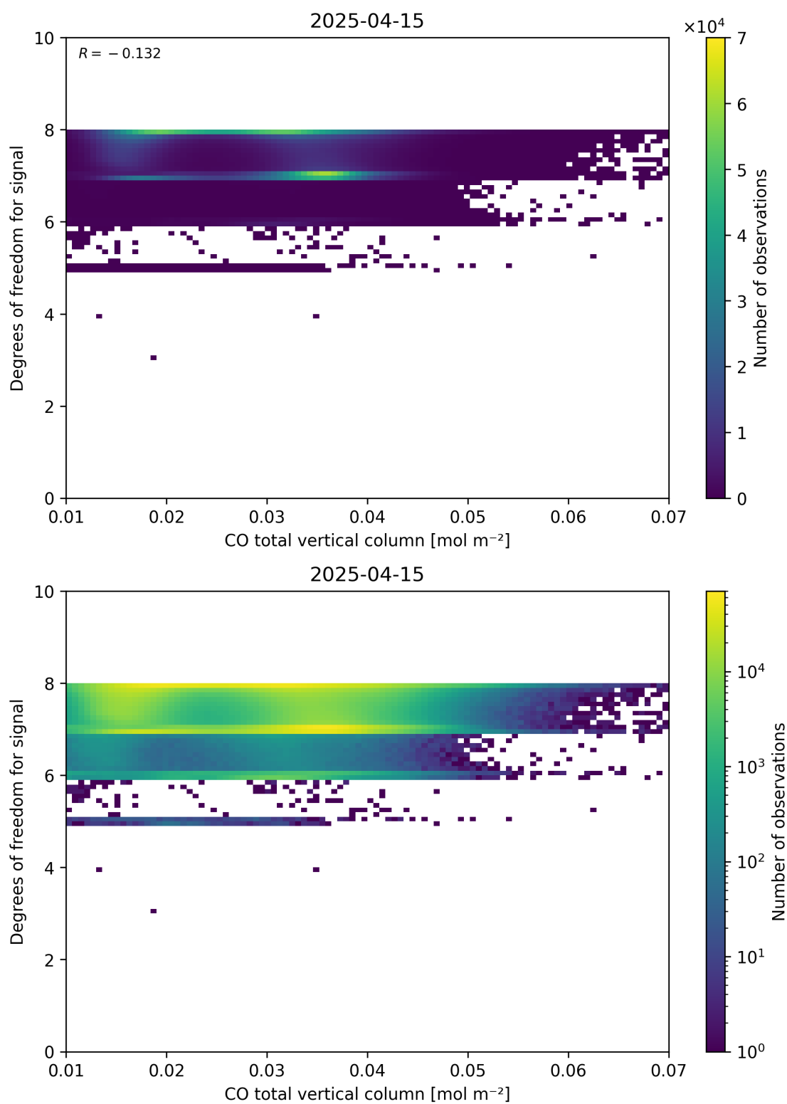
Figure 41: Scatter density plot of “CO total vertical column” against “Degrees of freedom for signal” for 2025-04-14 to 2025-04-16.
