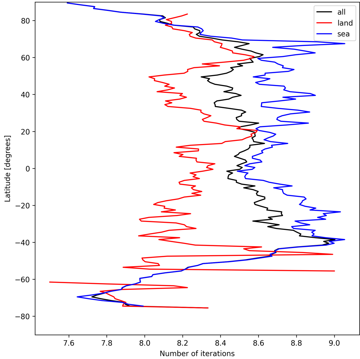
Figure 16: Zonal average of “Number of iterations” for 2025-04-14 to 2025-04-16.
