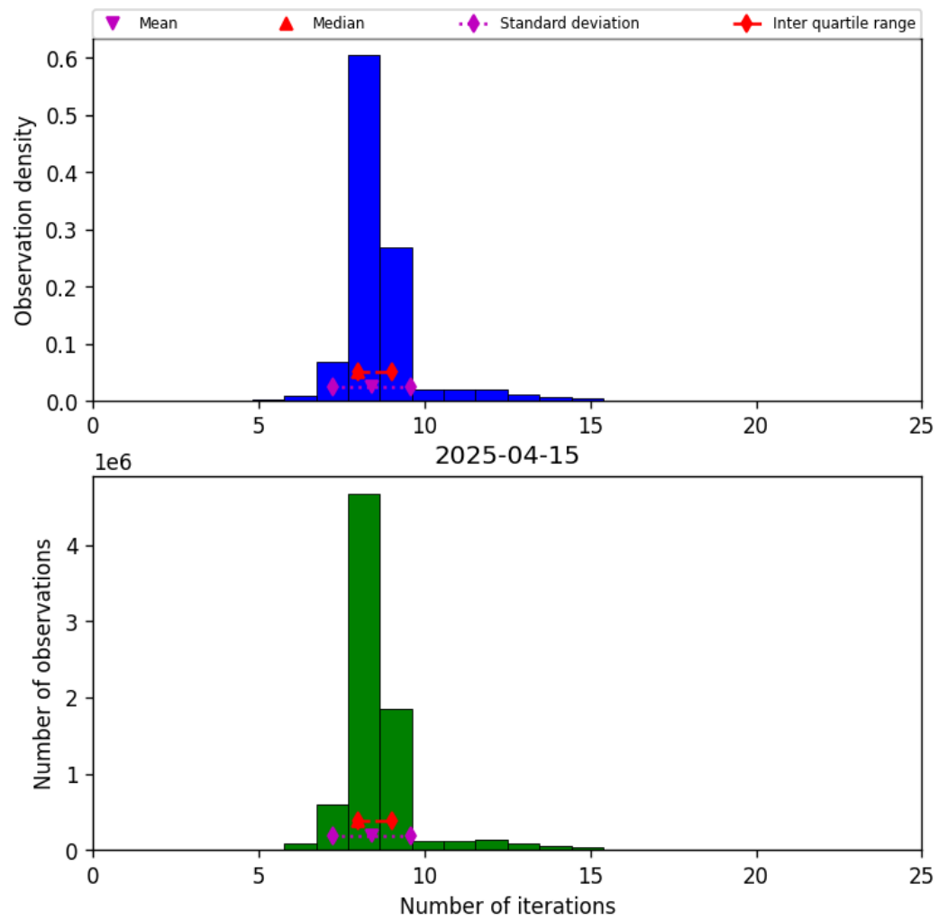
Figure 24: Histogram of “Number of iterations” for 2025-04-14 to 2025-04-16
