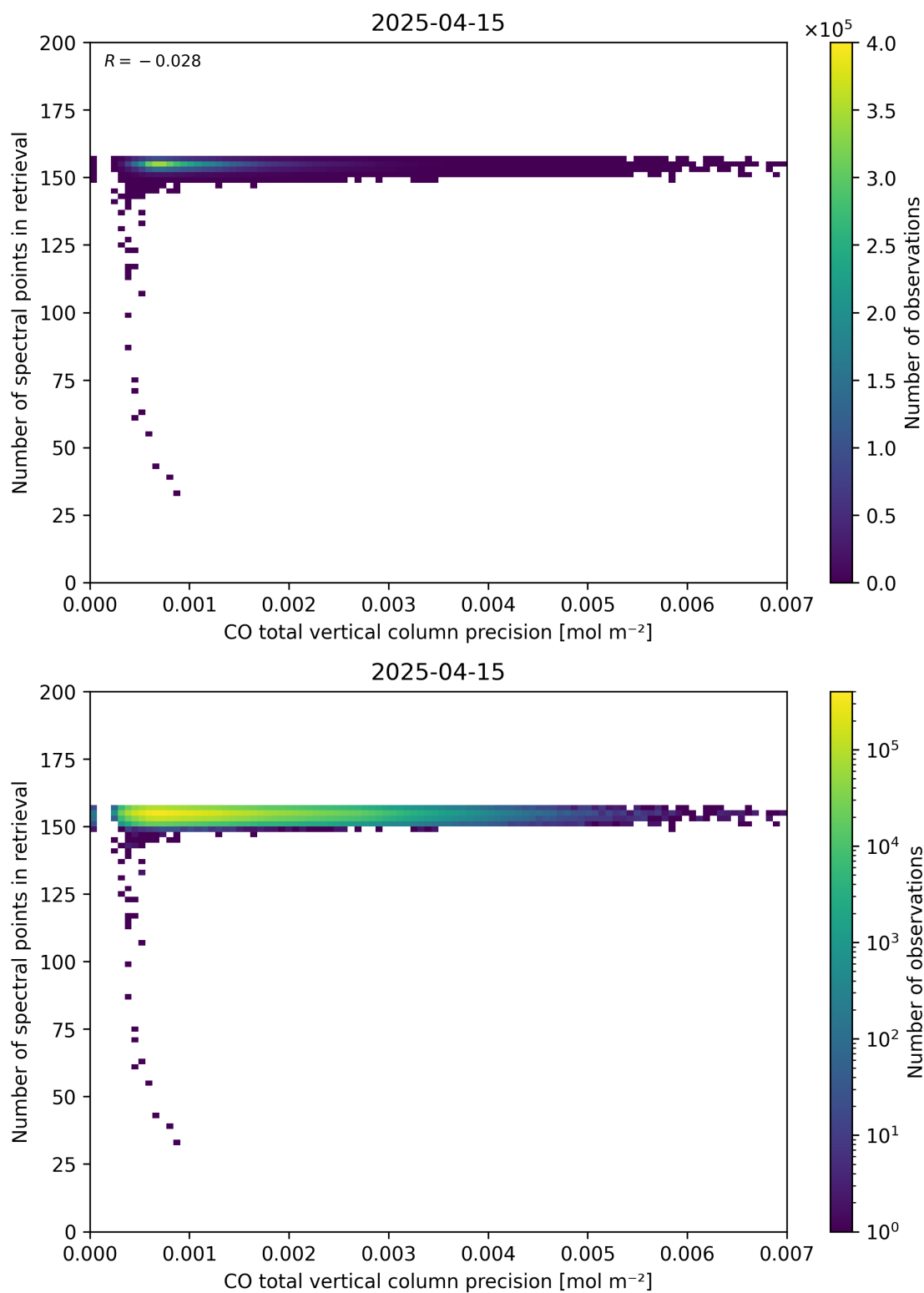
Figure 47: Scatter density plot of “CO total vertical column precision” against “Number of spectral points in retrieval” for 2025-04-14 to 2025-04-16.
