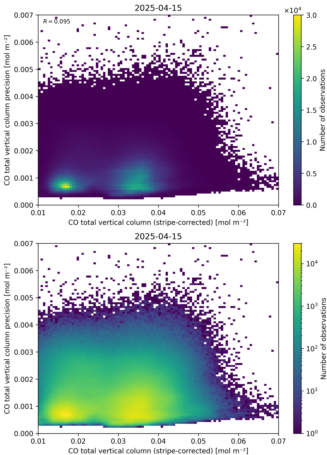
Figure 36: Scatter density plot of “CO total vertical column (stripe-corrected)” against “CO total vertical column precision” for 2025-04-14 to 2025-04-16.
