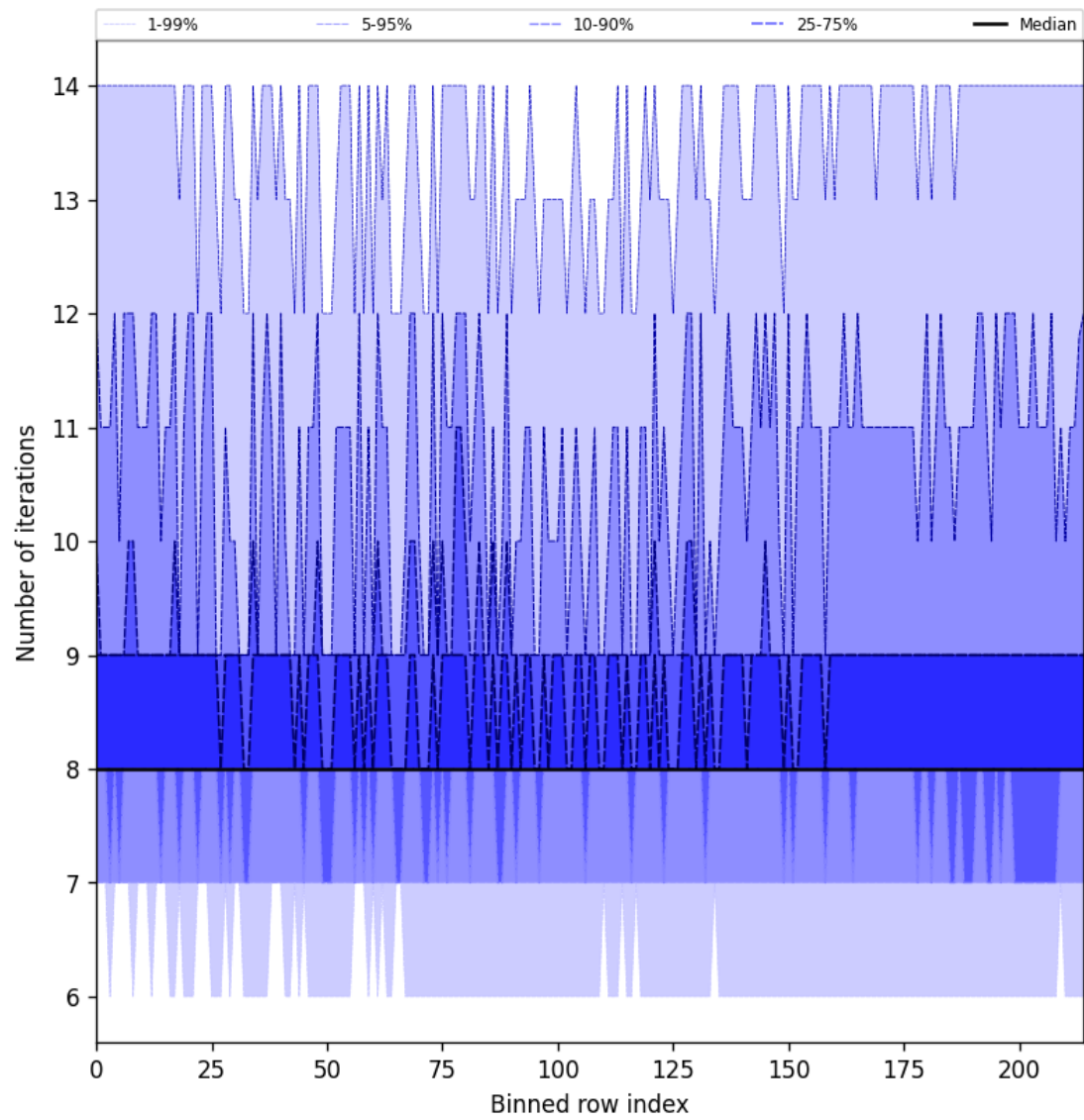
Figure 32: Along track statistics of “Number of iterations” for 2025-04-14 to 2025-04-16
