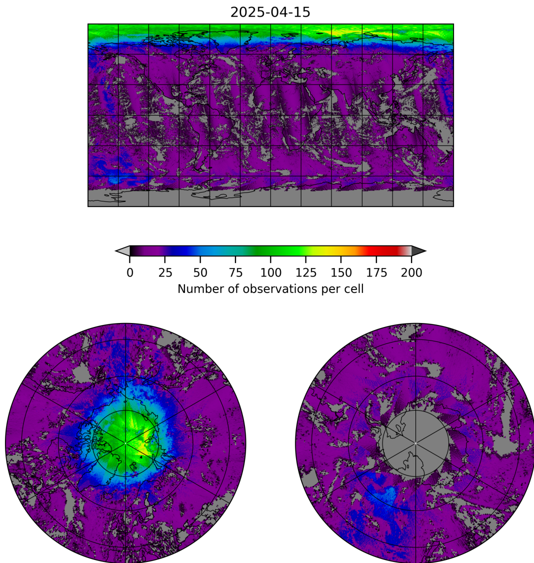
Figure 8: Map of the number of observations for 2025-04-14 to 2025-04-16
