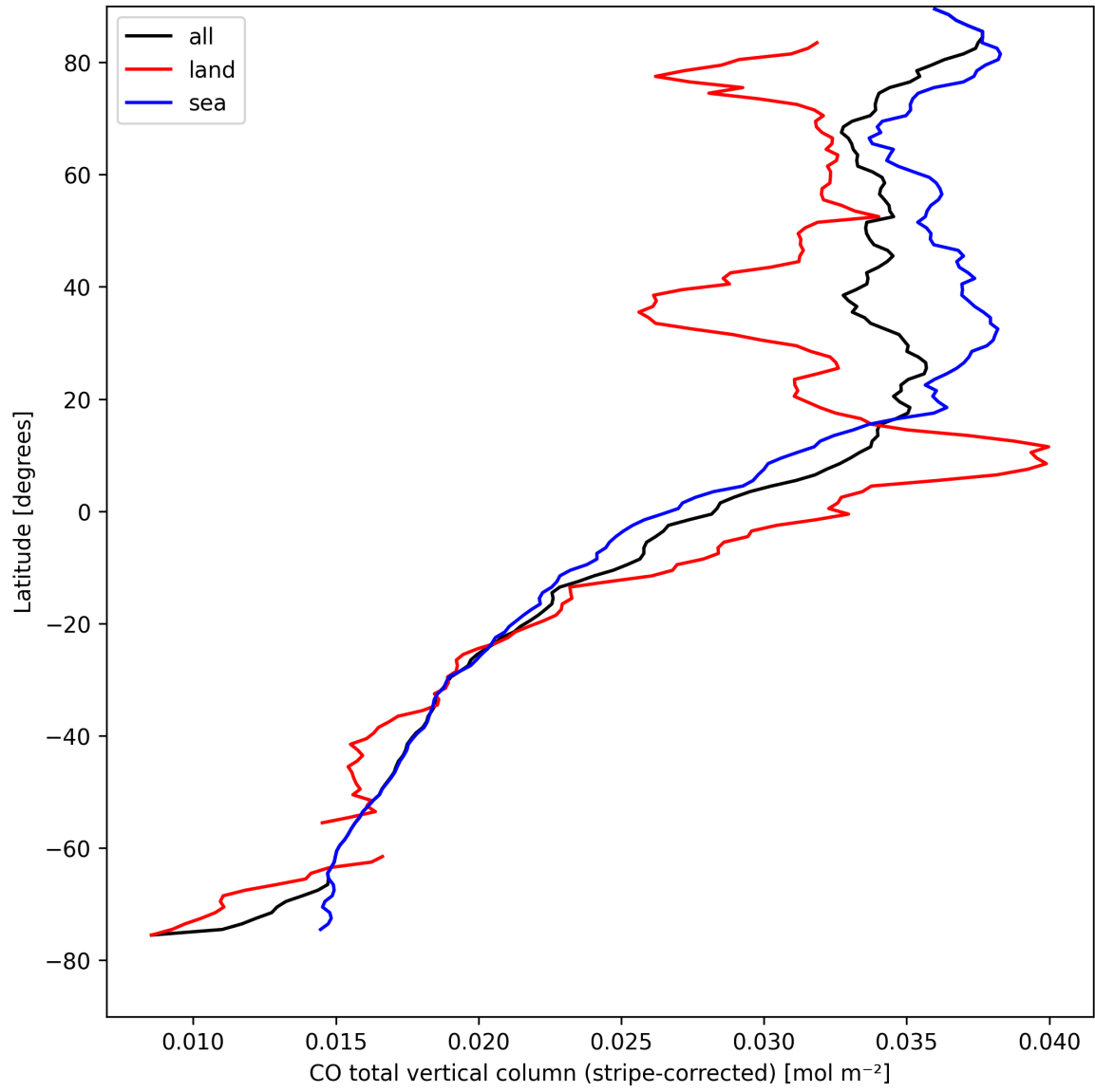
Figure 11: Zonal average of “CO total vertical column (stripe-corrected)” for 2025-04-14 to 2025-04-16.
