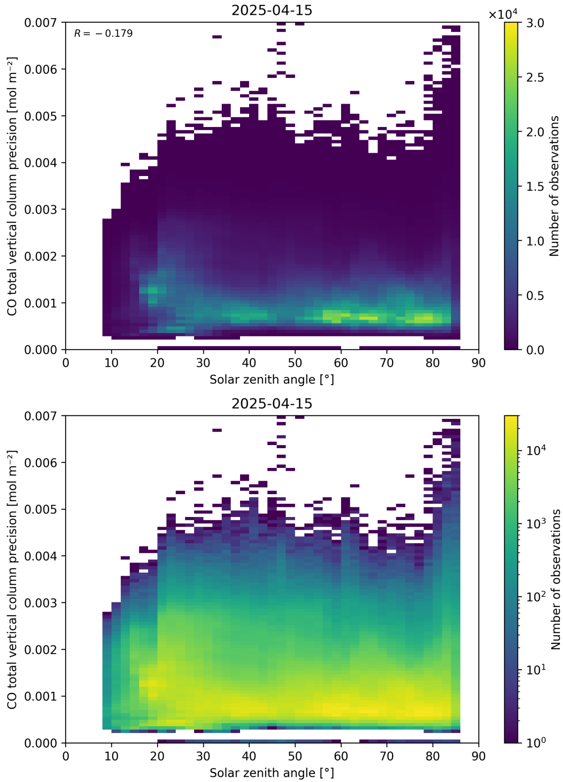
Figure 63: Scatter density plot of “Solar zenith angle” against “CO total vertical column precision” for 2025-04-14 to 2025-04-16.
