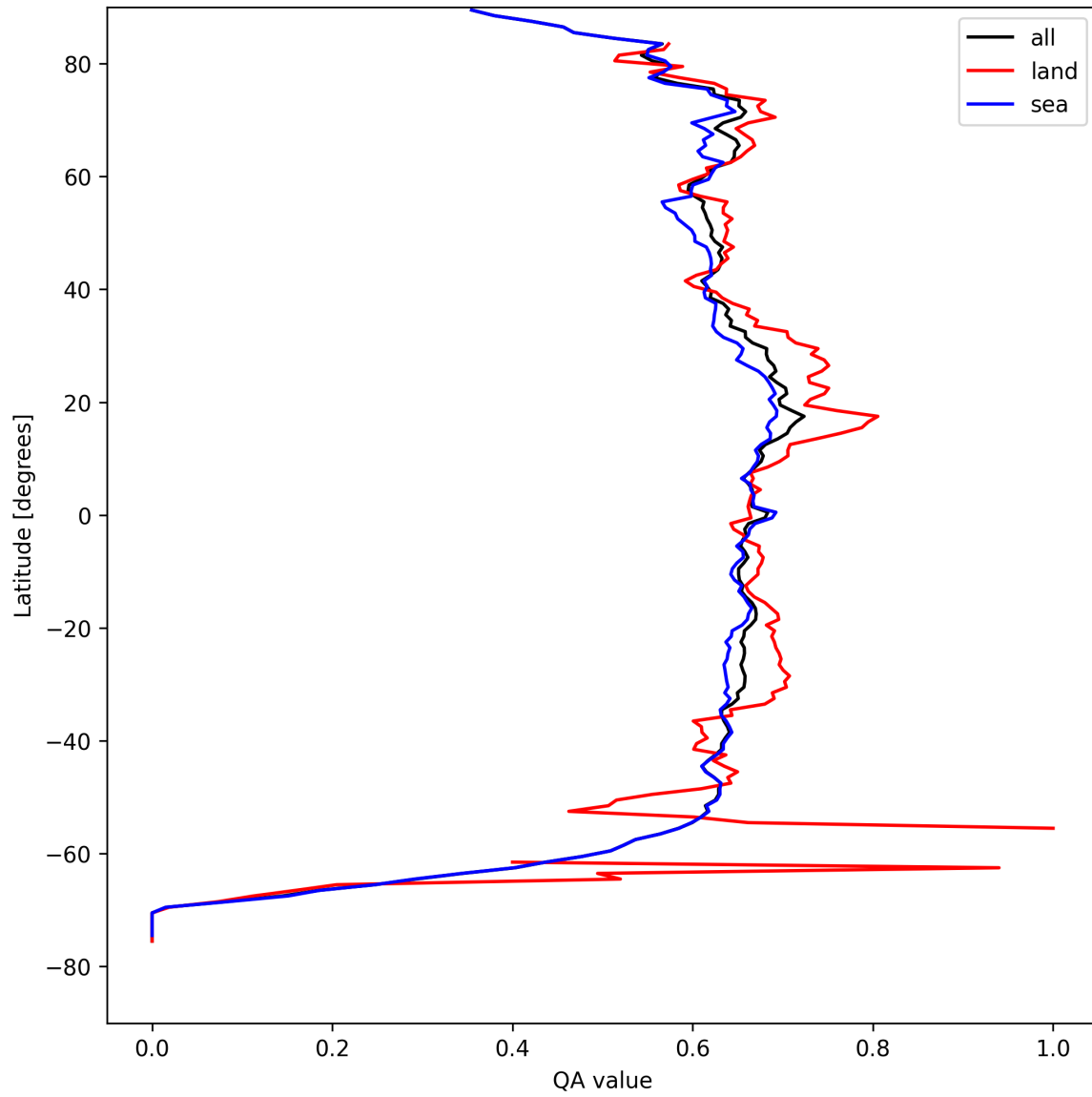
Figure 9: Zonal average of “QA value” for 2025-04-14 to 2025-04-16.
