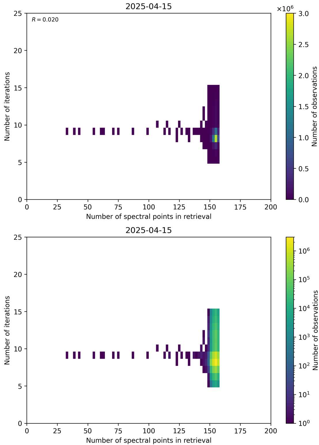
Figure 60: Scatter density plot of “Number of spectral points in retrieval” against “Number of iterations” for 2025-04-14 to 2025-04-16.
