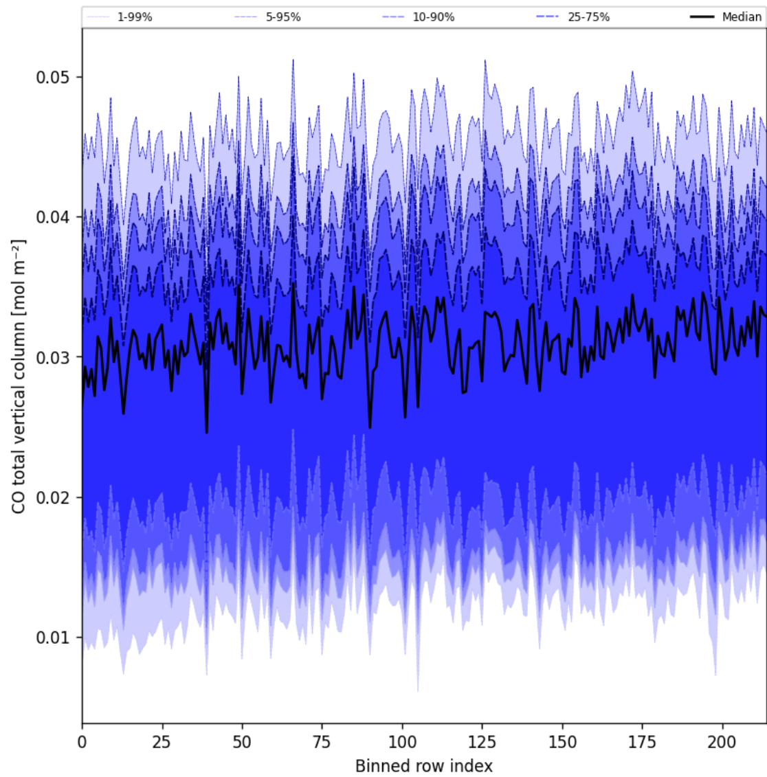
Figure 26: Along track statistics of “CO total vertical column” for 2025-04-14 to 2025-04-16
