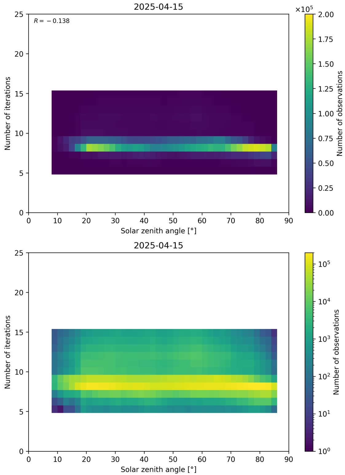
Figure 67: Scatter density plot of “Solar zenith angle” against “Number of iterations” for 2025-04-14 to 2025-04-16.
