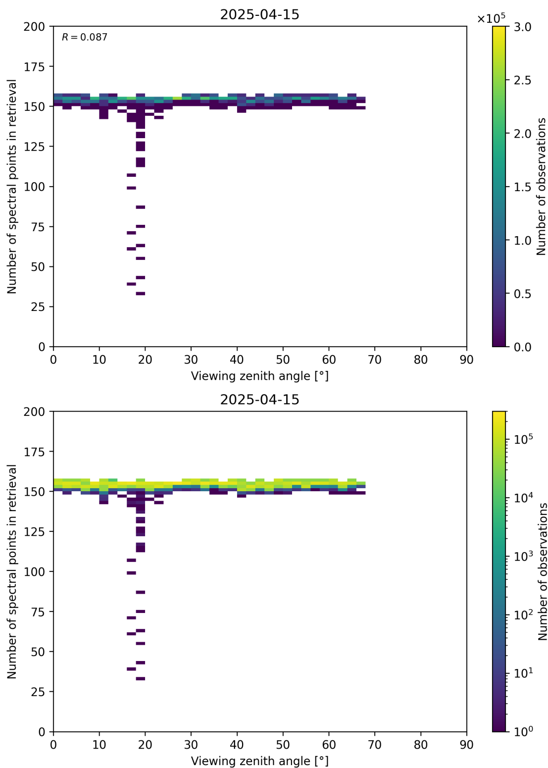
Figure 76: Scatter density plot of “Viewing zenith angle” against “Number of spectral points in retrieval” for 2025-04-14 to 2025-04-16.
