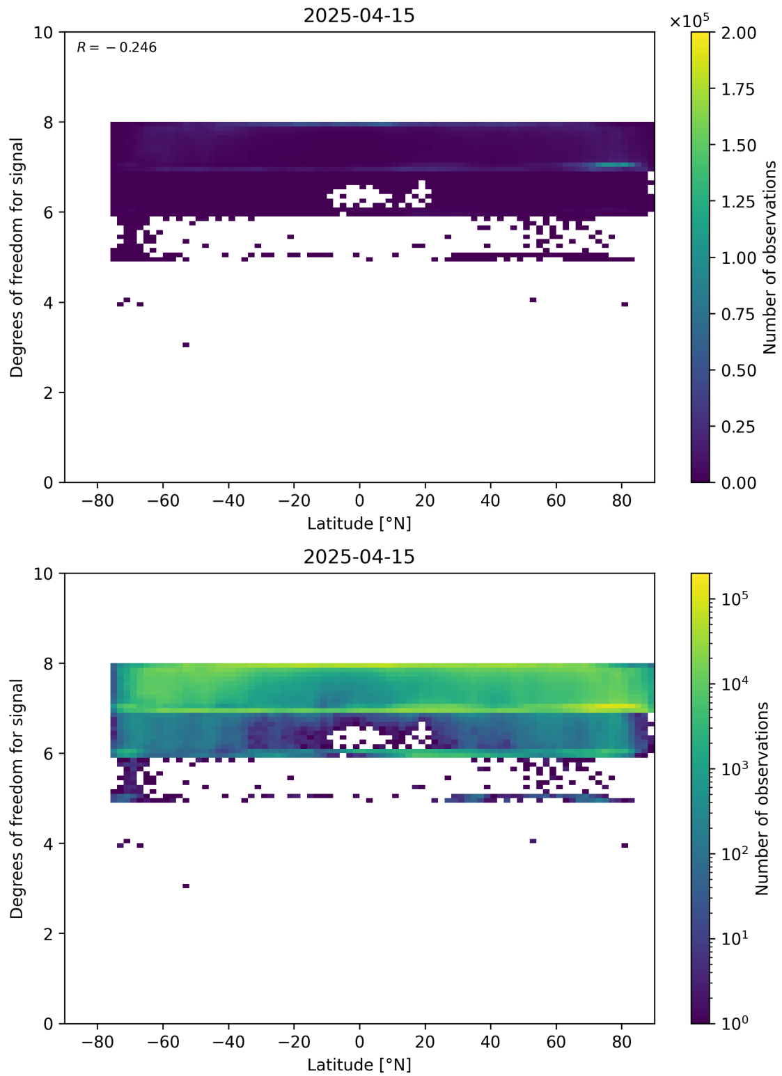
Figure 55: Scatter density plot of “Latitude” against “Degrees of freedom for signal” for 2025-04-14 to 2025-04-16.
