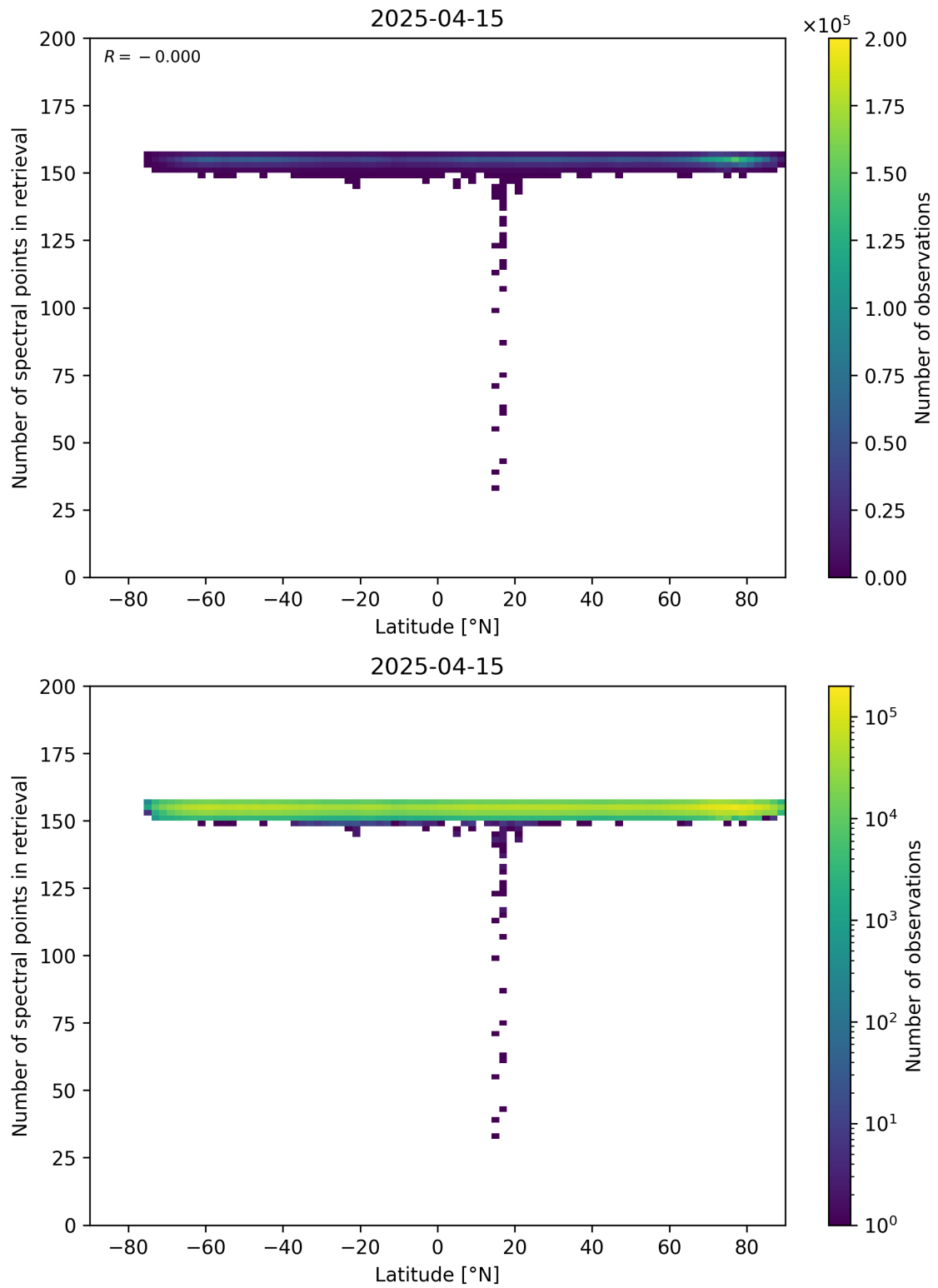
Figure 57: Scatter density plot of “Latitude” against “Number of spectral points in retrieval” for 2025-04-14 to 2025-04-16.
