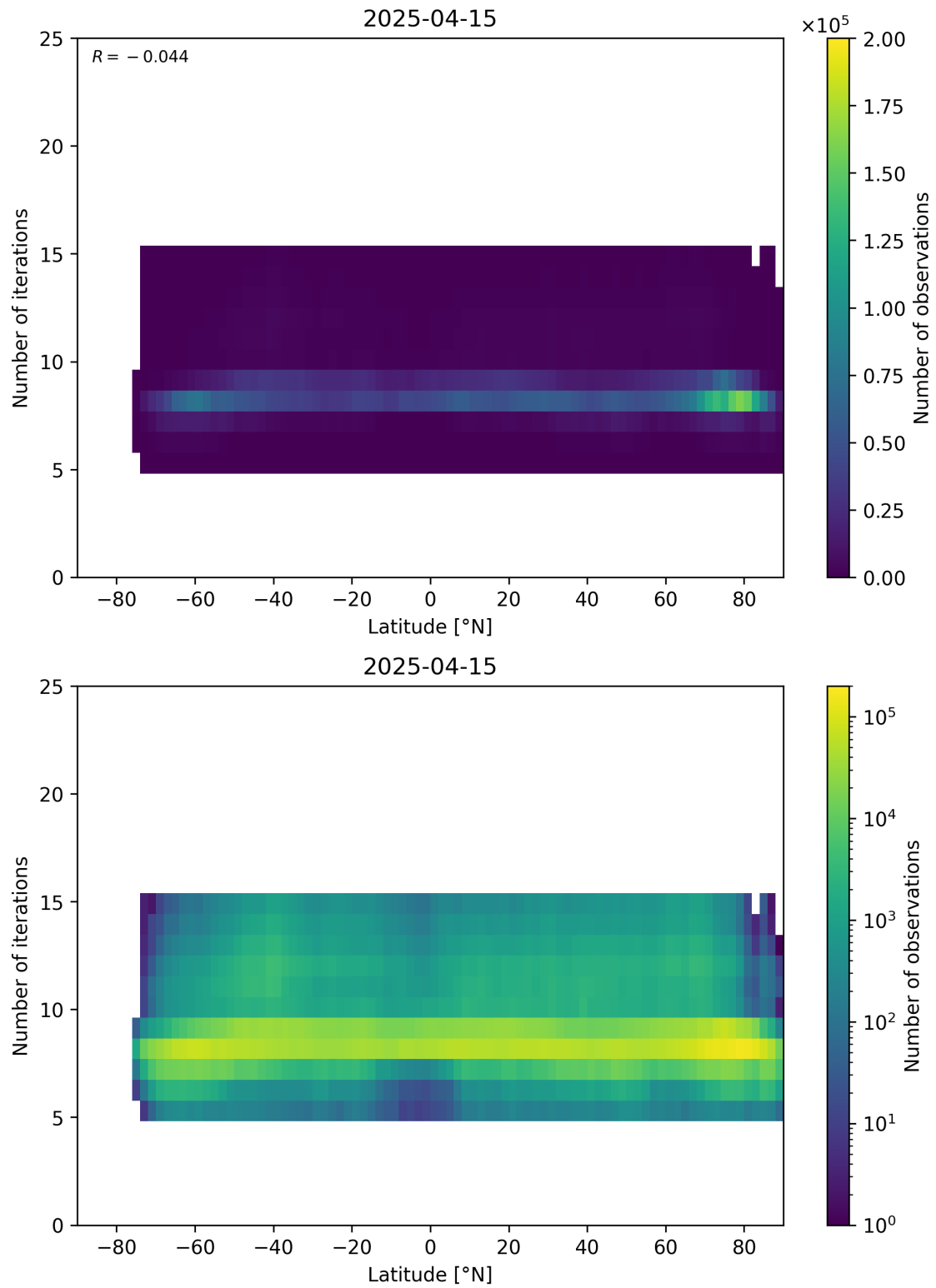
Figure 56: Scatter density plot of “Latitude” against “Number of iterations” for 2025-04-14 to 2025-04-16.
