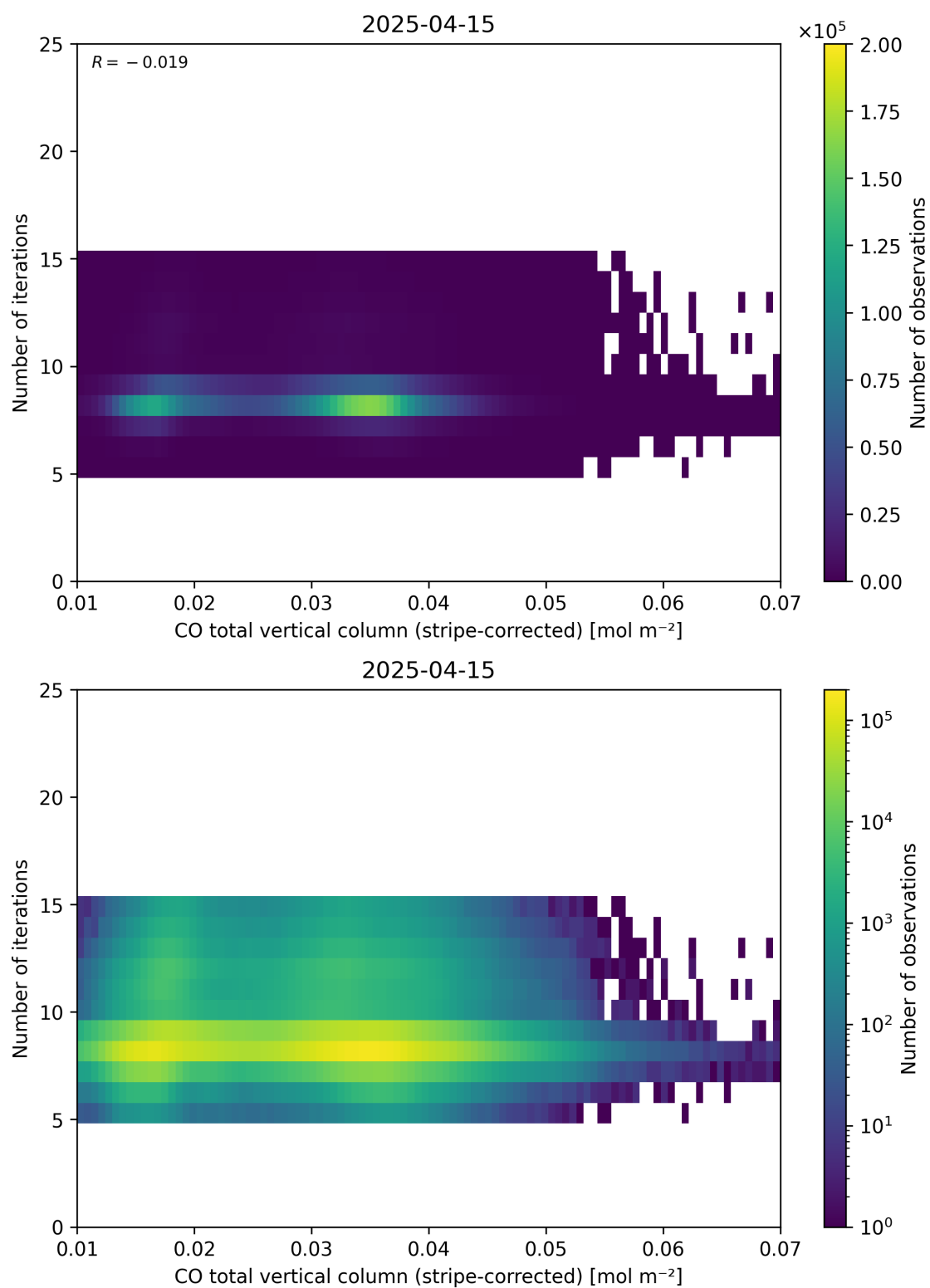
Figure 39: Scatter density plot of “CO total vertical column (stripe-corrected)” against “Number of iterations” for 2025-04-14 to 2025-04-16.
