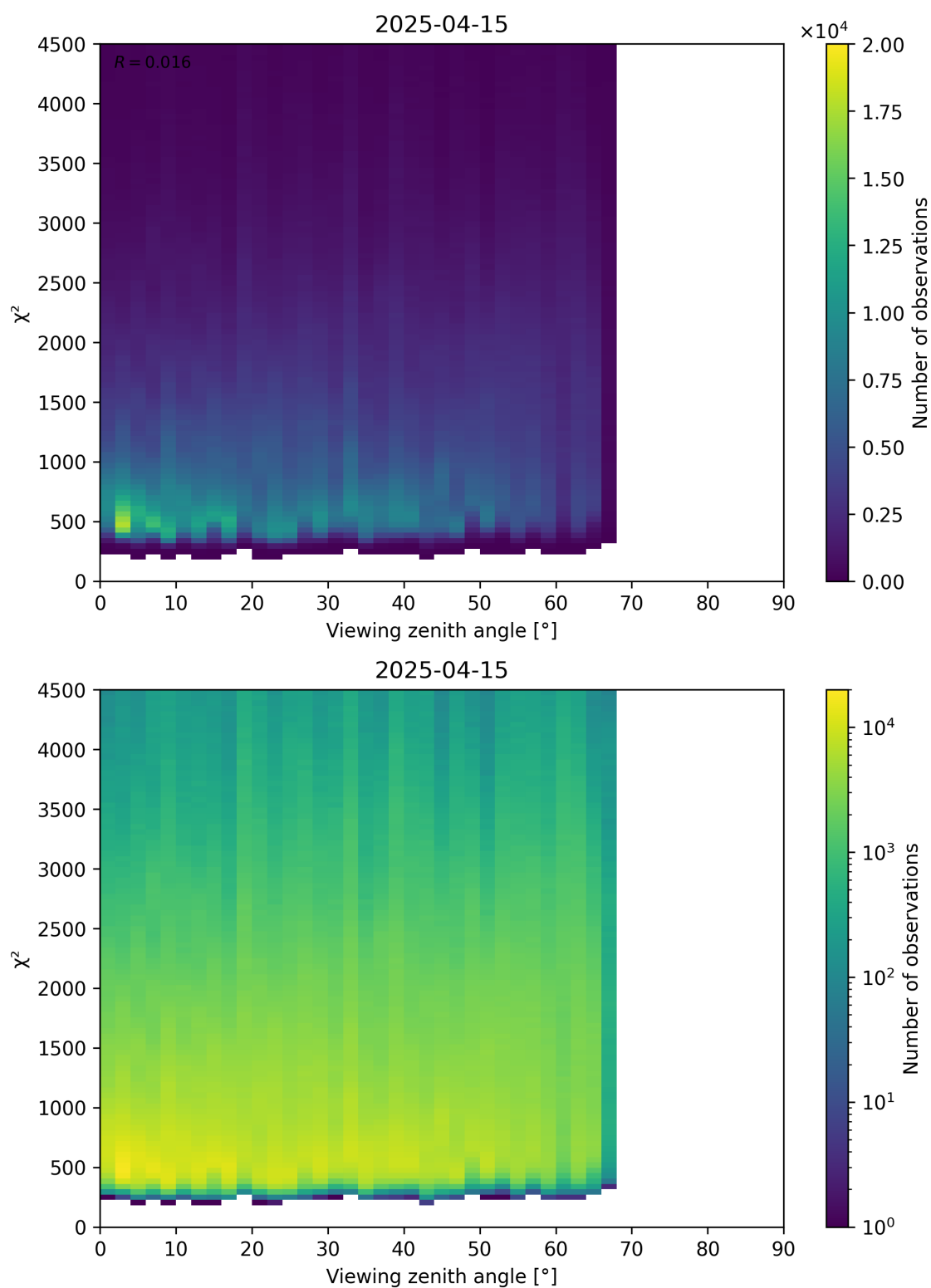
Figure 72: Scatter density plot of “Viewing zenith angle” against “ \chi^2 ” for 2025-04-14 to 2025-04-16.
