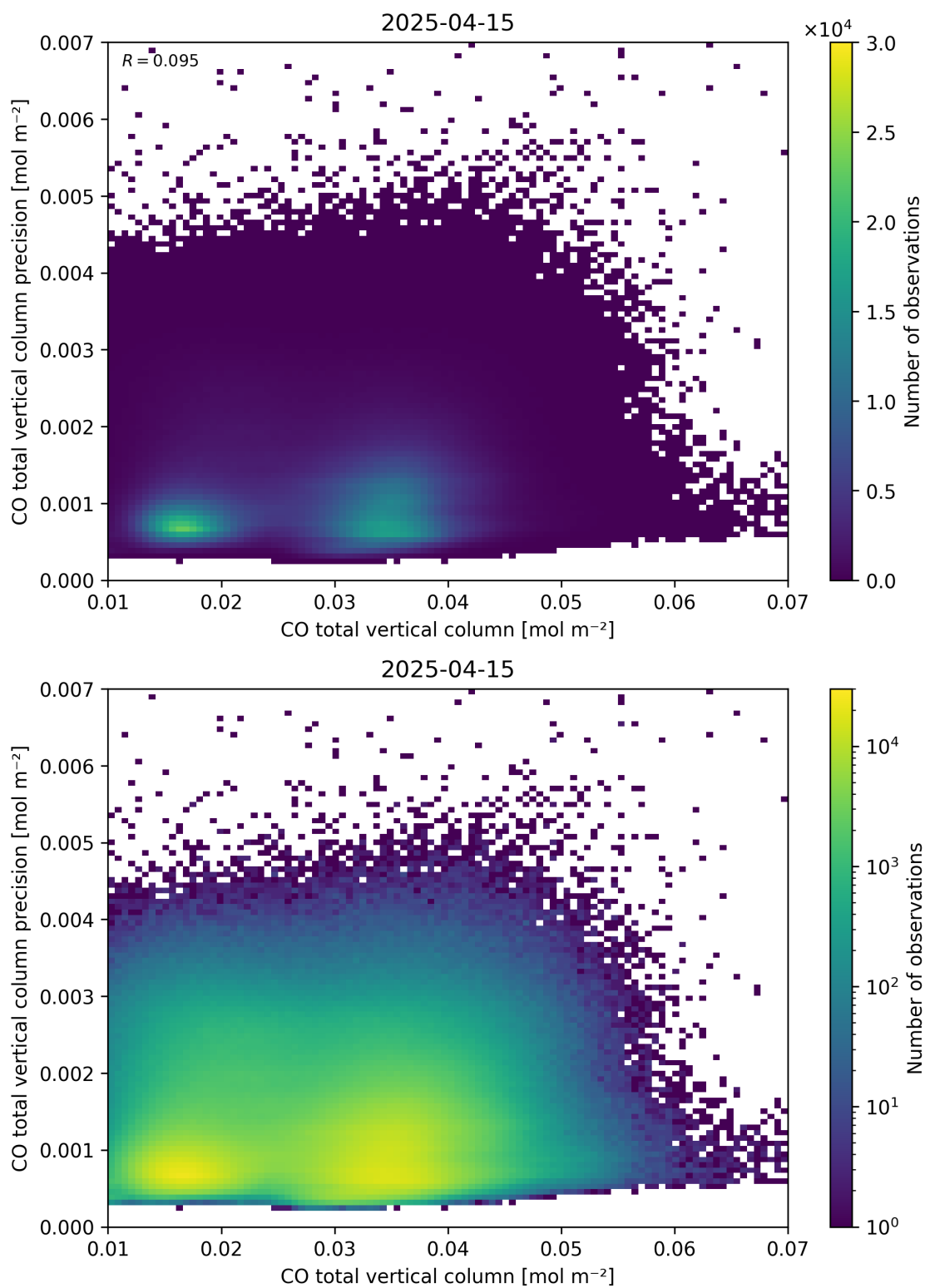
Figure 34: Scatter density plot of “CO total vertical column” against “CO total vertical column precision” for 2025-04-14 to 2025-04-16.
