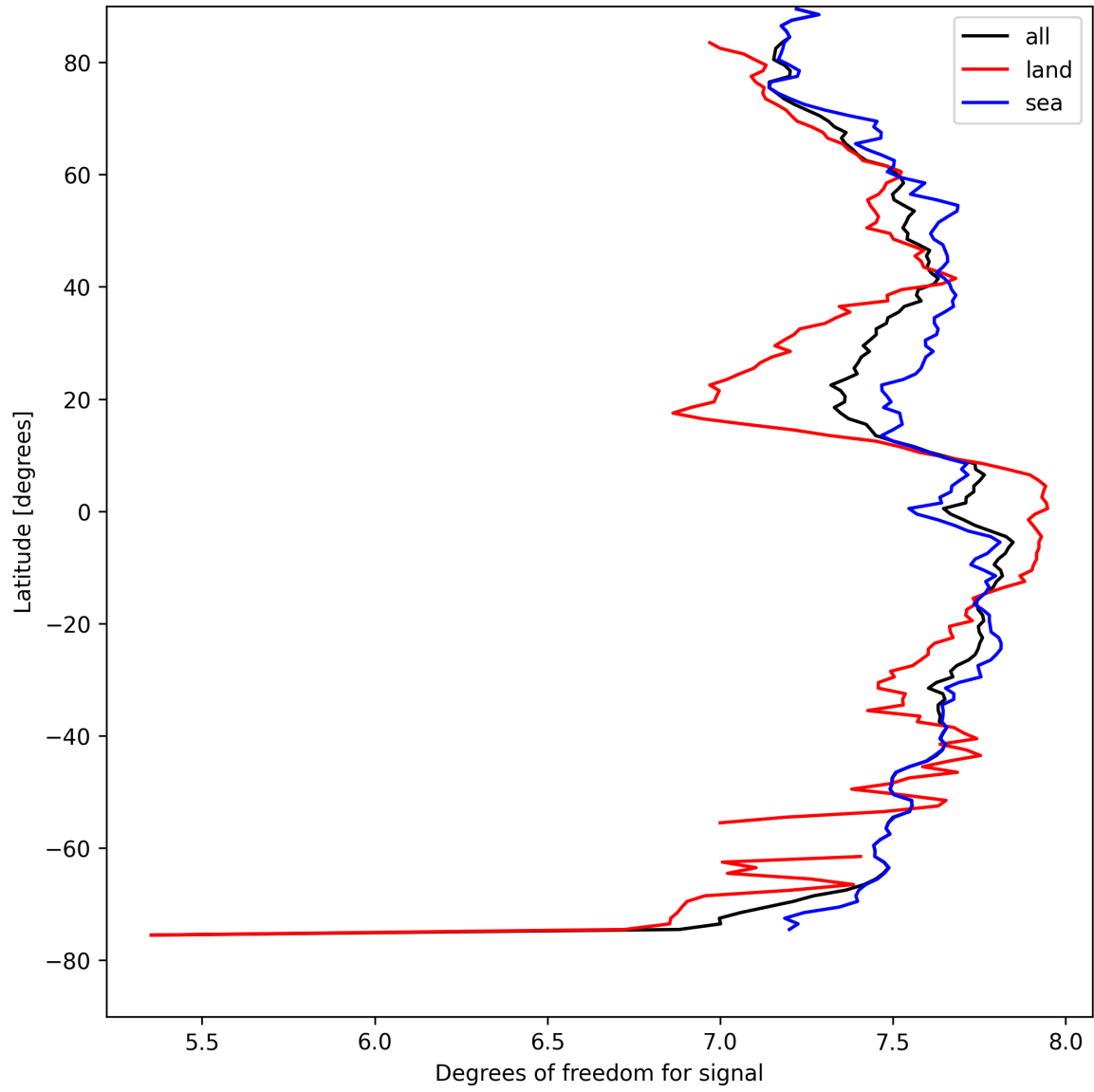
Figure 15: Zonal average of “Degrees of freedom for signal” for 2025-04-14 to 2025-04-16.
