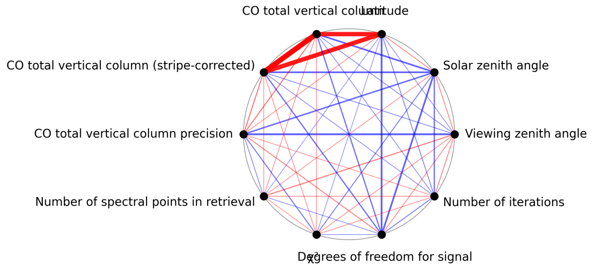
Figure 1: Map of correlation graph for 2025-04-14 to 2025-04-16.
