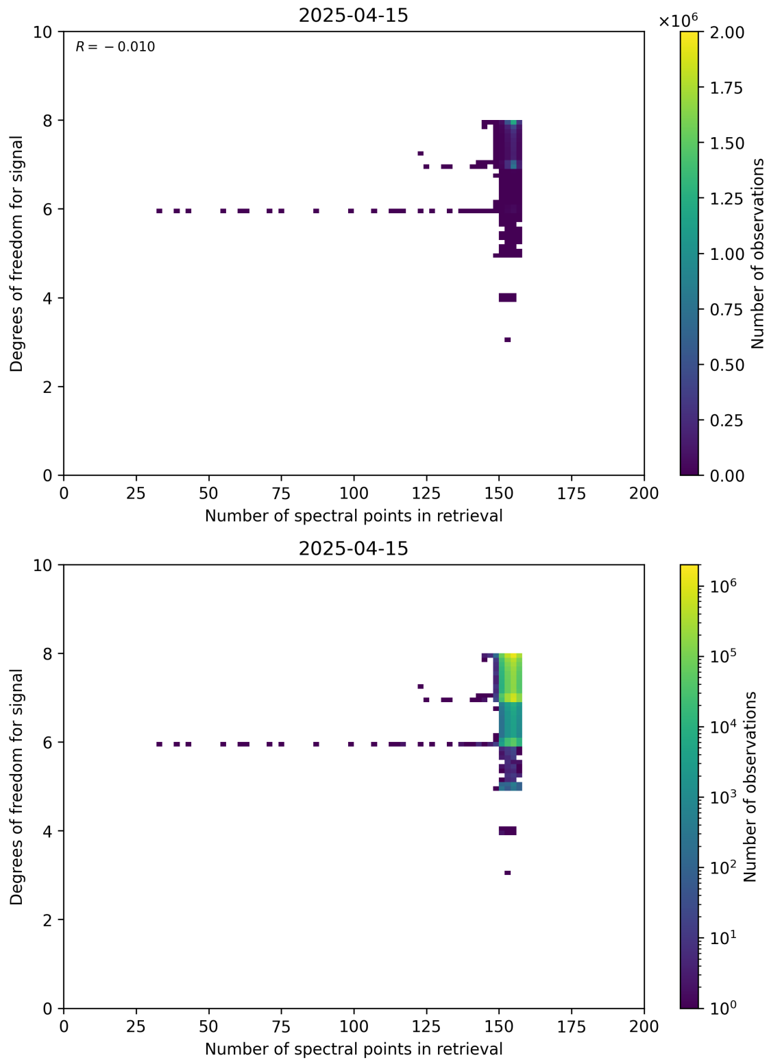
Figure 59: Scatter density plot of “Number of spectral points in retrieval” against “Degrees of freedom for signal” for 2025-04-14 to 2025-04-16.
