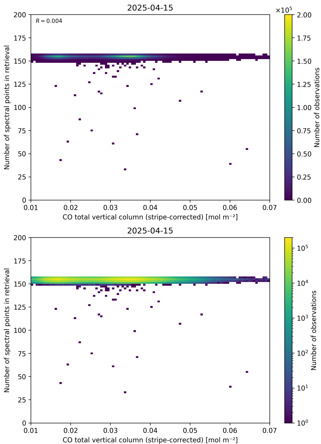
Figure 40: Scatter density plot of “CO total vertical column (stripe-corrected)” against “Number of spectral points in retrieval” for 2025-04-14 to 2025-04-16.
