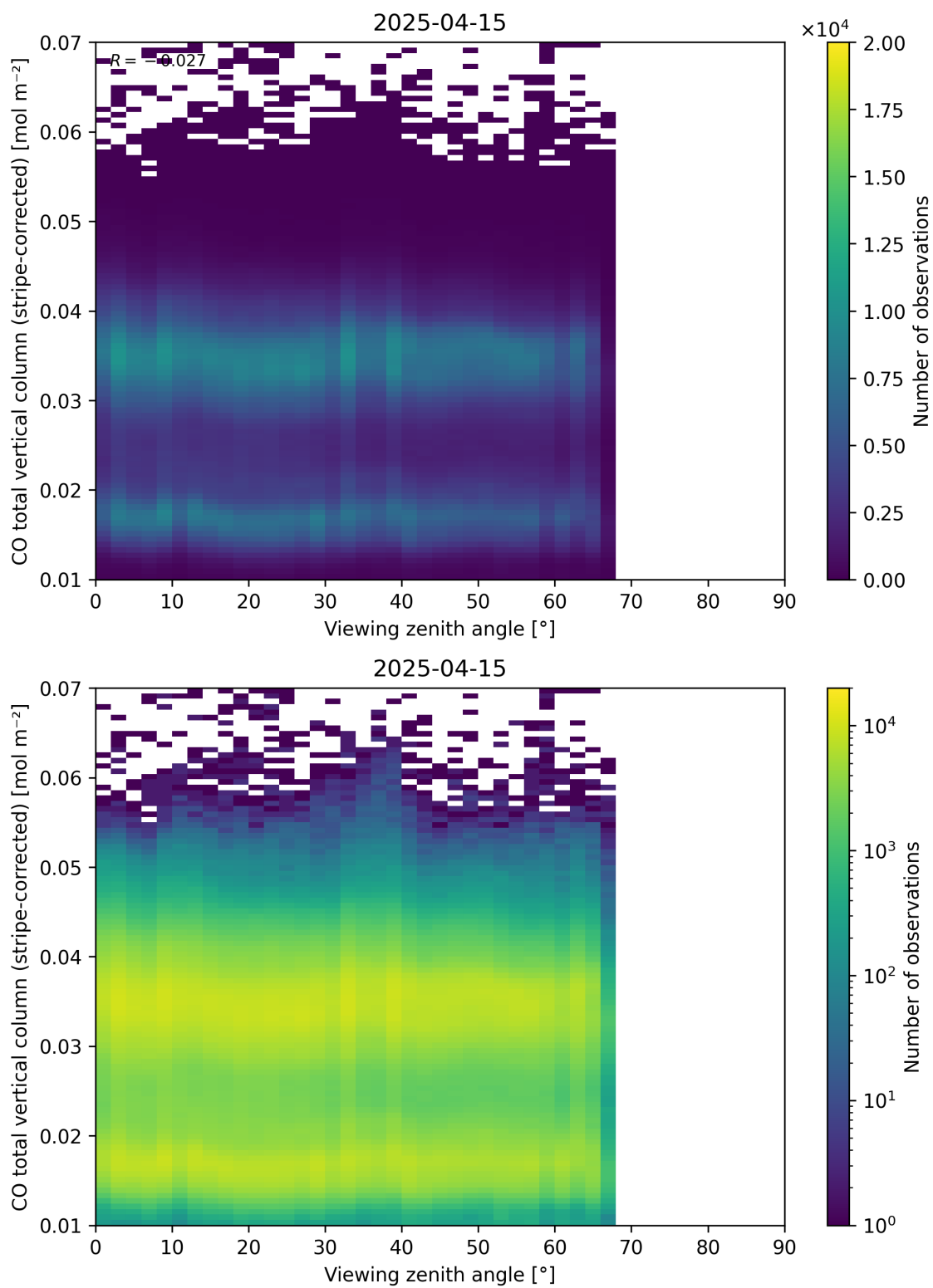
Figure 70: Scatter density plot of “Viewing zenith angle” against “CO total vertical column (stripe-corrected)” for 2025-04-14 to 2025-04-16.
