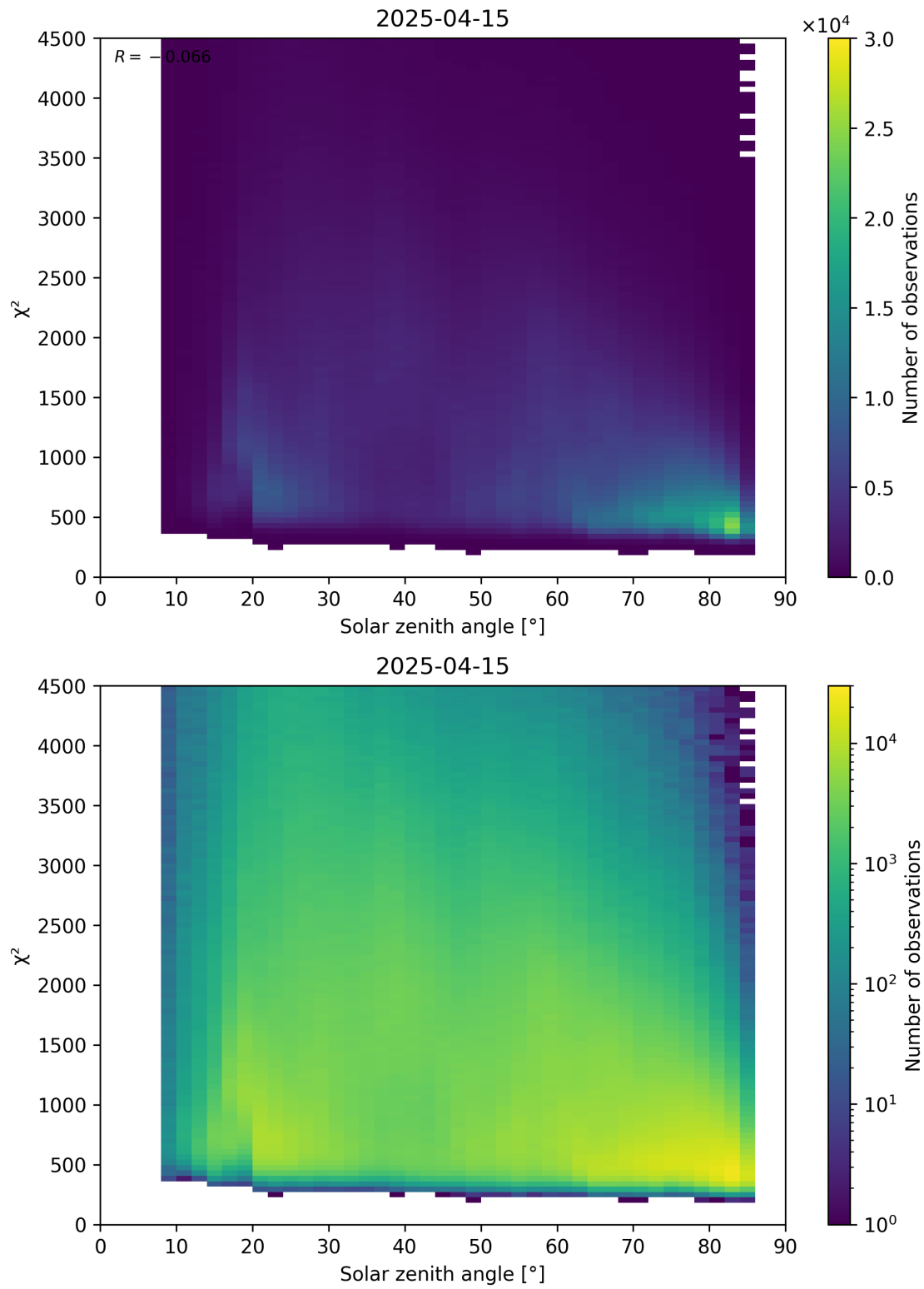
Figure 64: Scatter density plot of “Solar zenith angle” against “ \chi^2 ” for 2025-04-14 to 2025-04-16.
