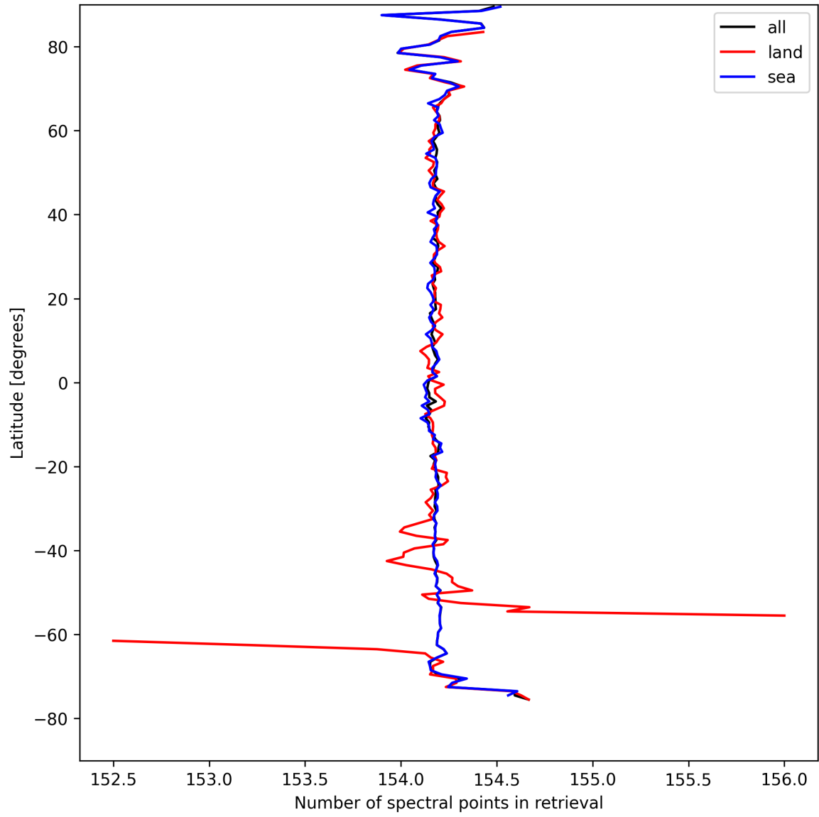
Figure 13: Zonal average of “Number of spectral points in retrieval” for 2025-04-14 to 2025-04-16.
