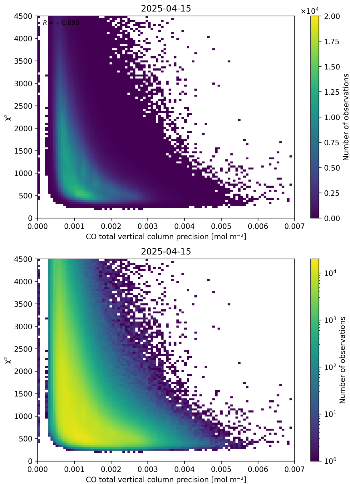
Figure 44: Scatter density plot of “CO total vertical column precision” against “ \chi^2 ” for 2025-04-14 to 2025-04-16.
