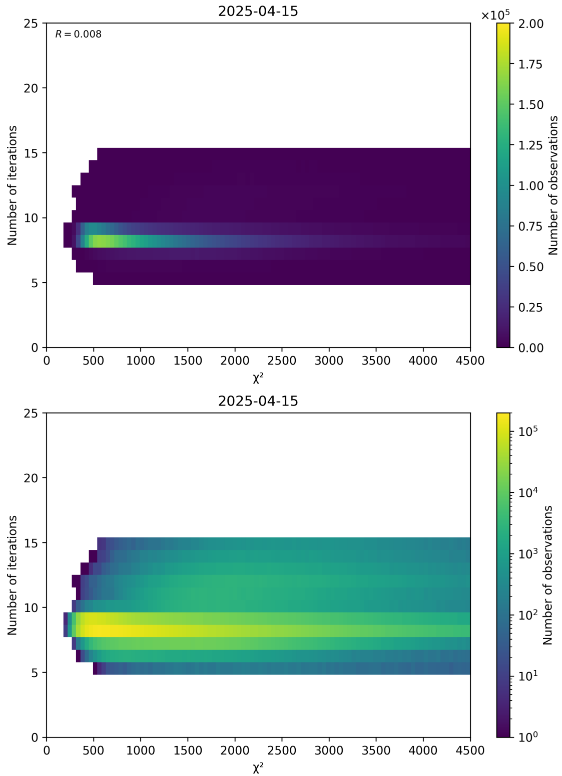
Figure 49: Scatter density plot of “ \chi^2 ” against “Number of iterations” for 2025-04-14 to 2025-04-16.
