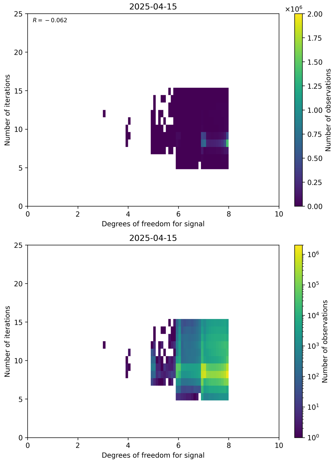
Figure 50: Scatter density plot of “Degrees of freedom for signal” against “Number of iterations” for 2025-04-14 to 2025-04-16.
