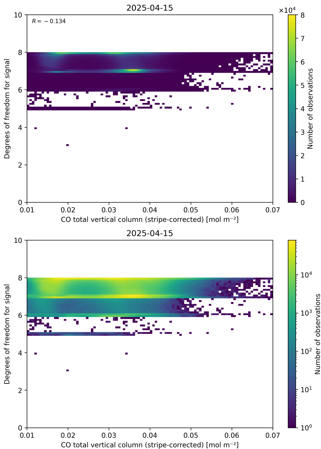
Figure 38: Scatter density plot of “CO total vertical column (stripe-corrected)” against “Degrees of freedom for signal” for 2025-04-14 to 2025-04-16.
