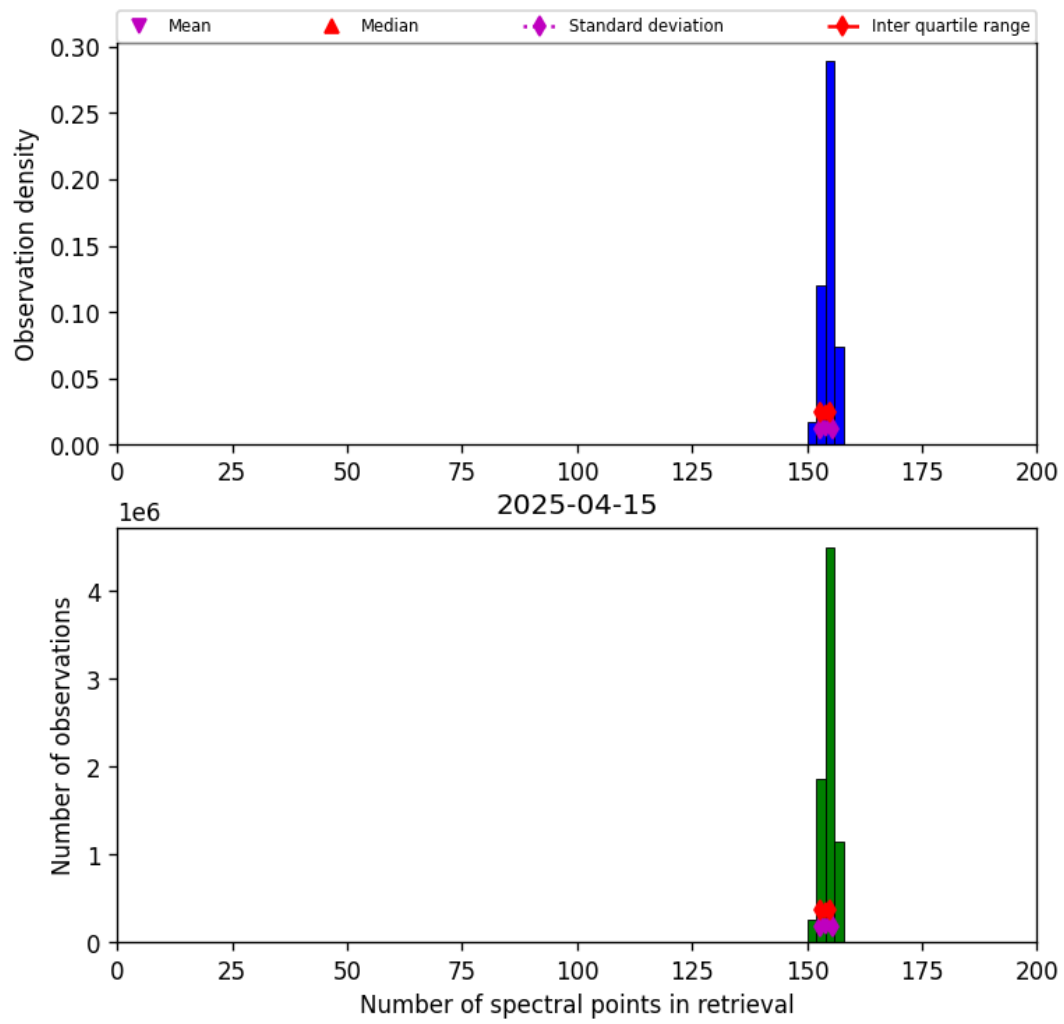
Figure 21: Histogram of “Number of spectral points in retrieval” for 2025-04-14 to 2025-04-16
