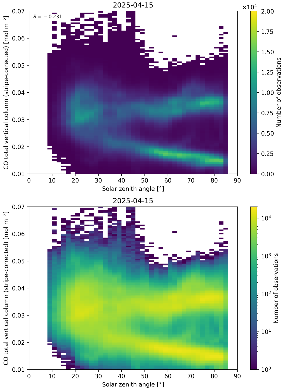
Figure 62: Scatter density plot of “Solar zenith angle” against “CO total vertical column (stripe-corrected)” for 2025-04-14 to 2025-04-16.
