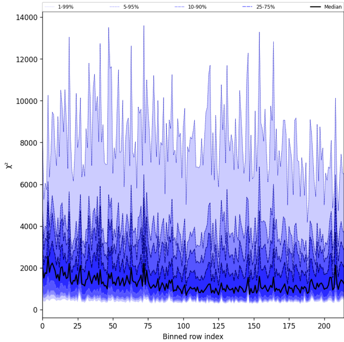
Figure 30: Along track statistics of “ \chi^2 ” for 2025-04-14 to 2025-04-16
