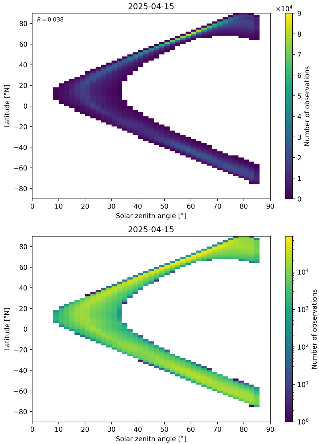
Figure 66: Scatter density plot of “Solar zenith angle” against “Latitude” for 2025-04-14 to 2025-04-16.
