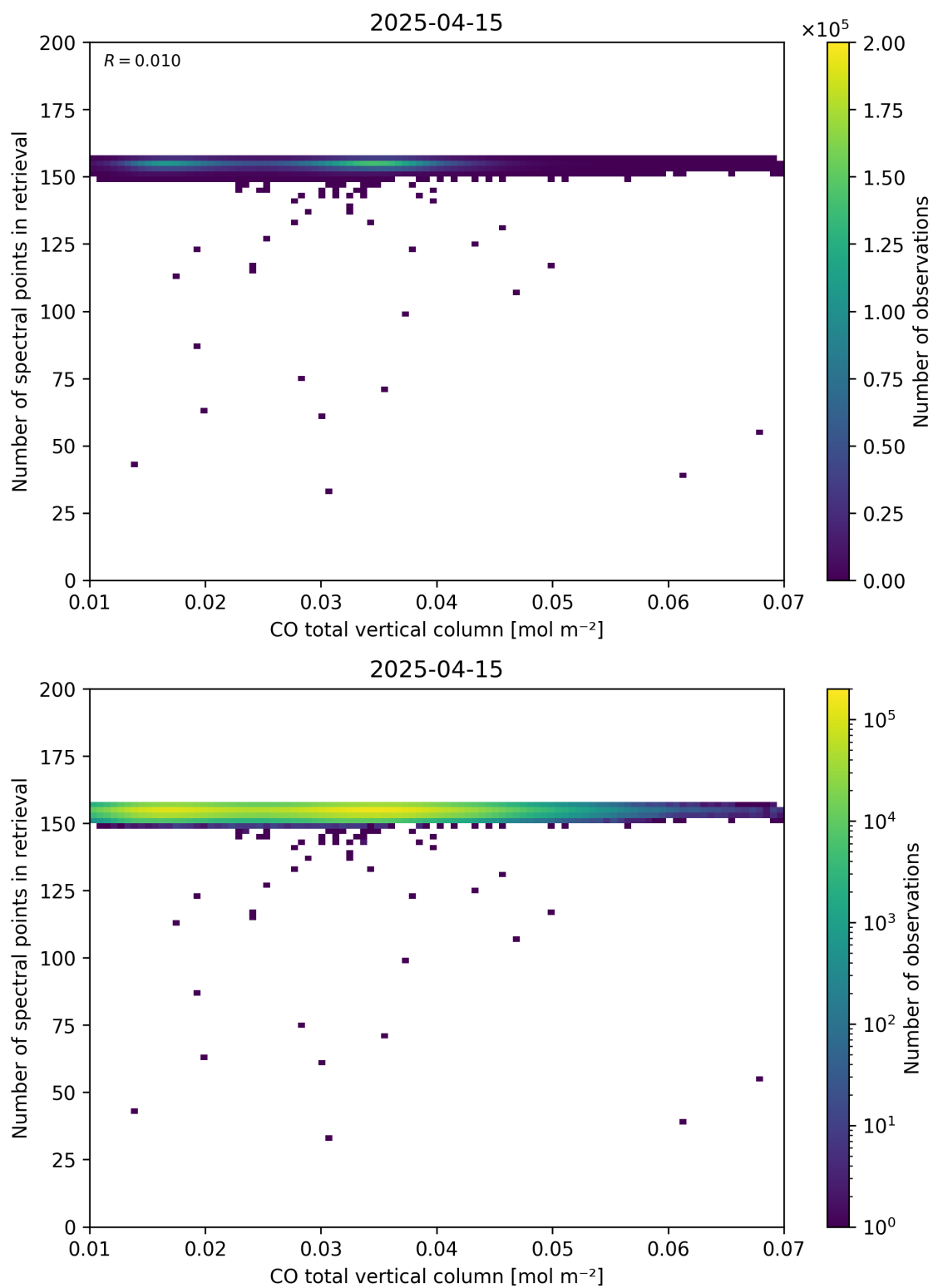
Figure 43: Scatter density plot of “CO total vertical column” against “Number of spectral points in retrieval” for 2025-04-14 to 2025-04-16.
