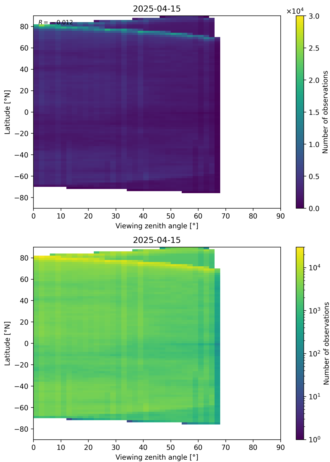
Figure 74: Scatter density plot of “Viewing zenith angle” against “Latitude” for 2025-04-14 to 2025-04-16.
