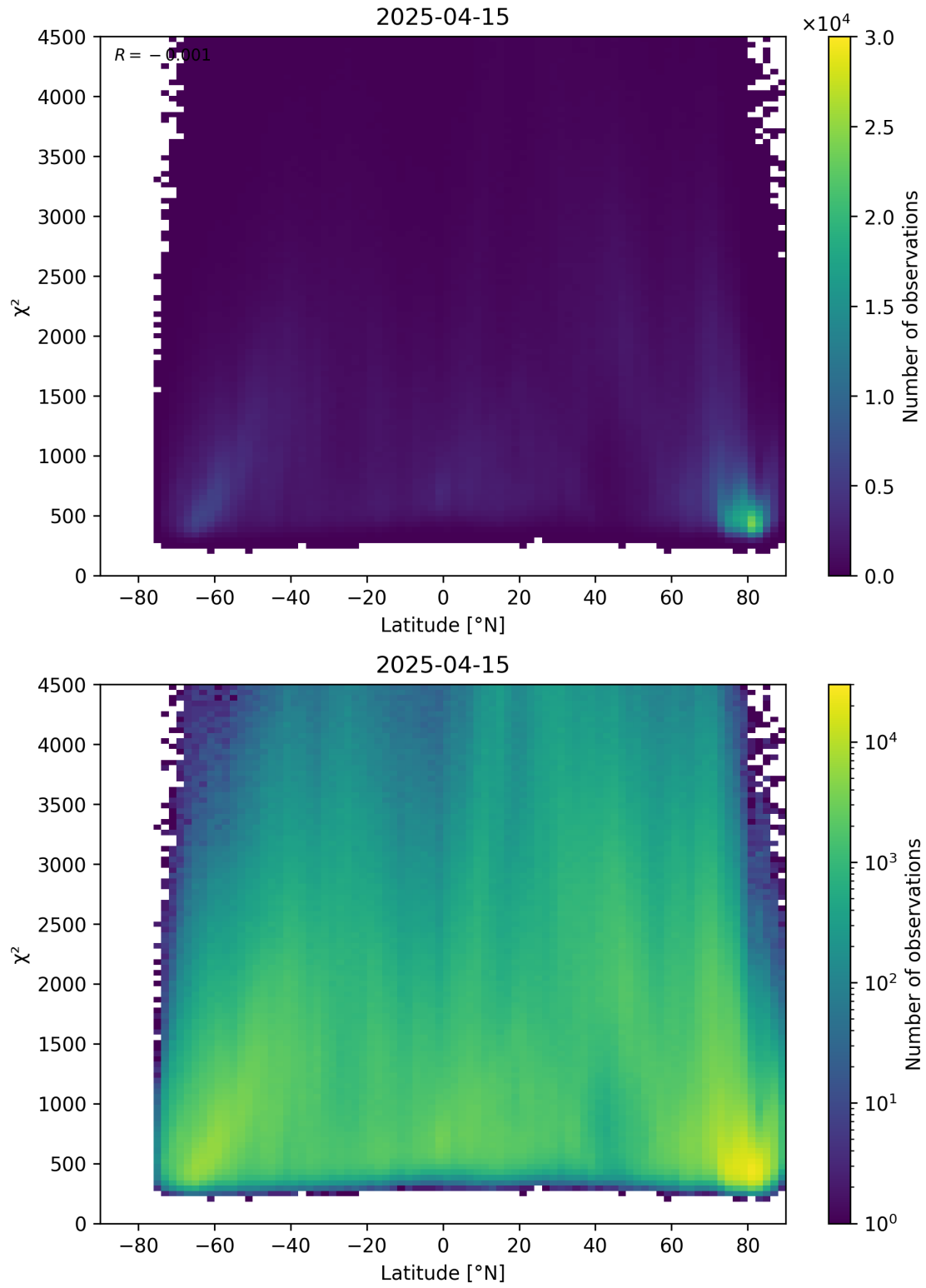
Figure 54: Scatter density plot of “Latitude” against “ \chi^2 ” for 2025-04-14 to 2025-04-16.
