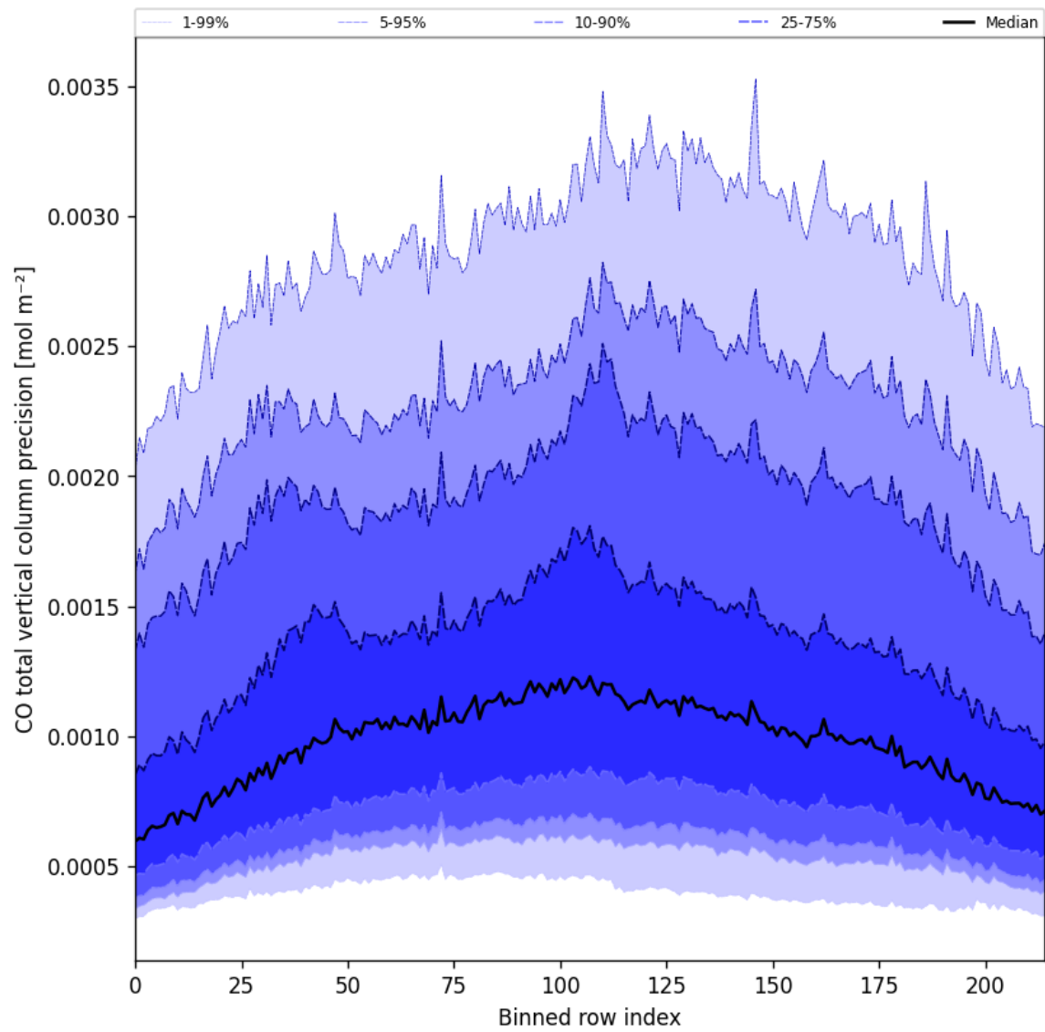
Figure 28: Along track statistics of “CO total vertical column precision” for 2025-04-14 to 2025-04-16
