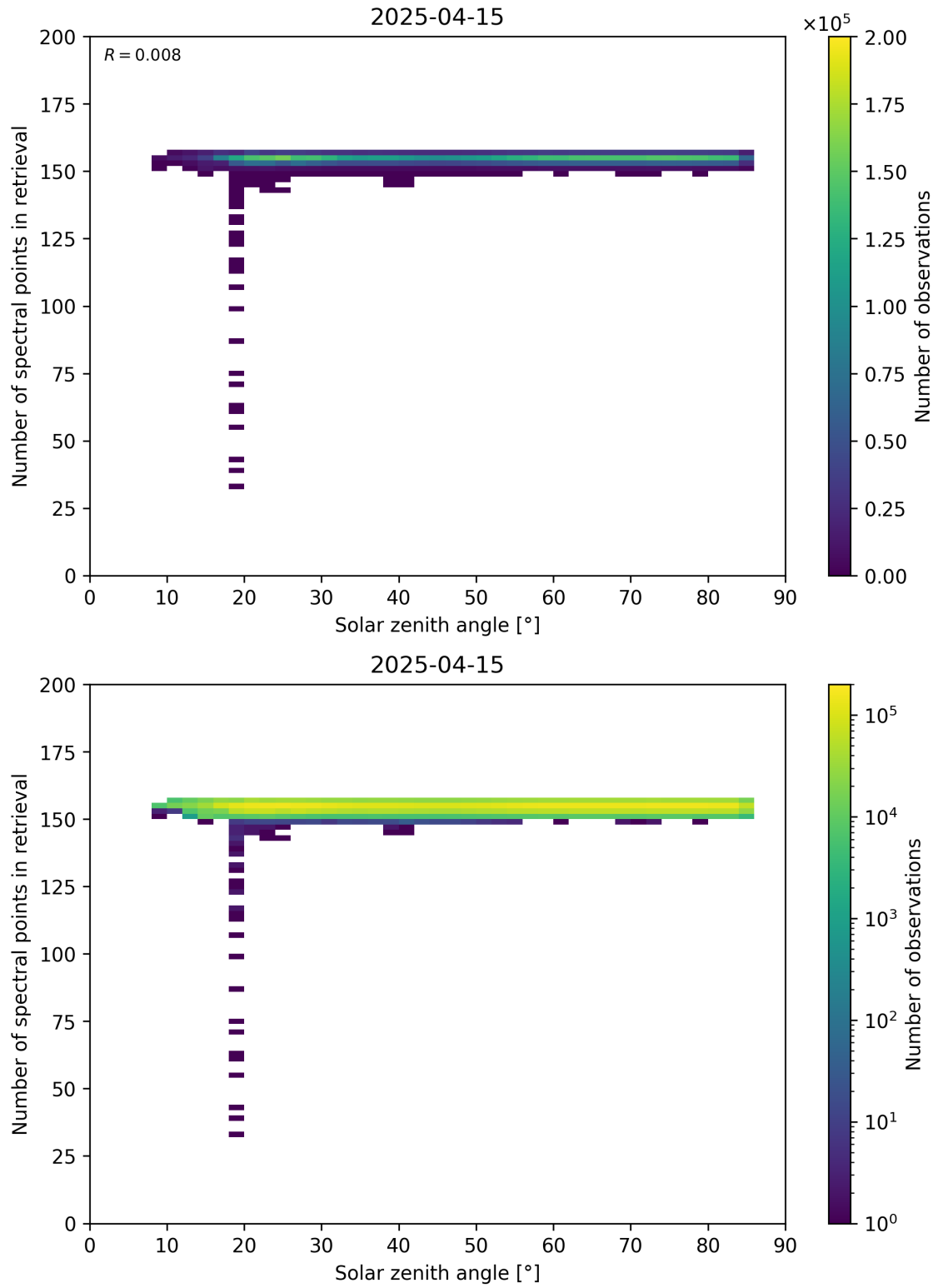
Figure 68: Scatter density plot of “Solar zenith angle” against “Number of spectral points in retrieval” for 2025-04-14 to 2025-04-16.
