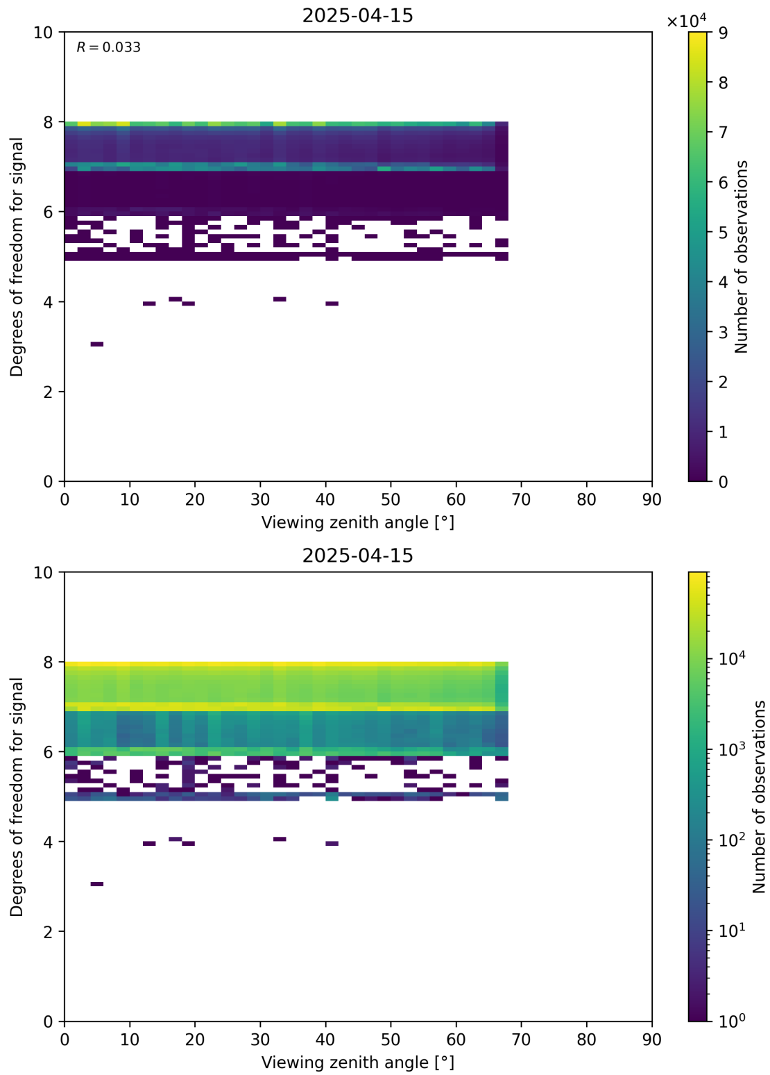
Figure 73: Scatter density plot of “Viewing zenith angle” against “Degrees of freedom for signal” for 2025-04-14 to 2025-04-16.
