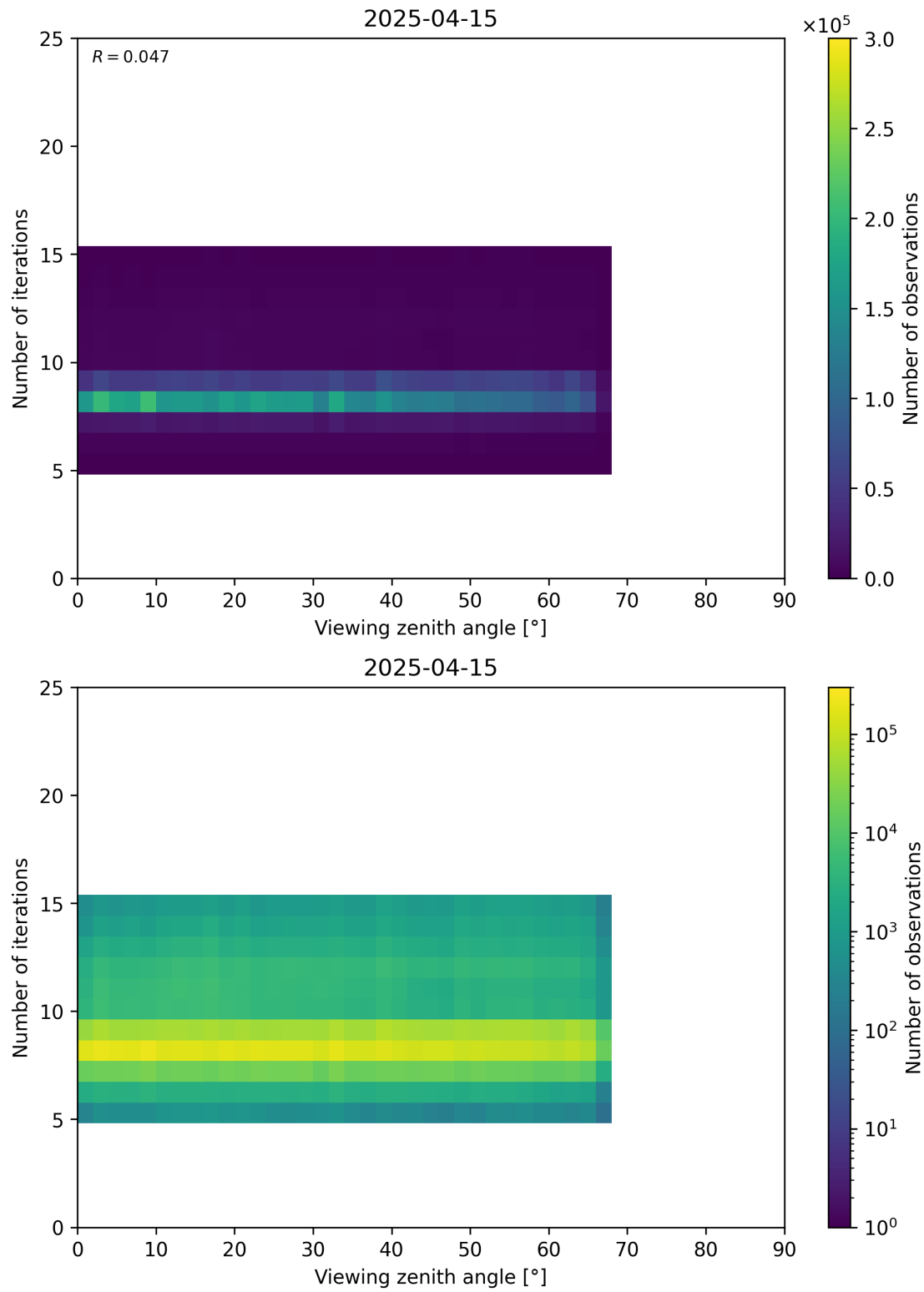
Figure 75: Scatter density plot of “Viewing zenith angle” against “Number of iterations” for 2025-04-14 to 2025-04-16.
