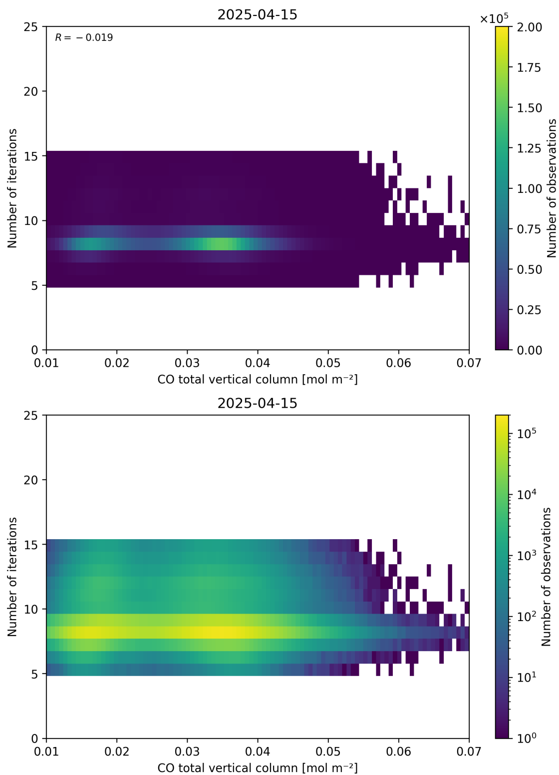
Figure 42: Scatter density plot of “CO total vertical column” against “Number of iterations” for 2025-04-14 to 2025-04-16.
