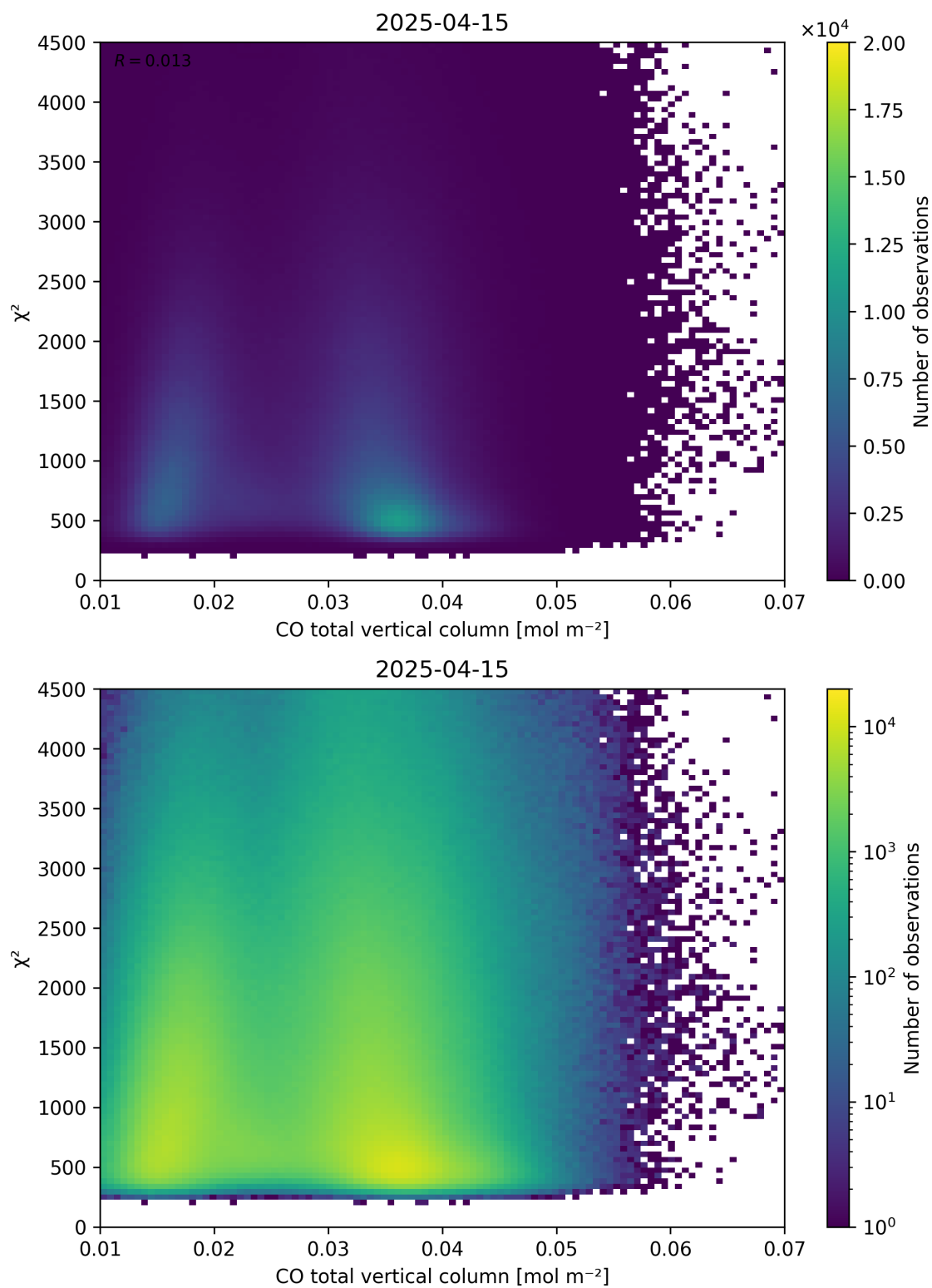
Figure 35: Scatter density plot of “CO total vertical column” against “ \chi^2 ” for 2025-04-14 to 2025-04-16.
