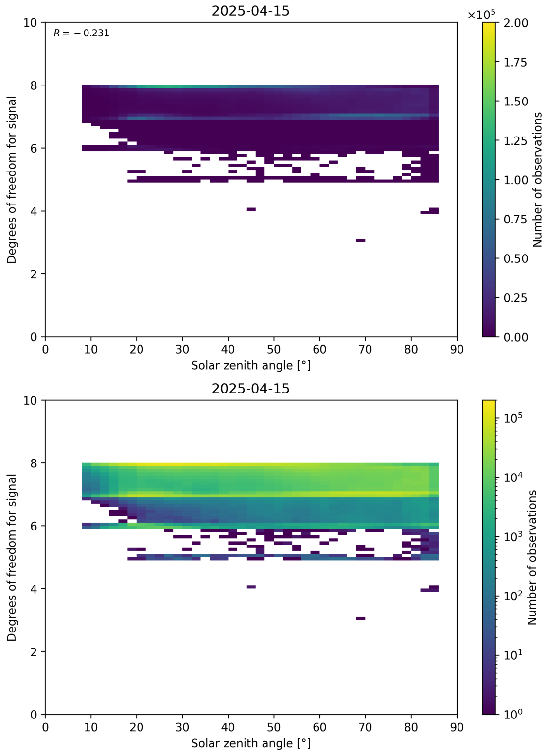
Figure 65: Scatter density plot of “Solar zenith angle” against “Degrees of freedom for signal” for 2025-04-14 to 2025-04-16.
