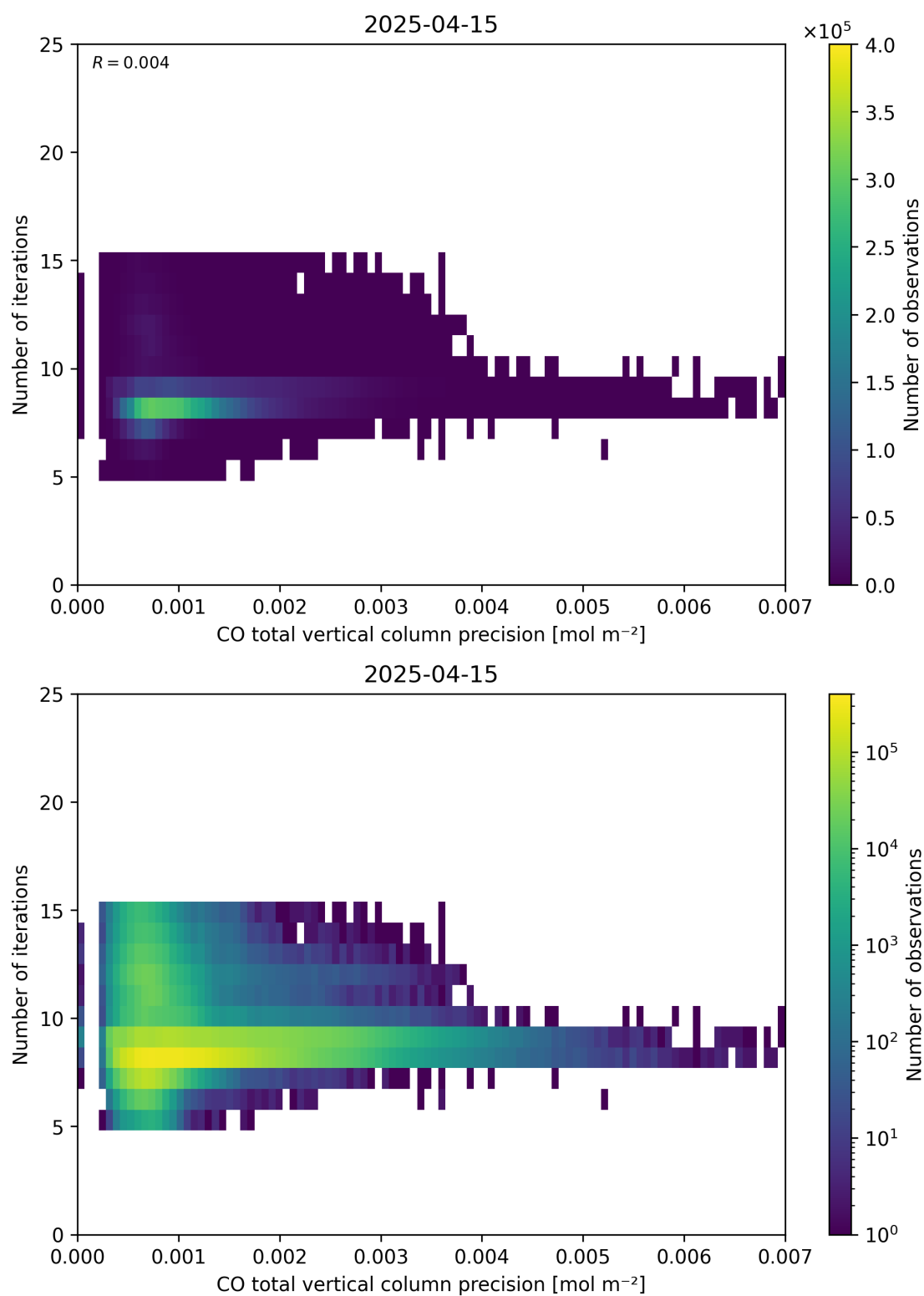
Figure 46: Scatter density plot of “CO total vertical column precision” against “Number of iterations” for 2025-04-14 to 2025-04-16.
