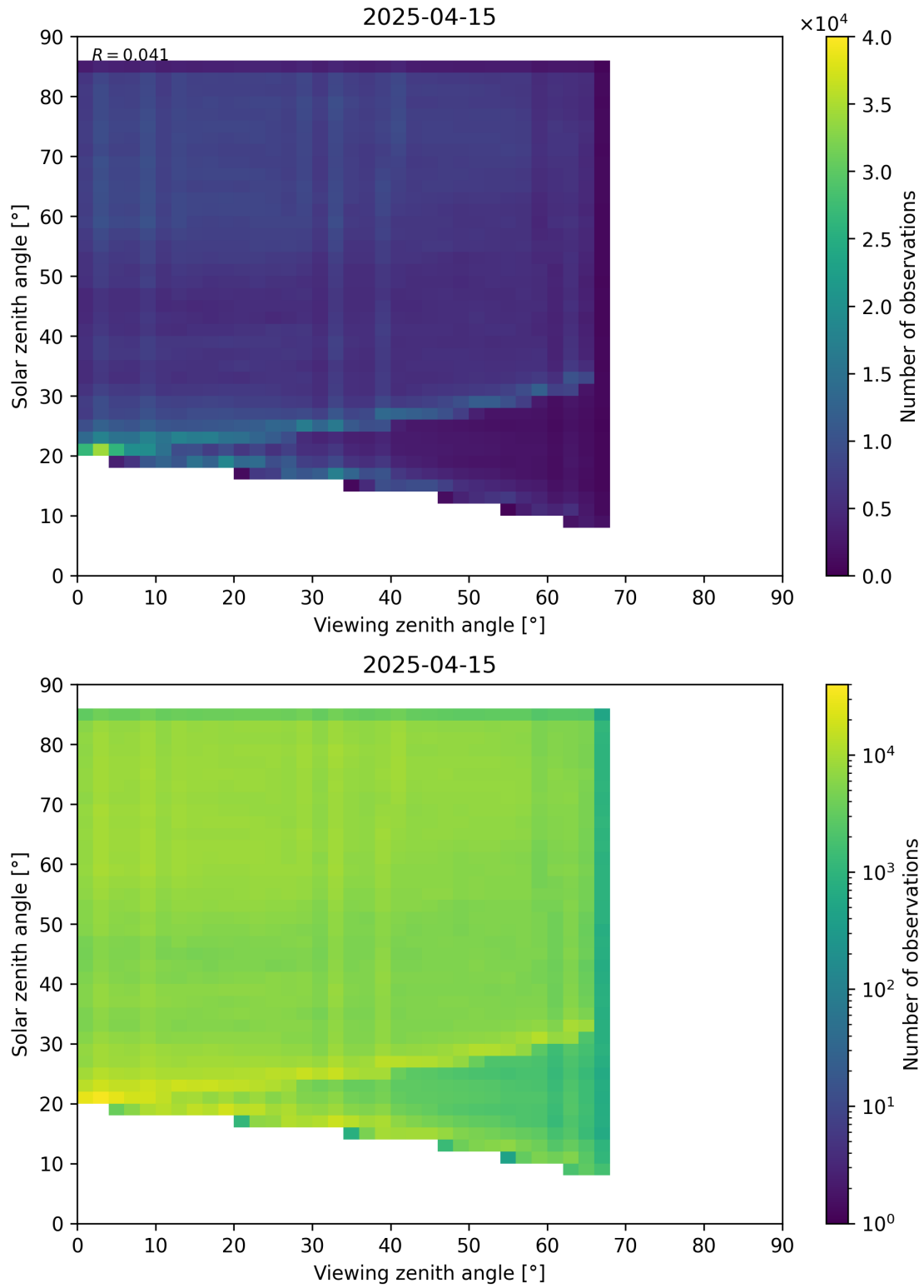
Figure 77: Scatter density plot of “Viewing zenith angle” against “Solar zenith angle” for 2025-04-14 to 2025-04-16.
