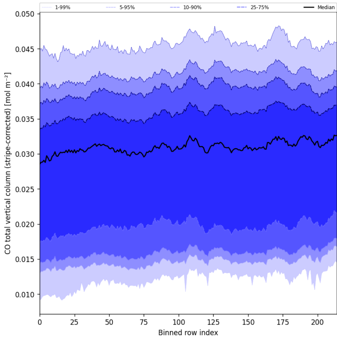
Figure 27: Along track statistics of “CO total vertical column (stripe-corrected)” for 2025-04-14 to 2025-04-16
