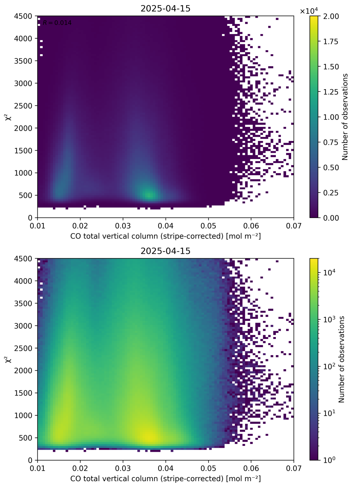
Figure 37: Scatter density plot of “CO total vertical column (stripe-corrected)” against “ \chi^2 ” for 2025-04-14 to 2025-04-16.
