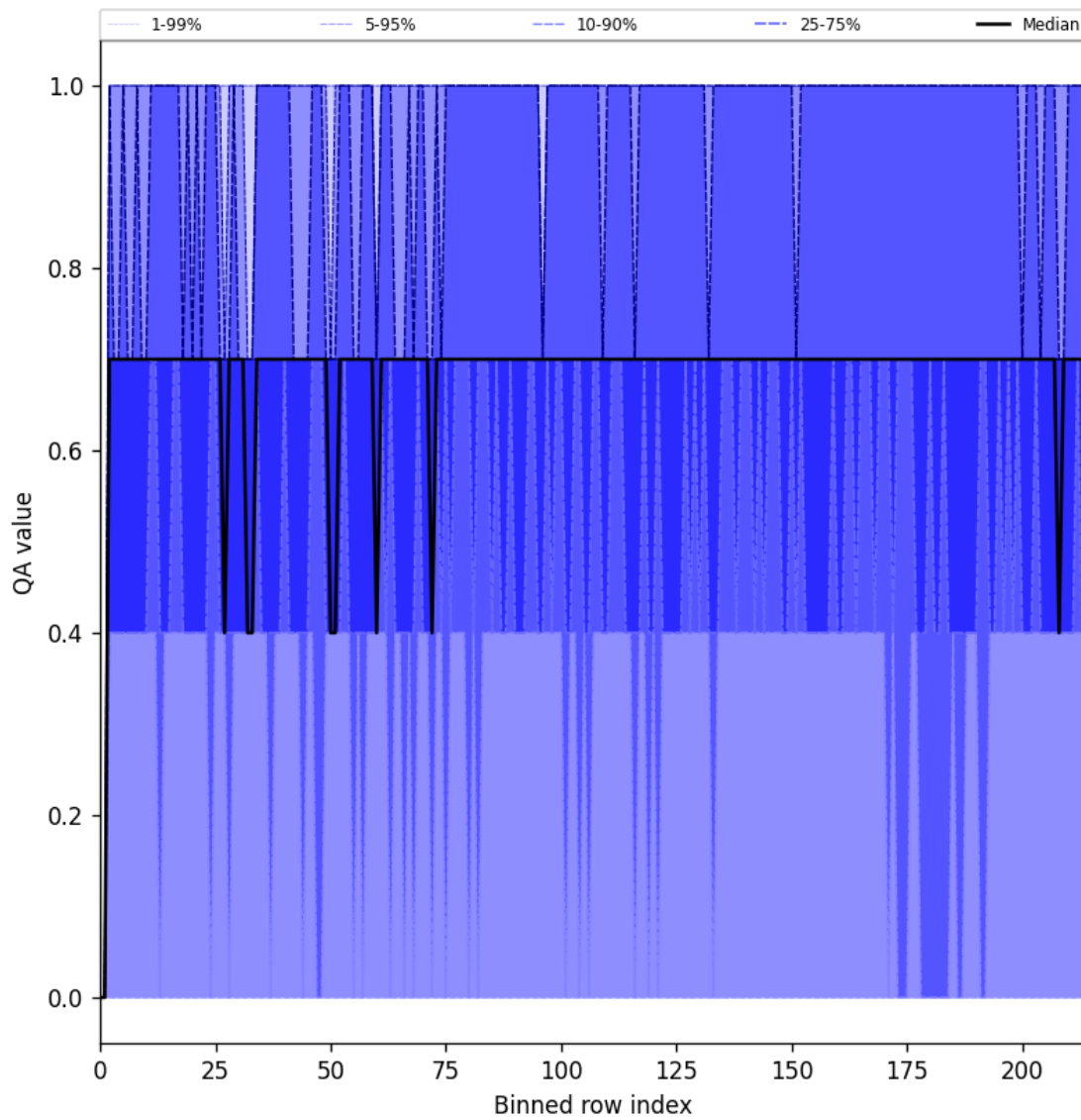
Figure 25: Along track statistics of “QA value” for 2025-04-14 to 2025-04-16
