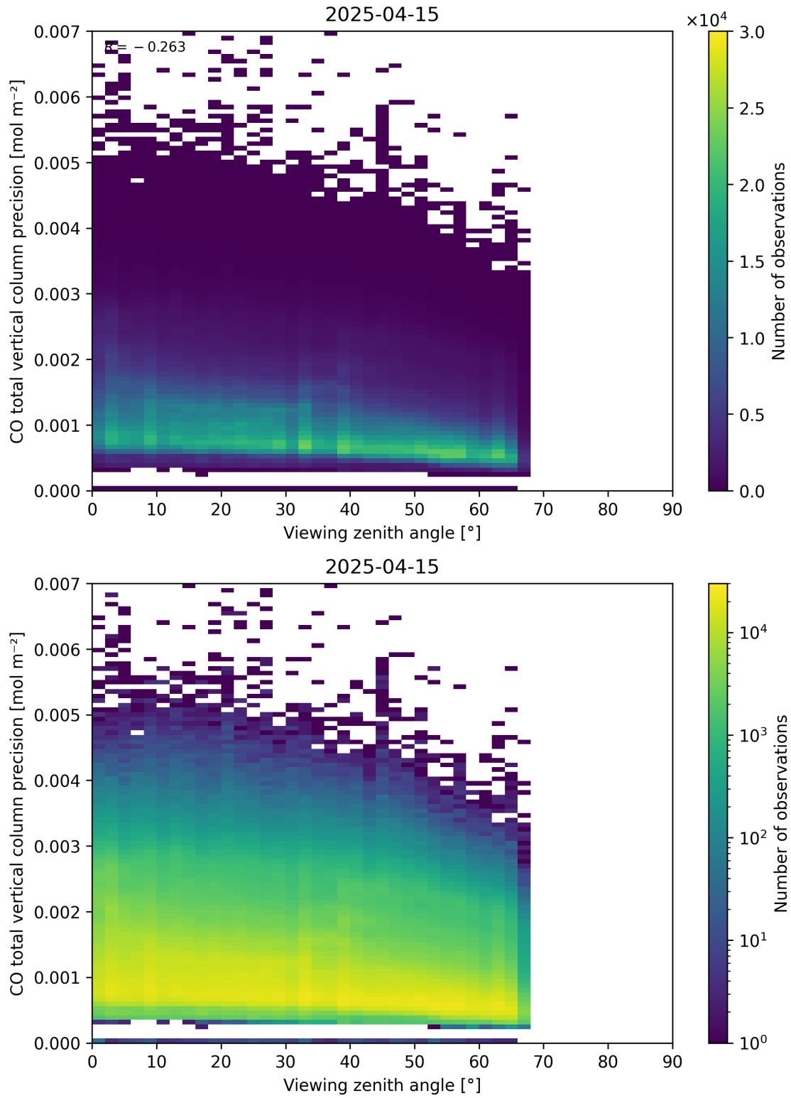
Figure 71: Scatter density plot of “Viewing zenith angle” against “CO total vertical column precision” for 2025-04-14 to 2025-04-16.
