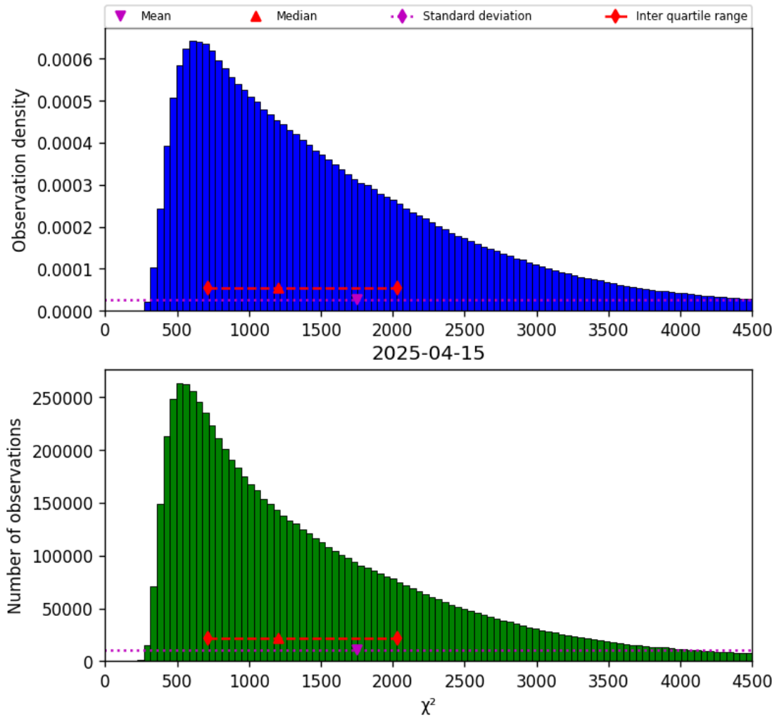
Figure 22: Histogram of “ \chi^2 ” for 2025-04-14 to 2025-04-16
