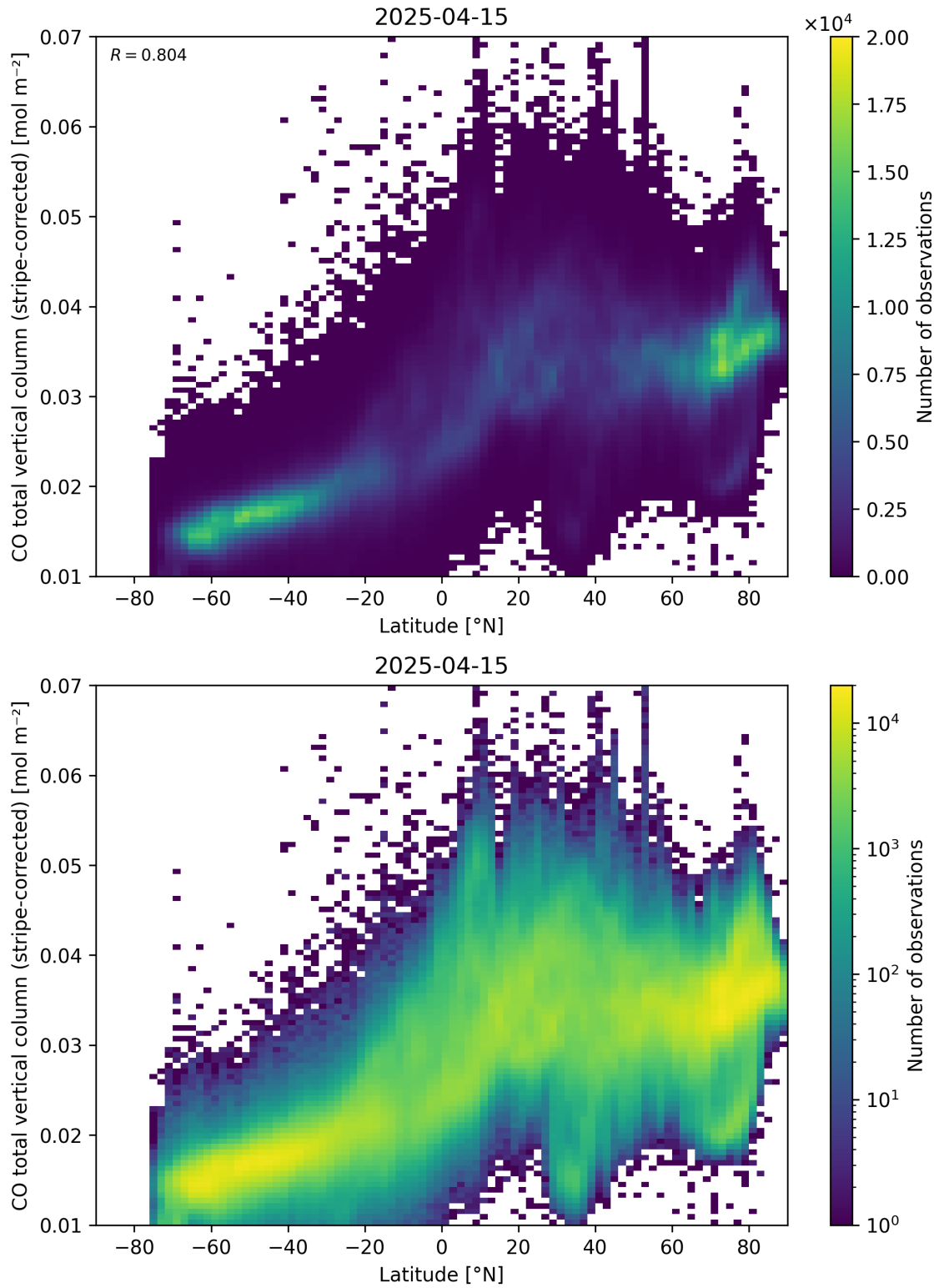
Figure 52: Scatter density plot of “Latitude” against “CO total vertical column (stripe-corrected)” for 2025-04-14 to 2025-04-16.
