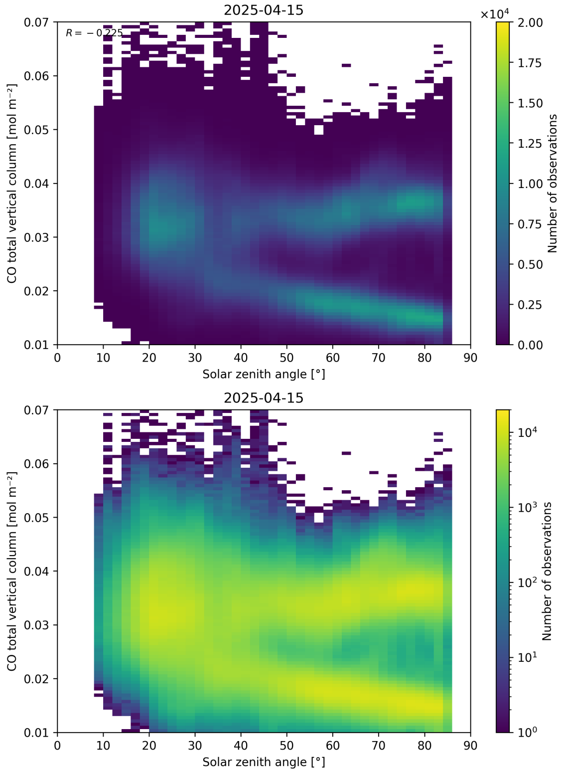
Figure 61: Scatter density plot of “Solar zenith angle” against “CO total vertical column” for 2025-04-14 to 2025-04-16.
