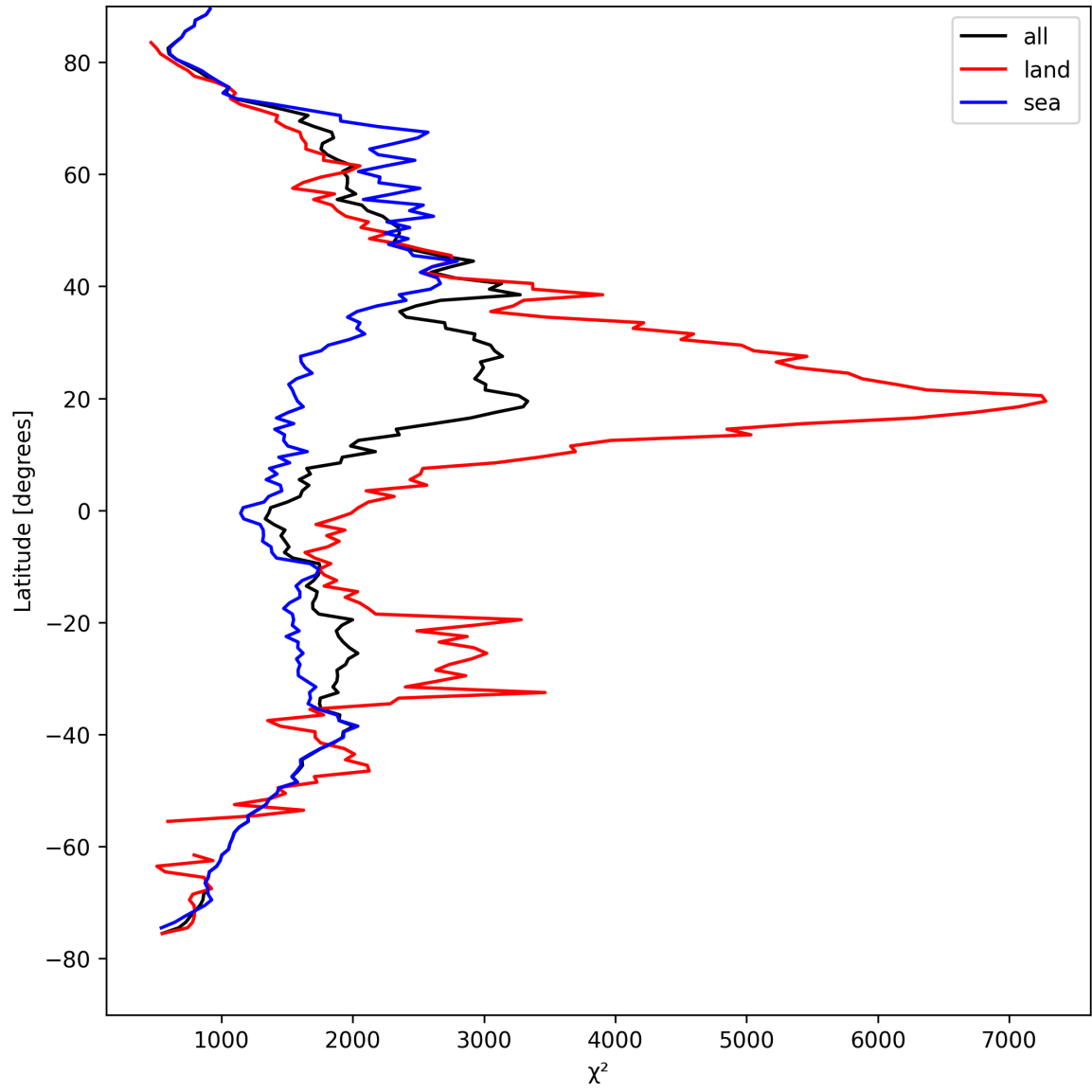
Figure 14: Zonal average of “ \chi^2 ” for 2025-04-14 to 2025-04-16.
