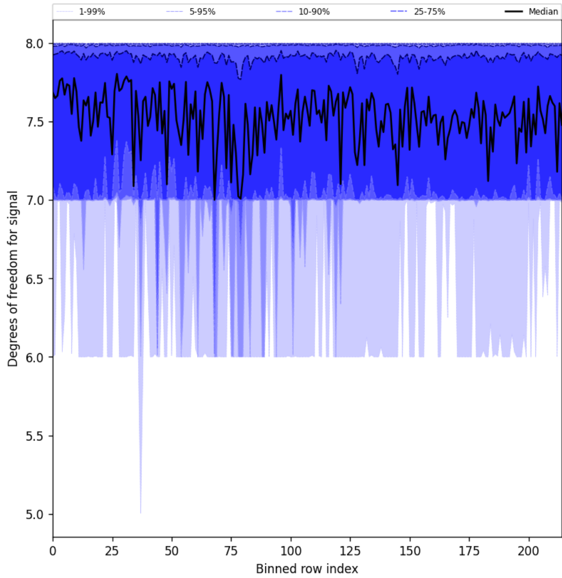
Figure 31: Along track statistics of “Degrees of freedom for signal” for 2025-04-14 to 2025-04-16
