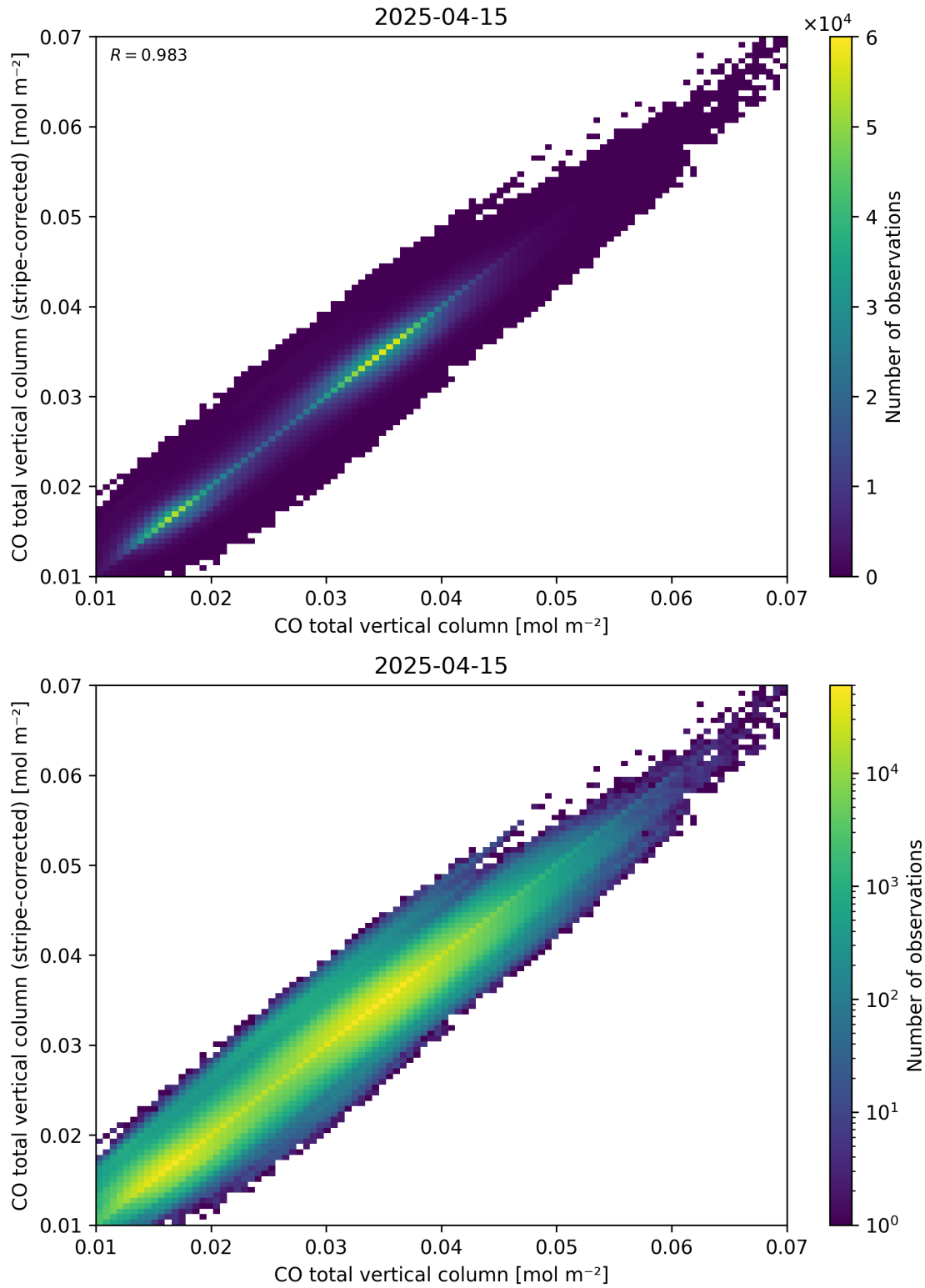
Figure 33: Scatter density plot of “CO total vertical column” against “CO total vertical column (stripe-corrected)” for 2025-04-14 to 2025-04-16.
