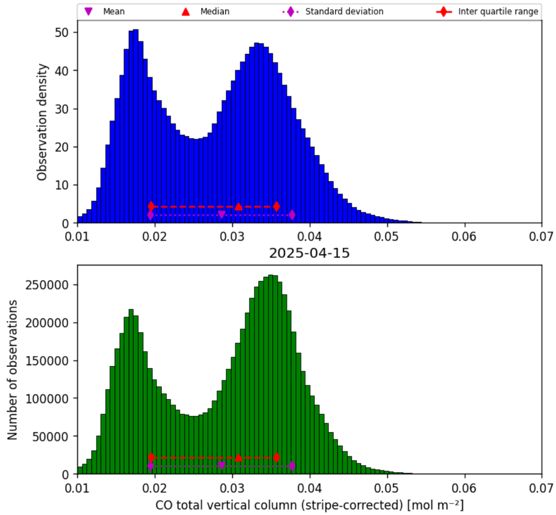
Figure 19: Histogram of “CO total vertical column (stripe-corrected)” for 2025-04-14 to 2025-04-16
