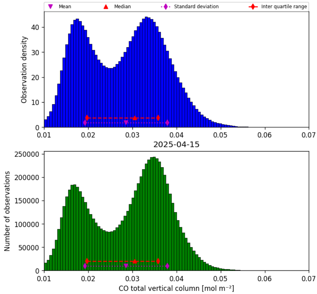
Figure 18: Histogram of “CO total vertical column” for 2025-04-14 to 2025-04-16
