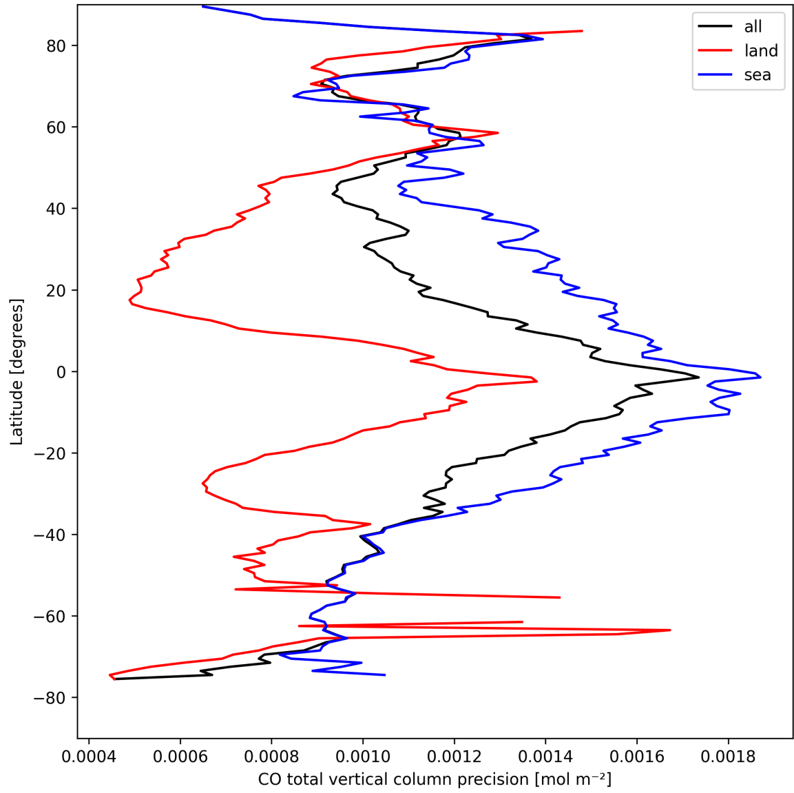
Figure 12: Zonal average of “CO total vertical column precision” for 2025-04-14 to 2025-04-16.
