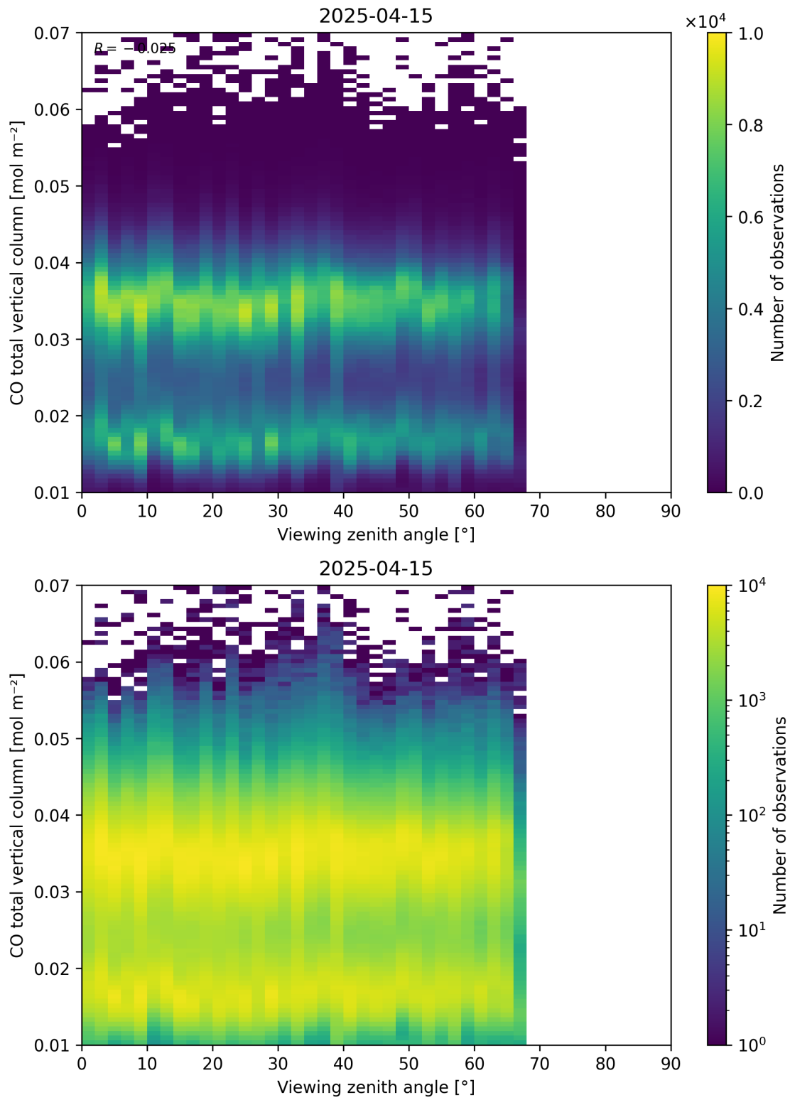
Figure 69: Scatter density plot of “Viewing zenith angle” against “CO total vertical column” for 2025-04-14 to 2025-04-16.
