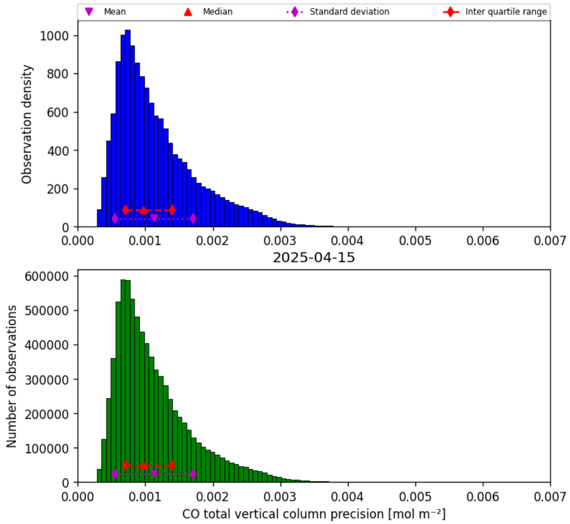
Figure 20: Histogram of “CO total vertical column precision” for 2025-04-14 to 2025-04-16
