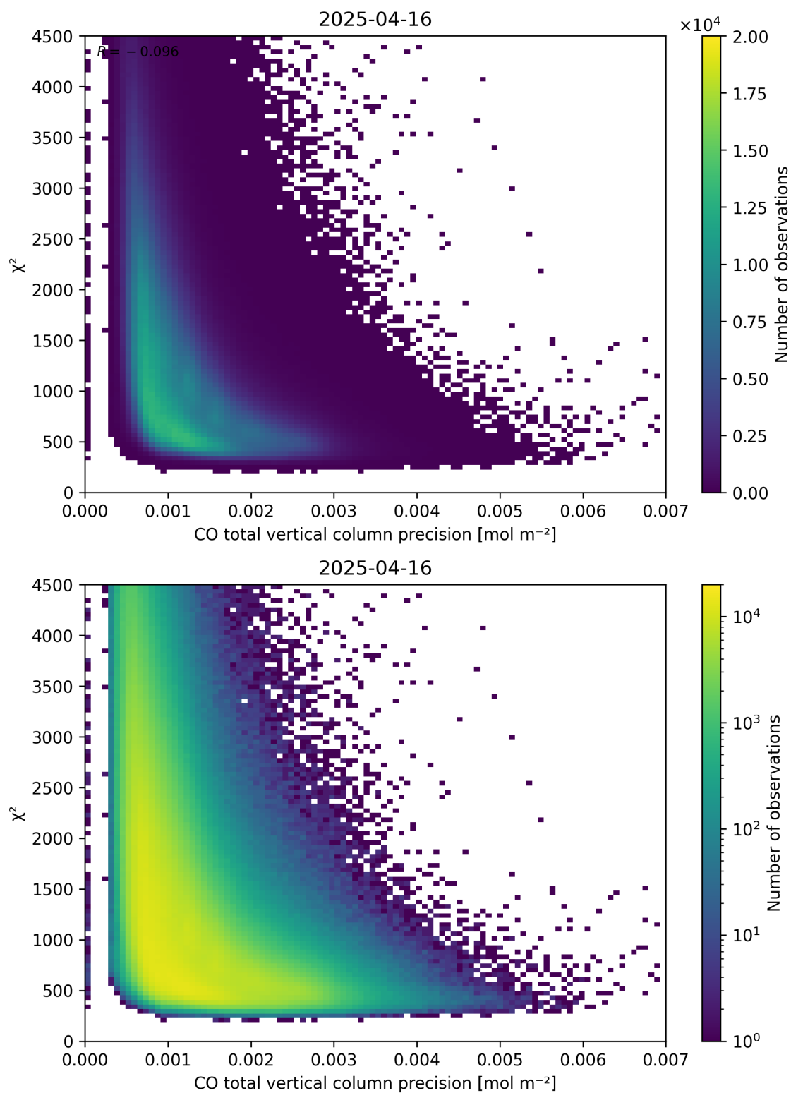
Figure 44: Scatter density plot of “CO total vertical column precision” against “ \chi^2 ” for 2025-04-15 to 2025-04-17.
