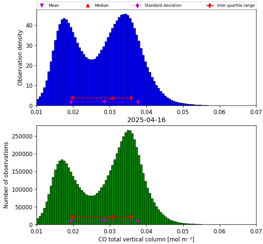
Figure 18: Histogram of “CO total vertical column” for 2025-04-15 to 2025-04-17
