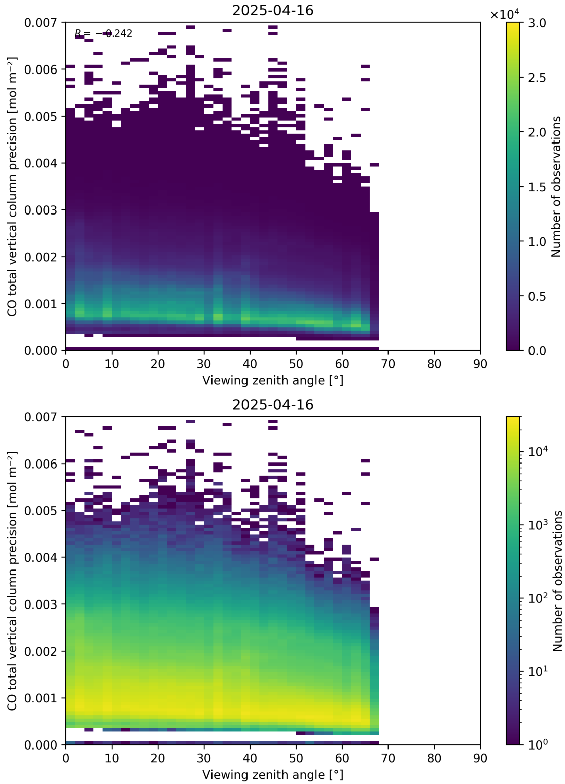
Figure 71: Scatter density plot of “Viewing zenith angle” against “CO total vertical column precision” for 2025-04-15 to 2025-04-17.
