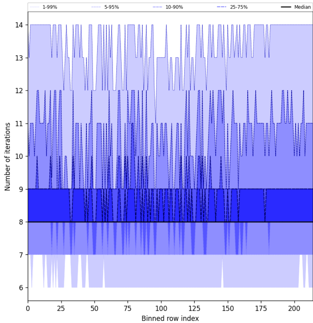
Figure 32: Along track statistics of “Number of iterations” for 2025-04-15 to 2025-04-17
