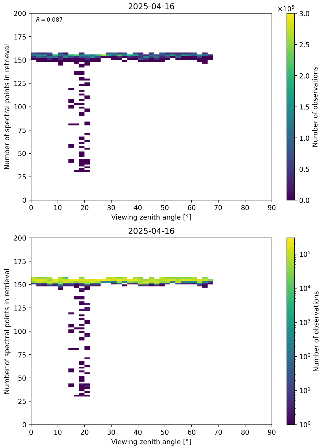
Figure 76: Scatter density plot of “Viewing zenith angle” against “Number of spectral points in retrieval” for 2025-04-15 to 2025-04-17.
