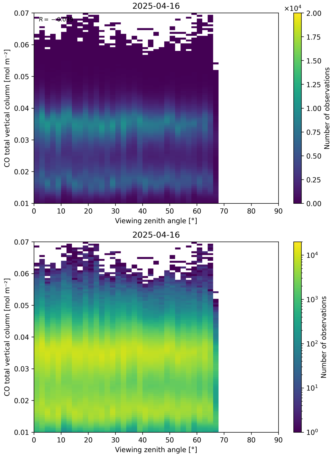
Figure 69: Scatter density plot of “Viewing zenith angle” against “CO total vertical column” for 2025-04-15 to 2025-04-17.
