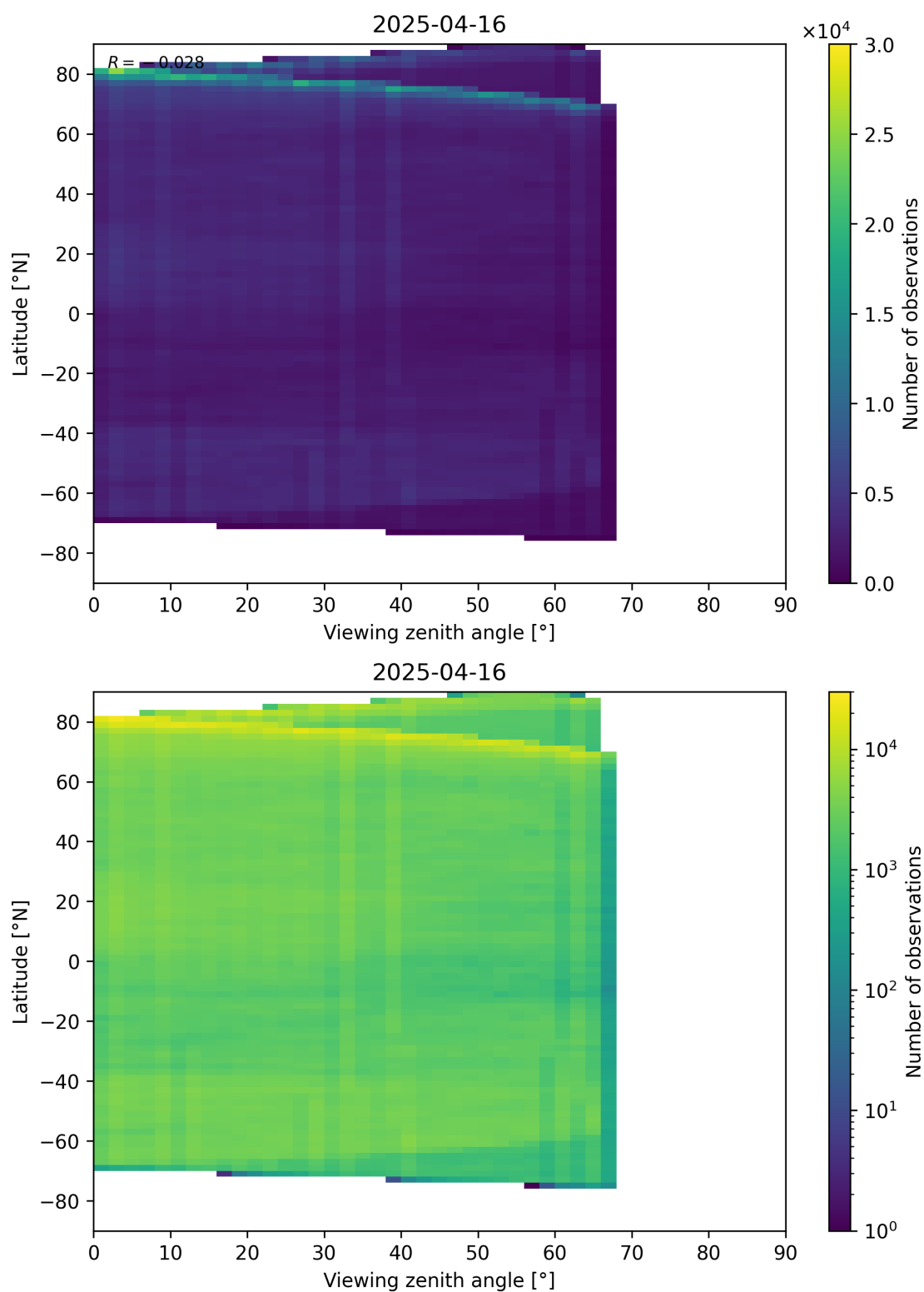
Figure 74: Scatter density plot of “Viewing zenith angle” against “Latitude” for 2025-04-15 to 2025-04-17.
