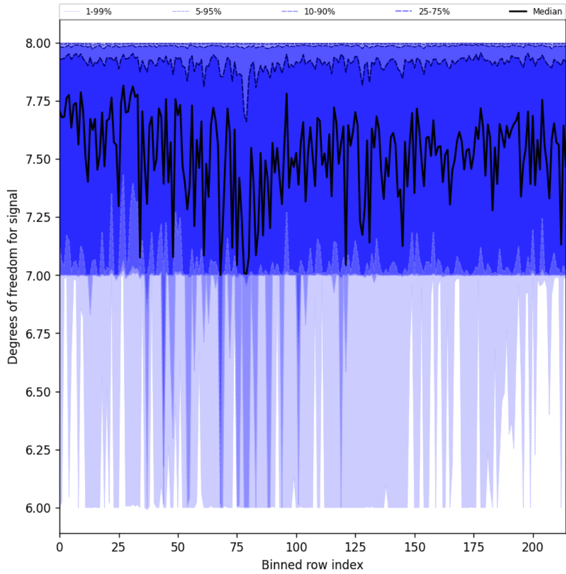
Figure 31: Along track statistics of “Degrees of freedom for signal” for 2025-04-15 to 2025-04-17
