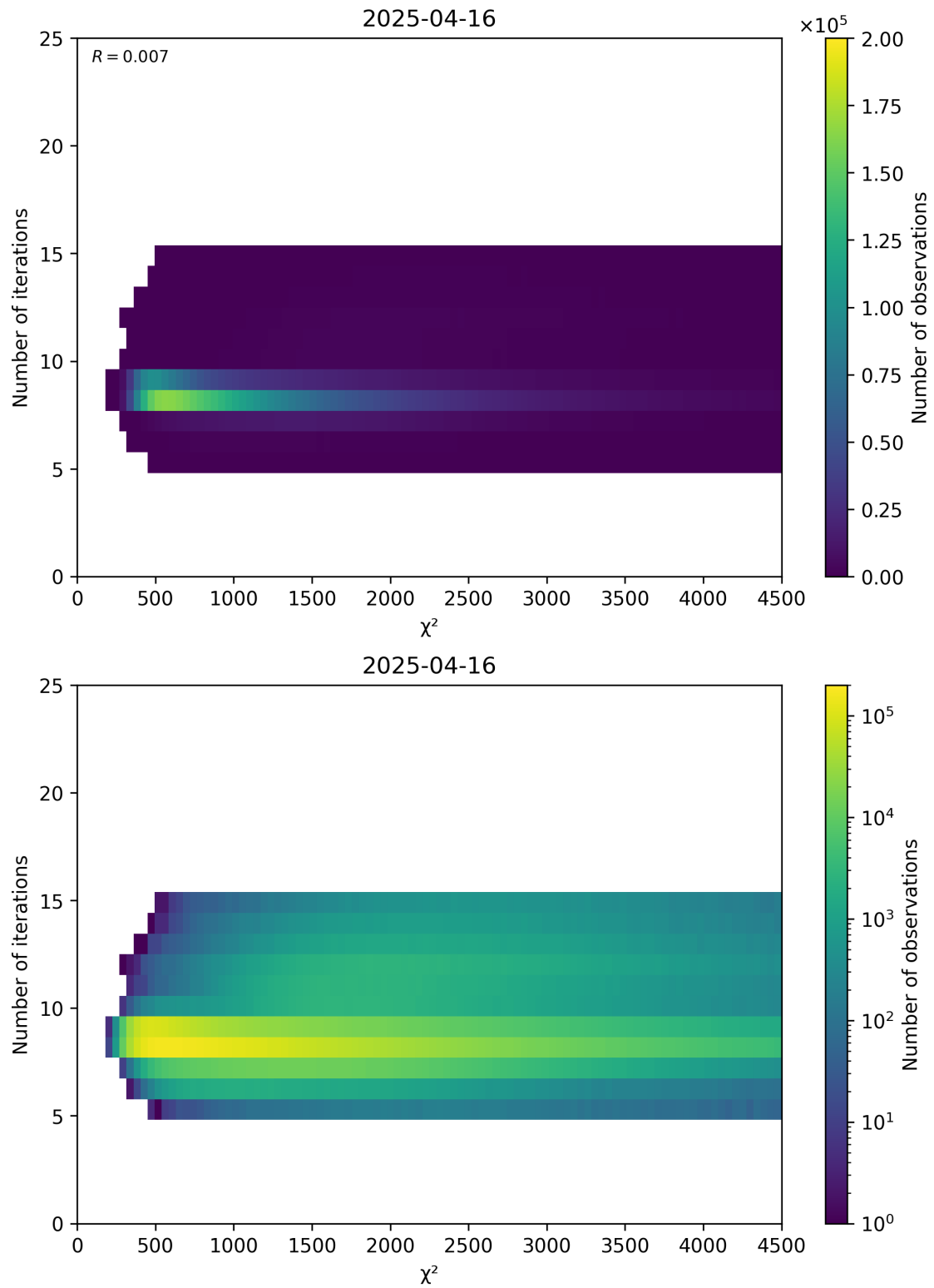
Figure 49: Scatter density plot of “ \chi^2 ” against “Number of iterations” for 2025-04-15 to 2025-04-17.
