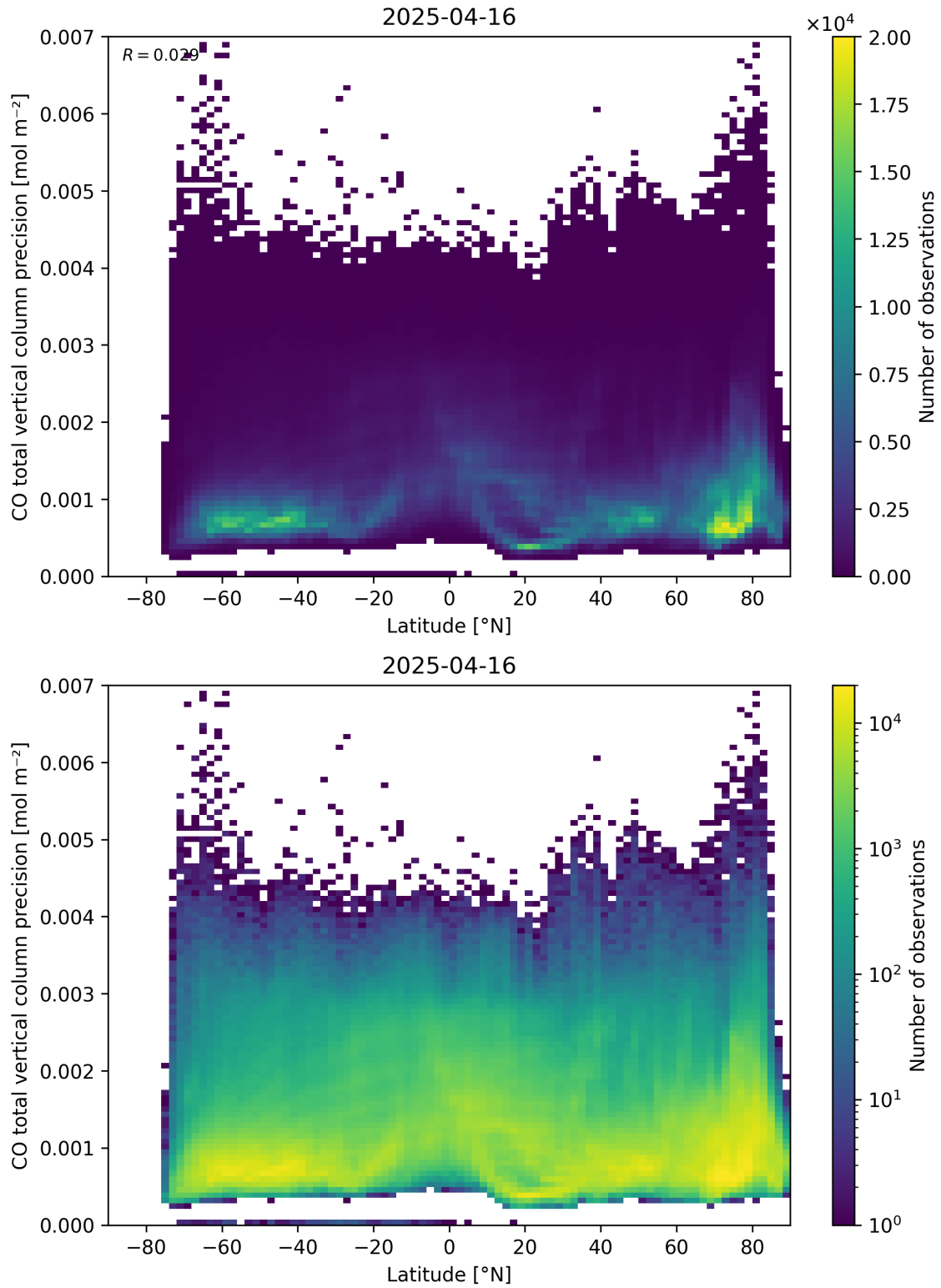
Figure 53: Scatter density plot of “Latitude” against “CO total vertical column precision” for 2025-04-15 to 2025-04-17.
