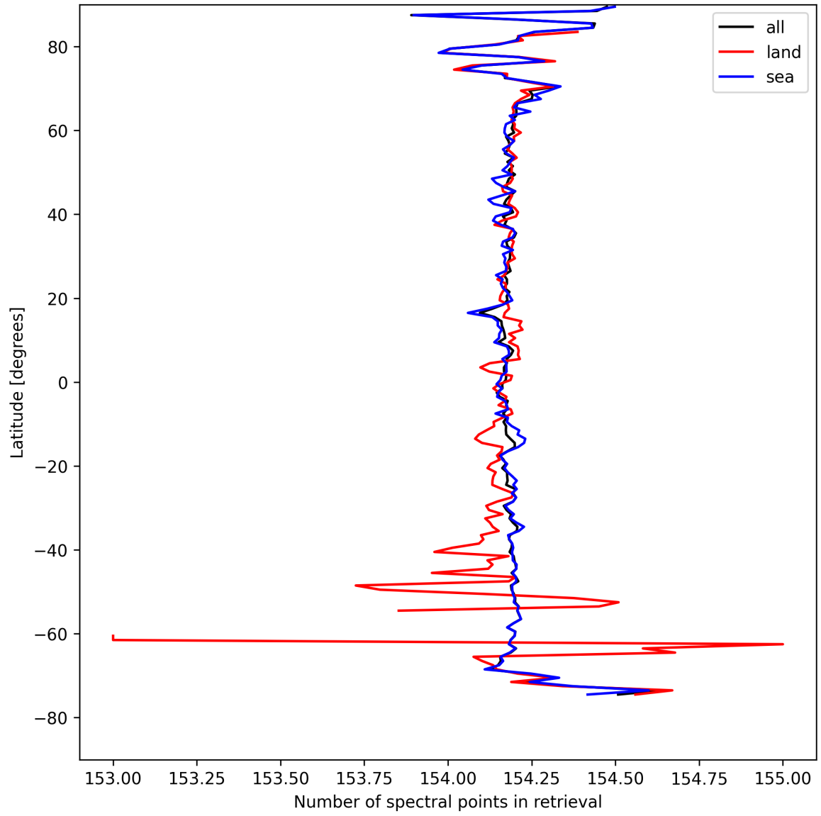
Figure 13: Zonal average of “Number of spectral points in retrieval” for 2025-04-15 to 2025-04-17.
