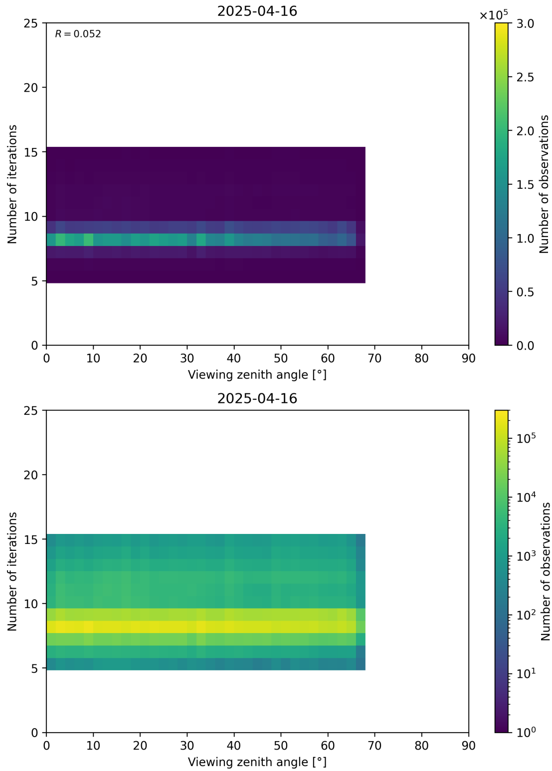
Figure 75: Scatter density plot of “Viewing zenith angle” against “Number of iterations” for 2025-04-15 to 2025-04-17.
