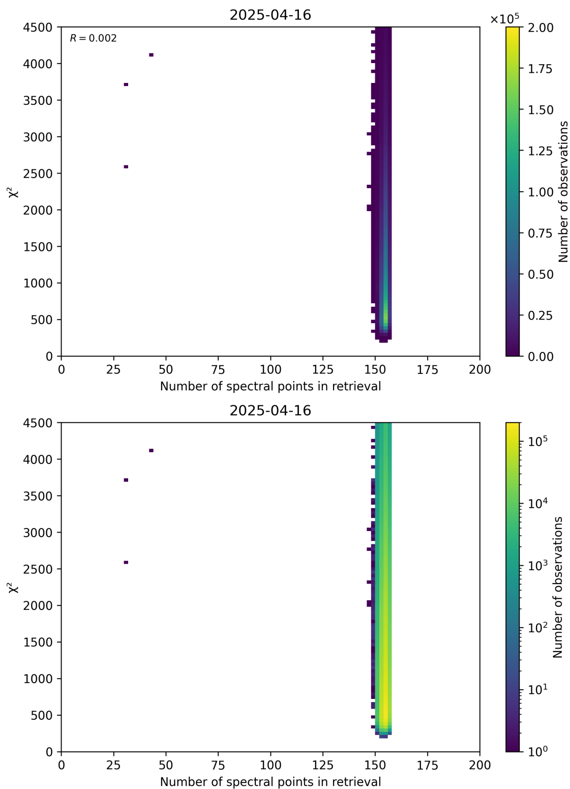
Figure 58: Scatter density plot of “Number of spectral points in retrieval” against “ \chi^2 ” for 2025-04-15 to 2025-04-17.
