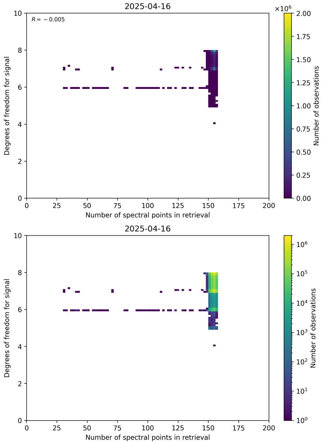
Figure 59: Scatter density plot of “Number of spectral points in retrieval” against “Degrees of freedom for signal” for 2025-04-15 to 2025-04-17.
