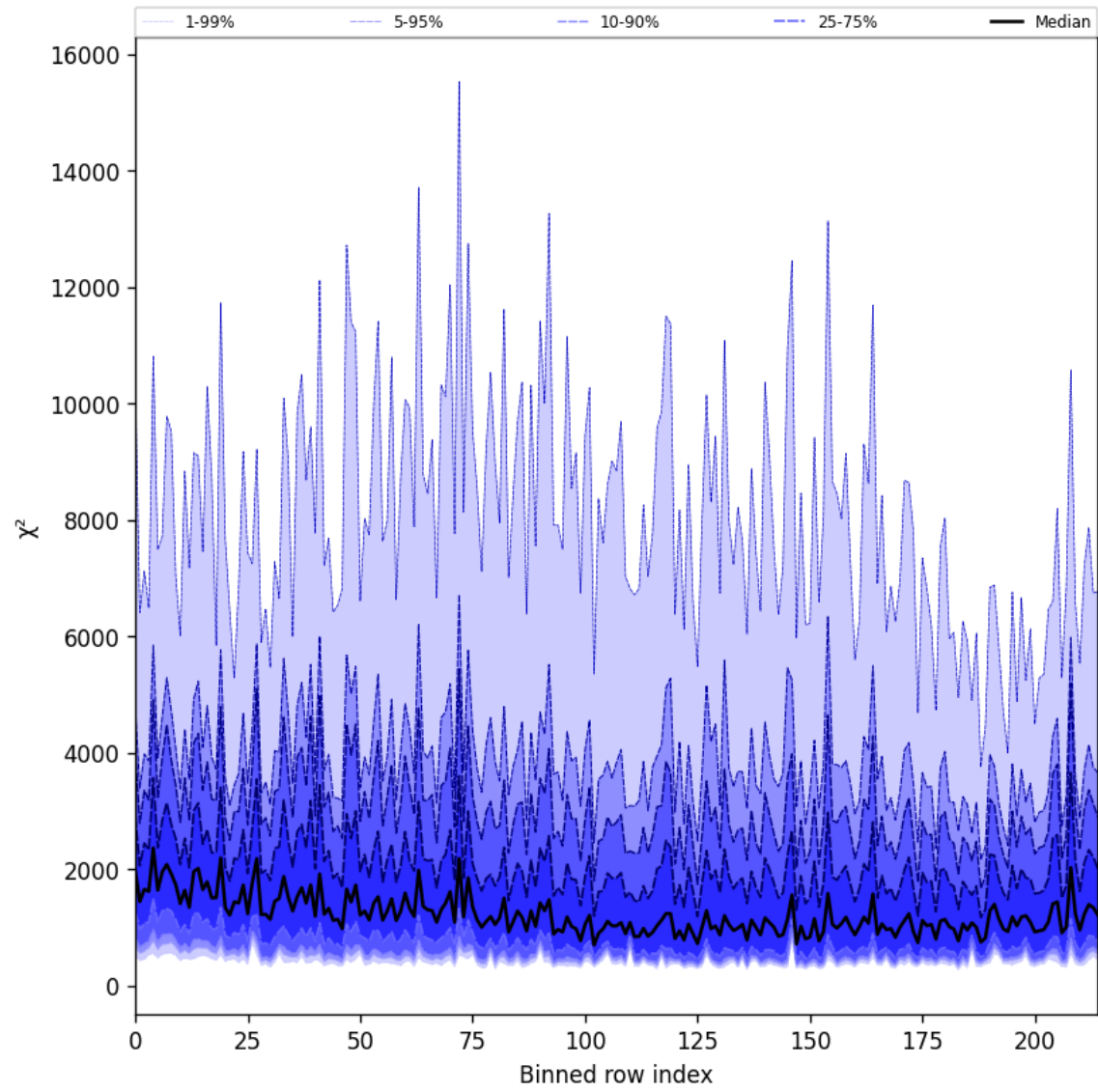
Figure 30: Along track statistics of “ \chi^2 ” for 2025-04-15 to 2025-04-17
