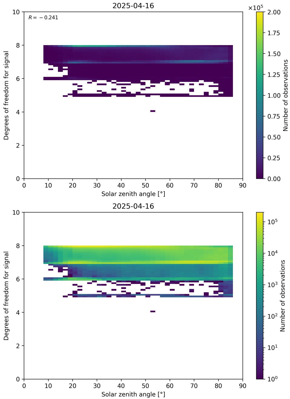
Figure 65: Scatter density plot of “Solar zenith angle” against “Degrees of freedom for signal” for 2025-04-15 to 2025-04-17.
