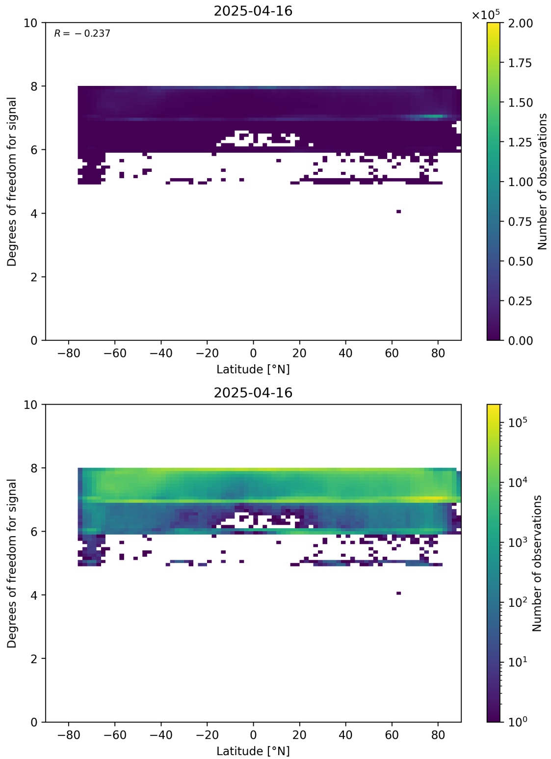
Figure 55: Scatter density plot of “Latitude” against “Degrees of freedom for signal” for 2025-04-15 to 2025-04-17.
