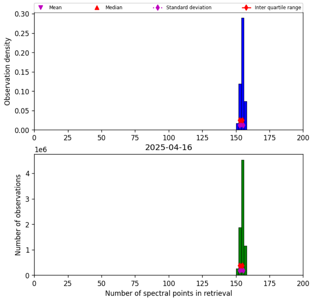
Figure 21: Histogram of “Number of spectral points in retrieval” for 2025-04-15 to 2025-04-17
