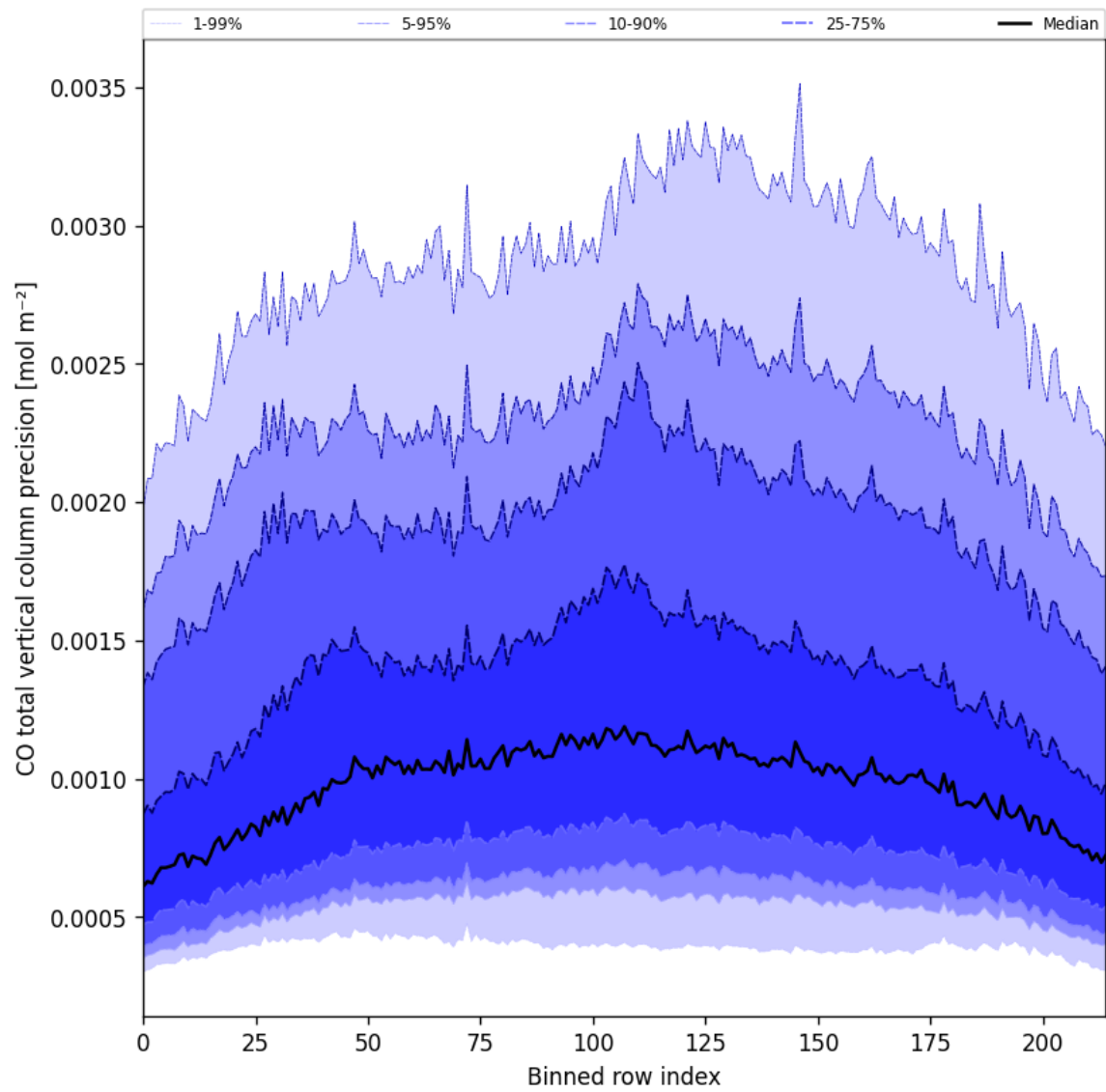
Figure 28: Along track statistics of “CO total vertical column precision” for 2025-04-15 to 2025-04-17
