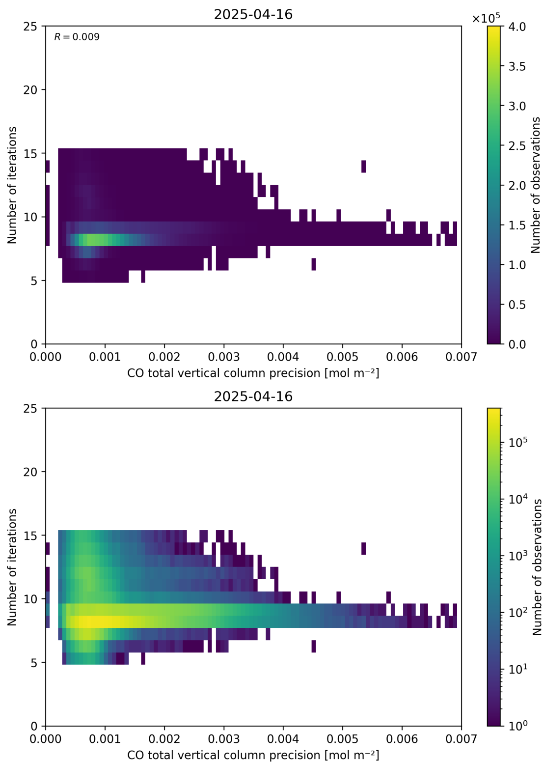
Figure 46: Scatter density plot of “CO total vertical column precision” against “Number of iterations” for 2025-04-15 to 2025-04-17.
