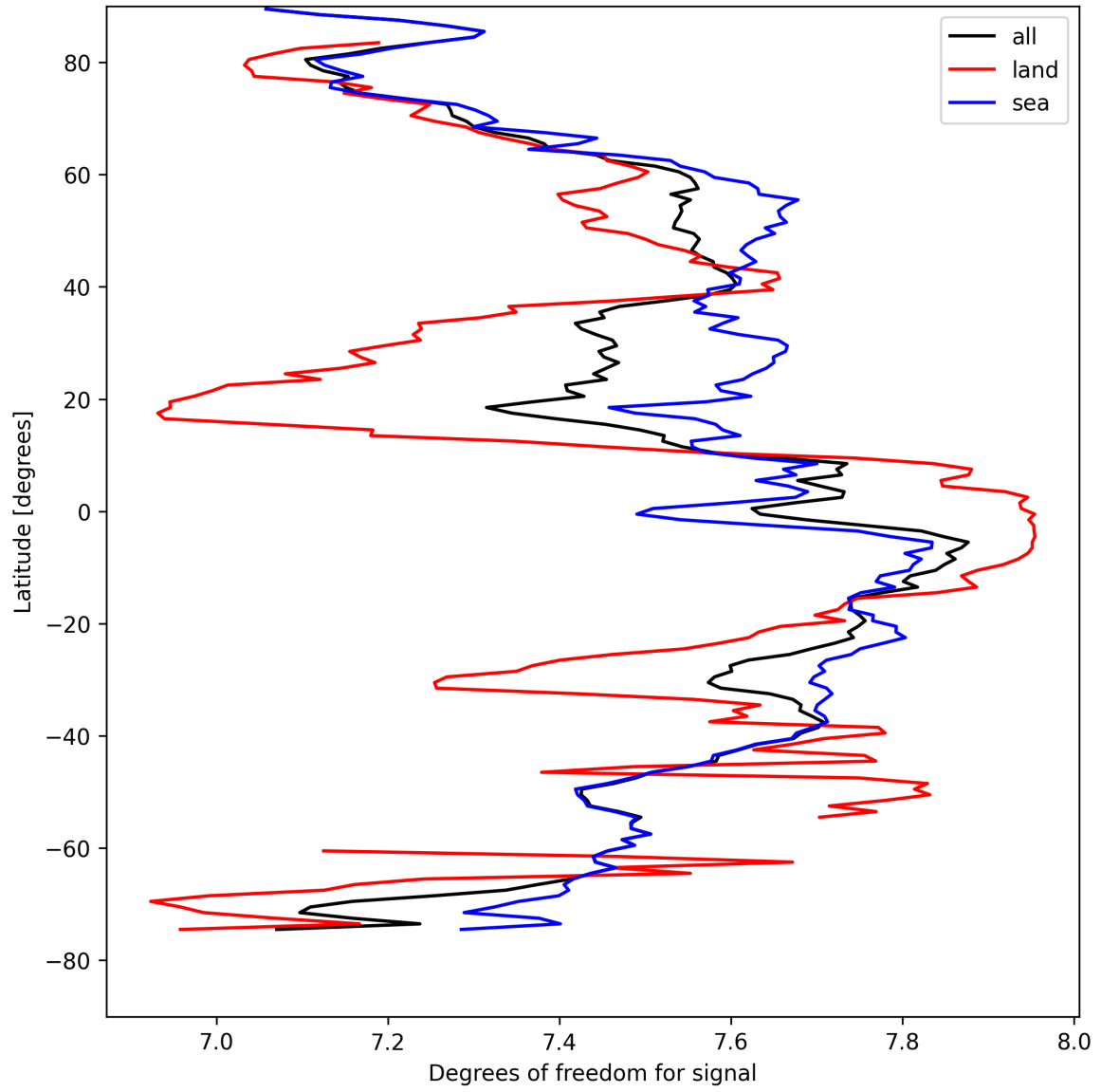
Figure 15: Zonal average of “Degrees of freedom for signal” for 2025-04-15 to 2025-04-17.
