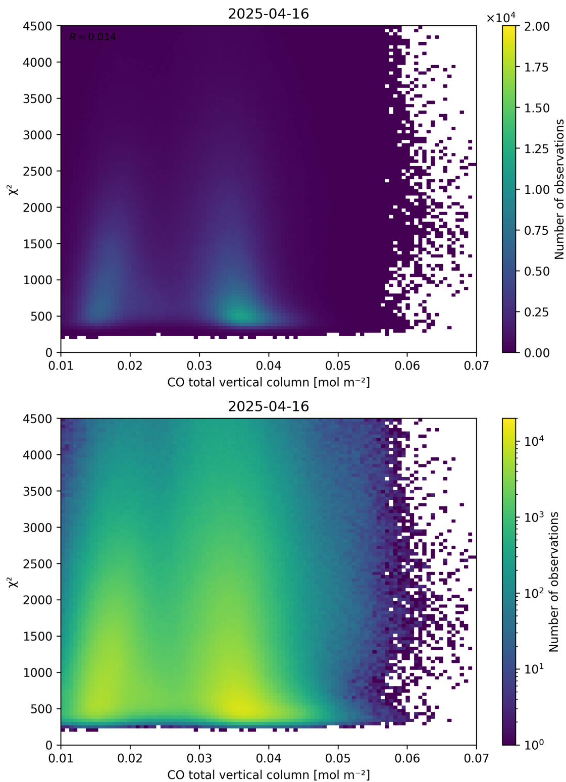
Figure 35: Scatter density plot of “CO total vertical column” against “ \chi^2 ” for 2025-04-15 to 2025-04-17.
