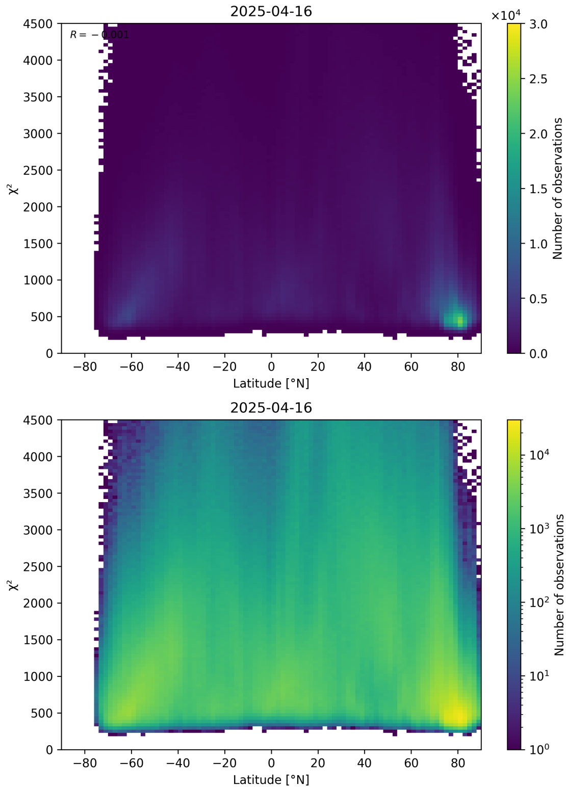
Figure 54: Scatter density plot of “Latitude” against “ \chi^2 ” for 2025-04-15 to 2025-04-17.
