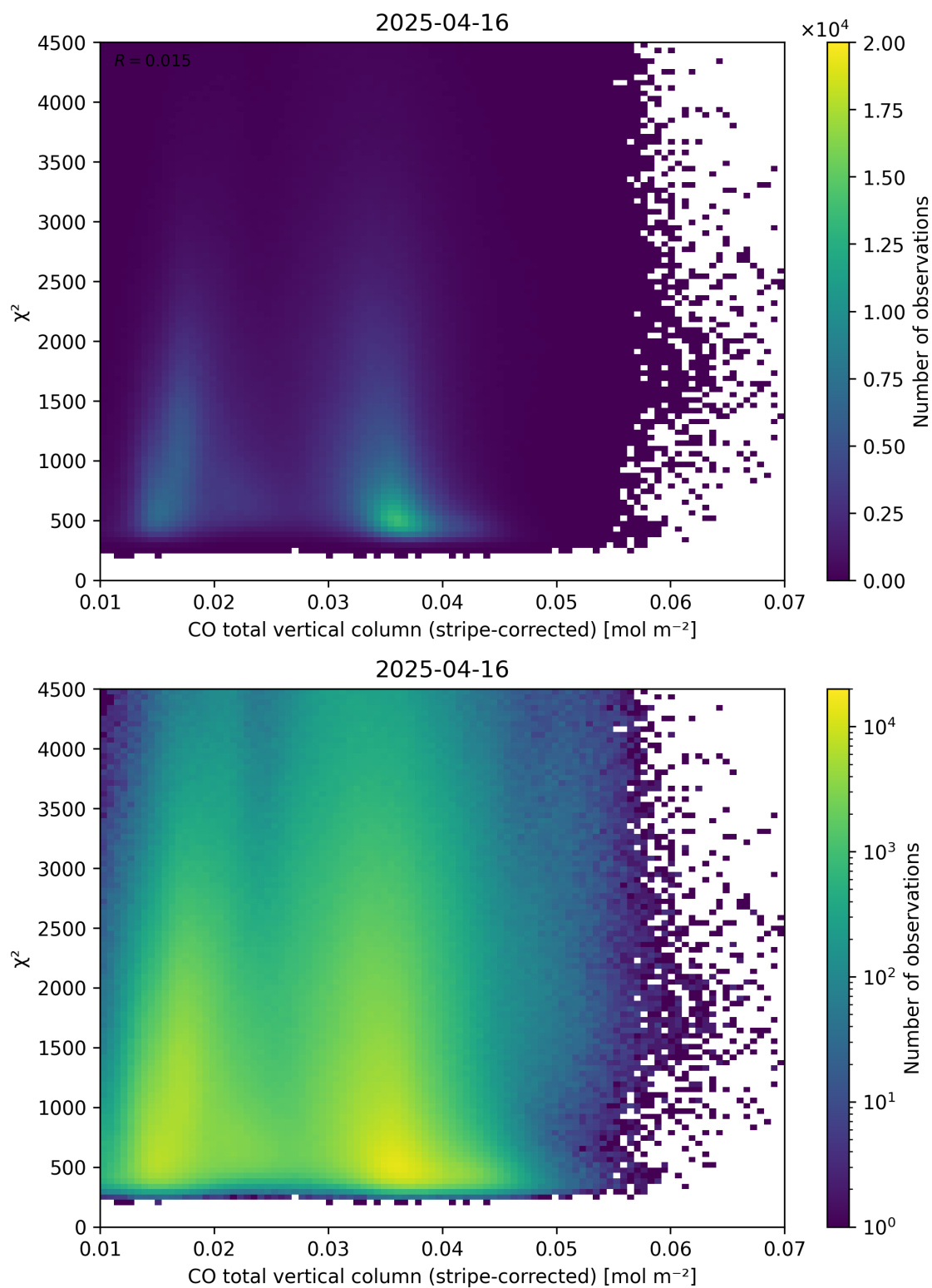
Figure 37: Scatter density plot of “CO total vertical column (stripe-corrected)” against “ \chi^2 ” for 2025-04-15 to 2025-04-17.
