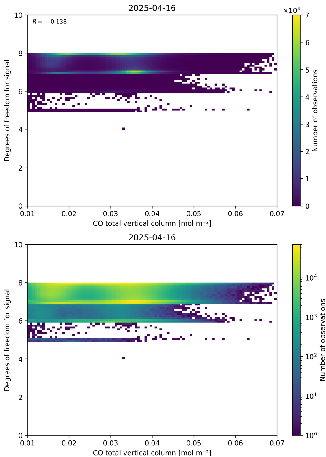
Figure 41: Scatter density plot of “CO total vertical column” against “Degrees of freedom for signal” for 2025-04-15 to 2025-04-17.
