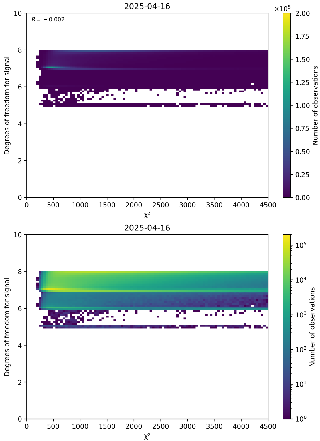
Figure 48: Scatter density plot of “ \chi^2 ” against “Degrees of freedom for signal” for 2025-04-15 to 2025-04-17.
