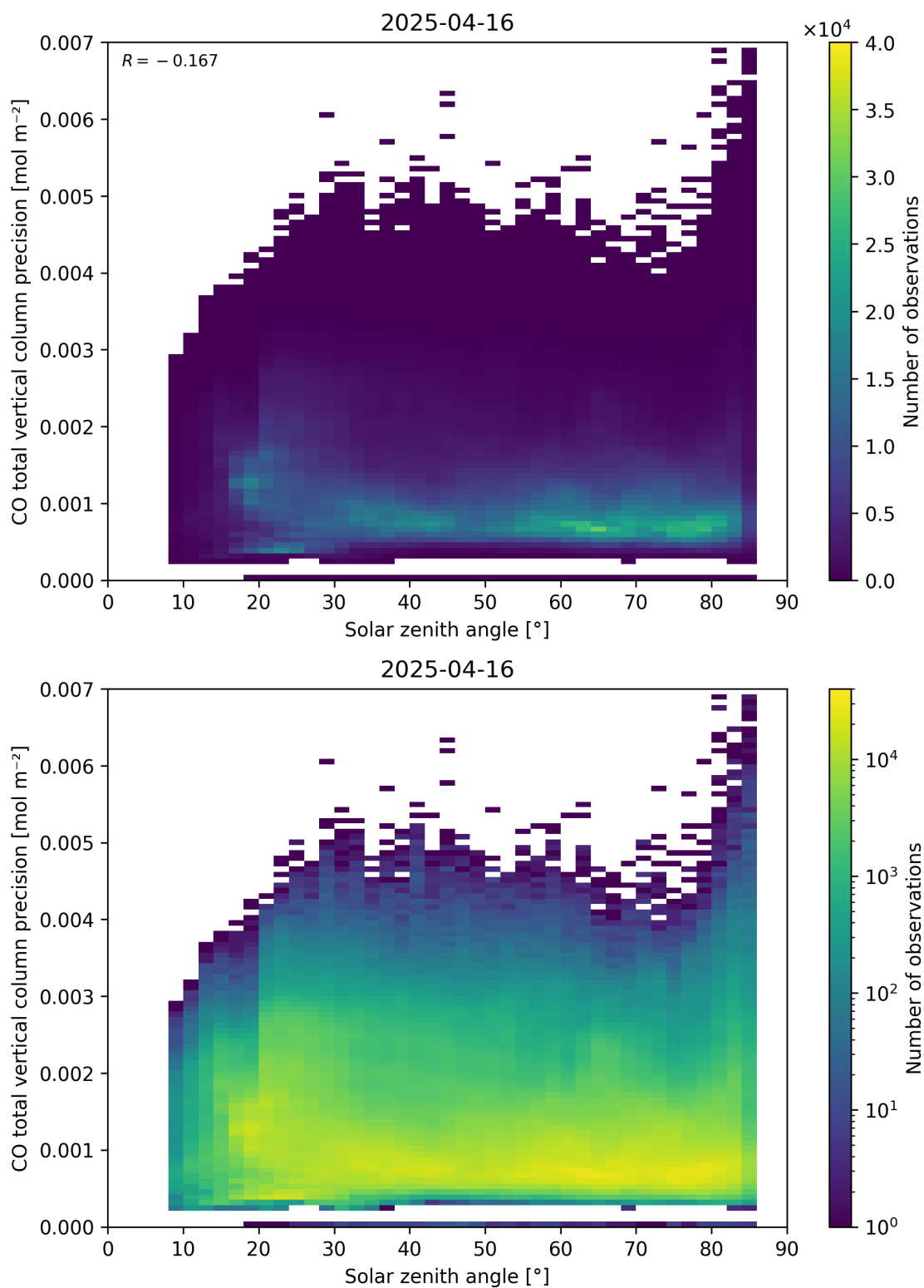
Figure 63: Scatter density plot of “Solar zenith angle” against “CO total vertical column precision” for 2025-04-15 to 2025-04-17.
