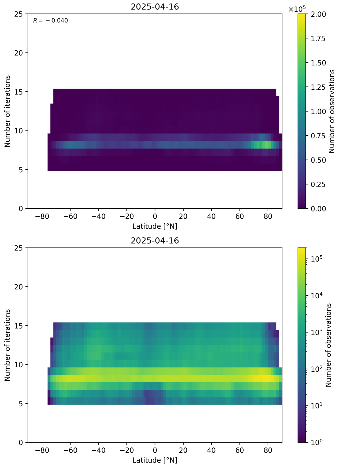
Figure 56: Scatter density plot of “Latitude” against “Number of iterations” for 2025-04-15 to 2025-04-17.
