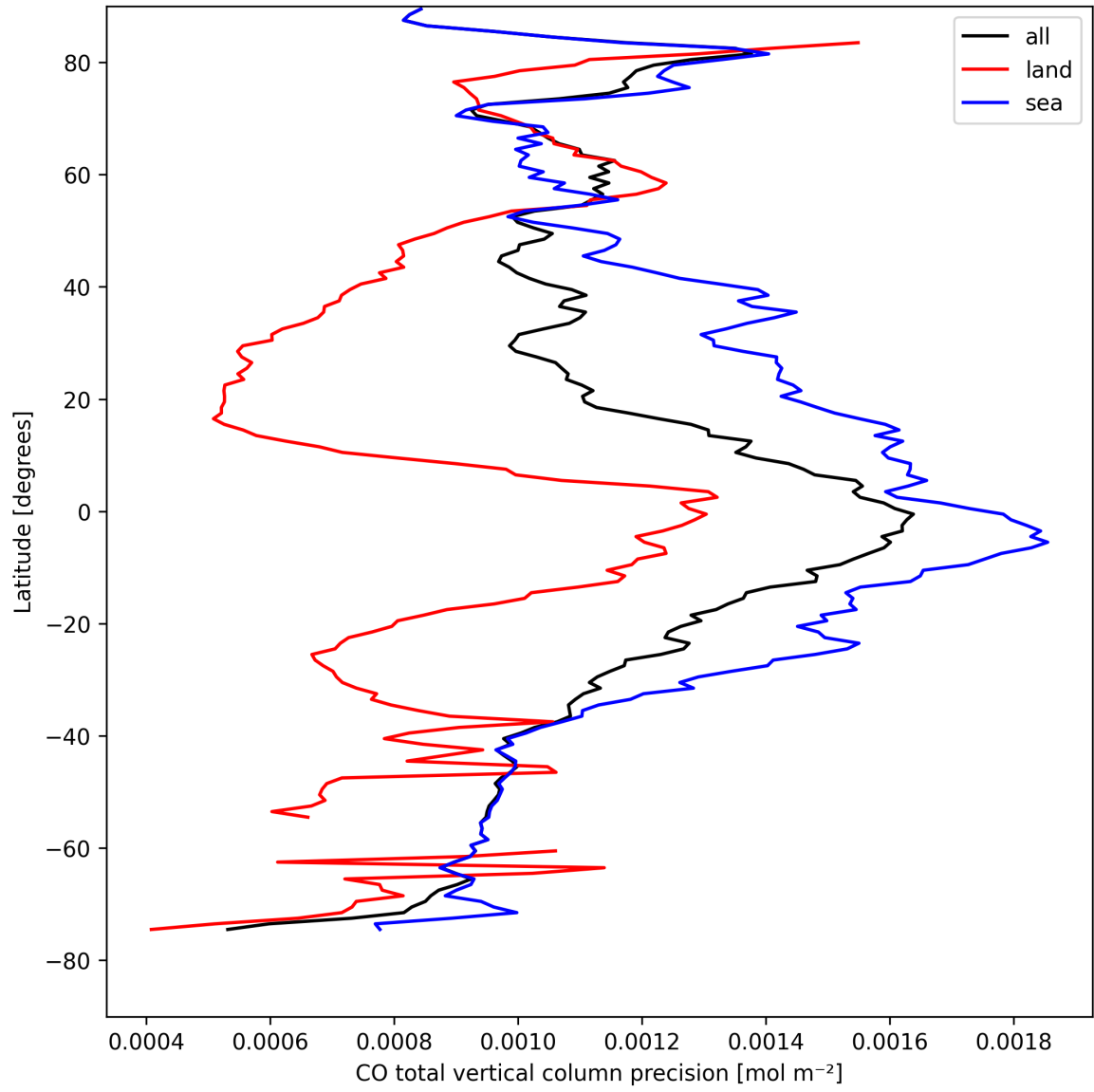
Figure 12: Zonal average of “CO total vertical column precision” for 2025-04-15 to 2025-04-17.
