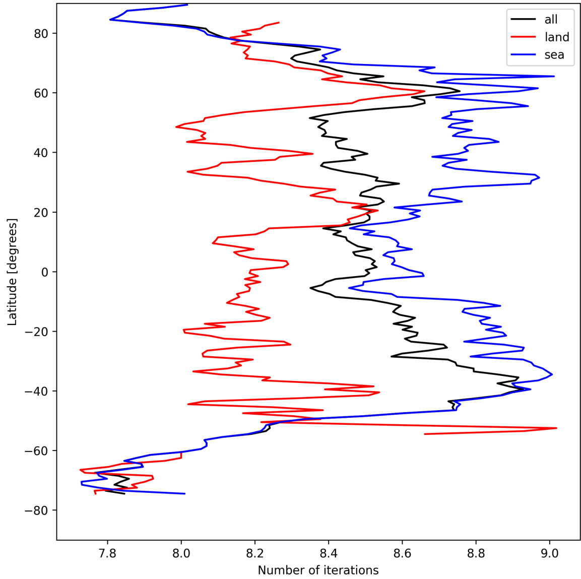
Figure 16: Zonal average of “Number of iterations” for 2025-04-15 to 2025-04-17.
