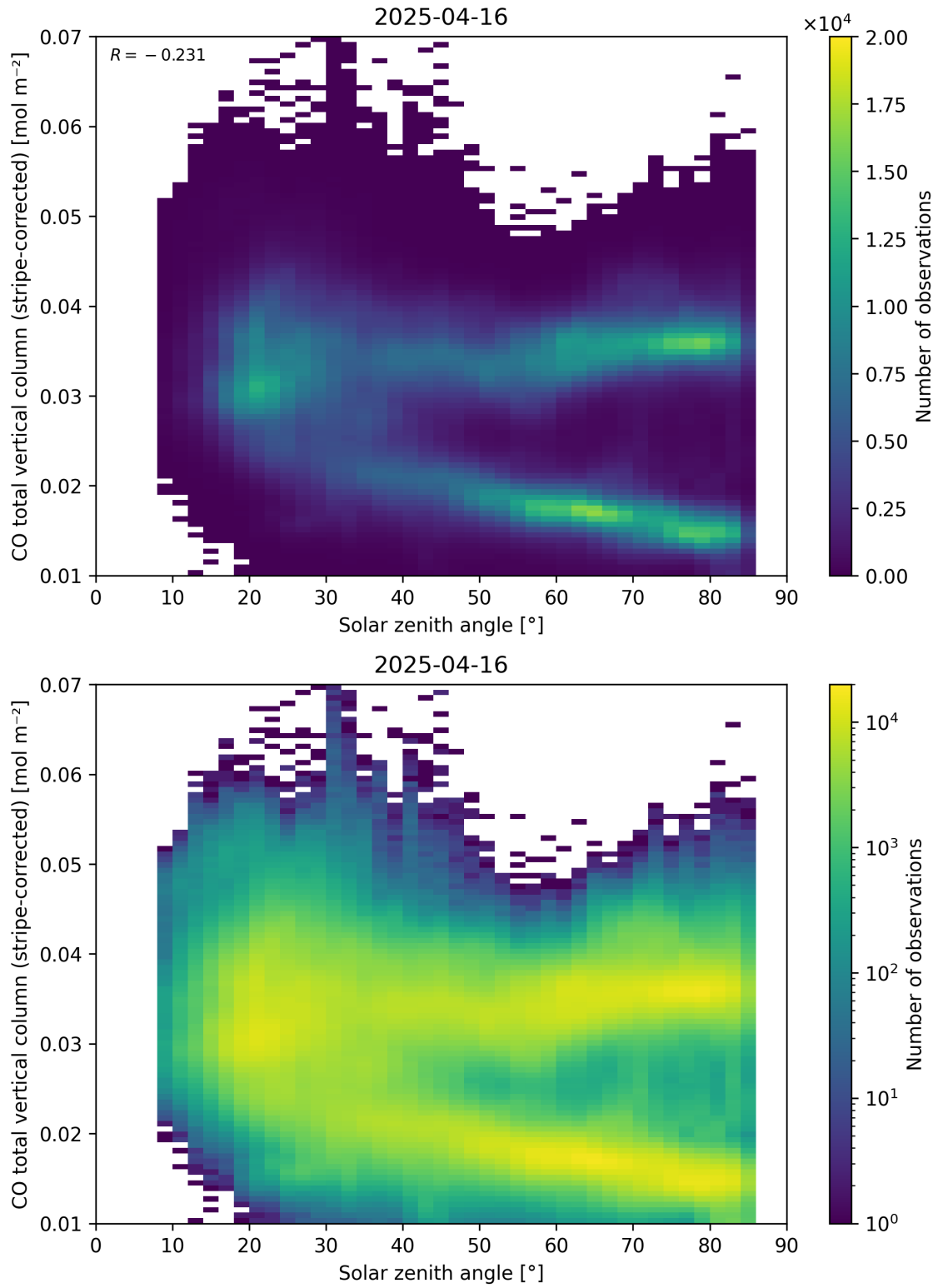
Figure 62: Scatter density plot of “Solar zenith angle” against “CO total vertical column (stripe-corrected)” for 2025-04-15 to 2025-04-17.
