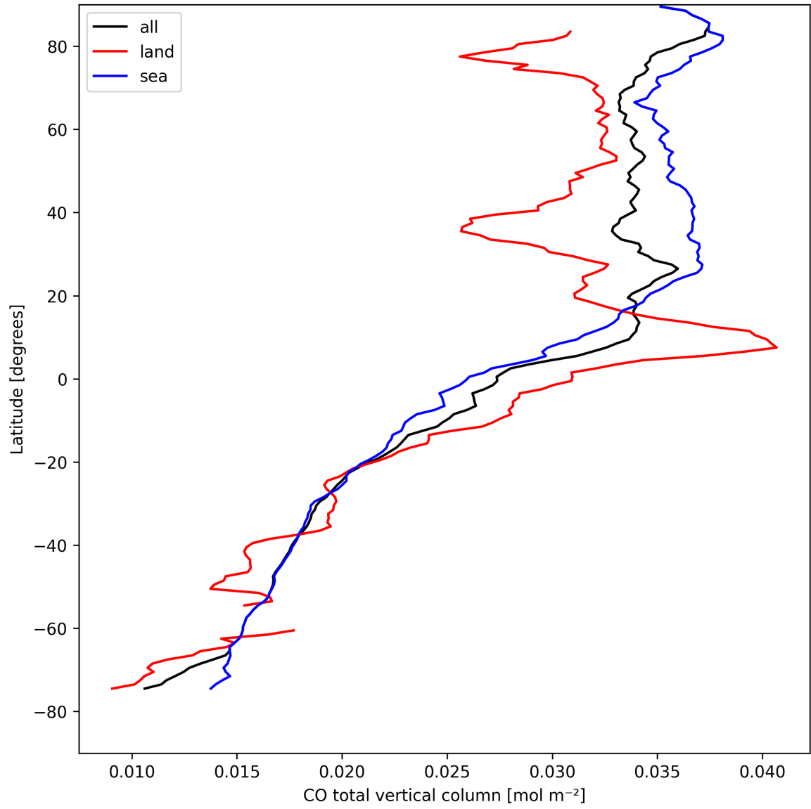
Figure 10: Zonal average of “CO total vertical column” for 2025-04-15 to 2025-04-17.
