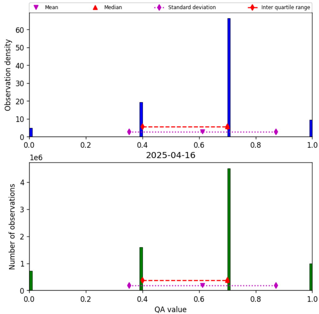
Figure 17: Histogram of “QA value” for 2025-04-15 to 2025-04-17
