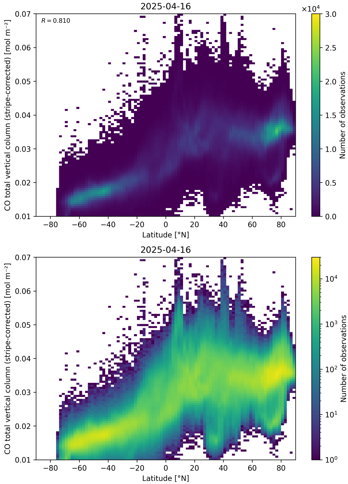
Figure 52: Scatter density plot of “Latitude” against “CO total vertical column (stripe-corrected)” for 2025-04-15 to 2025-04-17.
