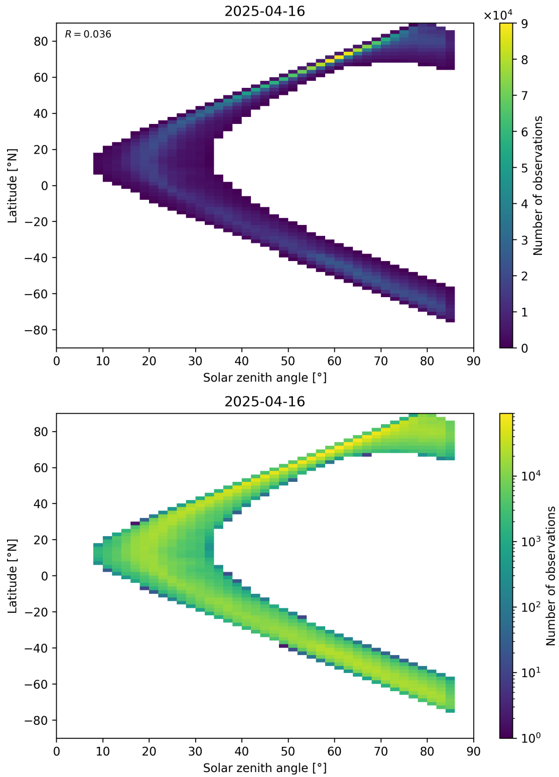
Figure 66: Scatter density plot of “Solar zenith angle” against “Latitude” for 2025-04-15 to 2025-04-17.
