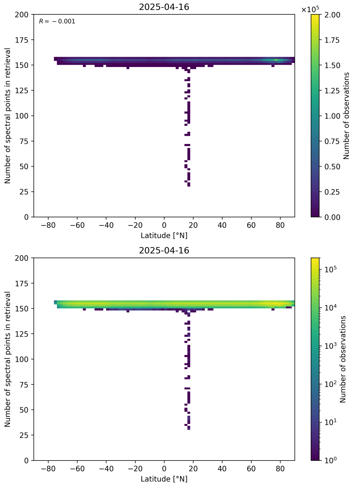
Figure 57: Scatter density plot of “Latitude” against “Number of spectral points in retrieval” for 2025-04-15 to 2025-04-17.
