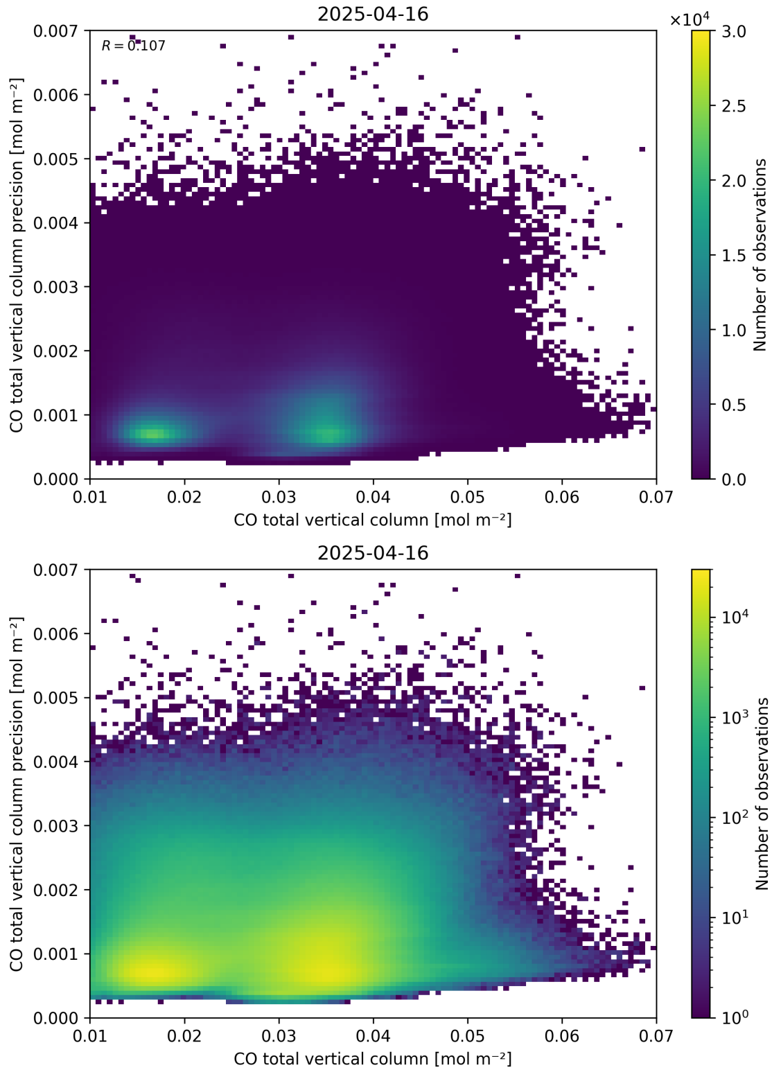
Figure 34: Scatter density plot of “CO total vertical column” against “CO total vertical column precision” for 2025-04-15 to 2025-04-17.
