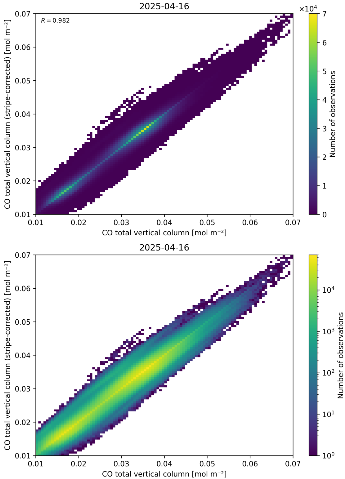
Figure 33: Scatter density plot of “CO total vertical column” against “CO total vertical column (stripe-corrected)” for 2025-04-15 to 2025-04-17.
