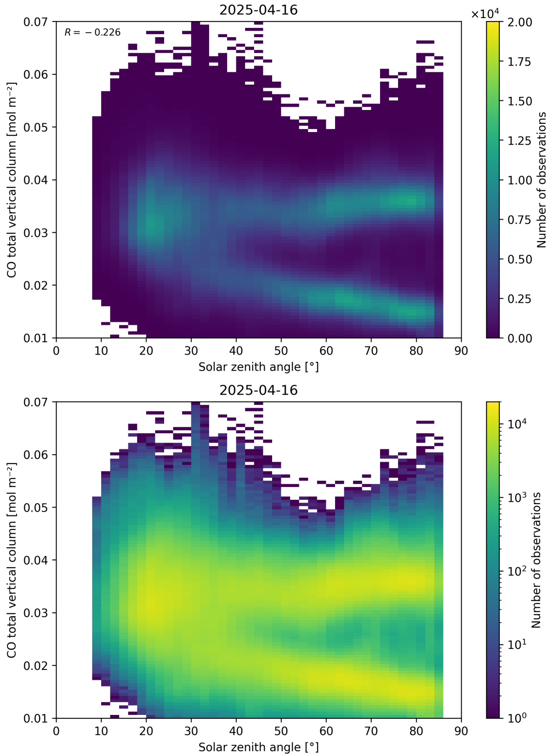
Figure 61: Scatter density plot of “Solar zenith angle” against “CO total vertical column” for 2025-04-15 to 2025-04-17.
