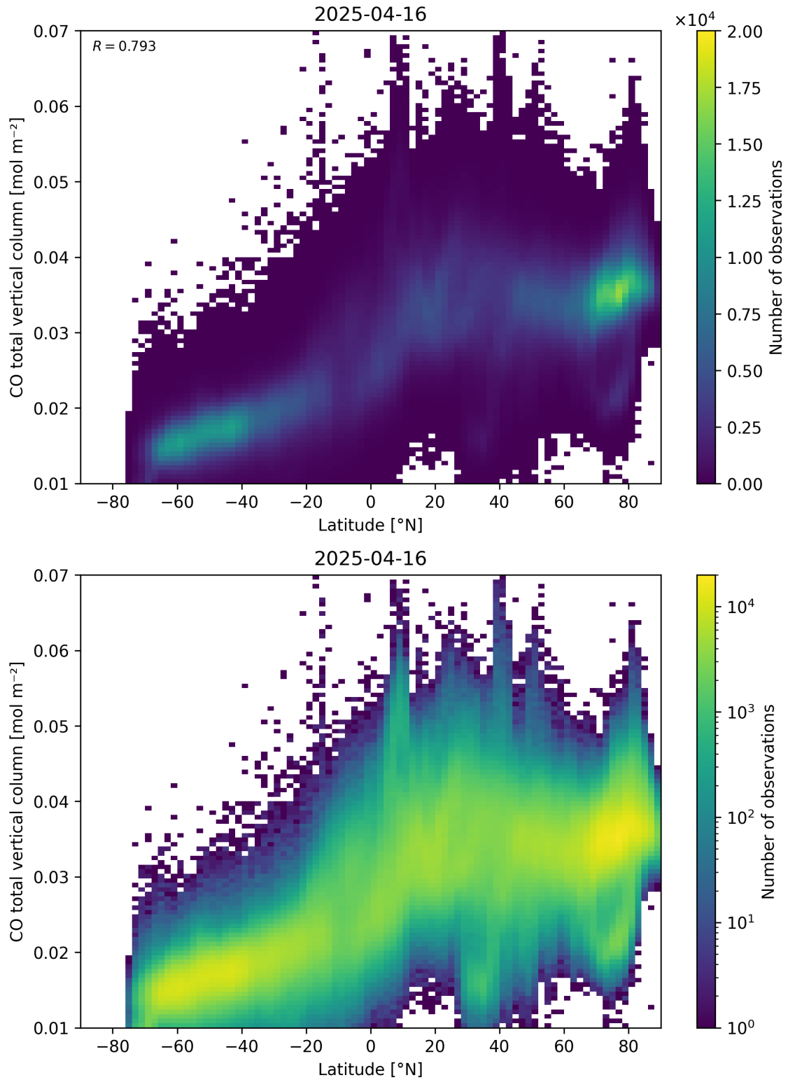
Figure 51: Scatter density plot of “Latitude” against “CO total vertical column” for 2025-04-15 to 2025-04-17.
