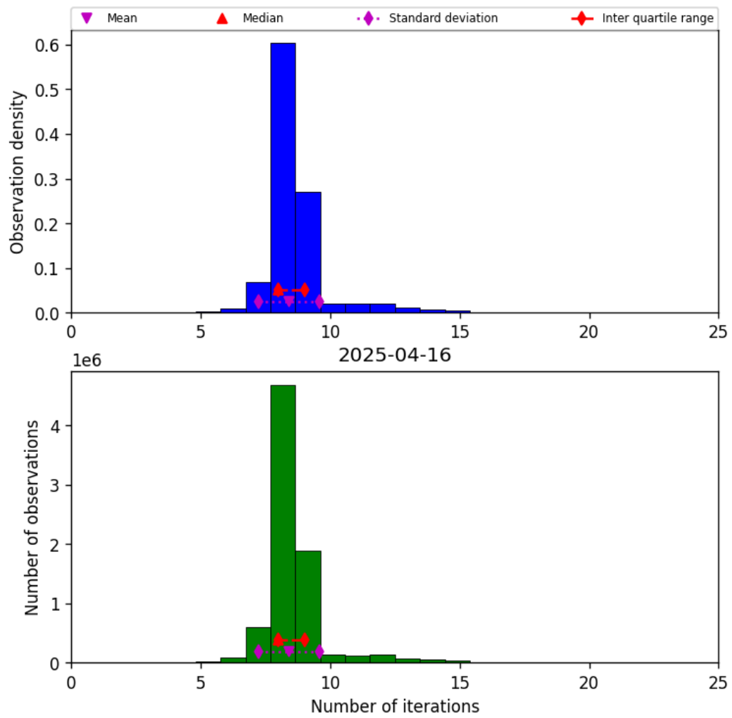
Figure 24: Histogram of “Number of iterations” for 2025-04-15 to 2025-04-17
