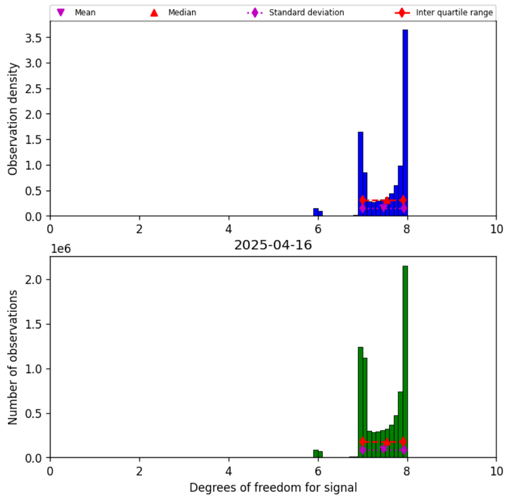
Figure 23: Histogram of “Degrees of freedom for signal” for 2025-04-15 to 2025-04-17
