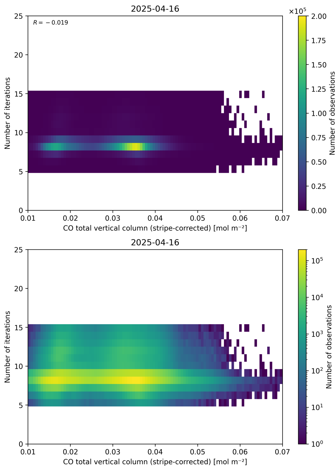
Figure 39: Scatter density plot of “CO total vertical column (stripe-corrected)” against “Number of iterations” for 2025-04-15 to 2025-04-17.
