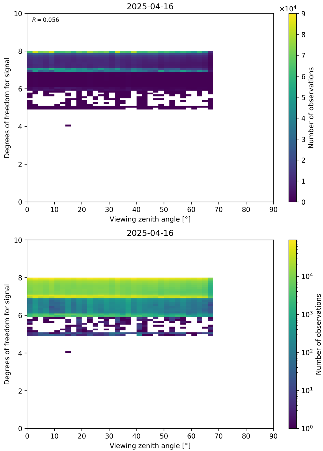
Figure 73: Scatter density plot of “Viewing zenith angle” against “Degrees of freedom for signal” for 2025-04-15 to 2025-04-17.
