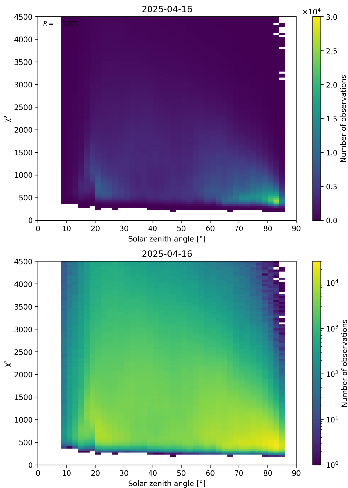
Figure 64: Scatter density plot of “Solar zenith angle” against “ \chi^2 ” for 2025-04-15 to 2025-04-17.
