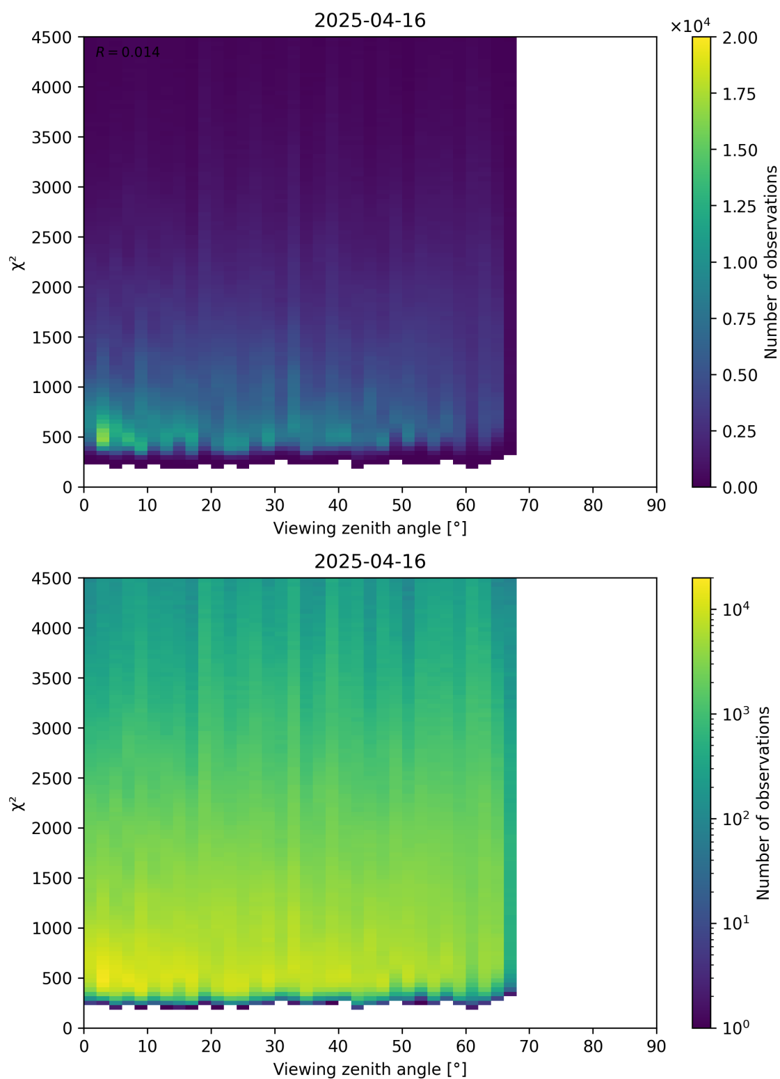
Figure 72: Scatter density plot of “Viewing zenith angle” against “ \chi^2 ” for 2025-04-15 to 2025-04-17.
