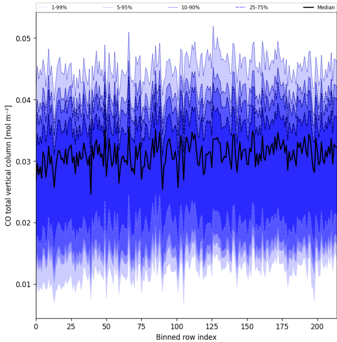
Figure 26: Along track statistics of "CO total vertical column" for 2025-04-15 to 2025-04-17
