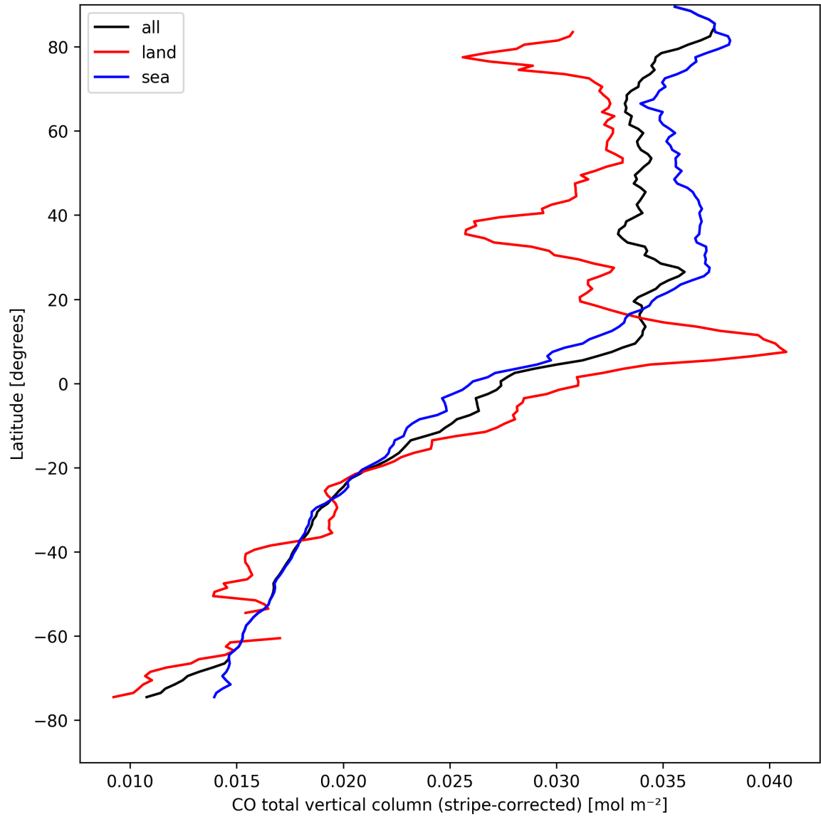
Figure 11: Zonal average of “CO total vertical column (stripe-corrected)” for 2025-04-15 to 2025-04-17.
