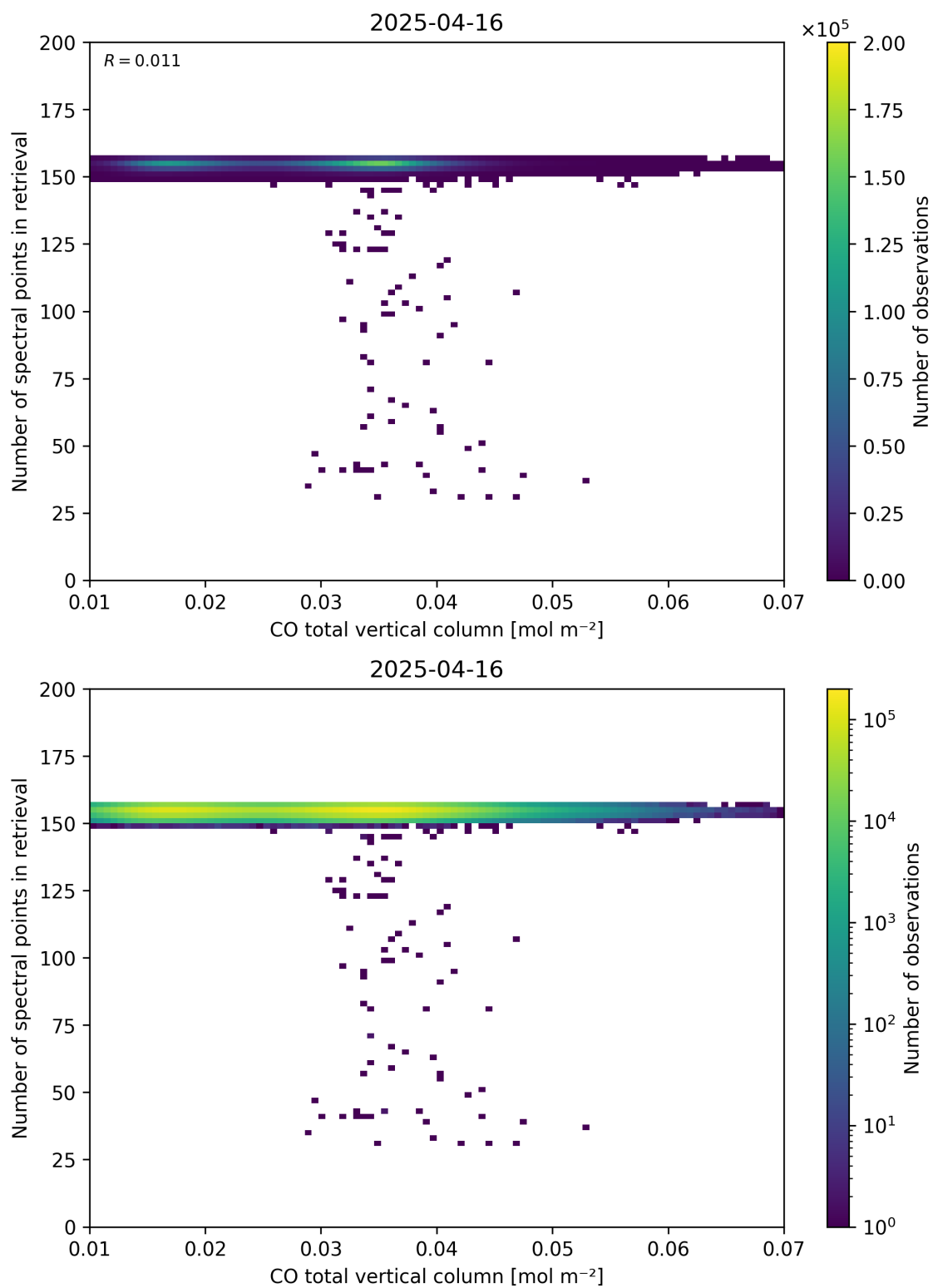
Figure 43: Scatter density plot of “CO total vertical column” against “Number of spectral points in retrieval” for 2025-04-15 to 2025-04-17.
