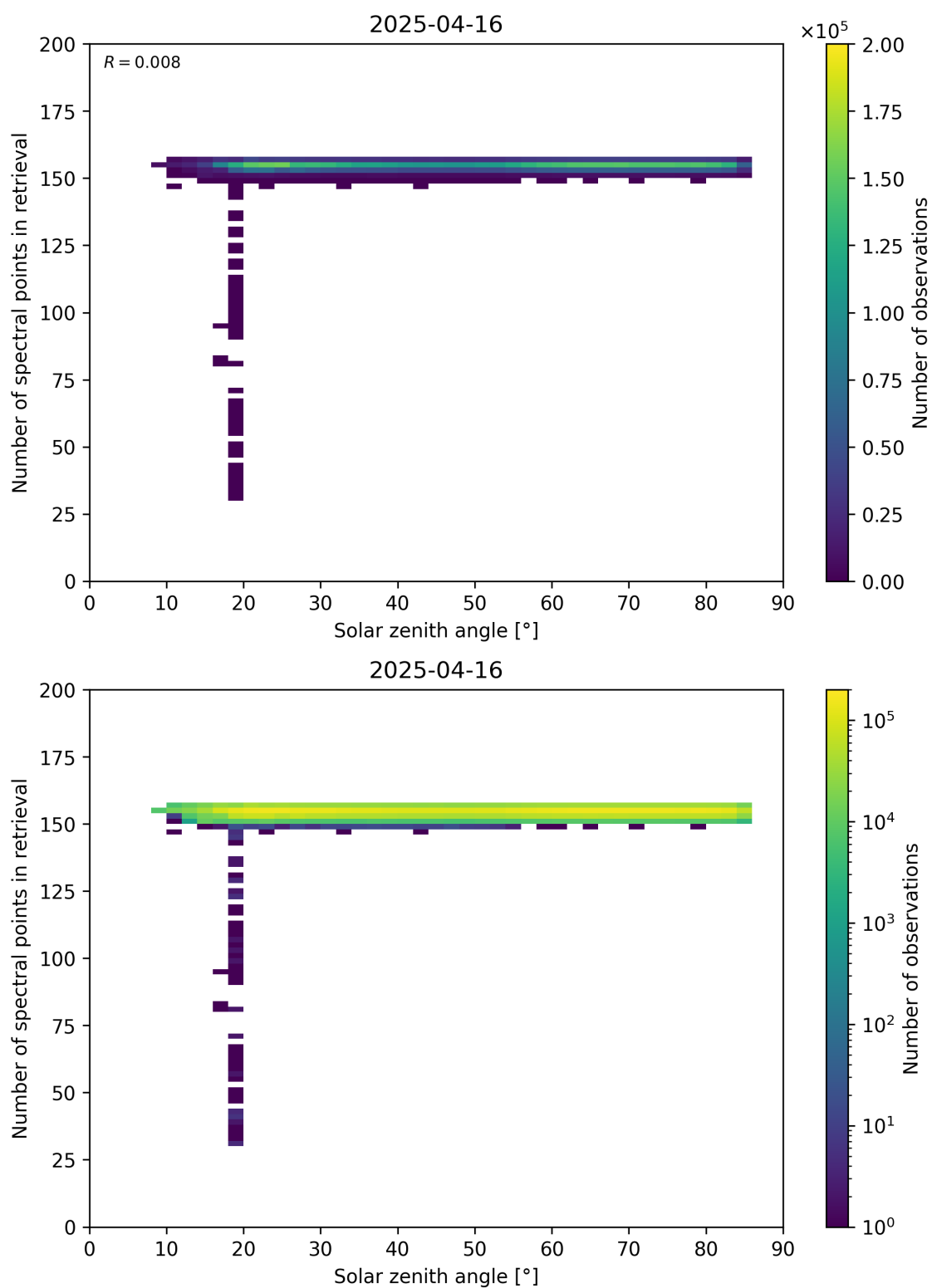
Figure 68: Scatter density plot of “Solar zenith angle” against “Number of spectral points in retrieval” for 2025-04-15 to 2025-04-17.
