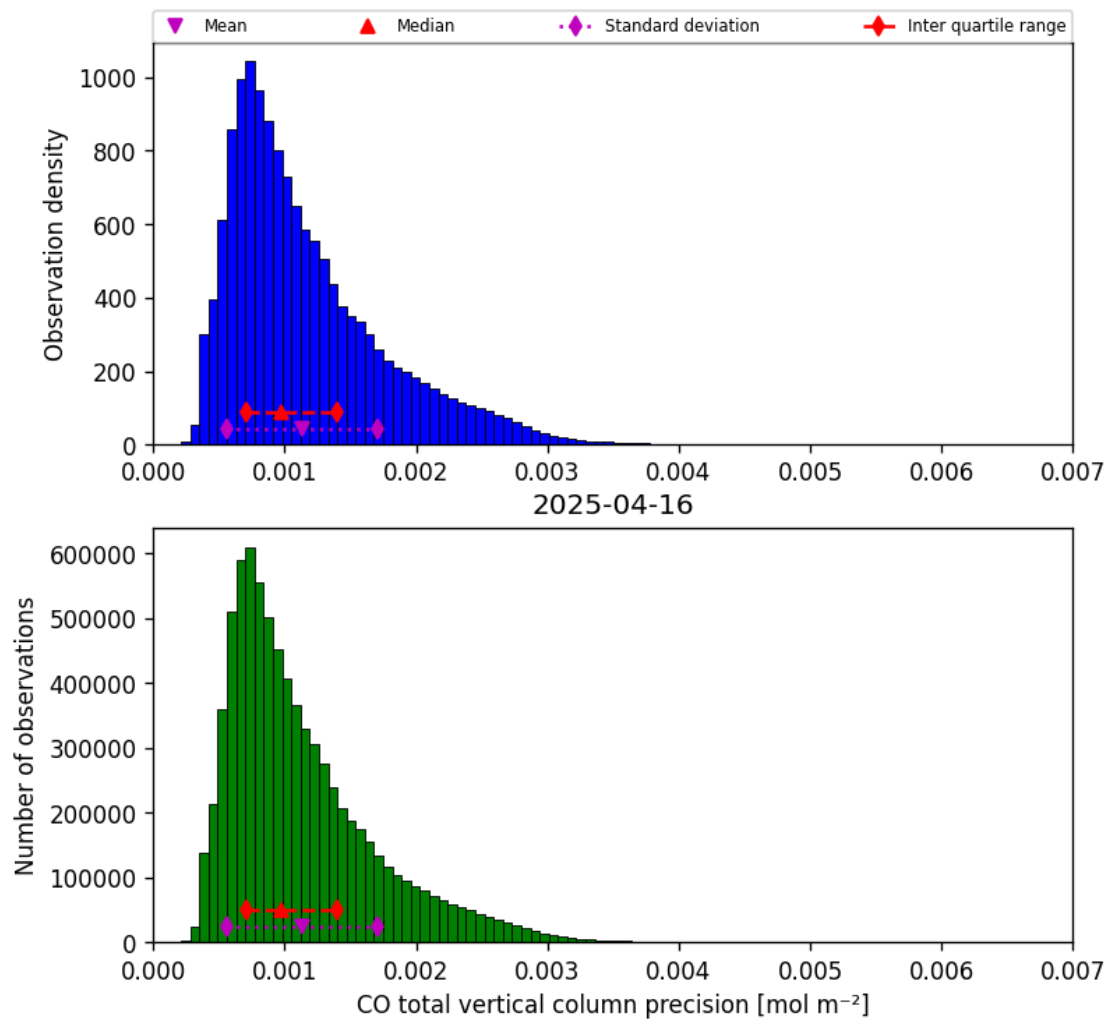
Figure 20: Histogram of “CO total vertical column precision” for 2025-04-15 to 2025-04-17
