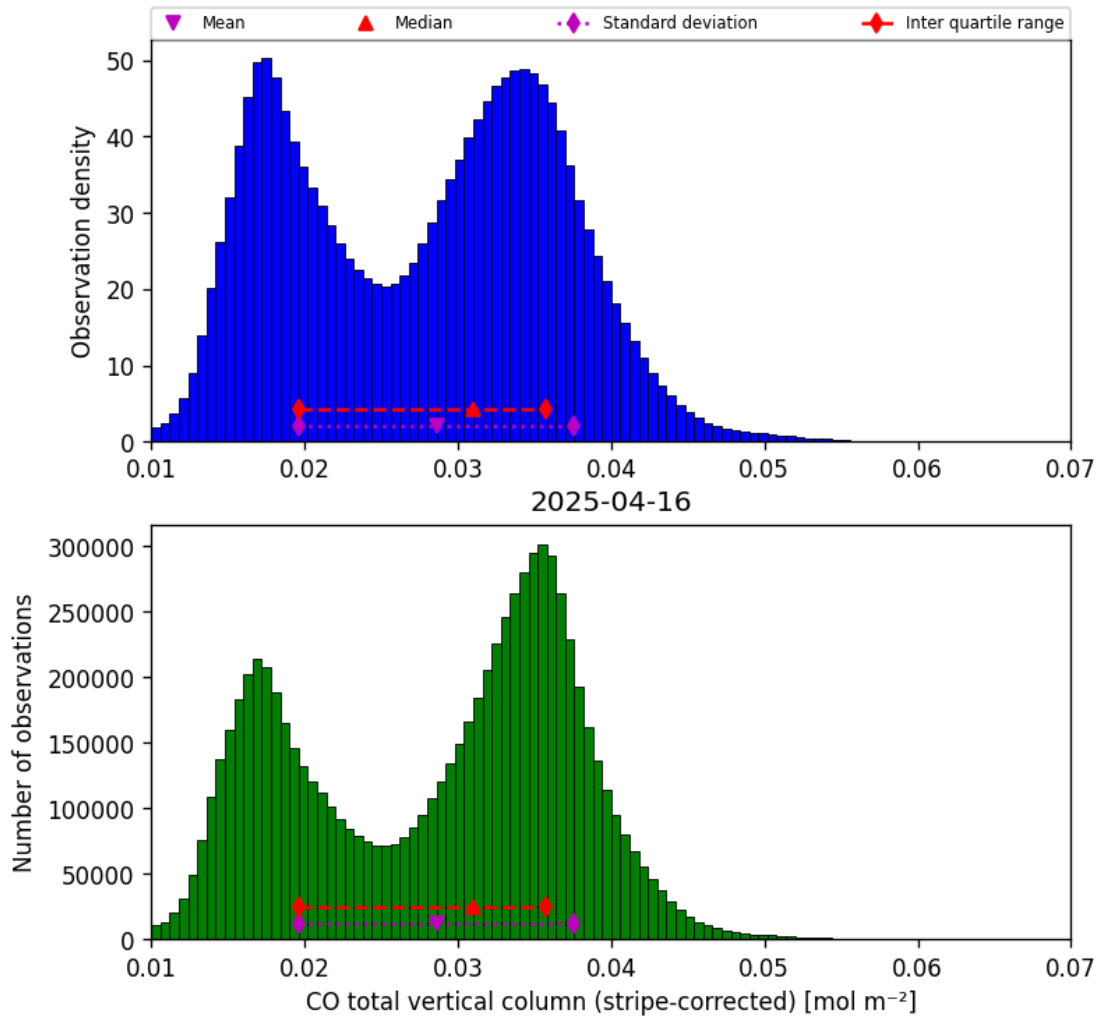
Figure 19: Histogram of “CO total vertical column (stripe-corrected)” for 2025-04-15 to 2025-04-17
