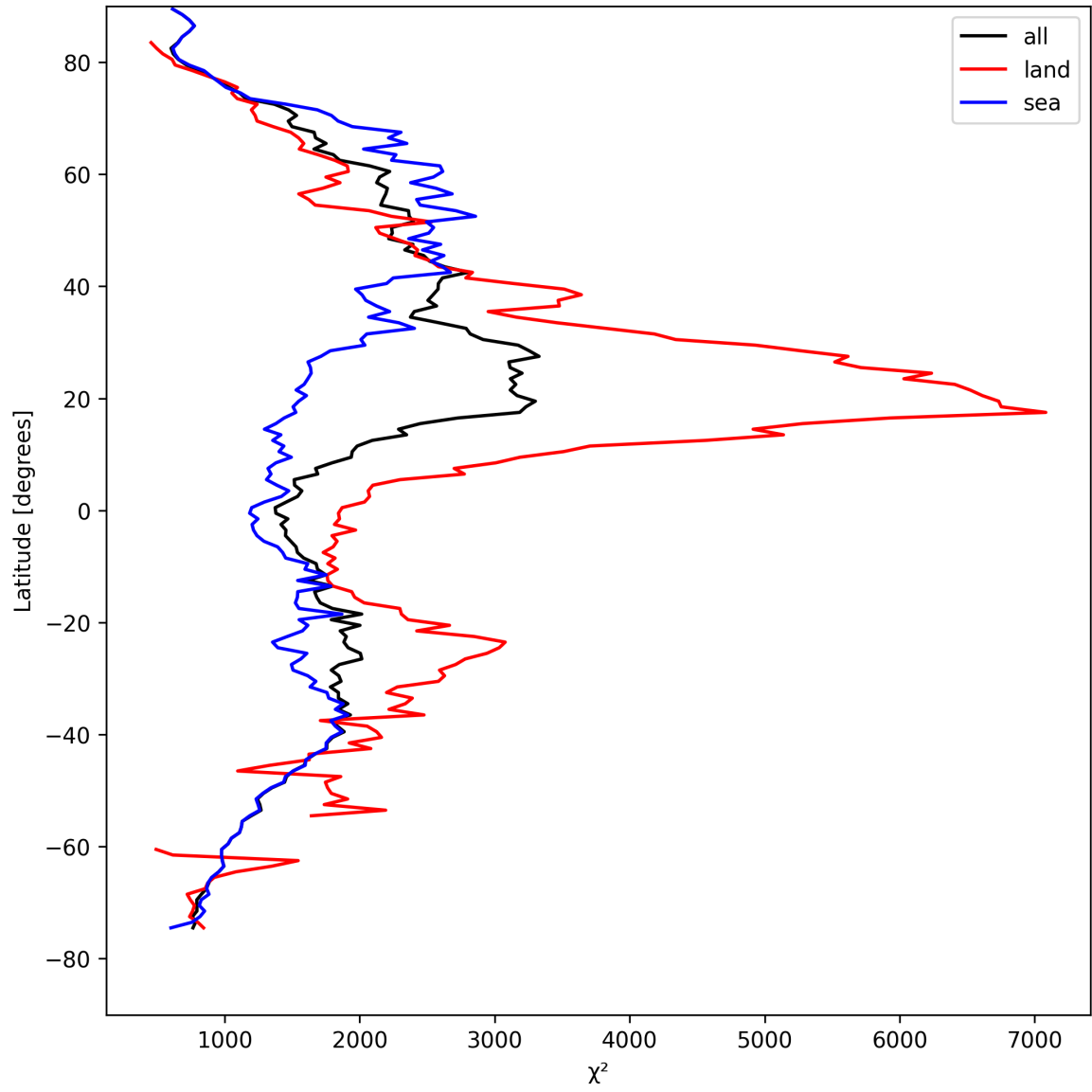
Figure 14: Zonal average of “ \chi^2 ” for 2025-04-15 to 2025-04-17.
