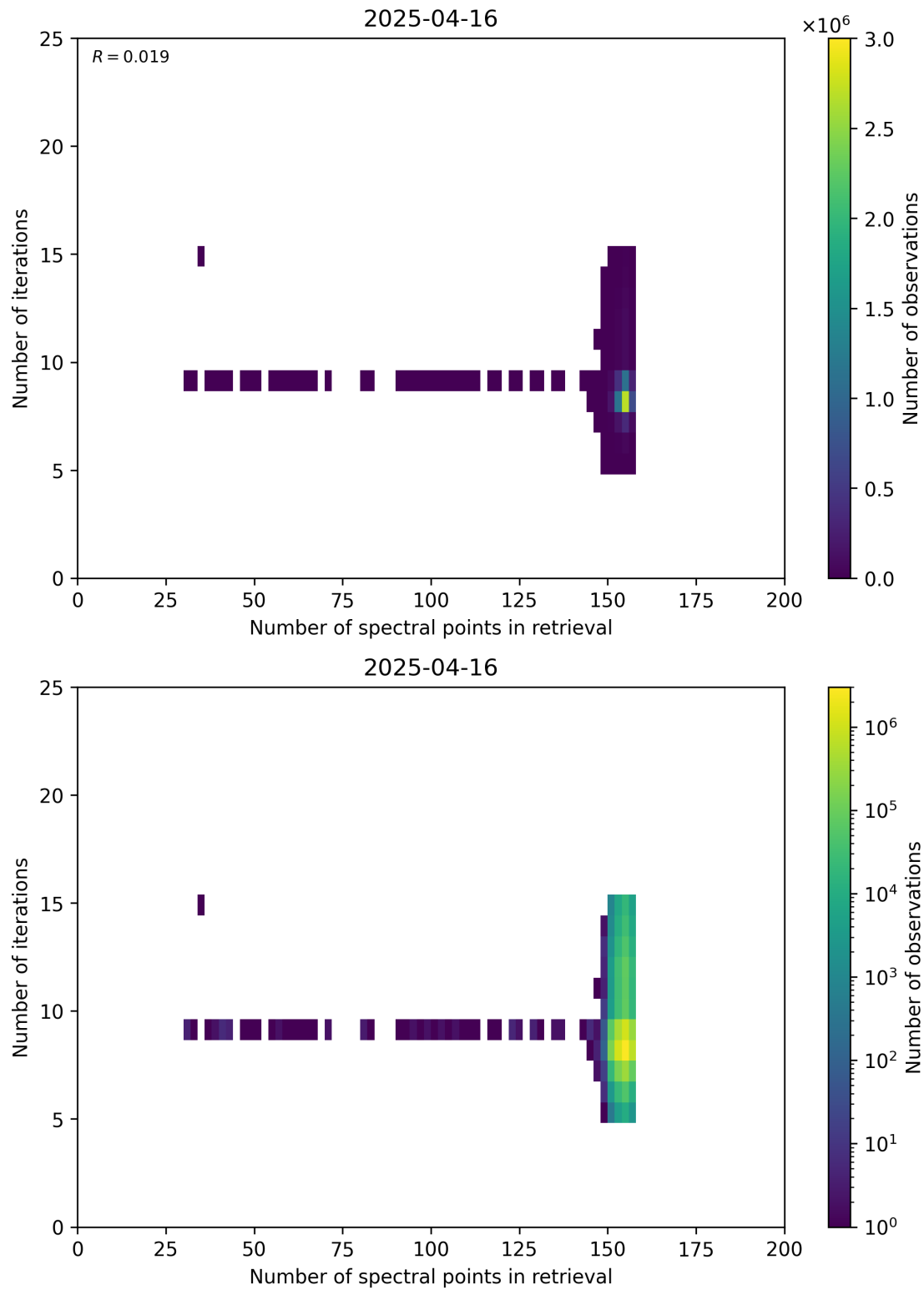
Figure 60: Scatter density plot of “Number of spectral points in retrieval” against “Number of iterations” for 2025-04-15 to 2025-04-17.
