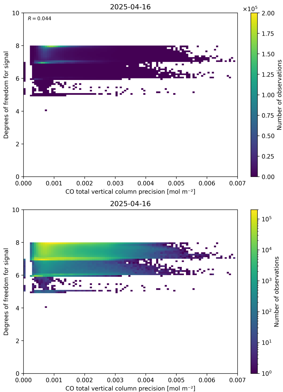
Figure 45: Scatter density plot of “CO total vertical column precision” against “Degrees of freedom for signal” for 2025-04-15 to 2025-04-17.
