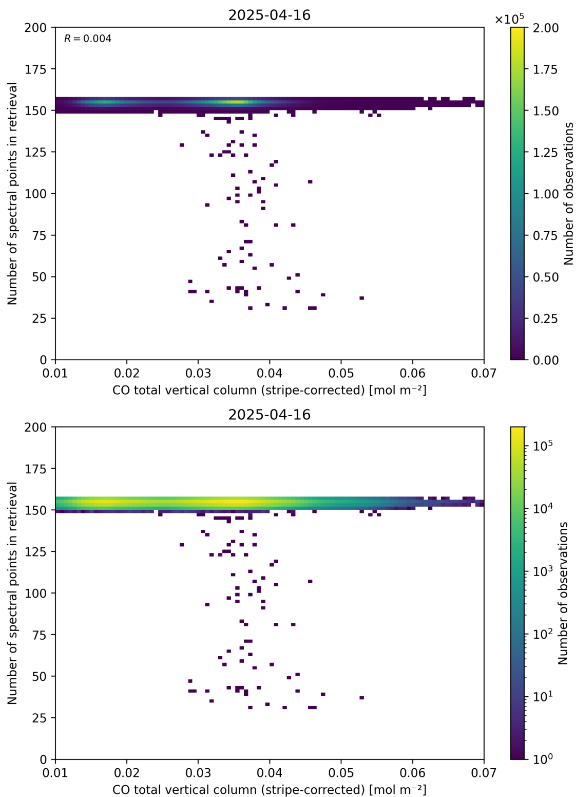
Figure 40: Scatter density plot of “CO total vertical column (stripe-corrected)” against “Number of spectral points in retrieval” for 2025-04-15 to 2025-04-17.
