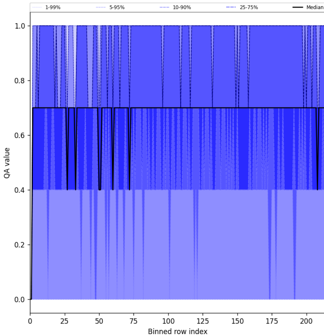
Figure 25: Along track statistics of “QA value” for 2025-04-15 to 2025-04-17
