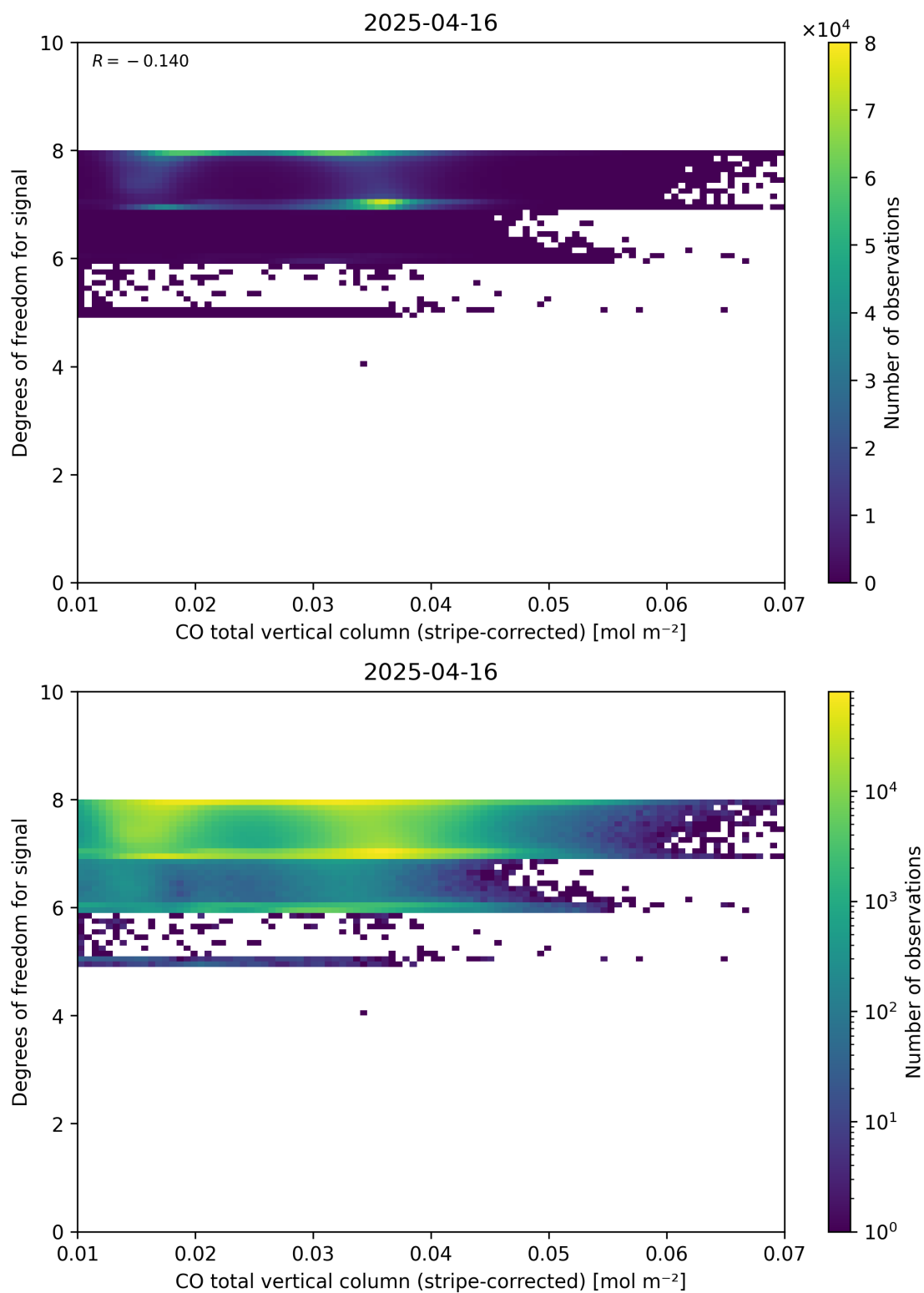
Figure 38: Scatter density plot of “CO total vertical column (stripe-corrected)” against “Degrees of freedom for signal” for 2025-04-15 to 2025-04-17.
