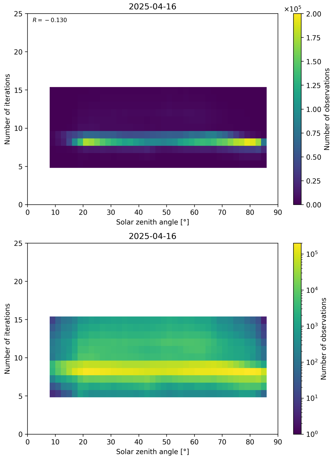
Figure 67: Scatter density plot of “Solar zenith angle” against “Number of iterations” for 2025-04-15 to 2025-04-17.
