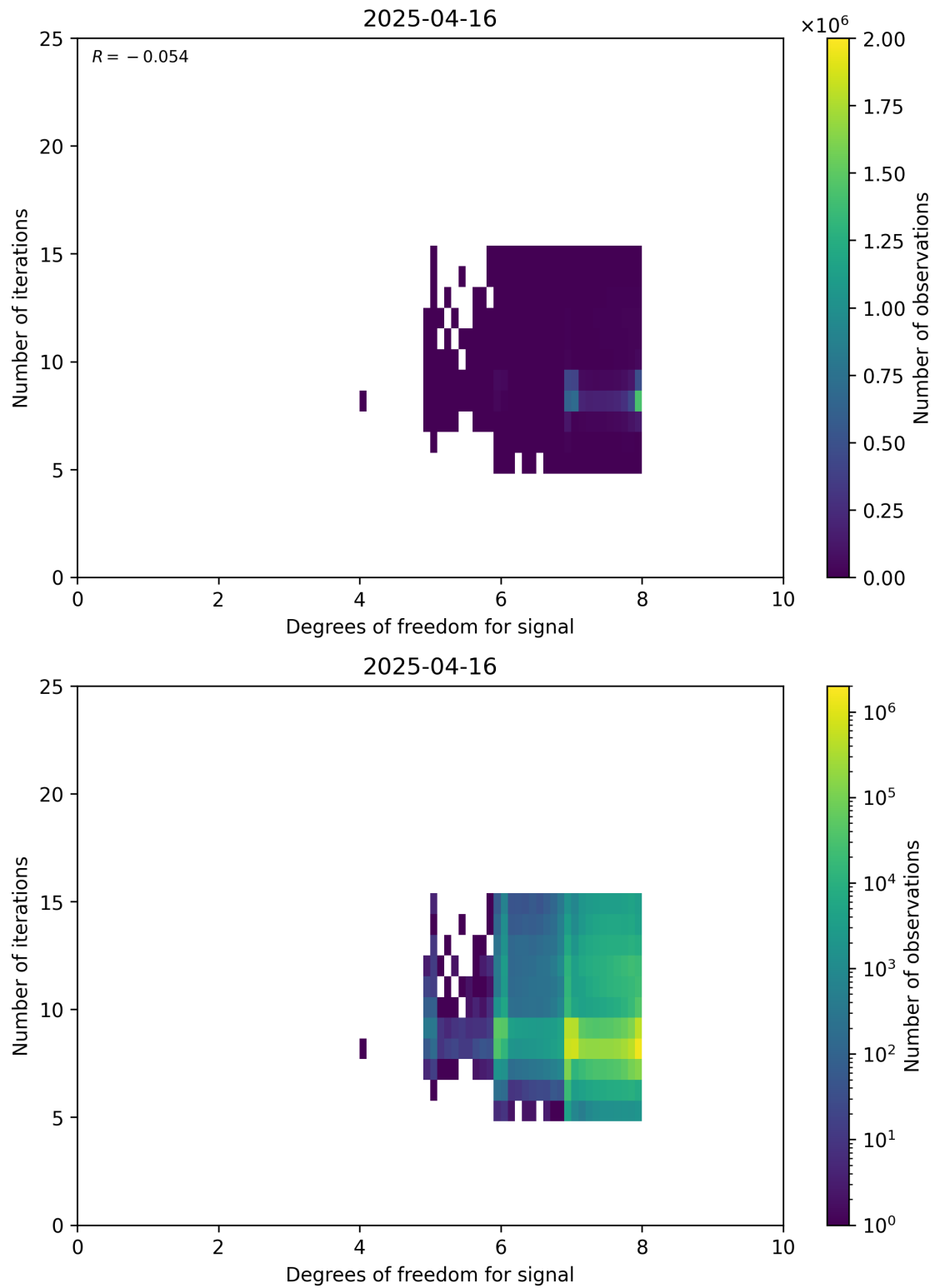
Figure 50: Scatter density plot of “Degrees of freedom for signal” against “Number of iterations” for 2025-04-15 to 2025-04-17.
