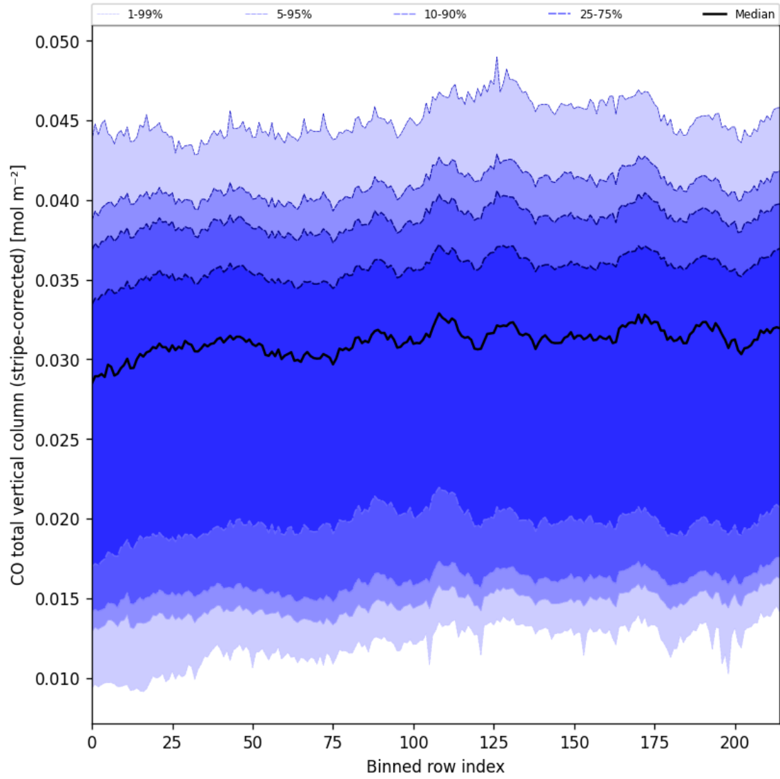
Figure 27: Along track statistics of “CO total vertical column (stripe-corrected)” for 2025-04-15 to 2025-04-17
