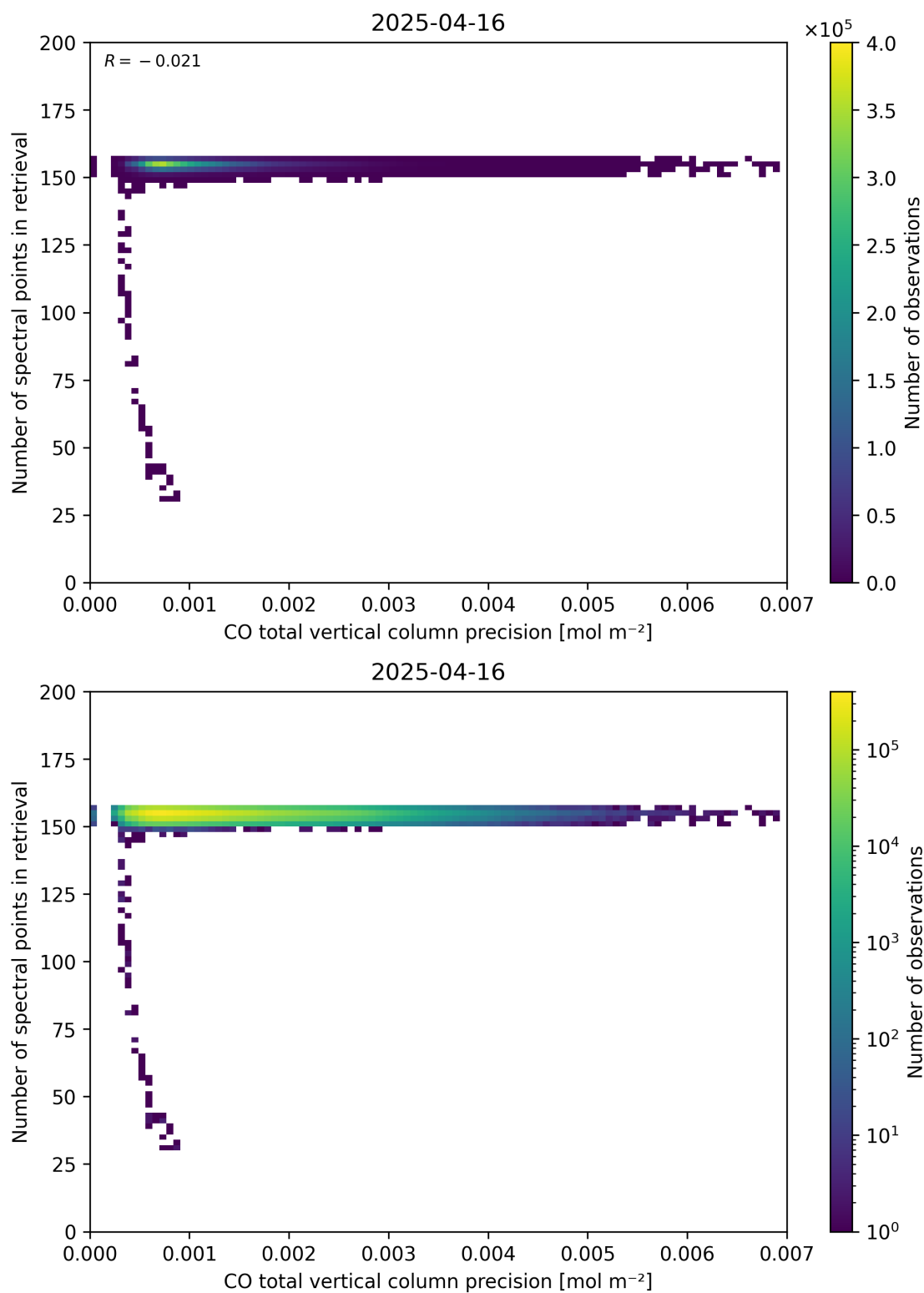
Figure 47: Scatter density plot of “CO total vertical column precision” against “Number of spectral points in retrieval” for 2025-04-15 to 2025-04-17.
