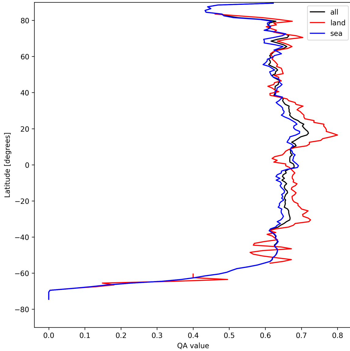
Figure 9: Zonal average of “QA value” for 2025-04-15 to 2025-04-17.
