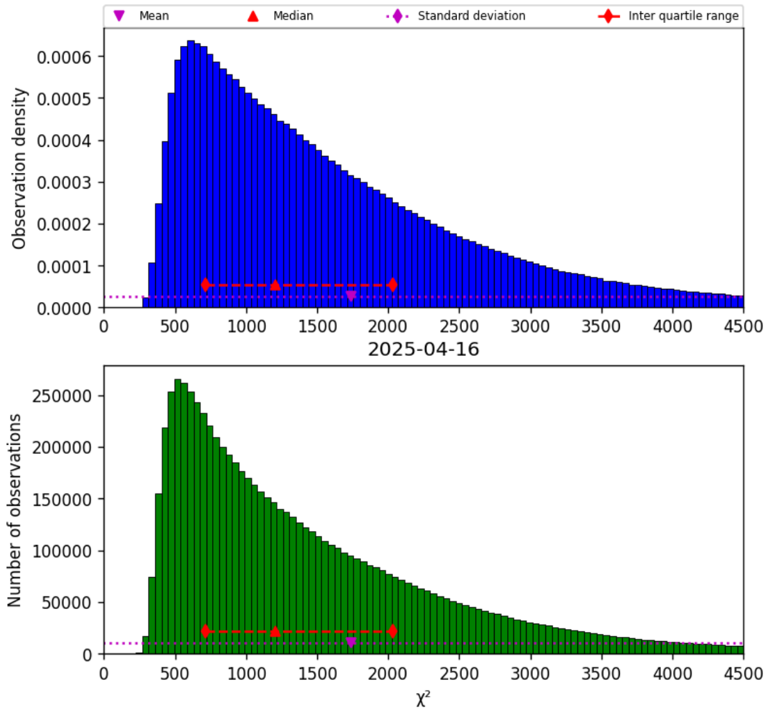
Figure 22: Histogram of “ \chi^2 ” for 2025-04-15 to 2025-04-17
