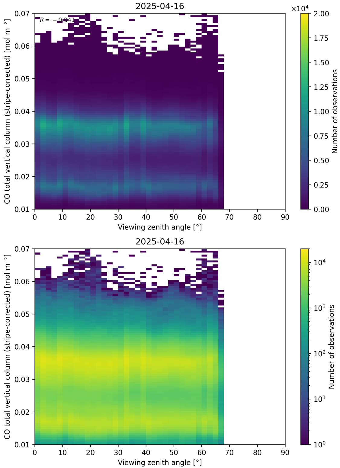
Figure 70: Scatter density plot of “Viewing zenith angle” against “CO total vertical column (stripe-corrected)” for 2025-04-15 to 2025-04-17.
