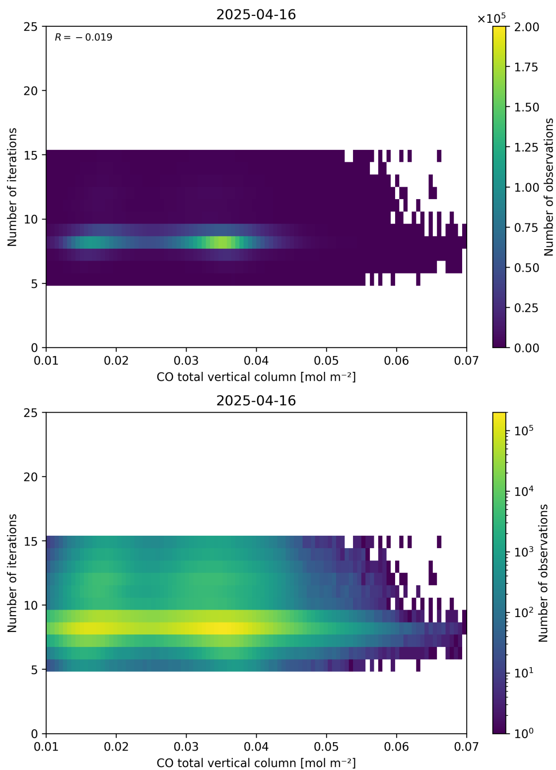
Figure 42: Scatter density plot of “CO total vertical column” against “Number of iterations” for 2025-04-15 to 2025-04-17.
