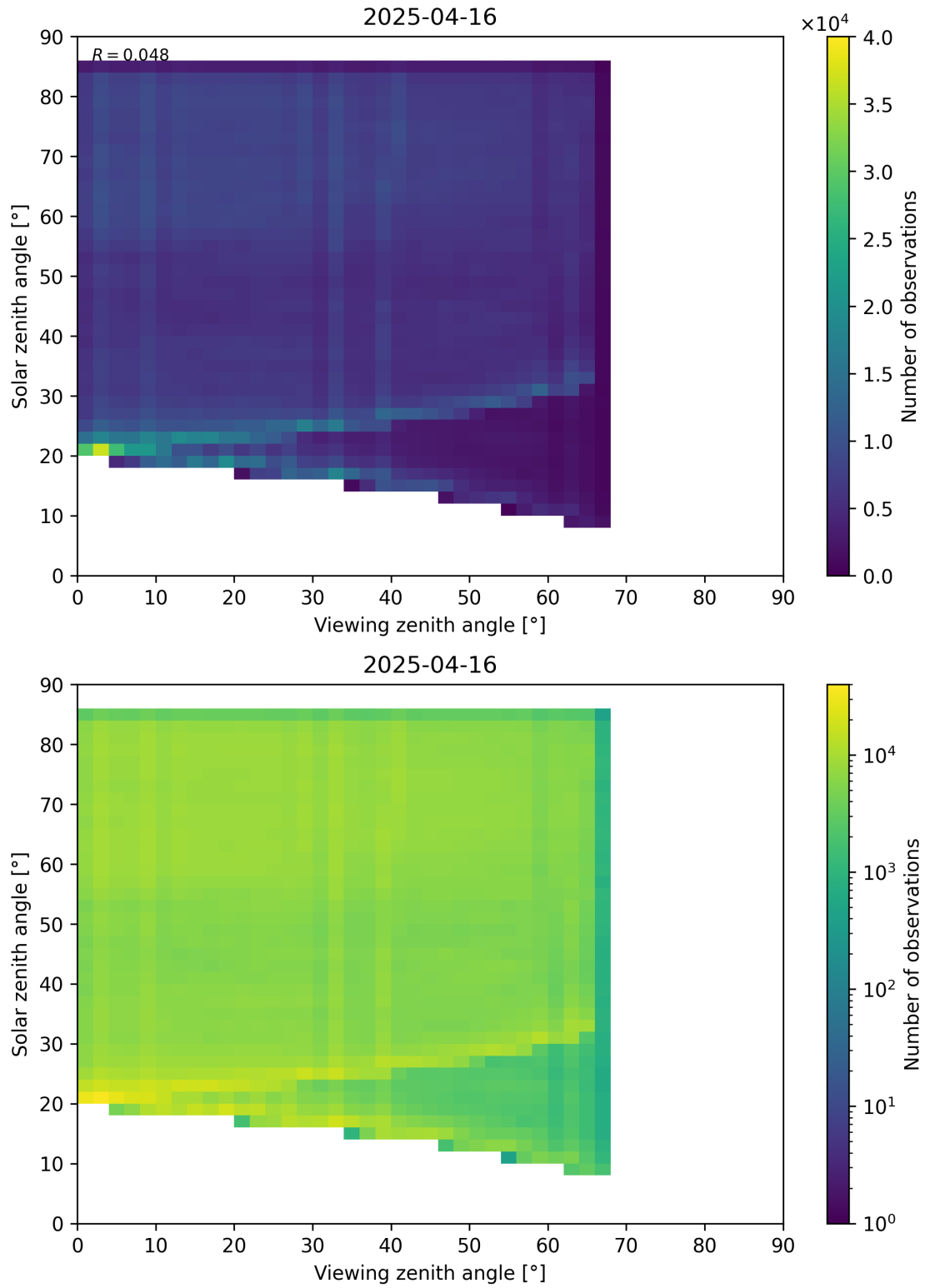
Figure 77: Scatter density plot of “Viewing zenith angle” against “Solar zenith angle” for 2025-04-15 to 2025-04-17.
