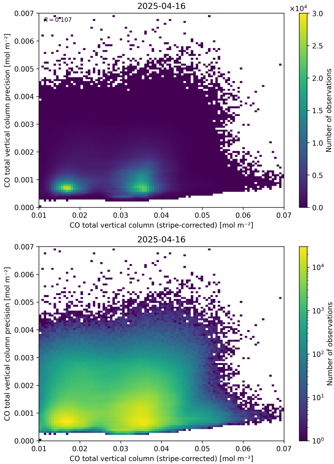
Figure 36: Scatter density plot of “CO total vertical column (stripe-corrected)” against “CO total vertical column precision” for 2025-04-15 to 2025-04-17.
