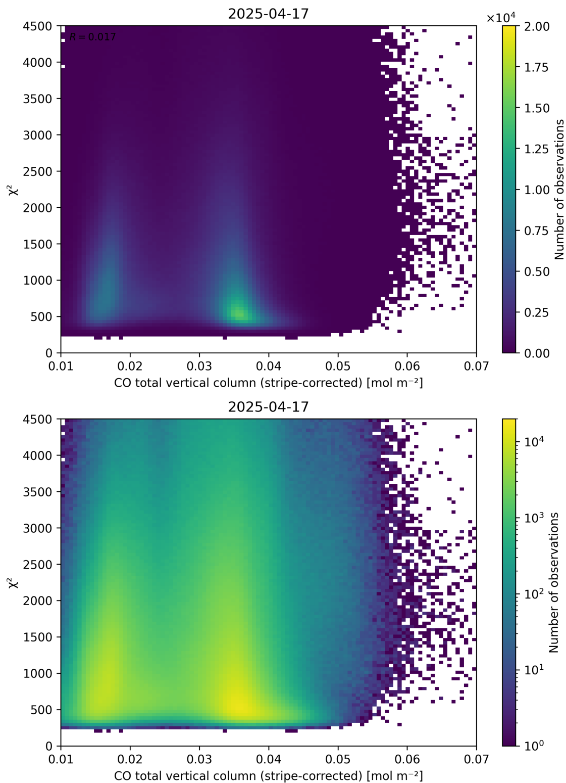
Figure 37: Scatter density plot of “CO total vertical column (stripe-corrected)” against “ \chi^2 ” for 2025-04-16 to 2025-04-18.
