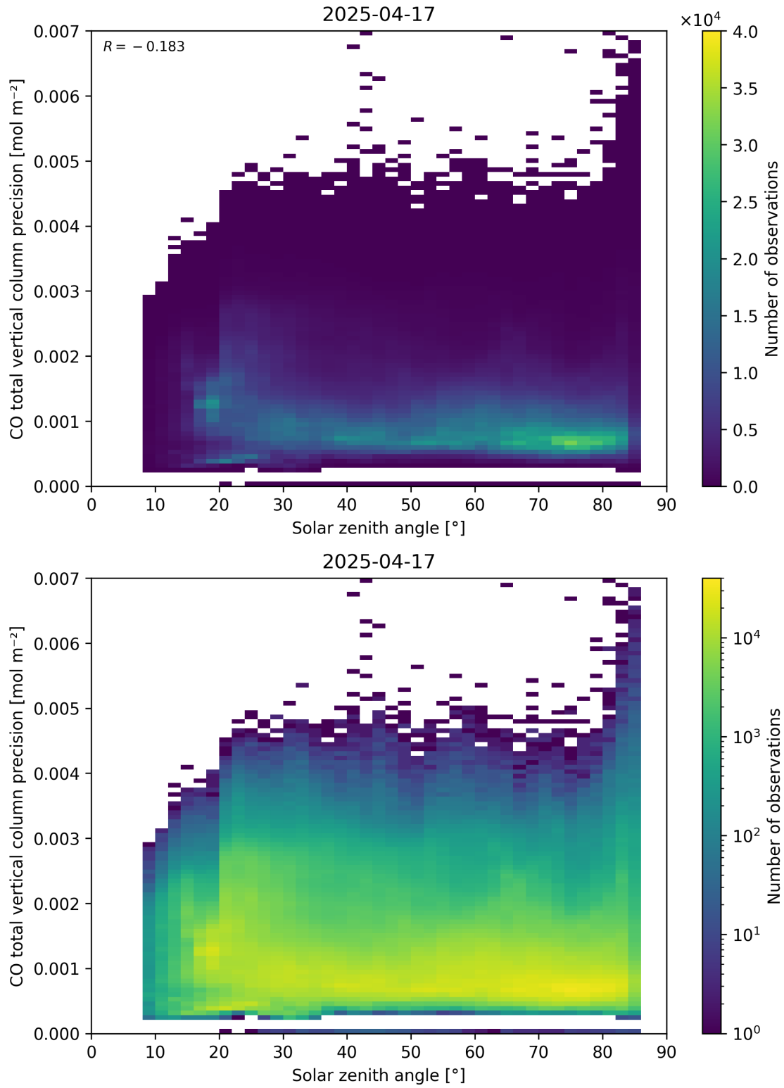
Figure 63: Scatter density plot of “Solar zenith angle” against “CO total vertical column precision” for 2025-04-16 to 2025-04-18.
