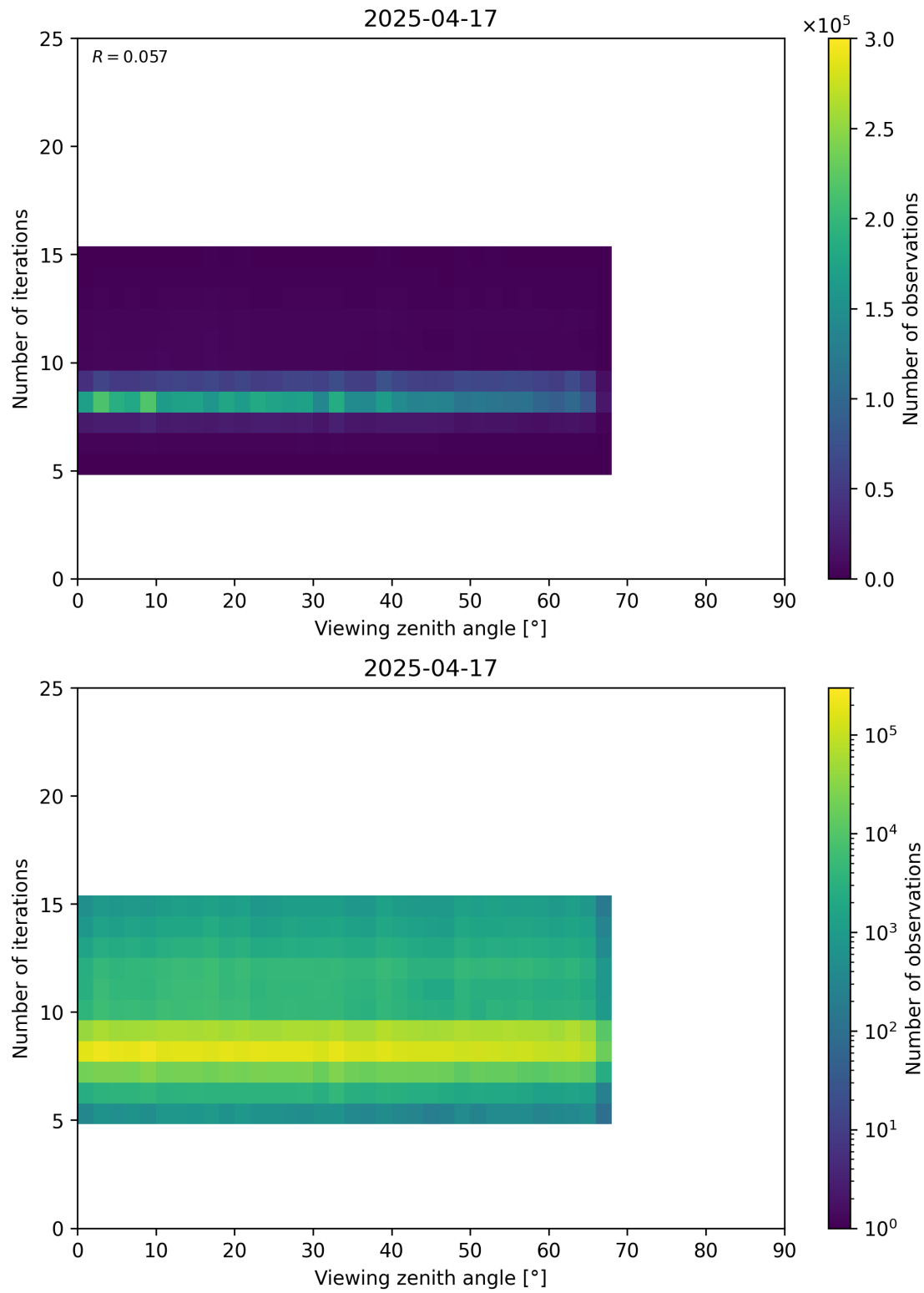
Figure 75: Scatter density plot of “Viewing zenith angle” against “Number of iterations” for 2025-04-16 to 2025-04-18.
