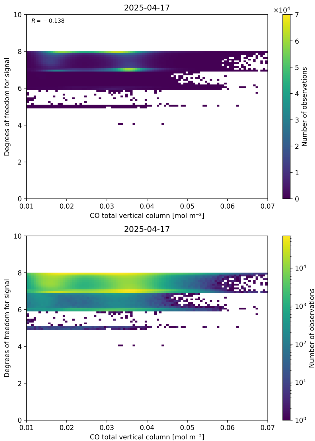
Figure 41: Scatter density plot of “CO total vertical column” against “Degrees of freedom for signal” for 2025-04-16 to 2025-04-18.
