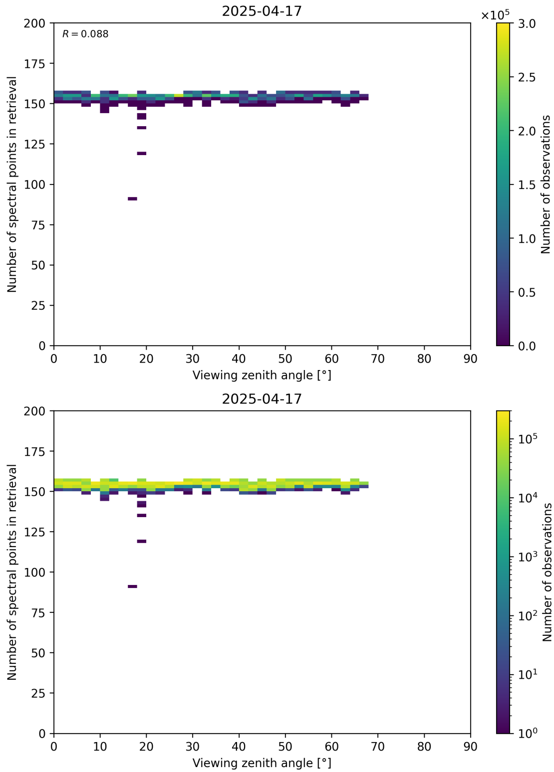
Figure 76: Scatter density plot of “Viewing zenith angle” against “Number of spectral points in retrieval” for 2025-04-16 to 2025-04-18.
