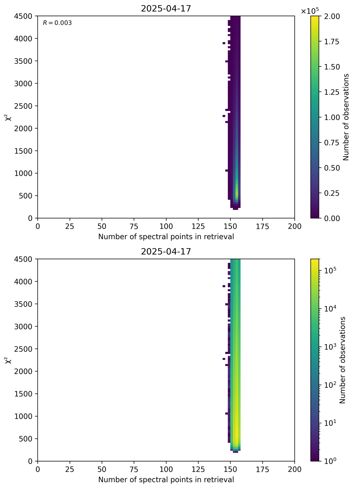
Figure 58: Scatter density plot of “Number of spectral points in retrieval” against “ \chi^2 ” for 2025-04-16 to 2025-04-18.
