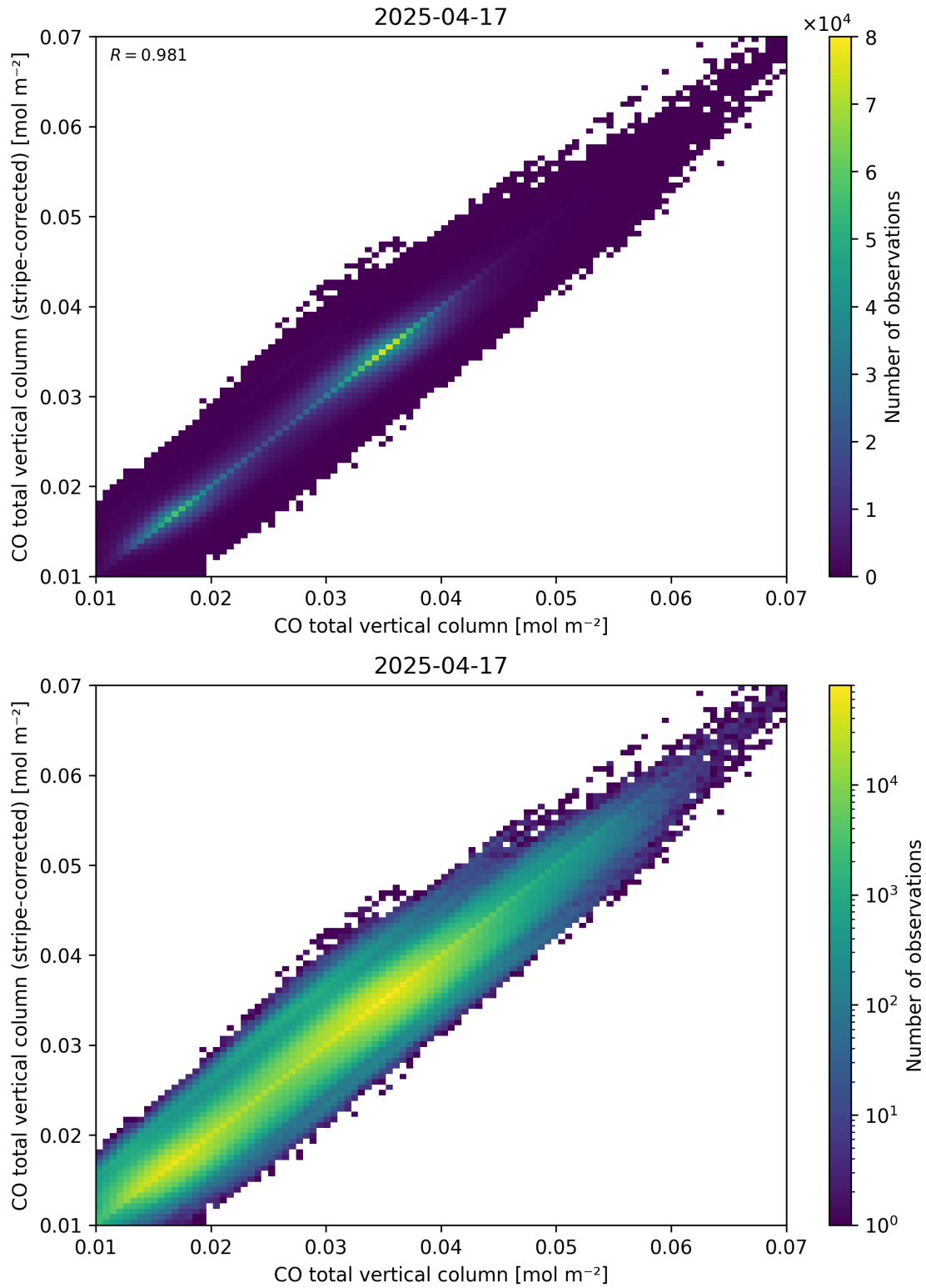
Figure 33: Scatter density plot of “CO total vertical column” against “CO total vertical column (stripe-corrected)” for 2025-04-16 to 2025-04-18.
