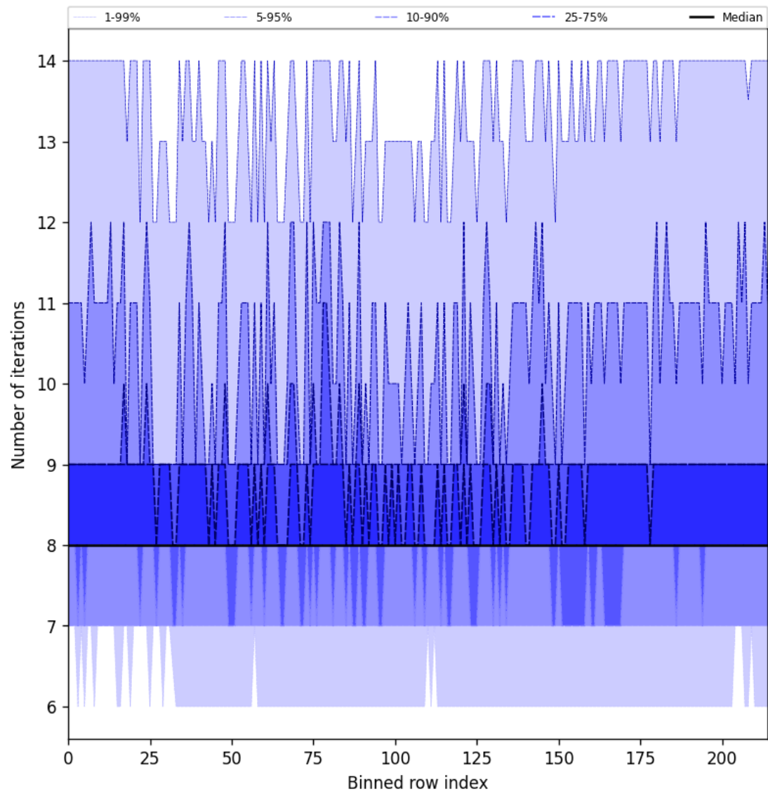
Figure 32: Along track statistics of “Number of iterations” for 2025-04-16 to 2025-04-18
