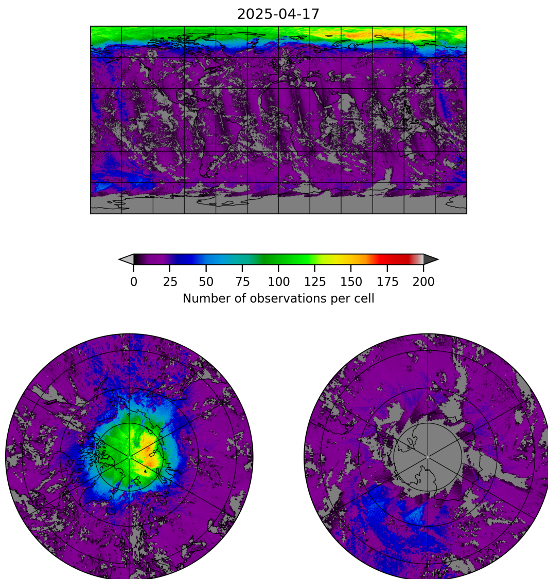
Figure 8: Map of the number of observations for 2025-04-16 to 2025-04-18
