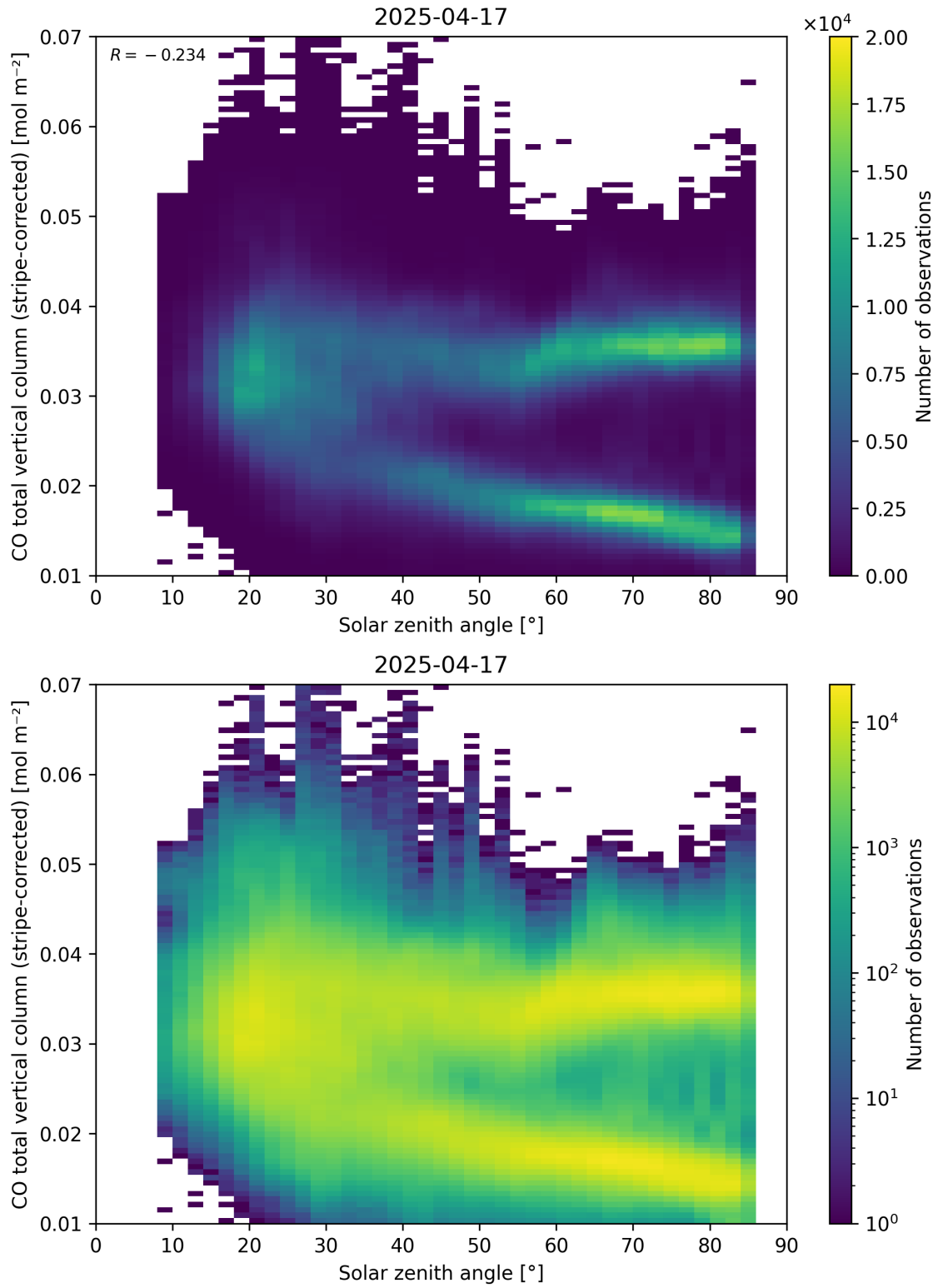
Figure 62: Scatter density plot of “Solar zenith angle” against “CO total vertical column (stripe-corrected)” for 2025-04-16 to 2025-04-18.
