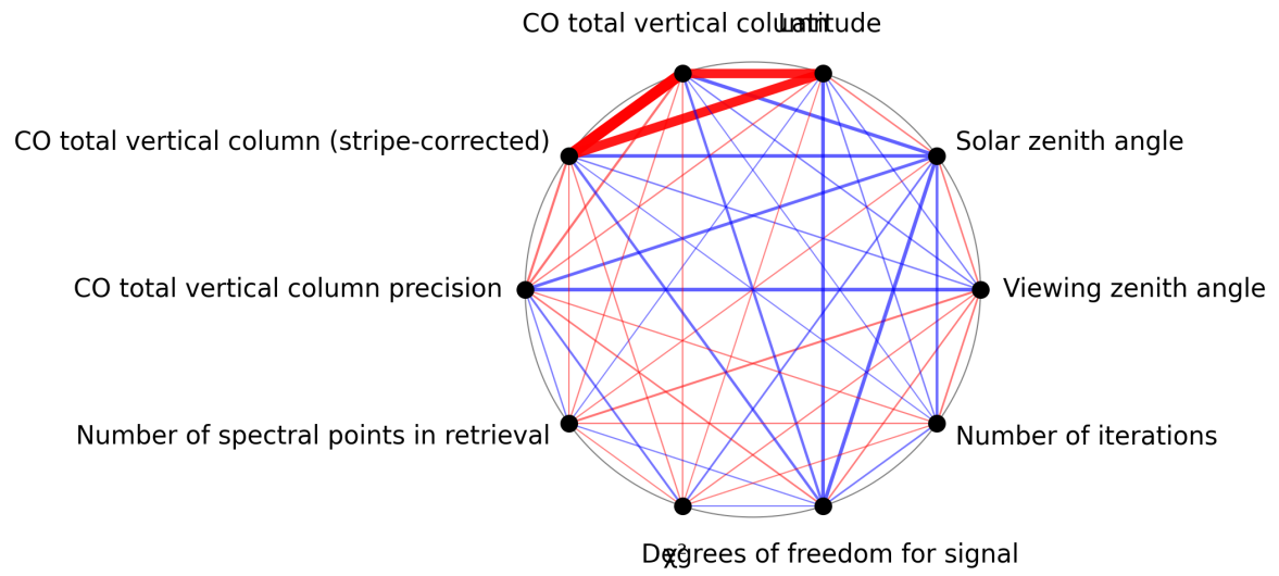
Figure 1: Map of correlation graph for 2025-04-16 to 2025-04-18.
