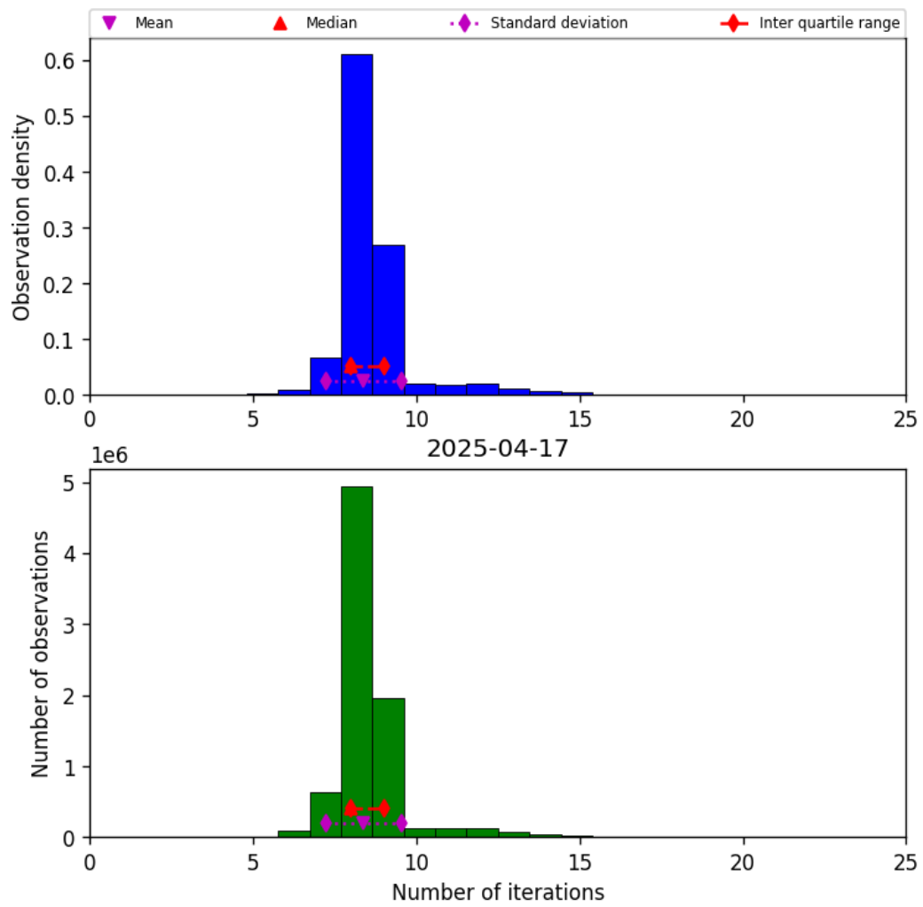
Figure 24: Histogram of “Number of iterations” for 2025-04-16 to 2025-04-18
