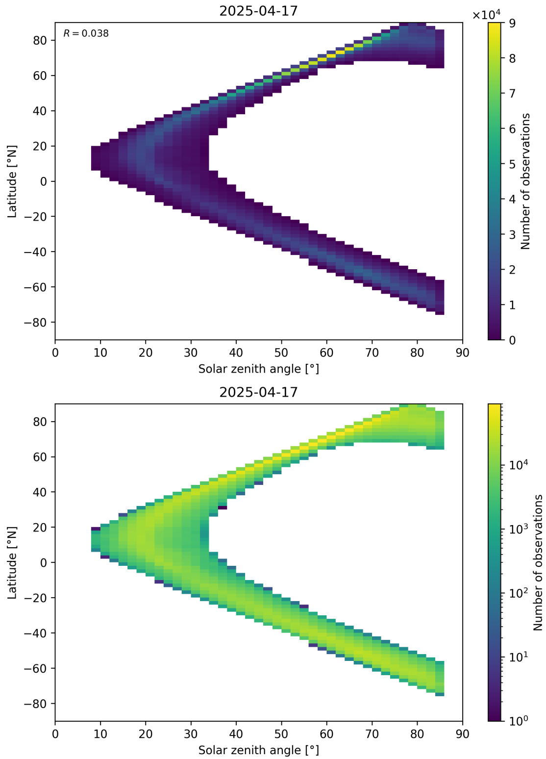
Figure 66: Scatter density plot of “Solar zenith angle” against “Latitude” for 2025-04-16 to 2025-04-18.
