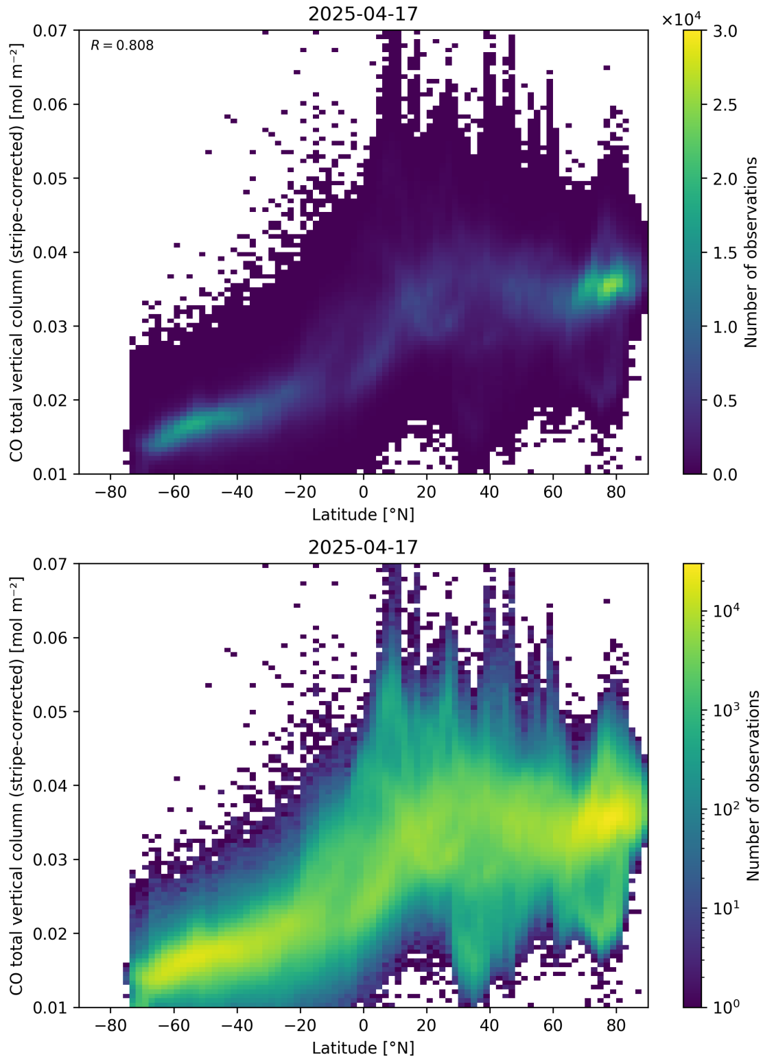
Figure 52: Scatter density plot of “Latitude” against “CO total vertical column (stripe-corrected)” for 2025-04-16 to 2025-04-18.
