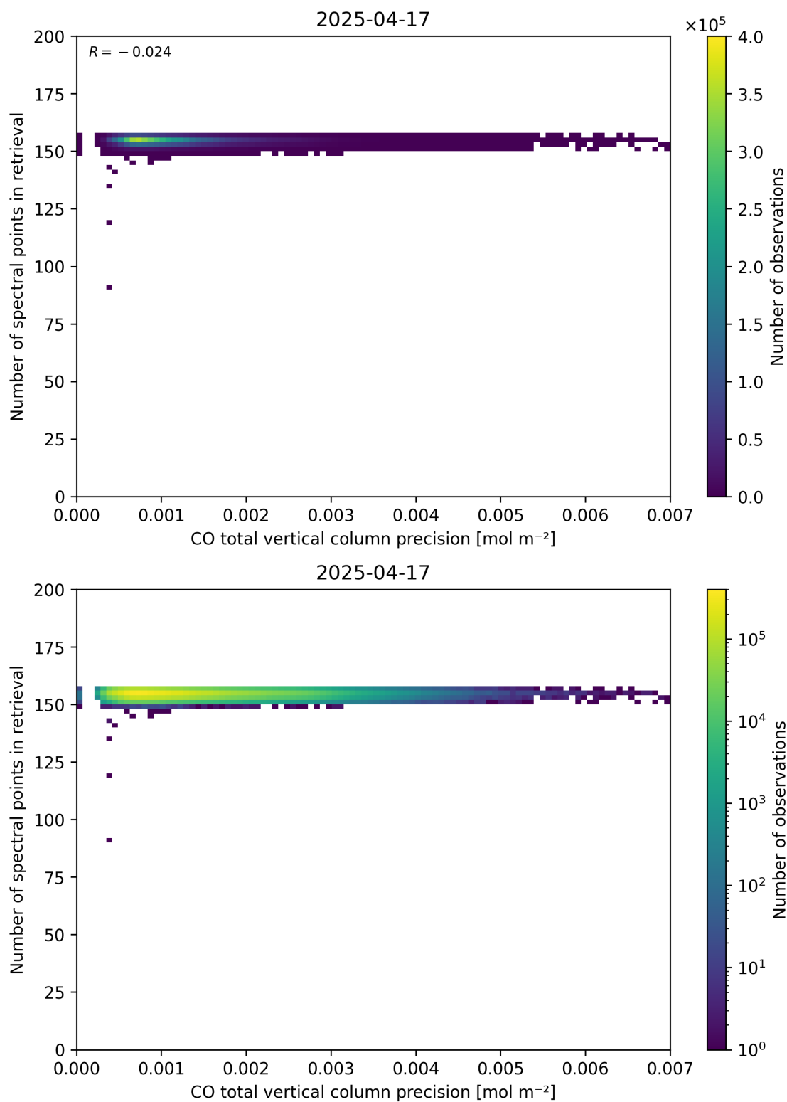
Figure 47: Scatter density plot of “CO total vertical column precision” against “Number of spectral points in retrieval” for 2025-04-16 to 2025-04-18.
