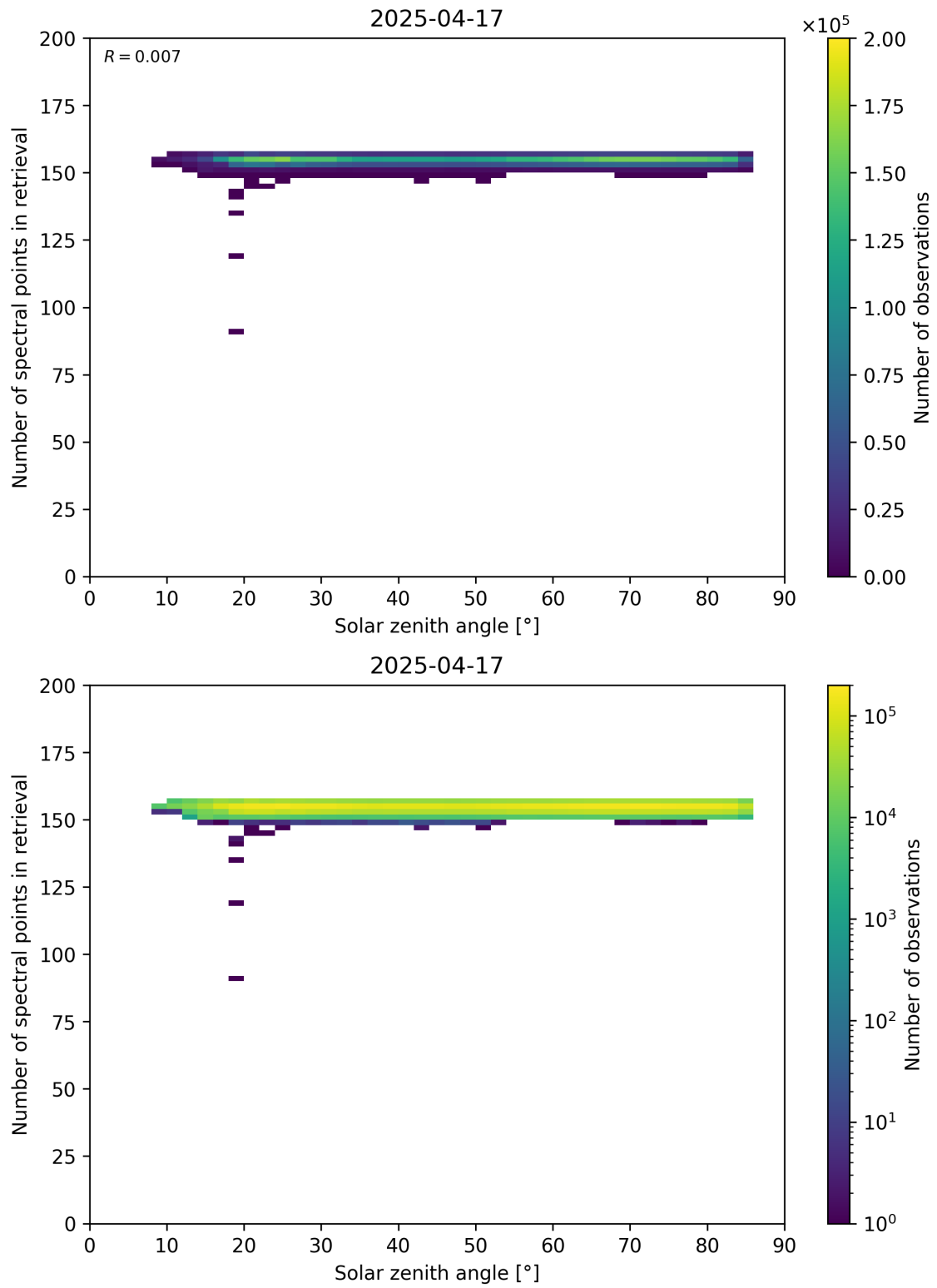
Figure 68: Scatter density plot of “Solar zenith angle” against “Number of spectral points in retrieval” for 2025-04-16 to 2025-04-18.
