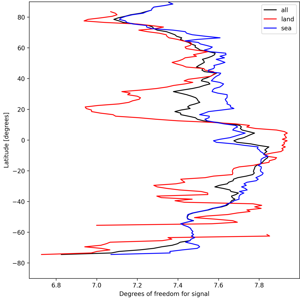
Figure 15: Zonal average of “Degrees of freedom for signal” for 2025-04-16 to 2025-04-18.
