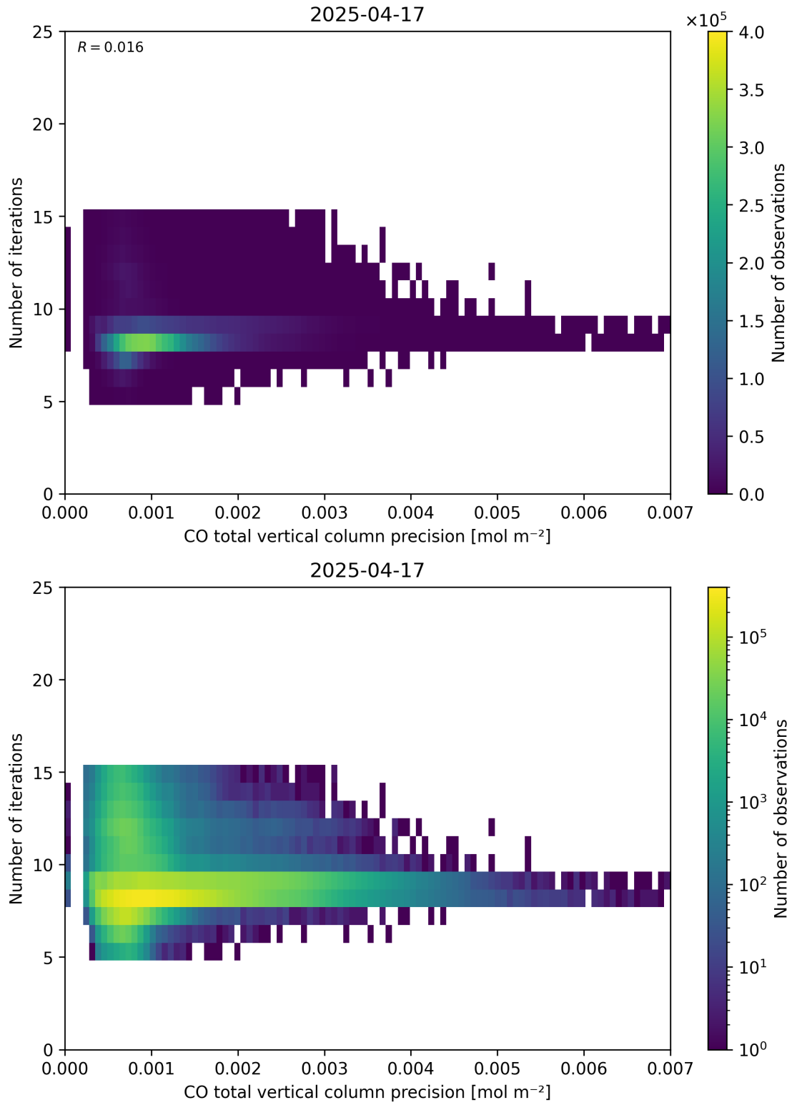
Figure 46: Scatter density plot of “CO total vertical column precision” against “Number of iterations” for 2025-04-16 to 2025-04-18.
