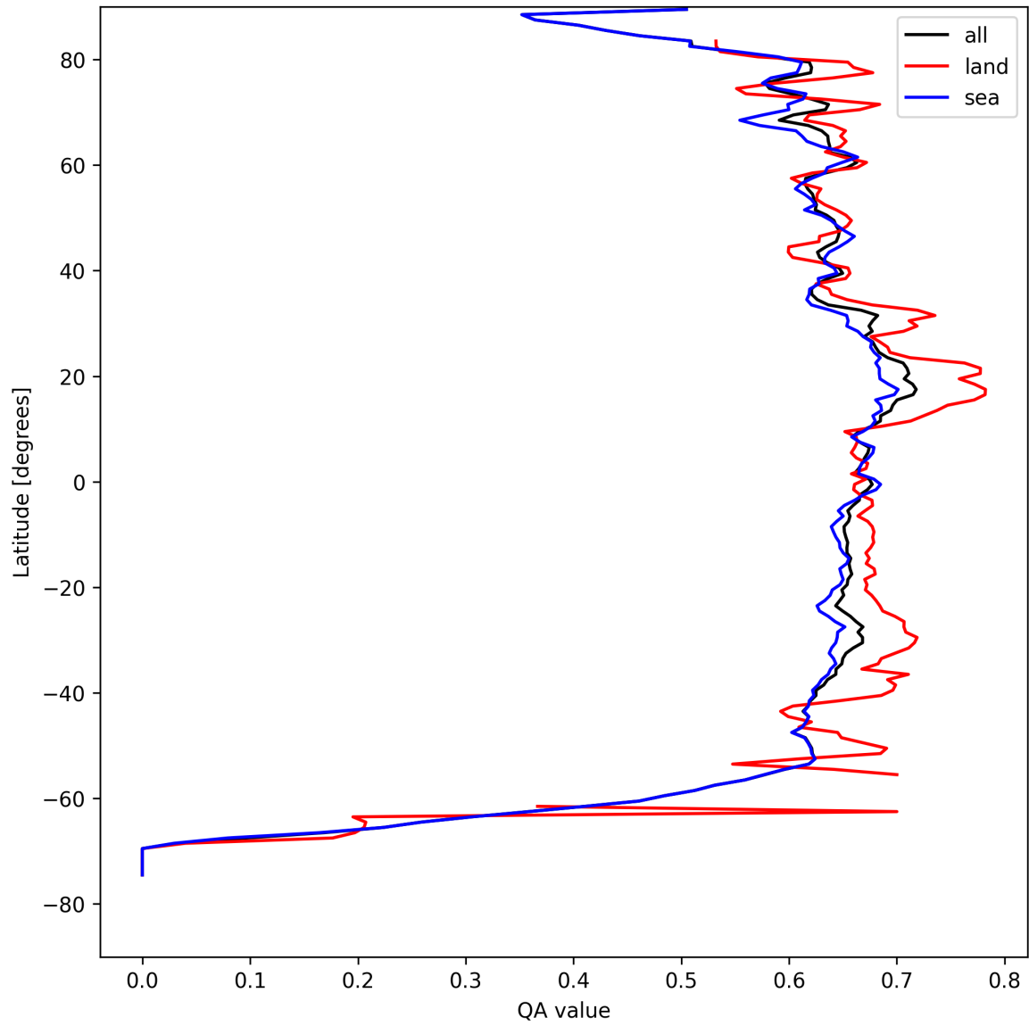
Figure 9: Zonal average of “QA value” for 2025-04-16 to 2025-04-18.
