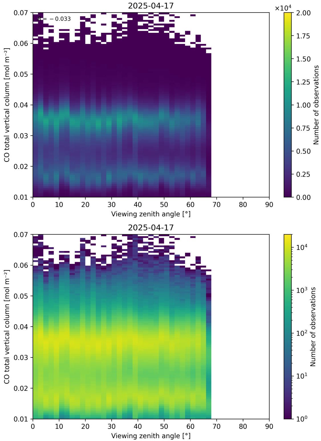
Figure 69: Scatter density plot of “Viewing zenith angle” against “CO total vertical column” for 2025-04-16 to 2025-04-18.
