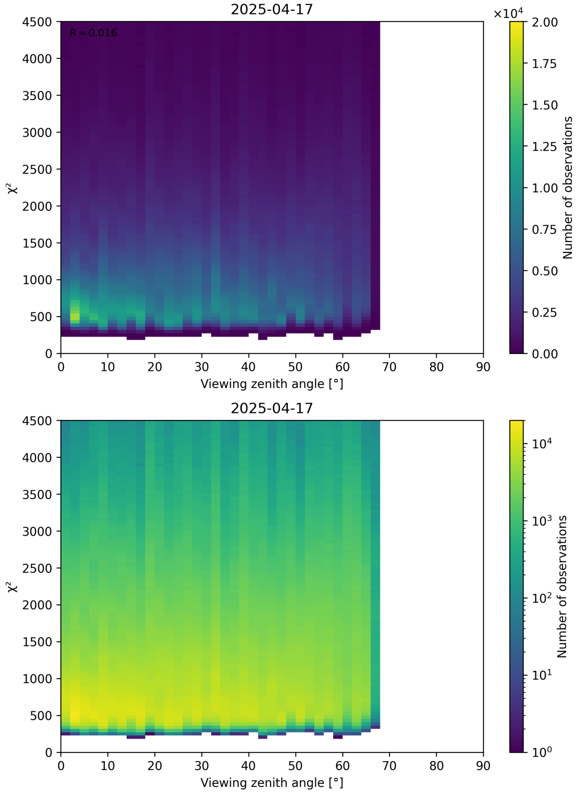
Figure 72: Scatter density plot of “Viewing zenith angle” against “ \chi^2 ” for 2025-04-16 to 2025-04-18.
