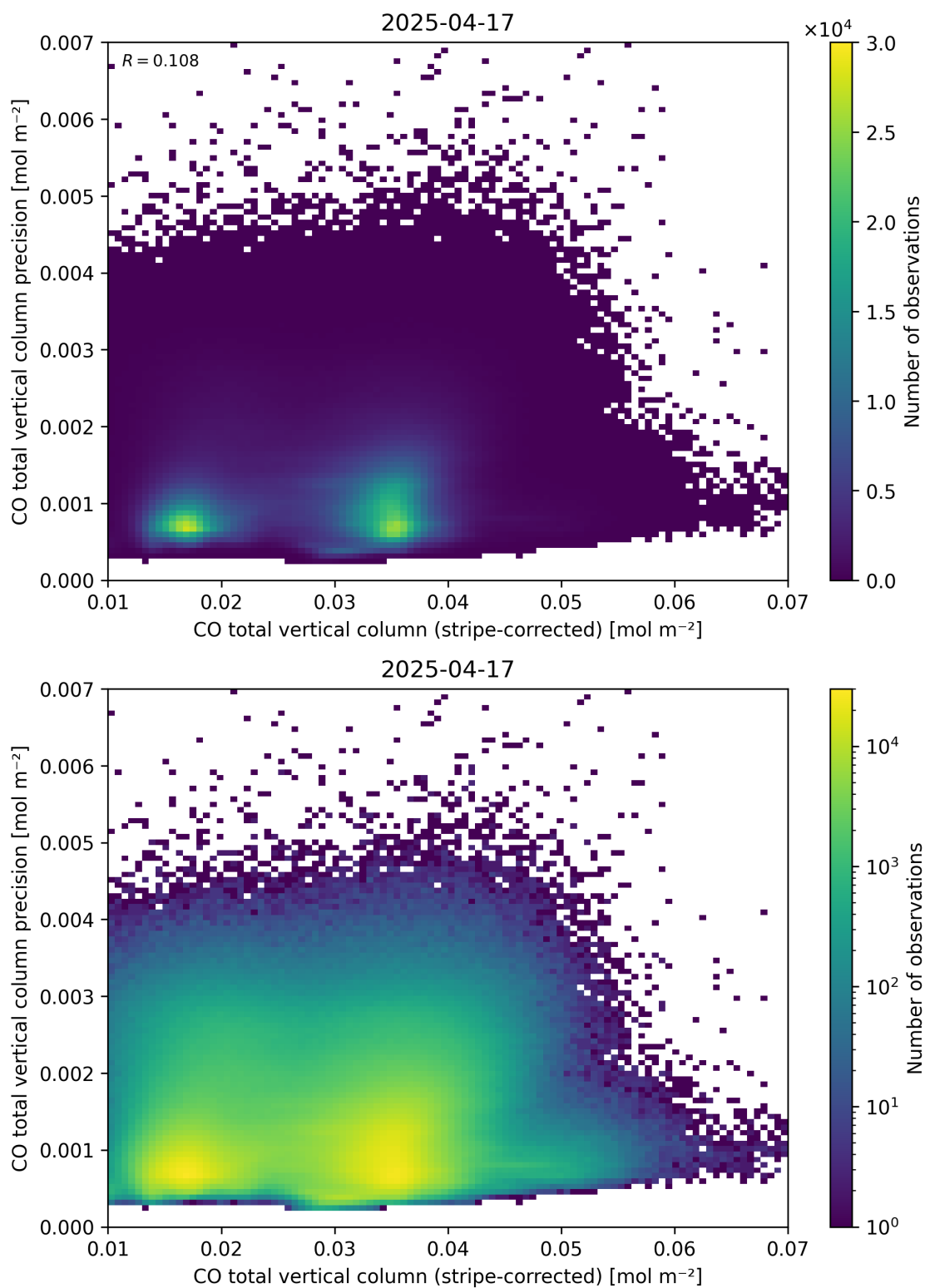
Figure 36: Scatter density plot of “CO total vertical column (stripe-corrected)” against “CO total vertical column precision” for 2025-04-16 to 2025-04-18.
