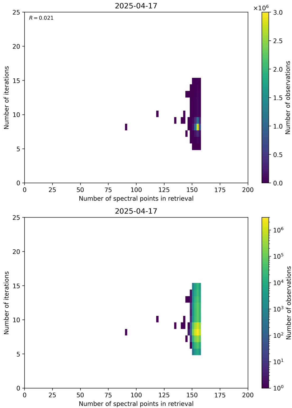
Figure 60: Scatter density plot of “Number of spectral points in retrieval” against “Number of iterations” for 2025-04-16 to 2025-04-18.
