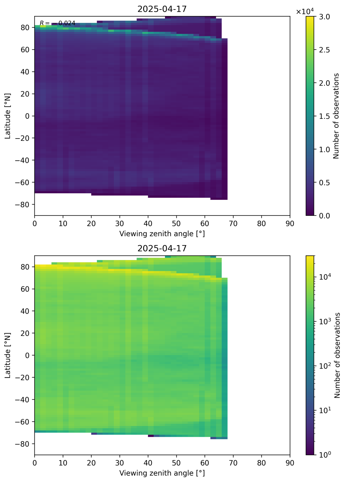
Figure 74: Scatter density plot of “Viewing zenith angle” against “Latitude” for 2025-04-16 to 2025-04-18.
