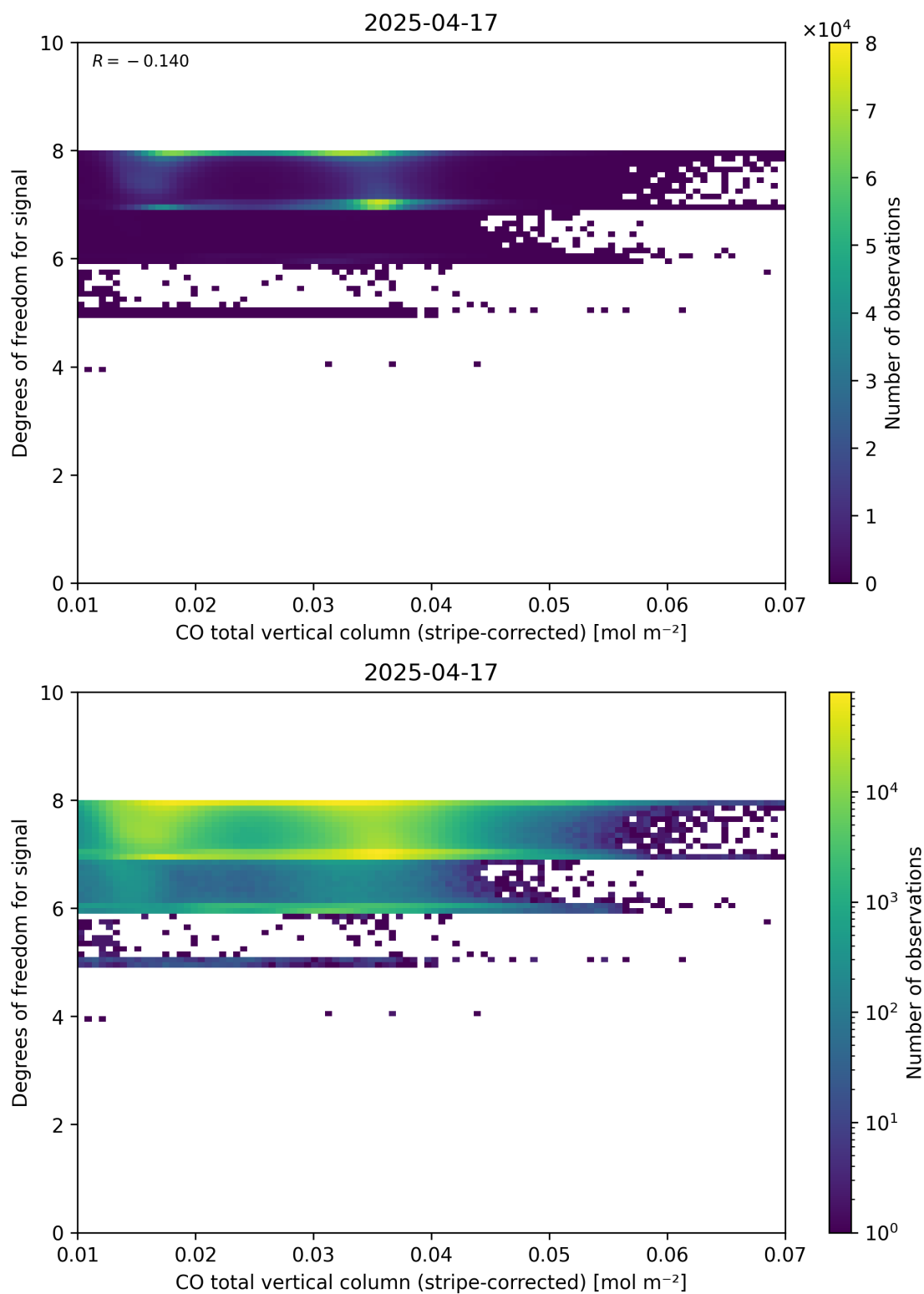
Figure 38: Scatter density plot of “CO total vertical column (stripe-corrected)” against “Degrees of freedom for signal” for 2025-04-16 to 2025-04-18.
