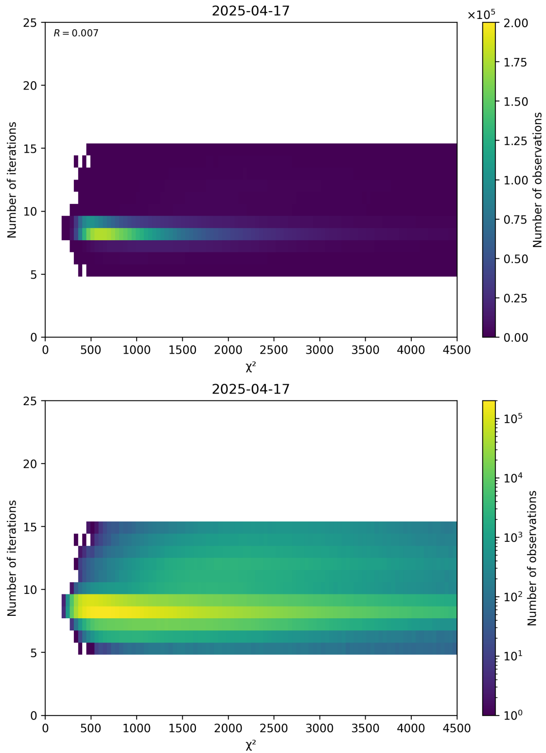
Figure 49: Scatter density plot of “ \chi^2 ” against “Number of iterations” for 2025-04-16 to 2025-04-18.
