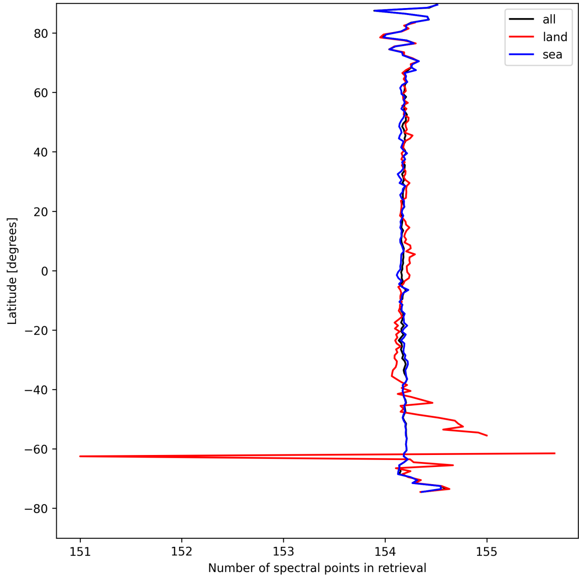
Figure 13: Zonal average of “Number of spectral points in retrieval” for 2025-04-16 to 2025-04-18.
