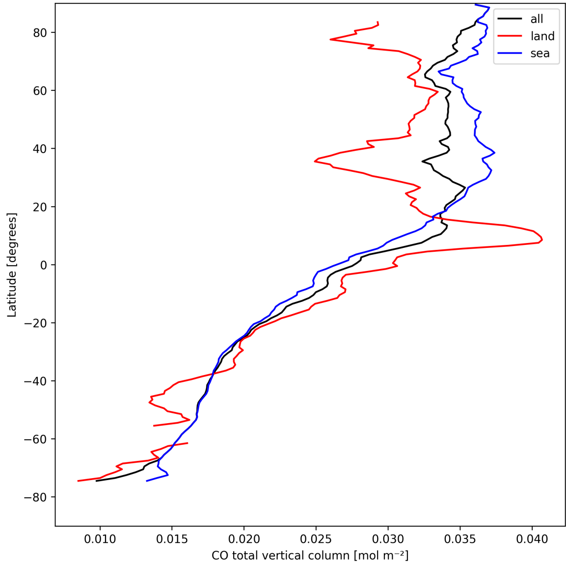
Figure 10: Zonal average of “CO total vertical column” for 2025-04-16 to 2025-04-18.
