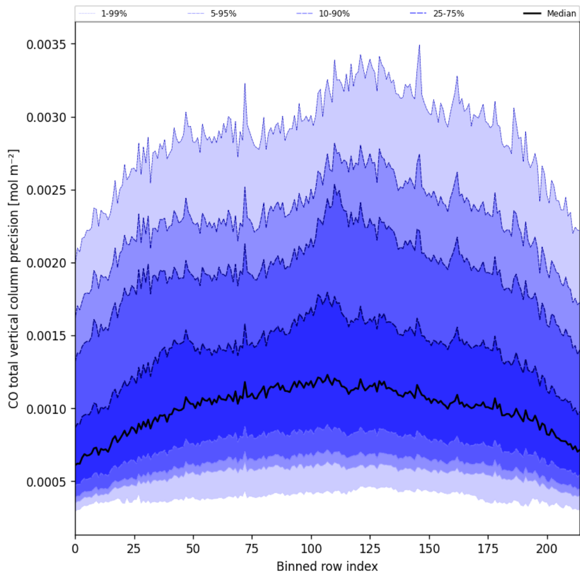
Figure 28: Along track statistics of “CO total vertical column precision” for 2025-04-16 to 2025-04-18
