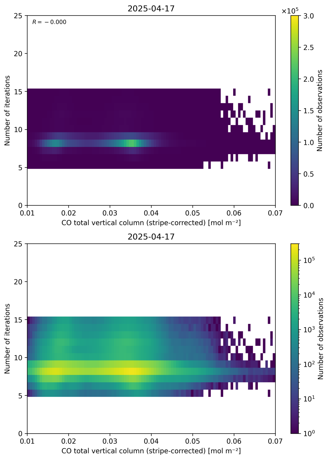
Figure 39: Scatter density plot of “CO total vertical column (stripe-corrected)” against “Number of iterations” for 2025-04-16 to 2025-04-18.
