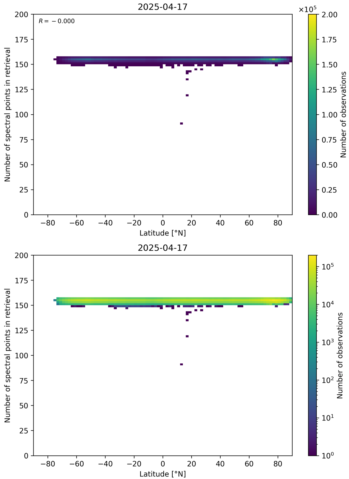
Figure 57: Scatter density plot of “Latitude” against “Number of spectral points in retrieval” for 2025-04-16 to 2025-04-18.
