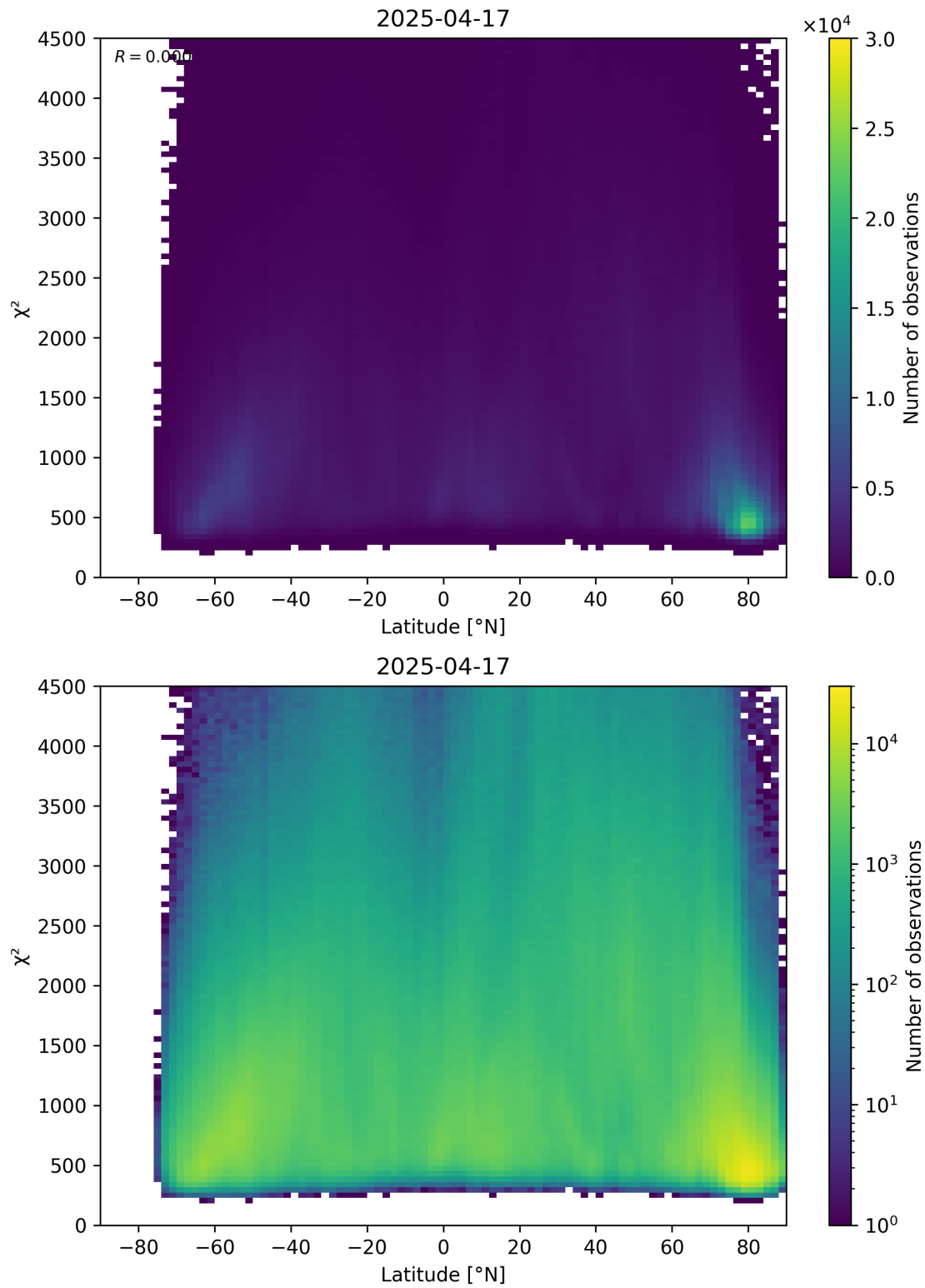
Figure 54: Scatter density plot of “Latitude” against “ \chi^2 ” for 2025-04-16 to 2025-04-18.
