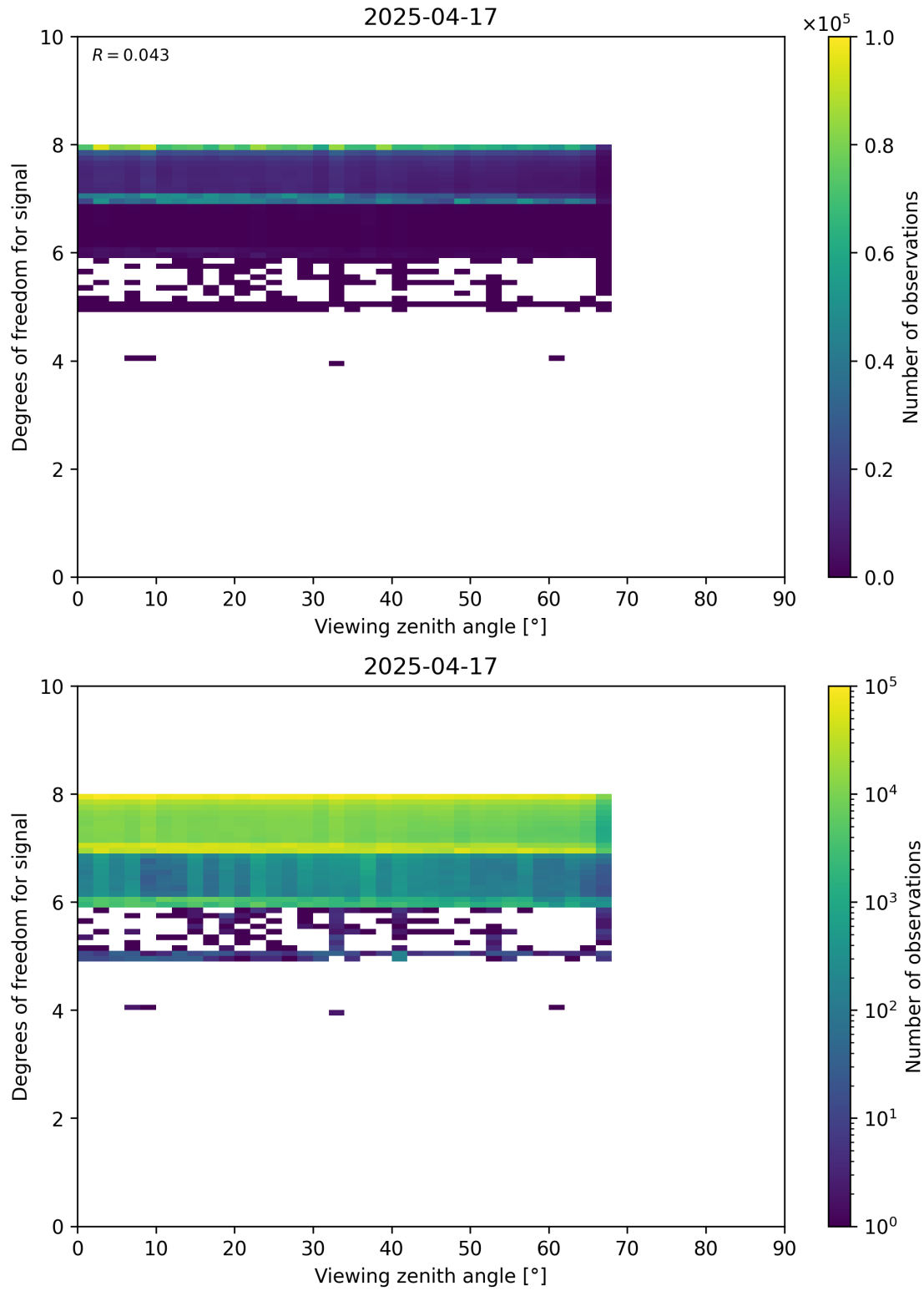
Figure 73: Scatter density plot of “Viewing zenith angle” against “Degrees of freedom for signal” for 2025-04-16 to 2025-04-18.
