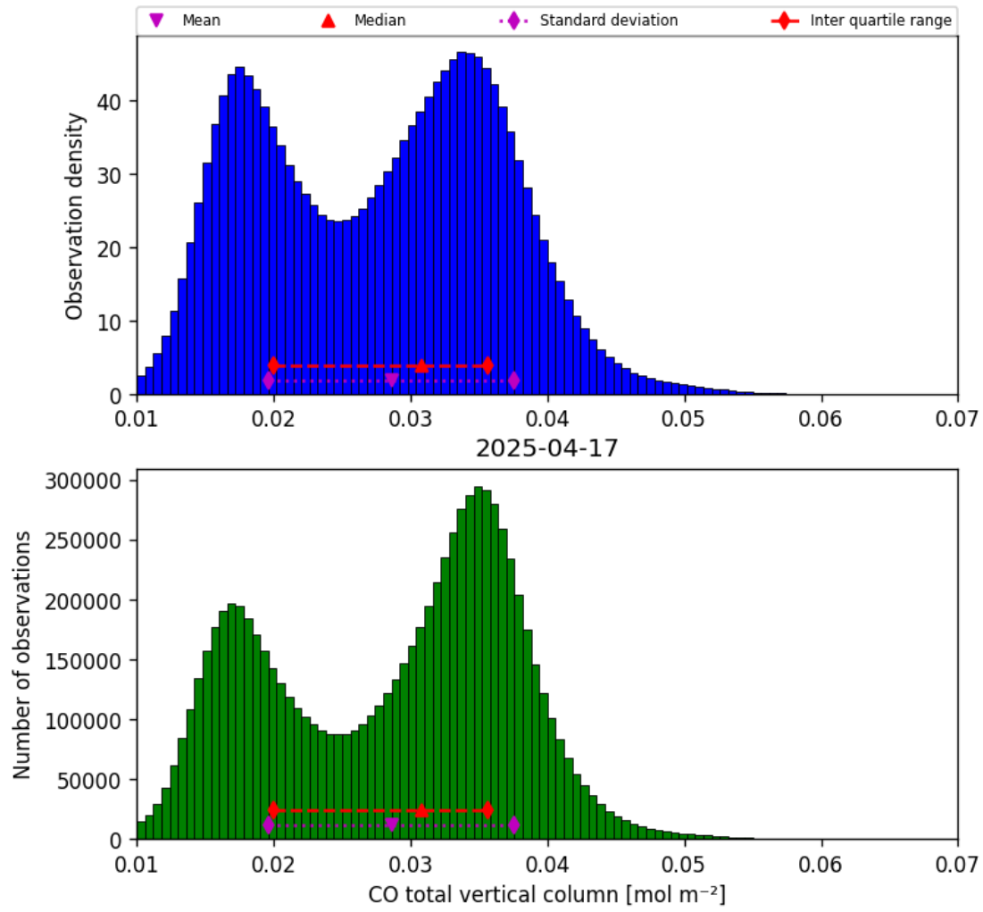
Figure 18: Histogram of “CO total vertical column” for 2025-04-16 to 2025-04-18
