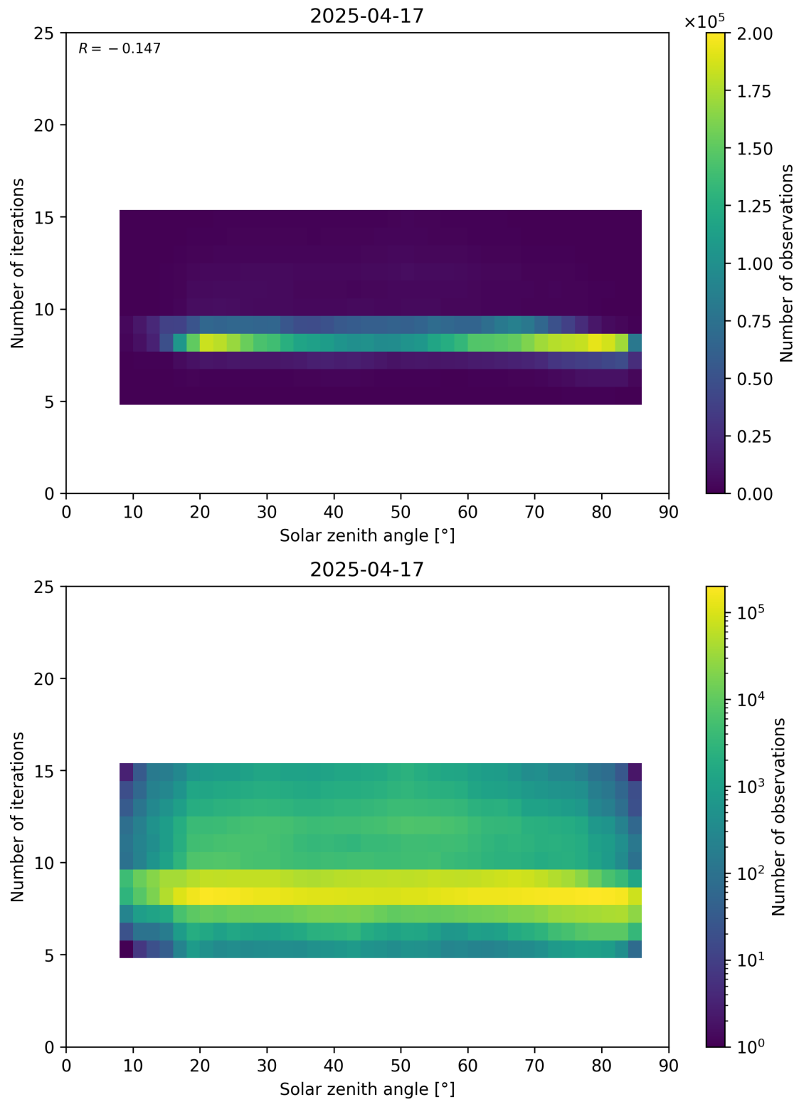
Figure 67: Scatter density plot of “Solar zenith angle” against “Number of iterations” for 2025-04-16 to 2025-04-18.
