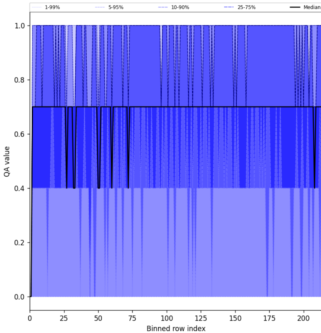
Figure 25: Along track statistics of “QA value” for 2025-04-16 to 2025-04-18
