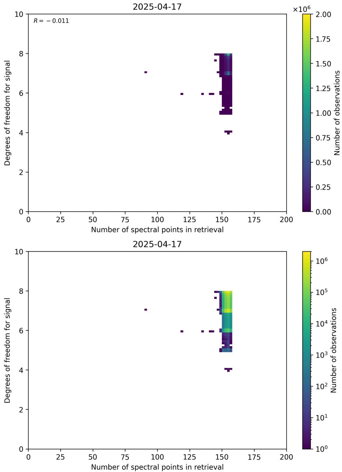
Figure 59: Scatter density plot of “Number of spectral points in retrieval” against “Degrees of freedom for signal” for 2025-04-16 to 2025-04-18.
