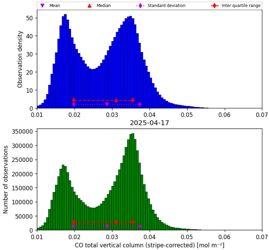
Figure 19: Histogram of “CO total vertical column (stripe-corrected)” for 2025-04-16 to 2025-04-18
