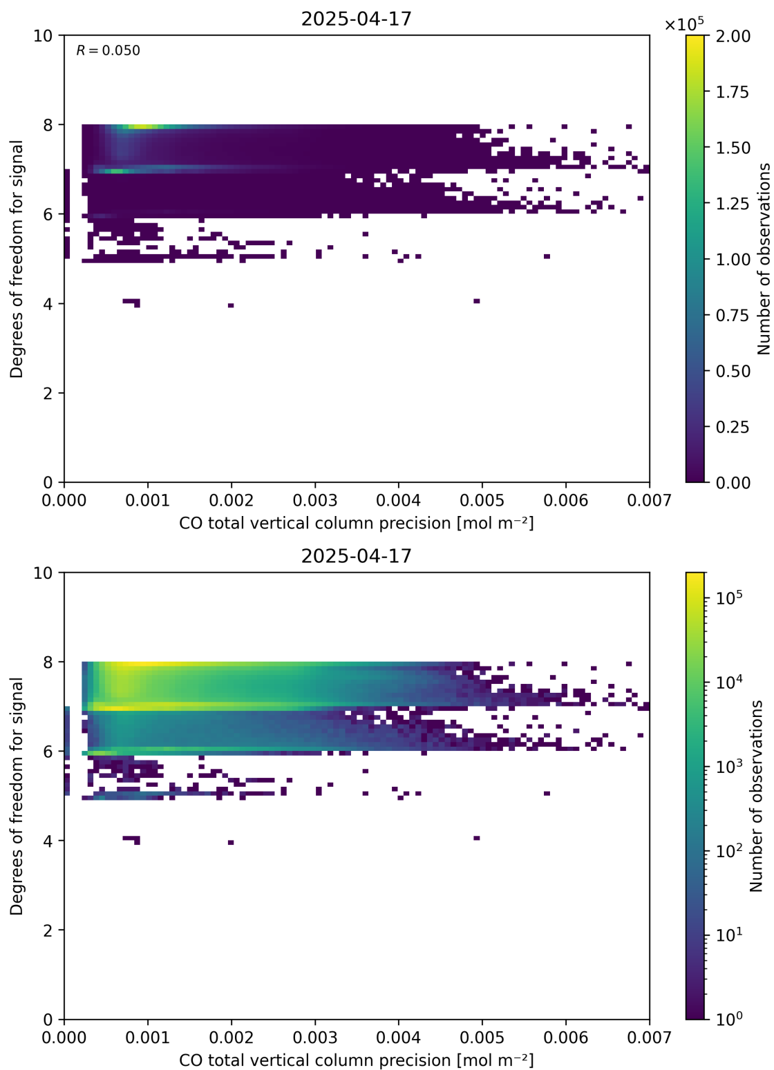
Figure 45: Scatter density plot of “CO total vertical column precision” against “Degrees of freedom for signal” for 2025-04-16 to 2025-04-18.
