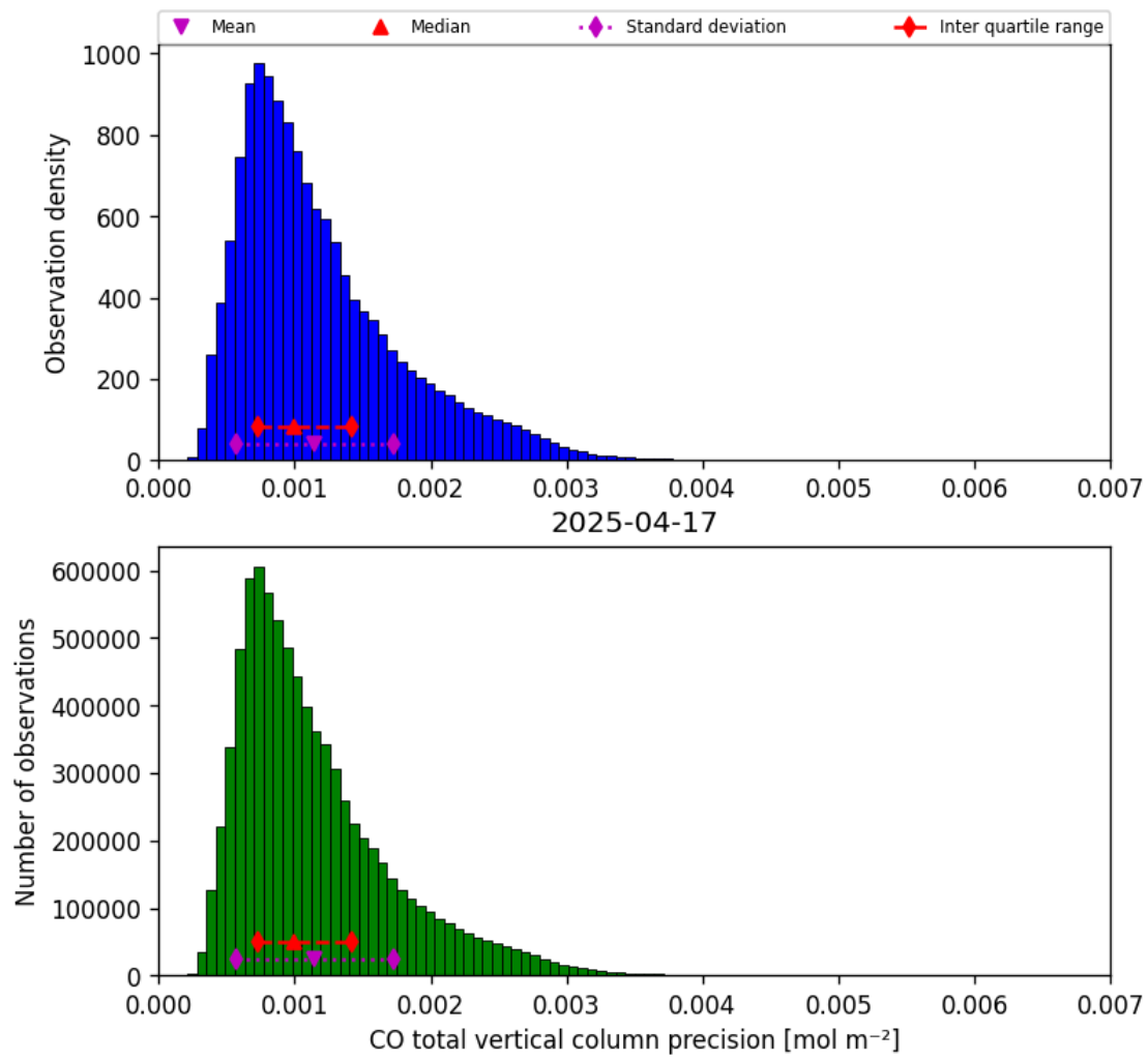
Figure 20: Histogram of “CO total vertical column precision” for 2025-04-16 to 2025-04-18
