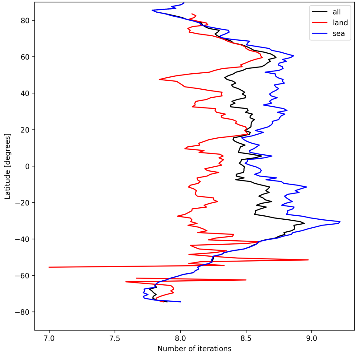
Figure 16: Zonal average of “Number of iterations” for 2025-04-16 to 2025-04-18.
