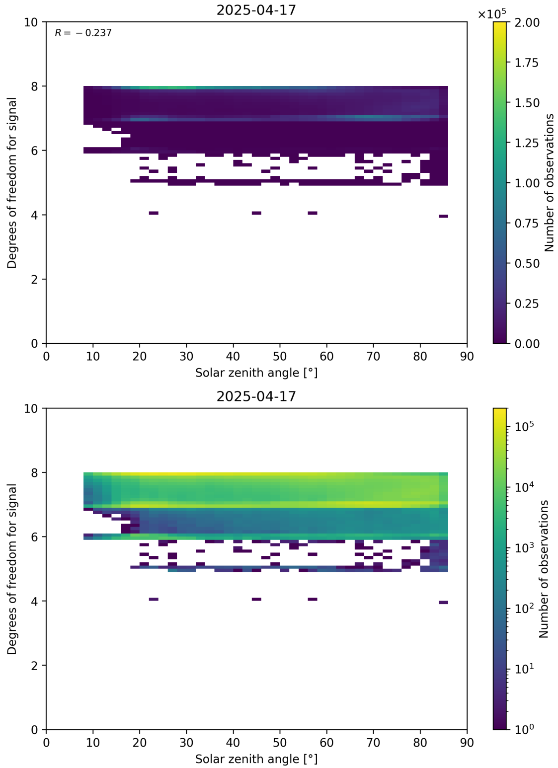
Figure 65: Scatter density plot of “Solar zenith angle” against “Degrees of freedom for signal” for 2025-04-16 to 2025-04-18.
