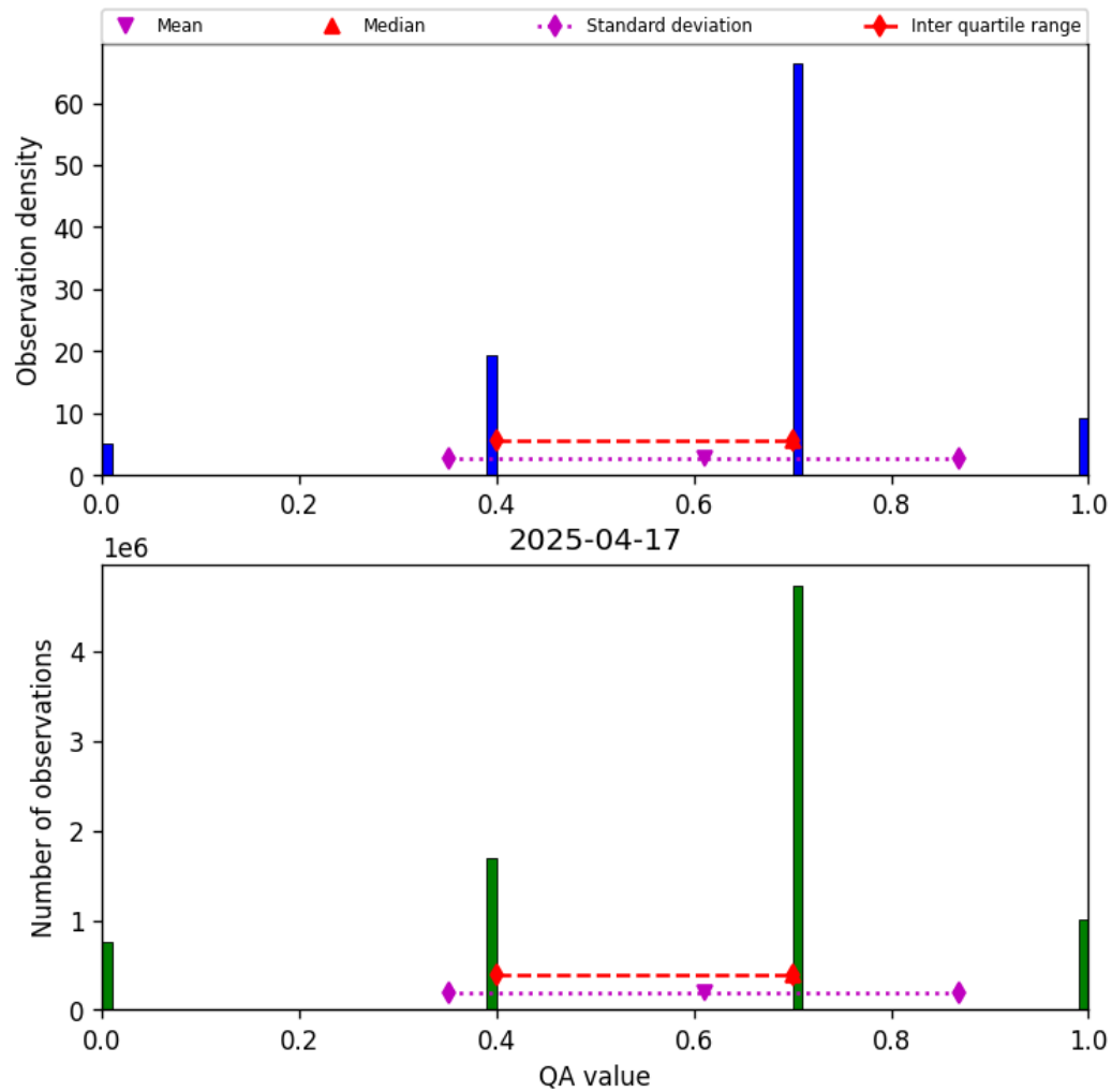
Figure 17: Histogram of “QA value” for 2025-04-16 to 2025-04-18
