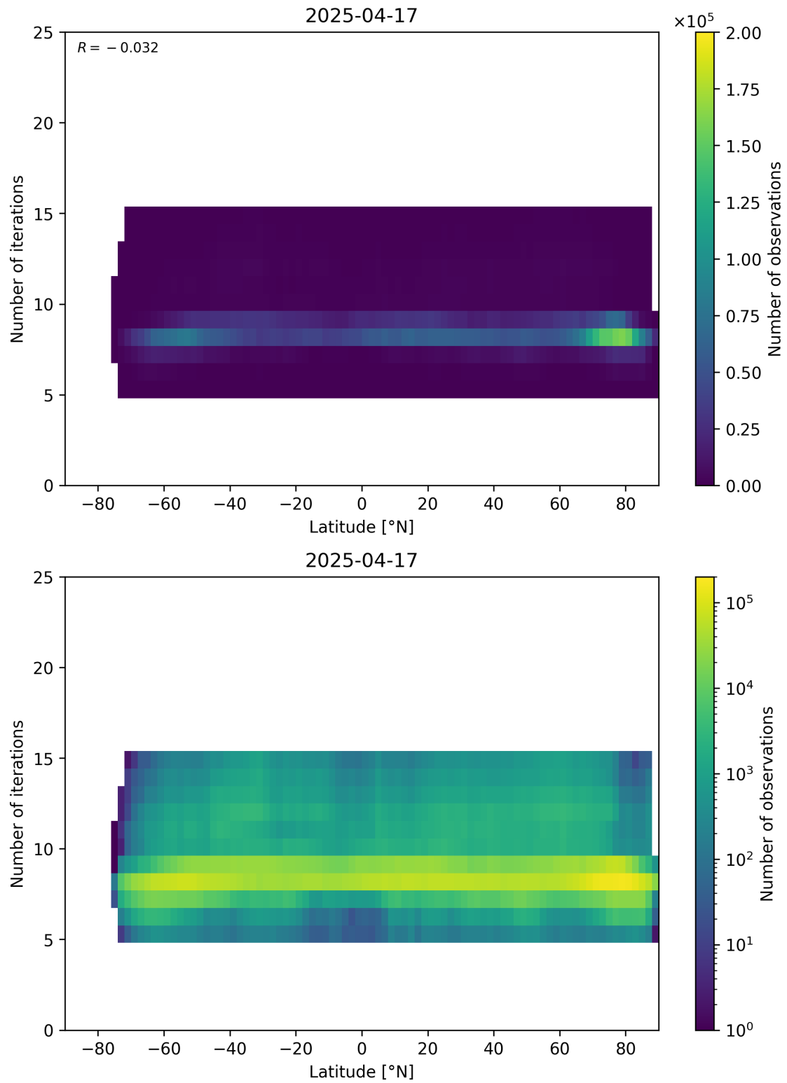
Figure 56: Scatter density plot of “Latitude” against “Number of iterations” for 2025-04-16 to 2025-04-18.
