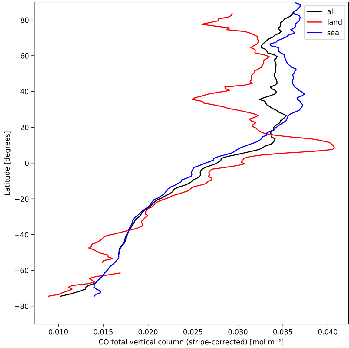
Figure 11: Zonal average of “CO total vertical column (stripe-corrected)” for 2025-04-16 to 2025-04-18.
