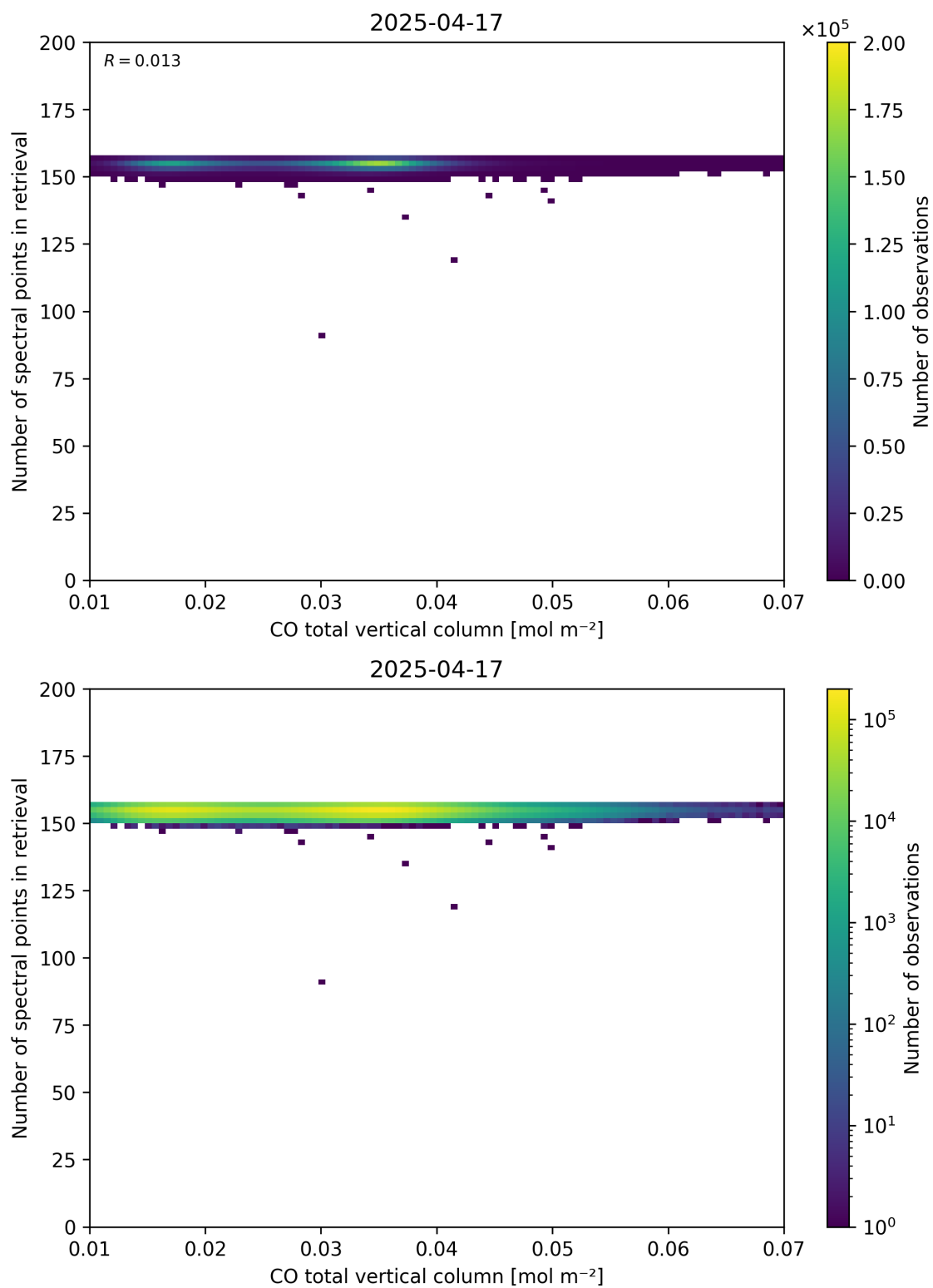
Figure 43: Scatter density plot of “CO total vertical column” against “Number of spectral points in retrieval” for 2025-04-16 to 2025-04-18.
