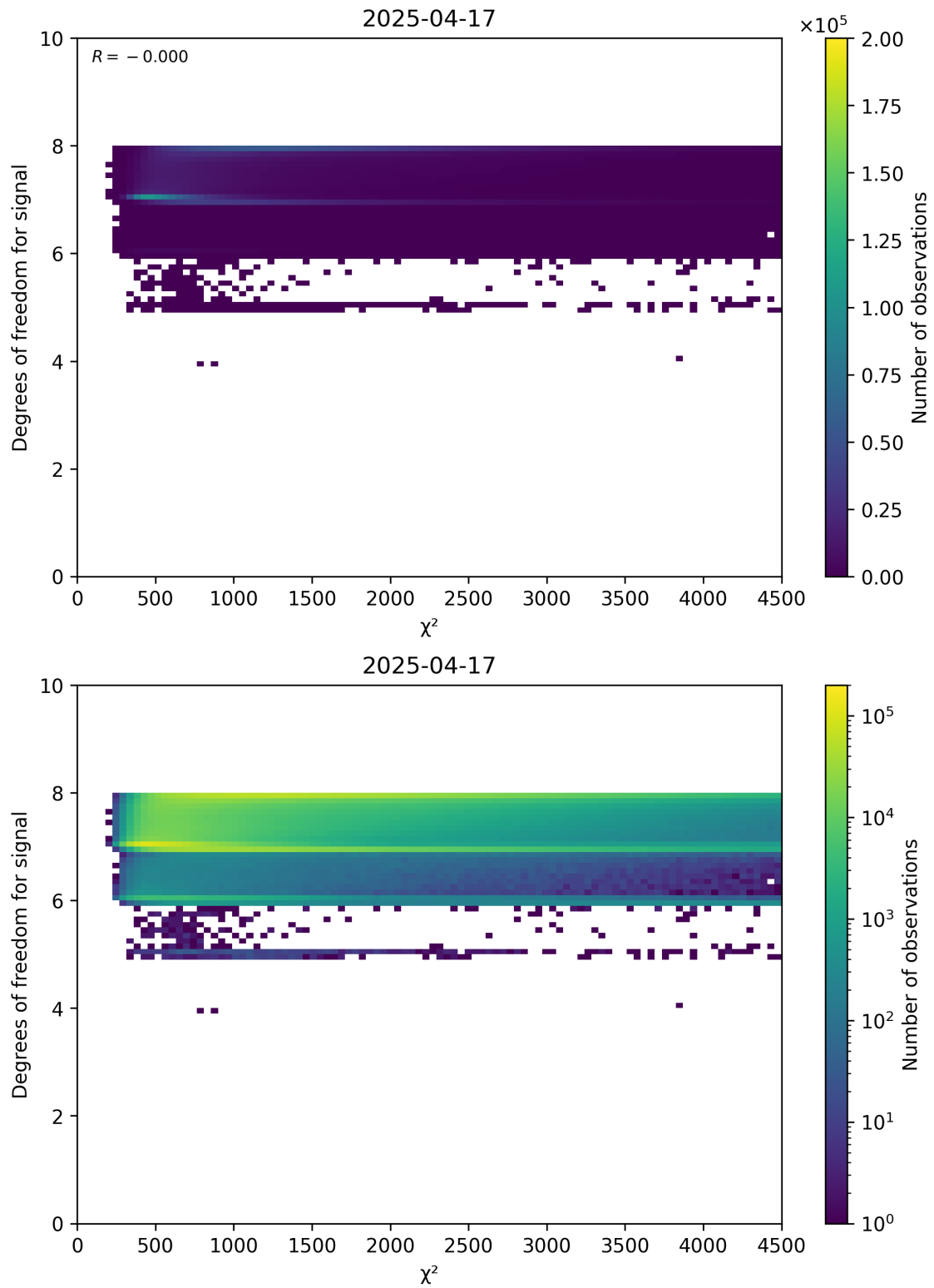
Figure 48: Scatter density plot of “ \chi^2 ” against “Degrees of freedom for signal” for 2025-04-16 to 2025-04-18.
