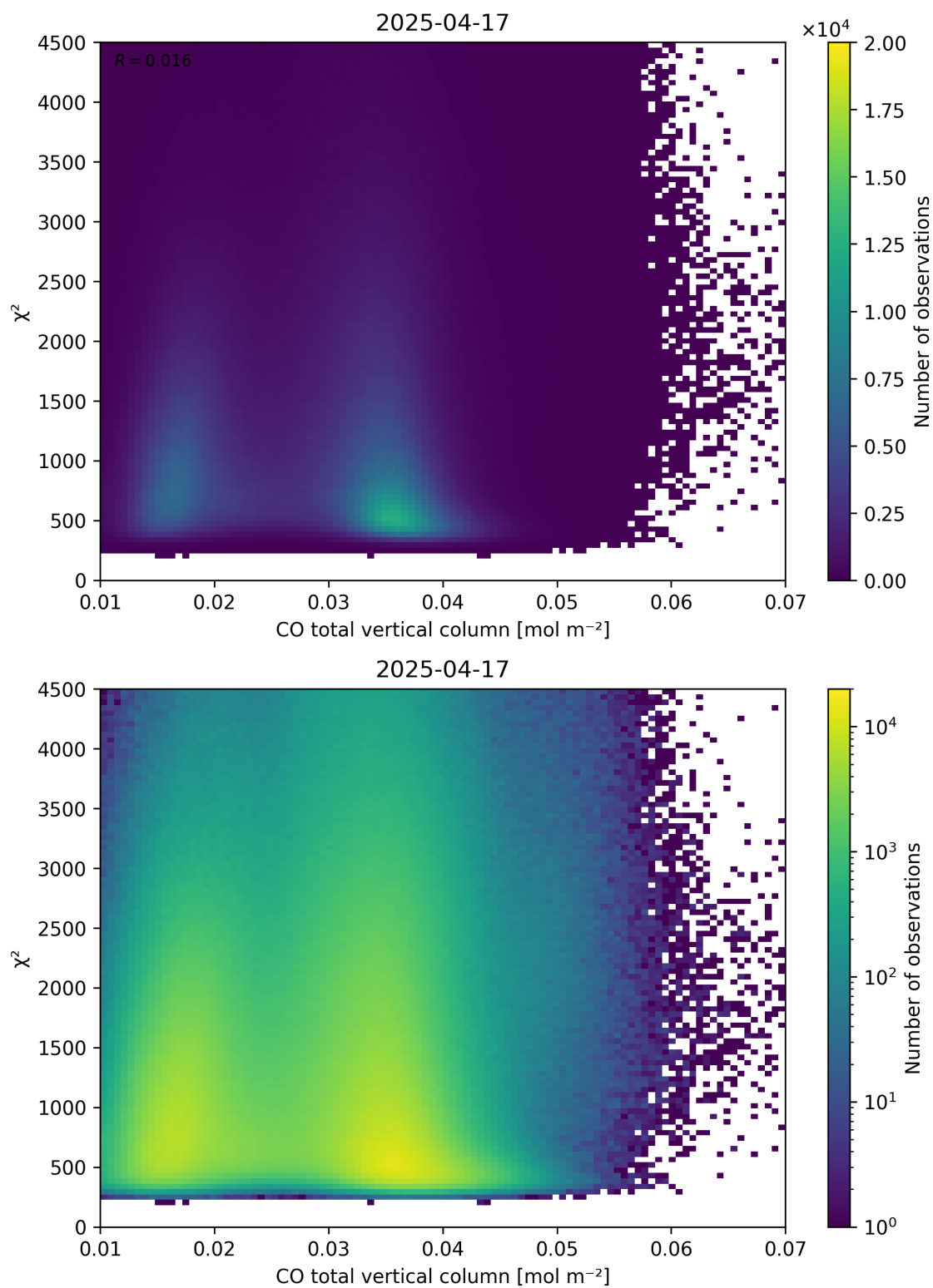
Figure 35: Scatter density plot of “CO total vertical column” against “ \chi^2 ” for 2025-04-16 to 2025-04-18.
