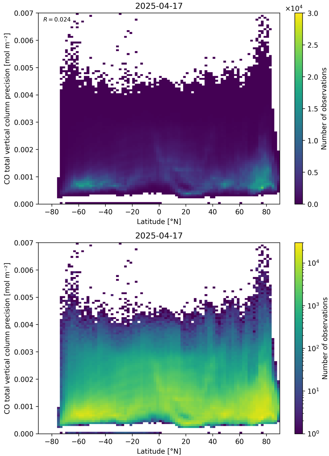
Figure 53: Scatter density plot of “Latitude” against “CO total vertical column precision” for 2025-04-16 to 2025-04-18.
