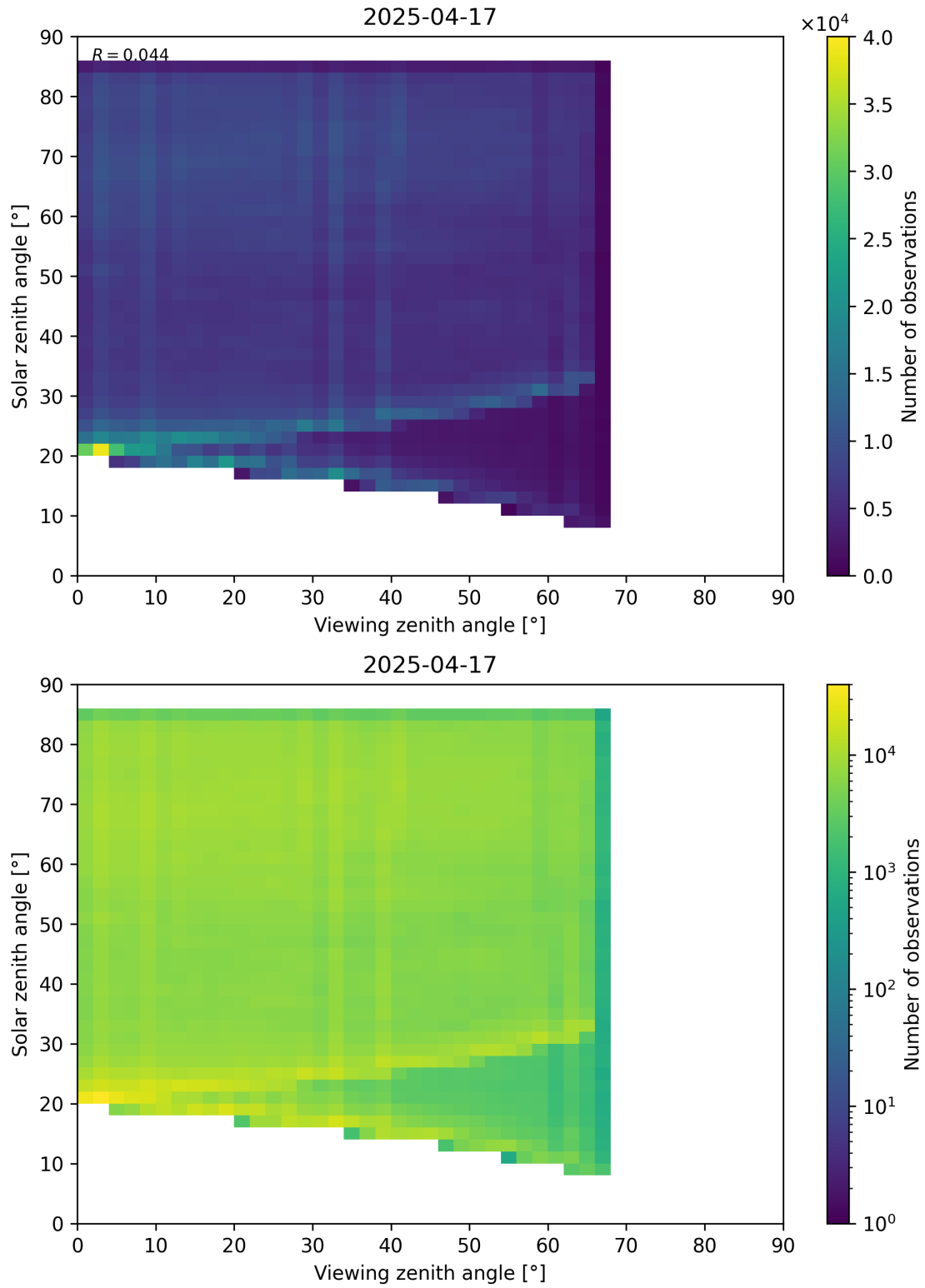
Figure 77: Scatter density plot of “Viewing zenith angle” against “Solar zenith angle” for 2025-04-16 to 2025-04-18.
