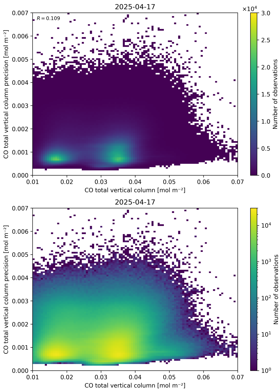
Figure 34: Scatter density plot of “CO total vertical column” against “CO total vertical column precision” for 2025-04-16 to 2025-04-18.
