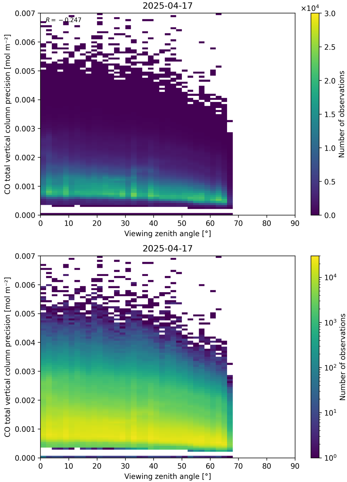
Figure 71: Scatter density plot of “Viewing zenith angle” against “CO total vertical column precision” for 2025-04-16 to 2025-04-18.
