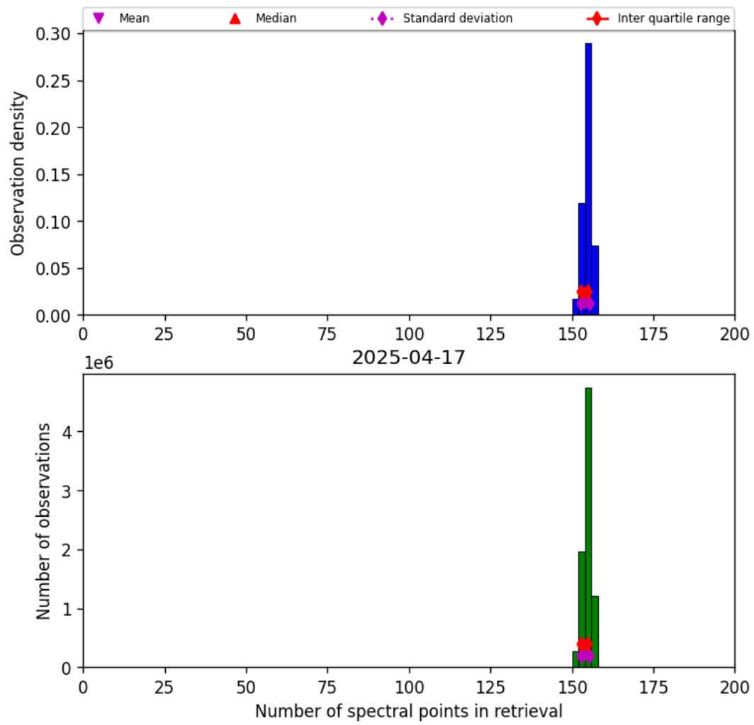
Figure 21: Histogram of “Number of spectral points in retrieval” for 2025-04-16 to 2025-04-18
