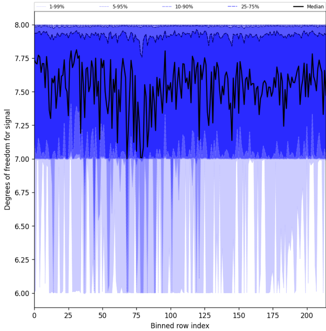
Figure 31: Along track statistics of “Degrees of freedom for signal” for 2025-04-16 to 2025-04-18
