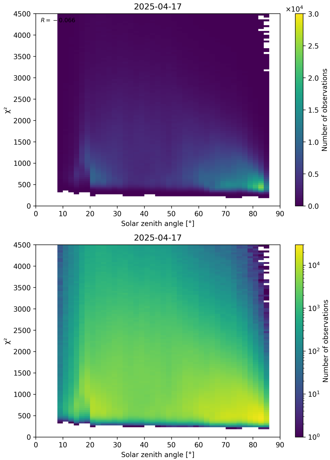
Figure 64: Scatter density plot of “Solar zenith angle” against “ \chi^2 ” for 2025-04-16 to 2025-04-18.
