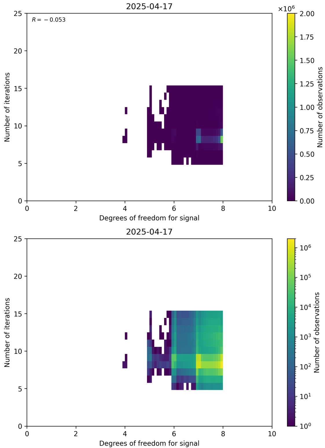
Figure 50: Scatter density plot of “Degrees of freedom for signal” against “Number of iterations” for 2025-04-16 to 2025-04-18.
