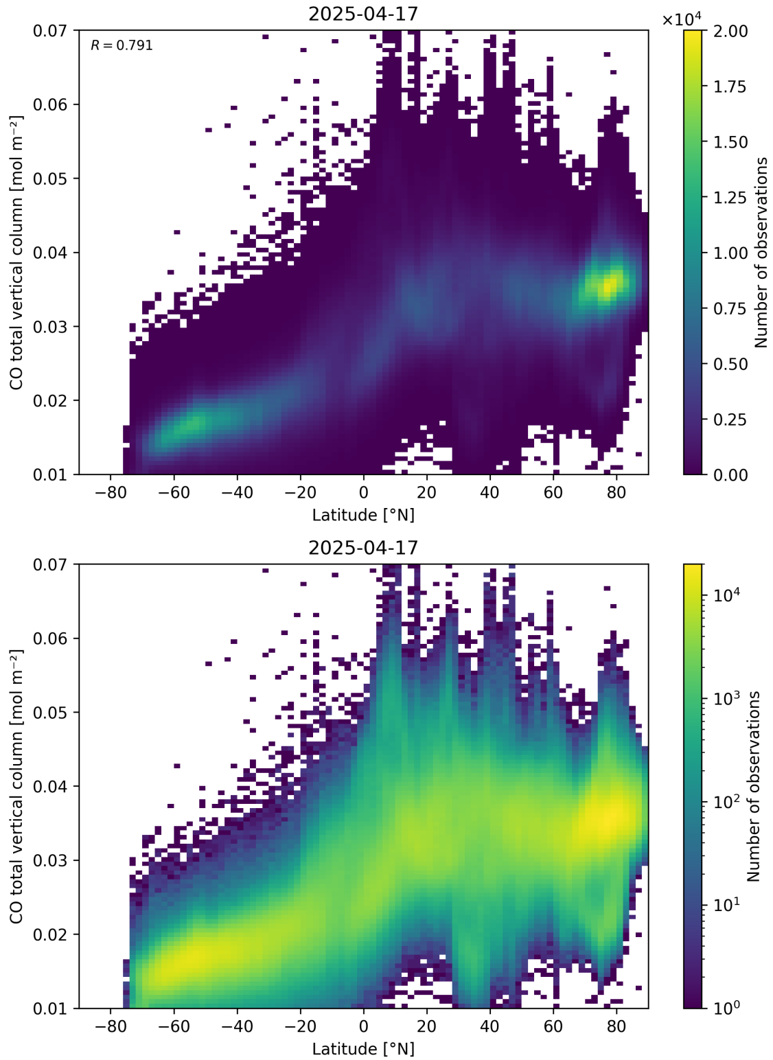
Figure 51: Scatter density plot of “Latitude” against “CO total vertical column” for 2025-04-16 to 2025-04-18.
