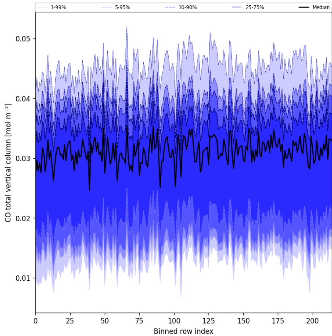
Figure 26: Along track statistics of “CO total vertical column” for 2025-04-16 to 2025-04-18
