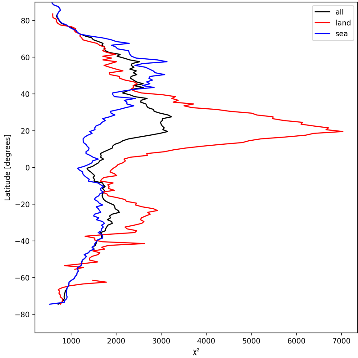
Figure 14: Zonal average of “ \chi^2 ” for 2025-04-16 to 2025-04-18.
