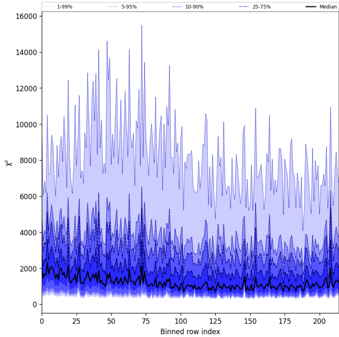
Figure 30: Along track statistics of “ \chi^2 ” for 2025-04-16 to 2025-04-18
