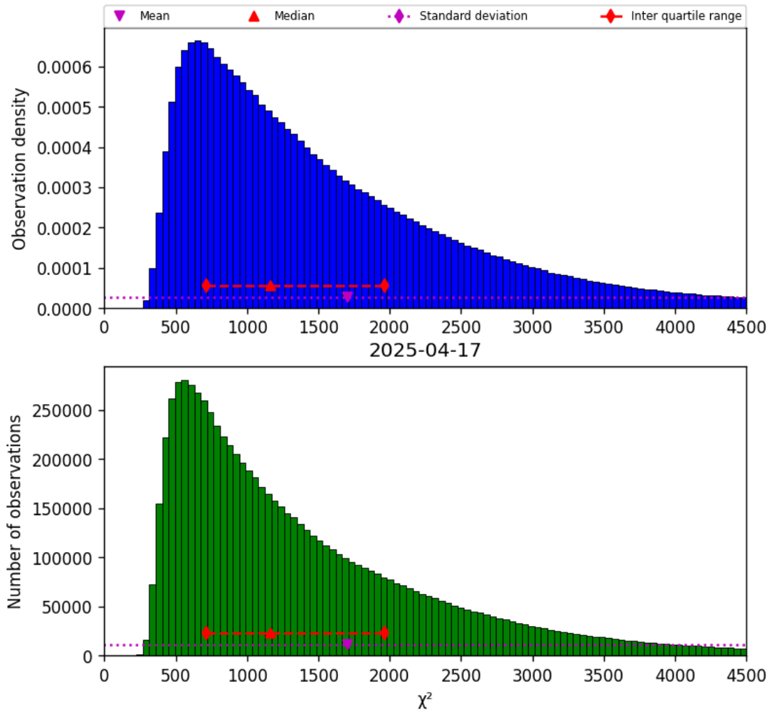
Figure 22: Histogram of “ \chi^2 ” for 2025-04-16 to 2025-04-18
