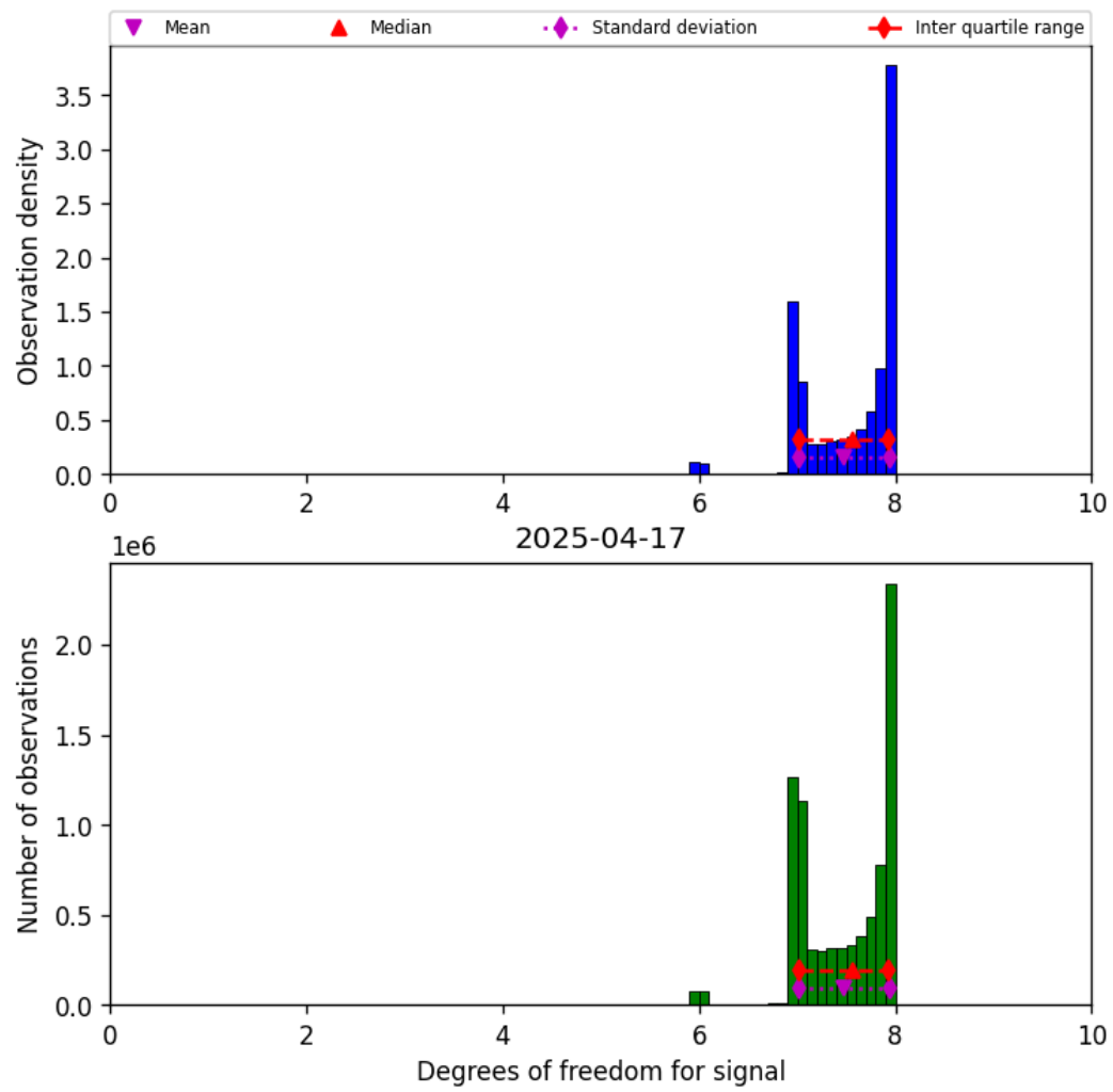
Figure 23: Histogram of “Degrees of freedom for signal” for 2025-04-16 to 2025-04-18
