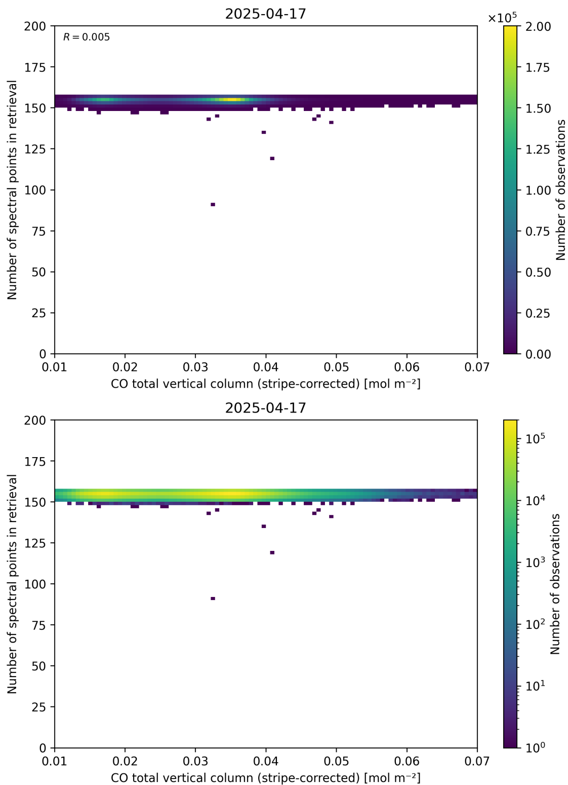
Figure 40: Scatter density plot of “CO total vertical column (stripe-corrected)” against “Number of spectral points in retrieval” for 2025-04-16 to 2025-04-18.
