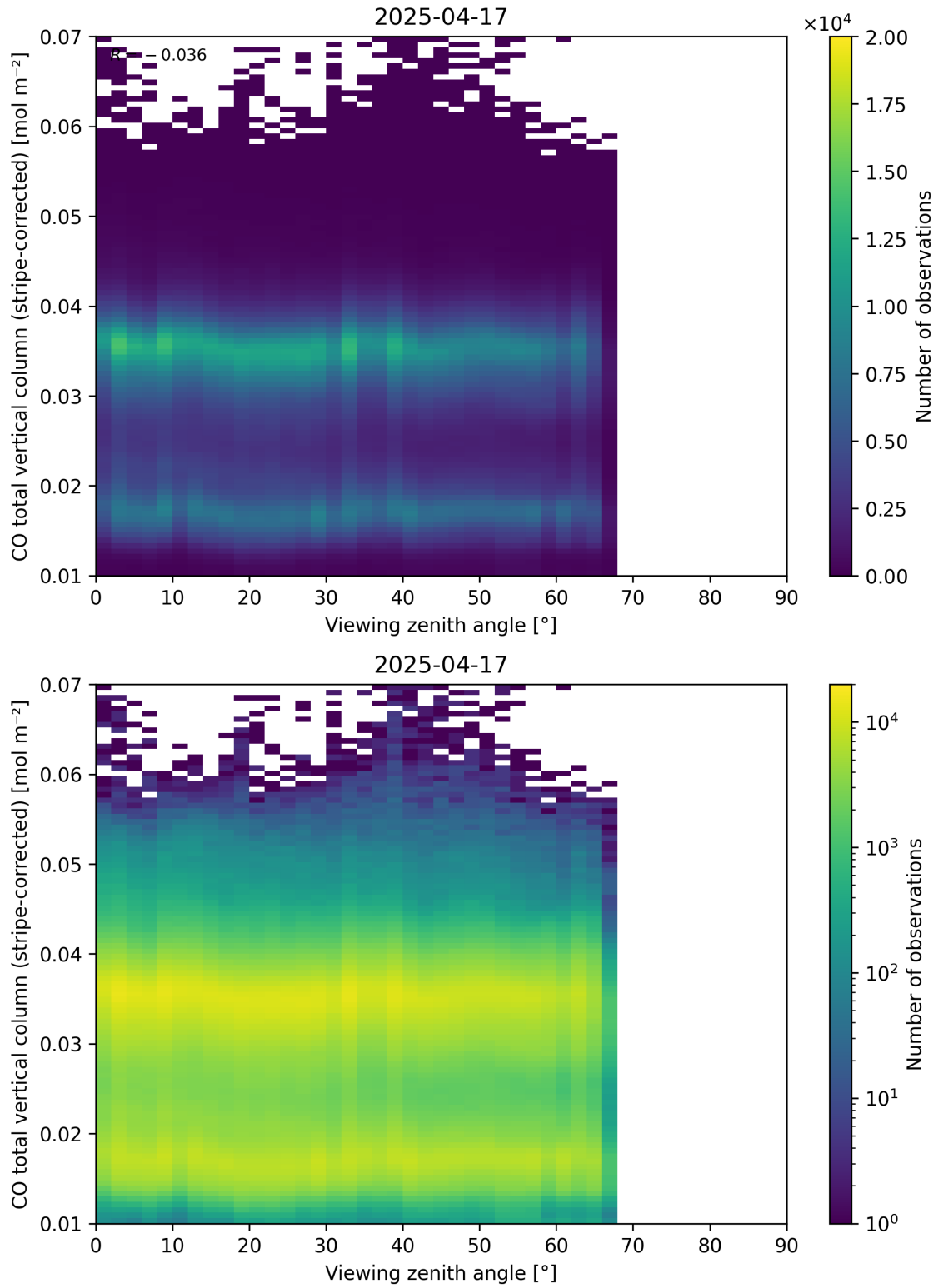
Figure 70: Scatter density plot of “Viewing zenith angle” against “CO total vertical column (stripe-corrected)” for 2025-04-16 to 2025-04-18.
