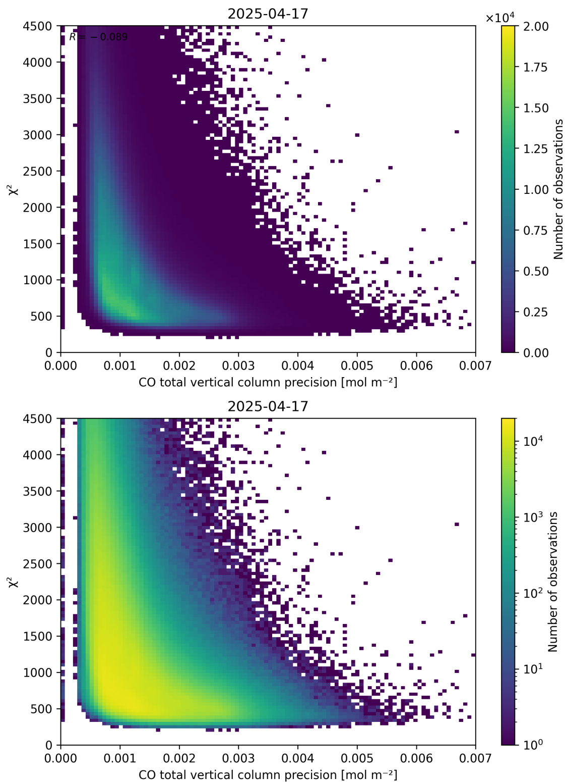
Figure 44: Scatter density plot of “CO total vertical column precision” against “ \chi^2 ” for 2025-04-16 to 2025-04-18.
