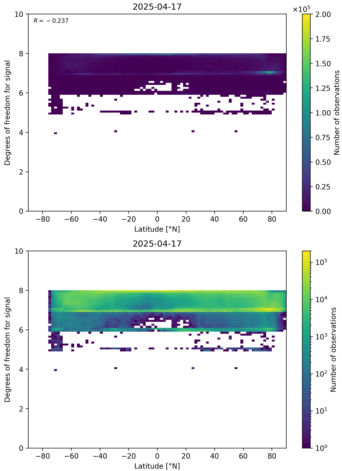
Figure 55: Scatter density plot of “Latitude” against “Degrees of freedom for signal” for 2025-04-16 to 2025-04-18.
