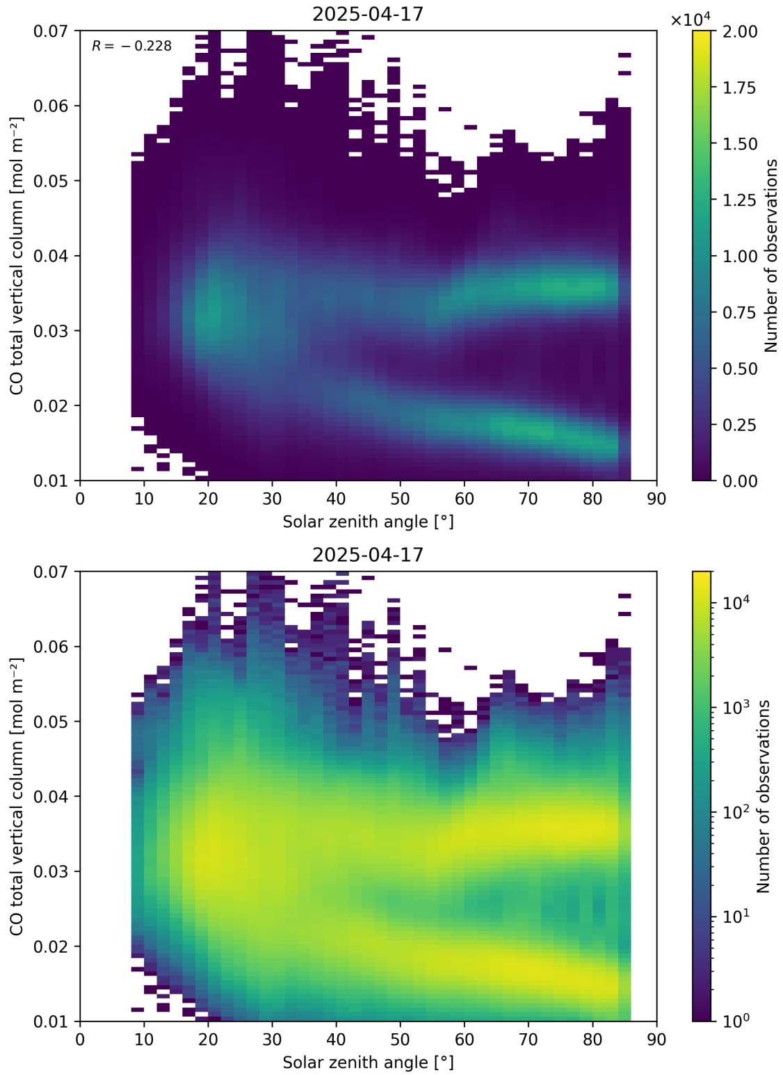
Figure 61: Scatter density plot of “Solar zenith angle” against “CO total vertical column” for 2025-04-16 to 2025-04-18.
