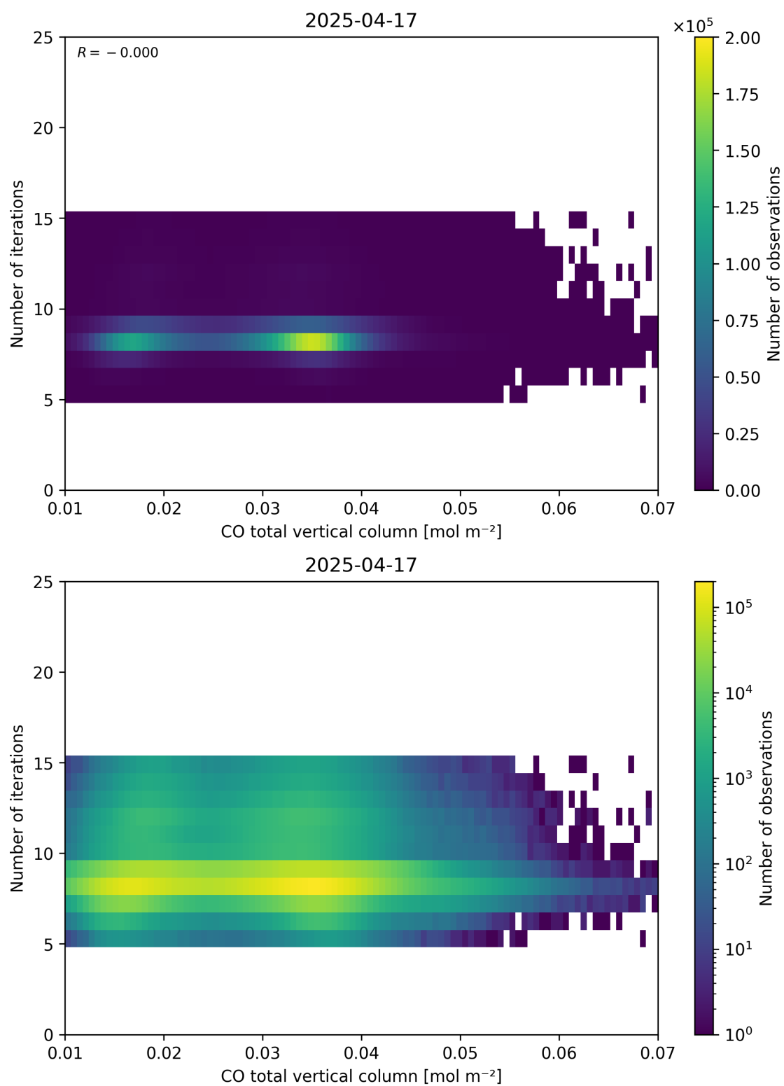
Figure 42: Scatter density plot of “CO total vertical column” against “Number of iterations” for 2025-04-16 to 2025-04-18.
