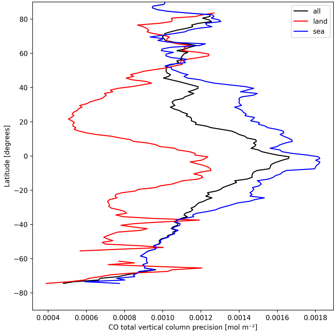
Figure 12: Zonal average of “CO total vertical column precision” for 2025-04-16 to 2025-04-18.
