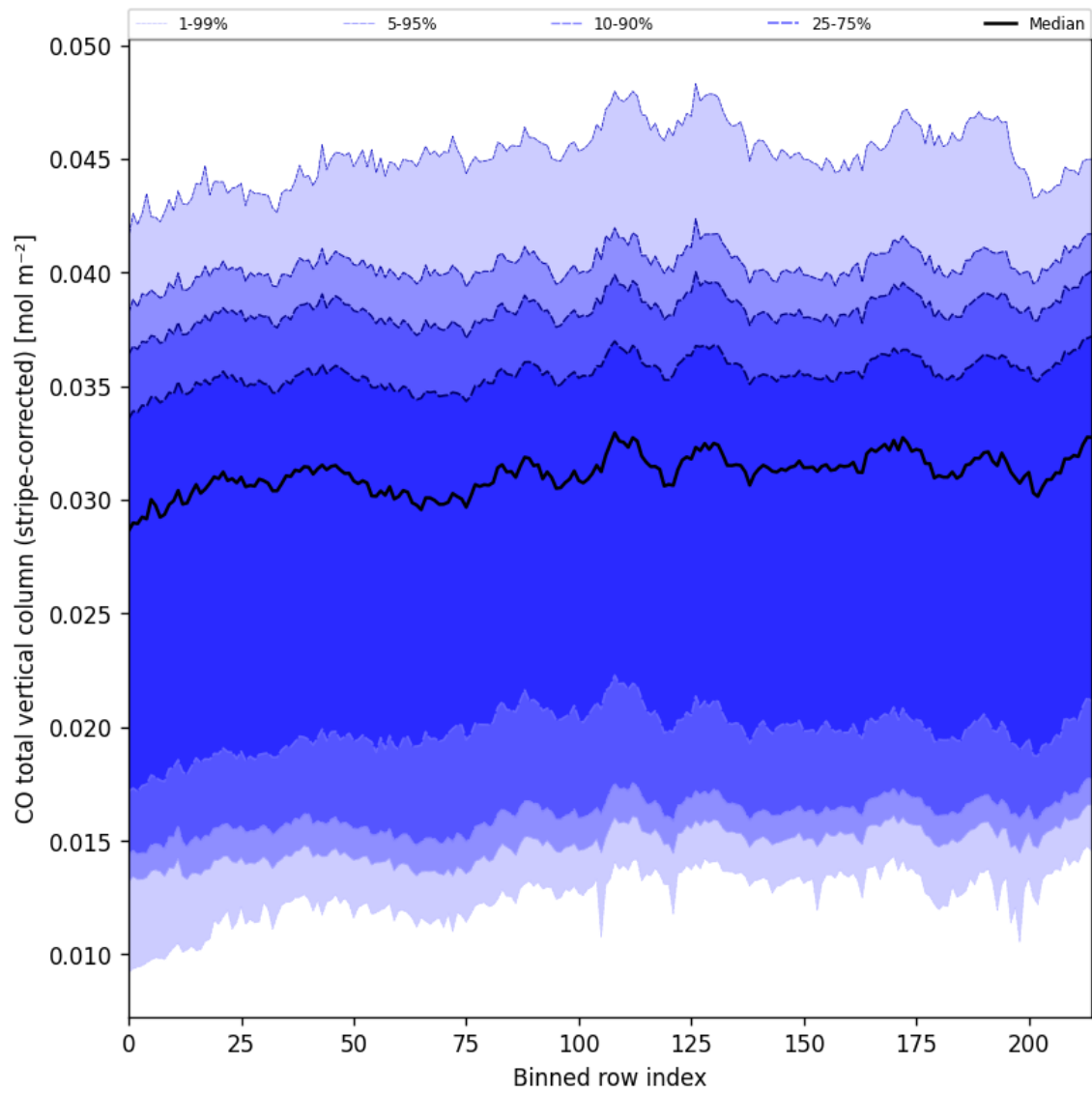
Figure 27: Along track statistics of “CO total vertical column (stripe-corrected)” for 2025-04-16 to 2025-04-18
