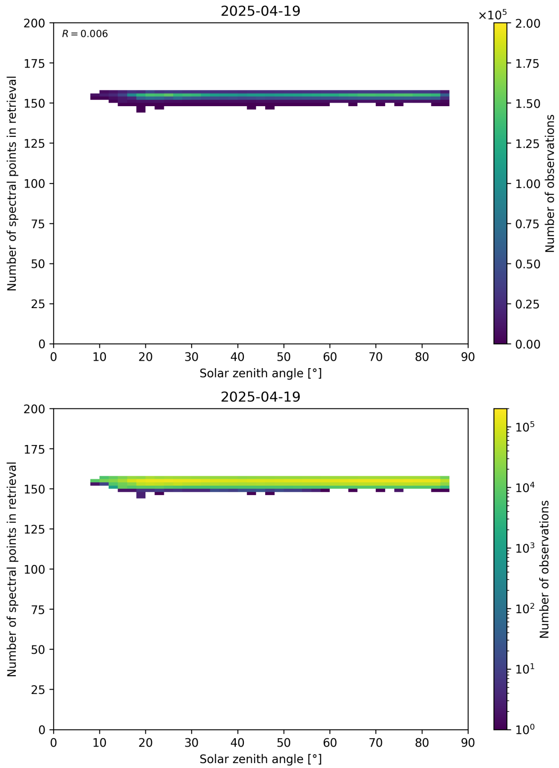
Figure 68: Scatter density plot of “Solar zenith angle” against “Number of spectral points in retrieval” for 2025-04-19 to 2025-04-20.
