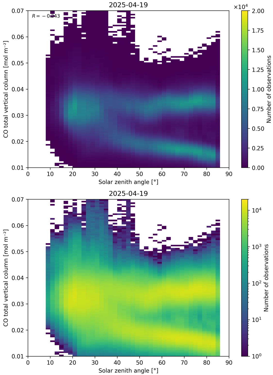
Figure 61: Scatter density plot of “Solar zenith angle” against “CO total vertical column” for 2025-04-19 to 2025-04-20.
