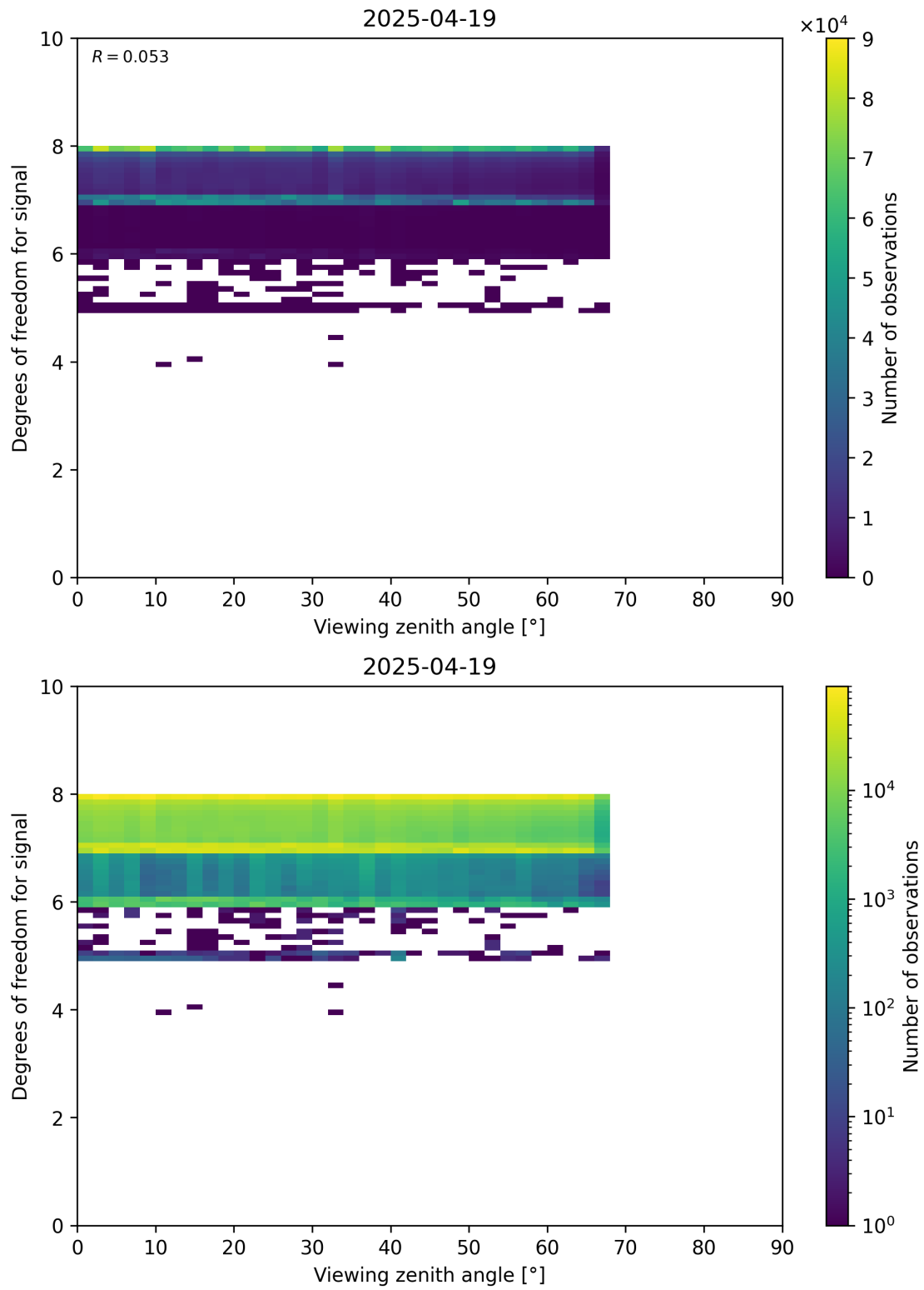
Figure 73: Scatter density plot of “Viewing zenith angle” against “Degrees of freedom for signal” for 2025-04-19 to 2025-04-20.
