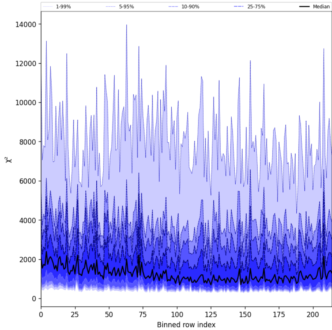
Figure 30: Along track statistics of “ \chi^2 ” for 2025-04-19 to 2025-04-20
