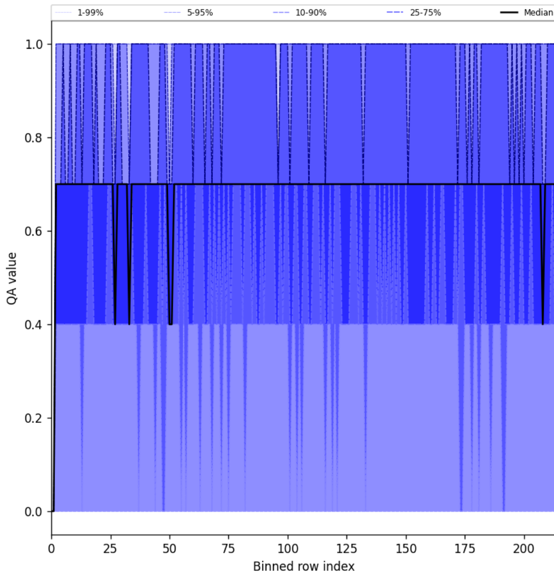
Figure 25: Along track statistics of “QA value” for 2025-04-19 to 2025-04-20
