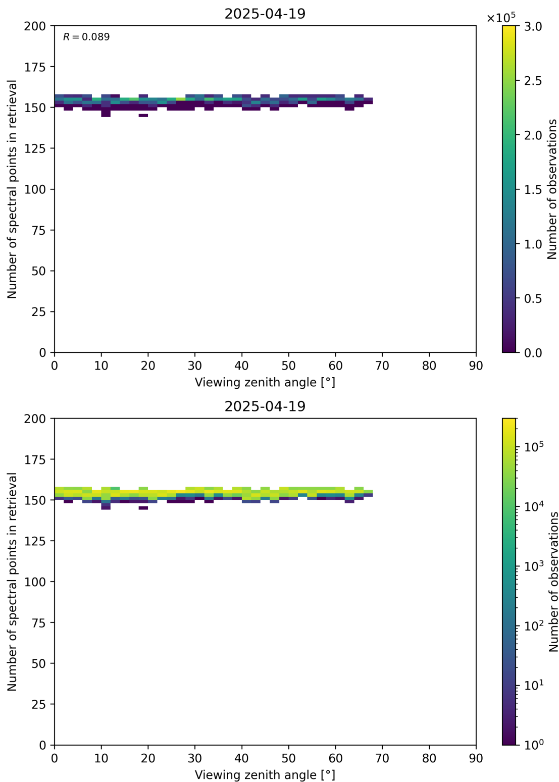
Figure 76: Scatter density plot of “Viewing zenith angle” against “Number of spectral points in retrieval” for 2025-04-19 to 2025-04-20.
