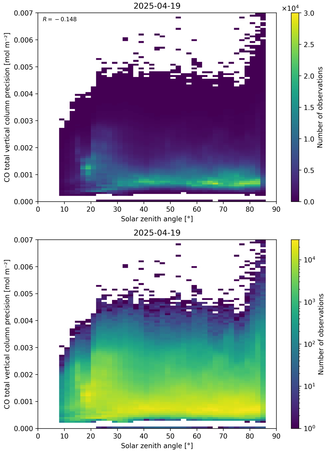
Figure 63: Scatter density plot of “Solar zenith angle” against “CO total vertical column precision” for 2025-04-19 to 2025-04-20.
