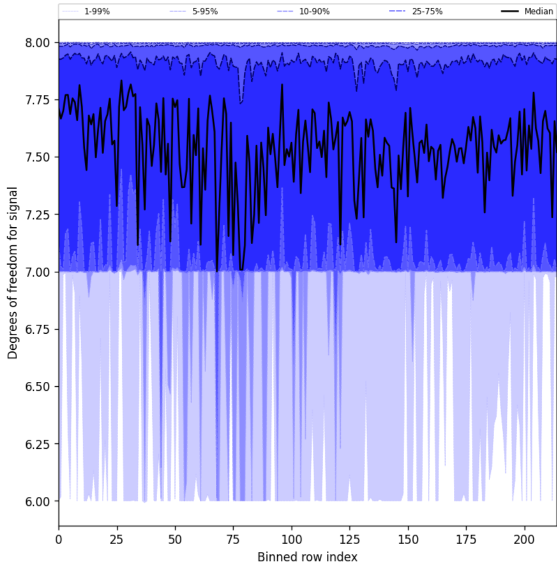
Figure 31: Along track statistics of “Degrees of freedom for signal” for 2025-04-19 to 2025-04-20
