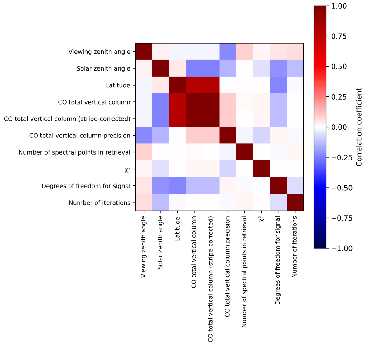
Figure 2: Map of correlation matrix for 2025-04-19 to 2025-04-20.
