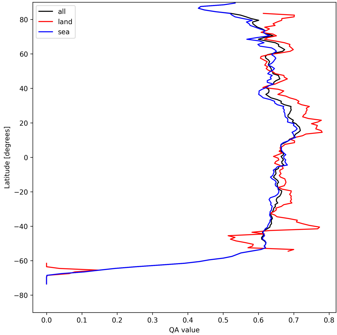
Figure 9: Zonal average of “QA value” for 2025-04-19 to 2025-04-20.
