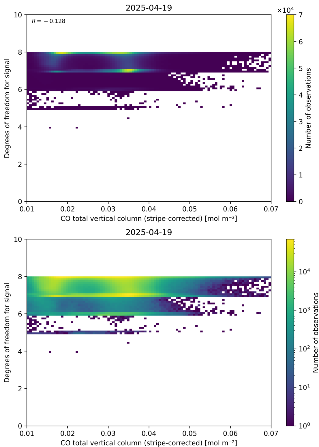
Figure 38: Scatter density plot of “CO total vertical column (stripe-corrected)” against “Degrees of freedom for signal” for 2025-04-19 to 2025-04-20.
