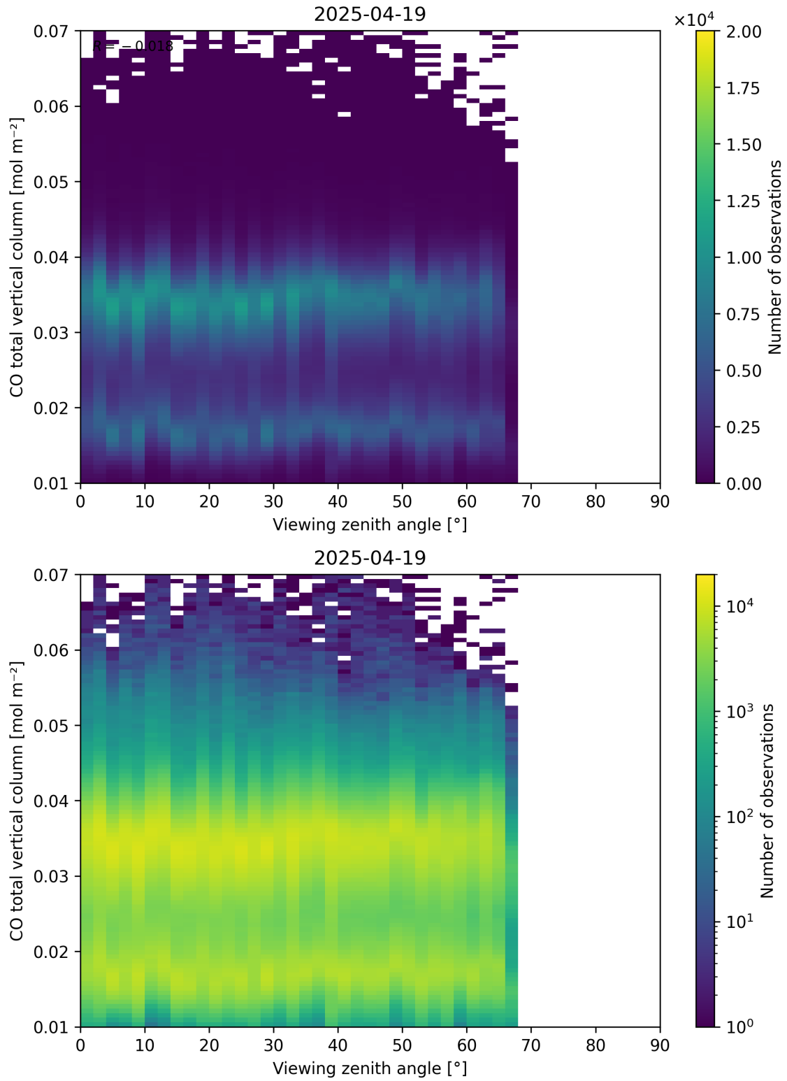
Figure 69: Scatter density plot of “Viewing zenith angle” against “CO total vertical column” for 2025-04-19 to 2025-04-20.
