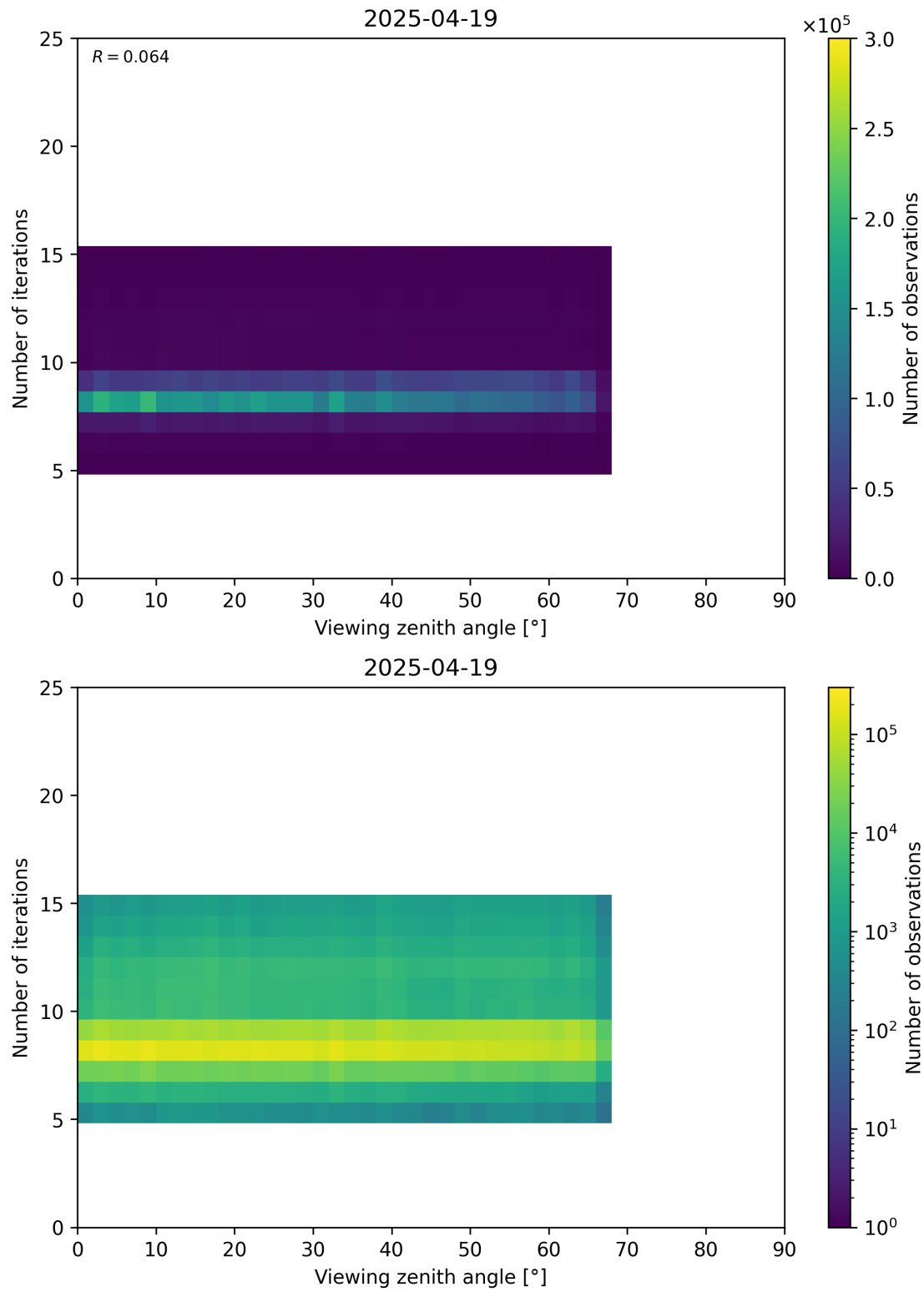
Figure 75: Scatter density plot of “Viewing zenith angle” against “Number of iterations” for 2025-04-19 to 2025-04-20.
