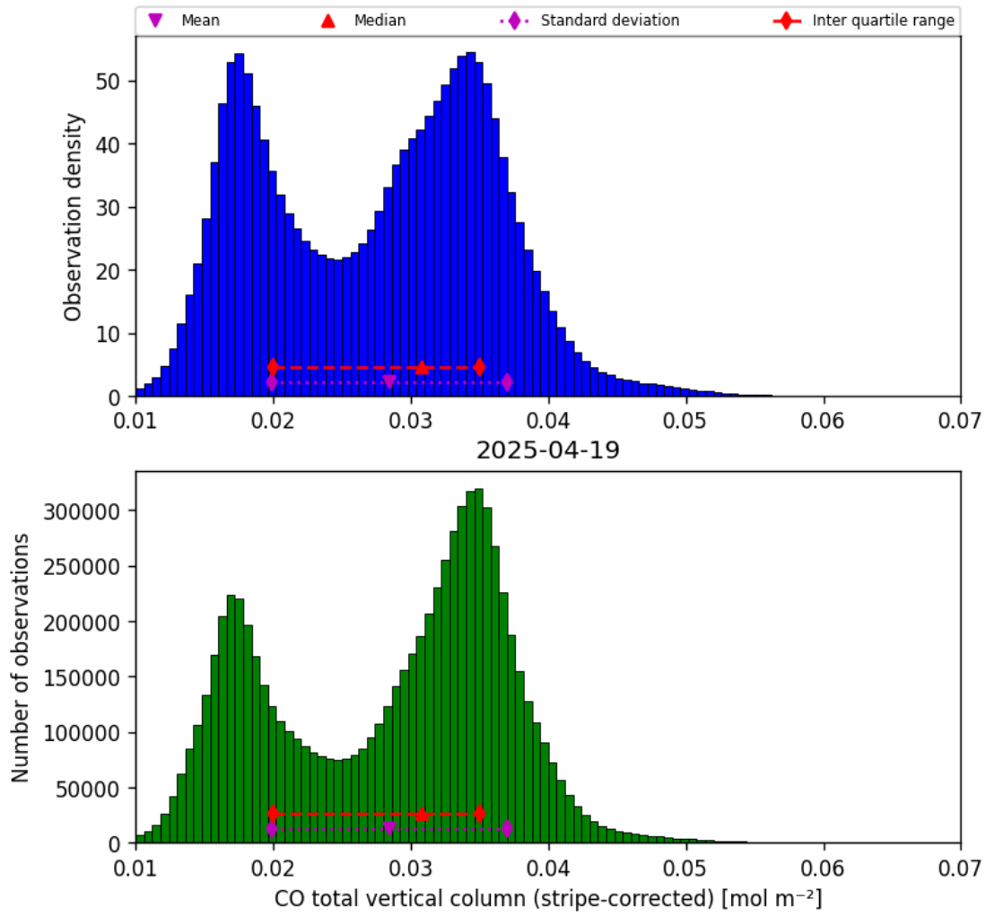
Figure 19: Histogram of “CO total vertical column (stripe-corrected)” for 2025-04-19 to 2025-04-20
