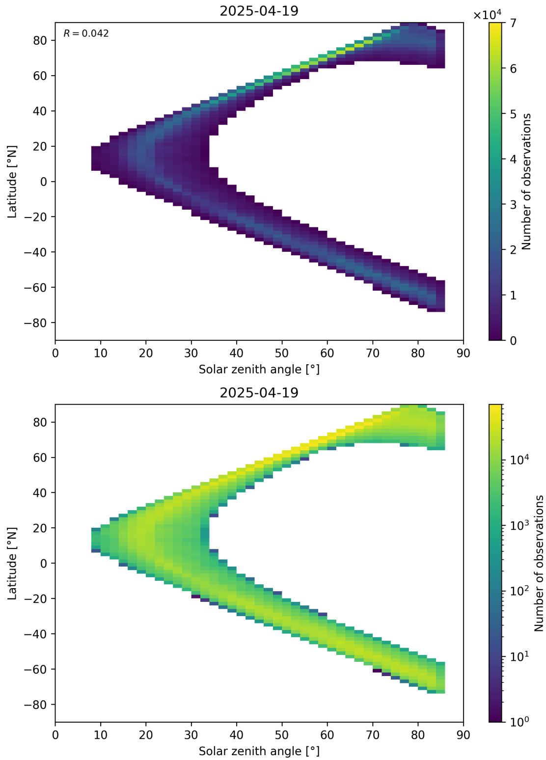
Figure 66: Scatter density plot of “Solar zenith angle” against “Latitude” for 2025-04-19 to 2025-04-20.
