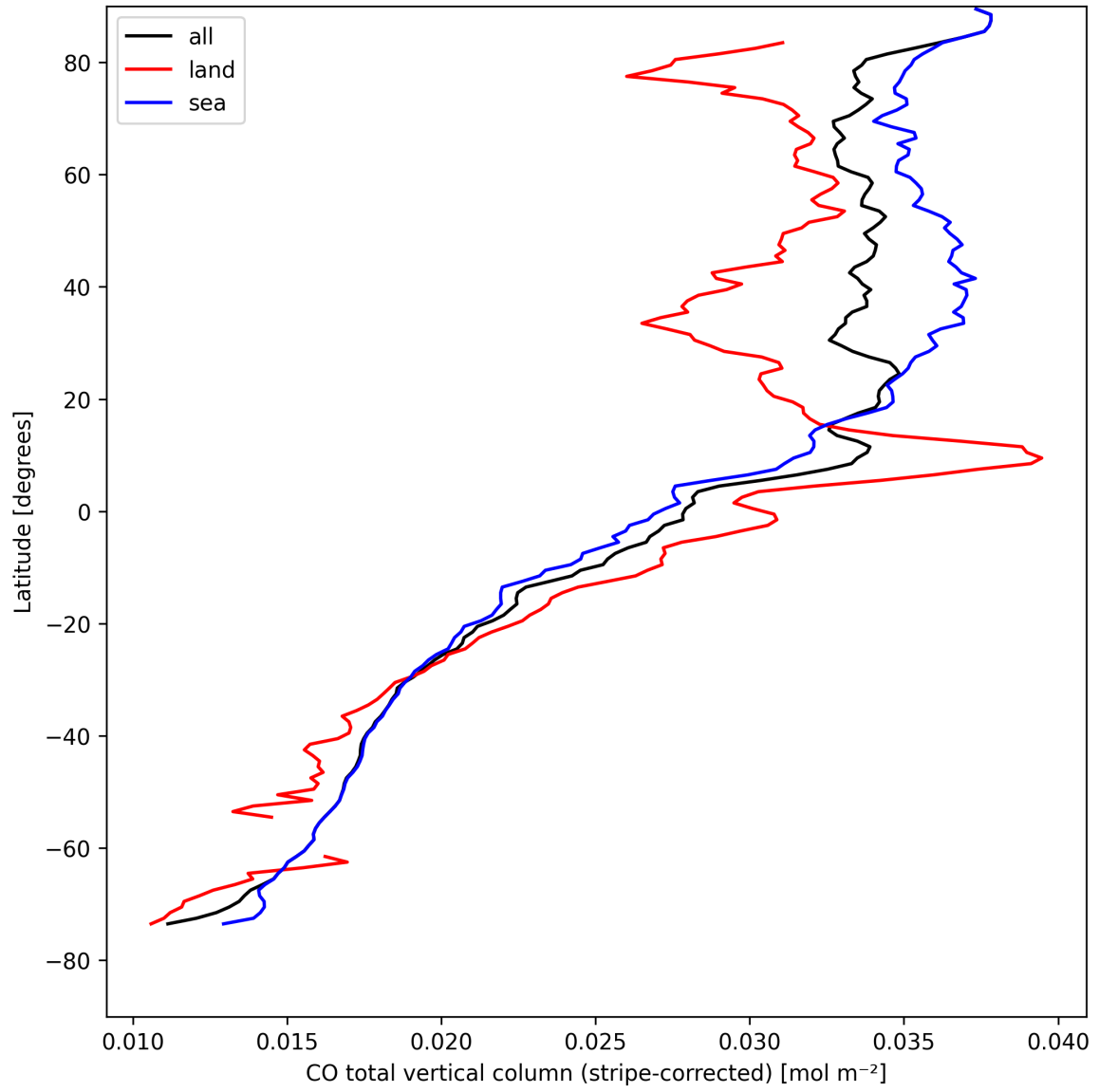
Figure 11: Zonal average of “CO total vertical column (stripe-corrected)” for 2025-04-19 to 2025-04-20.
