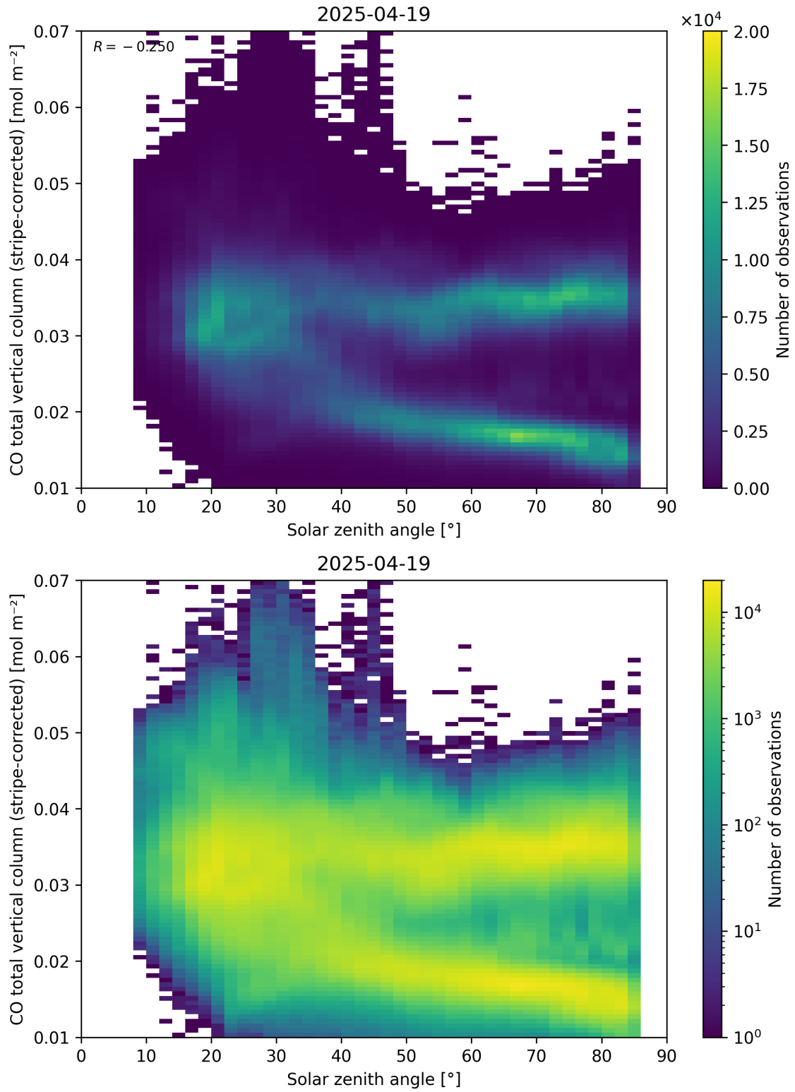
Figure 62: Scatter density plot of “Solar zenith angle” against “CO total vertical column (stripe-corrected)” for 2025-04-19 to 2025-04-20.
