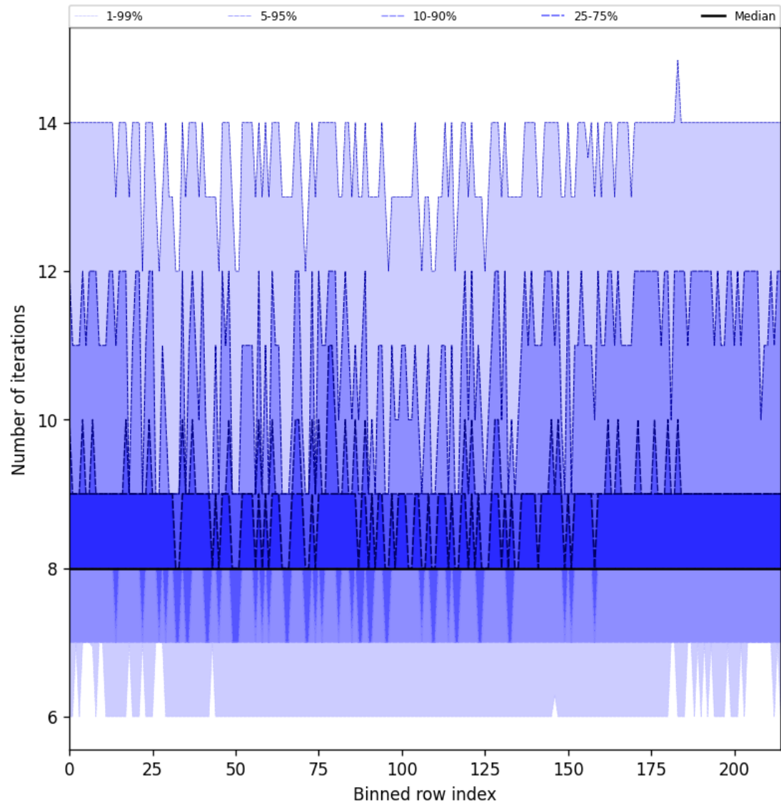
Figure 32: Along track statistics of “Number of iterations” for 2025-04-19 to 2025-04-20
