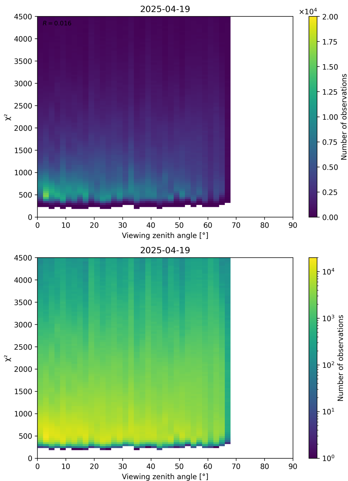
Figure 72: Scatter density plot of “Viewing zenith angle” against “ \chi^2 ” for 2025-04-19 to 2025-04-20.
