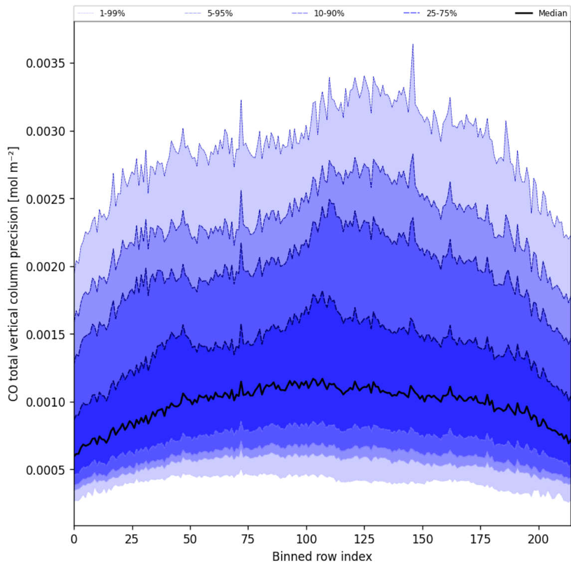
Figure 28: Along track statistics of “CO total vertical column precision” for 2025-04-19 to 2025-04-20
