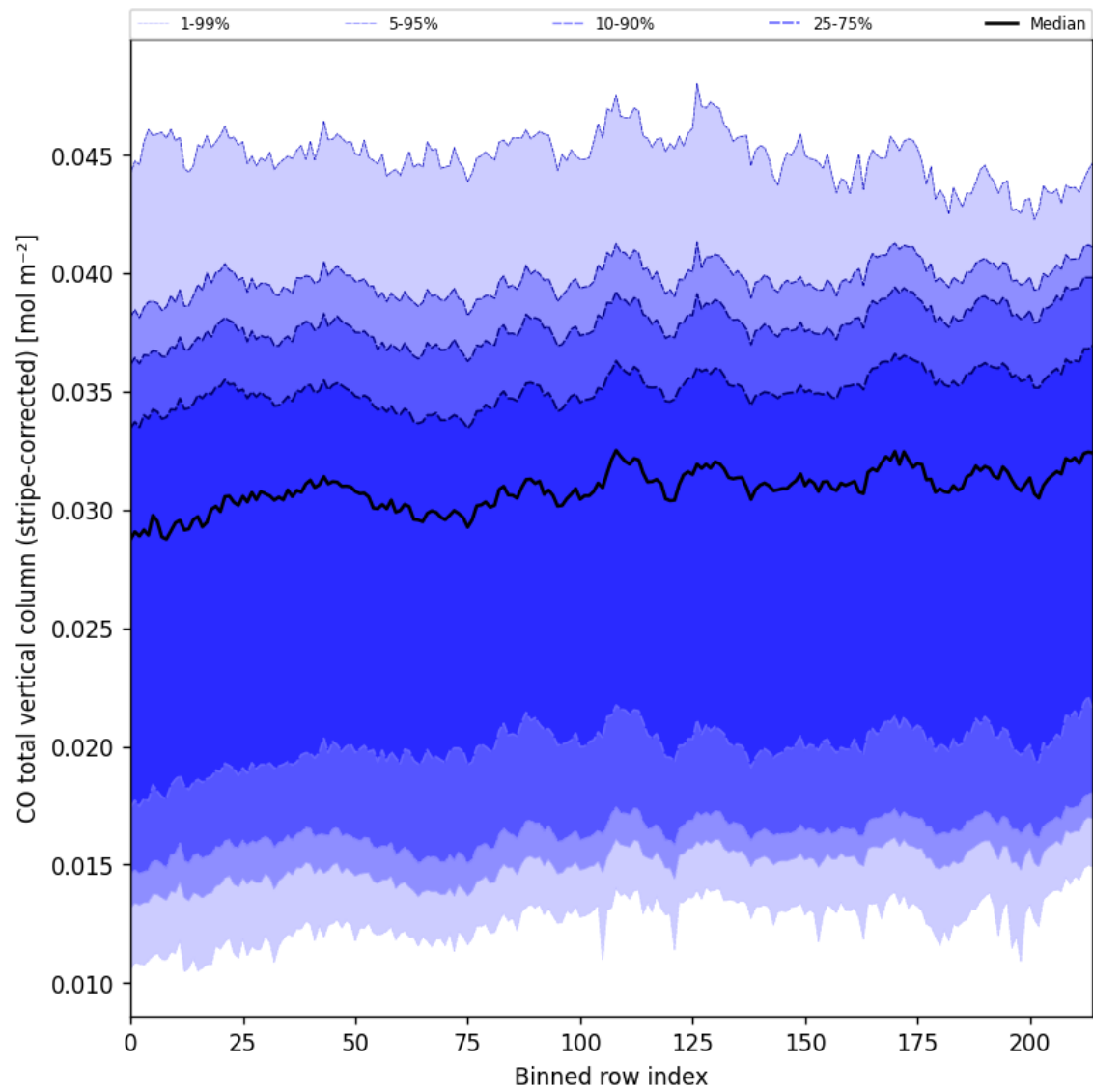
Figure 27: Along track statistics of “CO total vertical column (stripe-corrected)” for 2025-04-19 to 2025-04-20
