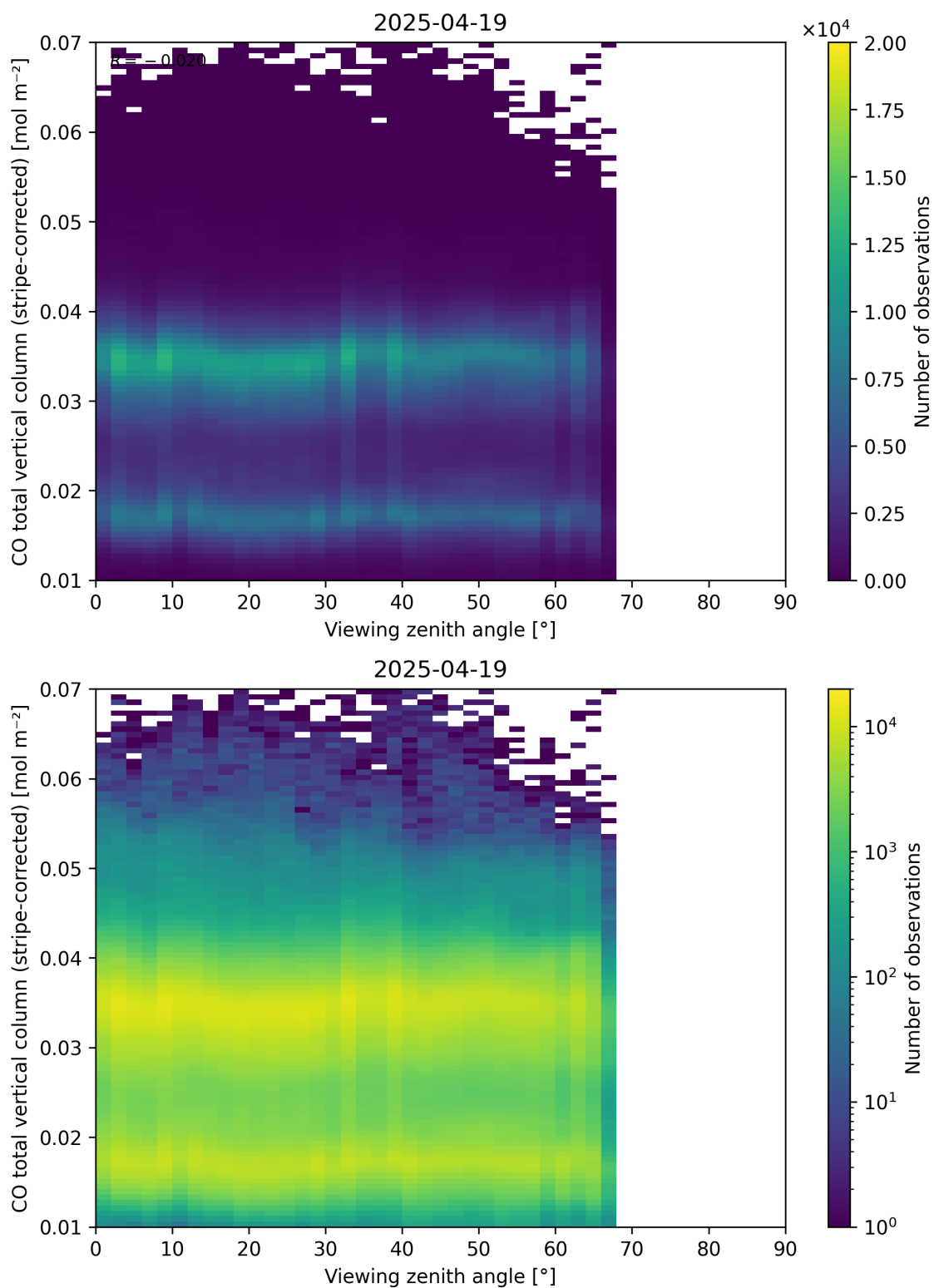
Figure 70: Scatter density plot of “Viewing zenith angle” against “CO total vertical column (stripe-corrected)” for 2025-04-19 to 2025-04-20.
