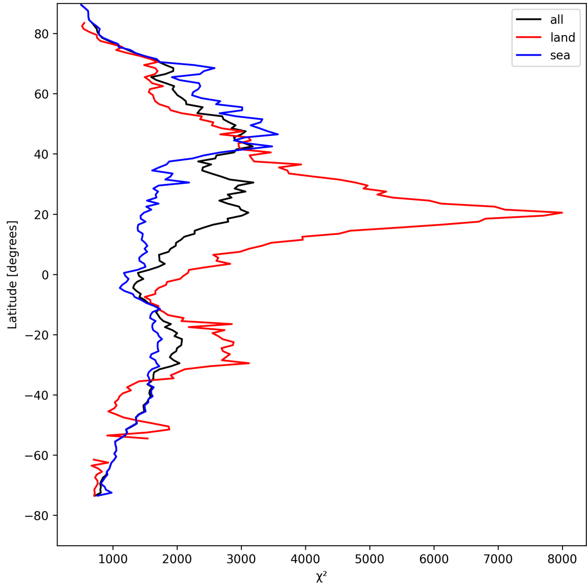
Figure 14: Zonal average of “ \chi^2 ” for 2025-04-19 to 2025-04-20.
