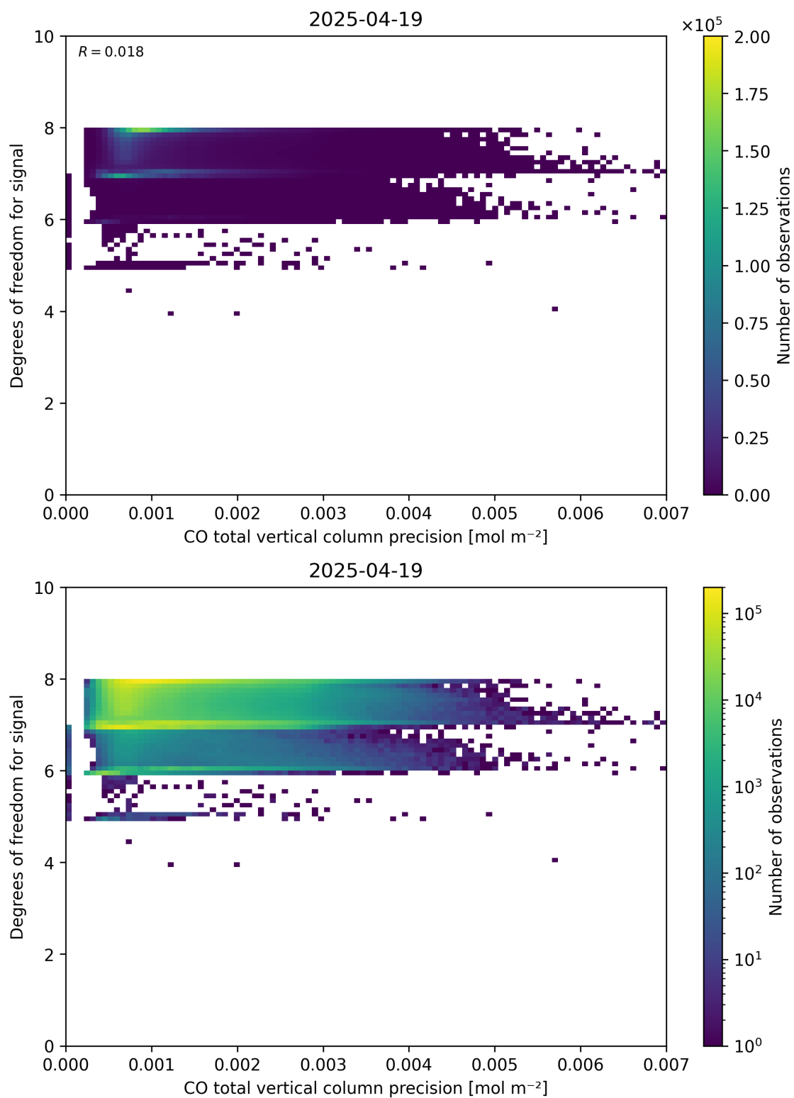
Figure 45: Scatter density plot of “CO total vertical column precision” against “Degrees of freedom for signal” for 2025-04-19 to 2025-04-20.
