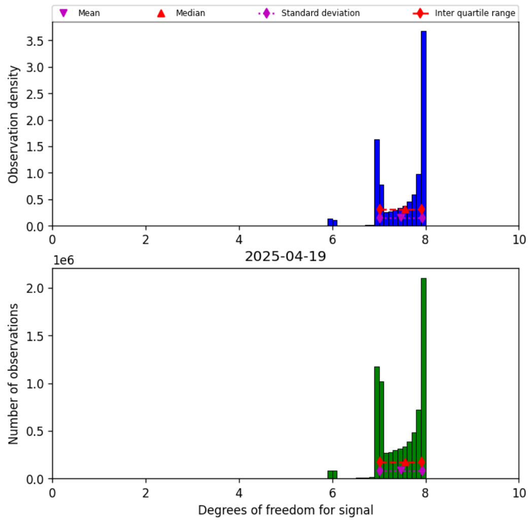
Figure 23: Histogram of “Degrees of freedom for signal” for 2025-04-19 to 2025-04-20
