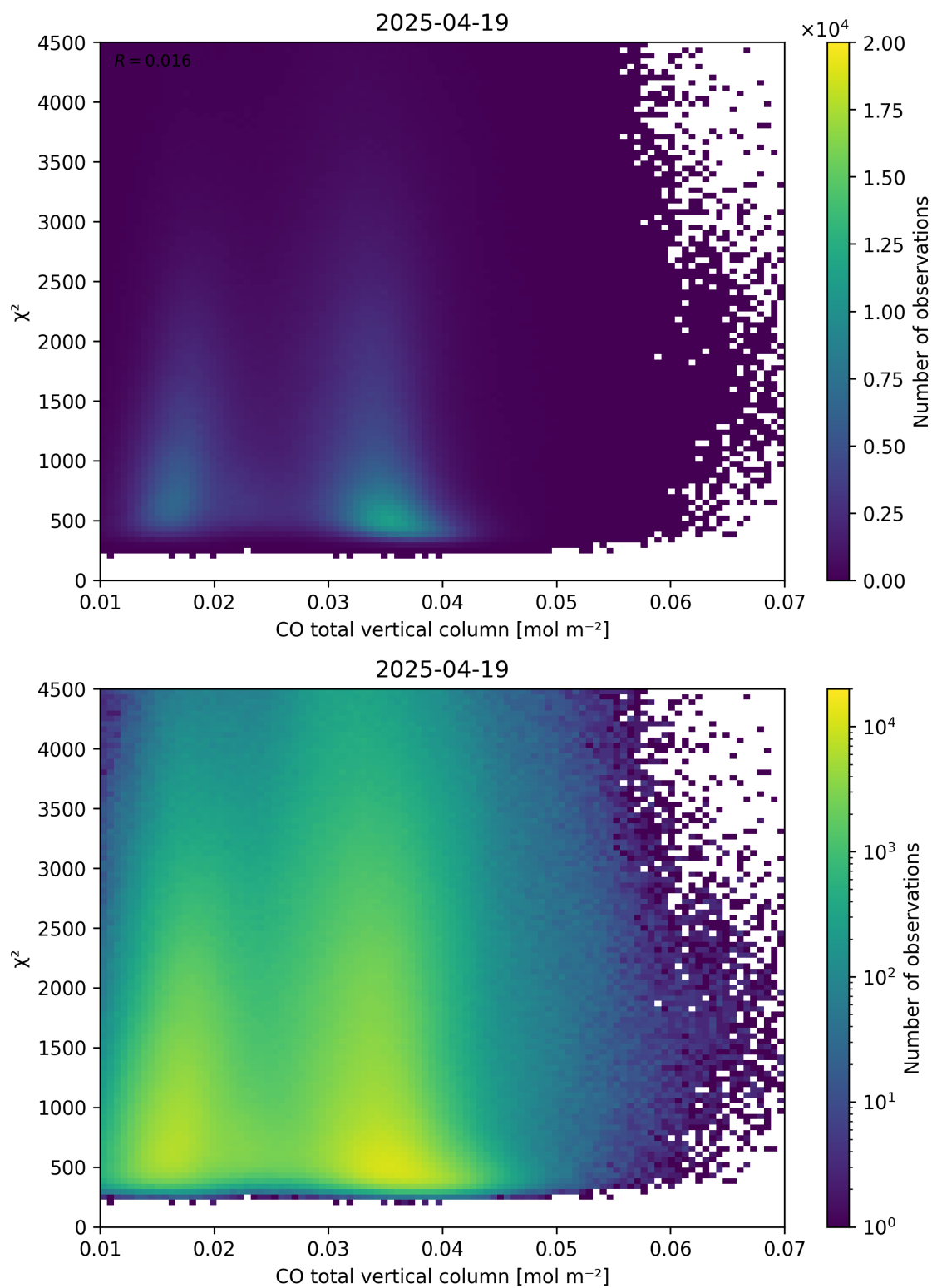
Figure 35: Scatter density plot of “CO total vertical column” against “ \chi^2 ” for 2025-04-19 to 2025-04-20.
