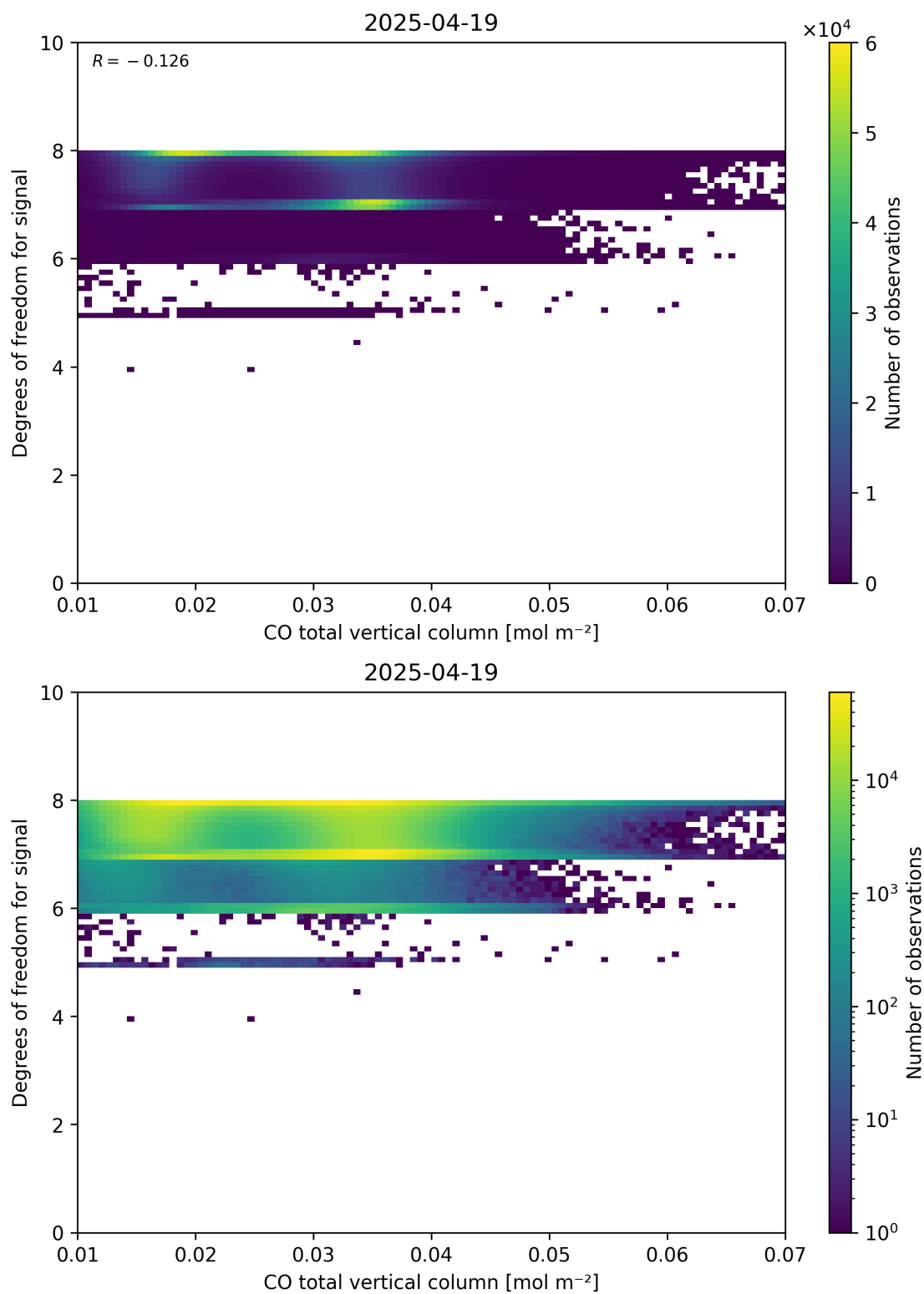
Figure 41: Scatter density plot of “CO total vertical column” against “Degrees of freedom for signal” for 2025-04-19 to 2025-04-20.
