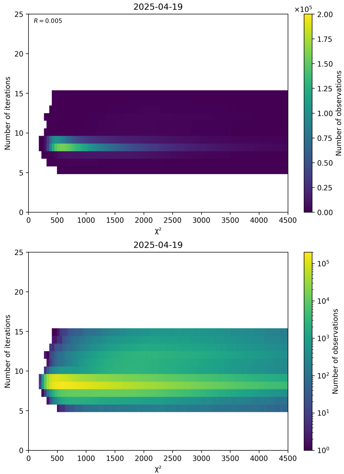
Figure 49: Scatter density plot of “ \chi^2 ” against “Number of iterations” for 2025-04-19 to 2025-04-20.
