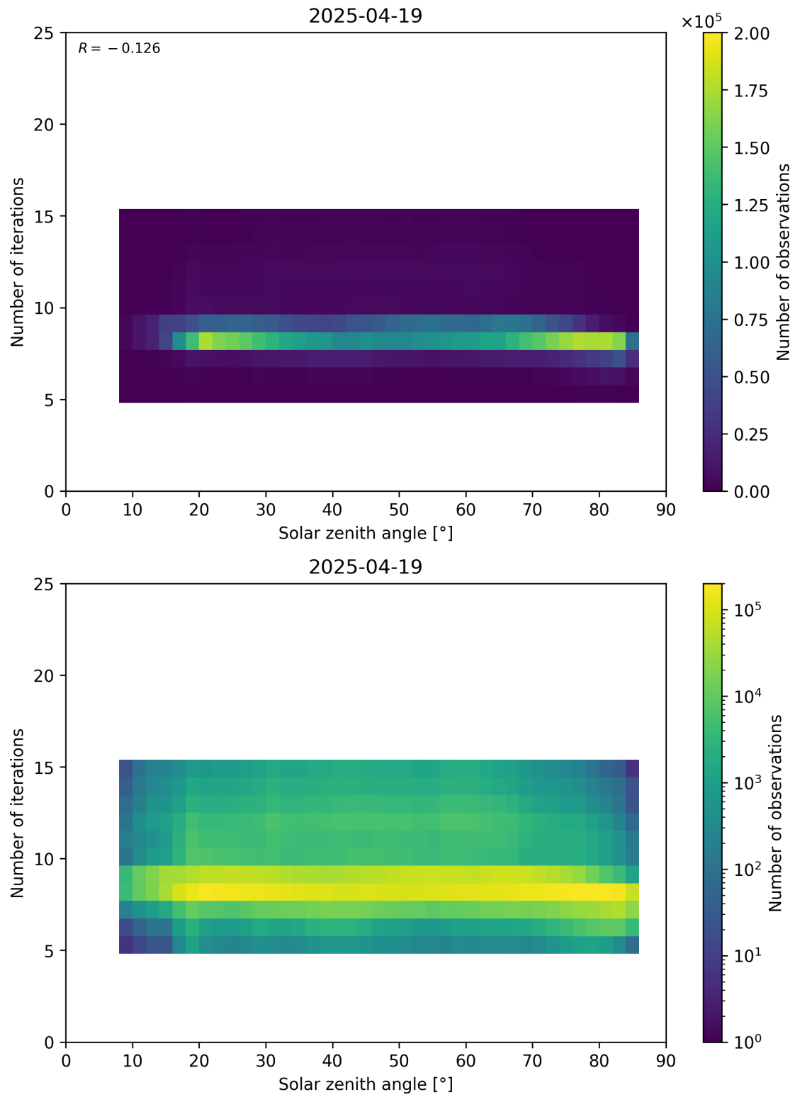
Figure 67: Scatter density plot of “Solar zenith angle” against “Number of iterations” for 2025-04-19 to 2025-04-20.
