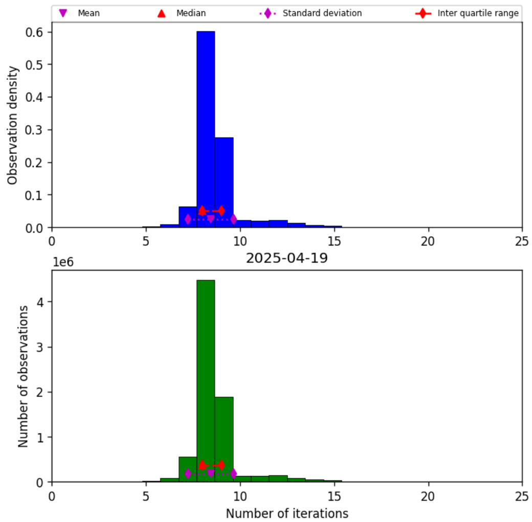
Figure 24: Histogram of “Number of iterations” for 2025-04-19 to 2025-04-20
