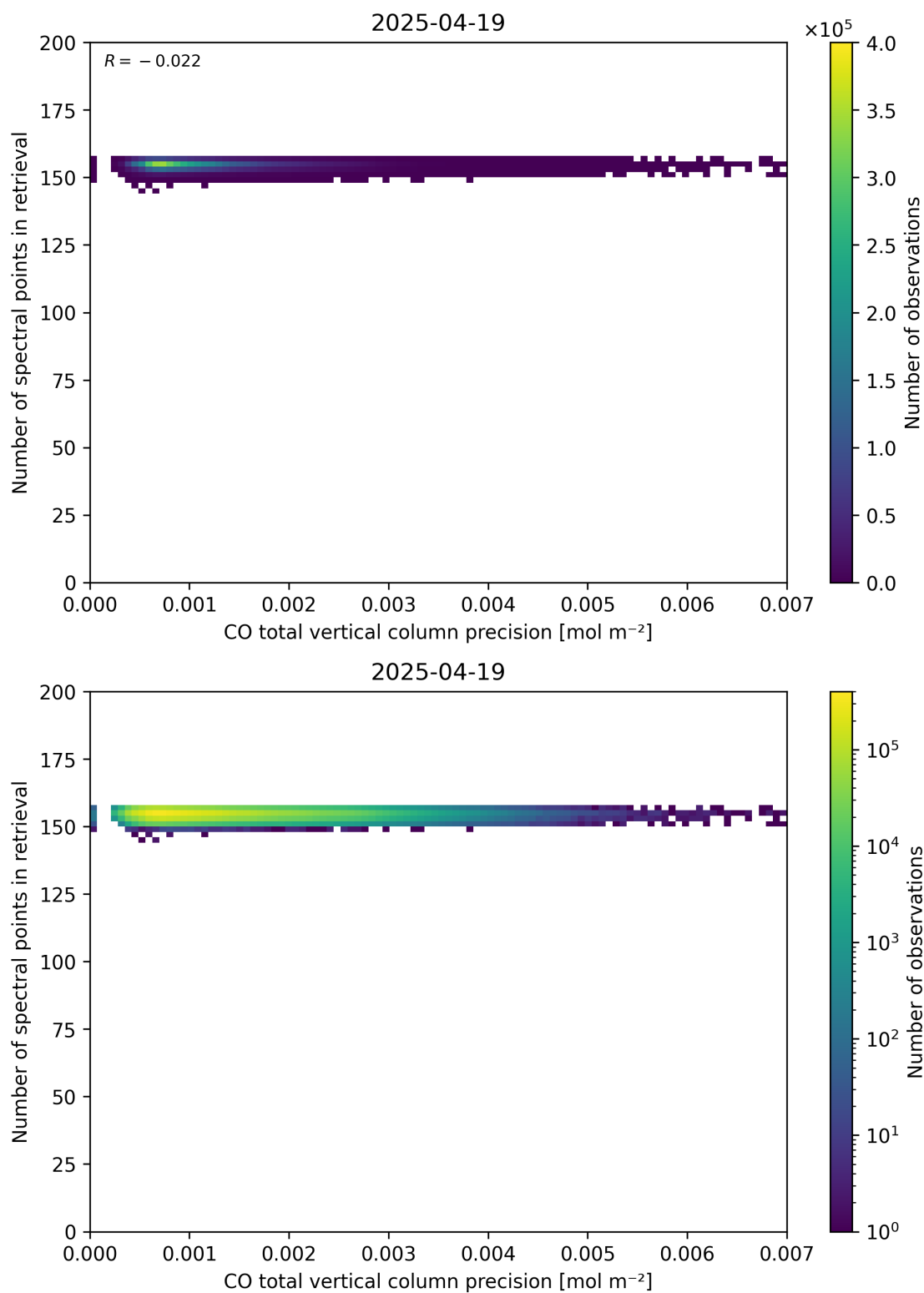
Figure 47: Scatter density plot of “CO total vertical column precision” against “Number of spectral points in retrieval” for 2025-04-19 to 2025-04-20.
