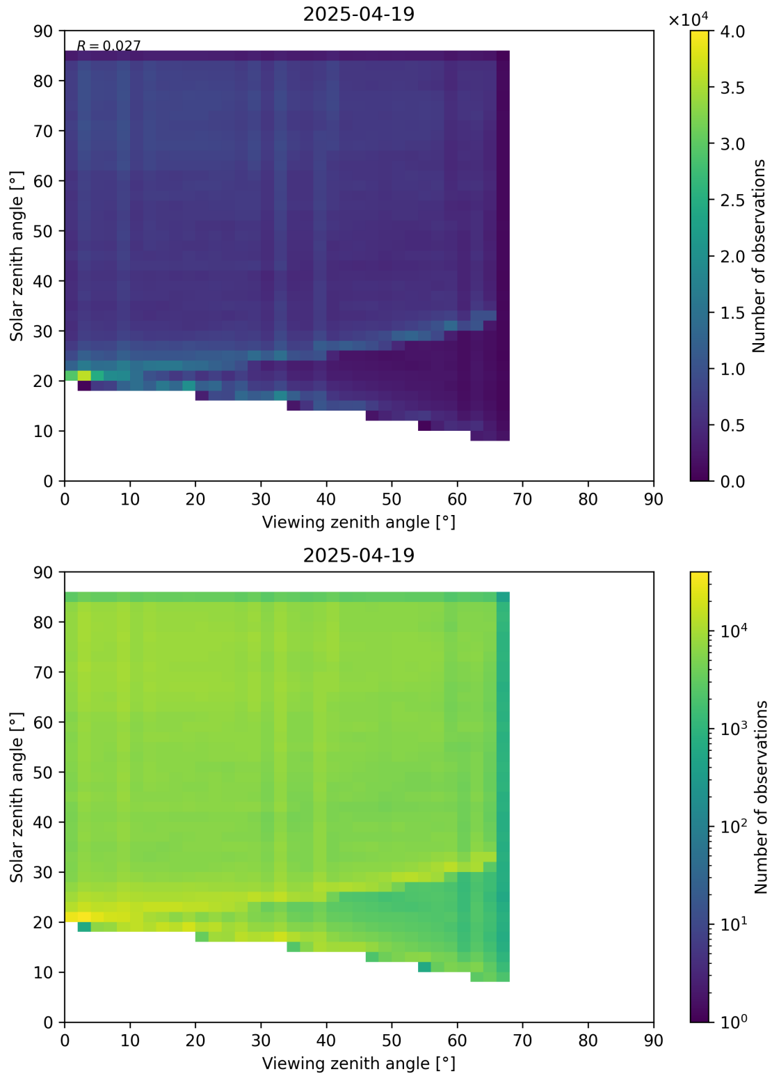
Figure 77: Scatter density plot of “Viewing zenith angle” against “Solar zenith angle” for 2025-04-19 to 2025-04-20.
