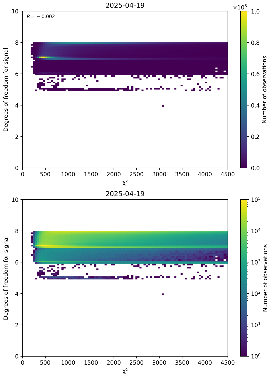
Figure 48: Scatter density plot of “ \chi^2 ” against “Degrees of freedom for signal” for 2025-04-19 to 2025-04-20.
