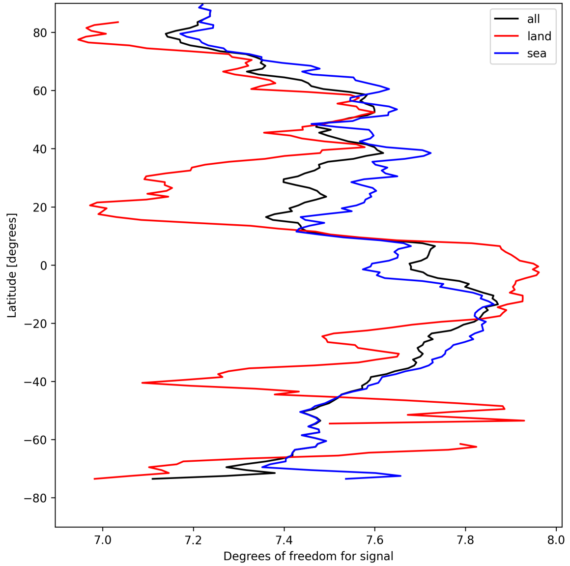
Figure 15: Zonal average of “Degrees of freedom for signal” for 2025-04-19 to 2025-04-20.
