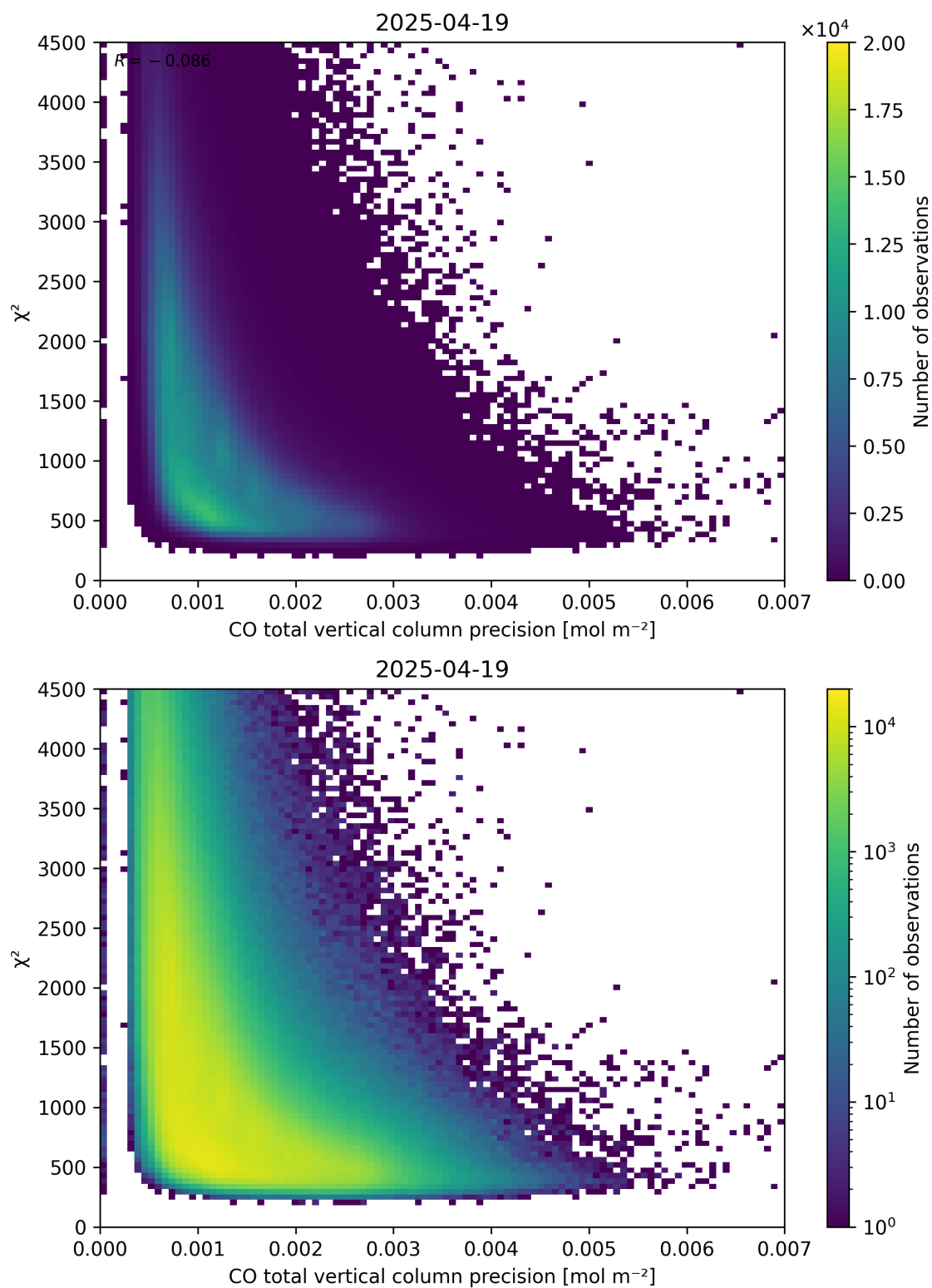
Figure 44: Scatter density plot of “CO total vertical column precision” against “ \chi^2 ” for 2025-04-19 to 2025-04-20.
