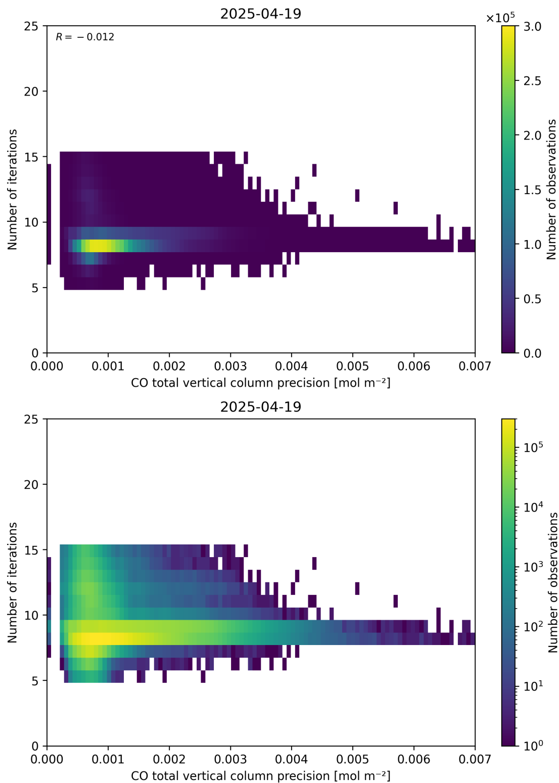
Figure 46: Scatter density plot of “CO total vertical column precision” against “Number of iterations” for 2025-04-19 to 2025-04-20.
