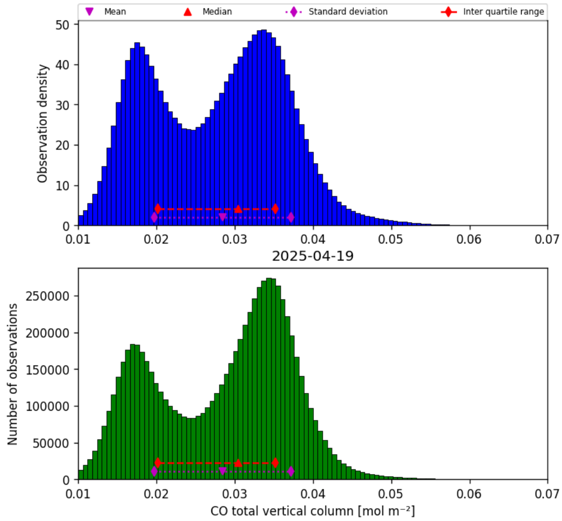
Figure 18: Histogram of “CO total vertical column” for 2025-04-19 to 2025-04-20
