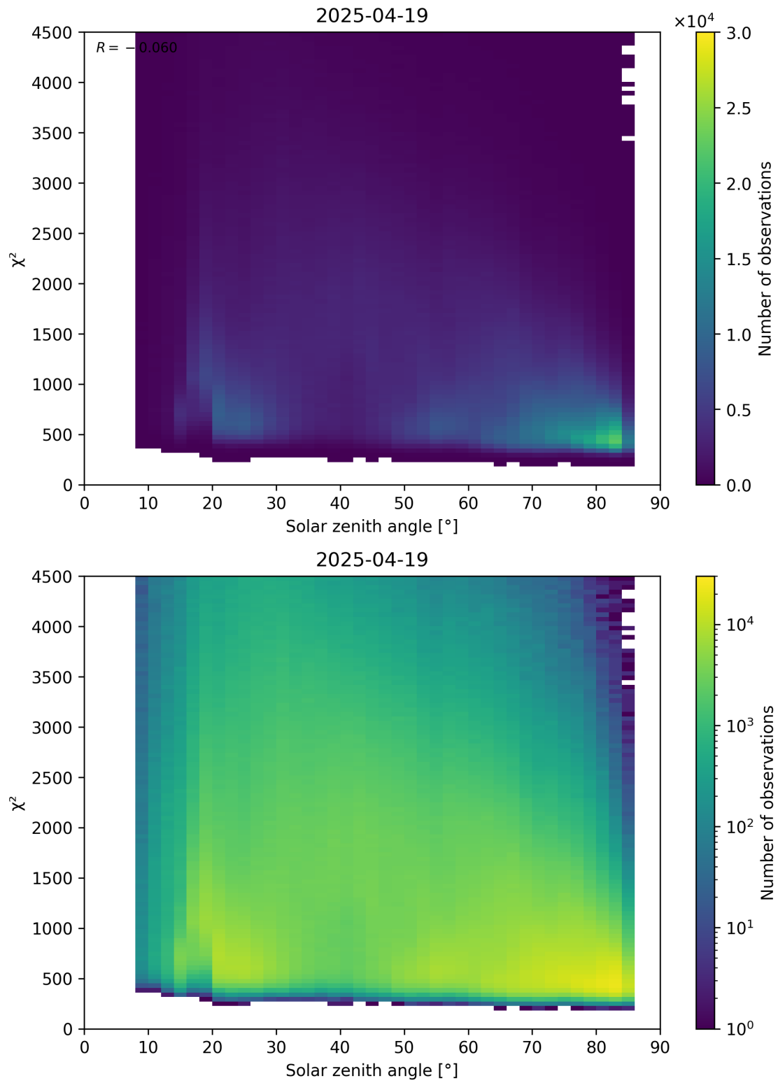
Figure 64: Scatter density plot of “Solar zenith angle” against “ \chi^2 ” for 2025-04-19 to 2025-04-20.
