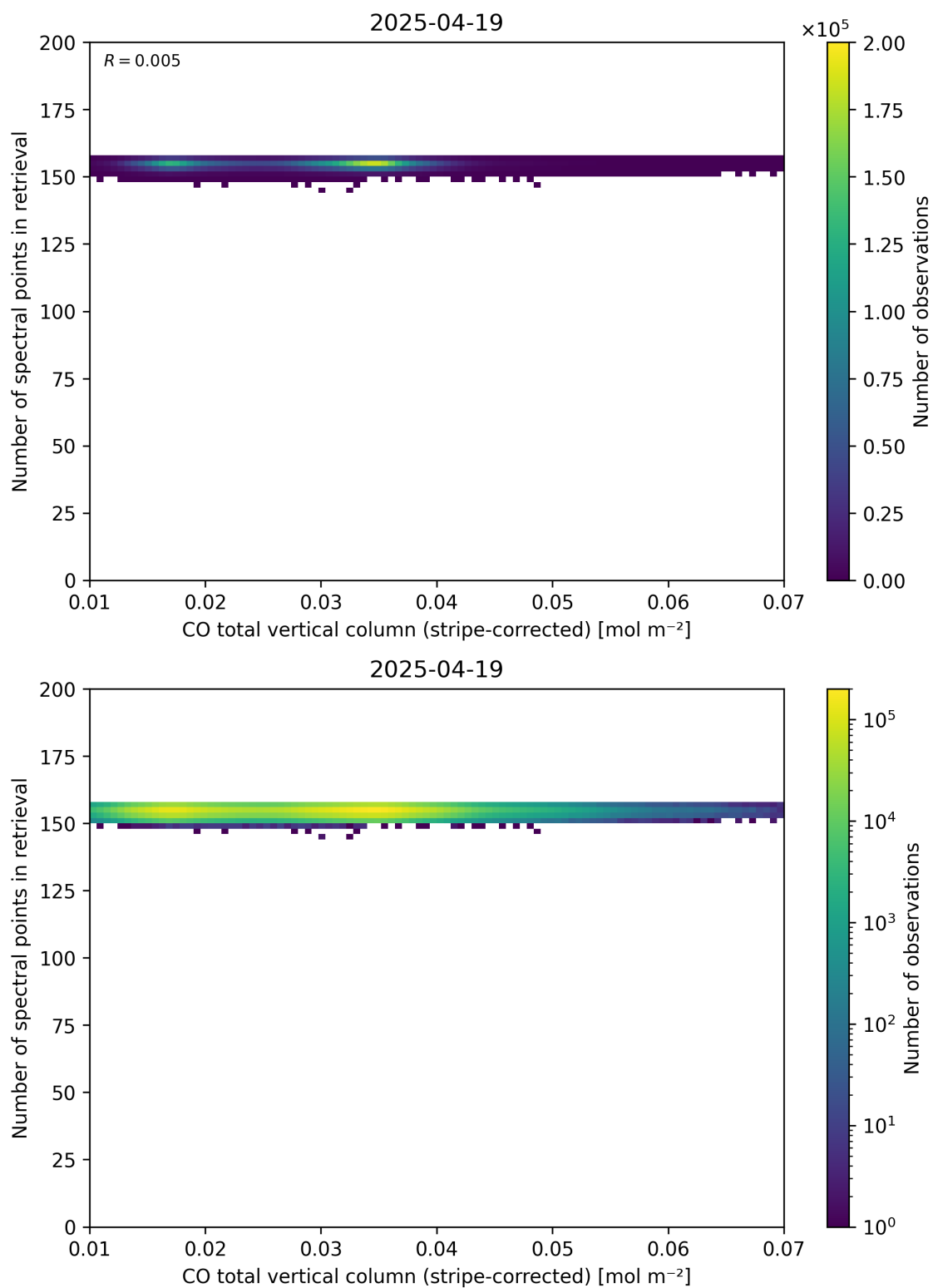
Figure 40: Scatter density plot of “CO total vertical column (stripe-corrected)” against “Number of spectral points in retrieval” for 2025-04-19 to 2025-04-20.
