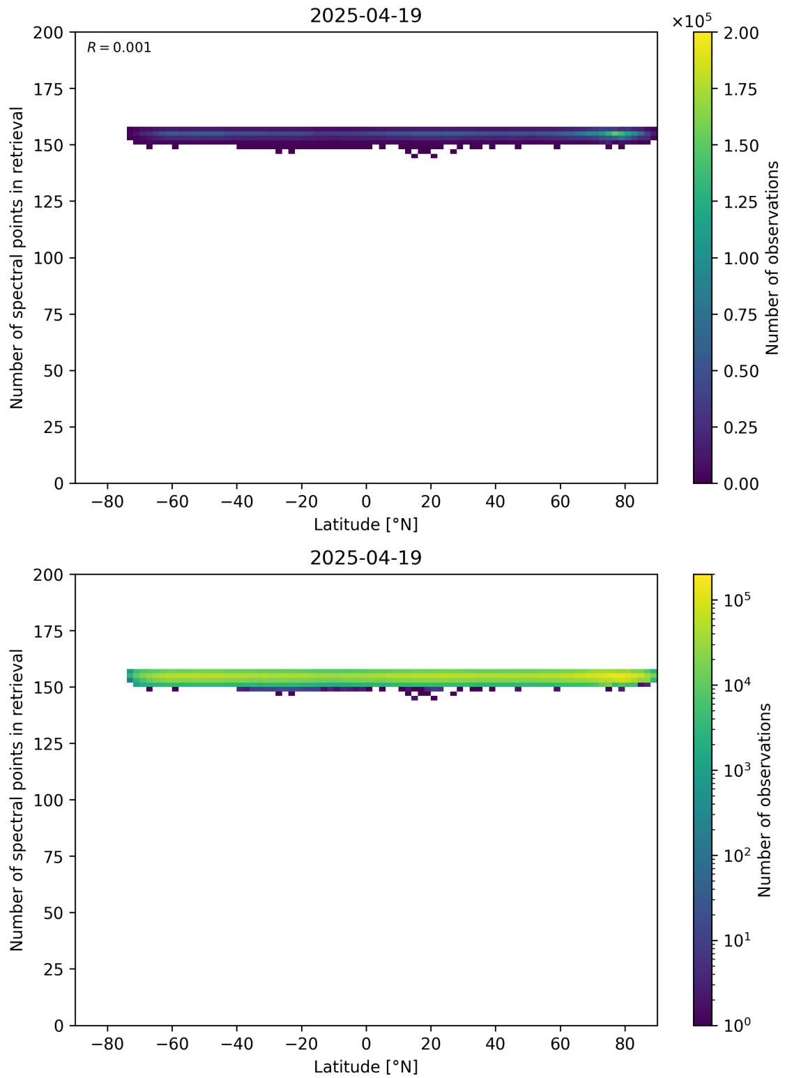
Figure 57: Scatter density plot of “Latitude” against “Number of spectral points in retrieval” for 2025-04-19 to 2025-04-20.
