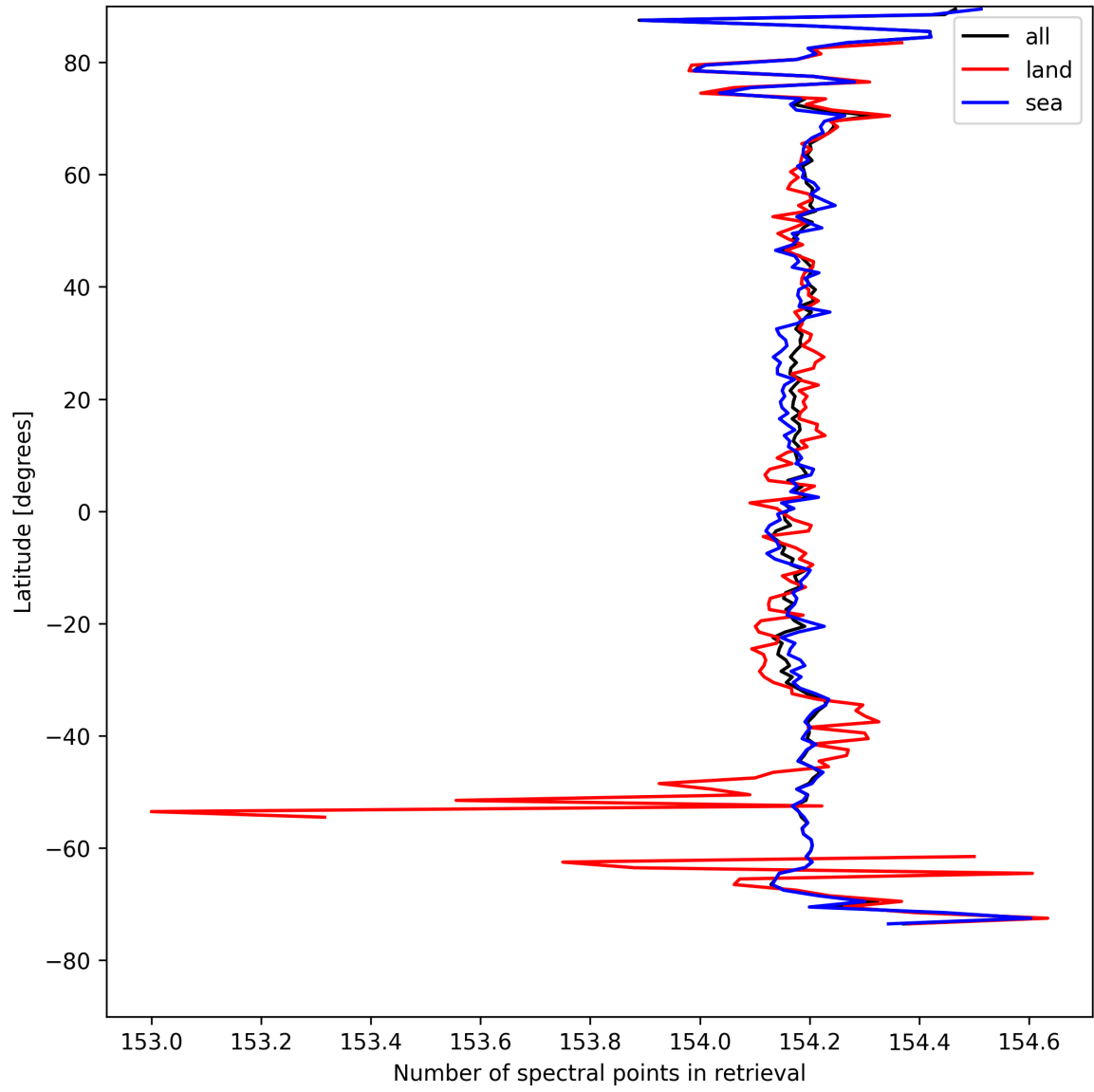
Figure 13: Zonal average of “Number of spectral points in retrieval” for 2025-04-19 to 2025-04-20.
