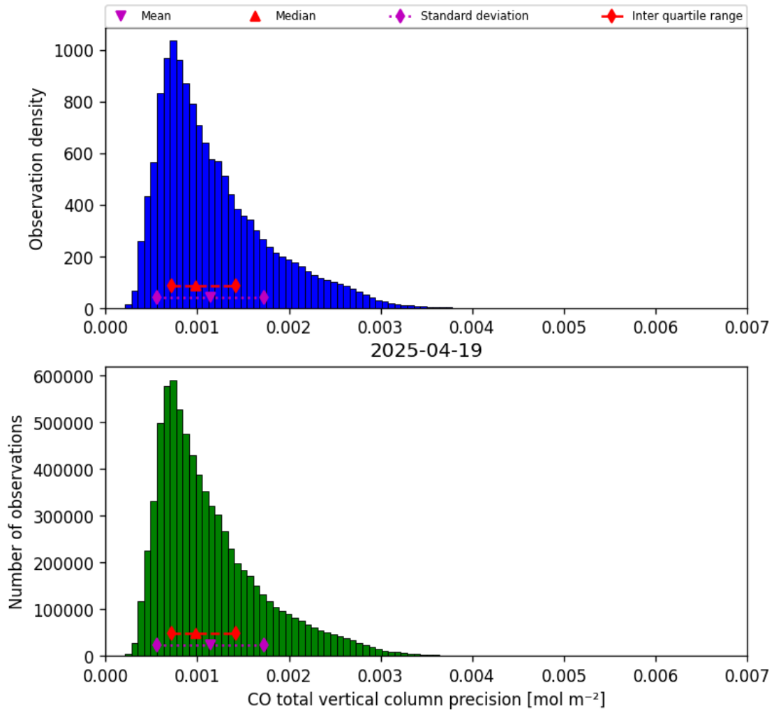
Figure 20: Histogram of “CO total vertical column precision” for 2025-04-19 to 2025-04-20
