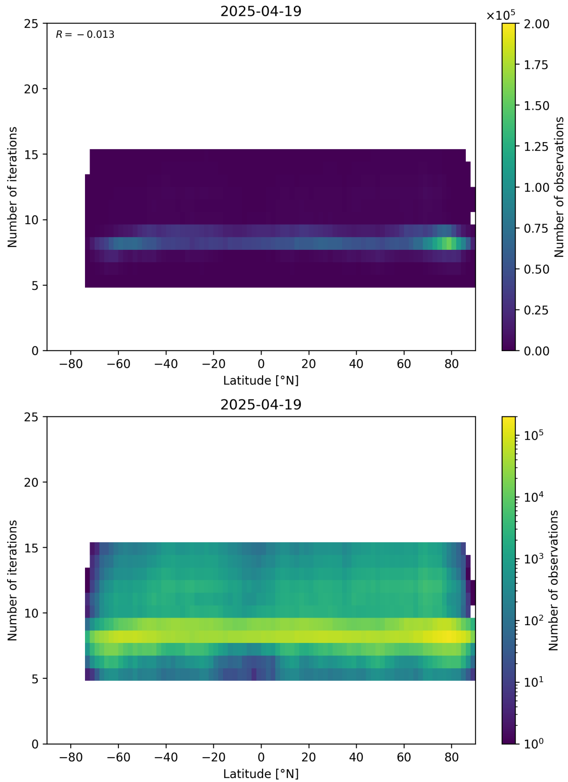
Figure 56: Scatter density plot of “Latitude” against “Number of iterations” for 2025-04-19 to 2025-04-20.
