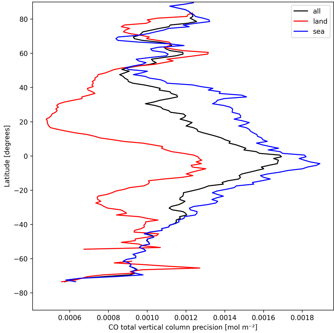
Figure 12: Zonal average of “CO total vertical column precision” for 2025-04-19 to 2025-04-20.
