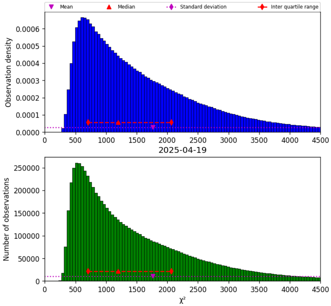
Figure 22: Histogram of “ \chi^2 ” for 2025-04-19 to 2025-04-20
