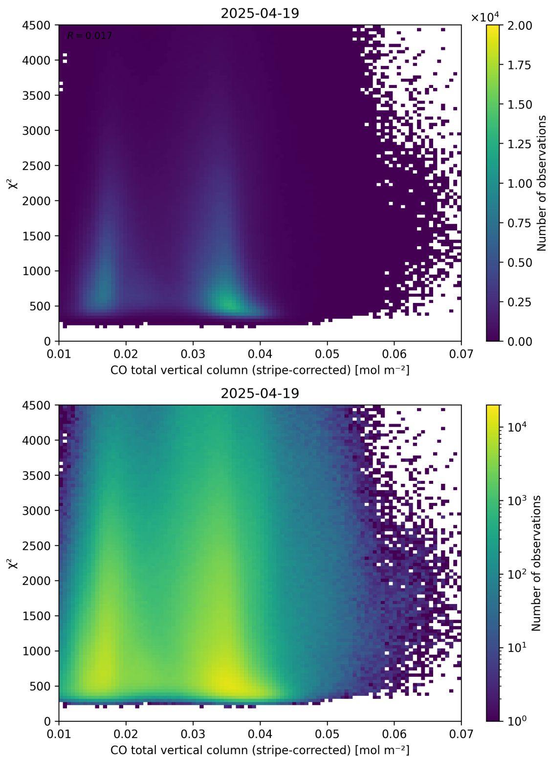
Figure 37: Scatter density plot of “CO total vertical column (stripe-corrected)” against “ \chi^2 ” for 2025-04-19 to 2025-04-20.
