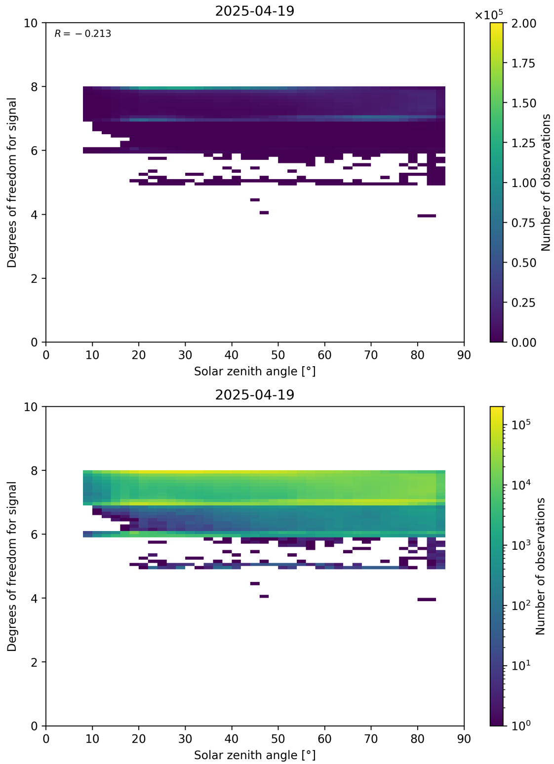
Figure 65: Scatter density plot of “Solar zenith angle” against “Degrees of freedom for signal” for 2025-04-19 to 2025-04-20.
