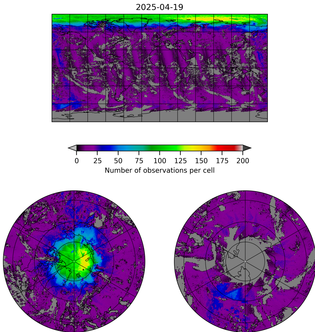
Figure 8: Map of the number of observations for 2025-04-19 to 2025-04-20
