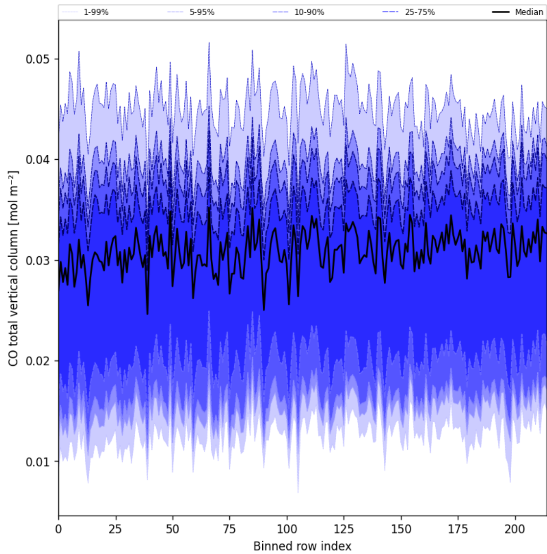
Figure 26: Along track statistics of “CO total vertical column” for 2025-04-19 to 2025-04-20
