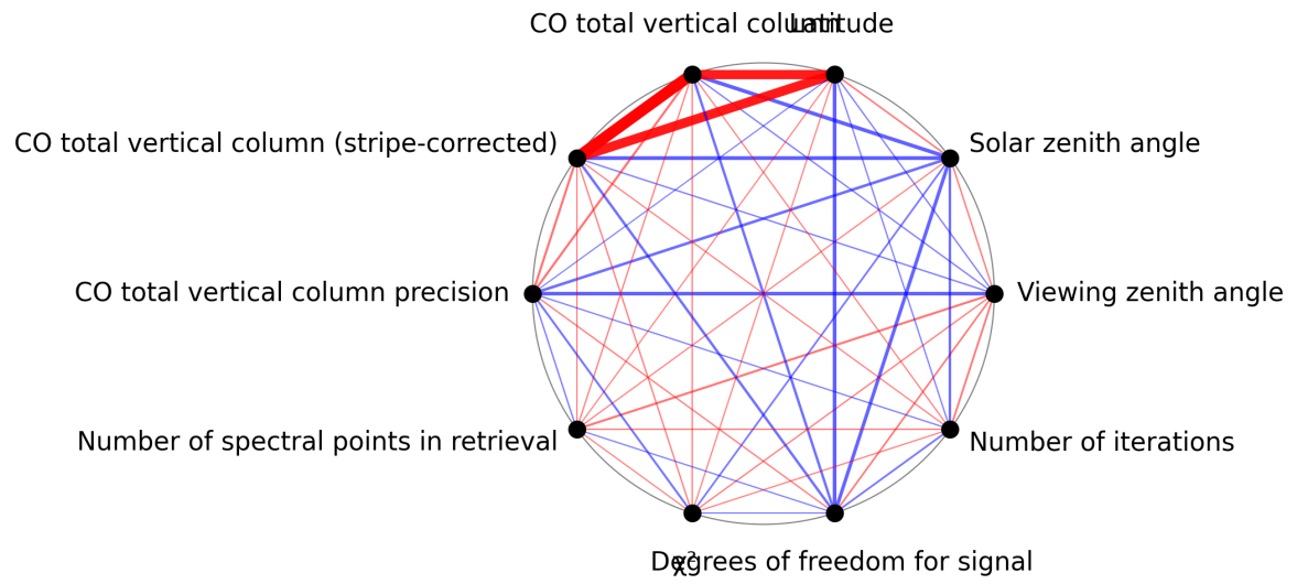
Figure 1: Map of correlation graph for 2025-04-19 to 2025-04-20.
