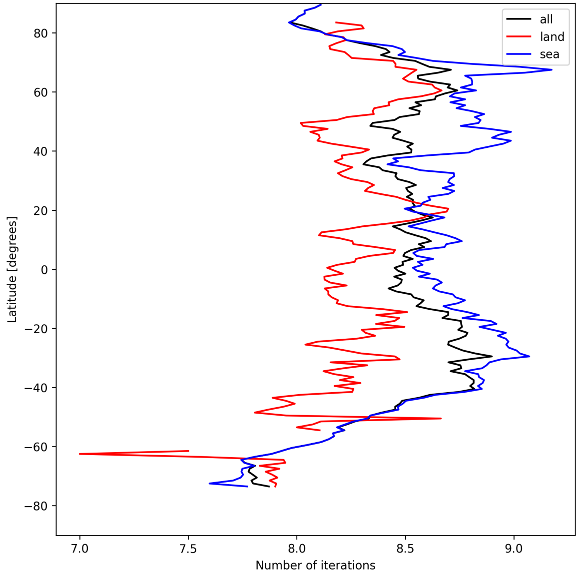
Figure 16: Zonal average of “Number of iterations” for 2025-04-19 to 2025-04-20.
