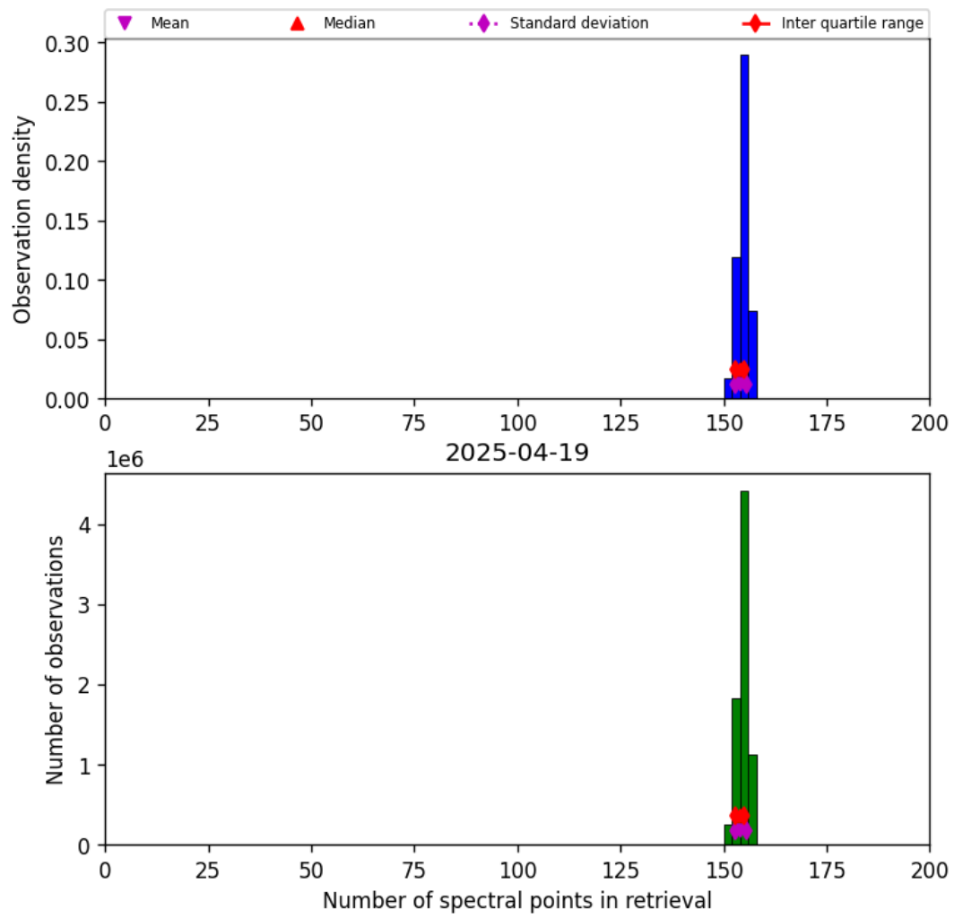
Figure 21: Histogram of “Number of spectral points in retrieval” for 2025-04-19 to 2025-04-20
