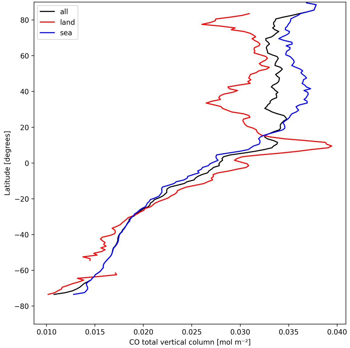
Figure 10: Zonal average of “CO total vertical column” for 2025-04-19 to 2025-04-20.
