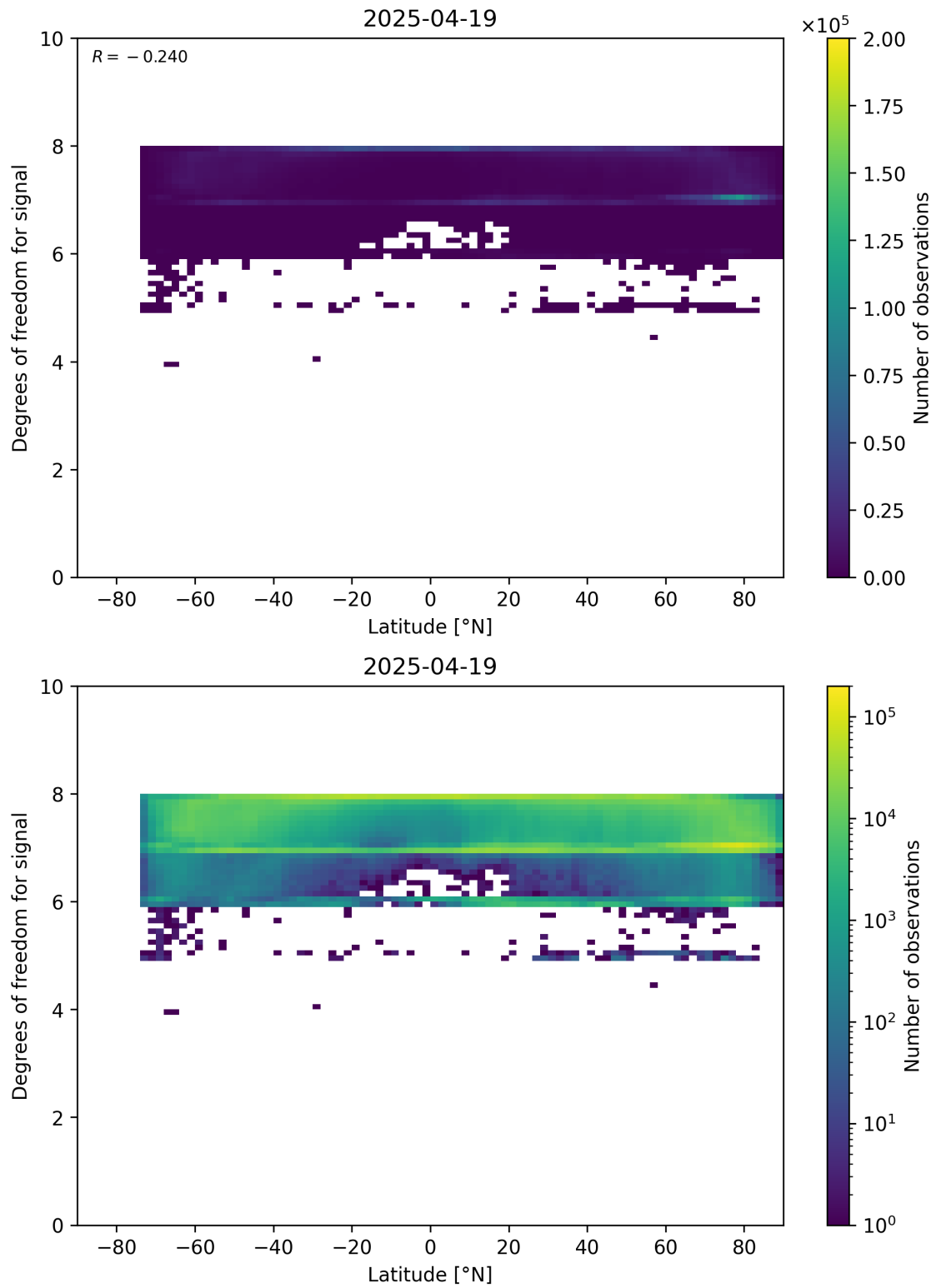
Figure 55: Scatter density plot of “Latitude” against “Degrees of freedom for signal” for 2025-04-19 to 2025-04-20.
