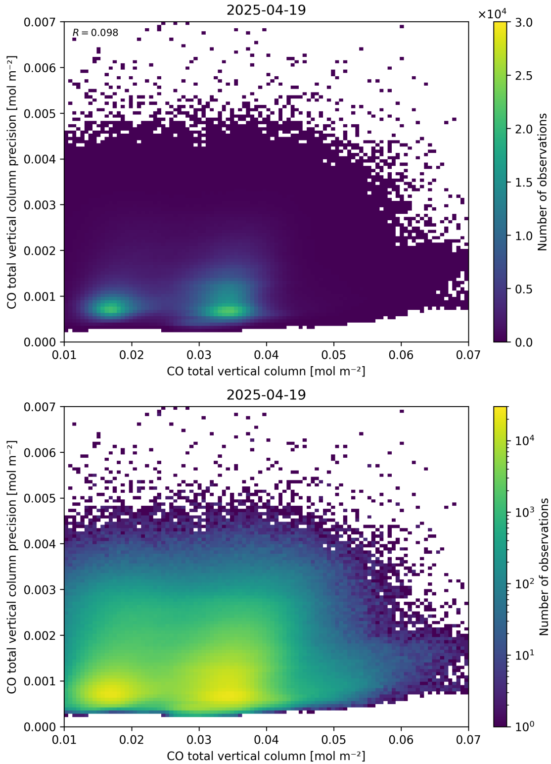
Figure 34: Scatter density plot of “CO total vertical column” against “CO total vertical column precision” for 2025-04-19 to 2025-04-20.
