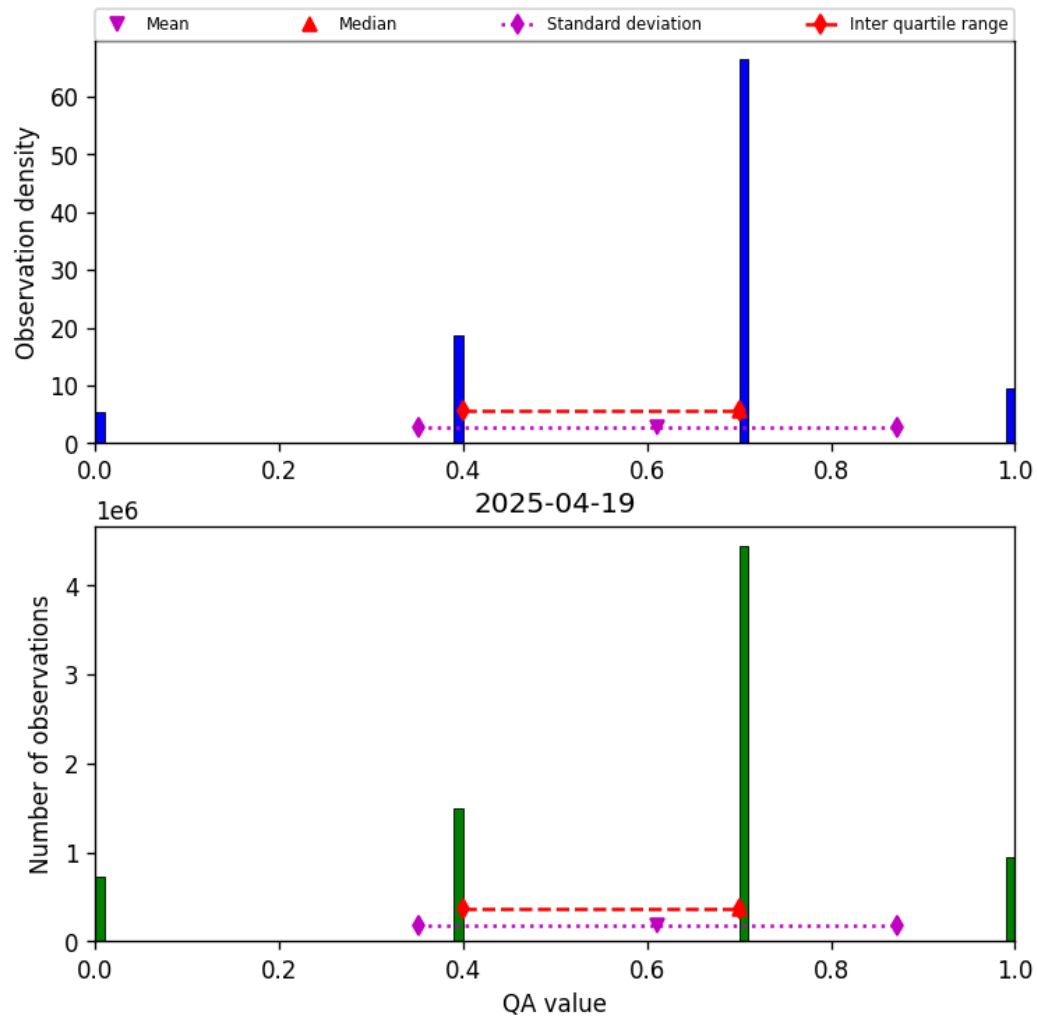
Figure 17: Histogram of “QA value” for 2025-04-19 to 2025-04-20
