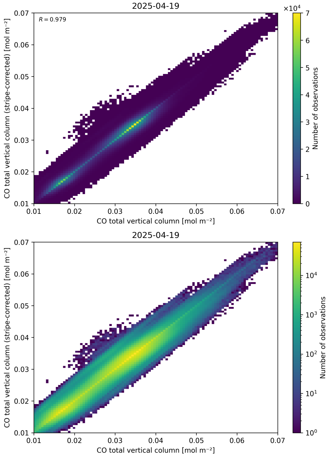
Figure 33: Scatter density plot of “CO total vertical column” against “CO total vertical column (stripe-corrected)” for 2025-04-19 to 2025-04-20.
