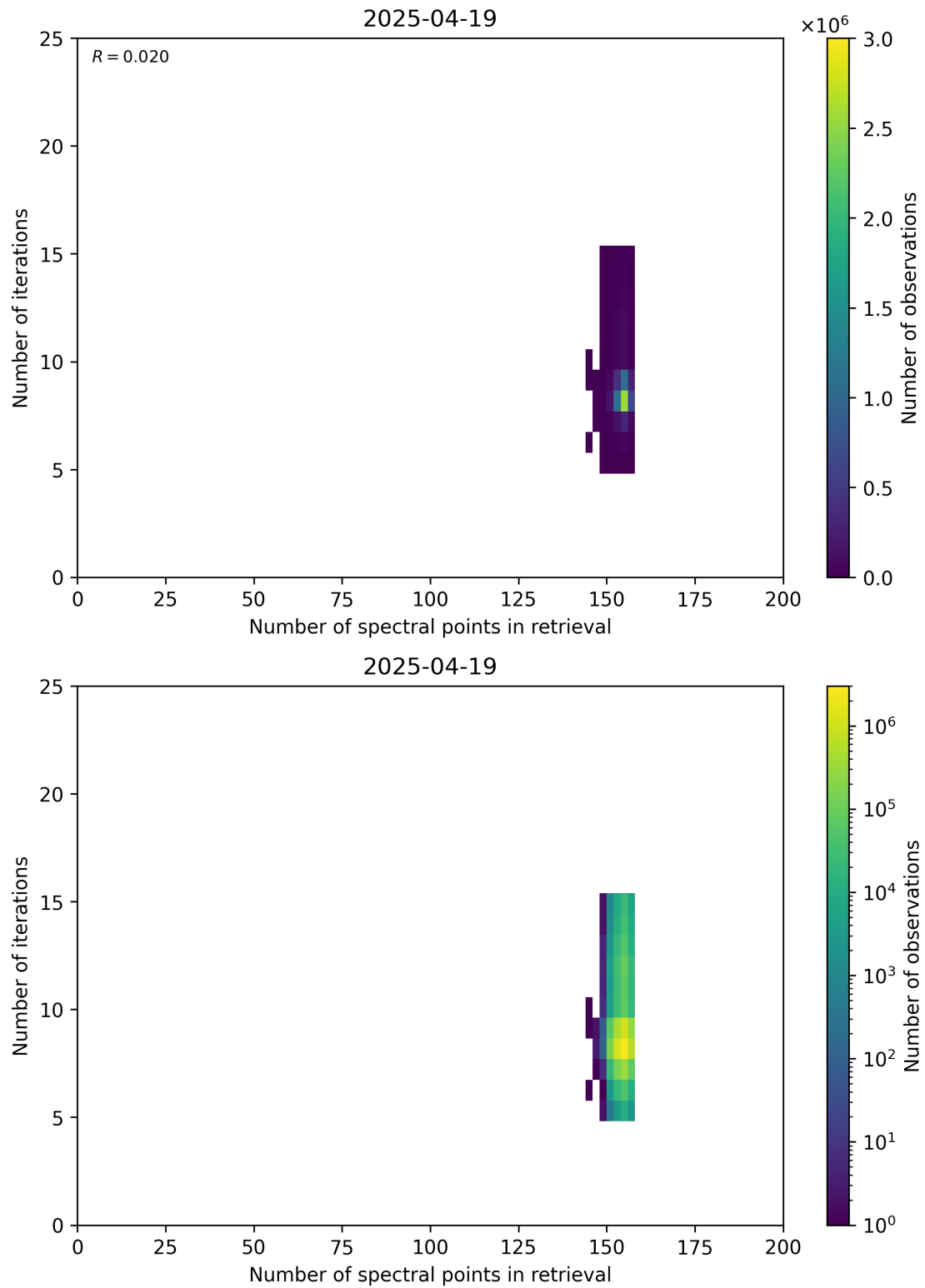
Figure 60: Scatter density plot of “Number of spectral points in retrieval” against “Number of iterations” for 2025-04-19 to 2025-04-20.
