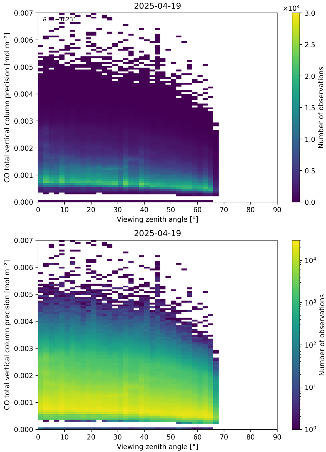
Figure 71: Scatter density plot of “Viewing zenith angle” against “CO total vertical column precision” for 2025-04-19 to 2025-04-20.
