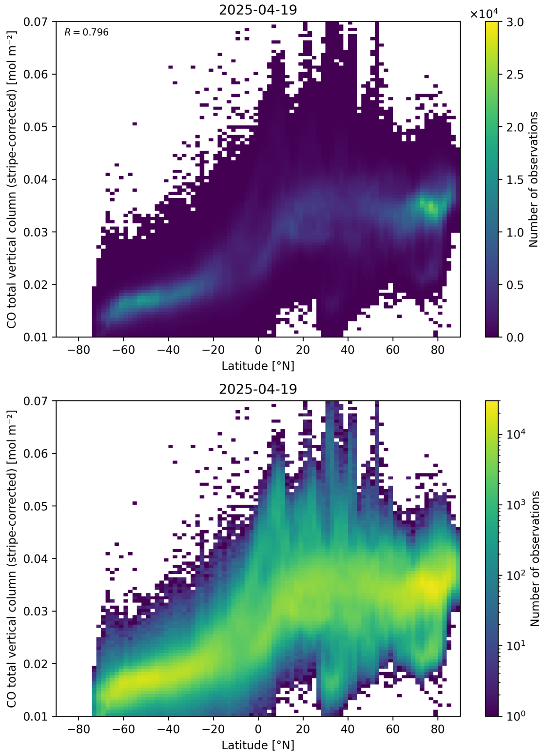
Figure 52: Scatter density plot of “Latitude” against “CO total vertical column (stripe-corrected)” for 2025-04-19 to 2025-04-20.
