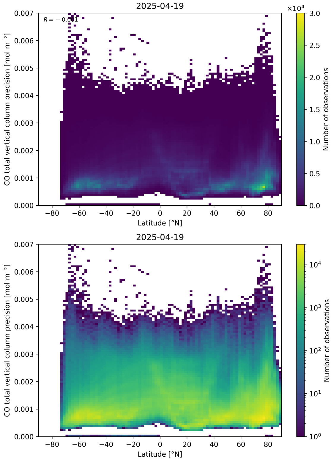
Figure 53: Scatter density plot of “Latitude” against “CO total vertical column precision” for 2025-04-19 to 2025-04-20.
