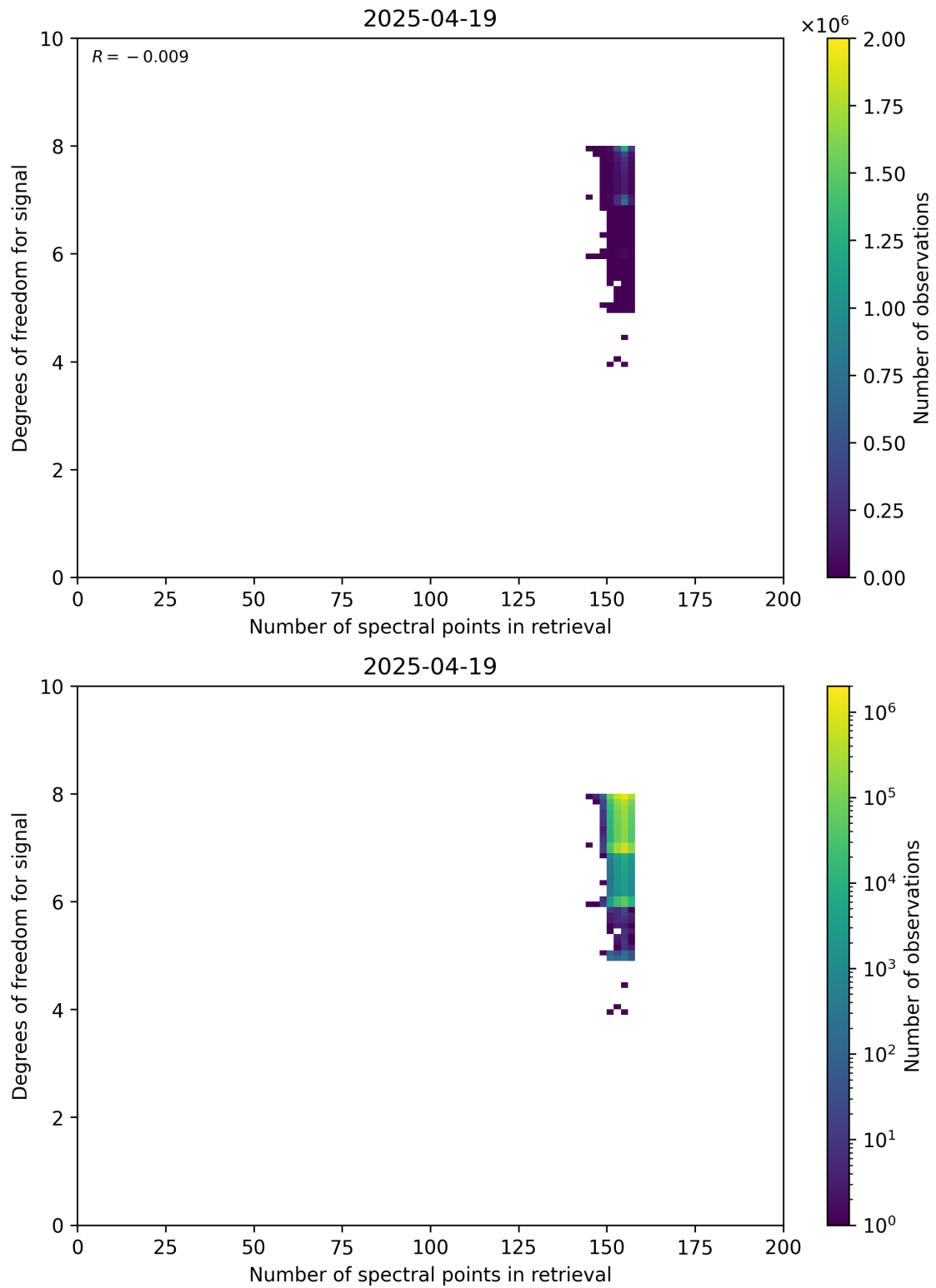
Figure 59: Scatter density plot of “Number of spectral points in retrieval” against “Degrees of freedom for signal” for 2025-04-19 to 2025-04-20.
