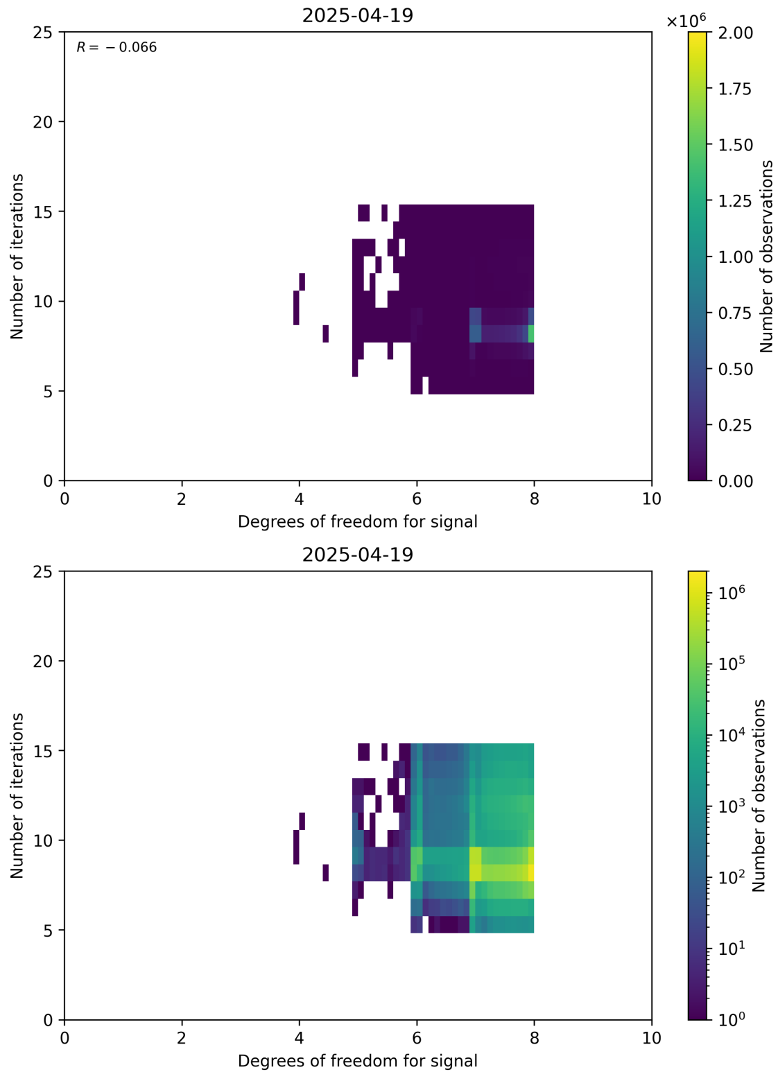
Figure 50: Scatter density plot of “Degrees of freedom for signal” against “Number of iterations” for 2025-04-19 to 2025-04-20.
