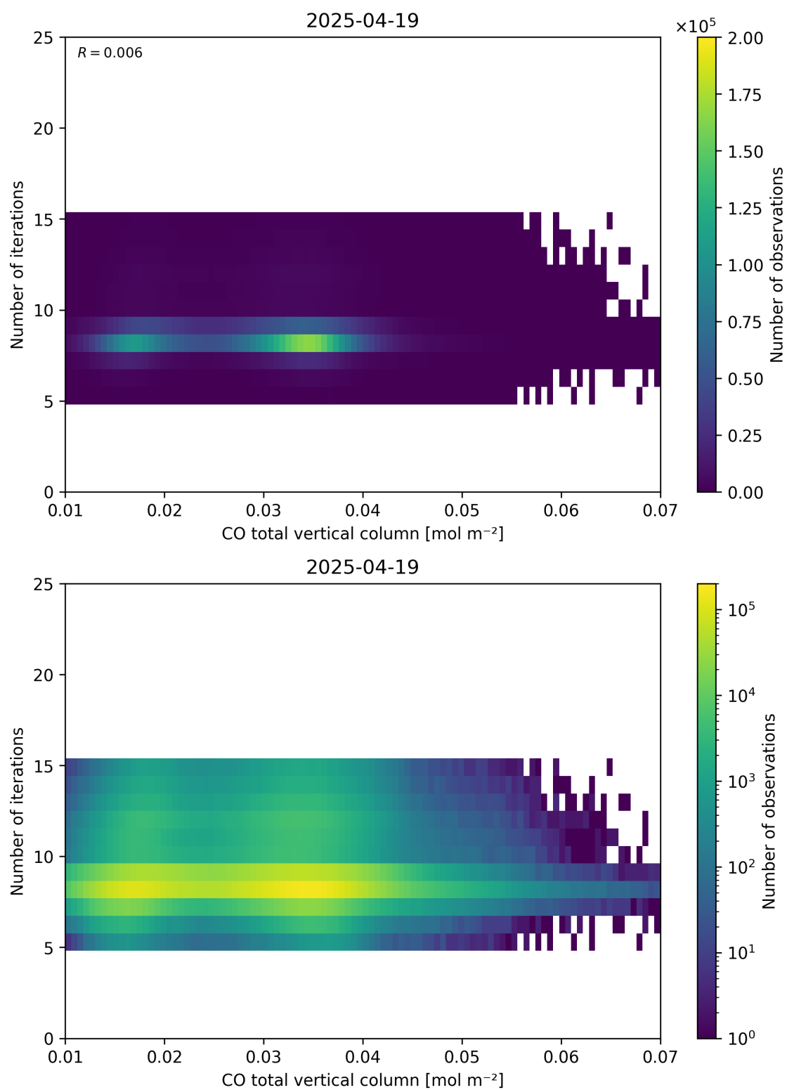
Figure 42: Scatter density plot of “CO total vertical column” against “Number of iterations” for 2025-04-19 to 2025-04-20.
