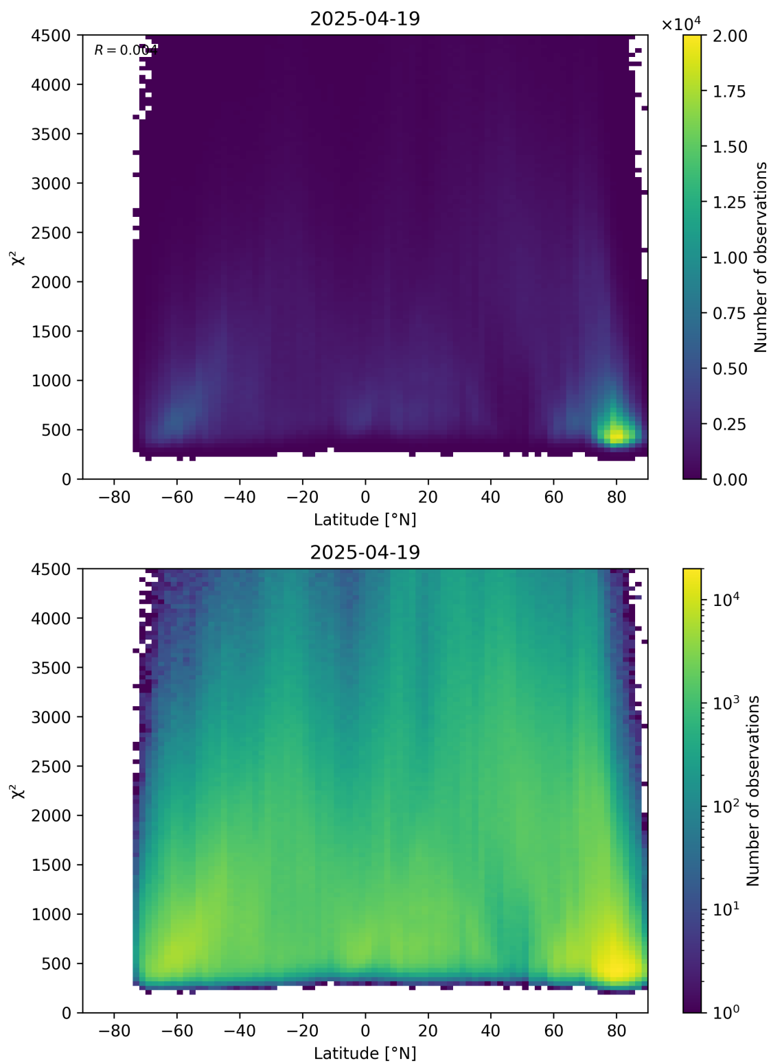
Figure 54: Scatter density plot of “Latitude” against “ \chi^2 ” for 2025-04-19 to 2025-04-20.
