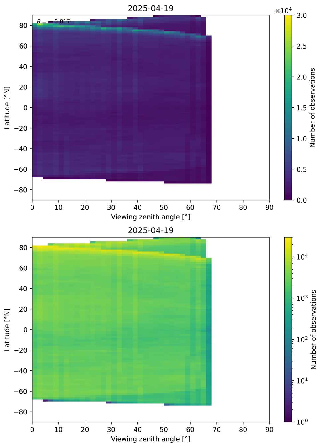
Figure 74: Scatter density plot of “Viewing zenith angle” against “Latitude” for 2025-04-19 to 2025-04-20.
