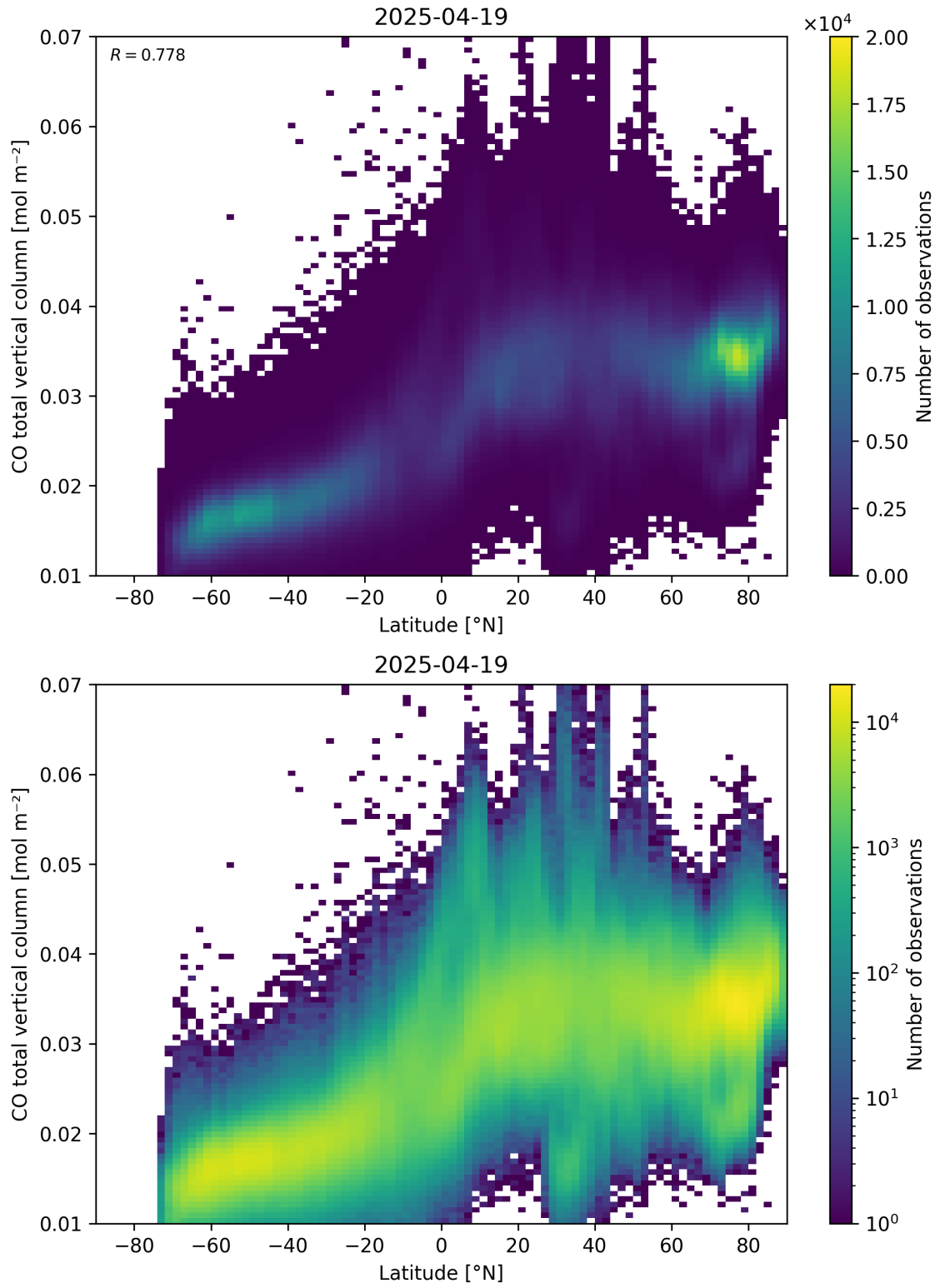
Figure 51: Scatter density plot of “Latitude” against “CO total vertical column” for 2025-04-19 to 2025-04-20.
