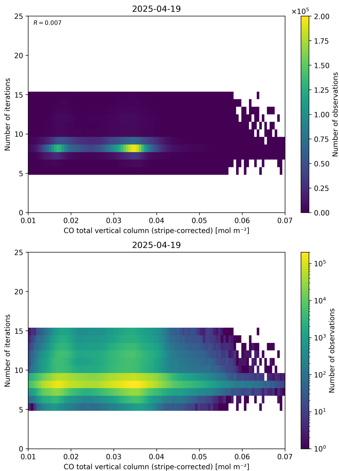
Figure 39: Scatter density plot of “CO total vertical column (stripe-corrected)” against “Number of iterations” for 2025-04-19 to 2025-04-20.
