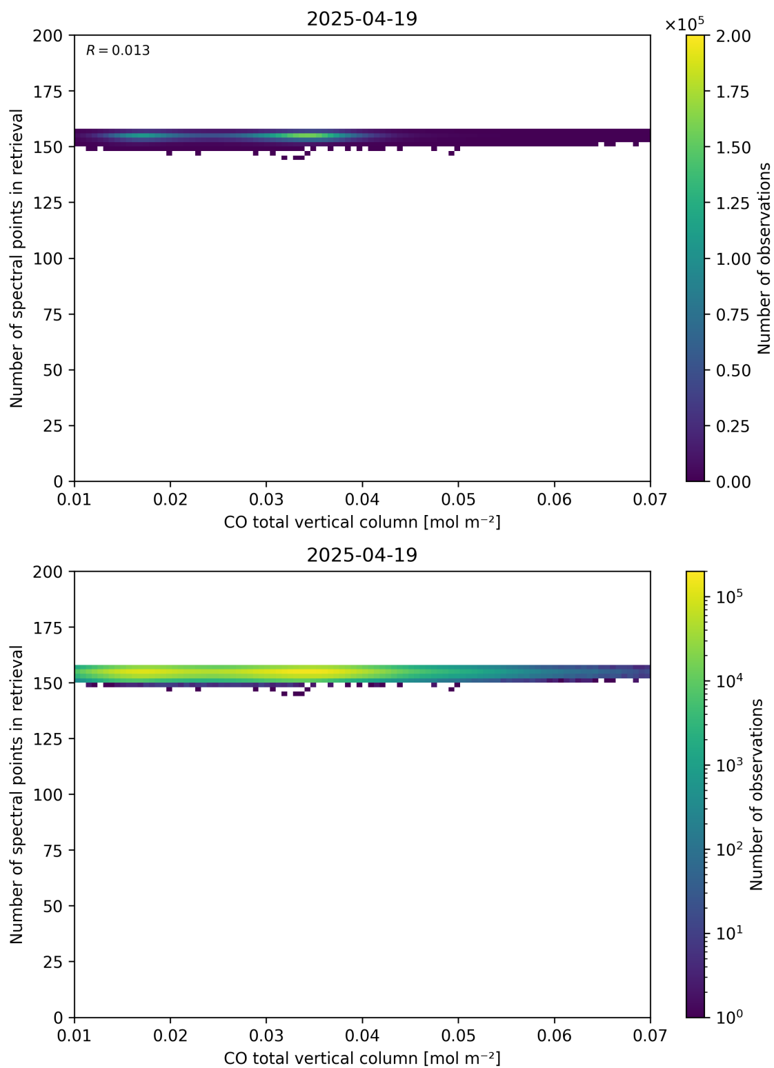
Figure 43: Scatter density plot of “CO total vertical column” against “Number of spectral points in retrieval” for 2025-04-19 to 2025-04-20.
