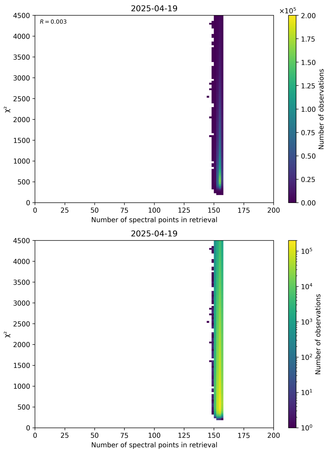
Figure 58: Scatter density plot of “Number of spectral points in retrieval” against “ \chi^2 ” for 2025-04-19 to 2025-04-20.
