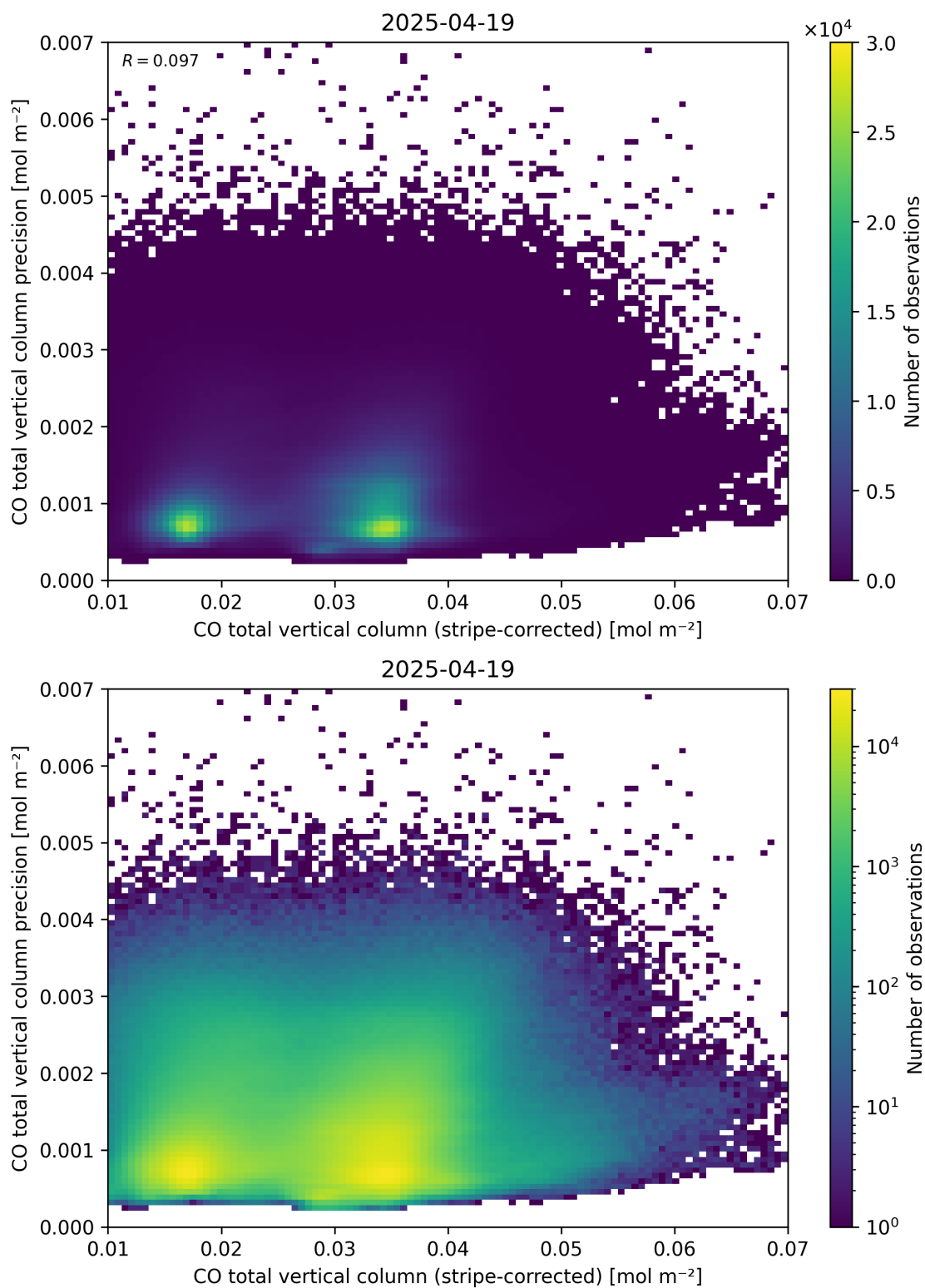
Figure 36: Scatter density plot of “CO total vertical column (stripe-corrected)” against “CO total vertical column precision” for 2025-04-19 to 2025-04-20.
