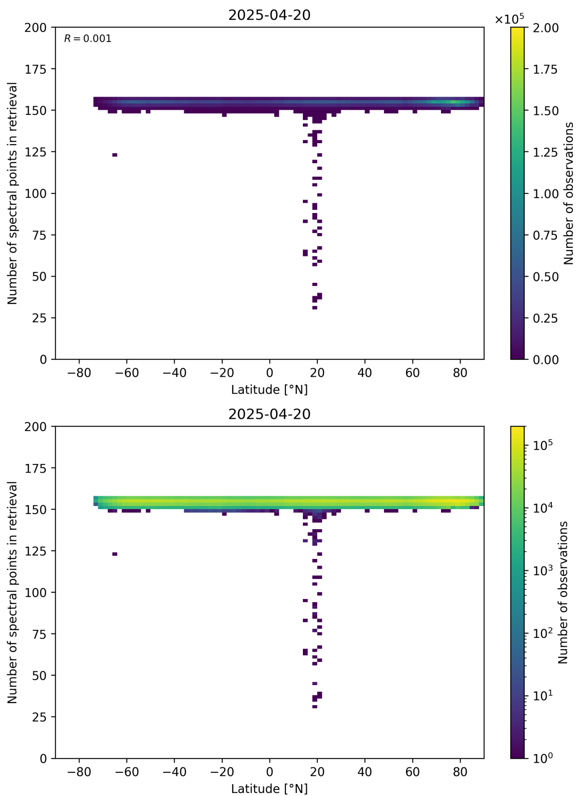
Figure 57: Scatter density plot of “Latitude” against “Number of spectral points in retrieval” for 2025-04-19 to 2025-04-21.
