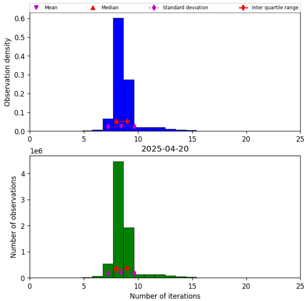
Figure 24: Histogram of “Number of iterations” for 2025-04-19 to 2025-04-21
