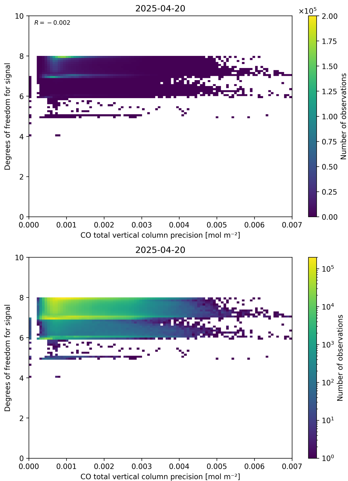
Figure 45: Scatter density plot of “CO total vertical column precision” against “Degrees of freedom for signal” for 2025-04-19 to 2025-04-21.
