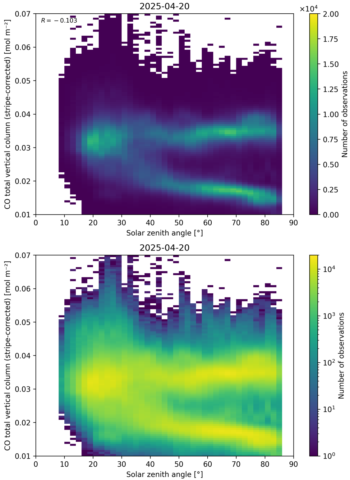
Figure 62: Scatter density plot of “Solar zenith angle” against “CO total vertical column (stripe-corrected)” for 2025-04-19 to 2025-04-21.
