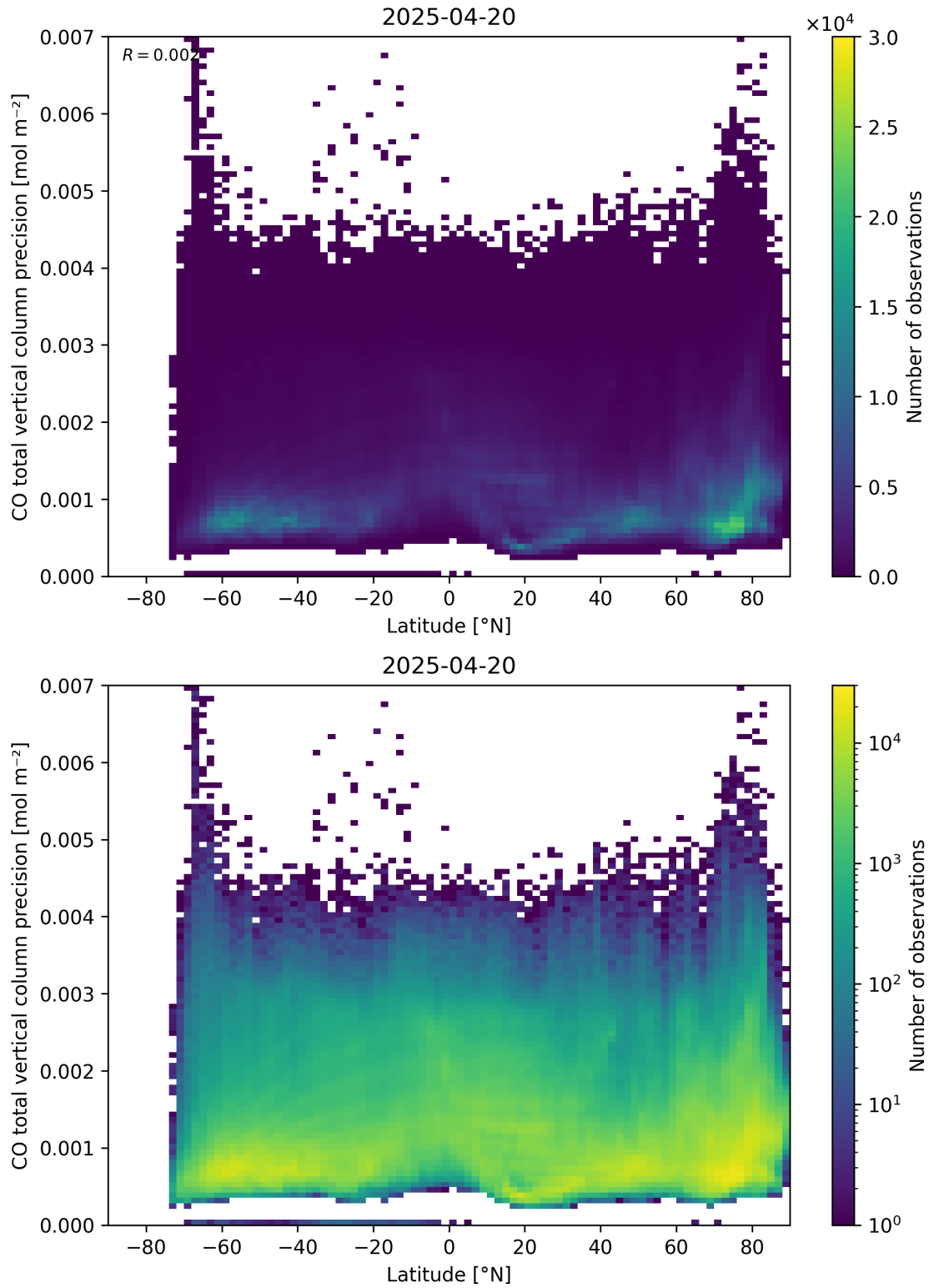
Figure 53: Scatter density plot of “Latitude” against “CO total vertical column precision” for 2025-04-19 to 2025-04-21.
