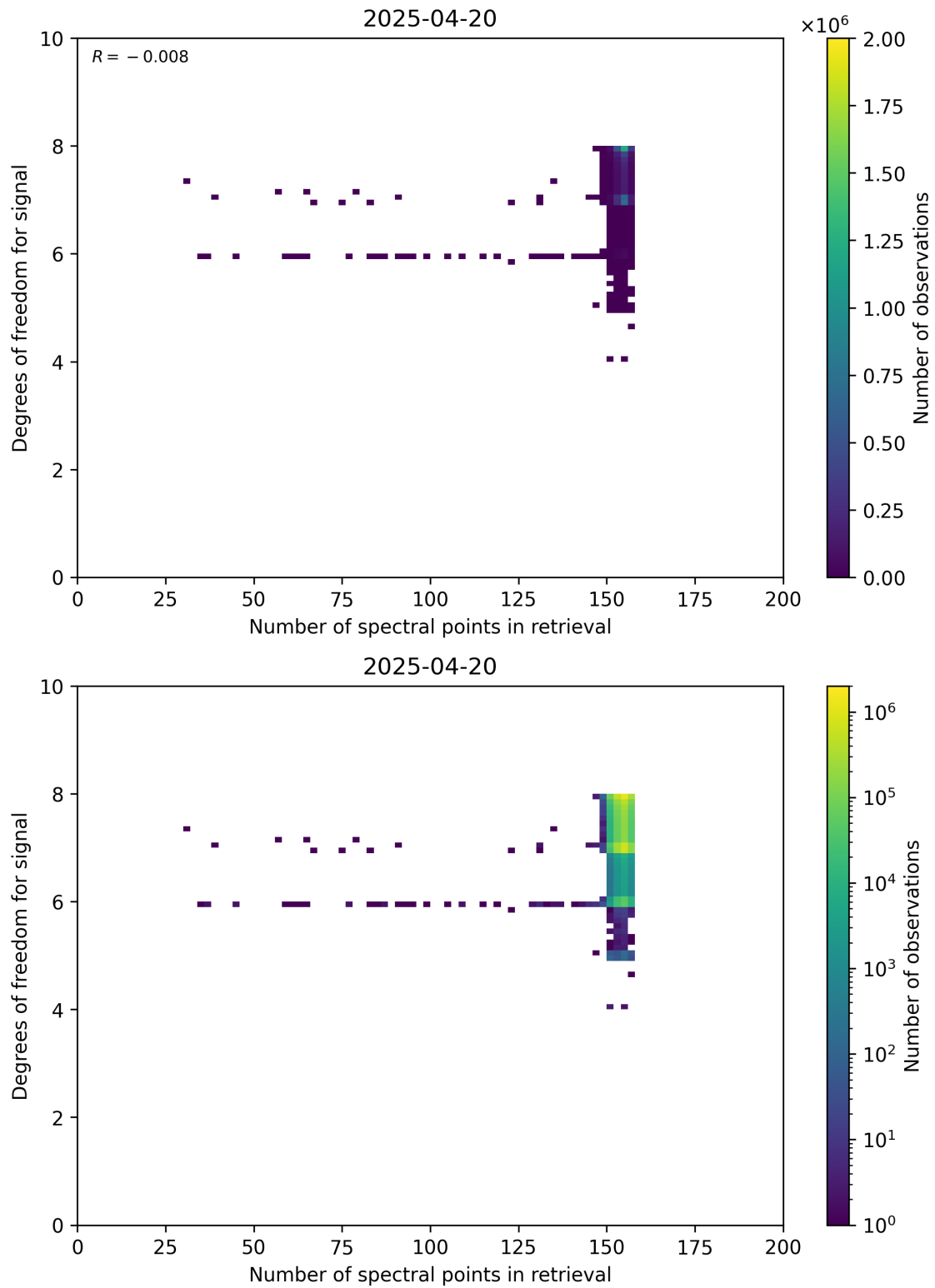
Figure 59: Scatter density plot of “Number of spectral points in retrieval” against “Degrees of freedom for signal” for 2025-04-19 to 2025-04-21.
