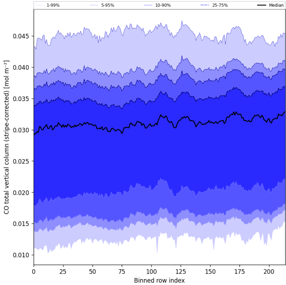
Figure 27: Along track statistics of “CO total vertical column (stripe-corrected)” for 2025-04-19 to 2025-04-21
