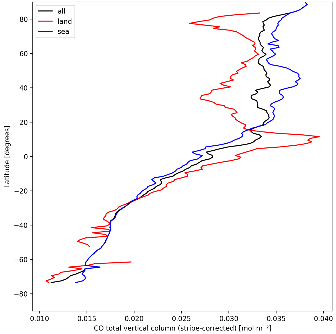
Figure 11: Zonal average of “CO total vertical column (stripe-corrected)” for 2025-04-19 to 2025-04-21.
