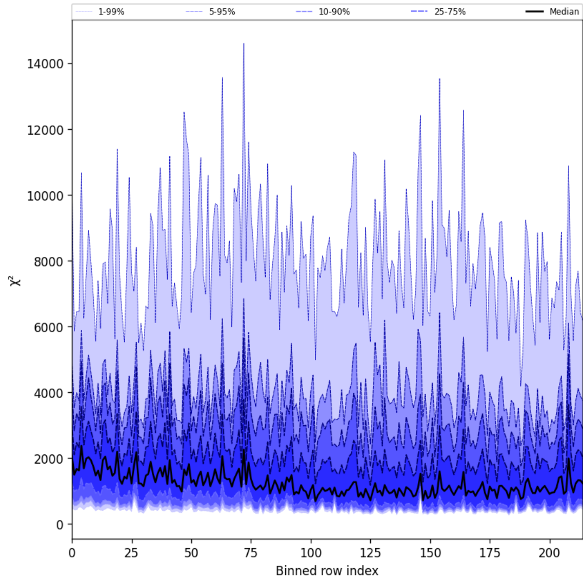
Figure 30: Along track statistics of “ \chi^2 ” for 2025-04-19 to 2025-04-21
