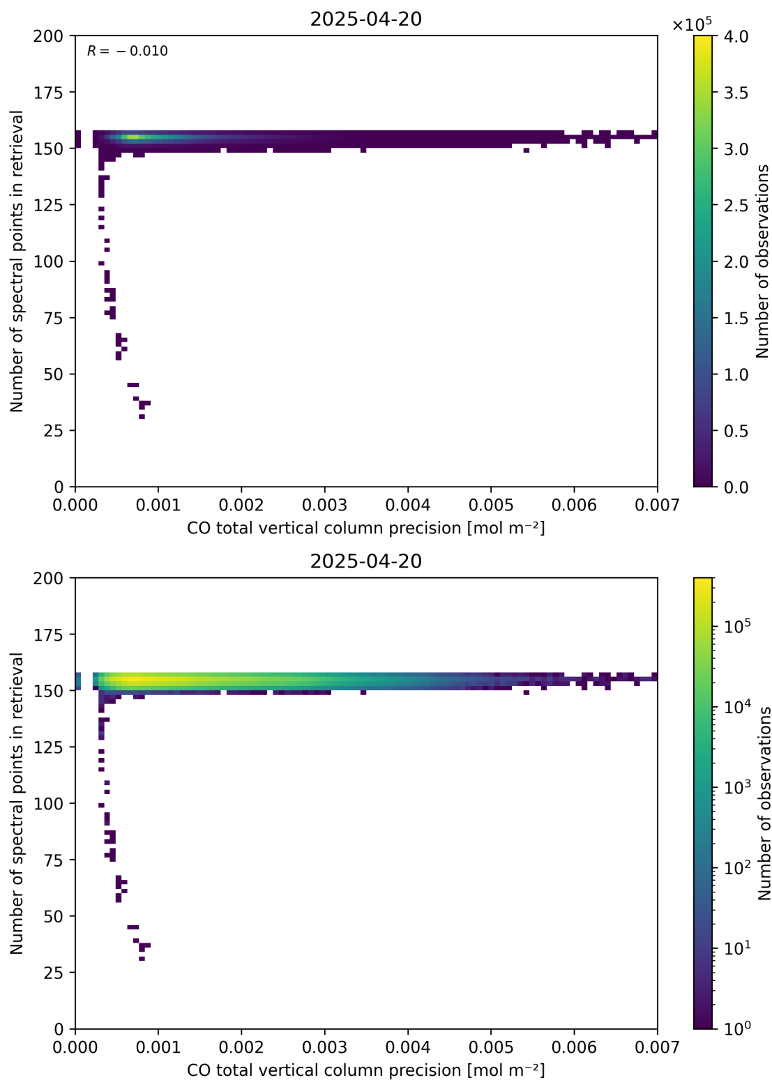
Figure 47: Scatter density plot of “CO total vertical column precision” against “Number of spectral points in retrieval” for 2025-04-19 to 2025-04-21.
