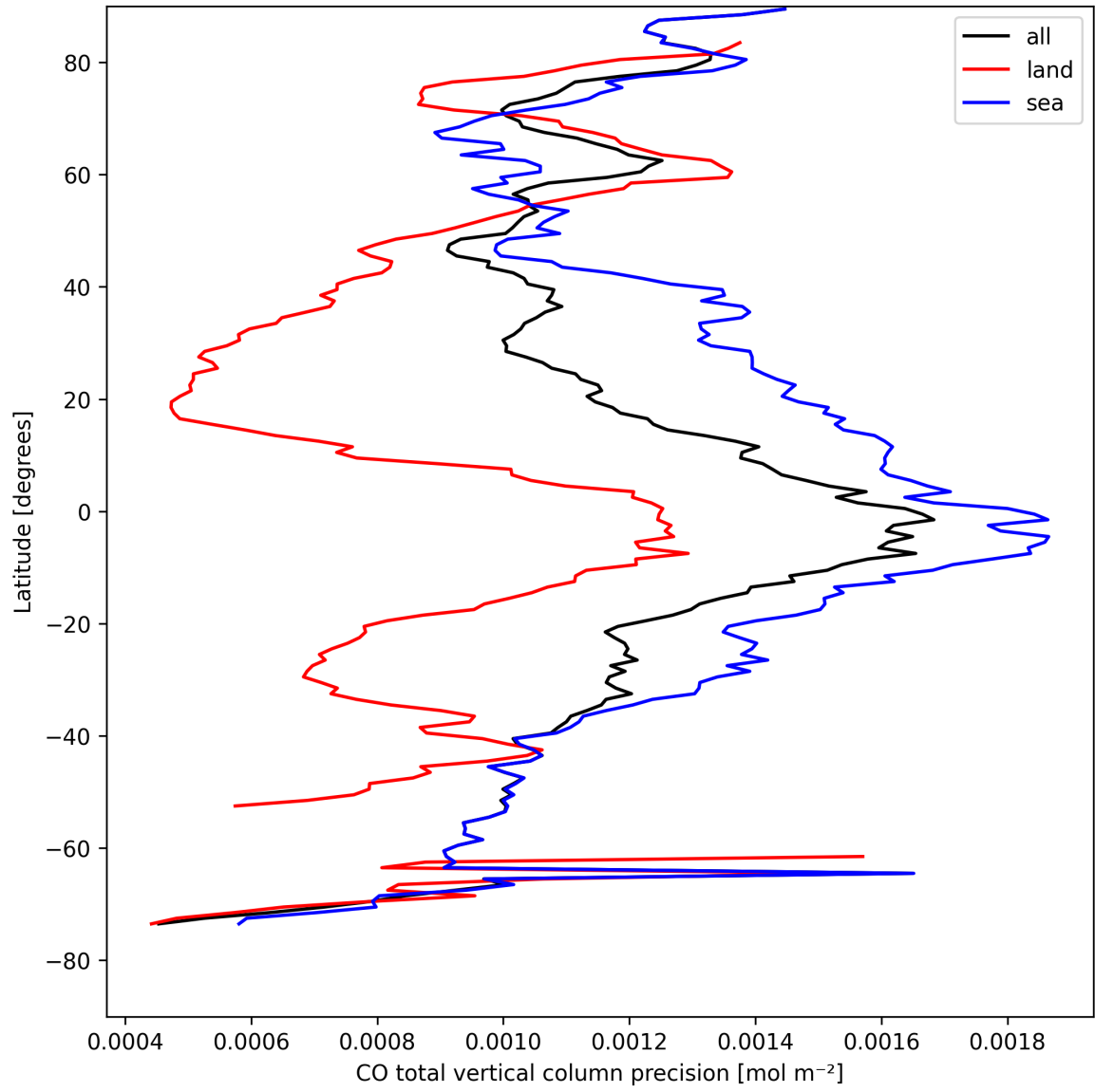
Figure 12: Zonal average of “CO total vertical column precision” for 2025-04-19 to 2025-04-21.
