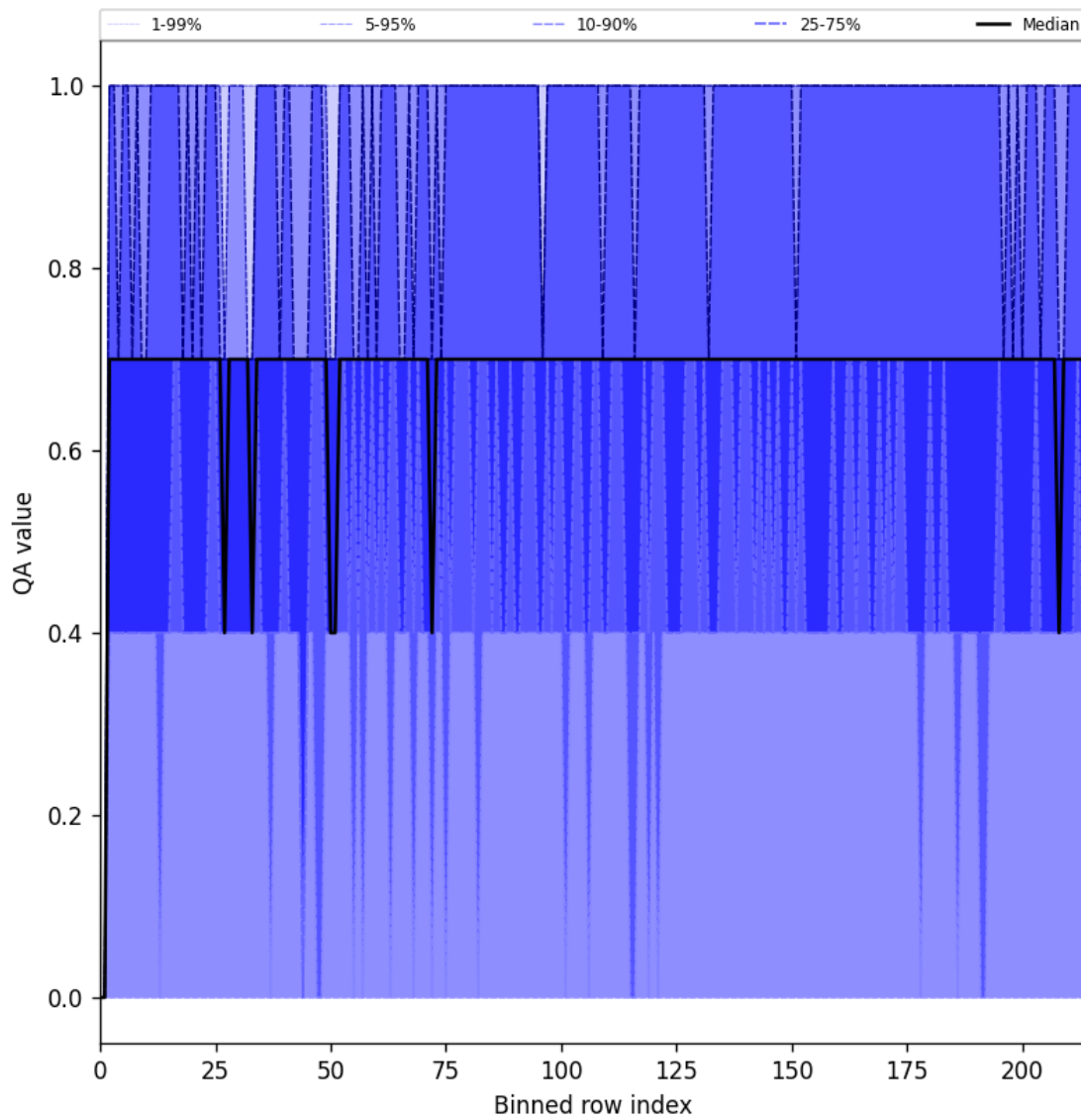
Figure 25: Along track statistics of “QA value” for 2025-04-19 to 2025-04-21
