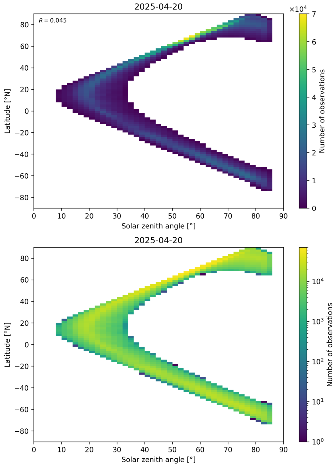
Figure 66: Scatter density plot of “Solar zenith angle” against “Latitude” for 2025-04-19 to 2025-04-21.
