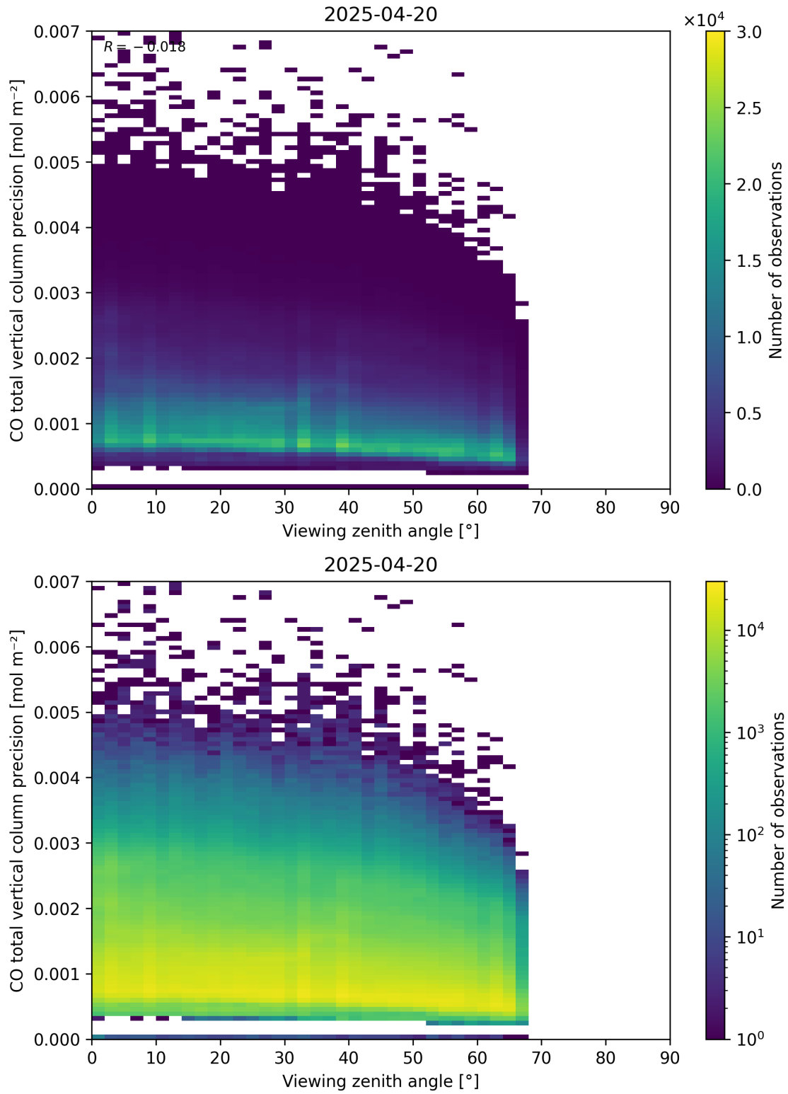
Figure 71: Scatter density plot of “Viewing zenith angle” against “CO total vertical column precision” for 2025-04-19 to 2025-04-21.
