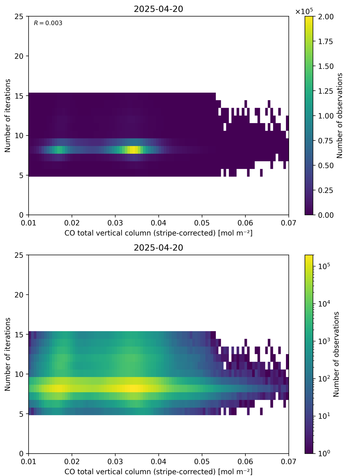
Figure 39: Scatter density plot of “CO total vertical column (stripe-corrected)” against “Number of iterations” for 2025-04-19 to 2025-04-21.
