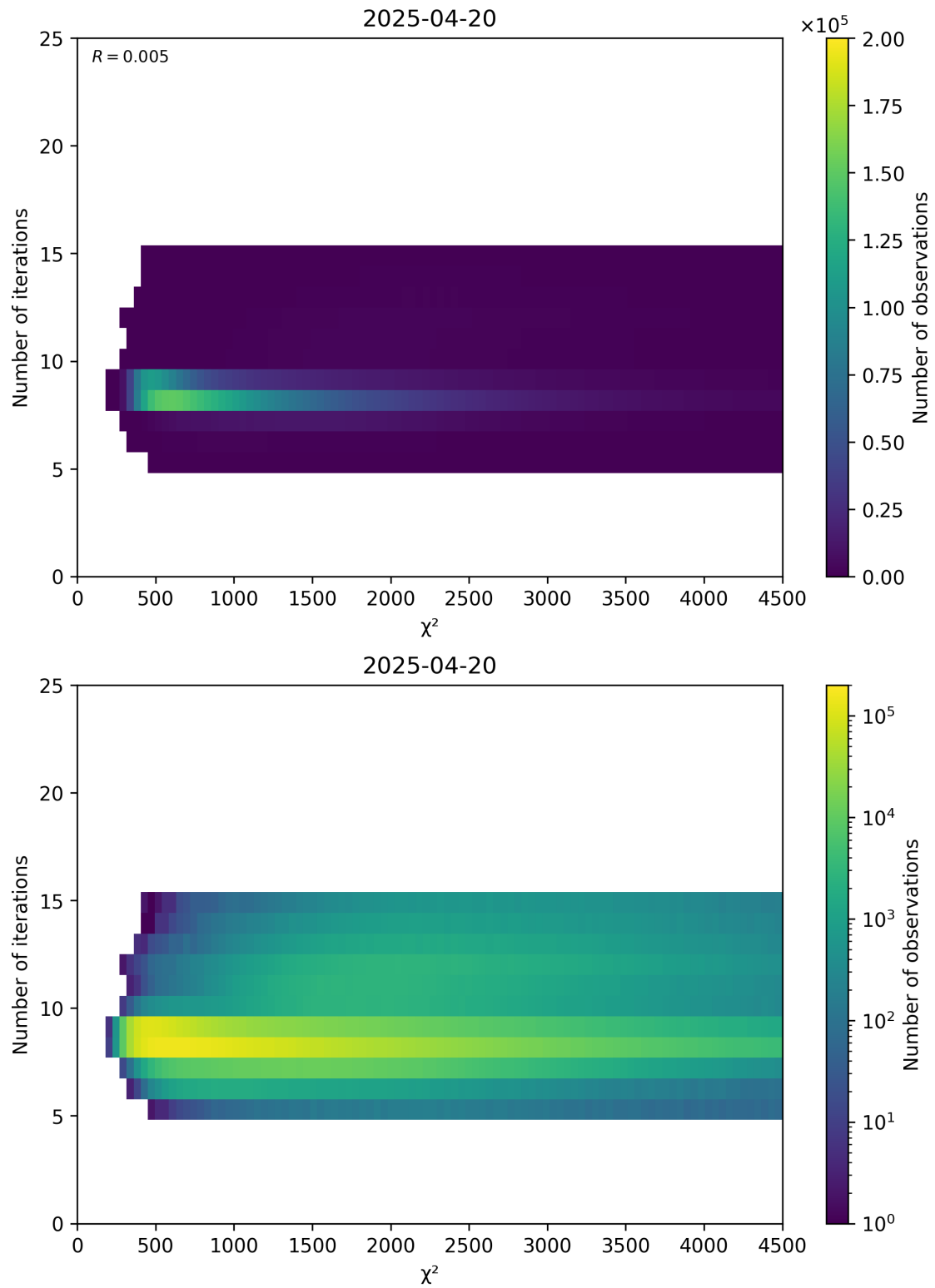
Figure 49: Scatter density plot of “ \chi^2 ” against “Number of iterations” for 2025-04-19 to 2025-04-21.
