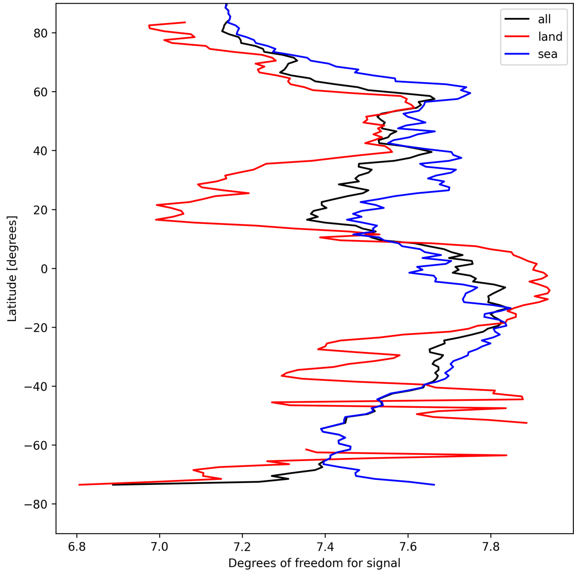
Figure 15: Zonal average of “Degrees of freedom for signal” for 2025-04-19 to 2025-04-21.
