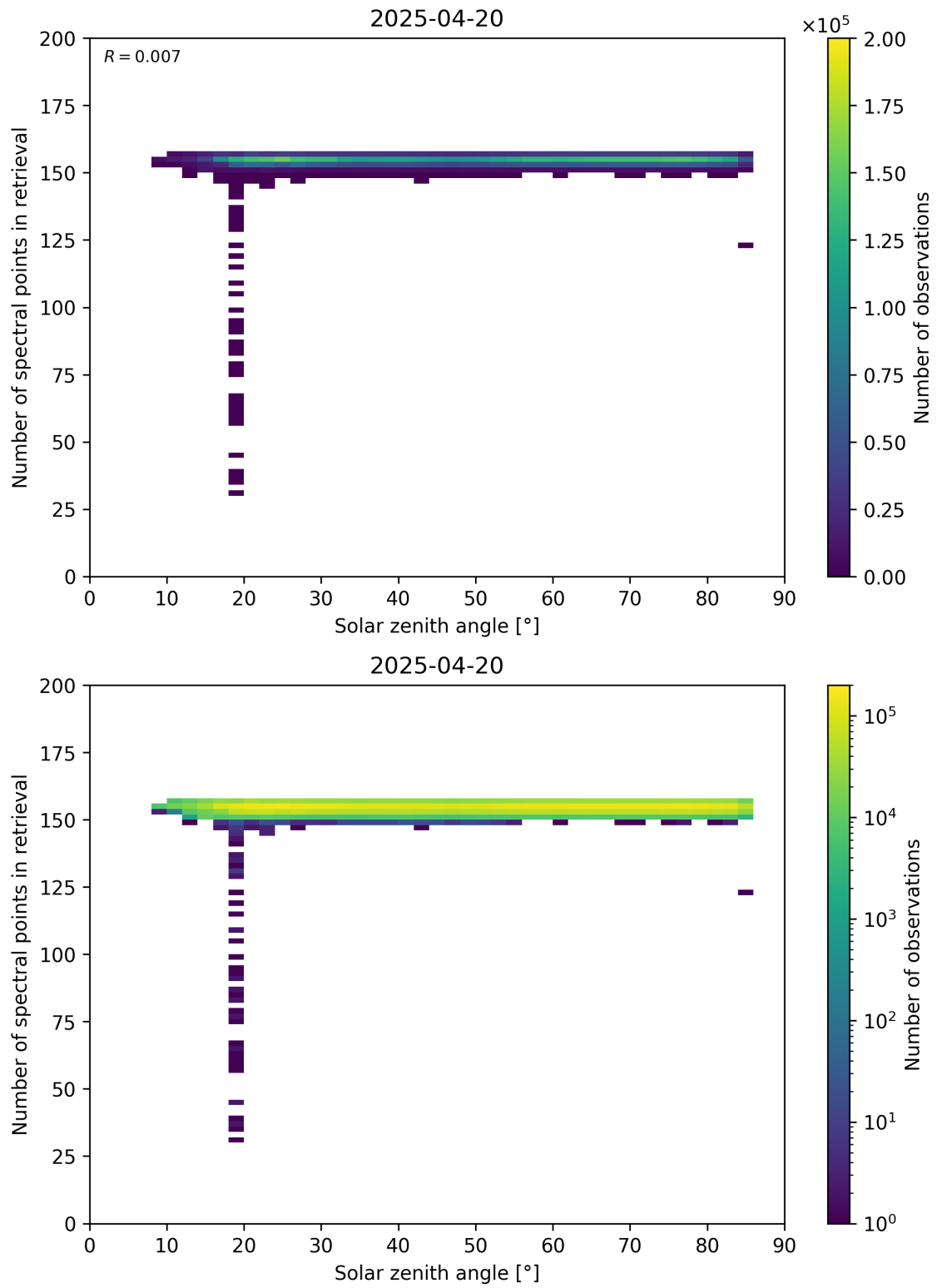
Figure 68: Scatter density plot of “Solar zenith angle” against “Number of spectral points in retrieval” for 2025-04-19 to 2025-04-21.
