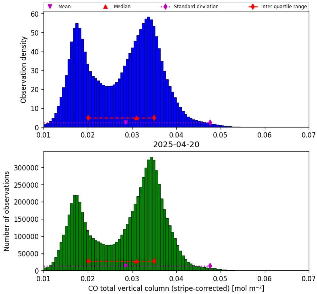
Figure 19: Histogram of “CO total vertical column (stripe-corrected)” for 2025-04-19 to 2025-04-21
