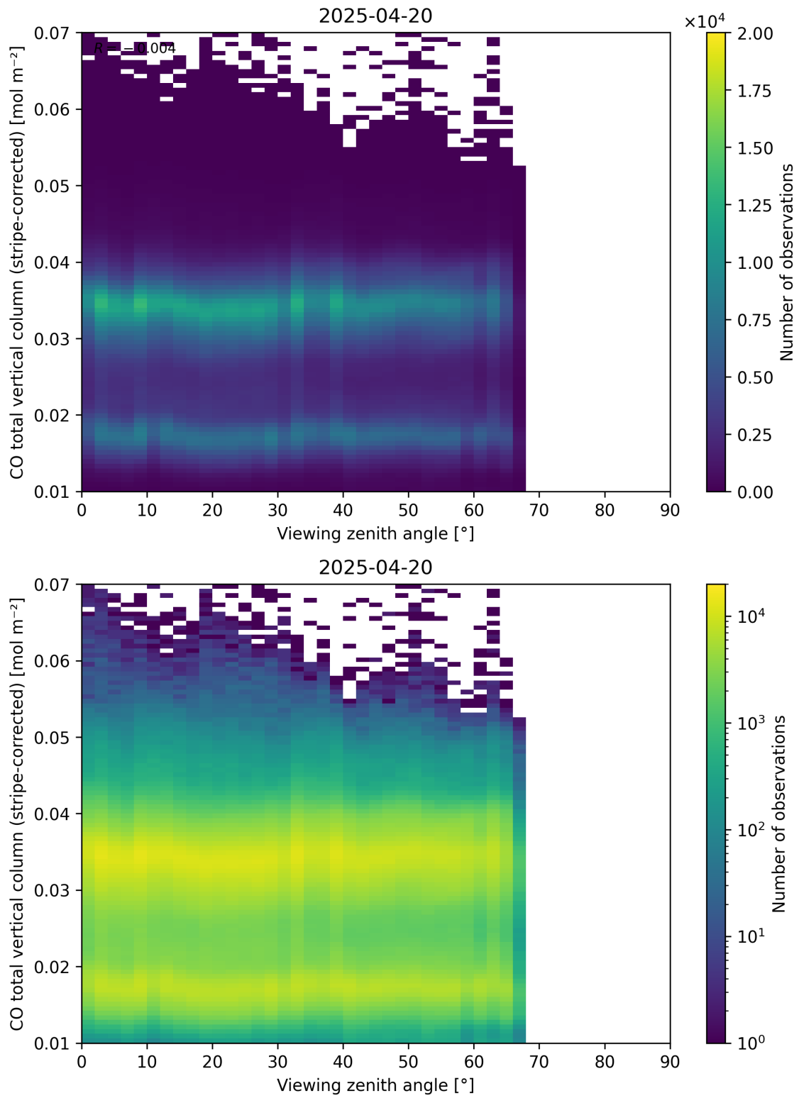
Figure 70: Scatter density plot of “Viewing zenith angle” against “CO total vertical column (stripe-corrected)” for 2025-04-19 to 2025-04-21.
