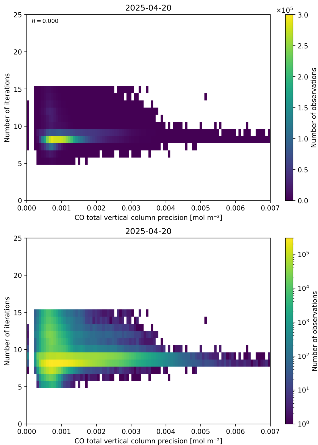
Figure 46: Scatter density plot of “CO total vertical column precision” against “Number of iterations” for 2025-04-19 to 2025-04-21.
