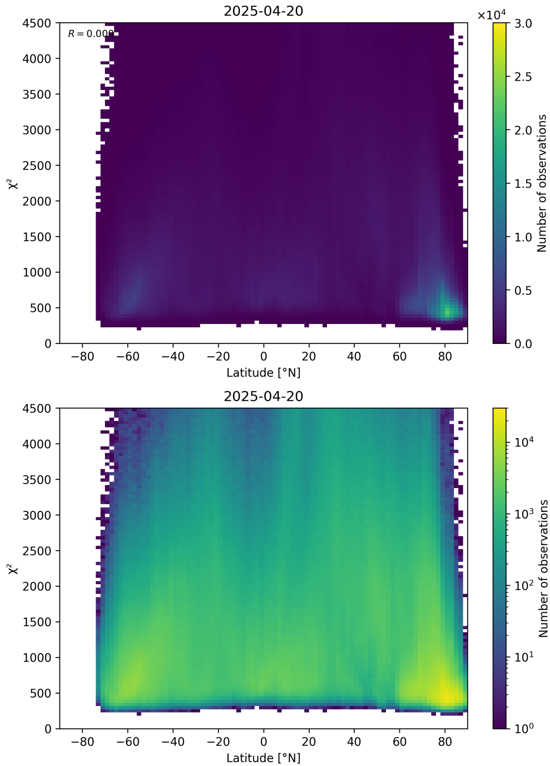
Figure 54: Scatter density plot of “Latitude” against “ \chi^2 ” for 2025-04-19 to 2025-04-21.
