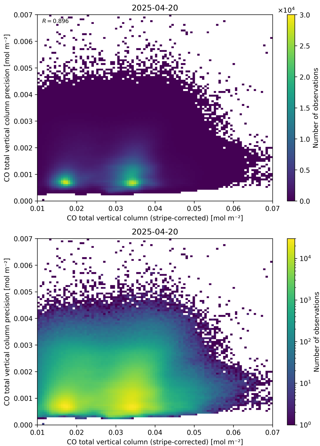
Figure 36: Scatter density plot of “CO total vertical column (stripe-corrected)” against “CO total vertical column precision” for 2025-04-19 to 2025-04-21.
