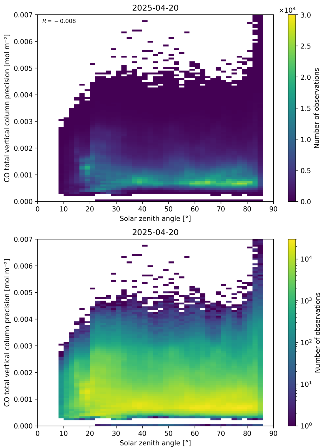
Figure 63: Scatter density plot of “Solar zenith angle” against “CO total vertical column precision” for 2025-04-19 to 2025-04-21.
