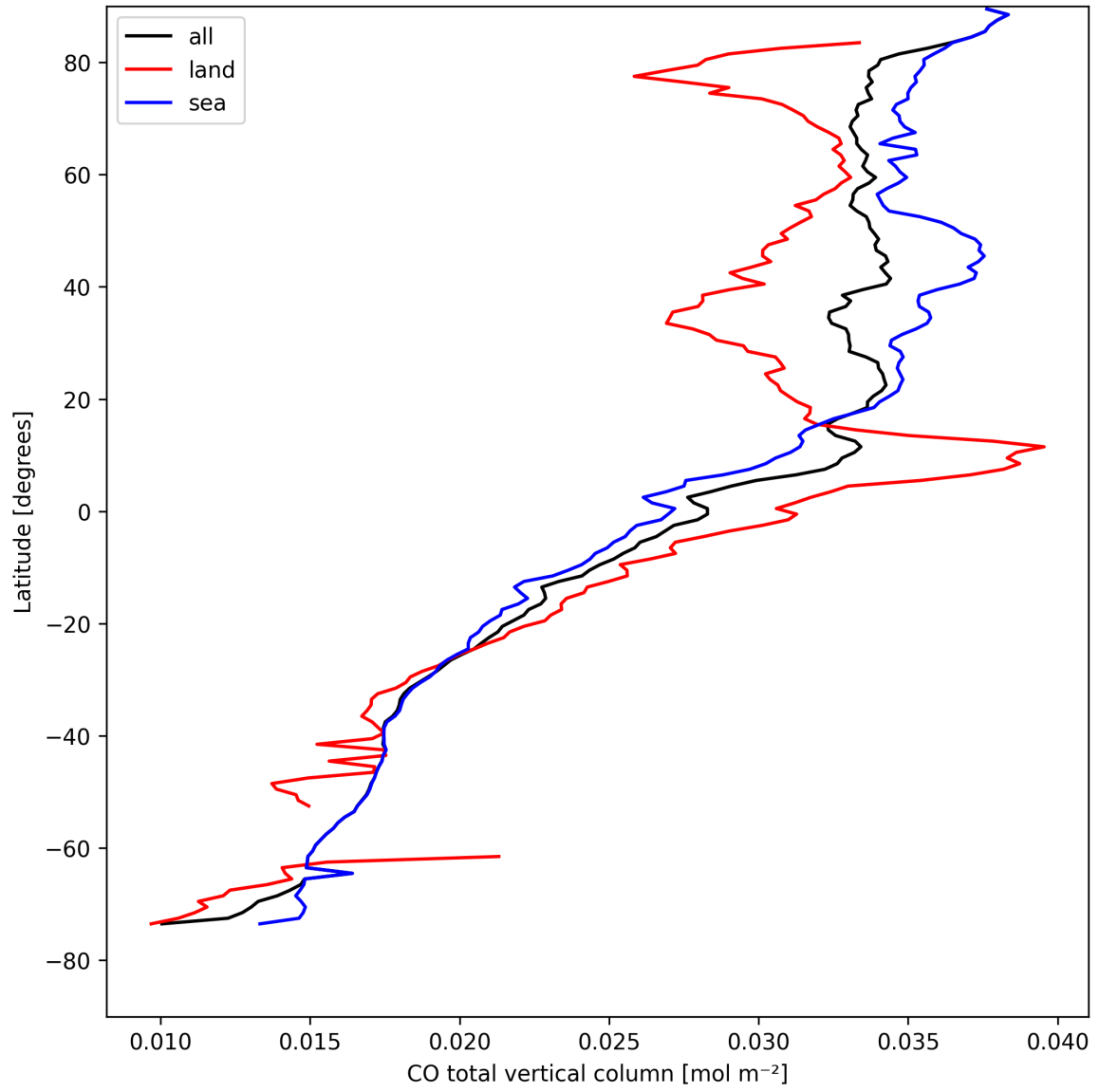
Figure 10: Zonal average of “CO total vertical column” for 2025-04-19 to 2025-04-21.
