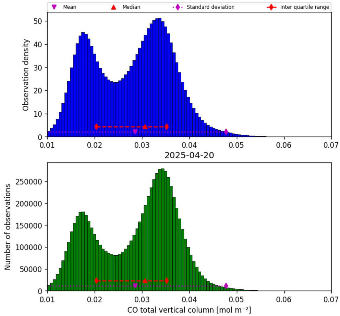
Figure 18: Histogram of “CO total vertical column” for 2025-04-19 to 2025-04-21
