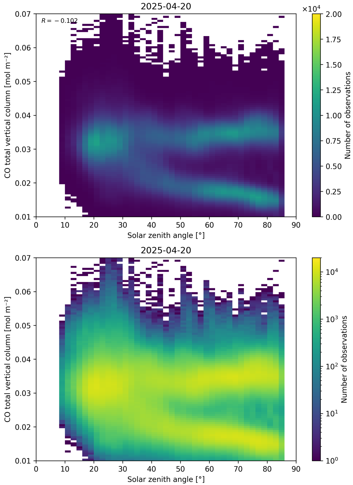
Figure 61: Scatter density plot of “Solar zenith angle” against “CO total vertical column” for 2025-04-19 to 2025-04-21.
