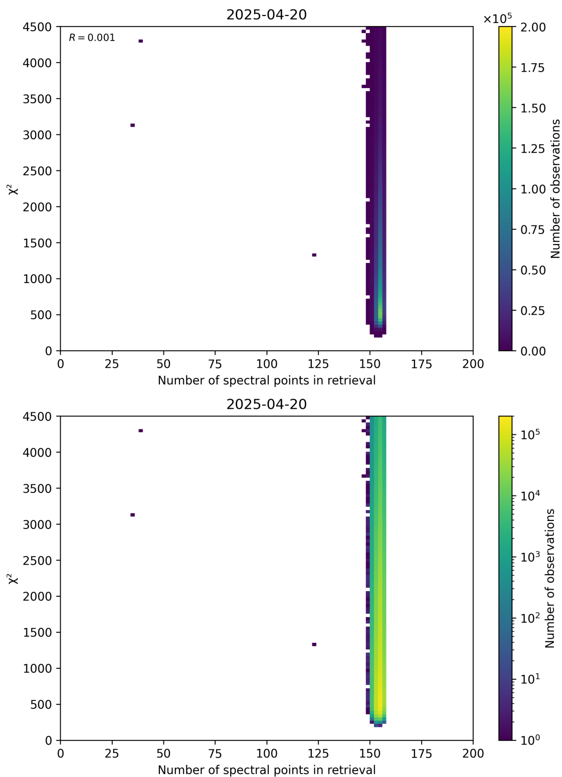
Figure 58: Scatter density plot of “Number of spectral points in retrieval” against “ \chi^2 ” for 2025-04-19 to 2025-04-21.
