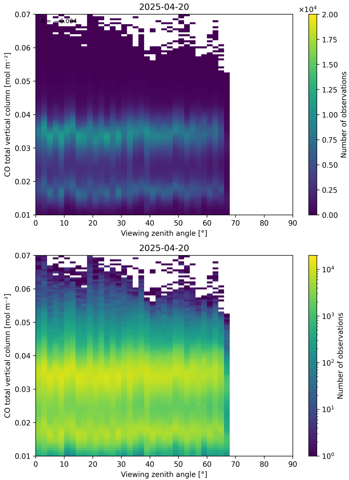
Figure 69: Scatter density plot of “Viewing zenith angle” against “CO total vertical column” for 2025-04-19 to 2025-04-21.
