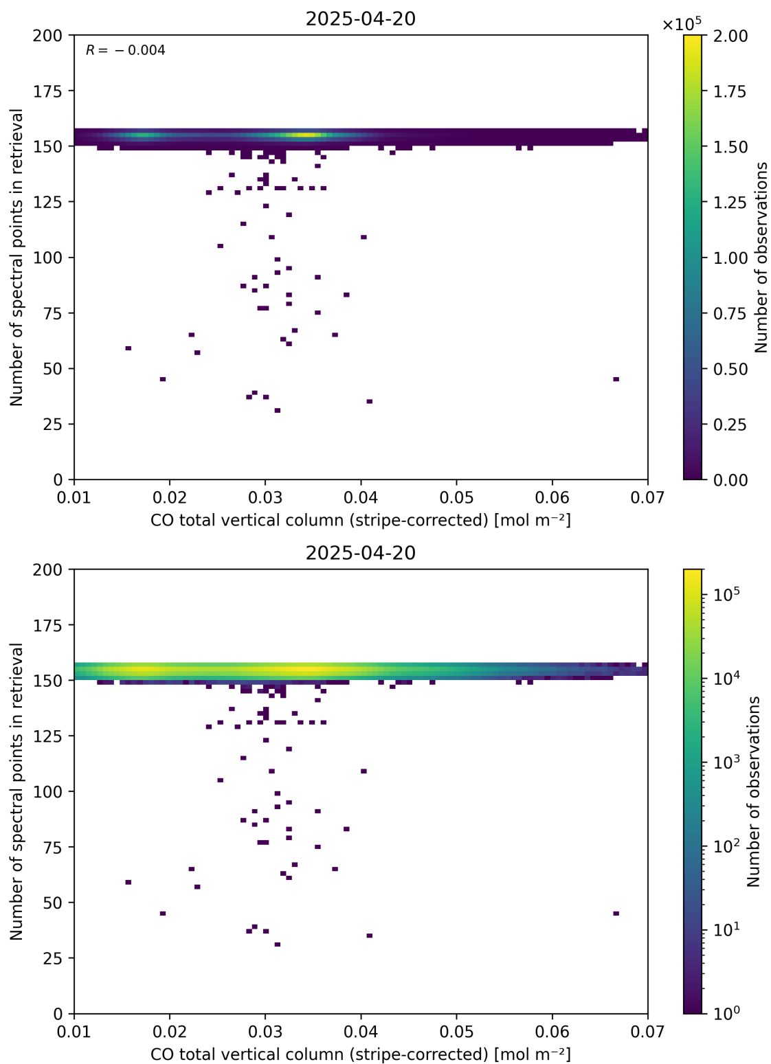
Figure 40: Scatter density plot of “CO total vertical column (stripe-corrected)” against “Number of spectral points in retrieval” for 2025-04-19 to 2025-04-21.
