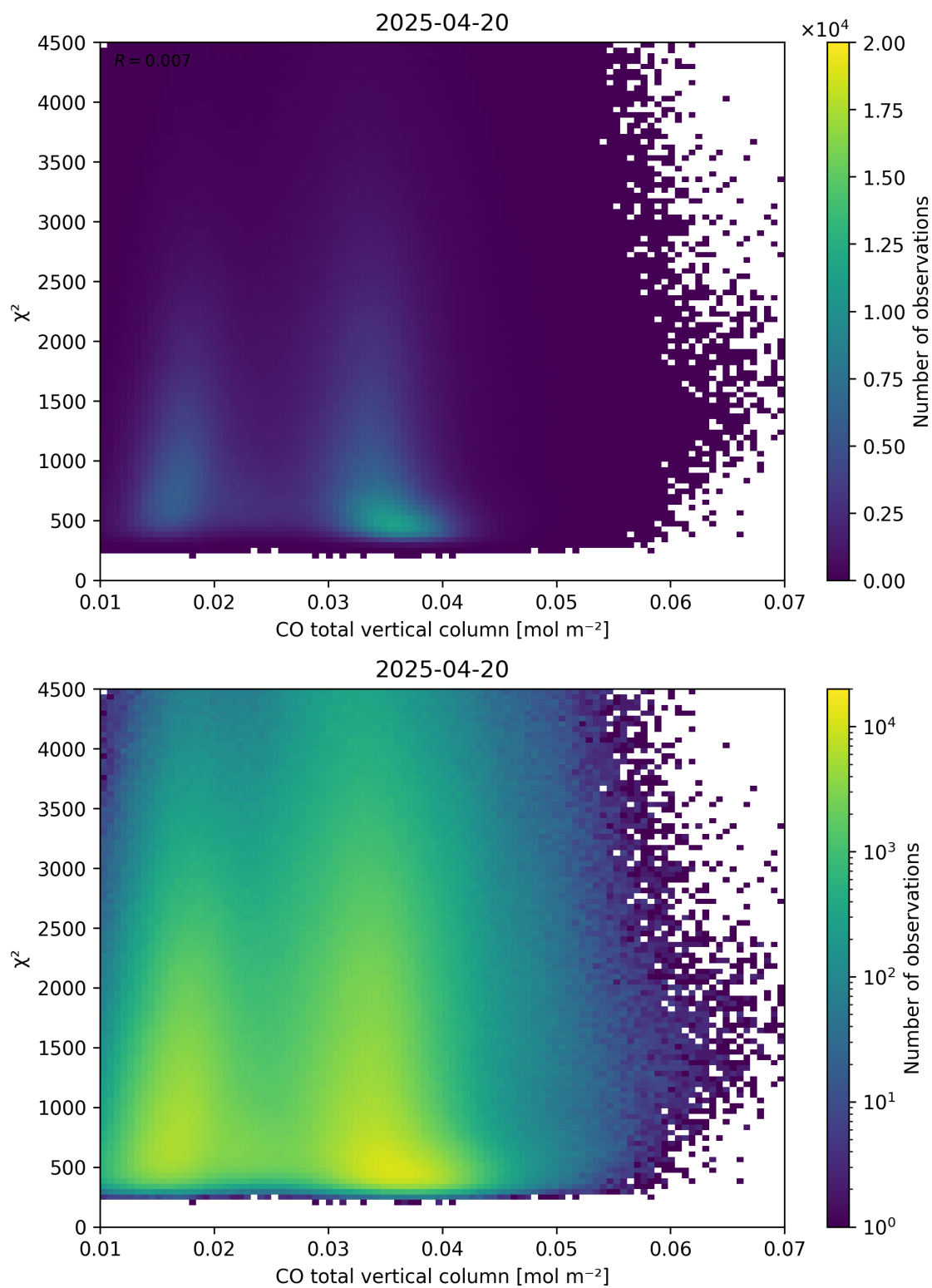
Figure 35: Scatter density plot of “CO total vertical column” against “ \chi^2 ” for 2025-04-19 to 2025-04-21.
