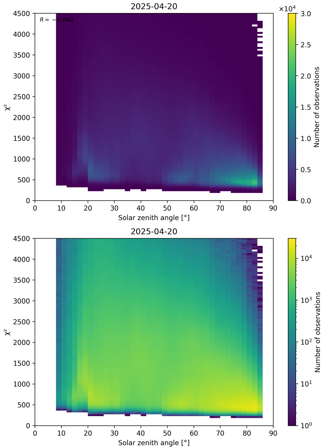
Figure 64: Scatter density plot of “Solar zenith angle” against “ \chi^2 ” for 2025-04-19 to 2025-04-21.
