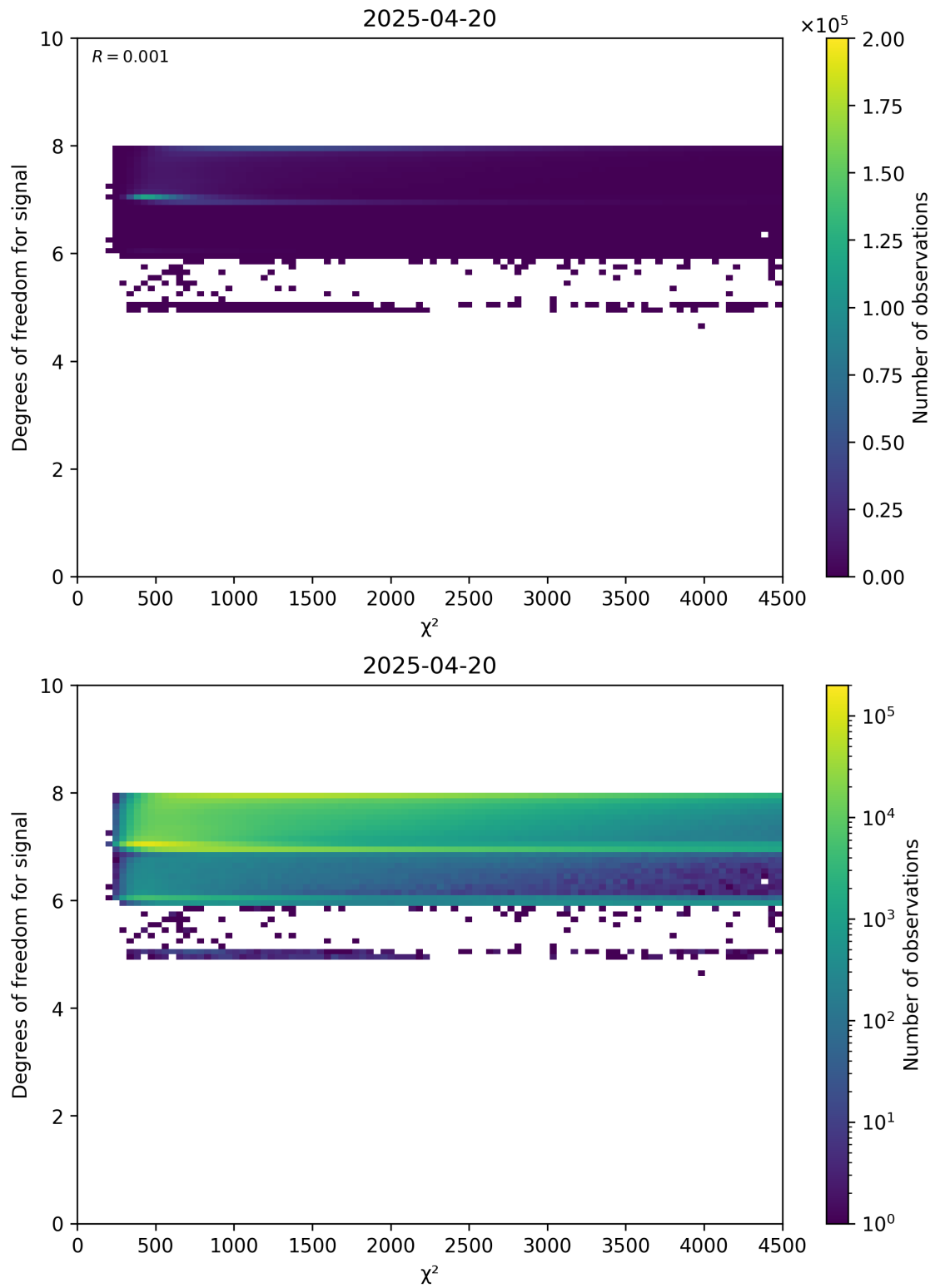
Figure 48: Scatter density plot of “ \chi^2 ” against “Degrees of freedom for signal” for 2025-04-19 to 2025-04-21.
