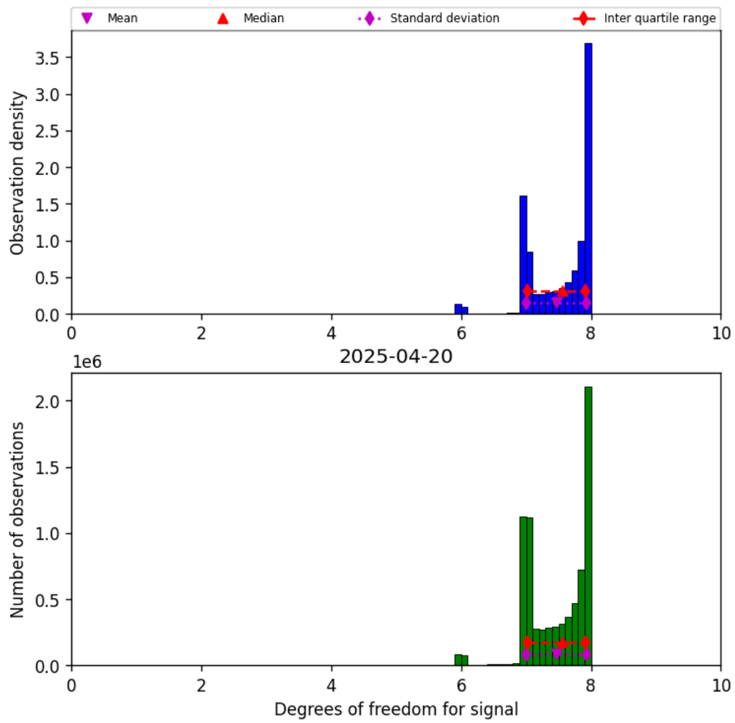
Figure 23: Histogram of “Degrees of freedom for signal” for 2025-04-19 to 2025-04-21
