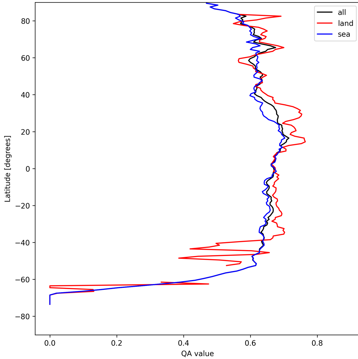
Figure 9: Zonal average of “QA value” for 2025-04-19 to 2025-04-21.
