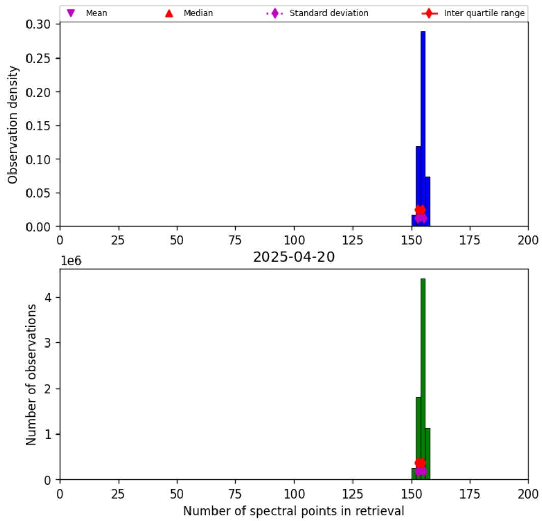
Figure 21: Histogram of “Number of spectral points in retrieval” for 2025-04-19 to 2025-04-21
