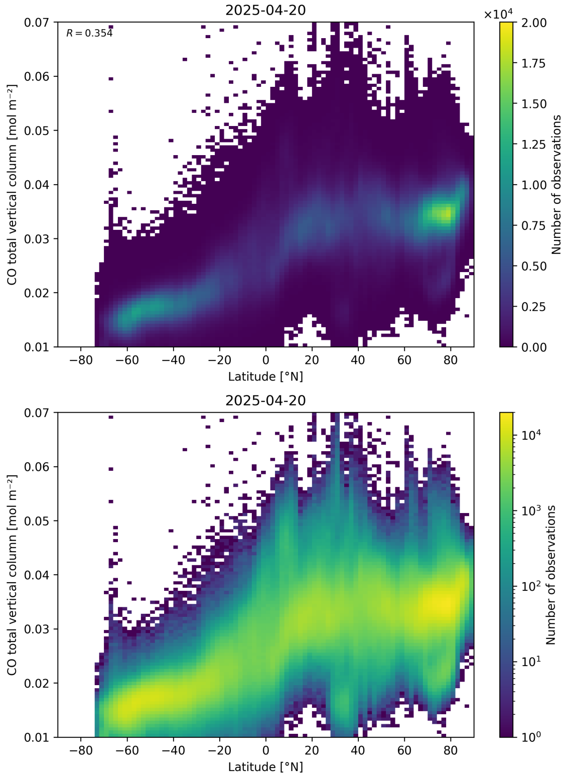
Figure 51: Scatter density plot of “Latitude” against “CO total vertical column” for 2025-04-19 to 2025-04-21.
