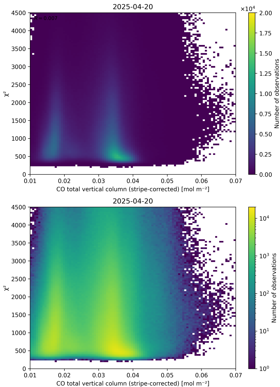
Figure 37: Scatter density plot of “CO total vertical column (stripe-corrected)” against “ \chi^2 ” for 2025-04-19 to 2025-04-21.
