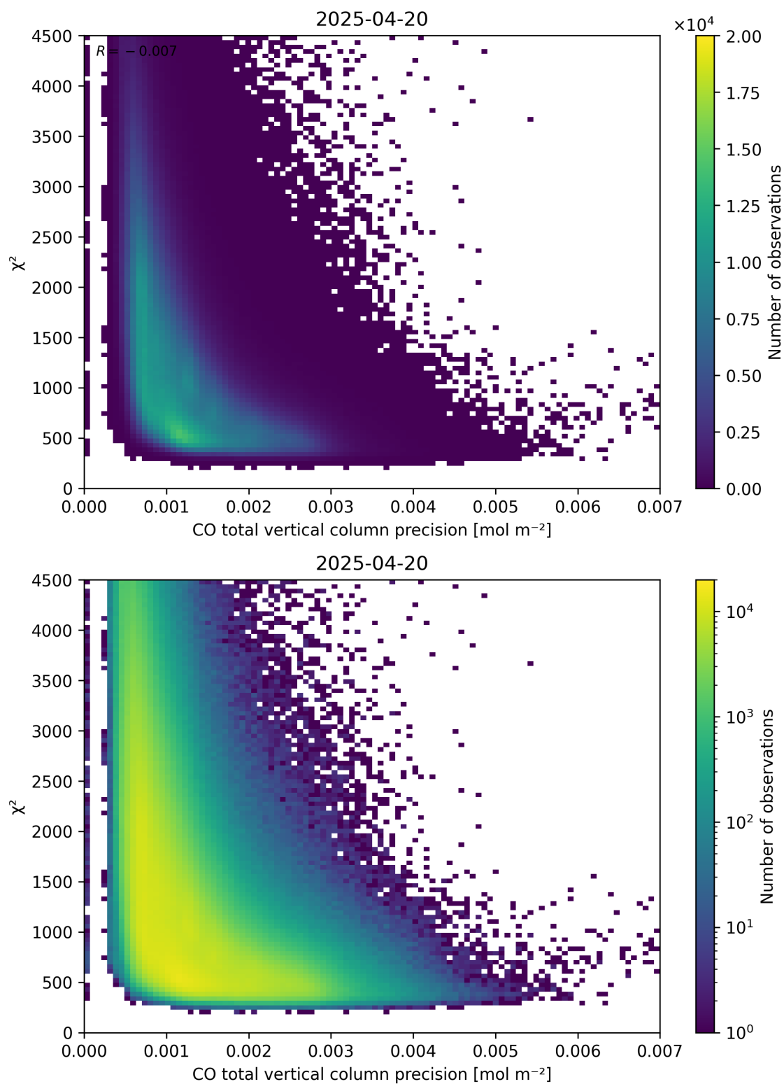
Figure 44: Scatter density plot of “CO total vertical column precision” against “ \chi^2 ” for 2025-04-19 to 2025-04-21.
