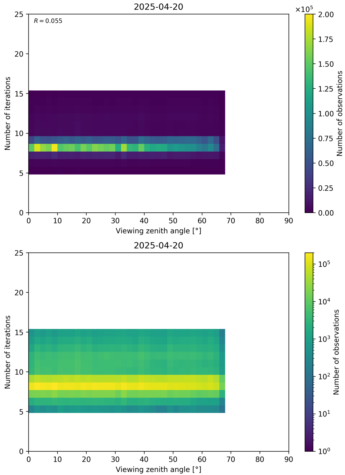
Figure 75: Scatter density plot of “Viewing zenith angle” against “Number of iterations” for 2025-04-19 to 2025-04-21.
