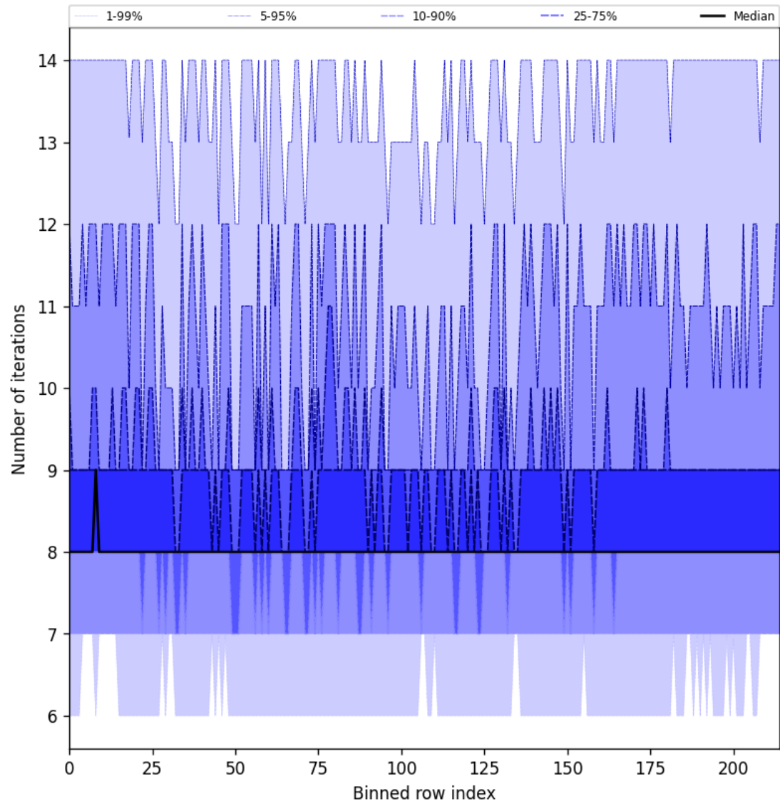
Figure 32: Along track statistics of “Number of iterations” for 2025-04-19 to 2025-04-21
