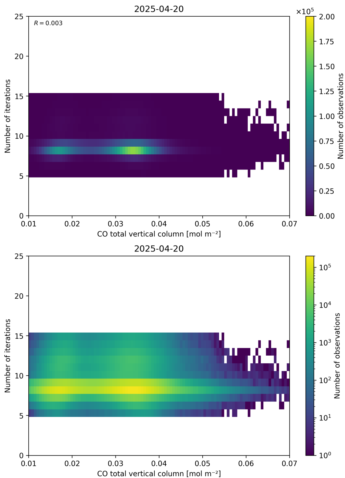
Figure 42: Scatter density plot of “CO total vertical column” against “Number of iterations” for 2025-04-19 to 2025-04-21.
