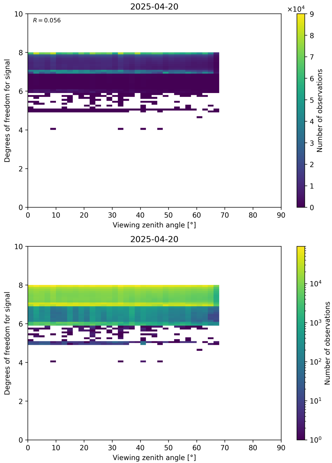
Figure 73: Scatter density plot of “Viewing zenith angle” against “Degrees of freedom for signal” for 2025-04-19 to 2025-04-21.
