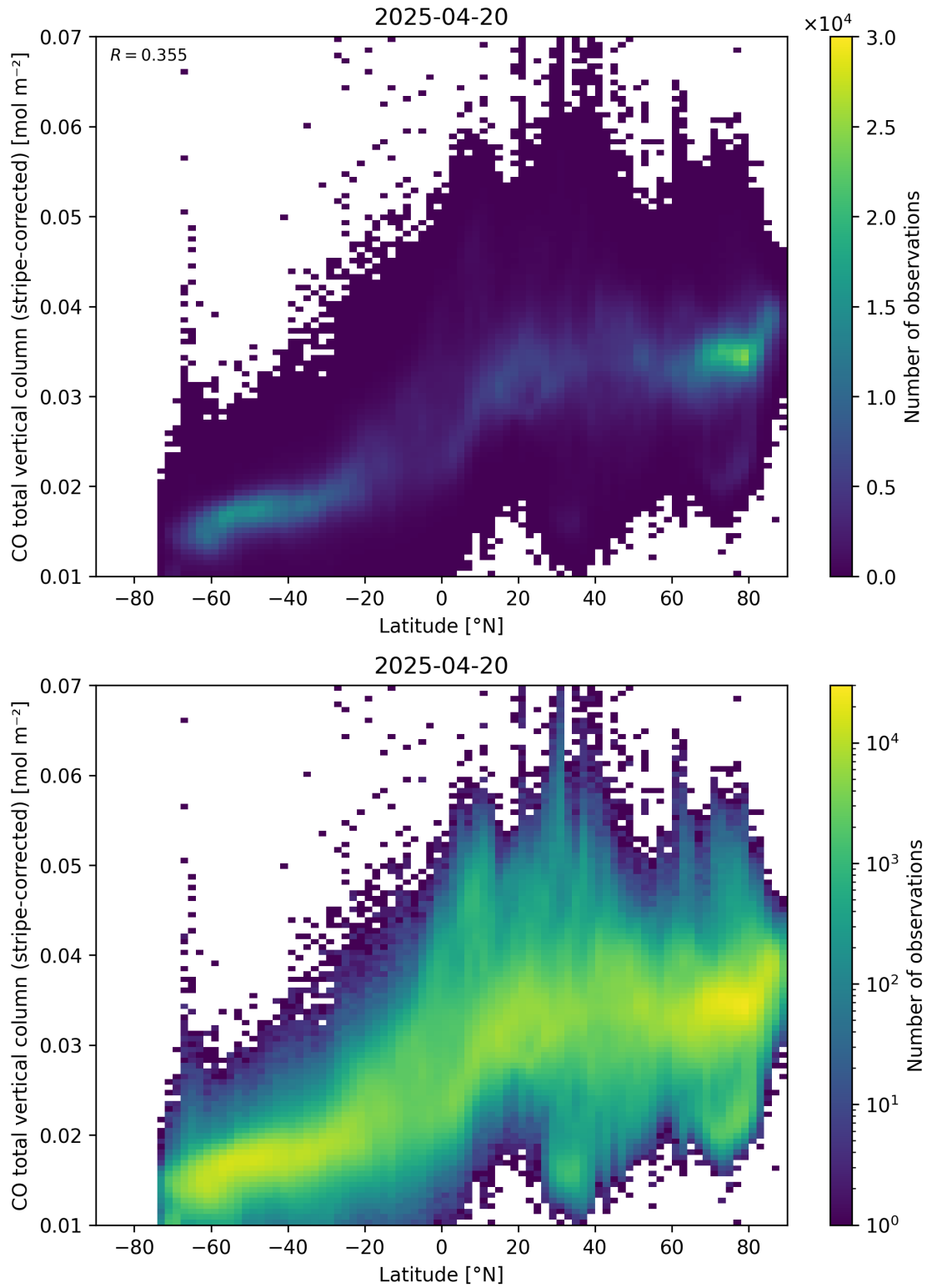
Figure 52: Scatter density plot of “Latitude” against “CO total vertical column (stripe-corrected)” for 2025-04-19 to 2025-04-21.
