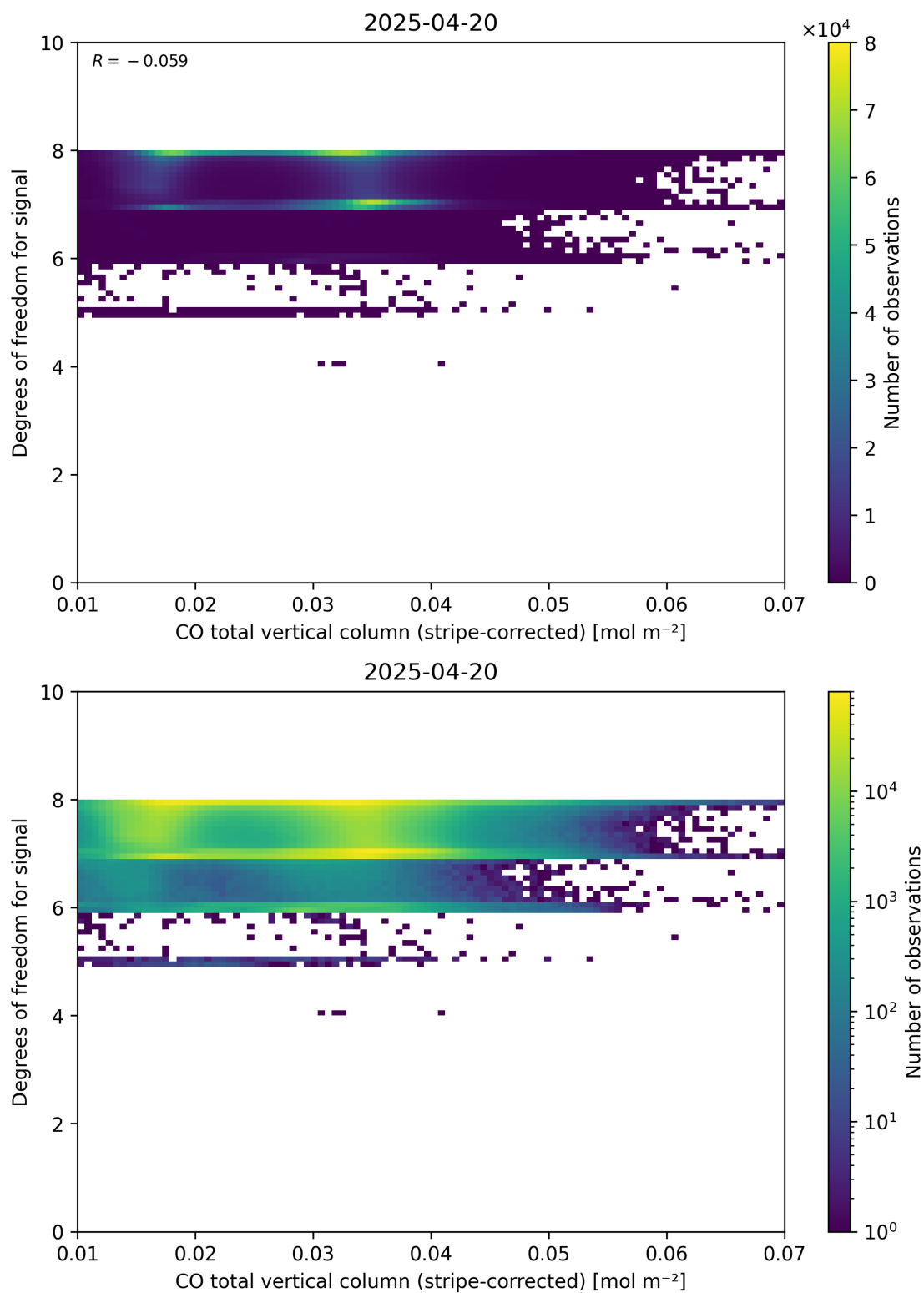
Figure 38: Scatter density plot of “CO total vertical column (stripe-corrected)” against “Degrees of freedom for signal” for 2025-04-19 to 2025-04-21.
