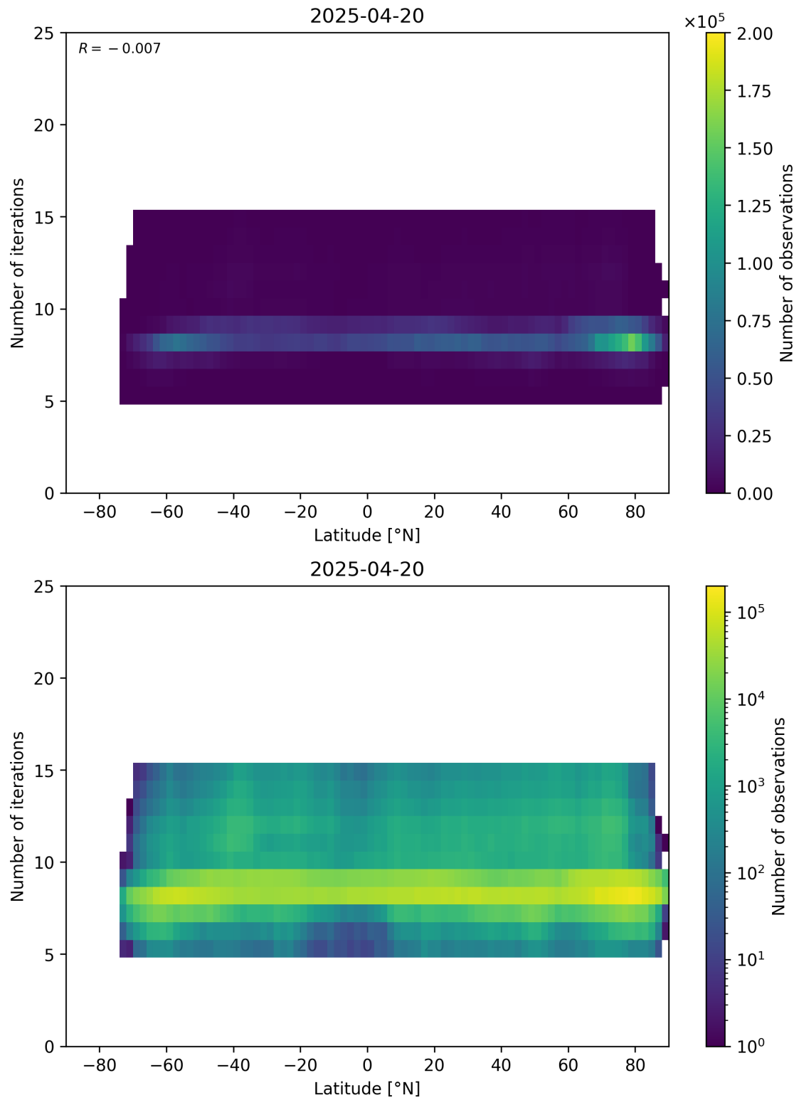
Figure 56: Scatter density plot of “Latitude” against “Number of iterations” for 2025-04-19 to 2025-04-21.
