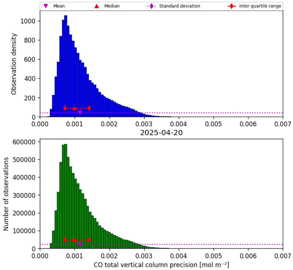
Figure 20: Histogram of “CO total vertical column precision” for 2025-04-19 to 2025-04-21
