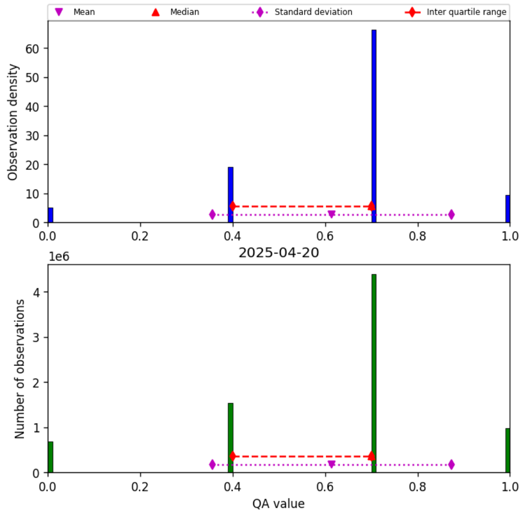
Figure 17: Histogram of “QA value” for 2025-04-19 to 2025-04-21
