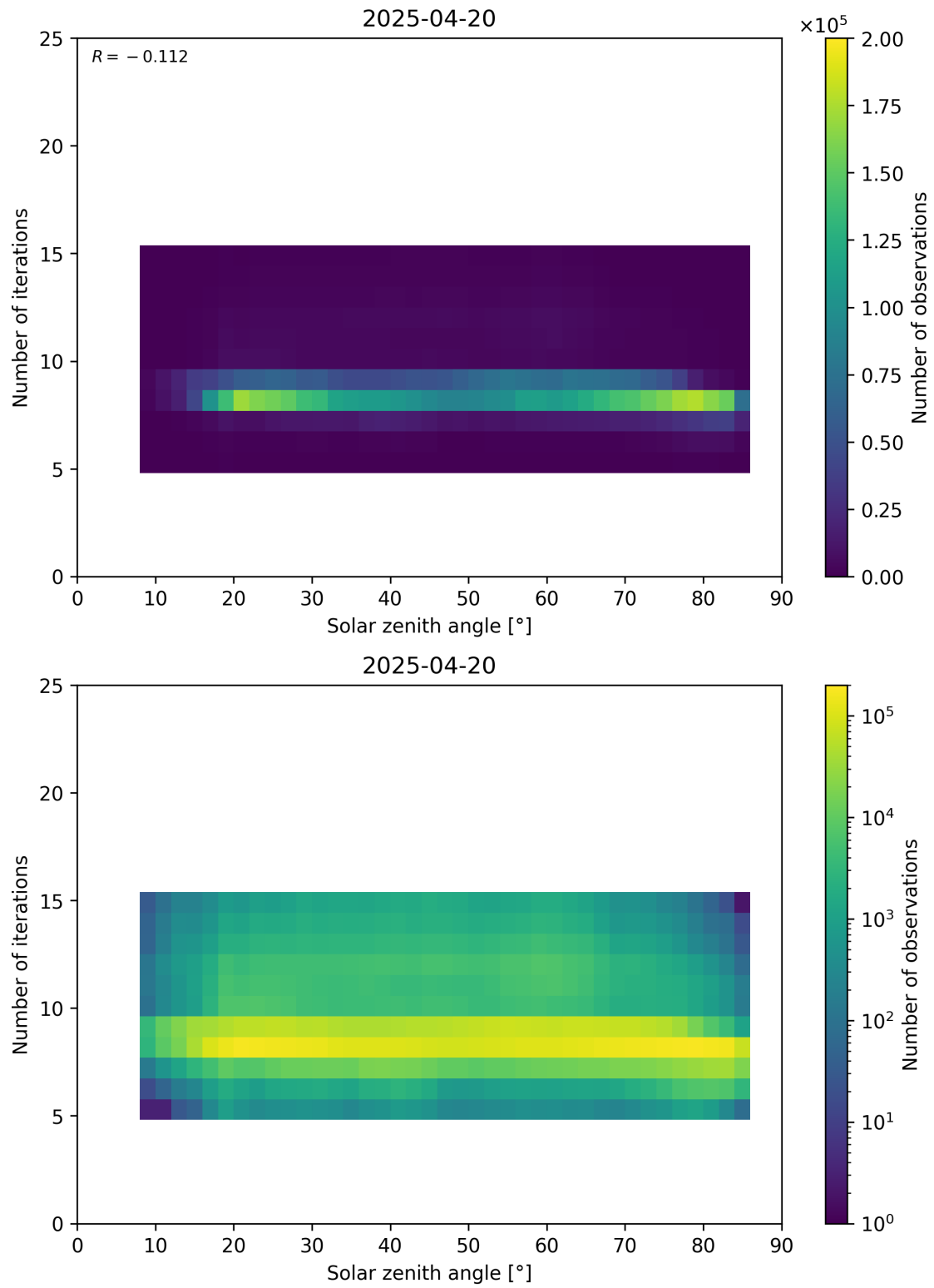
Figure 67: Scatter density plot of “Solar zenith angle” against “Number of iterations” for 2025-04-19 to 2025-04-21.
