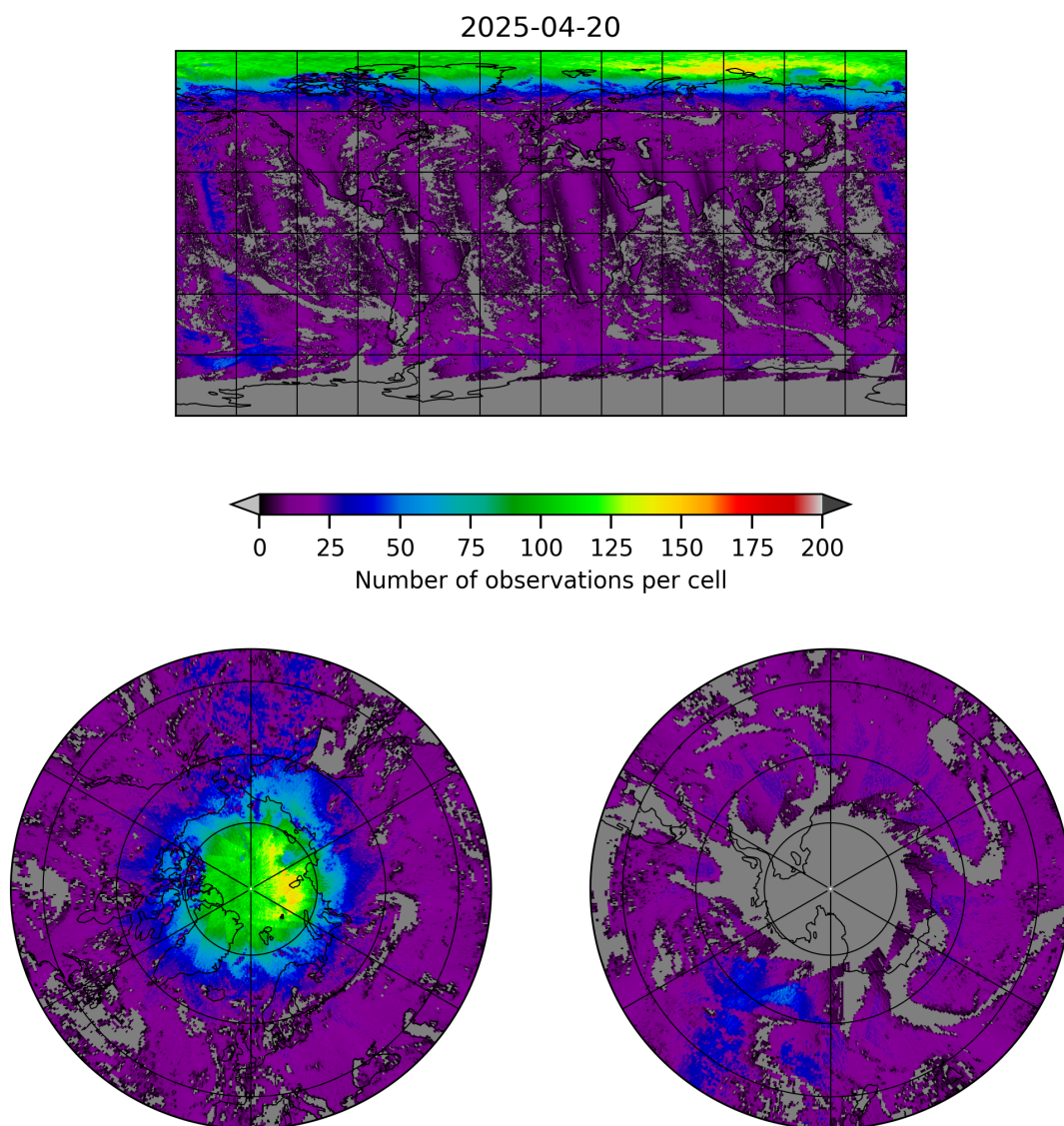
Figure 8: Map of the number of observations for 2025-04-19 to 2025-04-21
