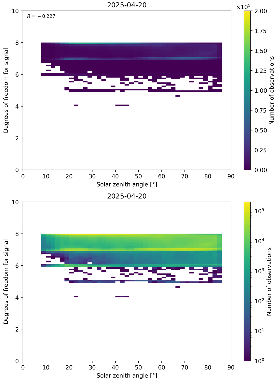
Figure 65: Scatter density plot of “Solar zenith angle” against “Degrees of freedom for signal” for 2025-04-19 to 2025-04-21.
