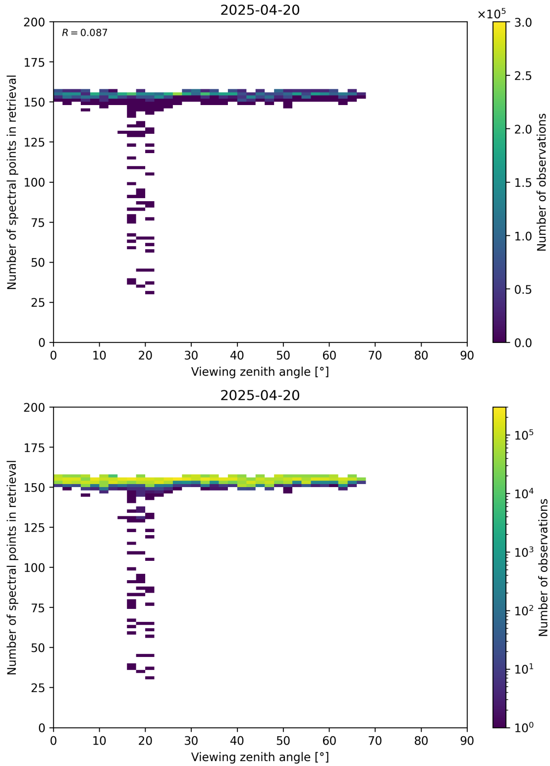
Figure 76: Scatter density plot of “Viewing zenith angle” against “Number of spectral points in retrieval” for 2025-04-19 to 2025-04-21.
