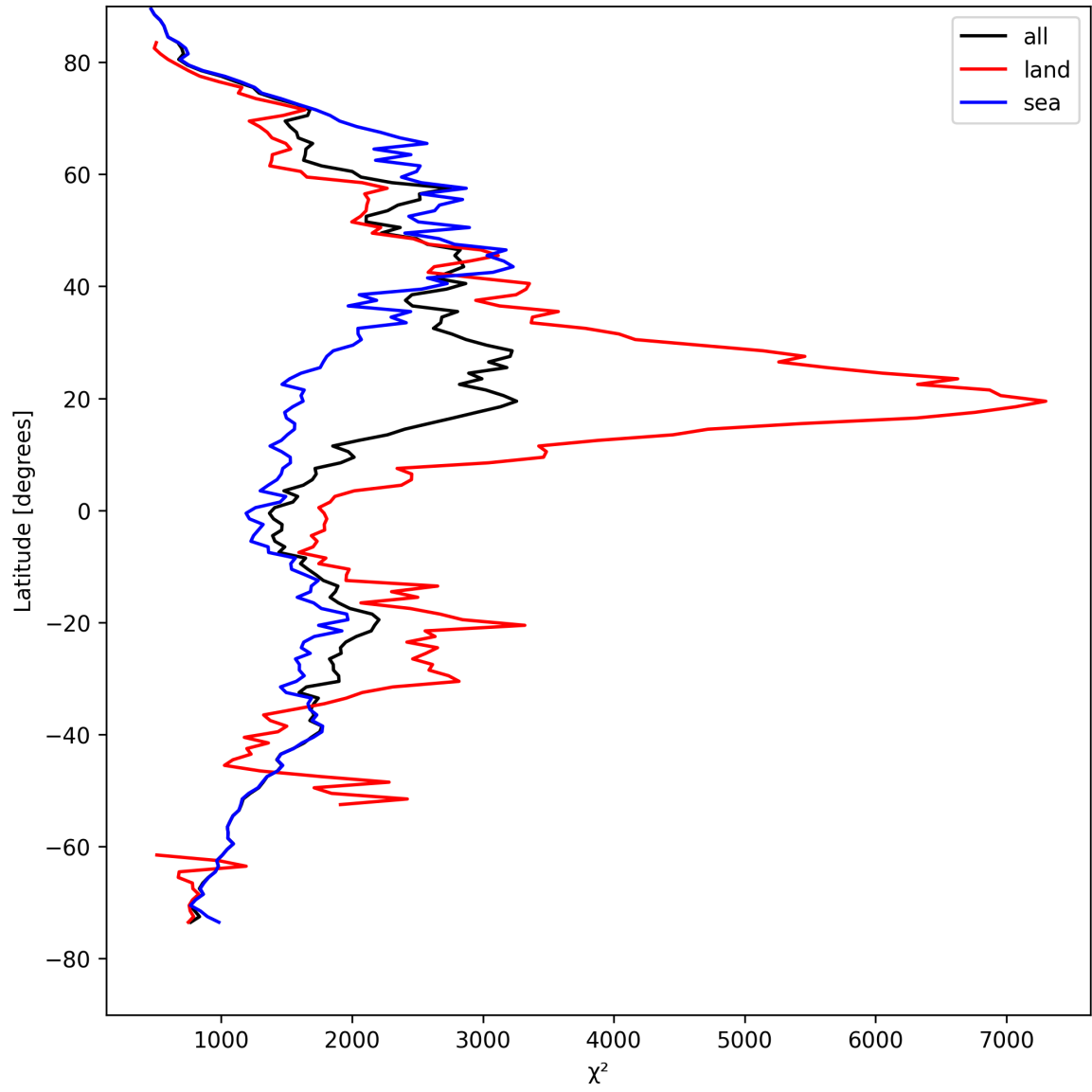
Figure 14: Zonal average of “ \chi^2 ” for 2025-04-19 to 2025-04-21.
