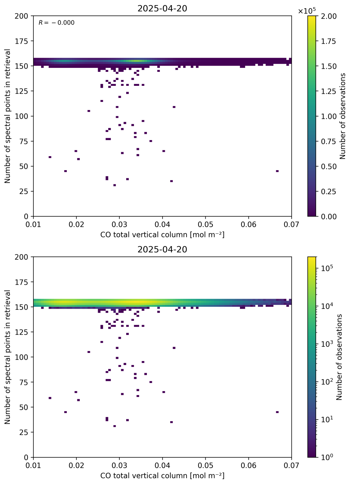
Figure 43: Scatter density plot of “CO total vertical column” against “Number of spectral points in retrieval” for 2025-04-19 to 2025-04-21.
