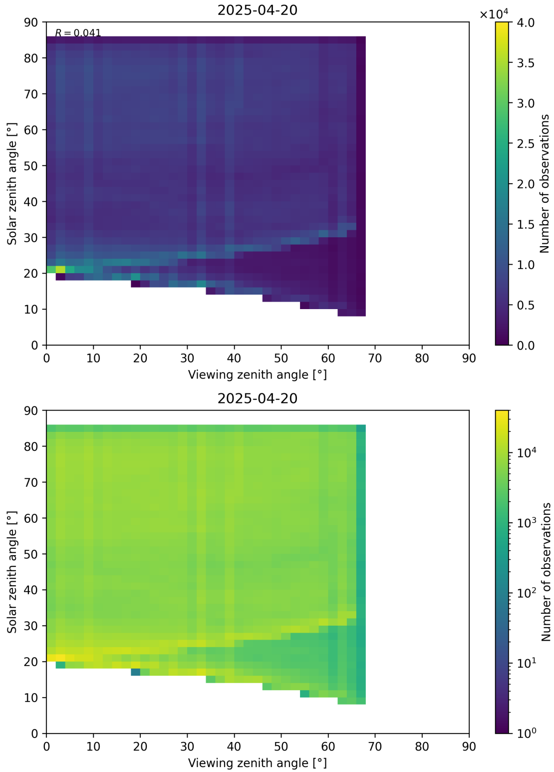
Figure 77: Scatter density plot of “Viewing zenith angle” against “Solar zenith angle” for 2025-04-19 to 2025-04-21.
