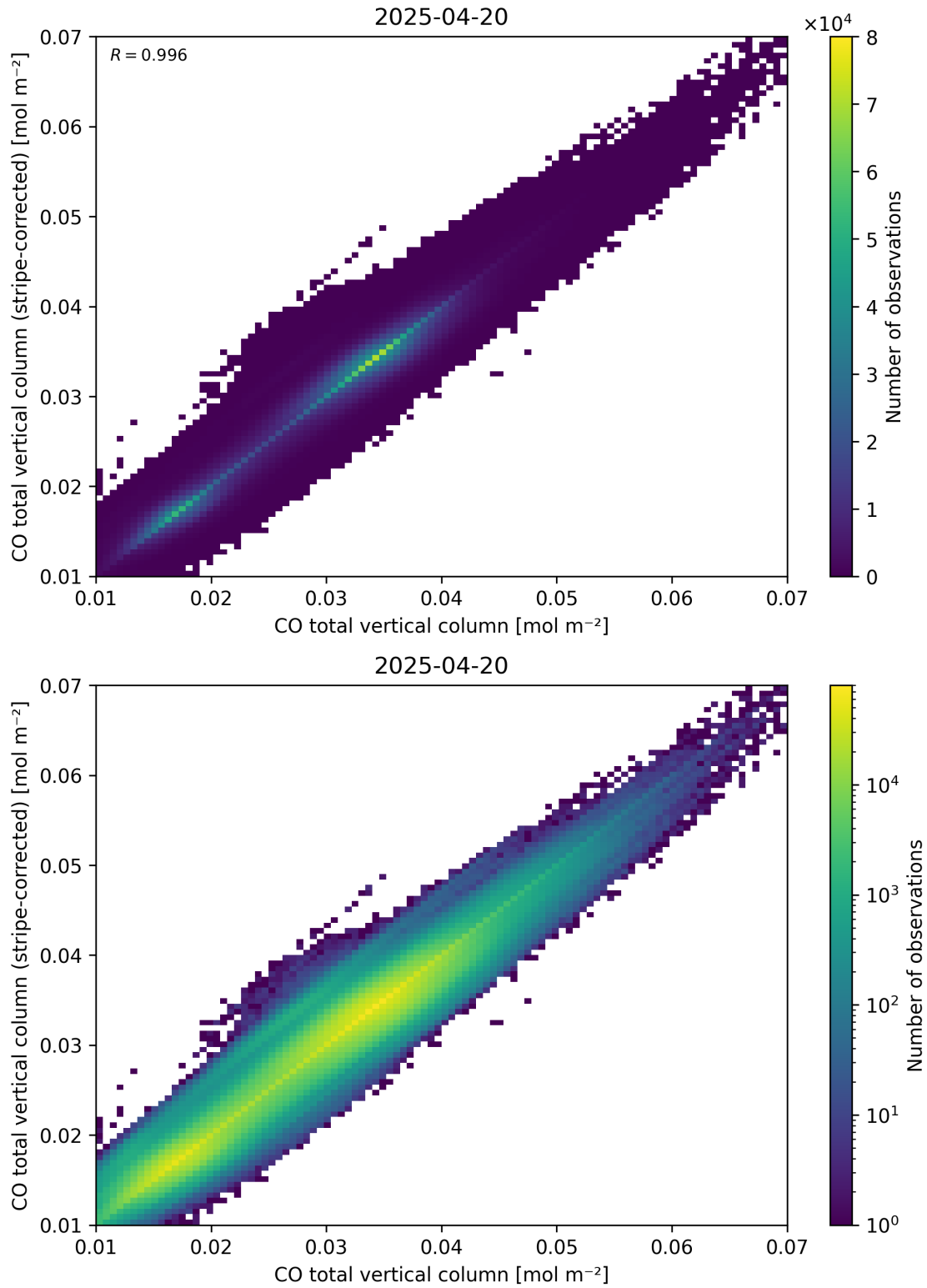
Figure 33: Scatter density plot of “CO total vertical column” against “CO total vertical column (stripe-corrected)” for 2025-04-19 to 2025-04-21.
