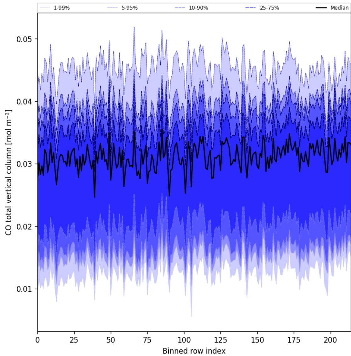
Figure 26: Along track statistics of “CO total vertical column” for 2025-04-19 to 2025-04-21
