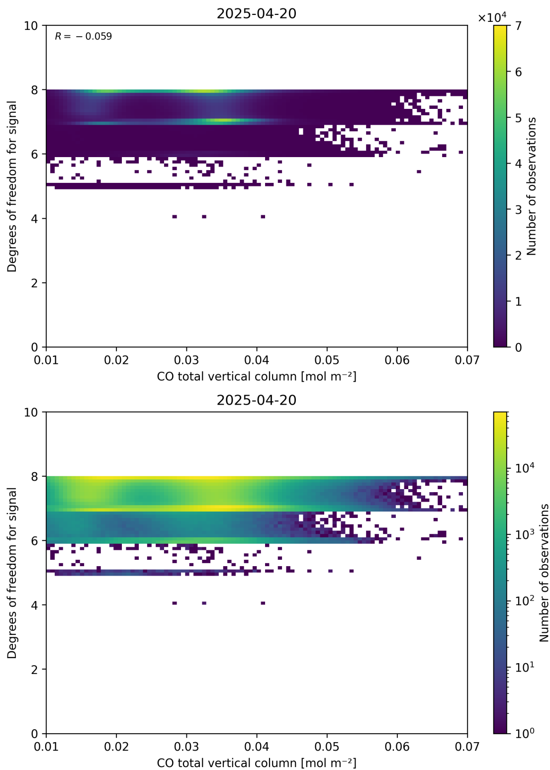
Figure 41: Scatter density plot of “CO total vertical column” against “Degrees of freedom for signal” for 2025-04-19 to 2025-04-21.
