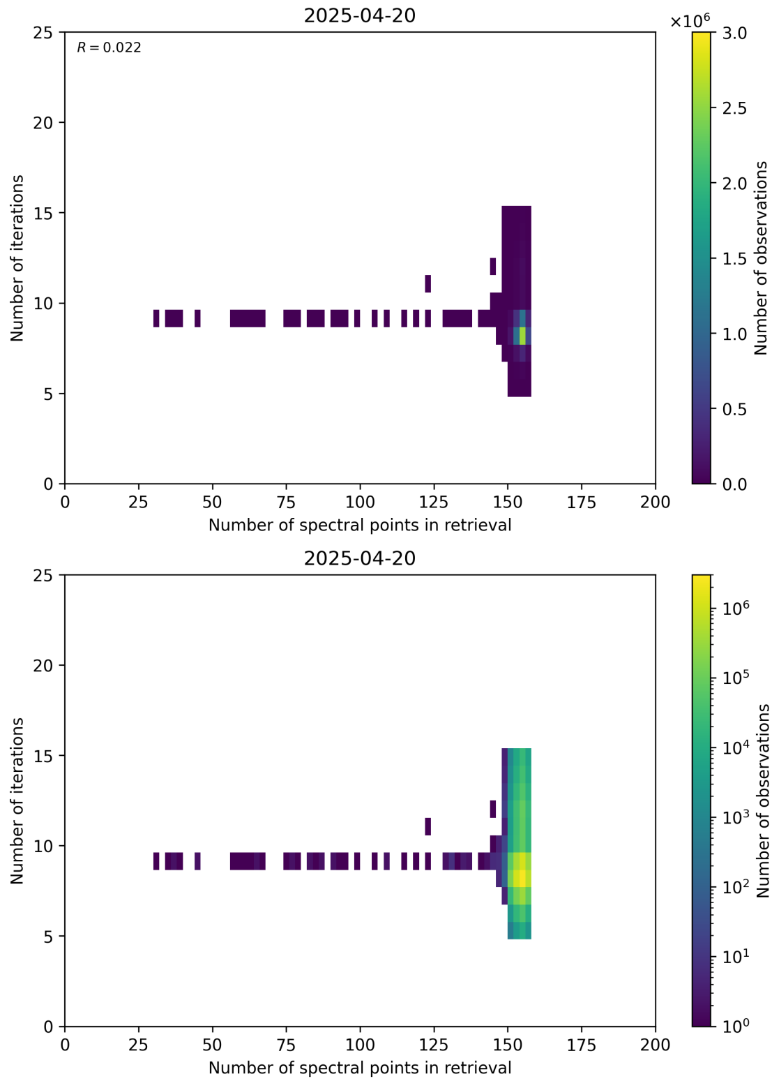
Figure 60: Scatter density plot of “Number of spectral points in retrieval” against “Number of iterations” for 2025-04-19 to 2025-04-21.
