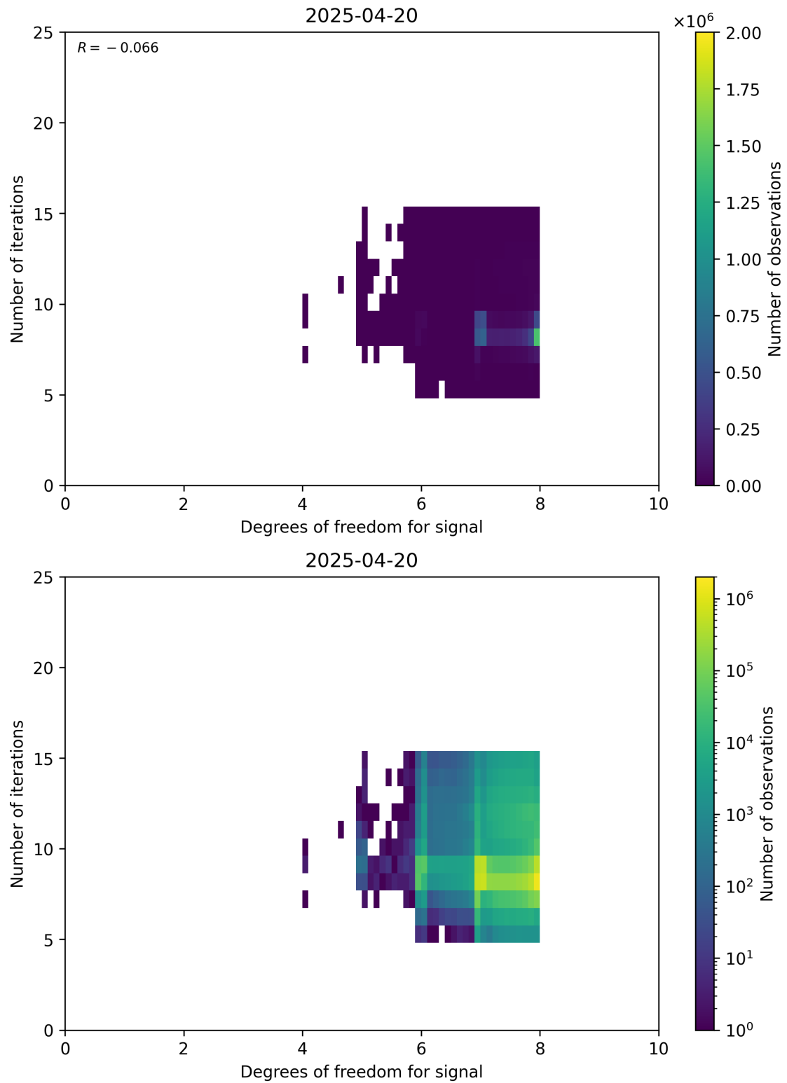
Figure 50: Scatter density plot of “Degrees of freedom for signal” against “Number of iterations” for 2025-04-19 to 2025-04-21.
