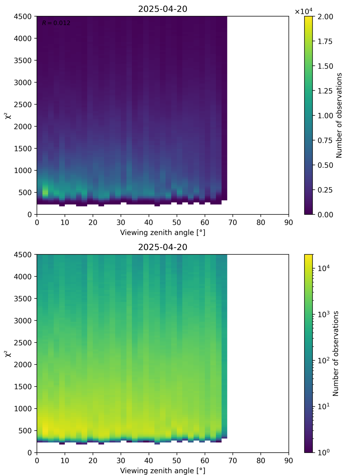
Figure 72: Scatter density plot of “Viewing zenith angle” against “ \chi^2 ” for 2025-04-19 to 2025-04-21.
