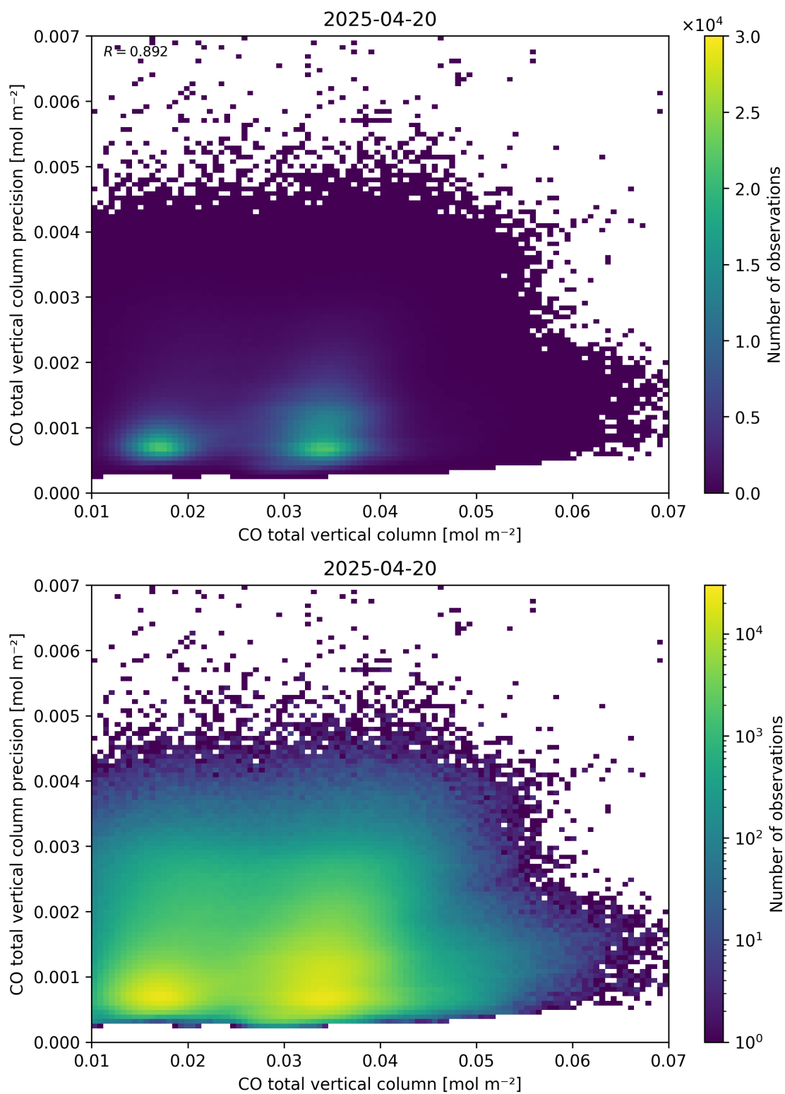
Figure 34: Scatter density plot of “CO total vertical column” against “CO total vertical column precision” for 2025-04-19 to 2025-04-21.
