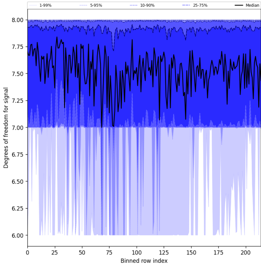
Figure 31: Along track statistics of “Degrees of freedom for signal” for 2025-04-19 to 2025-04-21
