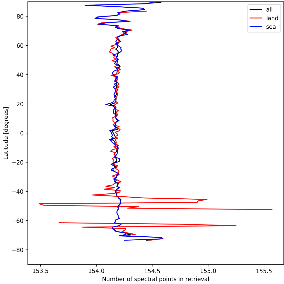
Figure 13: Zonal average of “Number of spectral points in retrieval” for 2025-04-19 to 2025-04-21.
