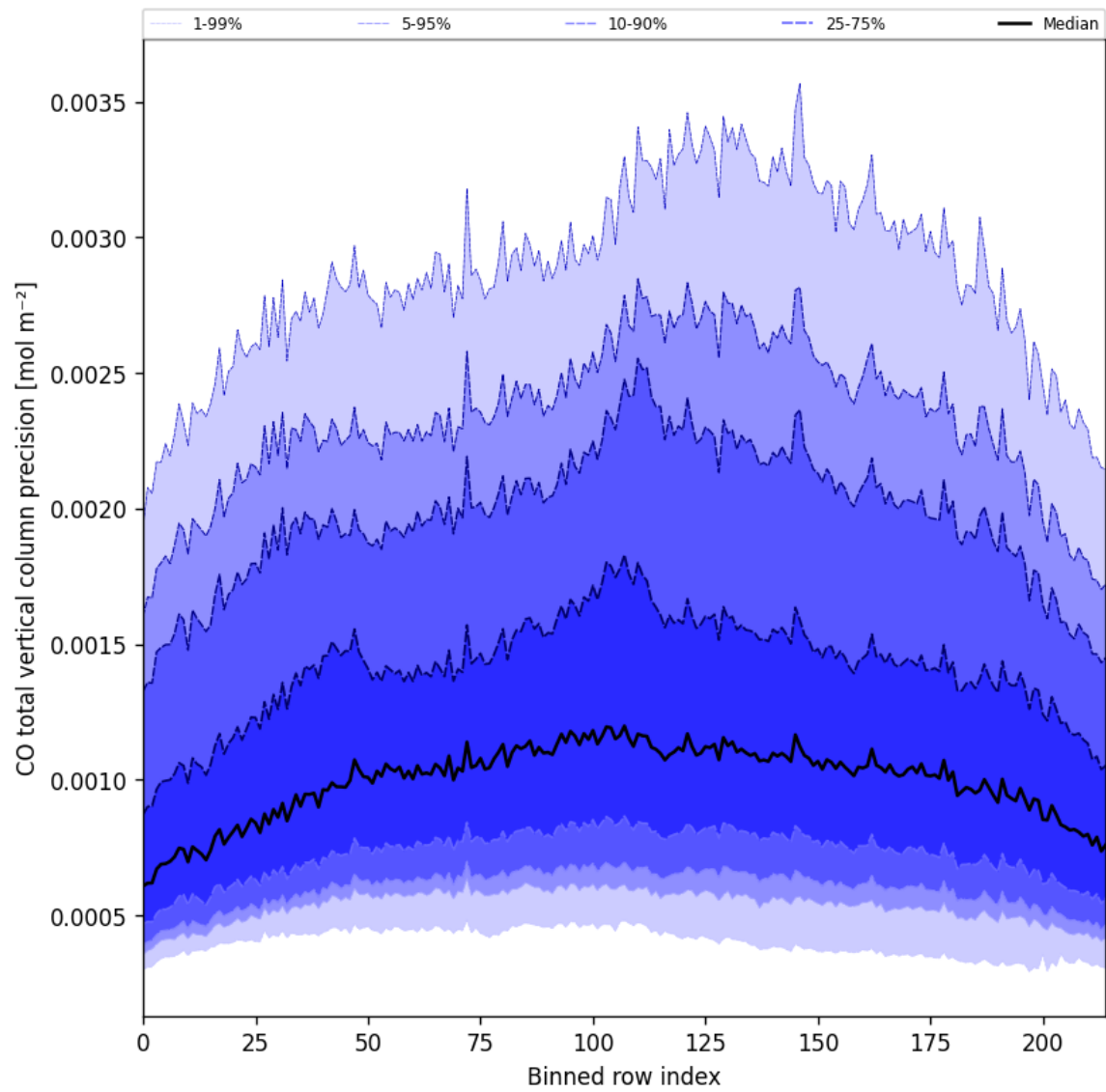
Figure 28: Along track statistics of “CO total vertical column precision” for 2025-04-19 to 2025-04-21
