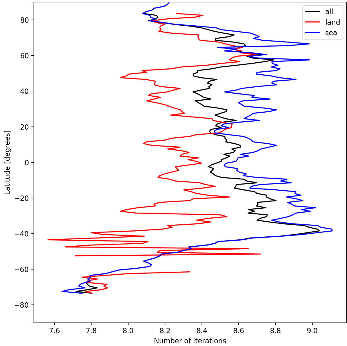
Figure 16: Zonal average of “Number of iterations” for 2025-04-19 to 2025-04-21.
