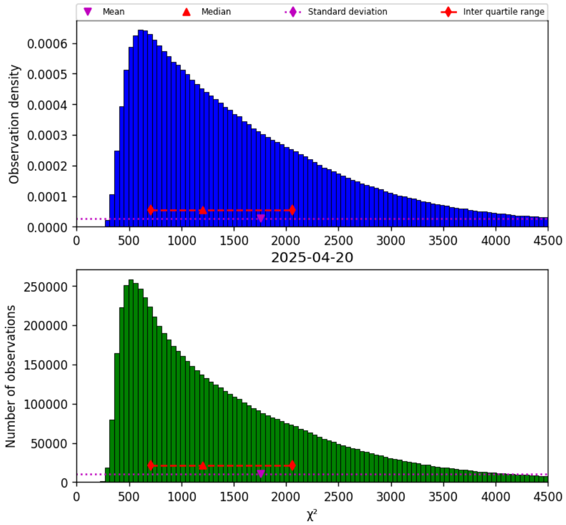
Figure 22: Histogram of “ \chi^2 ” for 2025-04-19 to 2025-04-21
