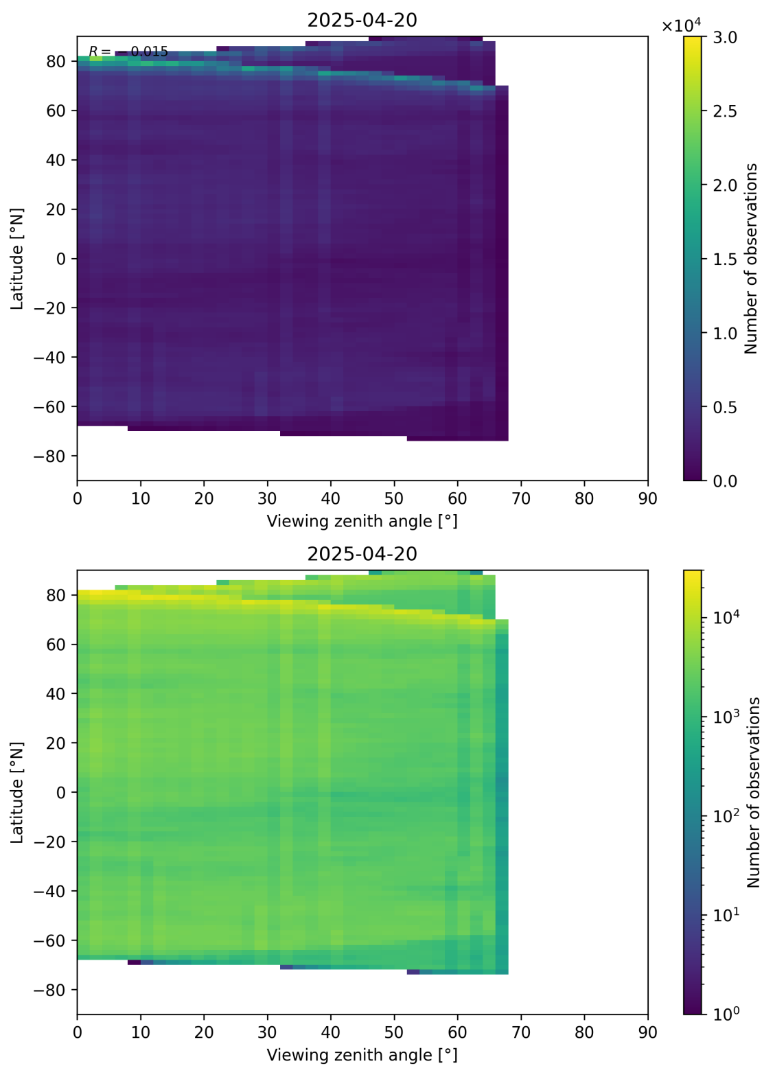
Figure 74: Scatter density plot of “Viewing zenith angle” against “Latitude” for 2025-04-19 to 2025-04-21.
