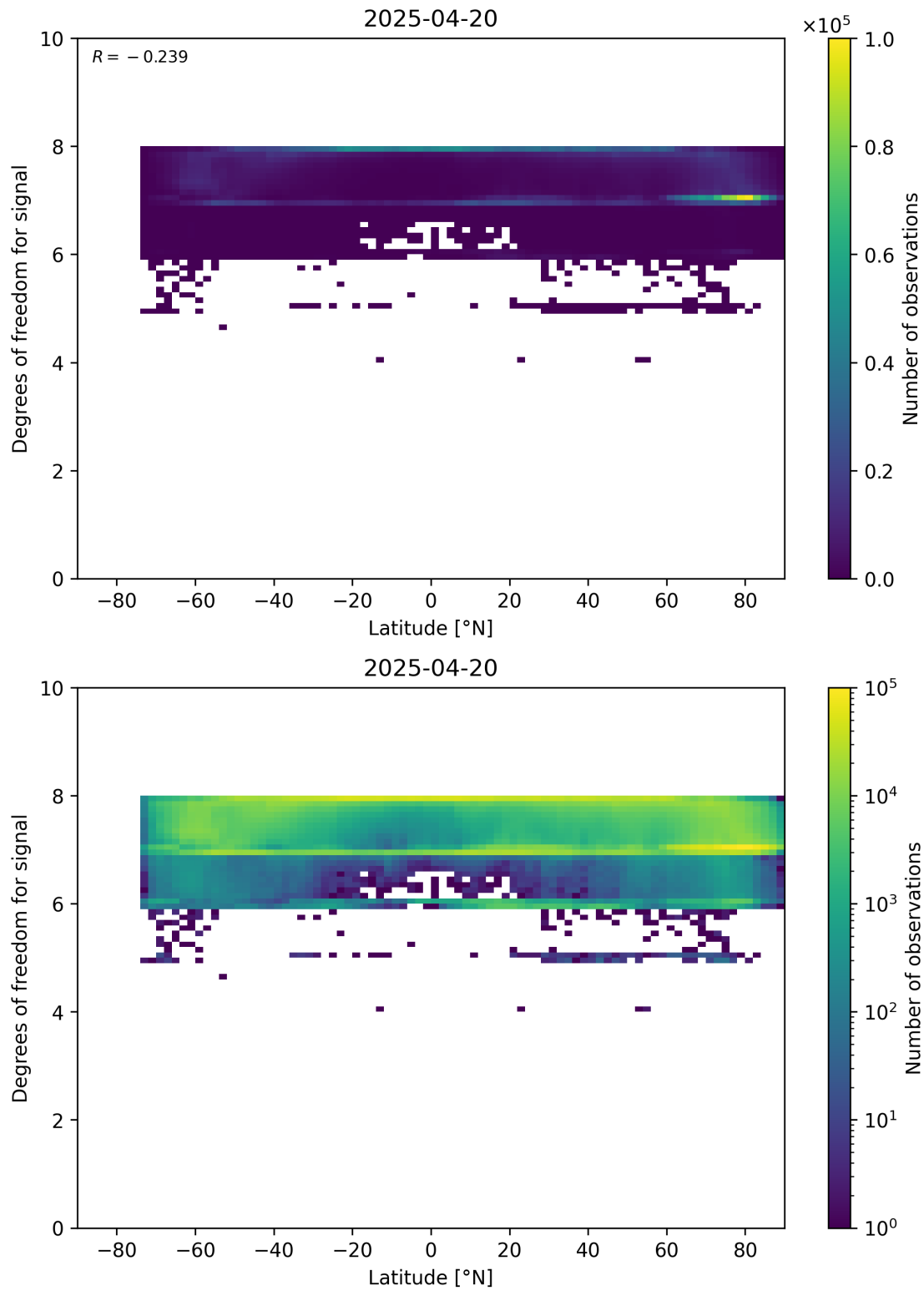
Figure 55: Scatter density plot of “Latitude” against “Degrees of freedom for signal” for 2025-04-19 to 2025-04-21.
