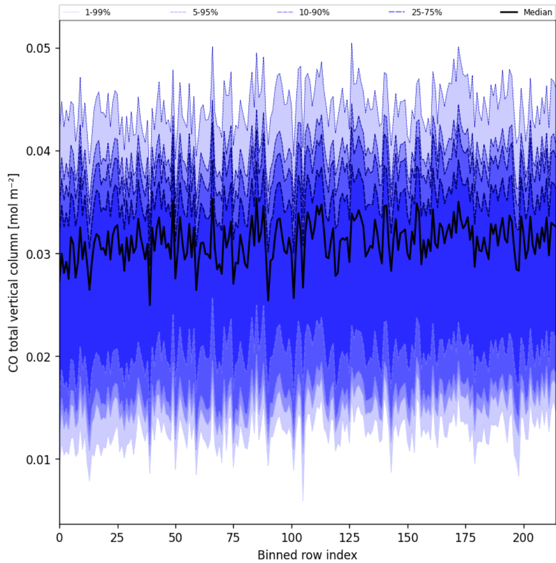
Figure 26: Along track statistics of “CO total vertical column” for 2025-04-20 to 2025-04-22
