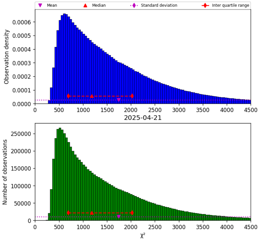
Figure 22: Histogram of “ \chi^2 ” for 2025-04-20 to 2025-04-22
