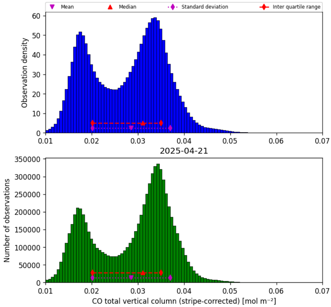
Figure 19: Histogram of “CO total vertical column (stripe-corrected)” for 2025-04-20 to 2025-04-22
