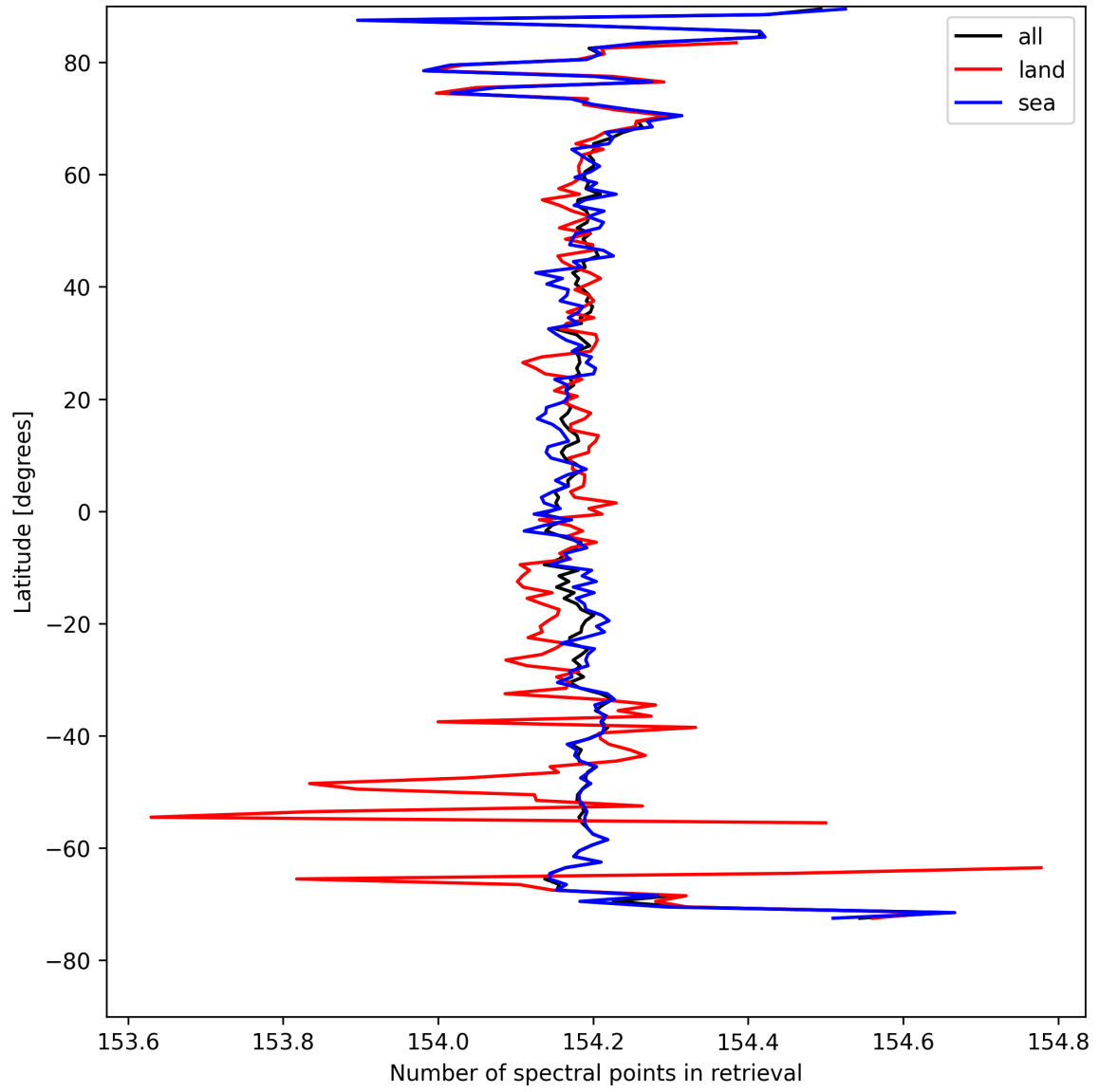
Figure 13: Zonal average of “Number of spectral points in retrieval” for 2025-04-20 to 2025-04-22.
