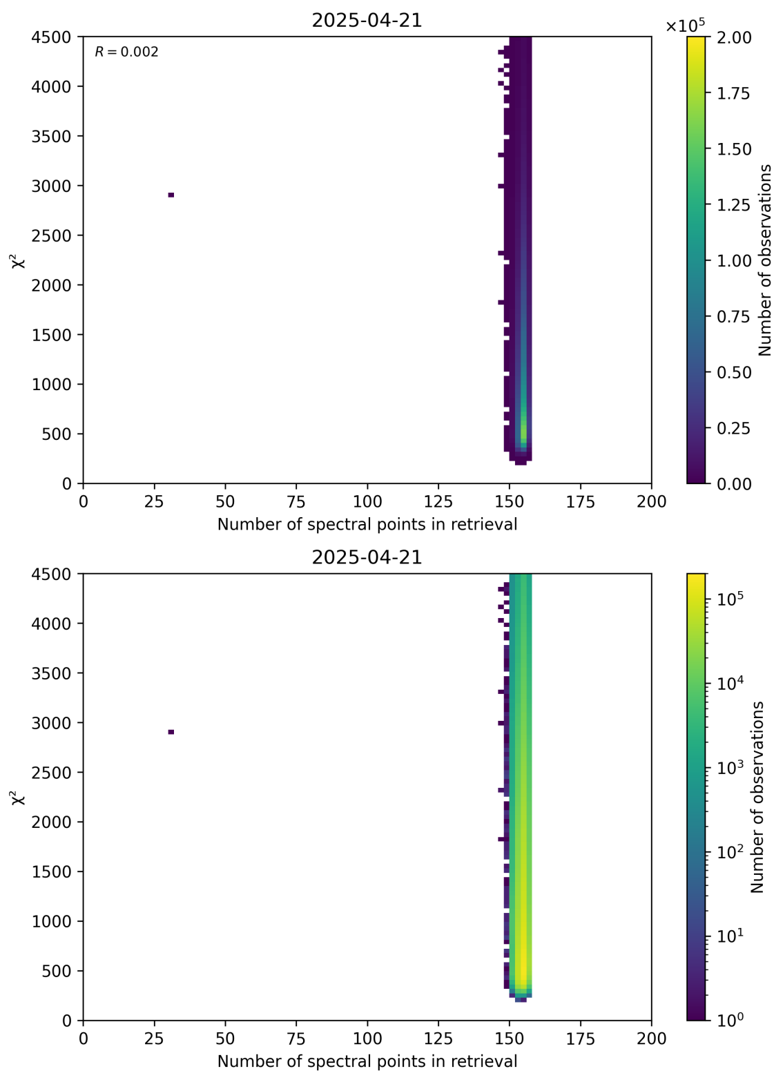
Figure 58: Scatter density plot of “Number of spectral points in retrieval” against “ \chi^2 ” for 2025-04-20 to 2025-04-22.
