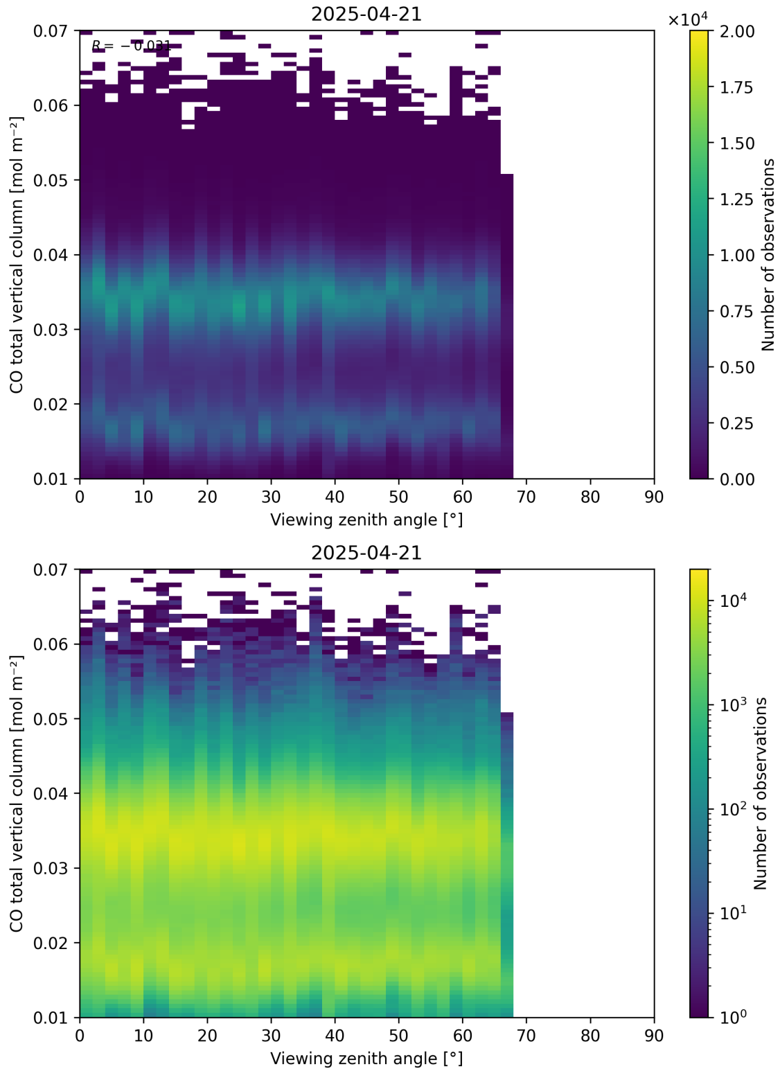
Figure 69: Scatter density plot of “Viewing zenith angle” against “CO total vertical column” for 2025-04-20 to 2025-04-22.
