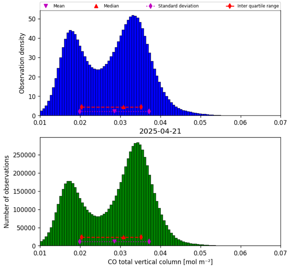
Figure 18: Histogram of “CO total vertical column” for 2025-04-20 to 2025-04-22
