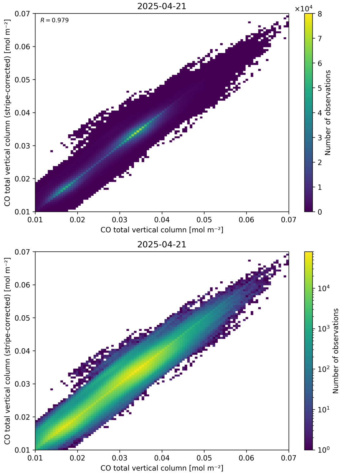
Figure 33: Scatter density plot of “CO total vertical column” against “CO total vertical column (stripe-corrected)” for 2025-04-20 to 2025-04-22.
