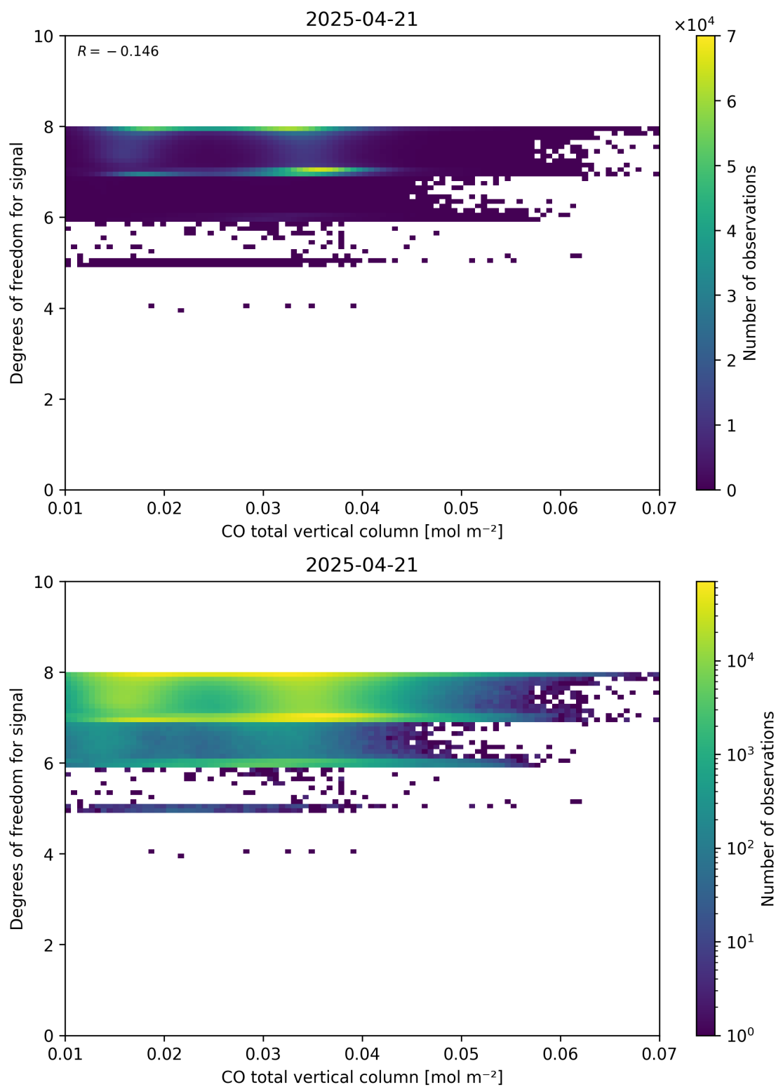
Figure 41: Scatter density plot of “CO total vertical column” against “Degrees of freedom for signal” for 2025-04-20 to 2025-04-22.
