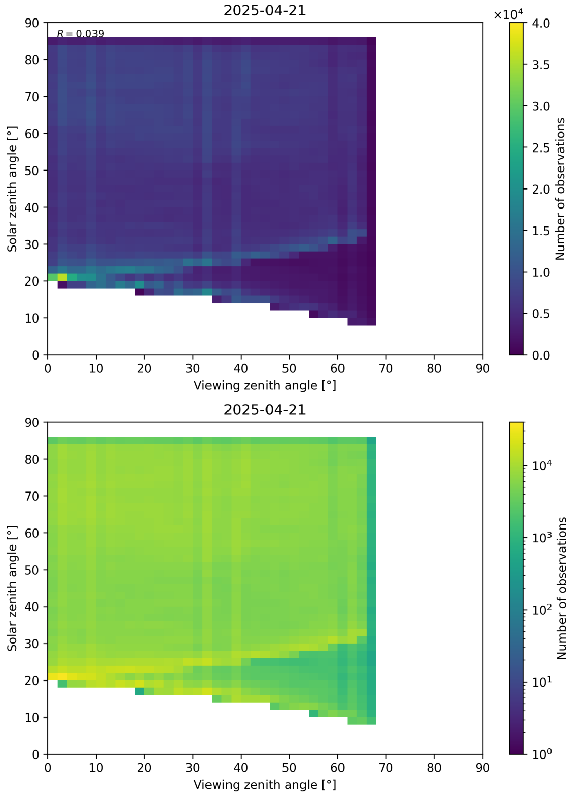
Figure 77: Scatter density plot of “Viewing zenith angle” against “Solar zenith angle” for 2025-04-20 to 2025-04-22.
