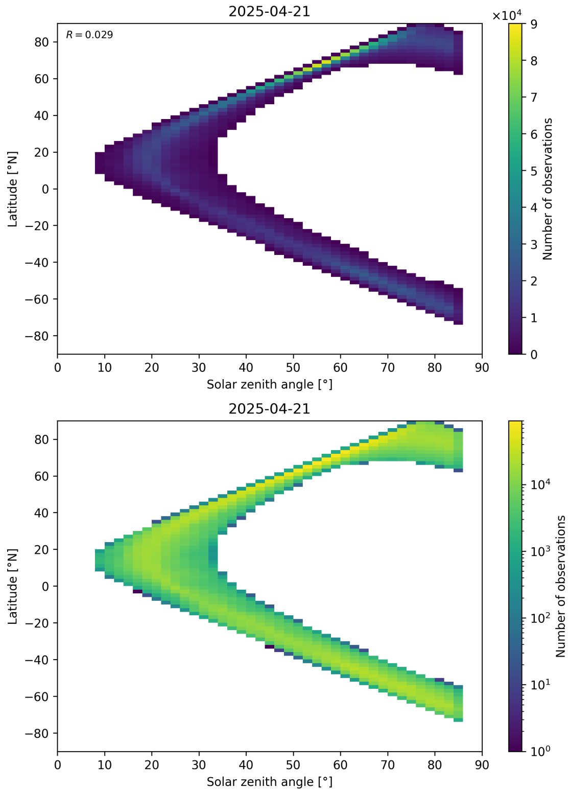
Figure 66: Scatter density plot of “Solar zenith angle” against “Latitude” for 2025-04-20 to 2025-04-22.
