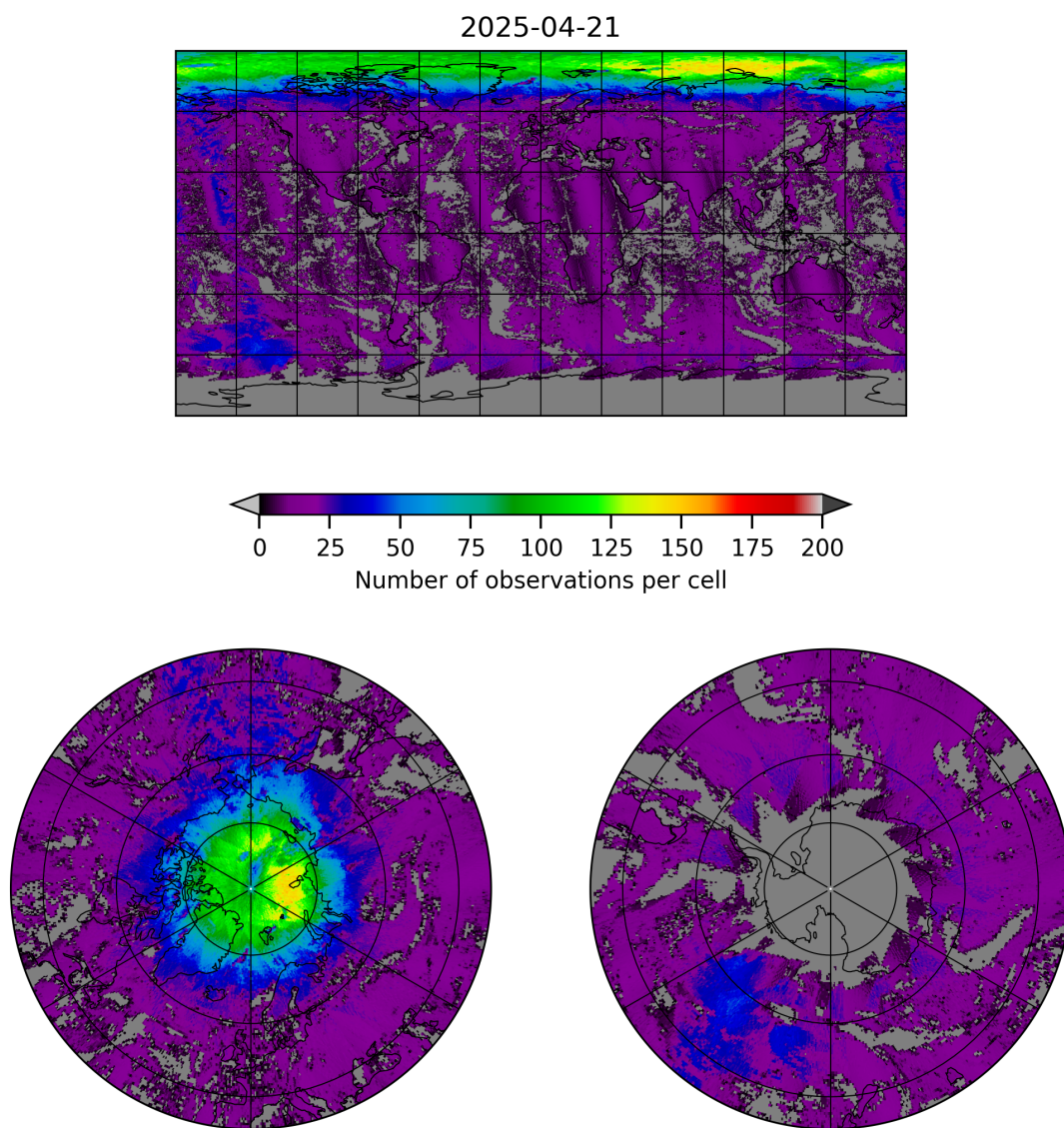
Figure 8: Map of the number of observations for 2025-04-20 to 2025-04-22
