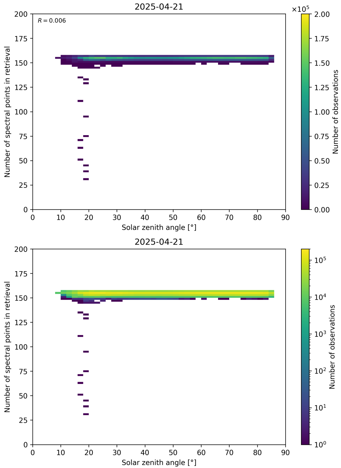
Figure 68: Scatter density plot of “Solar zenith angle” against “Number of spectral points in retrieval” for 2025-04-20 to 2025-04-22.
