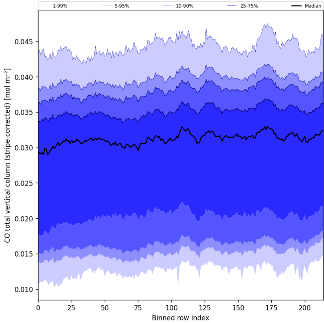
Figure 27: Along track statistics of “CO total vertical column (stripe-corrected)” for 2025-04-20 to 2025-04-22
