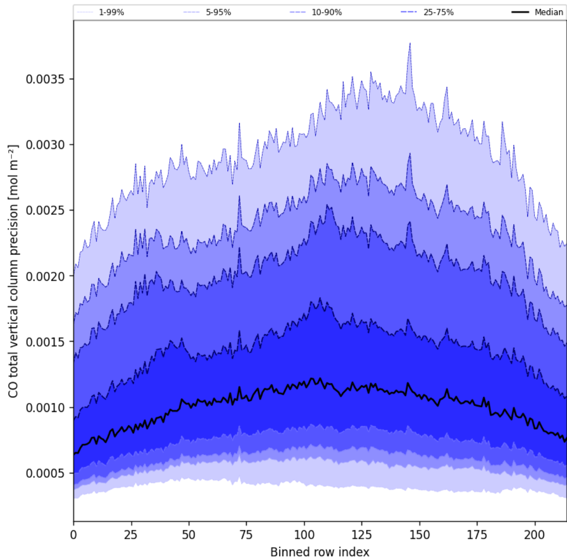
Figure 28: Along track statistics of “CO total vertical column precision” for 2025-04-20 to 2025-04-22
