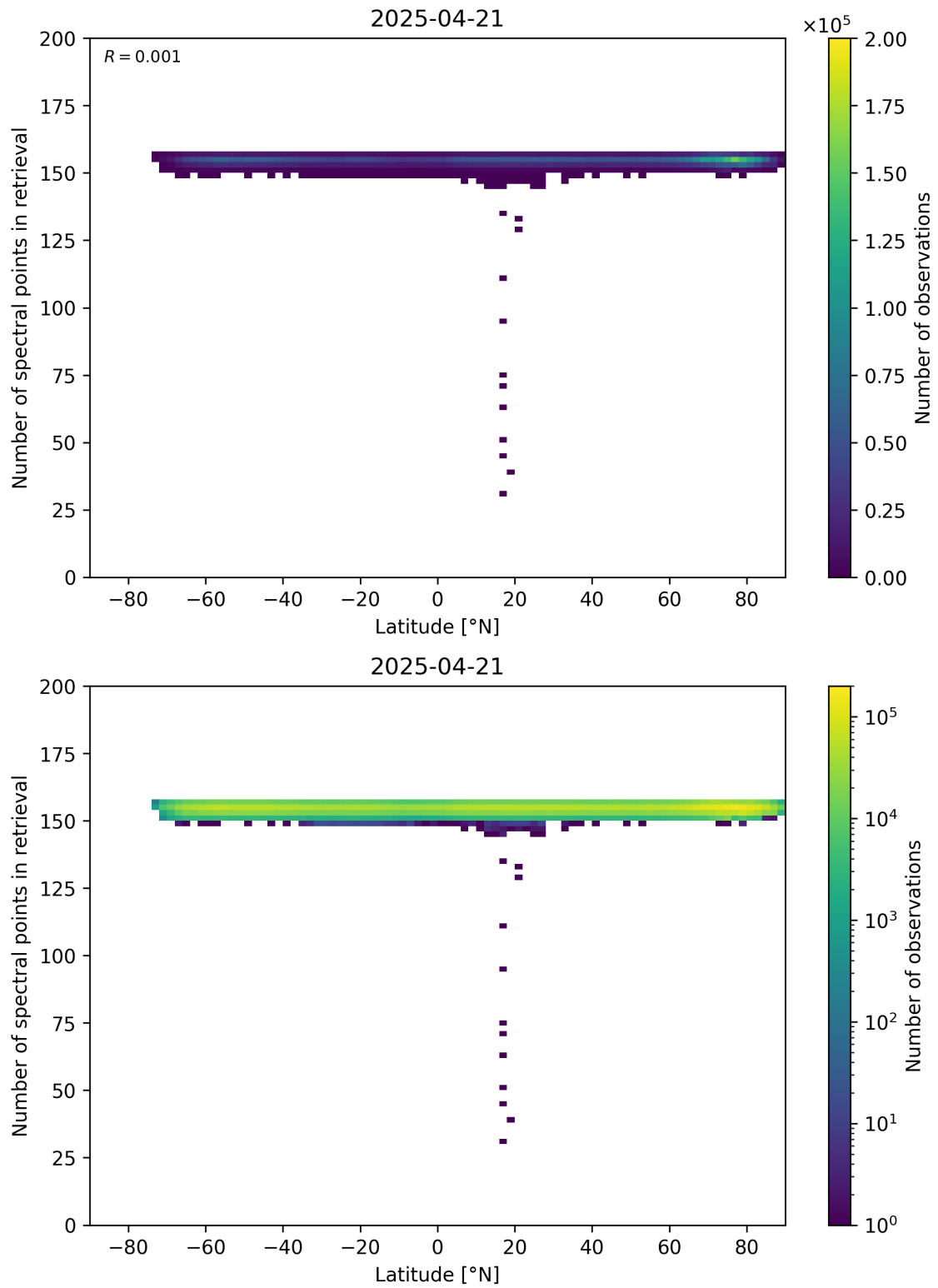
Figure 57: Scatter density plot of “Latitude” against “Number of spectral points in retrieval” for 2025-04-20 to 2025-04-22.
