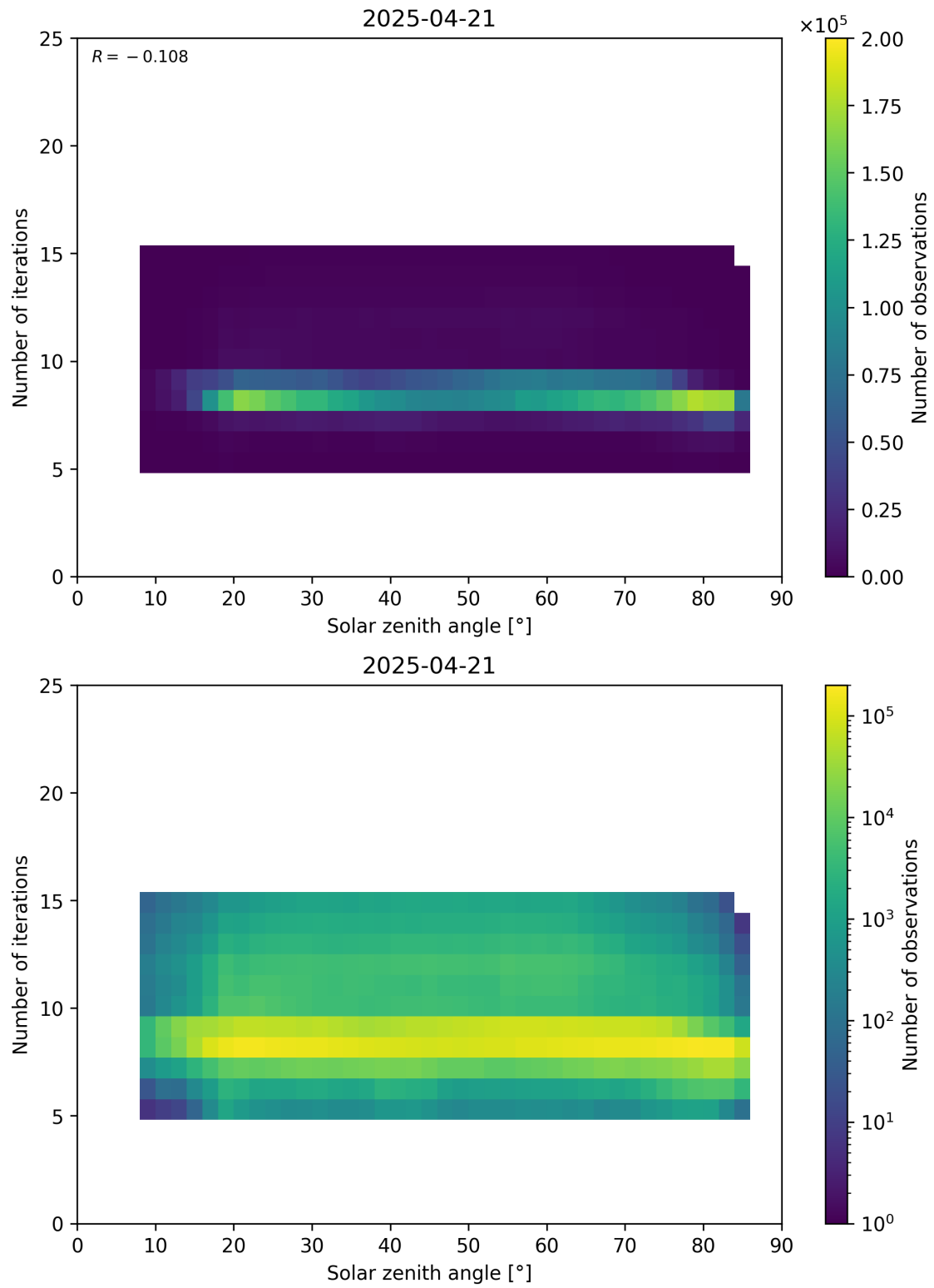
Figure 67: Scatter density plot of “Solar zenith angle” against “Number of iterations” for 2025-04-20 to 2025-04-22.
