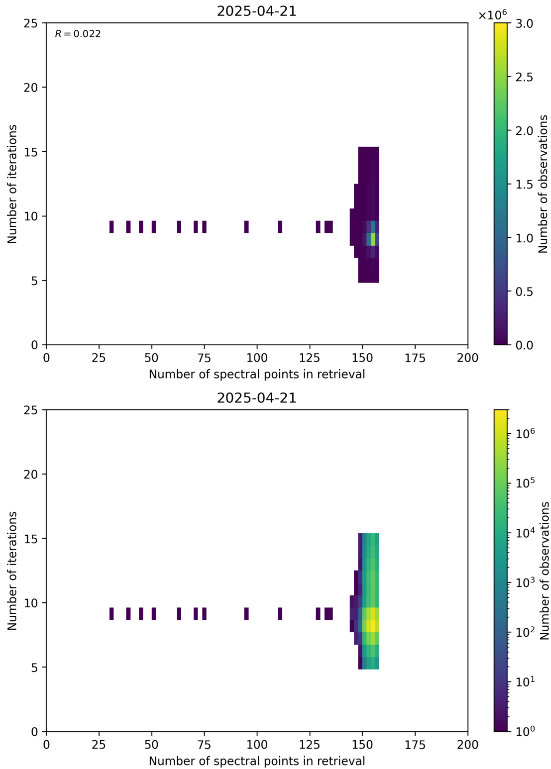
Figure 60: Scatter density plot of “Number of spectral points in retrieval” against “Number of iterations” for 2025-04-20 to 2025-04-22.
