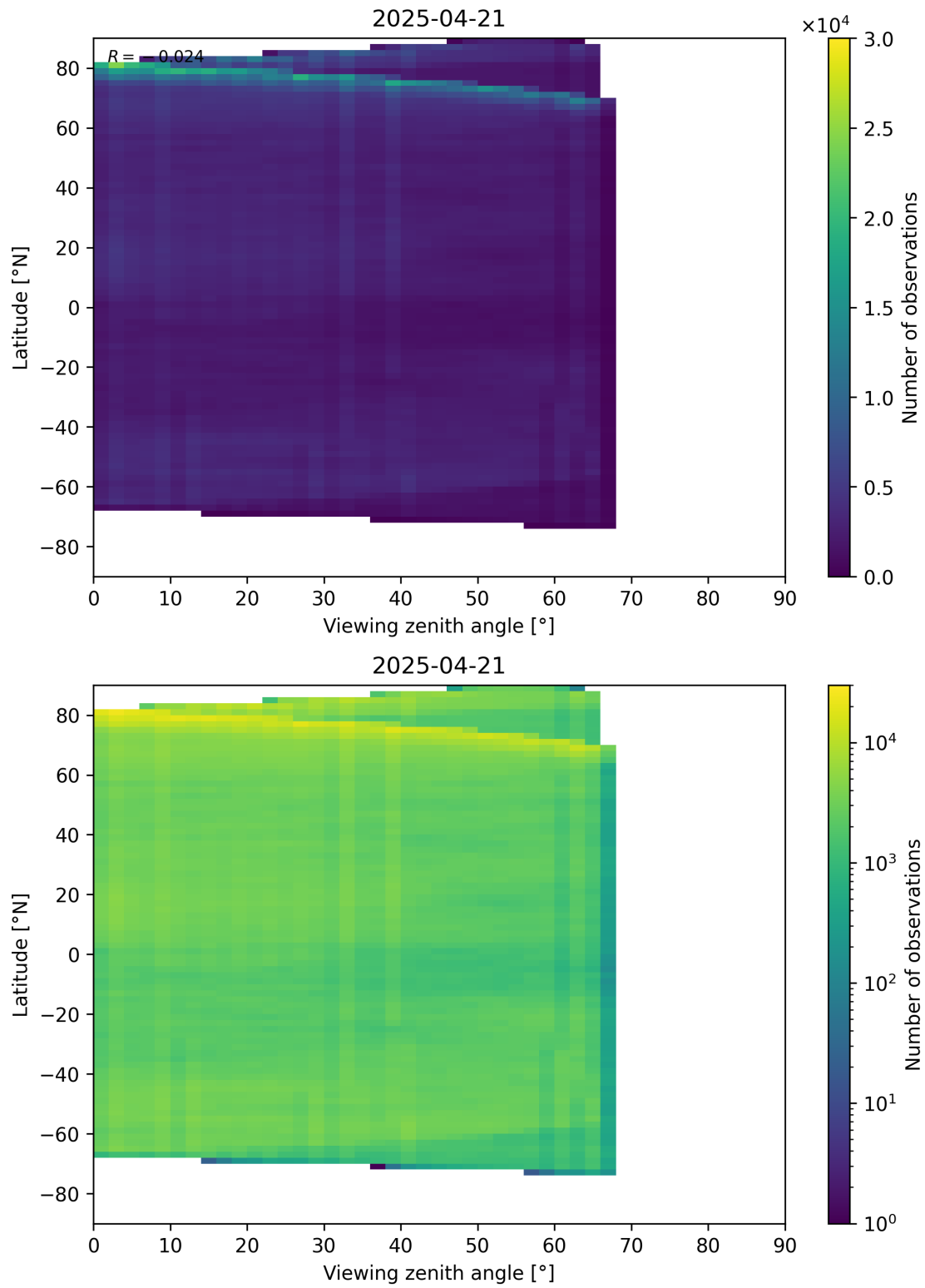
Figure 74: Scatter density plot of “Viewing zenith angle” against “Latitude” for 2025-04-20 to 2025-04-22.
