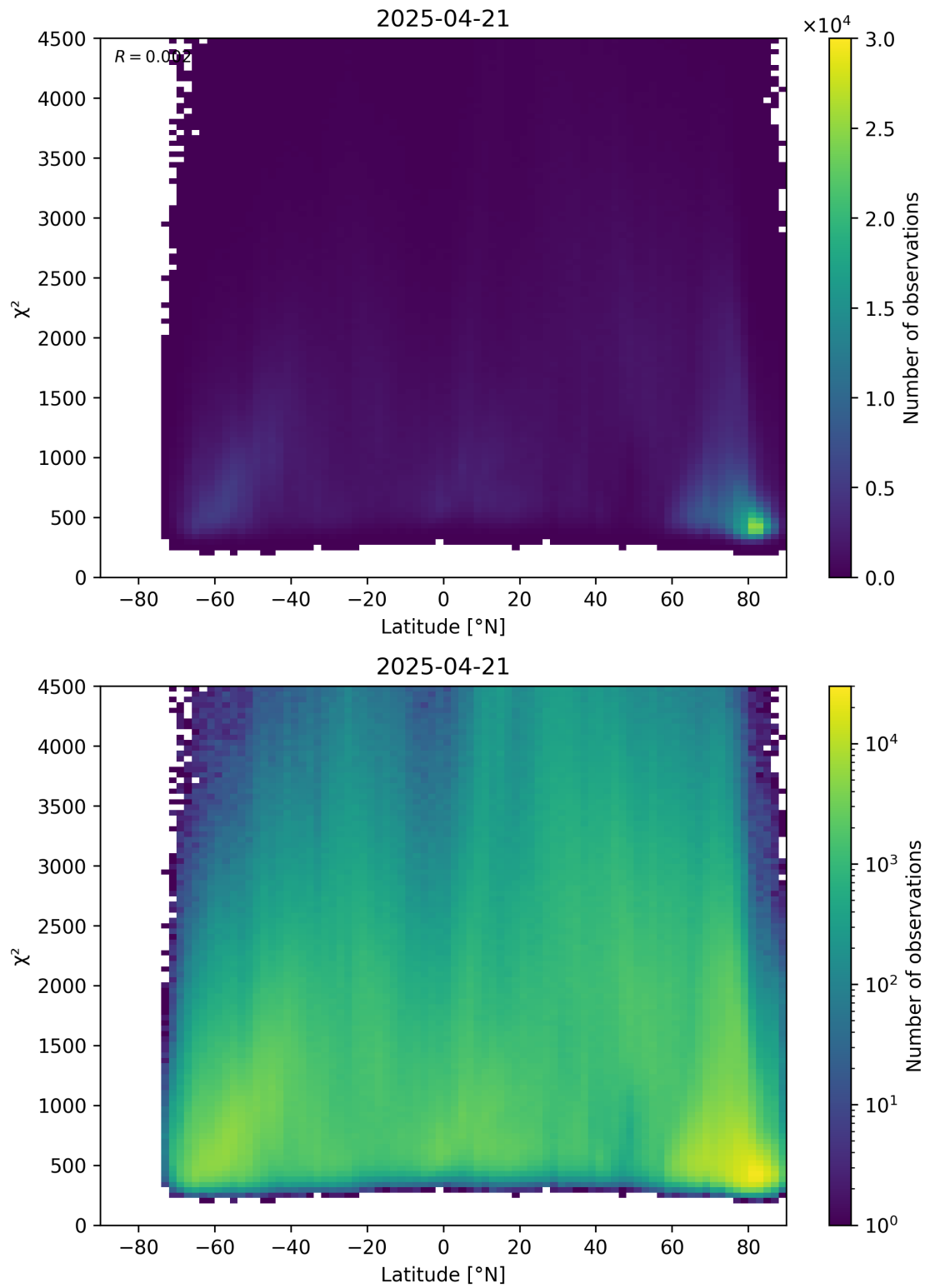
Figure 54: Scatter density plot of “Latitude” against “ \chi^2 ” for 2025-04-20 to 2025-04-22.
