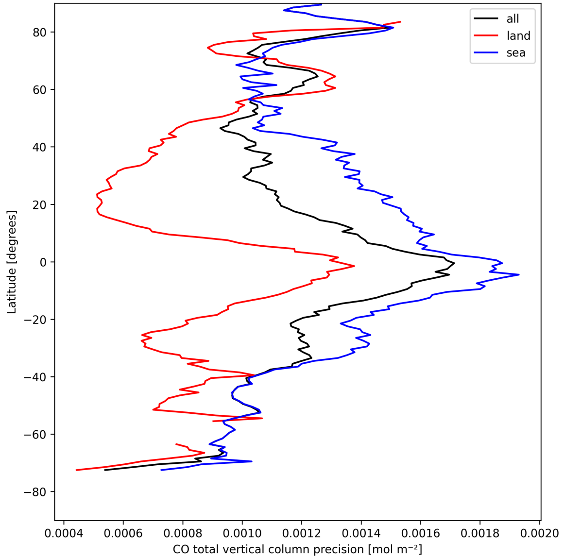
Figure 12: Zonal average of “CO total vertical column precision” for 2025-04-20 to 2025-04-22.
