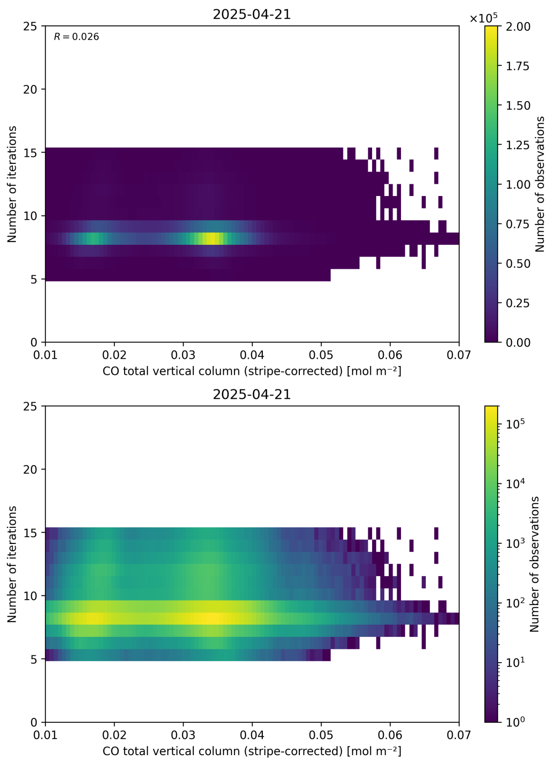
Figure 39: Scatter density plot of “CO total vertical column (stripe-corrected)” against “Number of iterations” for 2025-04-20 to 2025-04-22.
