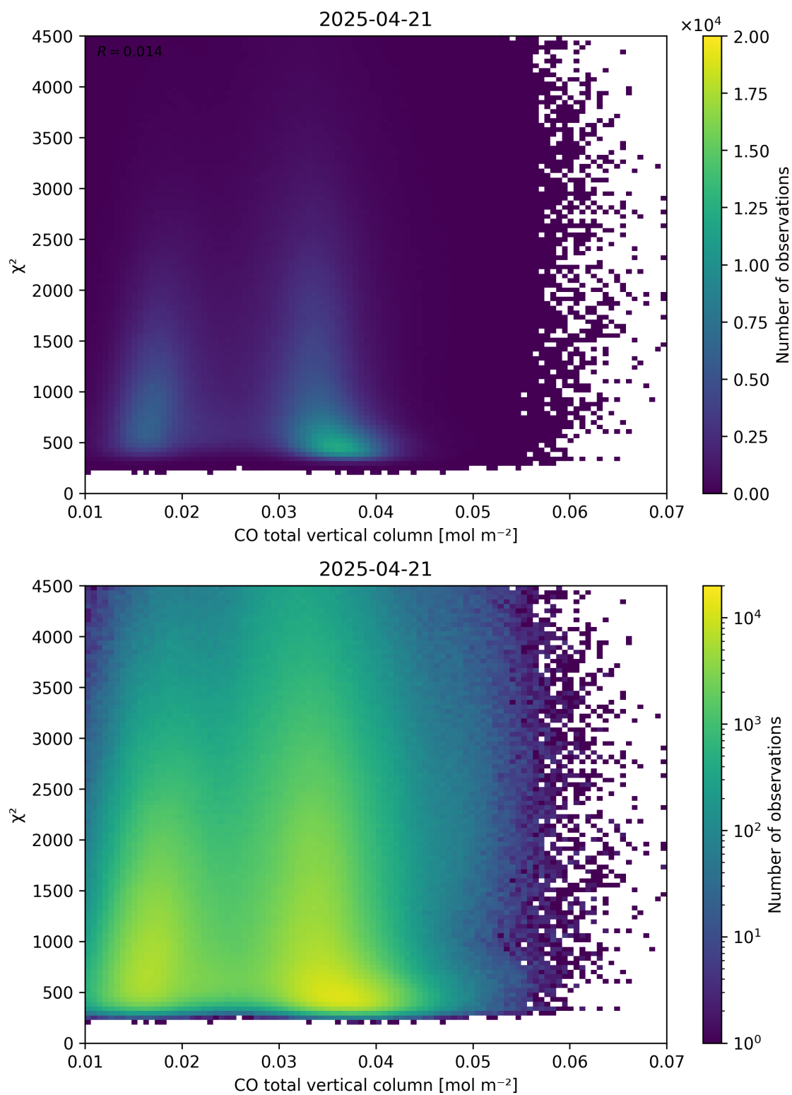
Figure 35: Scatter density plot of “CO total vertical column” against “ \chi^2 ” for 2025-04-20 to 2025-04-22.
