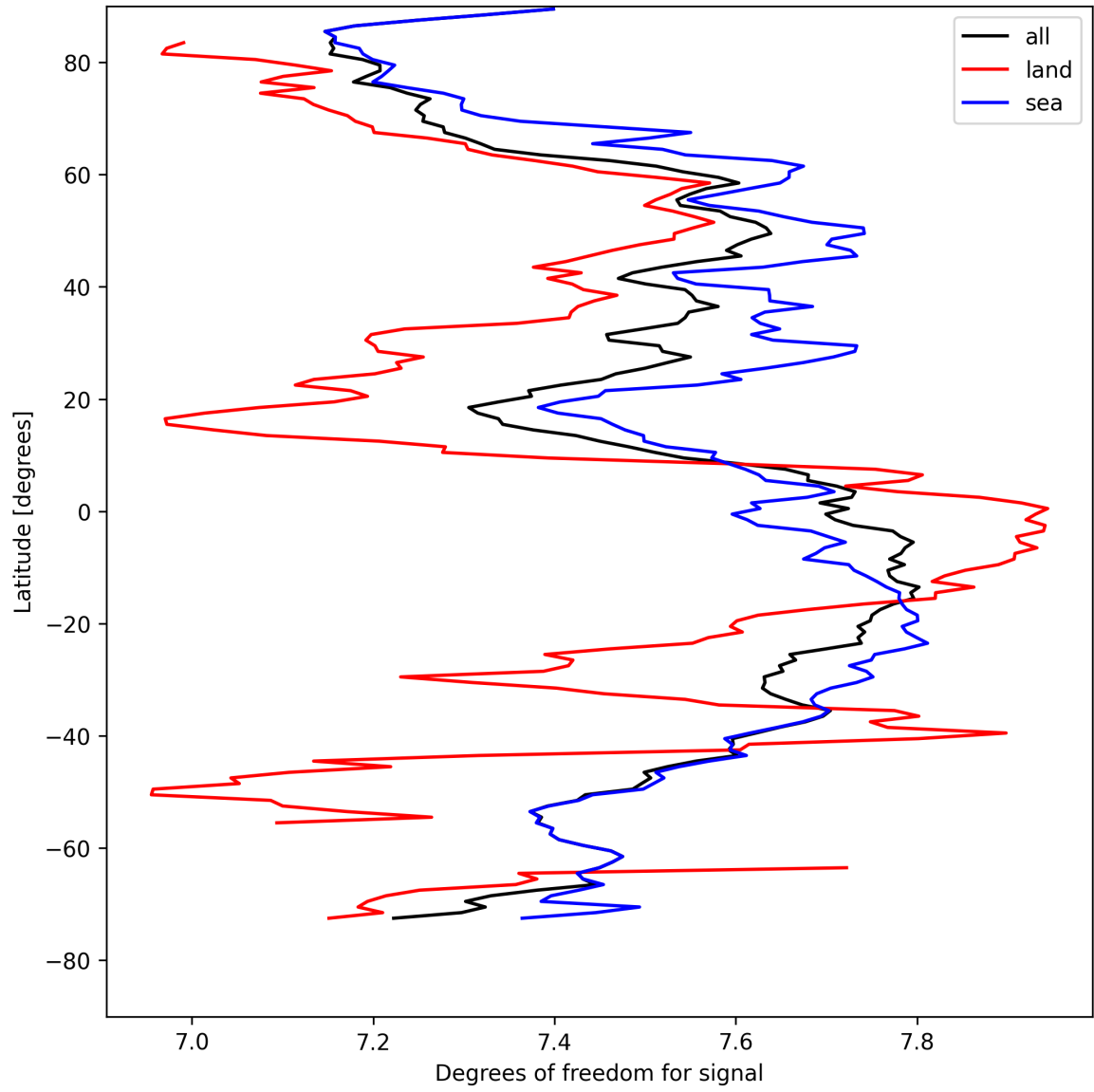
Figure 15: Zonal average of “Degrees of freedom for signal” for 2025-04-20 to 2025-04-22.
