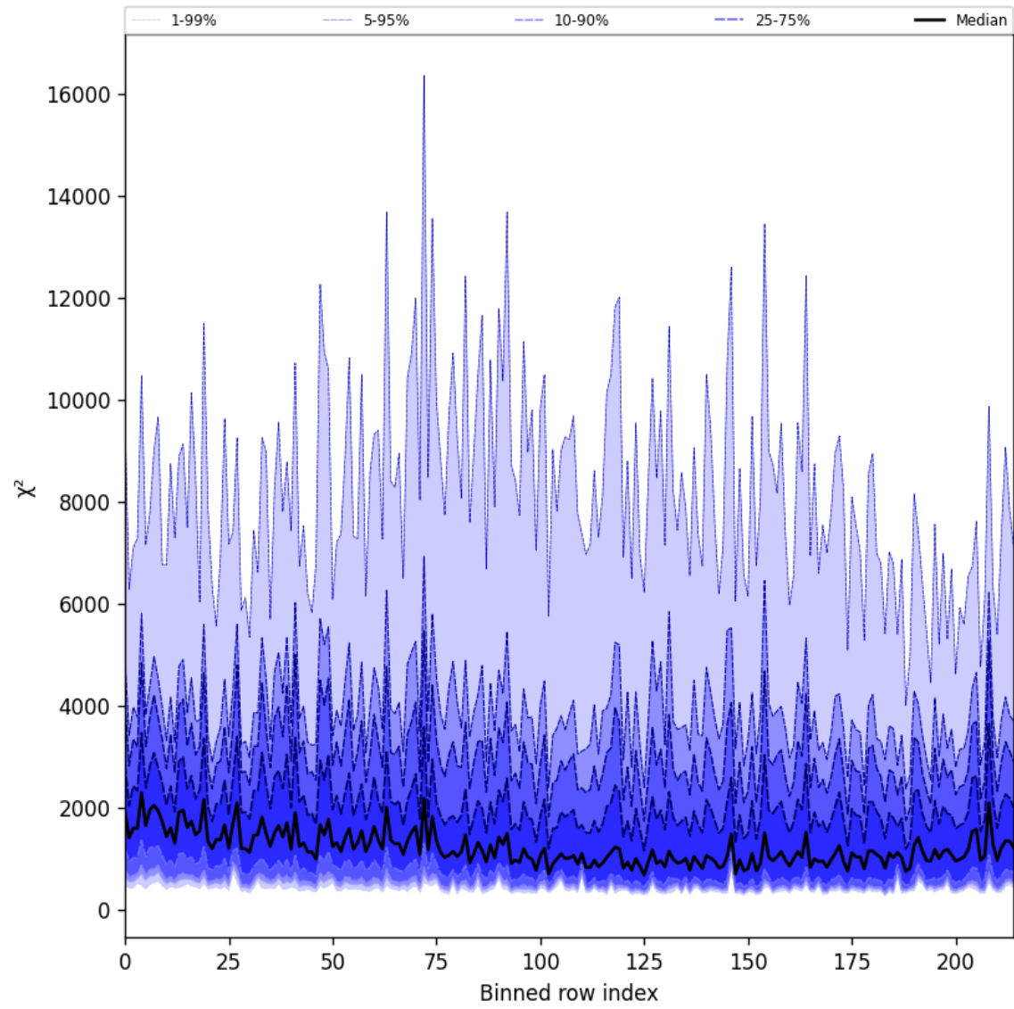
Figure 30: Along track statistics of “ \chi^2 ” for 2025-04-20 to 2025-04-22
