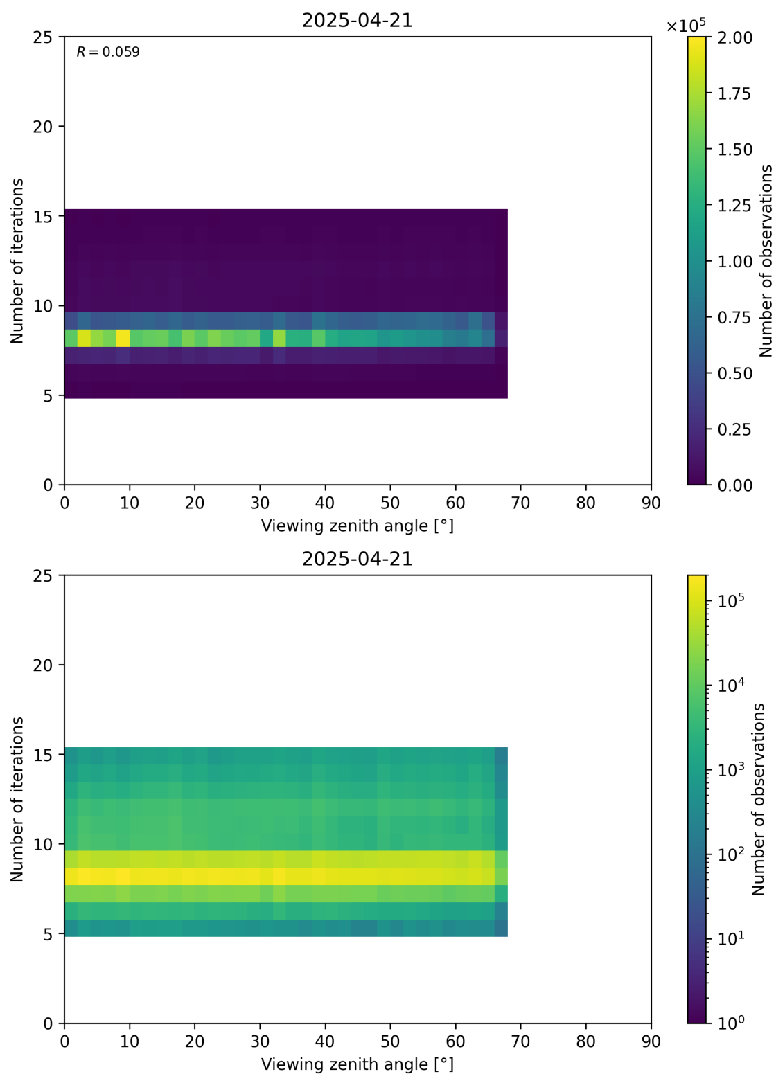
Figure 75: Scatter density plot of “Viewing zenith angle” against “Number of iterations” for 2025-04-20 to 2025-04-22.
