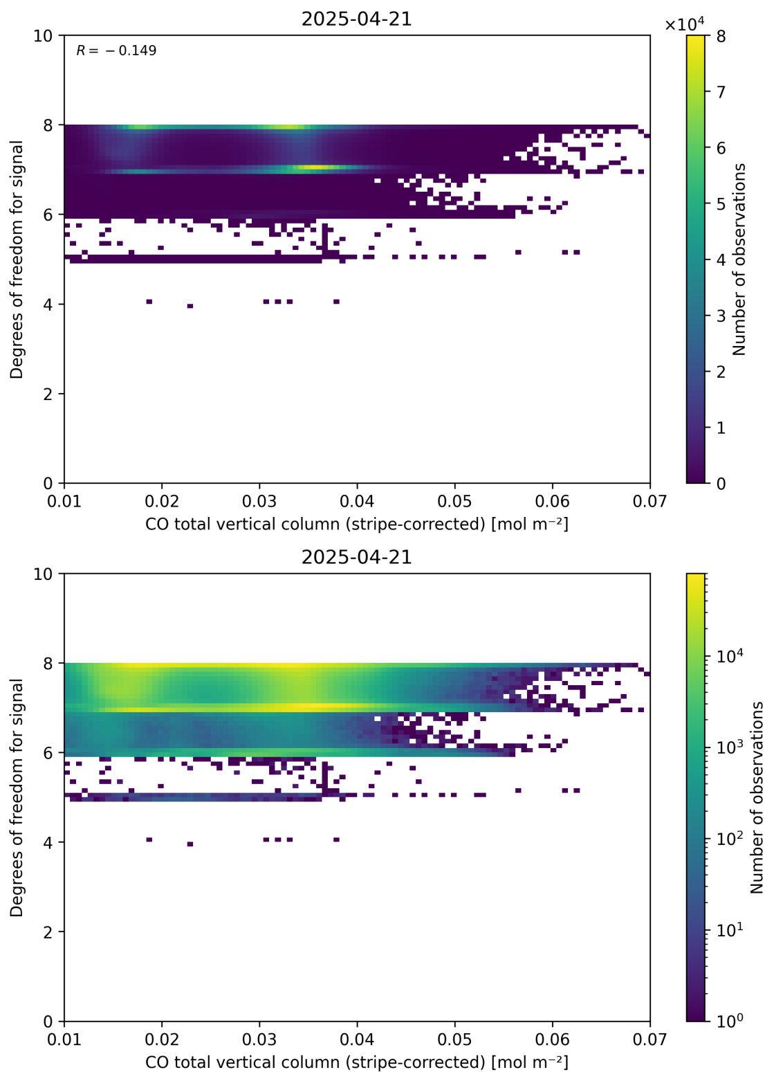
Figure 38: Scatter density plot of “CO total vertical column (stripe-corrected)” against “Degrees of freedom for signal” for 2025-04-20 to 2025-04-22.
