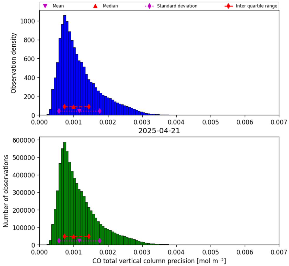
Figure 20: Histogram of “CO total vertical column precision” for 2025-04-20 to 2025-04-22
