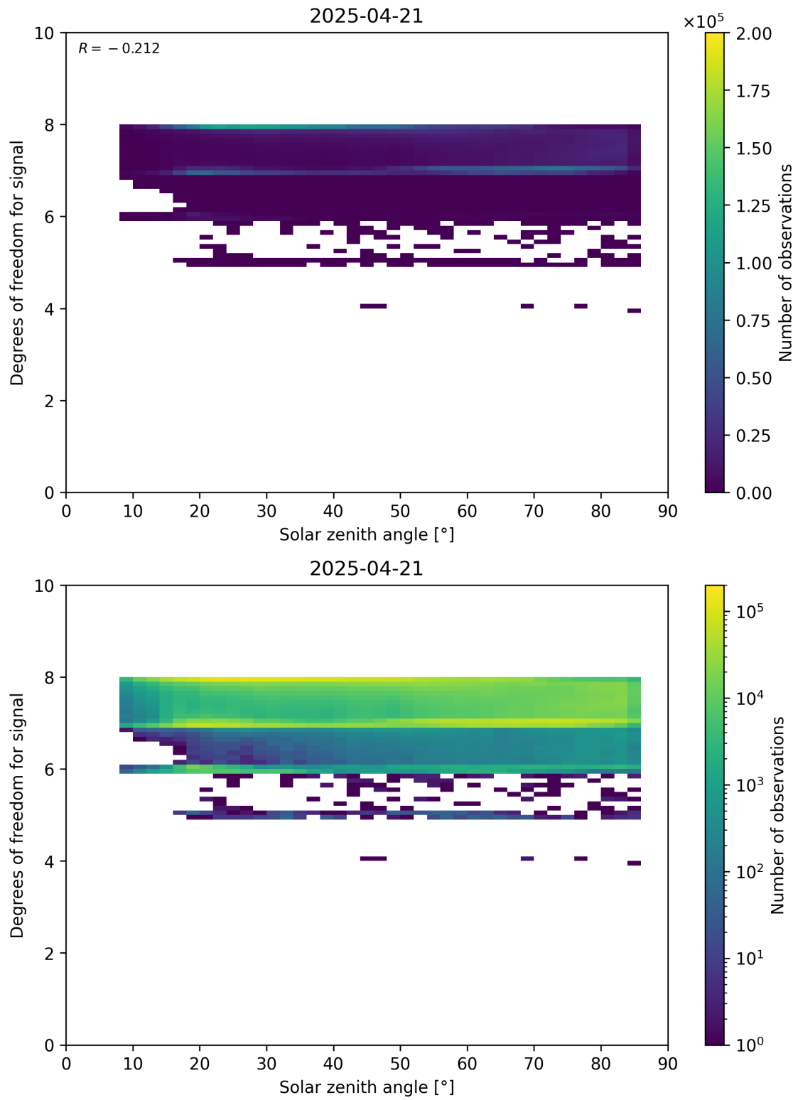
Figure 65: Scatter density plot of “Solar zenith angle” against “Degrees of freedom for signal” for 2025-04-20 to 2025-04-22.
