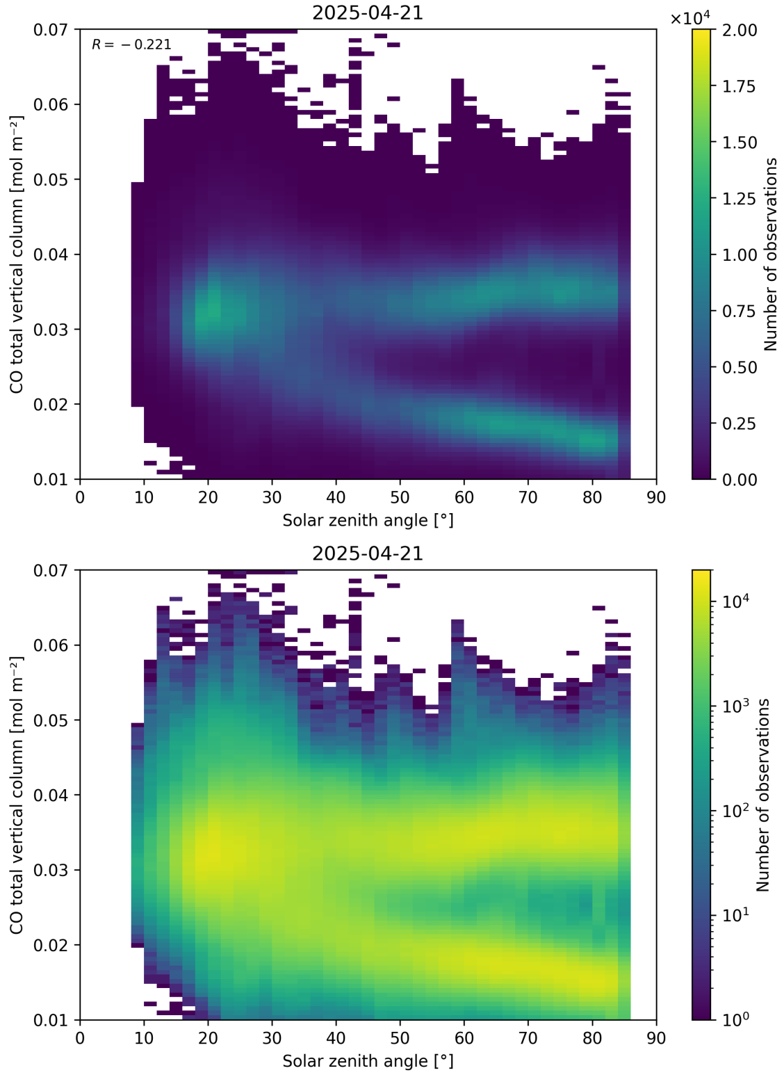
Figure 61: Scatter density plot of “Solar zenith angle” against “CO total vertical column” for 2025-04-20 to 2025-04-22.
