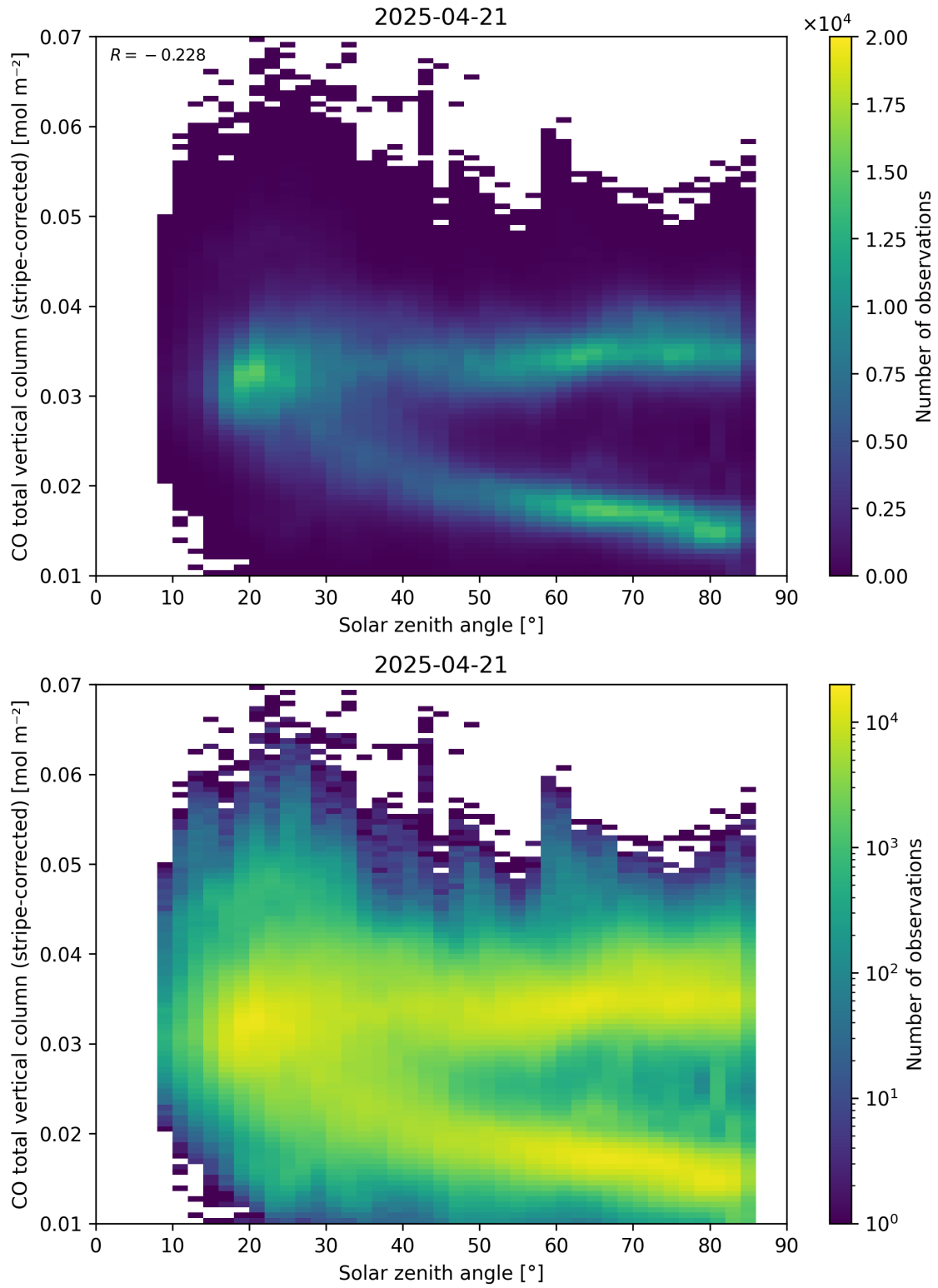
Figure 62: Scatter density plot of “Solar zenith angle” against “CO total vertical column (stripe-corrected)” for 2025-04-20 to 2025-04-22.
