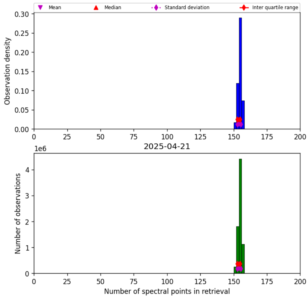
Figure 21: Histogram of “Number of spectral points in retrieval” for 2025-04-20 to 2025-04-22
