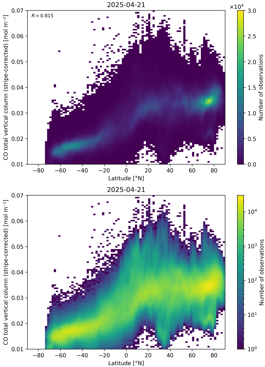
Figure 52: Scatter density plot of “Latitude” against “CO total vertical column (stripe-corrected)” for 2025-04-20 to 2025-04-22.
