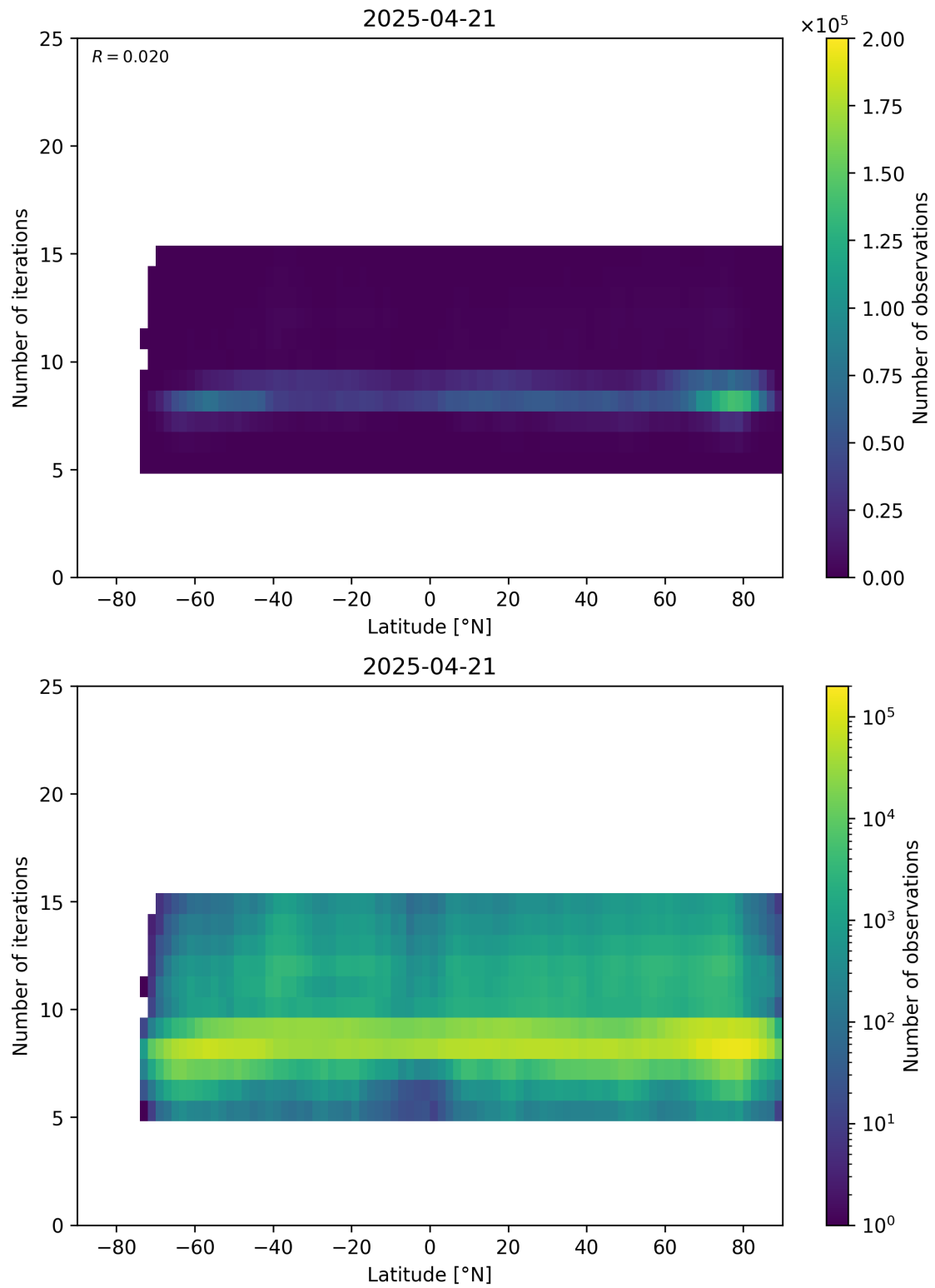
Figure 56: Scatter density plot of “Latitude” against “Number of iterations” for 2025-04-20 to 2025-04-22.
