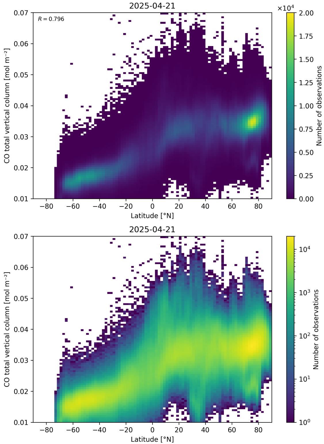
Figure 51: Scatter density plot of “Latitude” against “CO total vertical column” for 2025-04-20 to 2025-04-22.
