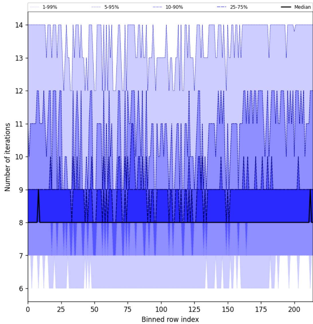
Figure 32: Along track statistics of “Number of iterations” for 2025-04-20 to 2025-04-22
