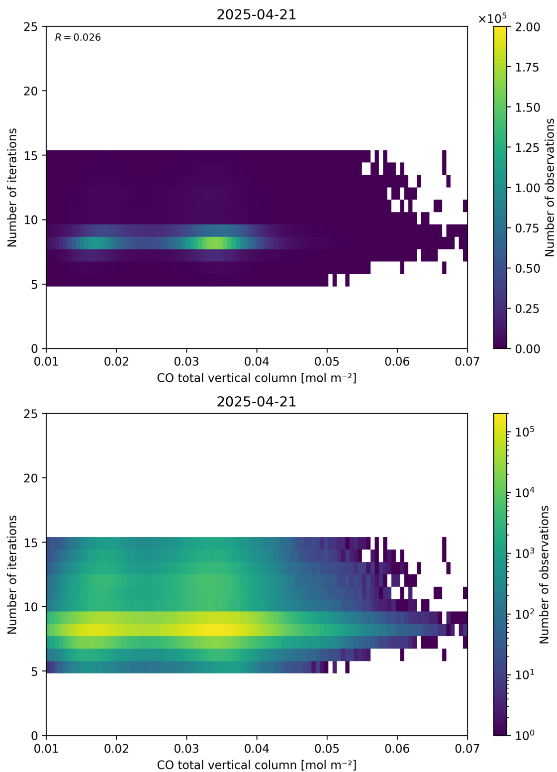
Figure 42: Scatter density plot of “CO total vertical column” against “Number of iterations” for 2025-04-20 to 2025-04-22.
