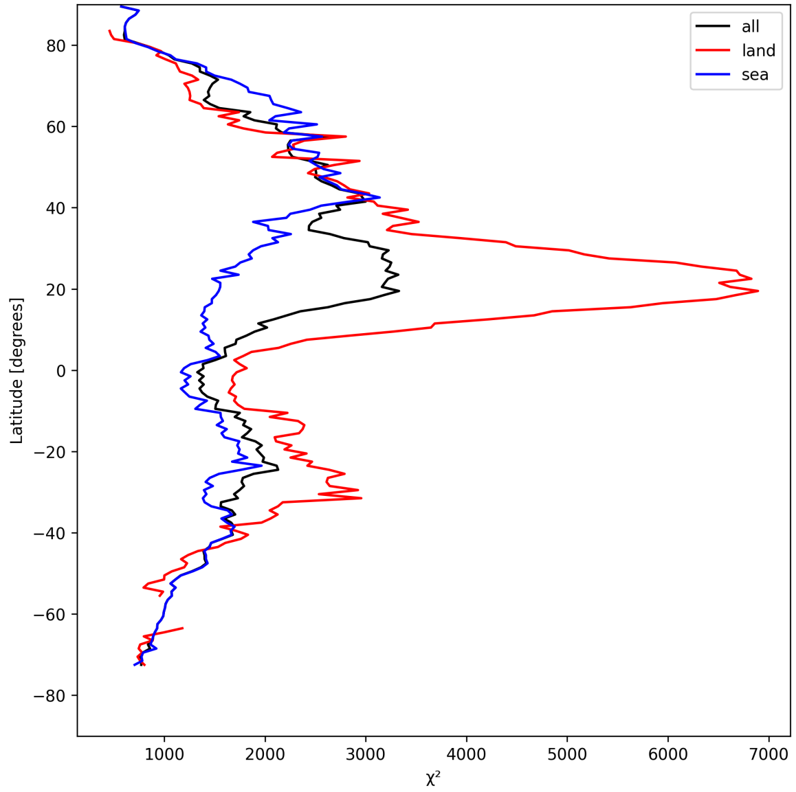
Figure 14: Zonal average of “ \chi^2 ” for 2025-04-20 to 2025-04-22.
