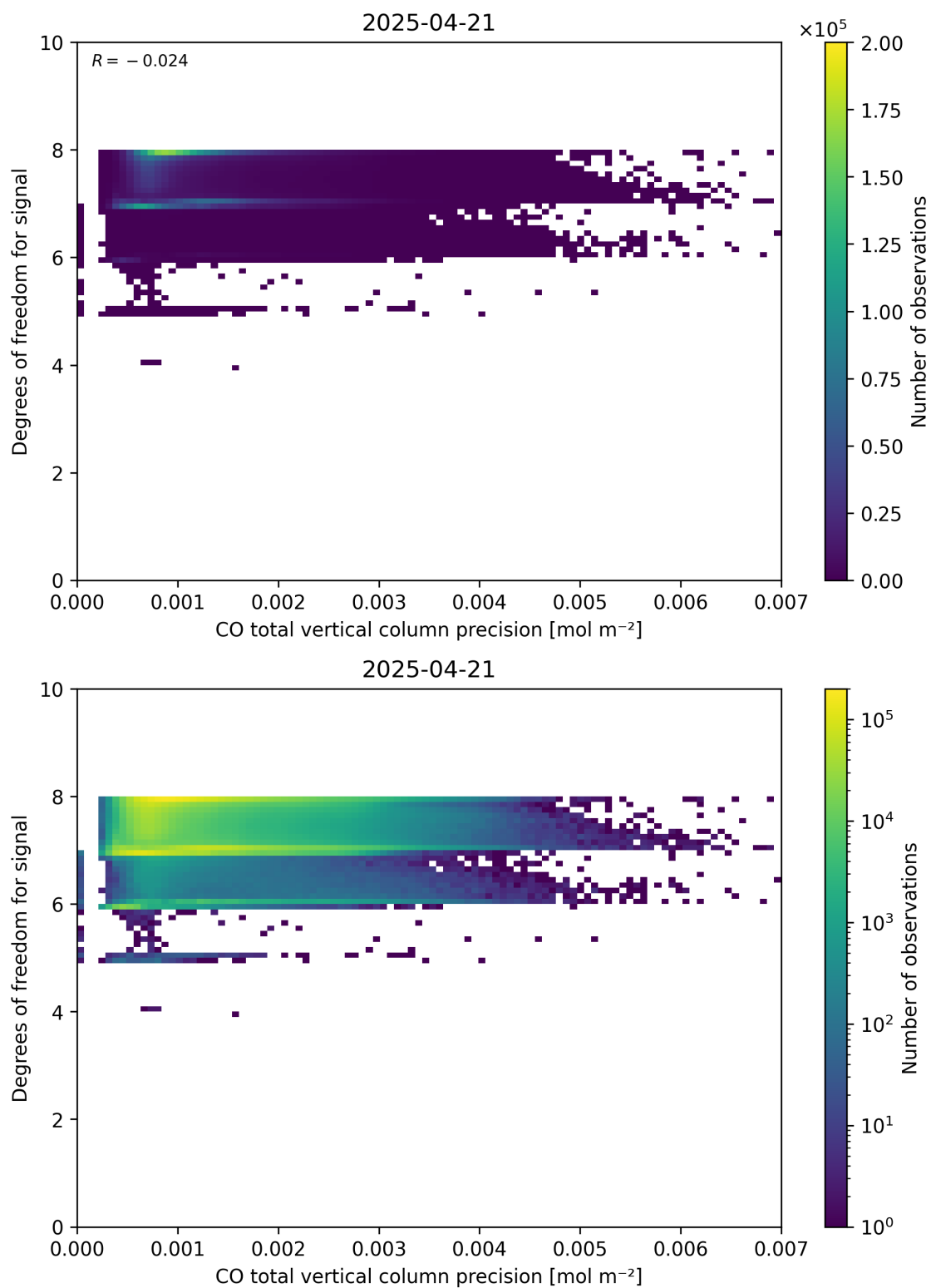
Figure 45: Scatter density plot of “CO total vertical column precision” against “Degrees of freedom for signal” for 2025-04-20 to 2025-04-22.
