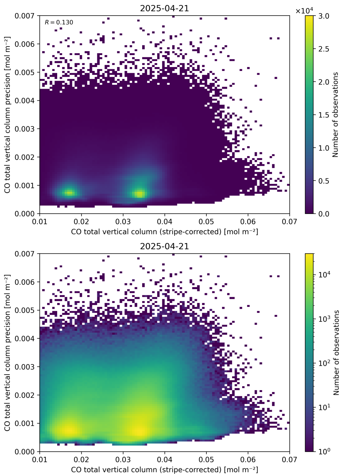
Figure 36: Scatter density plot of “CO total vertical column (stripe-corrected)” against “CO total vertical column precision” for 2025-04-20 to 2025-04-22.
