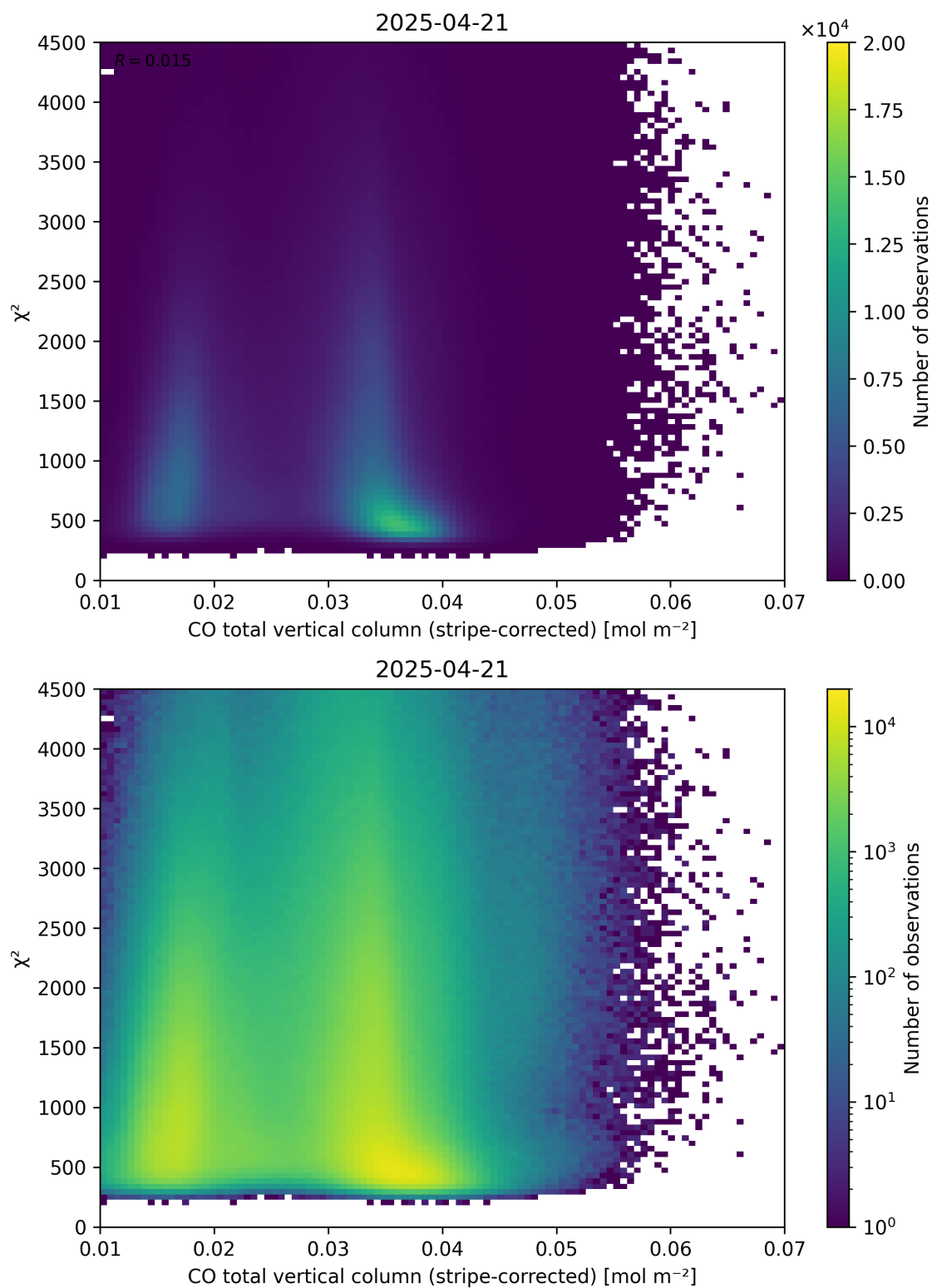
Figure 37: Scatter density plot of “CO total vertical column (stripe-corrected)” against “ \chi^2 ” for 2025-04-20 to 2025-04-22.
