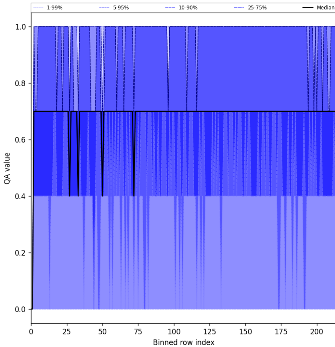
Figure 25: Along track statistics of “QA value” for 2025-04-20 to 2025-04-22
