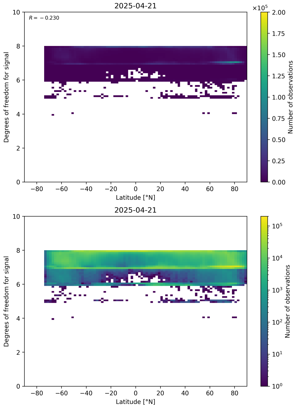
Figure 55: Scatter density plot of “Latitude” against “Degrees of freedom for signal” for 2025-04-20 to 2025-04-22.
