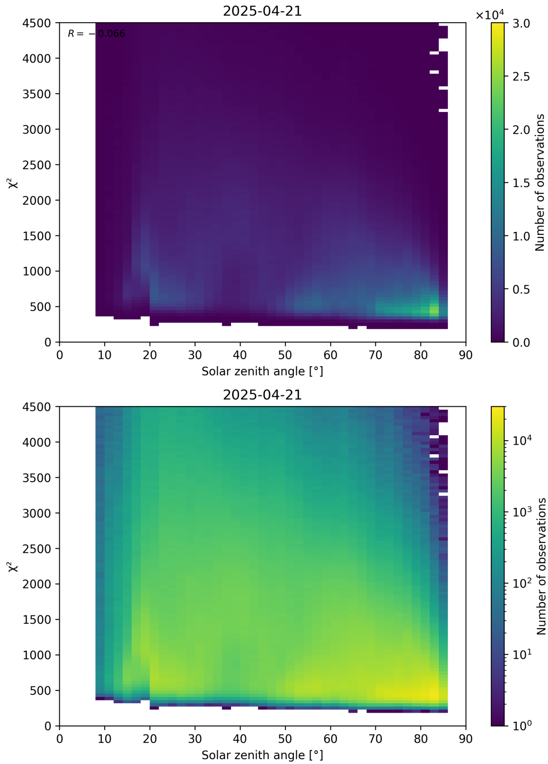
Figure 64: Scatter density plot of “Solar zenith angle” against “ \chi^2 ” for 2025-04-20 to 2025-04-22.
