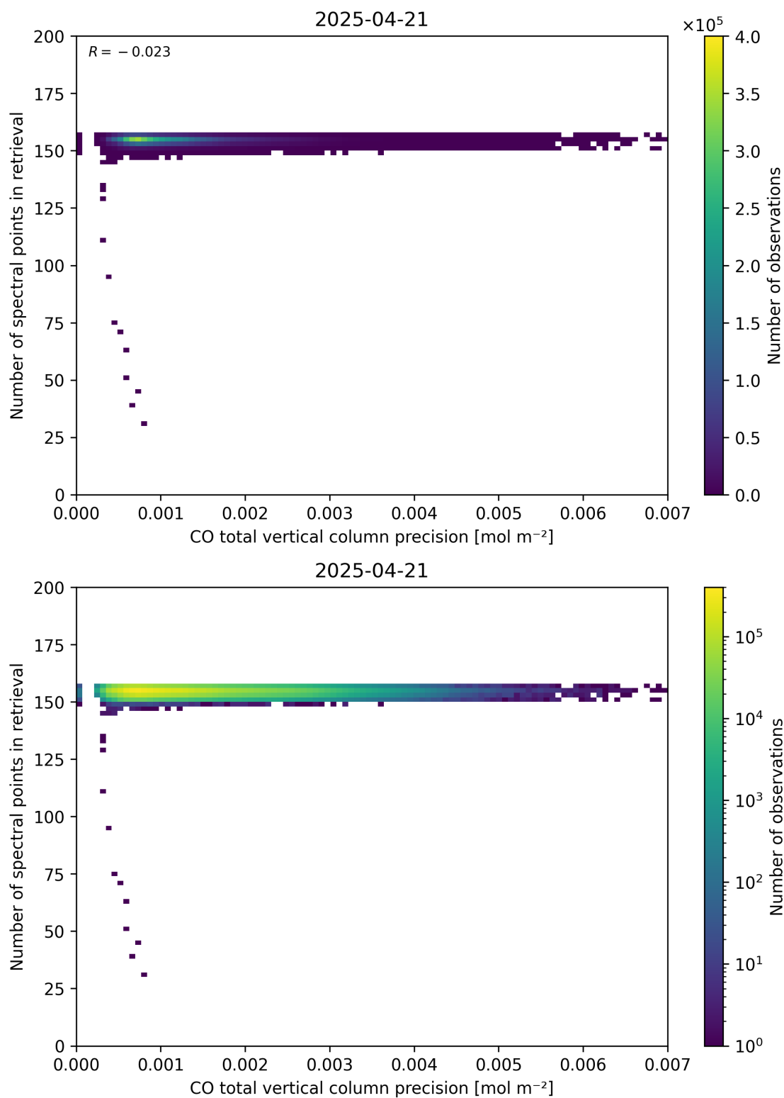
Figure 47: Scatter density plot of “CO total vertical column precision” against “Number of spectral points in retrieval” for 2025-04-20 to 2025-04-22.
