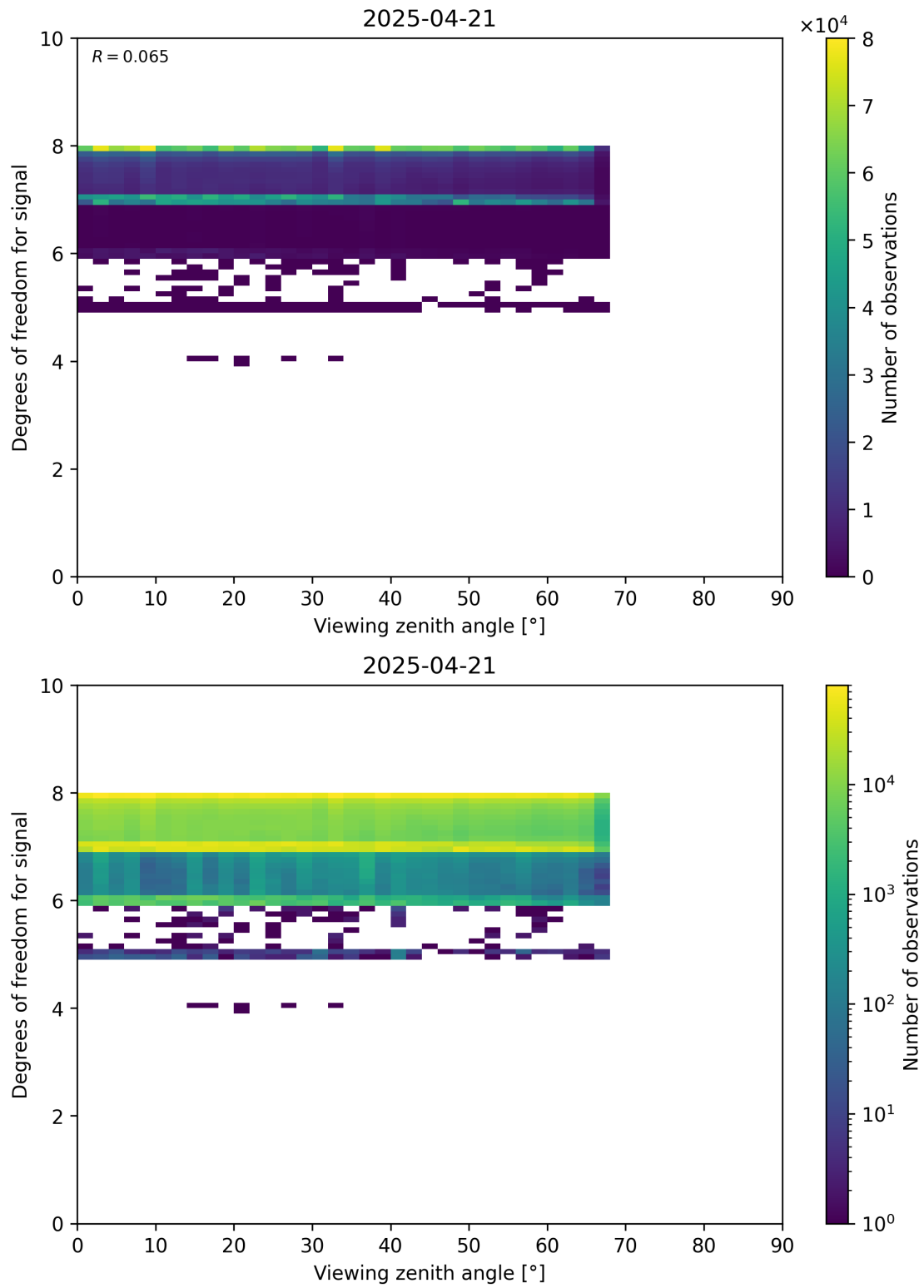
Figure 73: Scatter density plot of “Viewing zenith angle” against “Degrees of freedom for signal” for 2025-04-20 to 2025-04-22.
