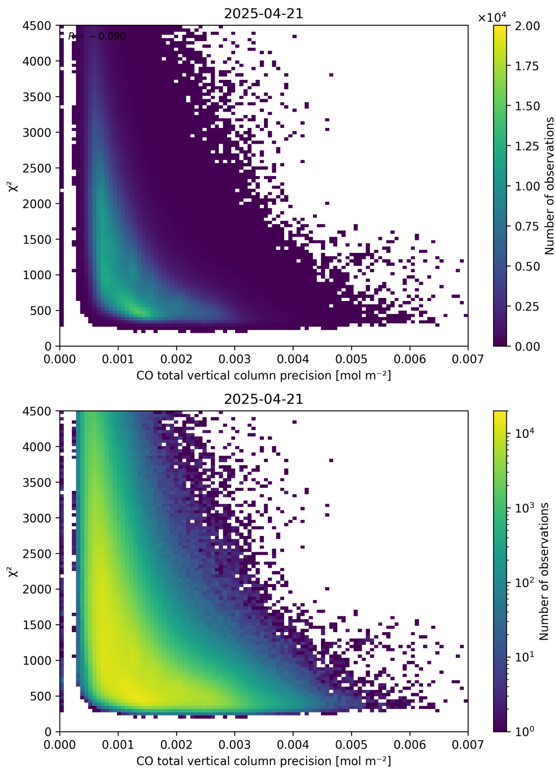
Figure 44: Scatter density plot of “CO total vertical column precision” against “ \chi^2 ” for 2025-04-20 to 2025-04-22.
