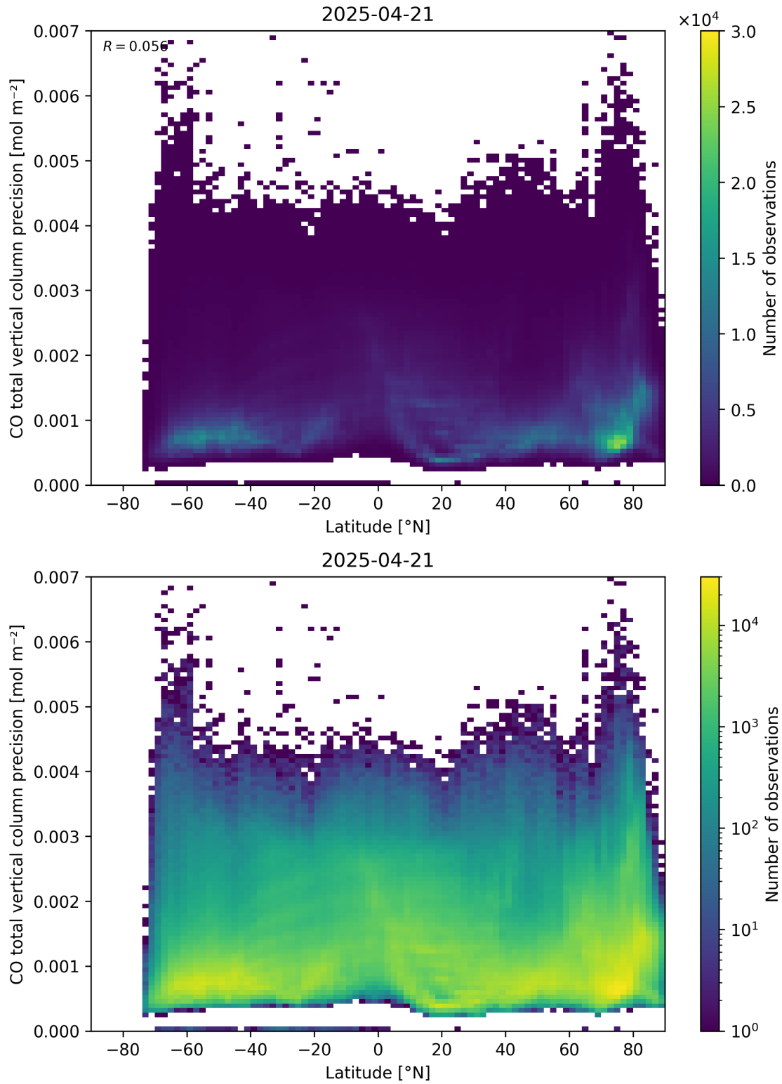
Figure 53: Scatter density plot of “Latitude” against “CO total vertical column precision” for 2025-04-20 to 2025-04-22.
