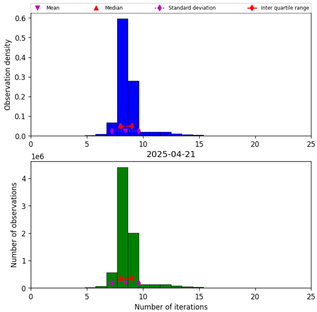
Figure 24: Histogram of “Number of iterations” for 2025-04-20 to 2025-04-22
