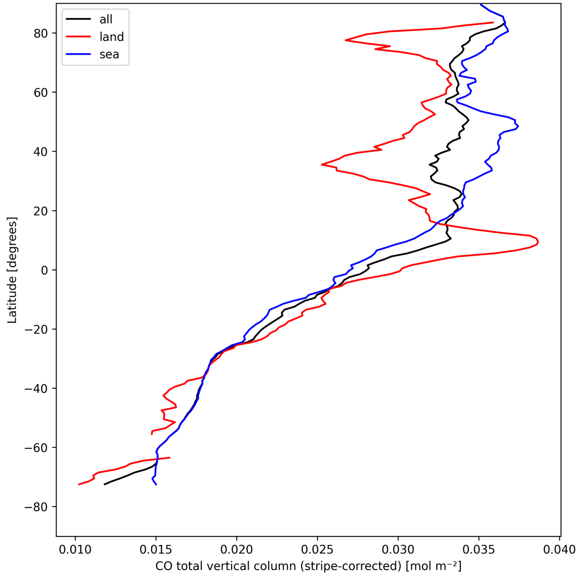
Figure 11: Zonal average of “CO total vertical column (stripe-corrected)” for 2025-04-20 to 2025-04-22.
