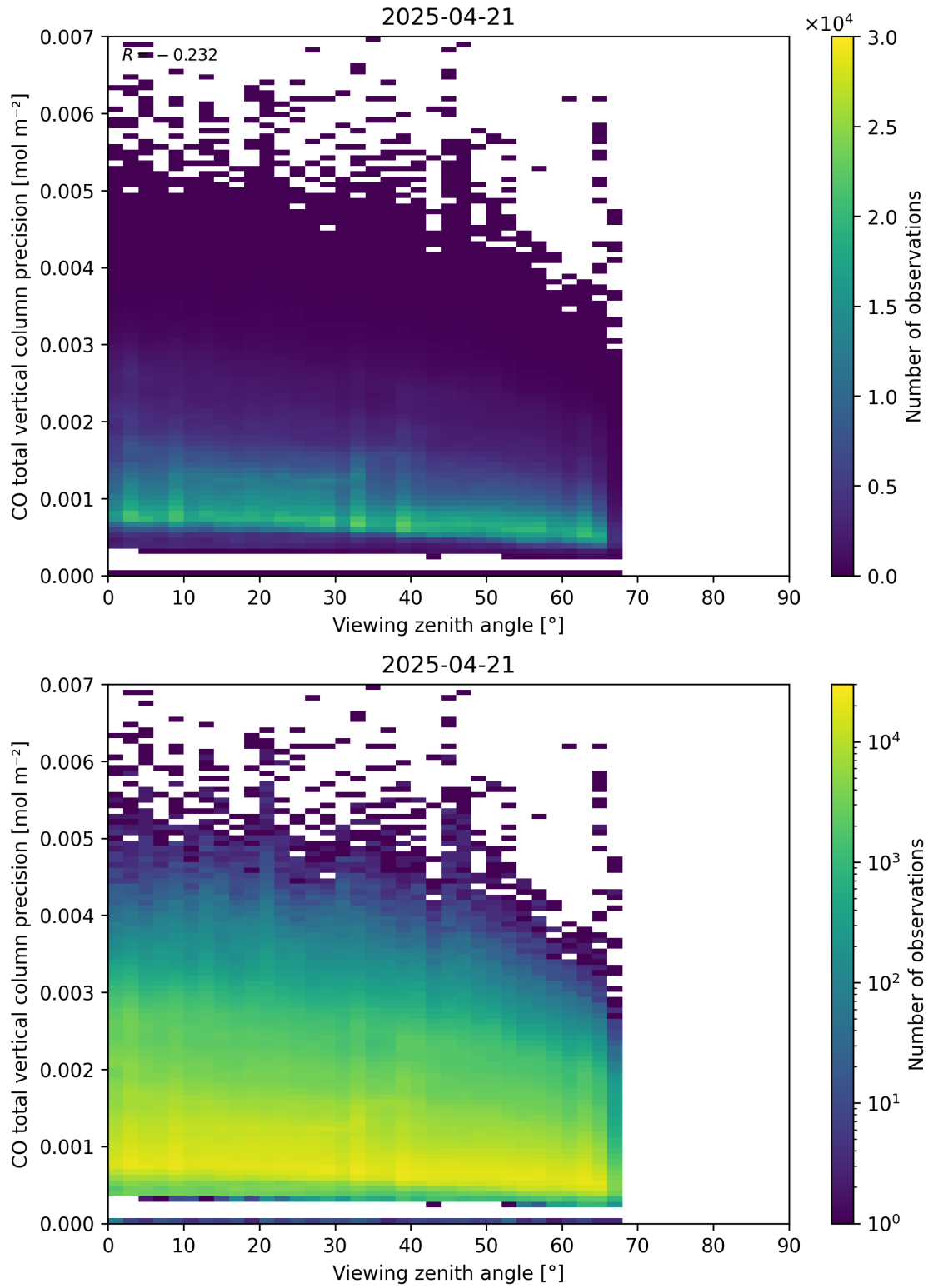
Figure 71: Scatter density plot of “Viewing zenith angle” against “CO total vertical column precision” for 2025-04-20 to 2025-04-22.
