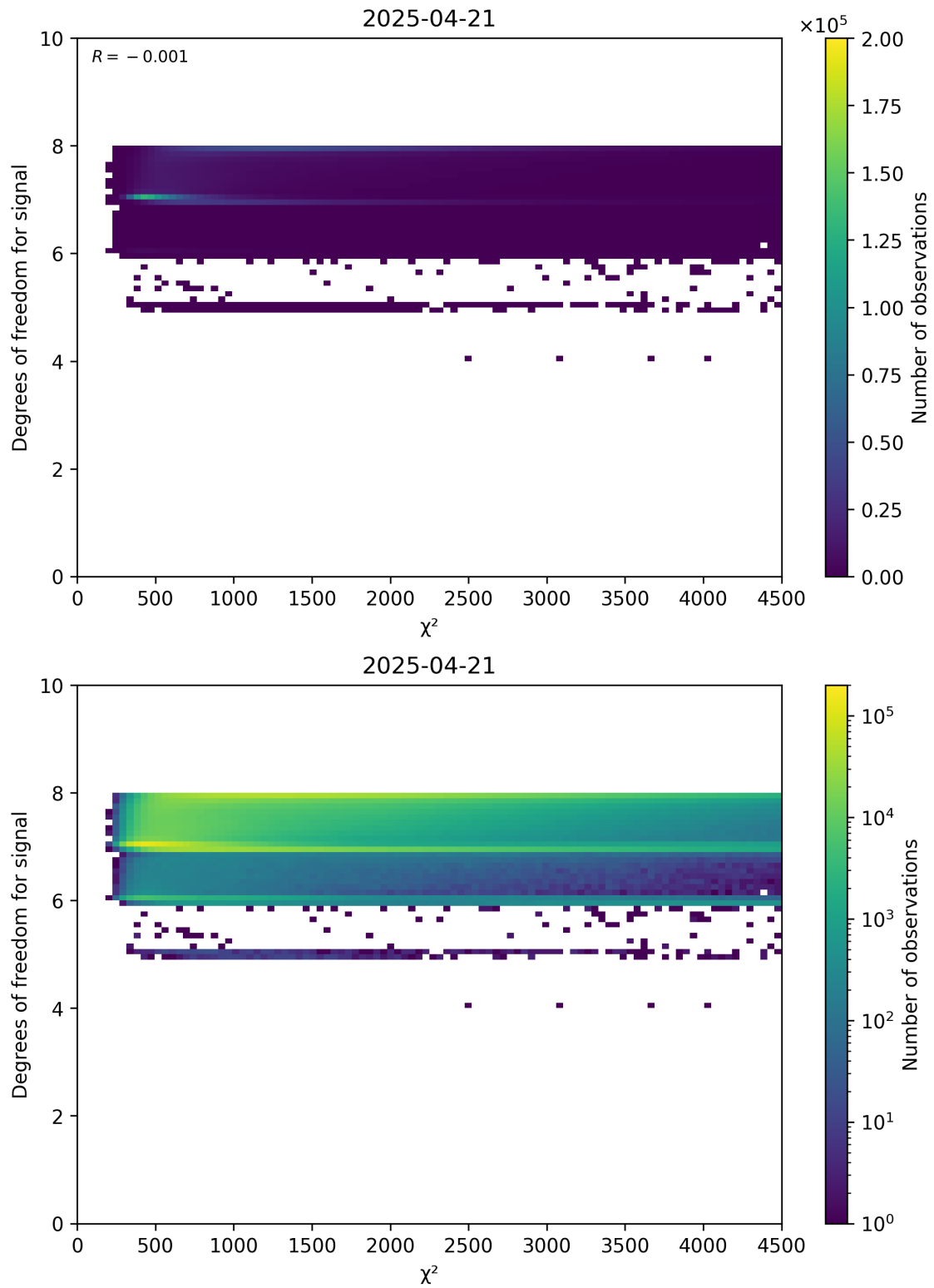
Figure 48: Scatter density plot of “ \chi^2 ” against “Degrees of freedom for signal” for 2025-04-20 to 2025-04-22.
