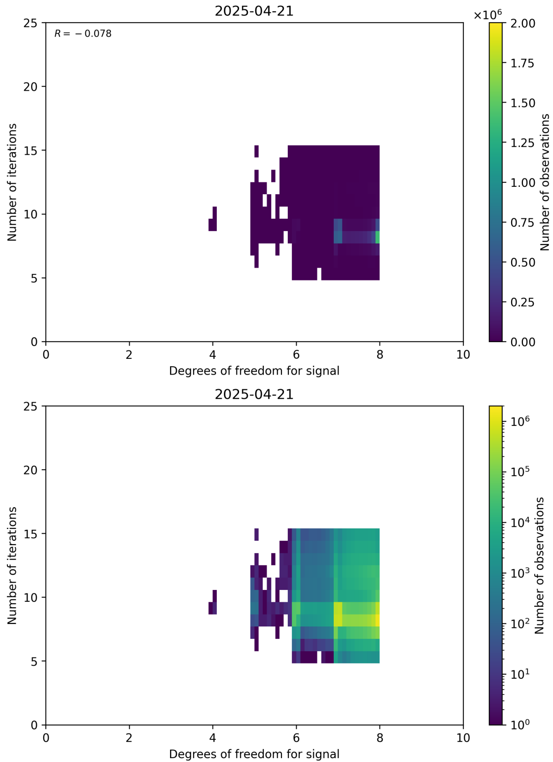
Figure 50: Scatter density plot of “Degrees of freedom for signal” against “Number of iterations” for 2025-04-20 to 2025-04-22.
