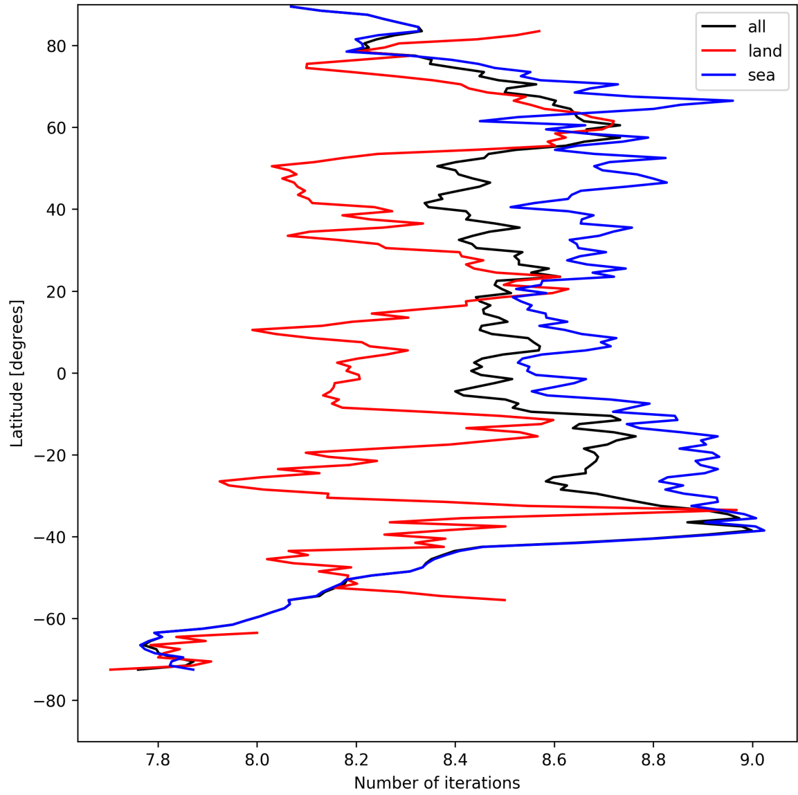
Figure 16: Zonal average of “Number of iterations” for 2025-04-20 to 2025-04-22.
