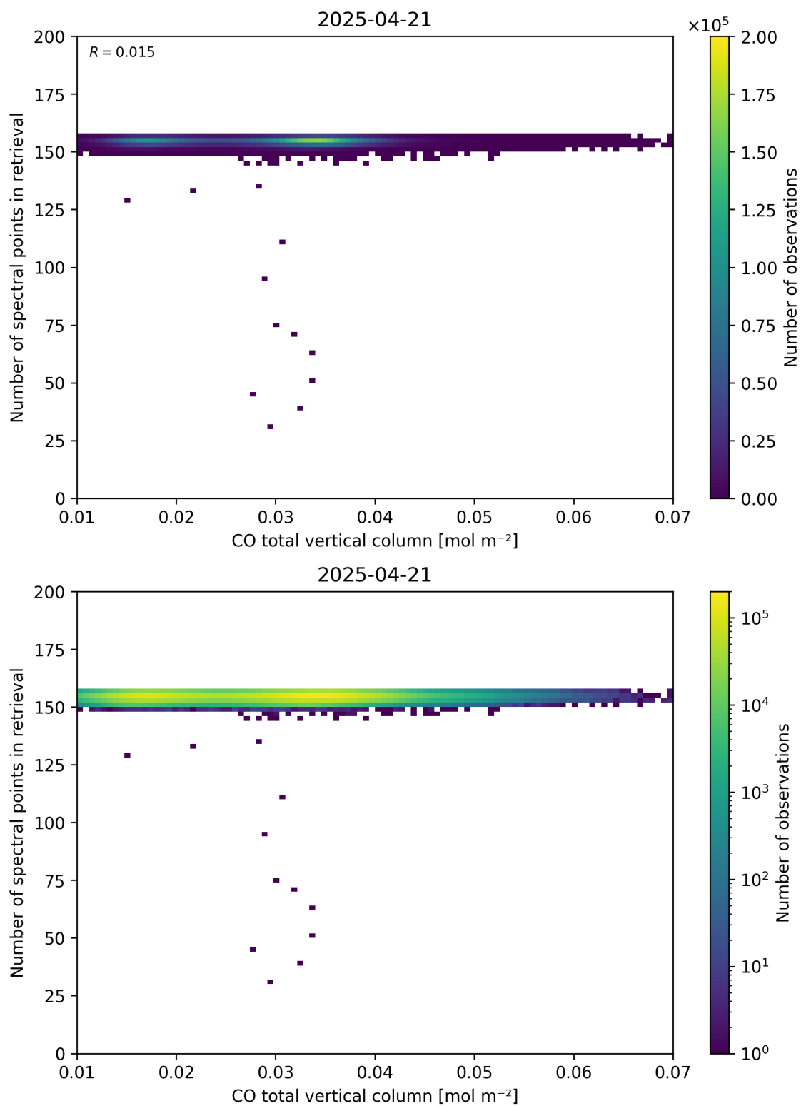
Figure 43: Scatter density plot of “CO total vertical column” against “Number of spectral points in retrieval” for 2025-04-20 to 2025-04-22.
