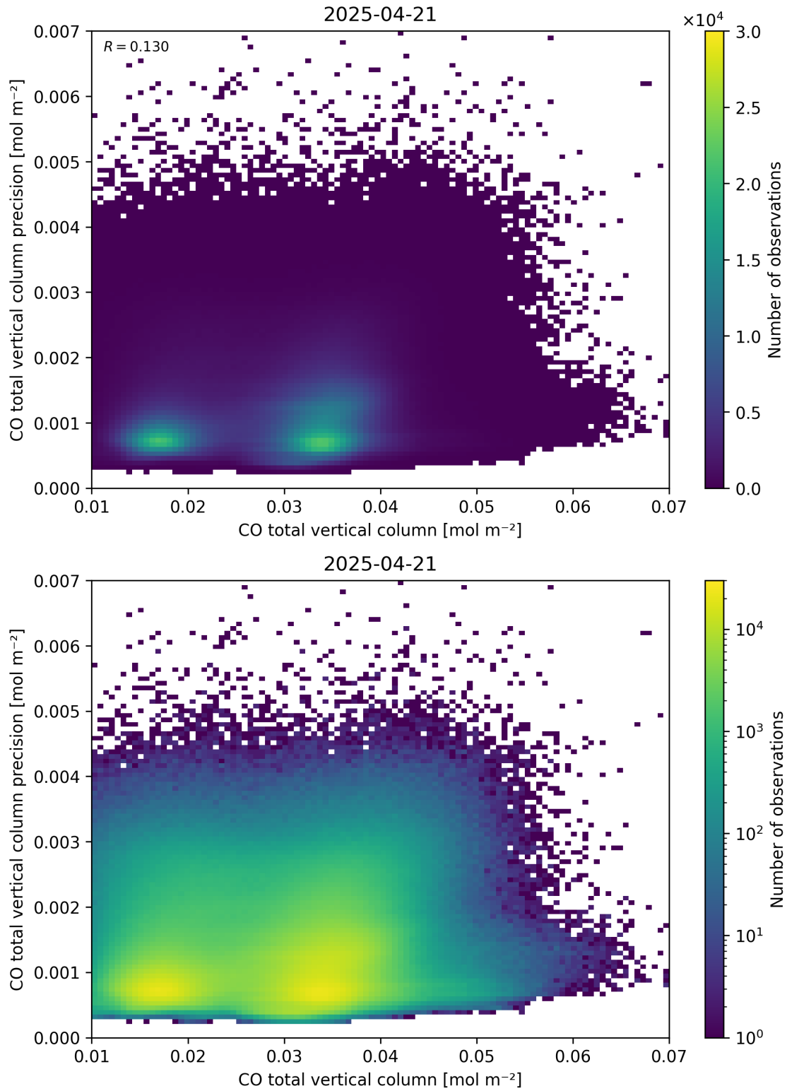
Figure 34: Scatter density plot of “CO total vertical column” against “CO total vertical column precision” for 2025-04-20 to 2025-04-22.
