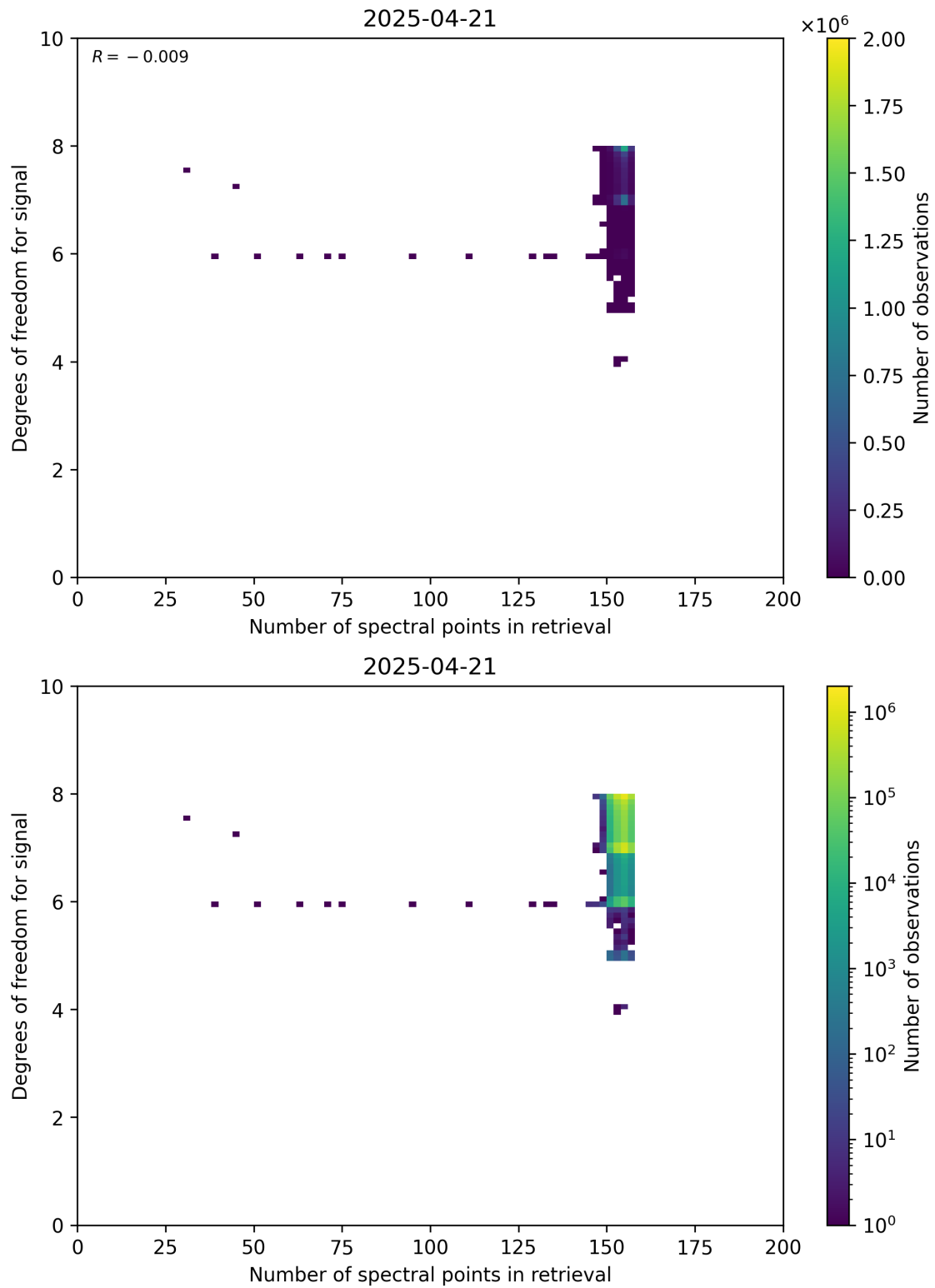
Figure 59: Scatter density plot of “Number of spectral points in retrieval” against “Degrees of freedom for signal” for 2025-04-20 to 2025-04-22.
