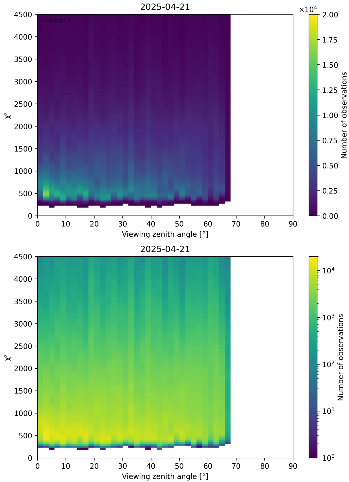
Figure 72: Scatter density plot of “Viewing zenith angle” against “ \chi^2 ” for 2025-04-20 to 2025-04-22.
