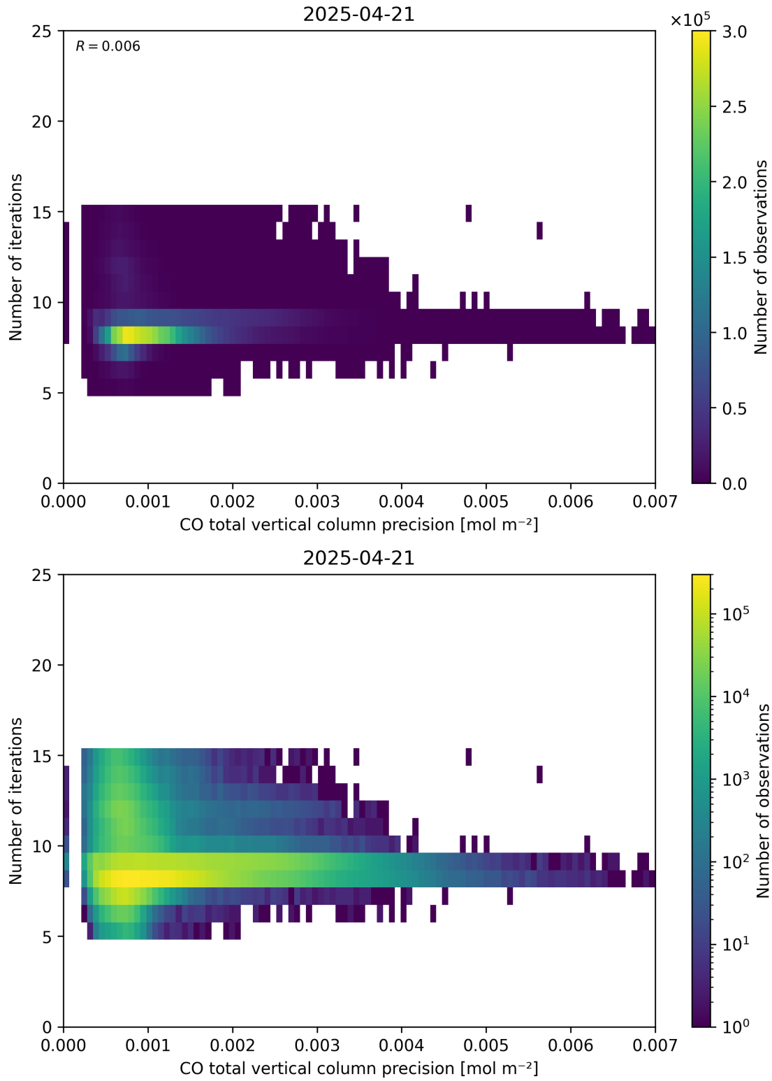
Figure 46: Scatter density plot of “CO total vertical column precision” against “Number of iterations” for 2025-04-20 to 2025-04-22.
