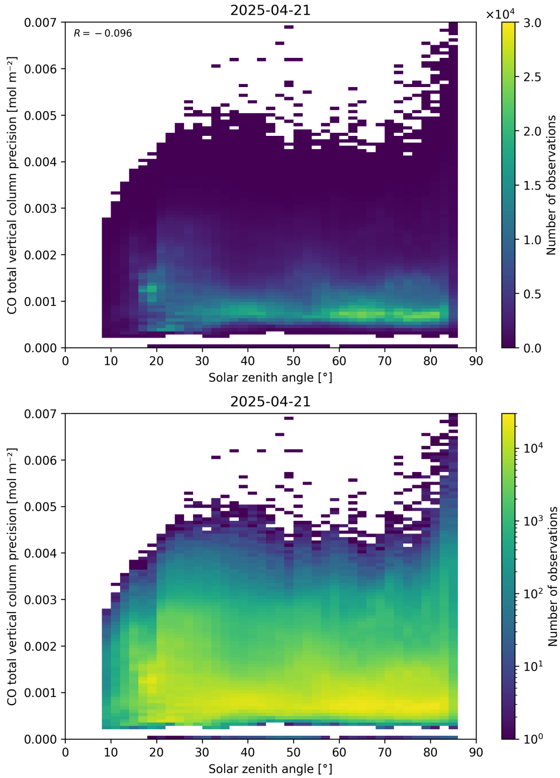
Figure 63: Scatter density plot of “Solar zenith angle” against “CO total vertical column precision” for 2025-04-20 to 2025-04-22.
