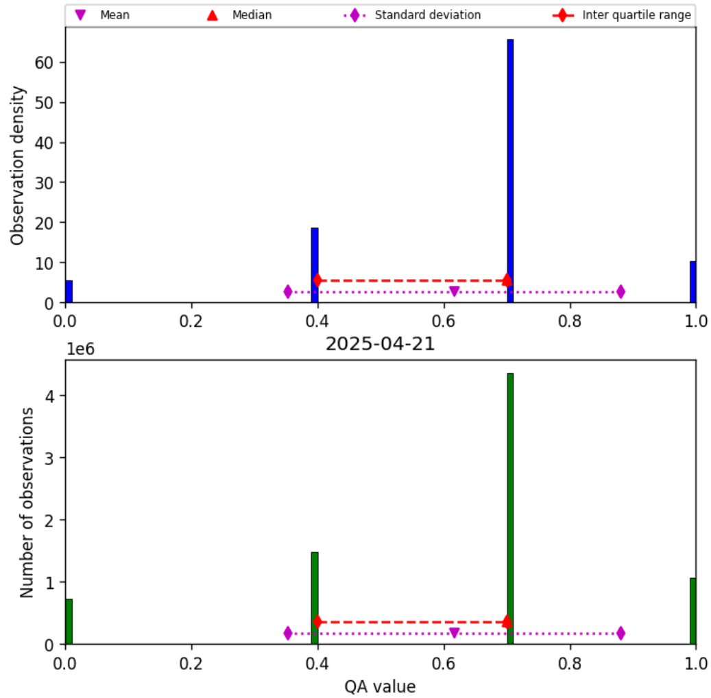
Figure 17: Histogram of “QA value” for 2025-04-20 to 2025-04-22
