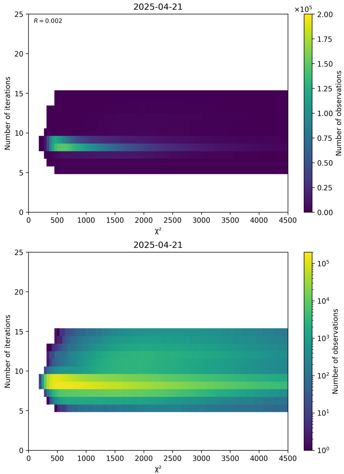
Figure 49: Scatter density plot of “ \chi^2 ” against “Number of iterations” for 2025-04-20 to 2025-04-22.
