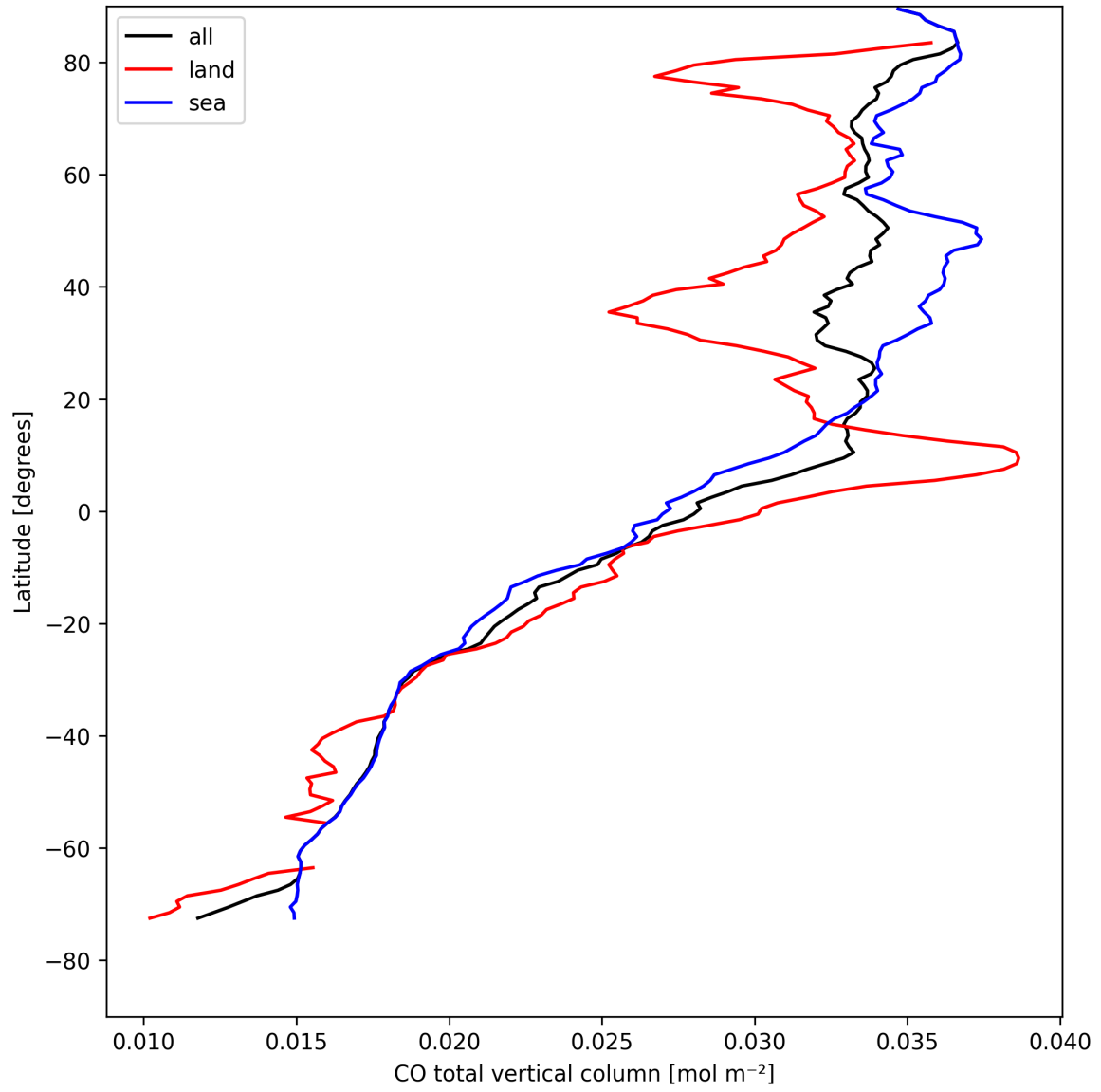
Figure 10: Zonal average of “CO total vertical column” for 2025-04-20 to 2025-04-22.
