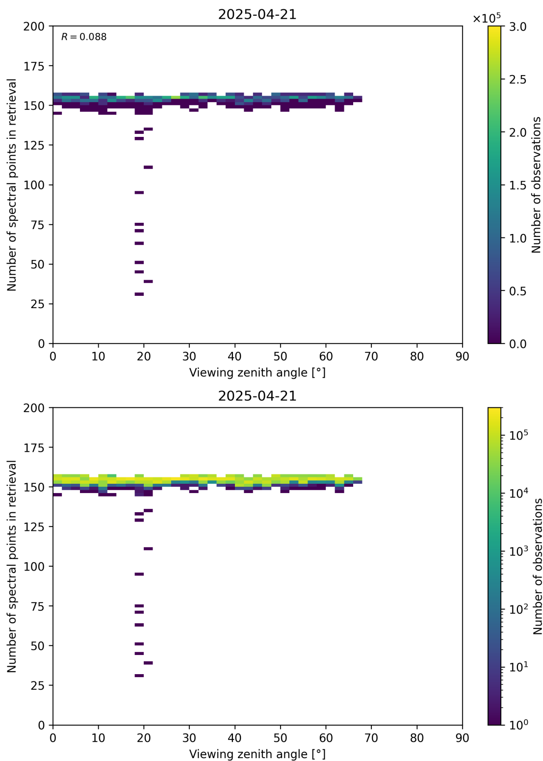
Figure 76: Scatter density plot of “Viewing zenith angle” against “Number of spectral points in retrieval” for 2025-04-20 to 2025-04-22.
