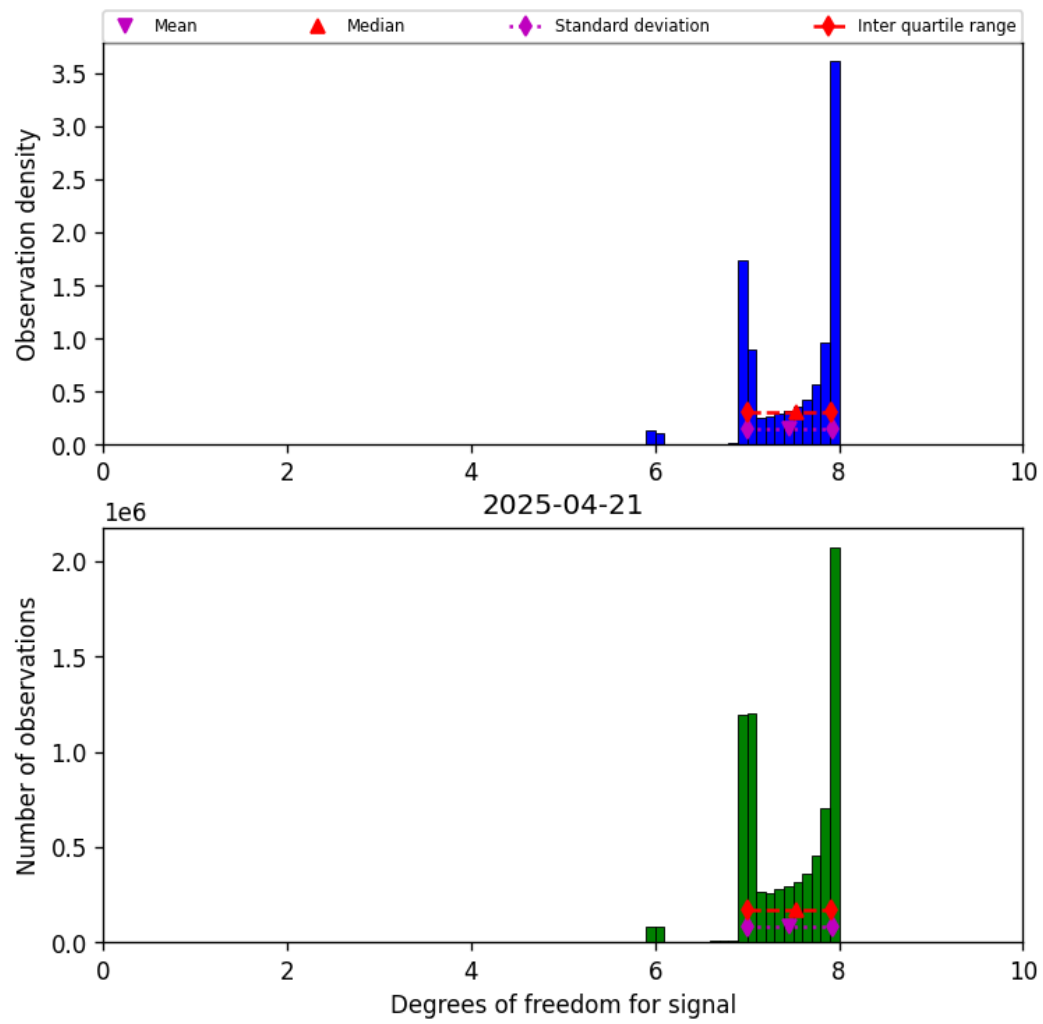
Figure 23: Histogram of “Degrees of freedom for signal” for 2025-04-20 to 2025-04-22
