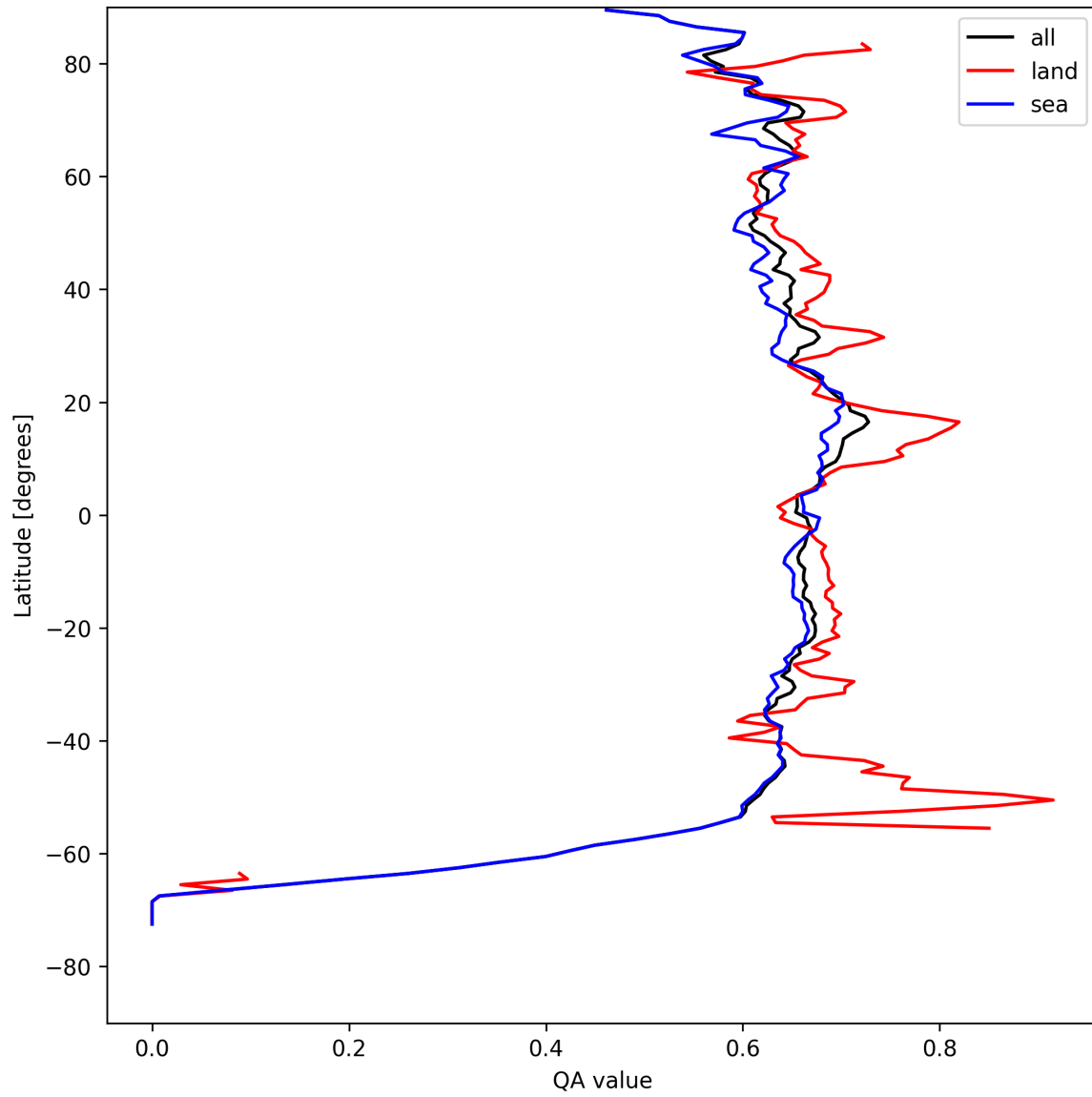
Figure 9: Zonal average of “QA value” for 2025-04-20 to 2025-04-22.
