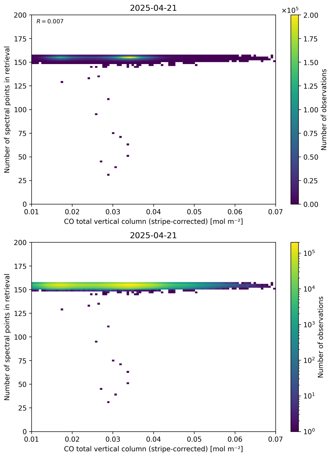
Figure 40: Scatter density plot of “CO total vertical column (stripe-corrected)” against “Number of spectral points in retrieval” for 2025-04-20 to 2025-04-22.
