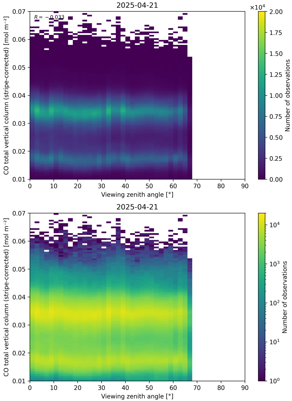
Figure 70: Scatter density plot of “Viewing zenith angle” against “CO total vertical column (stripe-corrected)” for 2025-04-20 to 2025-04-22.
