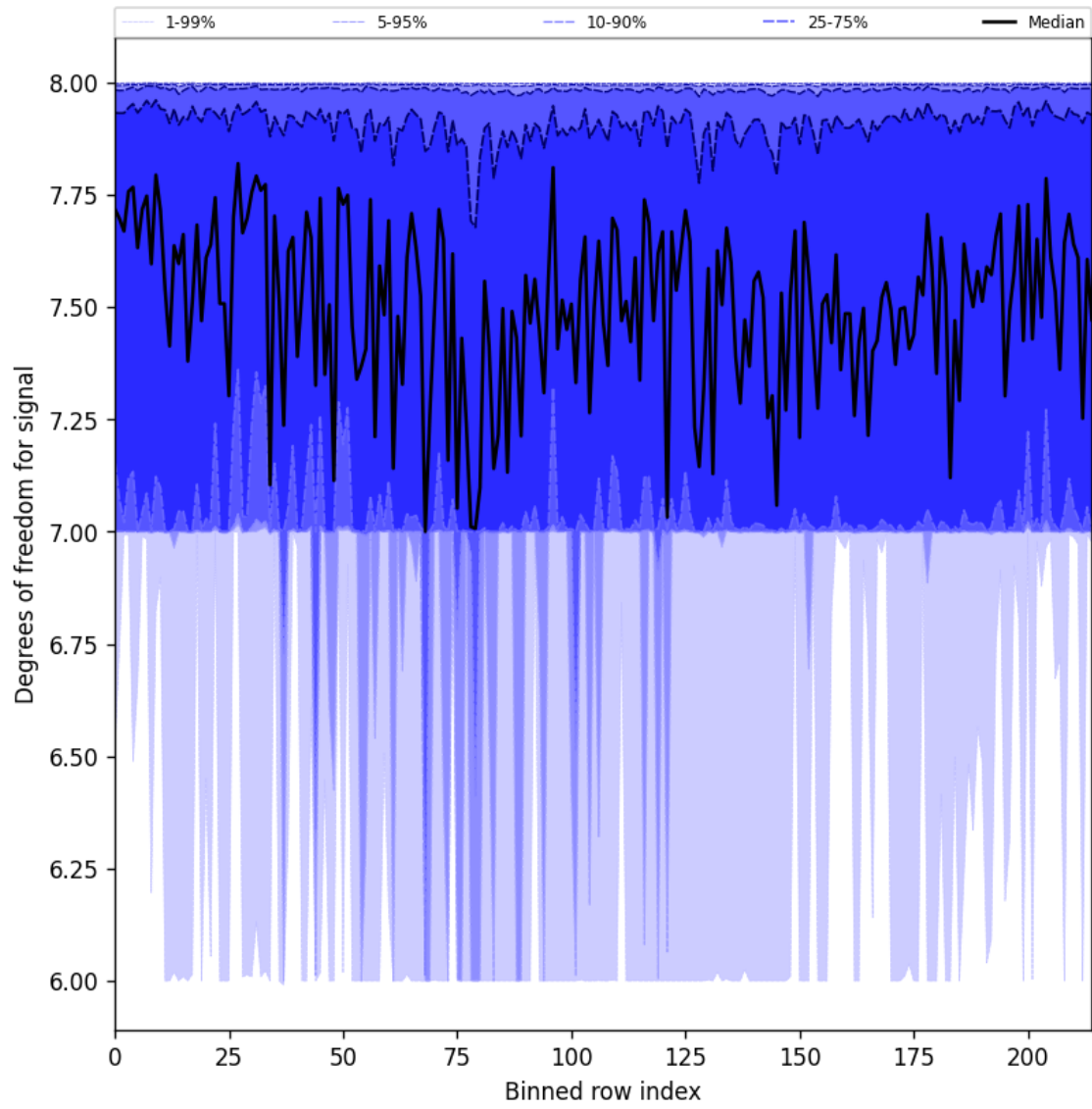
Figure 31: Along track statistics of “Degrees of freedom for signal” for 2025-04-20 to 2025-04-22
