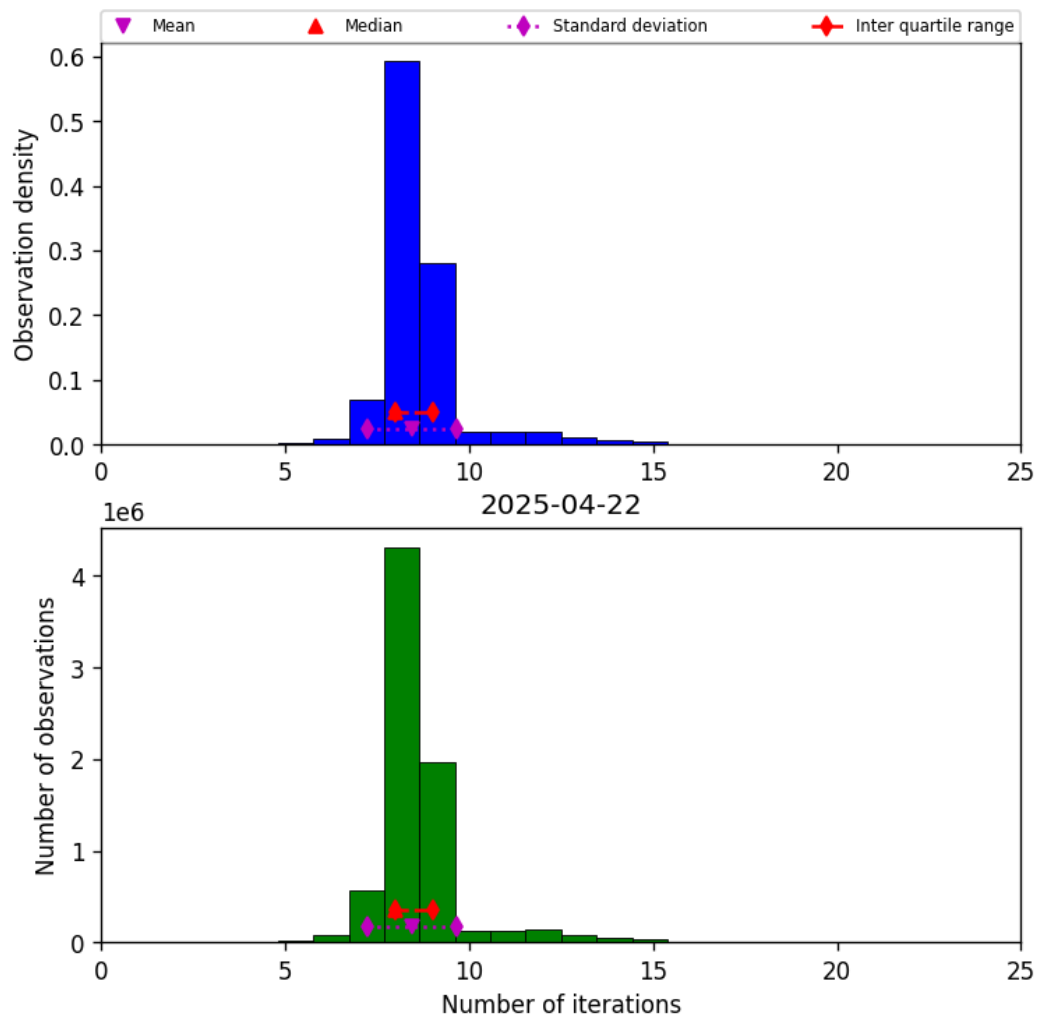
Figure 24: Histogram of “Number of iterations” for 2025-04-21 to 2025-04-23
