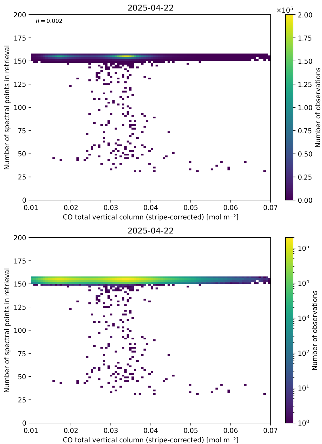
Figure 40: Scatter density plot of “CO total vertical column (stripe-corrected)” against “Number of spectral points in retrieval” for 2025-04-21 to 2025-04-23.
