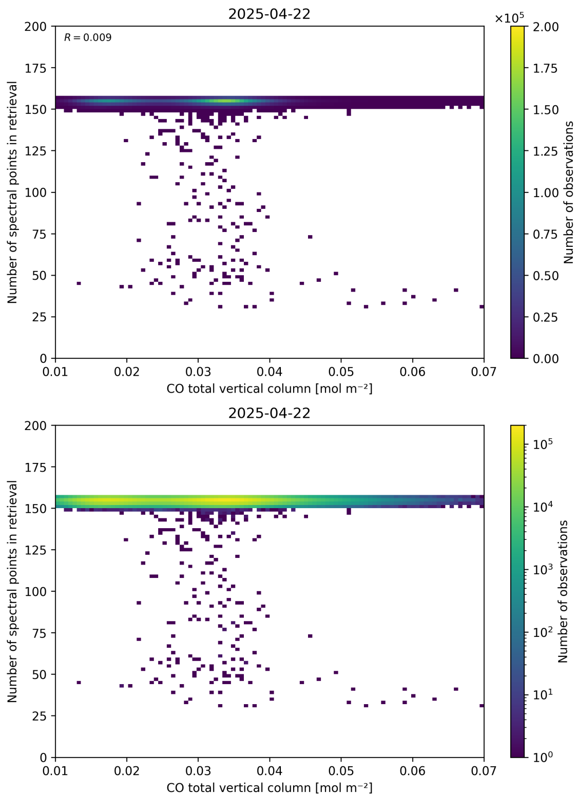
Figure 43: Scatter density plot of “CO total vertical column” against “Number of spectral points in retrieval” for 2025-04-21 to 2025-04-23.
