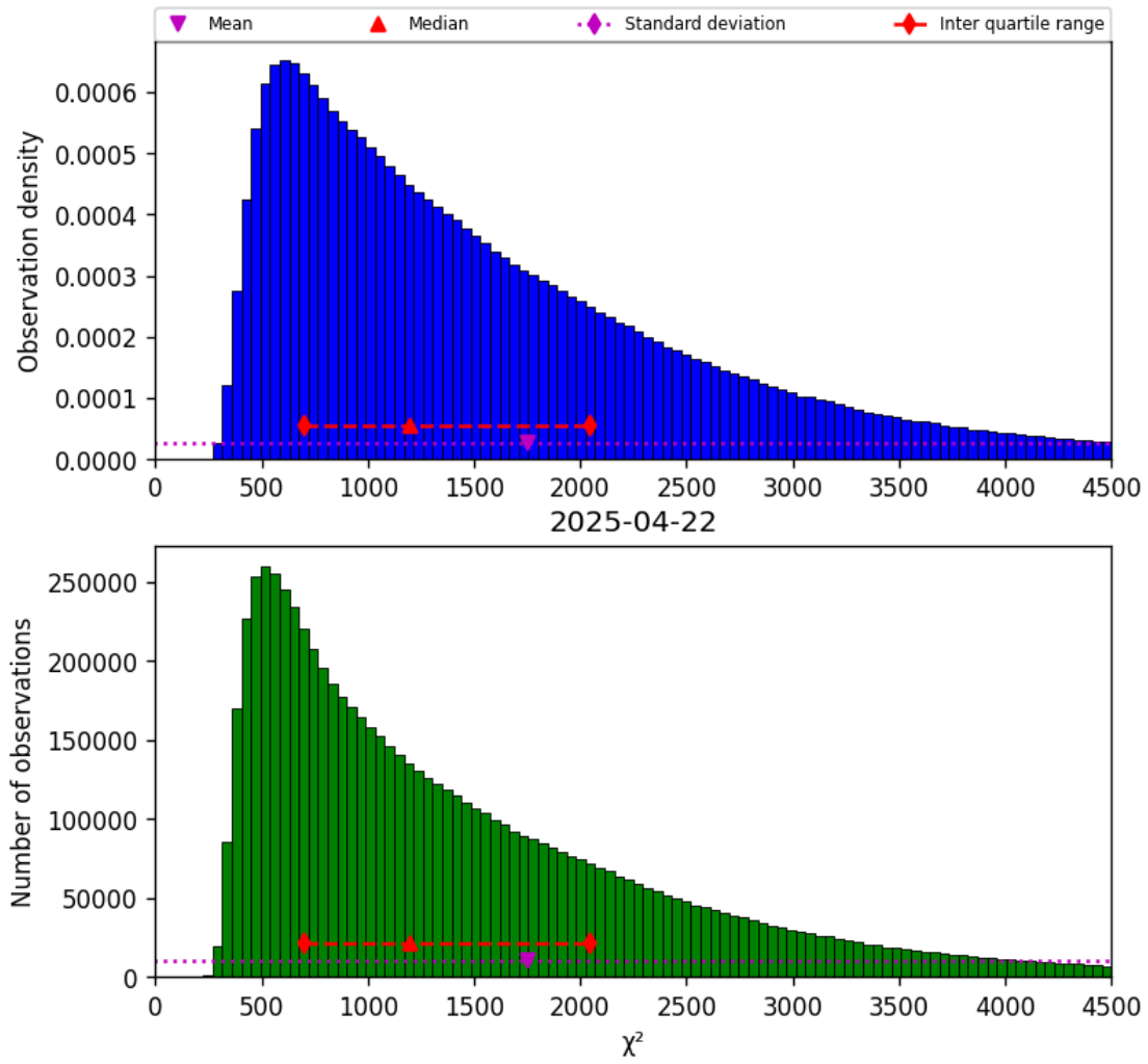
Figure 22: Histogram of “ \chi^2 ” for 2025-04-21 to 2025-04-23
