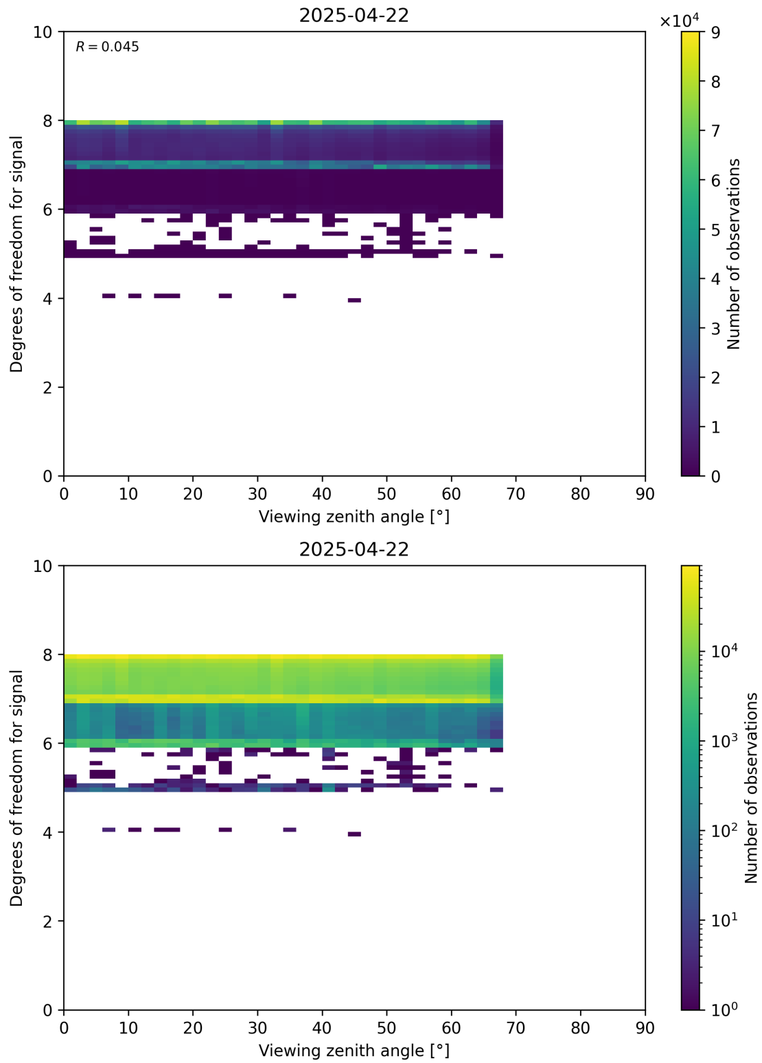
Figure 73: Scatter density plot of “Viewing zenith angle” against “Degrees of freedom for signal” for 2025-04-21 to 2025-04-23.
