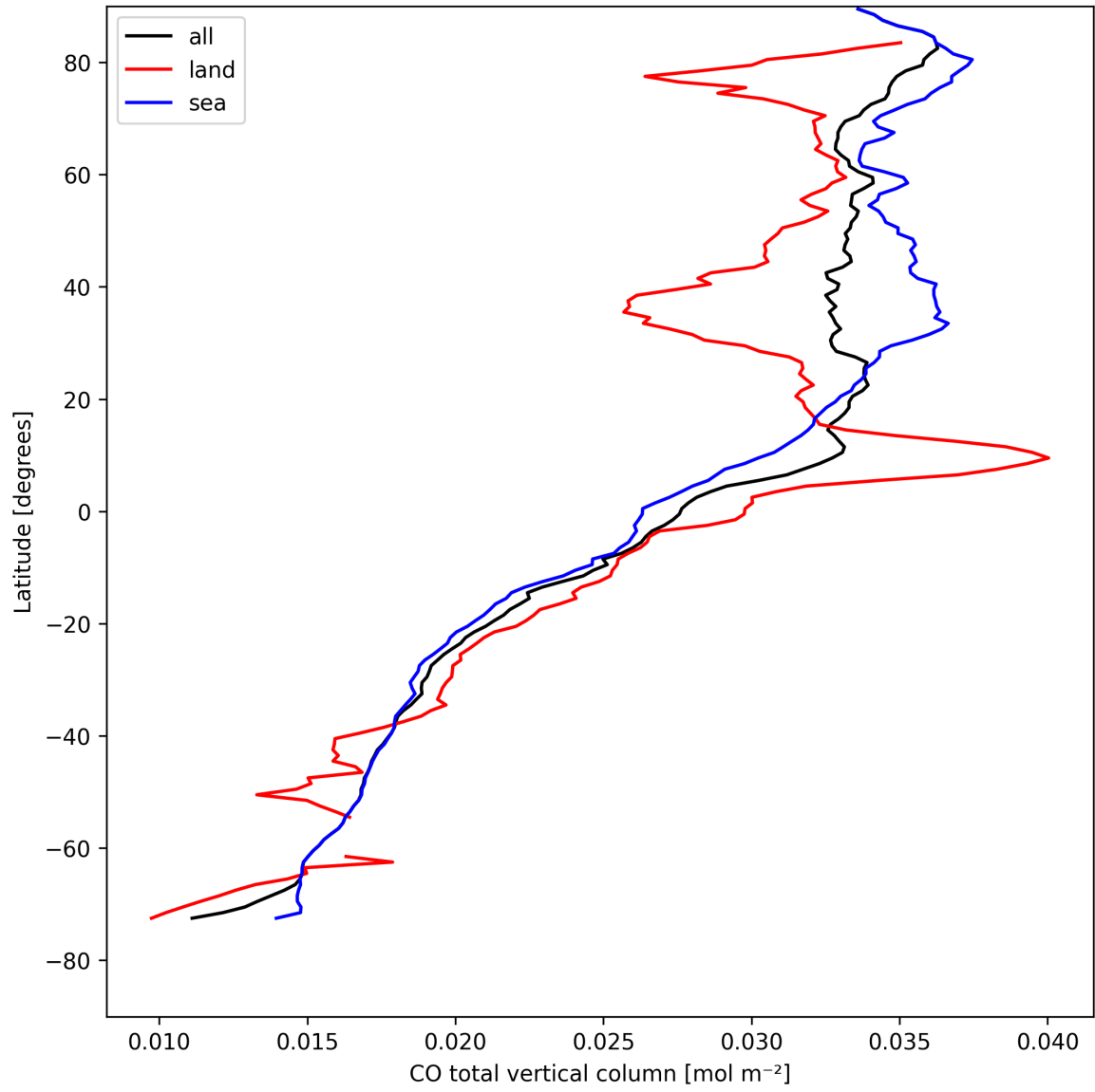
Figure 10: Zonal average of “CO total vertical column” for 2025-04-21 to 2025-04-23.
