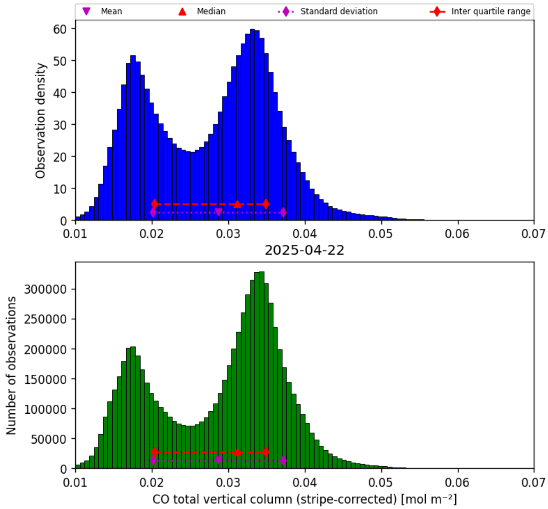
Figure 19: Histogram of “CO total vertical column (stripe-corrected)” for 2025-04-21 to 2025-04-23
