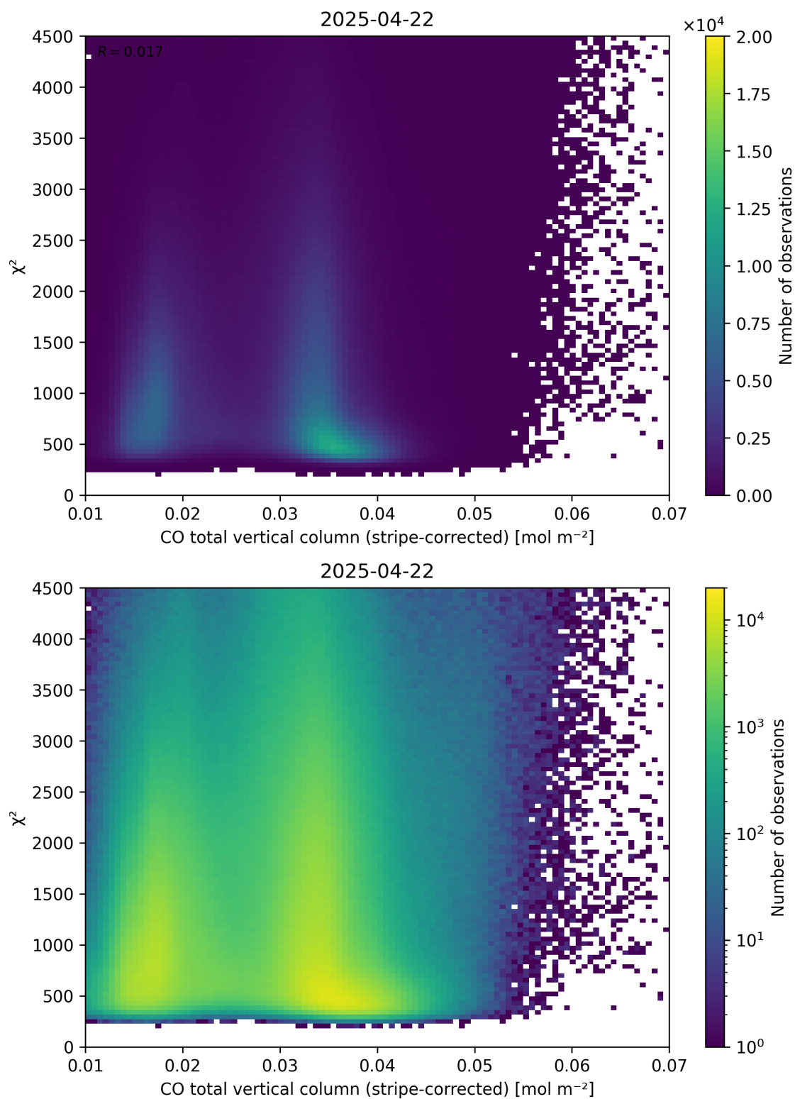
Figure 37: Scatter density plot of “CO total vertical column (stripe-corrected)” against “ \chi^2 ” for 2025-04-21 to 2025-04-23.
