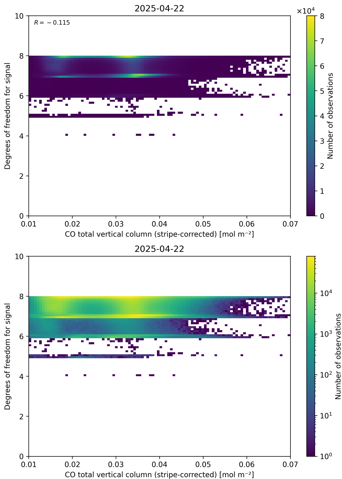
Figure 38: Scatter density plot of “CO total vertical column (stripe-corrected)” against “Degrees of freedom for signal” for 2025-04-21 to 2025-04-23.
