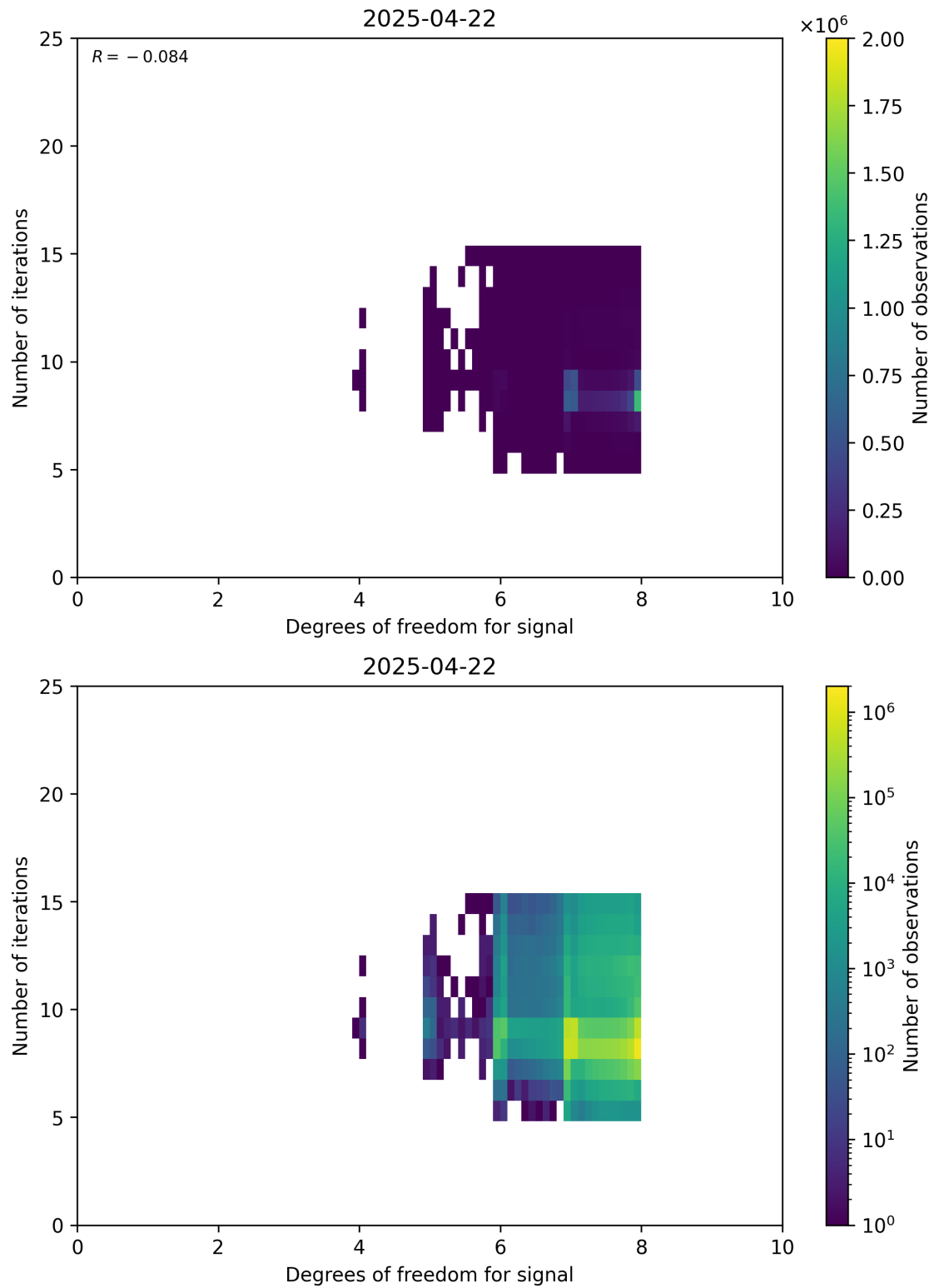
Figure 50: Scatter density plot of “Degrees of freedom for signal” against “Number of iterations” for 2025-04-21 to 2025-04-23.
