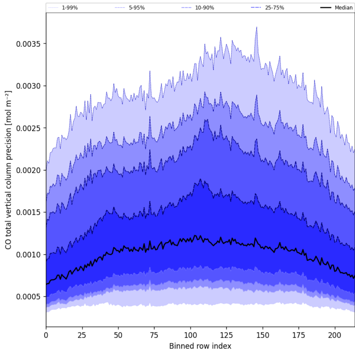
Figure 28: Along track statistics of “CO total vertical column precision” for 2025-04-21 to 2025-04-23
