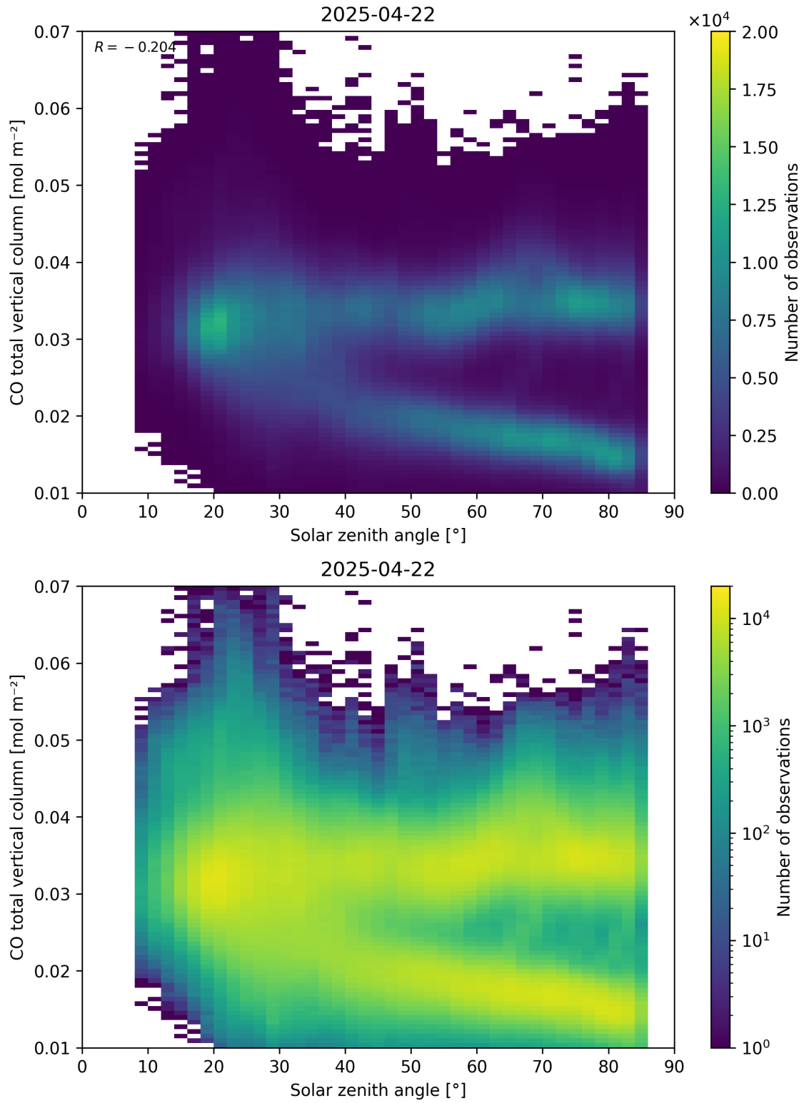
Figure 61: Scatter density plot of “Solar zenith angle” against “CO total vertical column” for 2025-04-21 to 2025-04-23.
