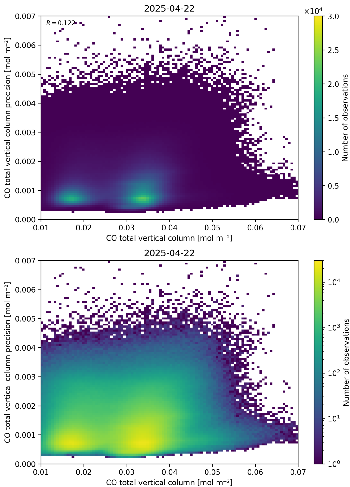
Figure 34: Scatter density plot of “CO total vertical column” against “CO total vertical column precision” for 2025-04-21 to 2025-04-23.
