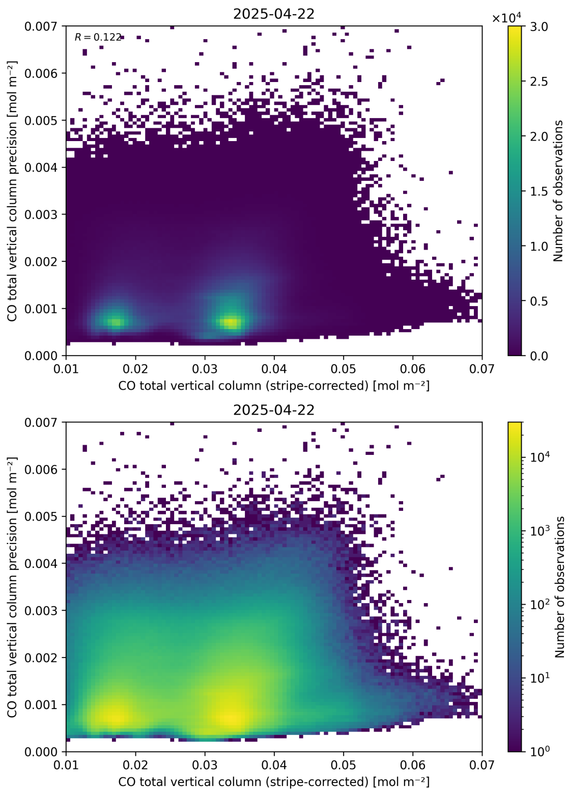
Figure 36: Scatter density plot of “CO total vertical column (stripe-corrected)” against “CO total vertical column precision” for 2025-04-21 to 2025-04-23.
