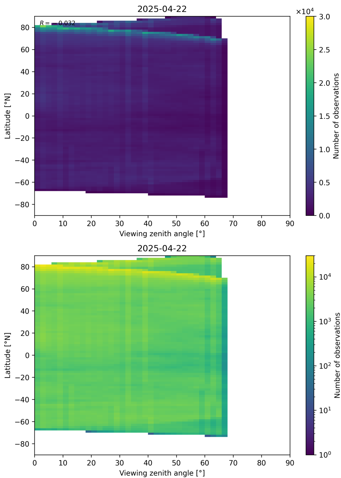
Figure 74: Scatter density plot of “Viewing zenith angle” against “Latitude” for 2025-04-21 to 2025-04-23.
