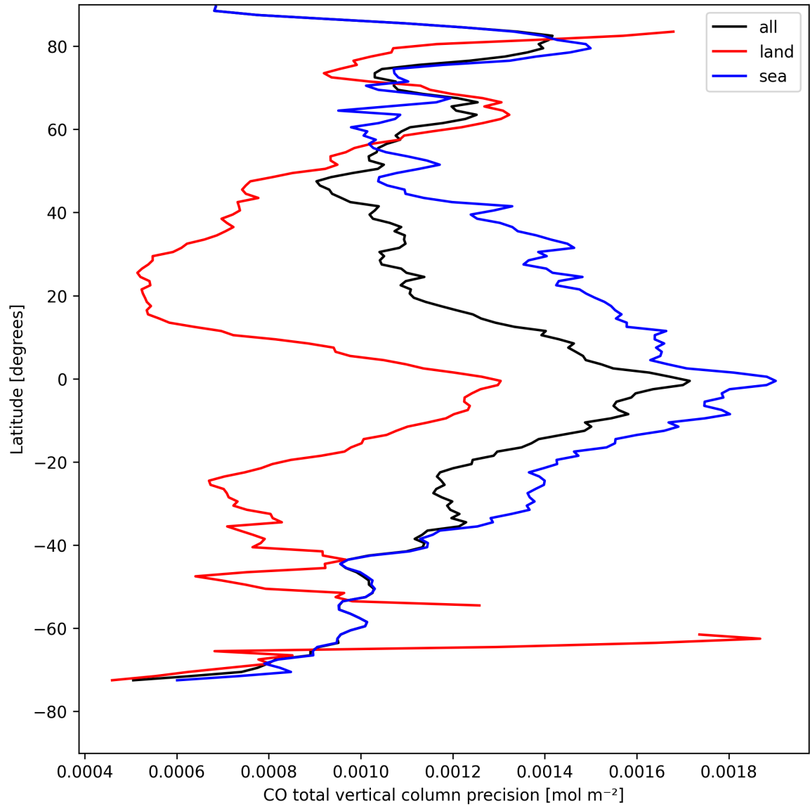
Figure 12: Zonal average of “CO total vertical column precision” for 2025-04-21 to 2025-04-23.
