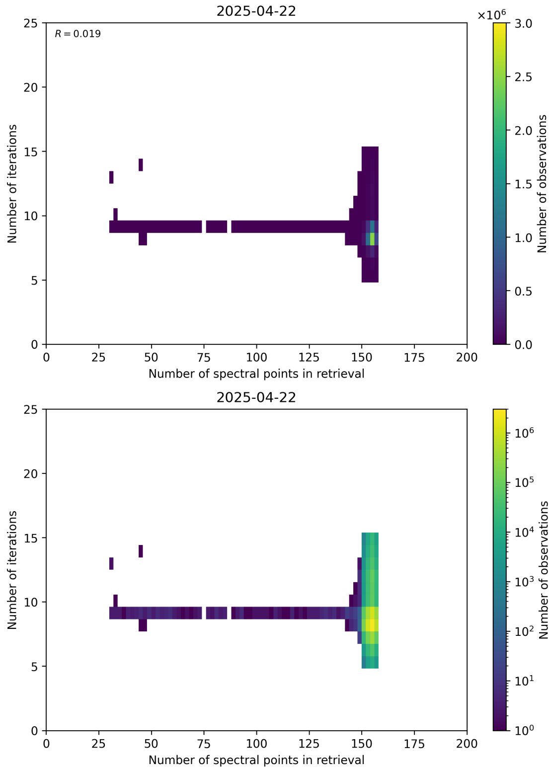
Figure 60: Scatter density plot of “Number of spectral points in retrieval” against “Number of iterations” for 2025-04-21 to 2025-04-23.
