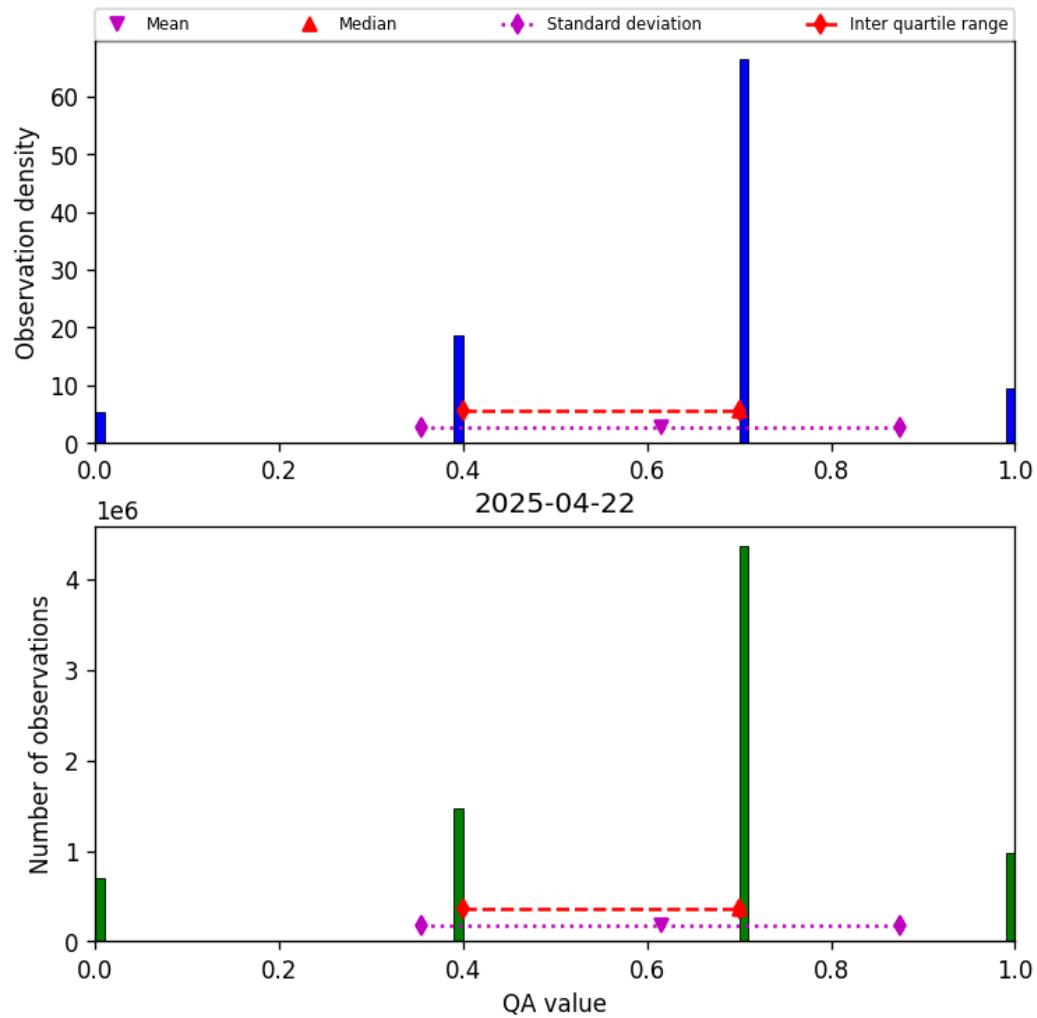
Figure 17: Histogram of “QA value” for 2025-04-21 to 2025-04-23
