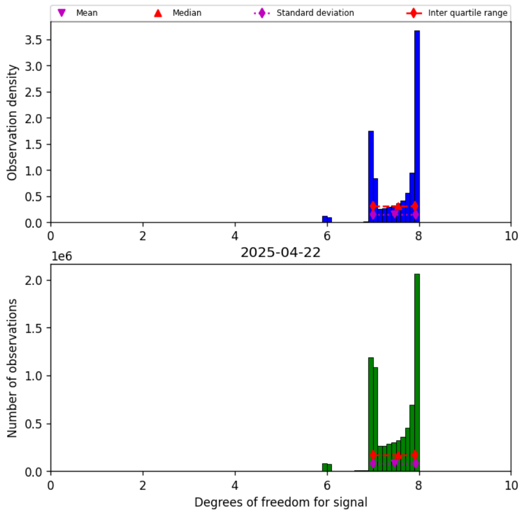
Figure 23: Histogram of “Degrees of freedom for signal” for 2025-04-21 to 2025-04-23
