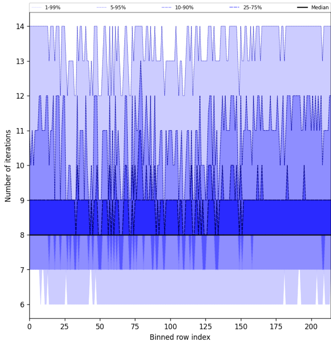
Figure 32: Along track statistics of “Number of iterations” for 2025-04-21 to 2025-04-23
