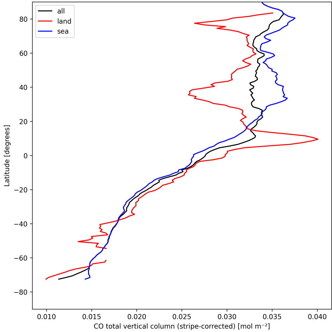
Figure 11: Zonal average of “CO total vertical column (stripe-corrected)” for 2025-04-21 to 2025-04-23.
