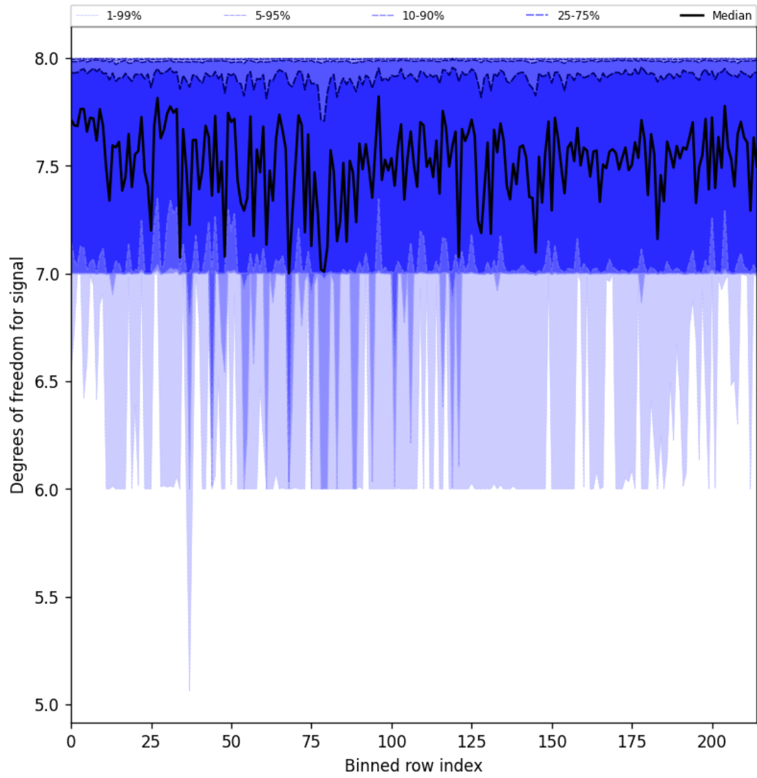
Figure 31: Along track statistics of “Degrees of freedom for signal” for 2025-04-21 to 2025-04-23
