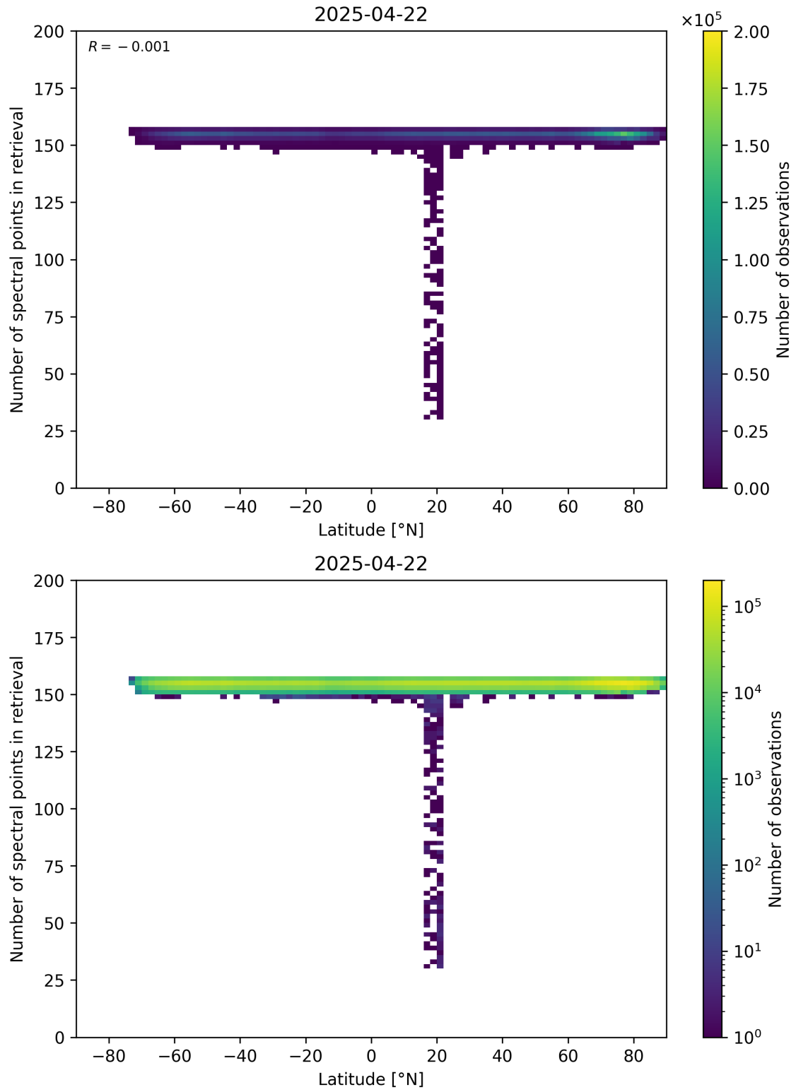
Figure 57: Scatter density plot of “Latitude” against “Number of spectral points in retrieval” for 2025-04-21 to 2025-04-23.
