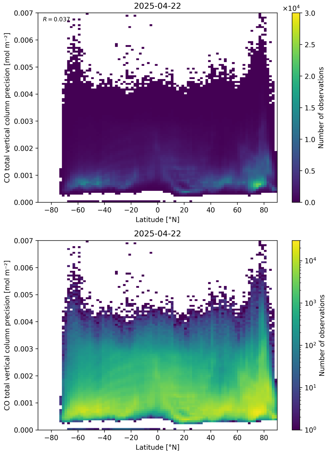
Figure 53: Scatter density plot of “Latitude” against “CO total vertical column precision” for 2025-04-21 to 2025-04-23.
