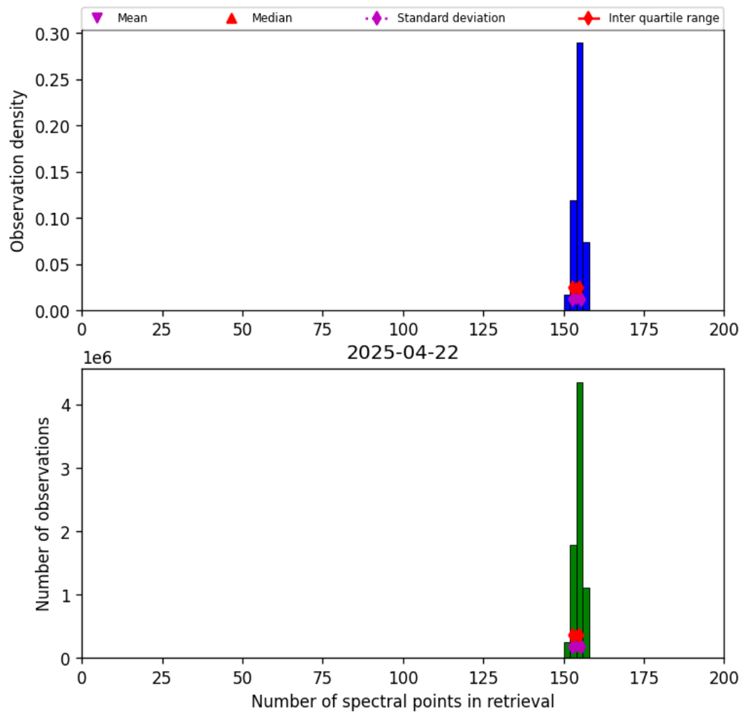
Figure 21: Histogram of “Number of spectral points in retrieval” for 2025-04-21 to 2025-04-23
