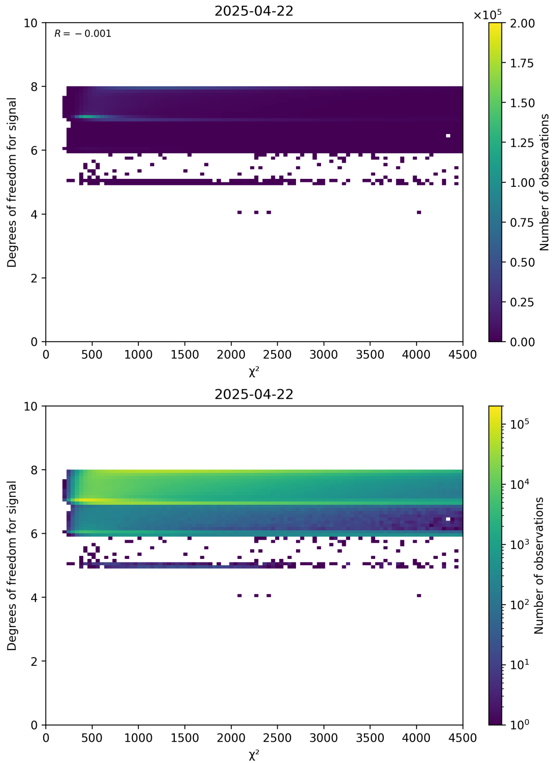
Figure 48: Scatter density plot of “ \chi^2 ” against “Degrees of freedom for signal” for 2025-04-21 to 2025-04-23.
