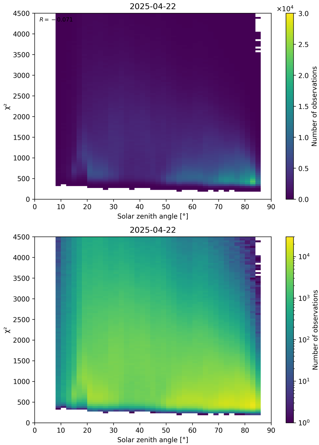
Figure 64: Scatter density plot of “Solar zenith angle” against “ \chi^2 ” for 2025-04-21 to 2025-04-23.
