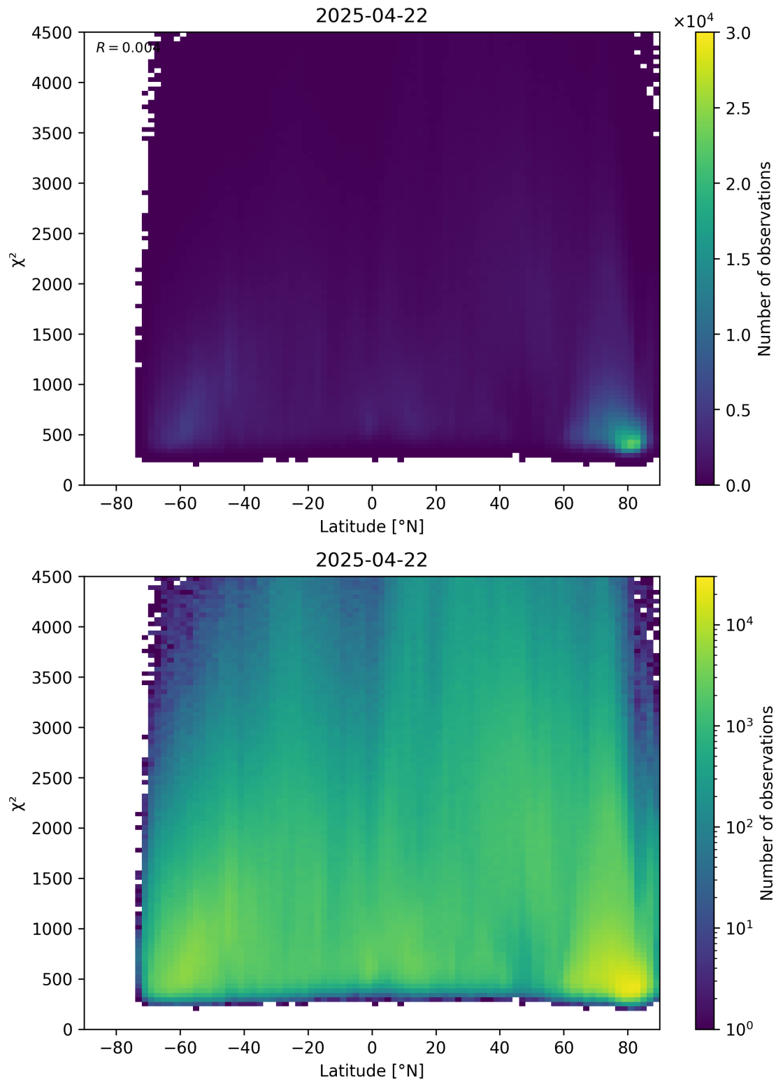
Figure 54: Scatter density plot of “Latitude” against “ \chi^2 ” for 2025-04-21 to 2025-04-23.
