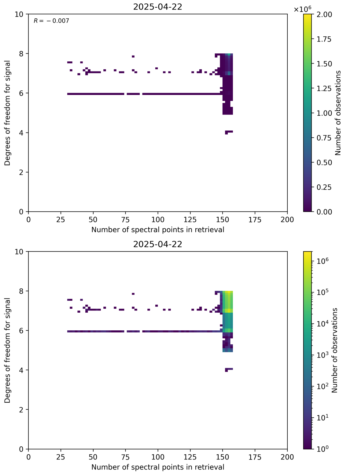
Figure 59: Scatter density plot of “Number of spectral points in retrieval” against “Degrees of freedom for signal” for 2025-04-21 to 2025-04-23.
