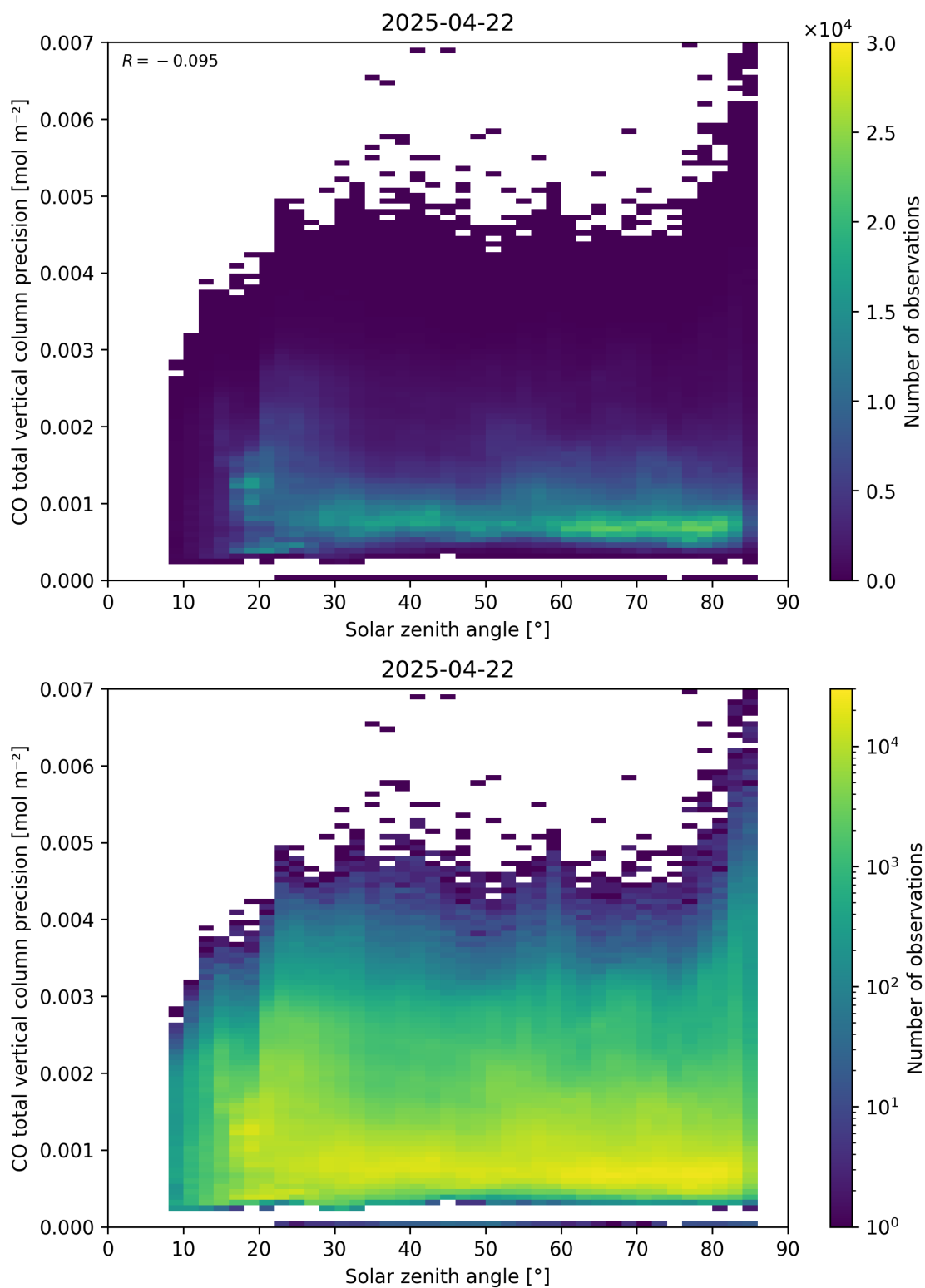
Figure 63: Scatter density plot of “Solar zenith angle” against “CO total vertical column precision” for 2025-04-21 to 2025-04-23.
