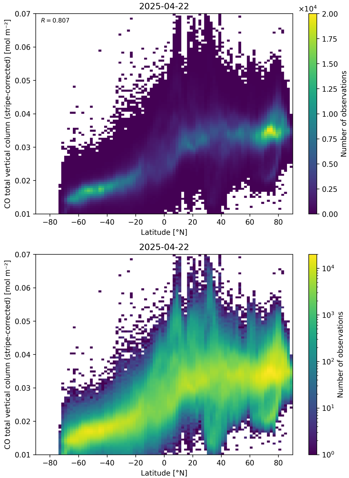
Figure 52: Scatter density plot of “Latitude” against “CO total vertical column (stripe-corrected)” for 2025-04-21 to 2025-04-23.
