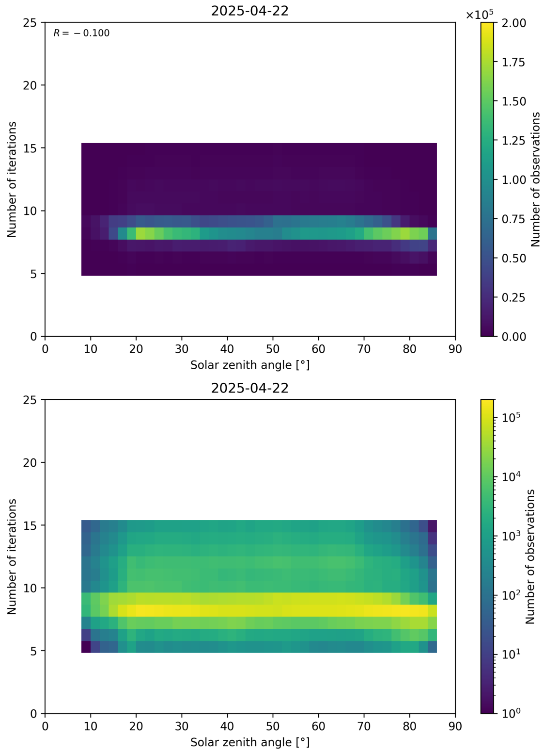
Figure 67: Scatter density plot of “Solar zenith angle” against “Number of iterations” for 2025-04-21 to 2025-04-23.
