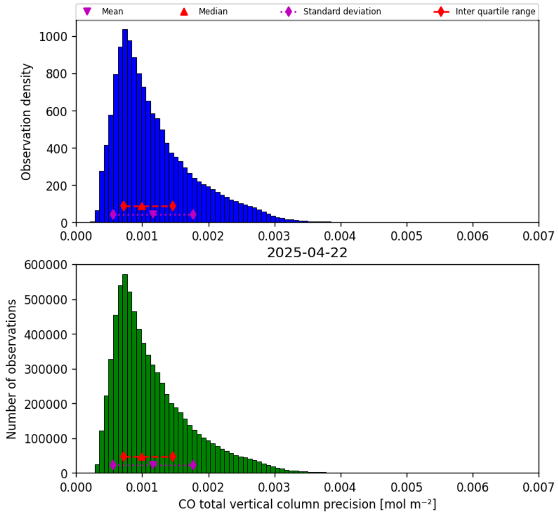
Figure 20: Histogram of “CO total vertical column precision” for 2025-04-21 to 2025-04-23
