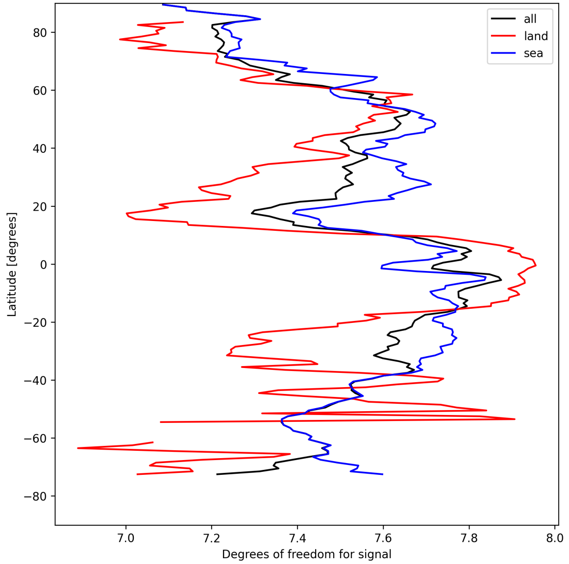
Figure 15: Zonal average of “Degrees of freedom for signal” for 2025-04-21 to 2025-04-23.
