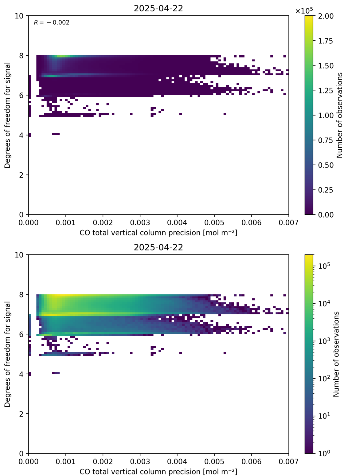
Figure 45: Scatter density plot of “CO total vertical column precision” against “Degrees of freedom for signal” for 2025-04-21 to 2025-04-23.
