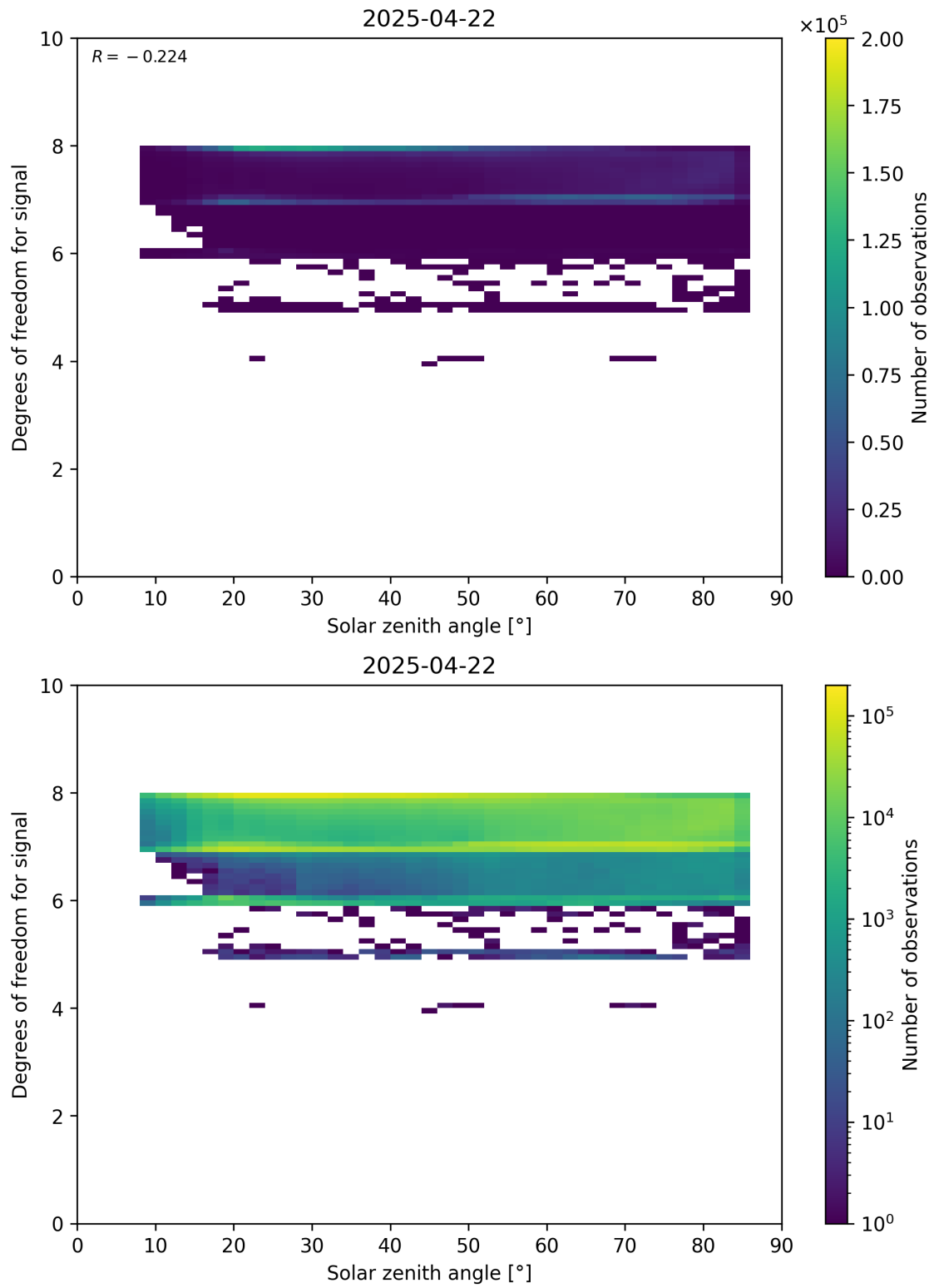
Figure 65: Scatter density plot of “Solar zenith angle” against “Degrees of freedom for signal” for 2025-04-21 to 2025-04-23.
