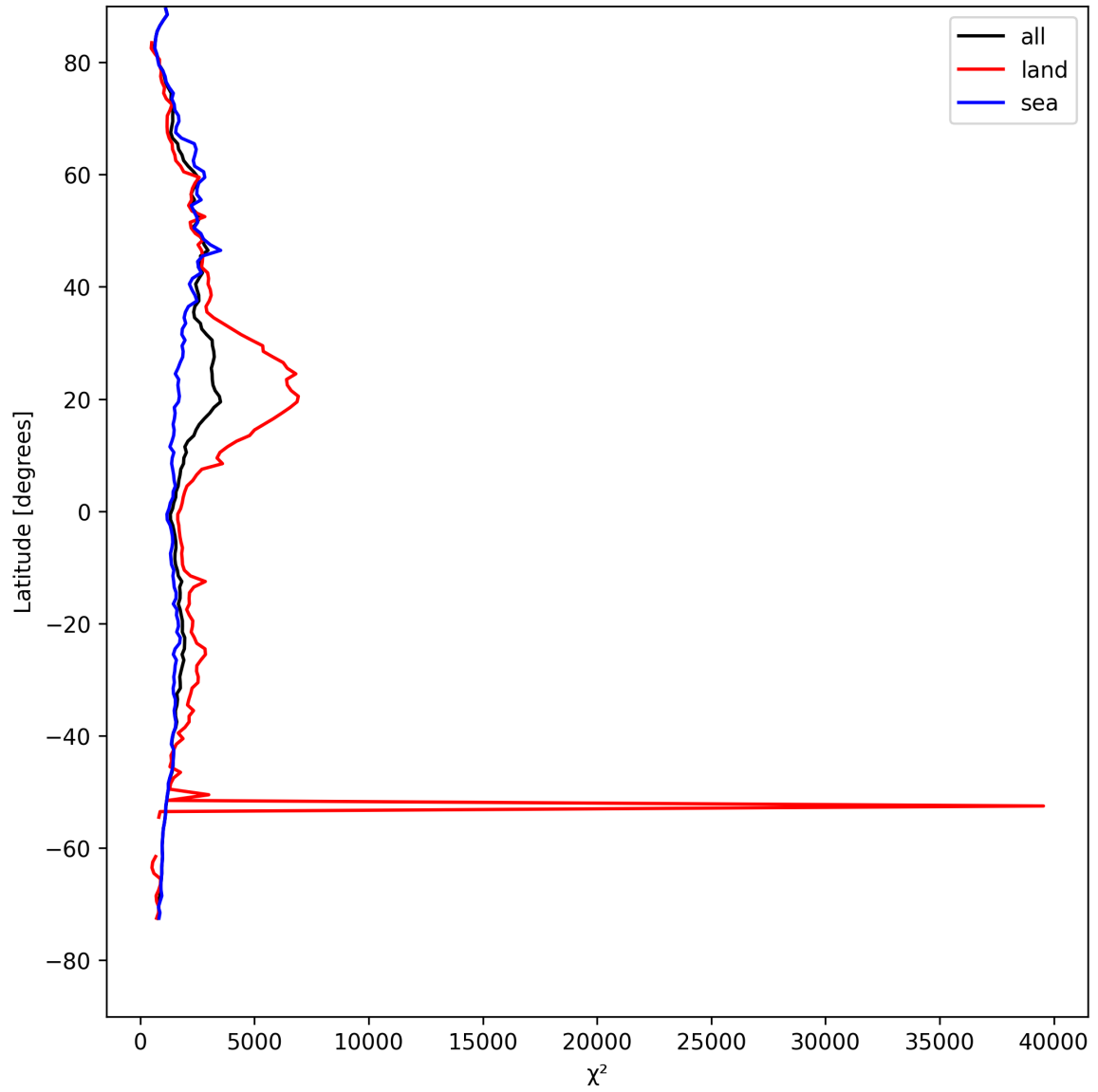
Figure 14: Zonal average of “ \chi^2 ” for 2025-04-21 to 2025-04-23.
