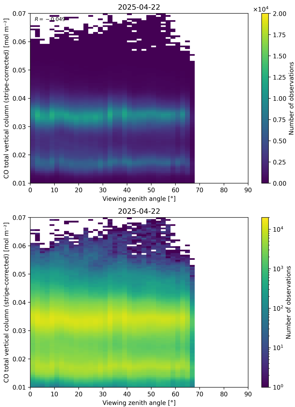
Figure 70: Scatter density plot of “Viewing zenith angle” against “CO total vertical column (stripe-corrected)” for 2025-04-21 to 2025-04-23.
