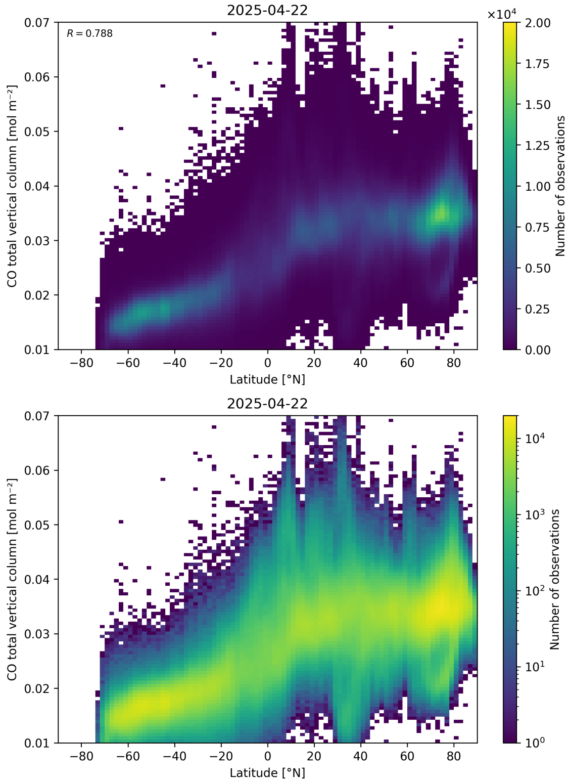
Figure 51: Scatter density plot of “Latitude” against “CO total vertical column” for 2025-04-21 to 2025-04-23.
