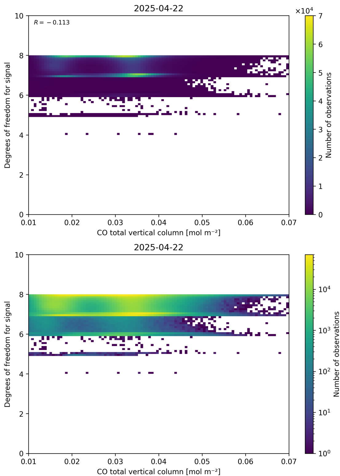
Figure 41: Scatter density plot of “CO total vertical column” against “Degrees of freedom for signal” for 2025-04-21 to 2025-04-23.
