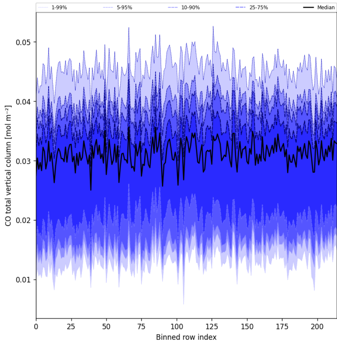
Figure 26: Along track statistics of “CO total vertical column” for 2025-04-21 to 2025-04-23
