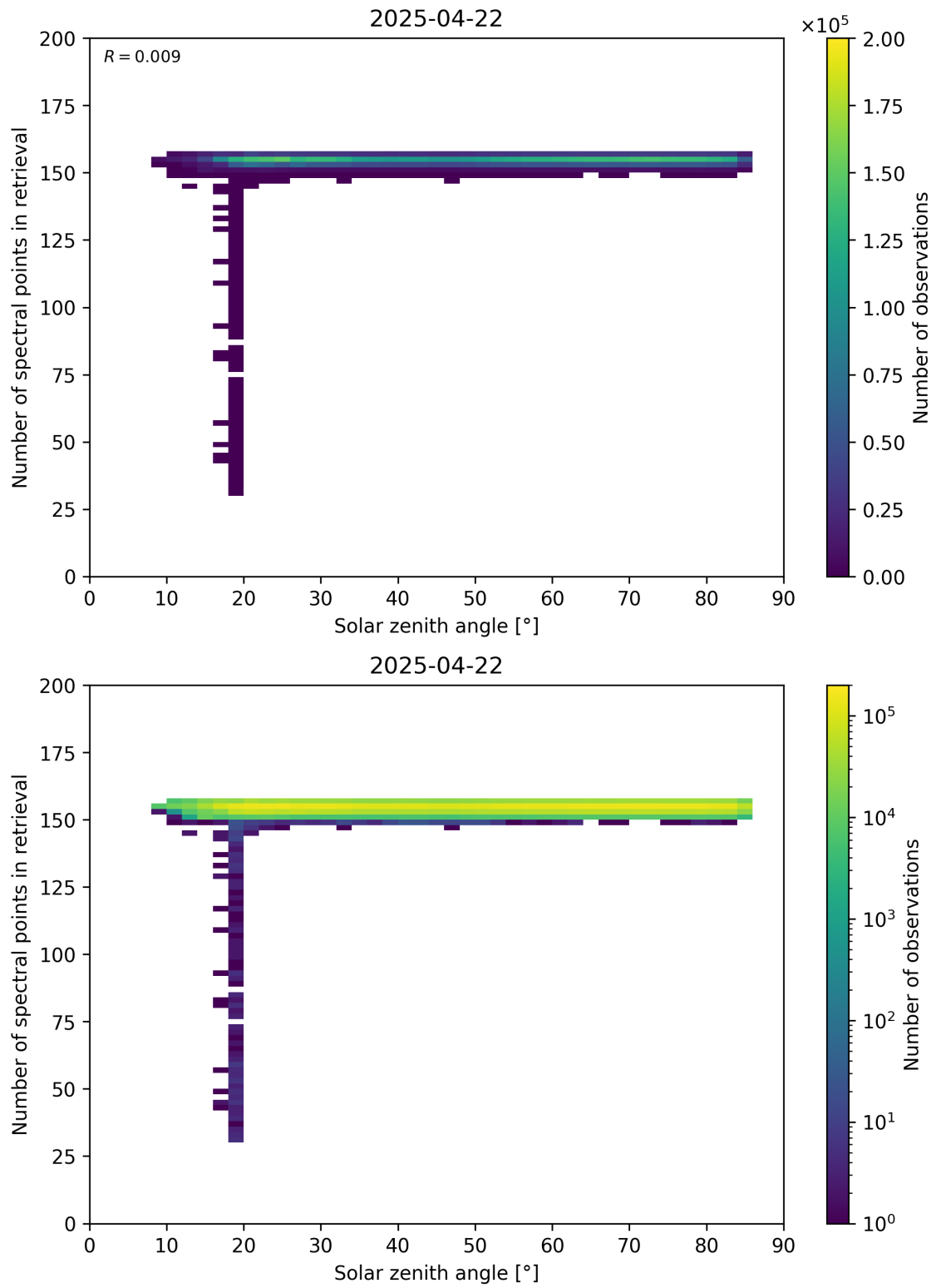
Figure 68: Scatter density plot of “Solar zenith angle” against “Number of spectral points in retrieval” for 2025-04-21 to 2025-04-23.
