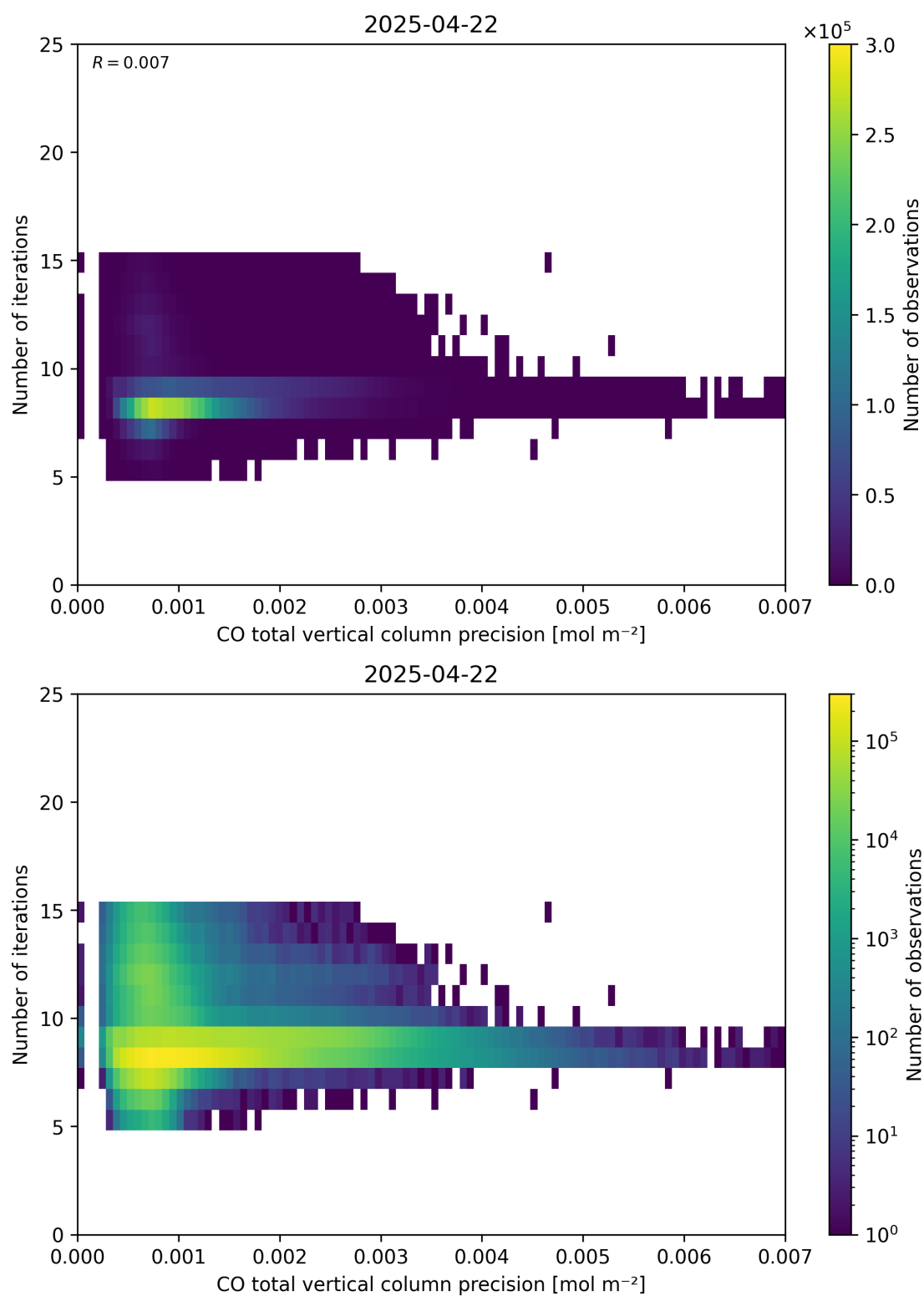
Figure 46: Scatter density plot of “CO total vertical column precision” against “Number of iterations” for 2025-04-21 to 2025-04-23.
