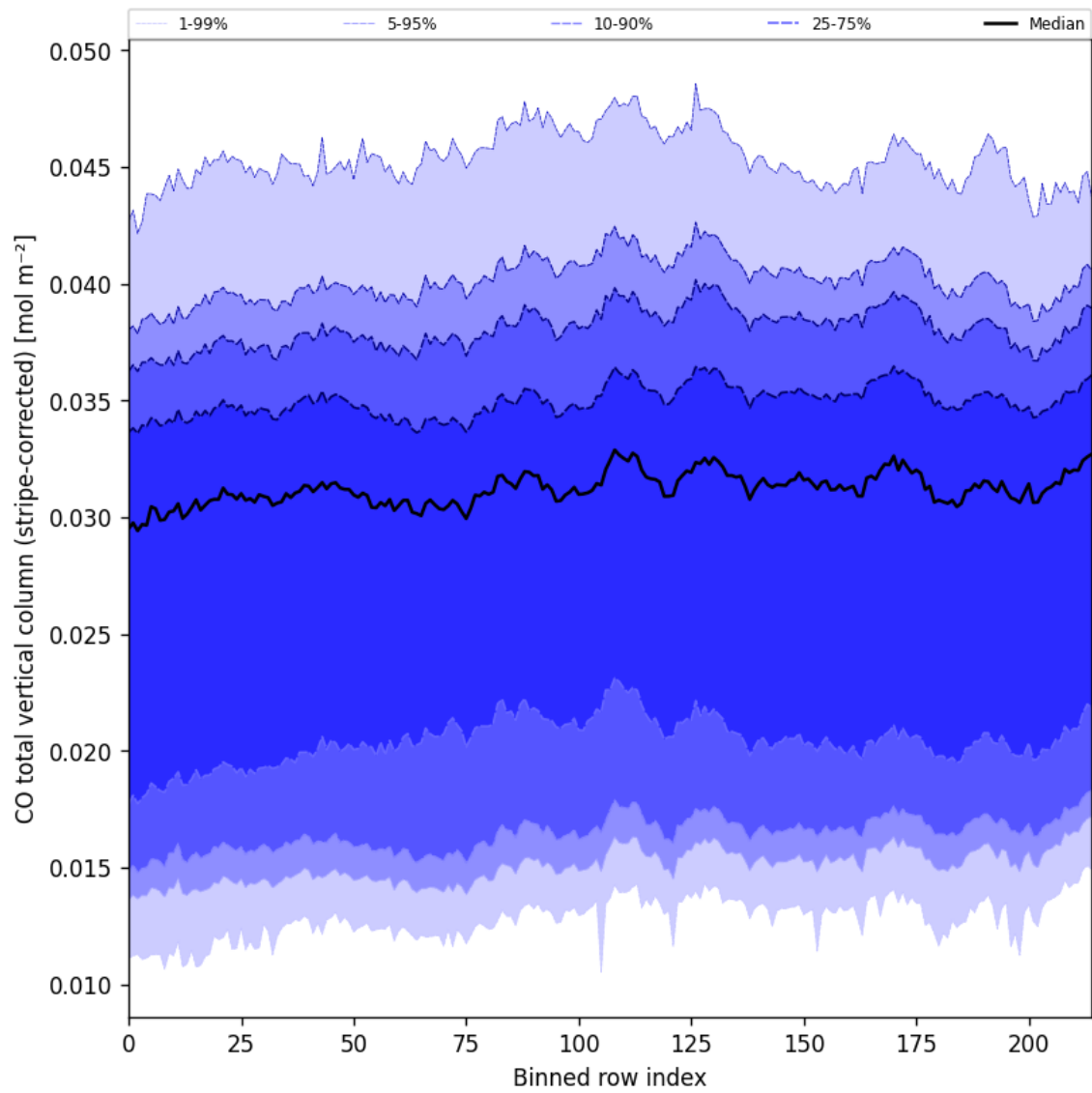
Figure 27: Along track statistics of “CO total vertical column (stripe-corrected)” for 2025-04-21 to 2025-04-23
