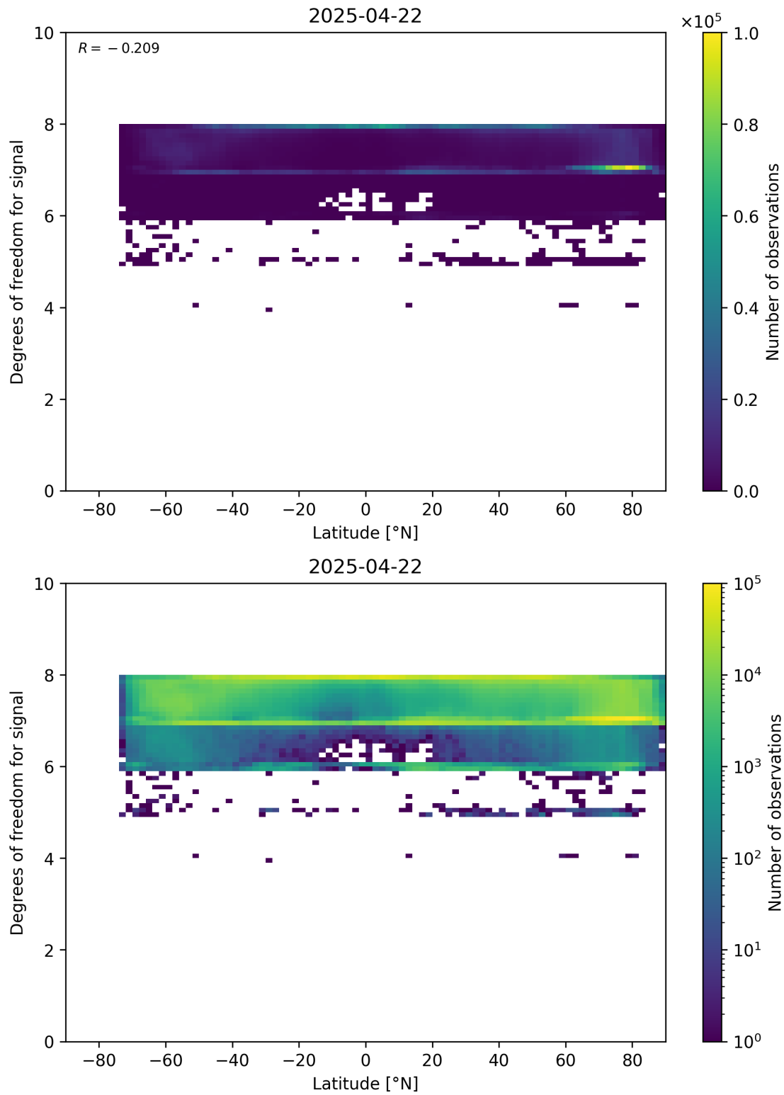
Figure 55: Scatter density plot of “Latitude” against “Degrees of freedom for signal” for 2025-04-21 to 2025-04-23.
