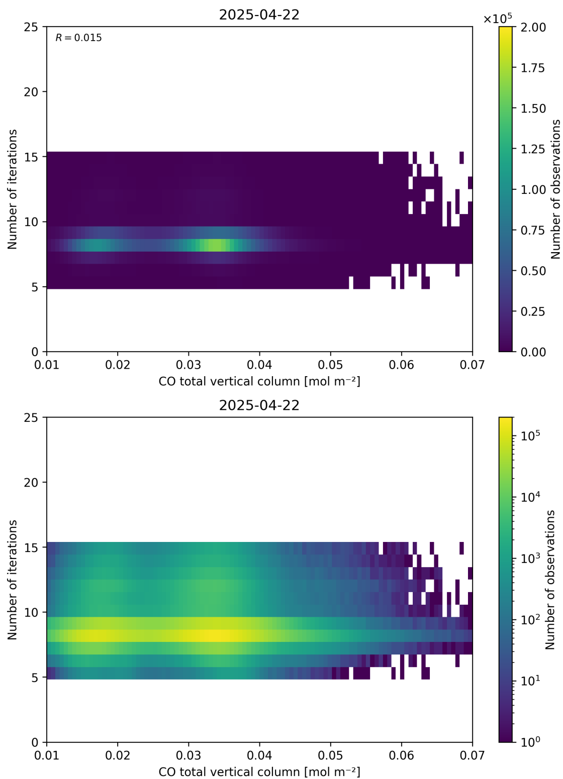
Figure 42: Scatter density plot of “CO total vertical column” against “Number of iterations” for 2025-04-21 to 2025-04-23.
