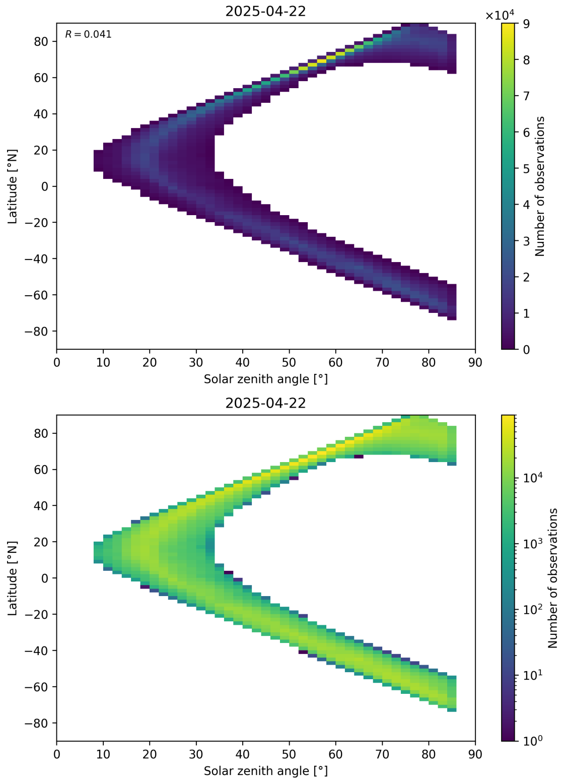
Figure 66: Scatter density plot of “Solar zenith angle” against “Latitude” for 2025-04-21 to 2025-04-23.
