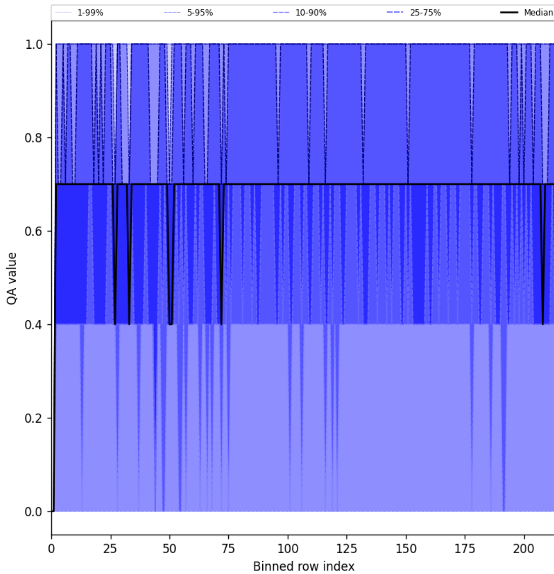
Figure 25: Along track statistics of “QA value” for 2025-04-21 to 2025-04-23
