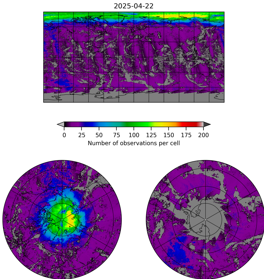
Figure 8: Map of the number of observations for 2025-04-21 to 2025-04-23
