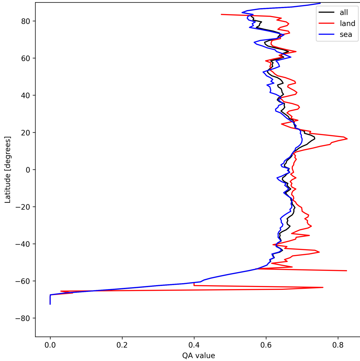
Figure 9: Zonal average of “QA value” for 2025-04-21 to 2025-04-23.
