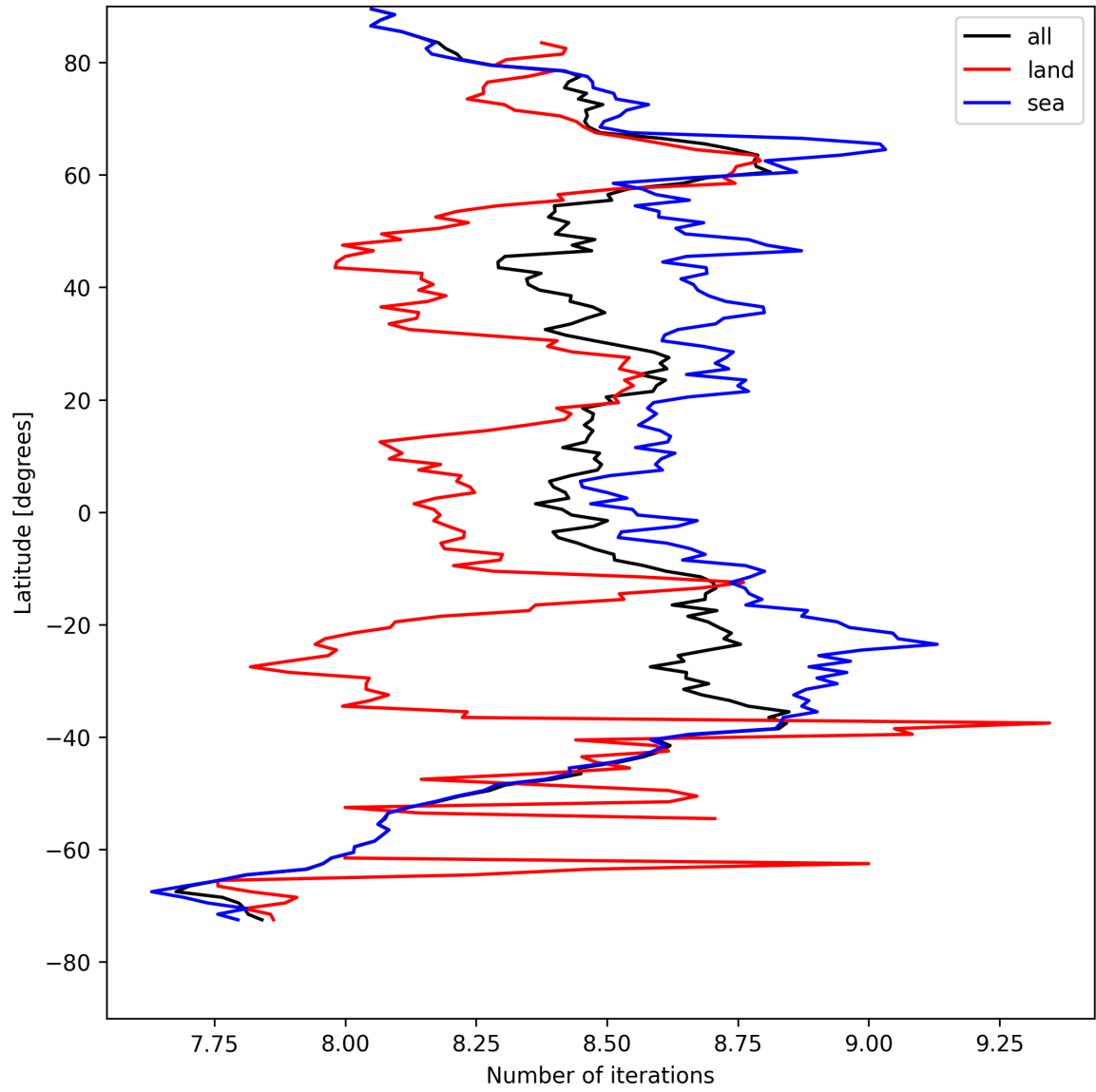
Figure 16: Zonal average of “Number of iterations” for 2025-04-21 to 2025-04-23.
