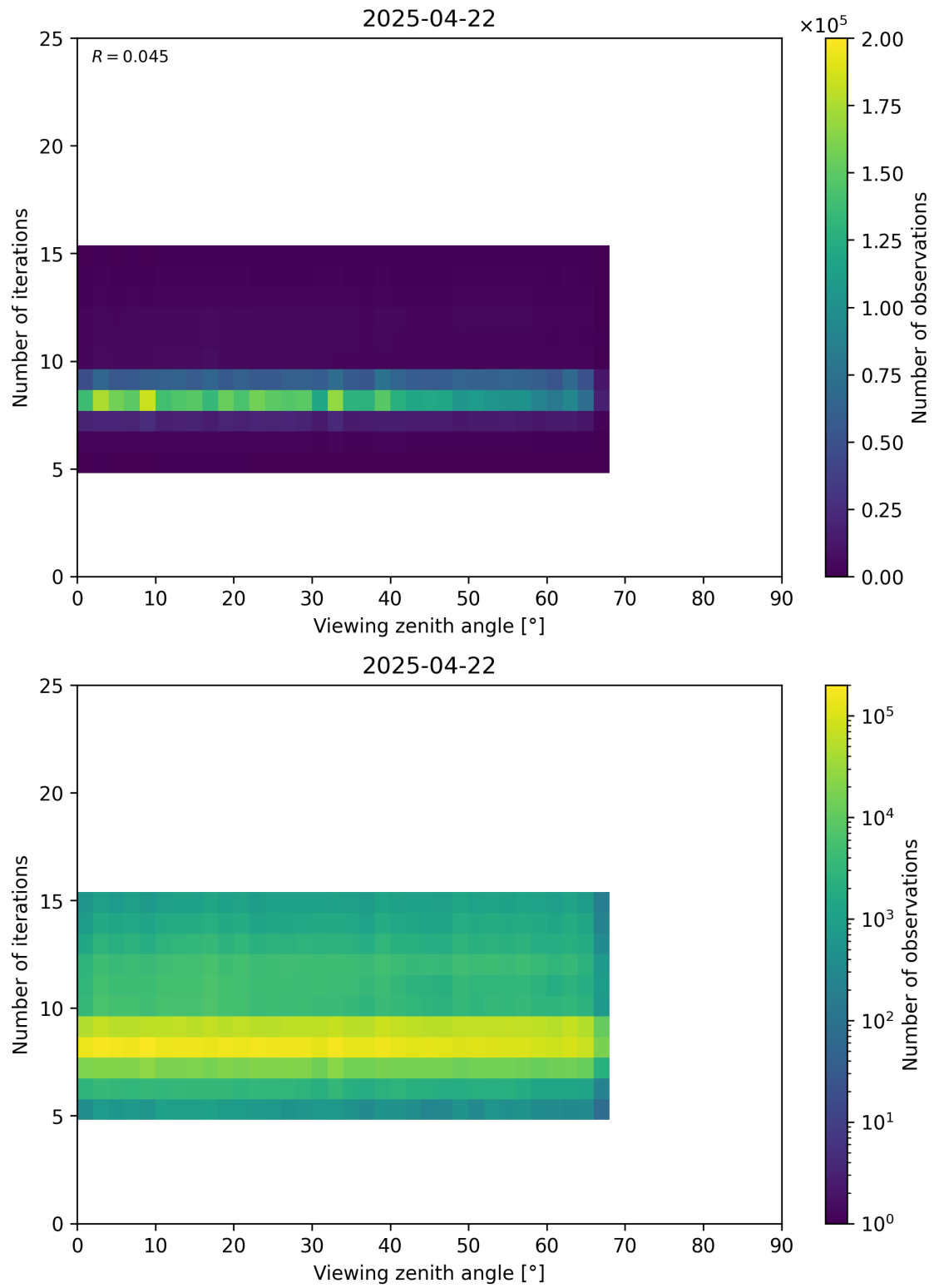
Figure 75: Scatter density plot of “Viewing zenith angle” against “Number of iterations” for 2025-04-21 to 2025-04-23.
