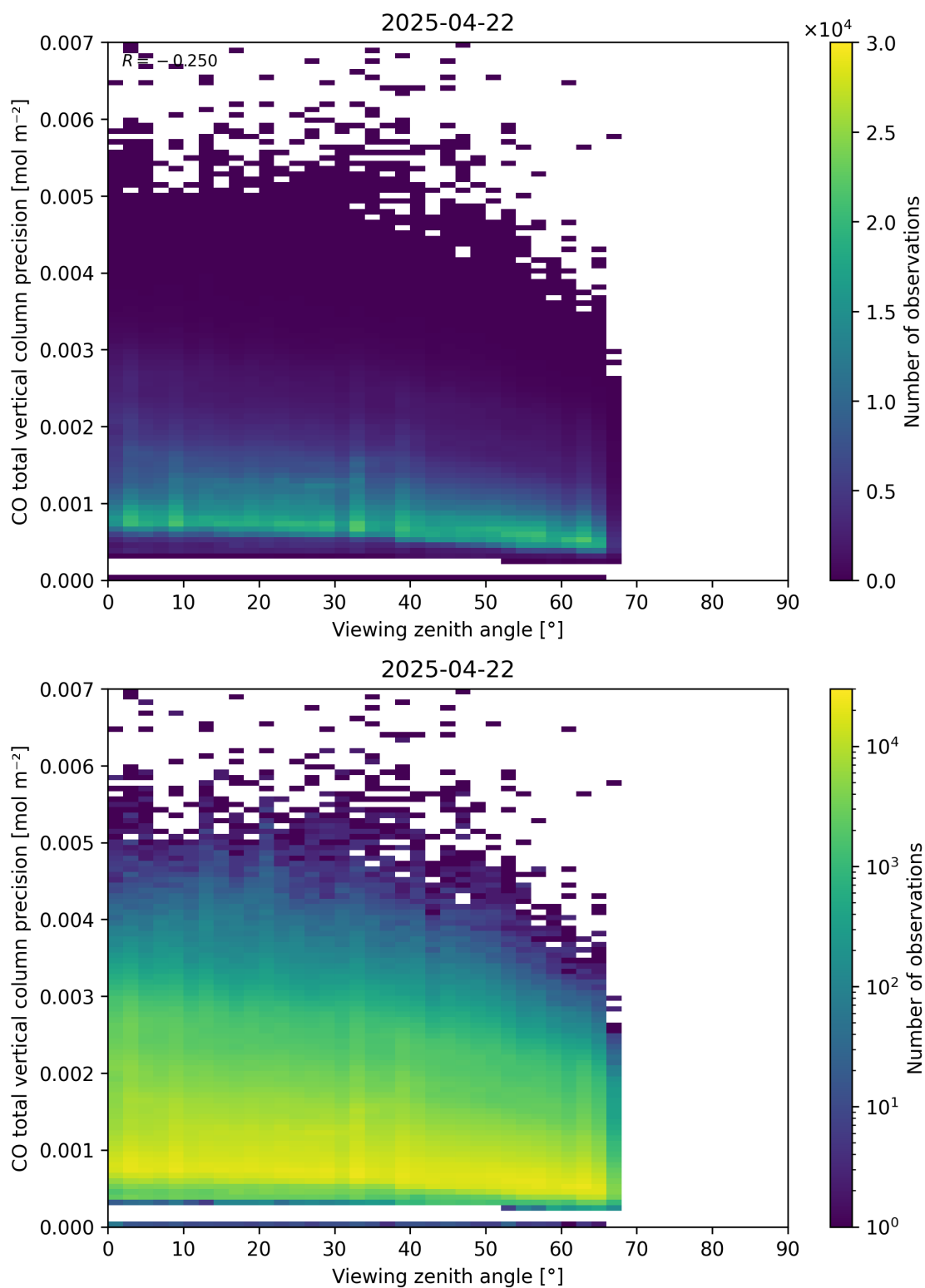
Figure 71: Scatter density plot of “Viewing zenith angle” against “CO total vertical column precision” for 2025-04-21 to 2025-04-23.
