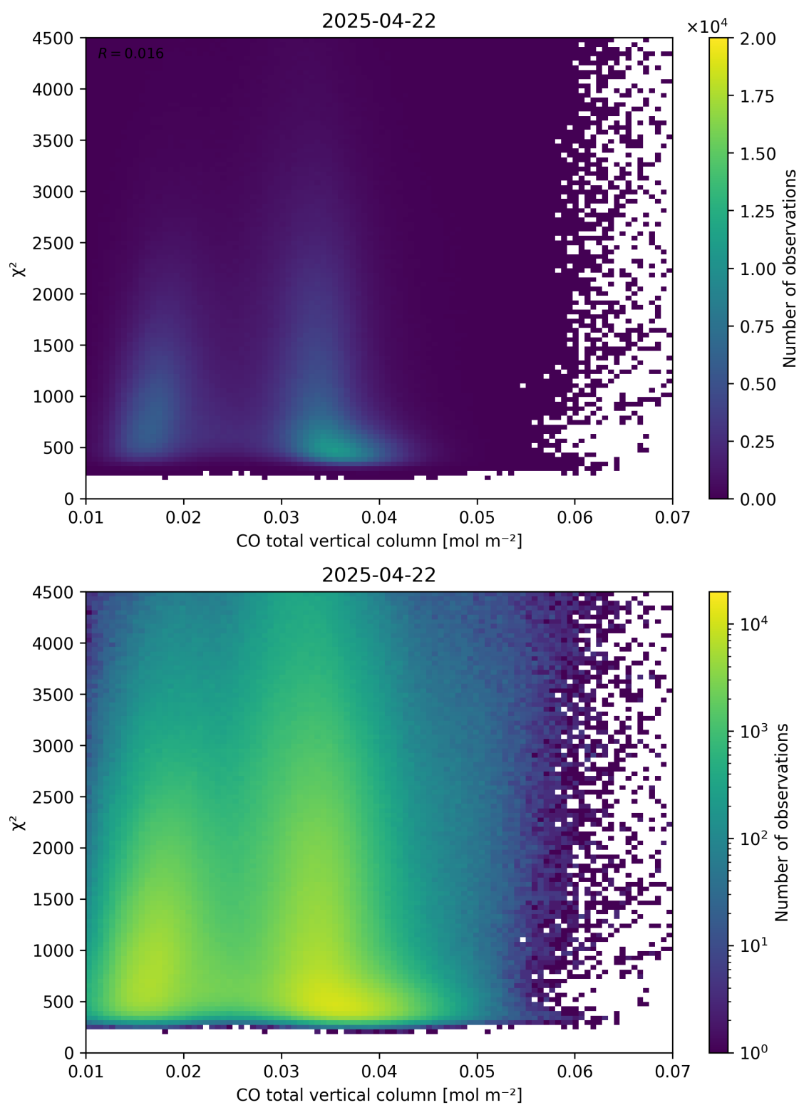
Figure 35: Scatter density plot of “CO total vertical column” against “ \chi^2 ” for 2025-04-21 to 2025-04-23.
