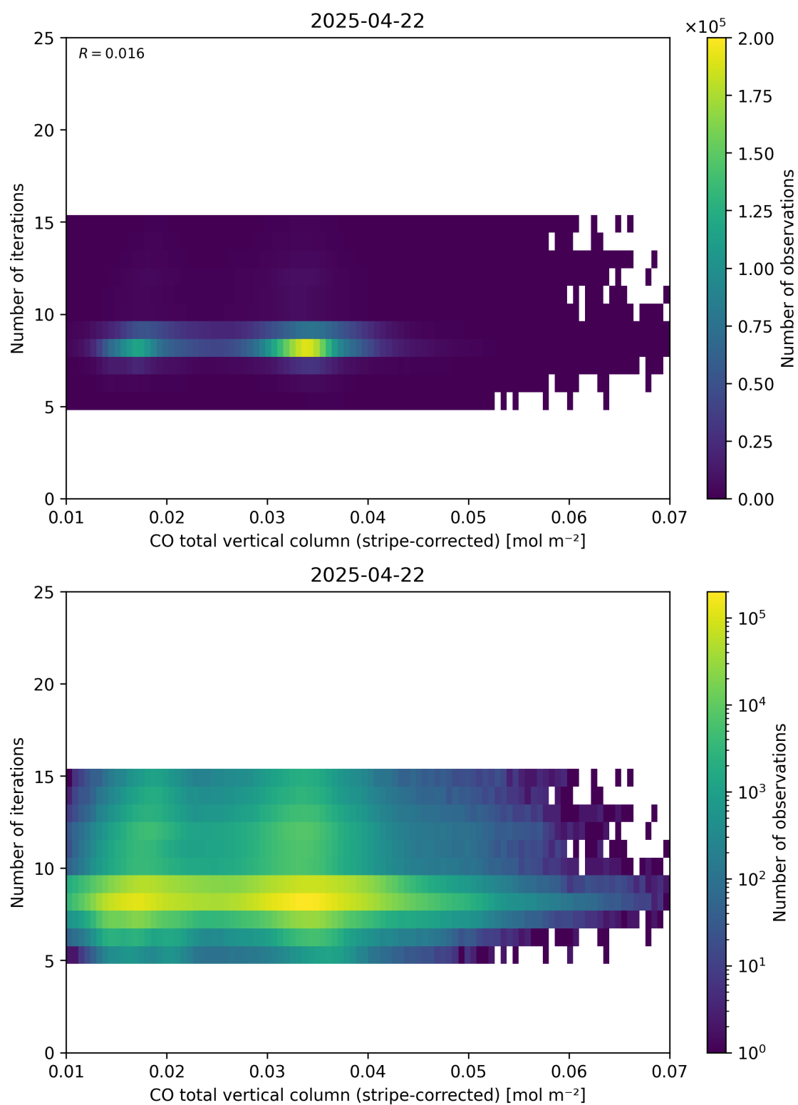
Figure 39: Scatter density plot of “CO total vertical column (stripe-corrected)” against “Number of iterations” for 2025-04-21 to 2025-04-23.
