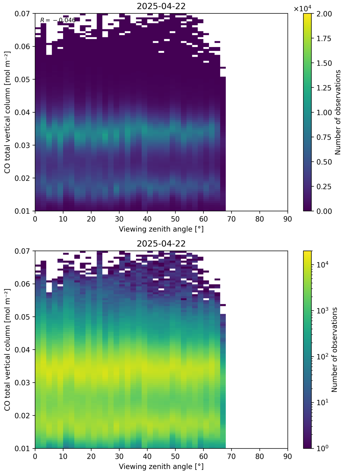
Figure 69: Scatter density plot of “Viewing zenith angle” against “CO total vertical column” for 2025-04-21 to 2025-04-23.
