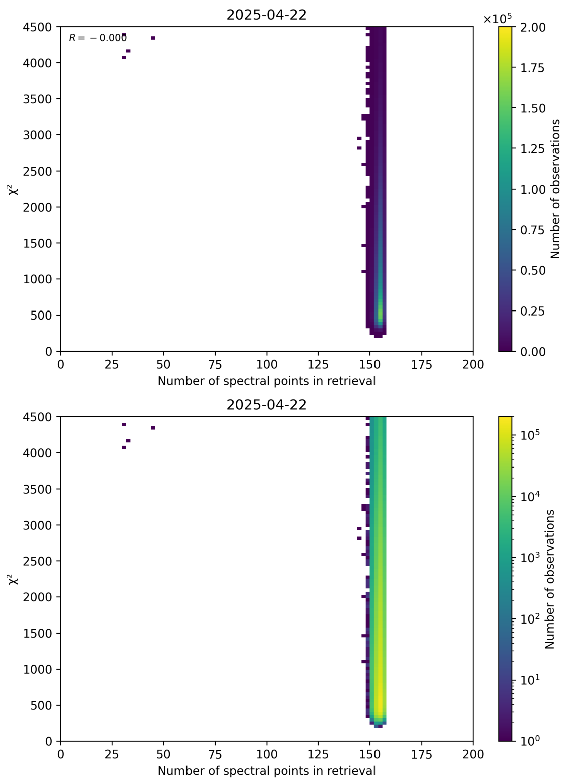
Figure 58: Scatter density plot of “Number of spectral points in retrieval” against “ \chi^2 ” for 2025-04-21 to 2025-04-23.
