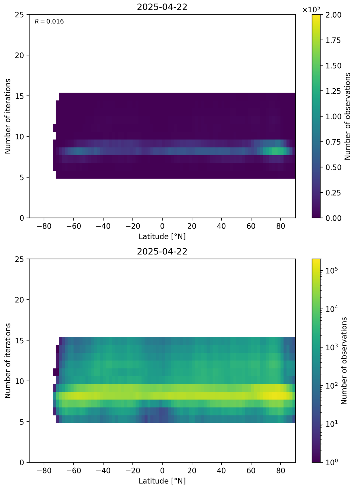
Figure 56: Scatter density plot of “Latitude” against “Number of iterations” for 2025-04-21 to 2025-04-23.
