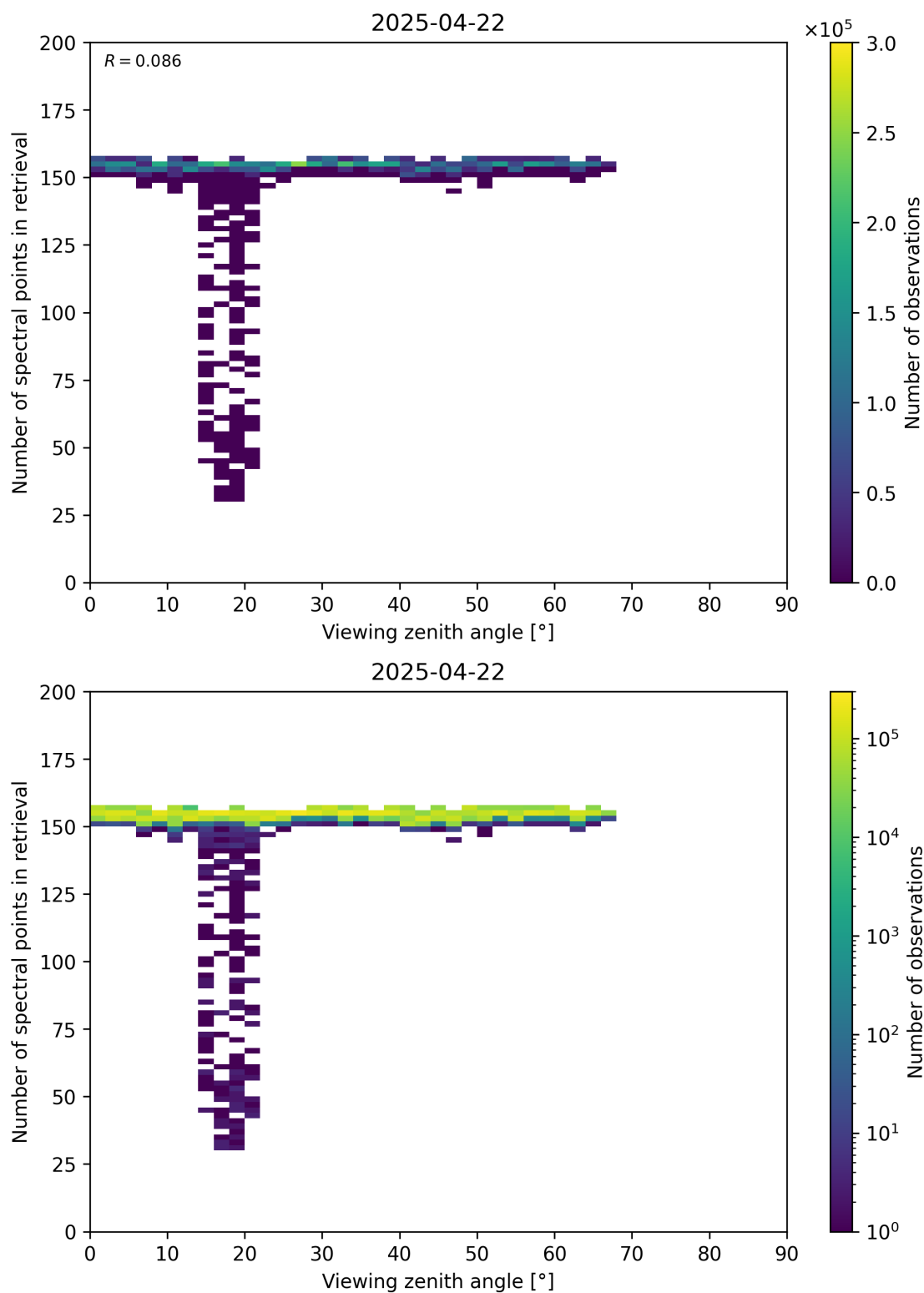
Figure 76: Scatter density plot of “Viewing zenith angle” against “Number of spectral points in retrieval” for 2025-04-21 to 2025-04-23.
