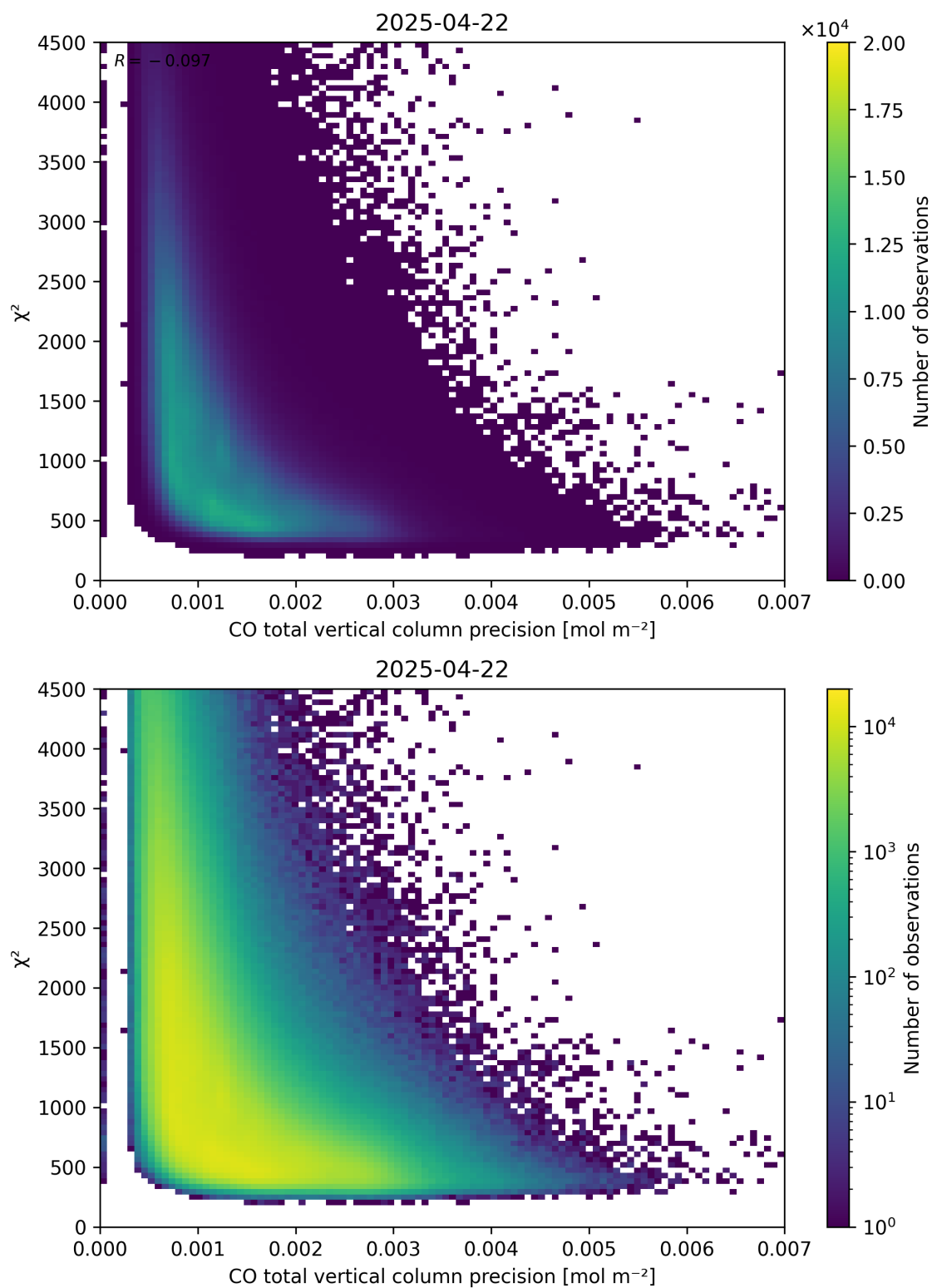
Figure 44: Scatter density plot of “CO total vertical column precision” against “ \chi^2 ” for 2025-04-21 to 2025-04-23.
