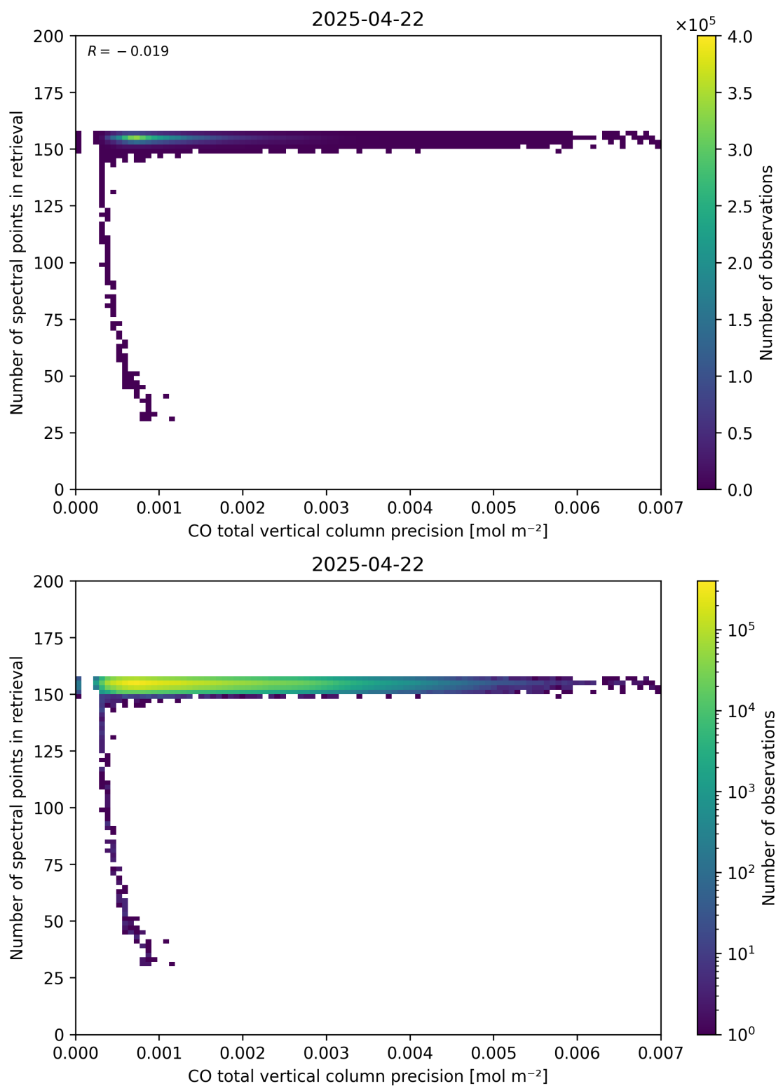
Figure 47: Scatter density plot of “CO total vertical column precision” against “Number of spectral points in retrieval” for 2025-04-21 to 2025-04-23.
