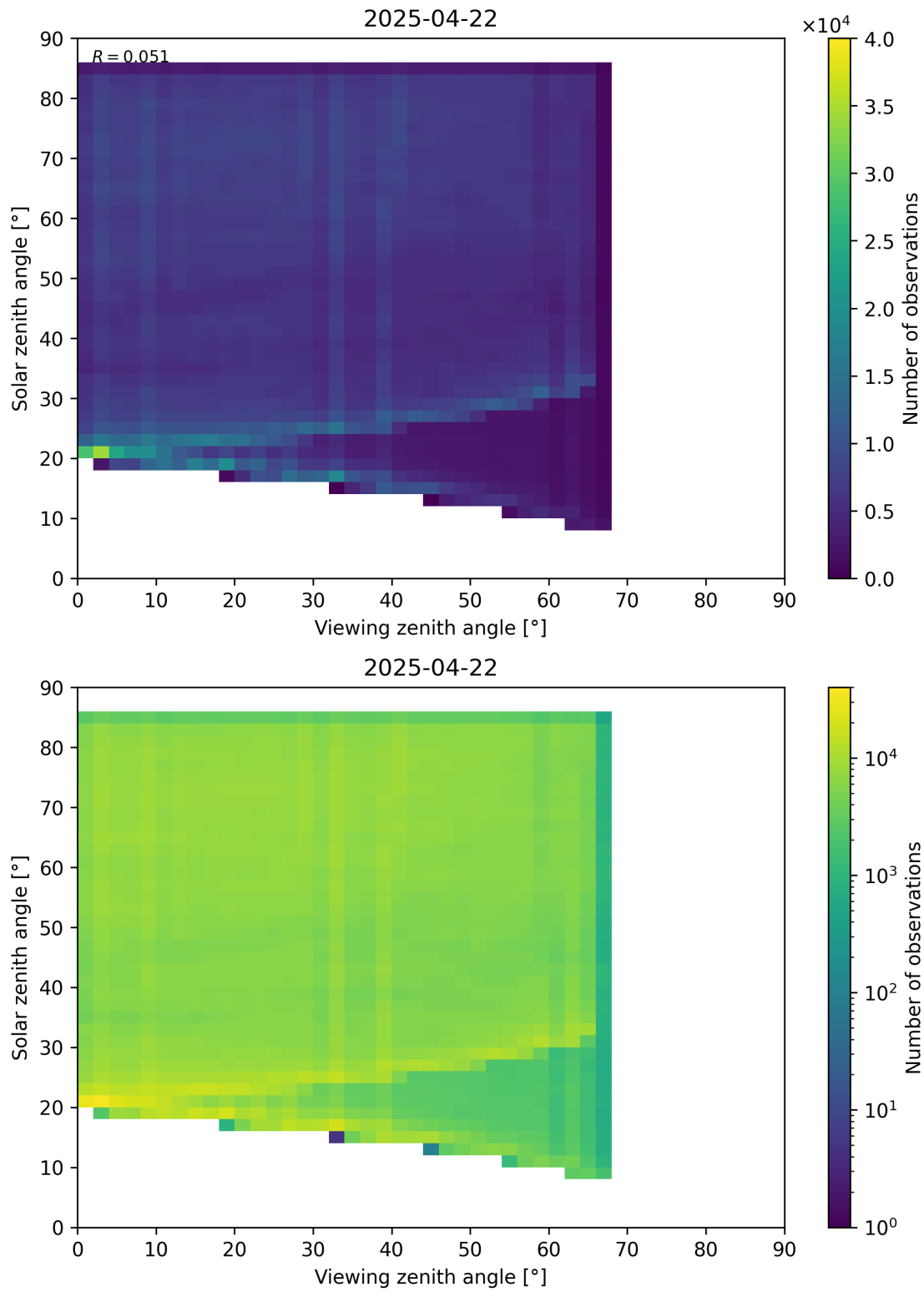
Figure 77: Scatter density plot of “Viewing zenith angle” against “Solar zenith angle” for 2025-04-21 to 2025-04-23.
