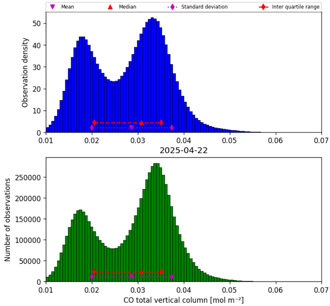
Figure 18: Histogram of “CO total vertical column” for 2025-04-21 to 2025-04-23
