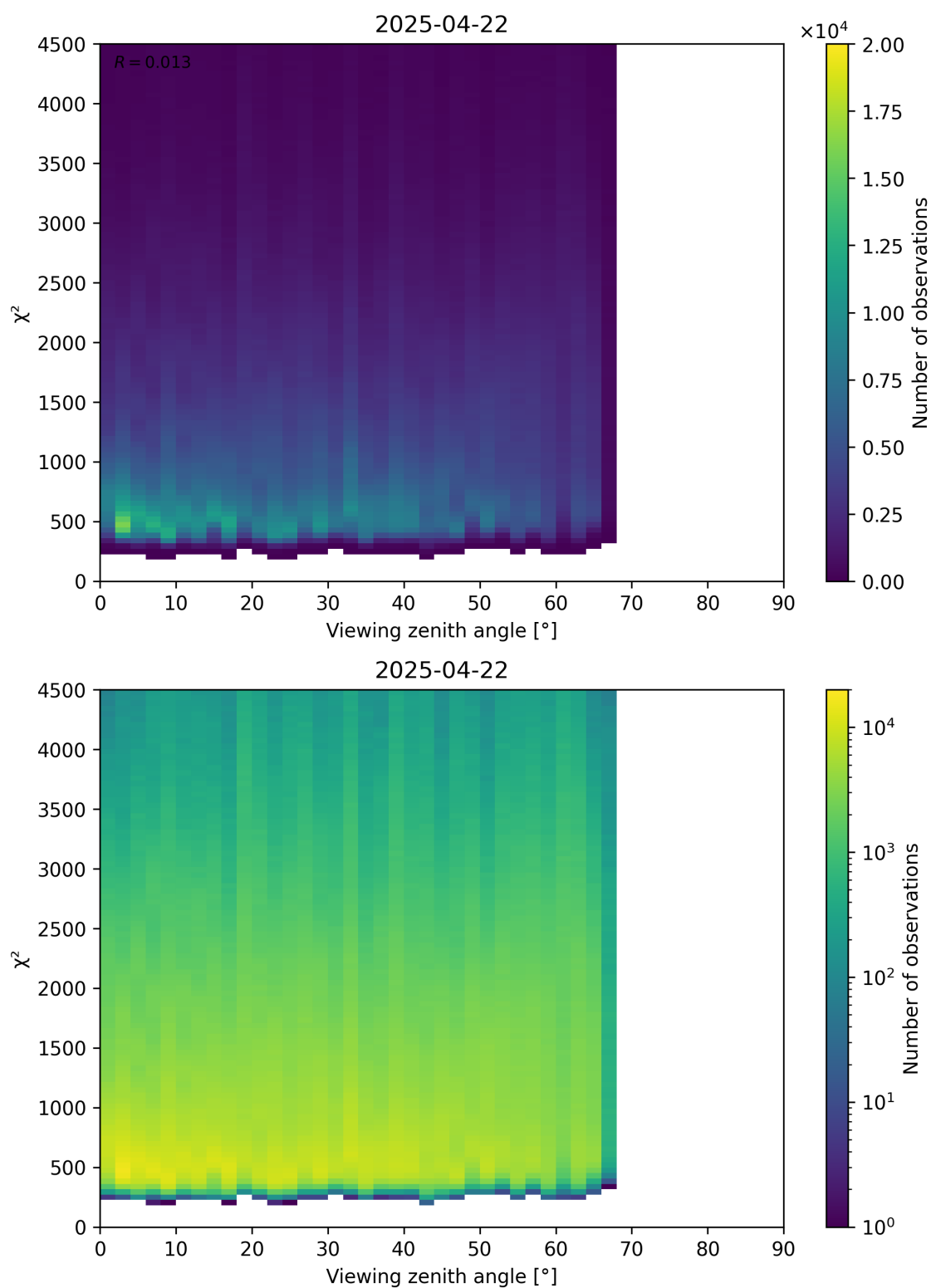
Figure 72: Scatter density plot of “Viewing zenith angle” against “ \chi^2 ” for 2025-04-21 to 2025-04-23.
