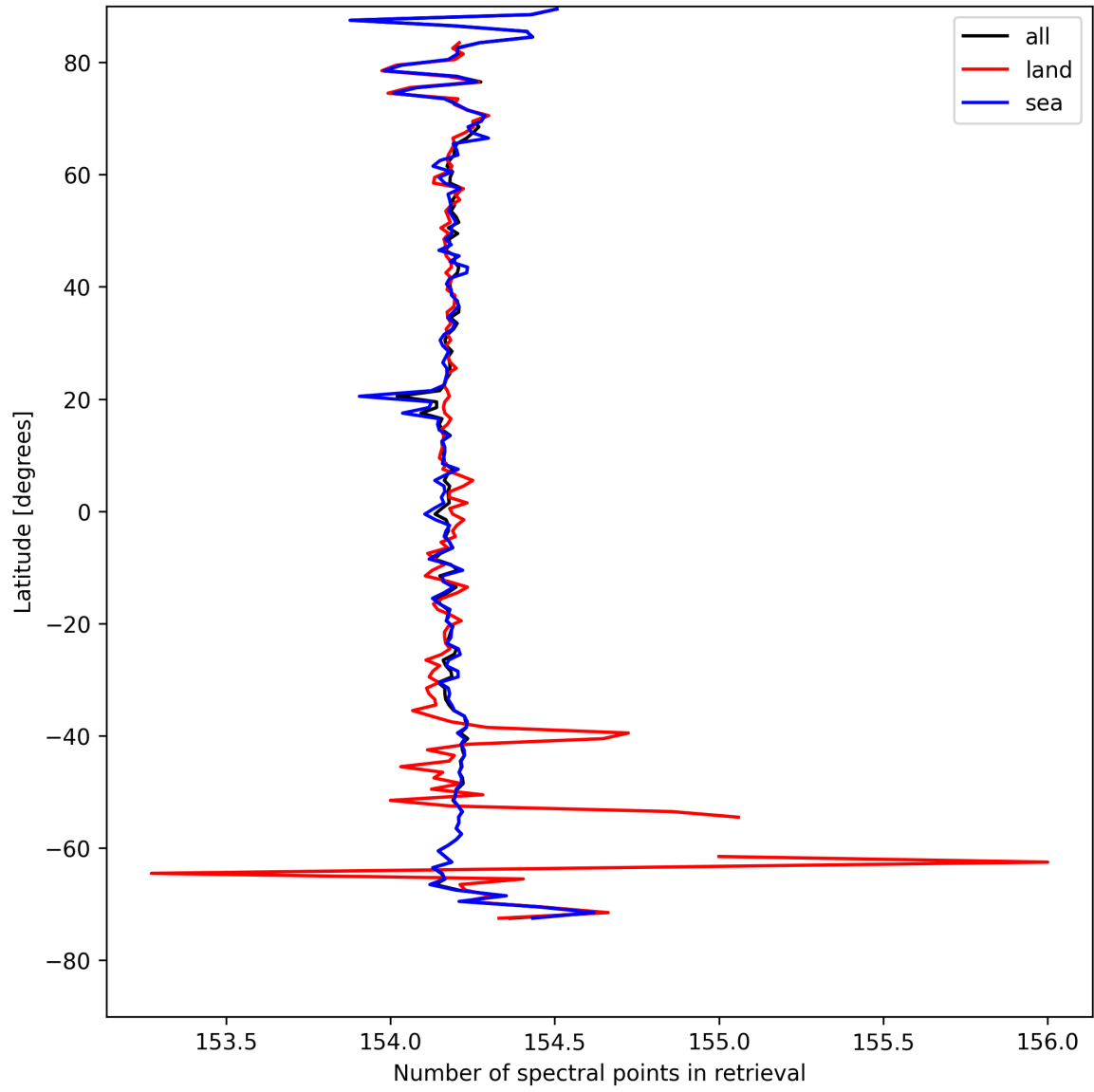
Figure 13: Zonal average of “Number of spectral points in retrieval” for 2025-04-21 to 2025-04-23.
