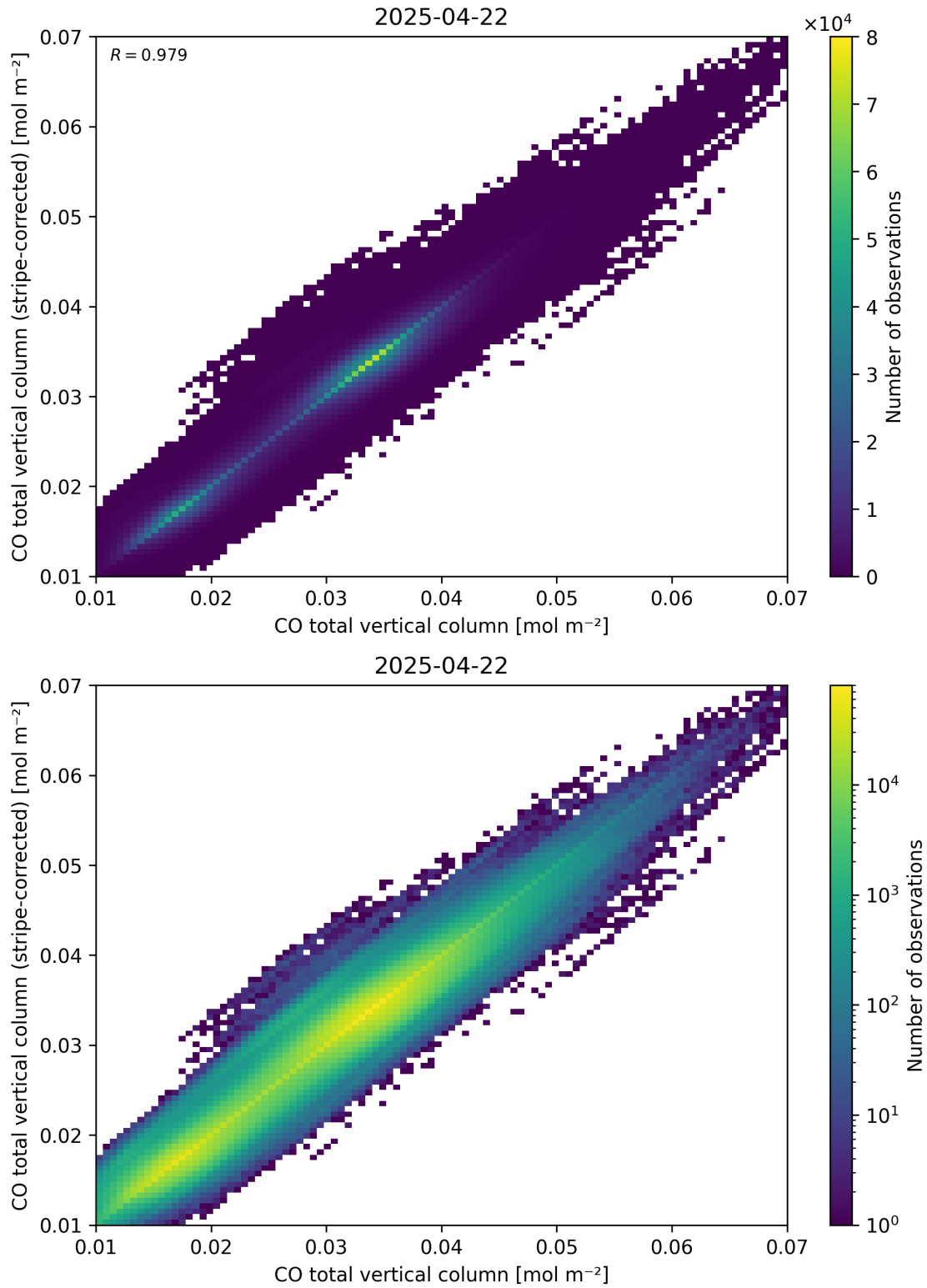
Figure 33: Scatter density plot of “CO total vertical column” against “CO total vertical column (stripe-corrected)” for 2025-04-21 to 2025-04-23.
