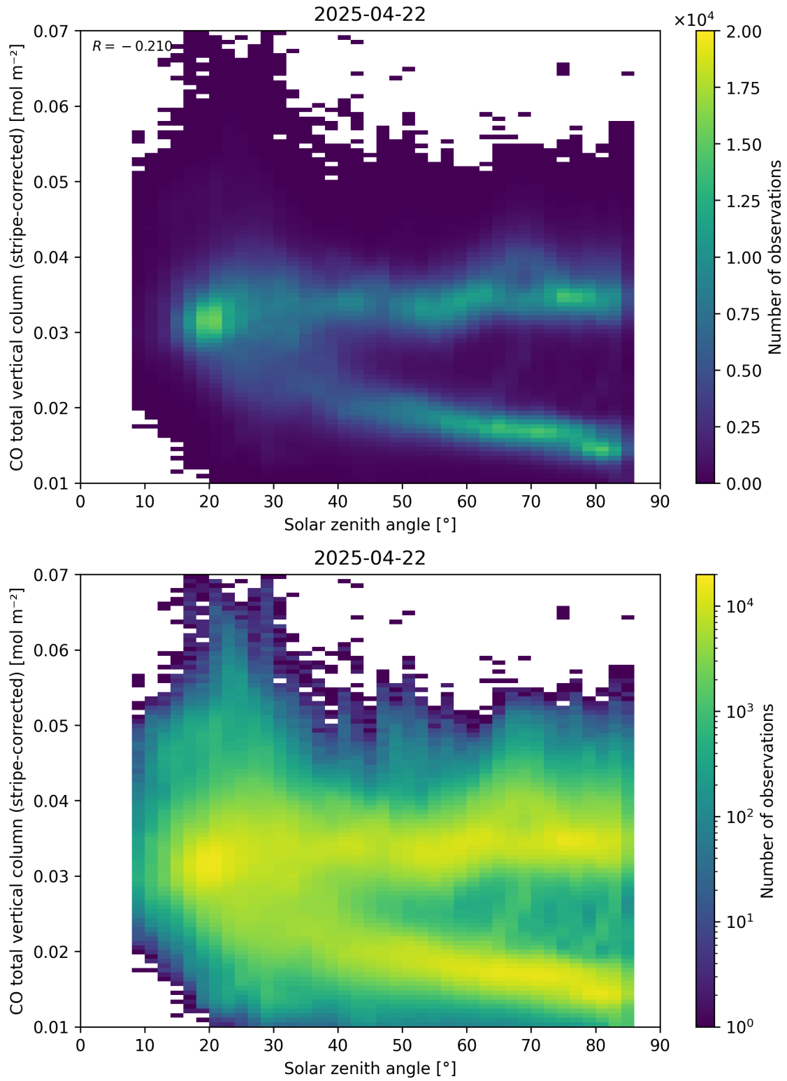
Figure 62: Scatter density plot of “Solar zenith angle” against “CO total vertical column (stripe-corrected)” for 2025-04-21 to 2025-04-23.
