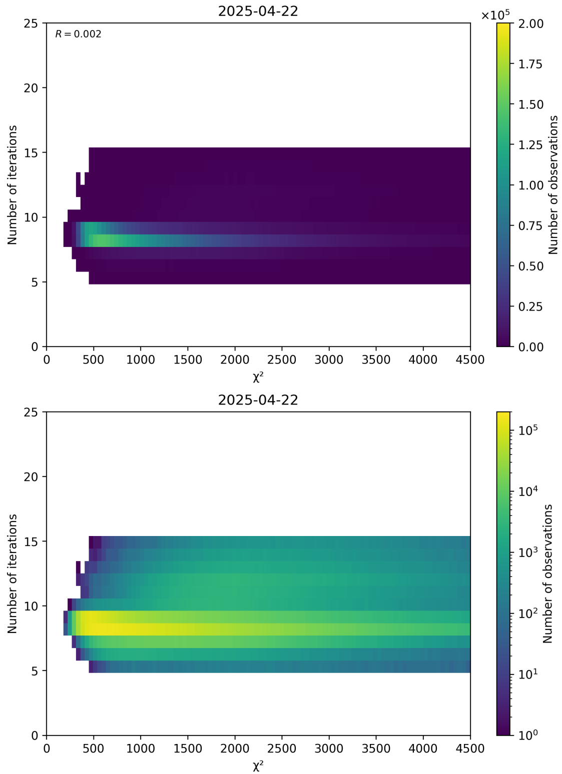
Figure 49: Scatter density plot of “ \chi^2 ” against “Number of iterations” for 2025-04-21 to 2025-04-23.
