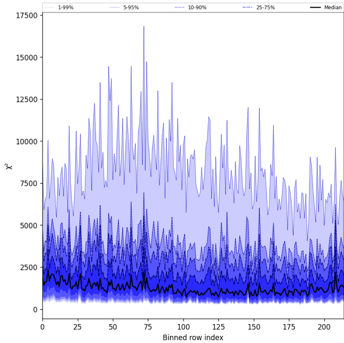
Figure 30: Along track statistics of “ \chi^2 ” for 2025-04-21 to 2025-04-23
