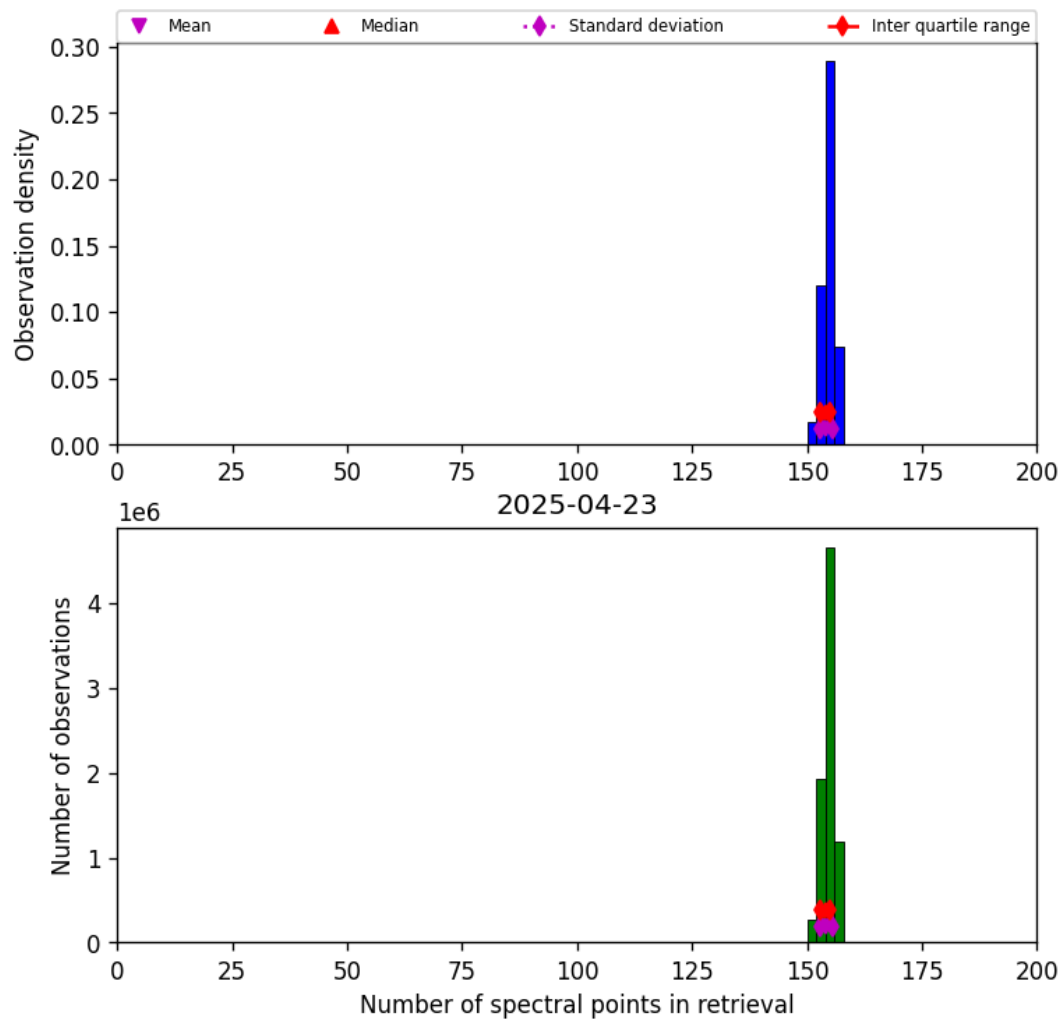
Figure 21: Histogram of “Number of spectral points in retrieval” for 2025-04-22 to 2025-04-24
