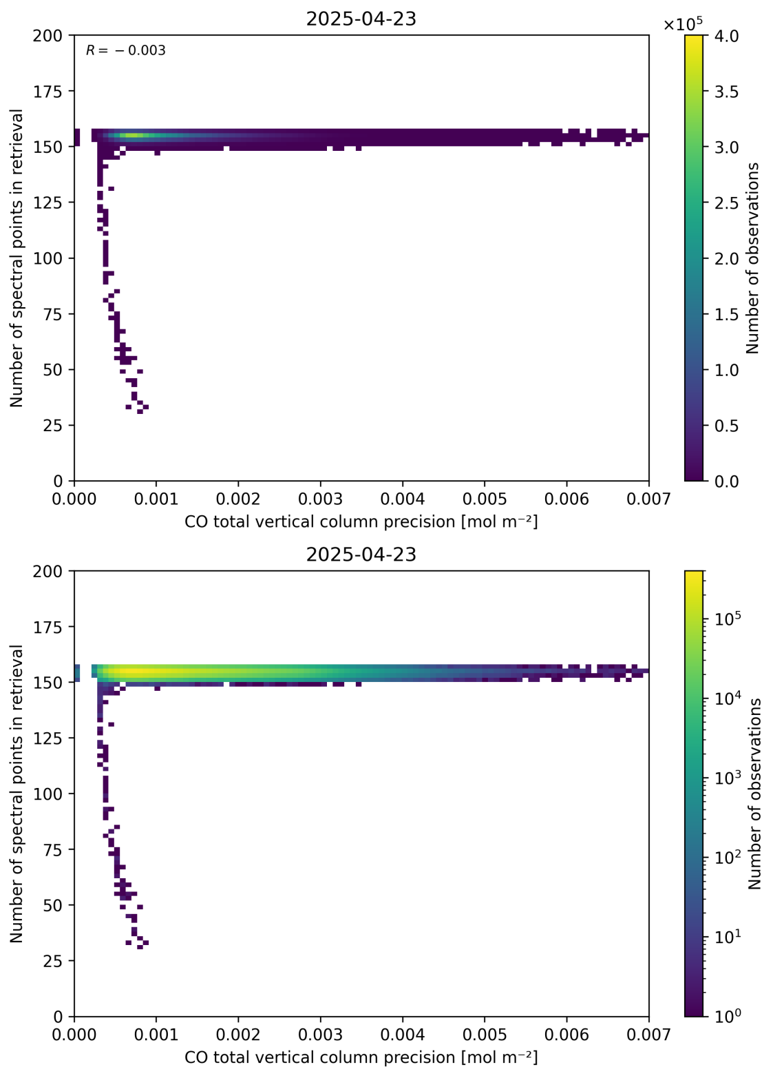
Figure 47: Scatter density plot of “CO total vertical column precision” against “Number of spectral points in retrieval” for 2025-04-22 to 2025-04-24.
