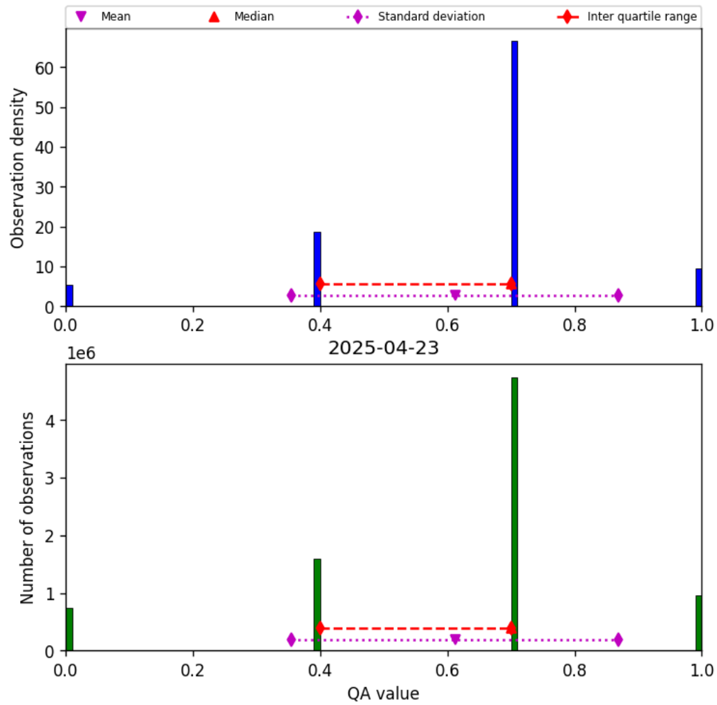
Figure 17: Histogram of “QA value” for 2025-04-22 to 2025-04-24
