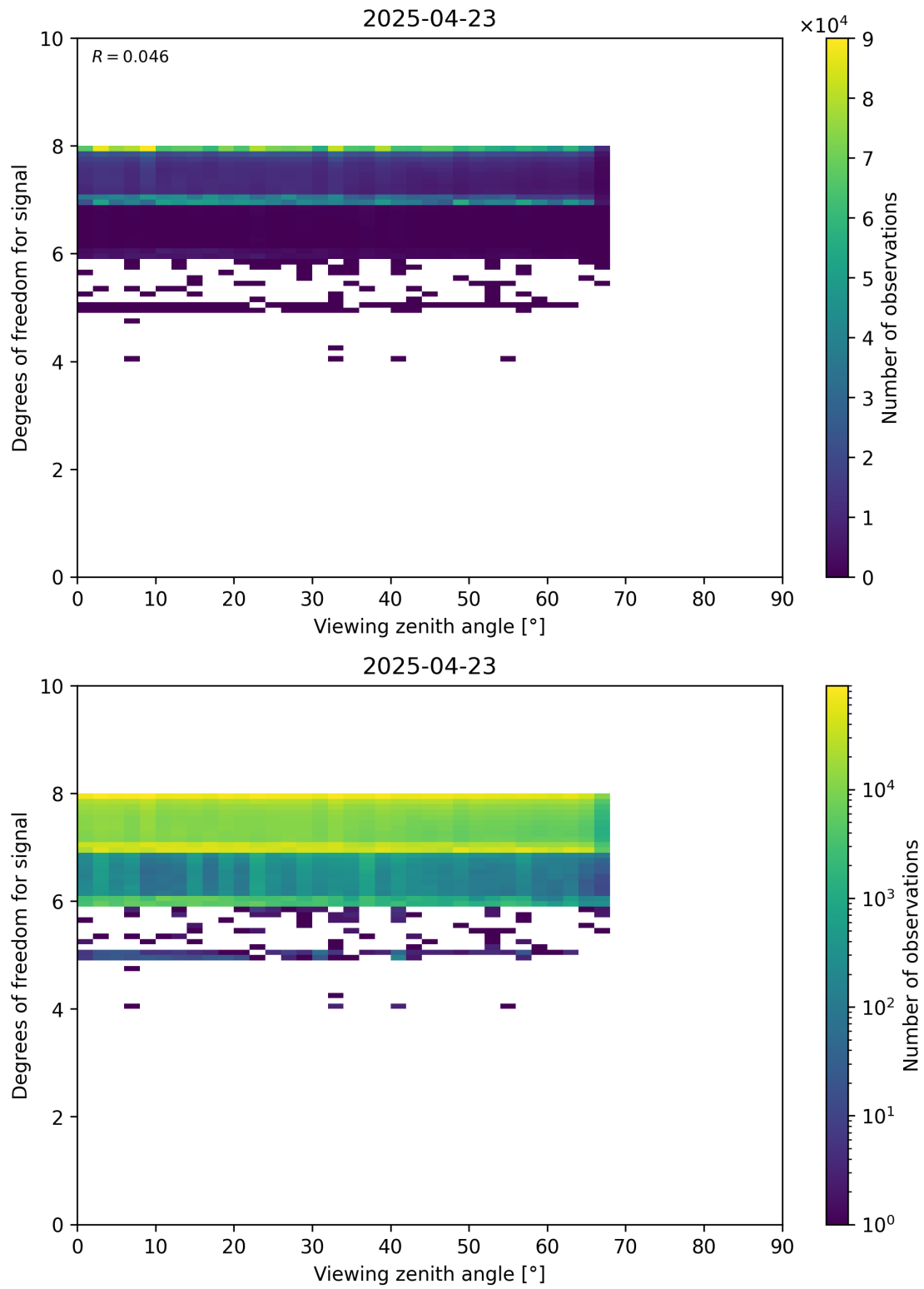
Figure 73: Scatter density plot of “Viewing zenith angle” against “Degrees of freedom for signal” for 2025-04-22 to 2025-04-24.
