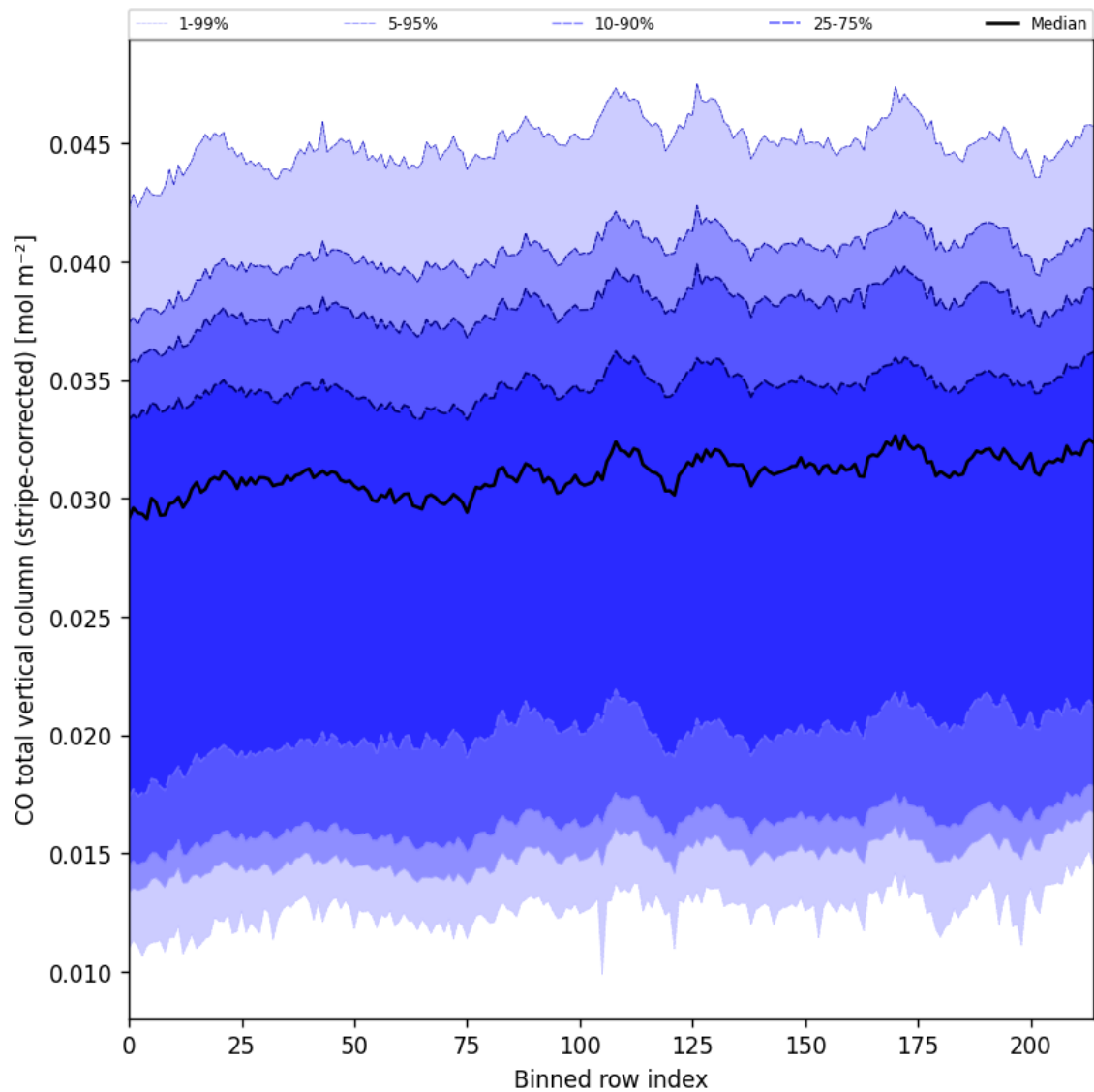
Figure 27: Along track statistics of “CO total vertical column (stripe-corrected)” for 2025-04-22 to 2025-04-24
