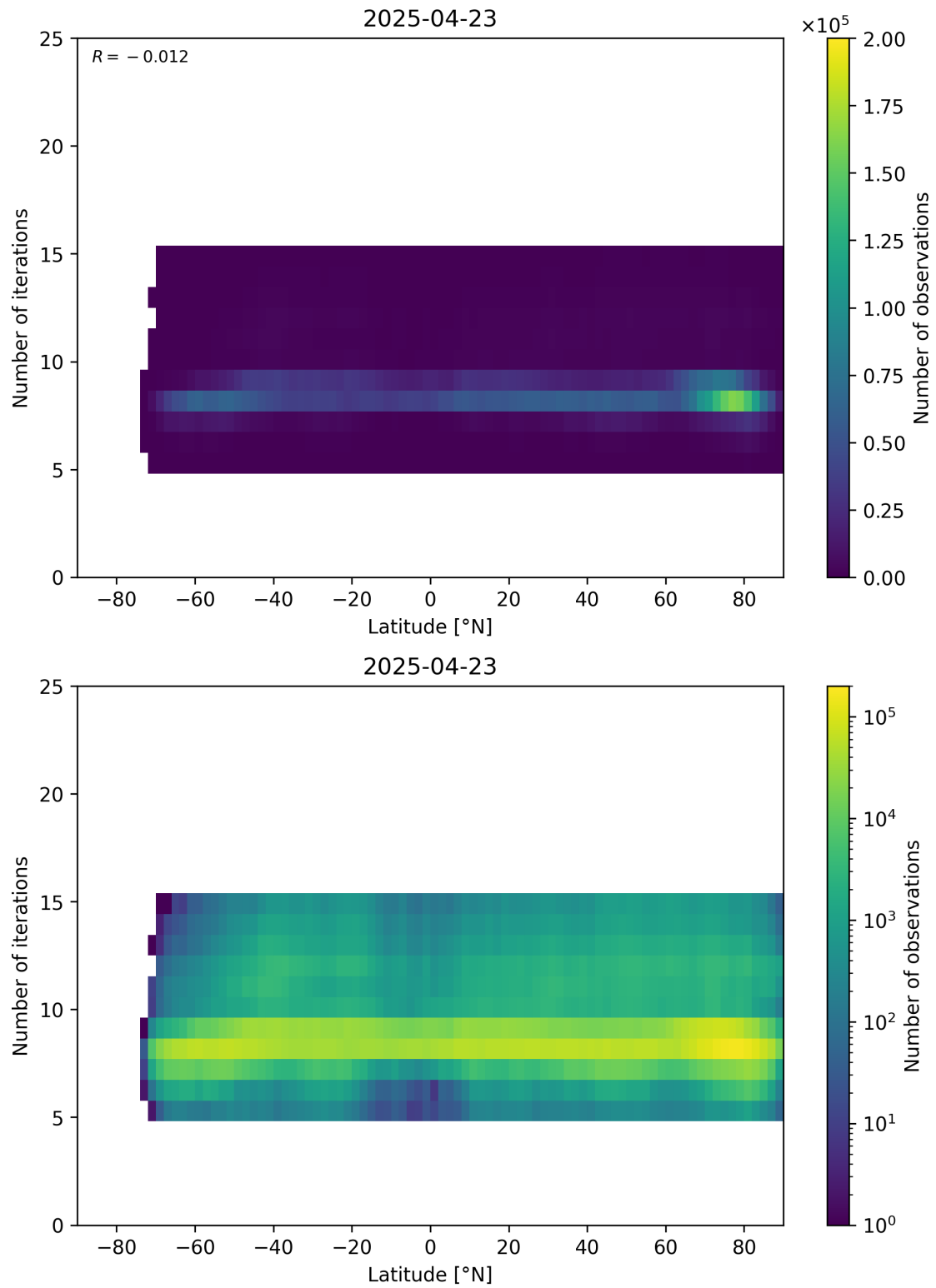
Figure 56: Scatter density plot of “Latitude” against “Number of iterations” for 2025-04-22 to 2025-04-24.
