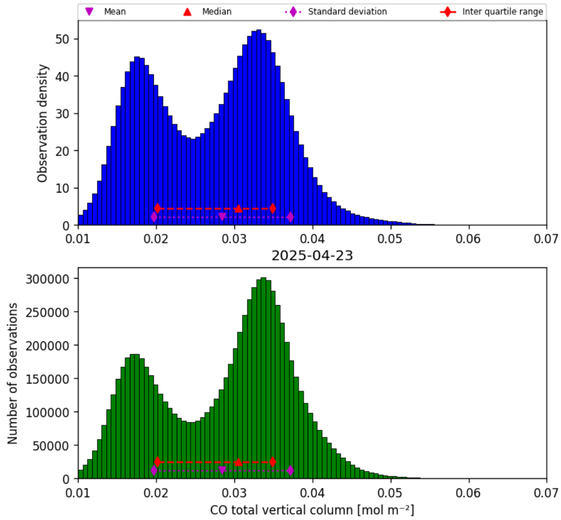
Figure 18: Histogram of “CO total vertical column” for 2025-04-22 to 2025-04-24
