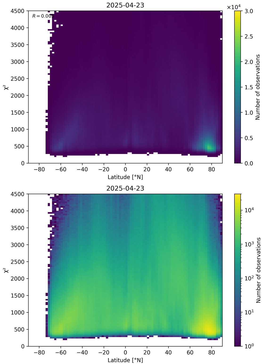
Figure 54: Scatter density plot of “Latitude” against “ \chi^2 ” for 2025-04-22 to 2025-04-24.
