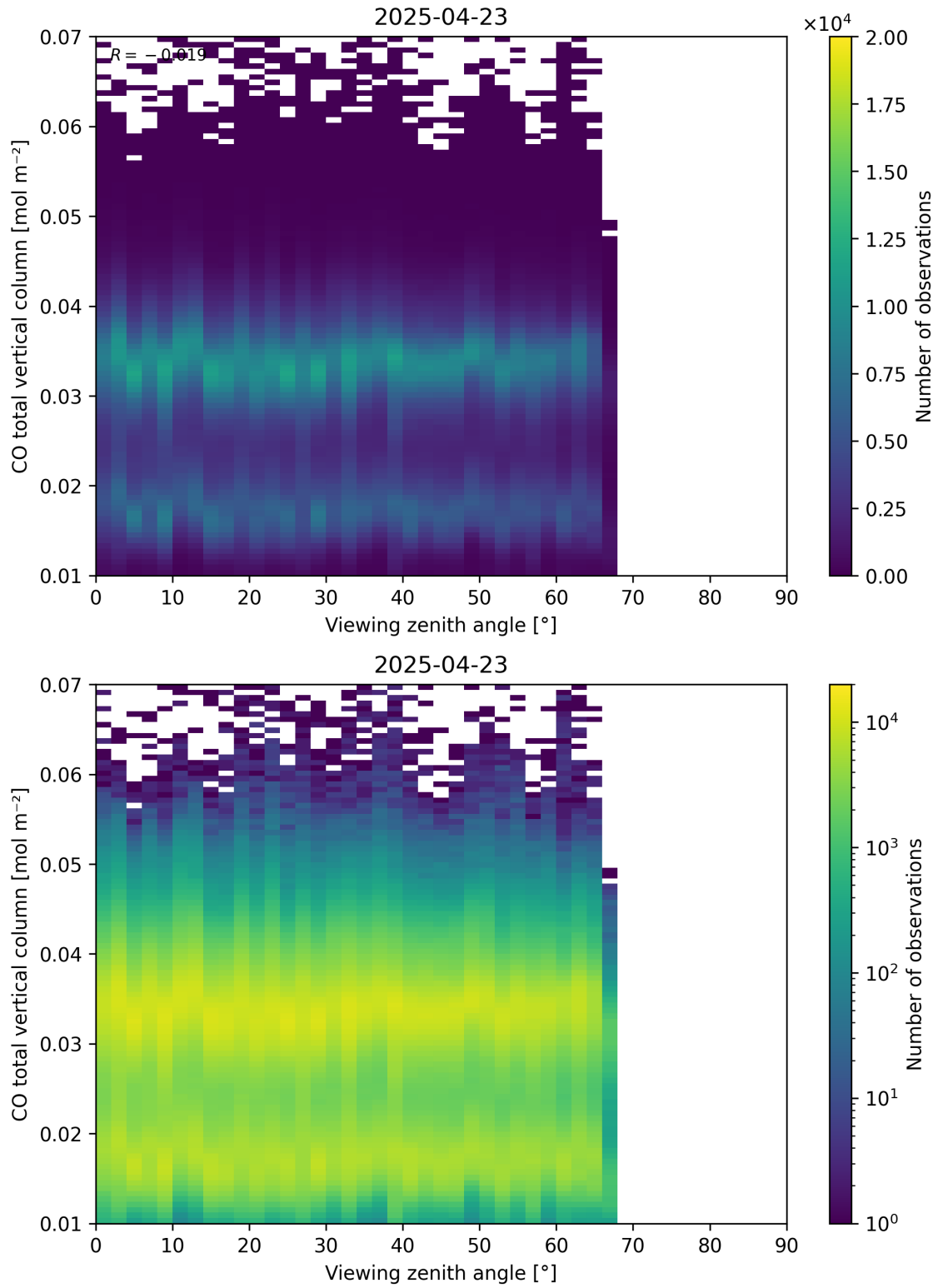
Figure 69: Scatter density plot of “Viewing zenith angle” against “CO total vertical column” for 2025-04-22 to 2025-04-24.
