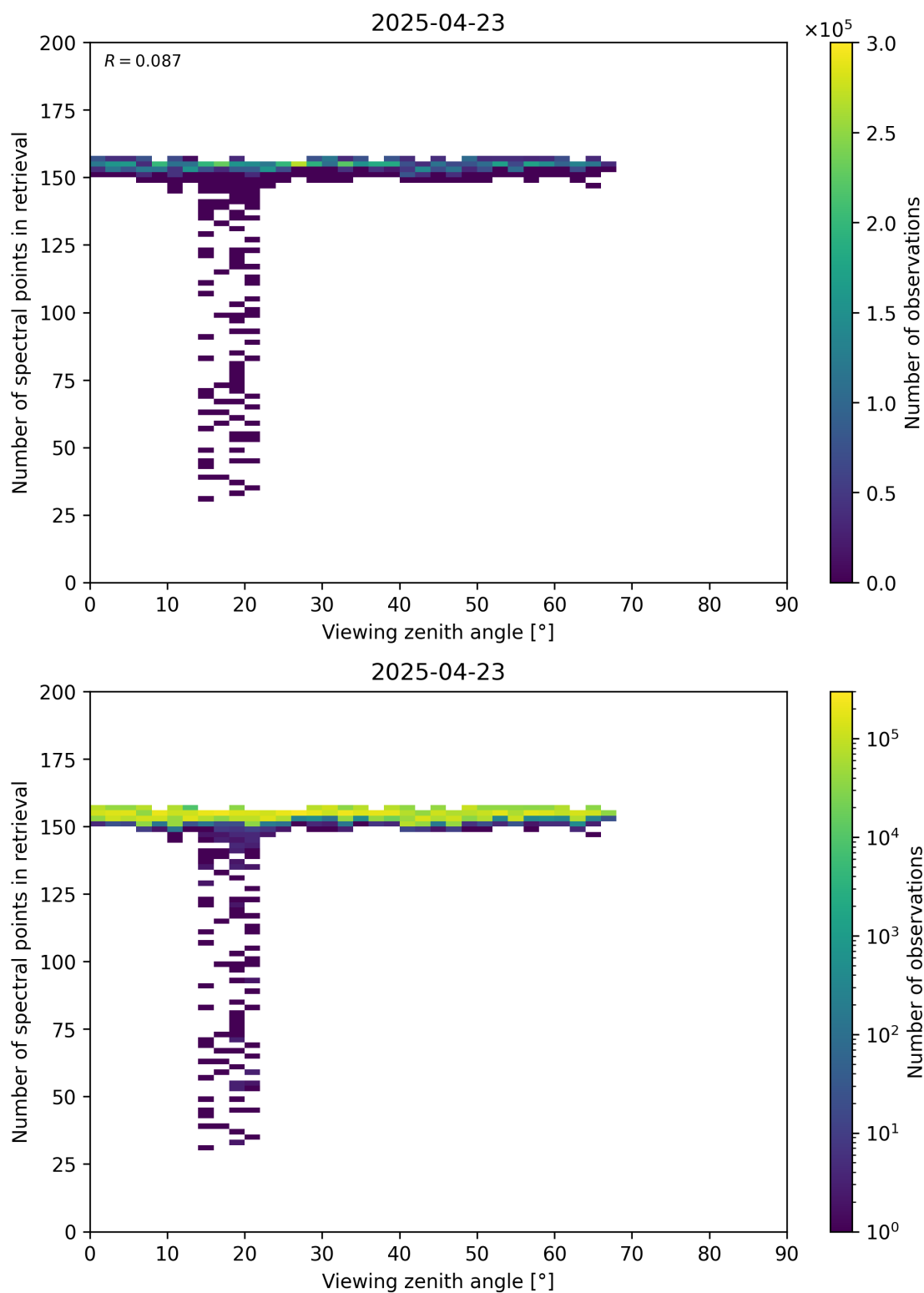
Figure 76: Scatter density plot of “Viewing zenith angle” against “Number of spectral points in retrieval” for 2025-04-22 to 2025-04-24.
