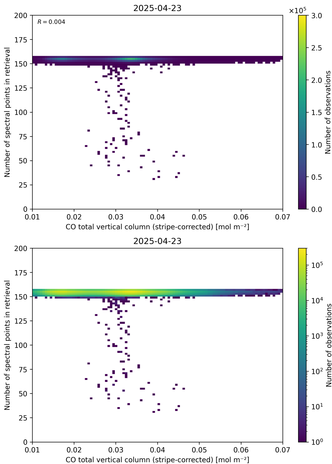
Figure 40: Scatter density plot of “CO total vertical column (stripe-corrected)” against “Number of spectral points in retrieval” for 2025-04-22 to 2025-04-24.
