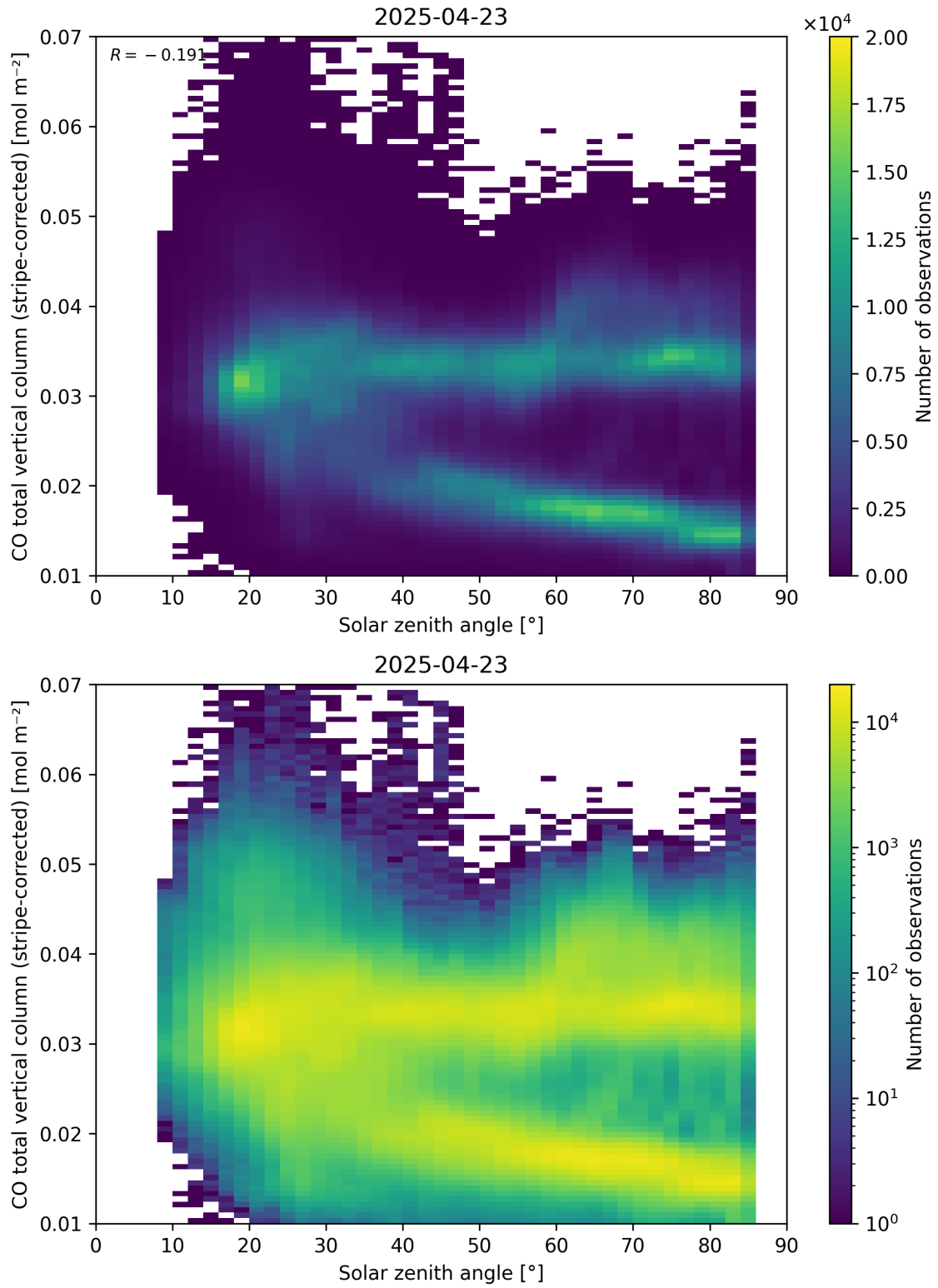
Figure 62: Scatter density plot of “Solar zenith angle” against “CO total vertical column (stripe-corrected)” for 2025-04-22 to 2025-04-24.
