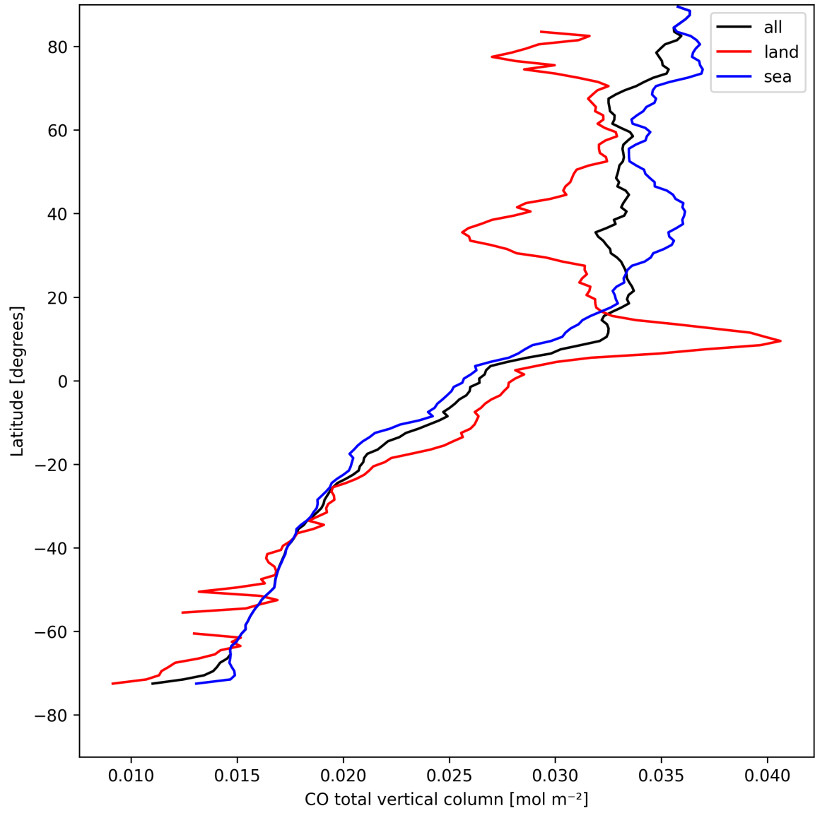
Figure 10: Zonal average of “CO total vertical column” for 2025-04-22 to 2025-04-24.
