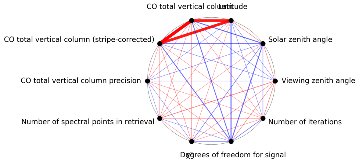
Figure 1: Map of correlation graph for 2025-04-22 to 2025-04-24.
