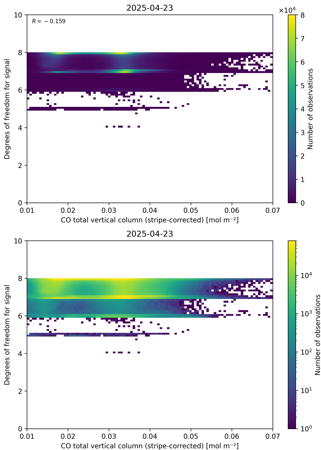
Figure 38: Scatter density plot of “CO total vertical column (stripe-corrected)” against “Degrees of freedom for signal” for 2025-04-22 to 2025-04-24.
