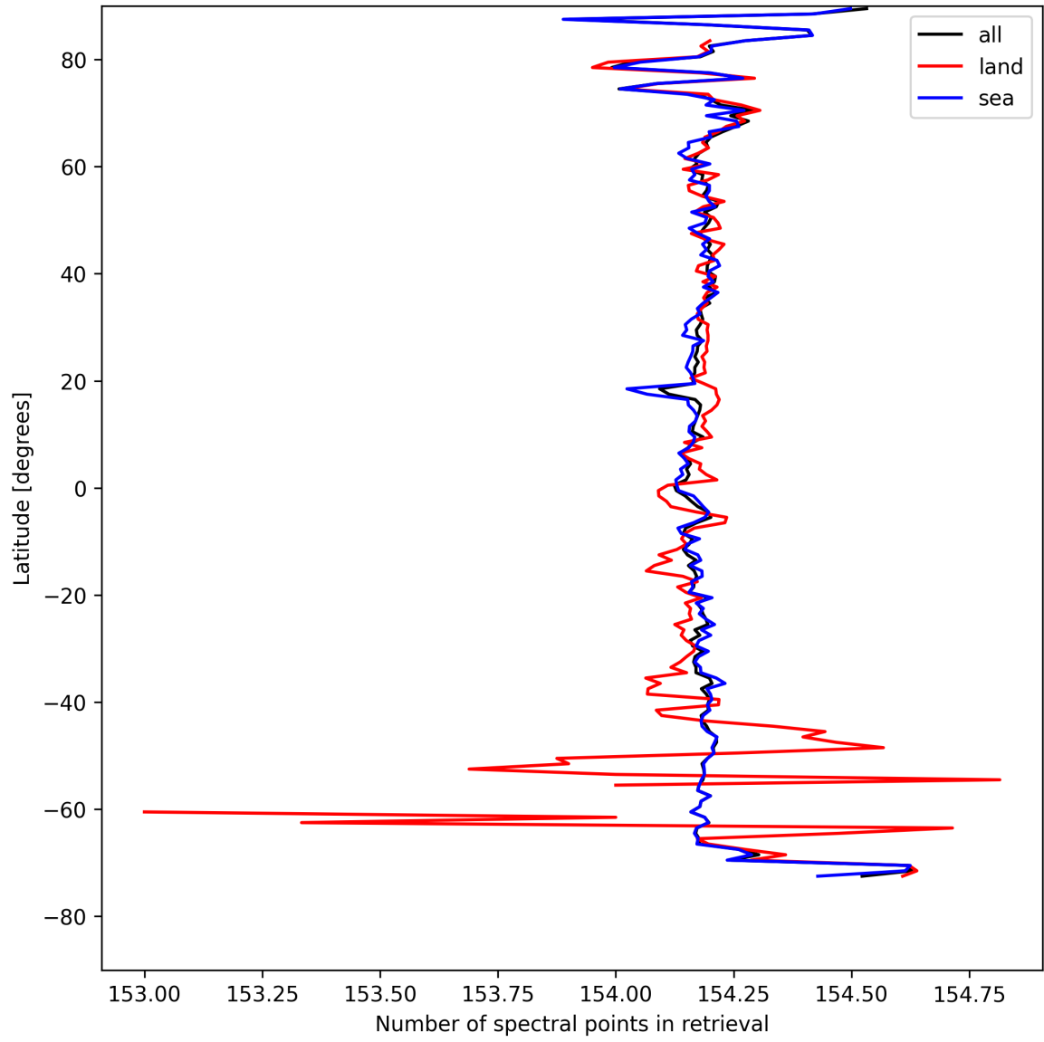
Figure 13: Zonal average of “Number of spectral points in retrieval” for 2025-04-22 to 2025-04-24.
