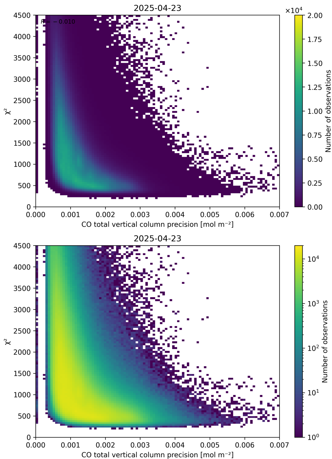
Figure 44: Scatter density plot of “CO total vertical column precision” against “ \chi^2 ” for 2025-04-22 to 2025-04-24.
