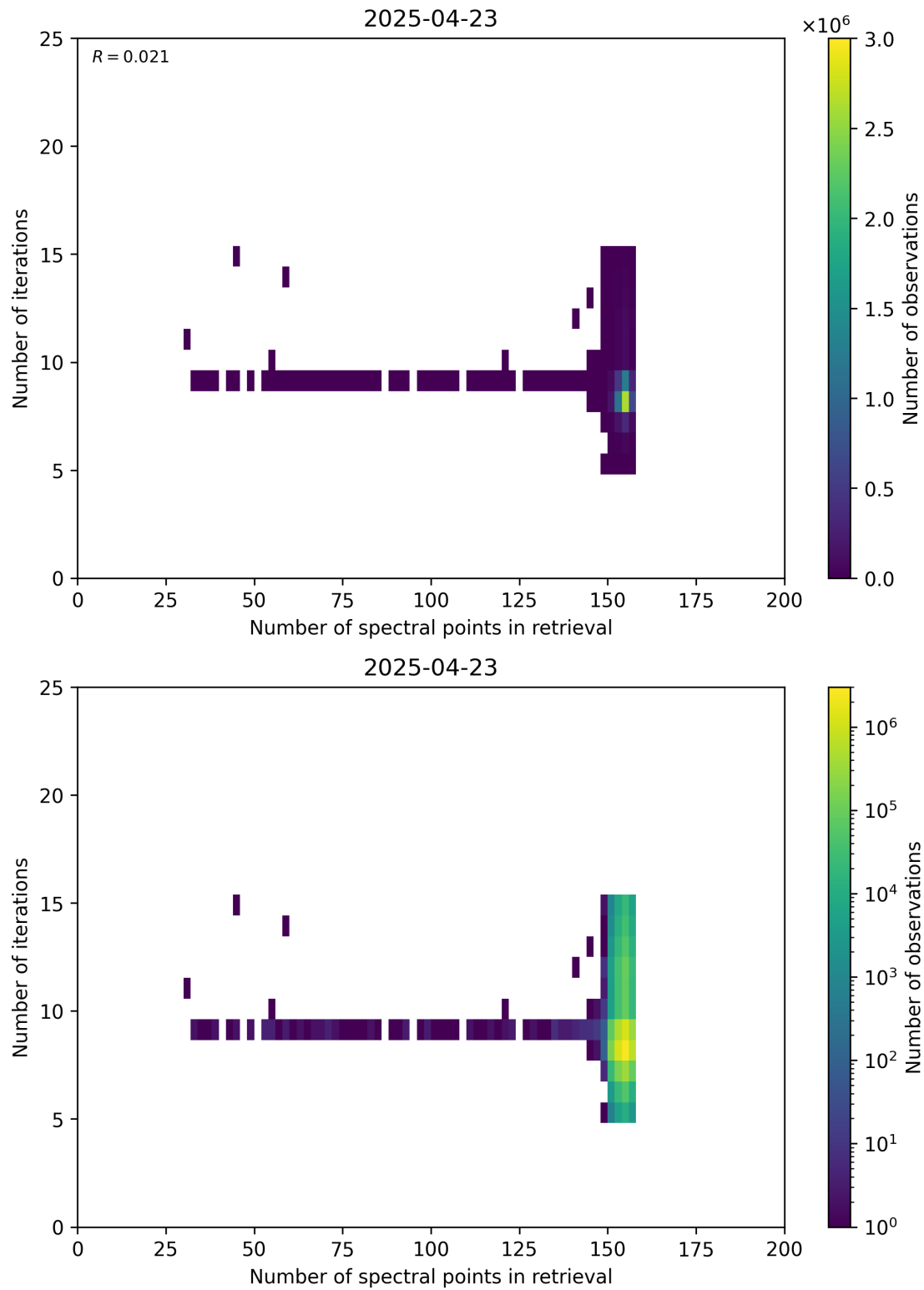
Figure 60: Scatter density plot of “Number of spectral points in retrieval” against “Number of iterations” for 2025-04-22 to 2025-04-24.
