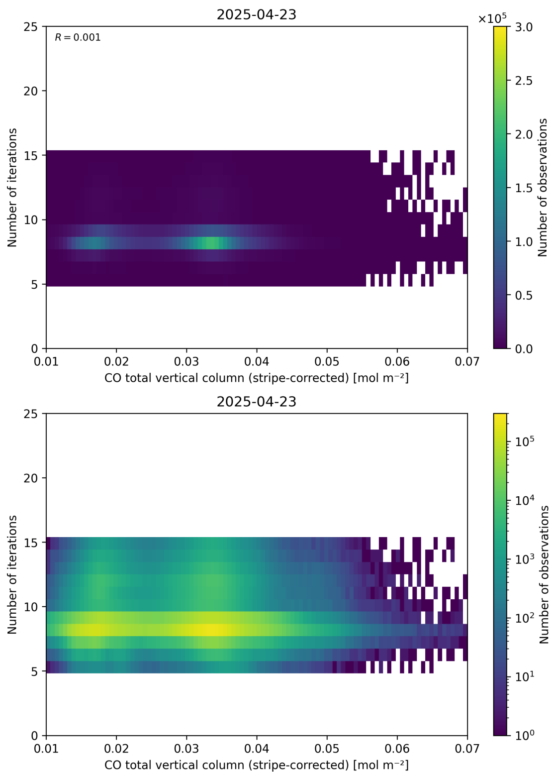
Figure 39: Scatter density plot of “CO total vertical column (stripe-corrected)” against “Number of iterations” for 2025-04-22 to 2025-04-24.
