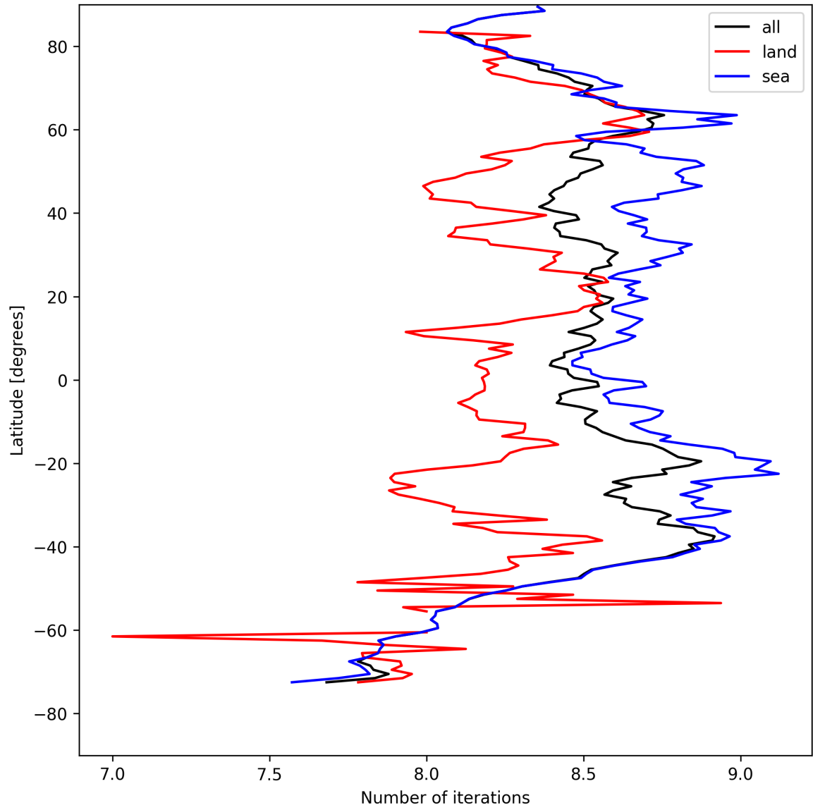
Figure 16: Zonal average of “Number of iterations” for 2025-04-22 to 2025-04-24.
