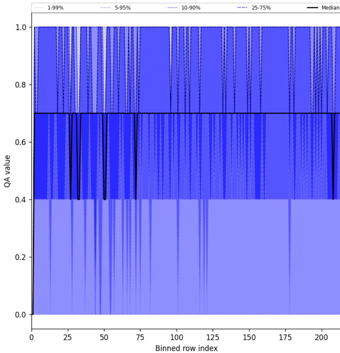
Figure 25: Along track statistics of “QA value” for 2025-04-22 to 2025-04-24
