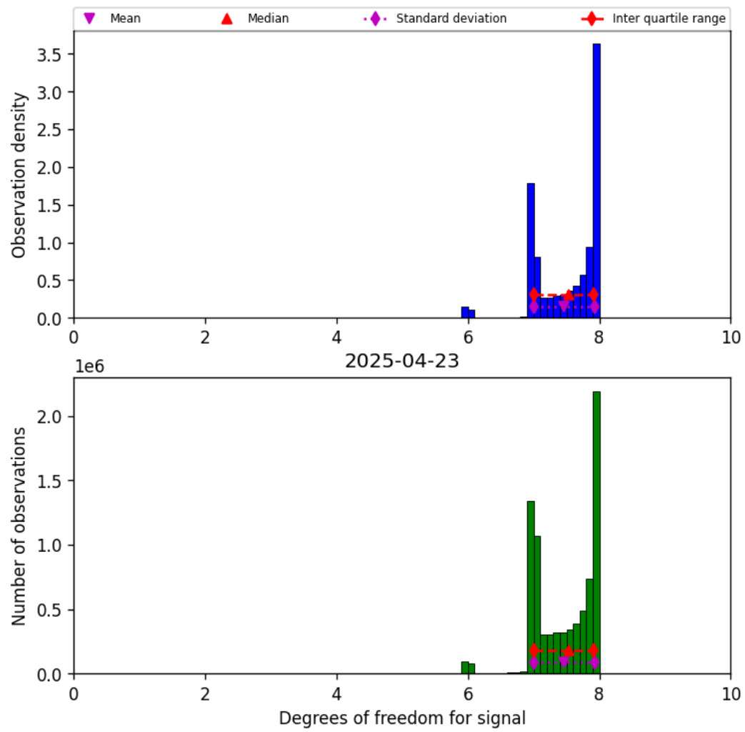
Figure 23: Histogram of “Degrees of freedom for signal” for 2025-04-22 to 2025-04-24
