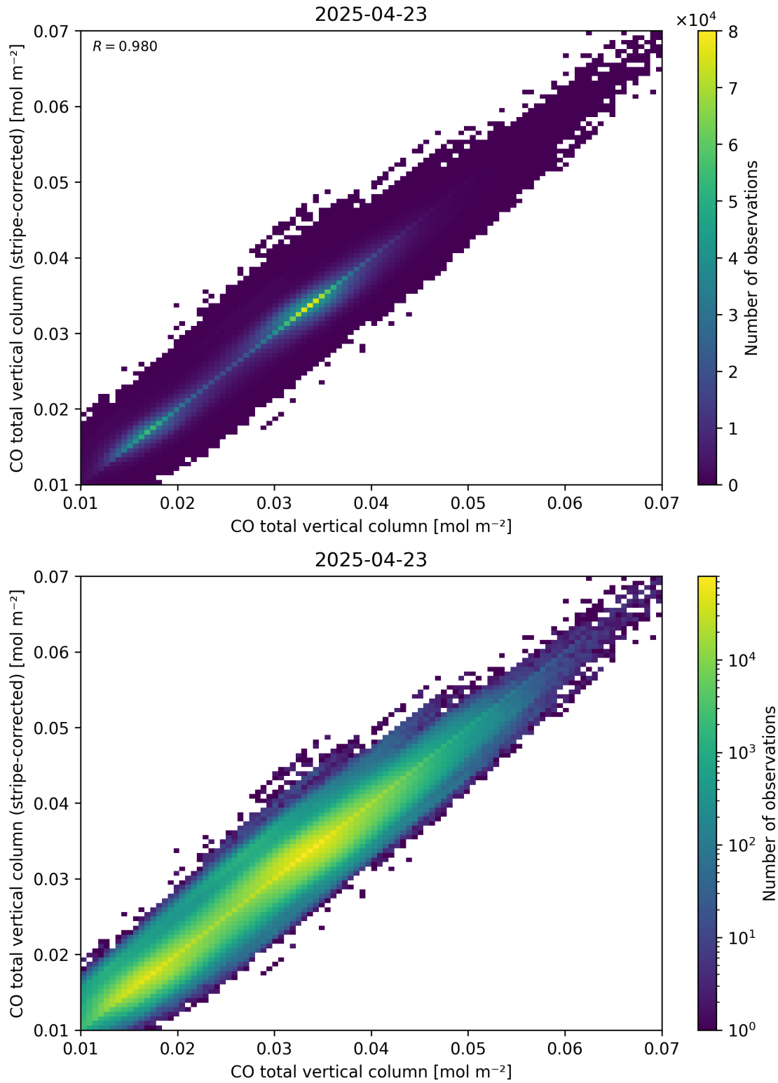
Figure 33: Scatter density plot of “CO total vertical column” against “CO total vertical column (stripe-corrected)” for 2025-04-22 to 2025-04-24.
