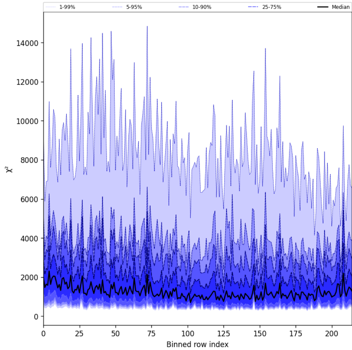
Figure 30: Along track statistics of “ \chi^2 ” for 2025-04-22 to 2025-04-24
