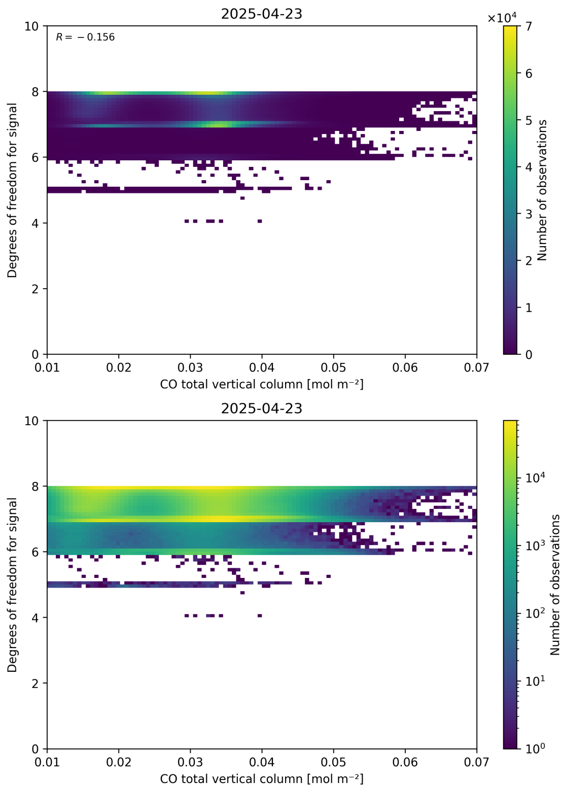
Figure 41: Scatter density plot of “CO total vertical column” against “Degrees of freedom for signal” for 2025-04-22 to 2025-04-24.
