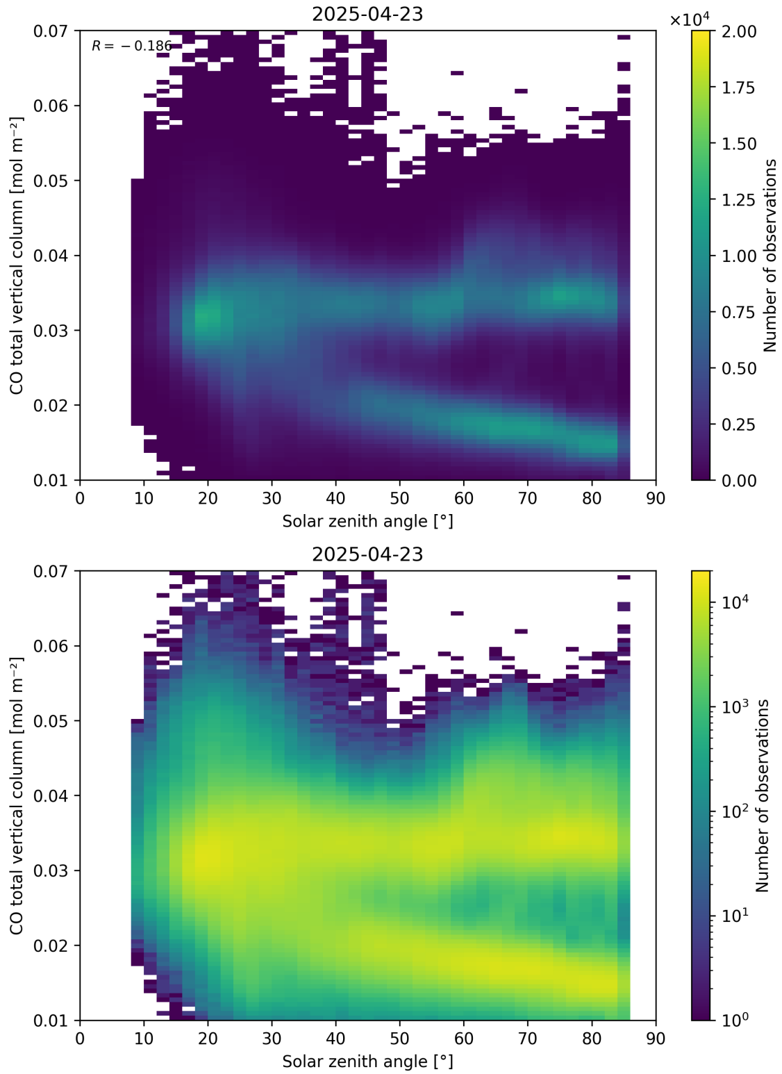
Figure 61: Scatter density plot of “Solar zenith angle” against “CO total vertical column” for 2025-04-22 to 2025-04-24.
