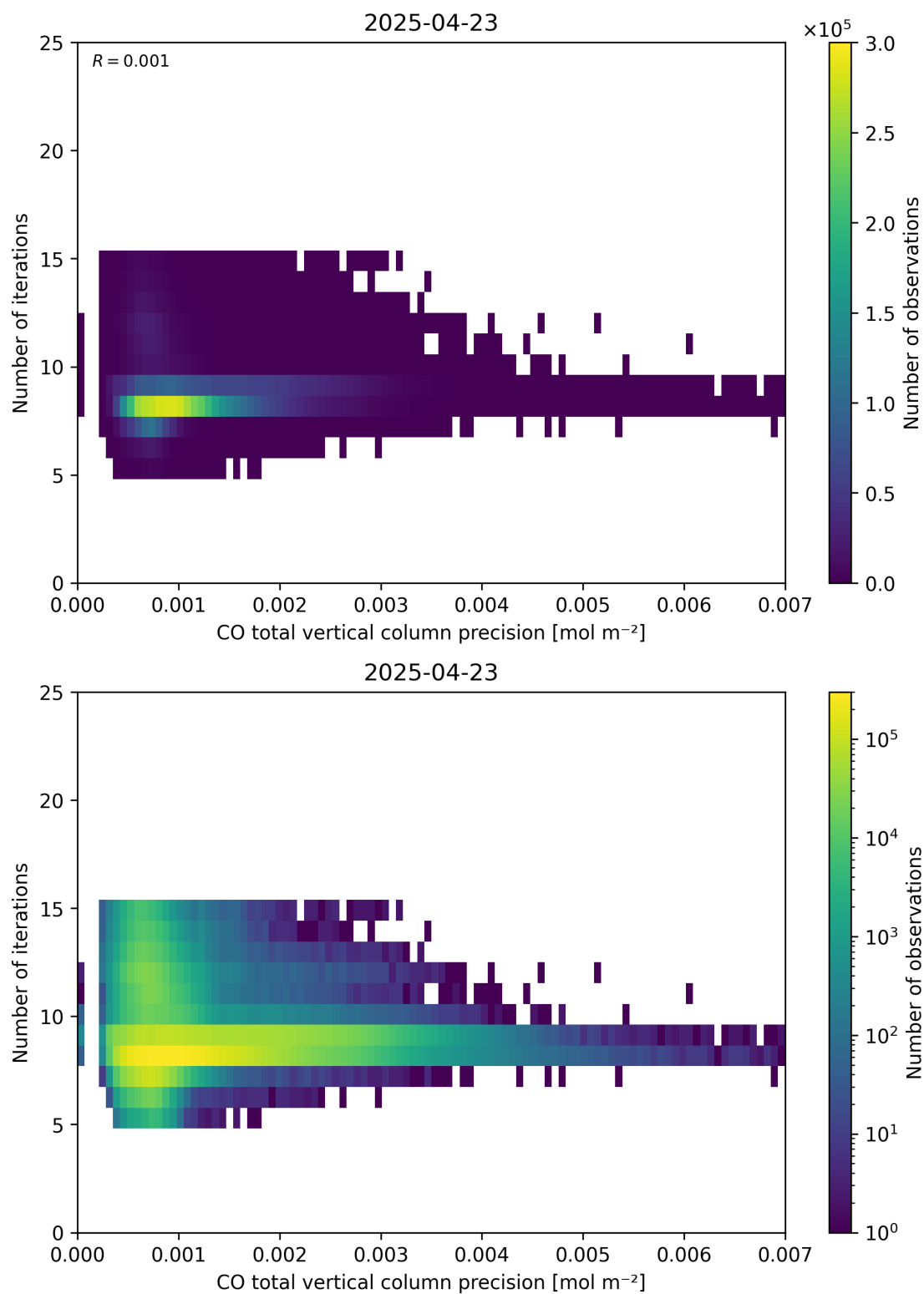
Figure 46: Scatter density plot of “CO total vertical column precision” against “Number of iterations” for 2025-04-22 to 2025-04-24.
