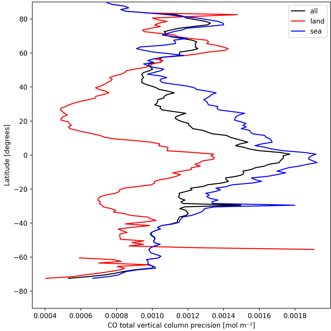
Figure 12: Zonal average of "CO total vertical column precision" for 2025-04-22 to 2025-04-24.
