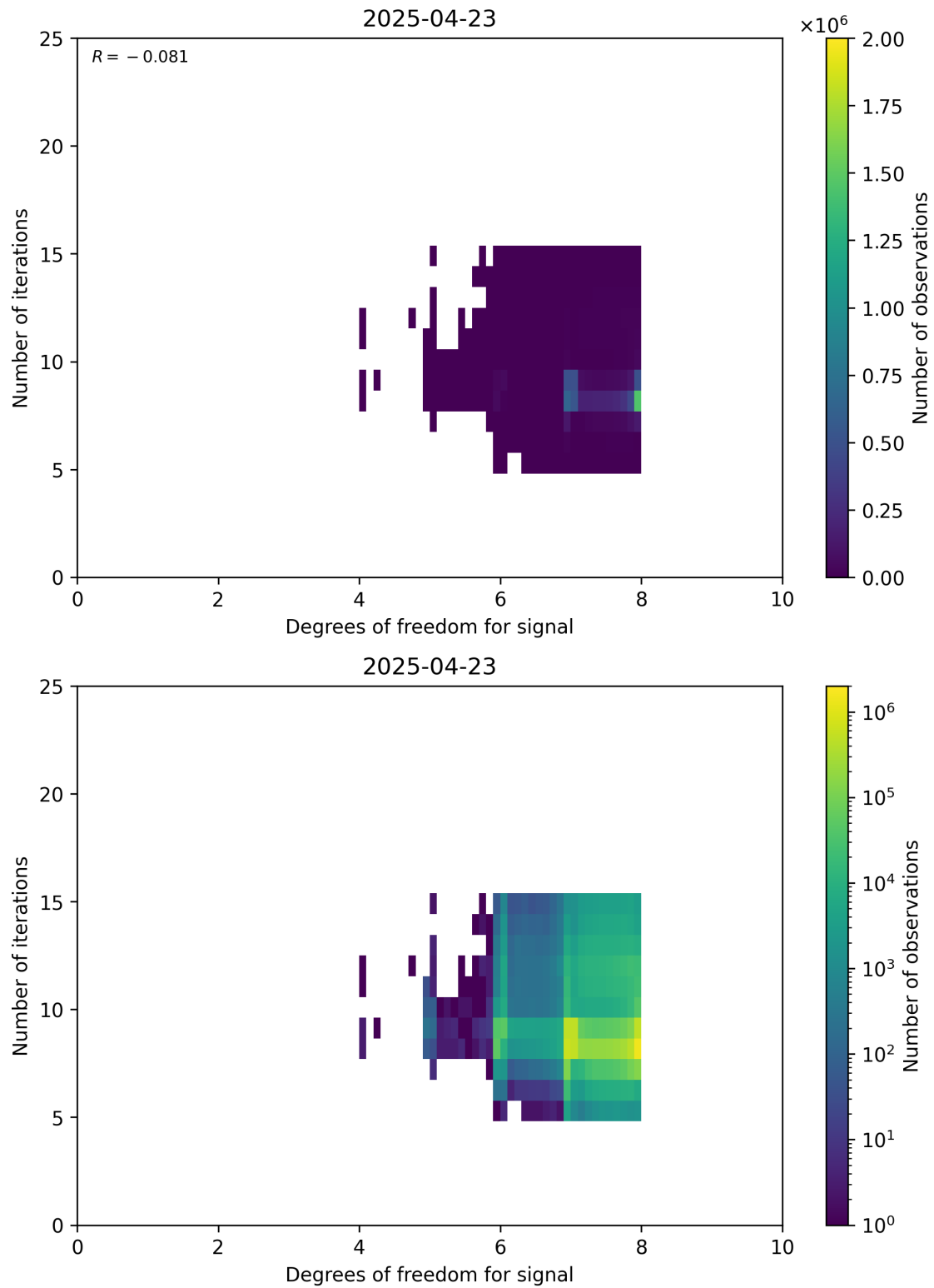
Figure 50: Scatter density plot of “Degrees of freedom for signal” against “Number of iterations” for 2025-04-22 to 2025-04-24.
