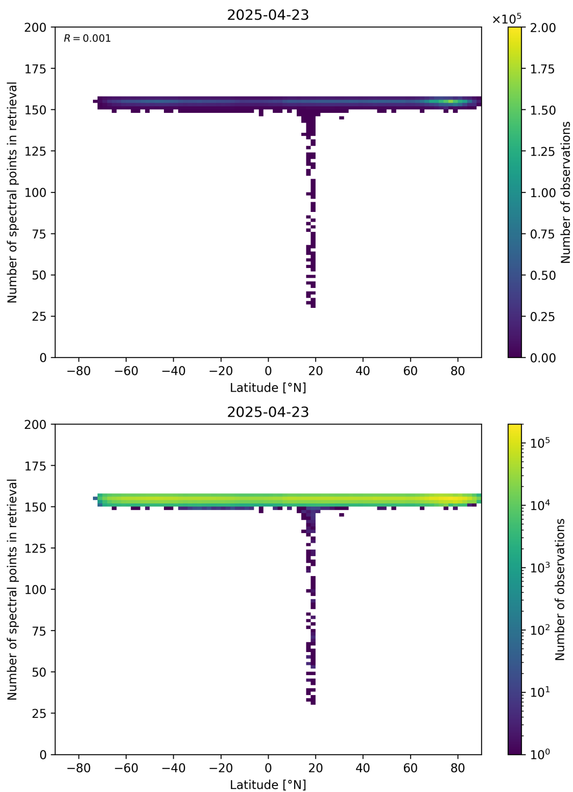
Figure 57: Scatter density plot of “Latitude” against “Number of spectral points in retrieval” for 2025-04-22 to 2025-04-24.
