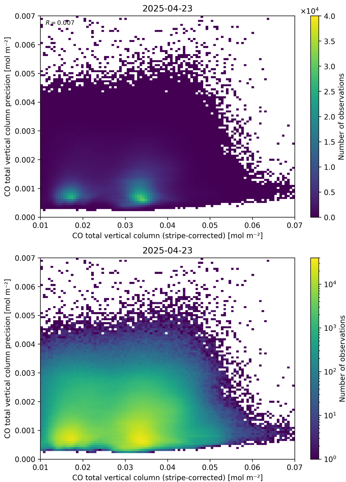
Figure 36: Scatter density plot of “CO total vertical column (stripe-corrected)” against “CO total vertical column precision” for 2025-04-22 to 2025-04-24.
