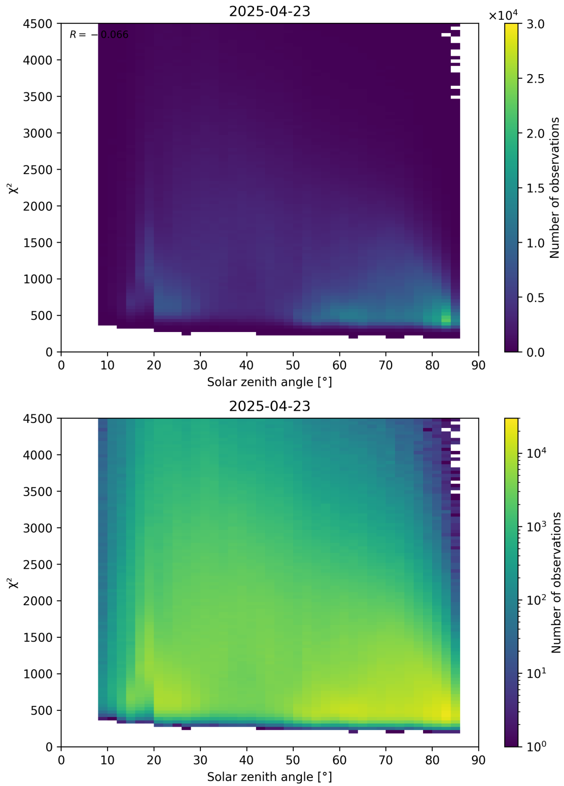
Figure 64: Scatter density plot of “Solar zenith angle” against “ \chi^2 ” for 2025-04-22 to 2025-04-24.
