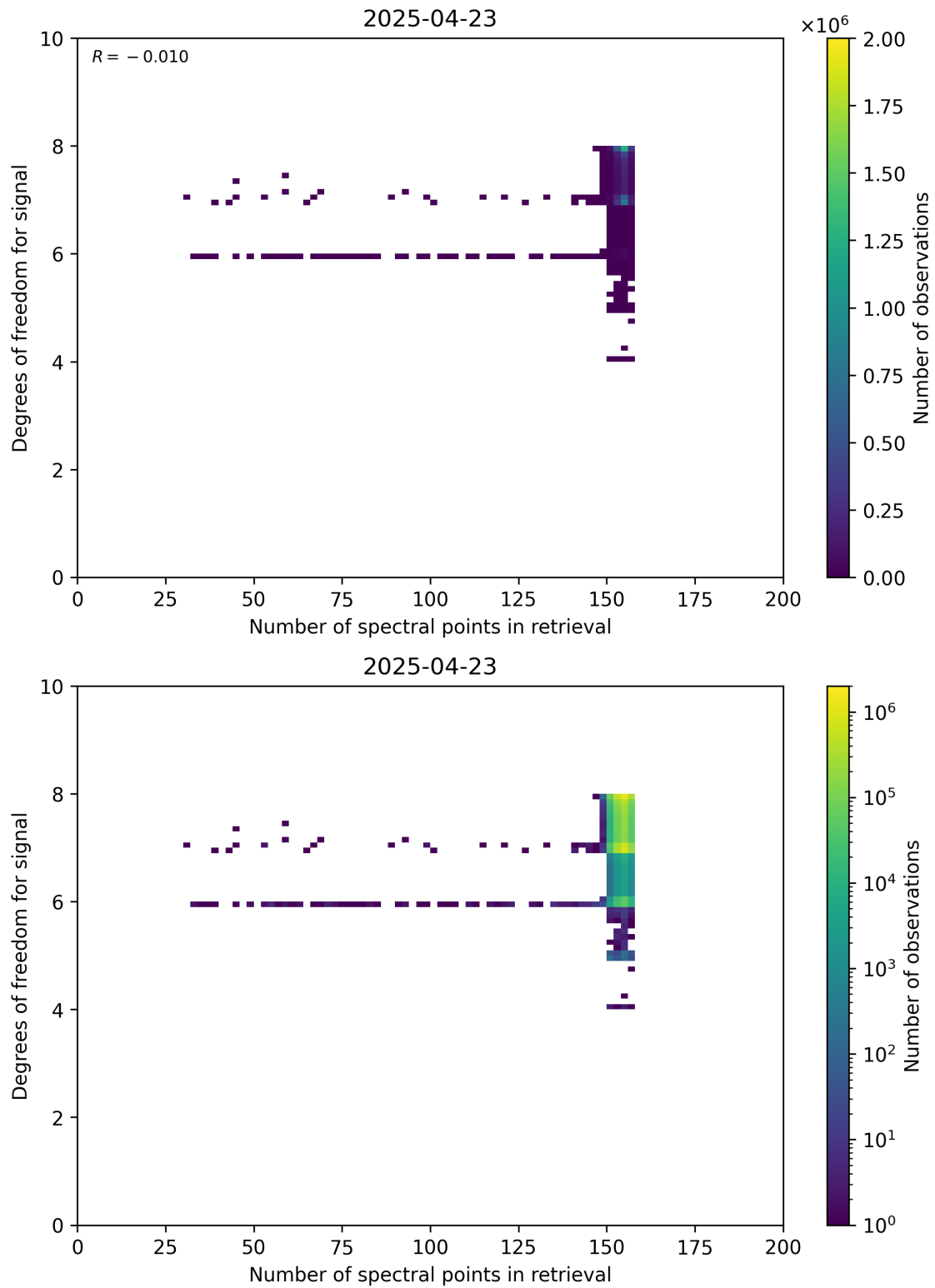
Figure 59: Scatter density plot of “Number of spectral points in retrieval” against “Degrees of freedom for signal” for 2025-04-22 to 2025-04-24.
