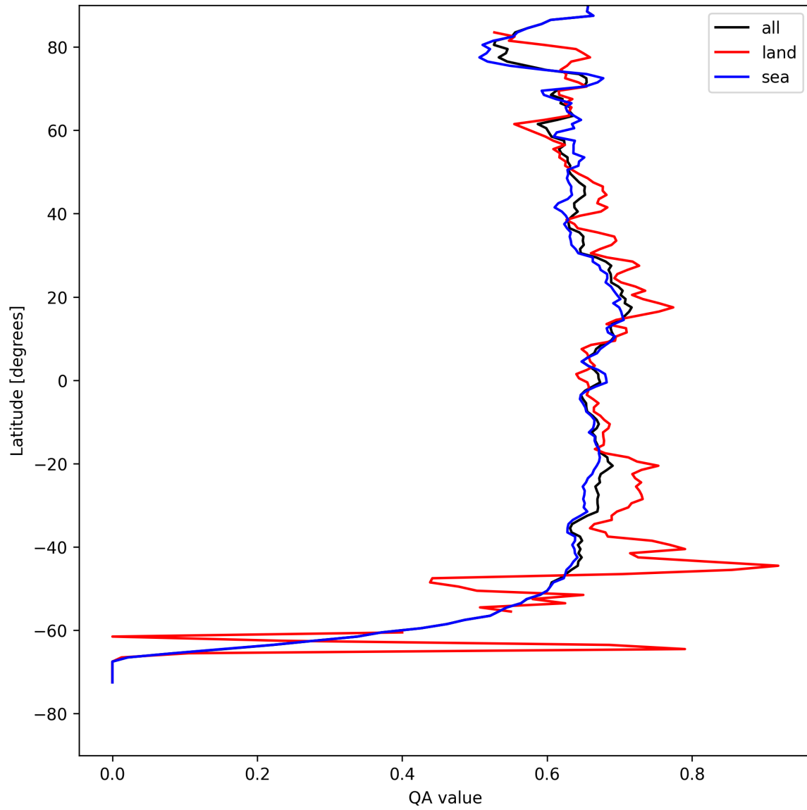
Figure 9: Zonal average of “QA value” for 2025-04-22 to 2025-04-24.
