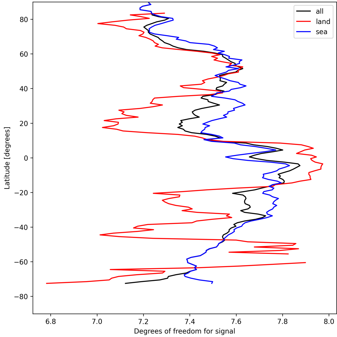
Figure 15: Zonal average of “Degrees of freedom for signal” for 2025-04-22 to 2025-04-24.
