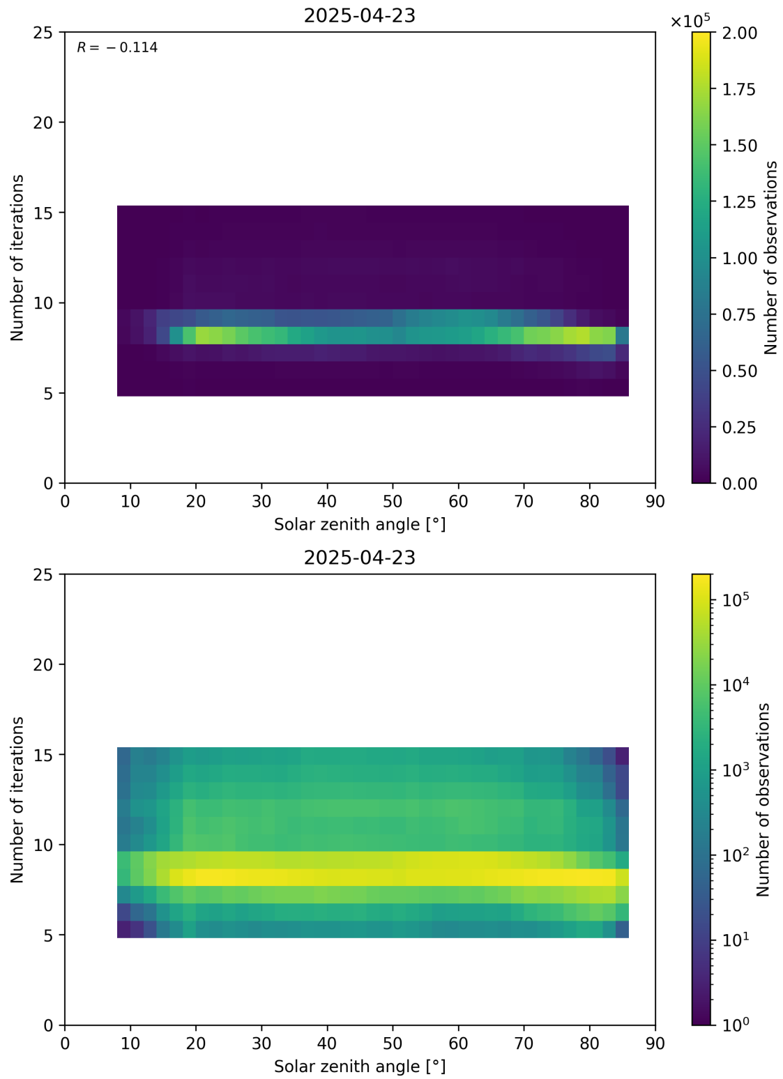
Figure 67: Scatter density plot of “Solar zenith angle” against “Number of iterations” for 2025-04-22 to 2025-04-24.
