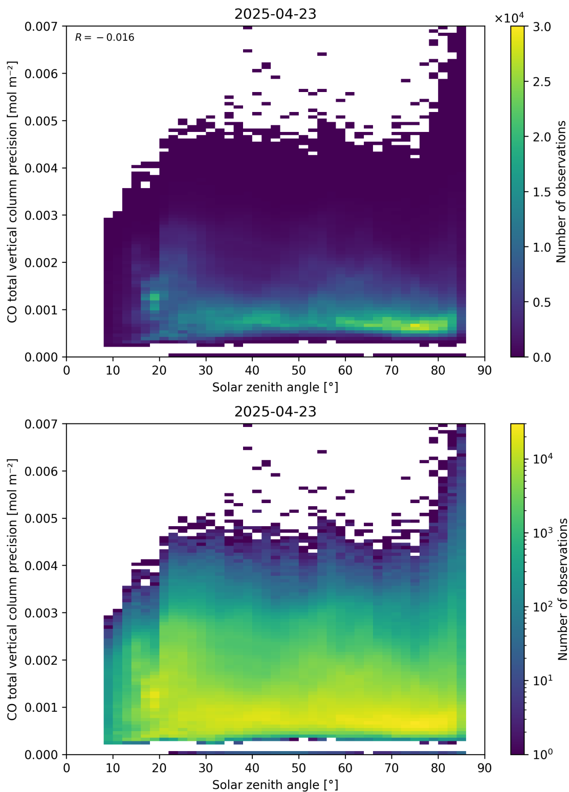
Figure 63: Scatter density plot of “Solar zenith angle” against “CO total vertical column precision” for 2025-04-22 to 2025-04-24.
