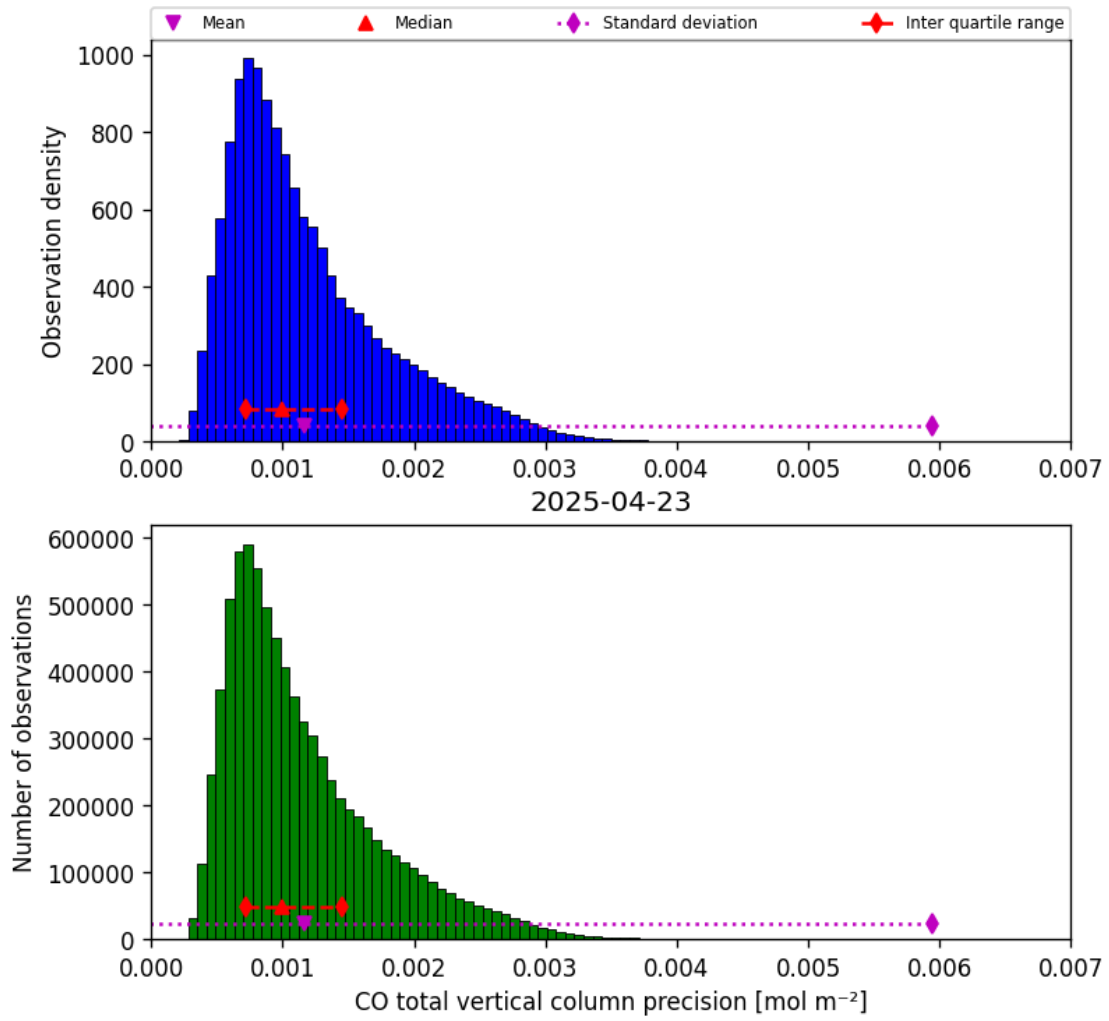
Figure 20: Histogram of “CO total vertical column precision” for 2025-04-22 to 2025-04-24
