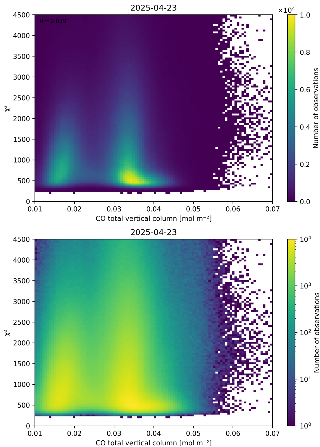
Figure 35: Scatter density plot of “CO total vertical column” against “ \chi^2 ” for 2025-04-22 to 2025-04-24.
