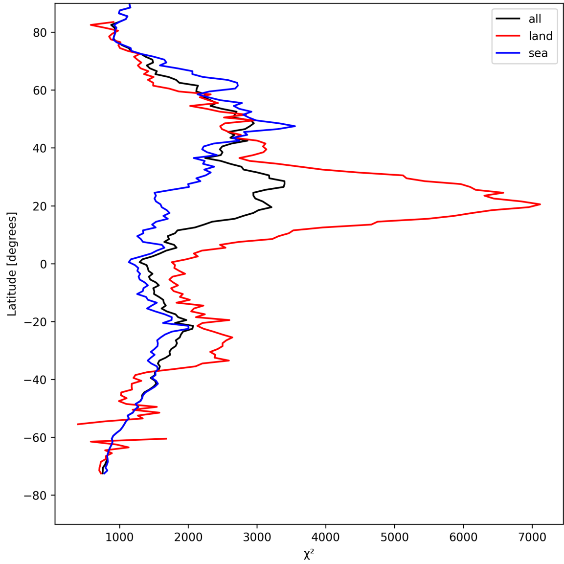
Figure 14: Zonal average of “ \chi^2 ” for 2025-04-22 to 2025-04-24.
