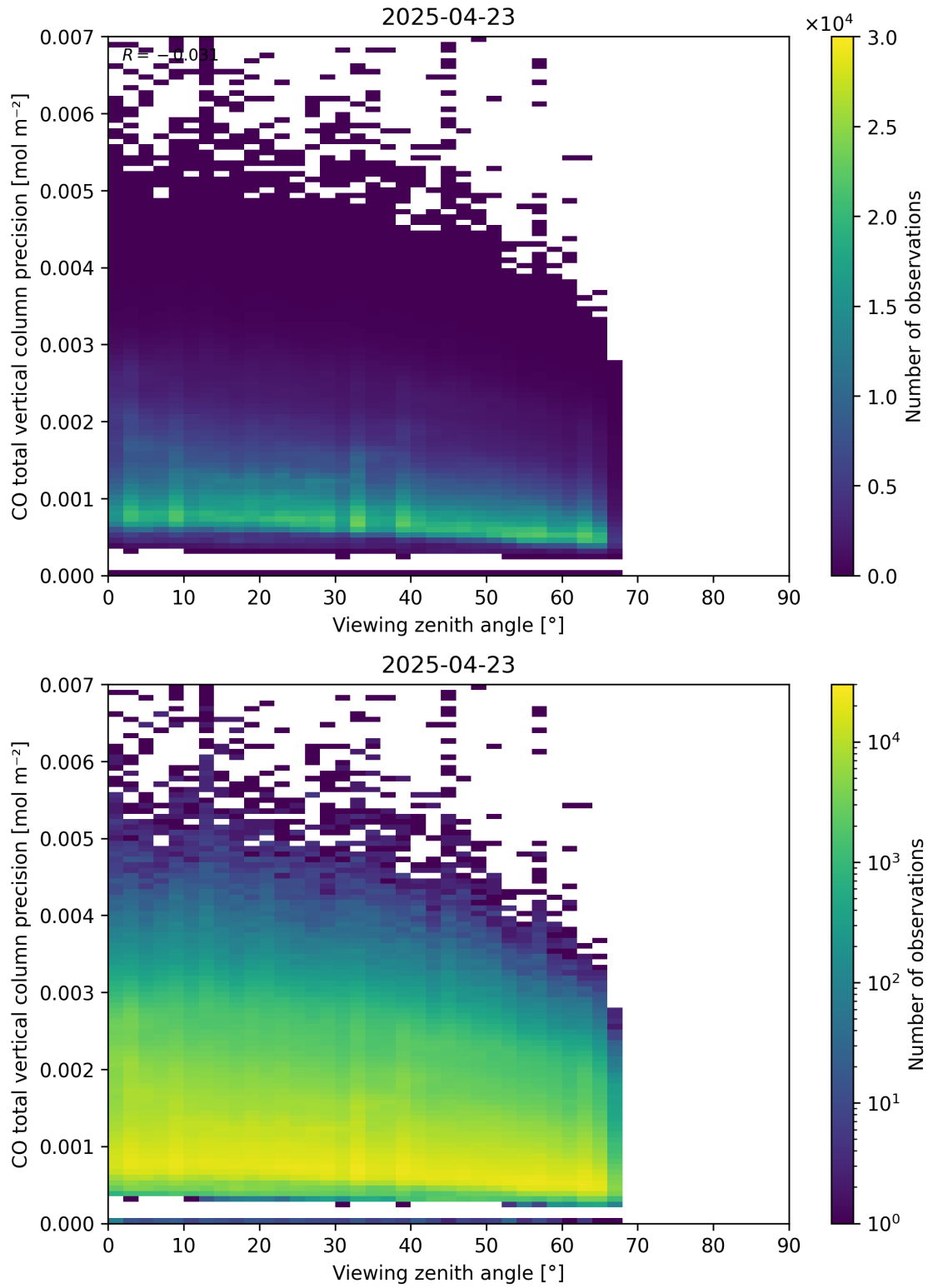
Figure 71: Scatter density plot of “Viewing zenith angle” against “CO total vertical column precision” for 2025-04-22 to 2025-04-24.
