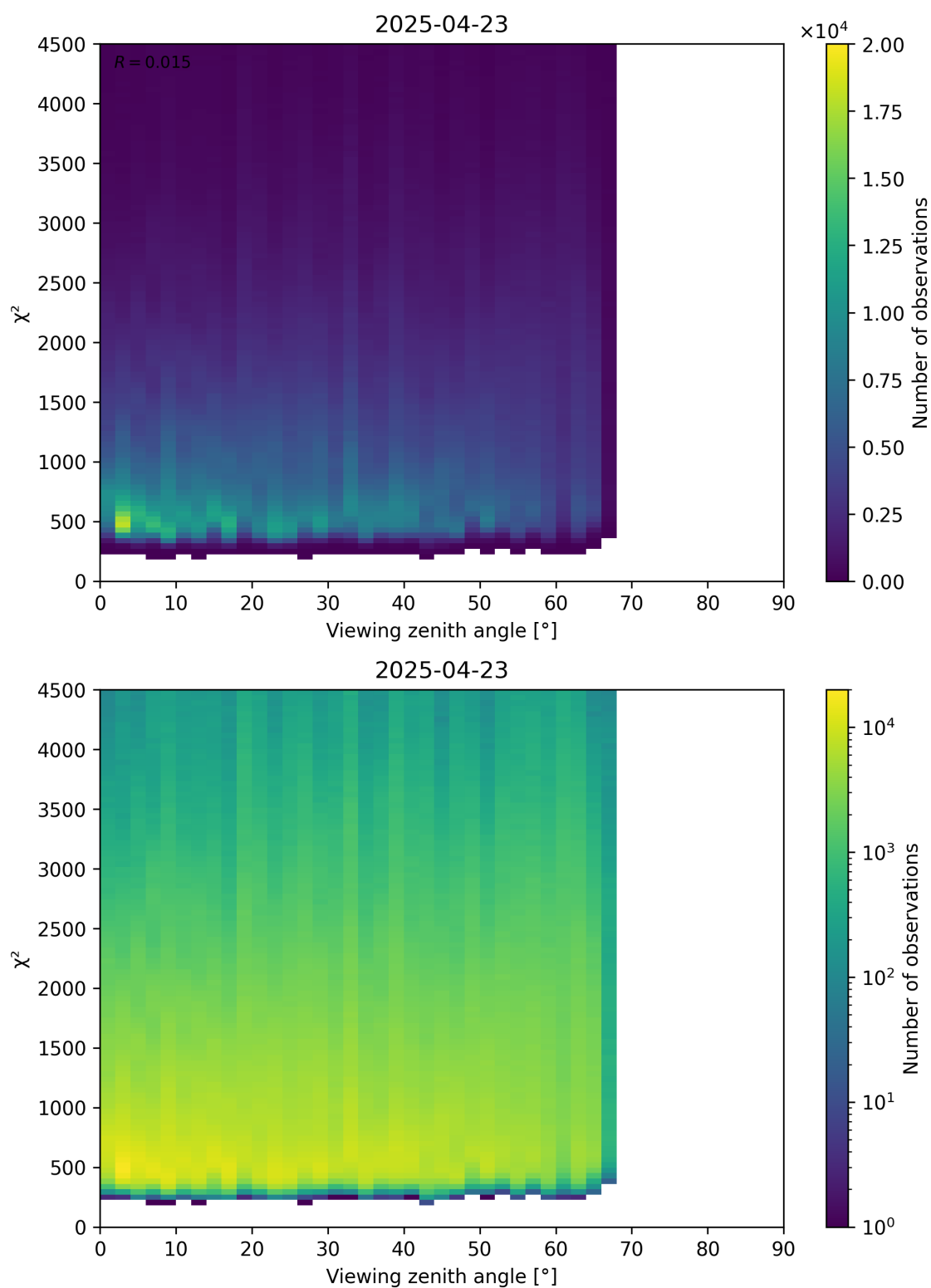
Figure 72: Scatter density plot of “Viewing zenith angle” against “ \chi^2 ” for 2025-04-22 to 2025-04-24.
