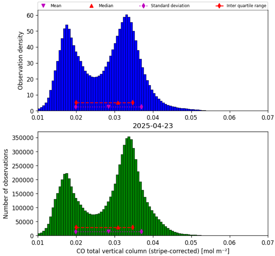
Figure 19: Histogram of “CO total vertical column (stripe-corrected)” for 2025-04-22 to 2025-04-24
