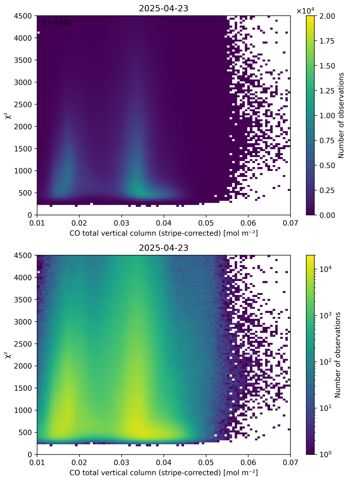
Figure 37: Scatter density plot of “CO total vertical column (stripe-corrected)” against “ \chi^2 ” for 2025-04-22 to 2025-04-24.
