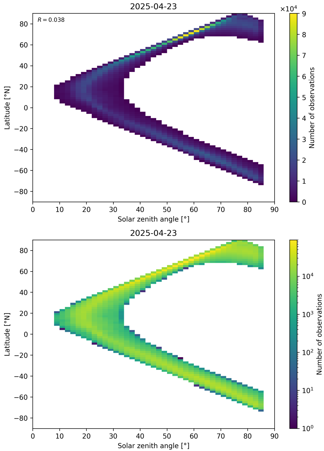
Figure 66: Scatter density plot of “Solar zenith angle” against “Latitude” for 2025-04-22 to 2025-04-24.
