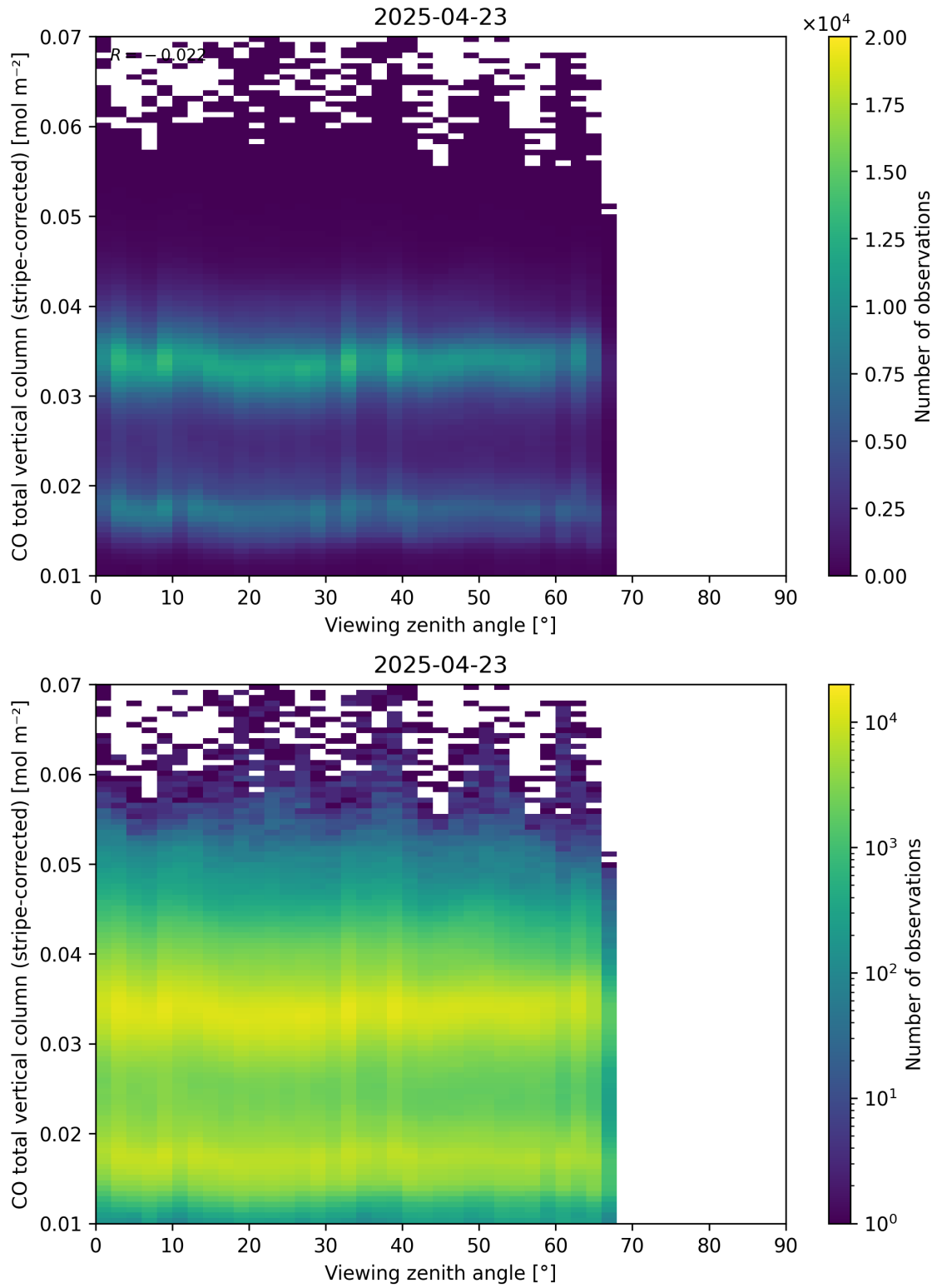
Figure 70: Scatter density plot of “Viewing zenith angle” against “CO total vertical column (stripe-corrected)” for 2025-04-22 to 2025-04-24.
