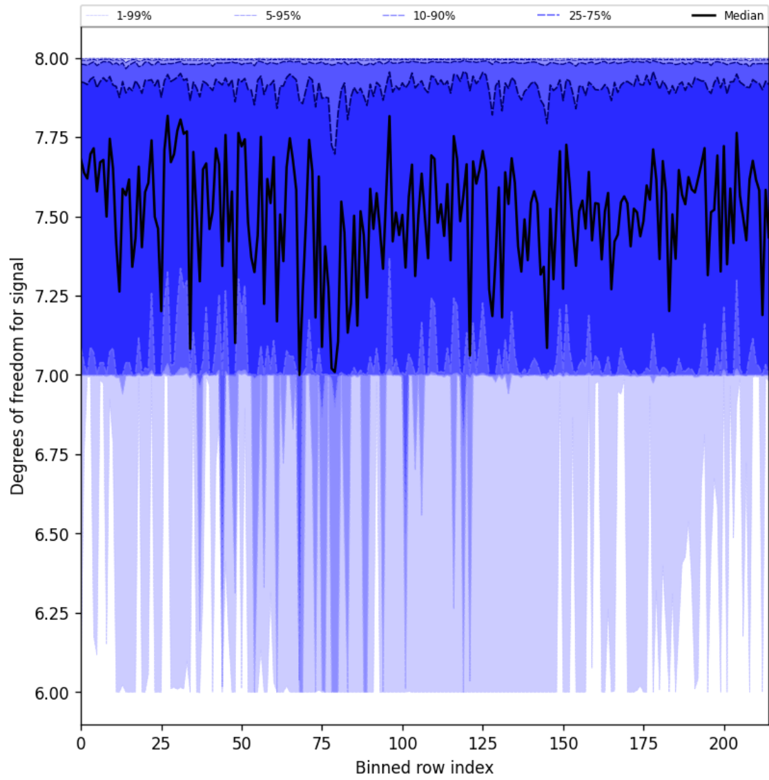
Figure 31: Along track statistics of “Degrees of freedom for signal” for 2025-04-22 to 2025-04-24
