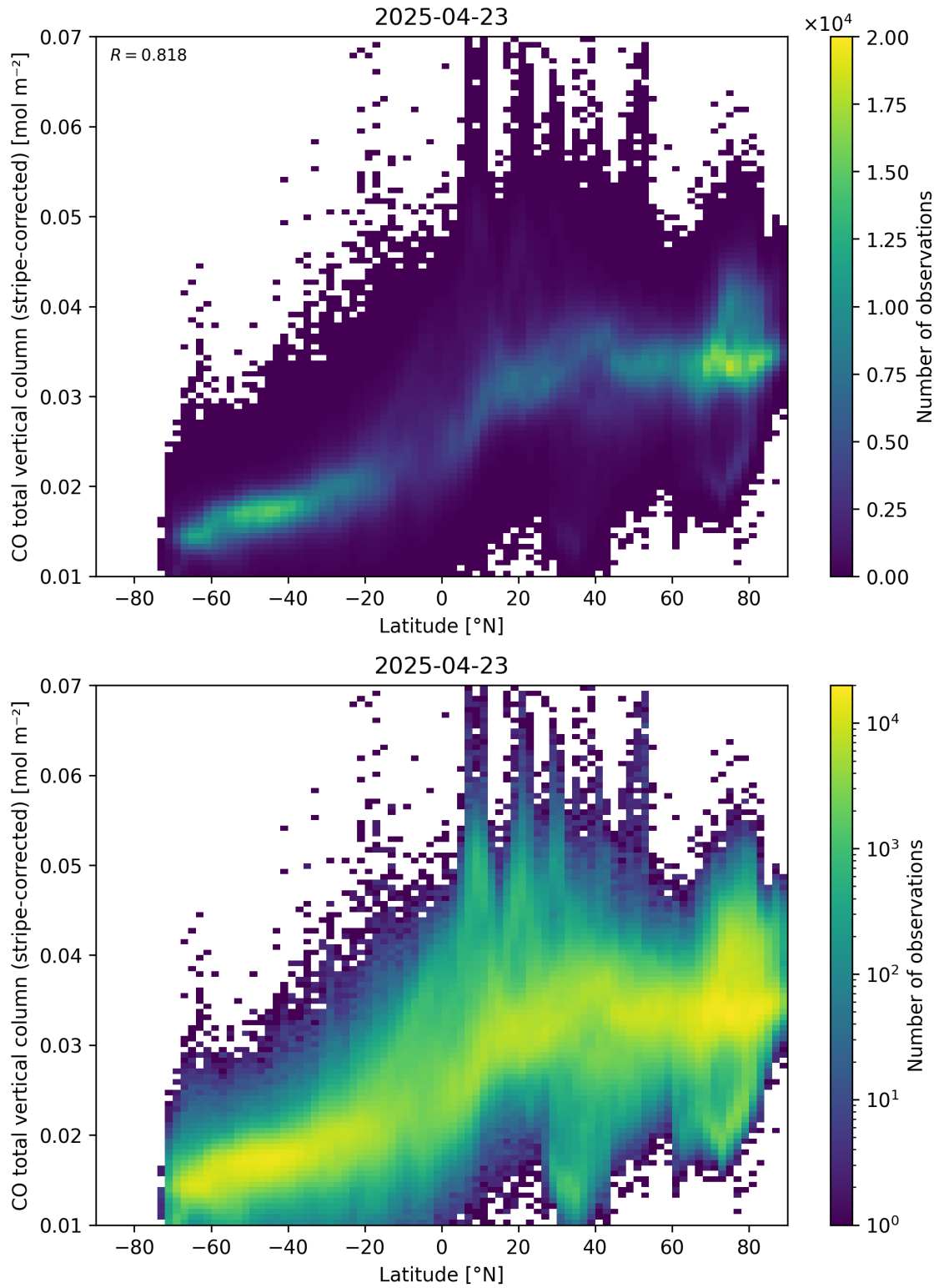
Figure 52: Scatter density plot of “Latitude” against “CO total vertical column (stripe-corrected)” for 2025-04-22 to 2025-04-24.
