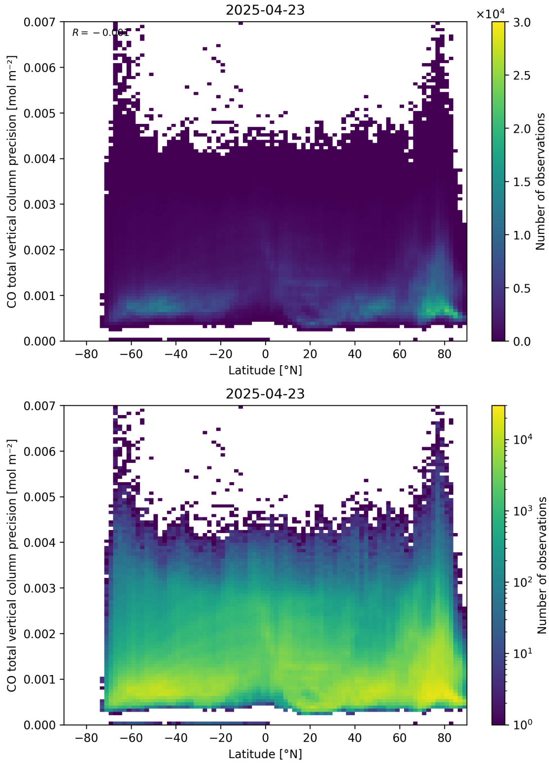
Figure 53: Scatter density plot of “Latitude” against “CO total vertical column precision” for 2025-04-22 to 2025-04-24.
