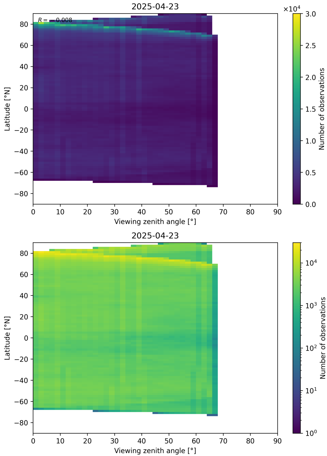
Figure 74: Scatter density plot of “Viewing zenith angle” against “Latitude” for 2025-04-22 to 2025-04-24.
