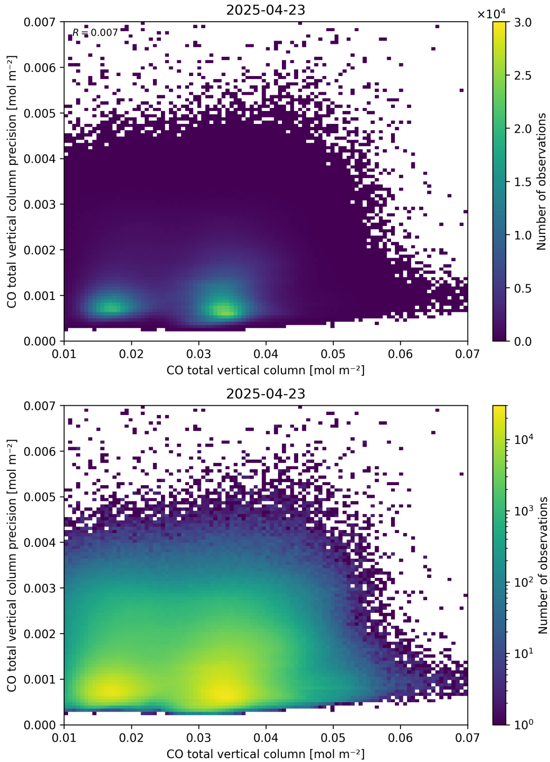
Figure 34: Scatter density plot of “CO total vertical column” against “CO total vertical column precision” for 2025-04-22 to 2025-04-24.
