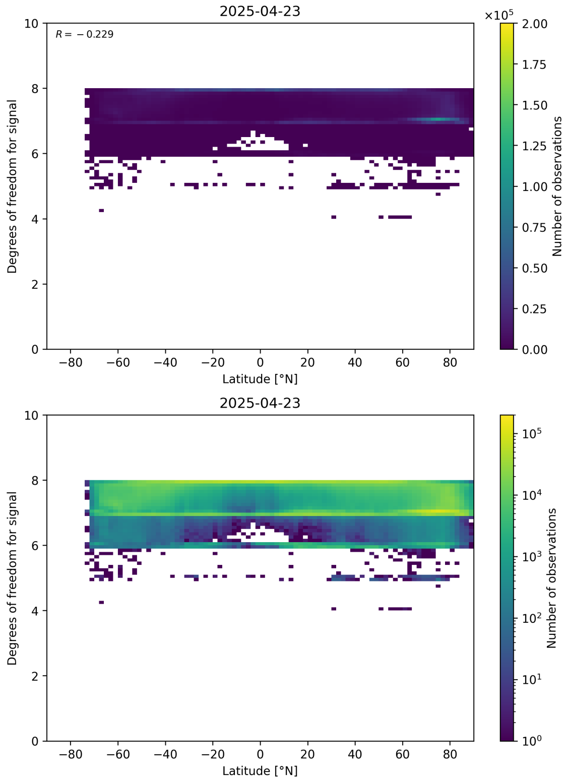
Figure 55: Scatter density plot of “Latitude” against “Degrees of freedom for signal” for 2025-04-22 to 2025-04-24.
