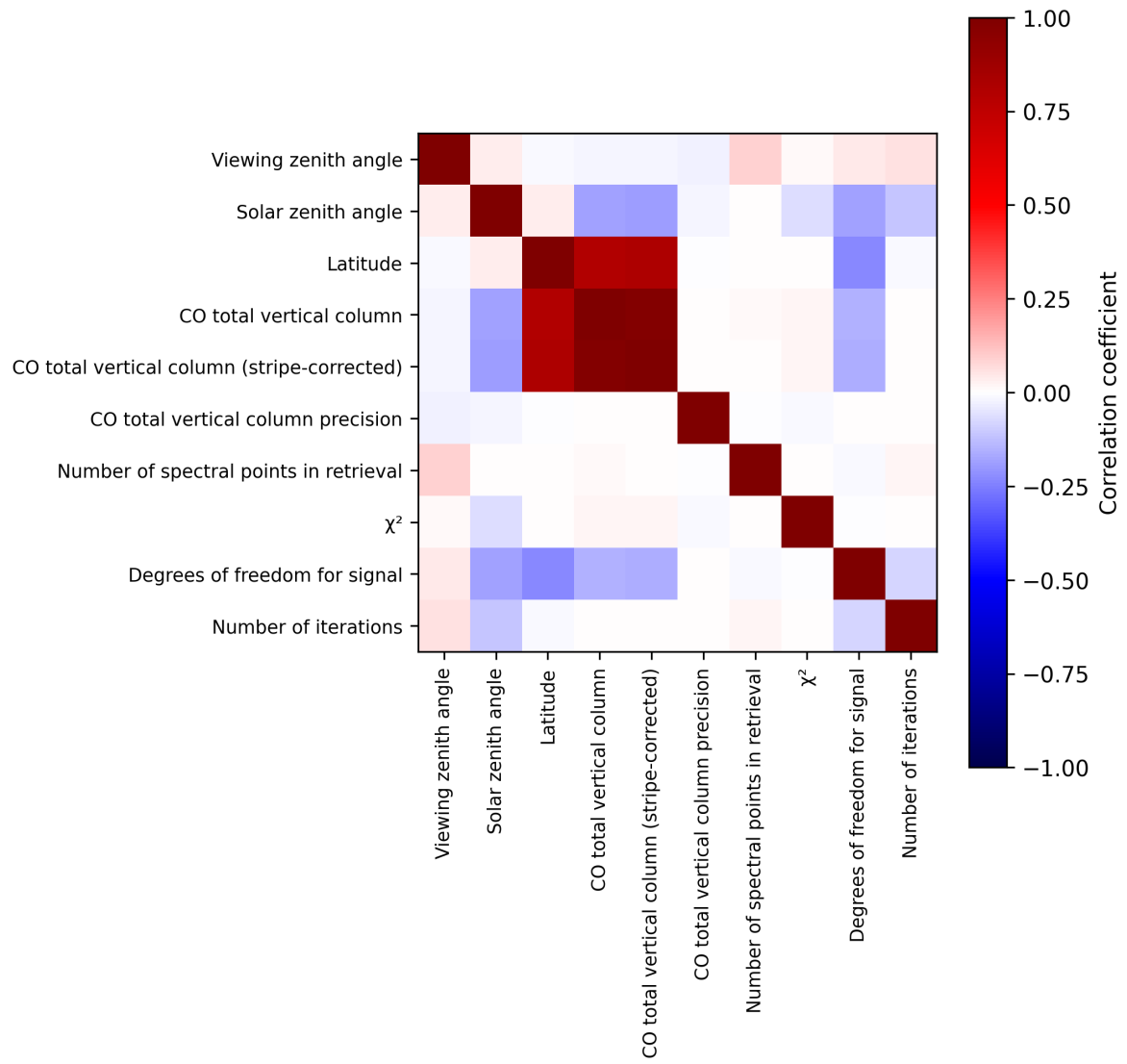
Figure 2: Map of correlation matrix for 2025-04-22 to 2025-04-24.
