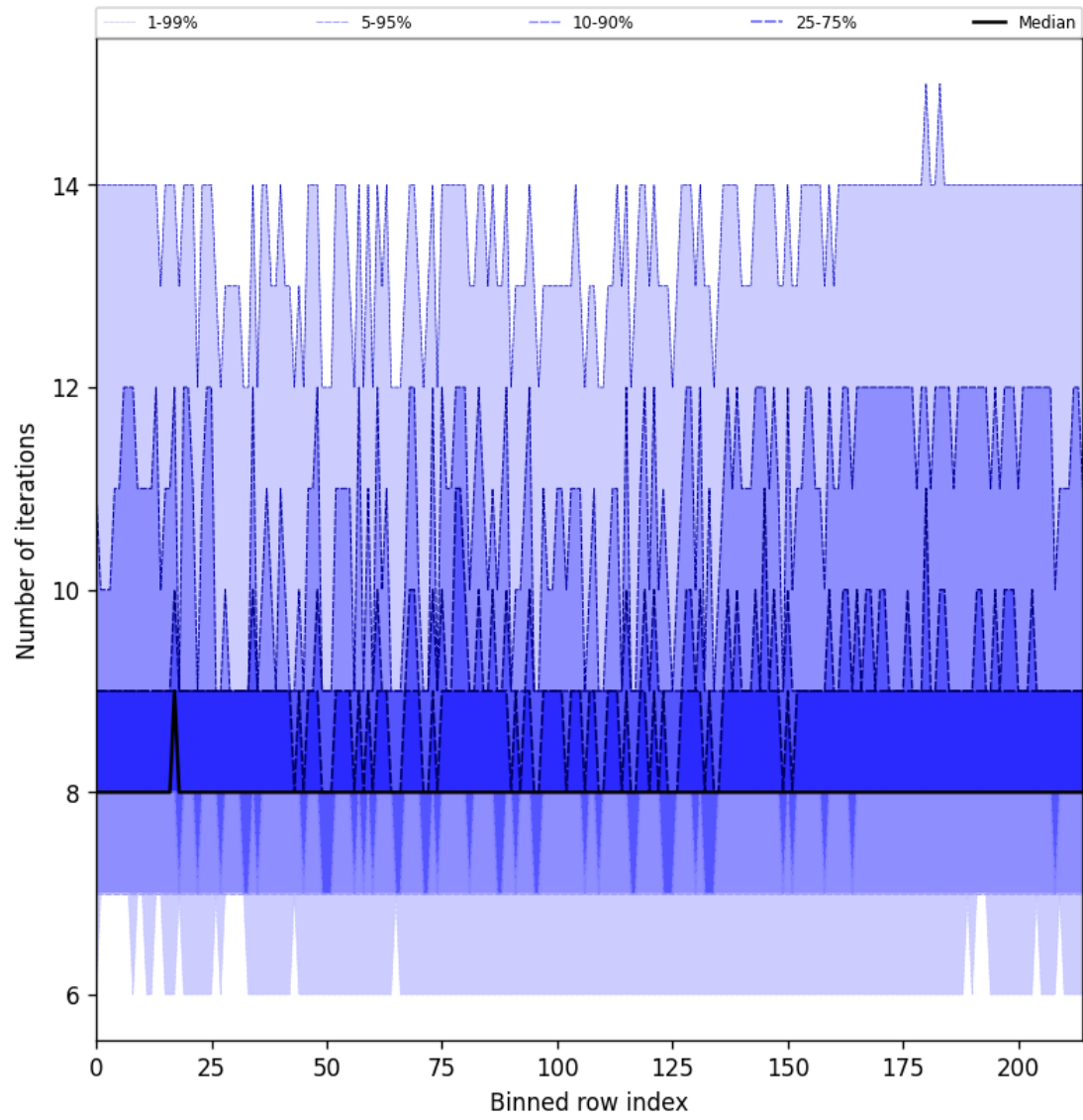
Figure 32: Along track statistics of “Number of iterations” for 2025-04-22 to 2025-04-24
