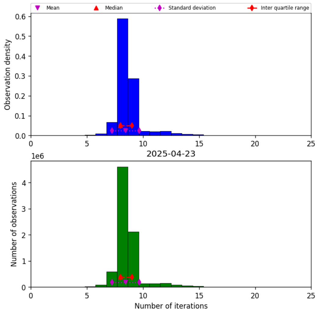
Figure 24: Histogram of “Number of iterations” for 2025-04-22 to 2025-04-24
