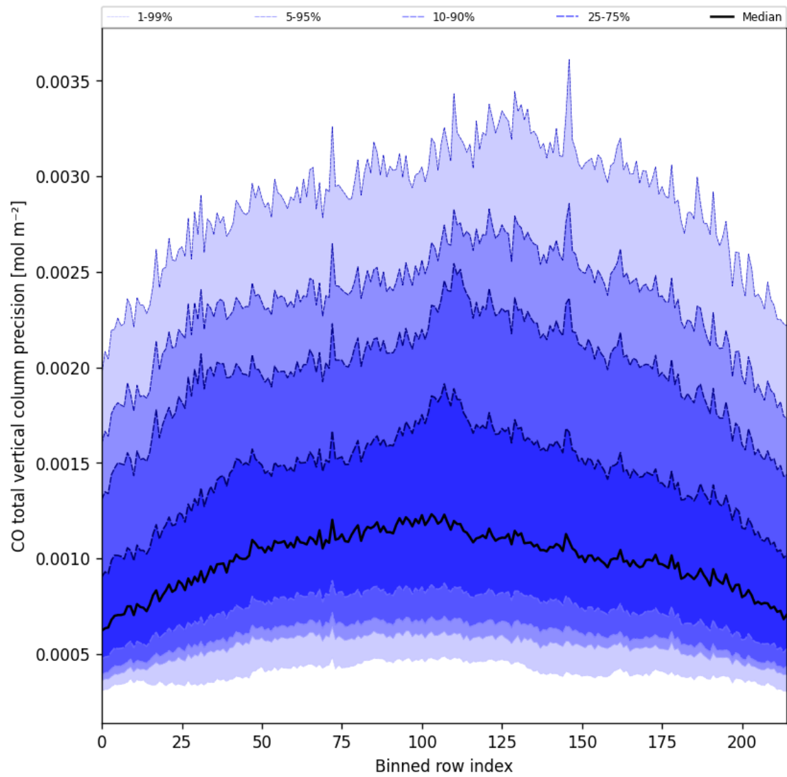
Figure 28: Along track statistics of “CO total vertical column precision” for 2025-04-22 to 2025-04-24
