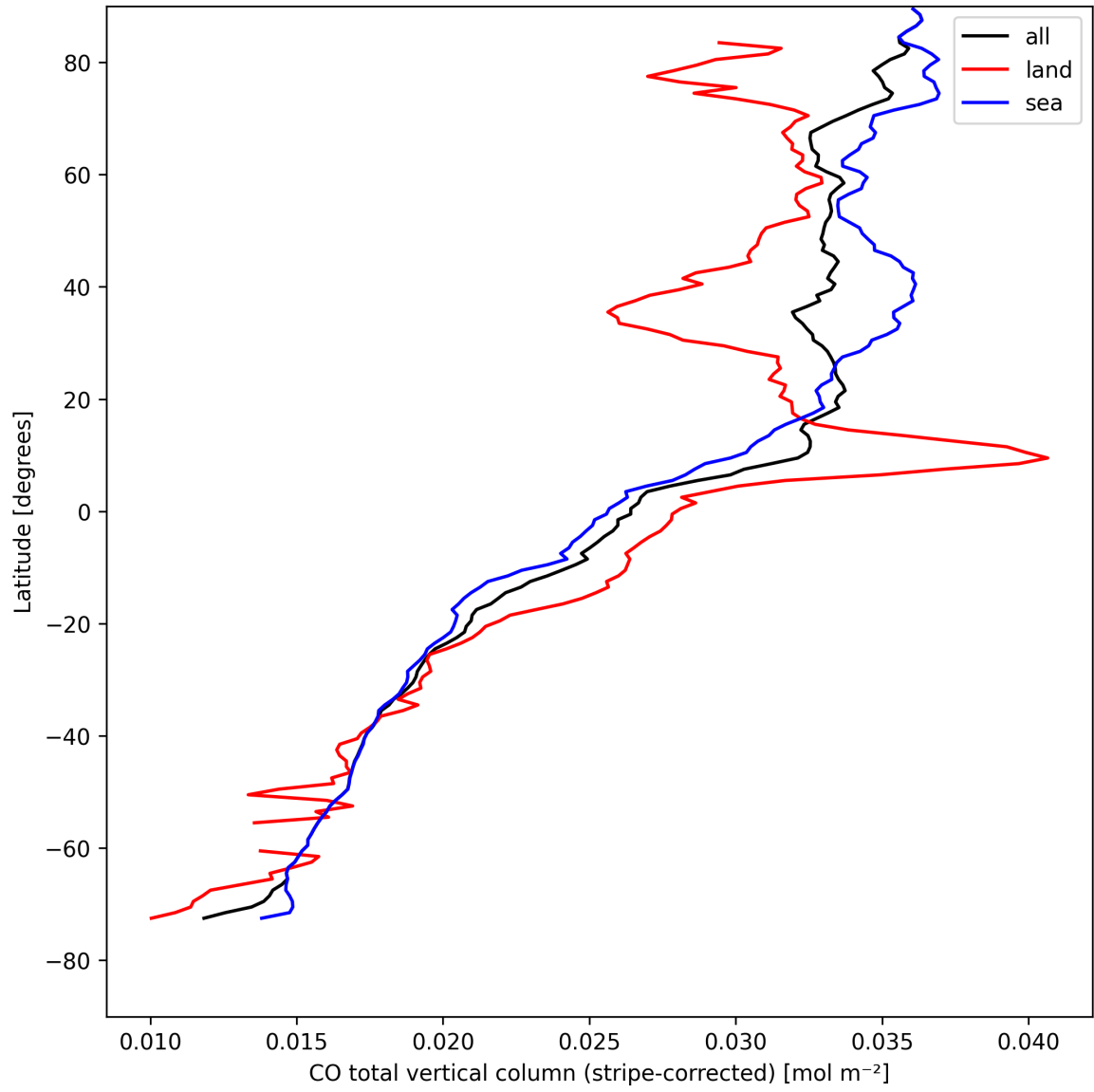
Figure 11: Zonal average of “CO total vertical column (stripe-corrected)” for 2025-04-22 to 2025-04-24.
