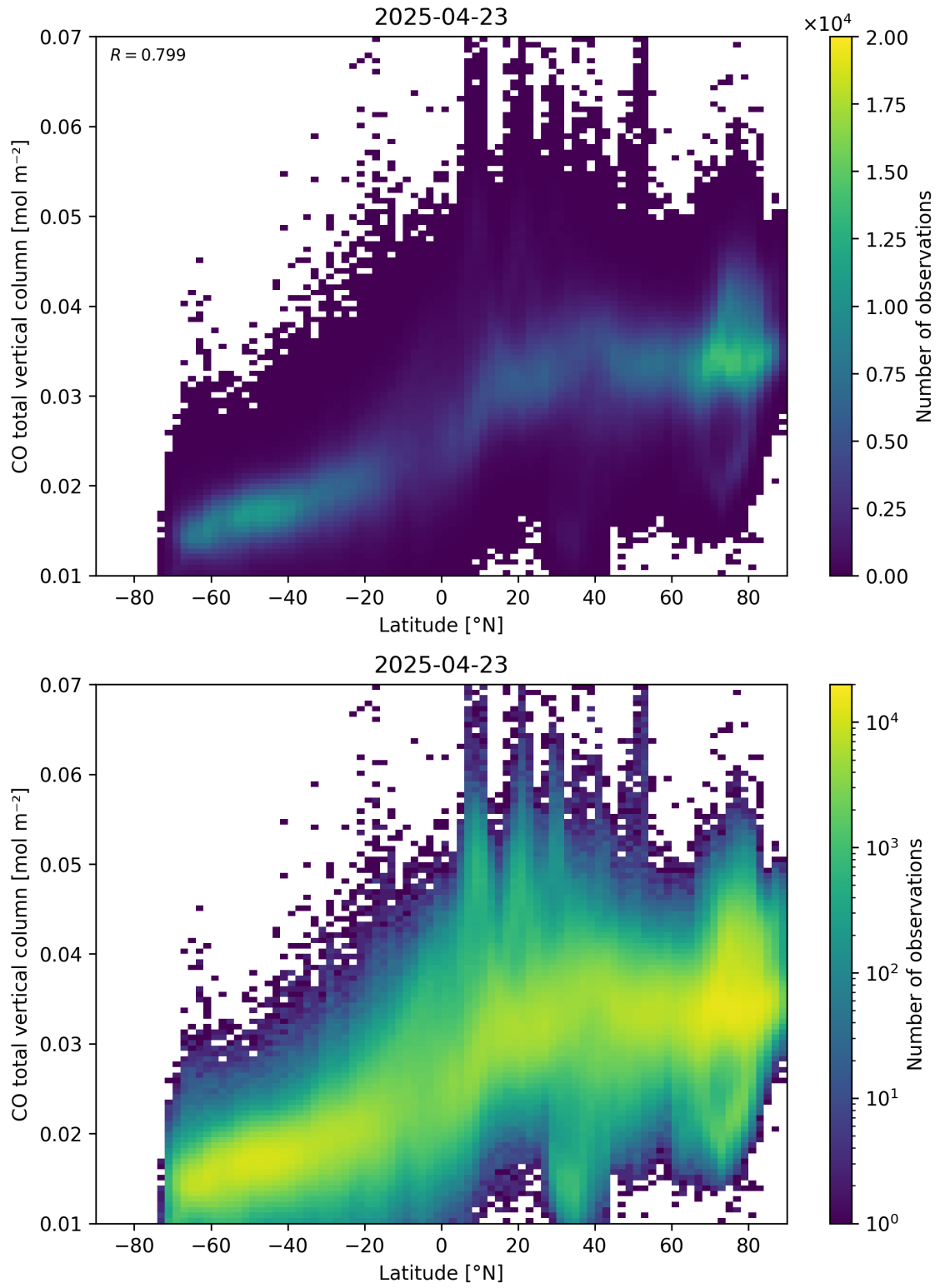
Figure 51: Scatter density plot of “Latitude” against “CO total vertical column” for 2025-04-22 to 2025-04-24.
