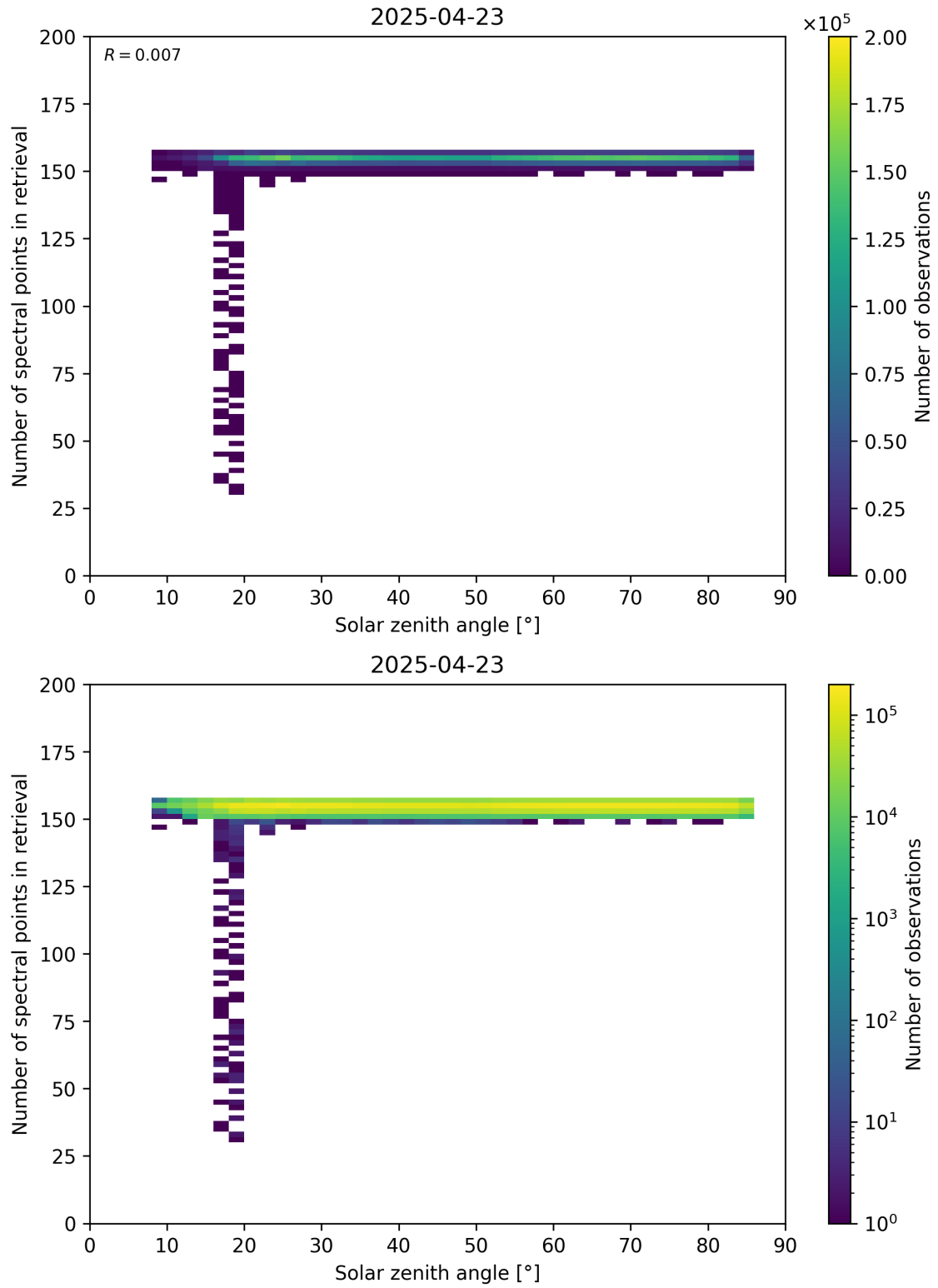
Figure 68: Scatter density plot of “Solar zenith angle” against “Number of spectral points in retrieval” for 2025-04-22 to 2025-04-24.
