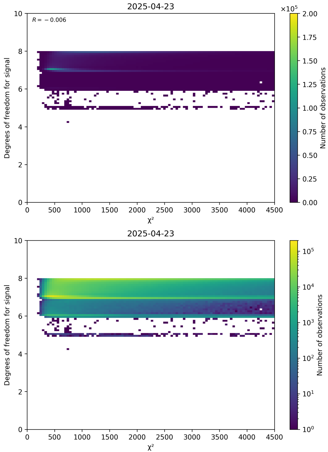
Figure 48: Scatter density plot of “ \chi^2 ” against “Degrees of freedom for signal” for 2025-04-22 to 2025-04-24.
