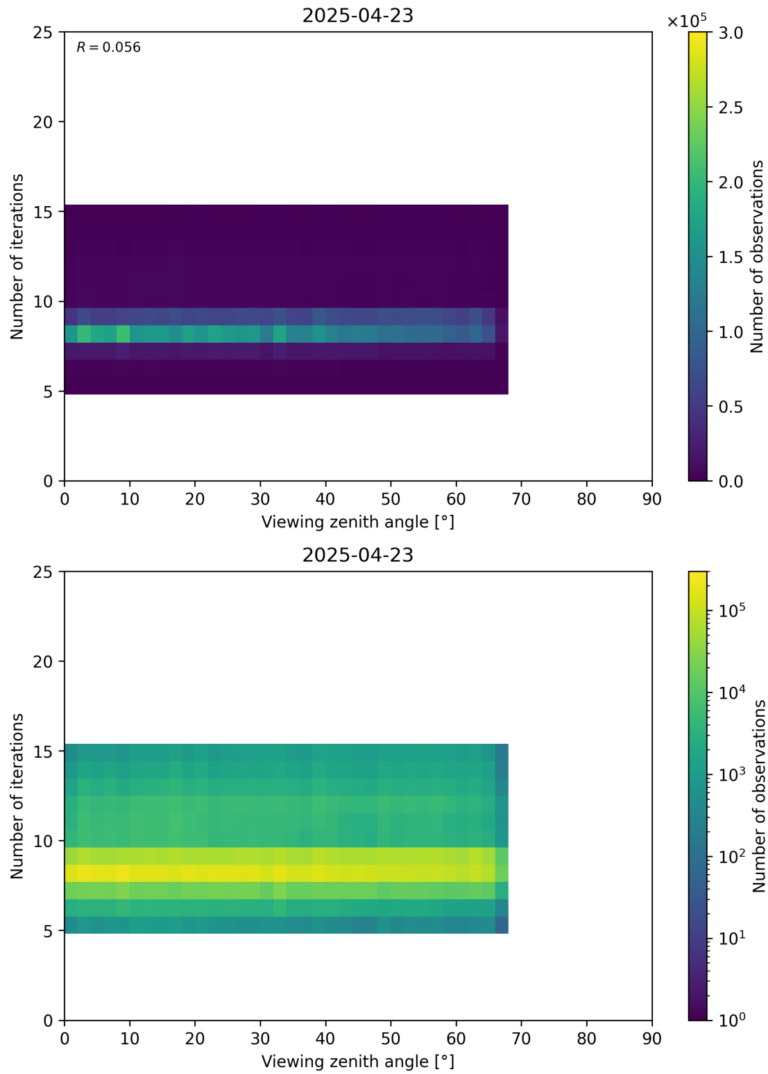
Figure 75: Scatter density plot of “Viewing zenith angle” against “Number of iterations” for 2025-04-22 to 2025-04-24.
