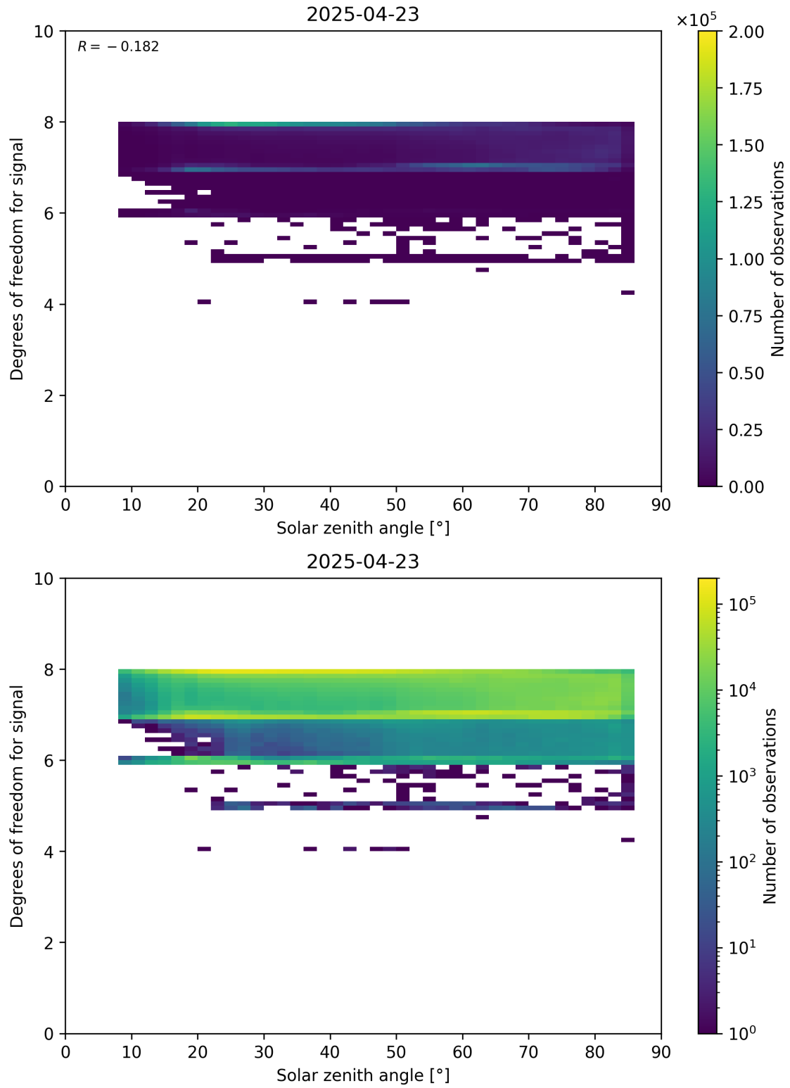
Figure 65: Scatter density plot of “Solar zenith angle” against “Degrees of freedom for signal” for 2025-04-22 to 2025-04-24.
