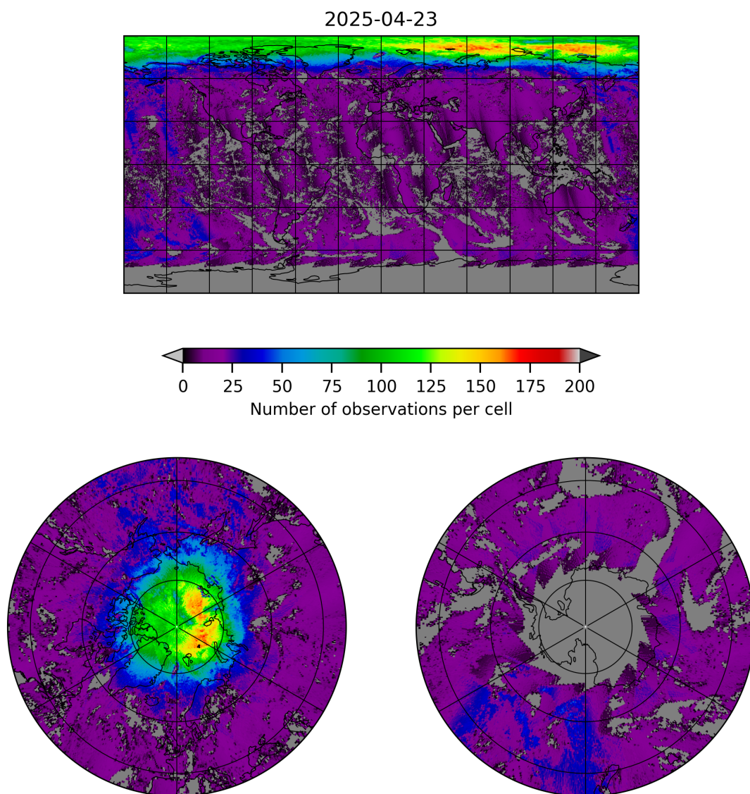
Figure 8: Map of the number of observations for 2025-04-22 to 2025-04-24
