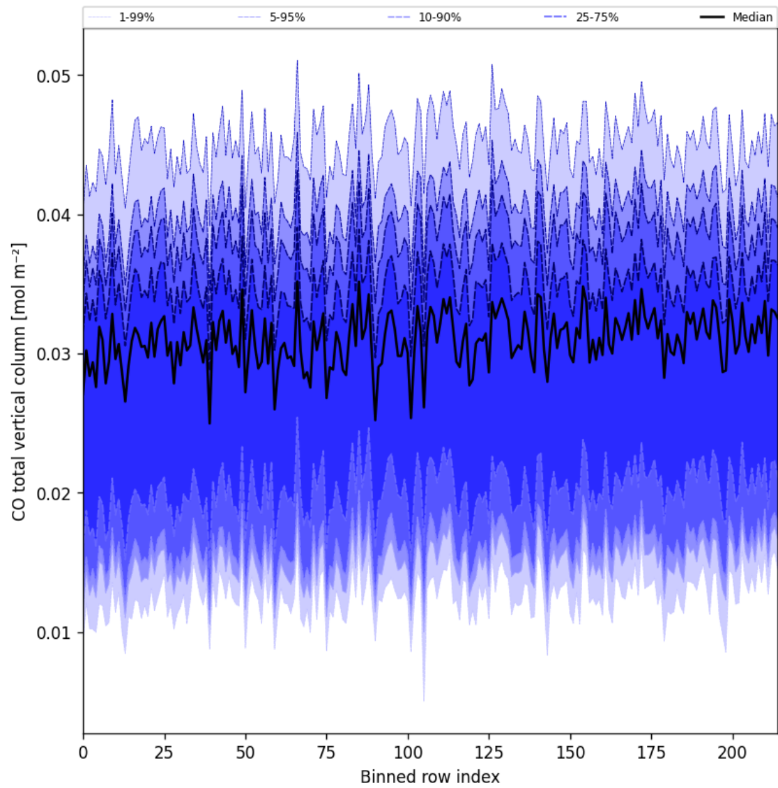
Figure 26: Along track statistics of “CO total vertical column” for 2025-04-22 to 2025-04-24
