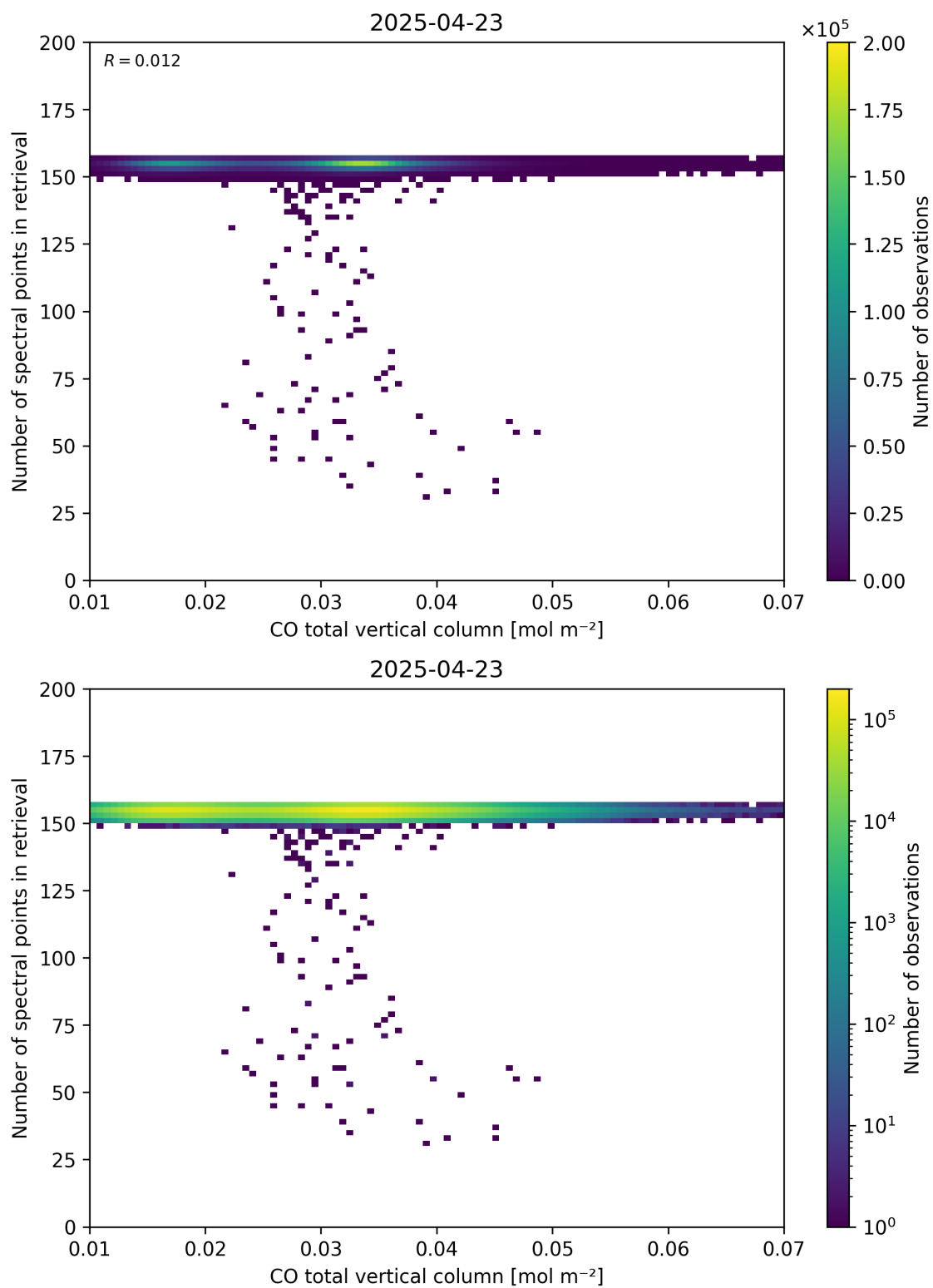
Figure 43: Scatter density plot of “CO total vertical column” against “Number of spectral points in retrieval” for 2025-04-22 to 2025-04-24.
