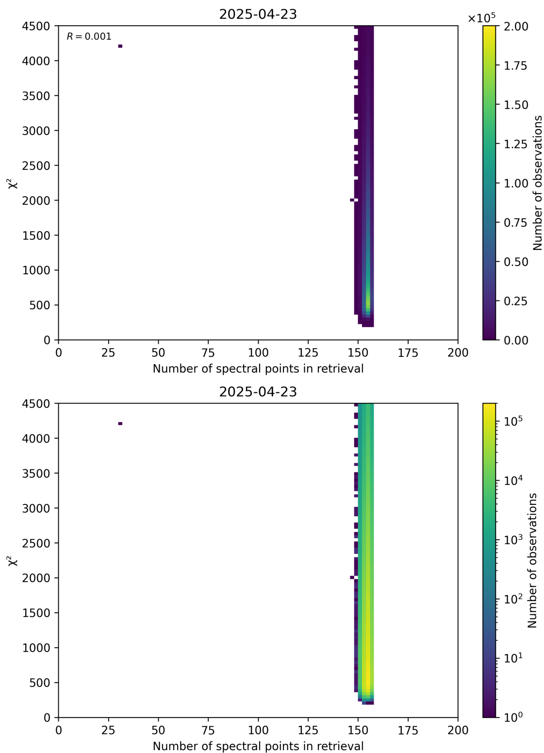
Figure 58: Scatter density plot of “Number of spectral points in retrieval” against “ \chi^2 ” for 2025-04-22 to 2025-04-24.
