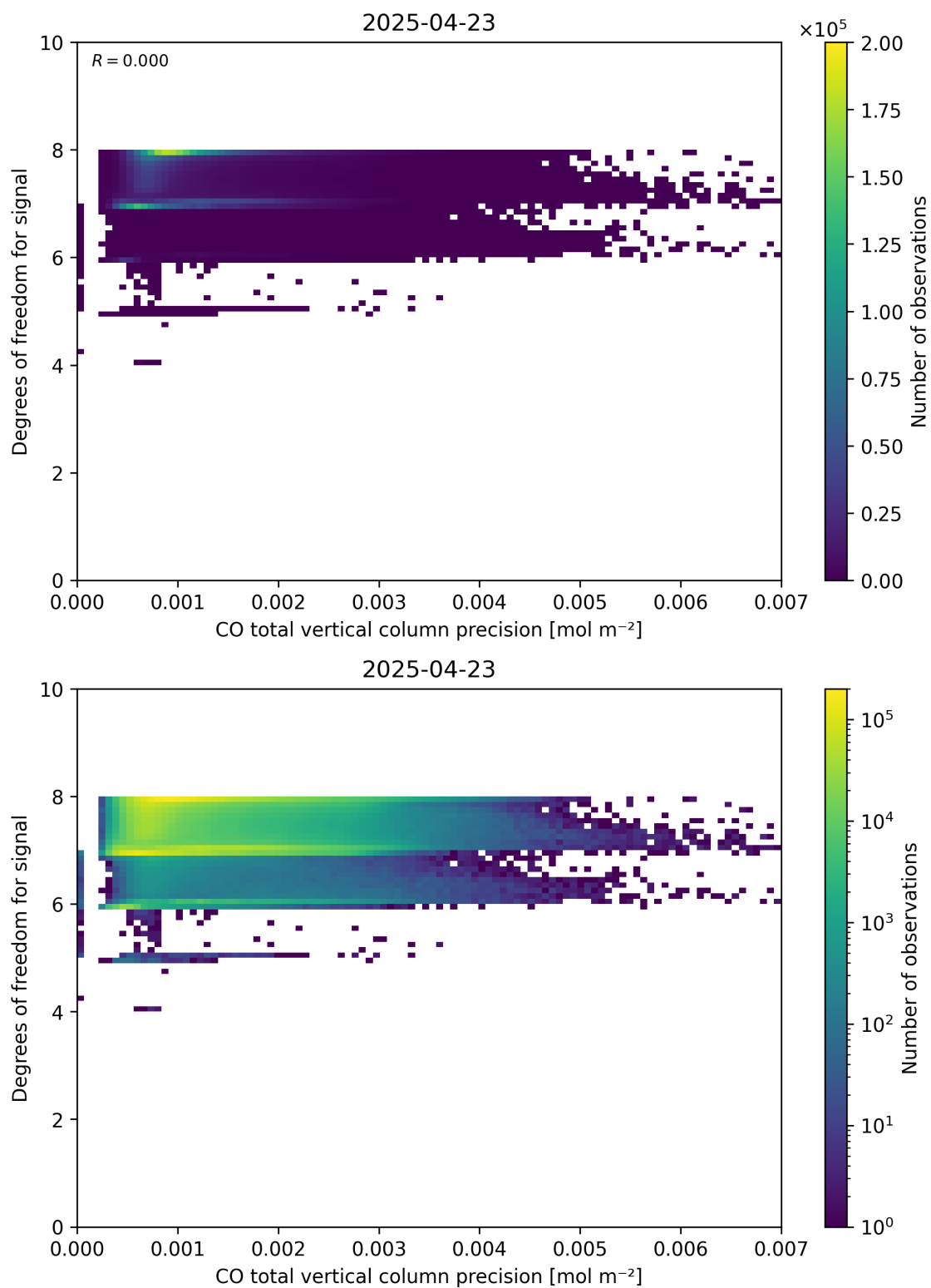
Figure 45: Scatter density plot of “CO total vertical column precision” against “Degrees of freedom for signal” for 2025-04-22 to 2025-04-24.
