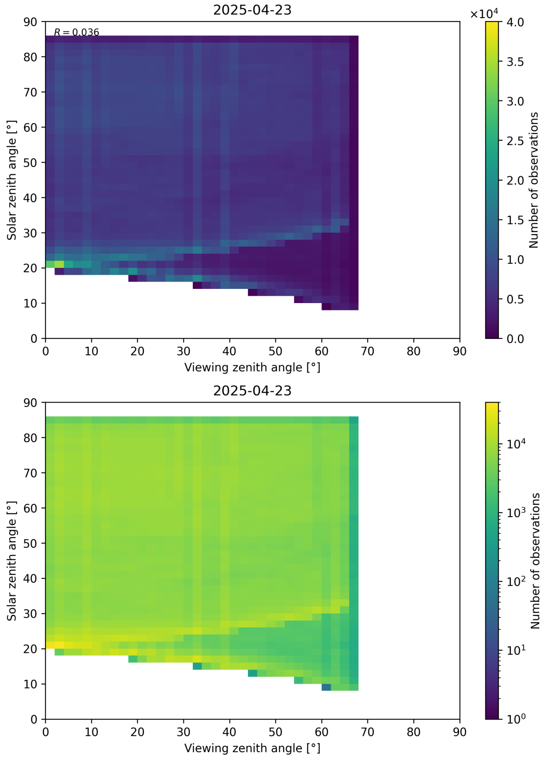
Figure 77: Scatter density plot of “Viewing zenith angle” against “Solar zenith angle” for 2025-04-22 to 2025-04-24.
