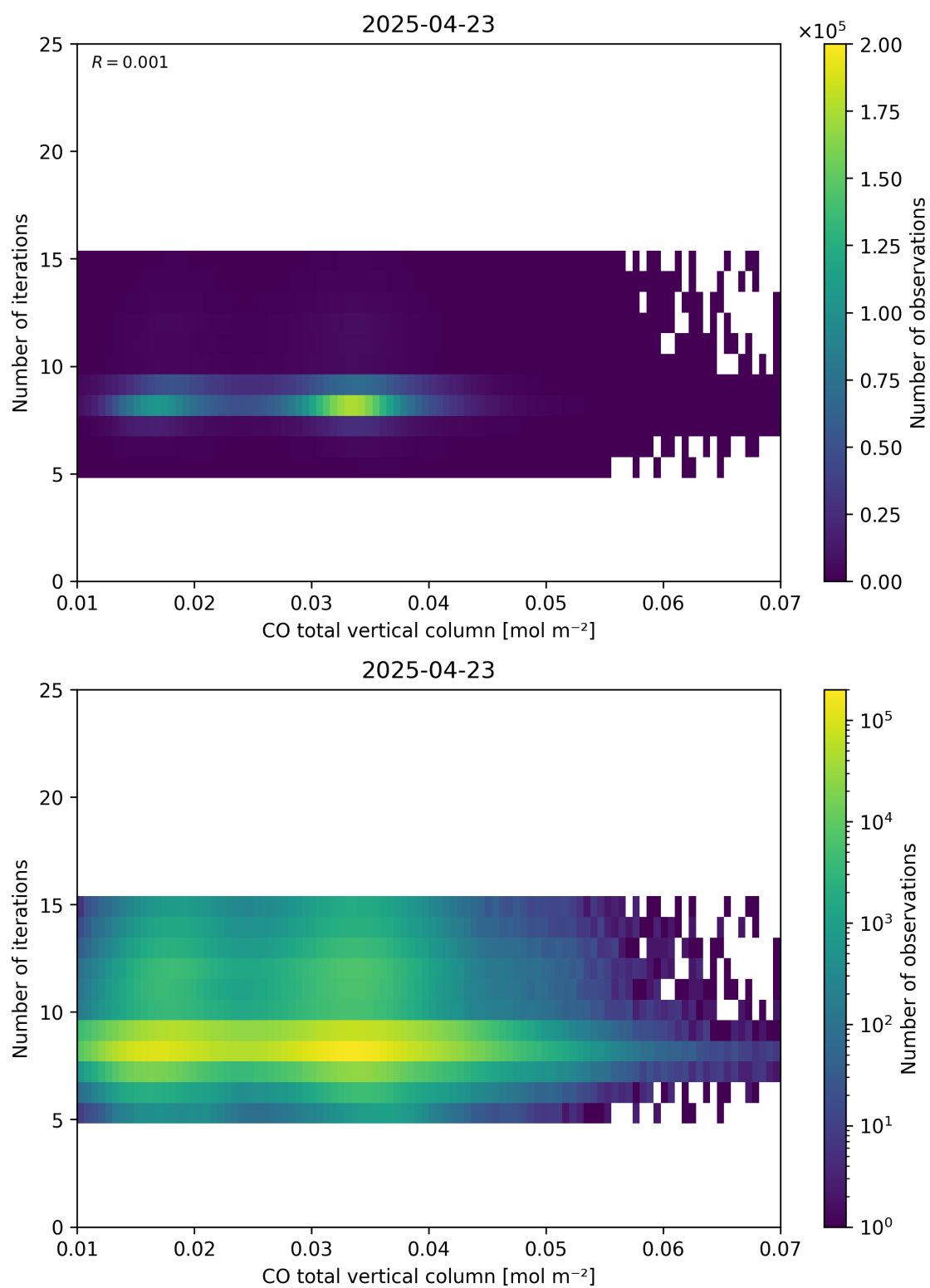
Figure 42: Scatter density plot of “CO total vertical column” against “Number of iterations” for 2025-04-22 to 2025-04-24.
