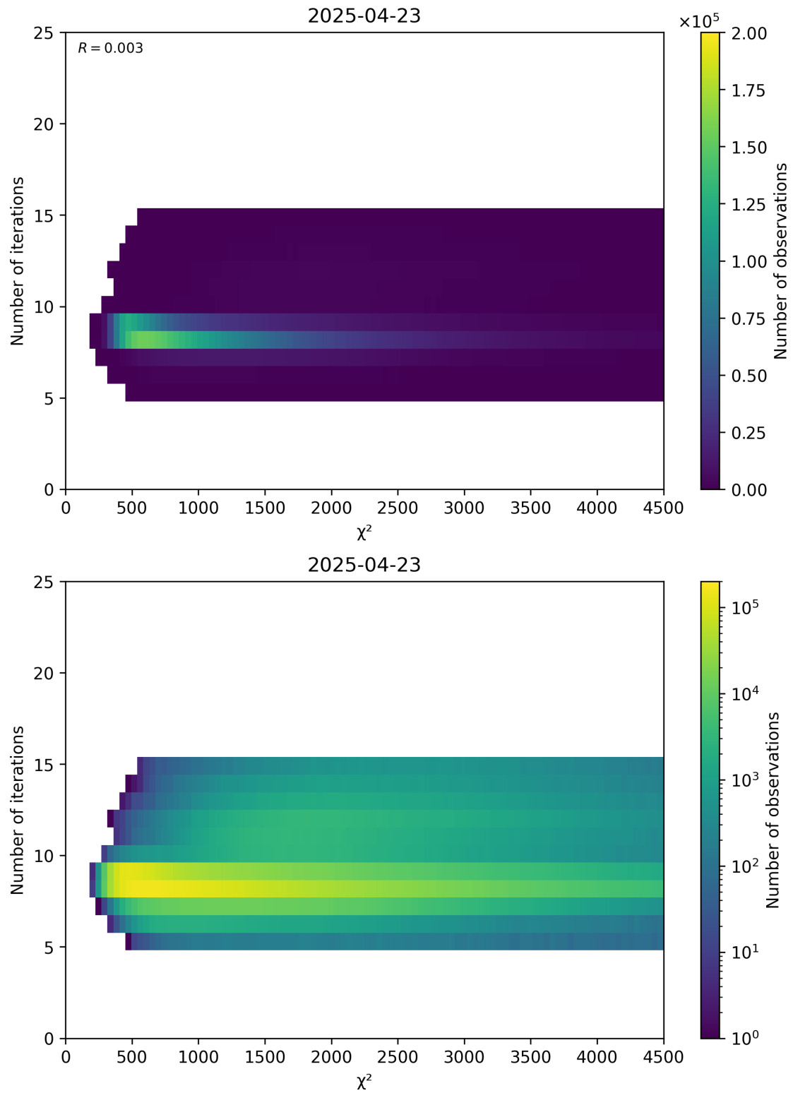
Figure 49: Scatter density plot of “ \chi^2 ” against “Number of iterations” for 2025-04-22 to 2025-04-24.
