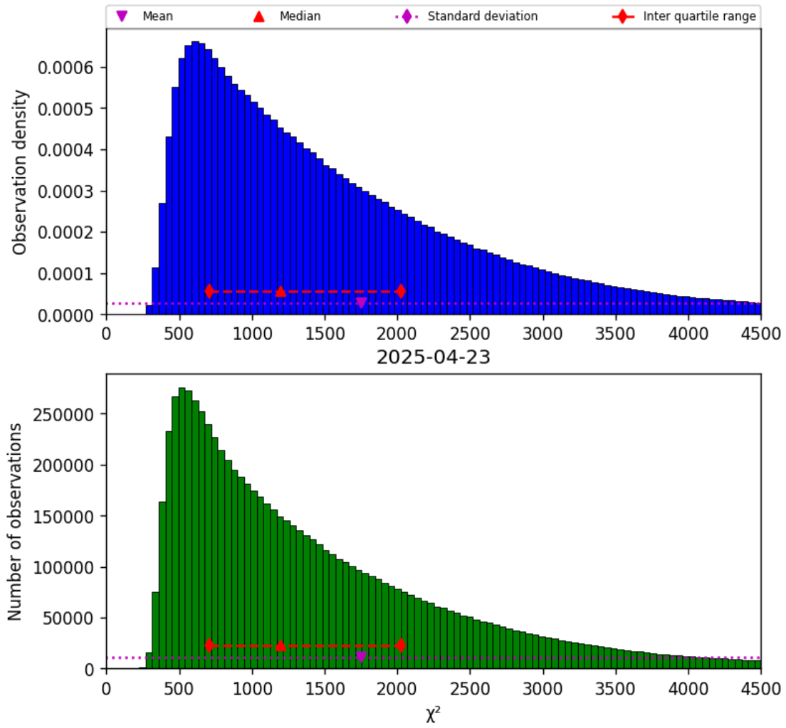
Figure 22: Histogram of “ \chi^2 ” for 2025-04-22 to 2025-04-24
