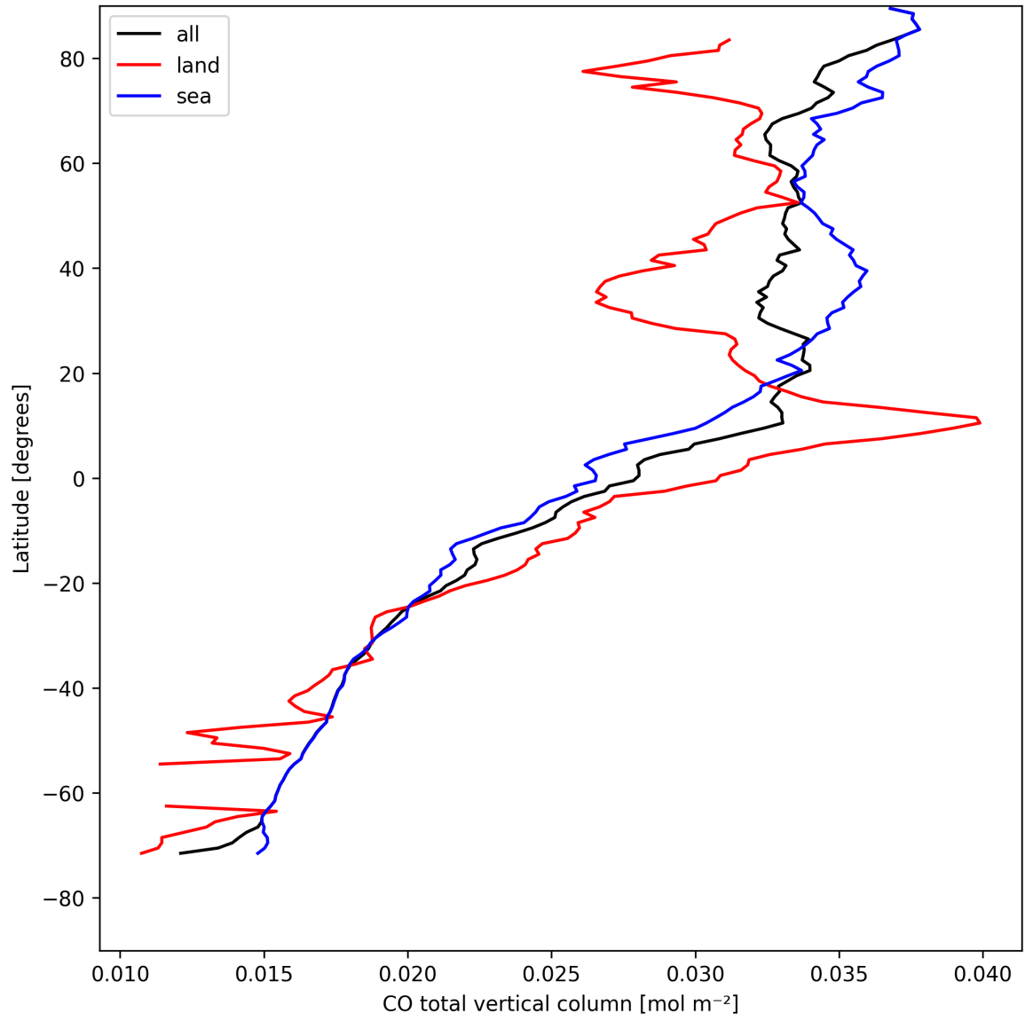
Figure 10: Zonal average of “CO total vertical column” for 2025-04-24 to 2025-04-25.
