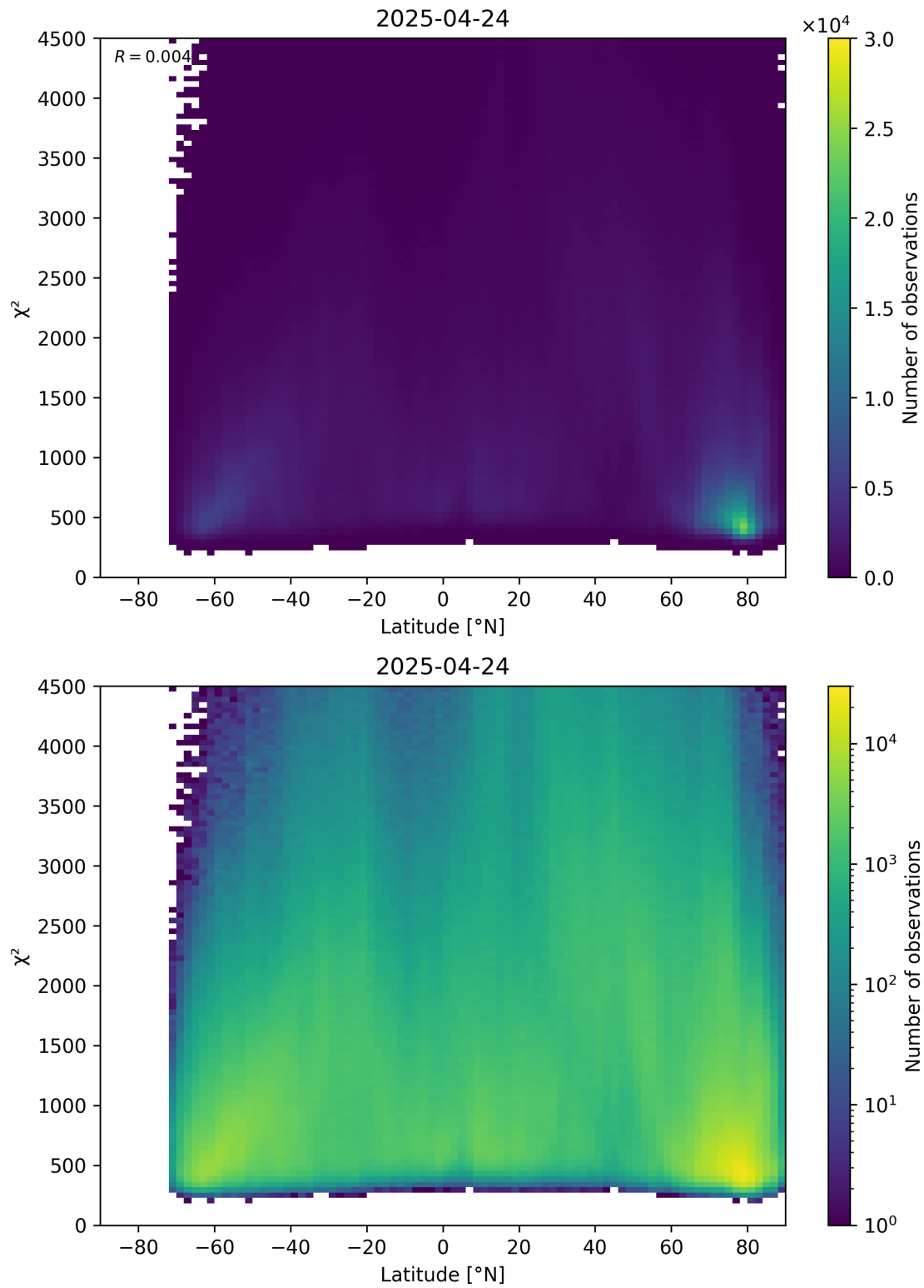
Figure 54: Scatter density plot of “Latitude” against “ \chi^2 ” for 2025-04-24 to 2025-04-25.
