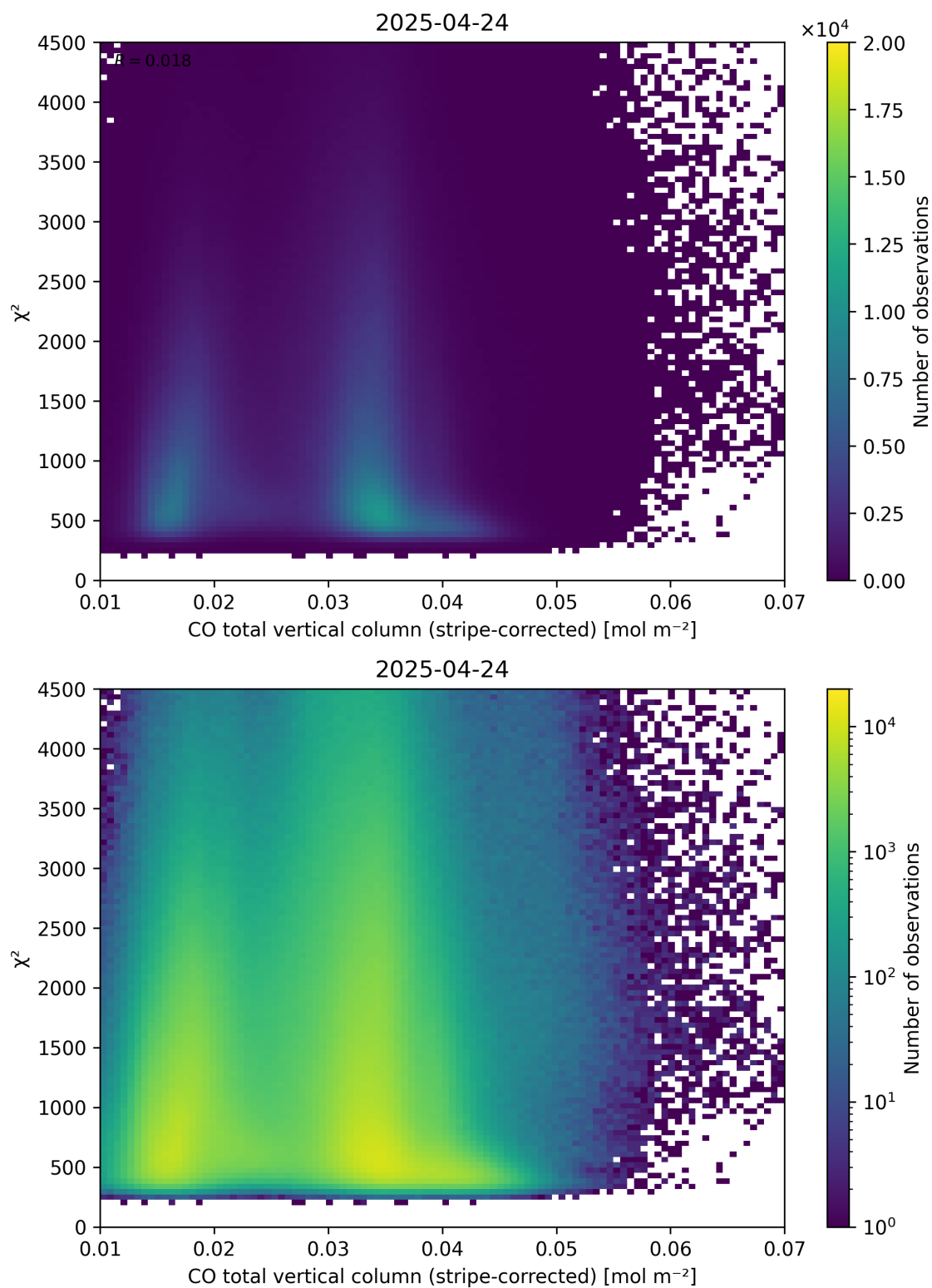
Figure 37: Scatter density plot of “CO total vertical column (stripe-corrected)” against “ \chi^2 ” for 2025-04-24 to 2025-04-25.
