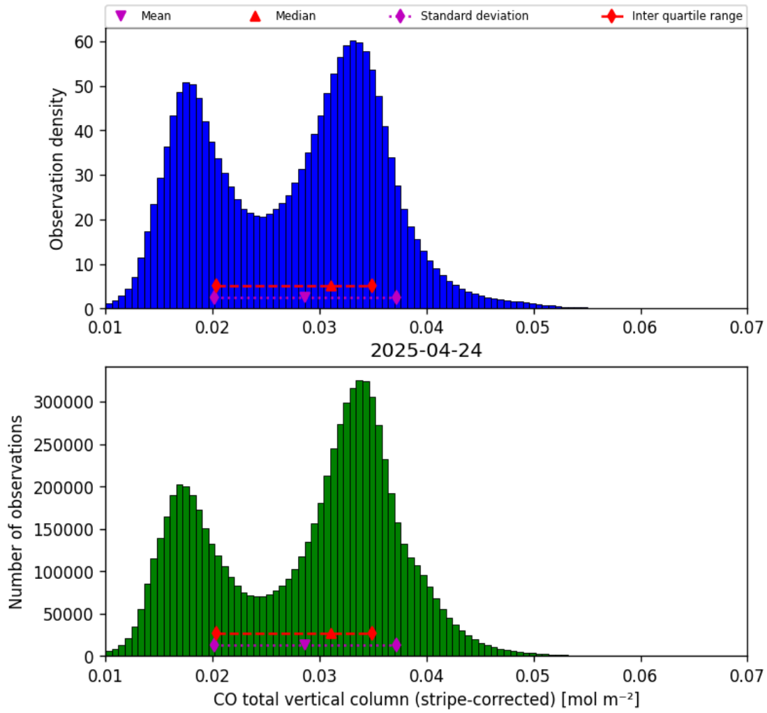
Figure 19: Histogram of “CO total vertical column (stripe-corrected)” for 2025-04-24 to 2025-04-25
