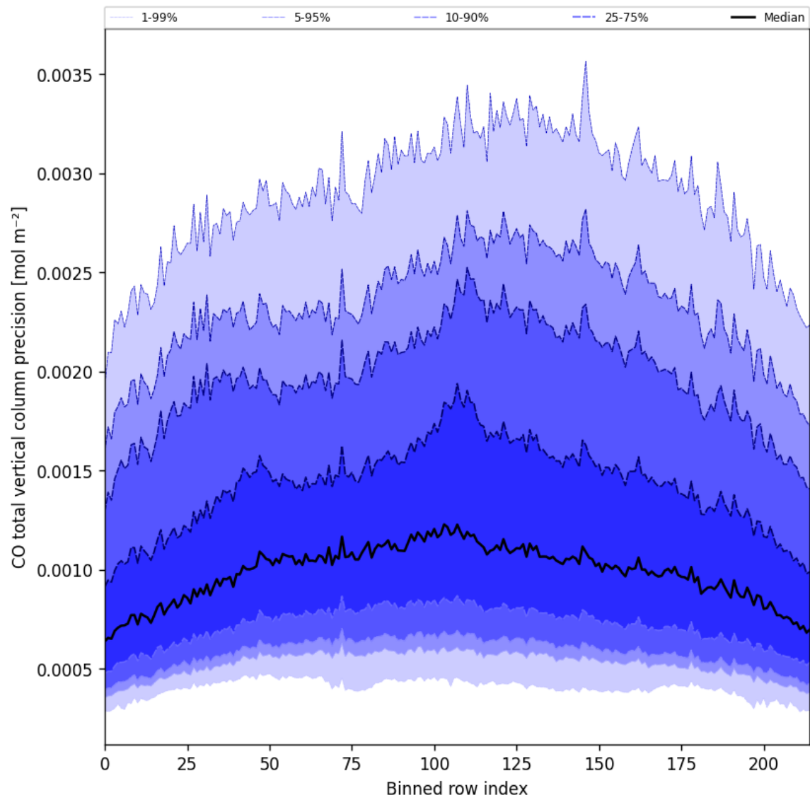
Figure 28: Along track statistics of “CO total vertical column precision” for 2025-04-24 to 2025-04-25
