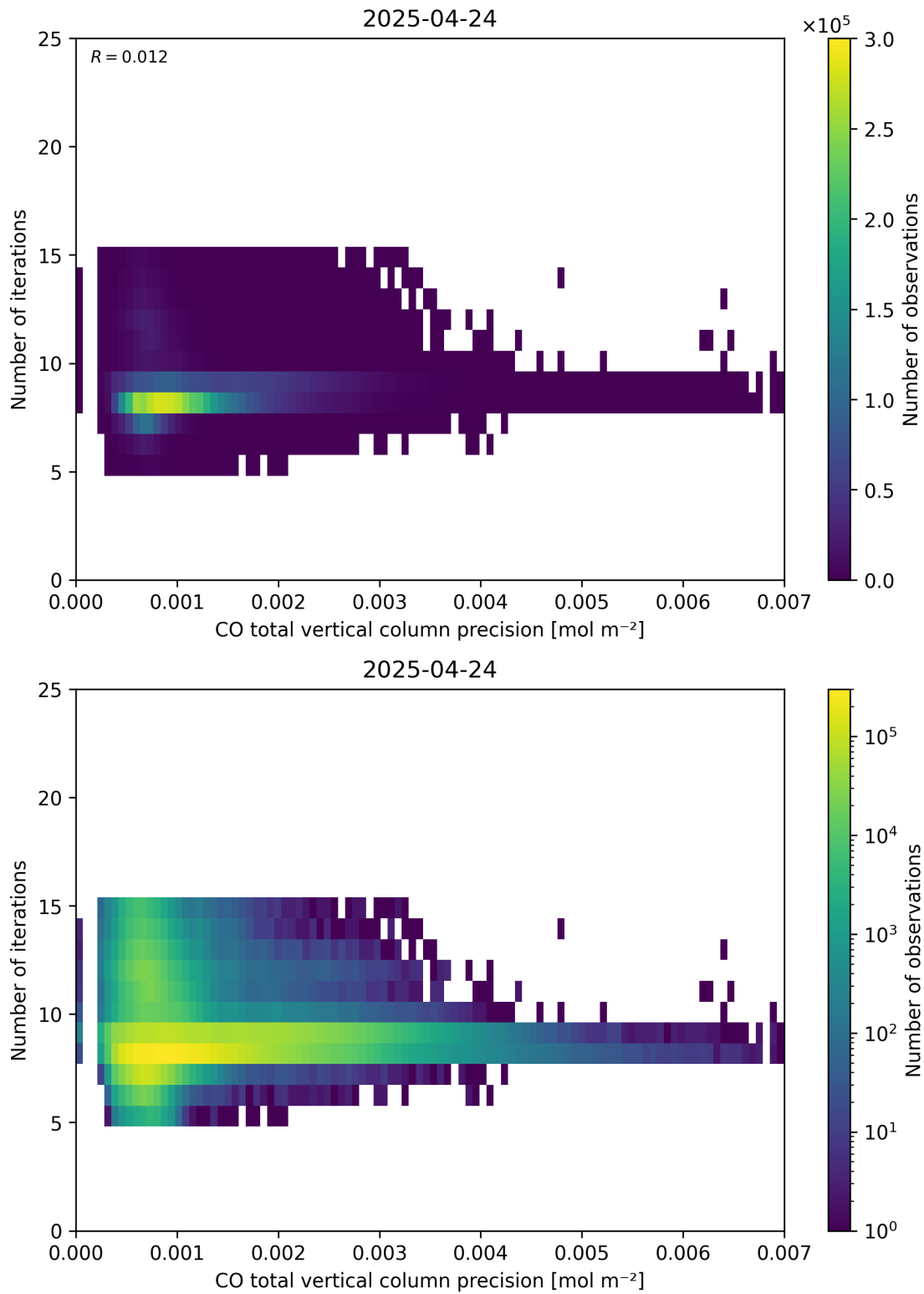
Figure 46: Scatter density plot of “CO total vertical column precision” against “Number of iterations” for 2025-04-24 to 2025-04-25.
