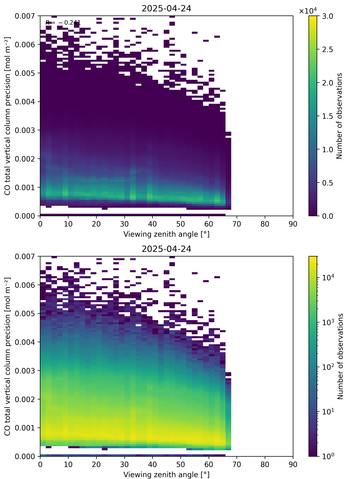
Figure 71: Scatter density plot of “Viewing zenith angle” against “CO total vertical column precision” for 2025-04-24 to 2025-04-25.
