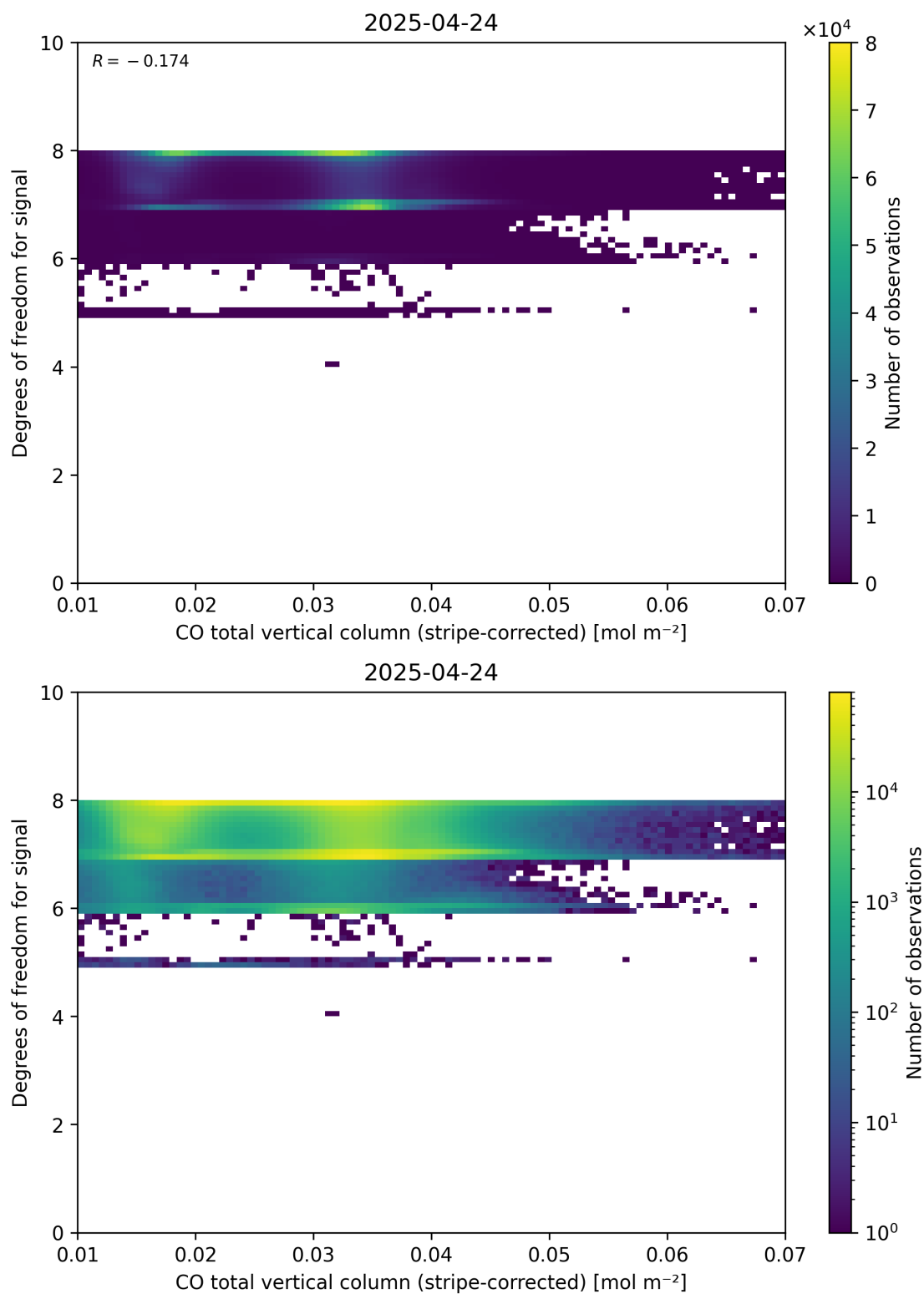
Figure 38: Scatter density plot of “CO total vertical column (stripe-corrected)” against “Degrees of freedom for signal” for 2025-04-24 to 2025-04-25.
