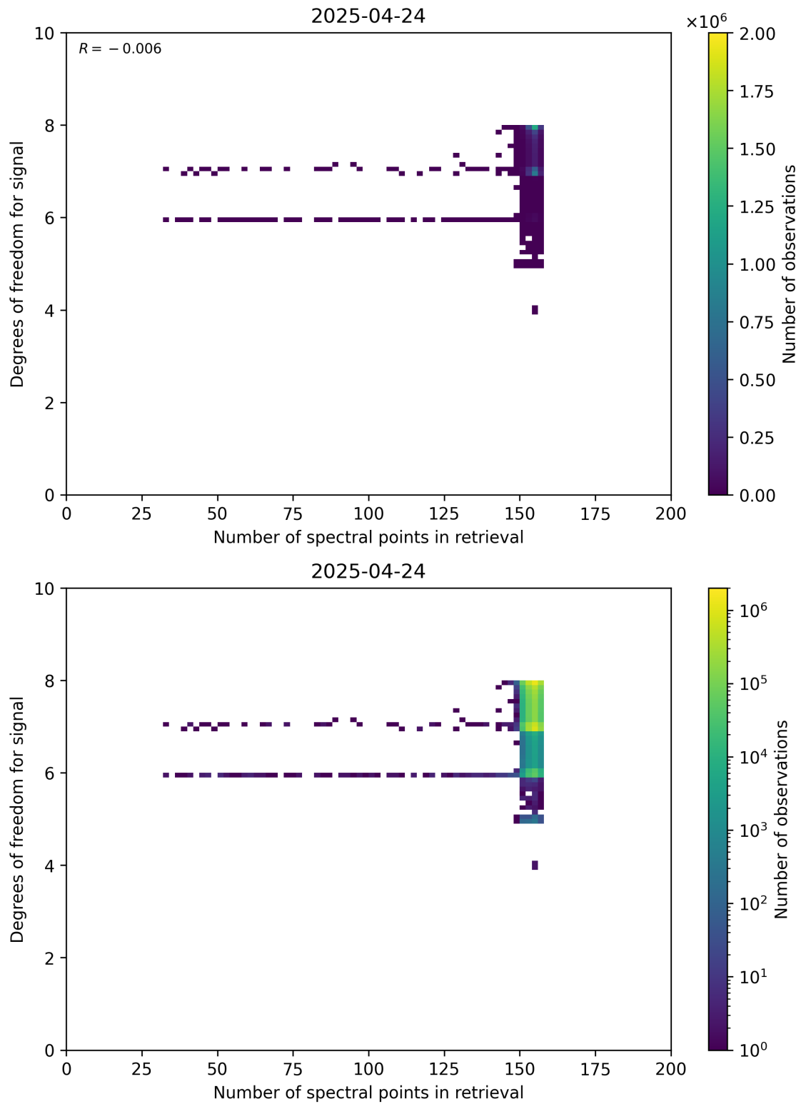
Figure 59: Scatter density plot of “Number of spectral points in retrieval” against “Degrees of freedom for signal” for 2025-04-24 to 2025-04-25.
