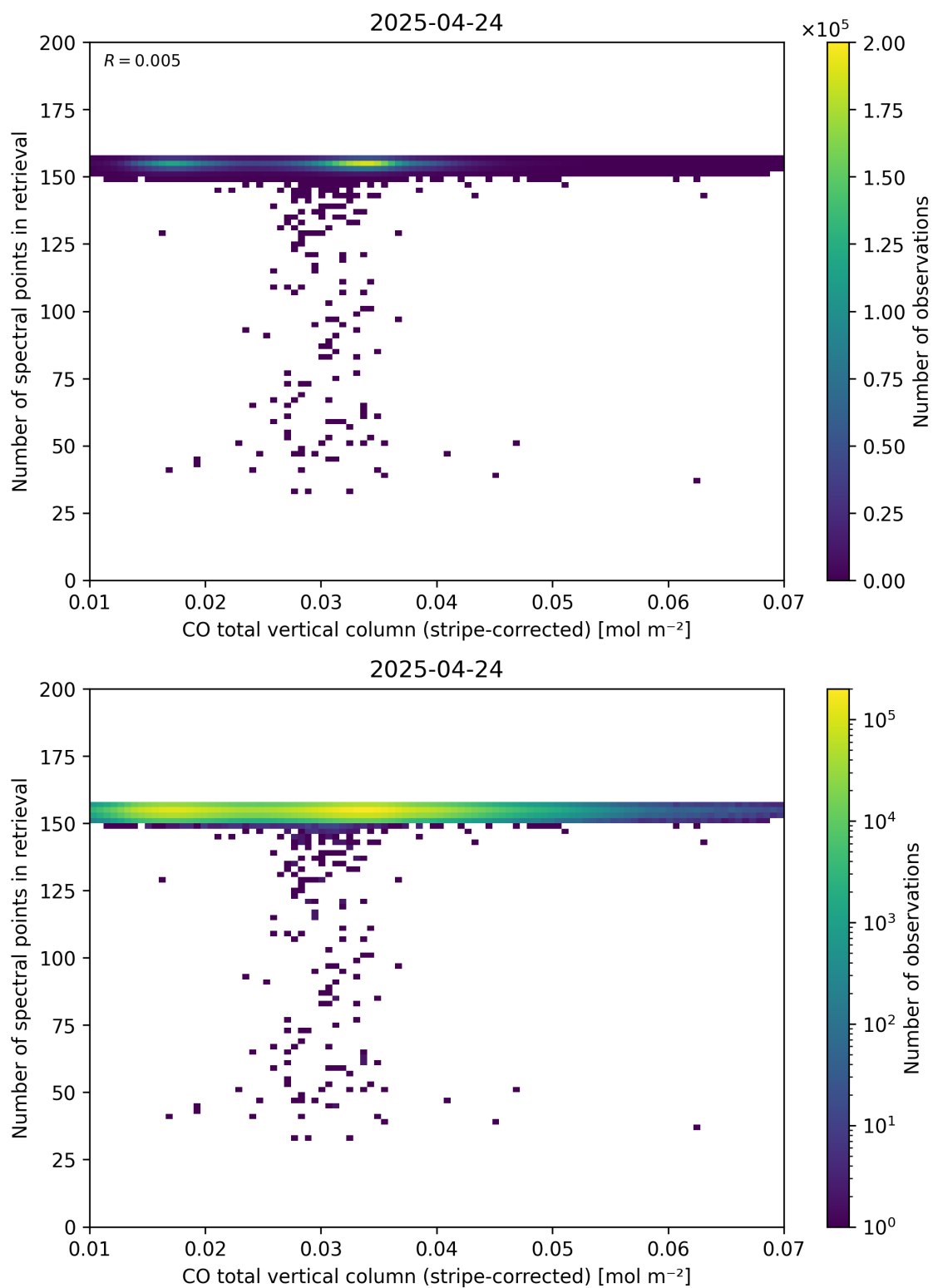
Figure 40: Scatter density plot of “CO total vertical column (stripe-corrected)” against “Number of spectral points in retrieval” for 2025-04-24 to 2025-04-25.
