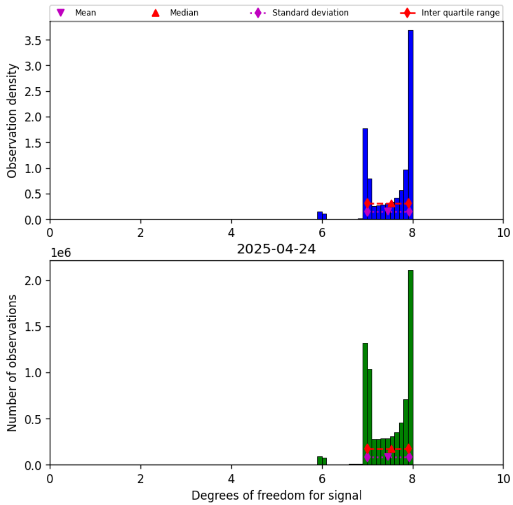
Figure 23: Histogram of “Degrees of freedom for signal” for 2025-04-24 to 2025-04-25
