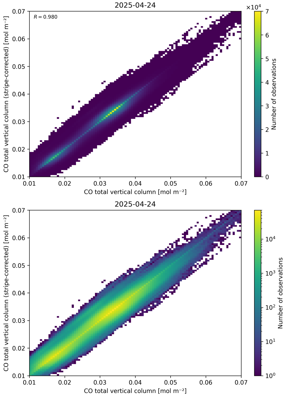
Figure 33: Scatter density plot of “CO total vertical column” against “CO total vertical column (stripe-corrected)” for 2025-04-24 to 2025-04-25.
