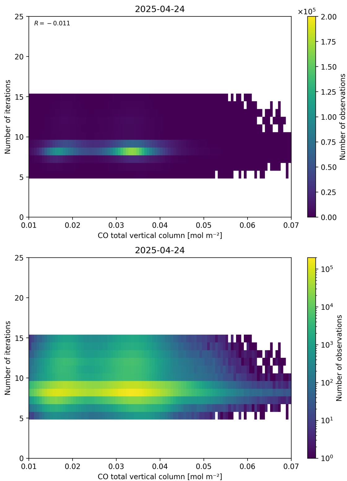
Figure 42: Scatter density plot of “CO total vertical column” against “Number of iterations” for 2025-04-24 to 2025-04-25.
