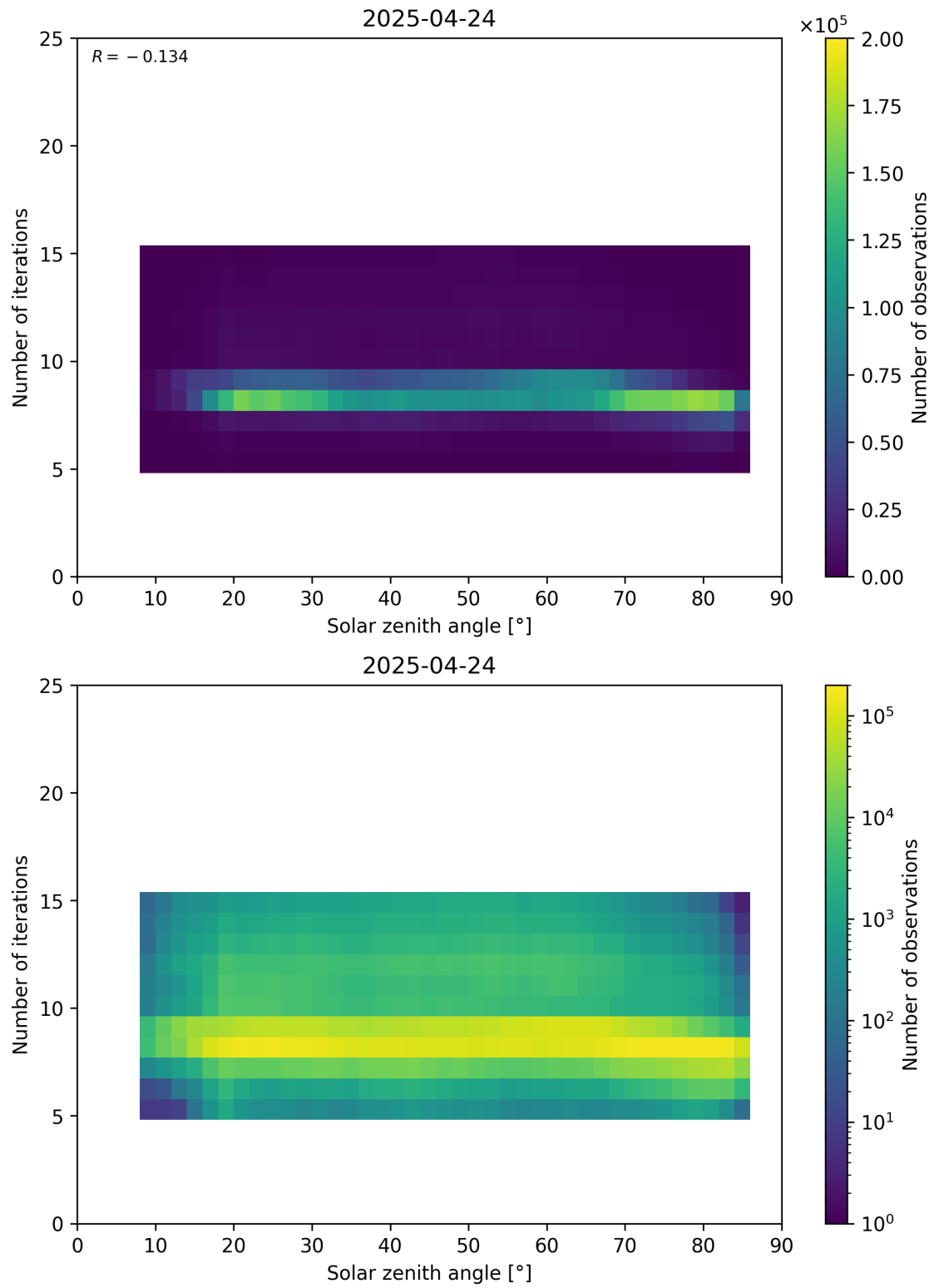
Figure 67: Scatter density plot of “Solar zenith angle” against “Number of iterations” for 2025-04-24 to 2025-04-25.
