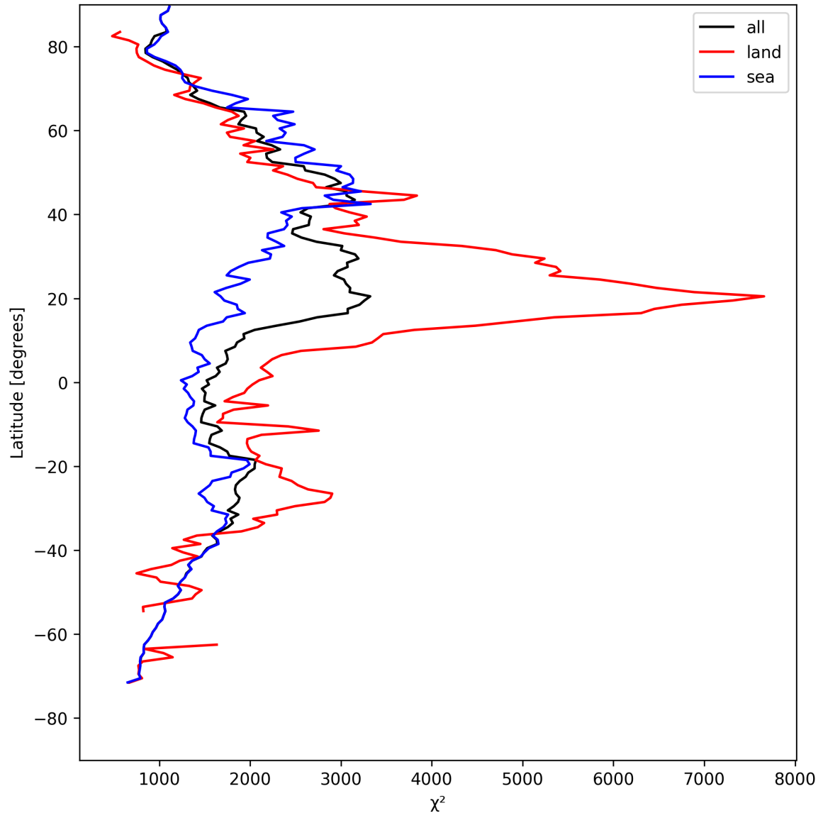
Figure 14: Zonal average of “ \chi^2 ” for 2025-04-24 to 2025-04-25.
