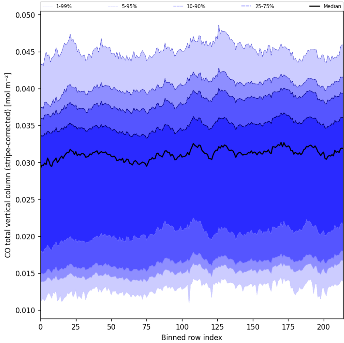
Figure 27: Along track statistics of “CO total vertical column (stripe-corrected)” for 2025-04-24 to 2025-04-25
