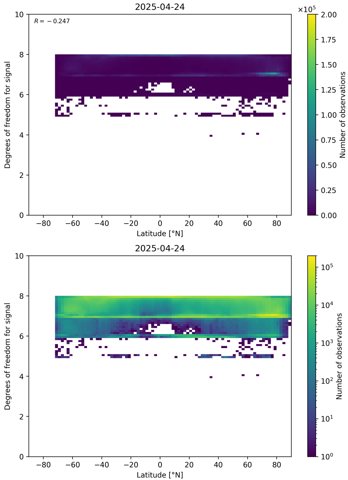
Figure 55: Scatter density plot of “Latitude” against “Degrees of freedom for signal” for 2025-04-24 to 2025-04-25.
