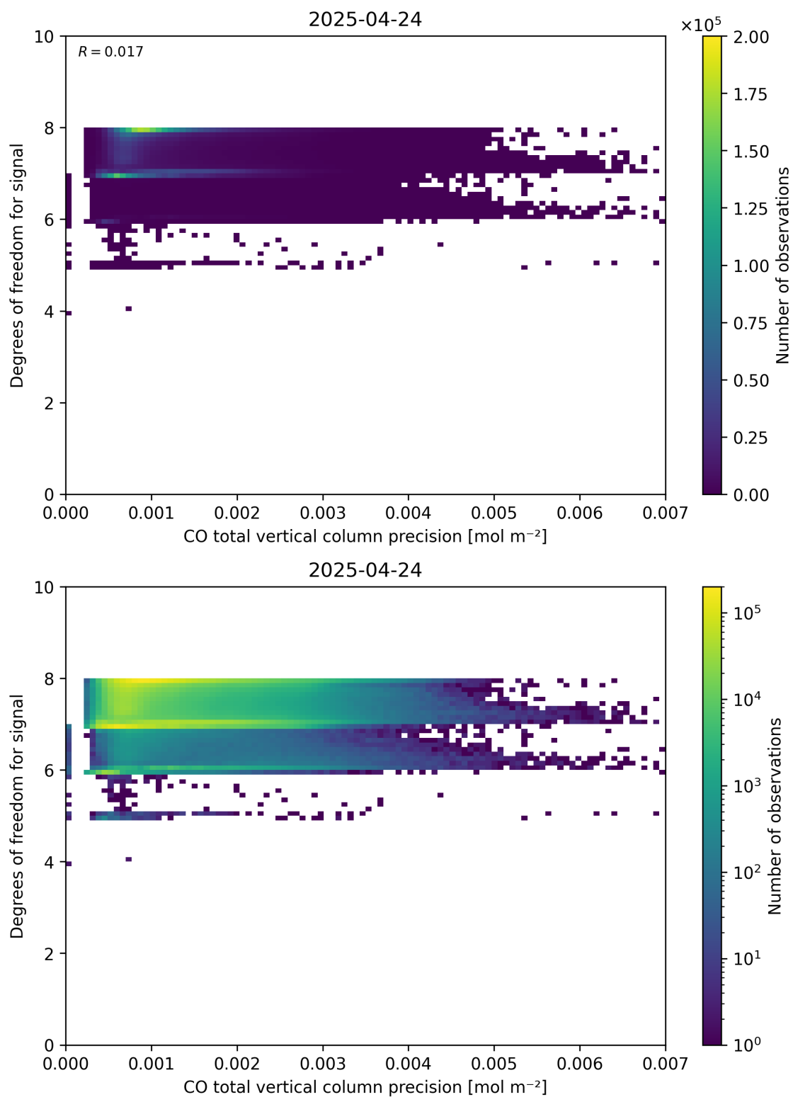
Figure 45: Scatter density plot of “CO total vertical column precision” against “Degrees of freedom for signal” for 2025-04-24 to 2025-04-25.
