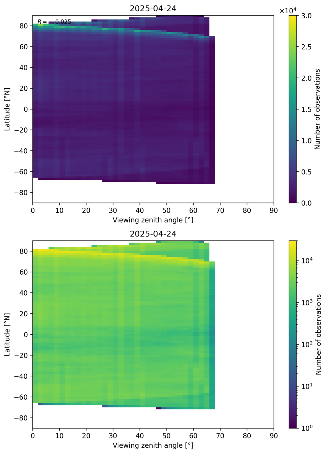
Figure 74: Scatter density plot of “Viewing zenith angle” against “Latitude” for 2025-04-24 to 2025-04-25.
