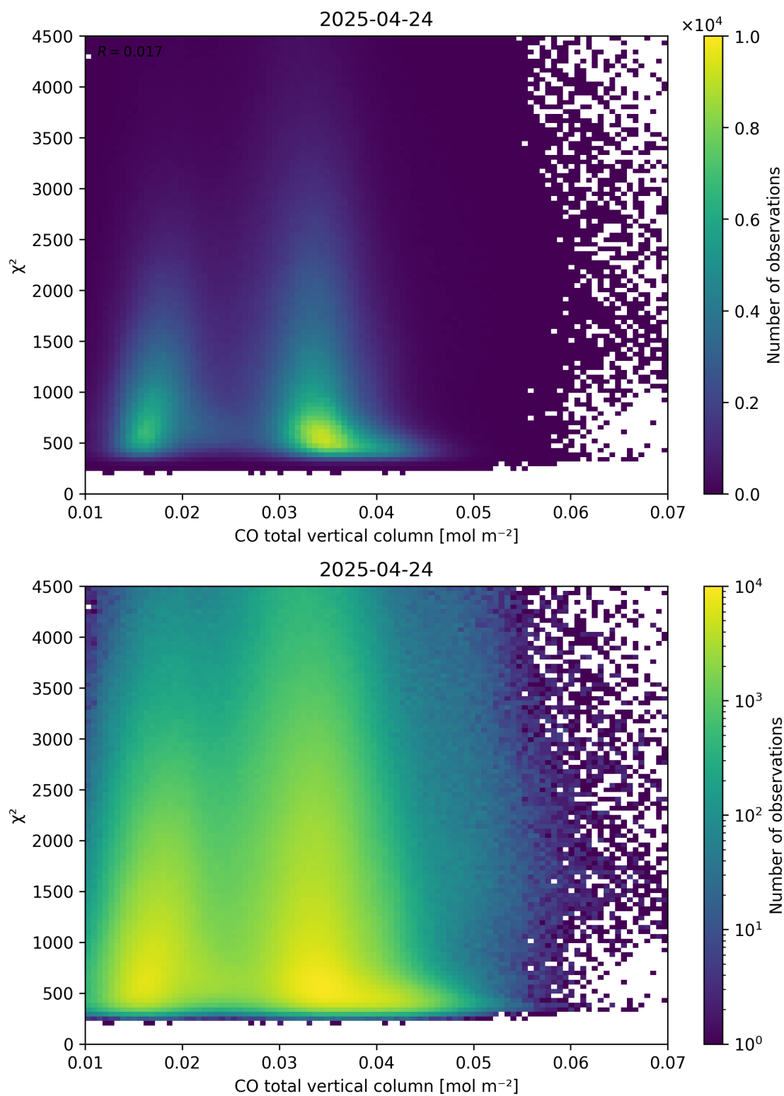
Figure 35: Scatter density plot of “CO total vertical column” against “ \chi^2 ” for 2025-04-24 to 2025-04-25.
