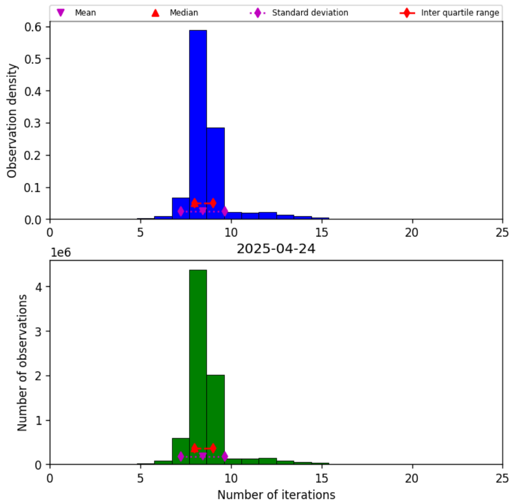
Figure 24: Histogram of “Number of iterations” for 2025-04-24 to 2025-04-25
