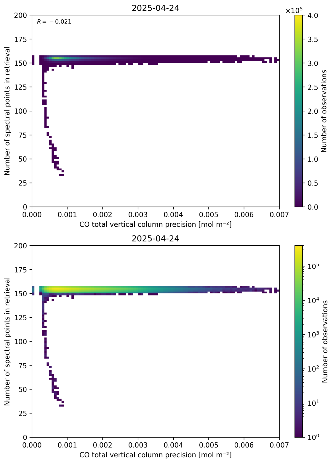
Figure 47: Scatter density plot of “CO total vertical column precision” against “Number of spectral points in retrieval” for 2025-04-24 to 2025-04-25.
