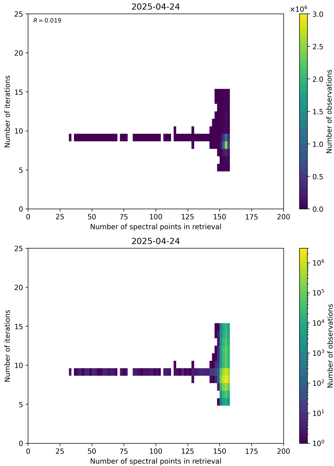
Figure 60: Scatter density plot of “Number of spectral points in retrieval” against “Number of iterations” for 2025-04-24 to 2025-04-25.
