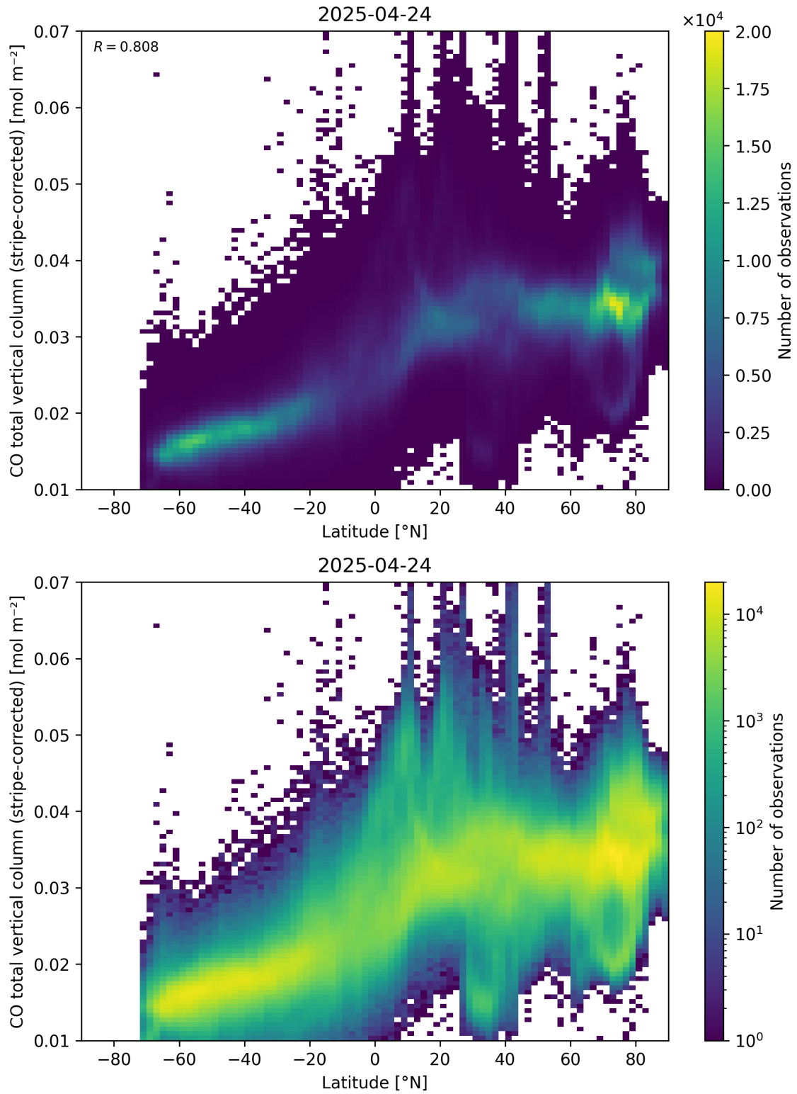
Figure 52: Scatter density plot of “Latitude” against “CO total vertical column (stripe-corrected)” for 2025-04-24 to 2025-04-25.
