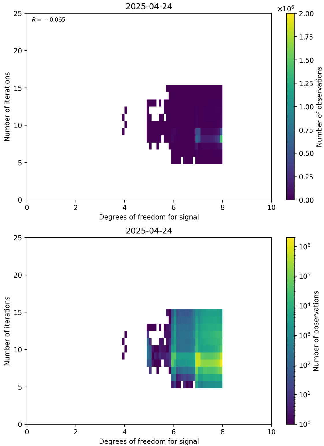
Figure 50: Scatter density plot of “Degrees of freedom for signal” against “Number of iterations” for 2025-04-24 to 2025-04-25.
