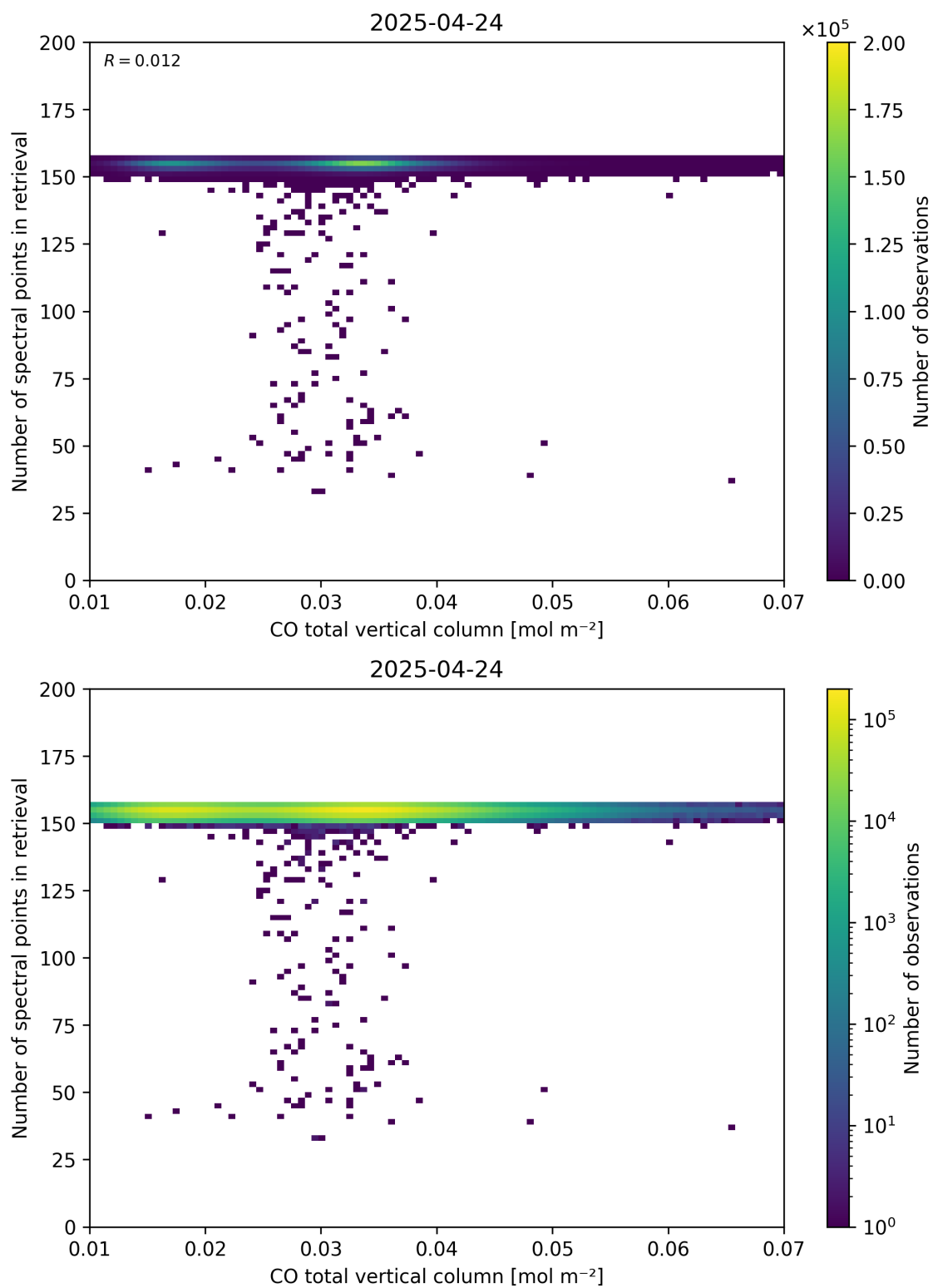
Figure 43: Scatter density plot of “CO total vertical column” against “Number of spectral points in retrieval” for 2025-04-24 to 2025-04-25.
