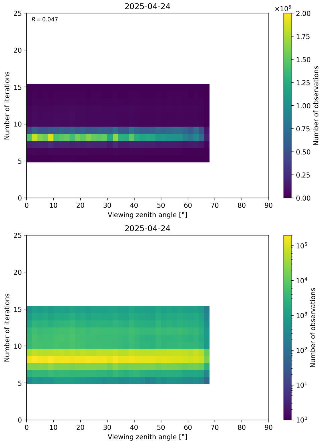
Figure 75: Scatter density plot of “Viewing zenith angle” against “Number of iterations” for 2025-04-24 to 2025-04-25.
