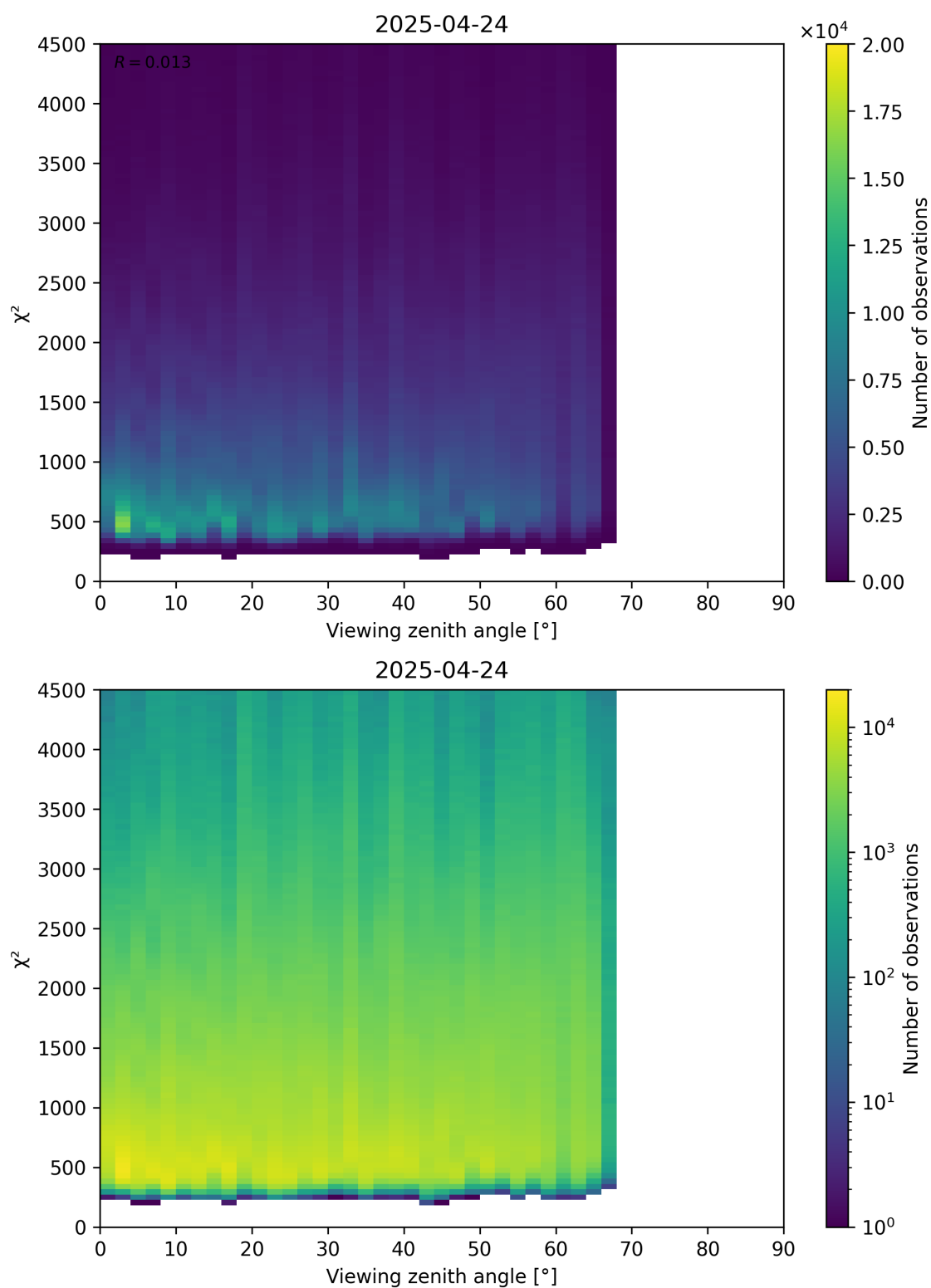
Figure 72: Scatter density plot of “Viewing zenith angle” against “ \chi^2 ” for 2025-04-24 to 2025-04-25.
