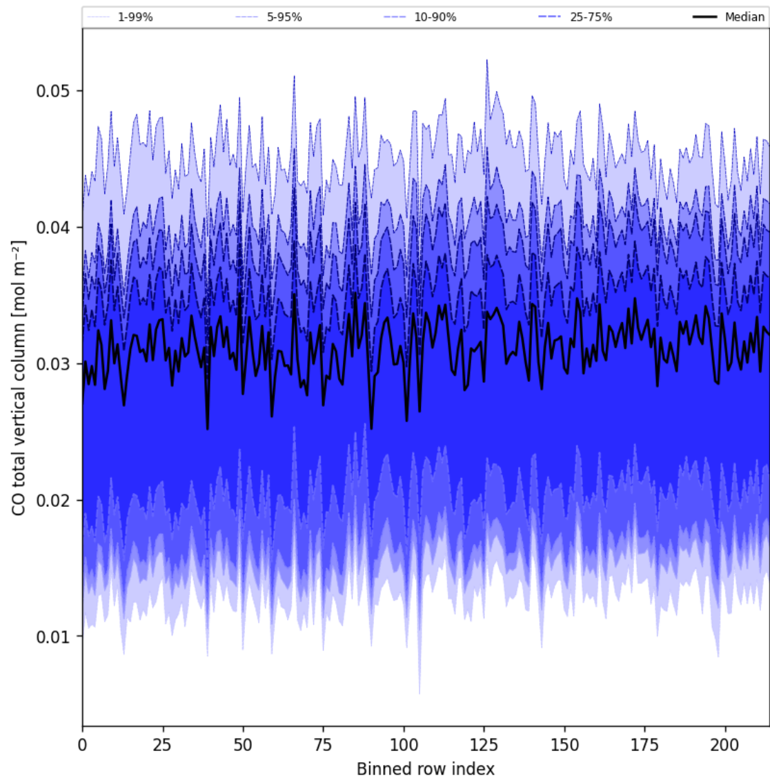
Figure 26: Along track statistics of “CO total vertical column” for 2025-04-24 to 2025-04-25
