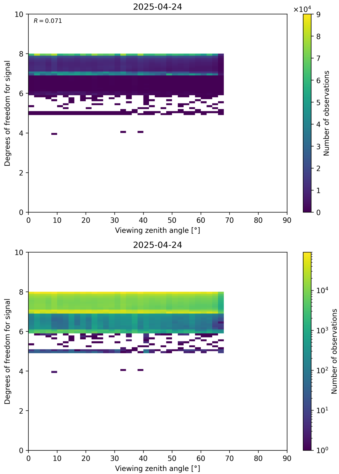
Figure 73: Scatter density plot of “Viewing zenith angle” against “Degrees of freedom for signal” for 2025-04-24 to 2025-04-25.
