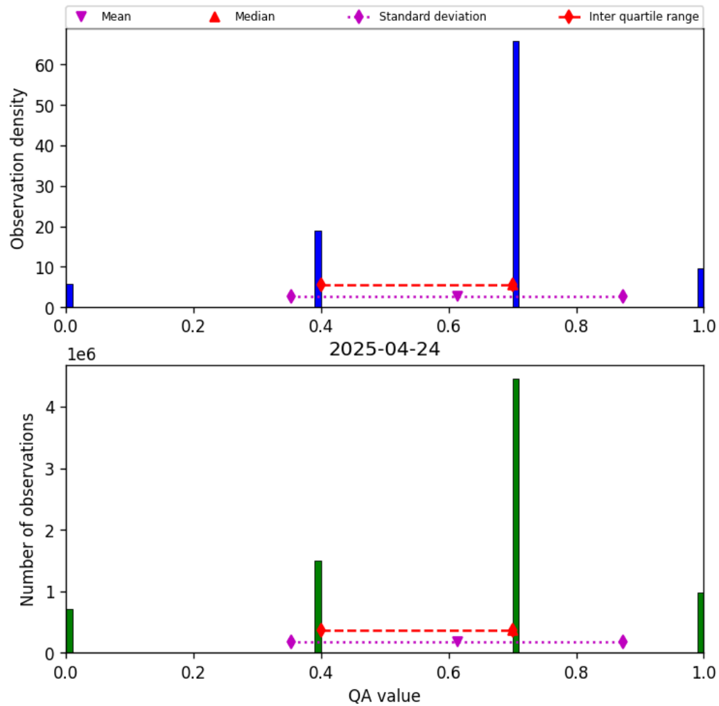
Figure 17: Histogram of “QA value” for 2025-04-24 to 2025-04-25
