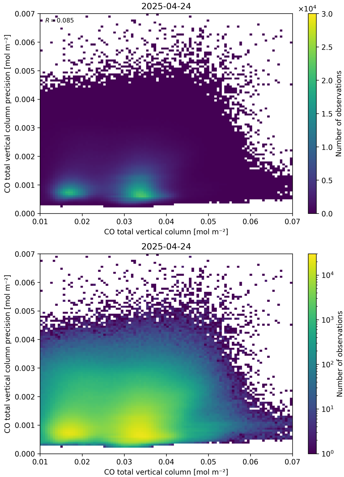
Figure 34: Scatter density plot of “CO total vertical column” against “CO total vertical column precision” for 2025-04-24 to 2025-04-25.
