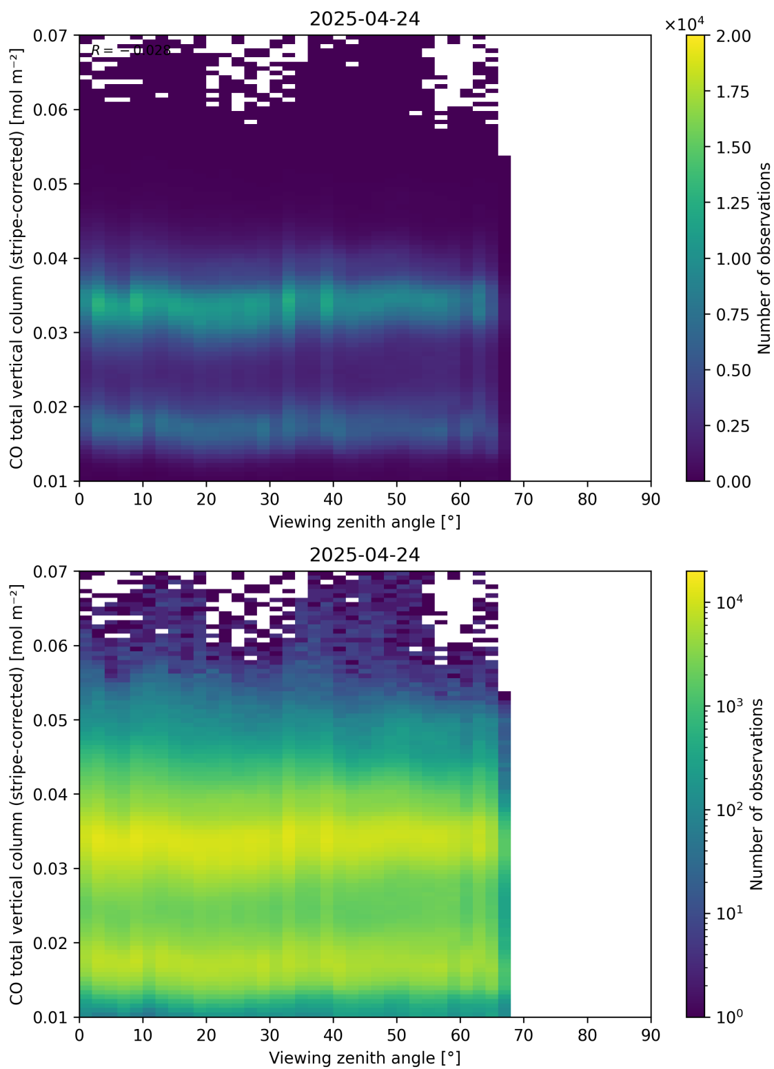
Figure 70: Scatter density plot of “Viewing zenith angle” against “CO total vertical column (stripe-corrected)” for 2025-04-24 to 2025-04-25.
