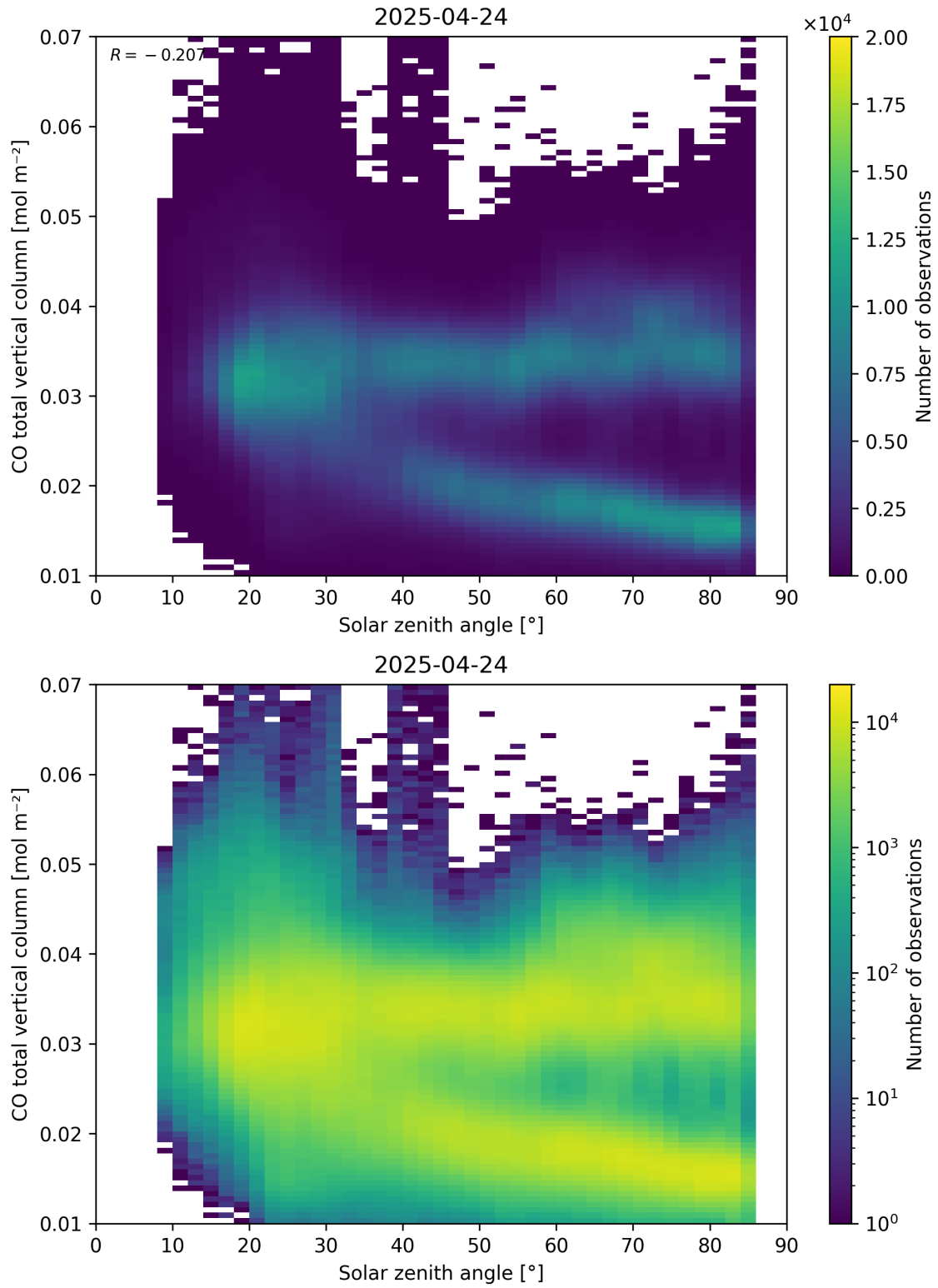
Figure 61: Scatter density plot of “Solar zenith angle” against “CO total vertical column” for 2025-04-24 to 2025-04-25.
