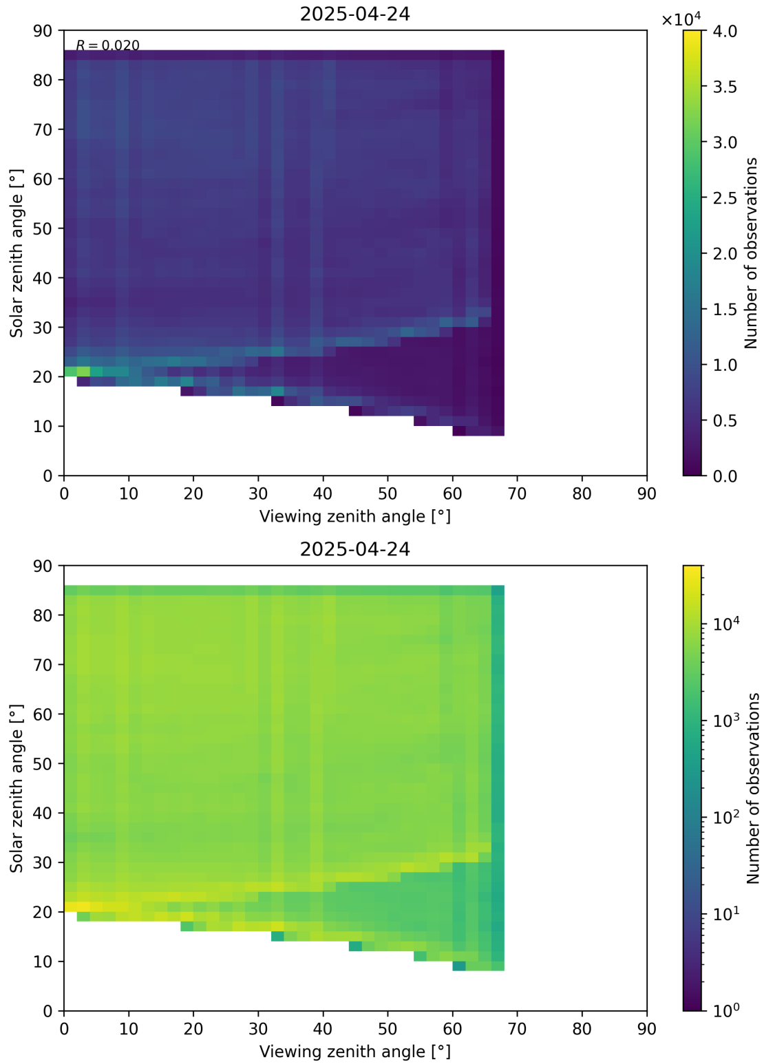
Figure 77: Scatter density plot of “Viewing zenith angle” against “Solar zenith angle” for 2025-04-24 to 2025-04-25.
