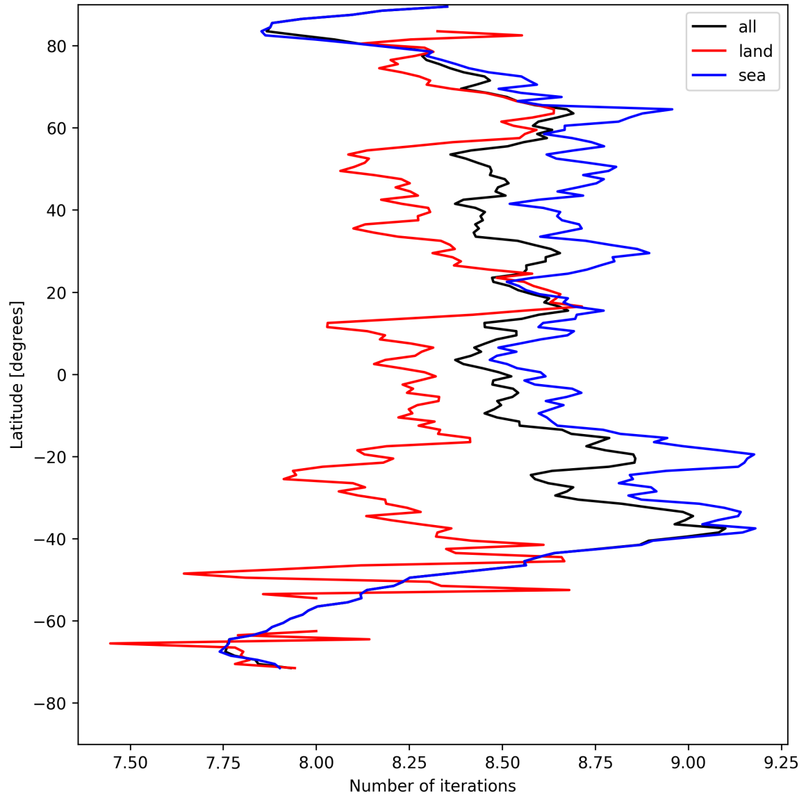
Figure 16: Zonal average of “Number of iterations” for 2025-04-24 to 2025-04-25.
