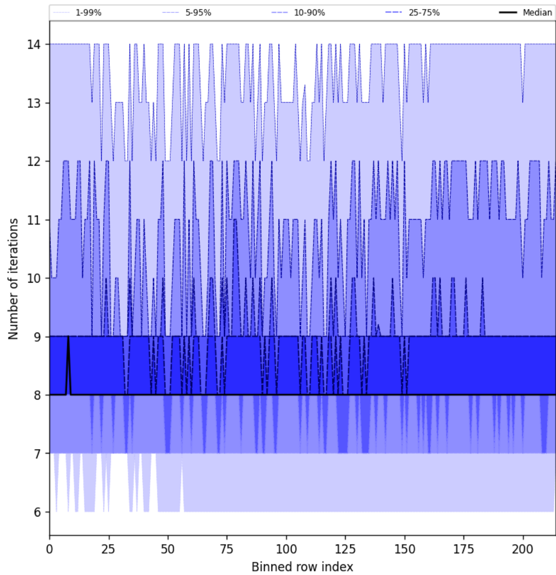
Figure 32: Along track statistics of “Number of iterations” for 2025-04-24 to 2025-04-25
