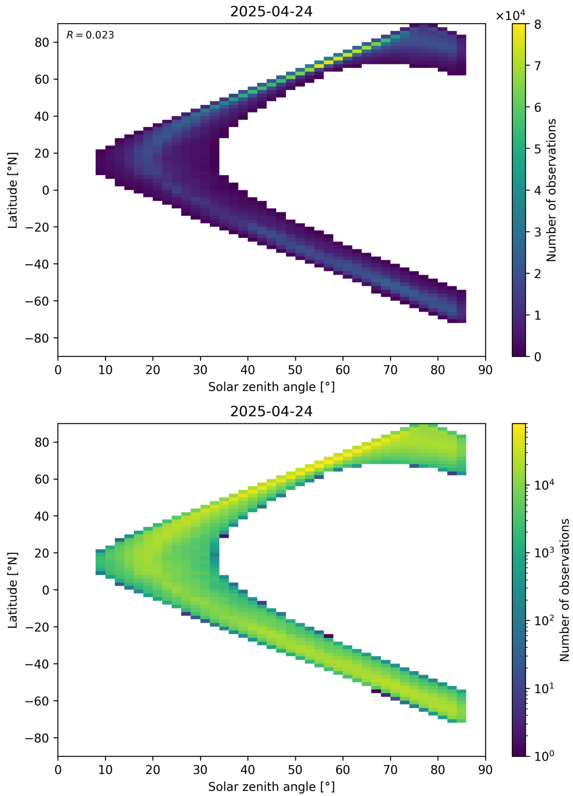
Figure 66: Scatter density plot of “Solar zenith angle” against “Latitude” for 2025-04-24 to 2025-04-25.
