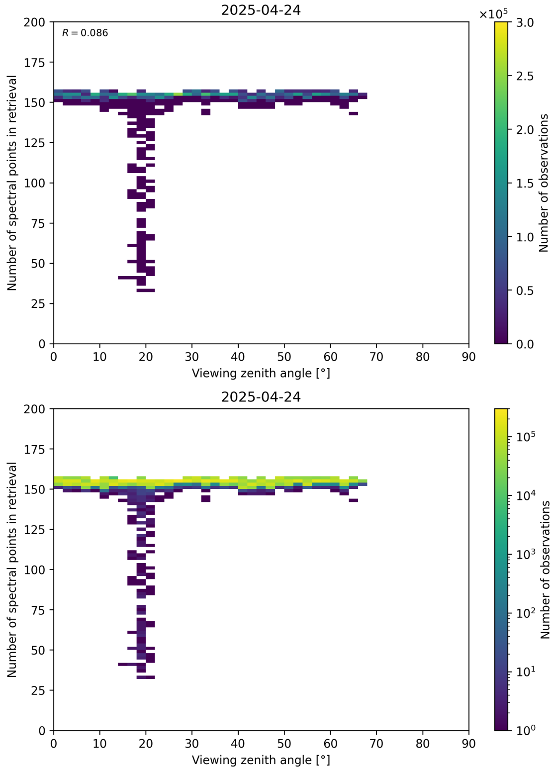
Figure 76: Scatter density plot of “Viewing zenith angle” against “Number of spectral points in retrieval” for 2025-04-24 to 2025-04-25.
