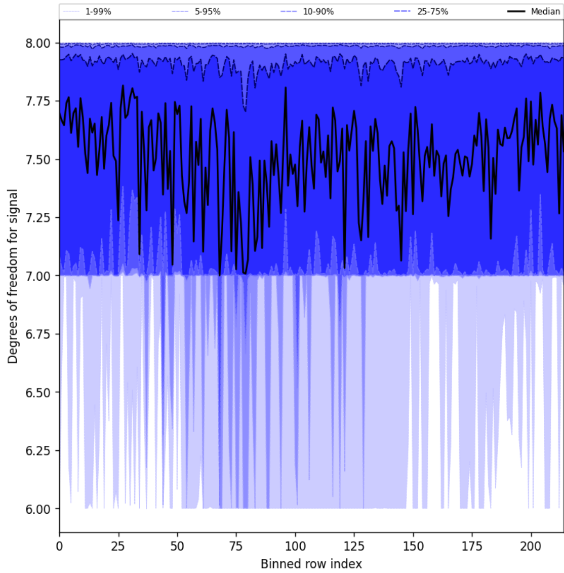
Figure 31: Along track statistics of “Degrees of freedom for signal” for 2025-04-24 to 2025-04-25
