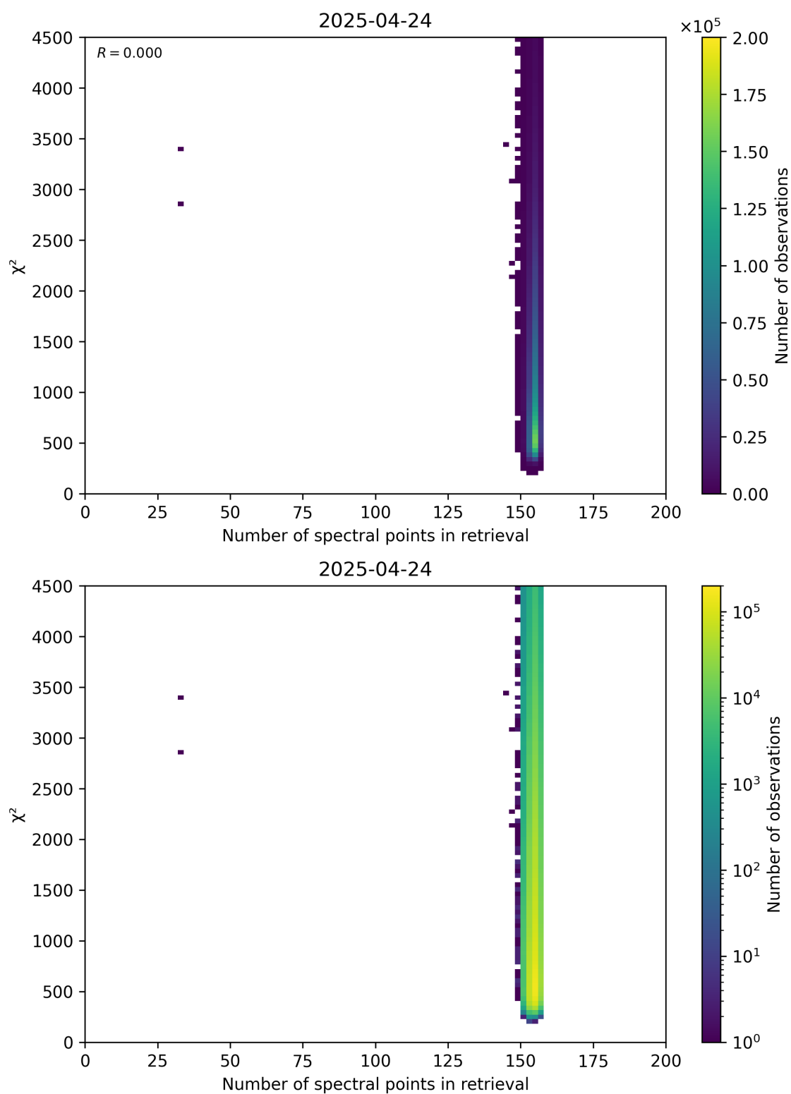
Figure 58: Scatter density plot of “Number of spectral points in retrieval” against “ \chi^2 ” for 2025-04-24 to 2025-04-25.
