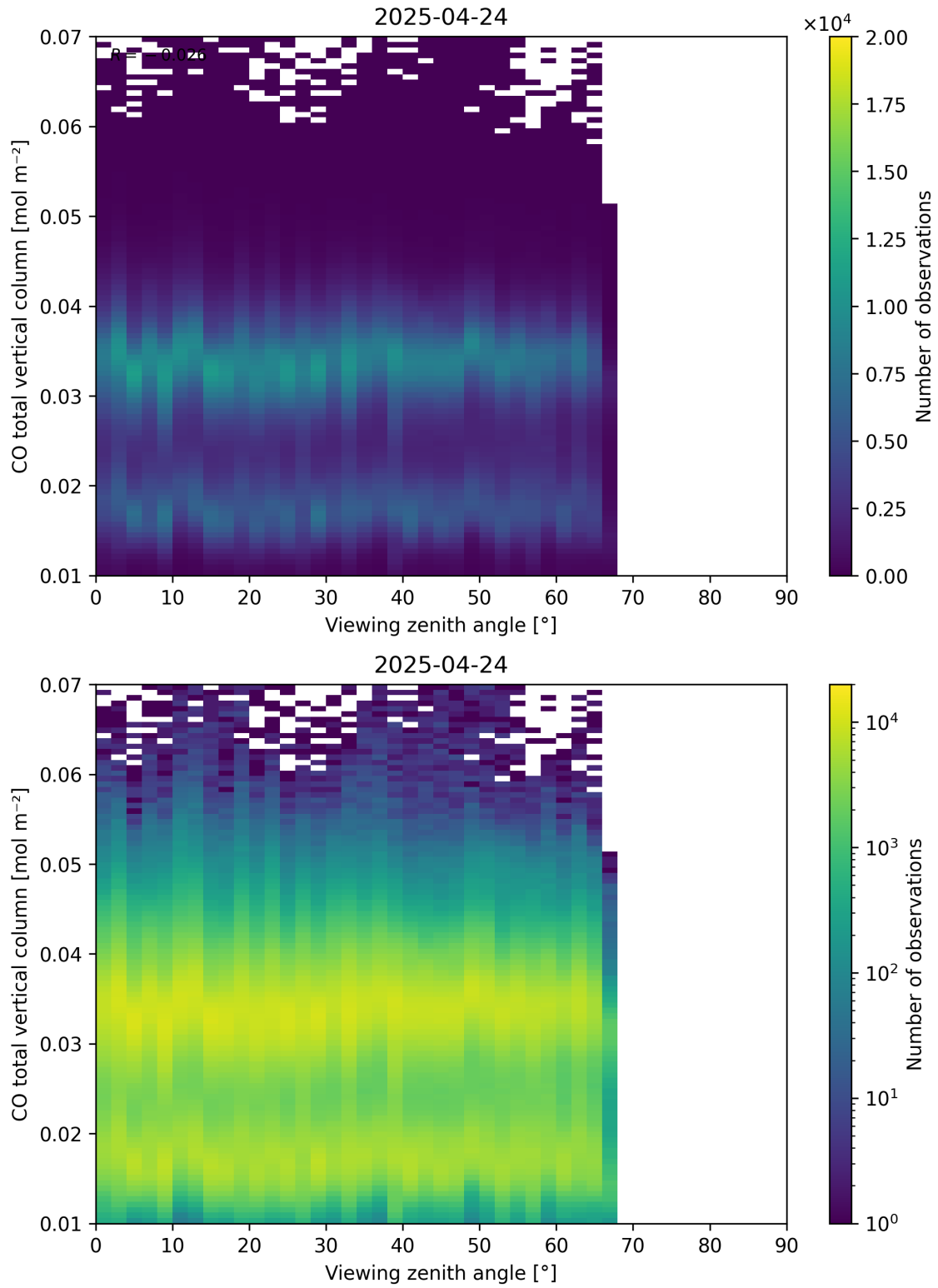
Figure 69: Scatter density plot of “Viewing zenith angle” against “CO total vertical column” for 2025-04-24 to 2025-04-25.
