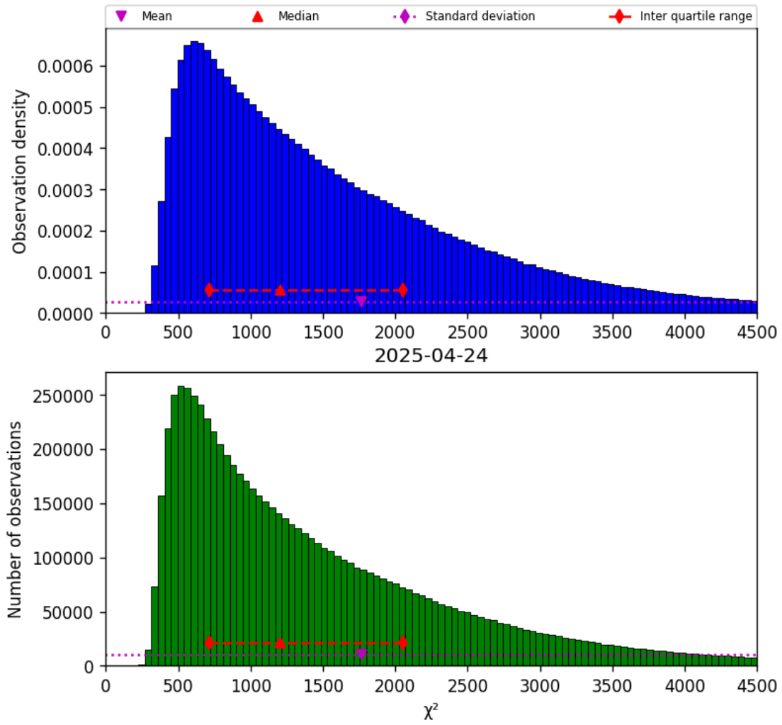
Figure 22: Histogram of “ \chi^2 ” for 2025-04-24 to 2025-04-25
