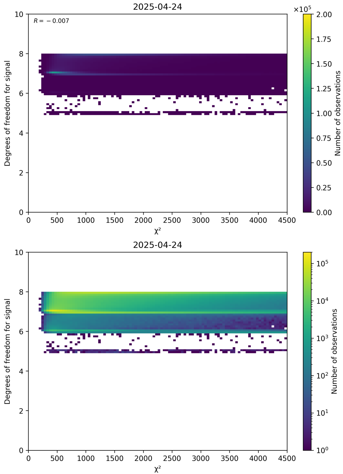
Figure 48: Scatter density plot of " \chi^2 " against "Degrees of freedom for signal" for 2025-04-24 to 2025-04-25.
