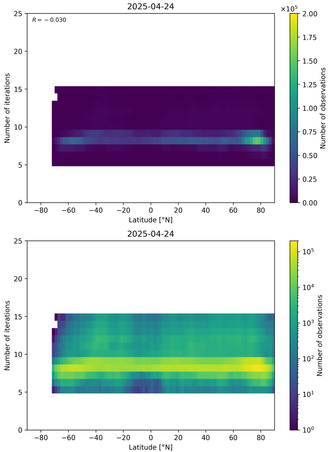
Figure 56: Scatter density plot of “Latitude” against “Number of iterations” for 2025-04-24 to 2025-04-25.
