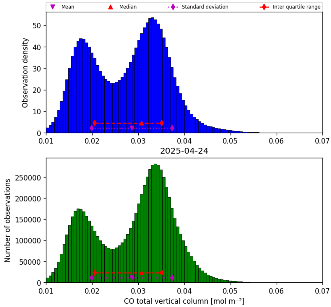
Figure 18: Histogram of “CO total vertical column” for 2025-04-24 to 2025-04-25
