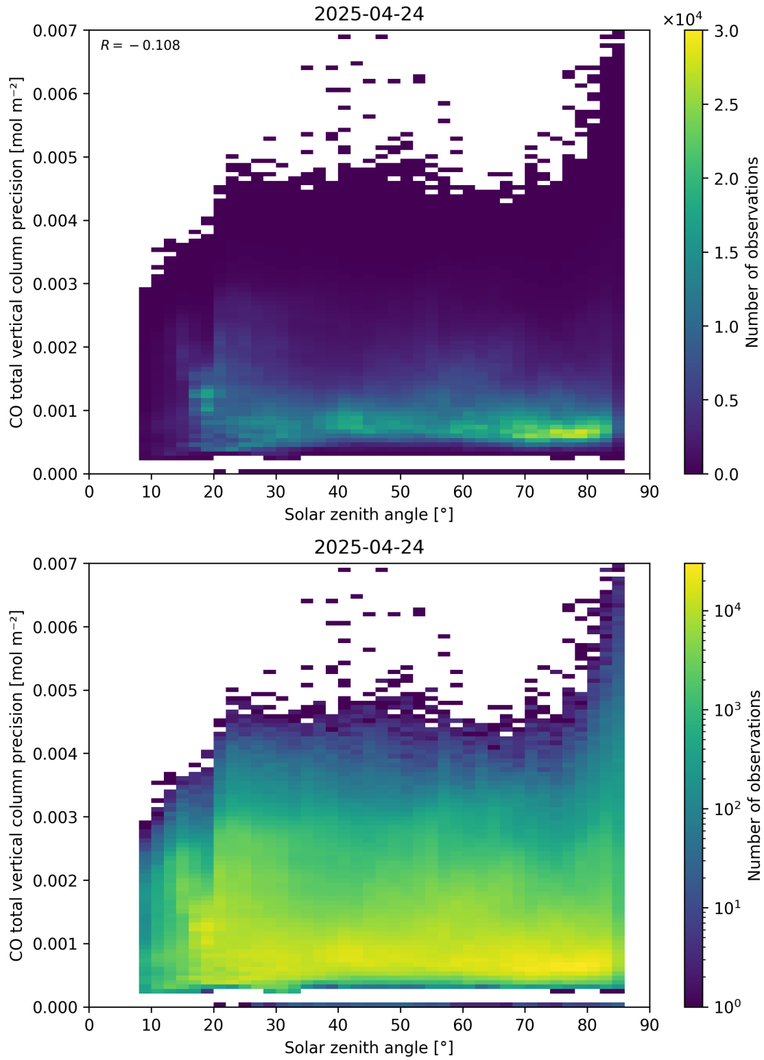
Figure 63: Scatter density plot of “Solar zenith angle” against “CO total vertical column precision” for 2025-04-24 to 2025-04-25.
