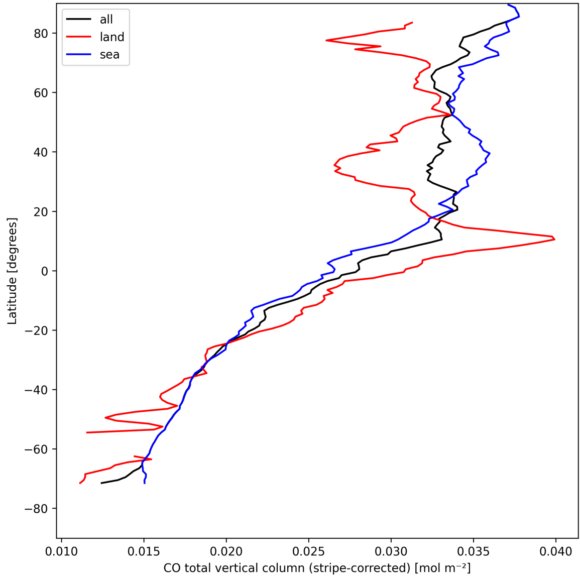
Figure 11: Zonal average of “CO total vertical column (stripe-corrected)” for 2025-04-24 to 2025-04-25.
