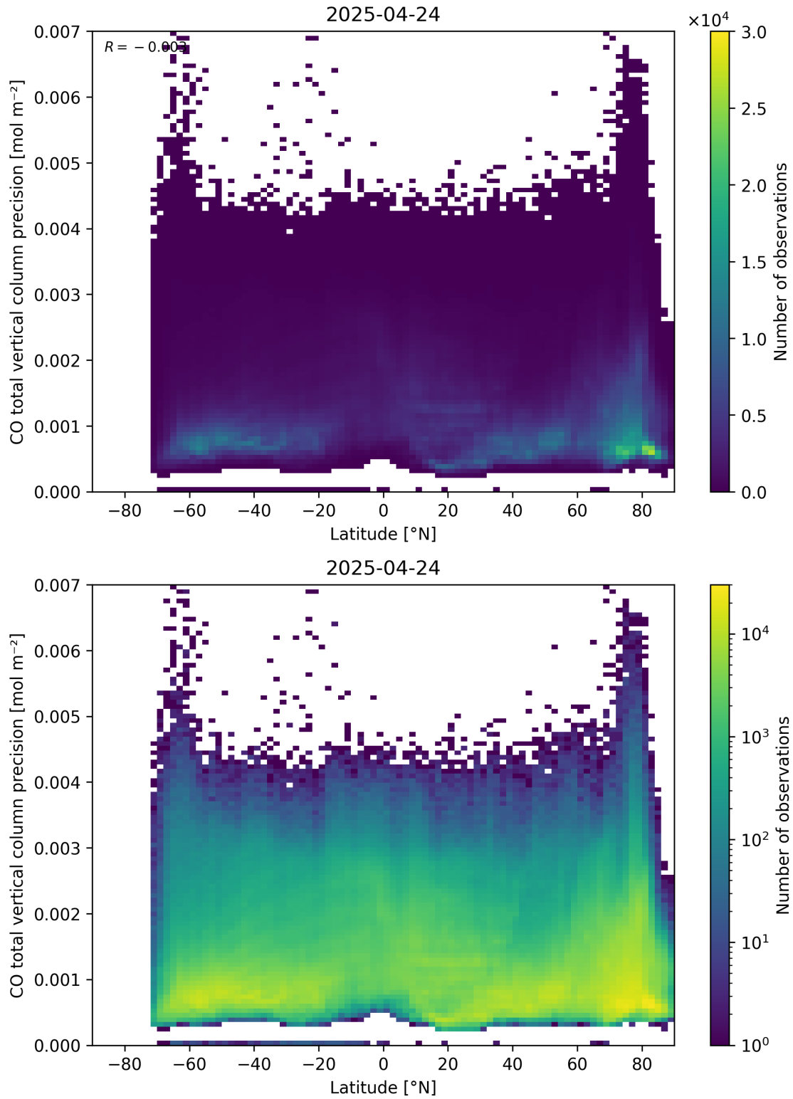
Figure 53: Scatter density plot of “Latitude” against “CO total vertical column precision” for 2025-04-24 to 2025-04-25.
