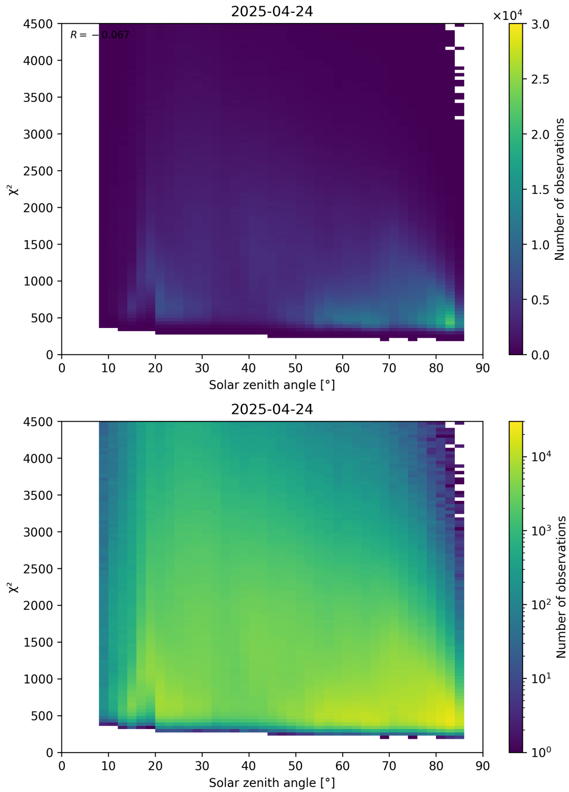
Figure 64: Scatter density plot of “Solar zenith angle” against “ \chi^2 ” for 2025-04-24 to 2025-04-25.
