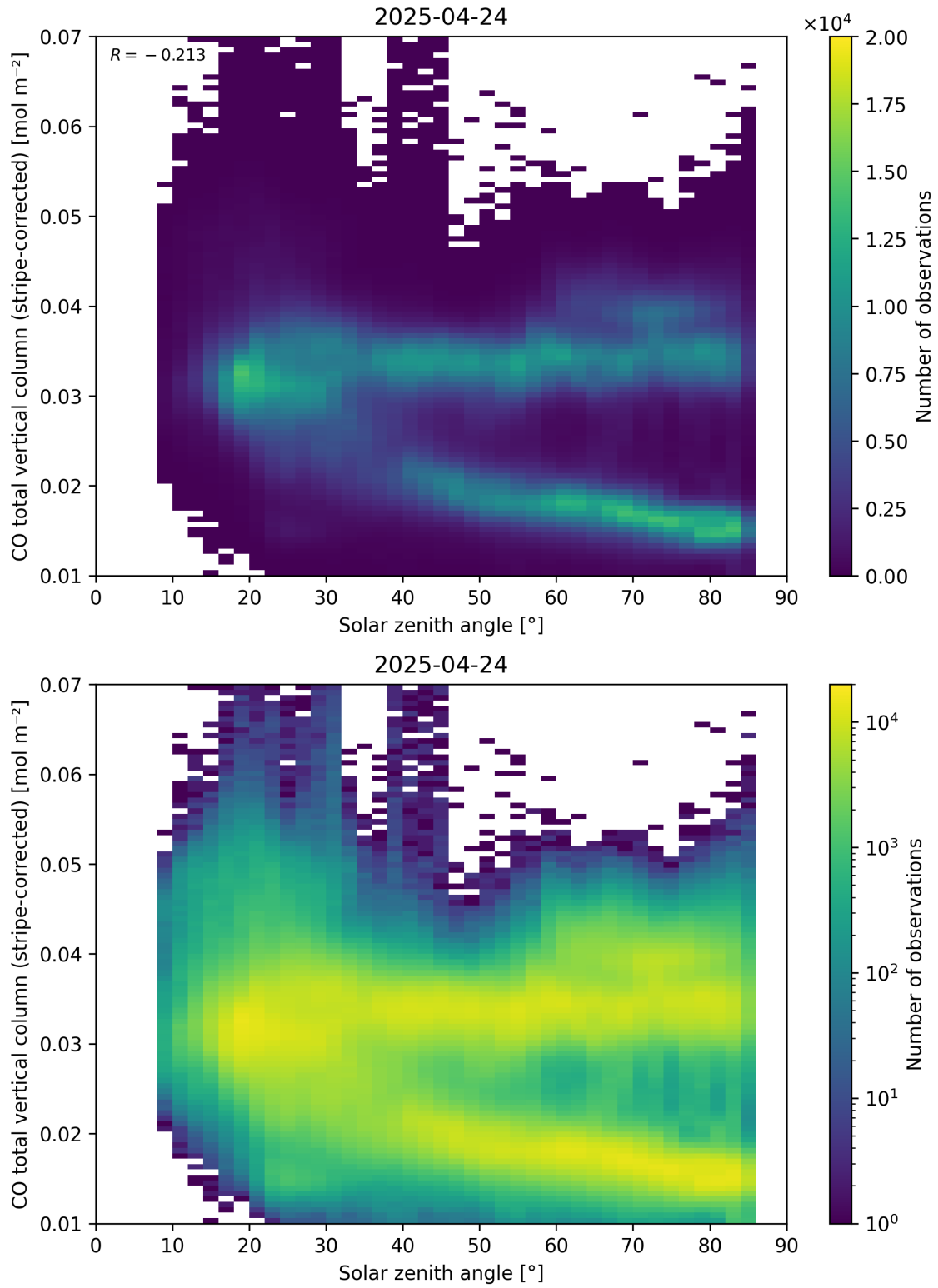
Figure 62: Scatter density plot of “Solar zenith angle” against “CO total vertical column (stripe-corrected)” for 2025-04-24 to 2025-04-25.
