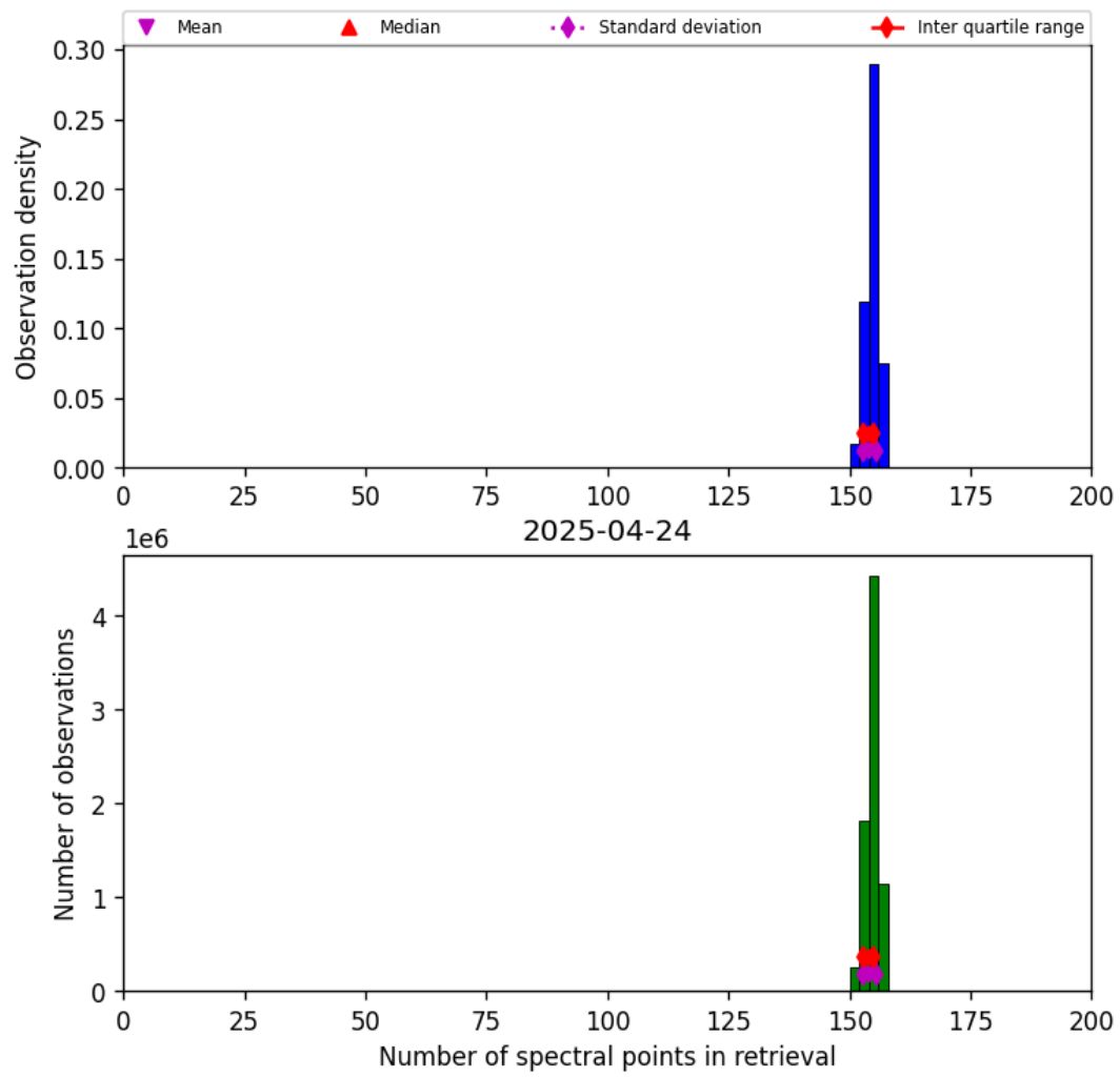
Figure 21: Histogram of “Number of spectral points in retrieval” for 2025-04-24 to 2025-04-25
