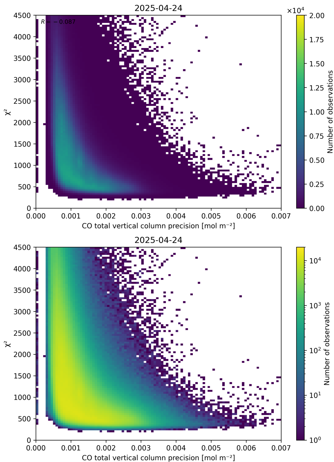
Figure 44: Scatter density plot of “CO total vertical column precision” against “ \chi^2 ” for 2025-04-24 to 2025-04-25.
