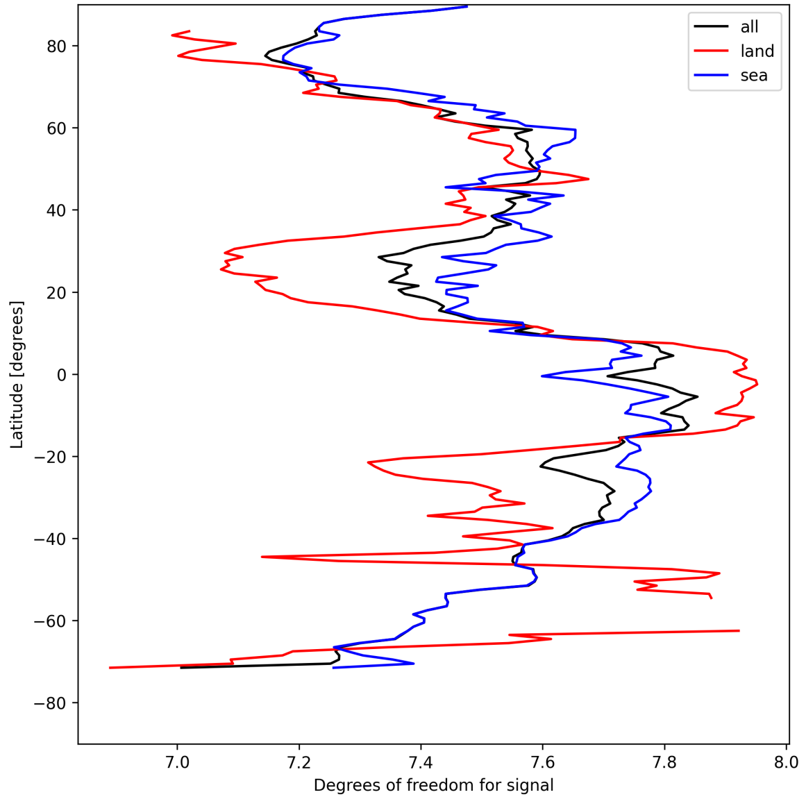
Figure 15: Zonal average of “Degrees of freedom for signal” for 2025-04-24 to 2025-04-25.
