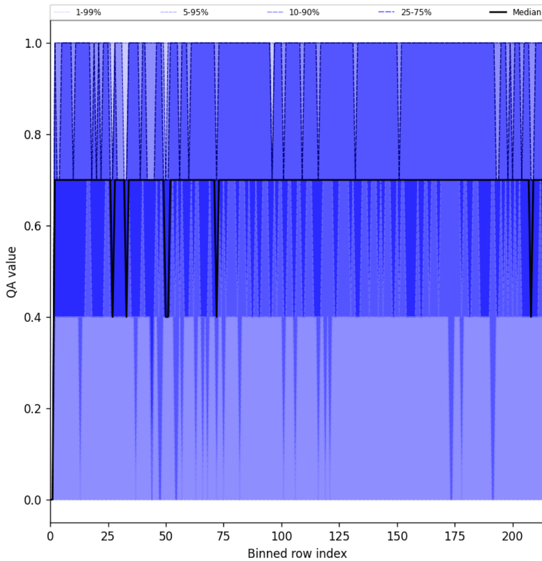
Figure 25: Along track statistics of “QA value” for 2025-04-24 to 2025-04-25
