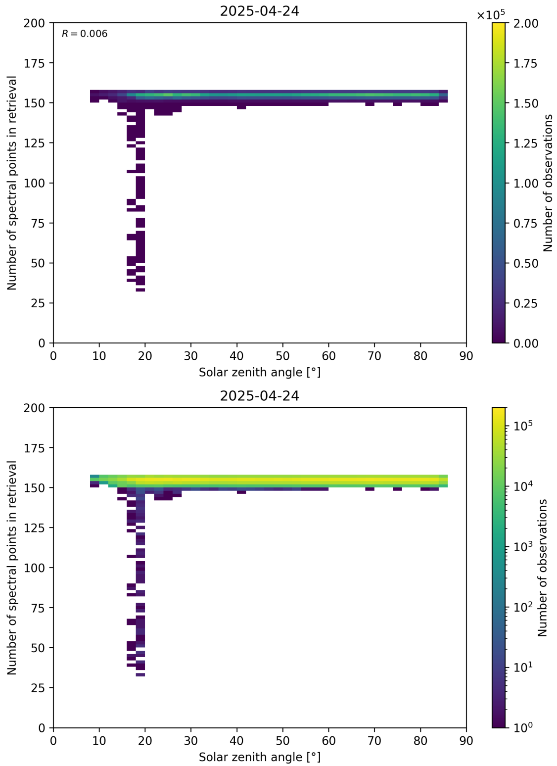
Figure 68: Scatter density plot of “Solar zenith angle” against “Number of spectral points in retrieval” for 2025-04-24 to 2025-04-25.
