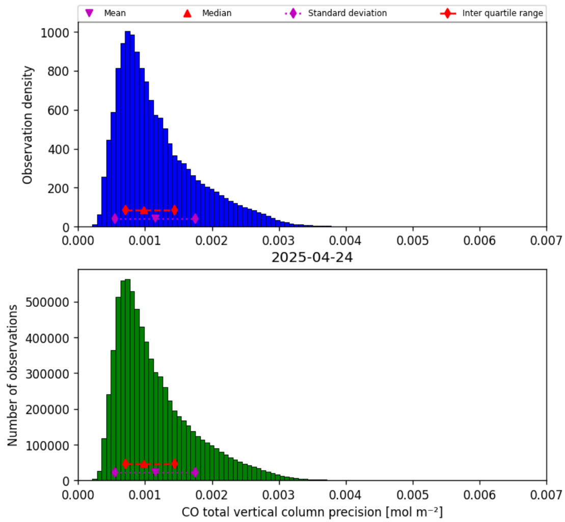
Figure 20: Histogram of “CO total vertical column precision” for 2025-04-24 to 2025-04-25
