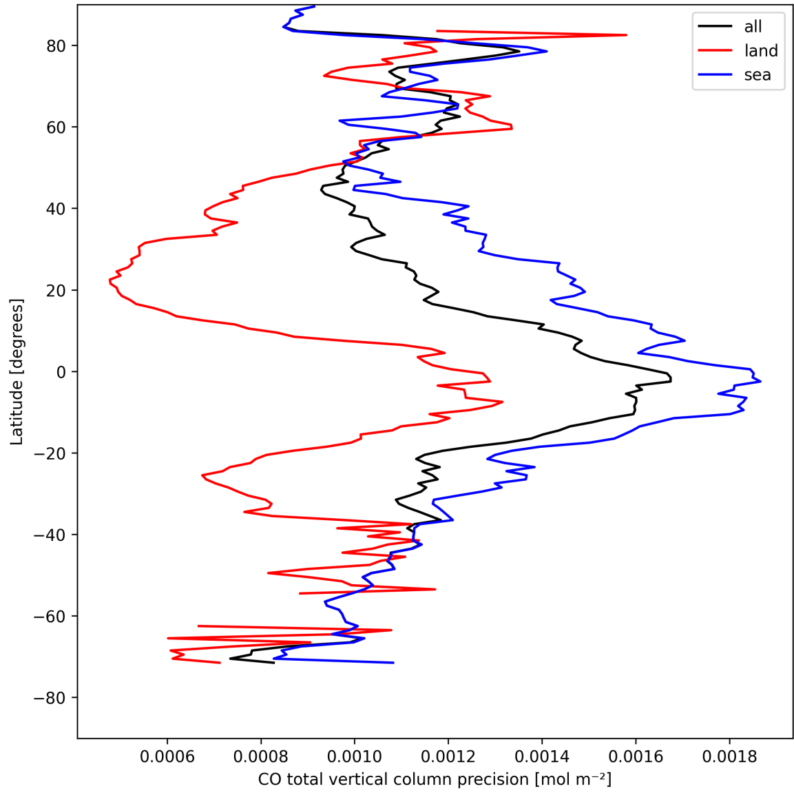
Figure 12: Zonal average of “CO total vertical column precision” for 2025-04-24 to 2025-04-25.
