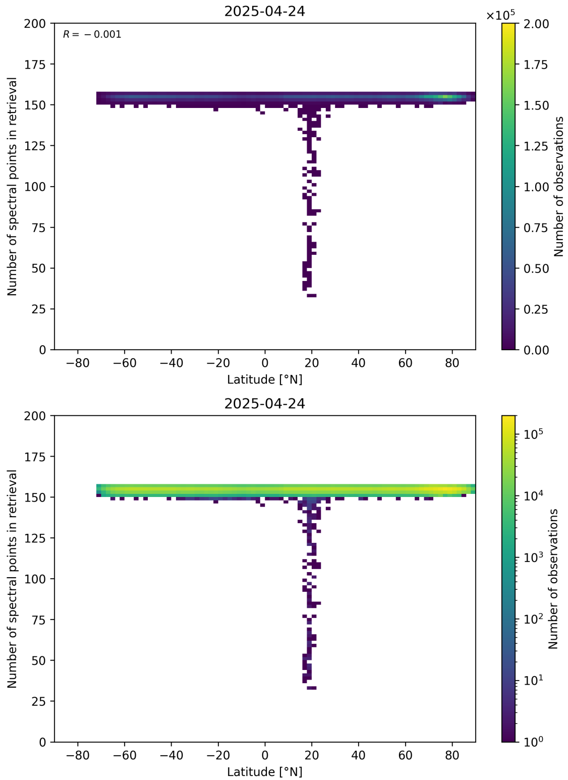
Figure 57: Scatter density plot of “Latitude” against “Number of spectral points in retrieval” for 2025-04-24 to 2025-04-25.
