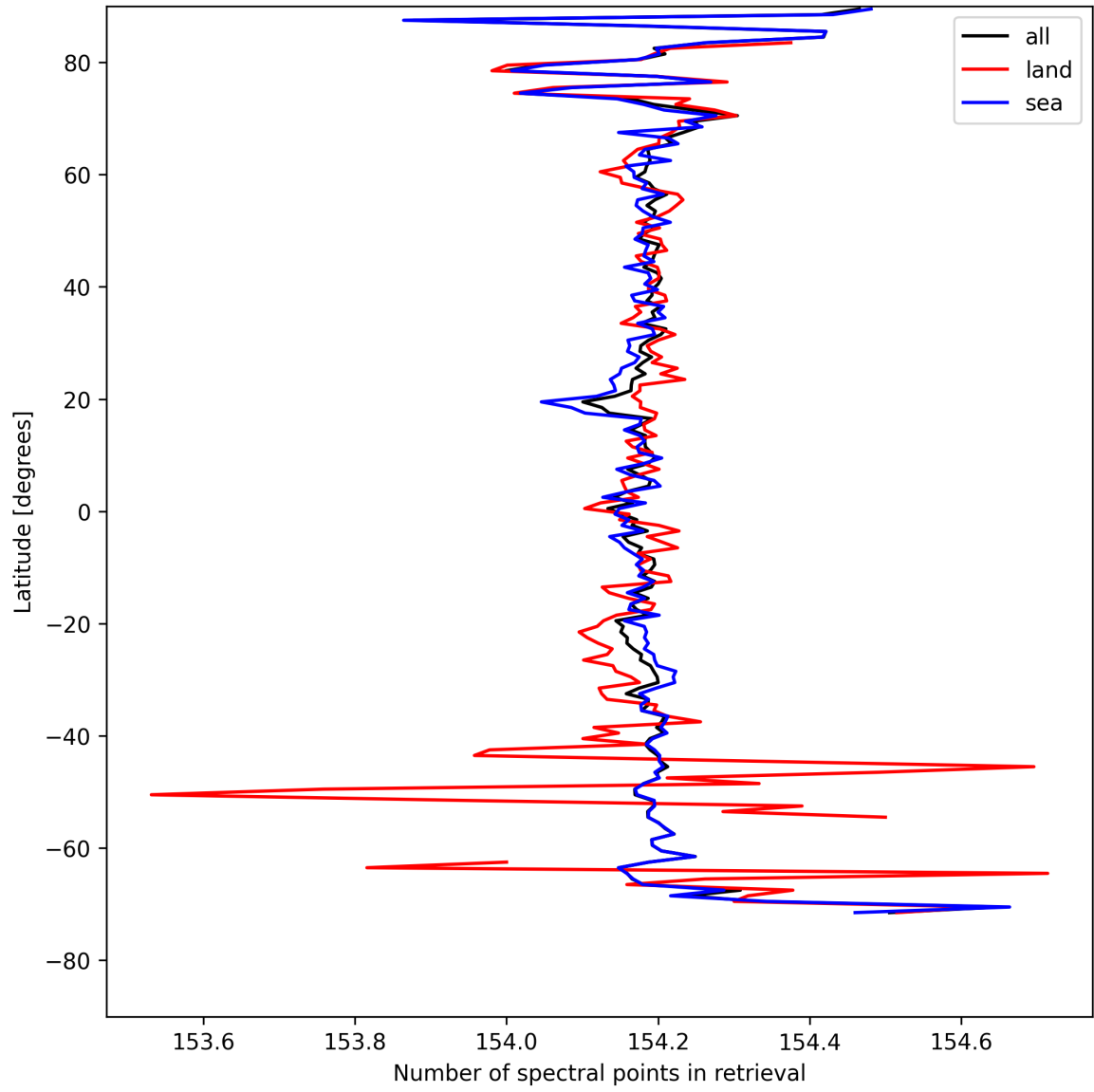
Figure 13: Zonal average of “Number of spectral points in retrieval” for 2025-04-24 to 2025-04-25.
