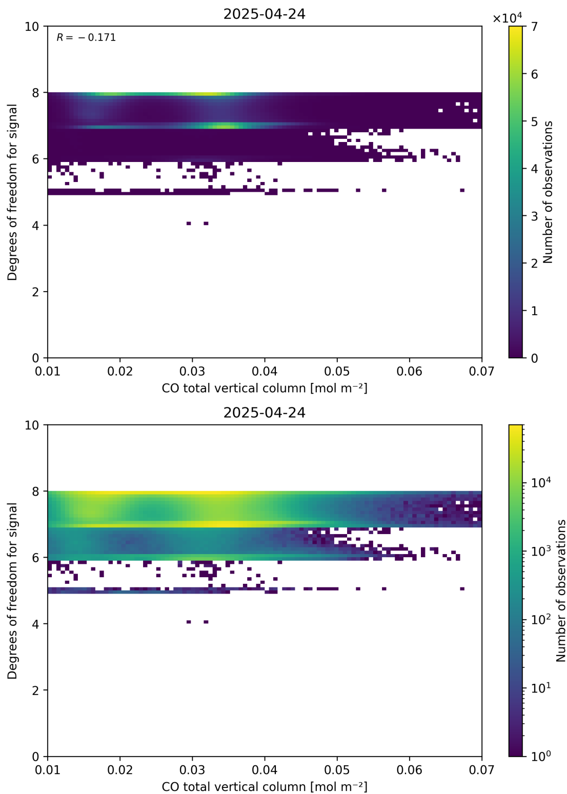
Figure 41: Scatter density plot of “CO total vertical column” against “Degrees of freedom for signal” for 2025-04-24 to 2025-04-25.
