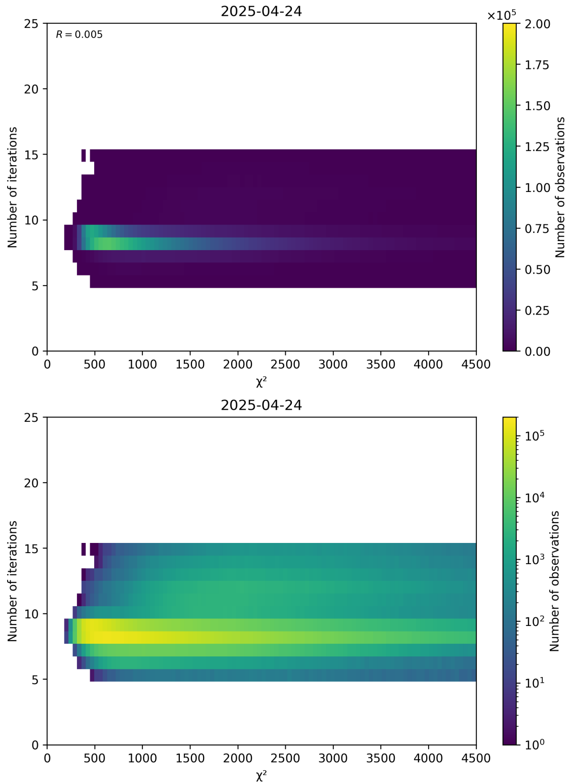
Figure 49: Scatter density plot of “ \chi^2 ” against “Number of iterations” for 2025-04-24 to 2025-04-25.
