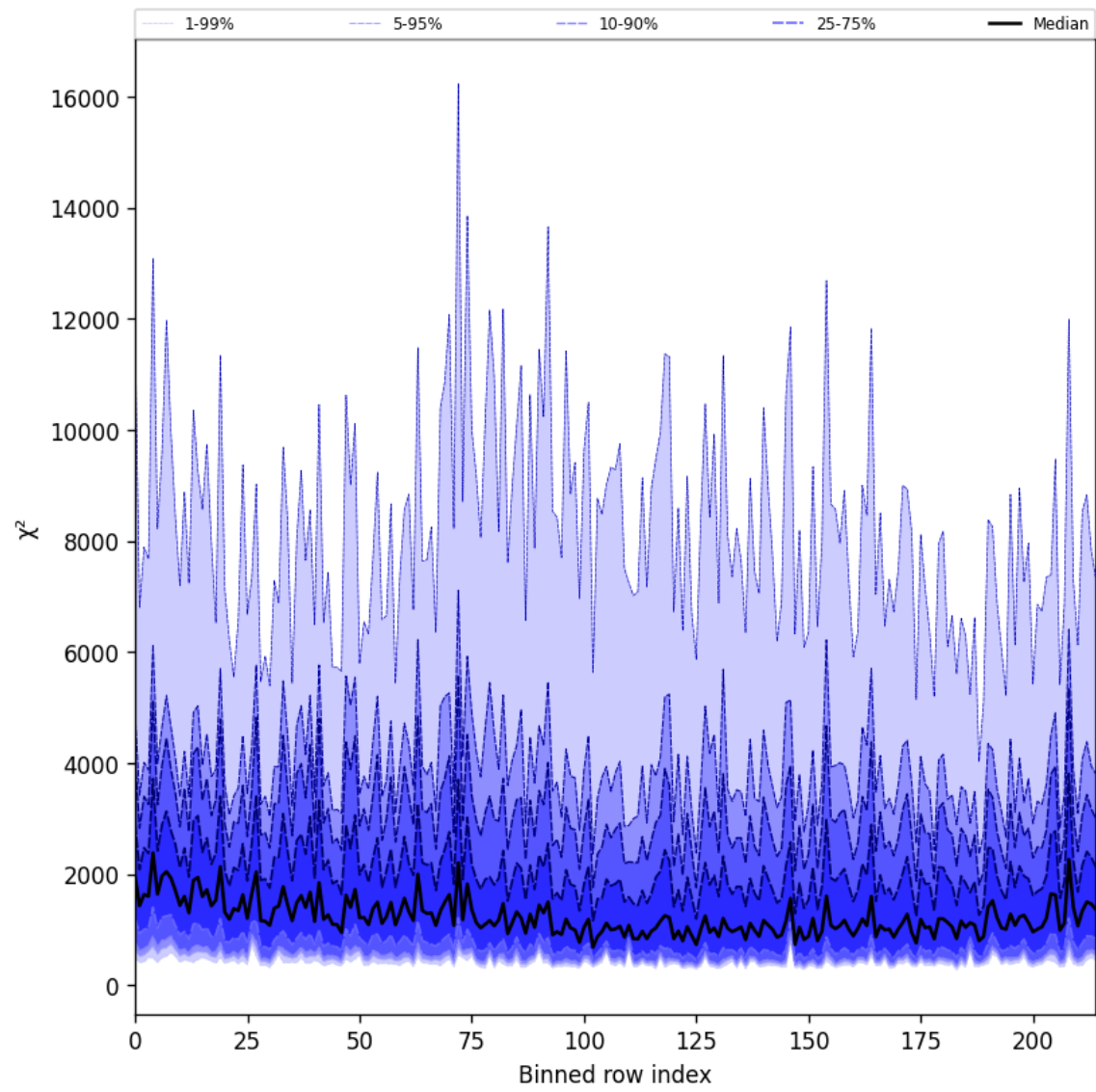
Figure 30: Along track statistics of “ \chi^2 ” for 2025-04-24 to 2025-04-25
