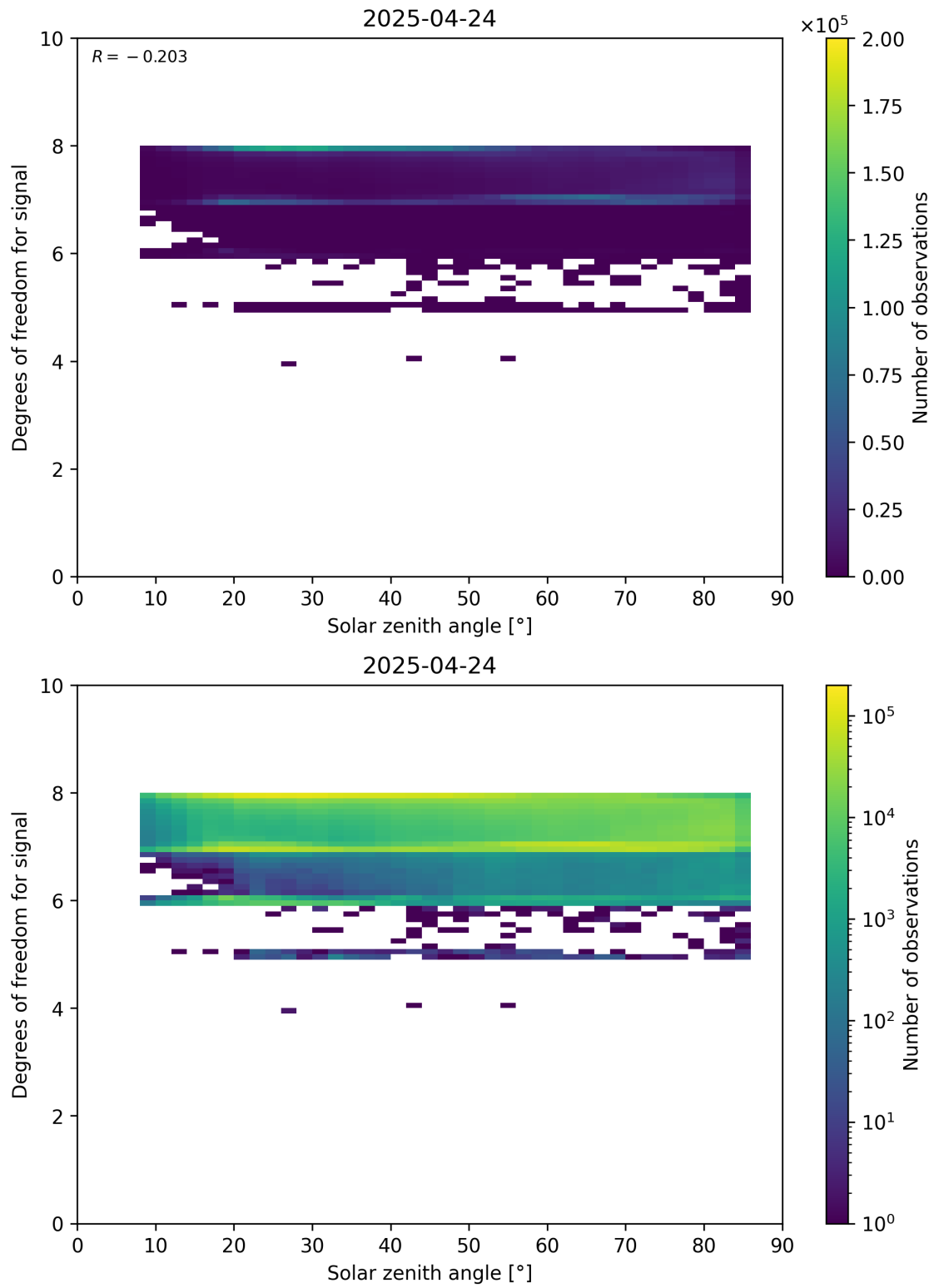
Figure 65: Scatter density plot of “Solar zenith angle” against “Degrees of freedom for signal” for 2025-04-24 to 2025-04-25.
