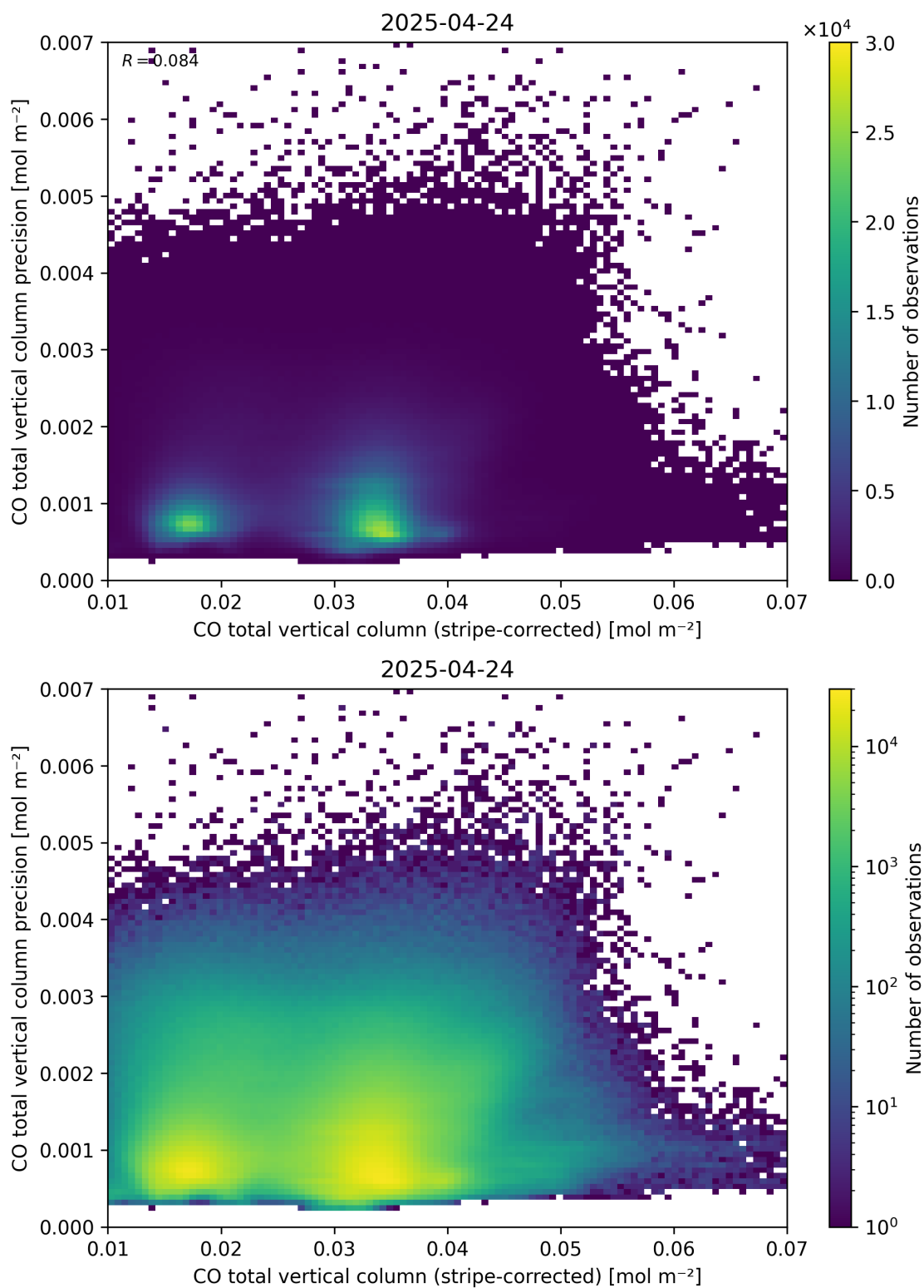
Figure 36: Scatter density plot of “CO total vertical column (stripe-corrected)” against “CO total vertical column precision” for 2025-04-24 to 2025-04-25.
