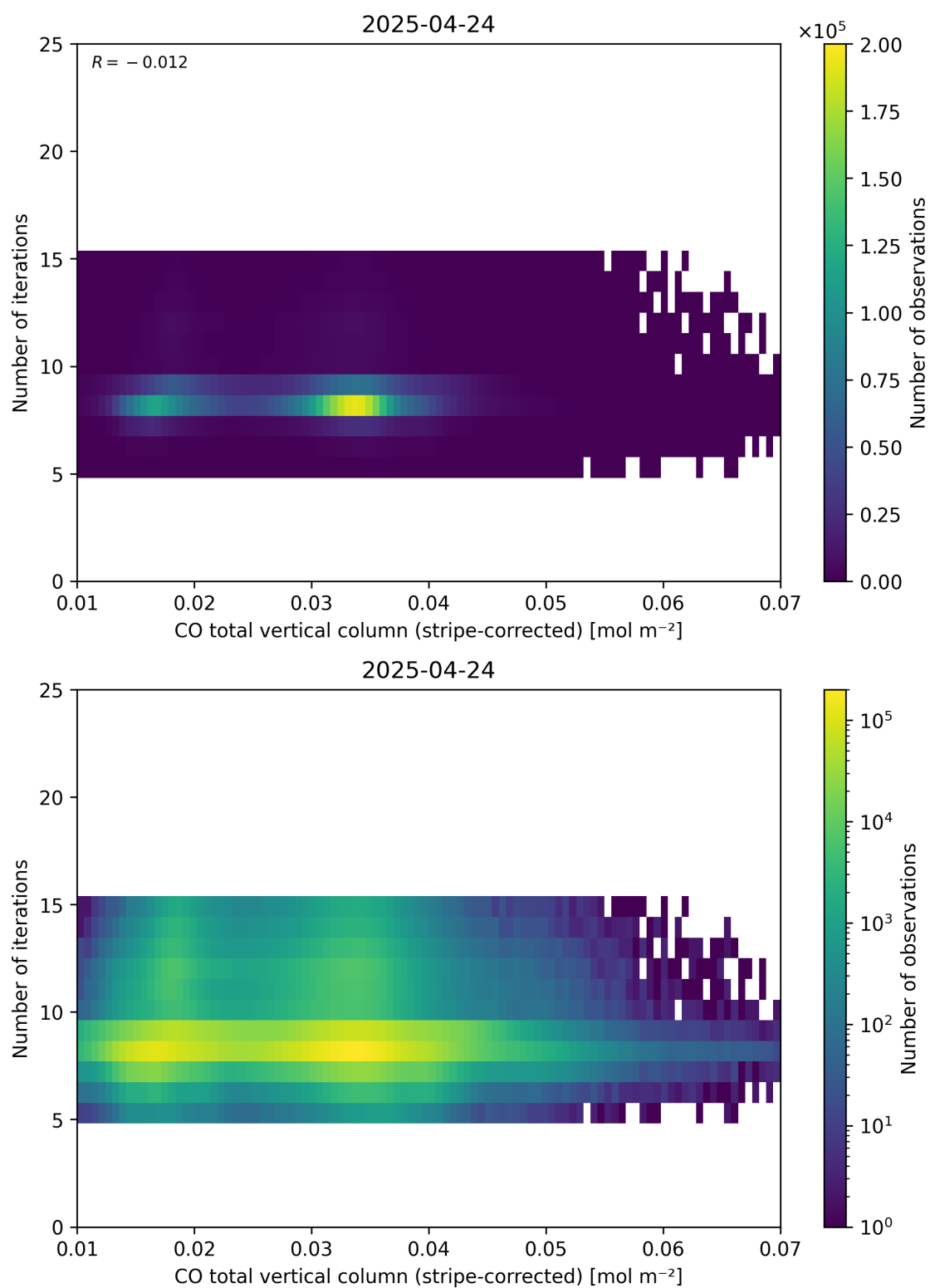
Figure 39: Scatter density plot of “CO total vertical column (stripe-corrected)” against “Number of iterations” for 2025-04-24 to 2025-04-25.
