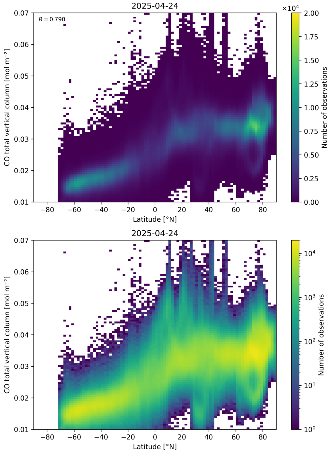
Figure 51: Scatter density plot of “Latitude” against “CO total vertical column” for 2025-04-24 to 2025-04-25.
