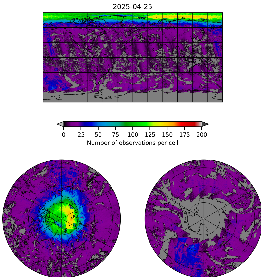
Figure 8: Map of the number of observations for 2025-04-24 to 2025-04-26
