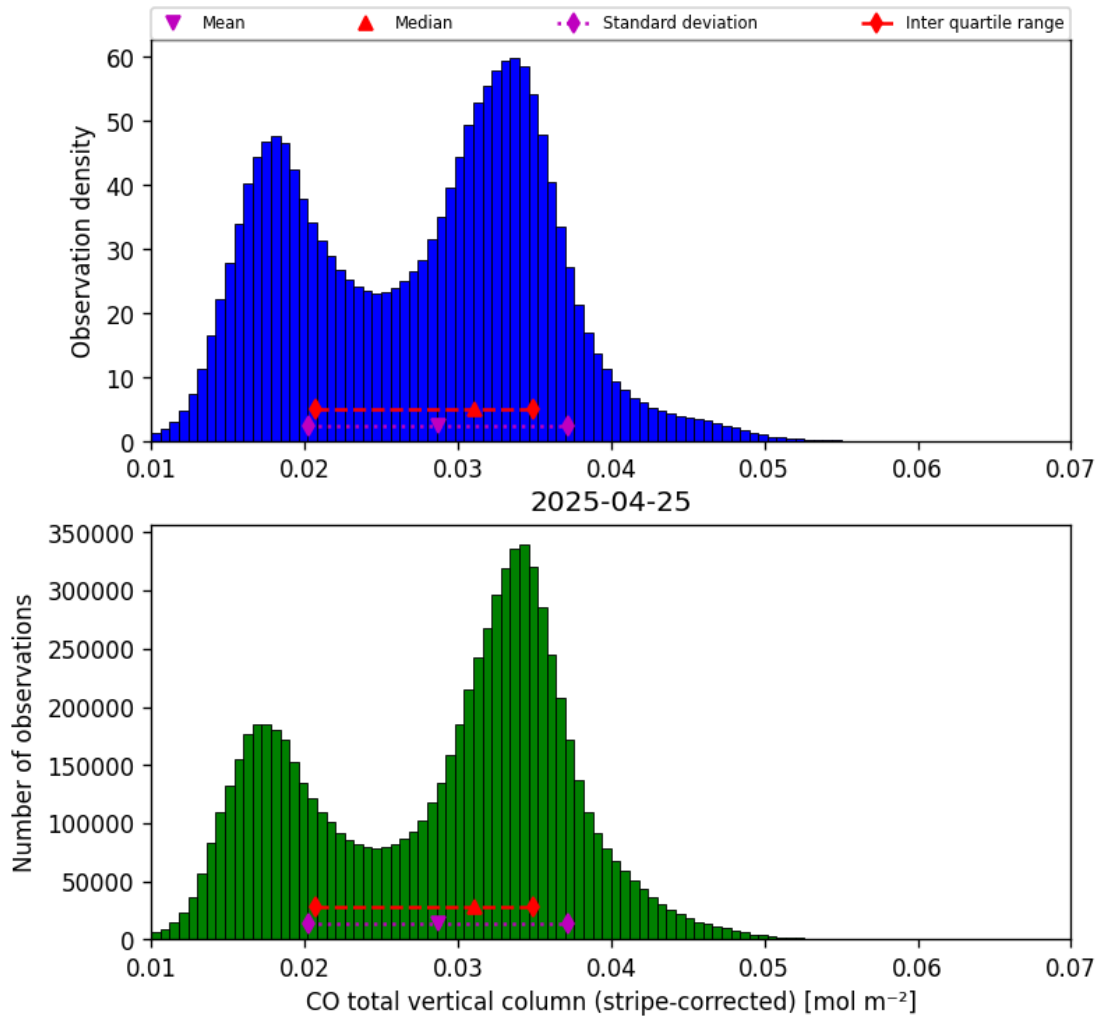
Figure 19: Histogram of “CO total vertical column (stripe-corrected)” for 2025-04-24 to 2025-04-26
