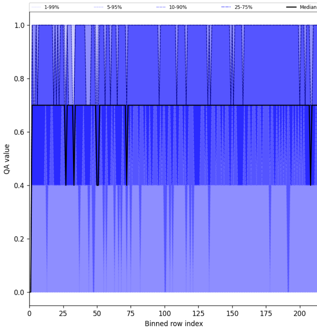
Figure 25: Along track statistics of “QA value” for 2025-04-24 to 2025-04-26
