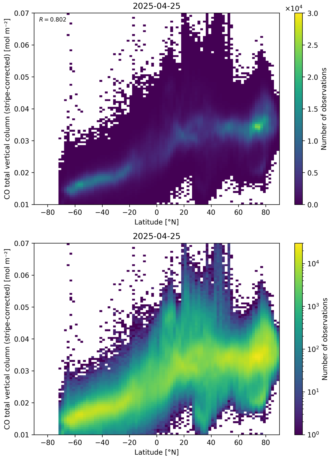
Figure 52: Scatter density plot of “Latitude” against “CO total vertical column (stripe-corrected)” for 2025-04-24 to 2025-04-26.
