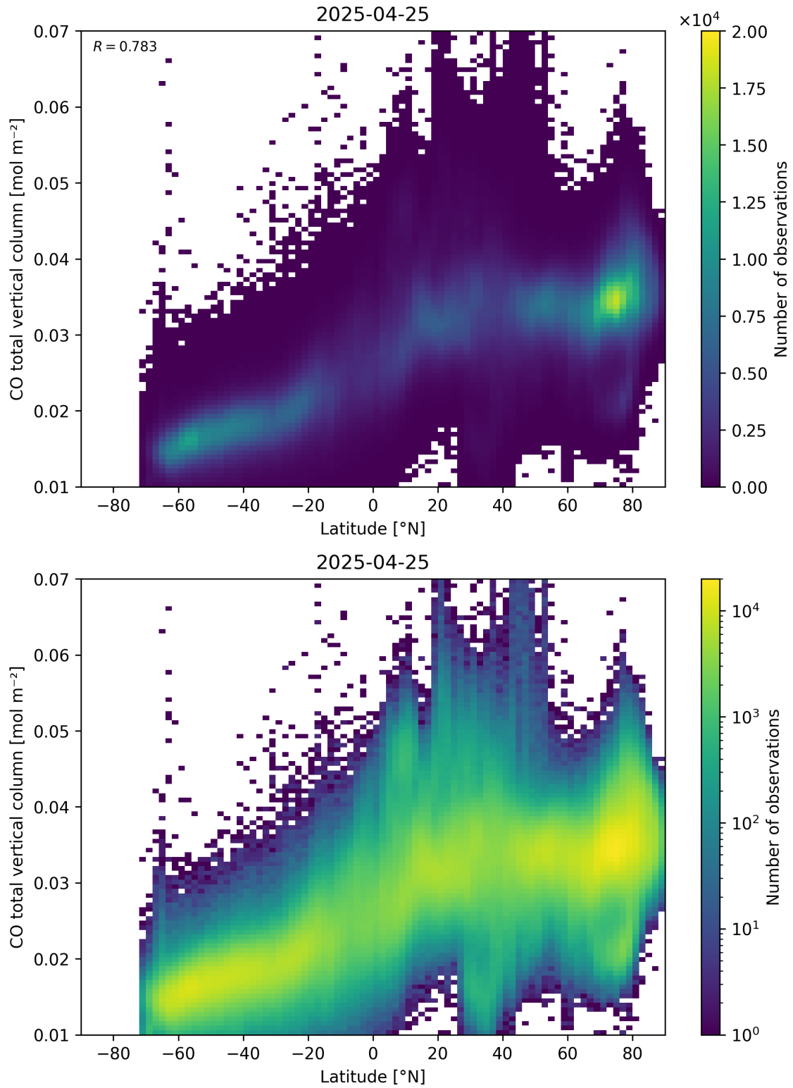
Figure 51: Scatter density plot of “Latitude” against “CO total vertical column” for 2025-04-24 to 2025-04-26.
