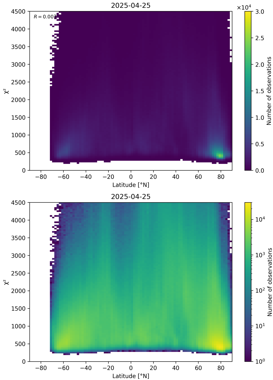
Figure 54: Scatter density plot of “Latitude” against “ \chi^2 ” for 2025-04-24 to 2025-04-26.
