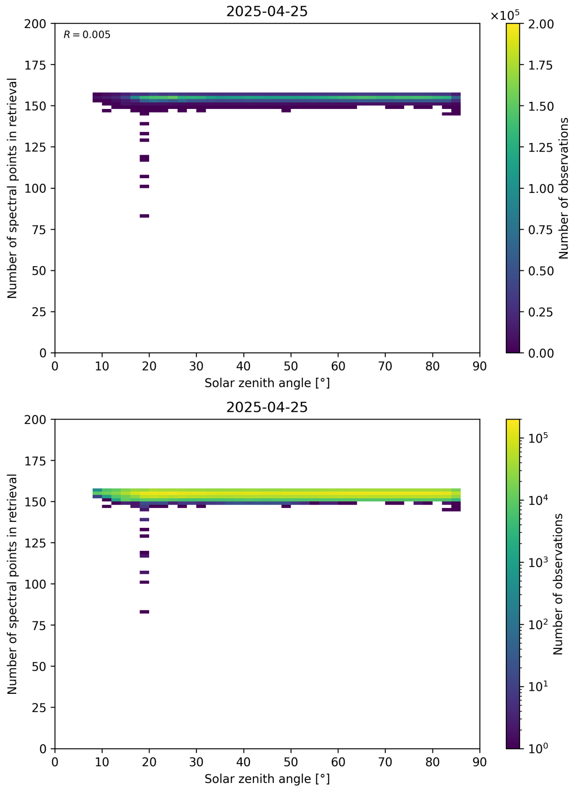
Figure 68: Scatter density plot of “Solar zenith angle” against “Number of spectral points in retrieval” for 2025-04-24 to 2025-04-26.
