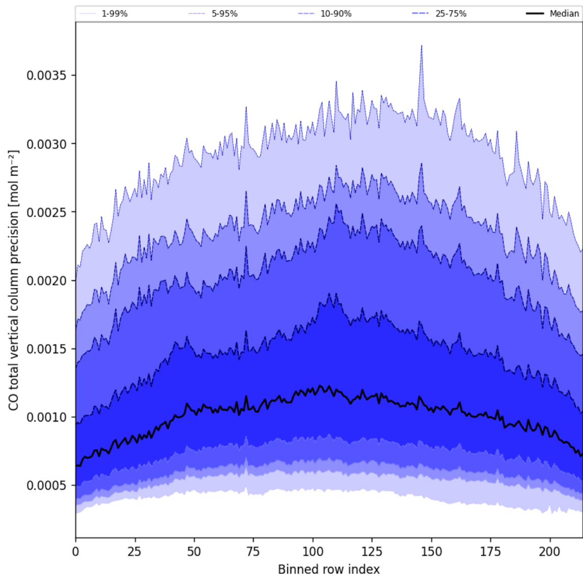
Figure 28: Along track statistics of “CO total vertical column precision” for 2025-04-24 to 2025-04-26
