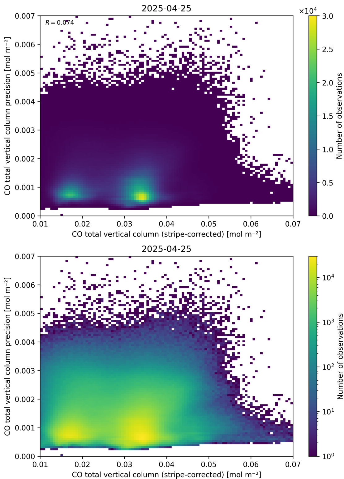
Figure 36: Scatter density plot of “CO total vertical column (stripe-corrected)” against “CO total vertical column precision” for 2025-04-24 to 2025-04-26.
