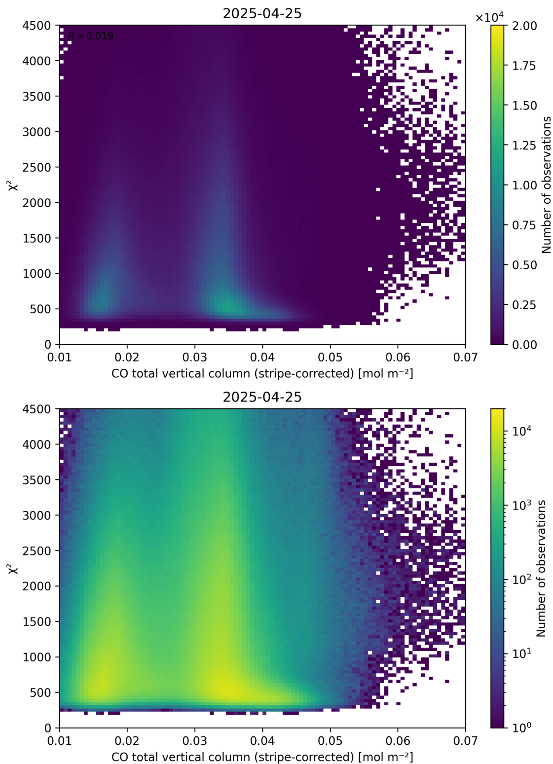
Figure 37: Scatter density plot of “CO total vertical column (stripe-corrected)” against “ \chi^2 ” for 2025-04-24 to 2025-04-26.
