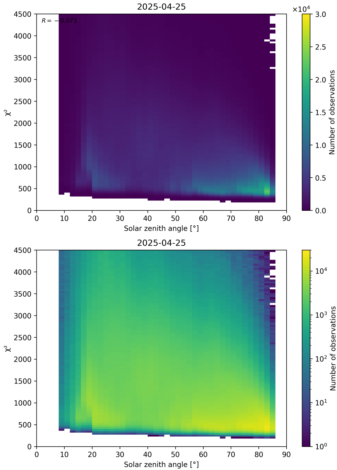
Figure 64: Scatter density plot of “Solar zenith angle” against “ \chi^2 ” for 2025-04-24 to 2025-04-26.
