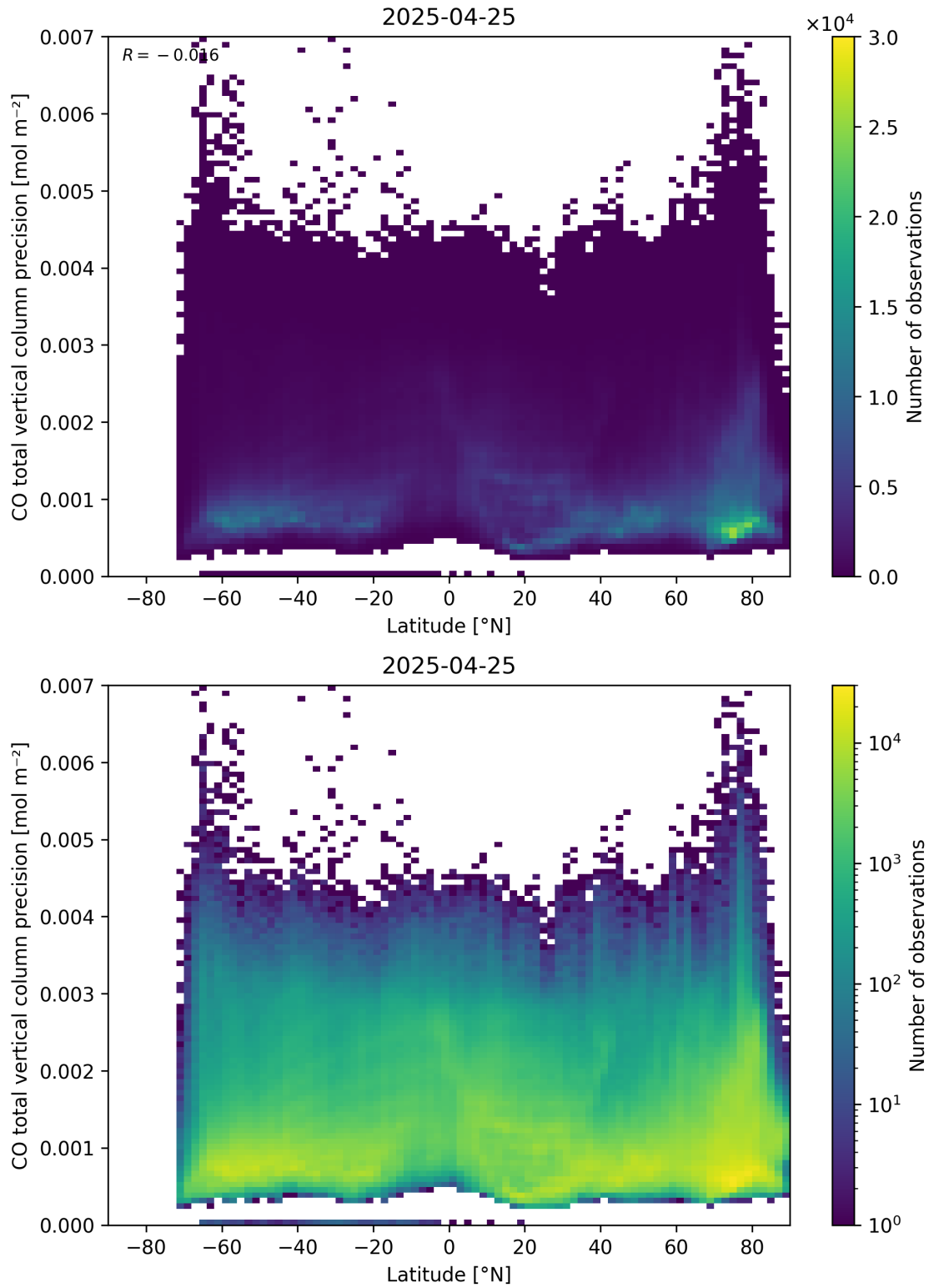
Figure 53: Scatter density plot of “Latitude” against “CO total vertical column precision” for 2025-04-24 to 2025-04-26.
