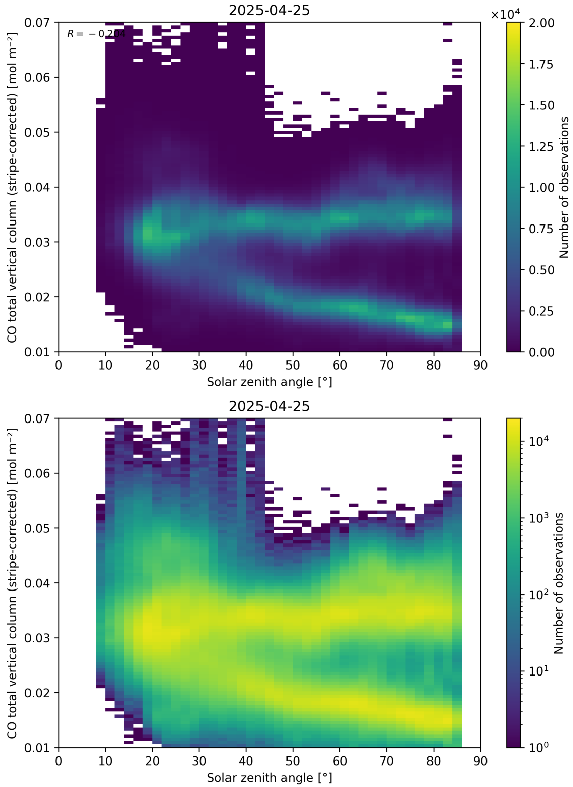
Figure 62: Scatter density plot of “Solar zenith angle” against “CO total vertical column (stripe-corrected)” for 2025-04-24 to 2025-04-26.
