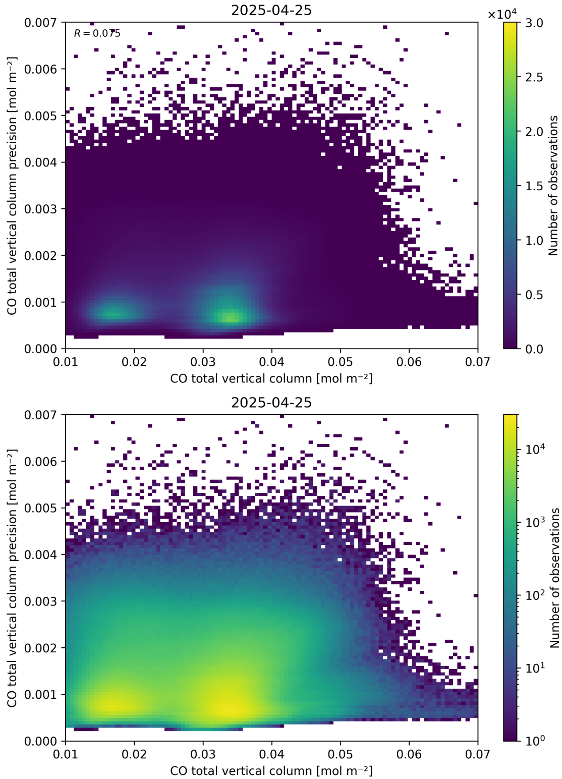
Figure 34: Scatter density plot of “CO total vertical column” against “CO total vertical column precision” for 2025-04-24 to 2025-04-26.
