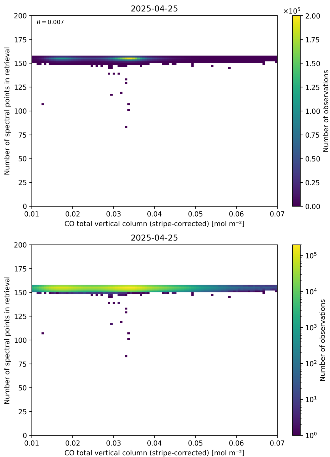
Figure 40: Scatter density plot of “CO total vertical column (stripe-corrected)” against “Number of spectral points in retrieval” for 2025-04-24 to 2025-04-26.
