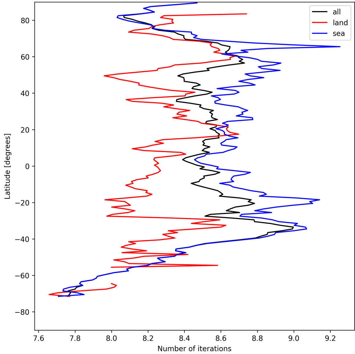
Figure 16: Zonal average of “Number of iterations” for 2025-04-24 to 2025-04-26.
