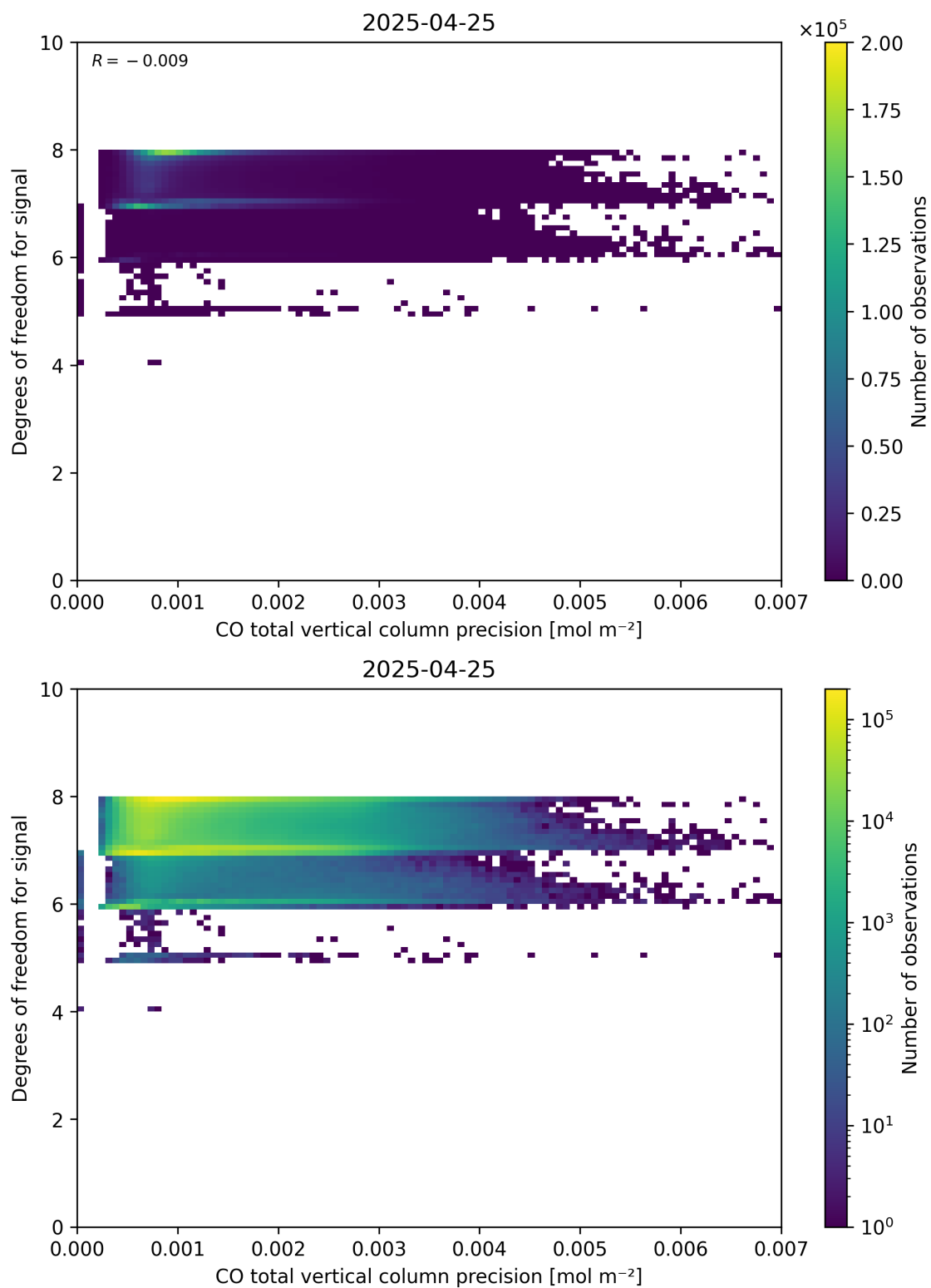
Figure 45: Scatter density plot of “CO total vertical column precision” against “Degrees of freedom for signal” for 2025-04-24 to 2025-04-26.
