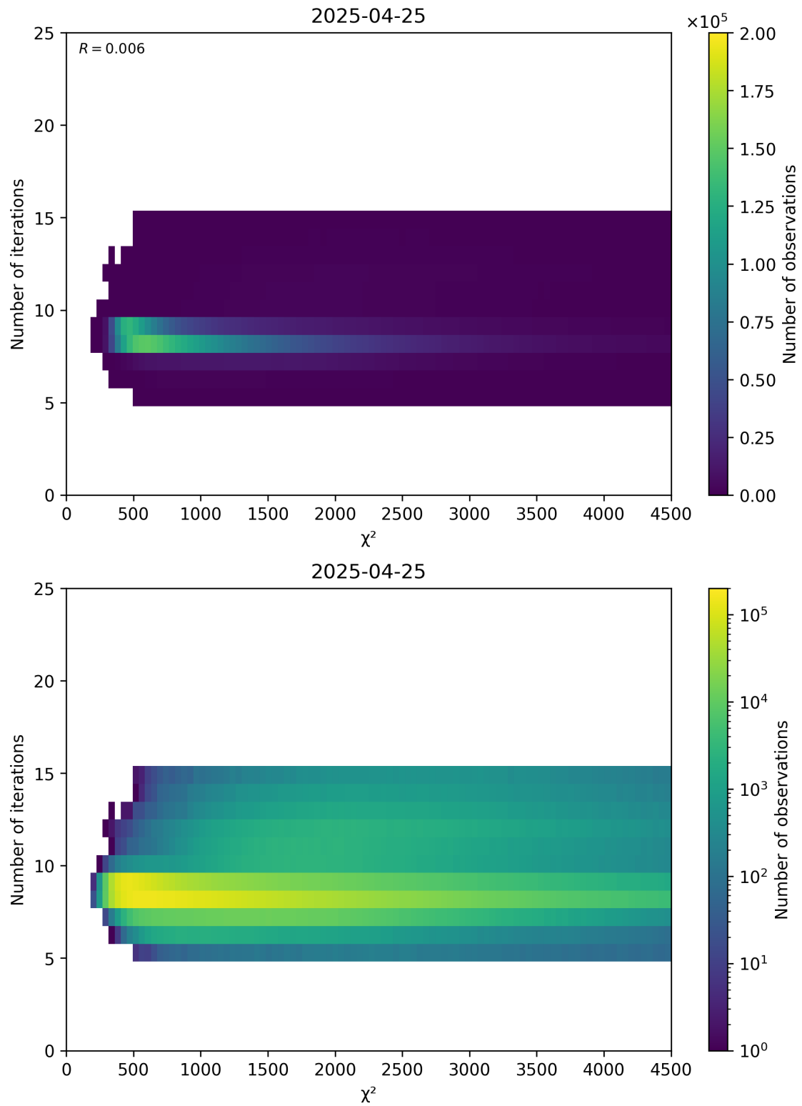
Figure 49: Scatter density plot of “ \chi^2 ” against “Number of iterations” for 2025-04-24 to 2025-04-26.
