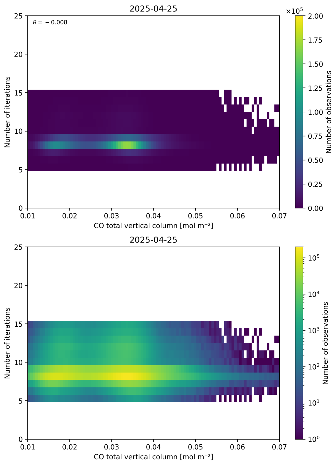
Figure 42: Scatter density plot of “CO total vertical column” against “Number of iterations” for 2025-04-24 to 2025-04-26.
