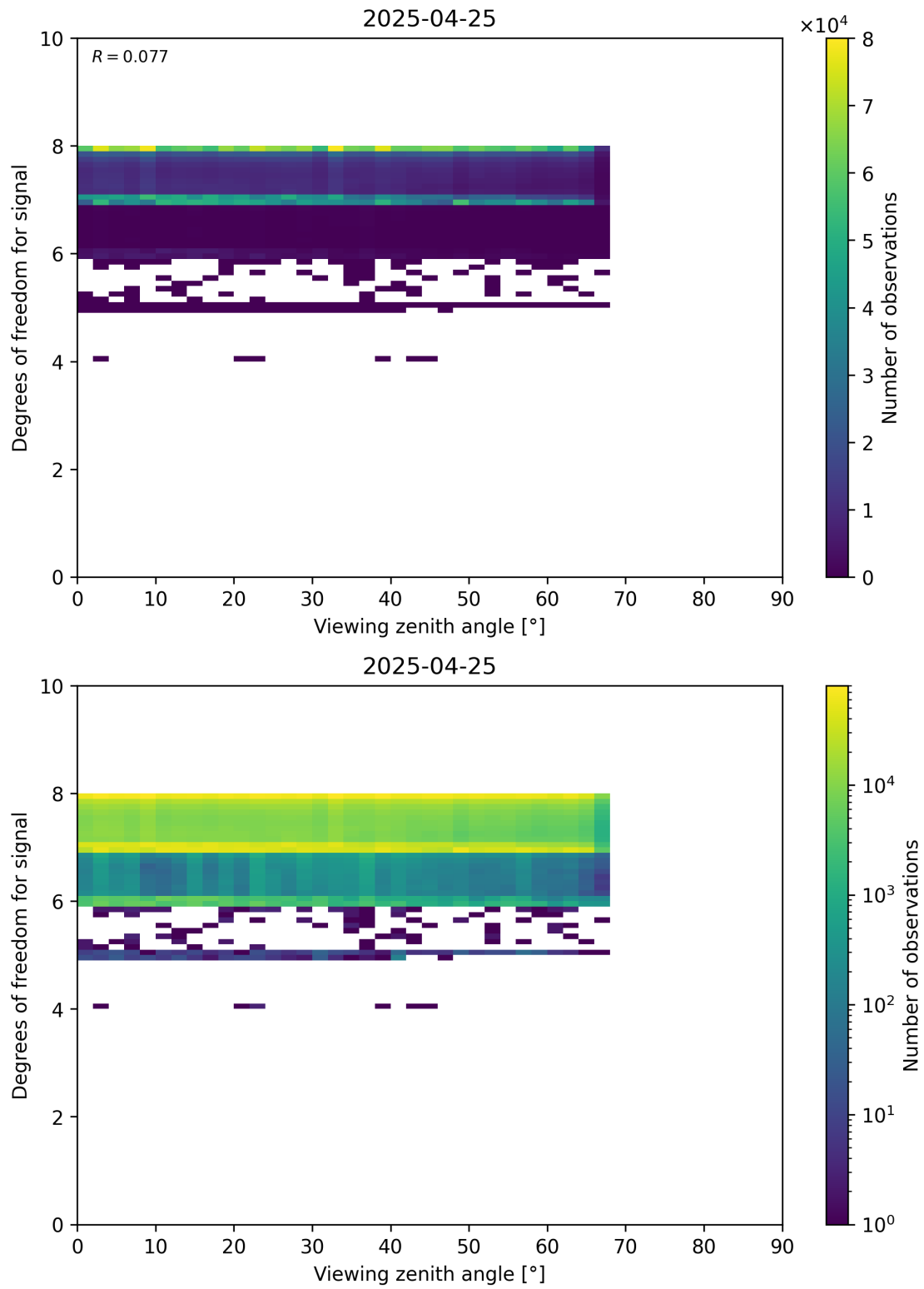
Figure 73: Scatter density plot of “Viewing zenith angle” against “Degrees of freedom for signal” for 2025-04-24 to 2025-04-26.
