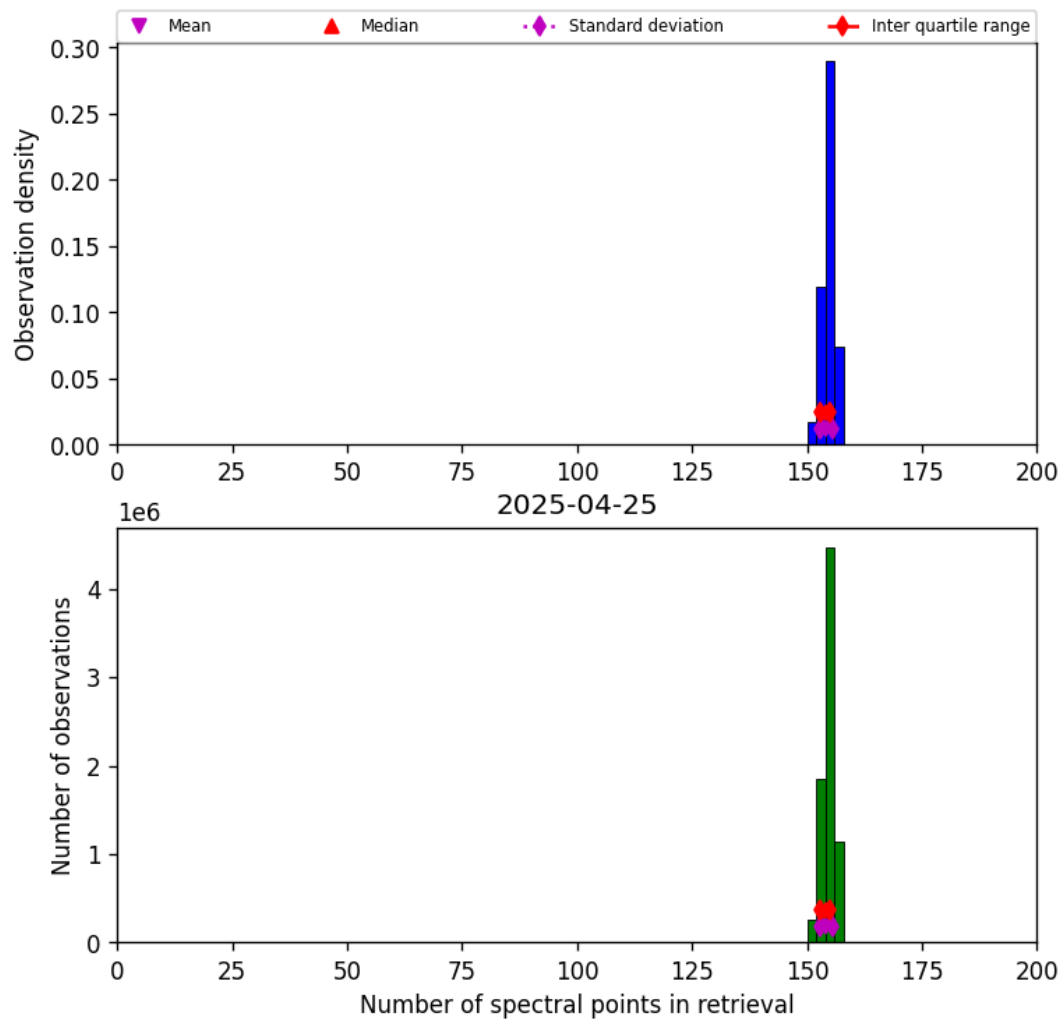
Figure 21: Histogram of “Number of spectral points in retrieval” for 2025-04-24 to 2025-04-26
