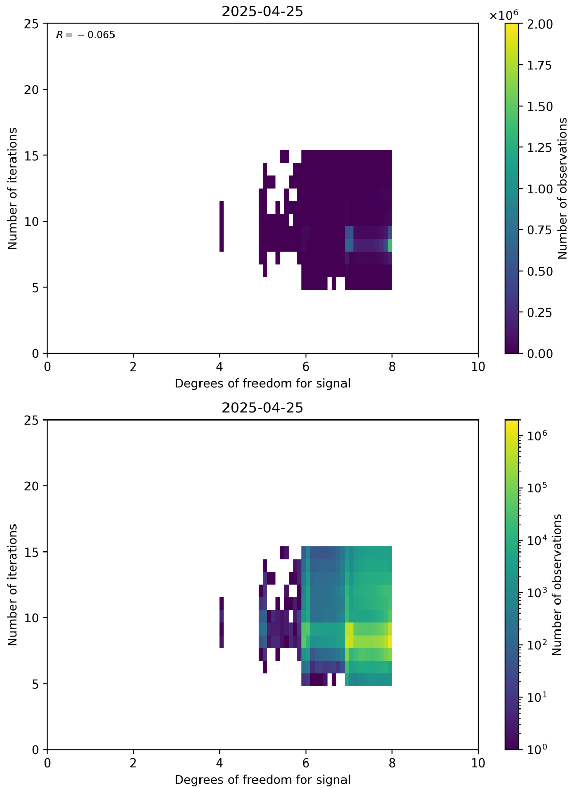
Figure 50: Scatter density plot of “Degrees of freedom for signal” against “Number of iterations” for 2025-04-24 to 2025-04-26.
