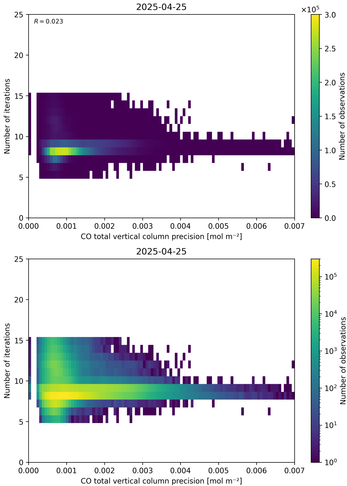
Figure 46: Scatter density plot of “CO total vertical column precision” against “Number of iterations” for 2025-04-24 to 2025-04-26.
