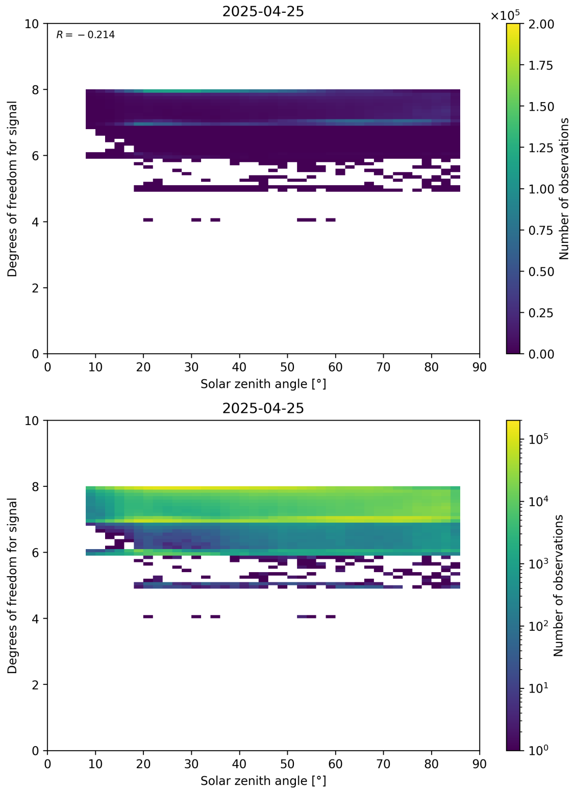
Figure 65: Scatter density plot of “Solar zenith angle” against “Degrees of freedom for signal” for 2025-04-24 to 2025-04-26.
