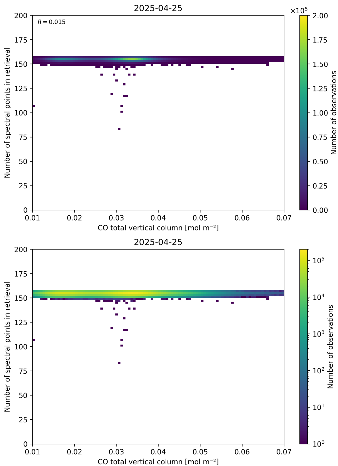
Figure 43: Scatter density plot of “CO total vertical column” against “Number of spectral points in retrieval” for 2025-04-24 to 2025-04-26.
