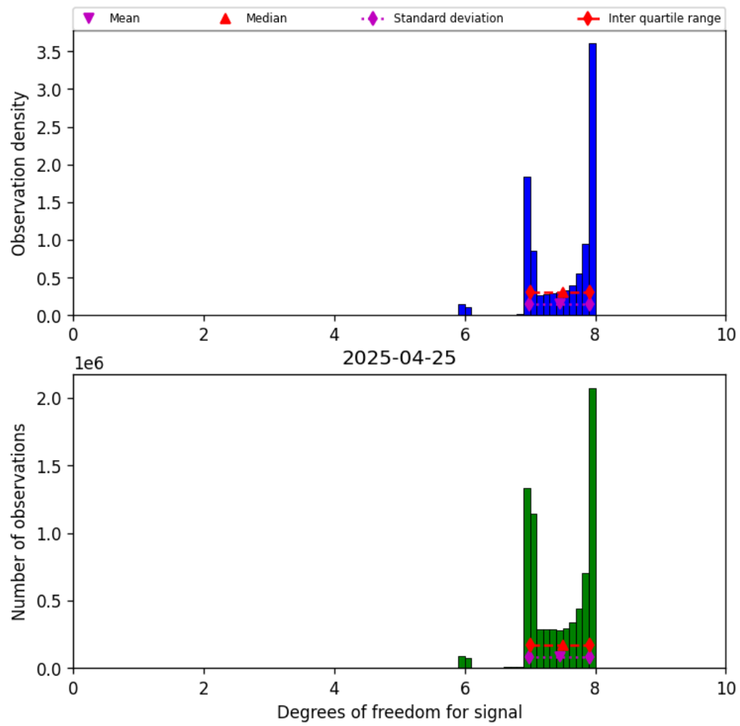
Figure 23: Histogram of “Degrees of freedom for signal” for 2025-04-24 to 2025-04-26
