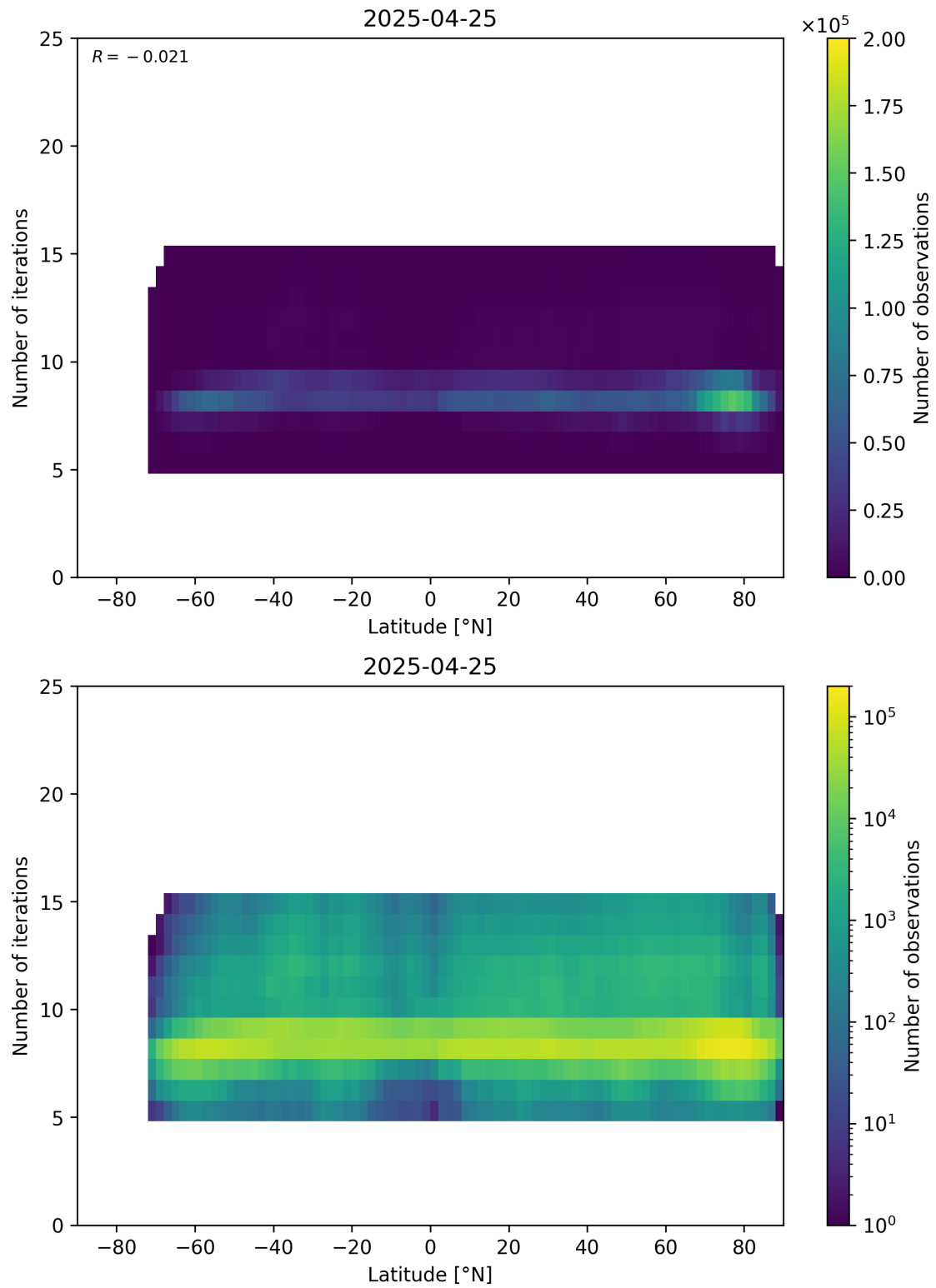
Figure 56: Scatter density plot of “Latitude” against “Number of iterations” for 2025-04-24 to 2025-04-26.
