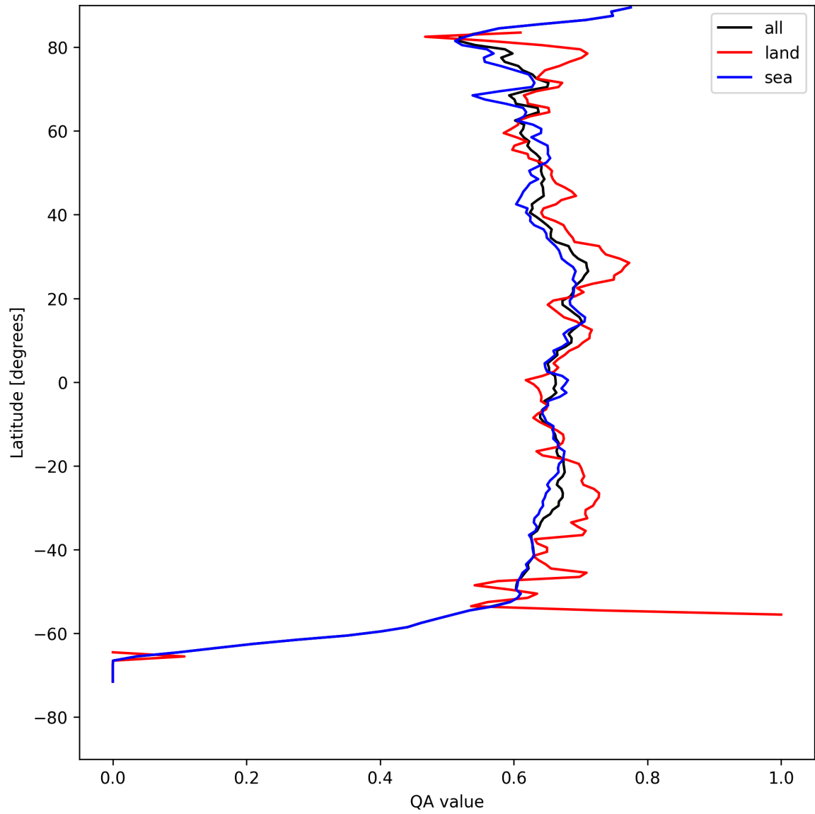
Figure 9: Zonal average of “QA value” for 2025-04-24 to 2025-04-26.
