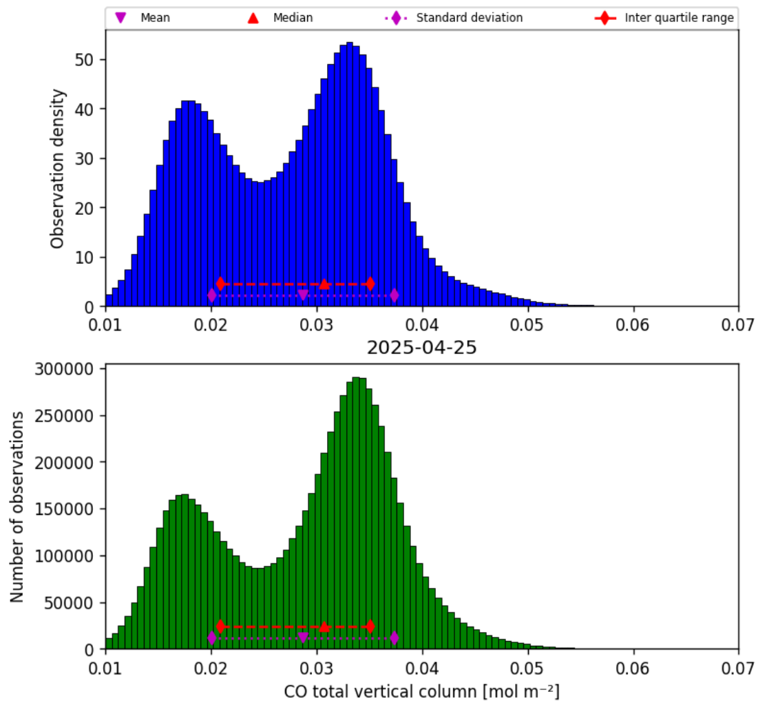
Figure 18: Histogram of “CO total vertical column” for 2025-04-24 to 2025-04-26
