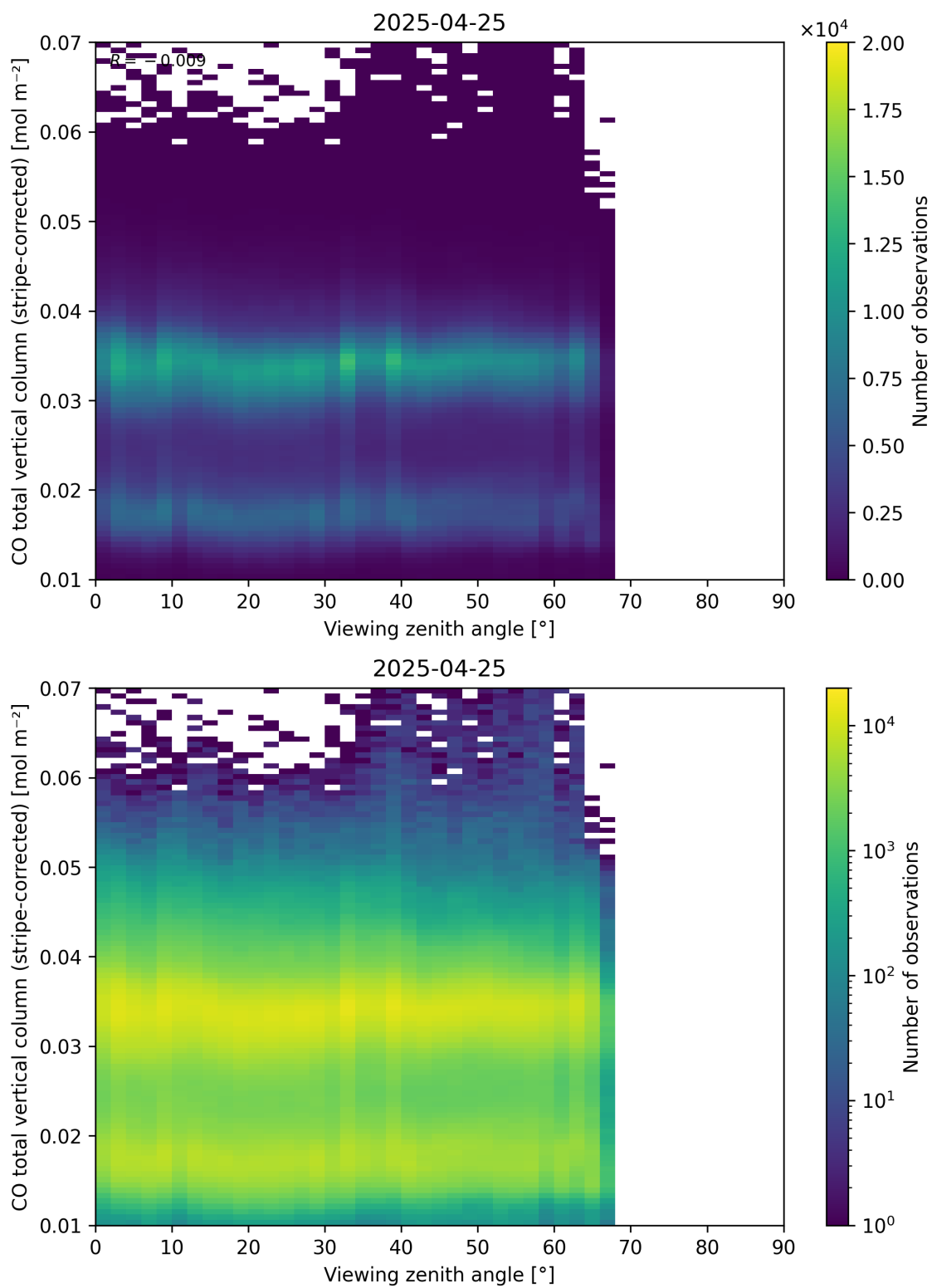
Figure 70: Scatter density plot of “Viewing zenith angle” against “CO total vertical column (stripe-corrected)” for 2025-04-24 to 2025-04-26.
