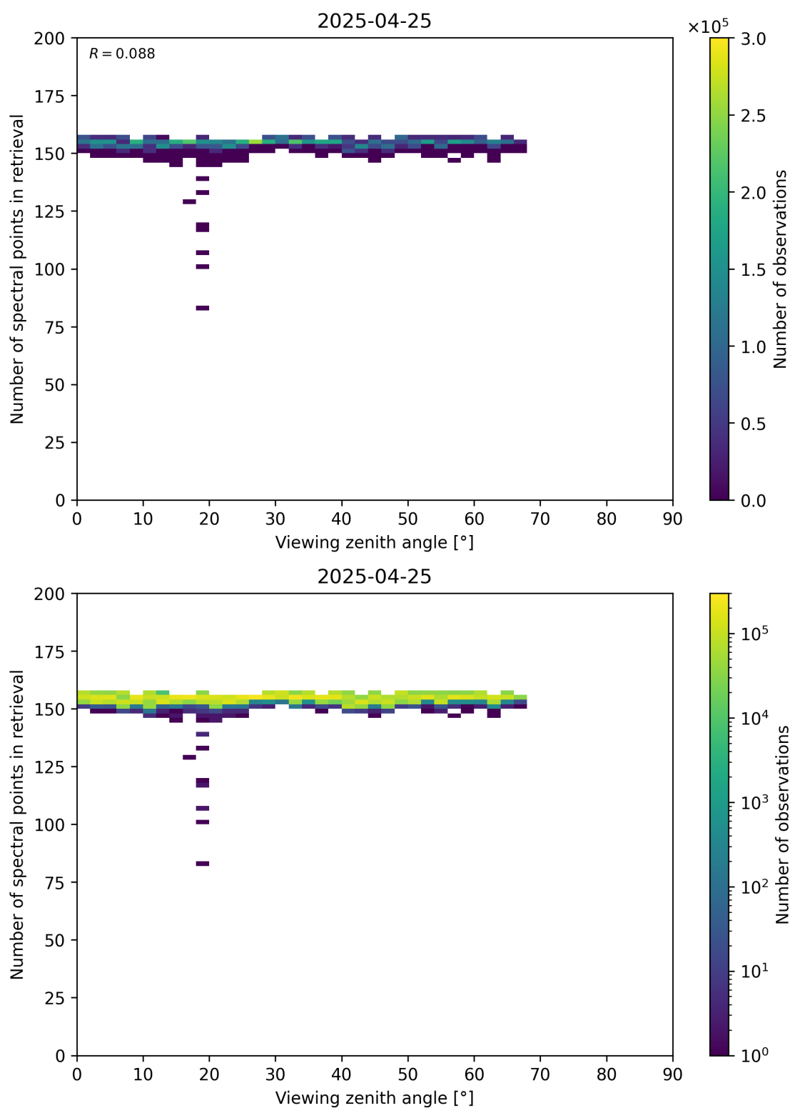
Figure 76: Scatter density plot of “Viewing zenith angle” against “Number of spectral points in retrieval” for 2025-04-24 to 2025-04-26.
