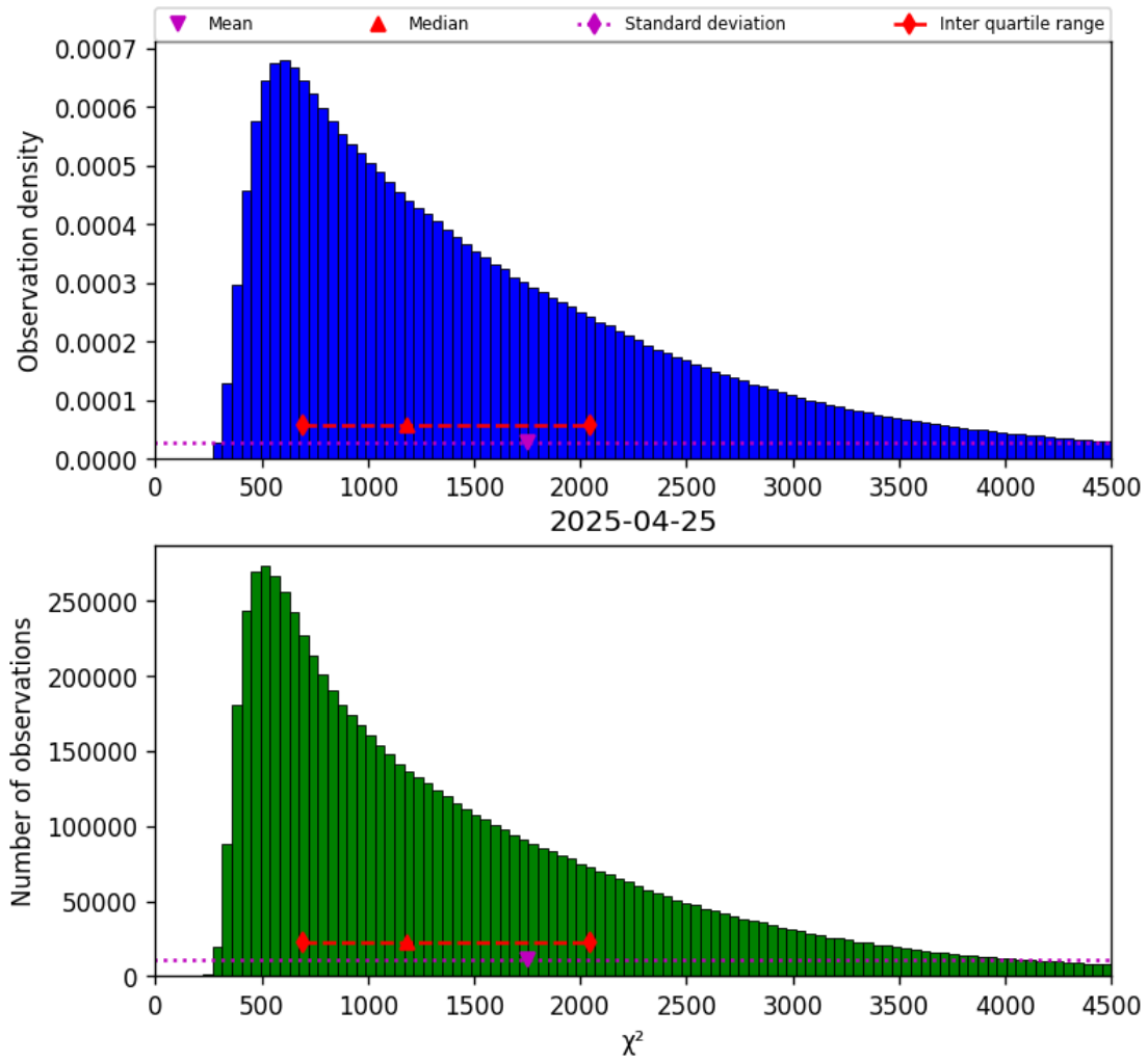
Figure 22: Histogram of “ \chi^2 ” for 2025-04-24 to 2025-04-26
