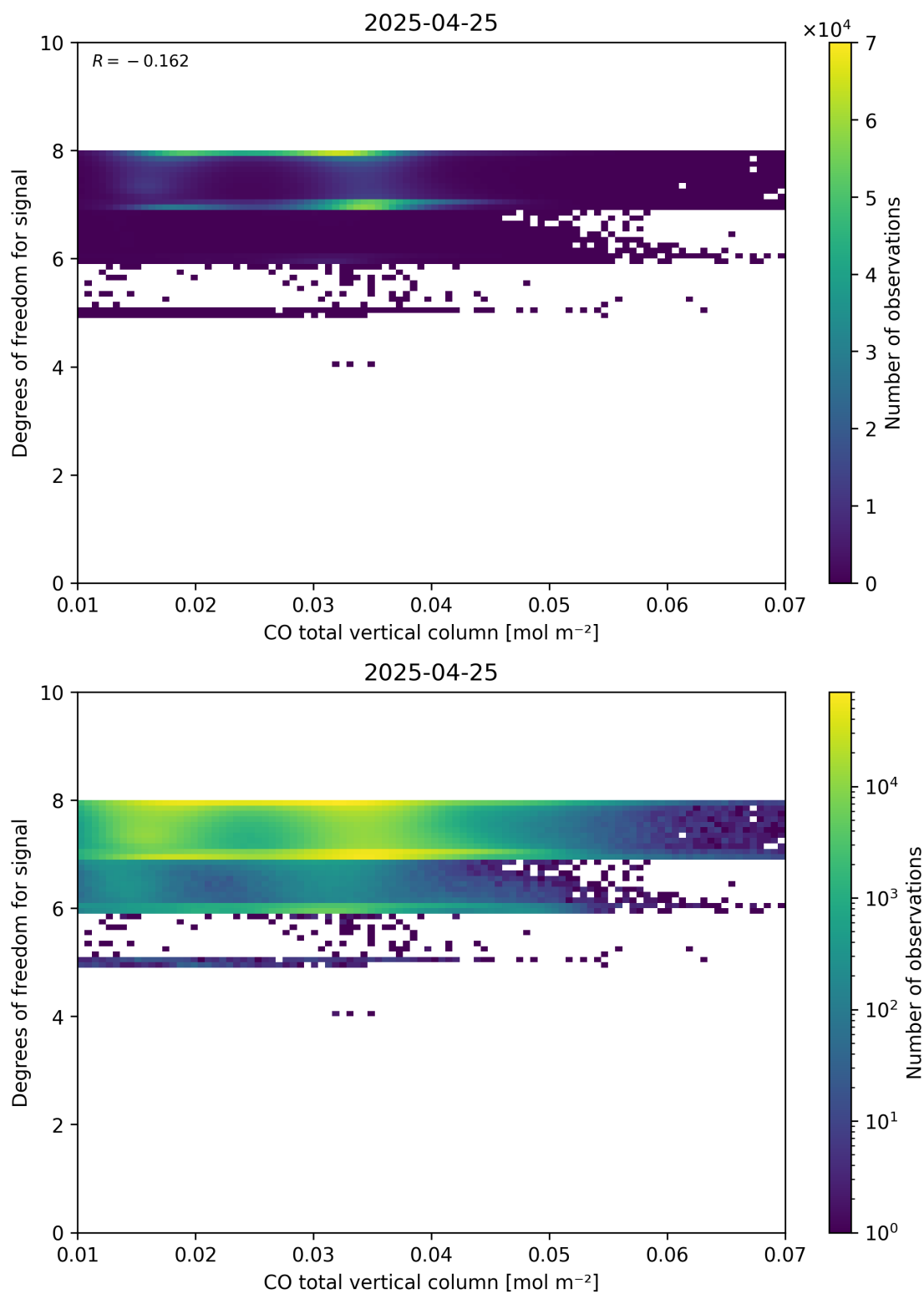
Figure 41: Scatter density plot of “CO total vertical column” against “Degrees of freedom for signal” for 2025-04-24 to 2025-04-26.
