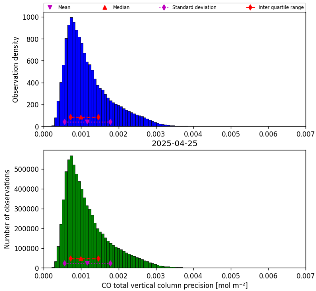
Figure 20: Histogram of “CO total vertical column precision” for 2025-04-24 to 2025-04-26
