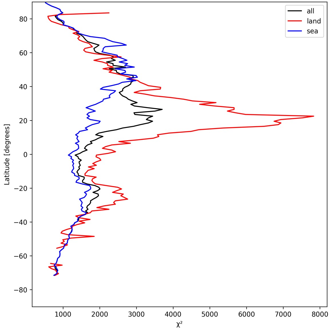
Figure 14: Zonal average of “ \chi^2 ” for 2025-04-24 to 2025-04-26.
