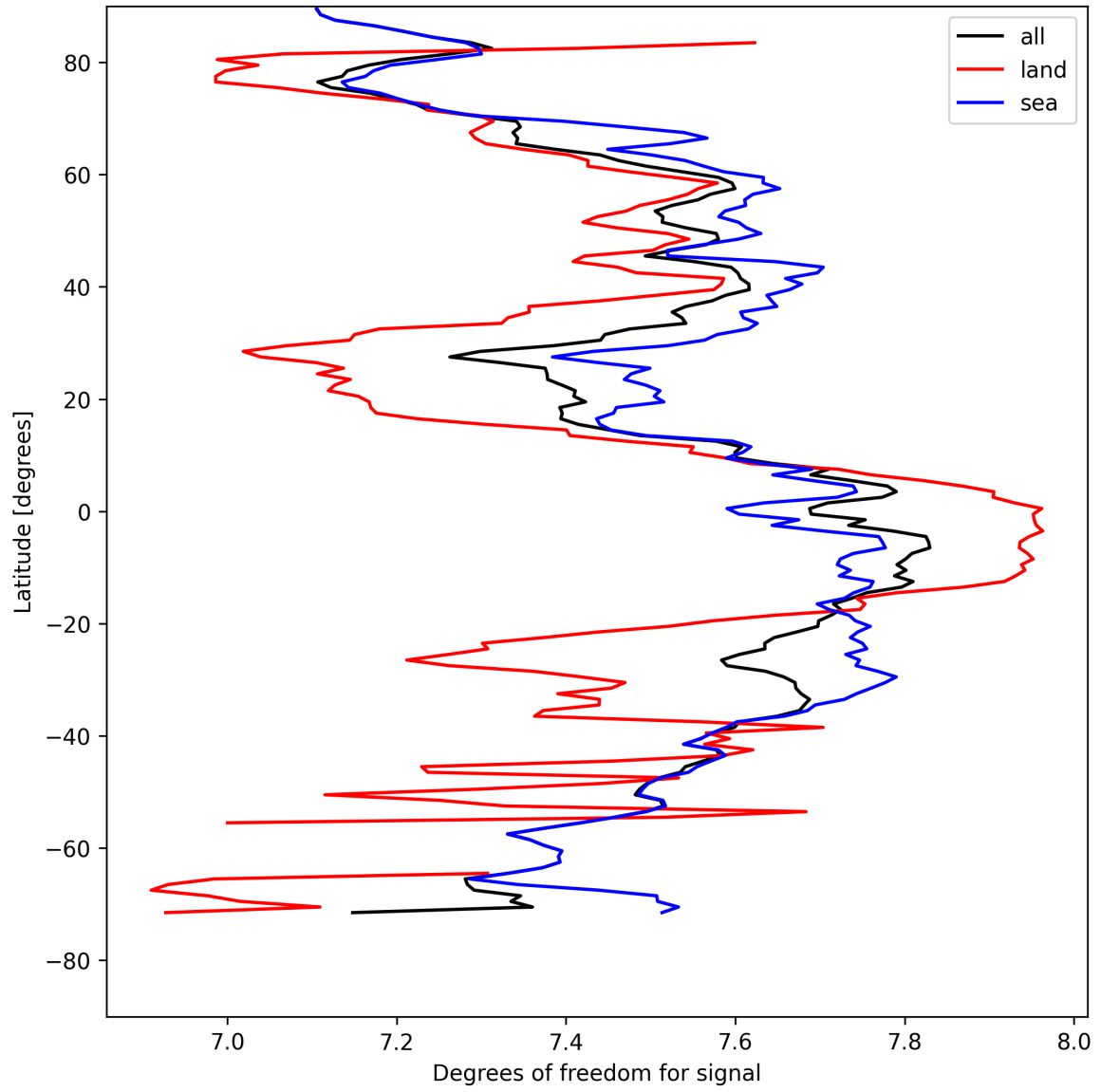
Figure 15: Zonal average of “Degrees of freedom for signal” for 2025-04-24 to 2025-04-26.
