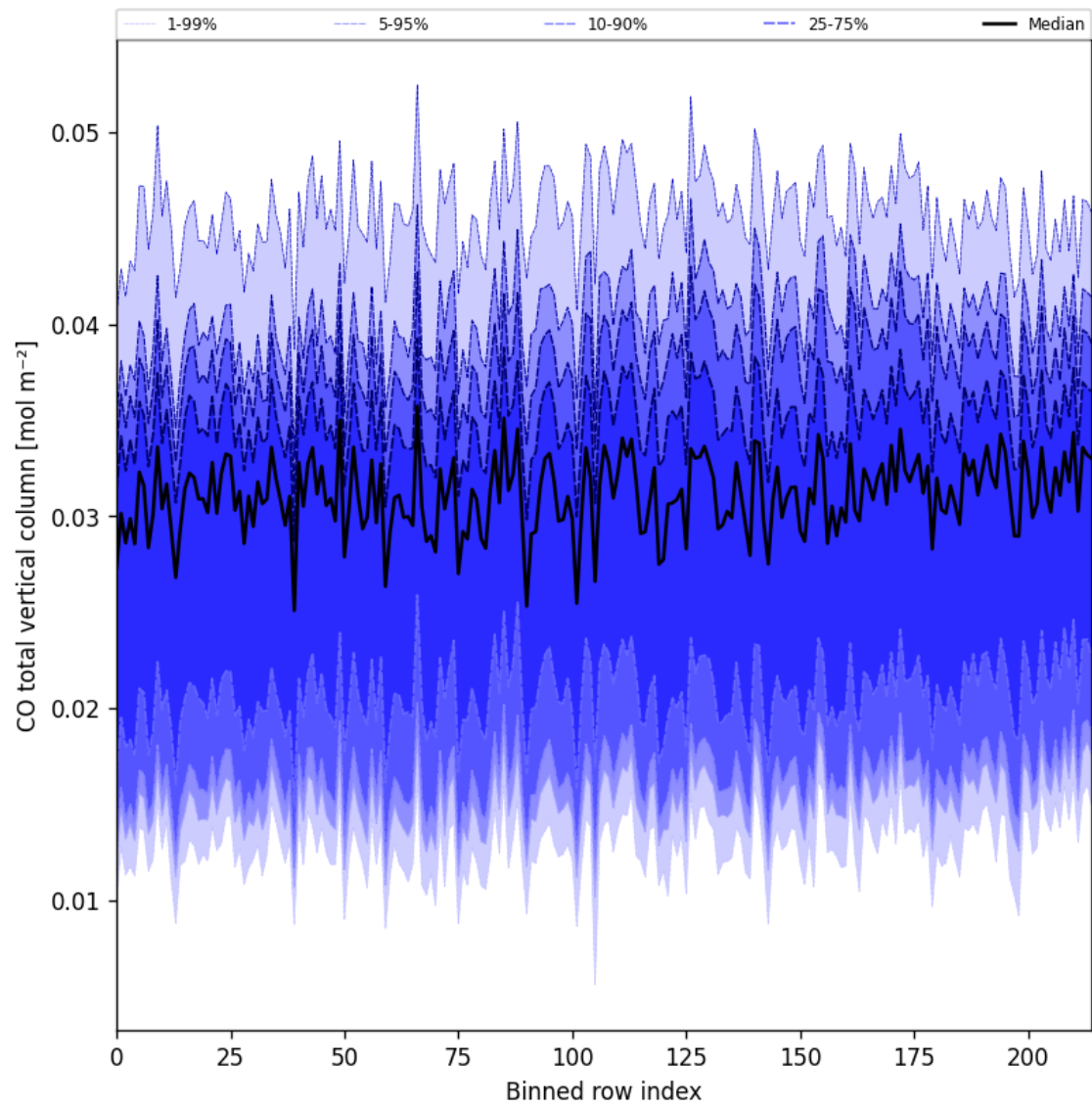
Figure 26: Along track statistics of "CO total vertical column" for 2025-04-24 to 2025-04-26
