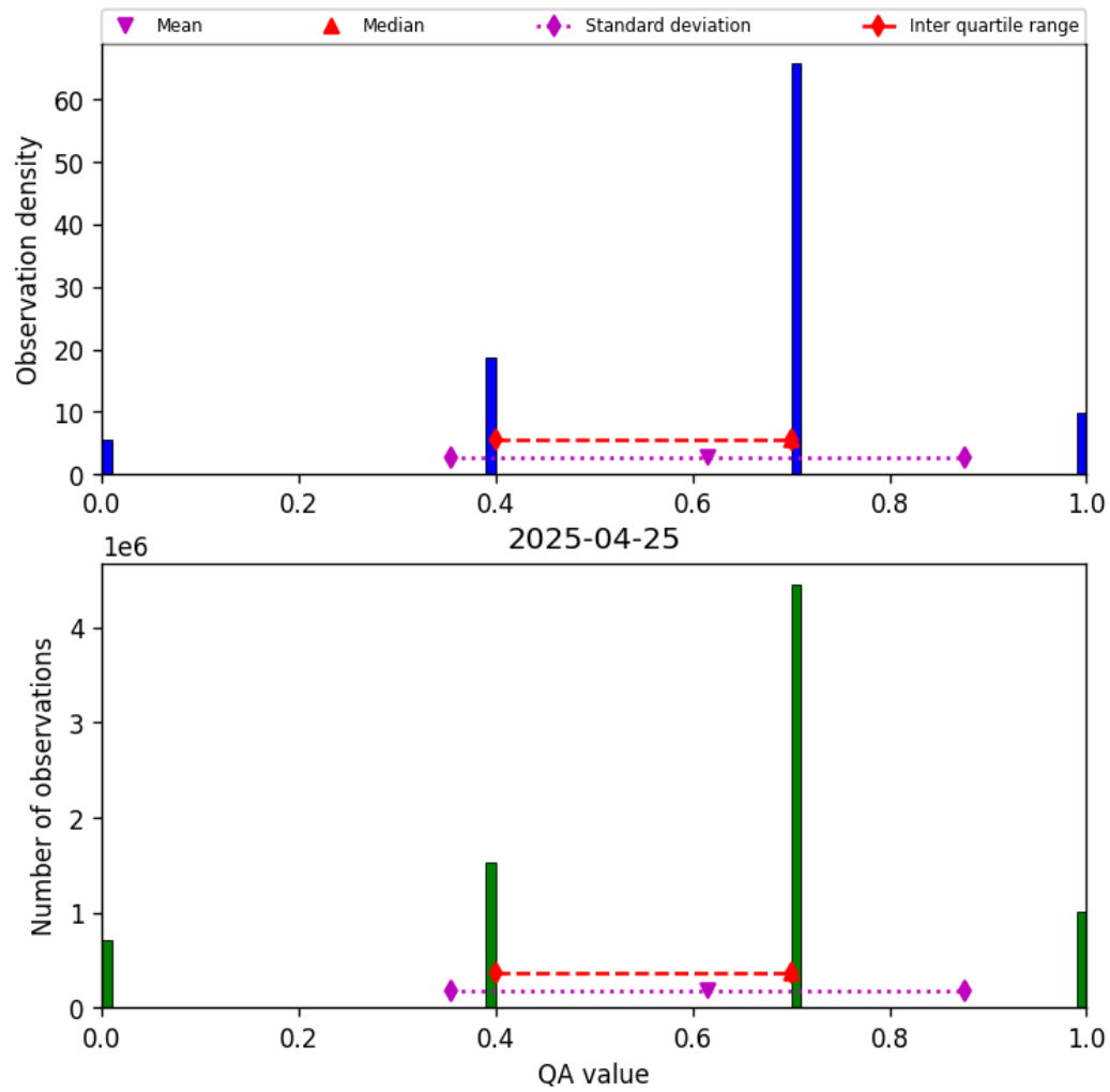
Figure 17: Histogram of “QA value” for 2025-04-24 to 2025-04-26
