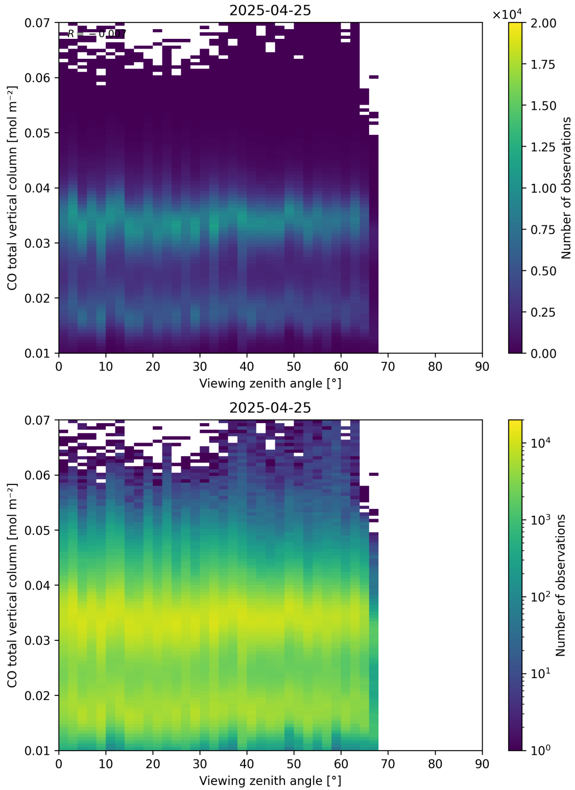
Figure 69: Scatter density plot of “Viewing zenith angle” against “CO total vertical column” for 2025-04-24 to 2025-04-26.
