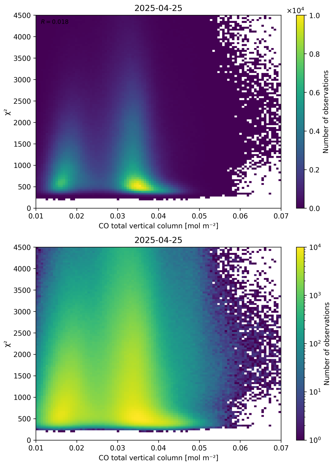
Figure 35: Scatter density plot of “CO total vertical column” against “ \chi^2 ” for 2025-04-24 to 2025-04-26.
