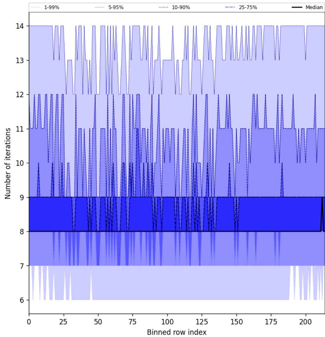
Figure 32: Along track statistics of “Number of iterations” for 2025-04-24 to 2025-04-26
