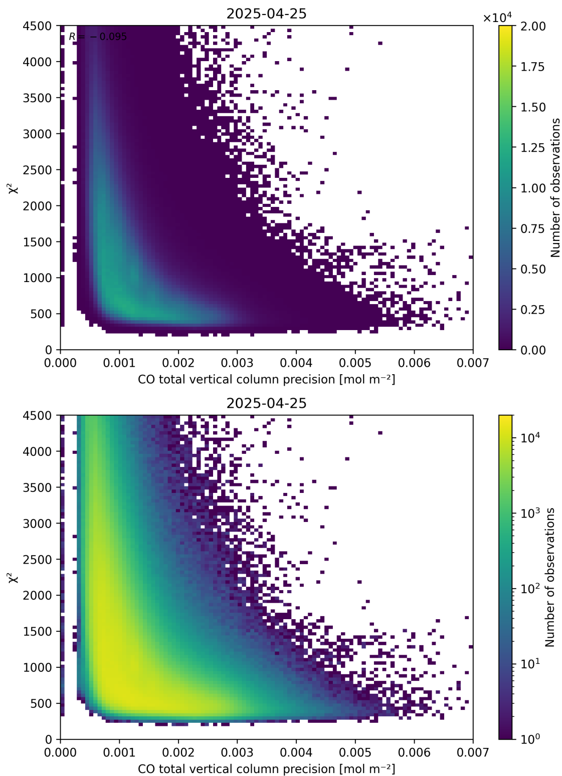
Figure 44: Scatter density plot of “CO total vertical column precision” against “ \chi^2 ” for 2025-04-24 to 2025-04-26.
