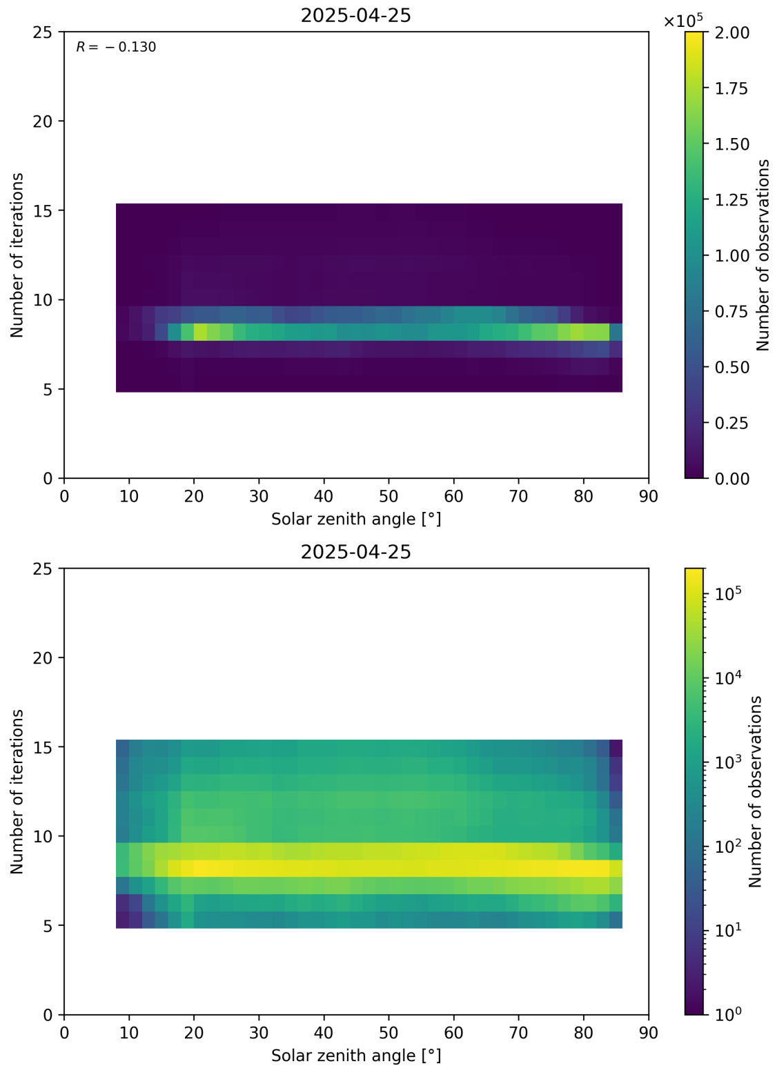
Figure 67: Scatter density plot of “Solar zenith angle” against “Number of iterations” for 2025-04-24 to 2025-04-26.
