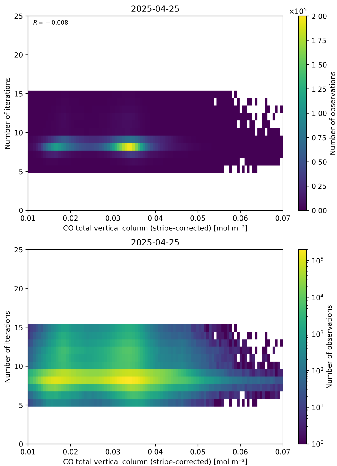
Figure 39: Scatter density plot of “CO total vertical column (stripe-corrected)” against “Number of iterations” for 2025-04-24 to 2025-04-26.
