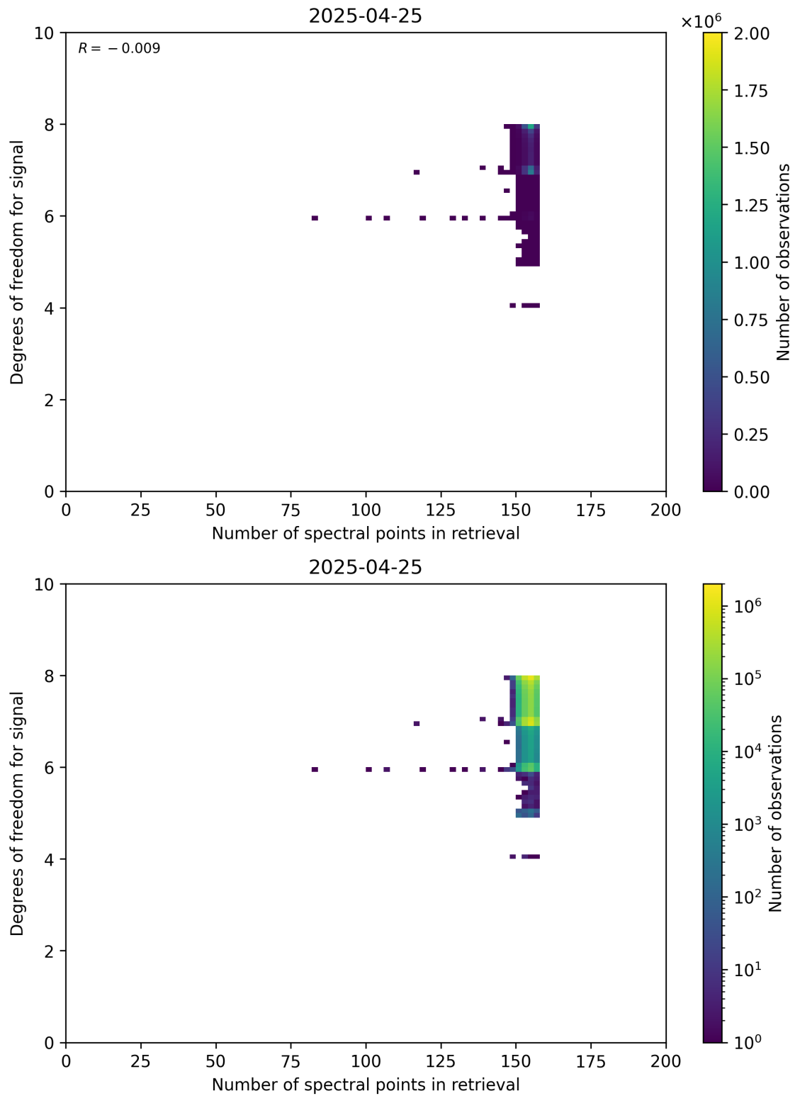
Figure 59: Scatter density plot of “Number of spectral points in retrieval” against “Degrees of freedom for signal” for 2025-04-24 to 2025-04-26.
