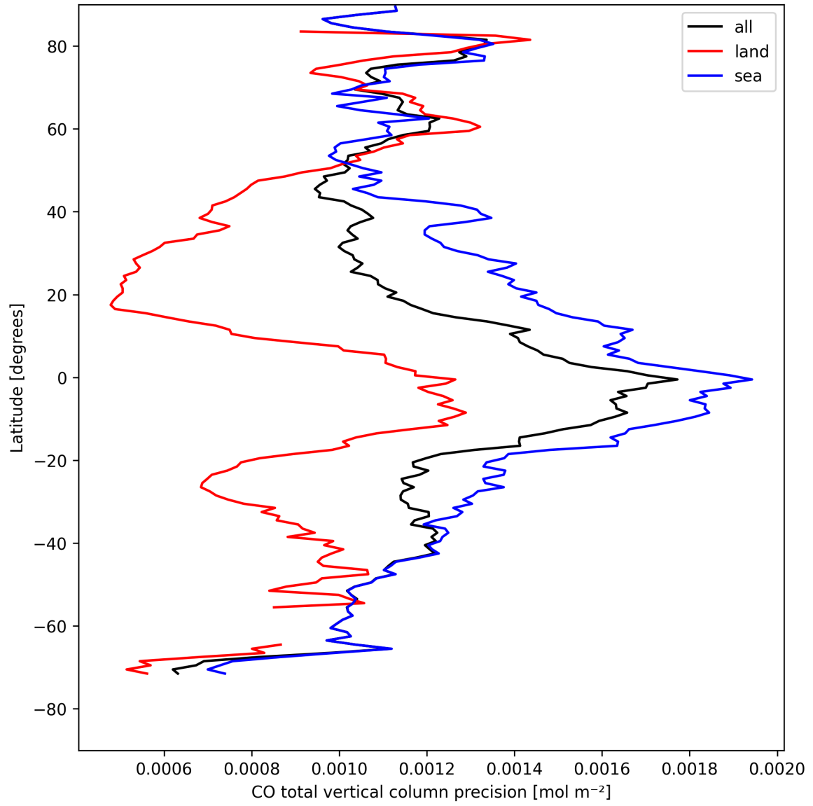
Figure 12: Zonal average of “CO total vertical column precision” for 2025-04-24 to 2025-04-26.
