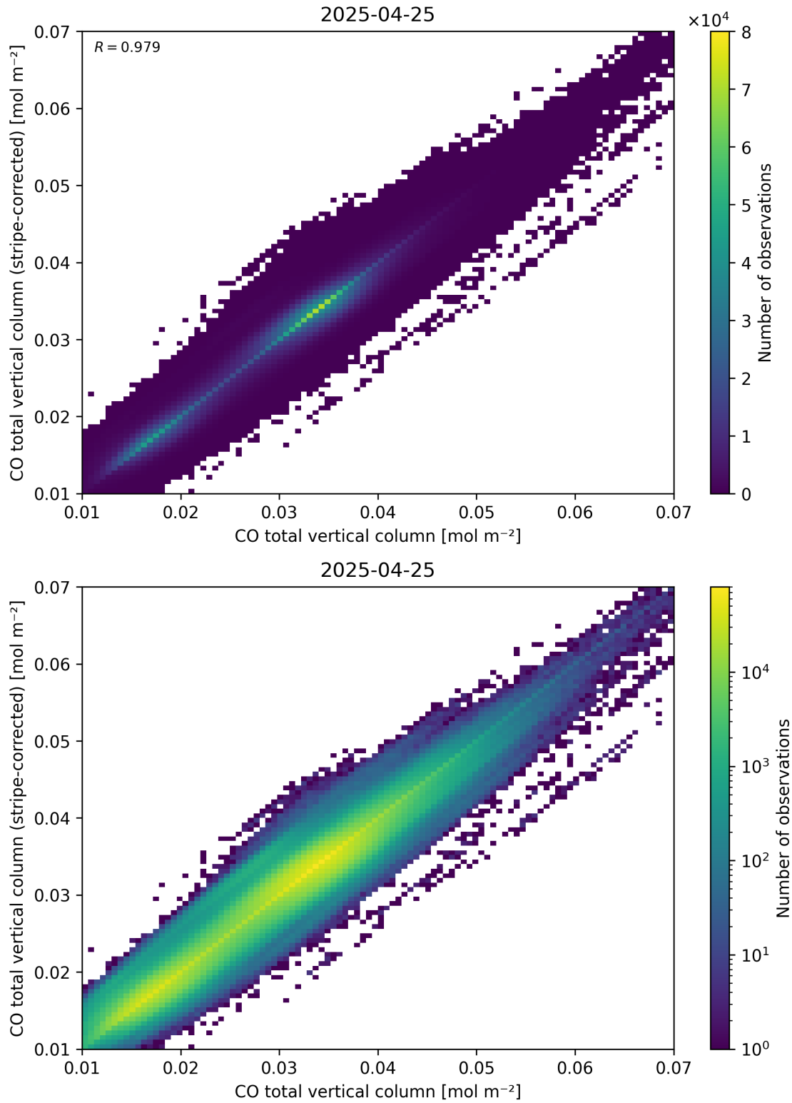
Figure 33: Scatter density plot of “CO total vertical column” against “CO total vertical column (stripe-corrected)” for 2025-04-24 to 2025-04-26.
