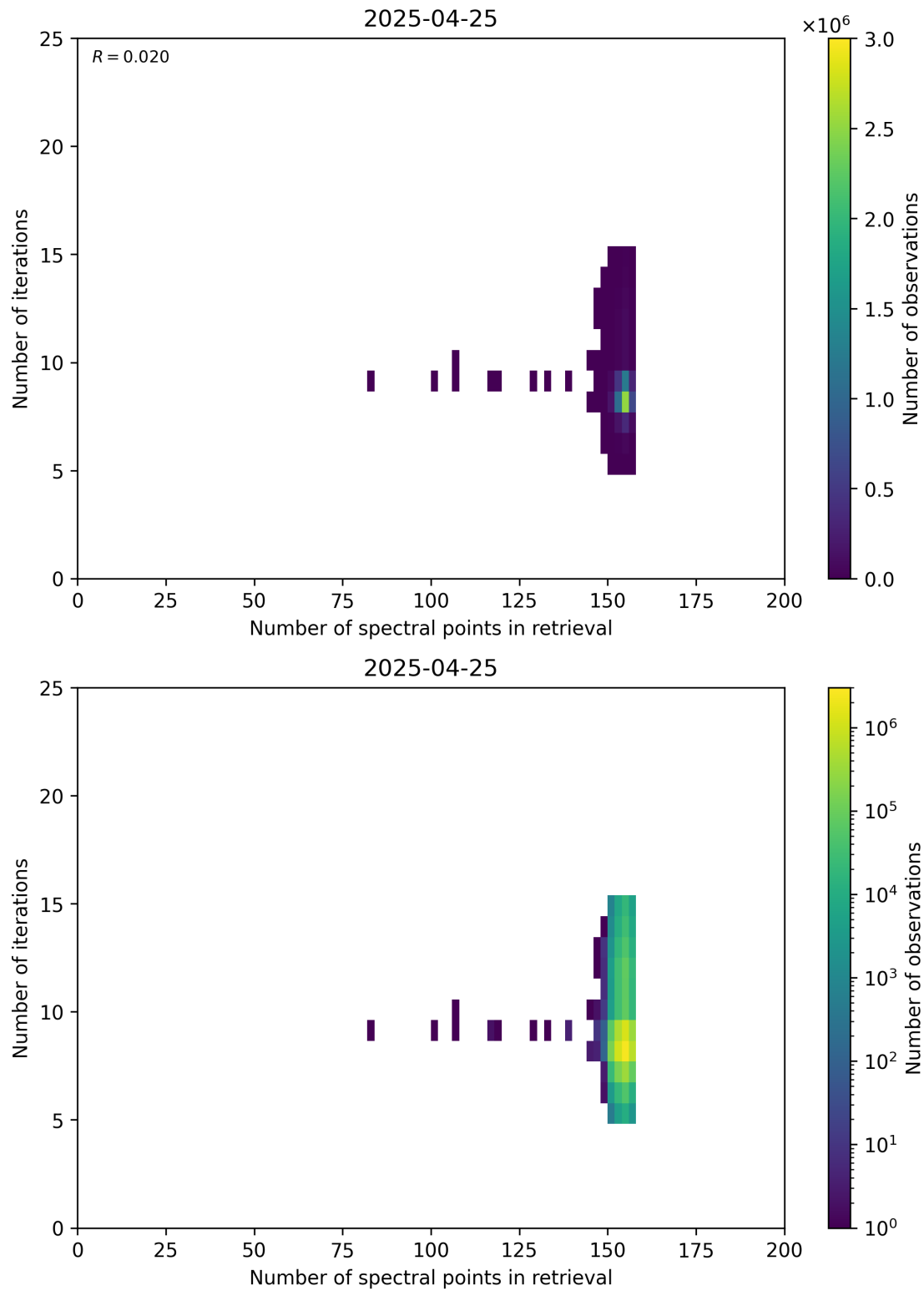
Figure 60: Scatter density plot of “Number of spectral points in retrieval” against “Number of iterations” for 2025-04-24 to 2025-04-26.
