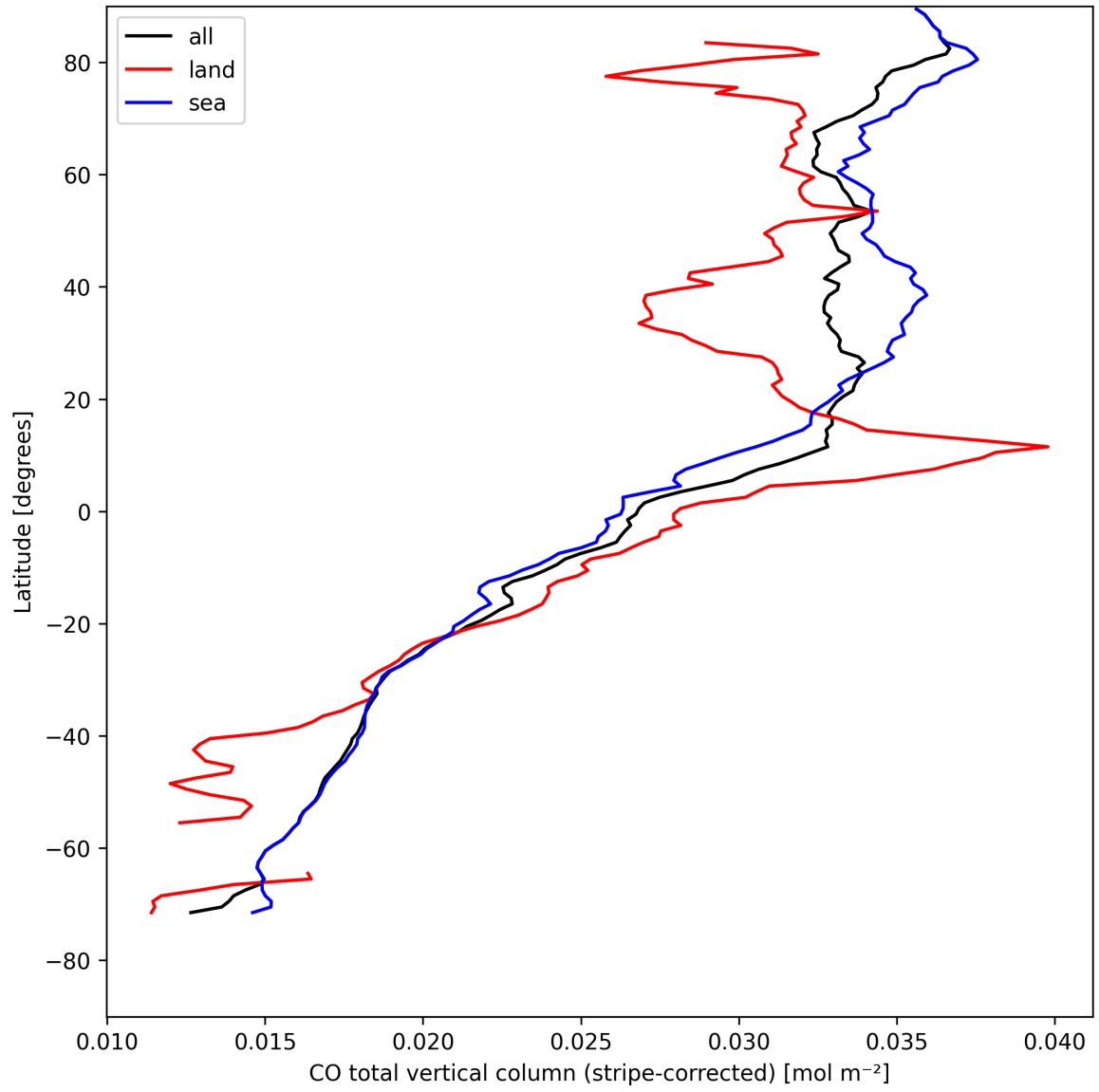
Figure 11: Zonal average of “CO total vertical column (stripe-corrected)” for 2025-04-24 to 2025-04-26.
