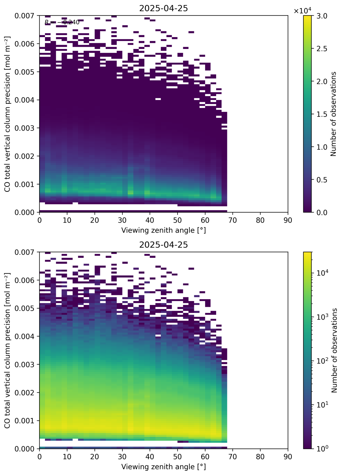
Figure 71: Scatter density plot of “Viewing zenith angle” against “CO total vertical column precision” for 2025-04-24 to 2025-04-26.
