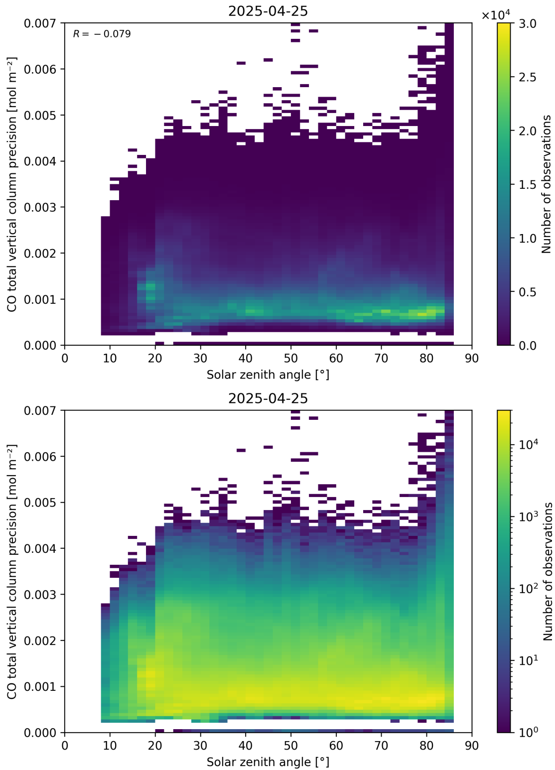
Figure 63: Scatter density plot of “Solar zenith angle” against “CO total vertical column precision” for 2025-04-24 to 2025-04-26.
