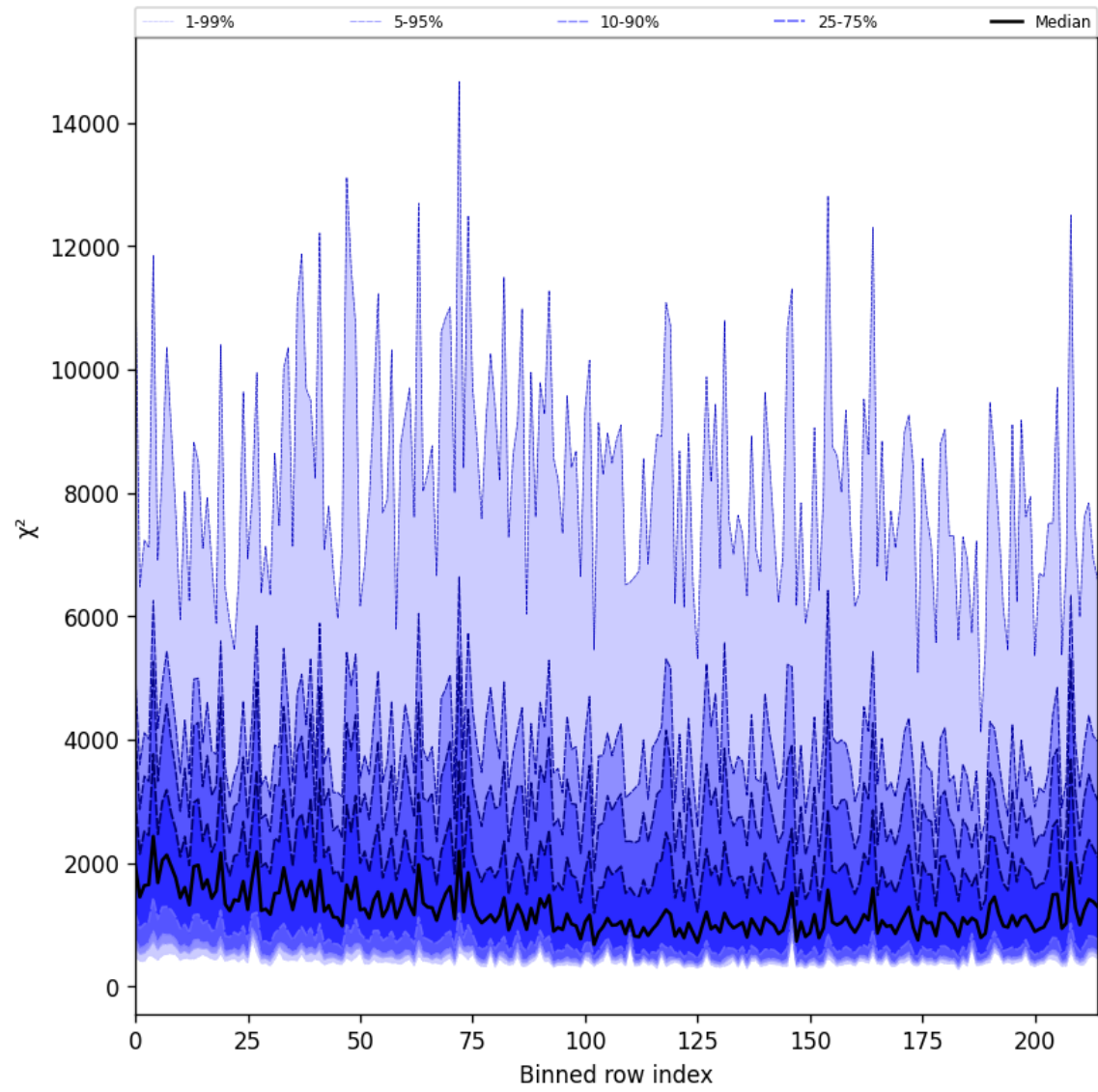
Figure 30: Along track statistics of “ \chi^2 ” for 2025-04-24 to 2025-04-26
