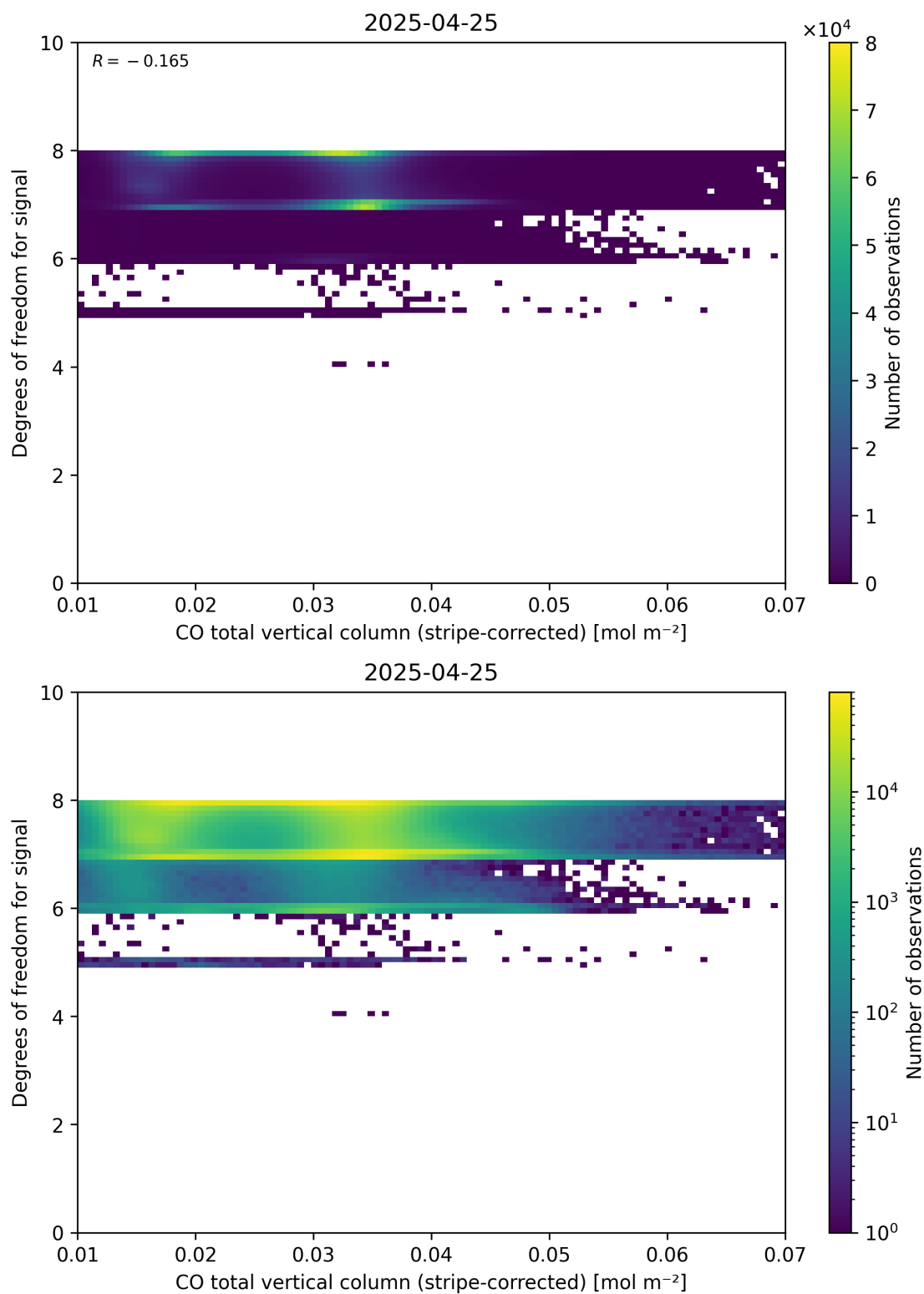
Figure 38: Scatter density plot of “CO total vertical column (stripe-corrected)” against “Degrees of freedom for signal” for 2025-04-24 to 2025-04-26.
