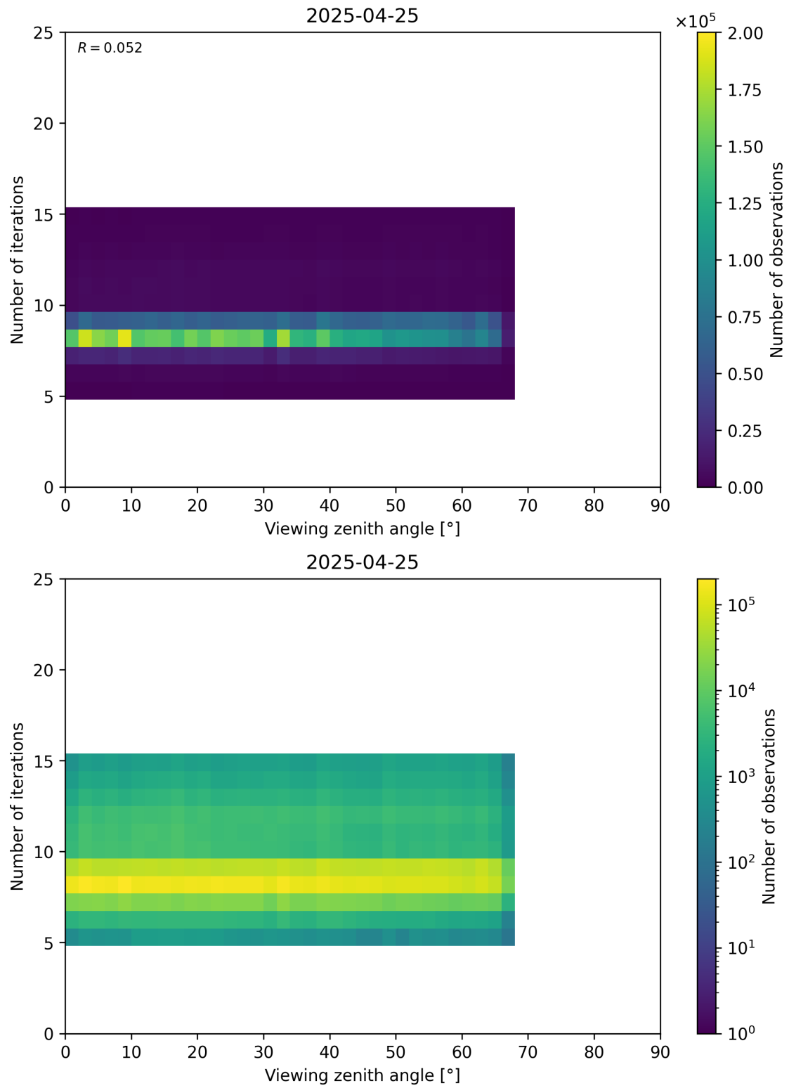
Figure 75: Scatter density plot of “Viewing zenith angle” against “Number of iterations” for 2025-04-24 to 2025-04-26.
