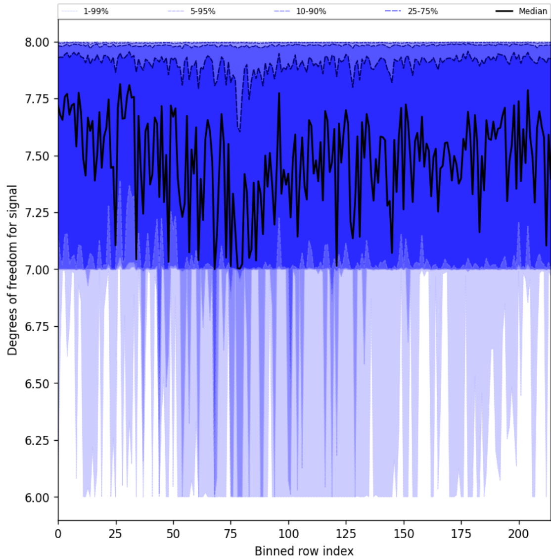
Figure 31: Along track statistics of “Degrees of freedom for signal” for 2025-04-24 to 2025-04-26
