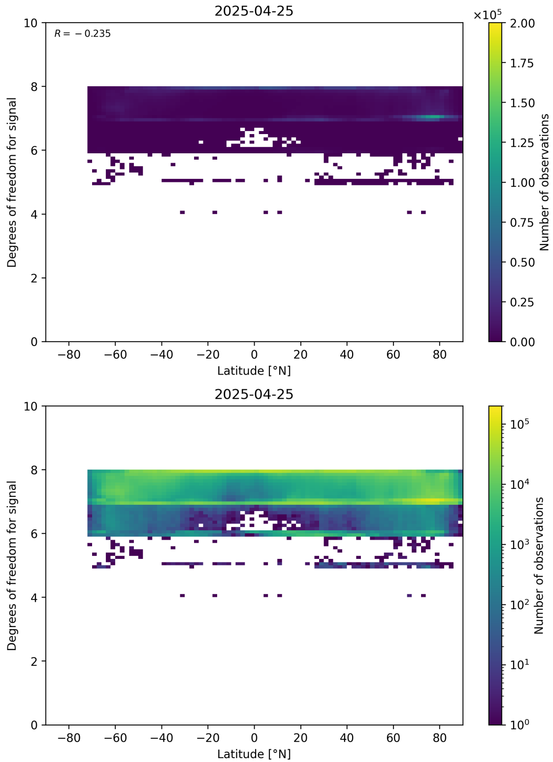
Figure 55: Scatter density plot of “Latitude” against “Degrees of freedom for signal” for 2025-04-24 to 2025-04-26.
