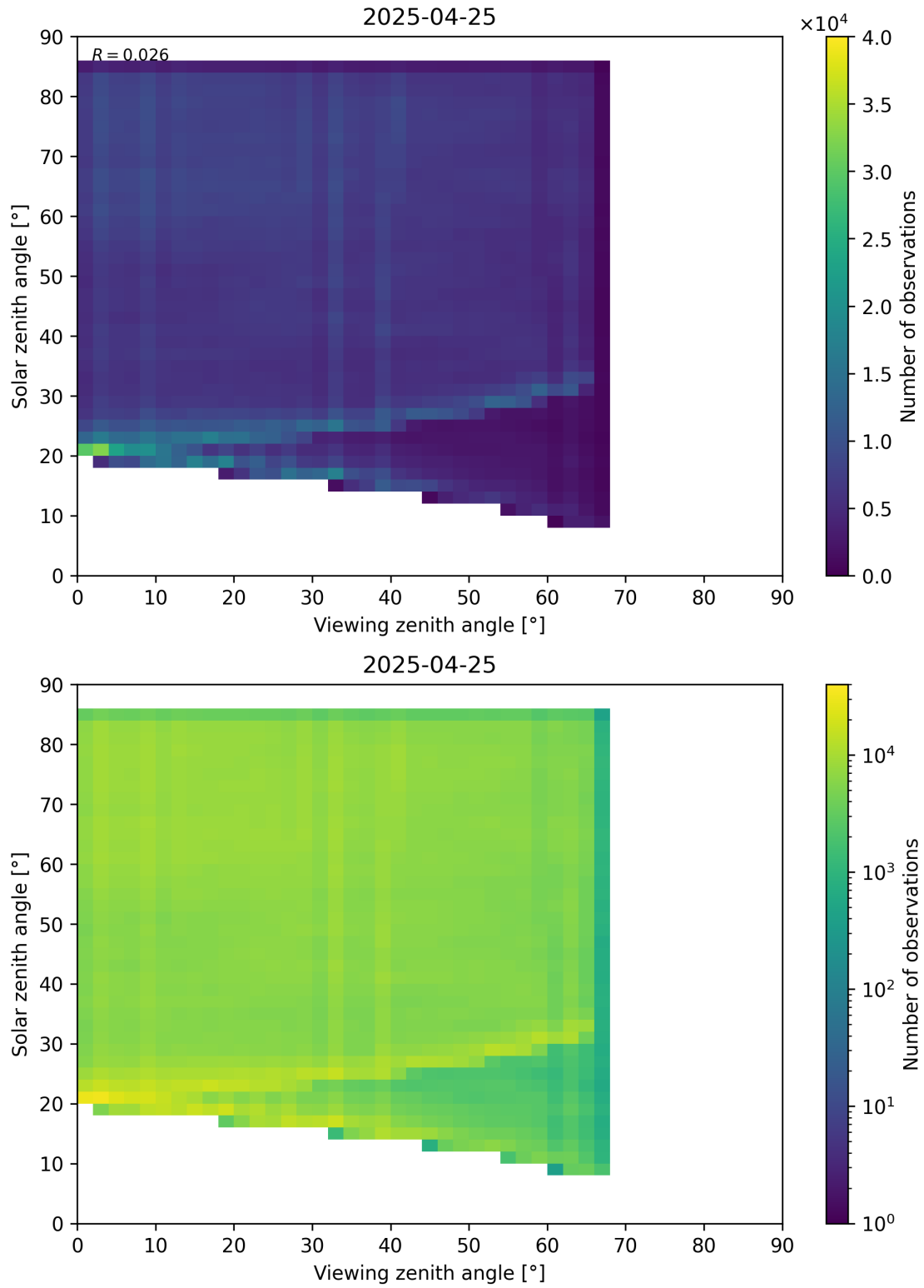
Figure 77: Scatter density plot of “Viewing zenith angle” against “Solar zenith angle” for 2025-04-24 to 2025-04-26.
