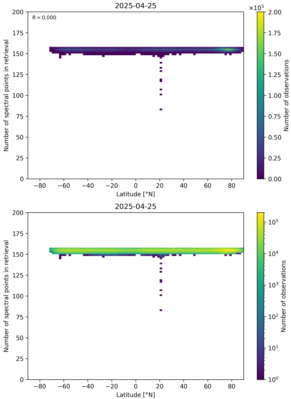
Figure 57: Scatter density plot of “Latitude” against “Number of spectral points in retrieval” for 2025-04-24 to 2025-04-26.
