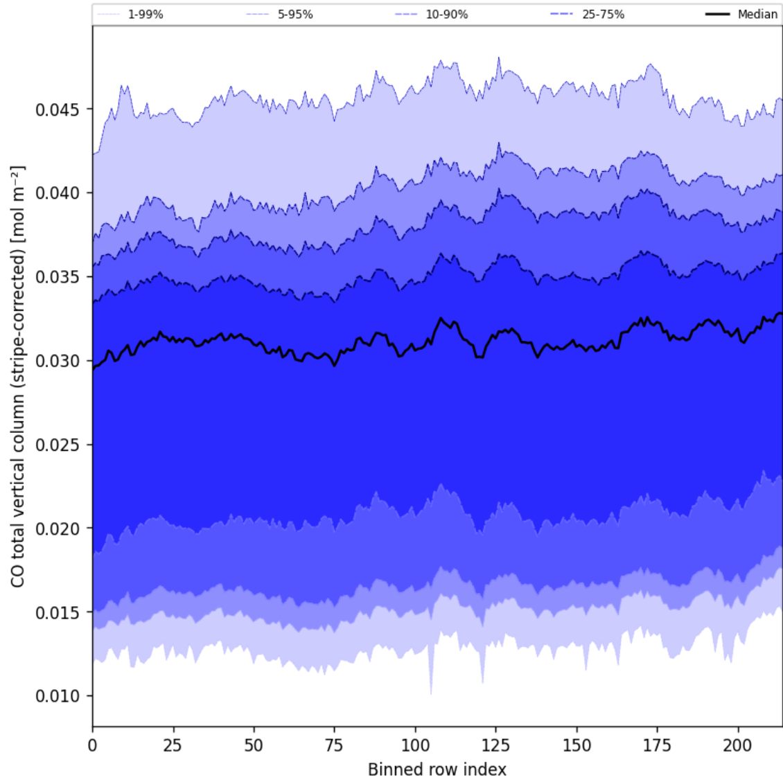
Figure 27: Along track statistics of “CO total vertical column (stripe-corrected)” for 2025-04-24 to 2025-04-26
