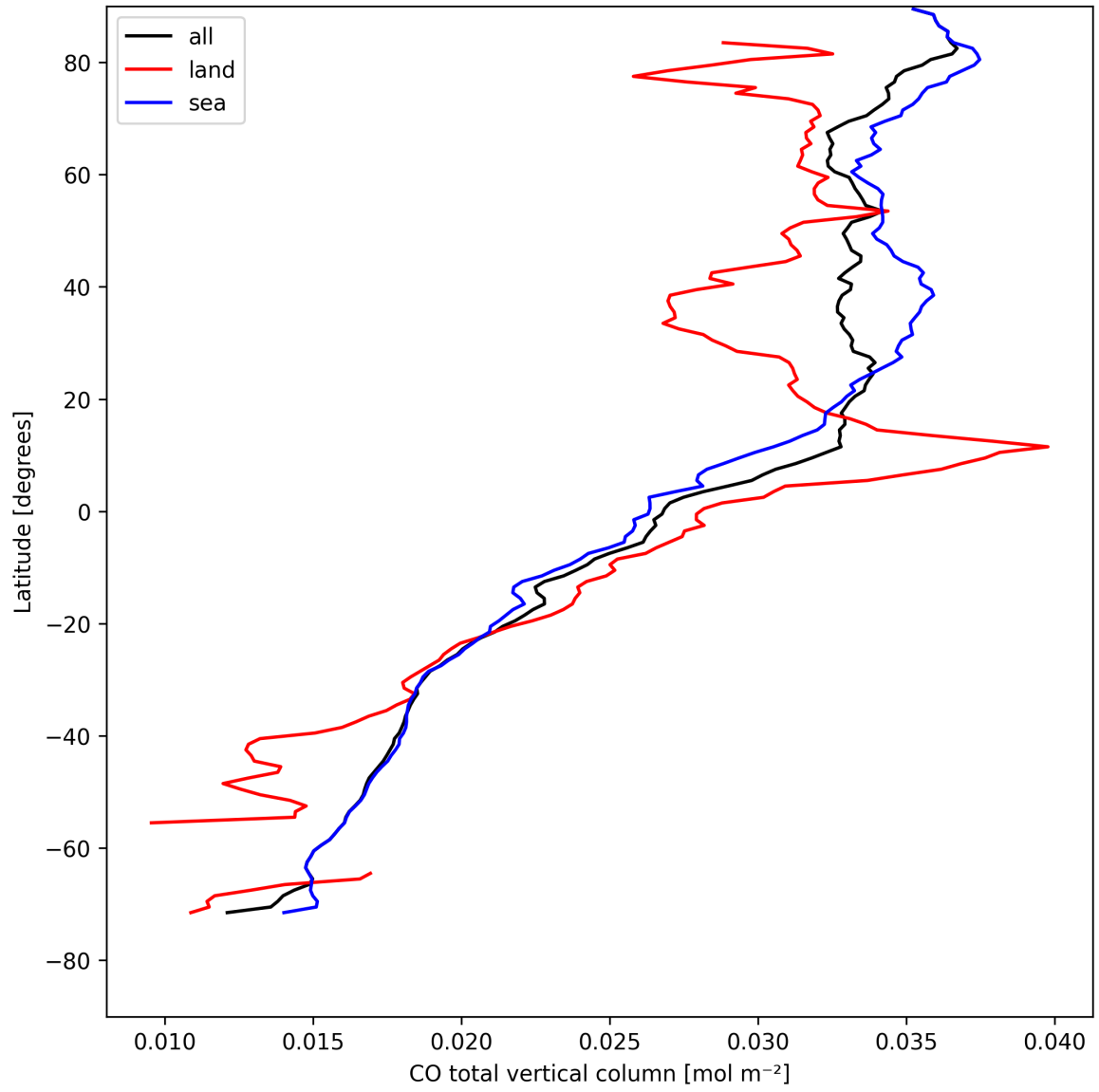
Figure 10: Zonal average of “CO total vertical column” for 2025-04-24 to 2025-04-26.
