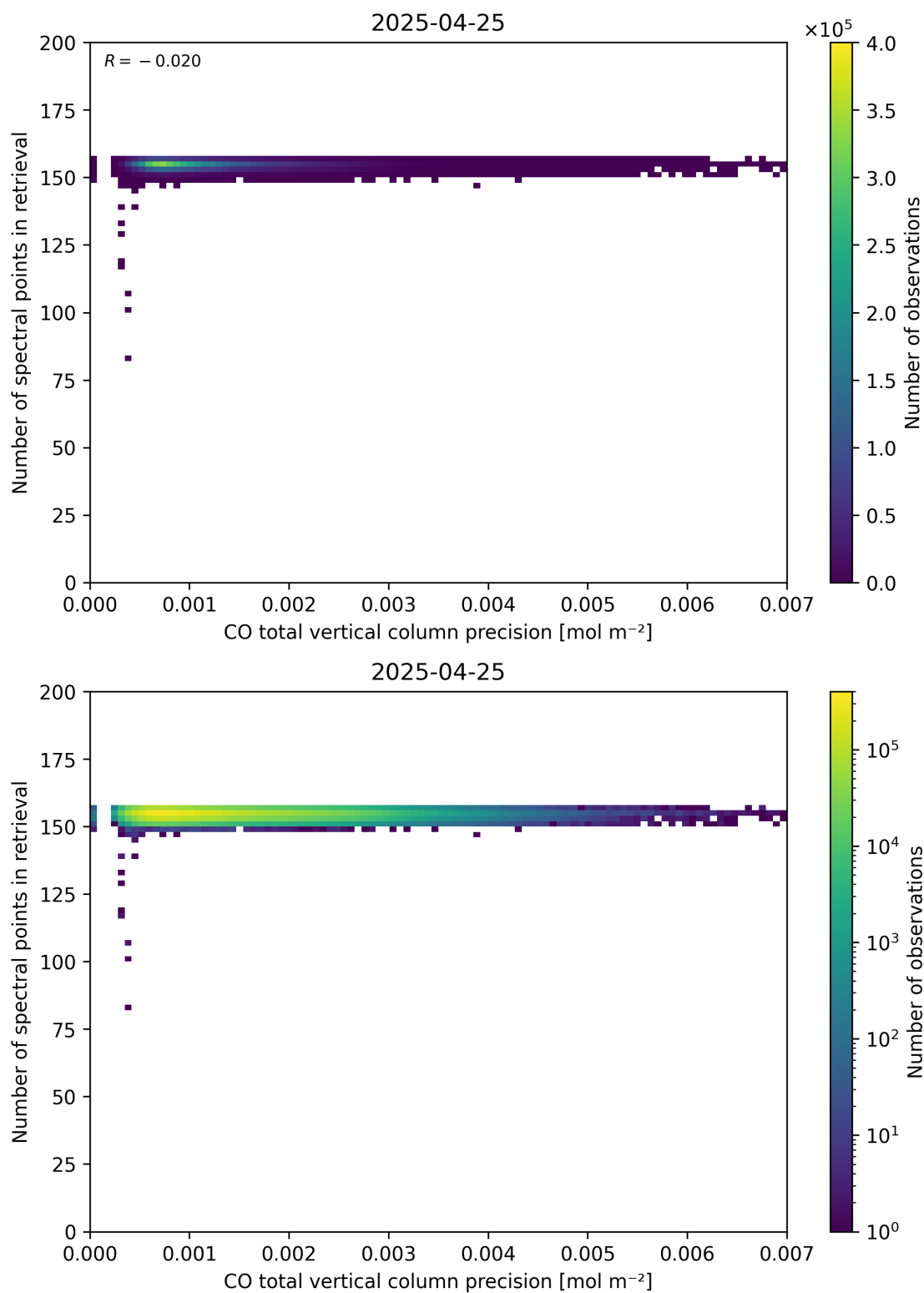
Figure 47: Scatter density plot of “CO total vertical column precision” against “Number of spectral points in retrieval” for 2025-04-24 to 2025-04-26.
