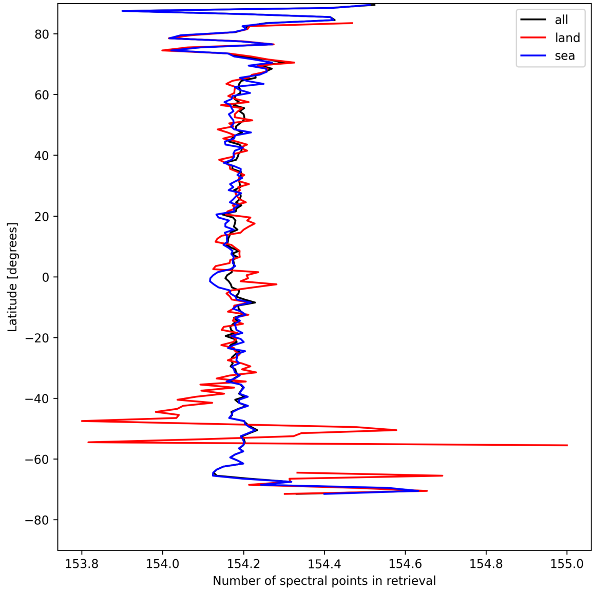
Figure 13: Zonal average of “Number of spectral points in retrieval” for 2025-04-24 to 2025-04-26.
