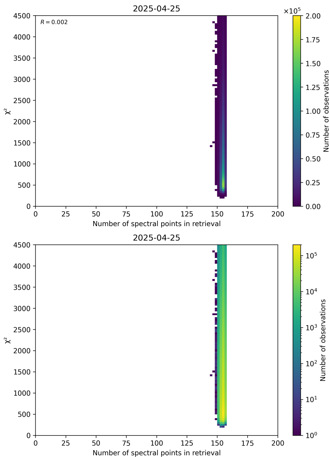
Figure 58: Scatter density plot of “Number of spectral points in retrieval” against “ \chi^2 ” for 2025-04-24 to 2025-04-26.
