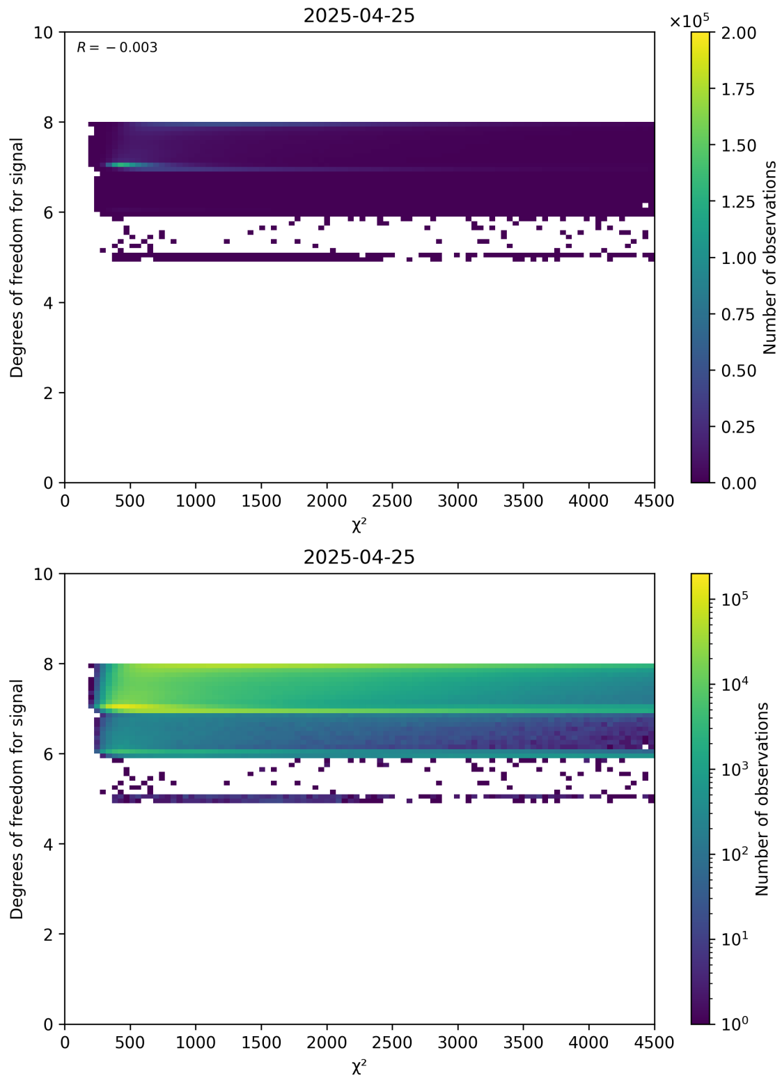
Figure 48: Scatter density plot of “ \chi^2 ” against “Degrees of freedom for signal” for 2025-04-24 to 2025-04-26.
