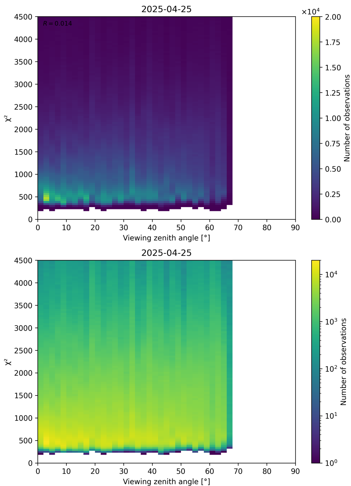
Figure 72: Scatter density plot of “Viewing zenith angle” against “ \chi^2 ” for 2025-04-24 to 2025-04-26.
