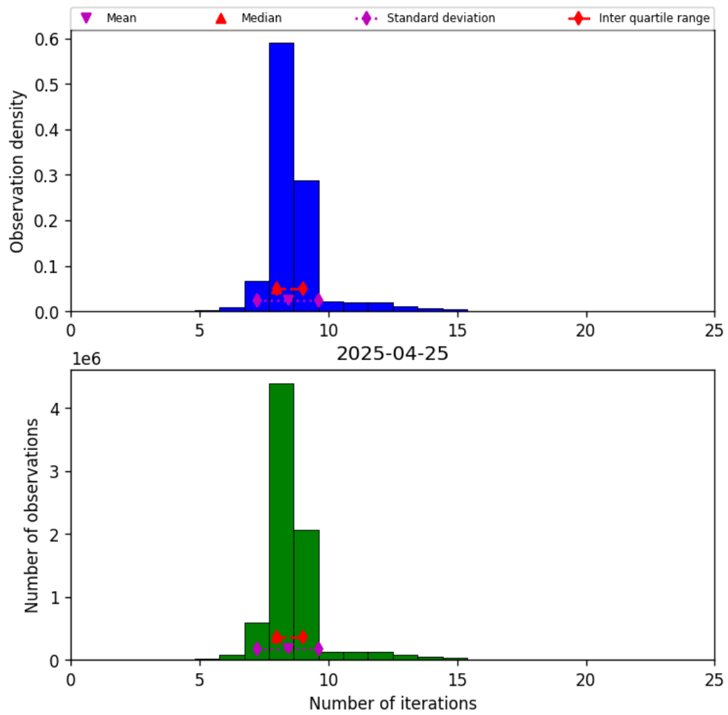
Figure 24: Histogram of “Number of iterations” for 2025-04-24 to 2025-04-26
