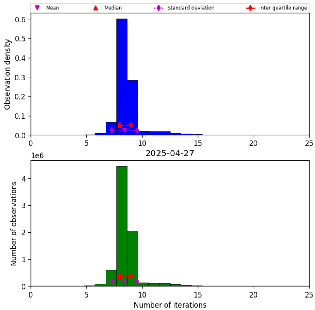
Figure 24: Histogram of “Number of iterations” for 2025-04-26 to 2025-04-28
