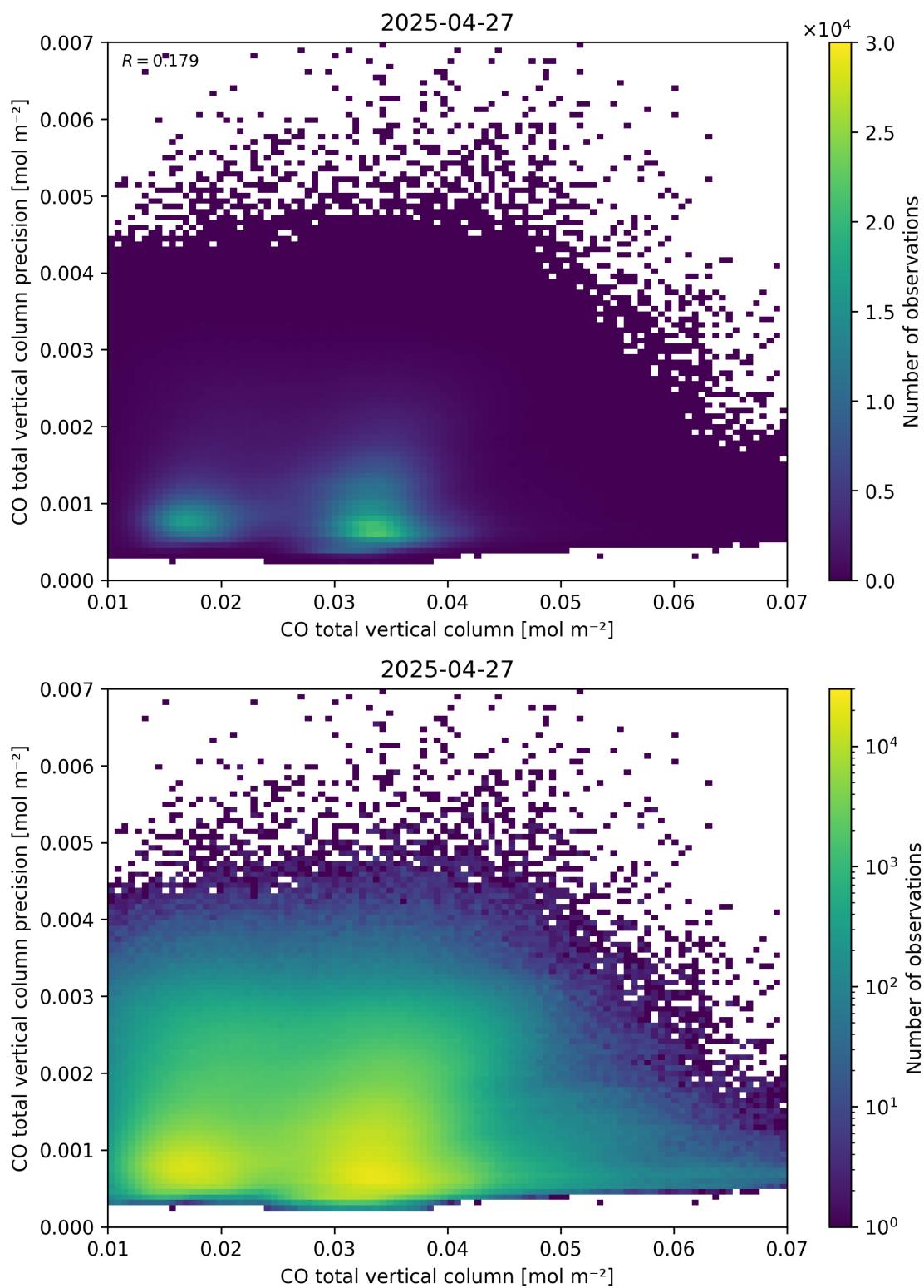
Figure 34: Scatter density plot of “CO total vertical column” against “CO total vertical column precision” for 2025-04-26 to 2025-04-28.
