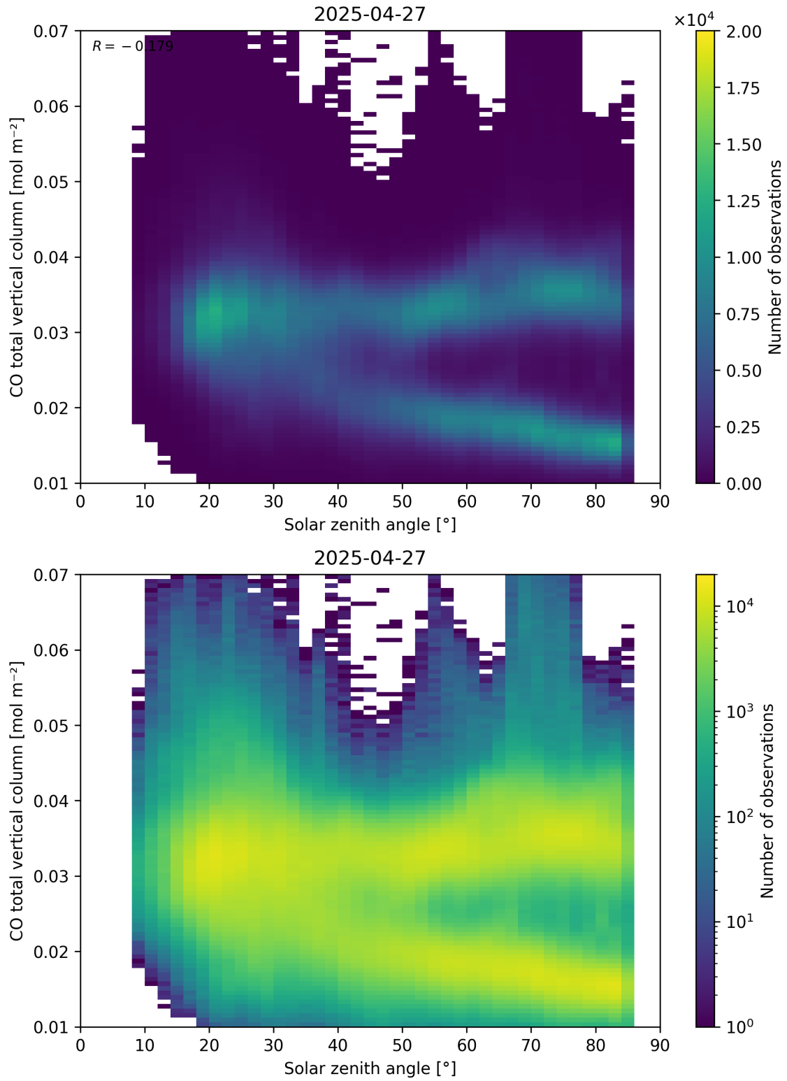
Figure 61: Scatter density plot of “Solar zenith angle” against “CO total vertical column” for 2025-04-26 to 2025-04-28.
