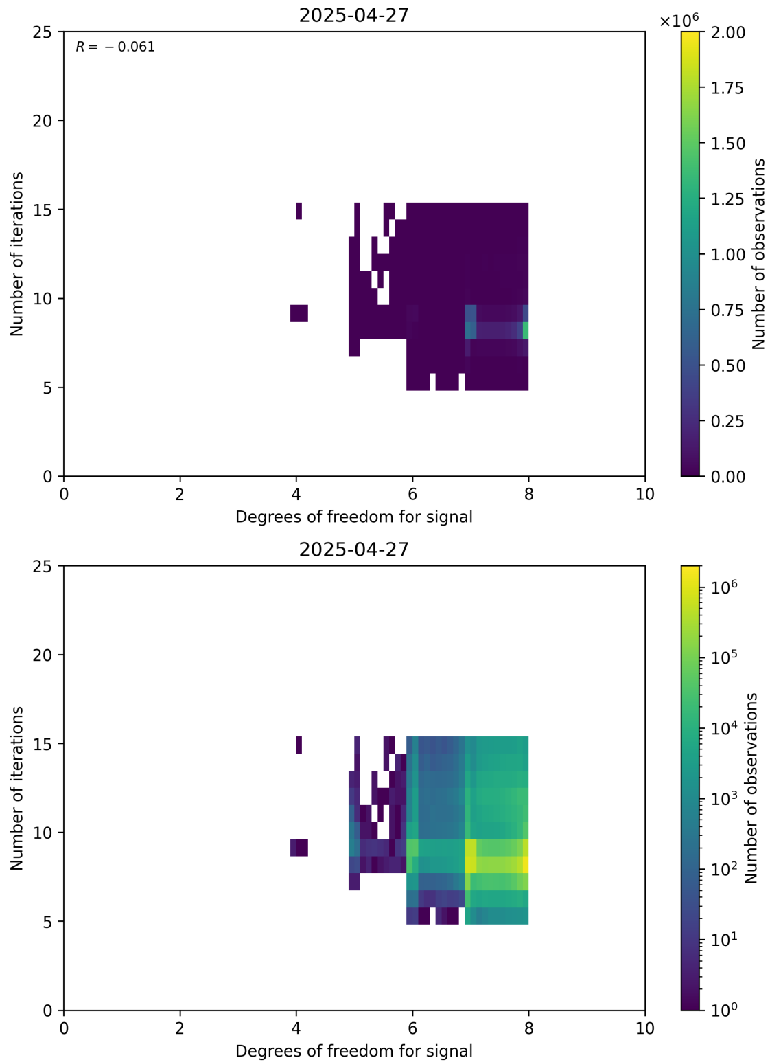
Figure 50: Scatter density plot of “Degrees of freedom for signal” against “Number of iterations” for 2025-04-26 to 2025-04-28.
