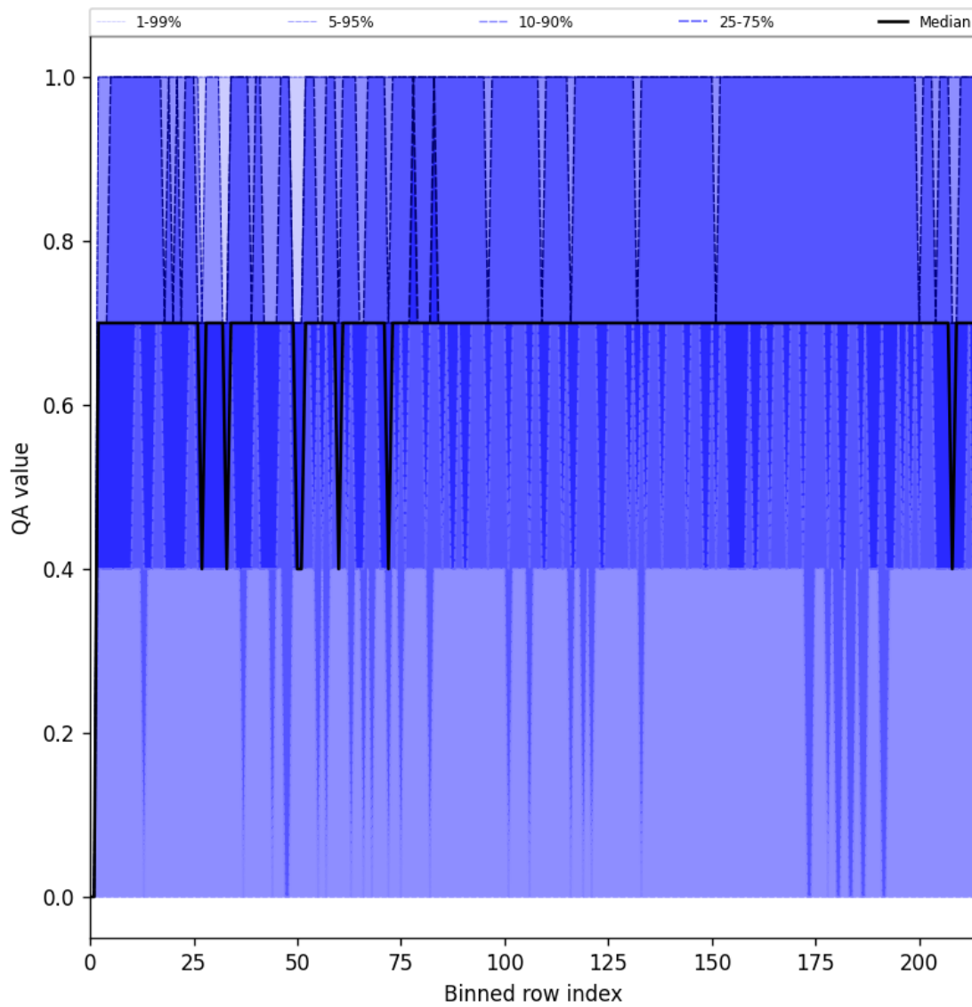
Figure 25: Along track statistics of “QA value” for 2025-04-26 to 2025-04-28
