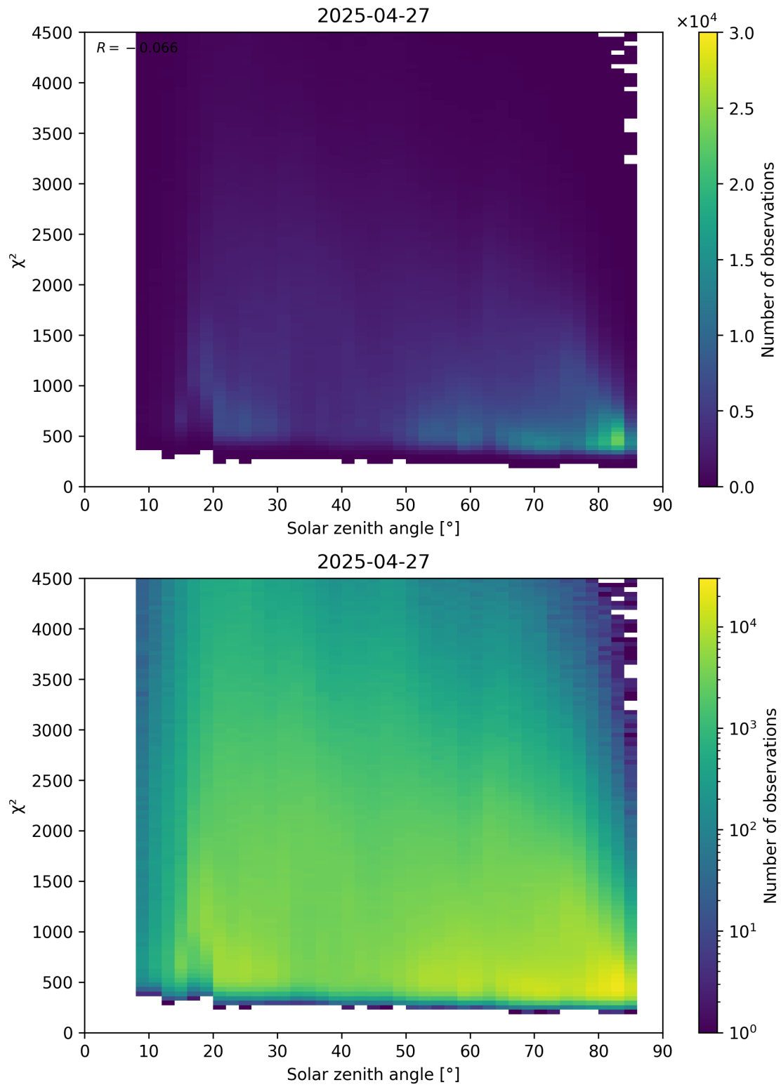
Figure 64: Scatter density plot of “Solar zenith angle” against “ \chi^2 ” for 2025-04-26 to 2025-04-28.
