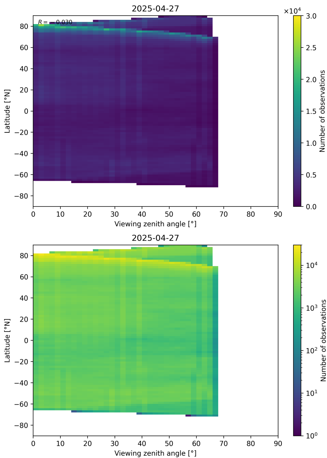
Figure 74: Scatter density plot of “Viewing zenith angle” against “Latitude” for 2025-04-26 to 2025-04-28.
