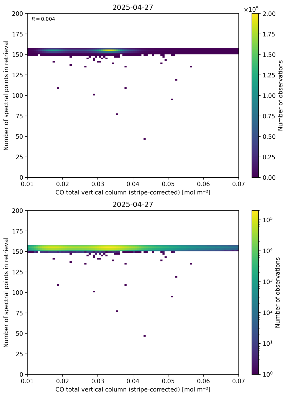
Figure 40: Scatter density plot of “CO total vertical column (stripe-corrected)” against “Number of spectral points in retrieval” for 2025-04-26 to 2025-04-28.
