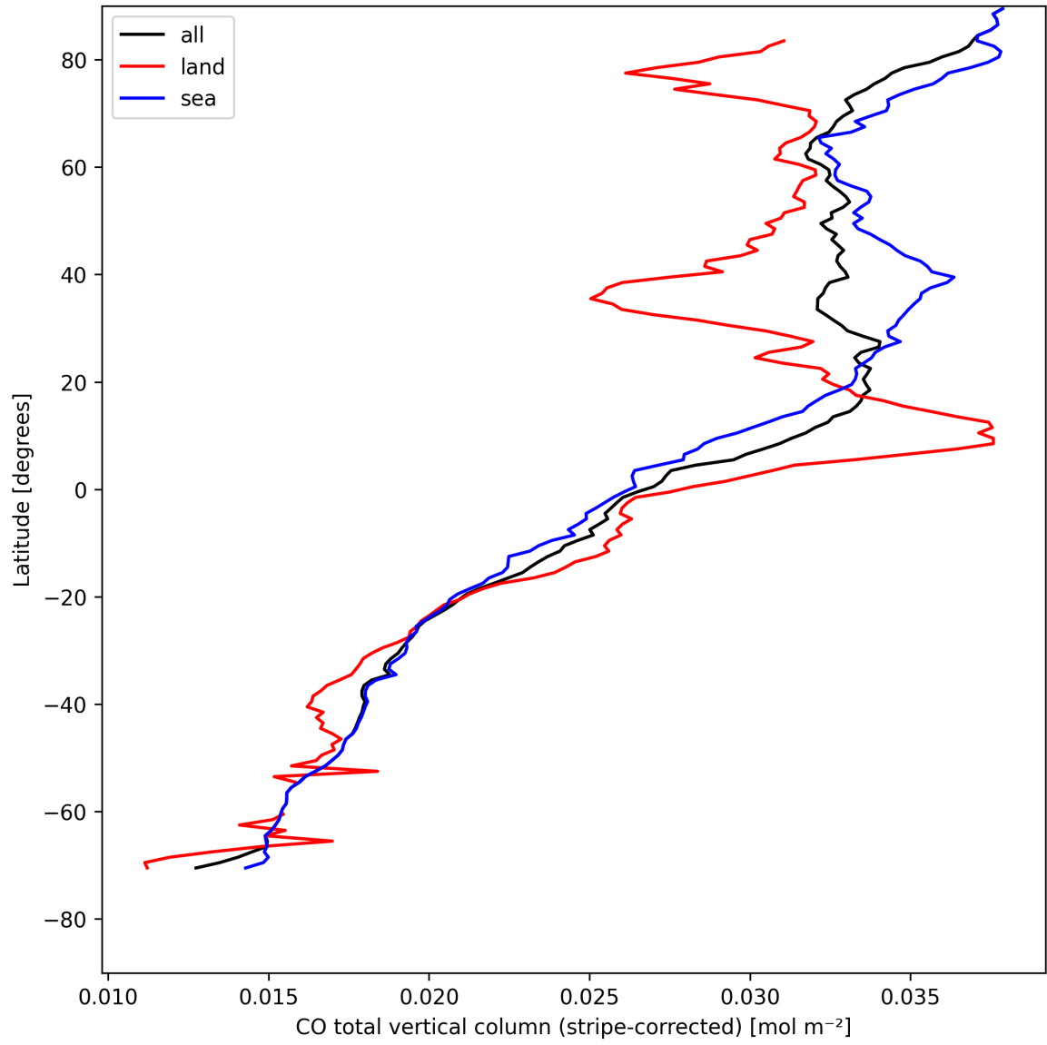
Figure 11: Zonal average of “CO total vertical column (stripe-corrected)” for 2025-04-26 to 2025-04-28.
