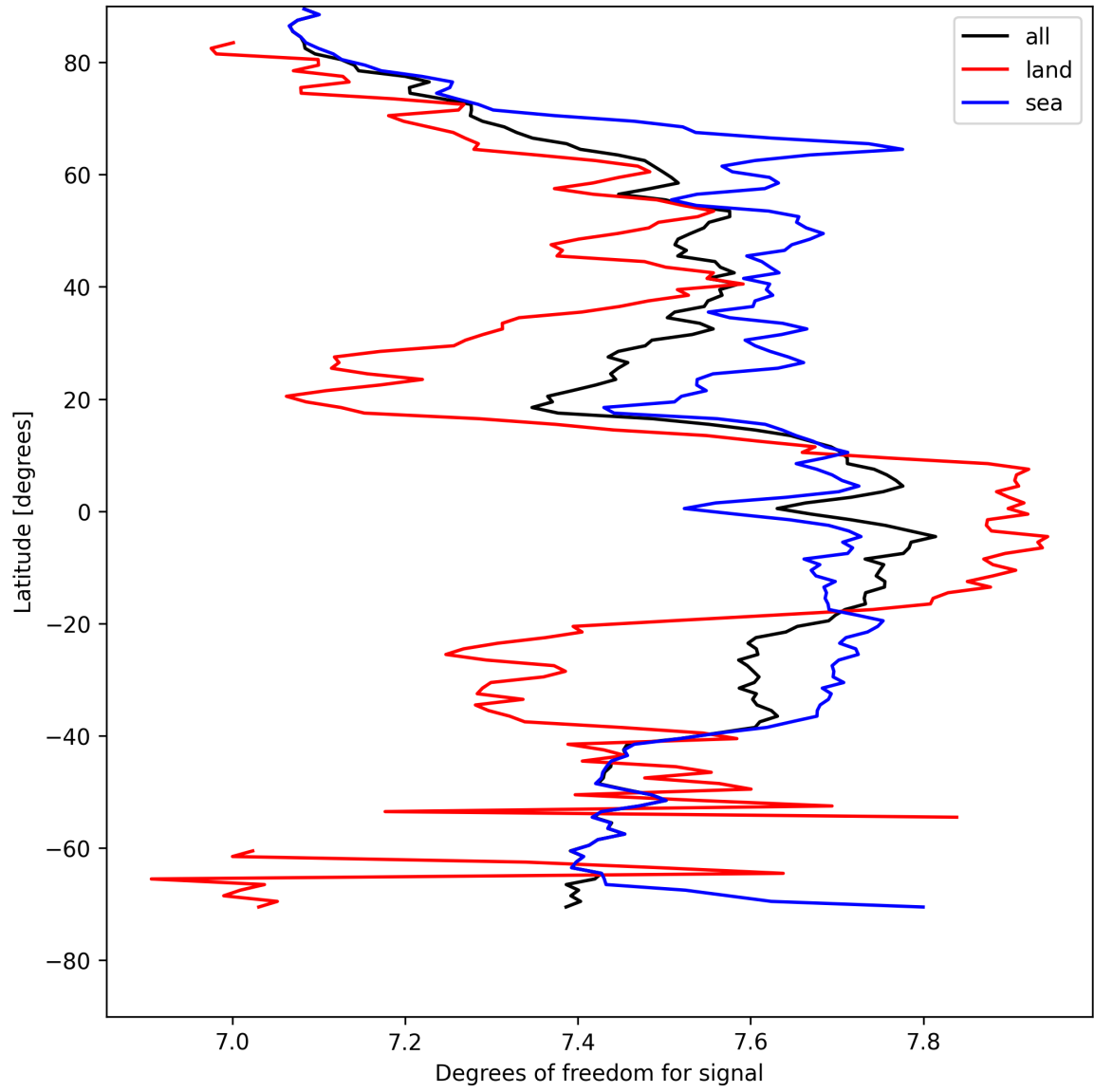
Figure 15: Zonal average of “Degrees of freedom for signal” for 2025-04-26 to 2025-04-28.
