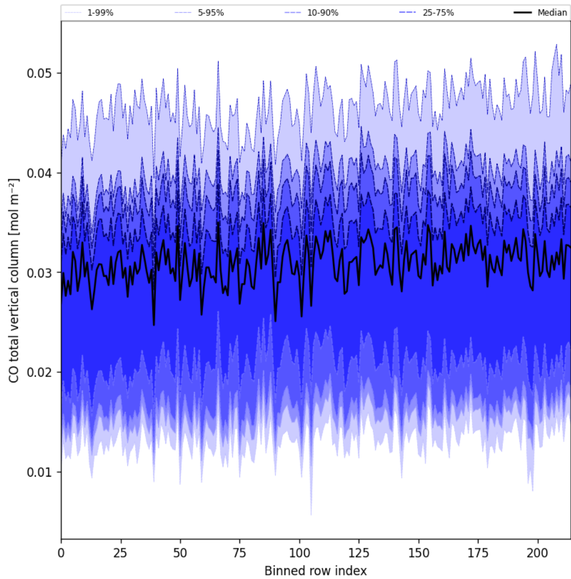
Figure 26: Along track statistics of “CO total vertical column” for 2025-04-26 to 2025-04-28
