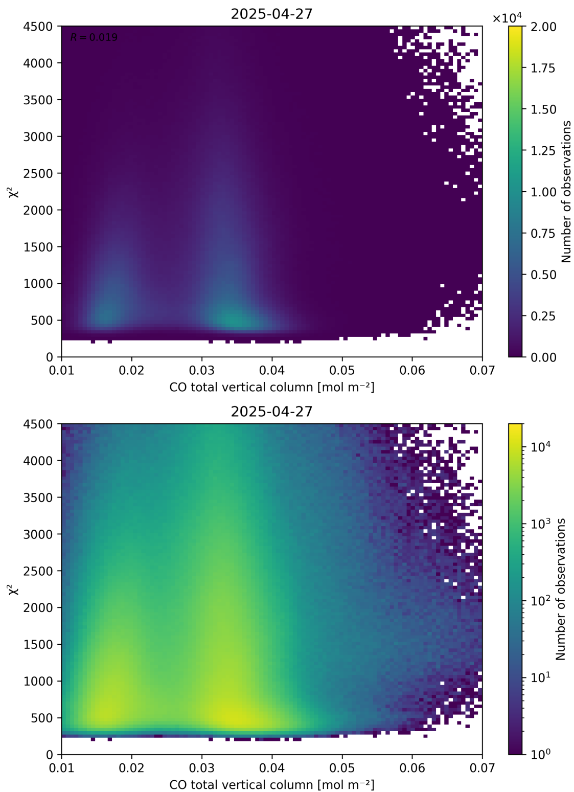
Figure 35: Scatter density plot of “CO total vertical column” against “ \chi^2 ” for 2025-04-26 to 2025-04-28.
