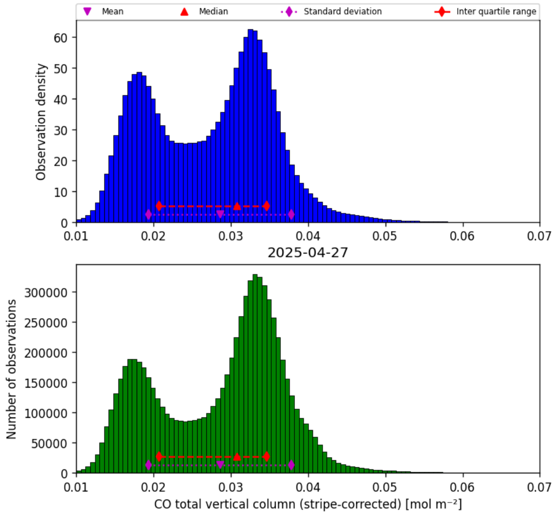
Figure 19: Histogram of “CO total vertical column (stripe-corrected)” for 2025-04-26 to 2025-04-28
