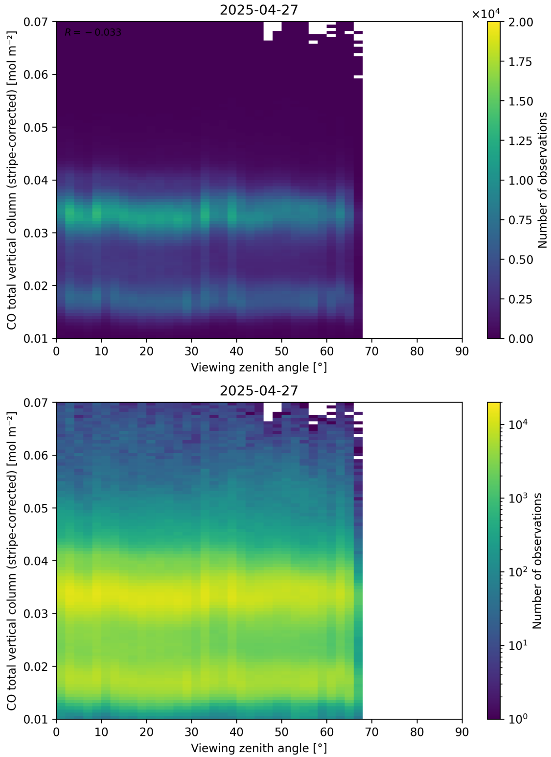
Figure 70: Scatter density plot of “Viewing zenith angle” against “CO total vertical column (stripe-corrected)” for 2025-04-26 to 2025-04-28.
