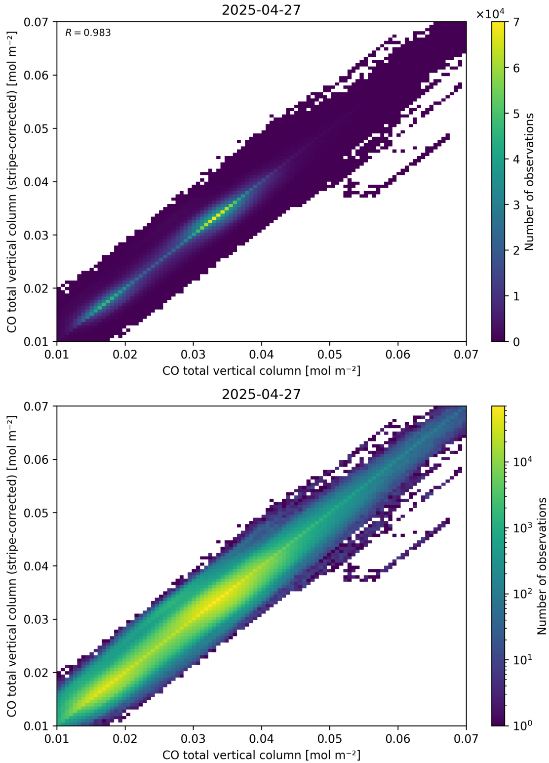
Figure 33: Scatter density plot of “CO total vertical column” against “CO total vertical column (stripe-corrected)” for 2025-04-26 to 2025-04-28.
