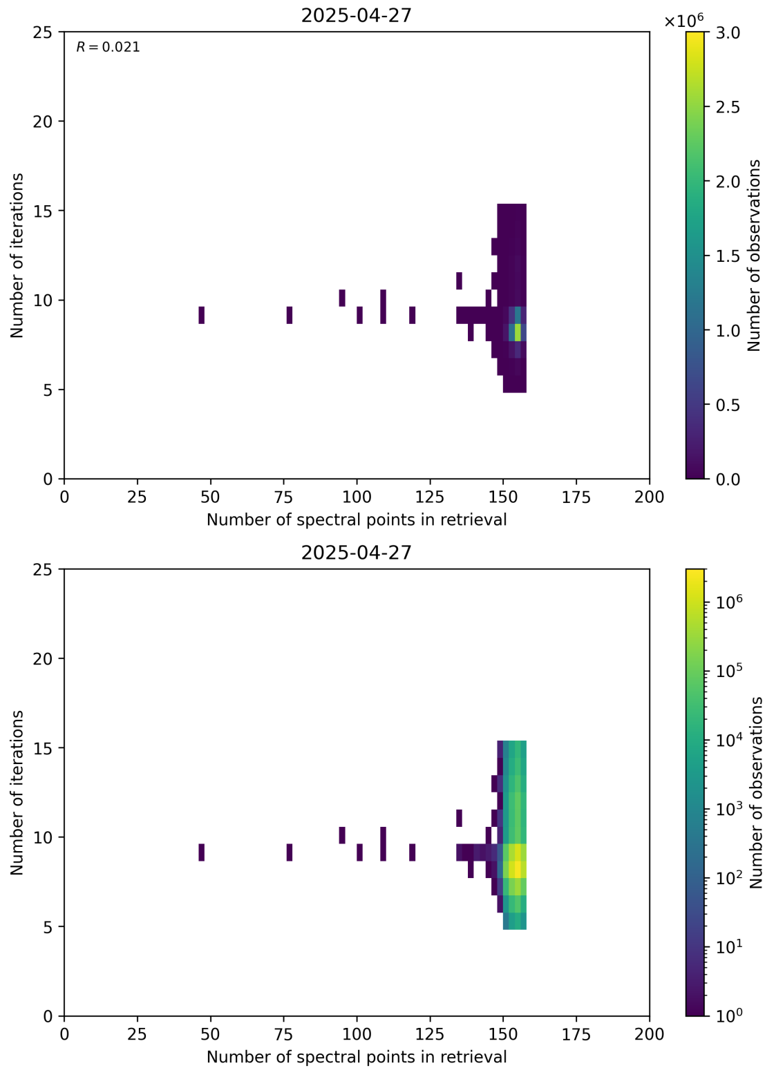
Figure 60: Scatter density plot of “Number of spectral points in retrieval” against “Number of iterations” for 2025-04-26 to 2025-04-28.
