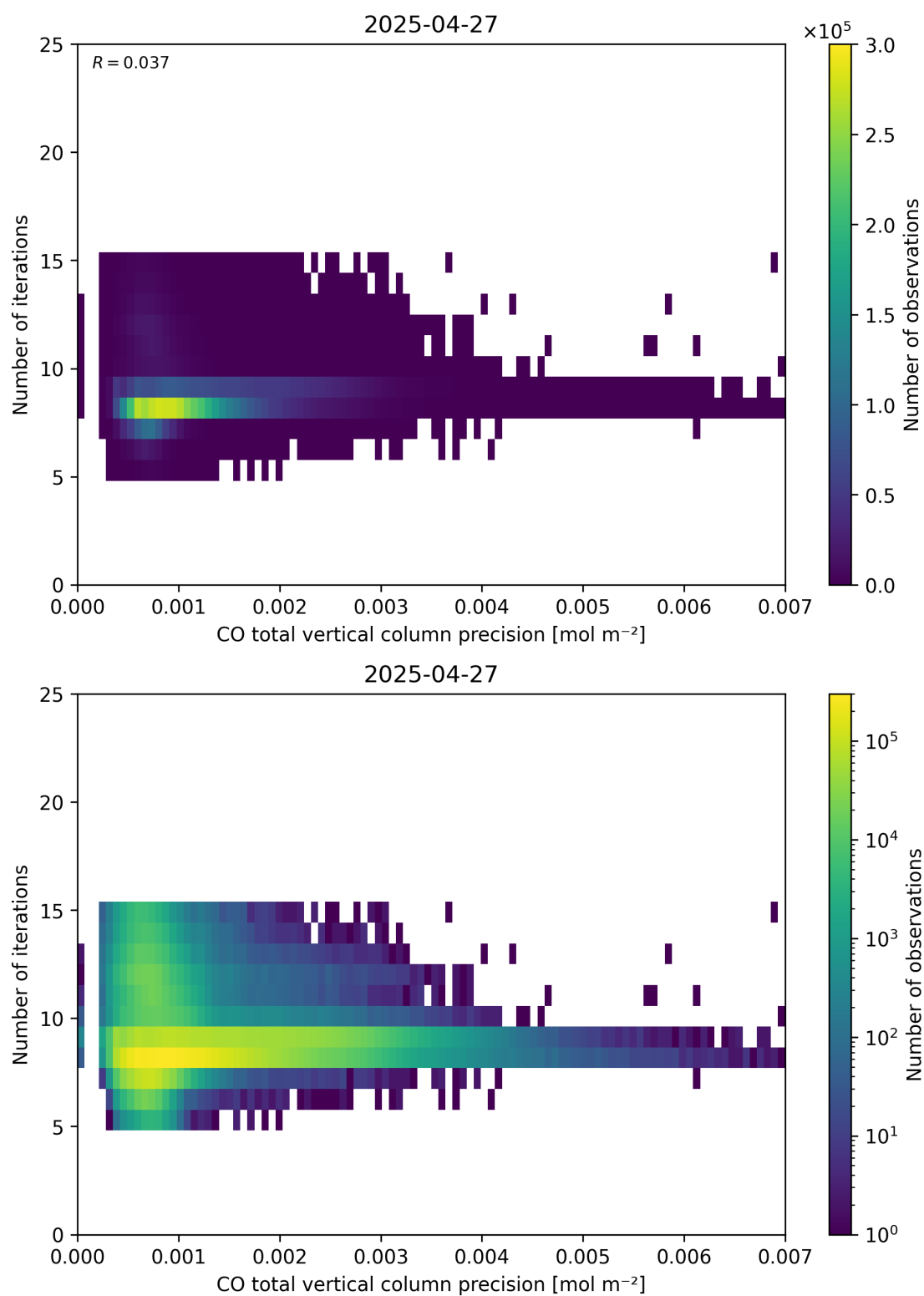
Figure 46: Scatter density plot of “CO total vertical column precision” against “Number of iterations” for 2025-04-26 to 2025-04-28.
