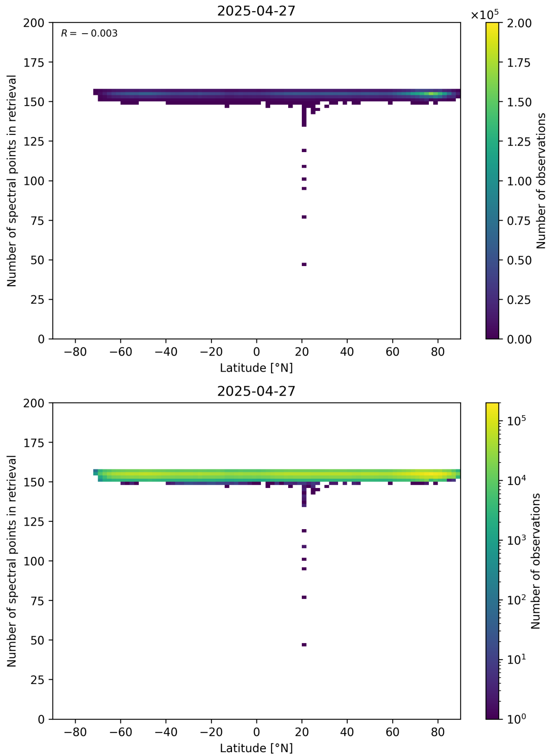
Figure 57: Scatter density plot of “Latitude” against “Number of spectral points in retrieval” for 2025-04-26 to 2025-04-28.
