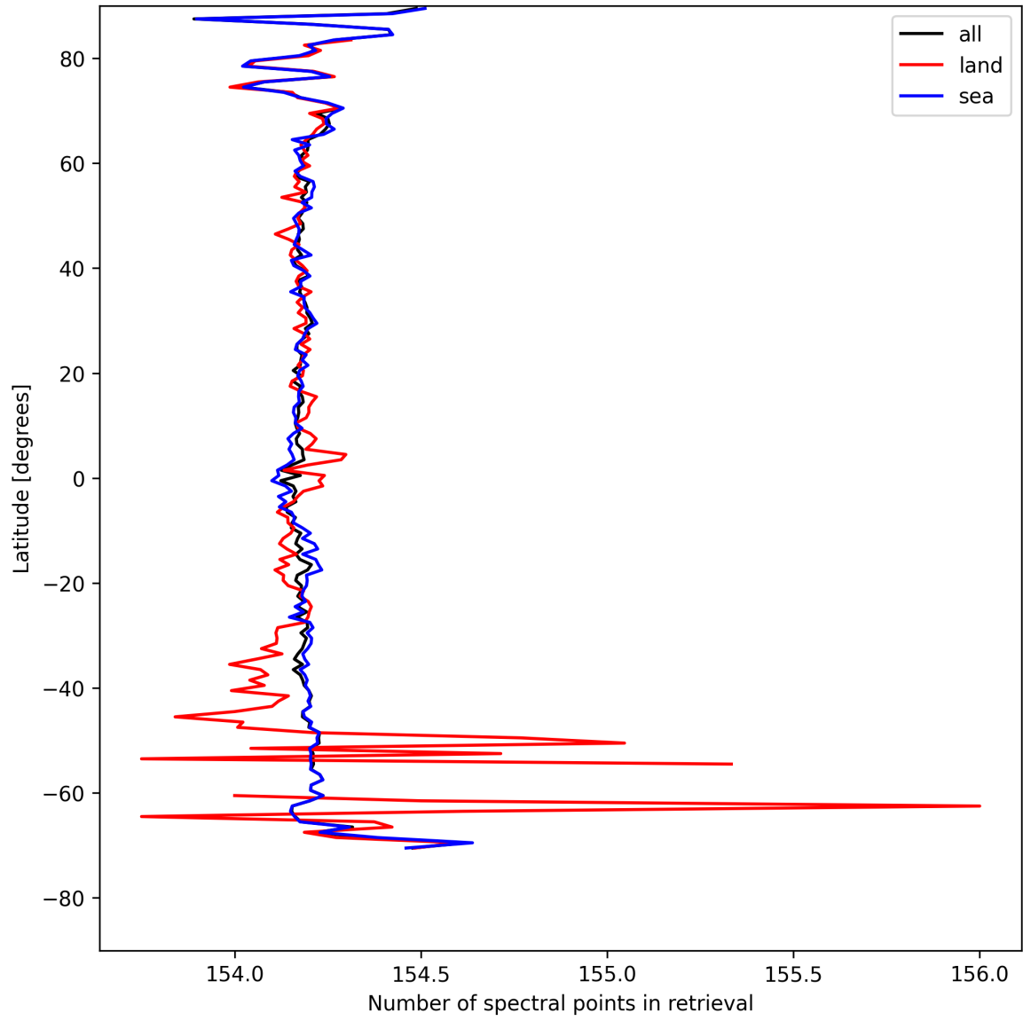
Figure 13: Zonal average of “Number of spectral points in retrieval” for 2025-04-26 to 2025-04-28.
