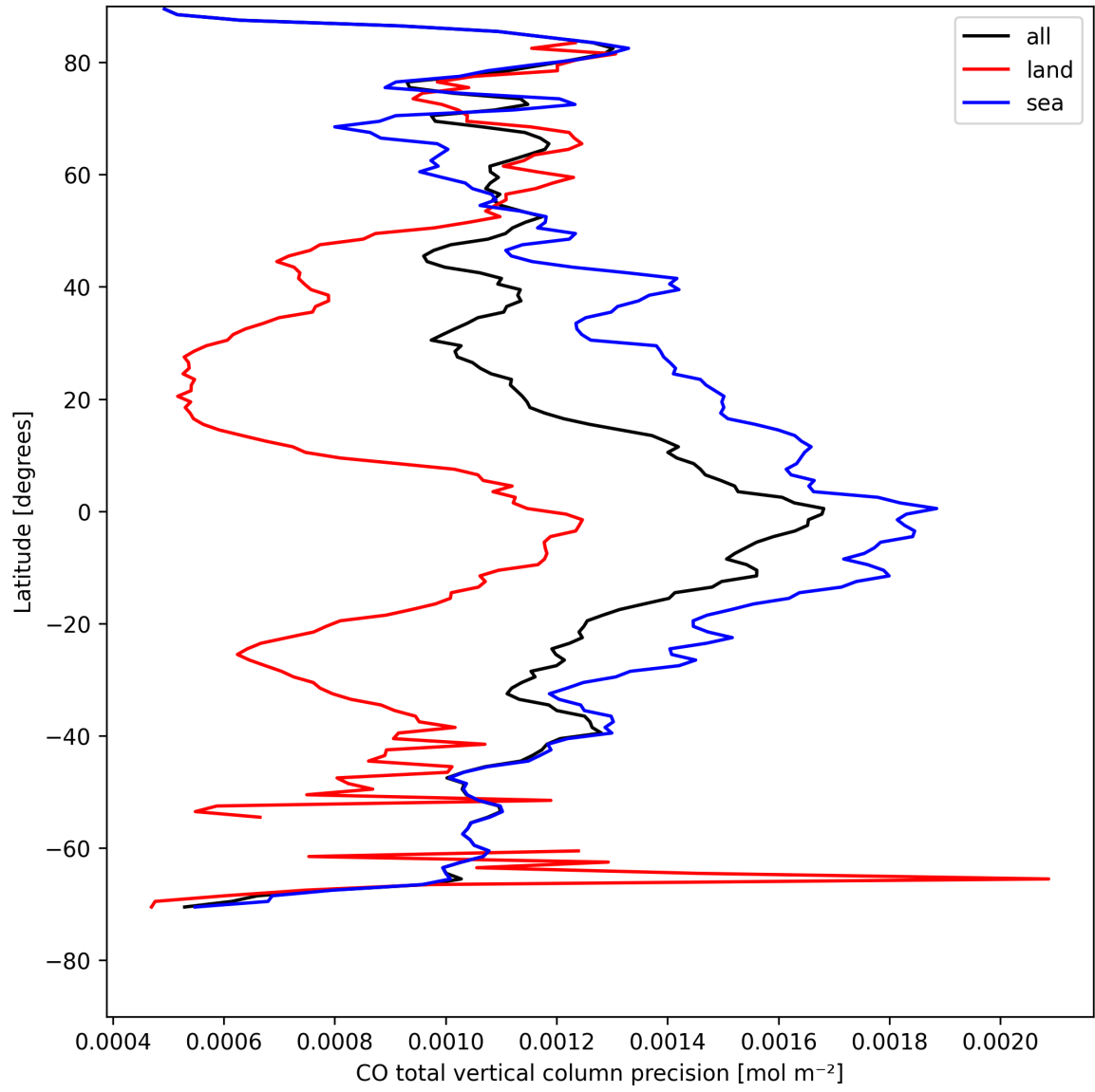
Figure 12: Zonal average of “CO total vertical column precision” for 2025-04-26 to 2025-04-28.
