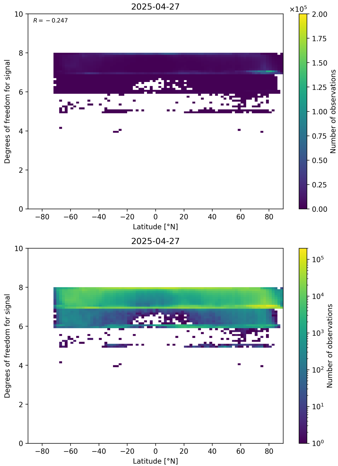
Figure 55: Scatter density plot of “Latitude” against “Degrees of freedom for signal” for 2025-04-26 to 2025-04-28.
