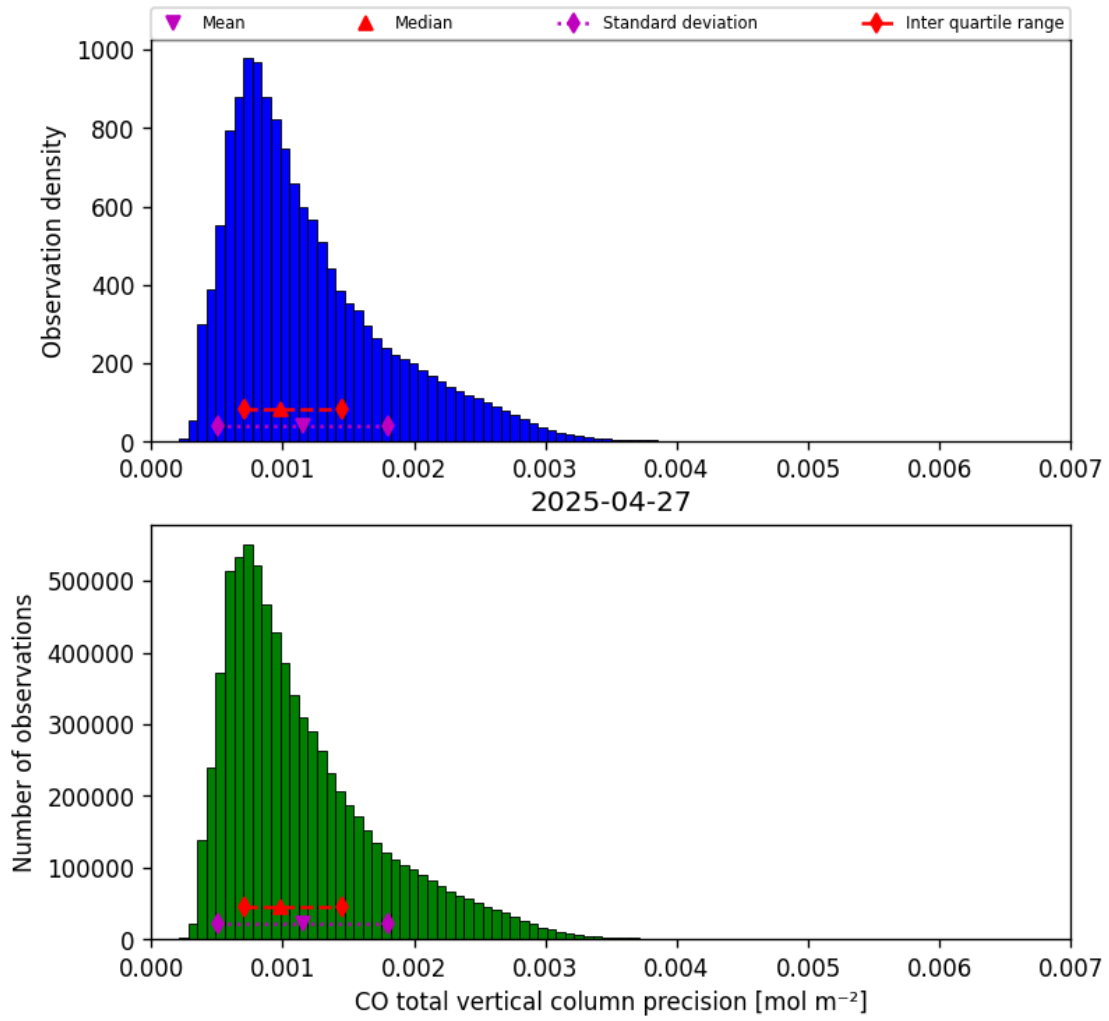
Figure 20: Histogram of “CO total vertical column precision” for 2025-04-26 to 2025-04-28
