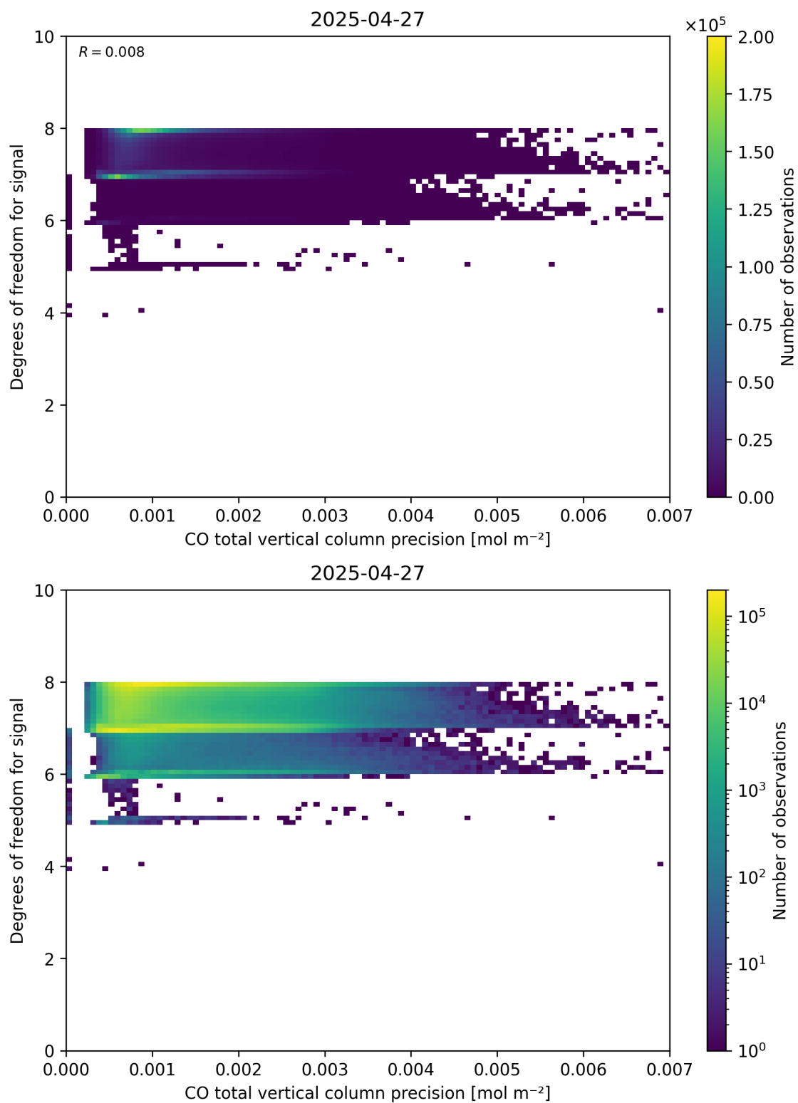
Figure 45: Scatter density plot of “CO total vertical column precision” against “Degrees of freedom for signal” for 2025-04-26 to 2025-04-28.
