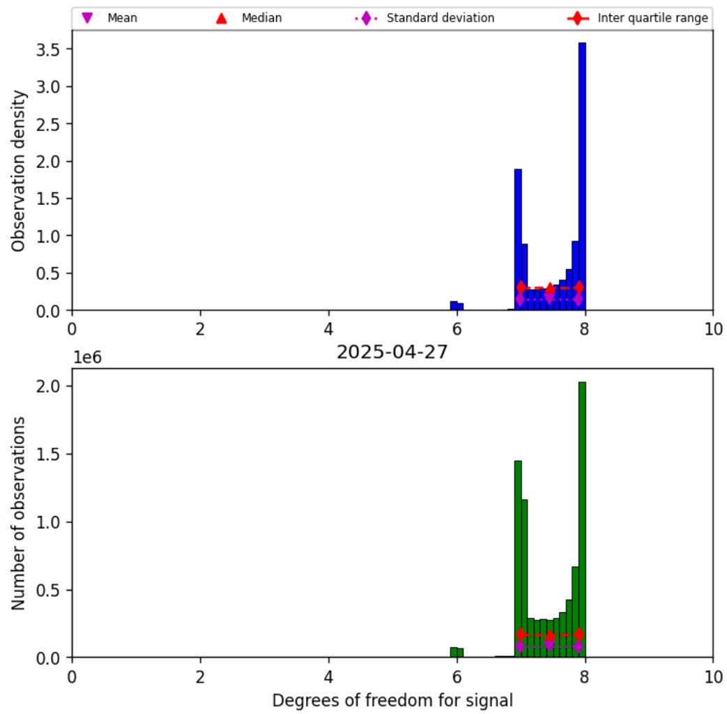
Figure 23: Histogram of “Degrees of freedom for signal” for 2025-04-26 to 2025-04-28
