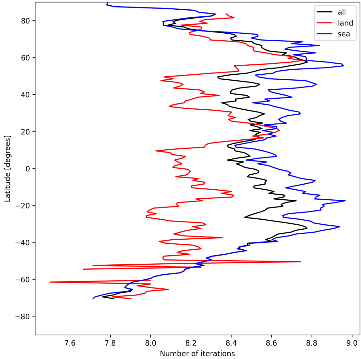
Figure 16: Zonal average of “Number of iterations” for 2025-04-26 to 2025-04-28.
