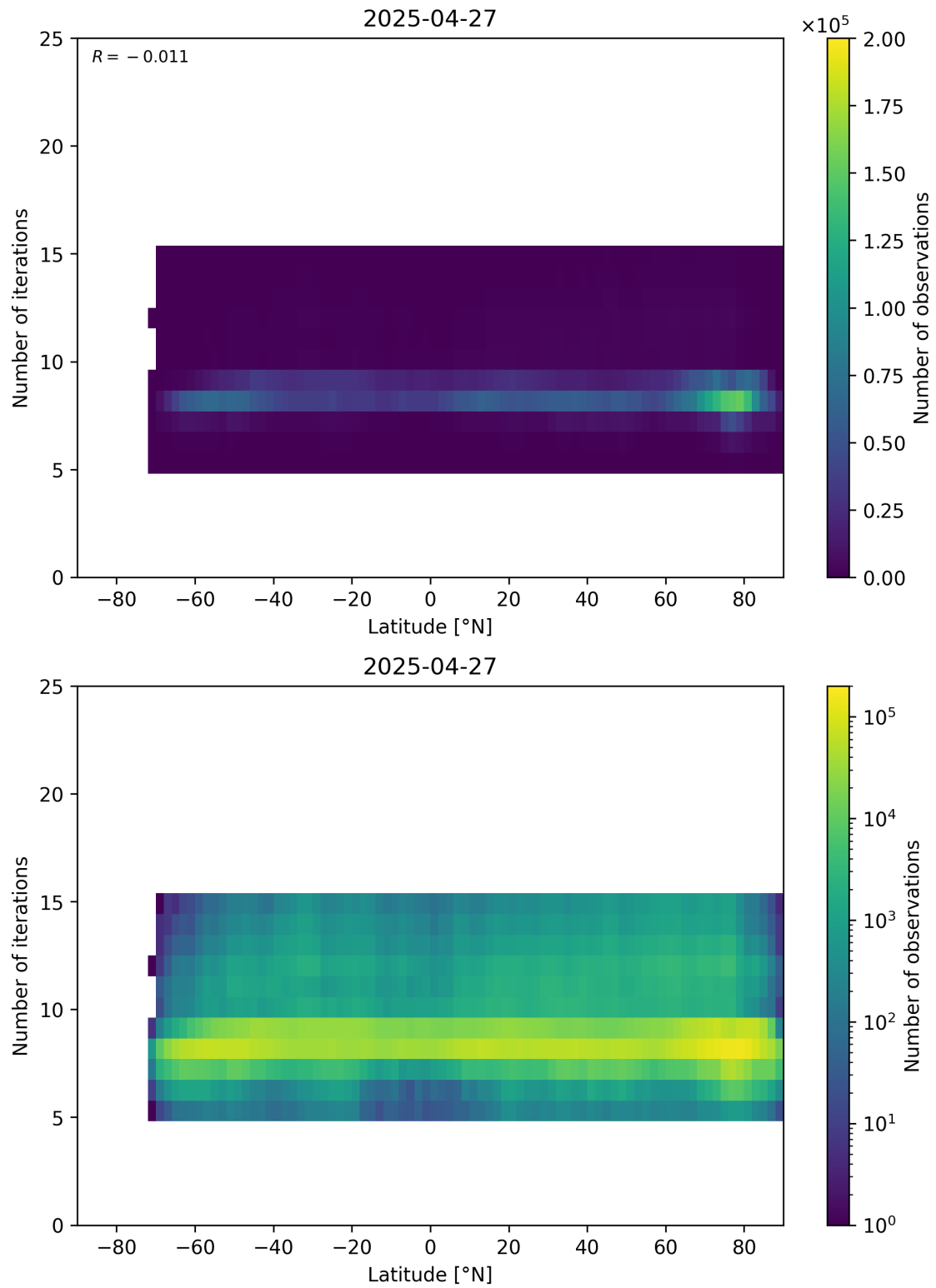
Figure 56: Scatter density plot of “Latitude” against “Number of iterations” for 2025-04-26 to 2025-04-28.
