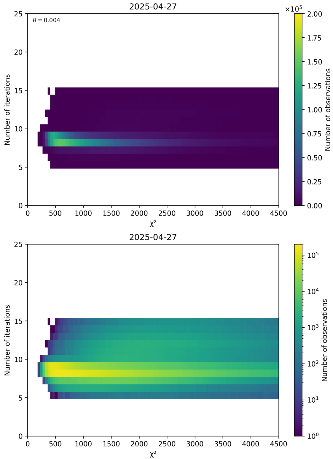
Figure 49: Scatter density plot of “ \chi^2 ” against “Number of iterations” for 2025-04-26 to 2025-04-28.
