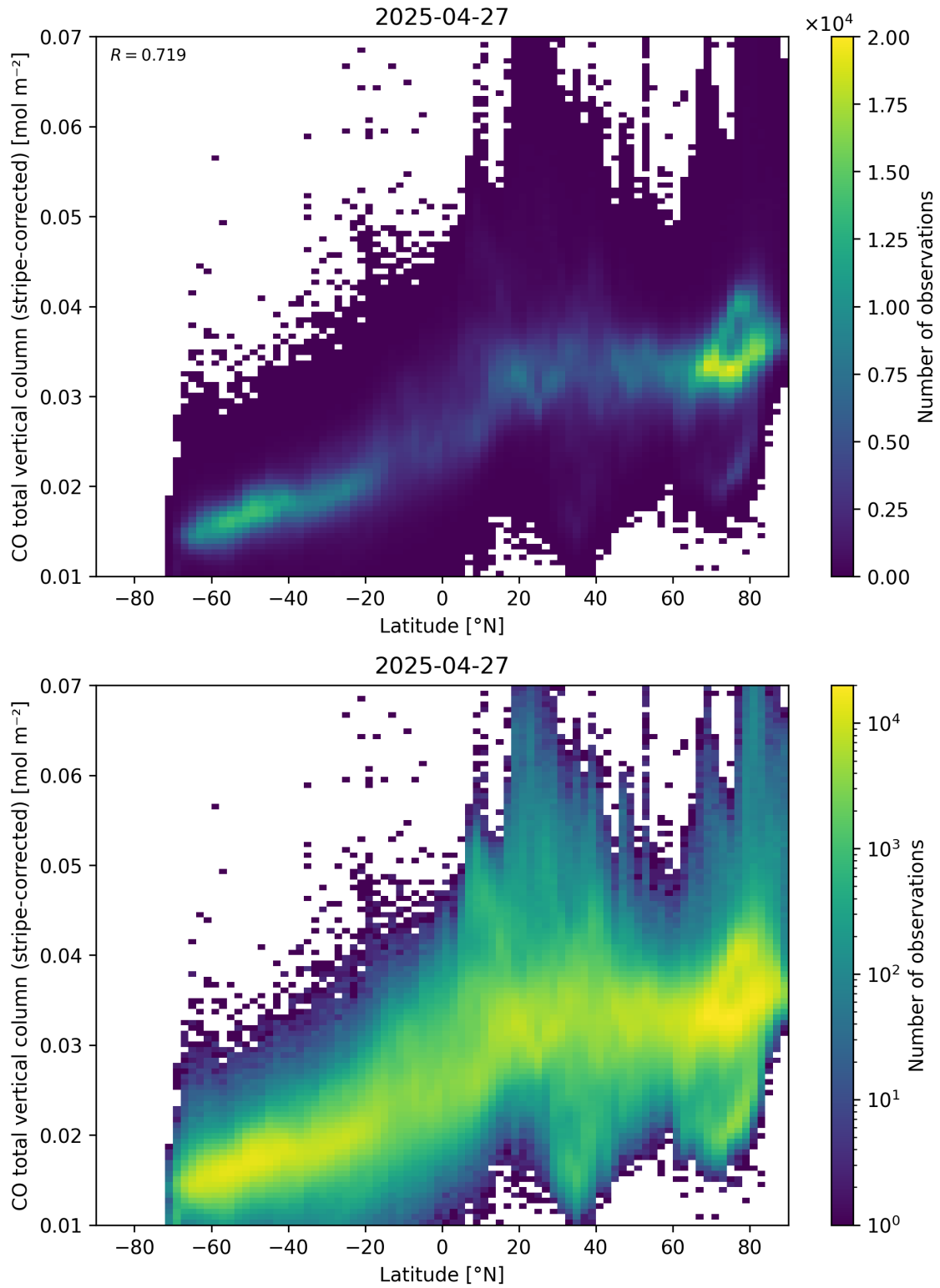
Figure 52: Scatter density plot of “Latitude” against “CO total vertical column (stripe-corrected)” for 2025-04-26 to 2025-04-28.
