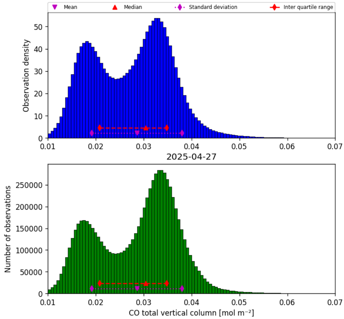
Figure 18: Histogram of “CO total vertical column” for 2025-04-26 to 2025-04-28
