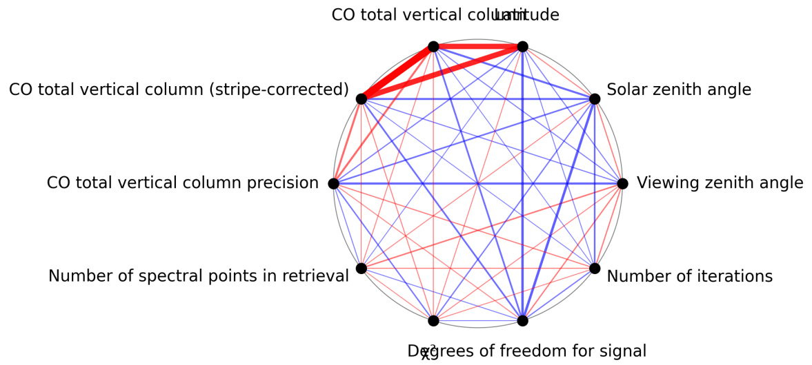
Figure 1: Map of correlation graph for 2025-04-26 to 2025-04-28.
