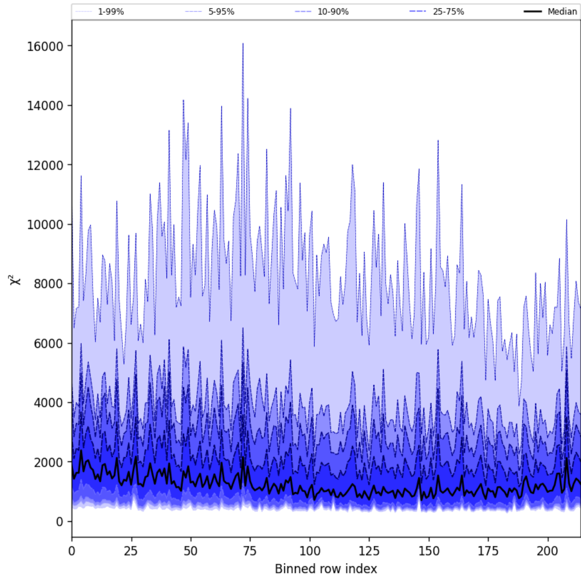
Figure 30: Along track statistics of “ \chi^2 ” for 2025-04-26 to 2025-04-28
