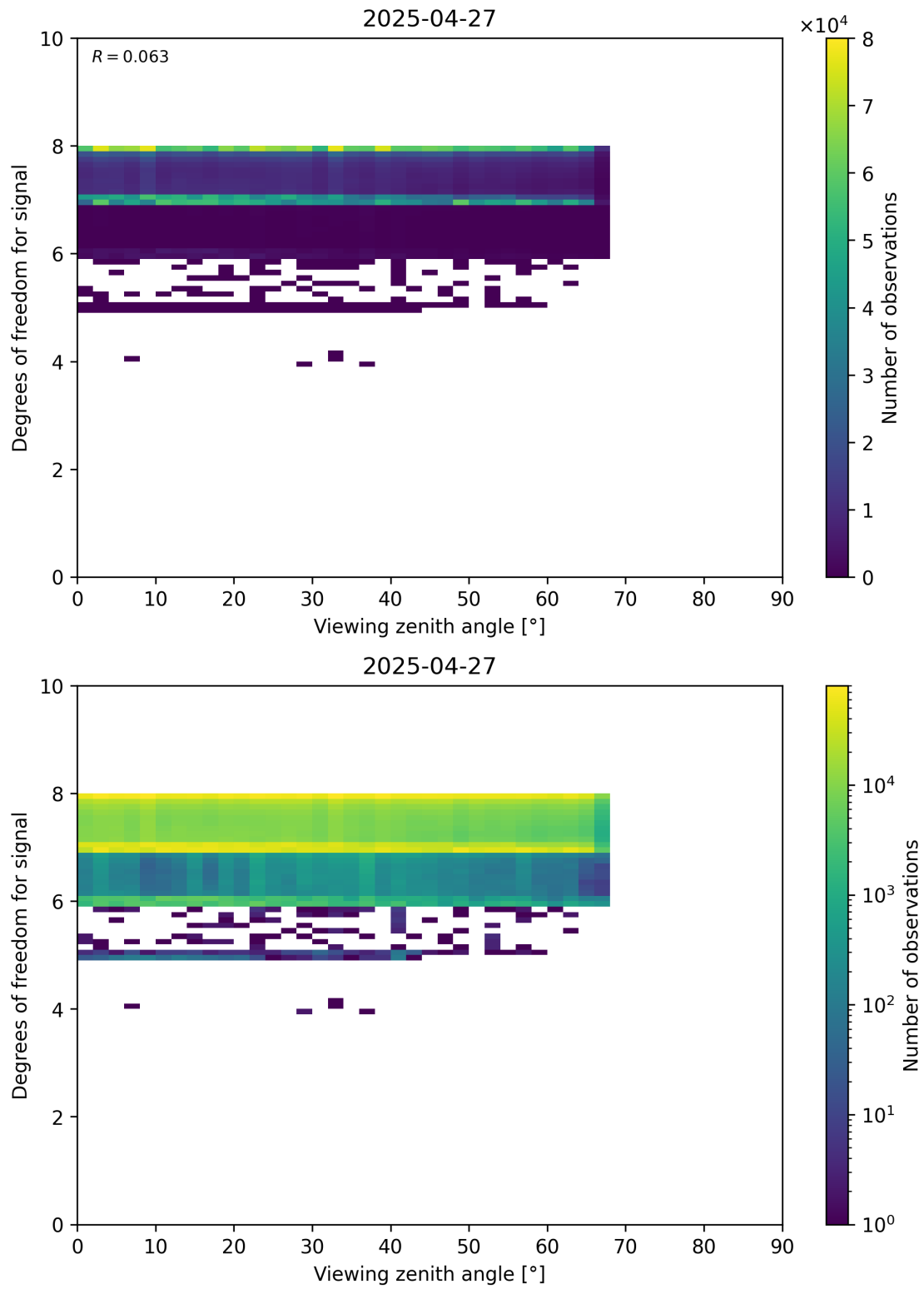
Figure 73: Scatter density plot of “Viewing zenith angle” against “Degrees of freedom for signal” for 2025-04-26 to 2025-04-28.
