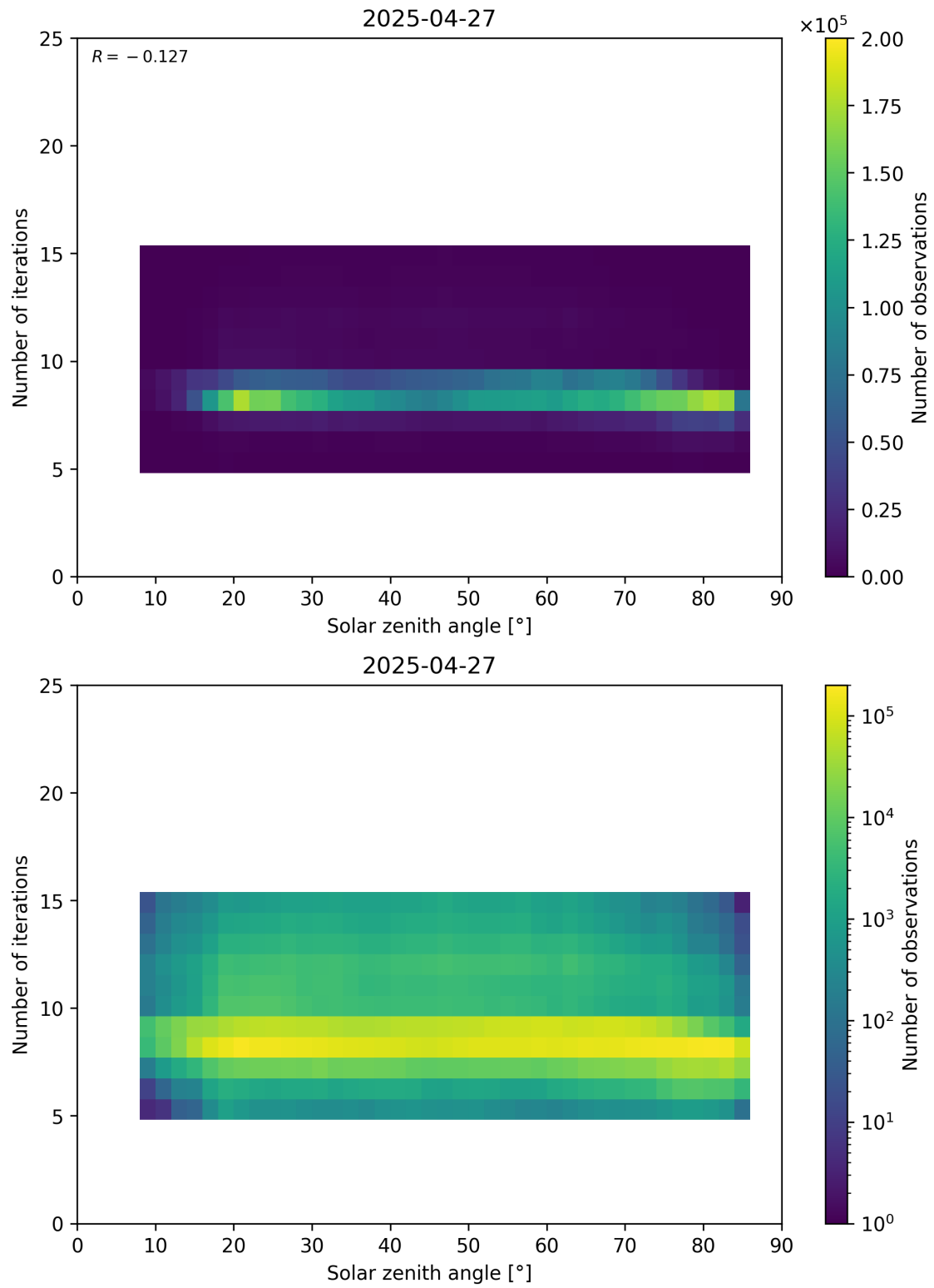
Figure 67: Scatter density plot of “Solar zenith angle” against “Number of iterations” for 2025-04-26 to 2025-04-28.
