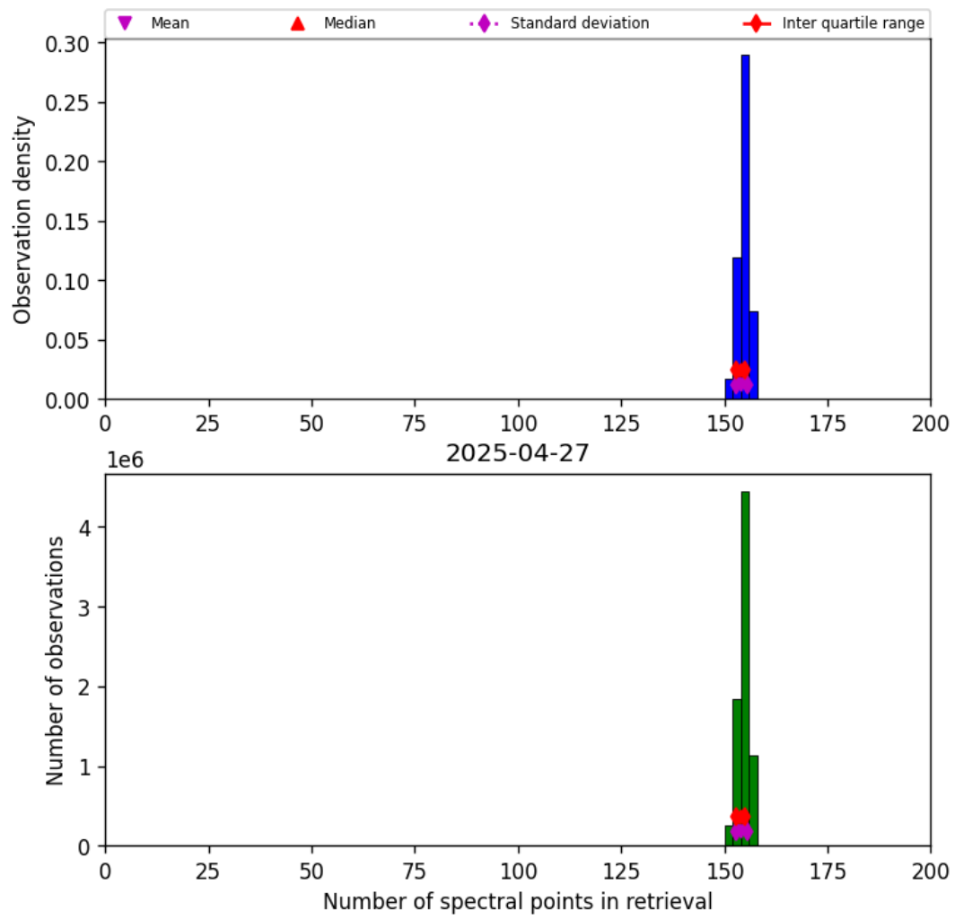
Figure 21: Histogram of “Number of spectral points in retrieval” for 2025-04-26 to 2025-04-28
