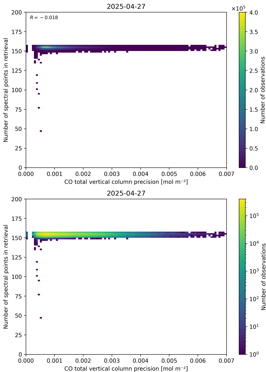
Figure 47: Scatter density plot of “CO total vertical column precision” against “Number of spectral points in retrieval” for 2025-04-26 to 2025-04-28.
