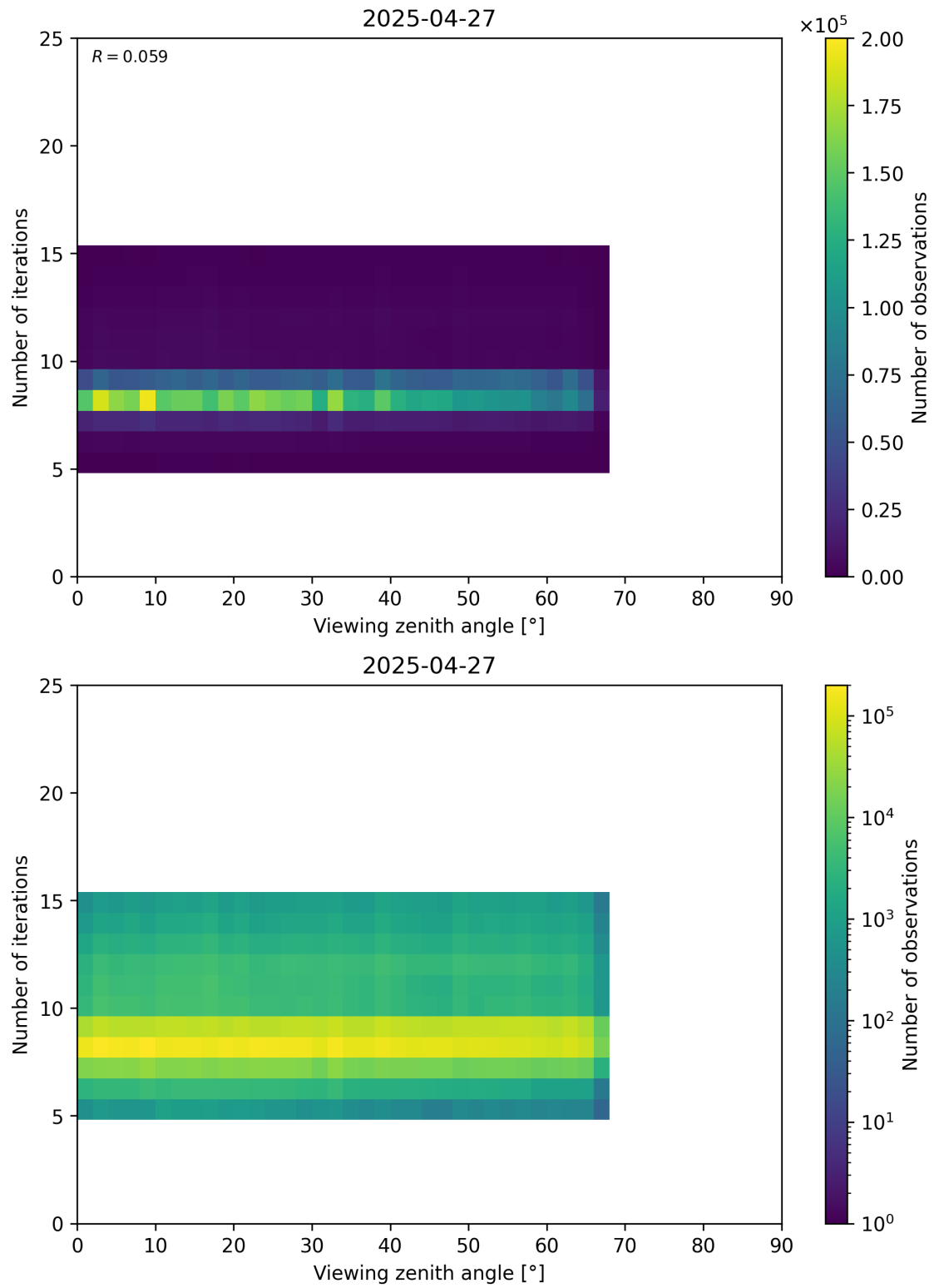
Figure 75: Scatter density plot of “Viewing zenith angle” against “Number of iterations” for 2025-04-26 to 2025-04-28.
