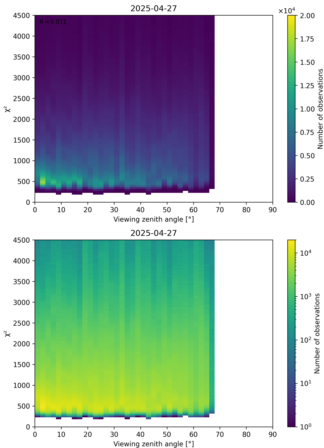
Figure 72: Scatter density plot of “Viewing zenith angle” against “ \chi^2 ” for 2025-04-26 to 2025-04-28.
