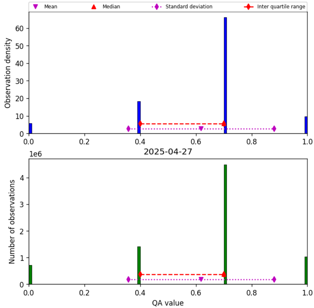
Figure 17: Histogram of “QA value” for 2025-04-26 to 2025-04-28
