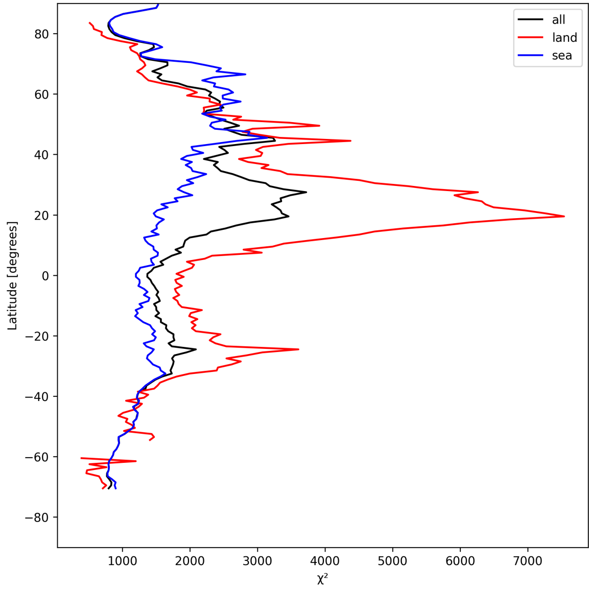
Figure 14: Zonal average of “ \chi^2 ” for 2025-04-26 to 2025-04-28.
