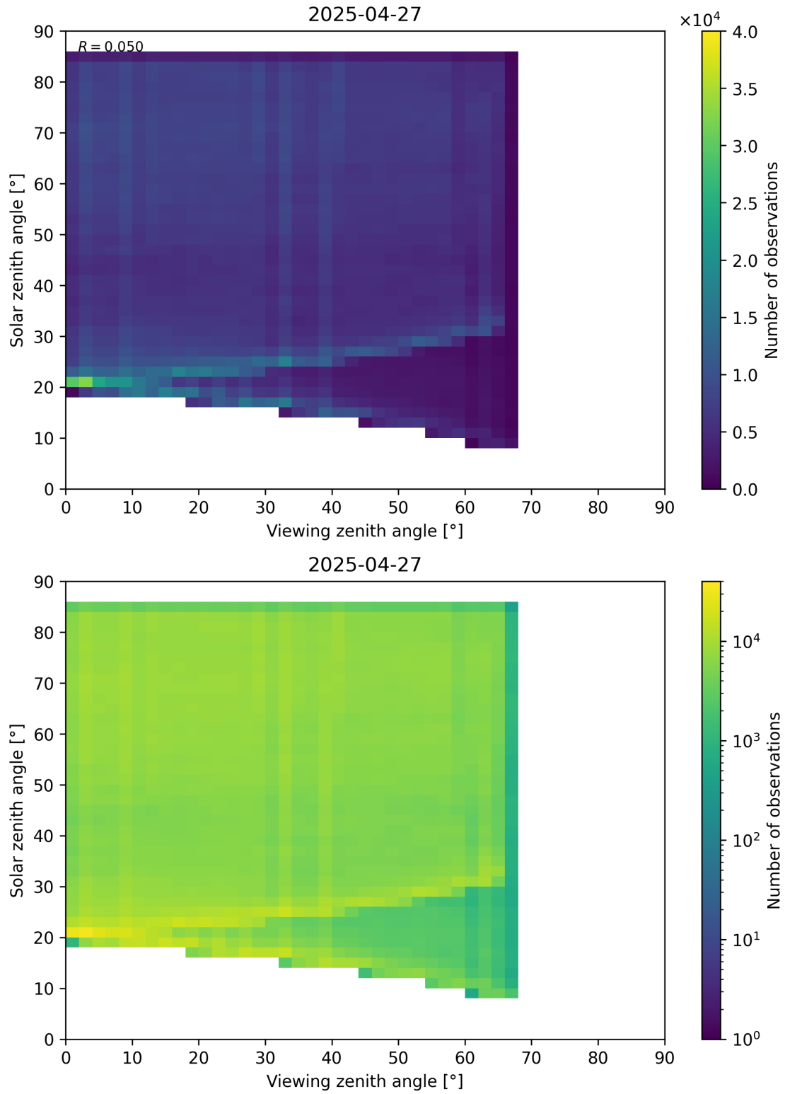
Figure 77: Scatter density plot of “Viewing zenith angle” against “Solar zenith angle” for 2025-04-26 to 2025-04-28.
