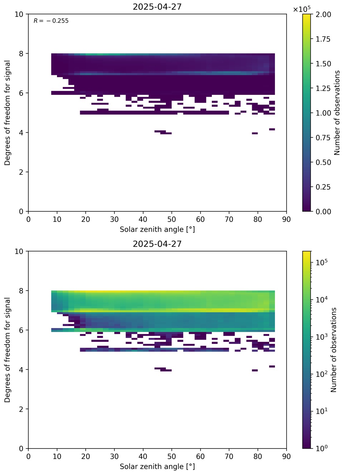
Figure 65: Scatter density plot of “Solar zenith angle” against “Degrees of freedom for signal” for 2025-04-26 to 2025-04-28.
