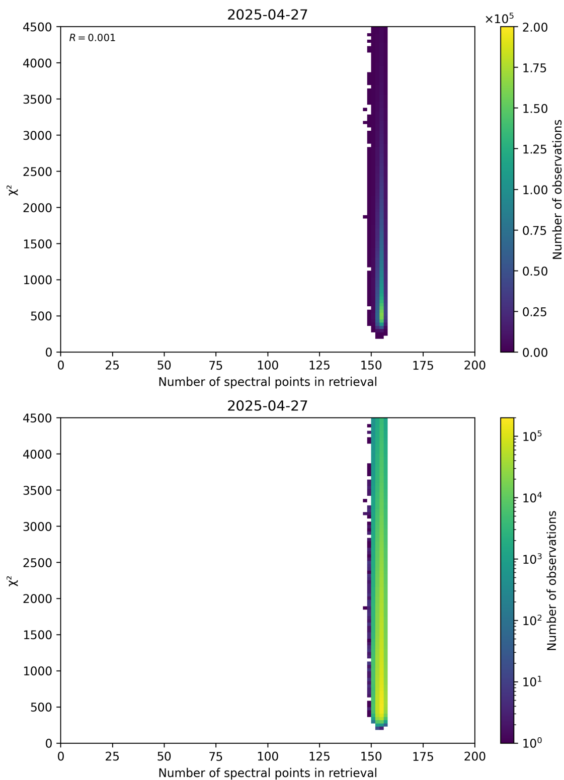
Figure 58: Scatter density plot of “Number of spectral points in retrieval” against “ \chi^2 ” for 2025-04-26 to 2025-04-28.
