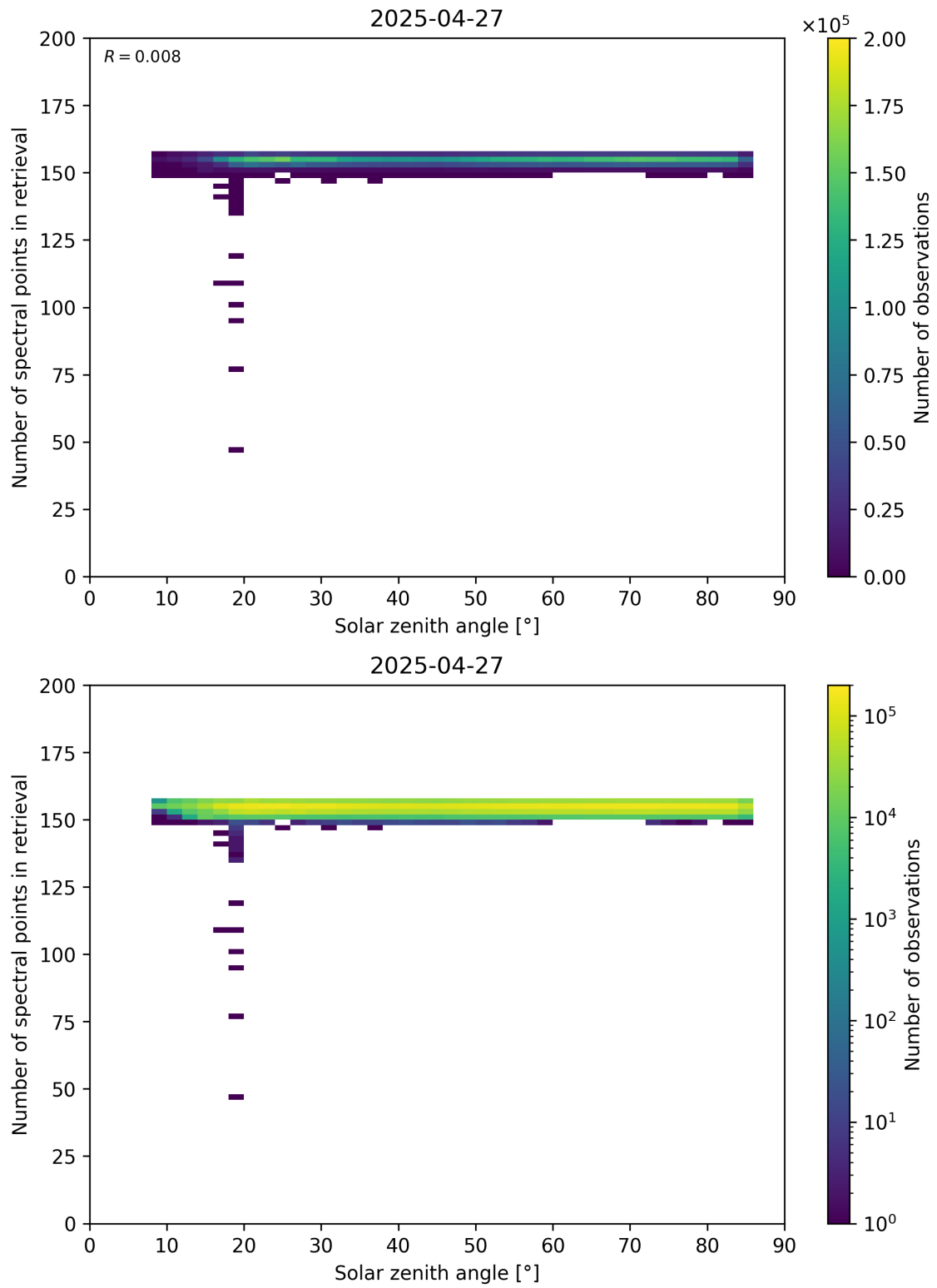
Figure 68: Scatter density plot of “Solar zenith angle” against “Number of spectral points in retrieval” for 2025-04-26 to 2025-04-28.
