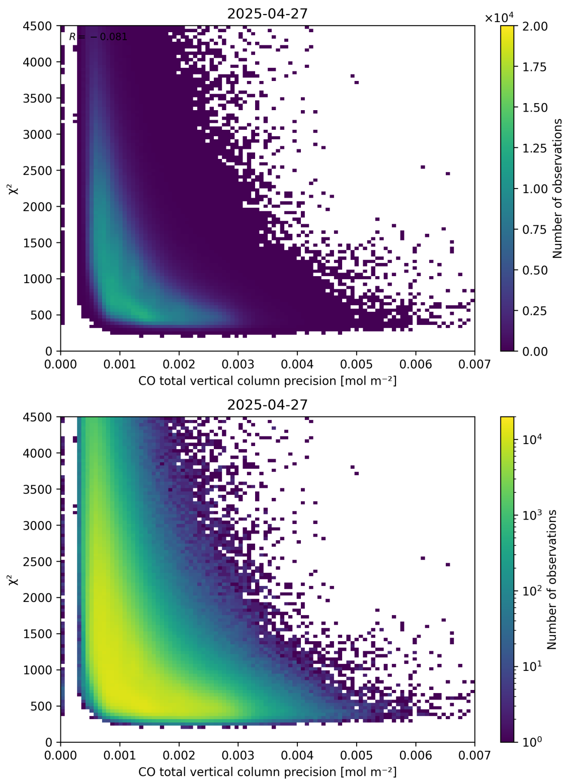
Figure 44: Scatter density plot of “CO total vertical column precision” against “ \chi^2 ” for 2025-04-26 to 2025-04-28.
