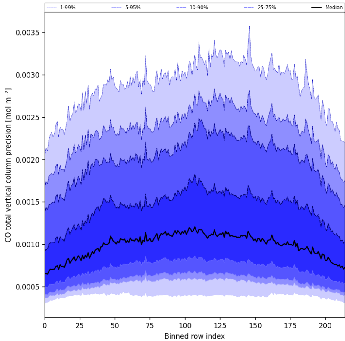
Figure 28: Along track statistics of “CO total vertical column precision” for 2025-04-26 to 2025-04-28
