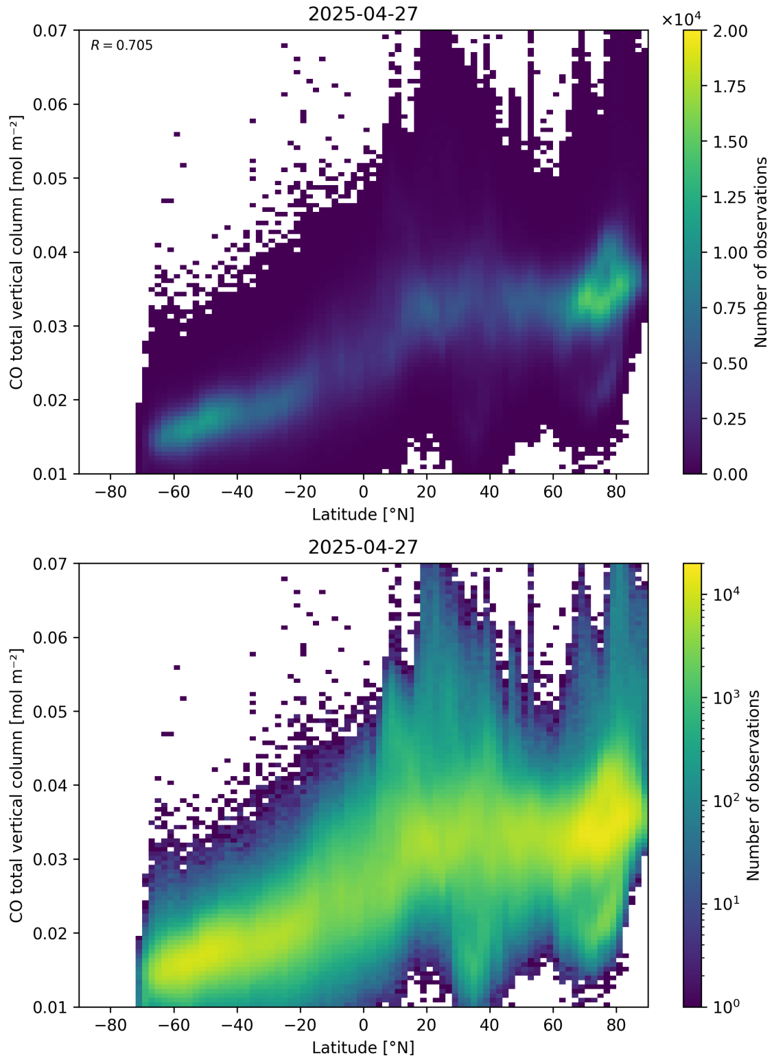
Figure 51: Scatter density plot of “Latitude” against “CO total vertical column” for 2025-04-26 to 2025-04-28.
