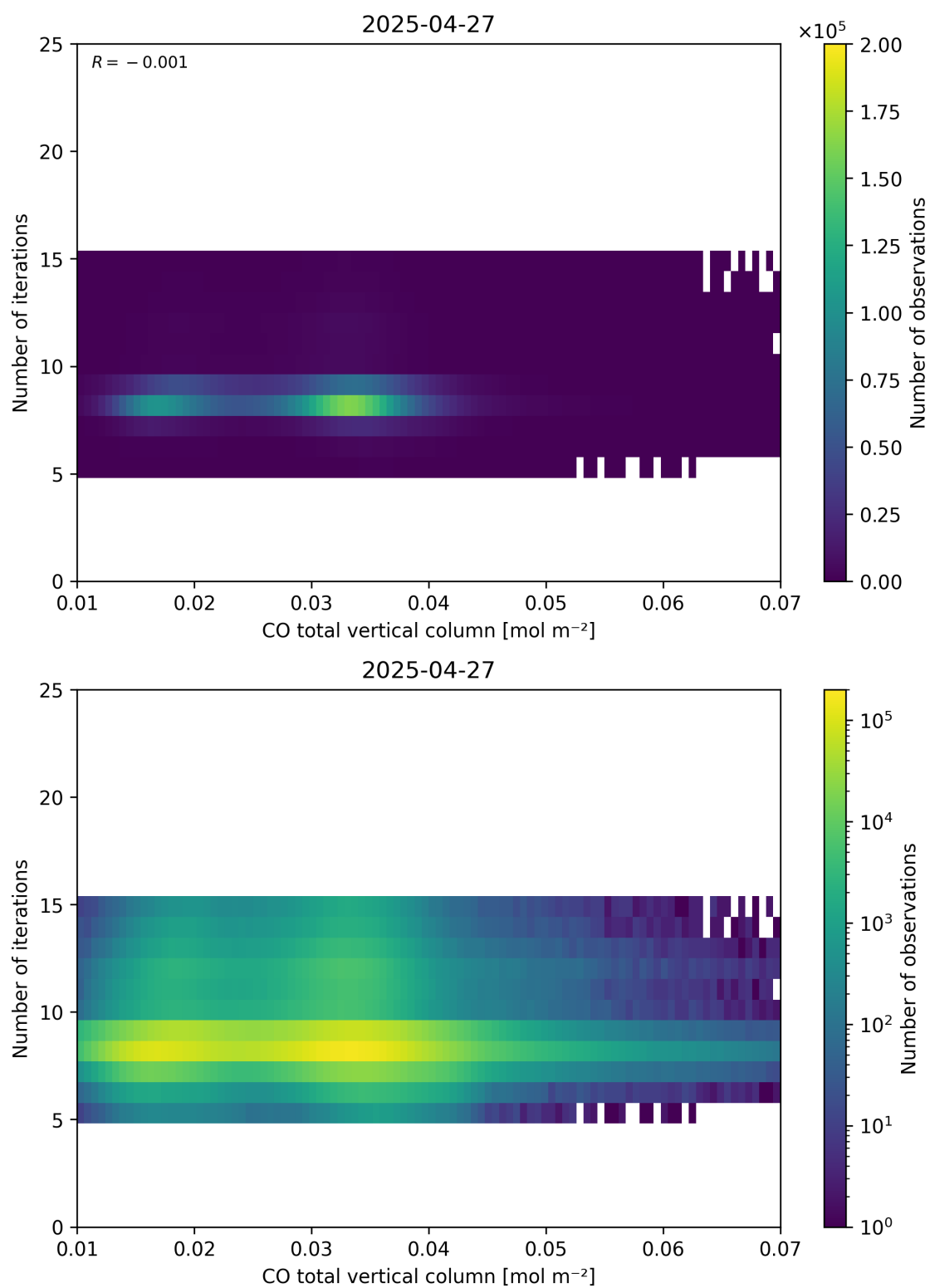
Figure 42: Scatter density plot of “CO total vertical column” against “Number of iterations” for 2025-04-26 to 2025-04-28.
