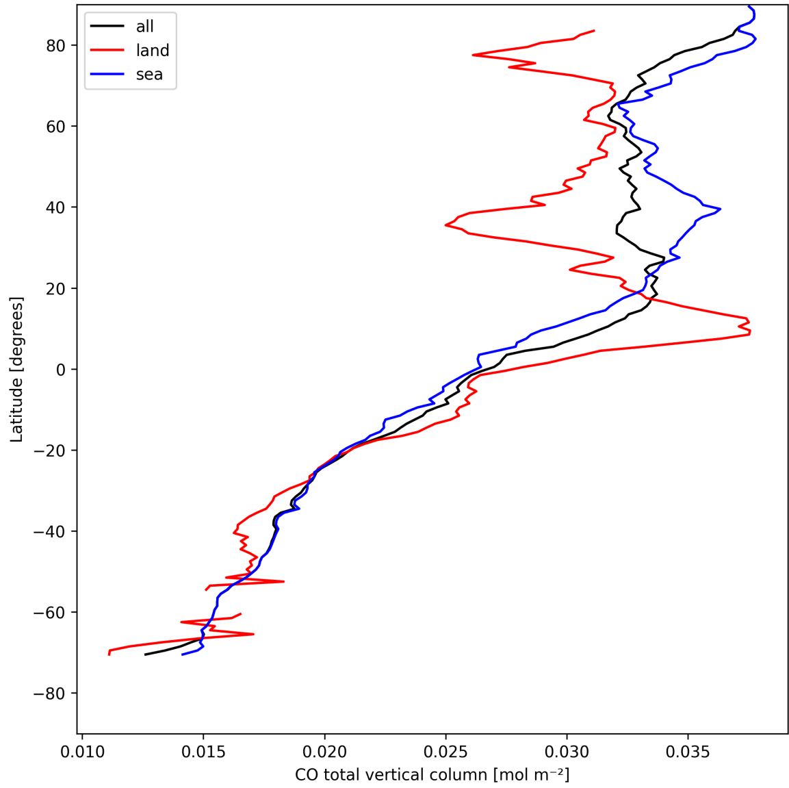
Figure 10: Zonal average of “CO total vertical column” for 2025-04-26 to 2025-04-28.
