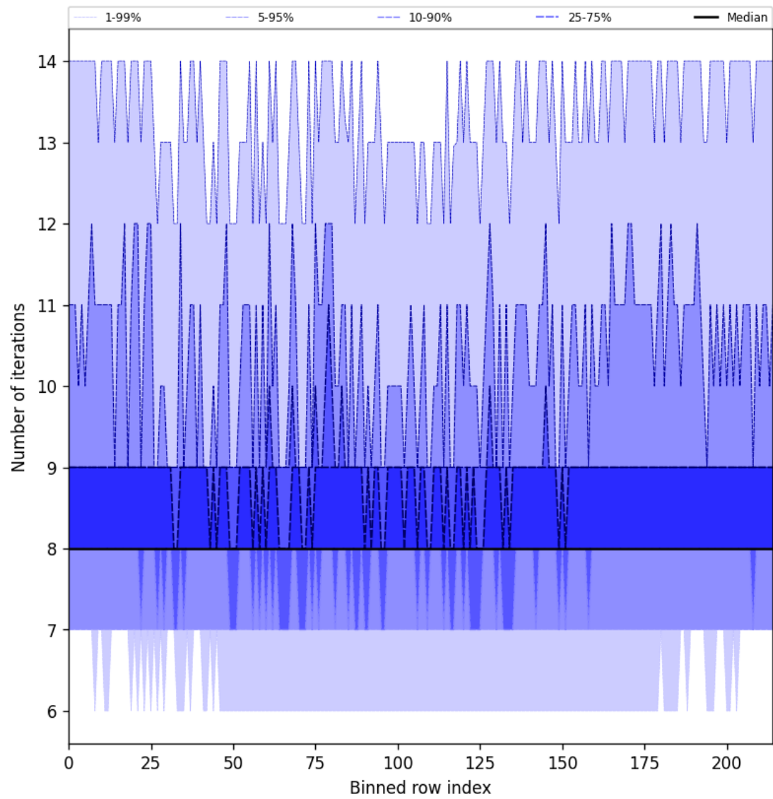
Figure 32: Along track statistics of “Number of iterations” for 2025-04-26 to 2025-04-28
