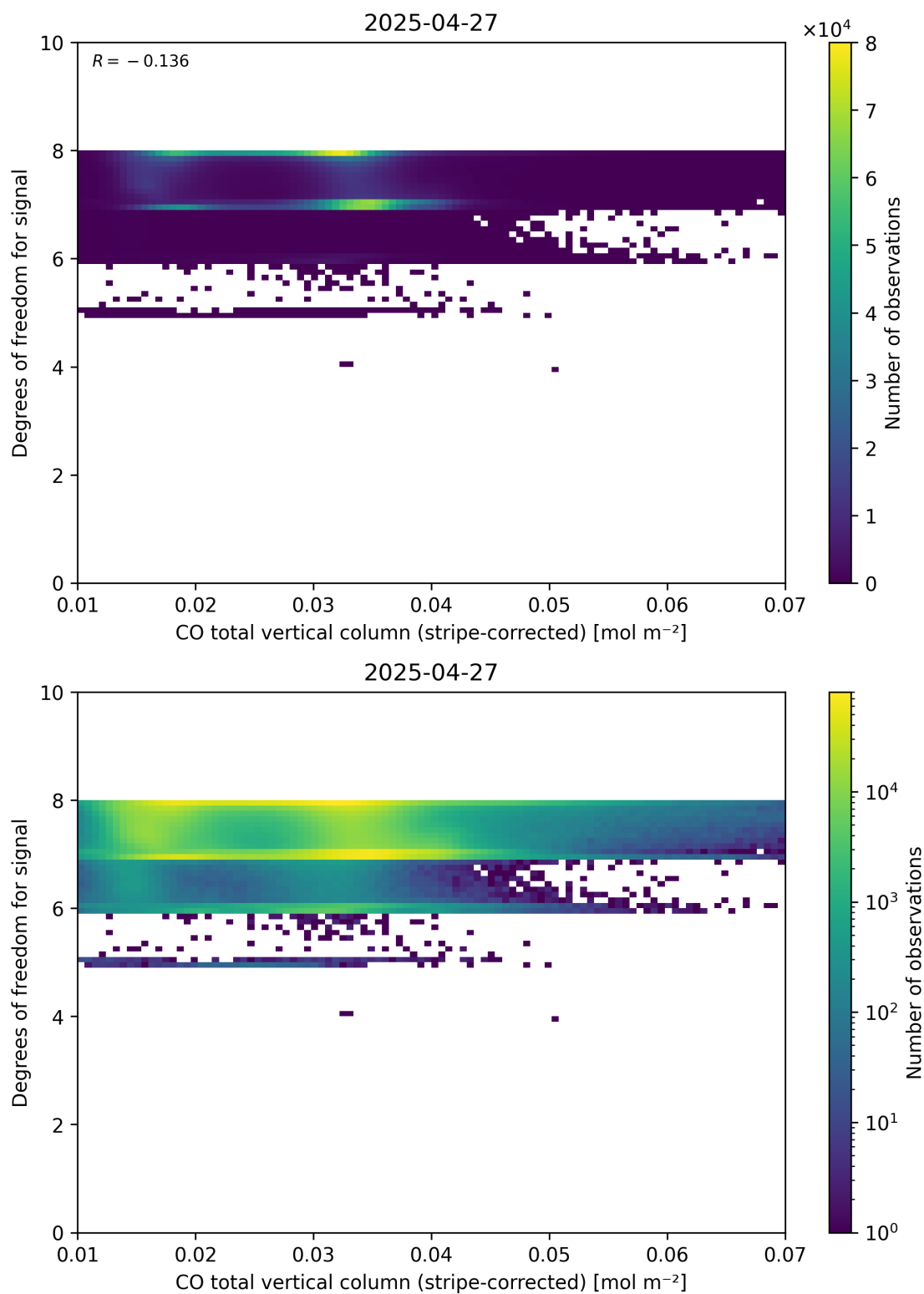
Figure 38: Scatter density plot of “CO total vertical column (stripe-corrected)” against “Degrees of freedom for signal” for 2025-04-26 to 2025-04-28.
