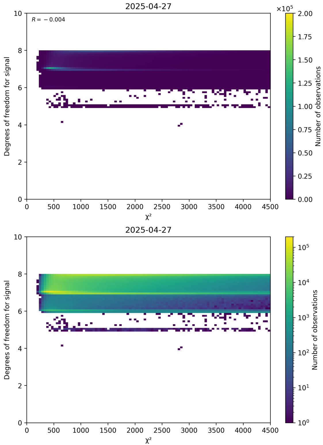
Figure 48: Scatter density plot of “ \chi^2 ” against “Degrees of freedom for signal” for 2025-04-26 to 2025-04-28.
