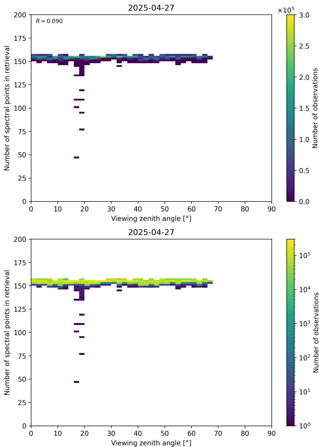
Figure 76: Scatter density plot of “Viewing zenith angle” against “Number of spectral points in retrieval” for 2025-04-26 to 2025-04-28.
