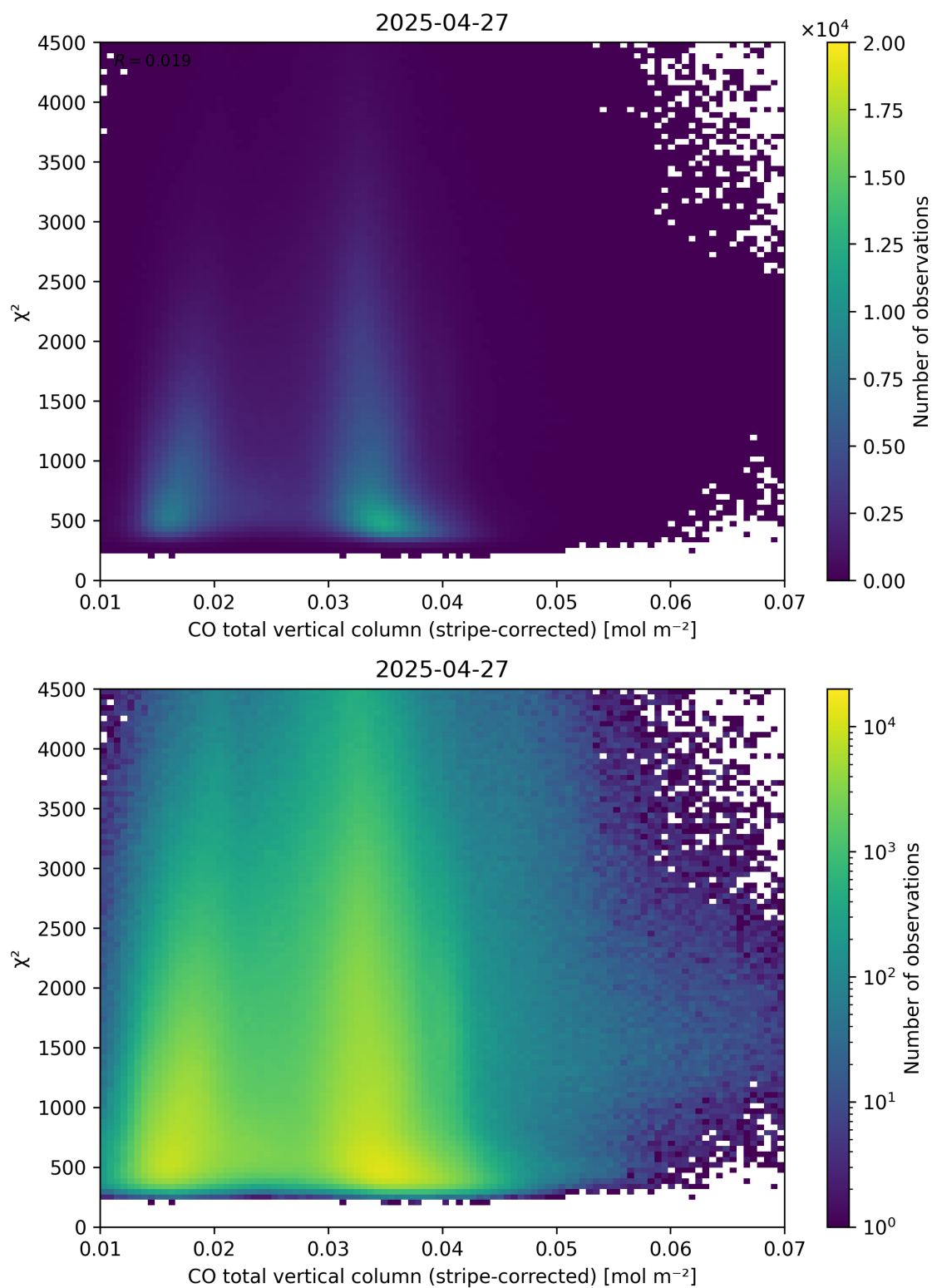
Figure 37: Scatter density plot of “CO total vertical column (stripe-corrected)” against “ \chi^2 ” for 2025-04-26 to 2025-04-28.
