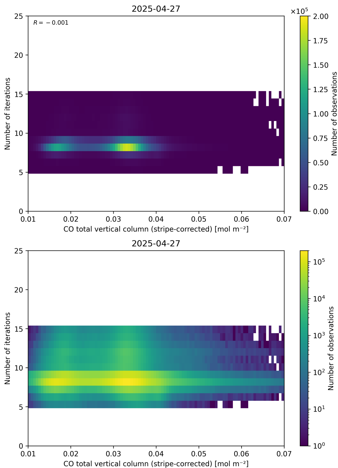
Figure 39: Scatter density plot of “CO total vertical column (stripe-corrected)” against “Number of iterations” for 2025-04-26 to 2025-04-28.
