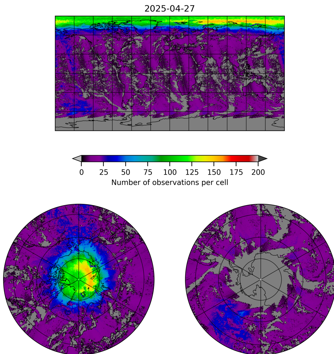
Figure 8: Map of the number of observations for 2025-04-26 to 2025-04-28
