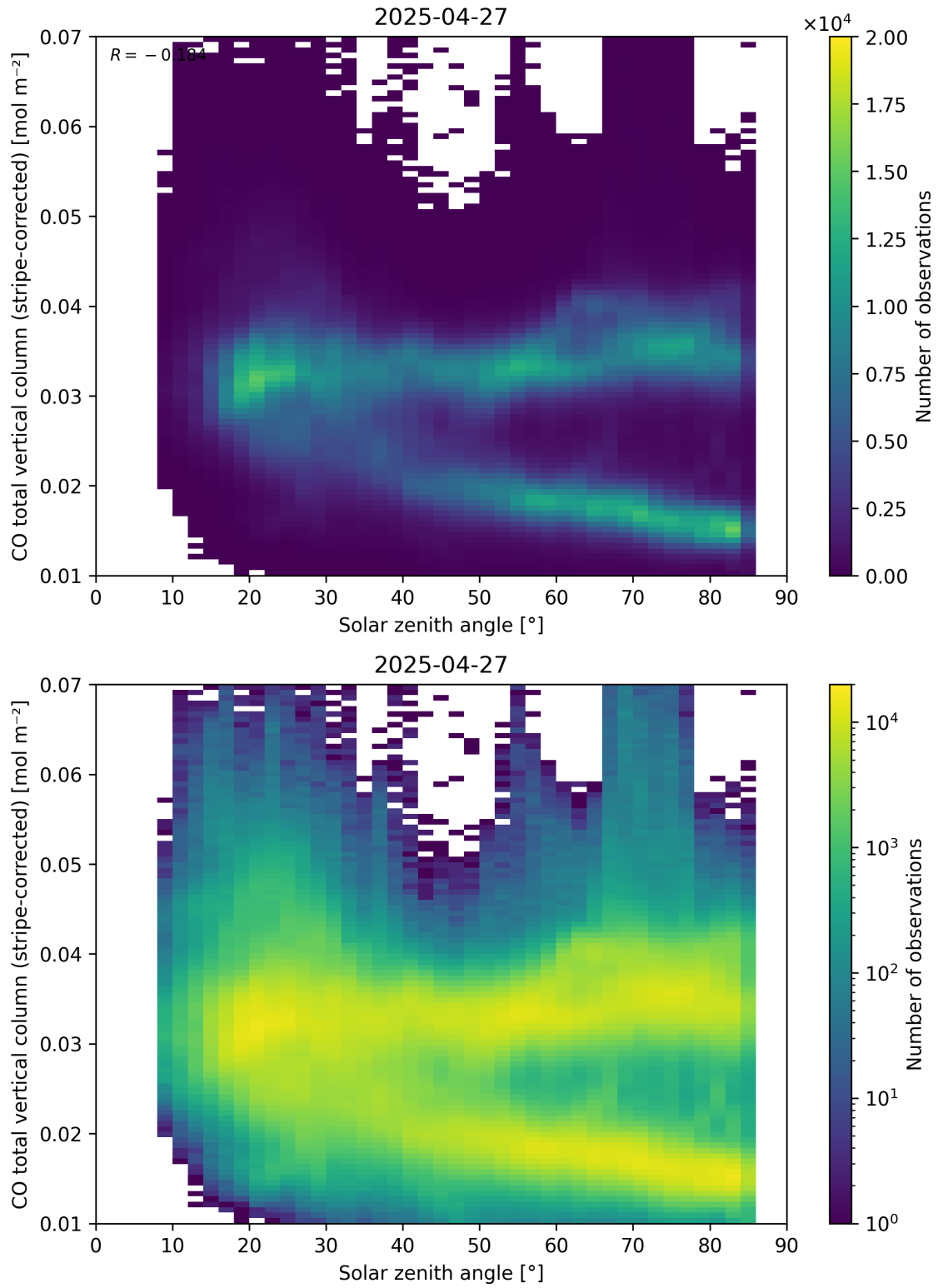
Figure 62: Scatter density plot of “Solar zenith angle” against “CO total vertical column (stripe-corrected)” for 2025-04-26 to 2025-04-28.
