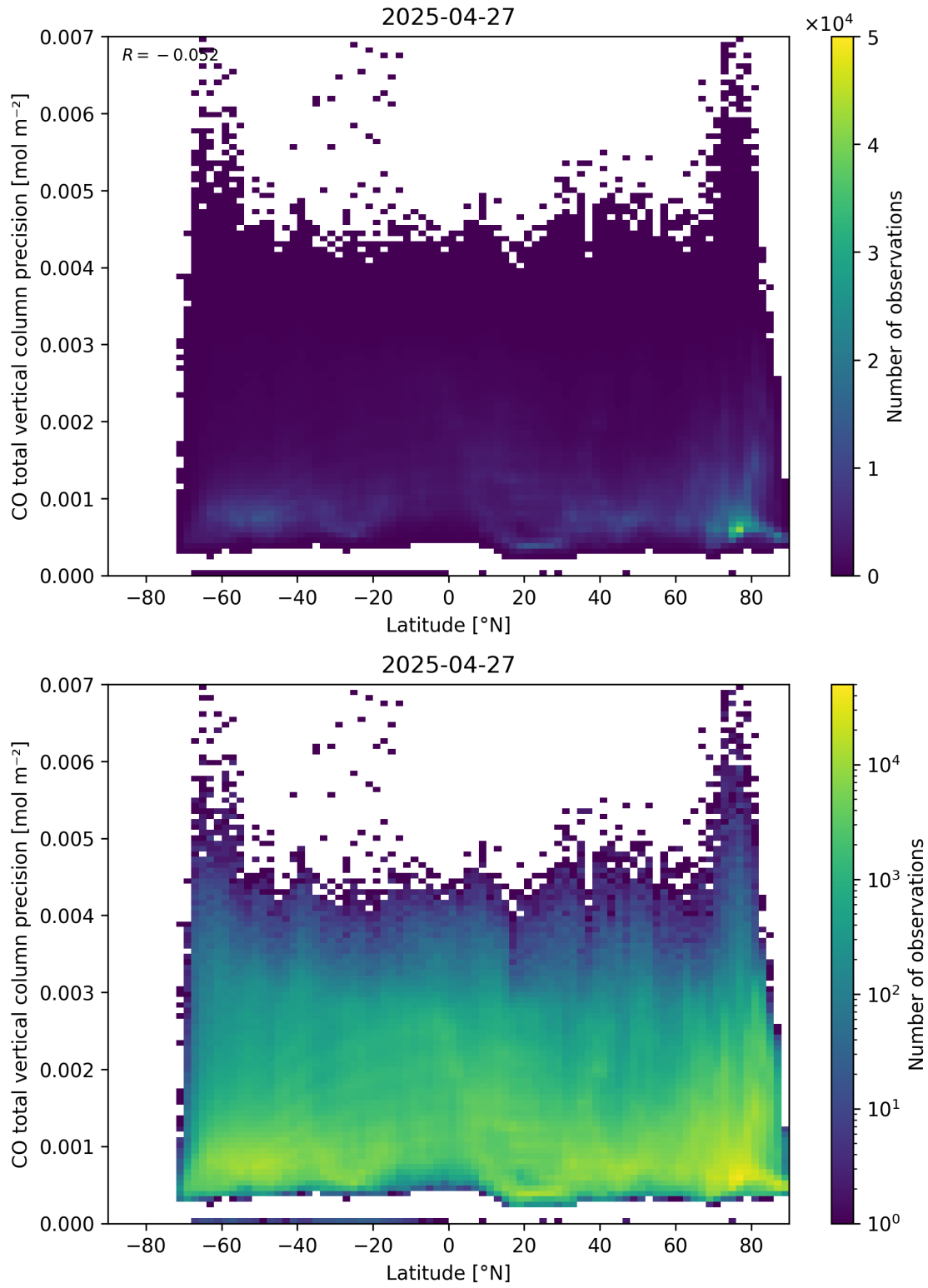
Figure 53: Scatter density plot of “Latitude” against “CO total vertical column precision” for 2025-04-26 to 2025-04-28.
