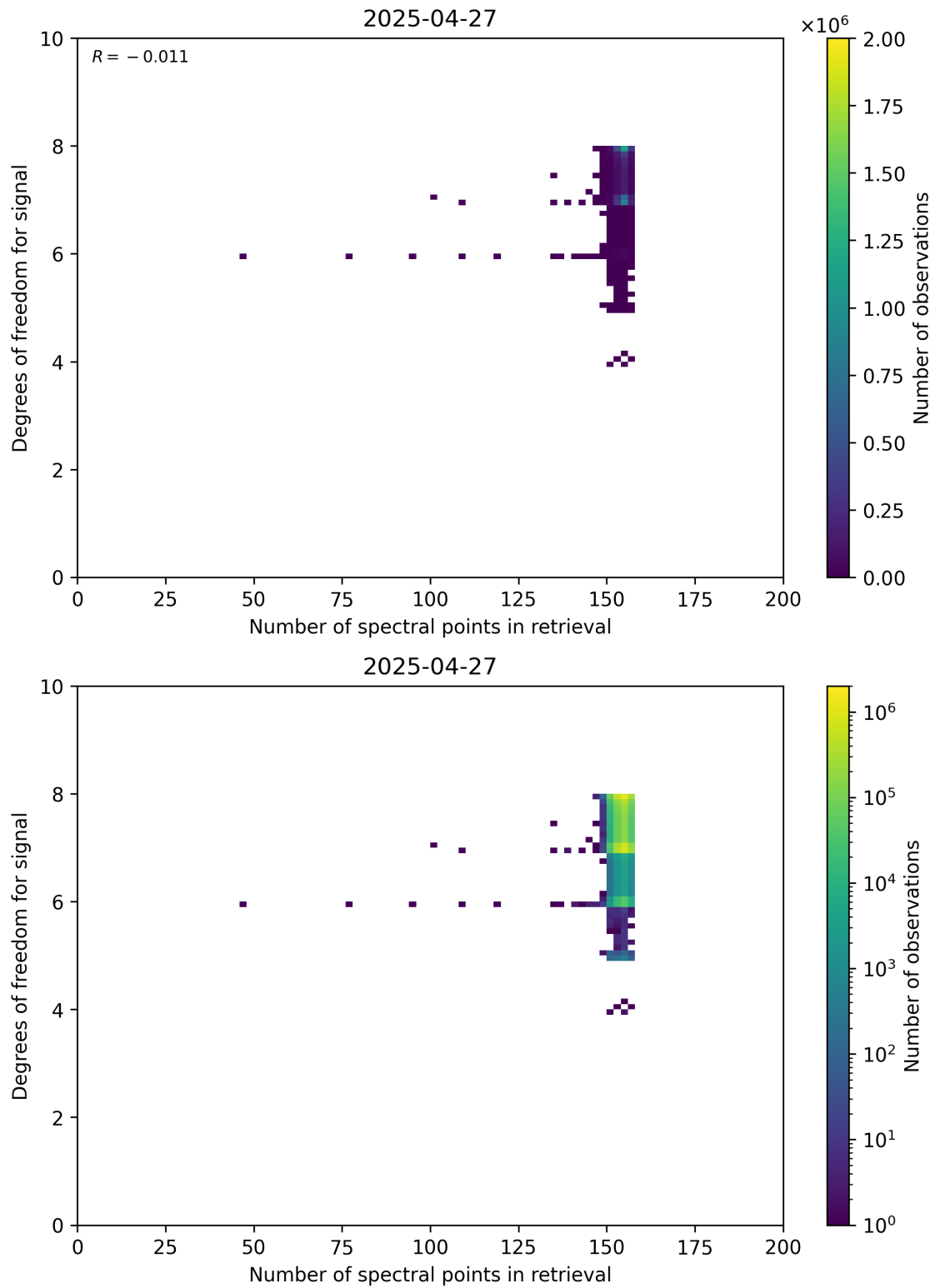
Figure 59: Scatter density plot of “Number of spectral points in retrieval” against “Degrees of freedom for signal” for 2025-04-26 to 2025-04-28.
