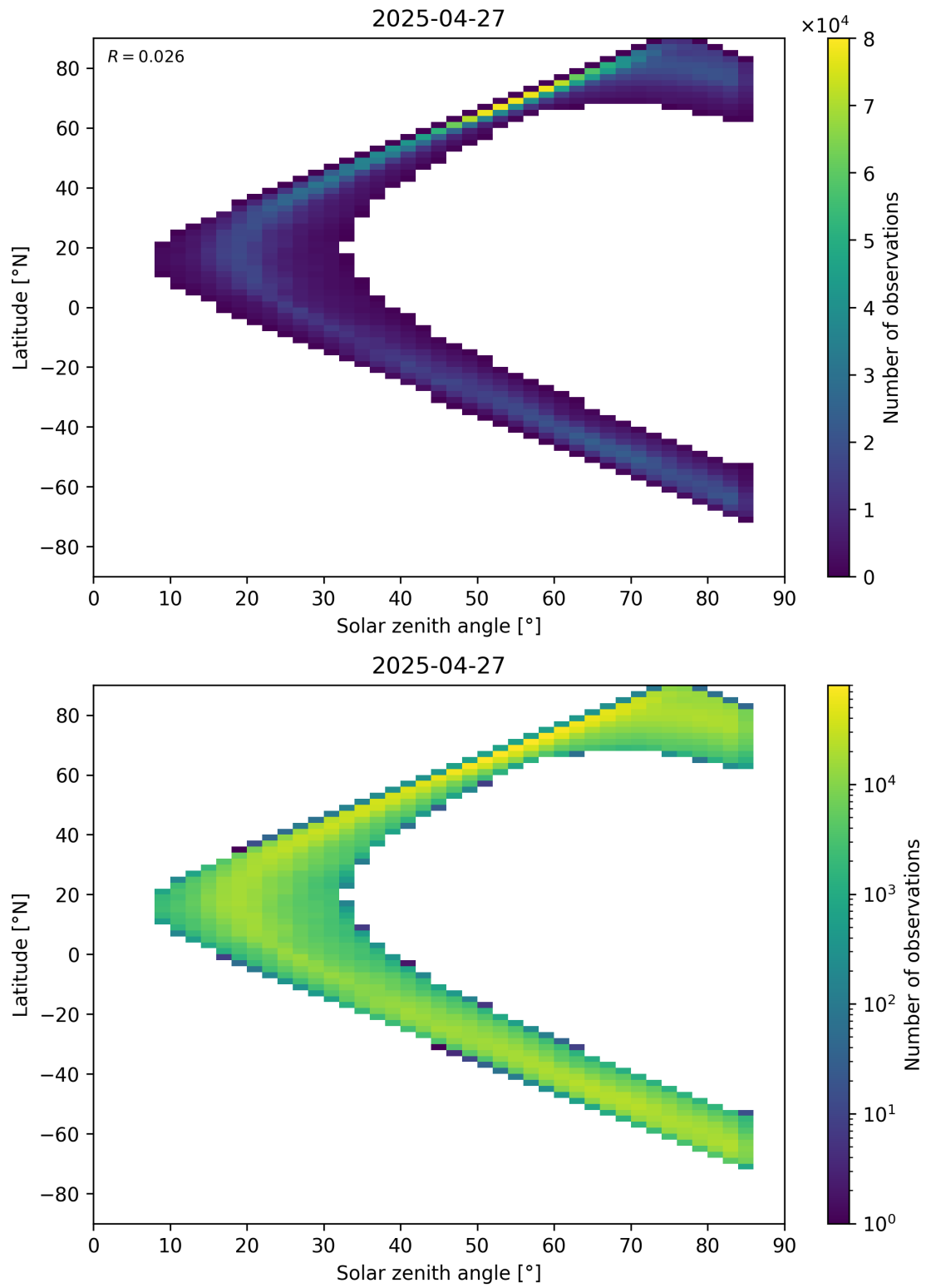
Figure 66: Scatter density plot of “Solar zenith angle” against “Latitude” for 2025-04-26 to 2025-04-28.
