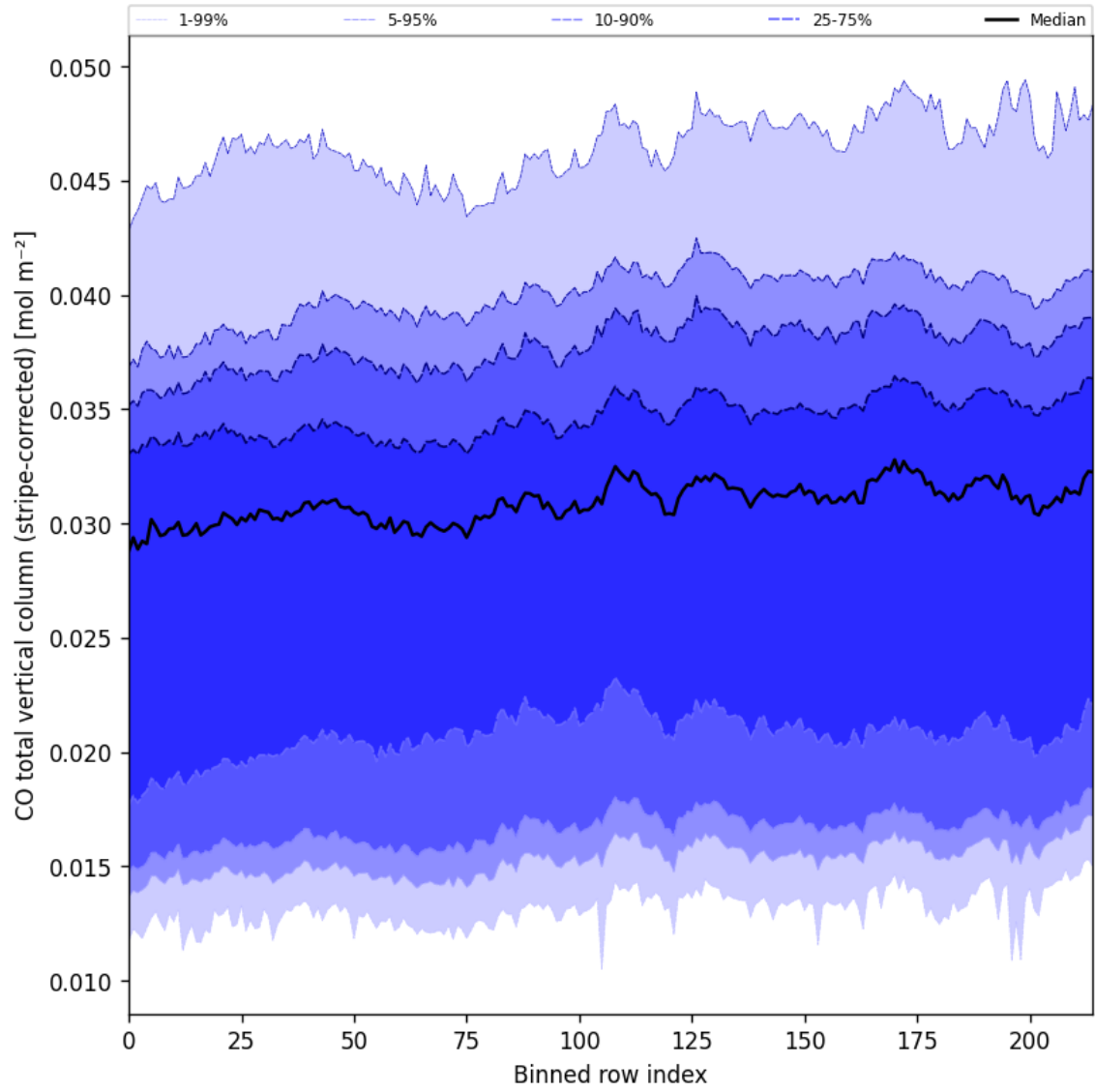
Figure 27: Along track statistics of “CO total vertical column (stripe-corrected)” for 2025-04-26 to 2025-04-28
