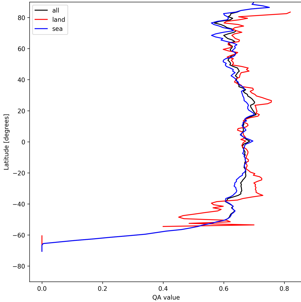
Figure 9: Zonal average of “QA value” for 2025-04-26 to 2025-04-28.
