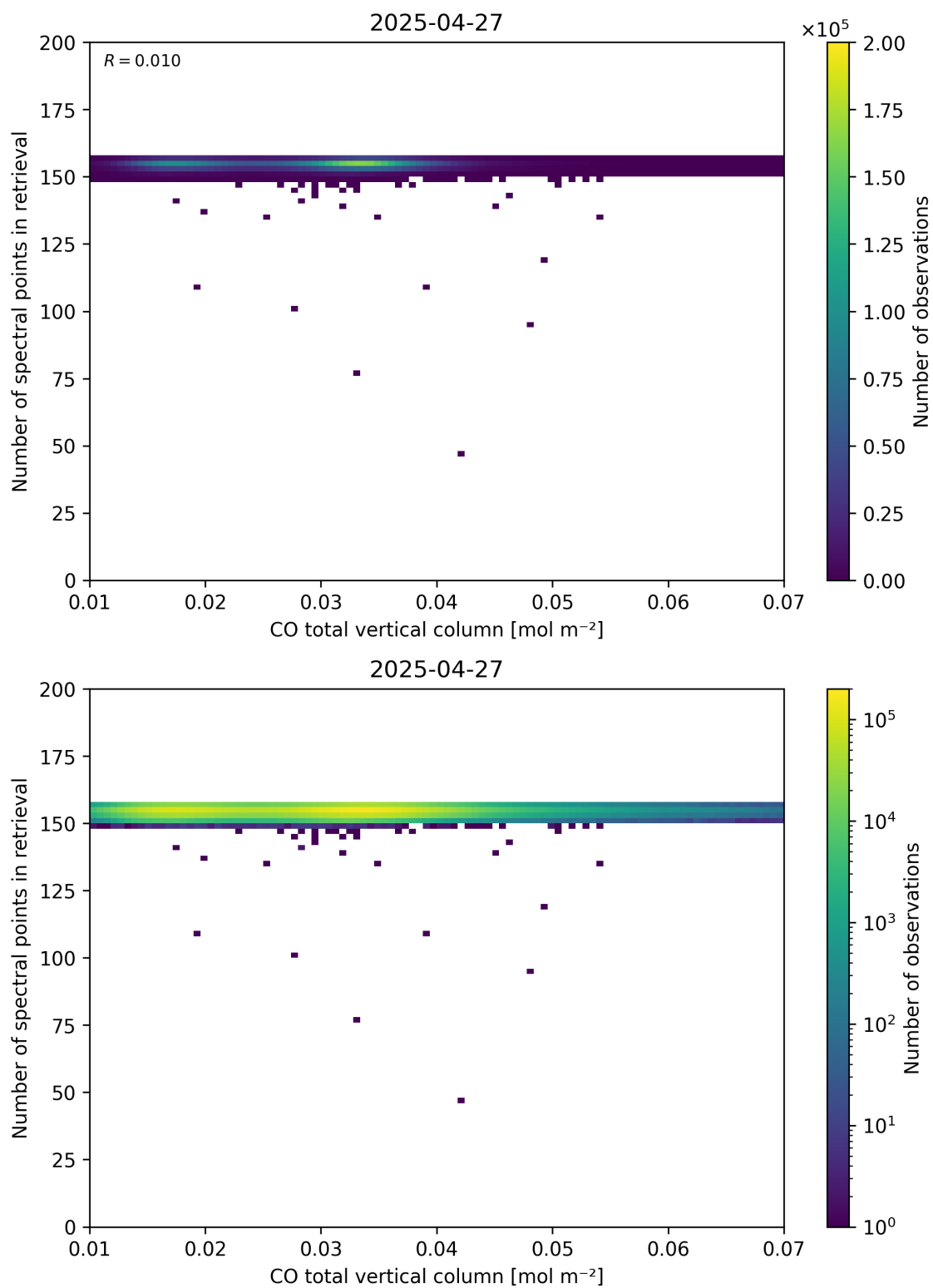
Figure 43: Scatter density plot of “CO total vertical column” against “Number of spectral points in retrieval” for 2025-04-26 to 2025-04-28.
