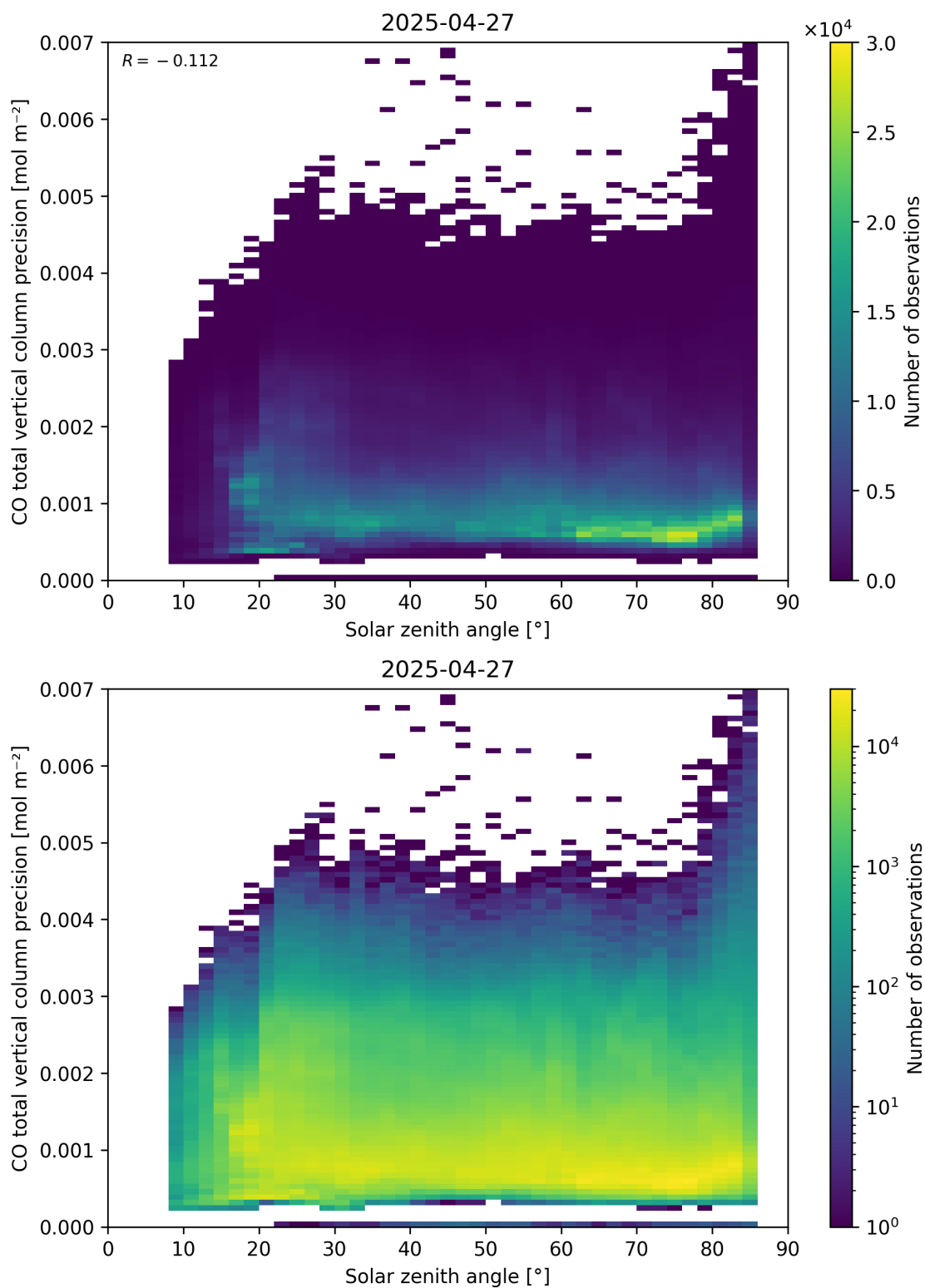
Figure 63: Scatter density plot of “Solar zenith angle” against “CO total vertical column precision” for 2025-04-26 to 2025-04-28.
