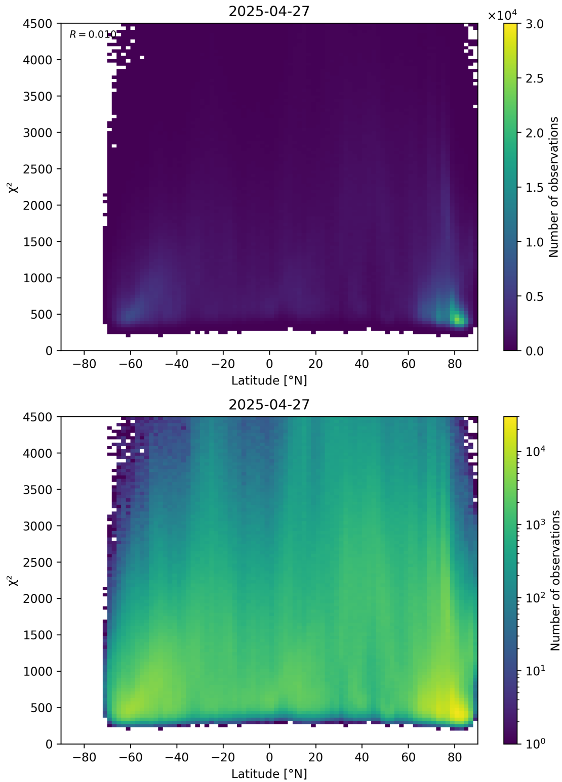
Figure 54: Scatter density plot of “Latitude” against “ \chi^2 ” for 2025-04-26 to 2025-04-28.
