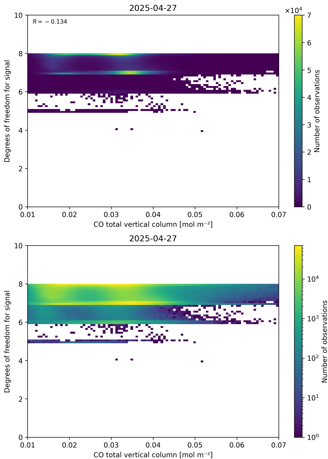
Figure 41: Scatter density plot of “CO total vertical column” against “Degrees of freedom for signal” for 2025-04-26 to 2025-04-28.
