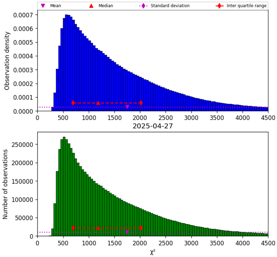
Figure 22: Histogram of “ \chi^2 ” for 2025-04-26 to 2025-04-28
