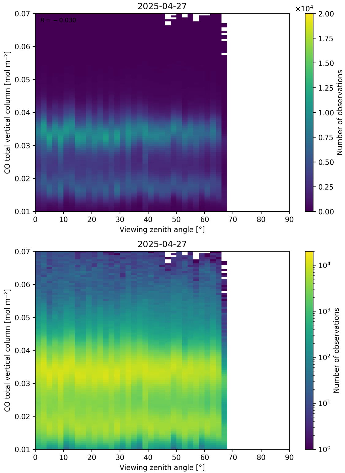
Figure 69: Scatter density plot of “Viewing zenith angle” against “CO total vertical column” for 2025-04-26 to 2025-04-28.
