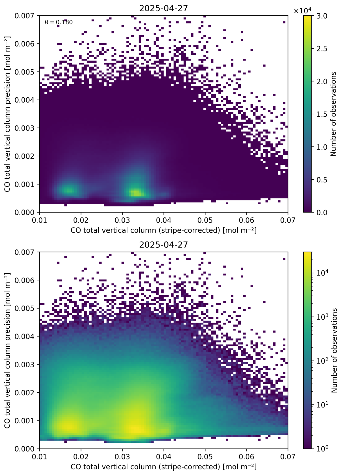
Figure 36: Scatter density plot of “CO total vertical column (stripe-corrected)” against “CO total vertical column precision” for 2025-04-26 to 2025-04-28.
