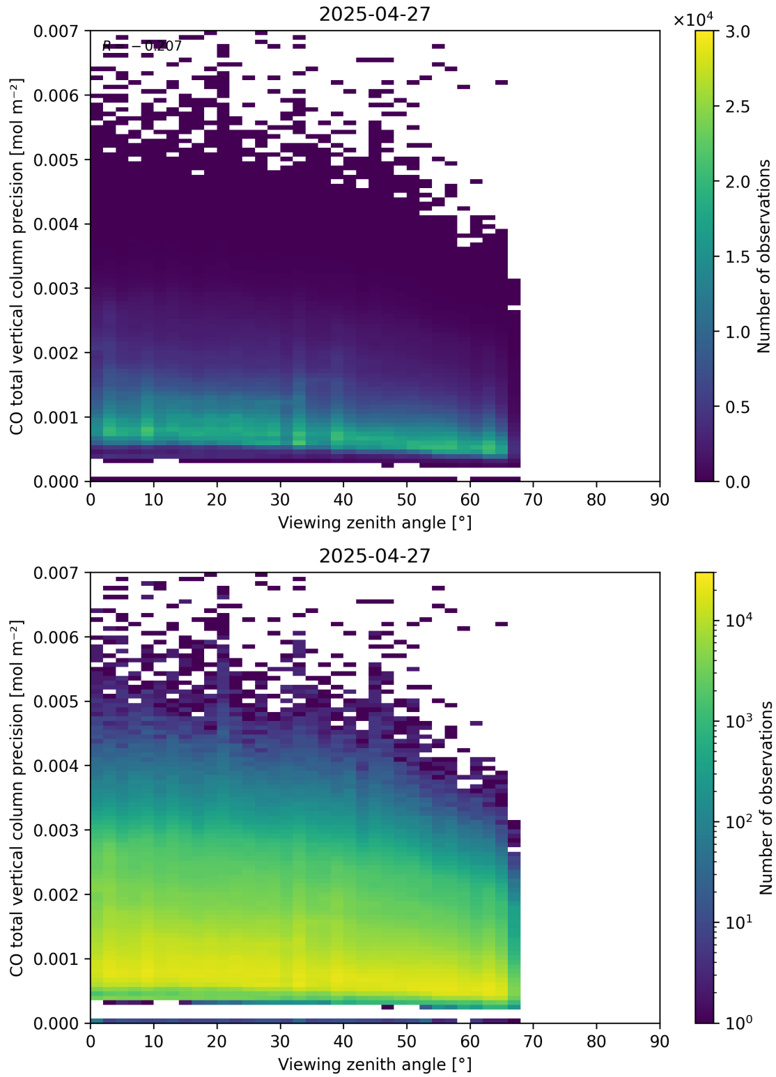
Figure 71: Scatter density plot of “Viewing zenith angle” against “CO total vertical column precision” for 2025-04-26 to 2025-04-28.
