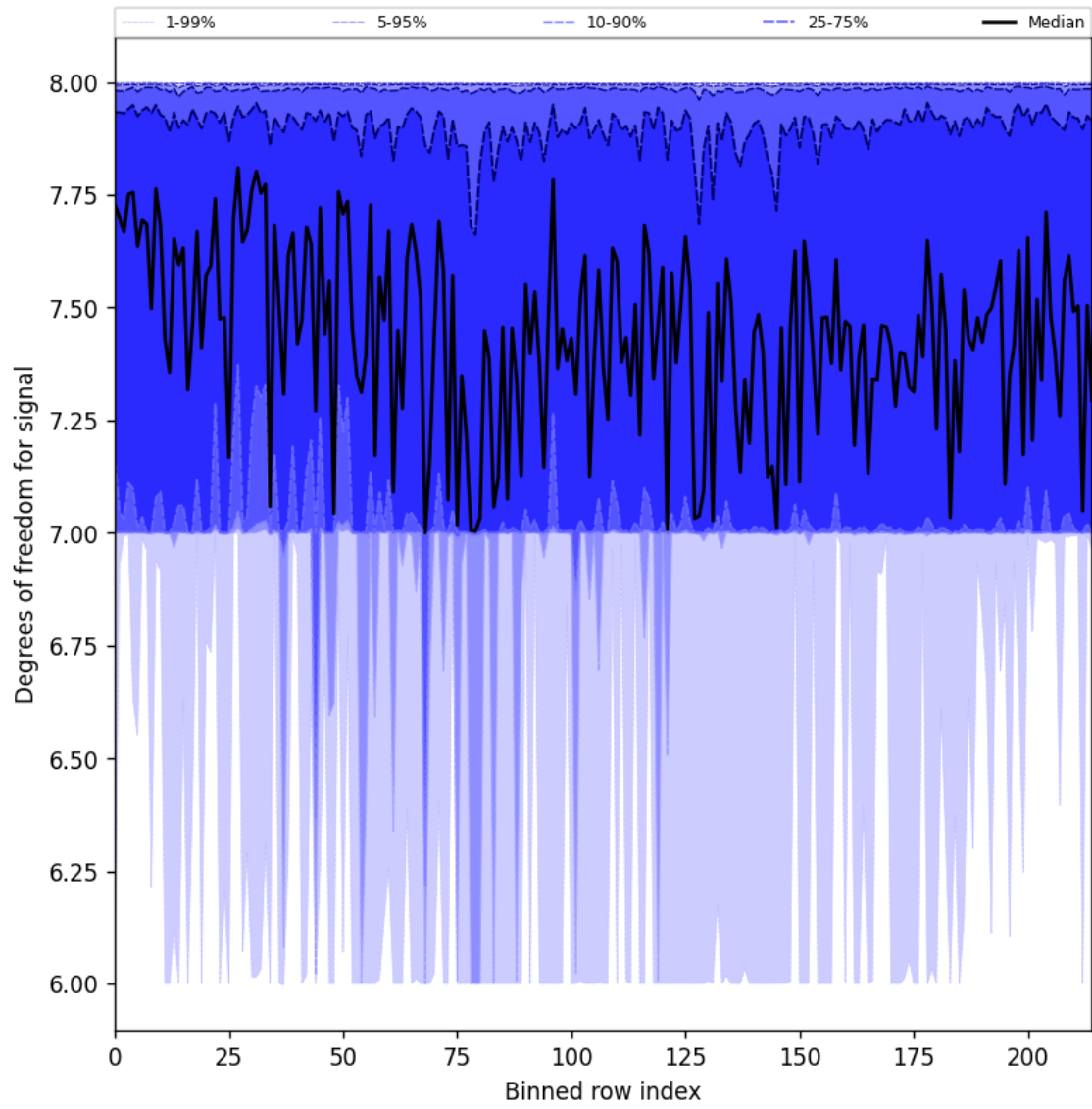
Figure 31: Along track statistics of “Degrees of freedom for signal” for 2025-04-26 to 2025-04-28
