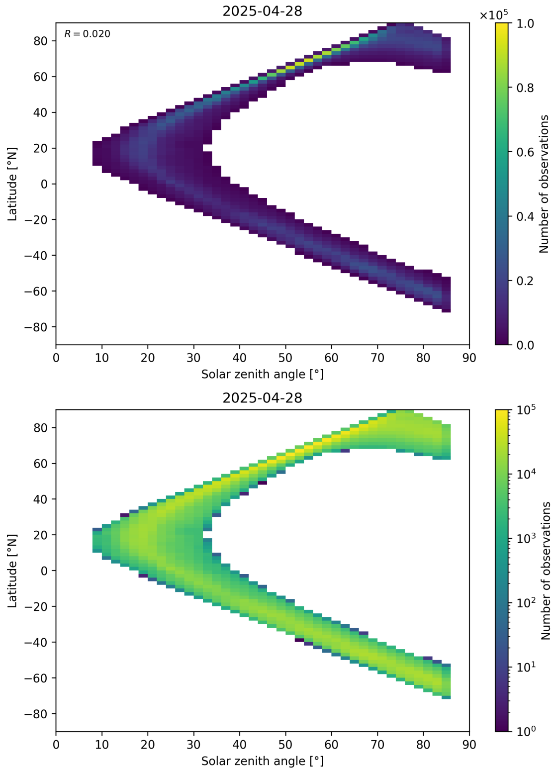
Figure 66: Scatter density plot of “Solar zenith angle” against “Latitude” for 2025-04-27 to 2025-04-29.
