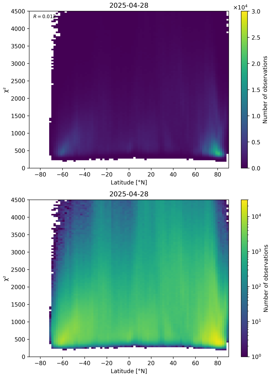
Figure 54: Scatter density plot of “Latitude” against “ \chi^2 ” for 2025-04-27 to 2025-04-29.
