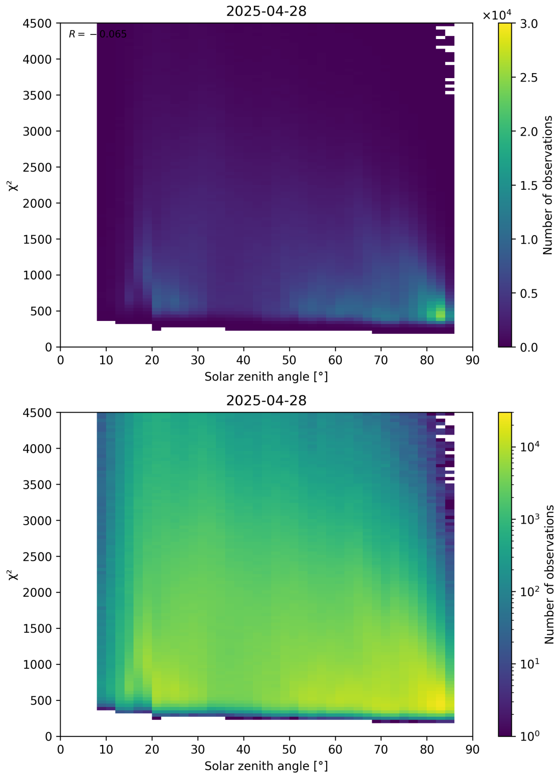
Figure 64: Scatter density plot of “Solar zenith angle” against “ \chi^2 ” for 2025-04-27 to 2025-04-29.
