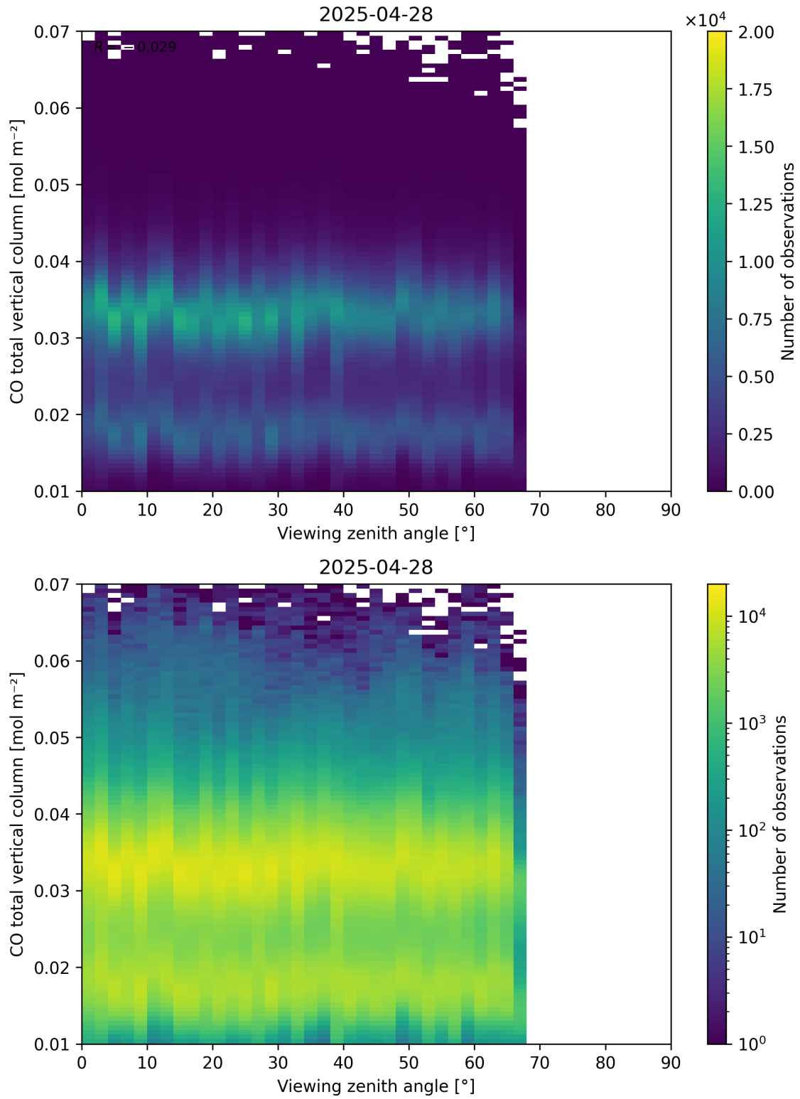
Figure 69: Scatter density plot of “Viewing zenith angle” against “CO total vertical column” for 2025-04-27 to 2025-04-29.
