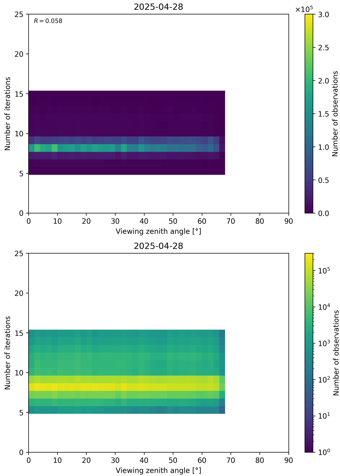
Figure 75: Scatter density plot of “Viewing zenith angle” against “Number of iterations” for 2025-04-27 to 2025-04-29.
