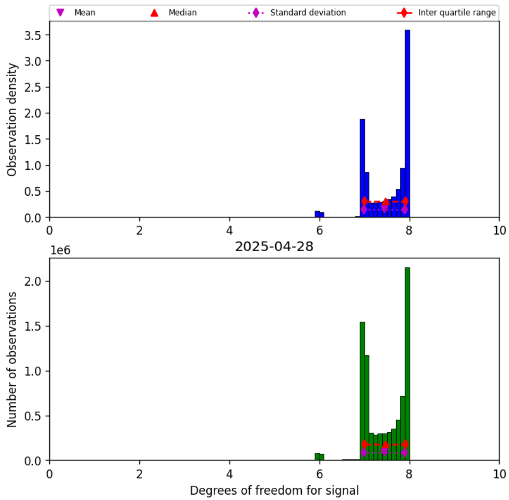
Figure 23: Histogram of “Degrees of freedom for signal” for 2025-04-27 to 2025-04-29
