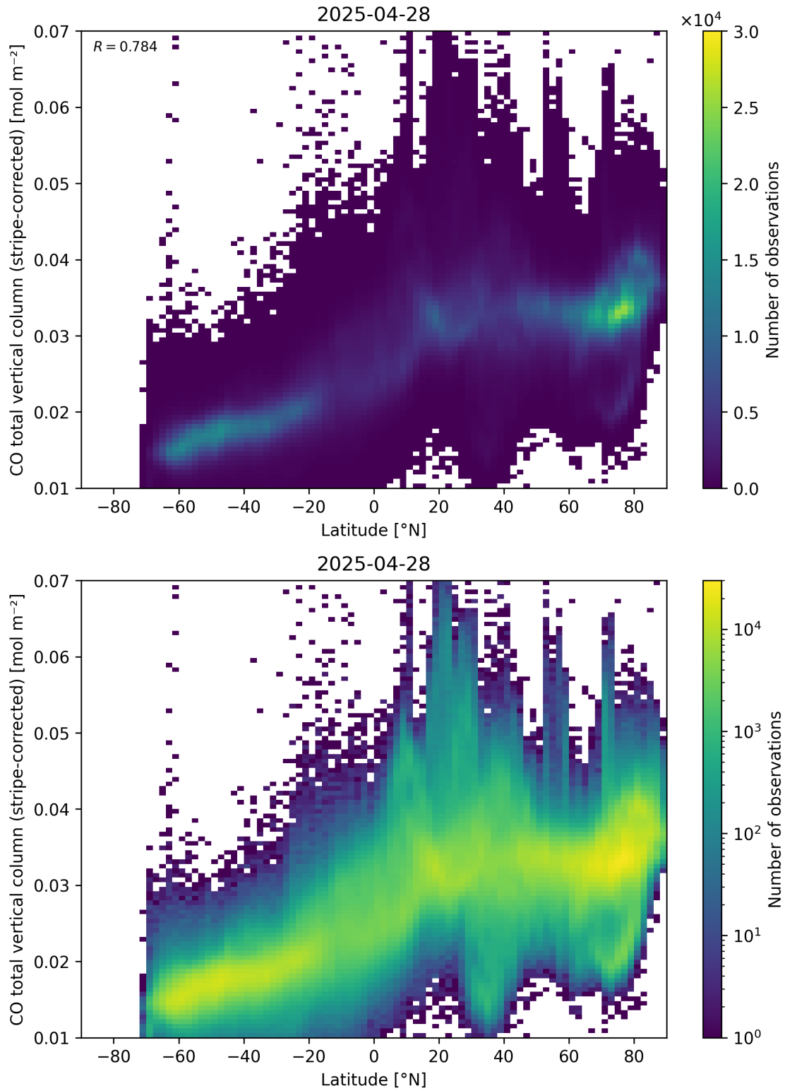
Figure 52: Scatter density plot of “Latitude” against “CO total vertical column (stripe-corrected)” for 2025-04-27 to 2025-04-29.
