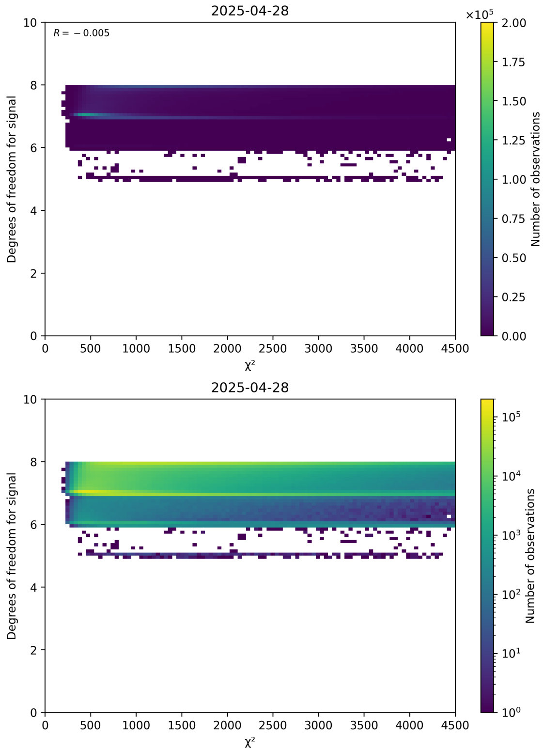
Figure 48: Scatter density plot of “ \chi^2 ” against “Degrees of freedom for signal” for 2025-04-27 to 2025-04-29.
