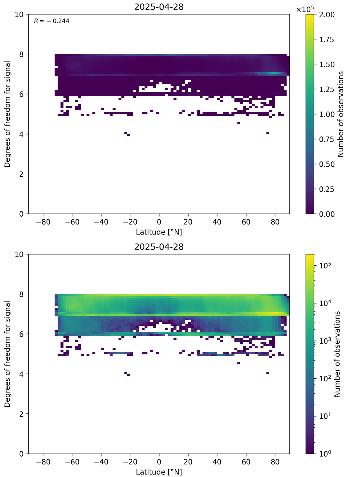
Figure 55: Scatter density plot of “Latitude” against “Degrees of freedom for signal” for 2025-04-27 to 2025-04-29.
