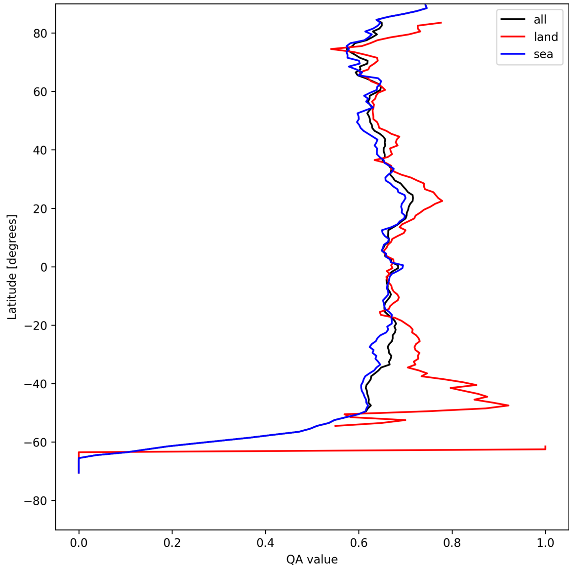
Figure 9: Zonal average of “QA value” for 2025-04-27 to 2025-04-29.
