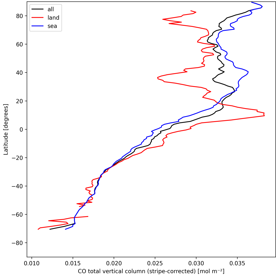
Figure 11: Zonal average of “CO total vertical column (stripe-corrected)” for 2025-04-27 to 2025-04-29.
