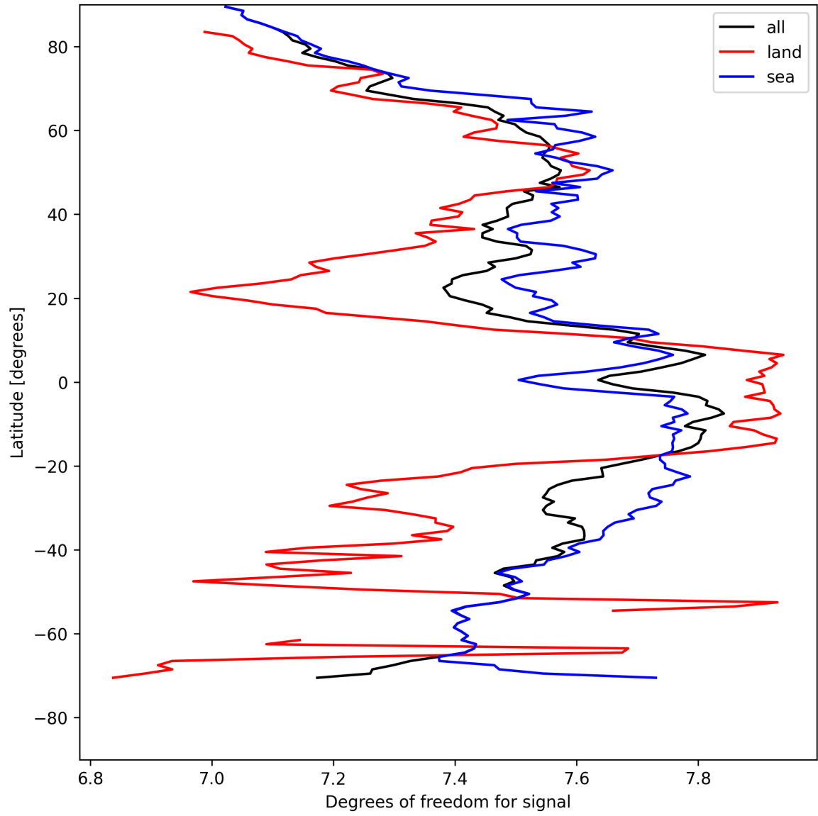
Figure 15: Zonal average of “Degrees of freedom for signal” for 2025-04-27 to 2025-04-29.
