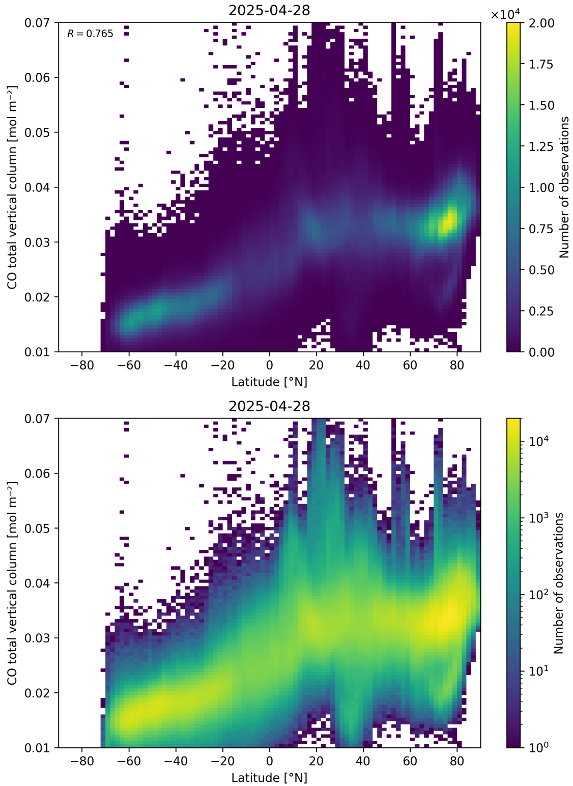
Figure 51: Scatter density plot of “Latitude” against “CO total vertical column” for 2025-04-27 to 2025-04-29.
