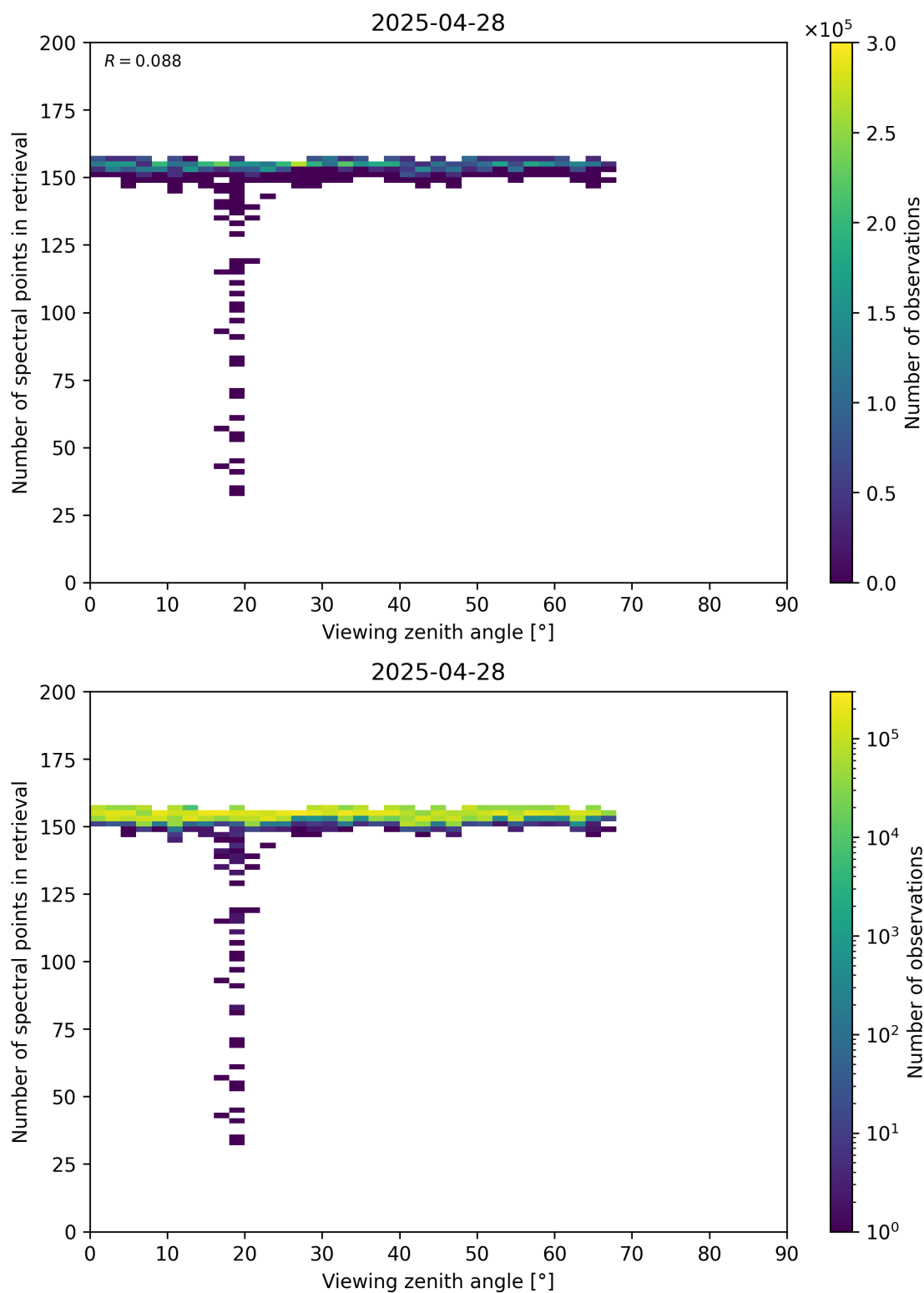
Figure 76: Scatter density plot of “Viewing zenith angle” against “Number of spectral points in retrieval” for 2025-04-27 to 2025-04-29.
