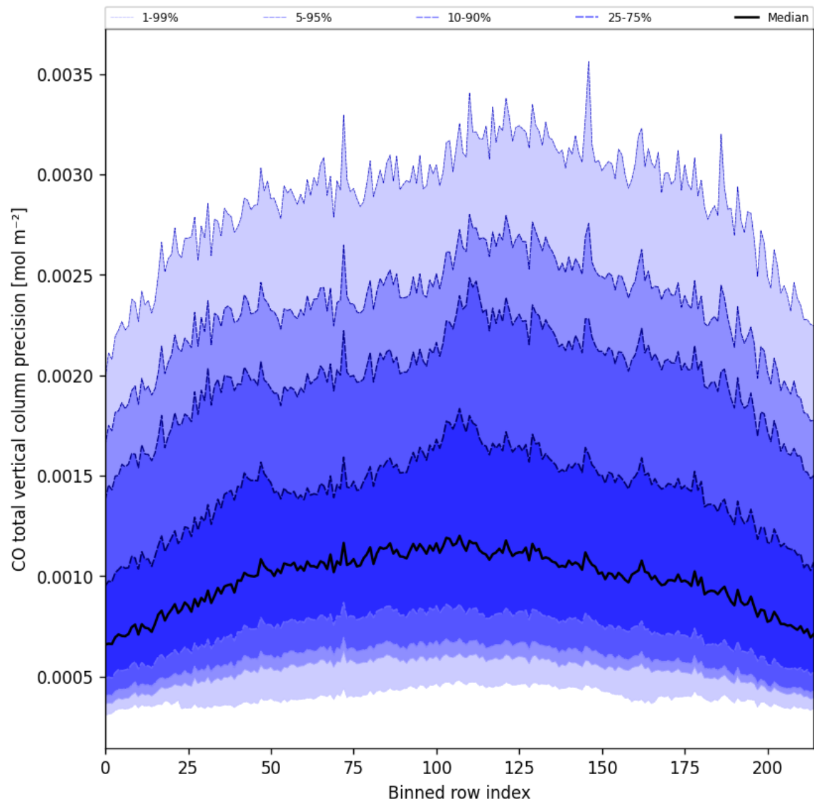
Figure 28: Along track statistics of “CO total vertical column precision” for 2025-04-27 to 2025-04-29
