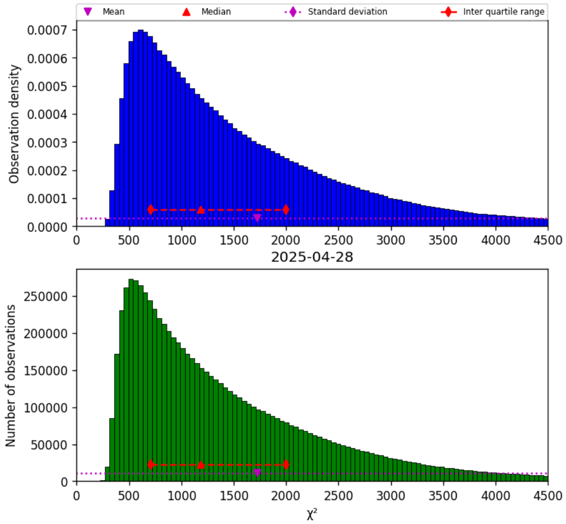
Figure 22: Histogram of “ \chi^2 ” for 2025-04-27 to 2025-04-29
