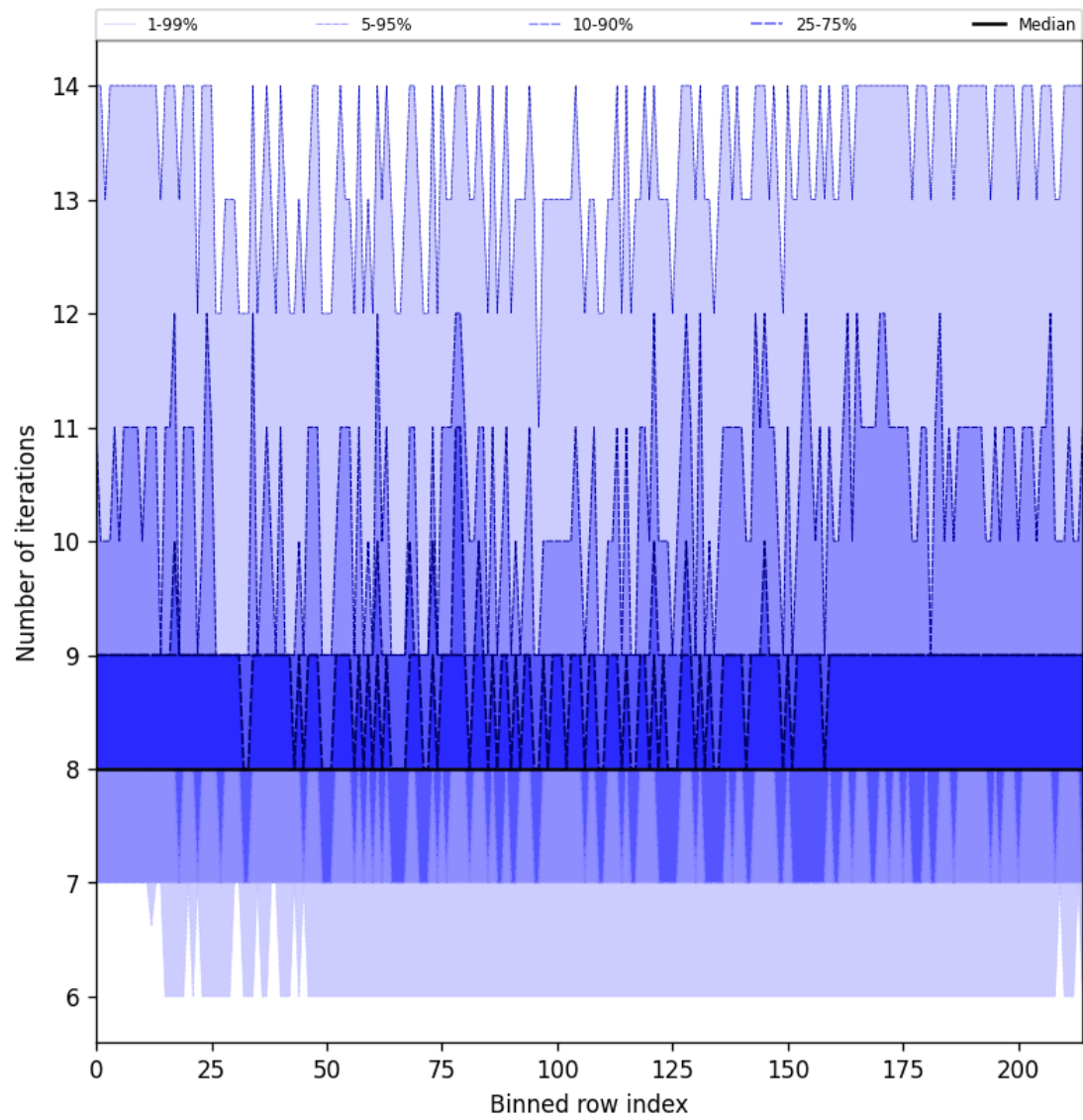
Figure 32: Along track statistics of “Number of iterations” for 2025-04-27 to 2025-04-29
