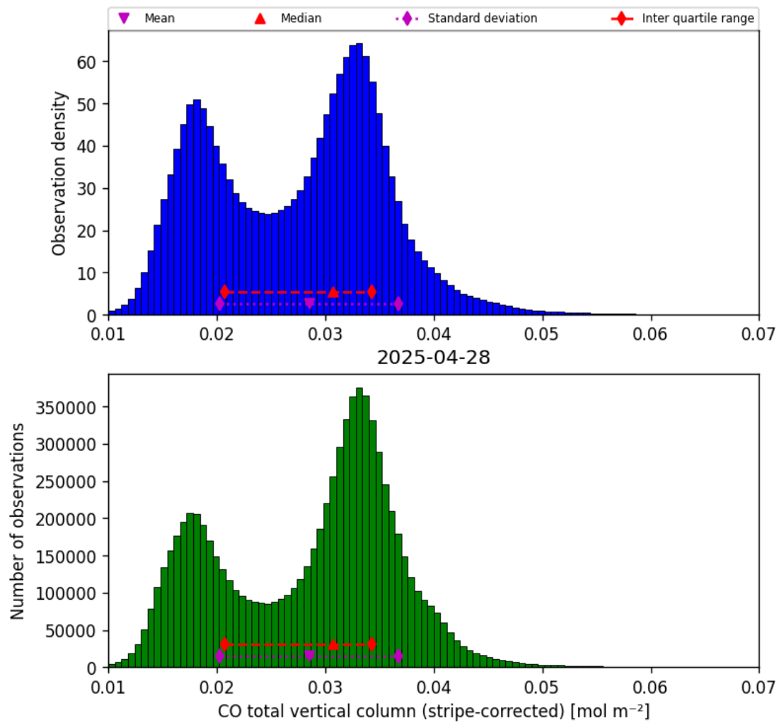
Figure 19: Histogram of “CO total vertical column (stripe-corrected)” for 2025-04-27 to 2025-04-29
