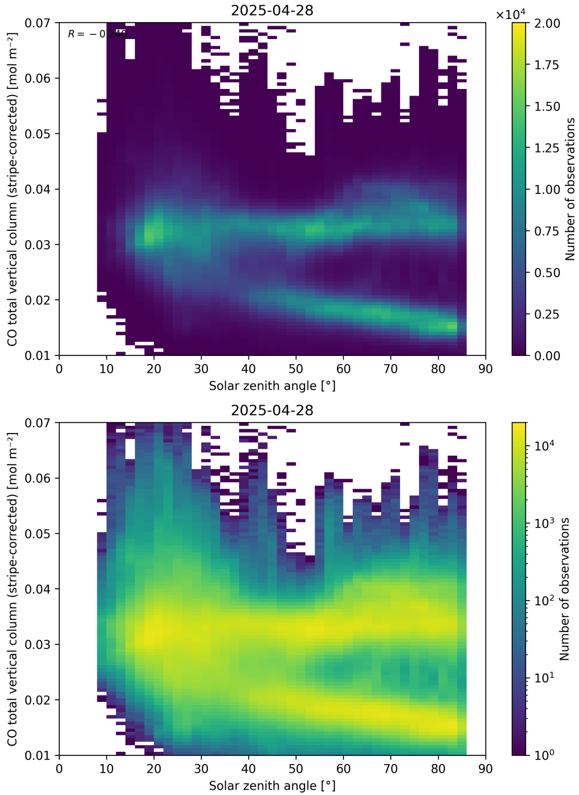
Figure 62: Scatter density plot of “Solar zenith angle” against “CO total vertical column (stripe-corrected)” for 2025-04-27 to 2025-04-29.
