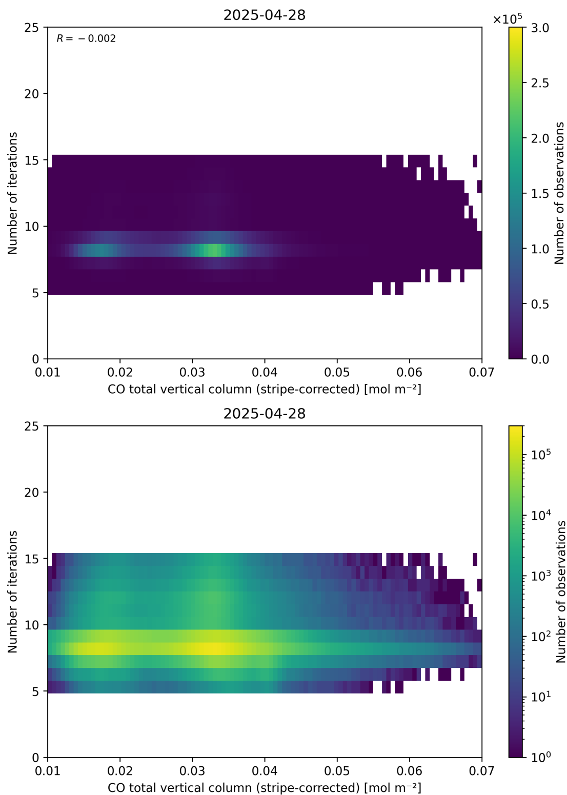
Figure 39: Scatter density plot of “CO total vertical column (stripe-corrected)” against “Number of iterations” for 2025-04-27 to 2025-04-29.
