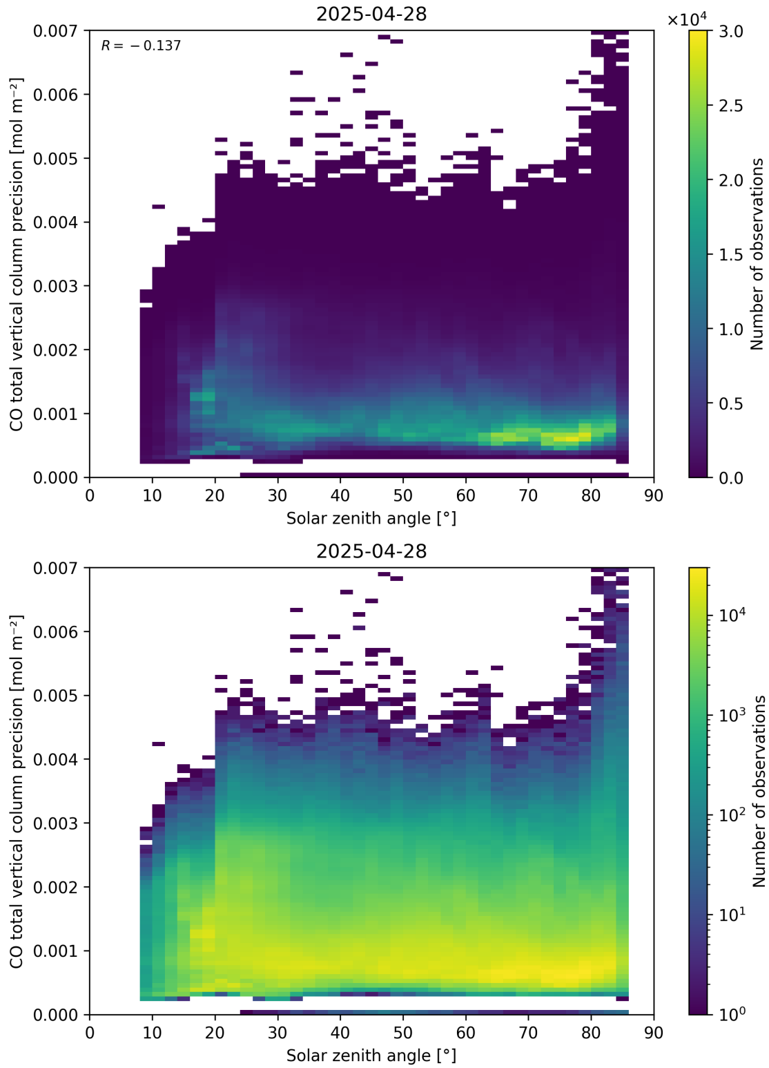
Figure 63: Scatter density plot of “Solar zenith angle” against “CO total vertical column precision” for 2025-04-27 to 2025-04-29.
