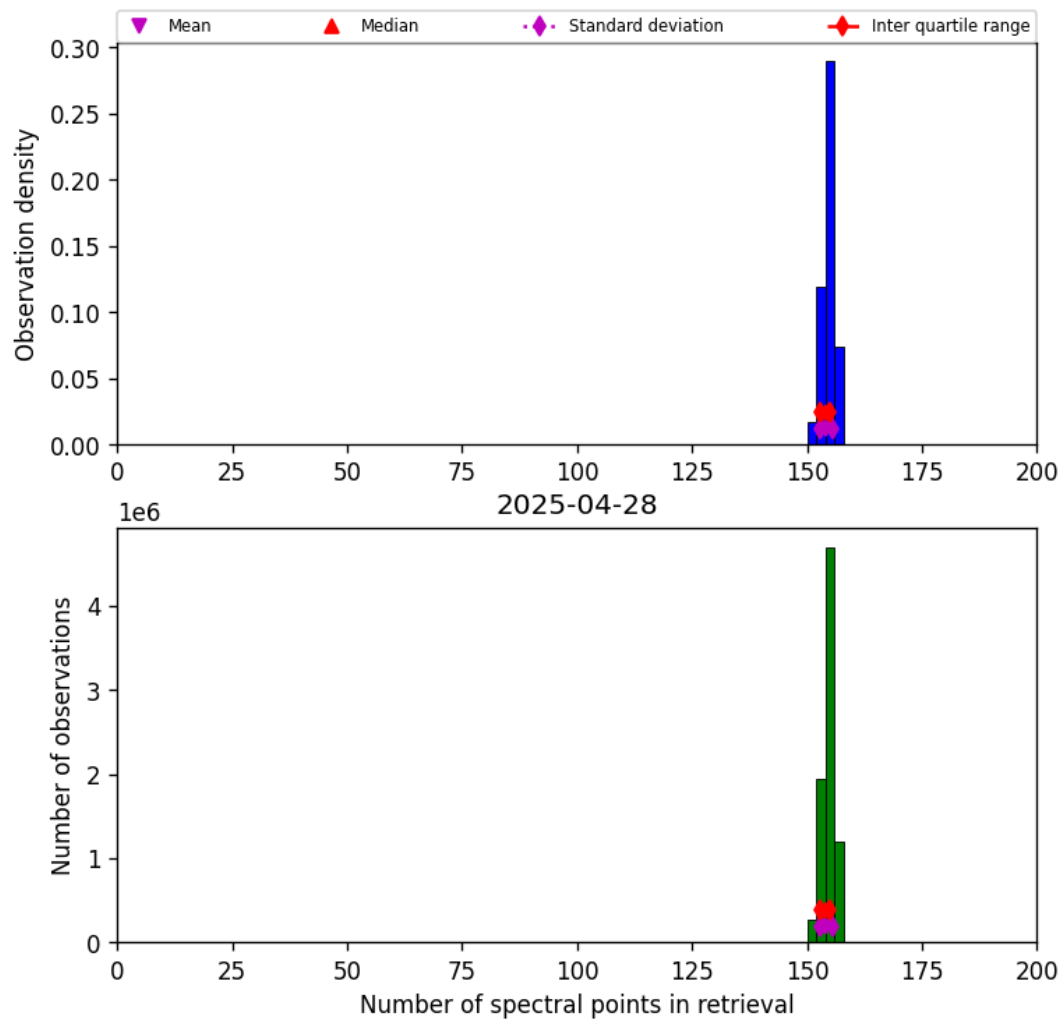
Figure 21: Histogram of “Number of spectral points in retrieval” for 2025-04-27 to 2025-04-29
