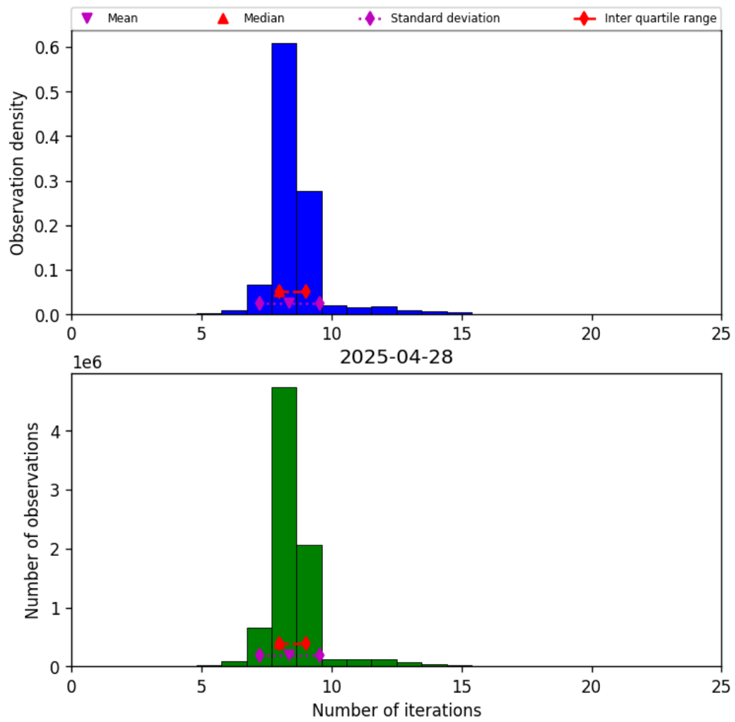
Figure 24: Histogram of “Number of iterations” for 2025-04-27 to 2025-04-29
