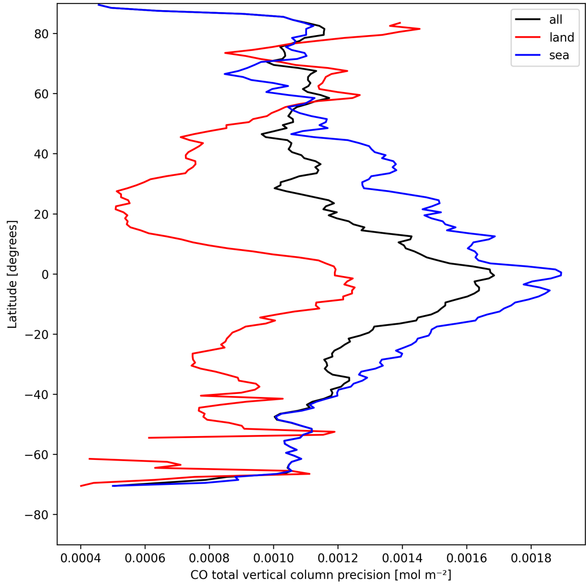
Figure 12: Zonal average of “CO total vertical column precision” for 2025-04-27 to 2025-04-29.
