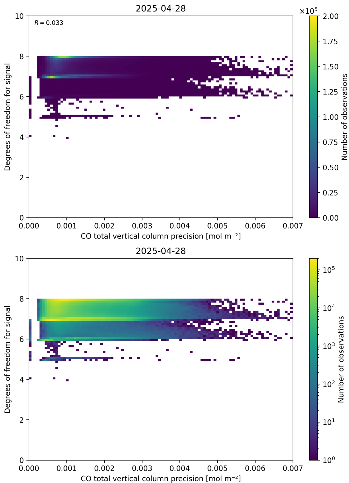
Figure 45: Scatter density plot of “CO total vertical column precision” against “Degrees of freedom for signal” for 2025-04-27 to 2025-04-29.
