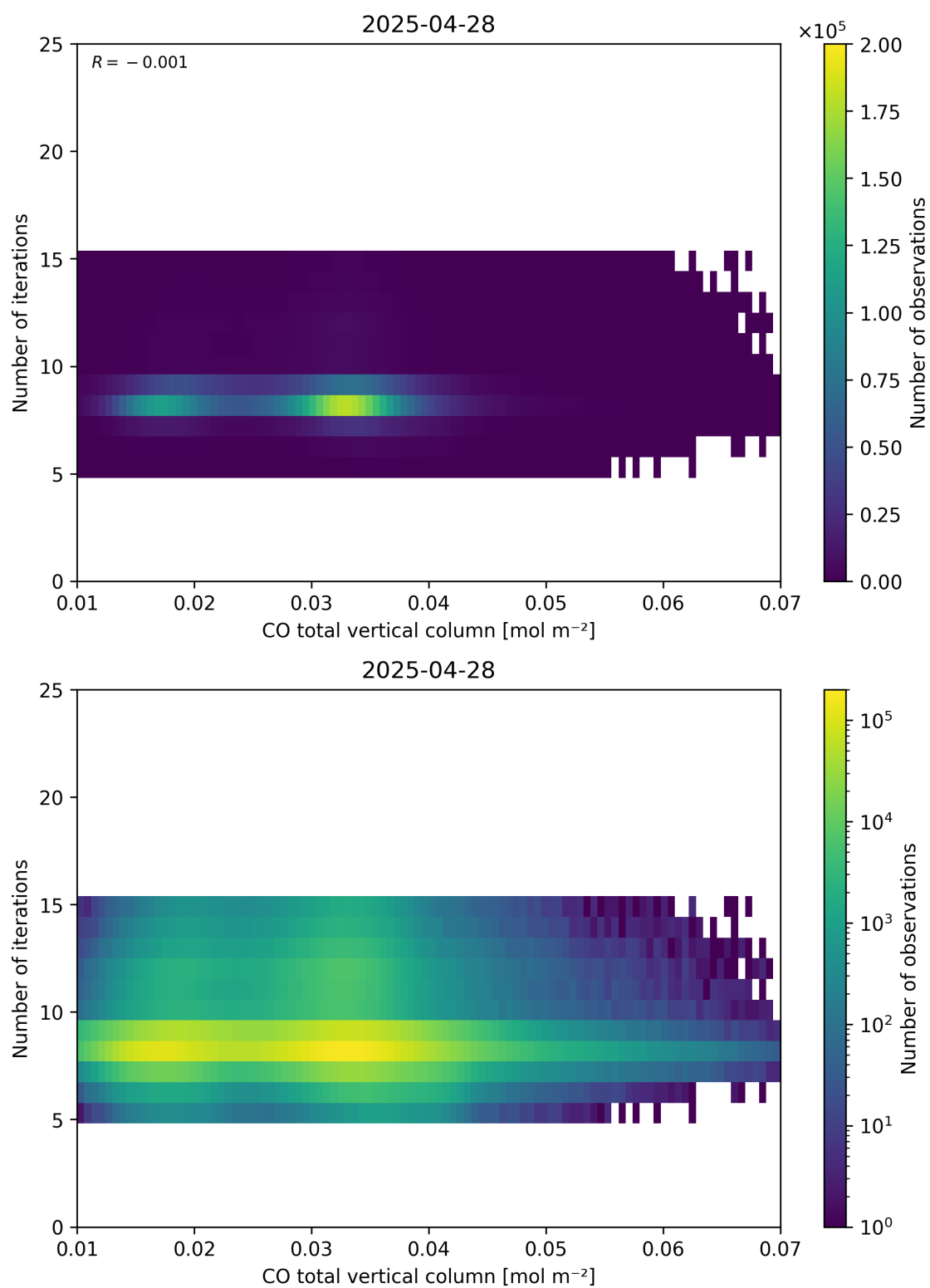
Figure 42: Scatter density plot of “CO total vertical column” against “Number of iterations” for 2025-04-27 to 2025-04-29.
