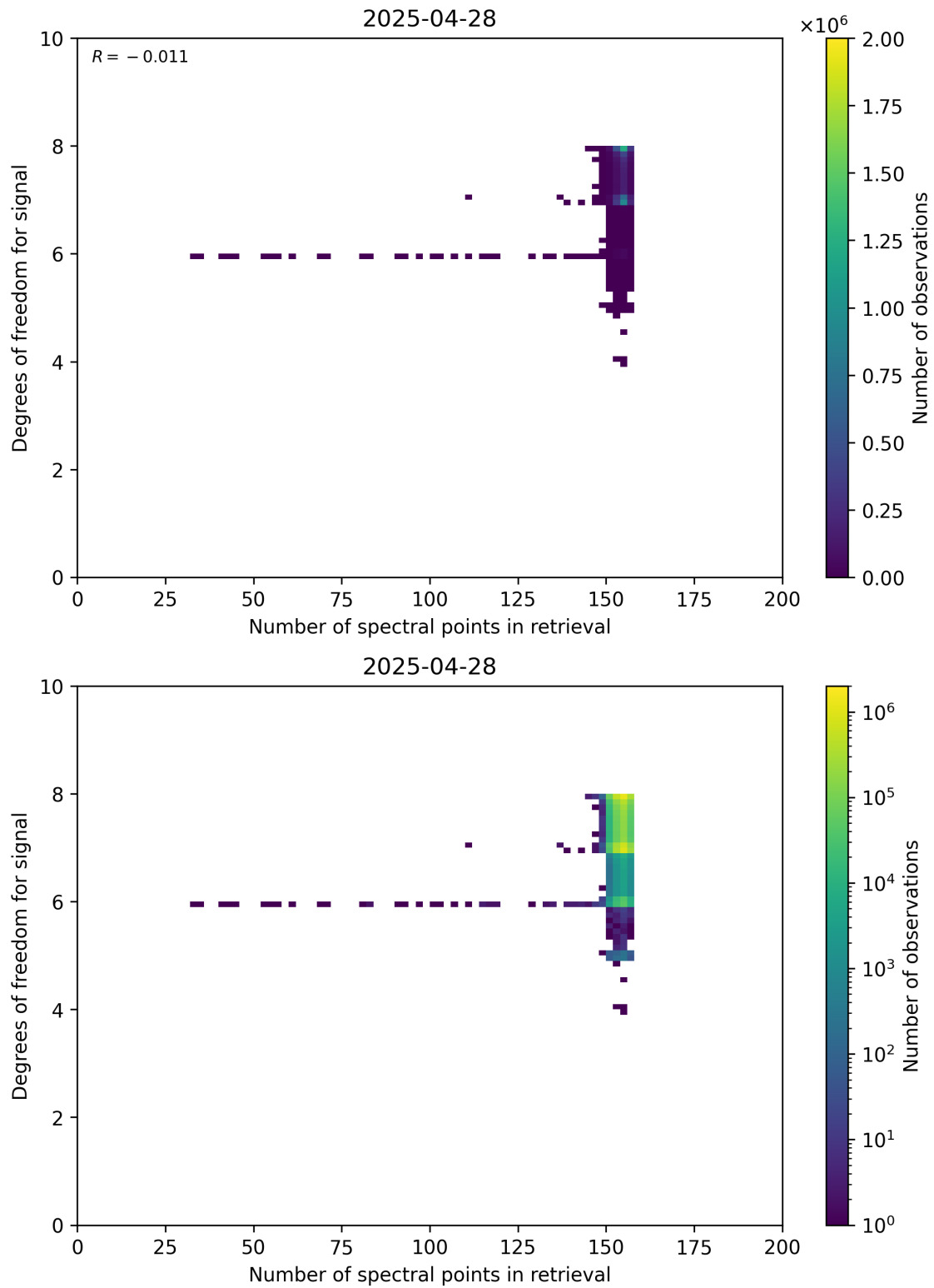
Figure 59: Scatter density plot of “Number of spectral points in retrieval” against “Degrees of freedom for signal” for 2025-04-27 to 2025-04-29.
