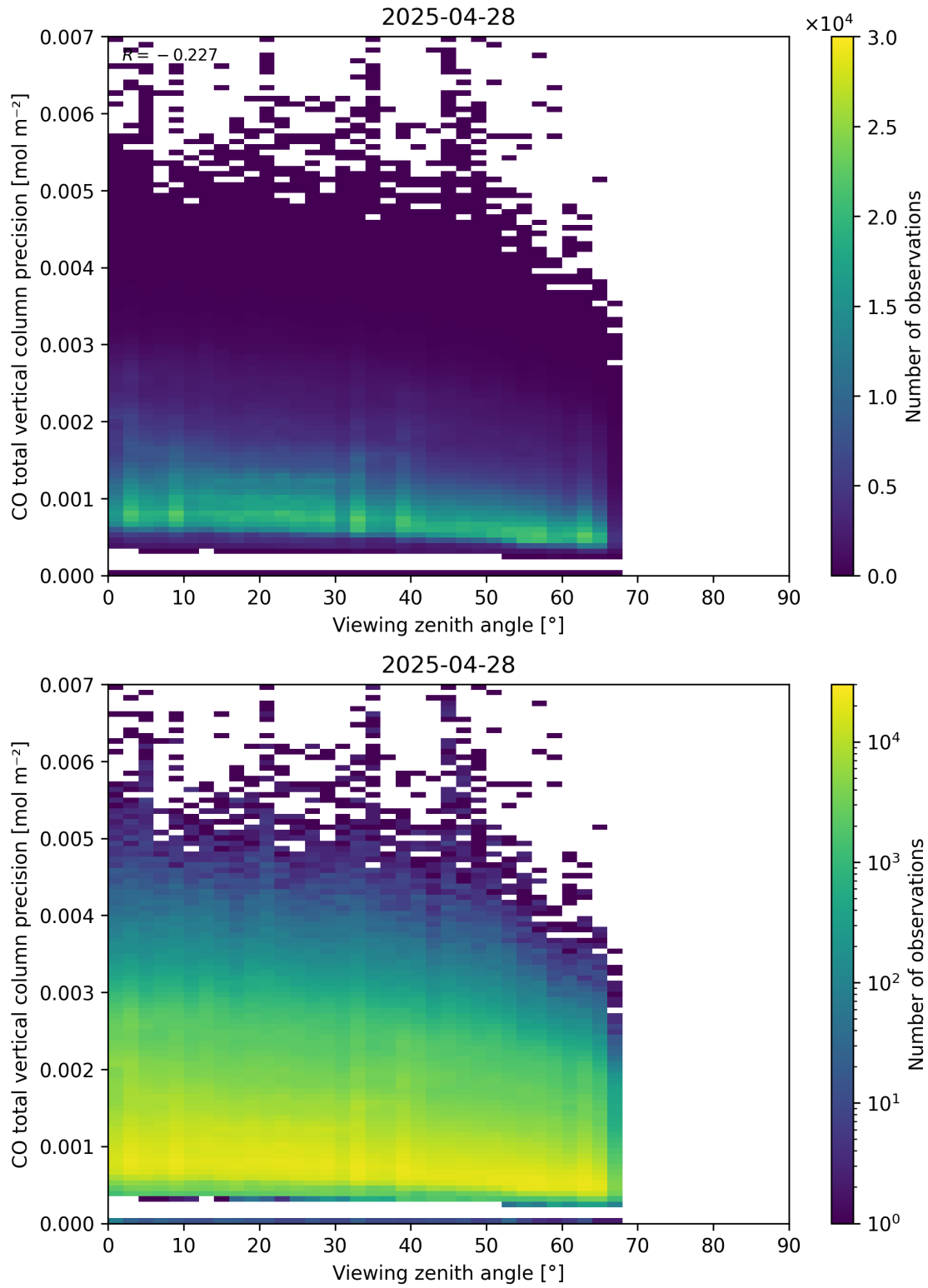
Figure 71: Scatter density plot of “Viewing zenith angle” against “CO total vertical column precision” for 2025-04-27 to 2025-04-29.
