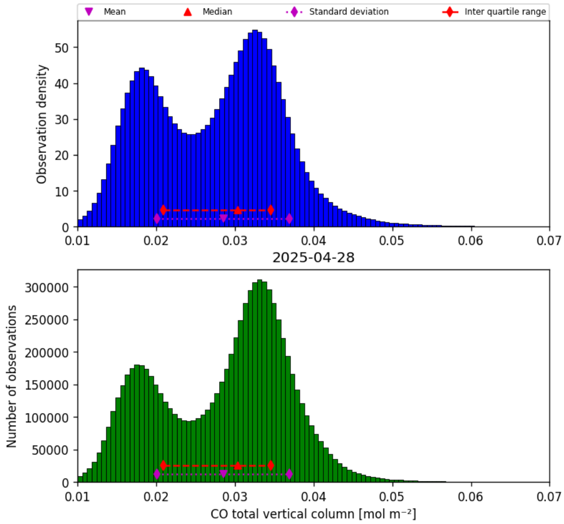
Figure 18: Histogram of “CO total vertical column” for 2025-04-27 to 2025-04-29
