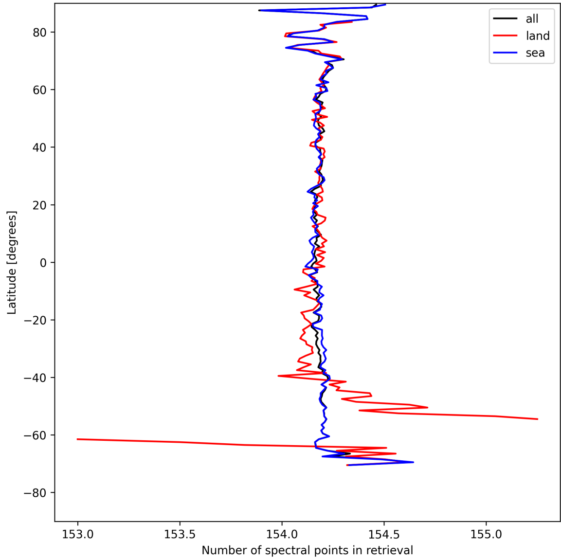
Figure 13: Zonal average of “Number of spectral points in retrieval” for 2025-04-27 to 2025-04-29.
