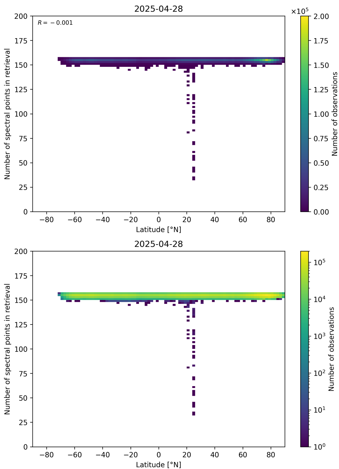
Figure 57: Scatter density plot of “Latitude” against “Number of spectral points in retrieval” for 2025-04-27 to 2025-04-29.
