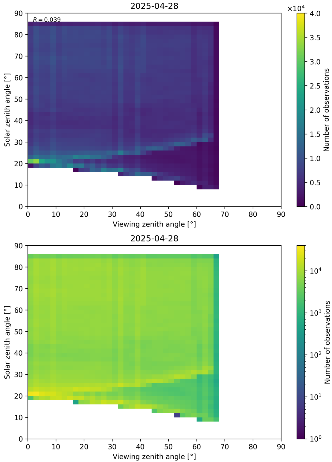
Figure 77: Scatter density plot of “Viewing zenith angle” against “Solar zenith angle” for 2025-04-27 to 2025-04-29.
