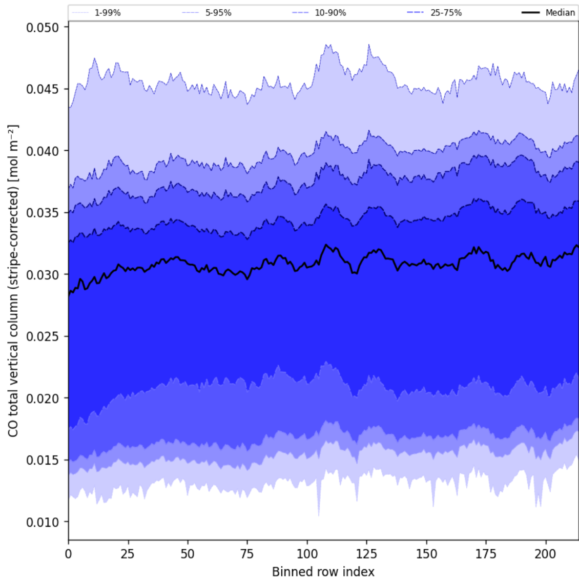
Figure 27: Along track statistics of “CO total vertical column (stripe-corrected)” for 2025-04-27 to 2025-04-29
