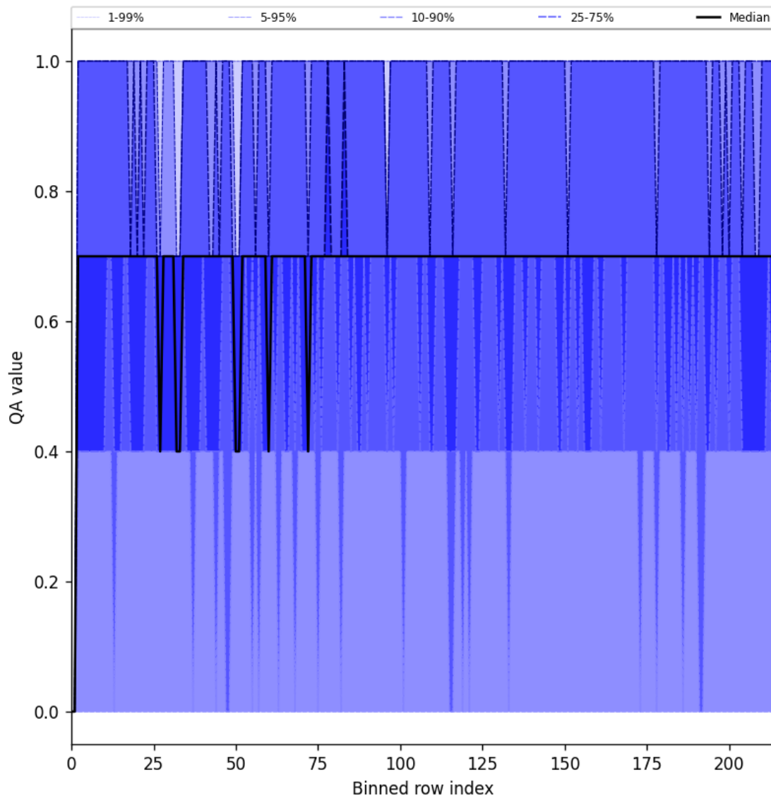
Figure 25: Along track statistics of “QA value” for 2025-04-27 to 2025-04-29
