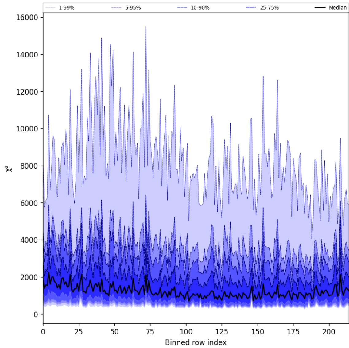
Figure 30: Along track statistics of “ \chi^2 ” for 2025-04-27 to 2025-04-29
