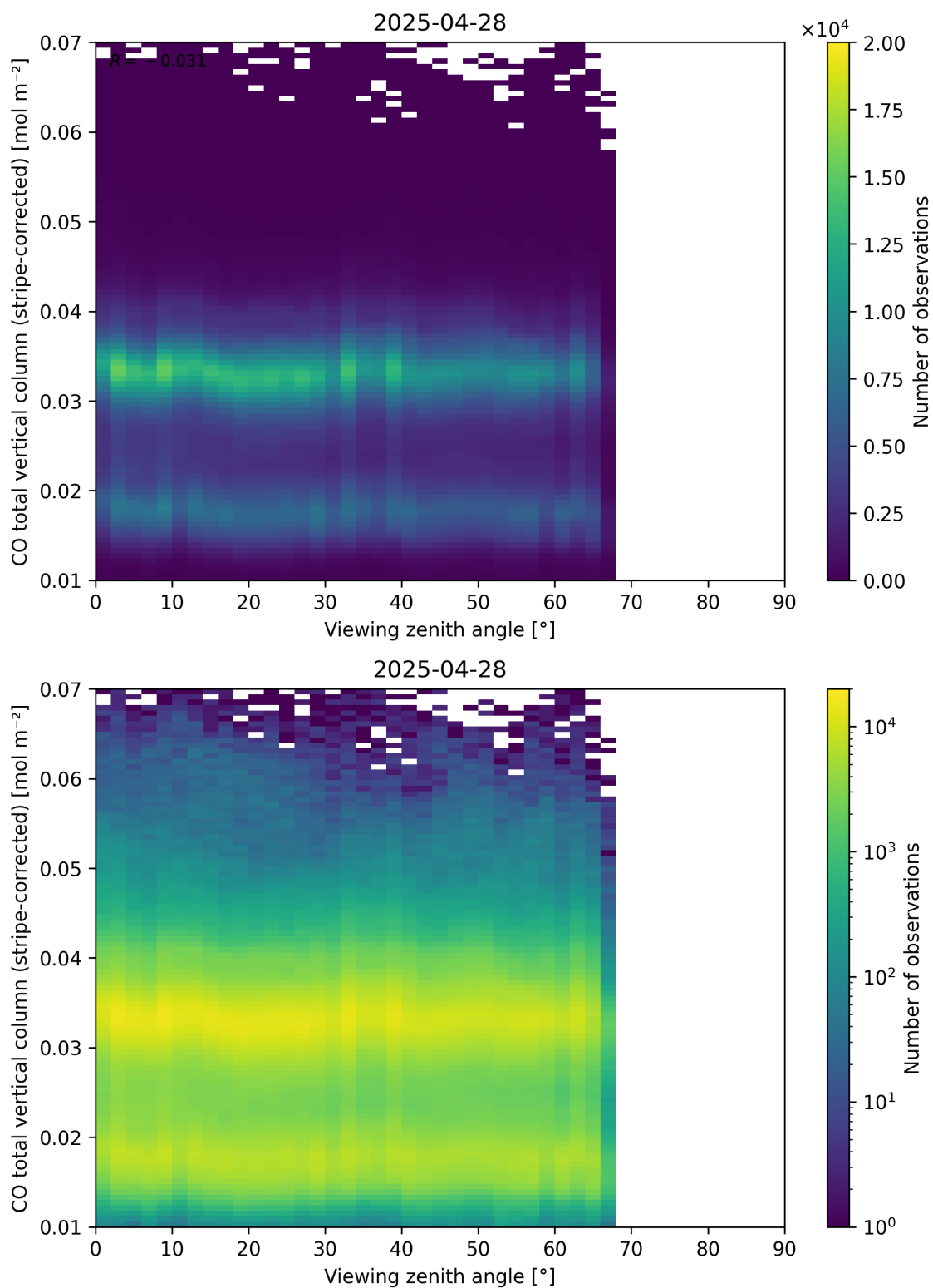
Figure 70: Scatter density plot of “Viewing zenith angle” against “CO total vertical column (stripe-corrected)” for 2025-04-27 to 2025-04-29.
