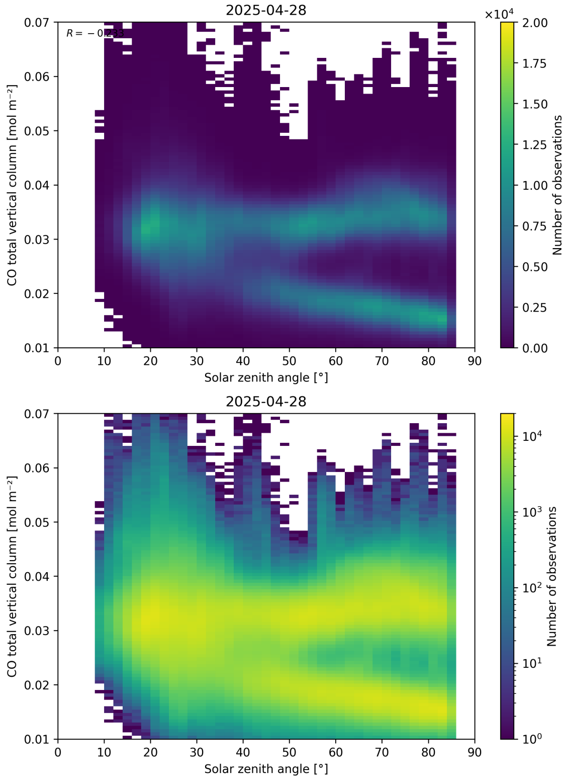
Figure 61: Scatter density plot of “Solar zenith angle” against “CO total vertical column” for 2025-04-27 to 2025-04-29.
