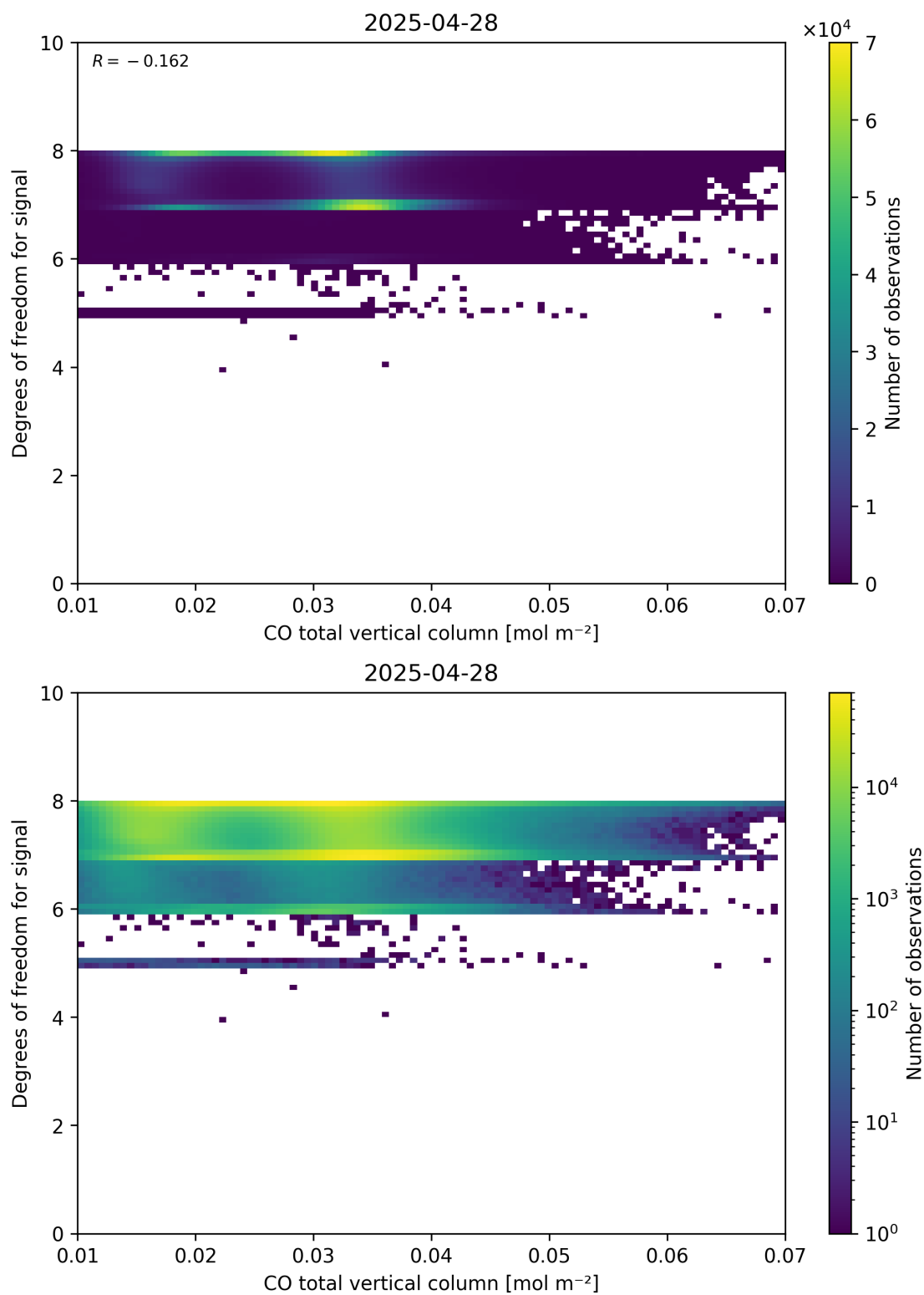
Figure 41: Scatter density plot of “CO total vertical column” against “Degrees of freedom for signal” for 2025-04-27 to 2025-04-29.
