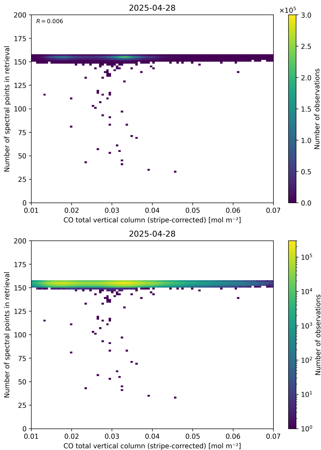
Figure 40: Scatter density plot of “CO total vertical column (stripe-corrected)” against “Number of spectral points in retrieval” for 2025-04-27 to 2025-04-29.
