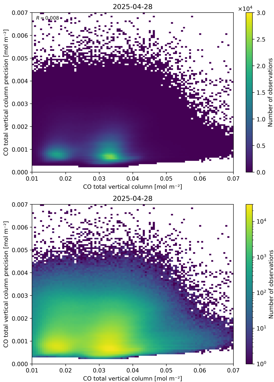
Figure 34: Scatter density plot of “CO total vertical column” against “CO total vertical column precision” for 2025-04-27 to 2025-04-29.
