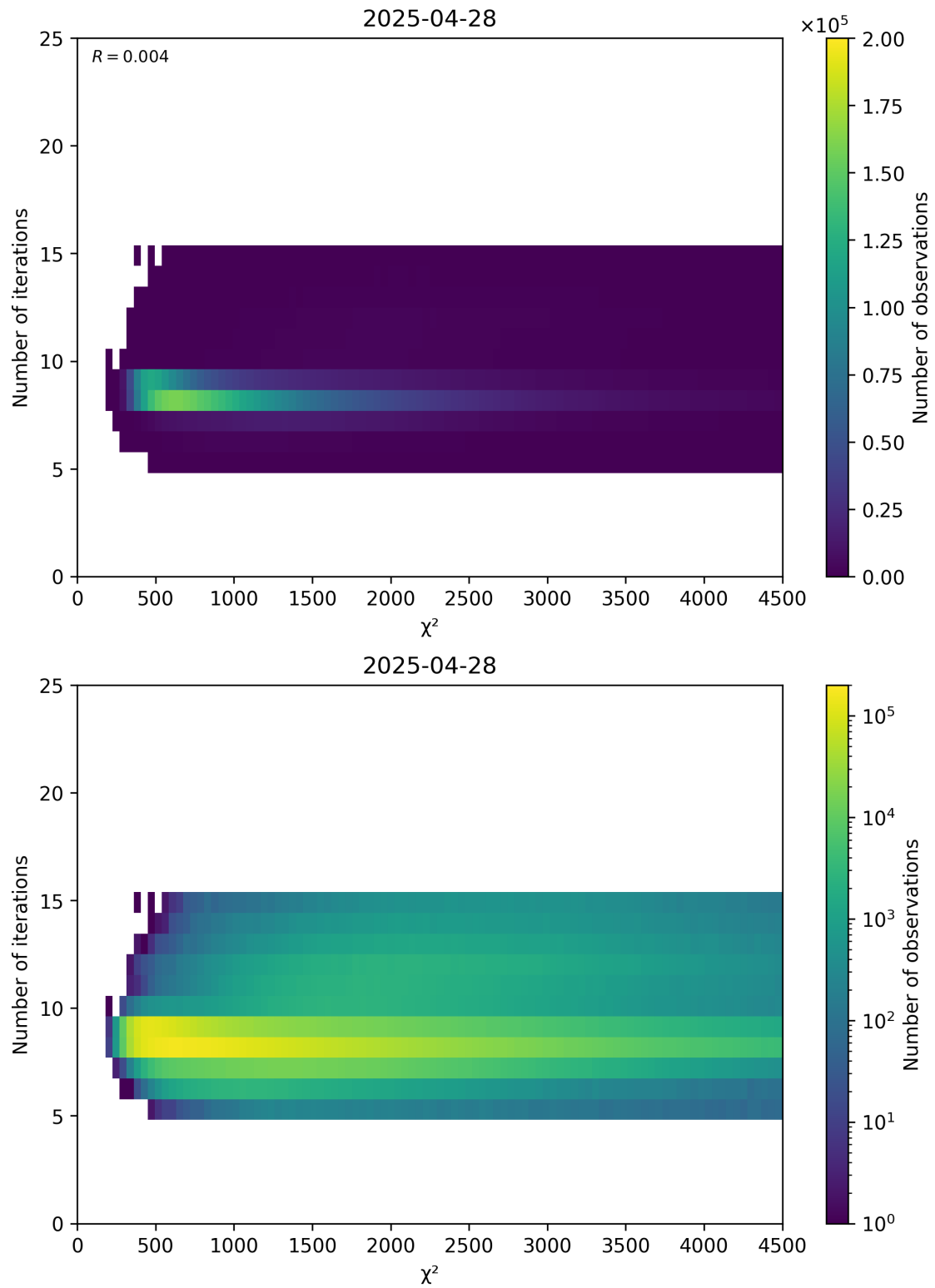
Figure 49: Scatter density plot of “ \chi^2 ” against “Number of iterations” for 2025-04-27 to 2025-04-29.
