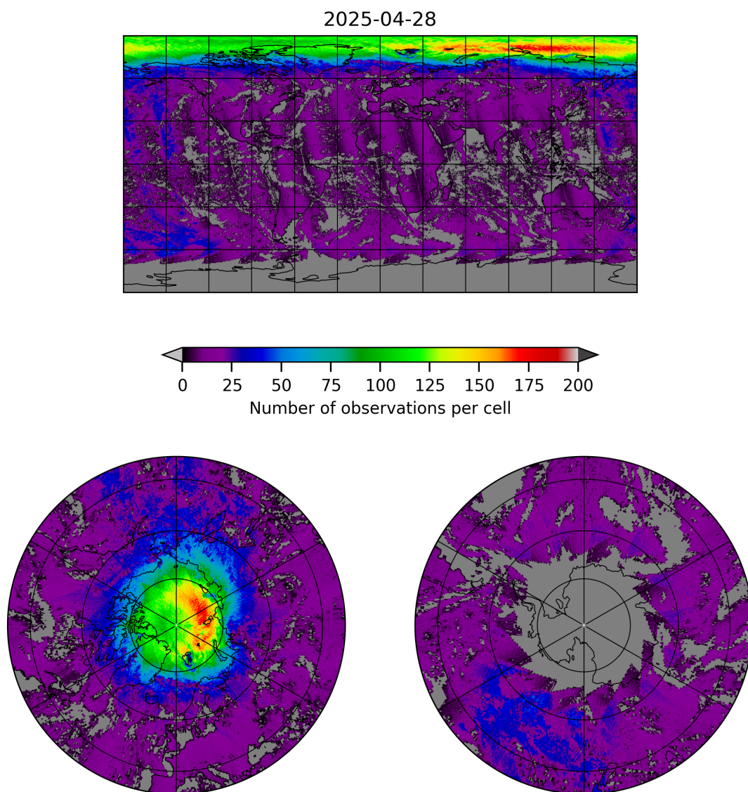
Figure 8: Map of the number of observations for 2025-04-27 to 2025-04-29
