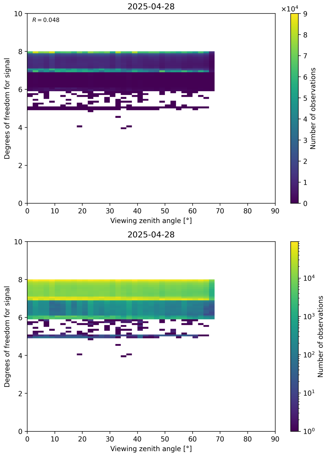
Figure 73: Scatter density plot of “Viewing zenith angle” against “Degrees of freedom for signal” for 2025-04-27 to 2025-04-29.
