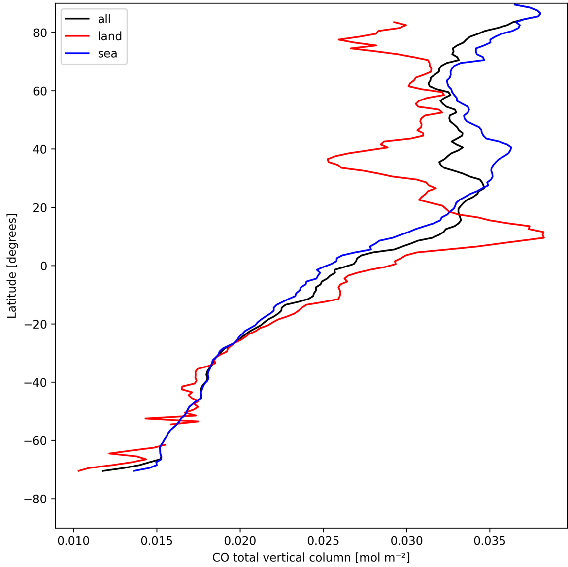
Figure 10: Zonal average of “CO total vertical column” for 2025-04-27 to 2025-04-29.
