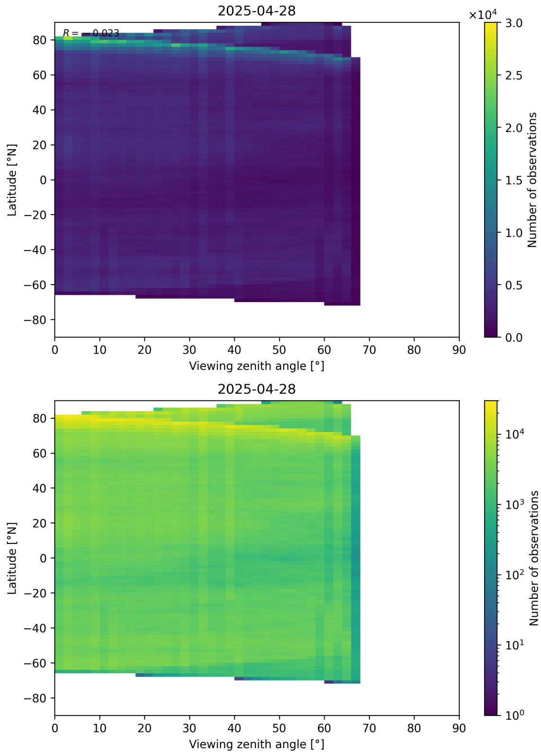
Figure 74: Scatter density plot of “Viewing zenith angle” against “Latitude” for 2025-04-27 to 2025-04-29.
