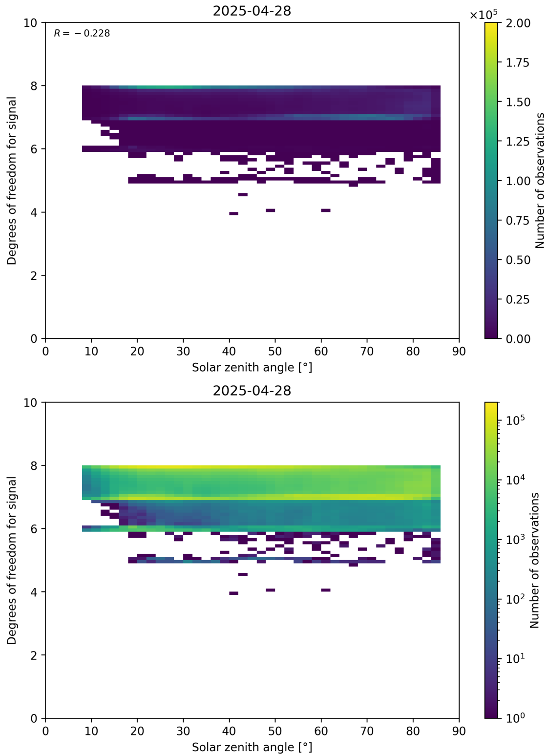
Figure 65: Scatter density plot of “Solar zenith angle” against “Degrees of freedom for signal” for 2025-04-27 to 2025-04-29.
