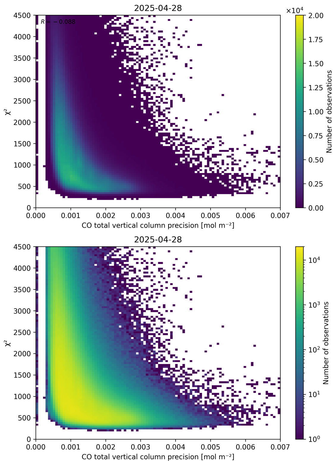
Figure 44: Scatter density plot of “CO total vertical column precision” against “ \chi^2 ” for 2025-04-27 to 2025-04-29.
