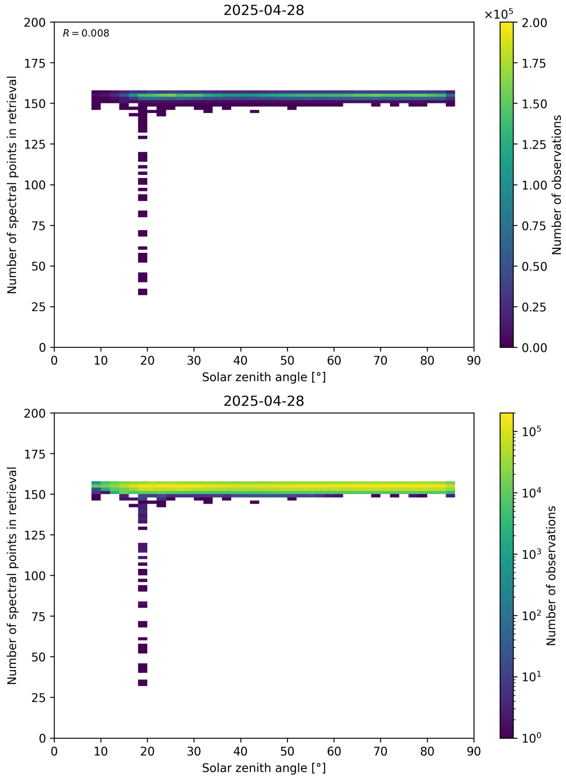
Figure 68: Scatter density plot of “Solar zenith angle” against “Number of spectral points in retrieval” for 2025-04-27 to 2025-04-29.
