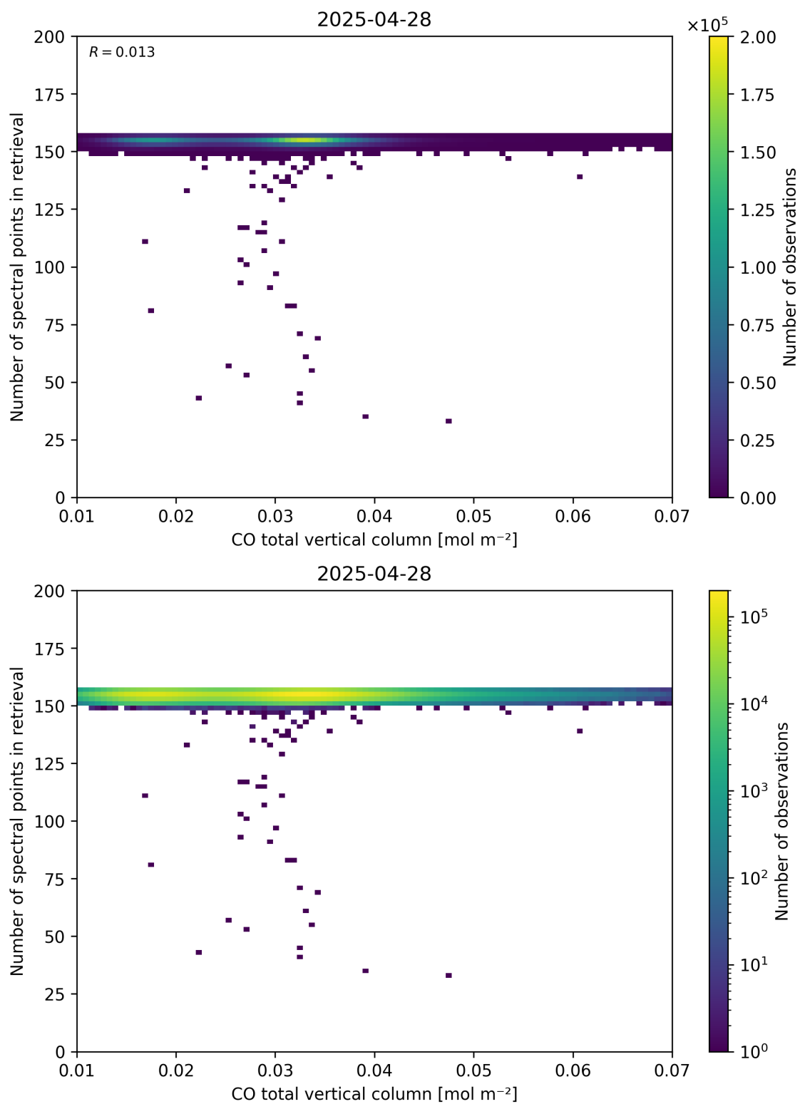
Figure 43: Scatter density plot of “CO total vertical column” against “Number of spectral points in retrieval” for 2025-04-27 to 2025-04-29.
