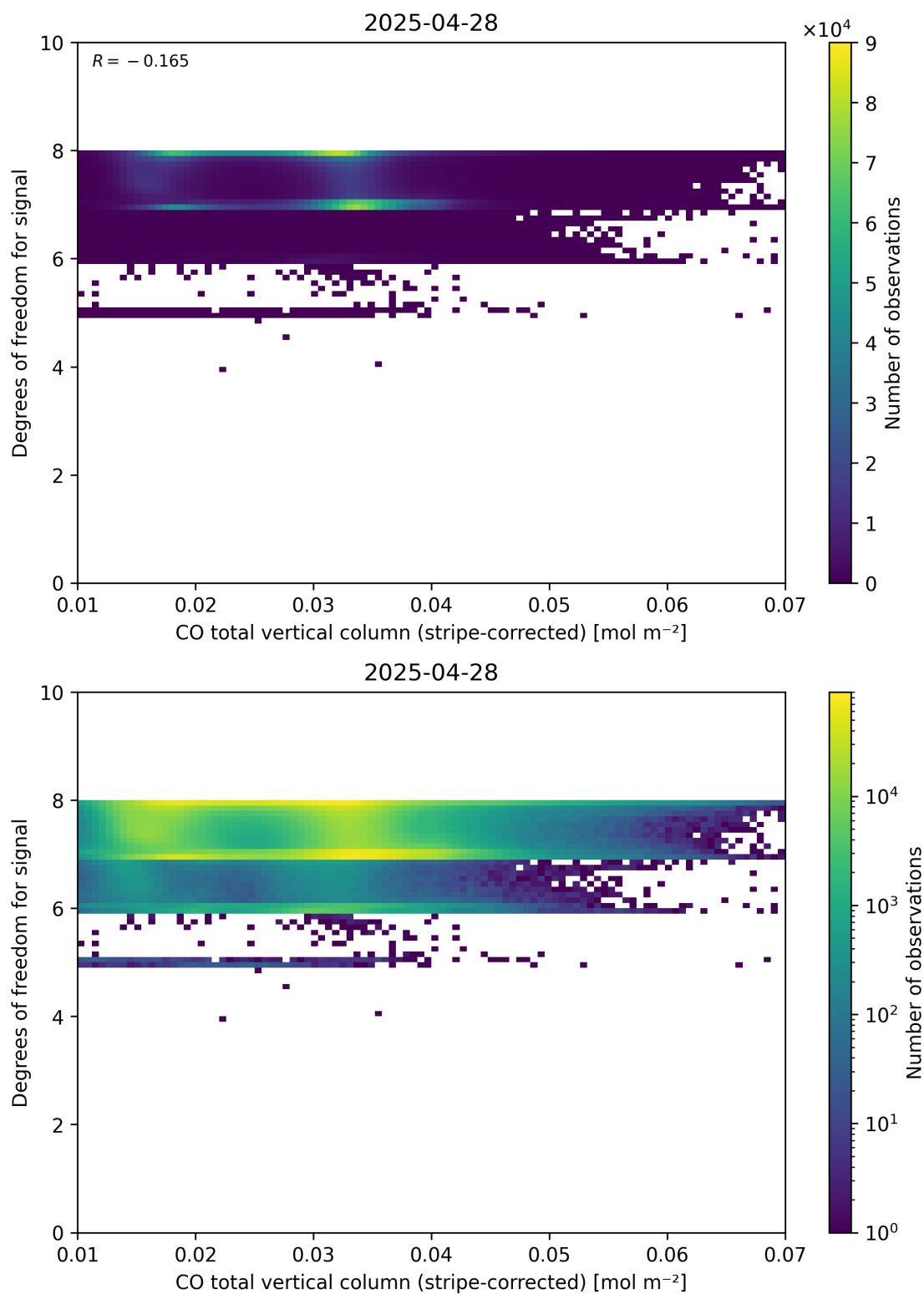
Figure 38: Scatter density plot of “CO total vertical column (stripe-corrected)” against “Degrees of freedom for signal” for 2025-04-27 to 2025-04-29.
