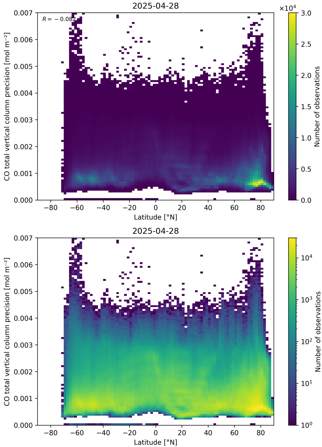
Figure 53: Scatter density plot of “Latitude” against “CO total vertical column precision” for 2025-04-27 to 2025-04-29.
