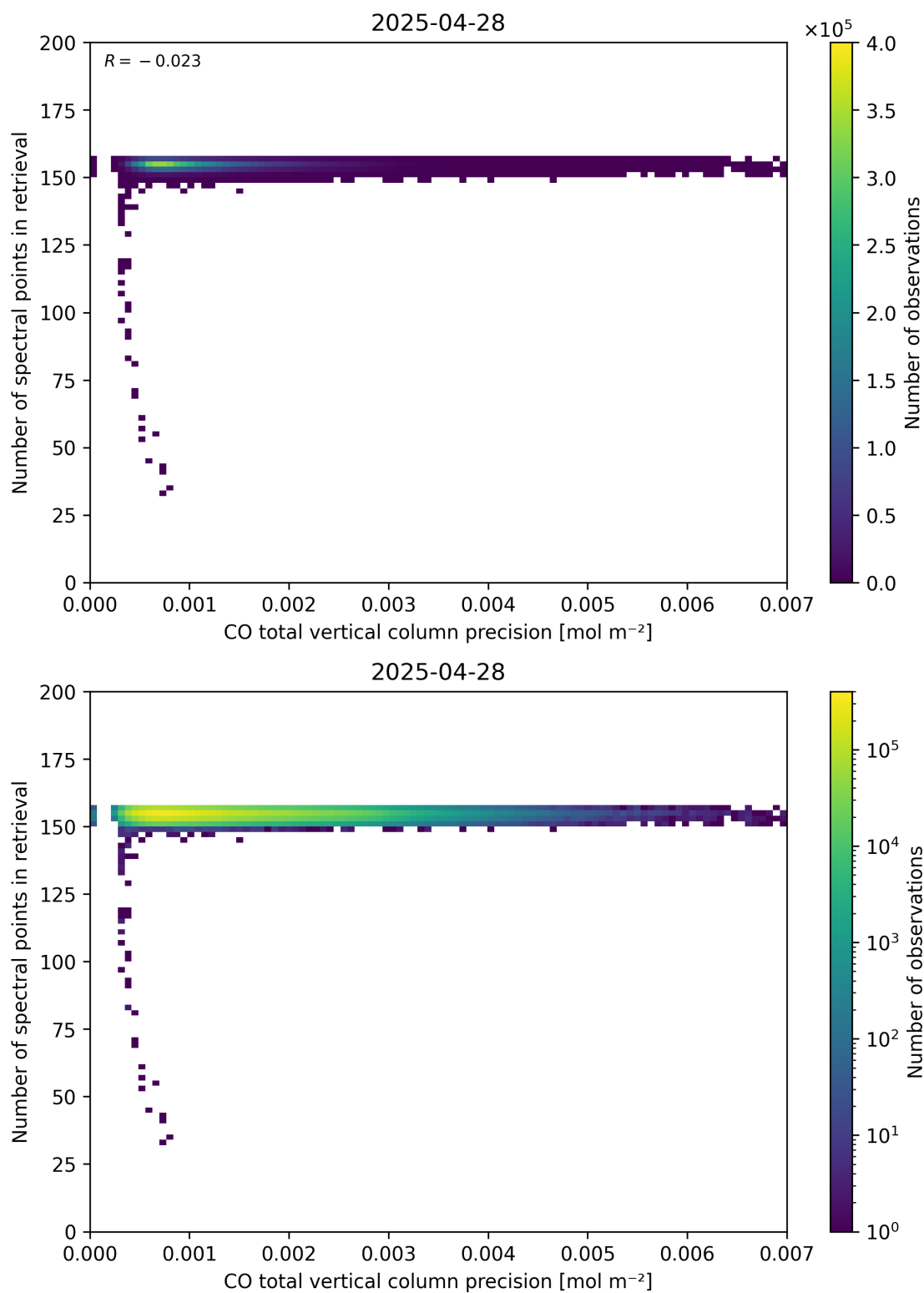
Figure 47: Scatter density plot of “CO total vertical column precision” against “Number of spectral points in retrieval” for 2025-04-27 to 2025-04-29.
