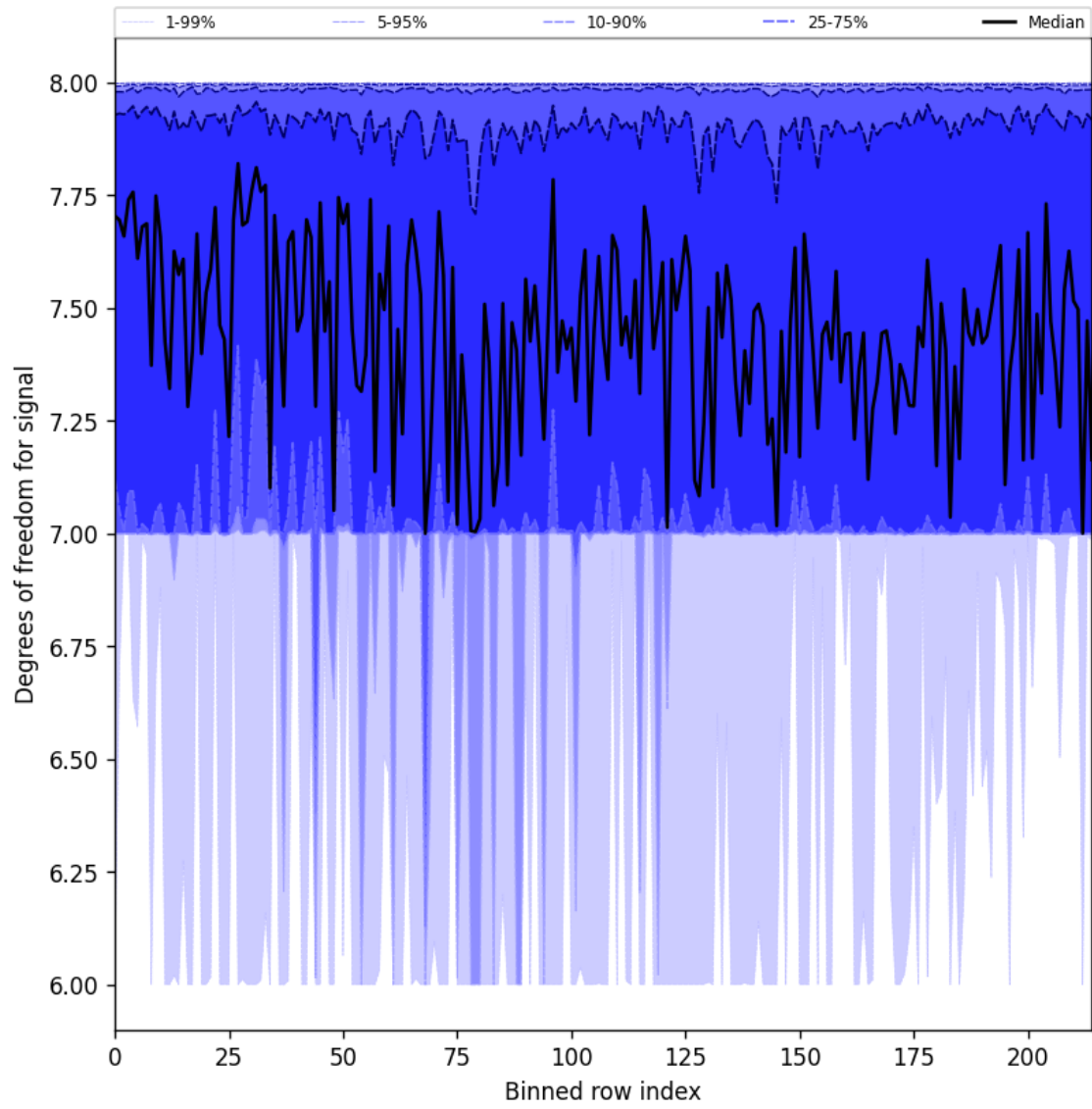
Figure 31: Along track statistics of “Degrees of freedom for signal” for 2025-04-27 to 2025-04-29
