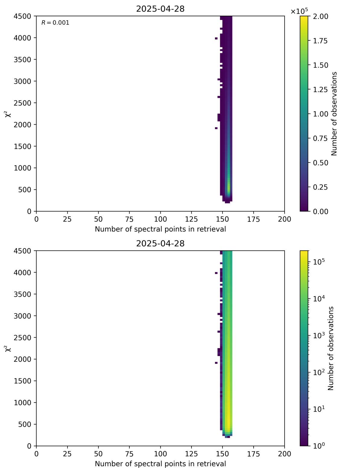
Figure 58: Scatter density plot of “Number of spectral points in retrieval” against “ \chi^2 ” for 2025-04-27 to 2025-04-29.
