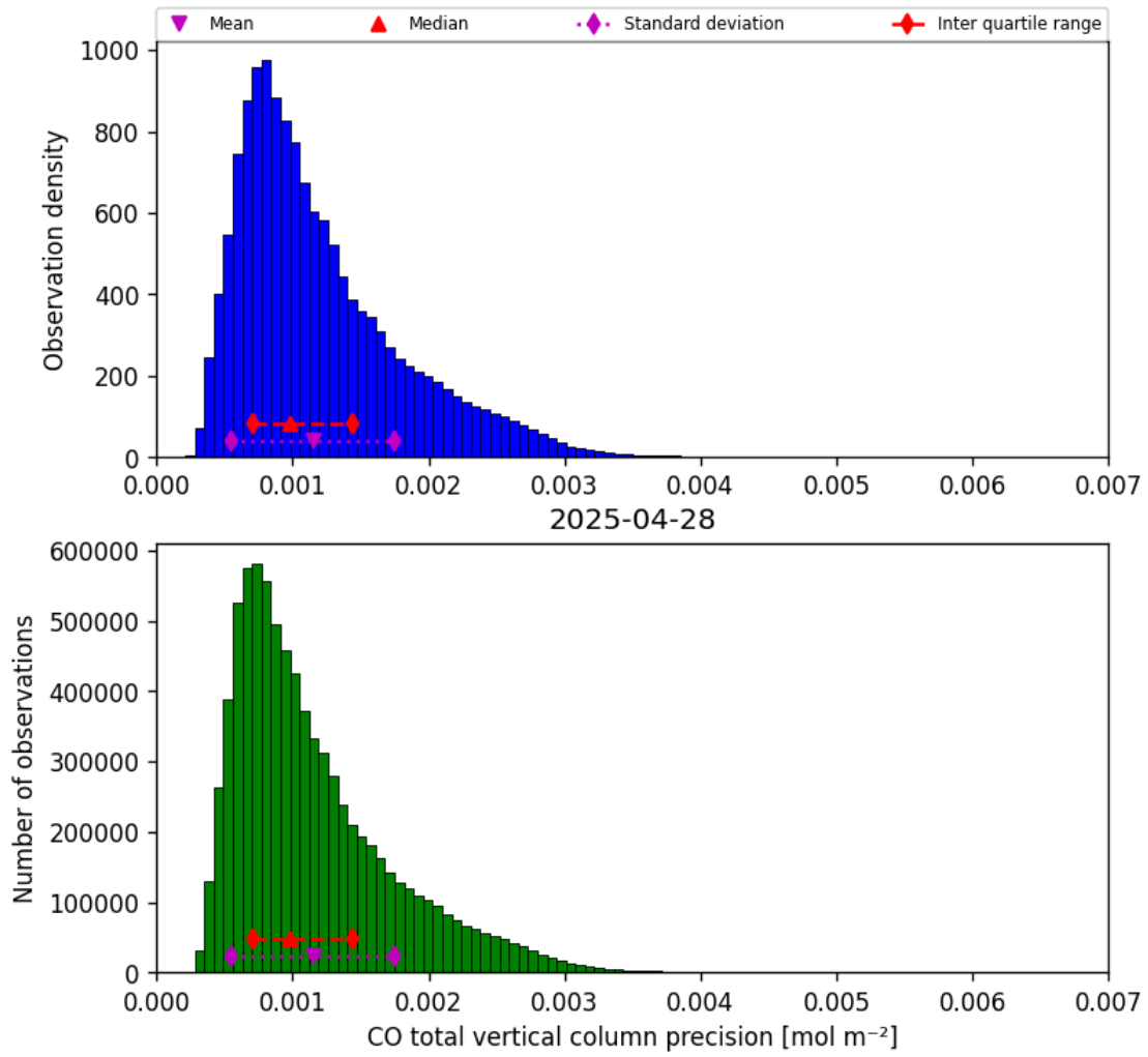
Figure 20: Histogram of “CO total vertical column precision” for 2025-04-27 to 2025-04-29
