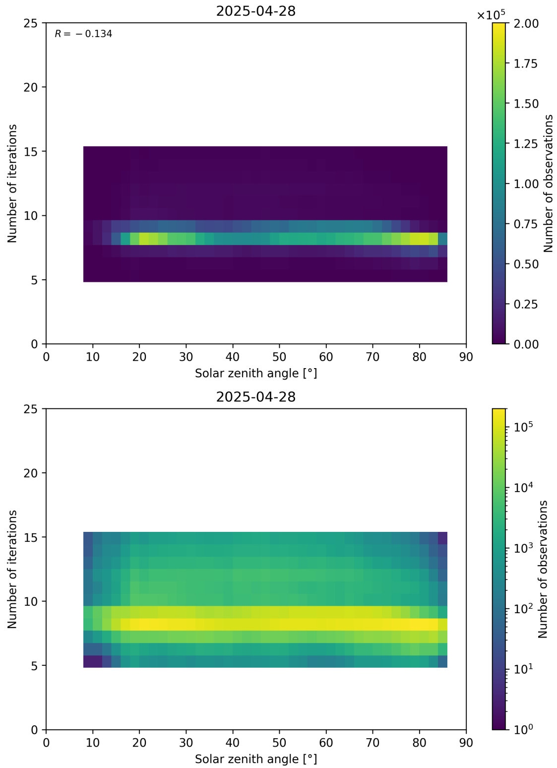
Figure 67: Scatter density plot of “Solar zenith angle” against “Number of iterations” for 2025-04-27 to 2025-04-29.
