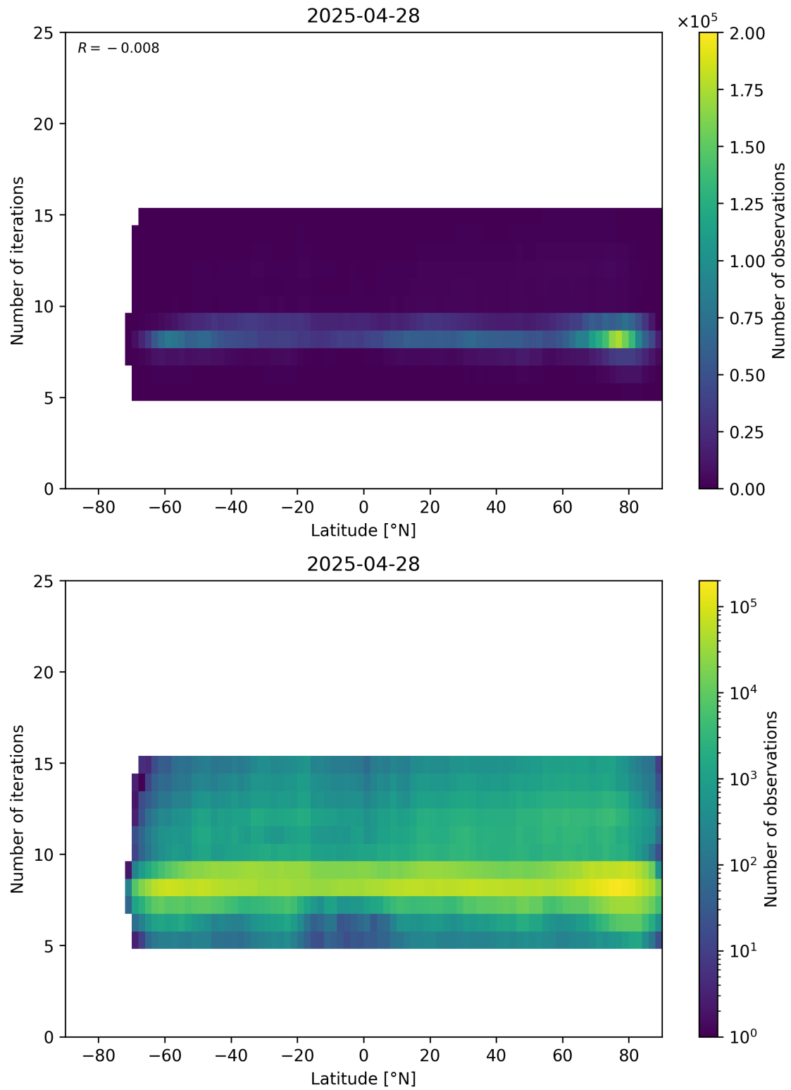
Figure 56: Scatter density plot of “Latitude” against “Number of iterations” for 2025-04-27 to 2025-04-29.
