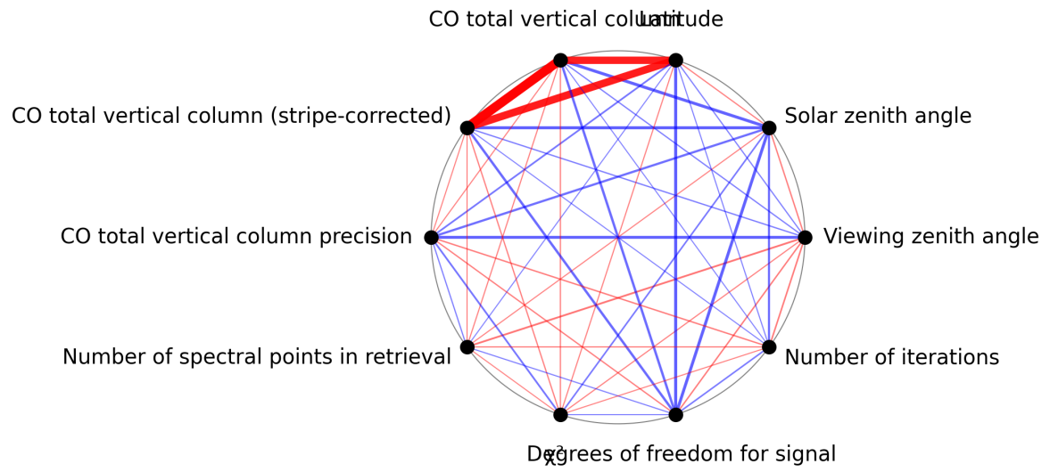
Figure 1: Map of correlation graph for 2025-04-27 to 2025-04-29.
