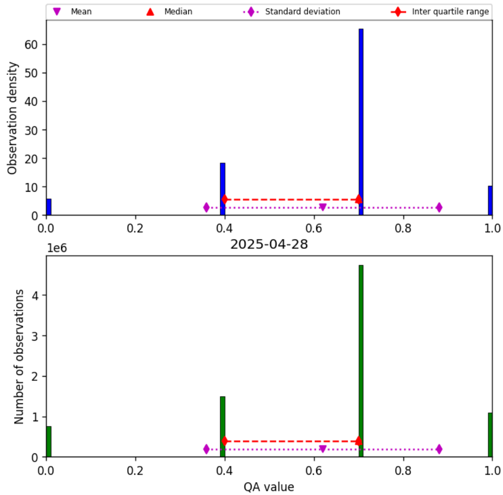
Figure 17: Histogram of “QA value” for 2025-04-27 to 2025-04-29
