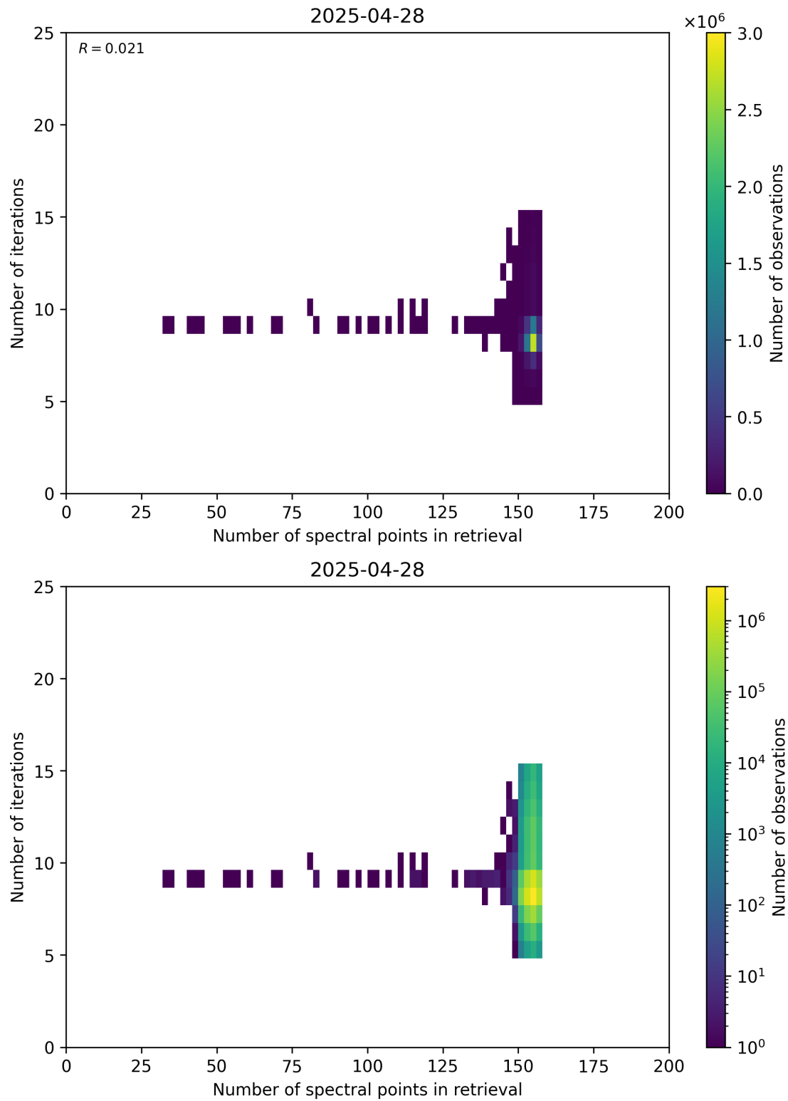
Figure 60: Scatter density plot of “Number of spectral points in retrieval” against “Number of iterations” for 2025-04-27 to 2025-04-29.
