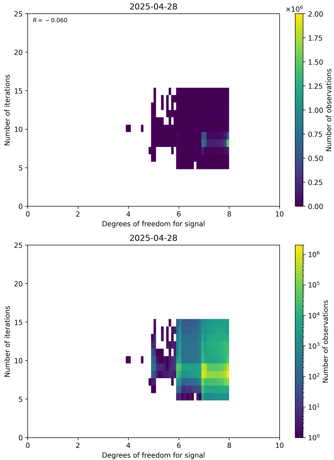
Figure 50: Scatter density plot of “Degrees of freedom for signal” against “Number of iterations” for 2025-04-27 to 2025-04-29.
