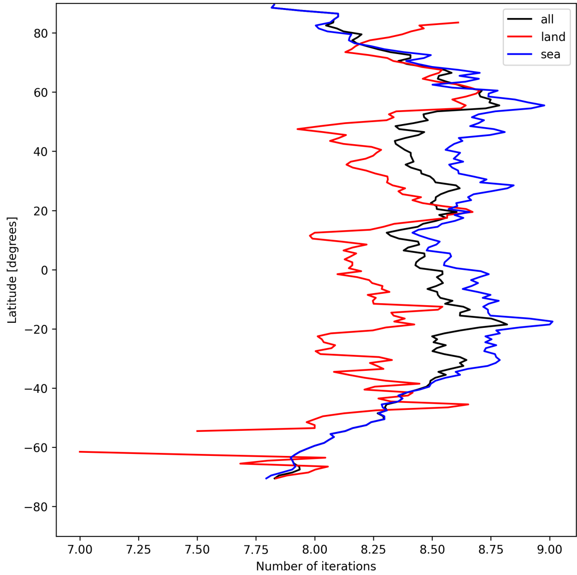
Figure 16: Zonal average of “Number of iterations” for 2025-04-27 to 2025-04-29.
