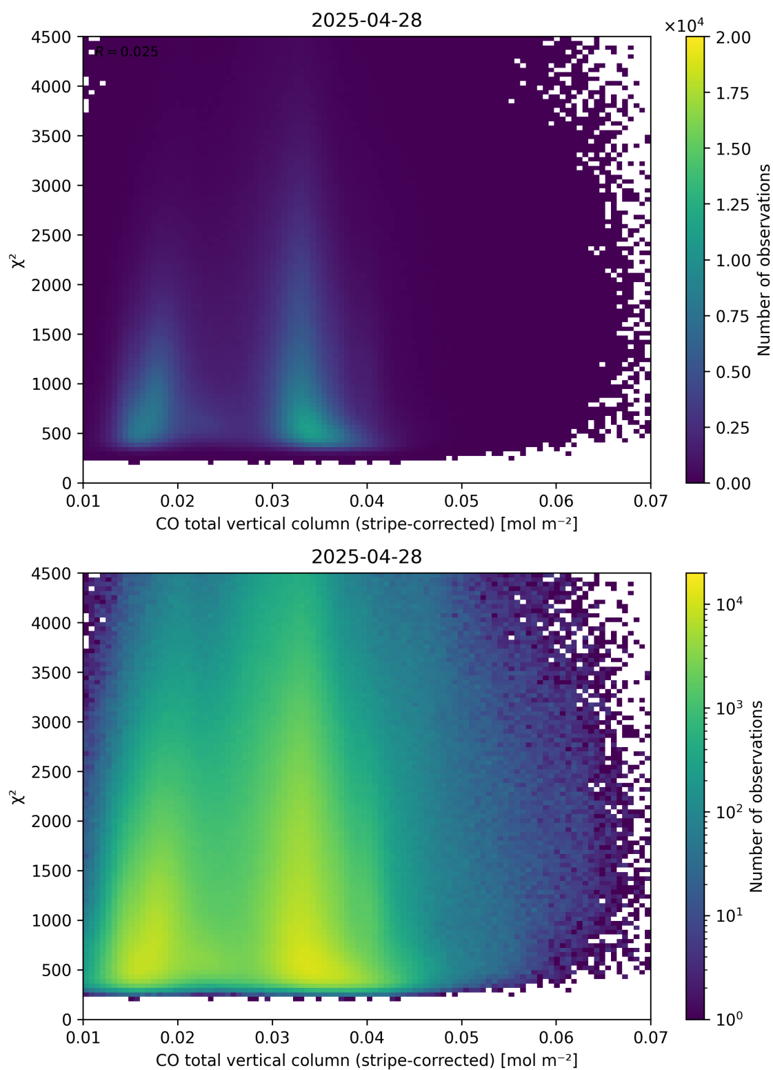
Figure 37: Scatter density plot of “CO total vertical column (stripe-corrected)” against “ \chi^2 ” for 2025-04-27 to 2025-04-29.
