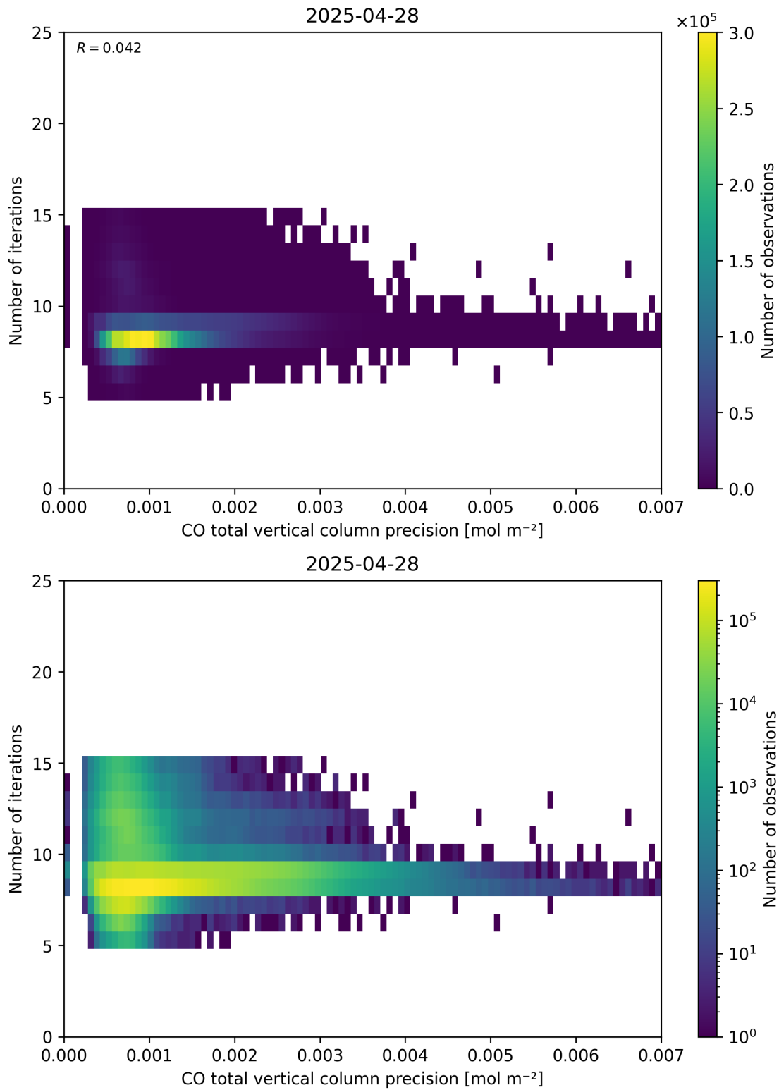
Figure 46: Scatter density plot of “CO total vertical column precision” against “Number of iterations” for 2025-04-27 to 2025-04-29.
