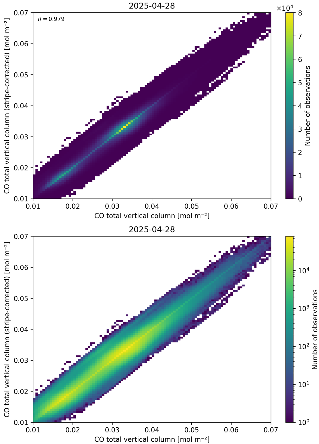
Figure 33: Scatter density plot of “CO total vertical column” against “CO total vertical column (stripe-corrected)” for 2025-04-27 to 2025-04-29.
