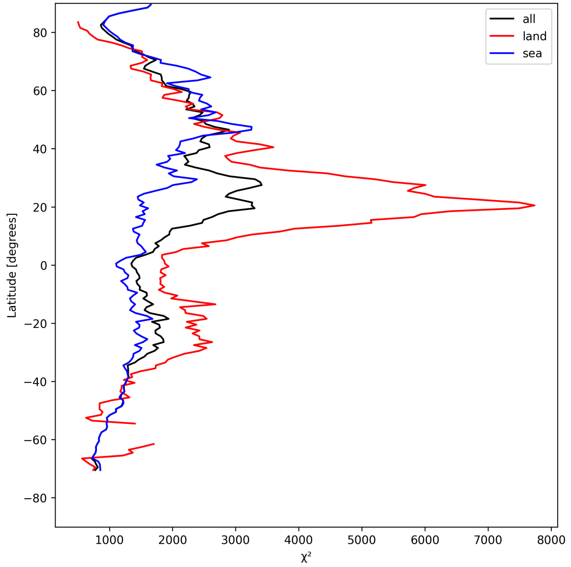
Figure 14: Zonal average of “ \chi^2 ” for 2025-04-27 to 2025-04-29.
