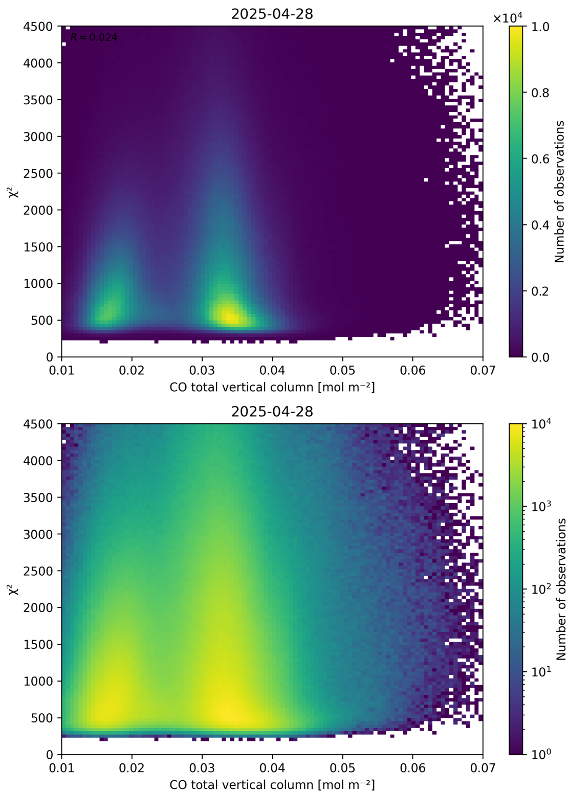
Figure 35: Scatter density plot of “CO total vertical column” against “ \chi^2 ” for 2025-04-27 to 2025-04-29.
