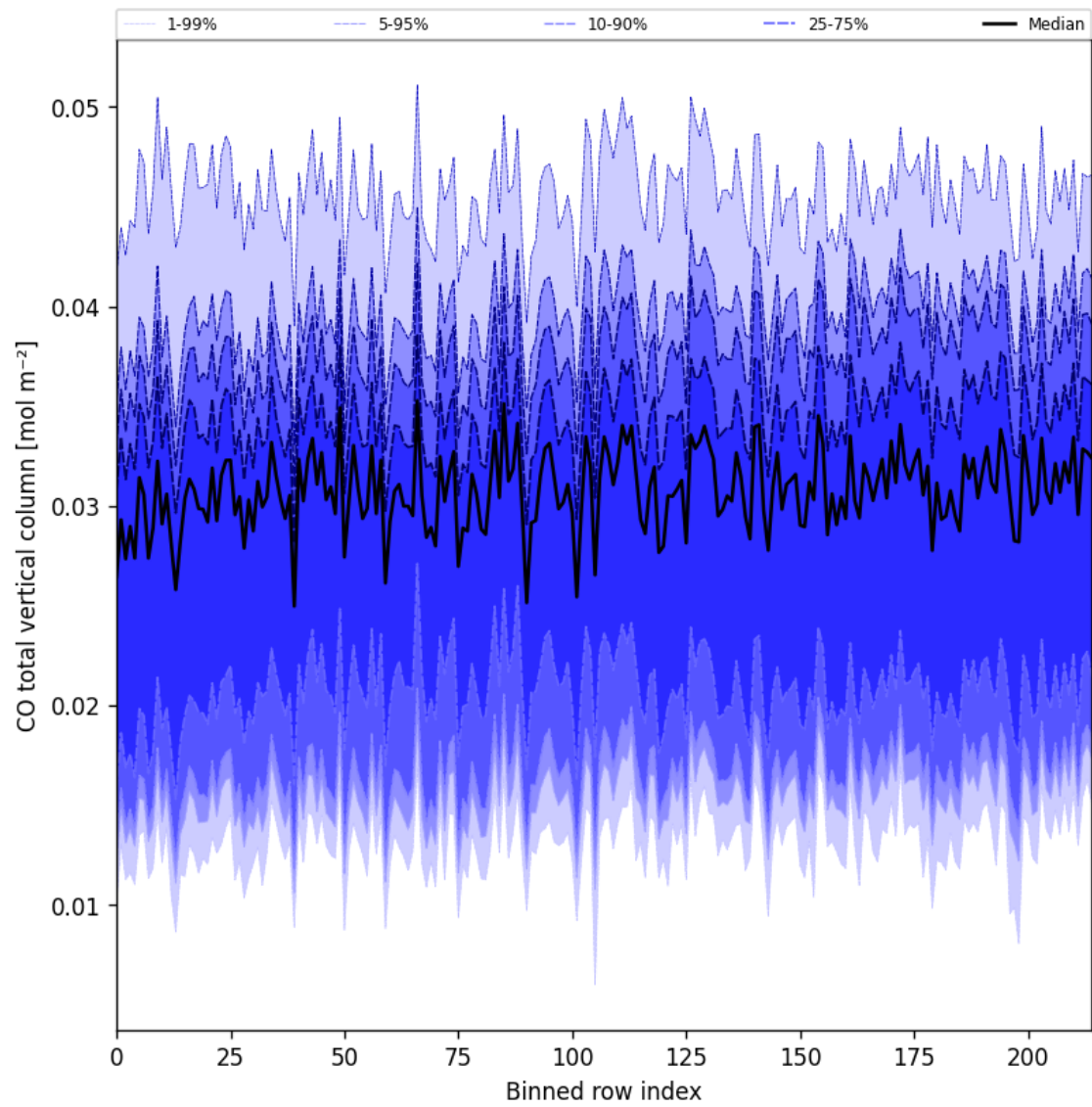
Figure 26: Along track statistics of “CO total vertical column” for 2025-04-27 to 2025-04-29
