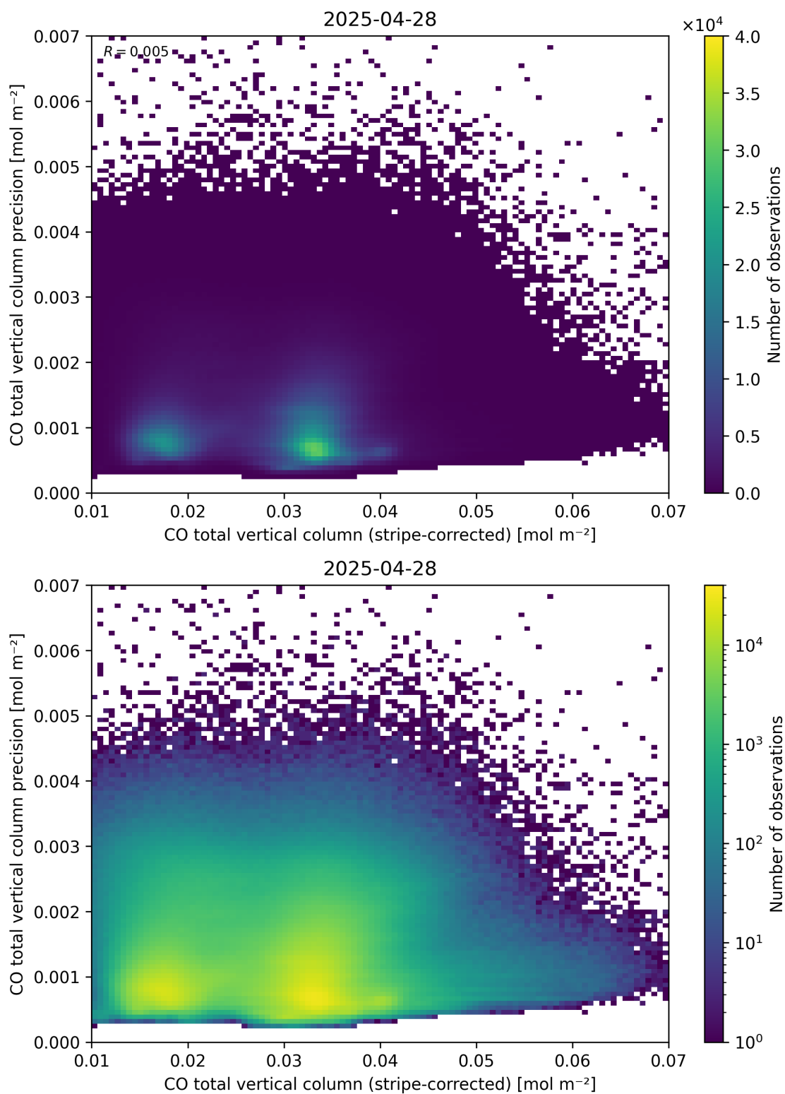
Figure 36: Scatter density plot of “CO total vertical column (stripe-corrected)” against “CO total vertical column precision” for 2025-04-27 to 2025-04-29.
