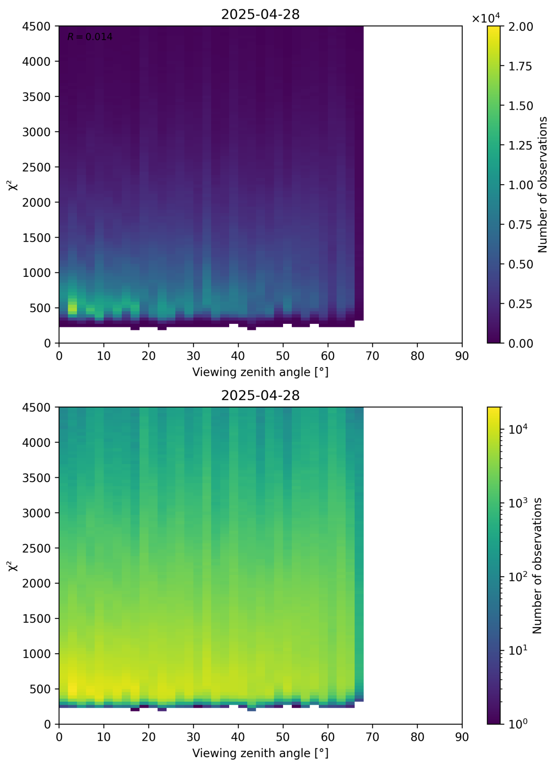
Figure 72: Scatter density plot of “Viewing zenith angle” against “ \chi^2 ” for 2025-04-27 to 2025-04-29.
