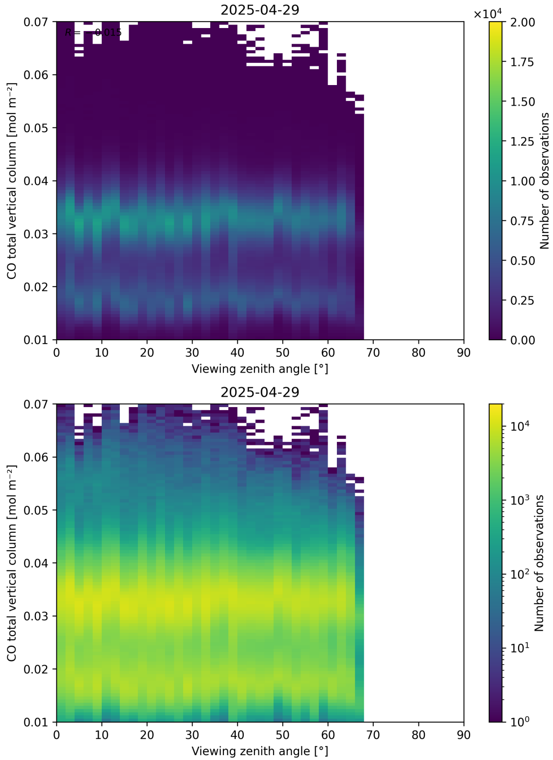
Figure 69: Scatter density plot of “Viewing zenith angle” against “CO total vertical column” for 2025-04-29 to 2025-04-30.
