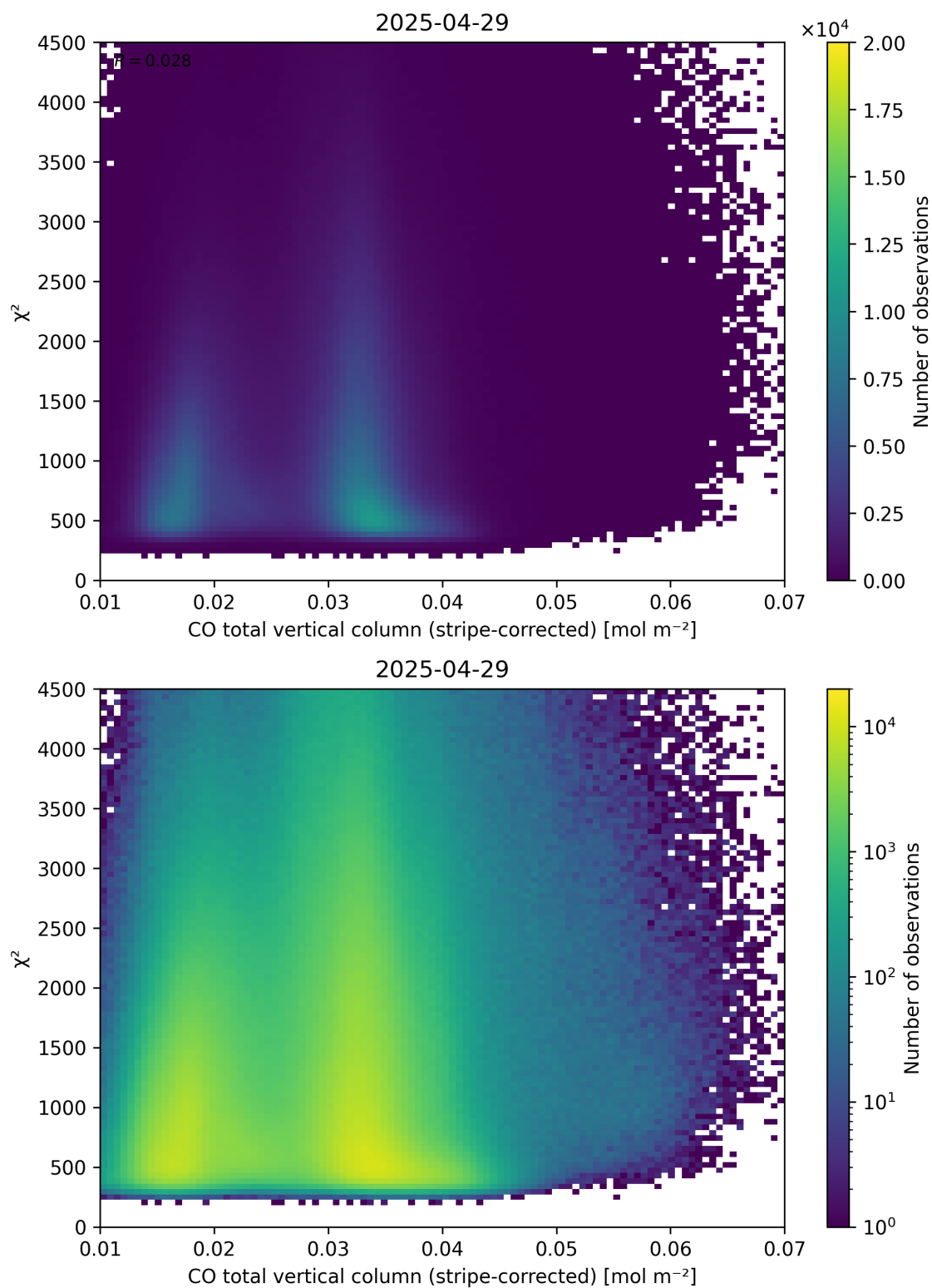
Figure 37: Scatter density plot of “CO total vertical column (stripe-corrected)” against “ \chi^2 ” for 2025-04-29 to 2025-04-30.
