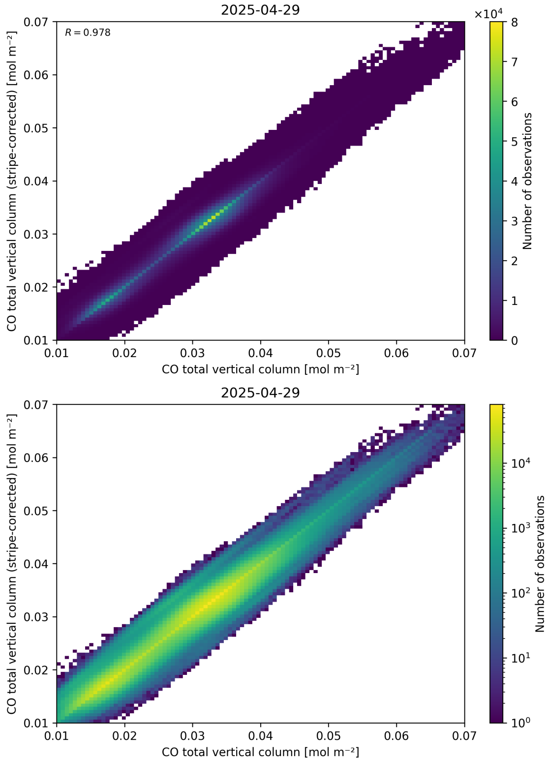
Figure 33: Scatter density plot of “CO total vertical column” against “CO total vertical column (stripe-corrected)” for 2025-04-29 to 2025-04-30.
