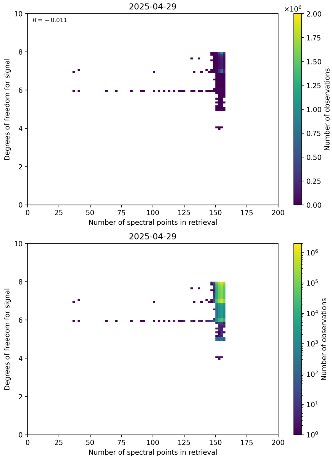
Figure 59: Scatter density plot of “Number of spectral points in retrieval” against “Degrees of freedom for signal” for 2025-04-29 to 2025-04-30.
