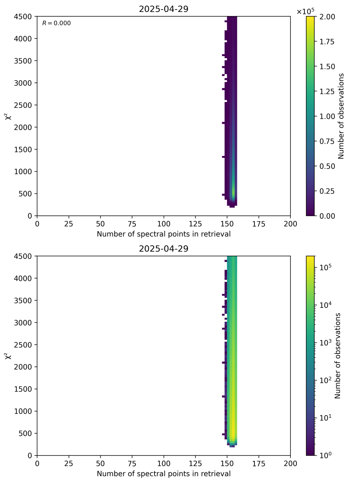
Figure 58: Scatter density plot of “Number of spectral points in retrieval” against “ \chi^2 ” for 2025-04-29 to 2025-04-30.
