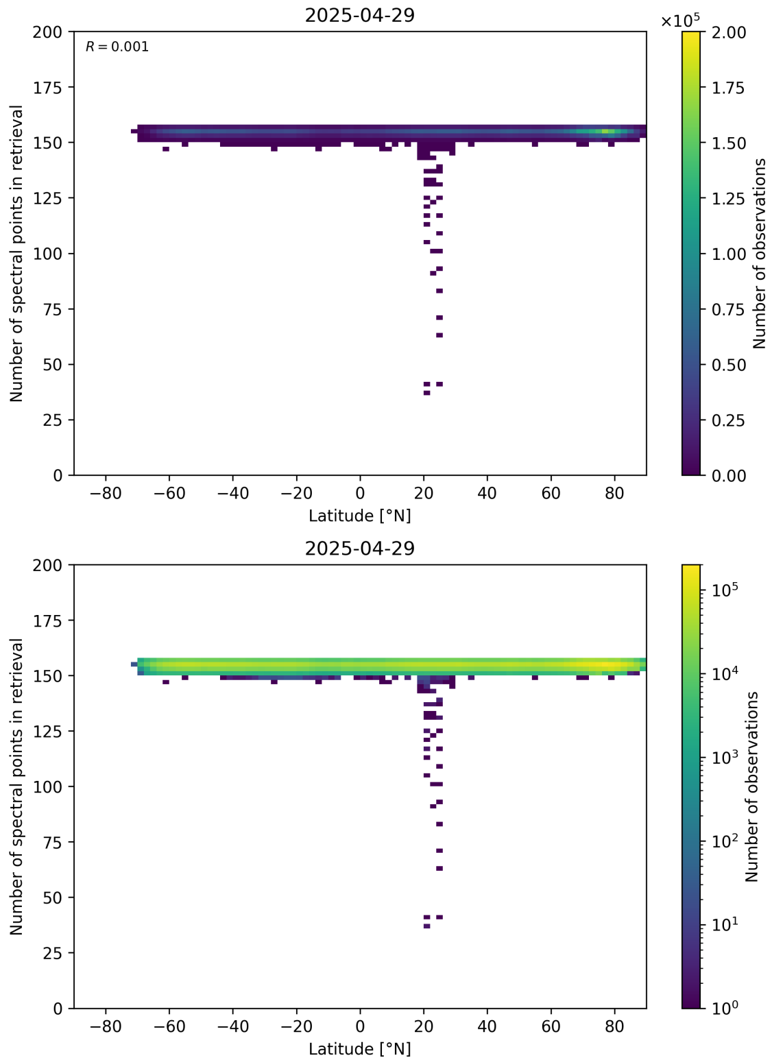
Figure 57: Scatter density plot of “Latitude” against “Number of spectral points in retrieval” for 2025-04-29 to 2025-04-30.
