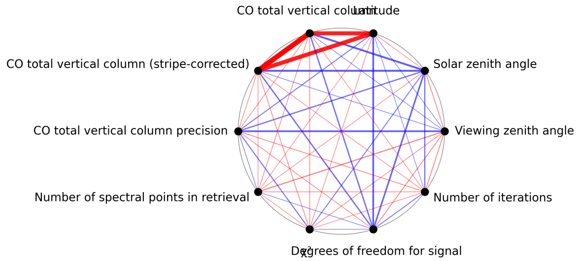
Figure 1: Map of correlation graph for 2025-04-29 to 2025-04-30.
