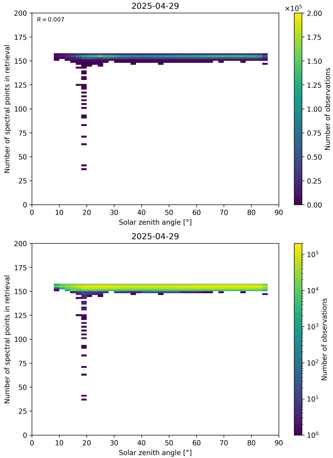
Figure 68: Scatter density plot of “Solar zenith angle” against “Number of spectral points in retrieval” for 2025-04-29 to 2025-04-30.
