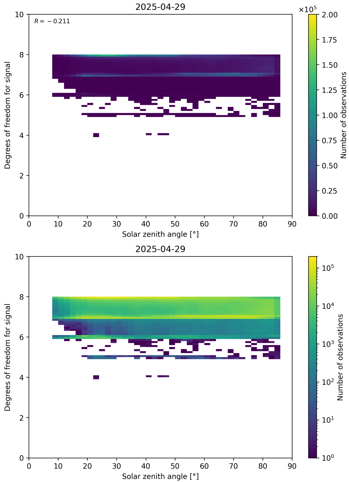
Figure 65: Scatter density plot of “Solar zenith angle” against “Degrees of freedom for signal” for 2025-04-29 to 2025-04-30.
