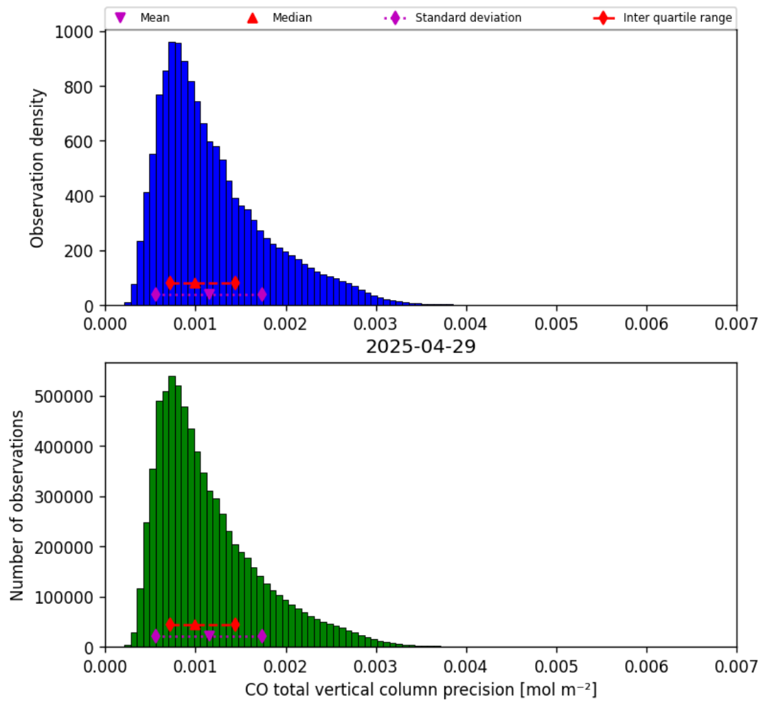
Figure 20: Histogram of “CO total vertical column precision” for 2025-04-29 to 2025-04-30
