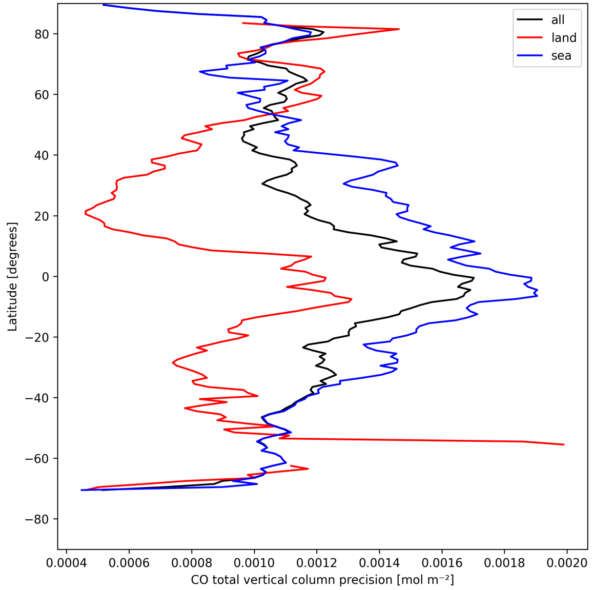
Figure 12: Zonal average of “CO total vertical column precision” for 2025-04-29 to 2025-04-30.
