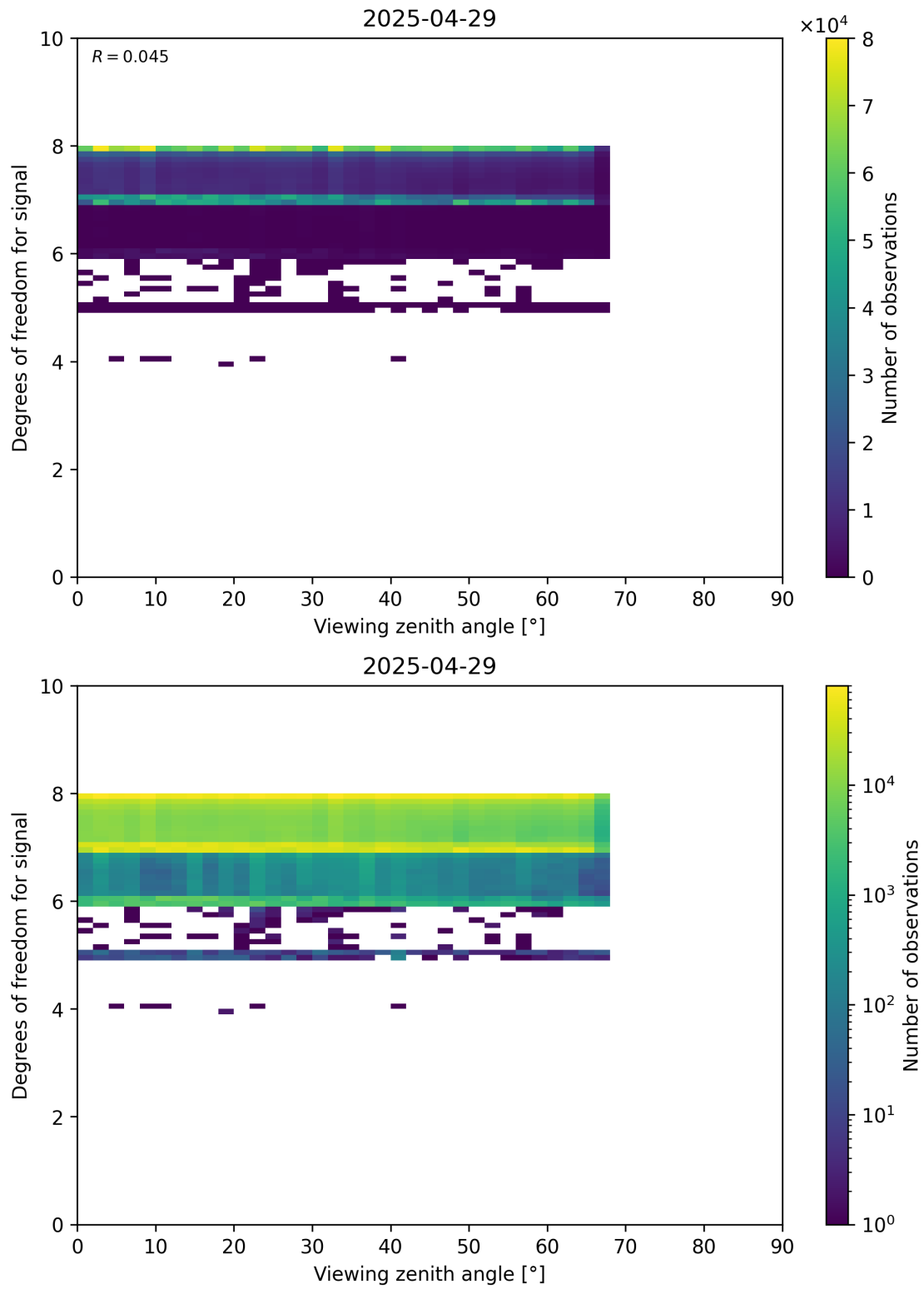
Figure 73: Scatter density plot of “Viewing zenith angle” against “Degrees of freedom for signal” for 2025-04-29 to 2025-04-30.
