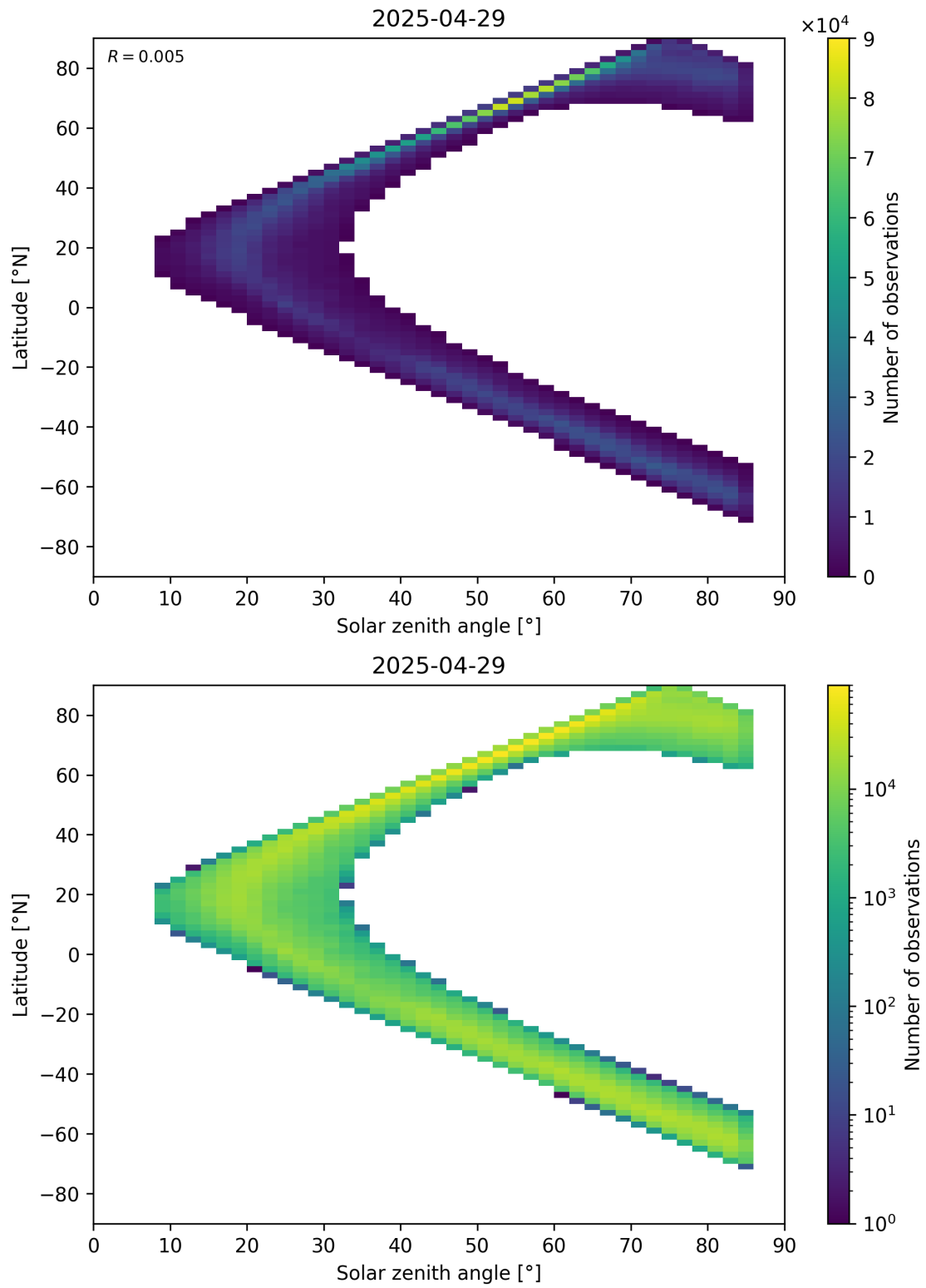
Figure 66: Scatter density plot of “Solar zenith angle” against “Latitude” for 2025-04-29 to 2025-04-30.
