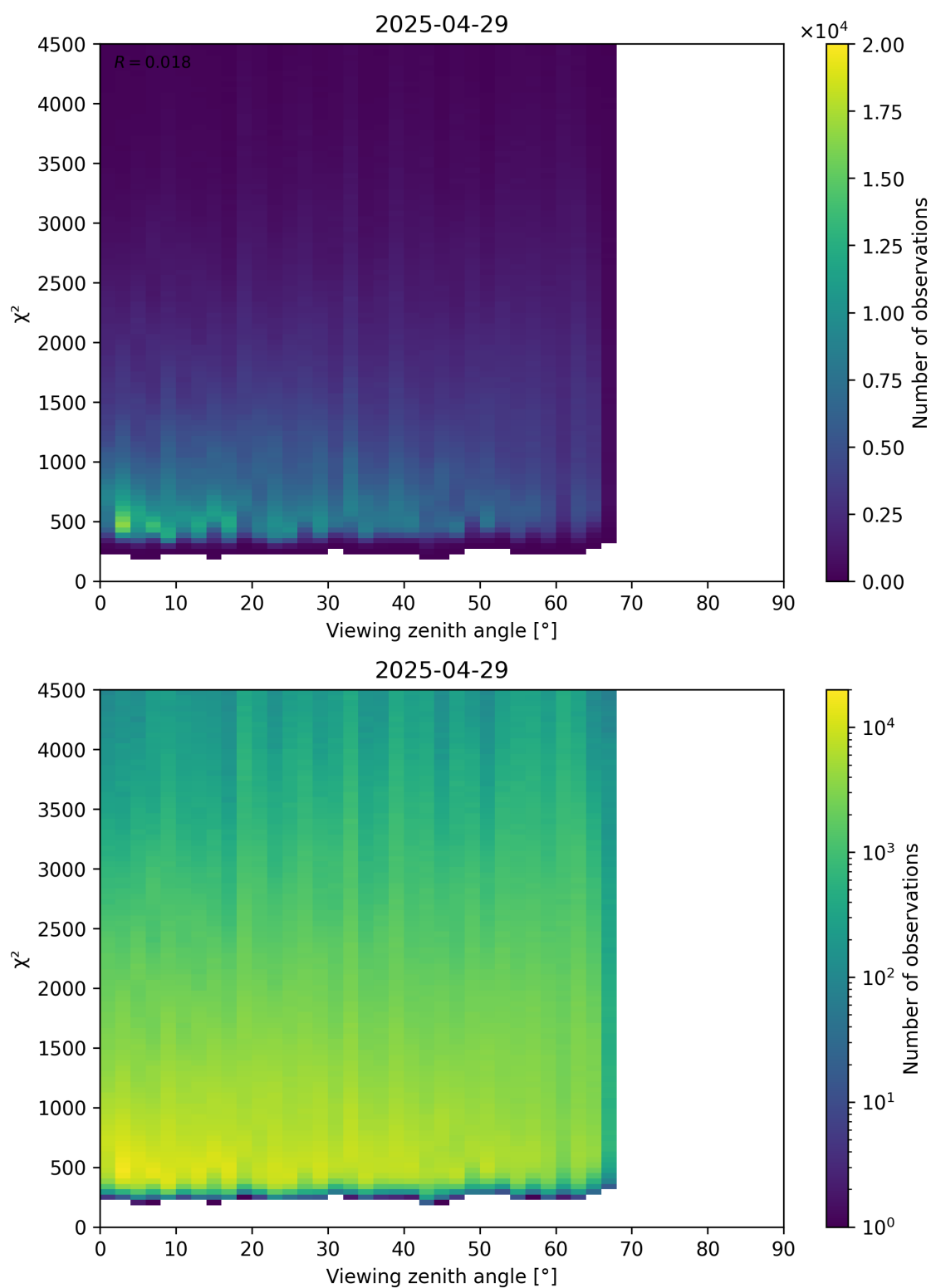
Figure 72: Scatter density plot of “Viewing zenith angle” against “ \chi^2 ” for 2025-04-29 to 2025-04-30.
