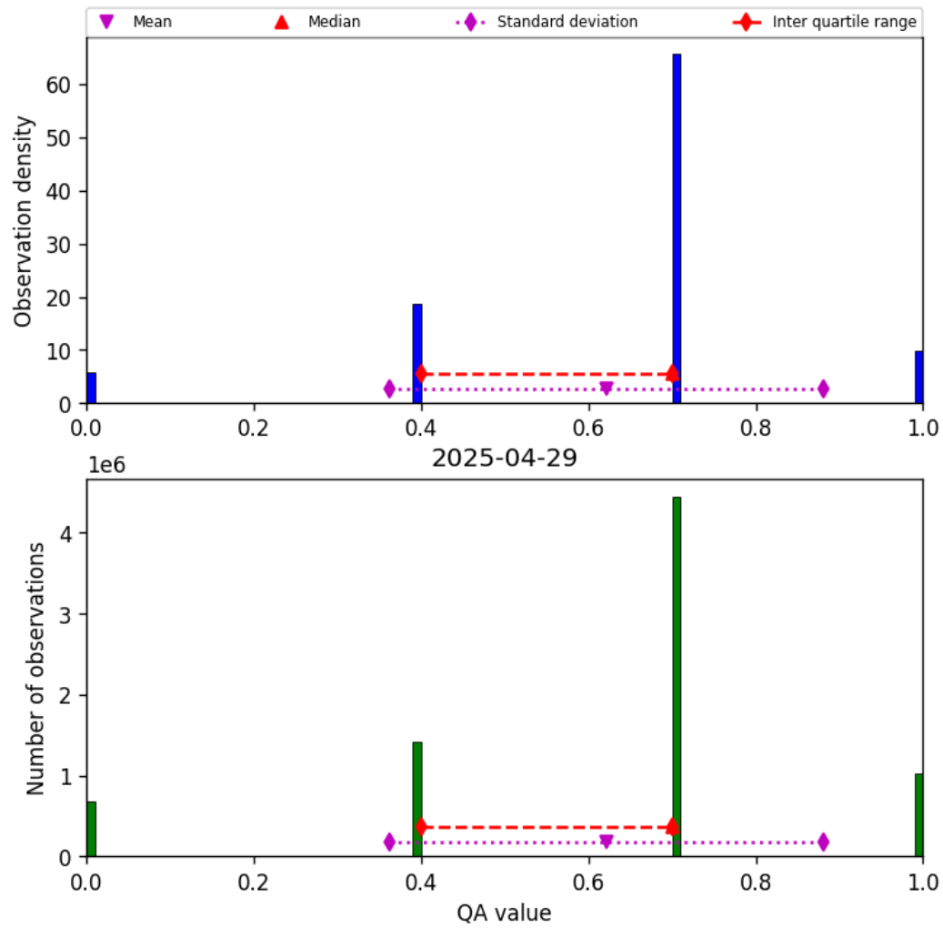
Figure 17: Histogram of “QA value” for 2025-04-29 to 2025-04-30
