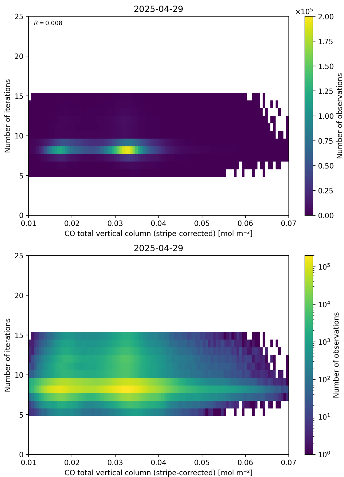
Figure 39: Scatter density plot of “CO total vertical column (stripe-corrected)” against “Number of iterations” for 2025-04-29 to 2025-04-30.
