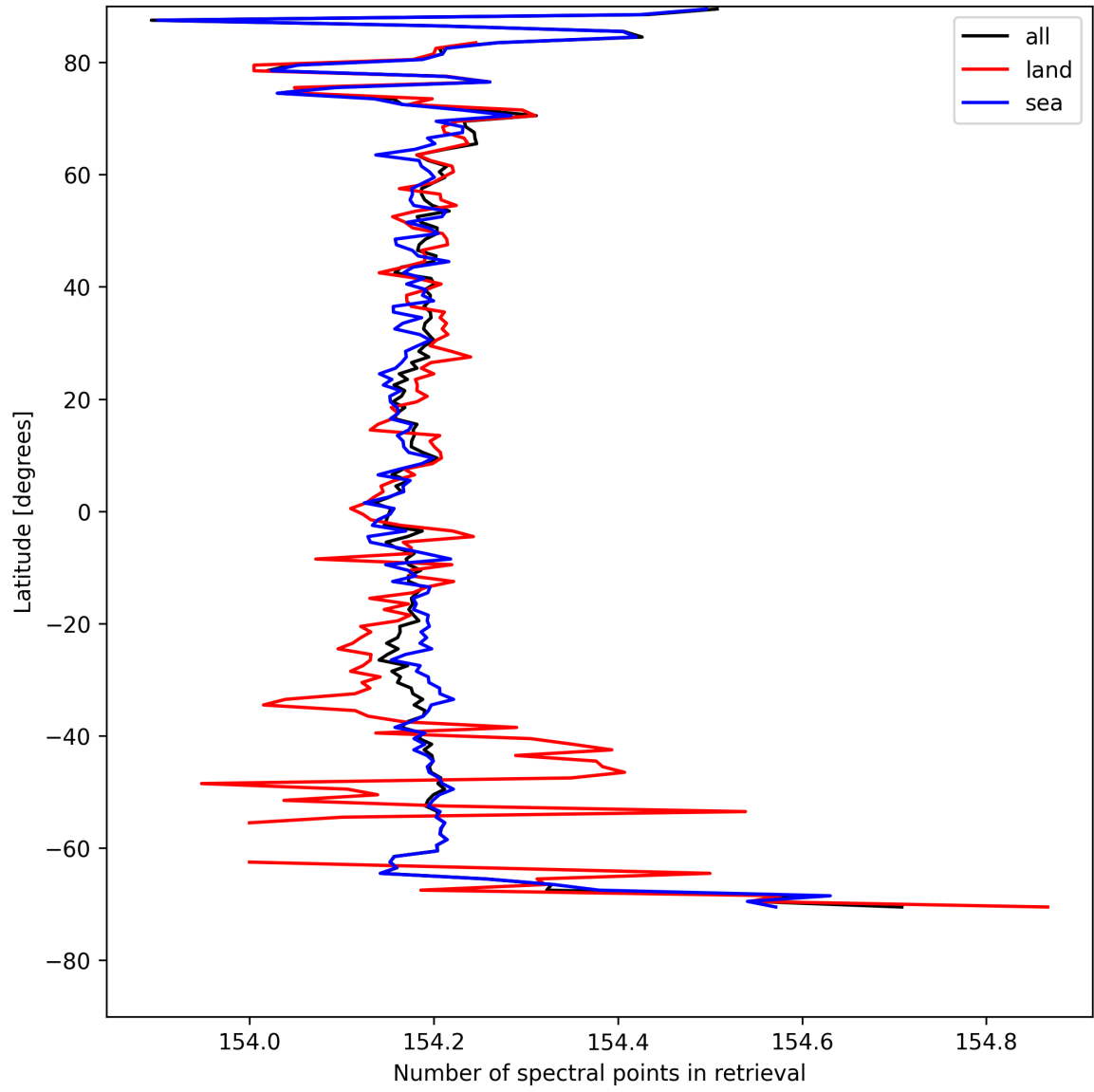
Figure 13: Zonal average of “Number of spectral points in retrieval” for 2025-04-29 to 2025-04-30.
