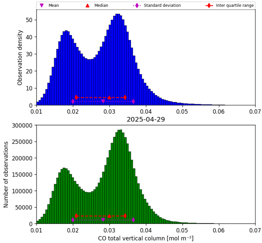
Figure 18: Histogram of “CO total vertical column” for 2025-04-29 to 2025-04-30
