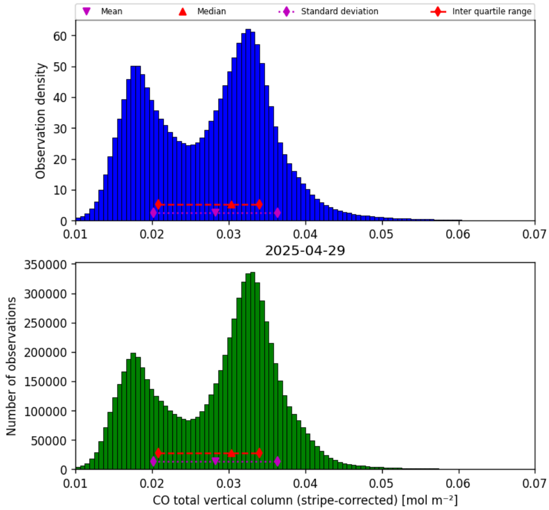
Figure 19: Histogram of “CO total vertical column (stripe-corrected)” for 2025-04-29 to 2025-04-30
