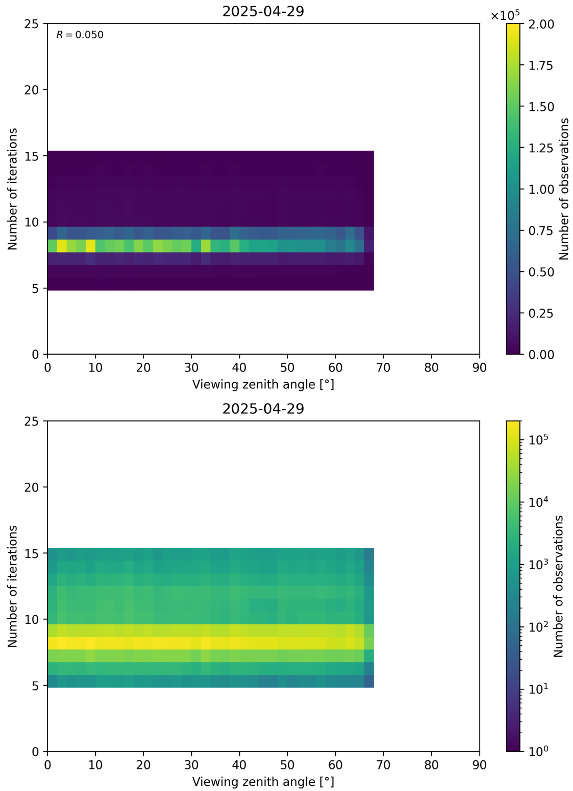
Figure 75: Scatter density plot of “Viewing zenith angle” against “Number of iterations” for 2025-04-29 to 2025-04-30.
