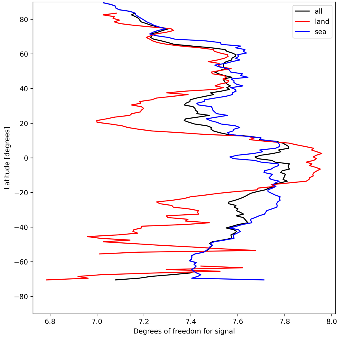
Figure 15: Zonal average of “Degrees of freedom for signal” for 2025-04-29 to 2025-04-30.
