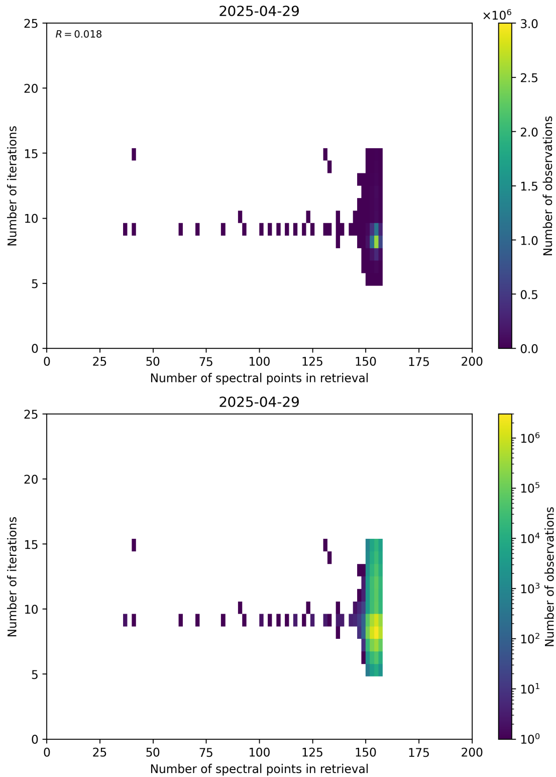
Figure 60: Scatter density plot of “Number of spectral points in retrieval” against “Number of iterations” for 2025-04-29 to 2025-04-30.
