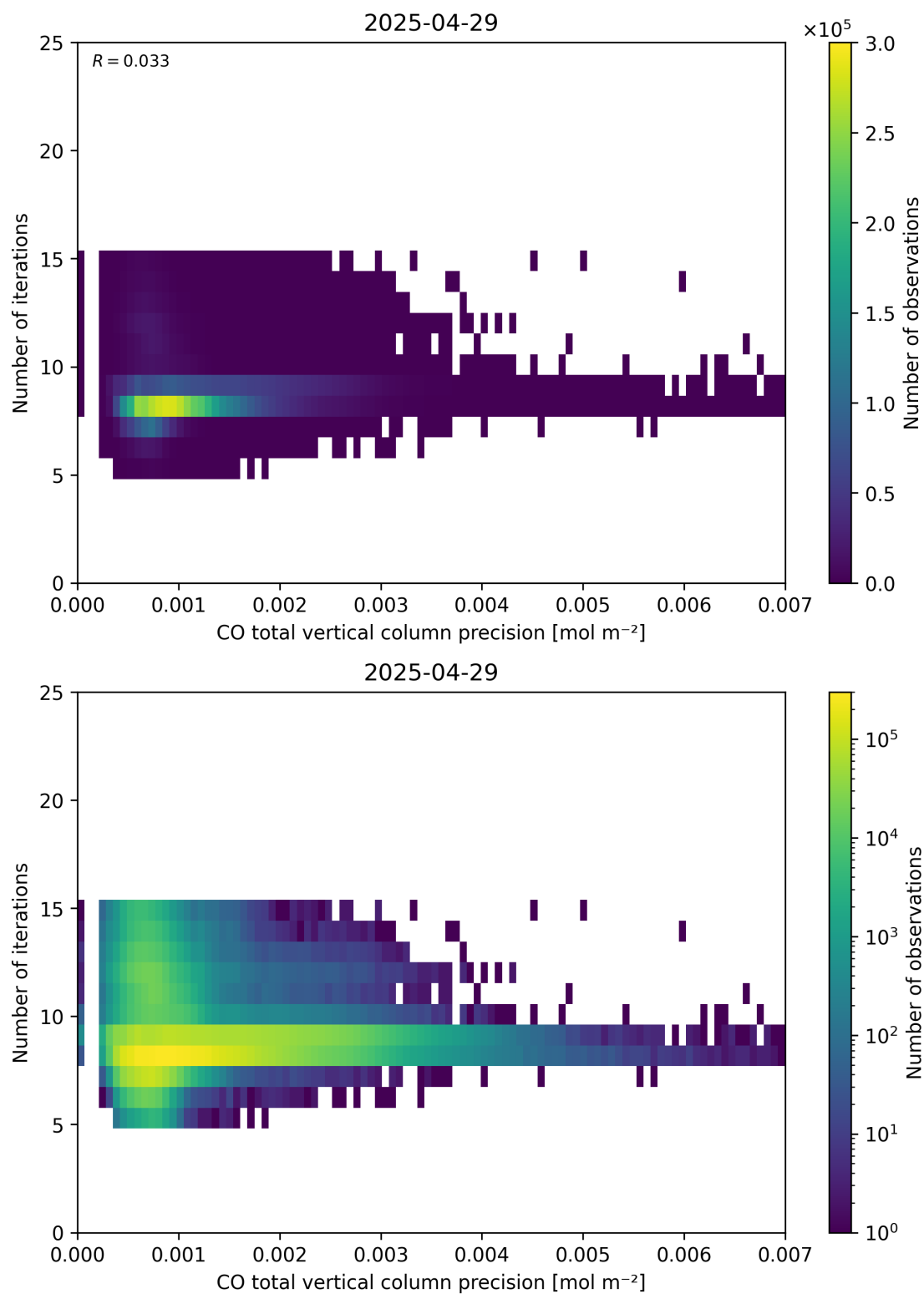
Figure 46: Scatter density plot of “CO total vertical column precision” against “Number of iterations” for 2025-04-29 to 2025-04-30.
