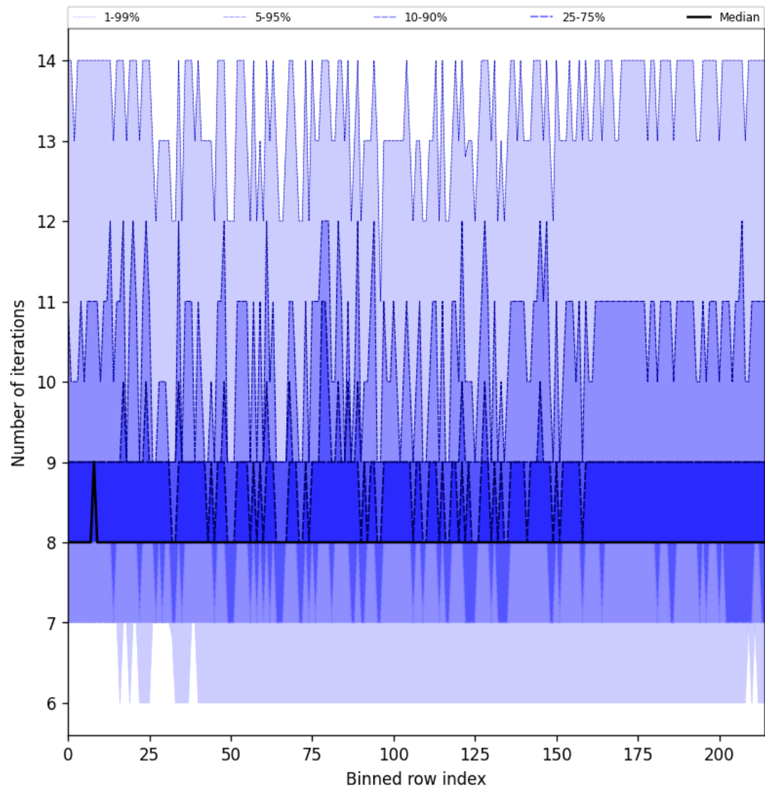
Figure 32: Along track statistics of “Number of iterations” for 2025-04-29 to 2025-04-30
