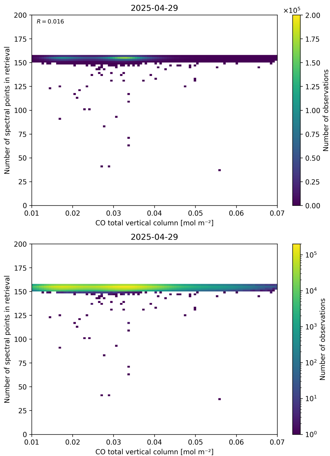
Figure 43: Scatter density plot of “CO total vertical column” against “Number of spectral points in retrieval” for 2025-04-29 to 2025-04-30.
