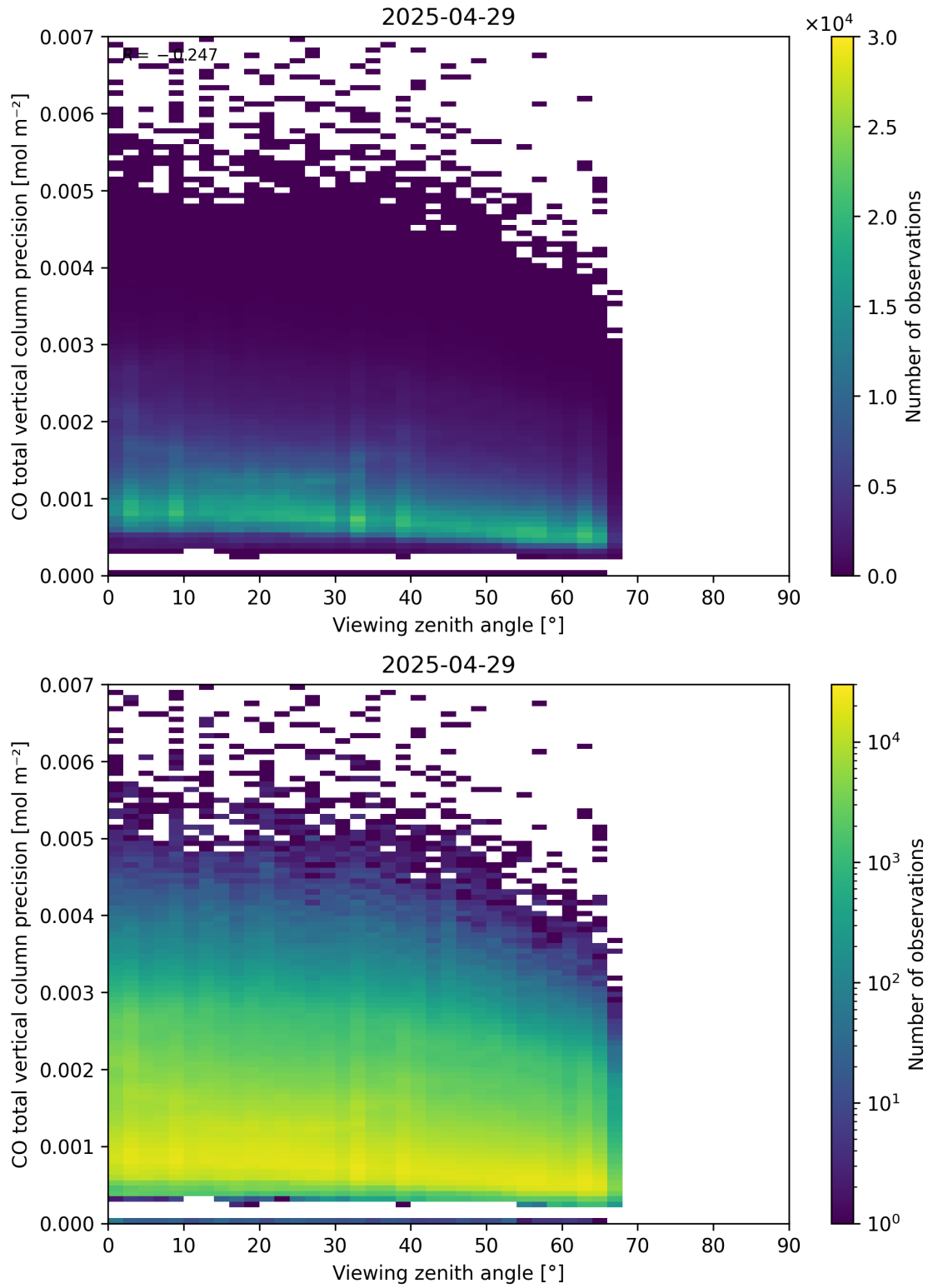
Figure 71: Scatter density plot of “Viewing zenith angle” against “CO total vertical column precision” for 2025-04-29 to 2025-04-30.
