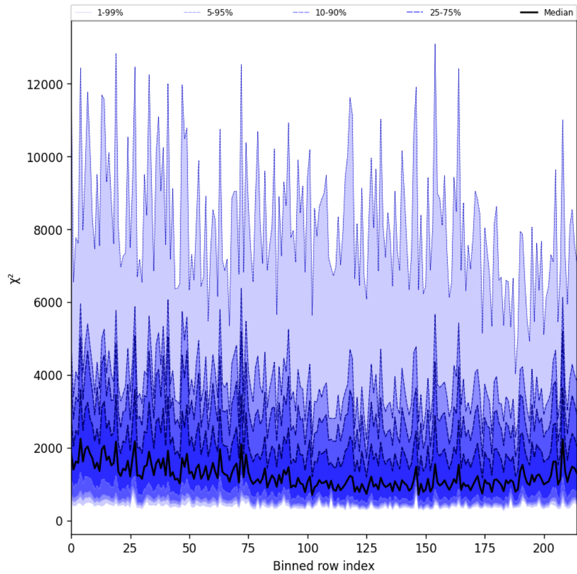
Figure 30: Along track statistics of “ \chi^2 ” for 2025-04-29 to 2025-04-30
