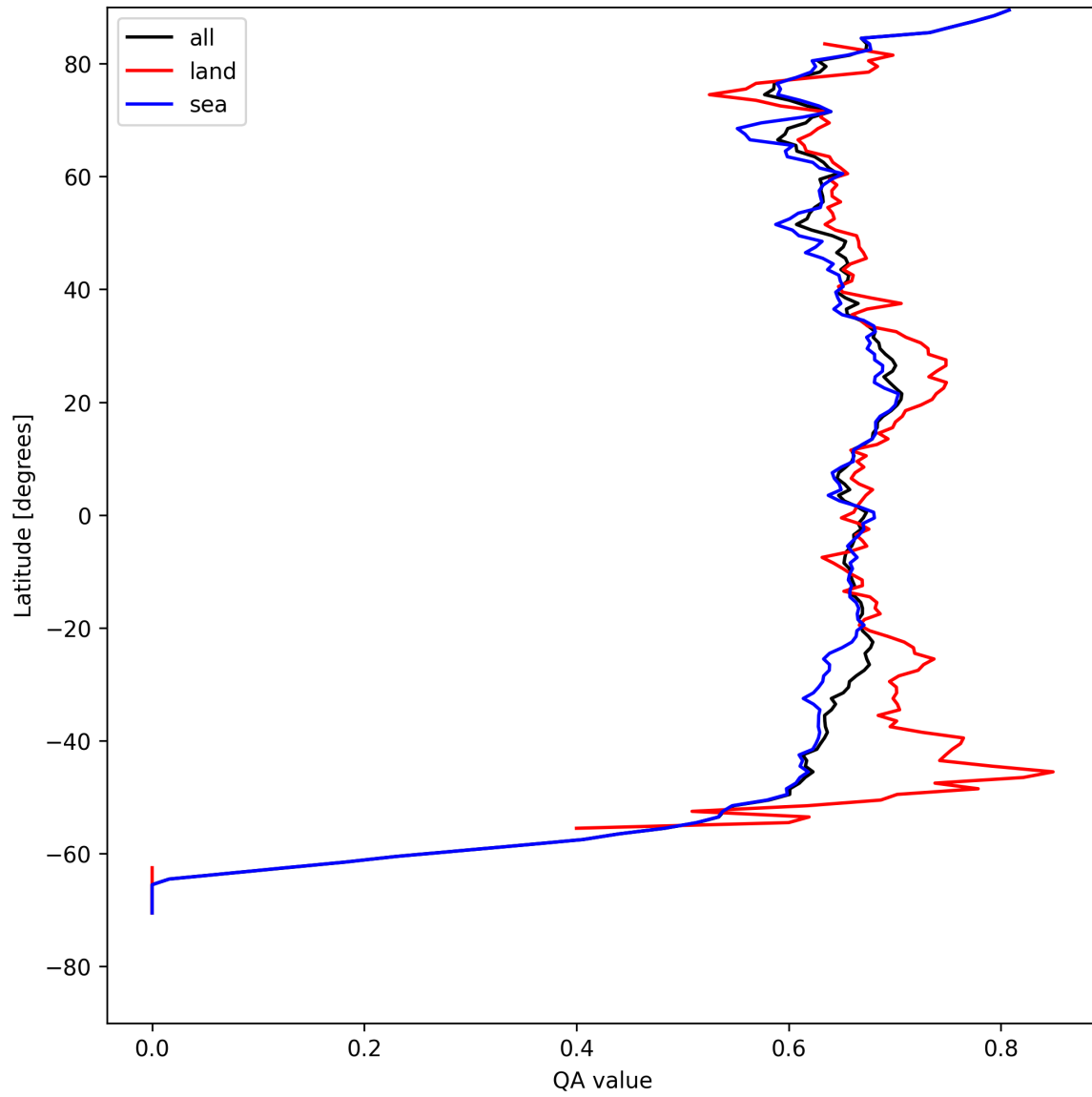
Figure 9: Zonal average of “QA value” for 2025-04-29 to 2025-04-30.
