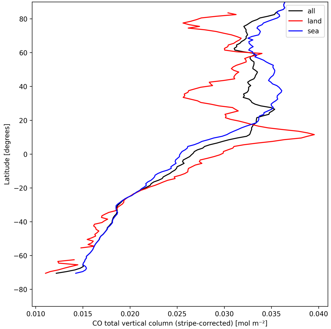
Figure 11: Zonal average of “CO total vertical column (stripe-corrected)” for 2025-04-29 to 2025-04-30.
