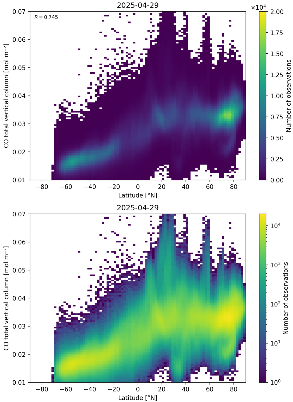
Figure 51: Scatter density plot of “Latitude” against “CO total vertical column” for 2025-04-29 to 2025-04-30.
