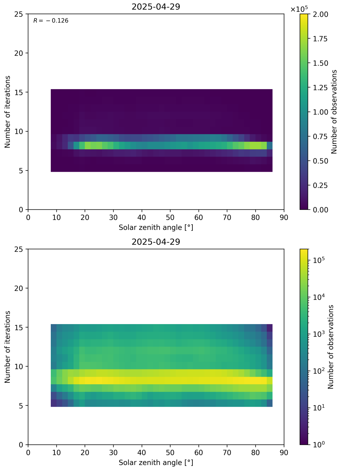
Figure 67: Scatter density plot of “Solar zenith angle” against “Number of iterations” for 2025-04-29 to 2025-04-30.
