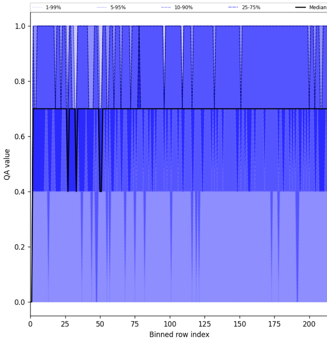
Figure 25: Along track statistics of “QA value” for 2025-04-29 to 2025-04-30
