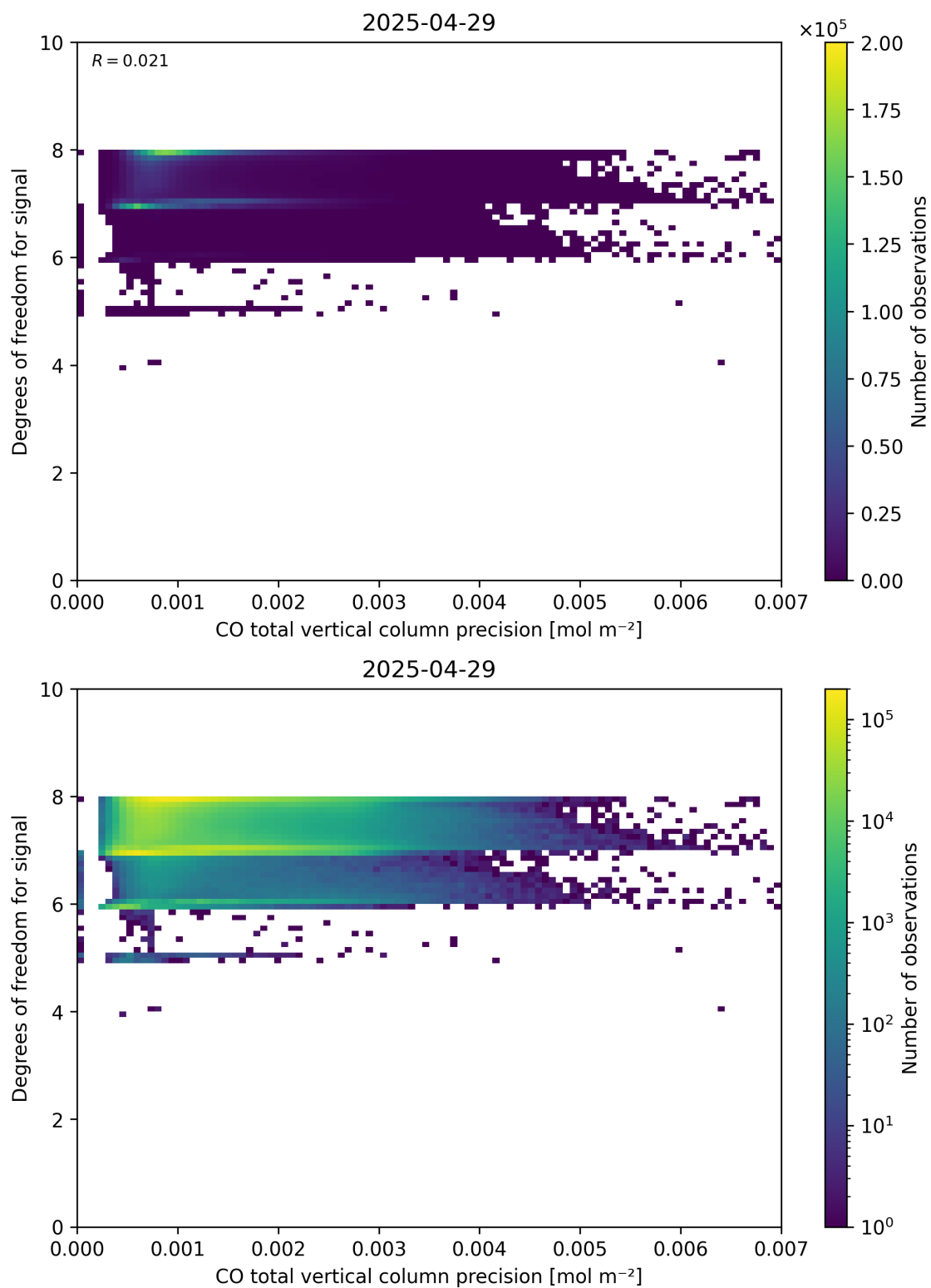
Figure 45: Scatter density plot of “CO total vertical column precision” against “Degrees of freedom for signal” for 2025-04-29 to 2025-04-30.
