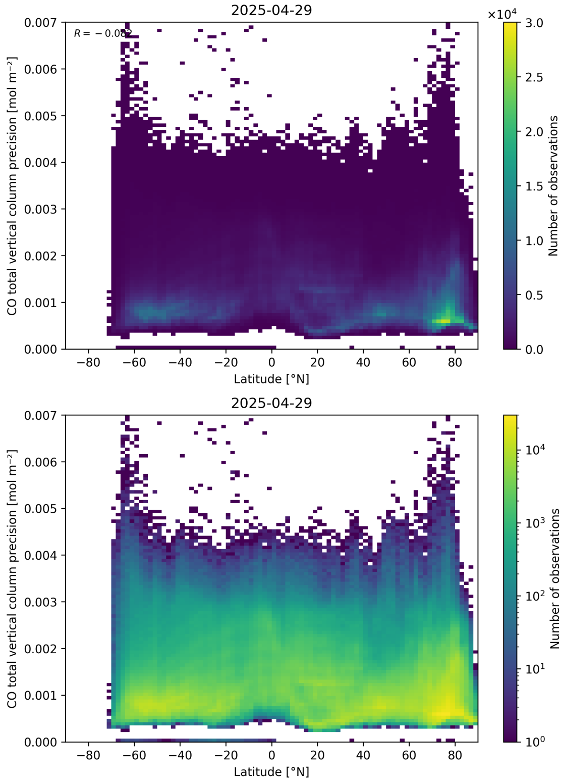
Figure 53: Scatter density plot of “Latitude” against “CO total vertical column precision” for 2025-04-29 to 2025-04-30.
