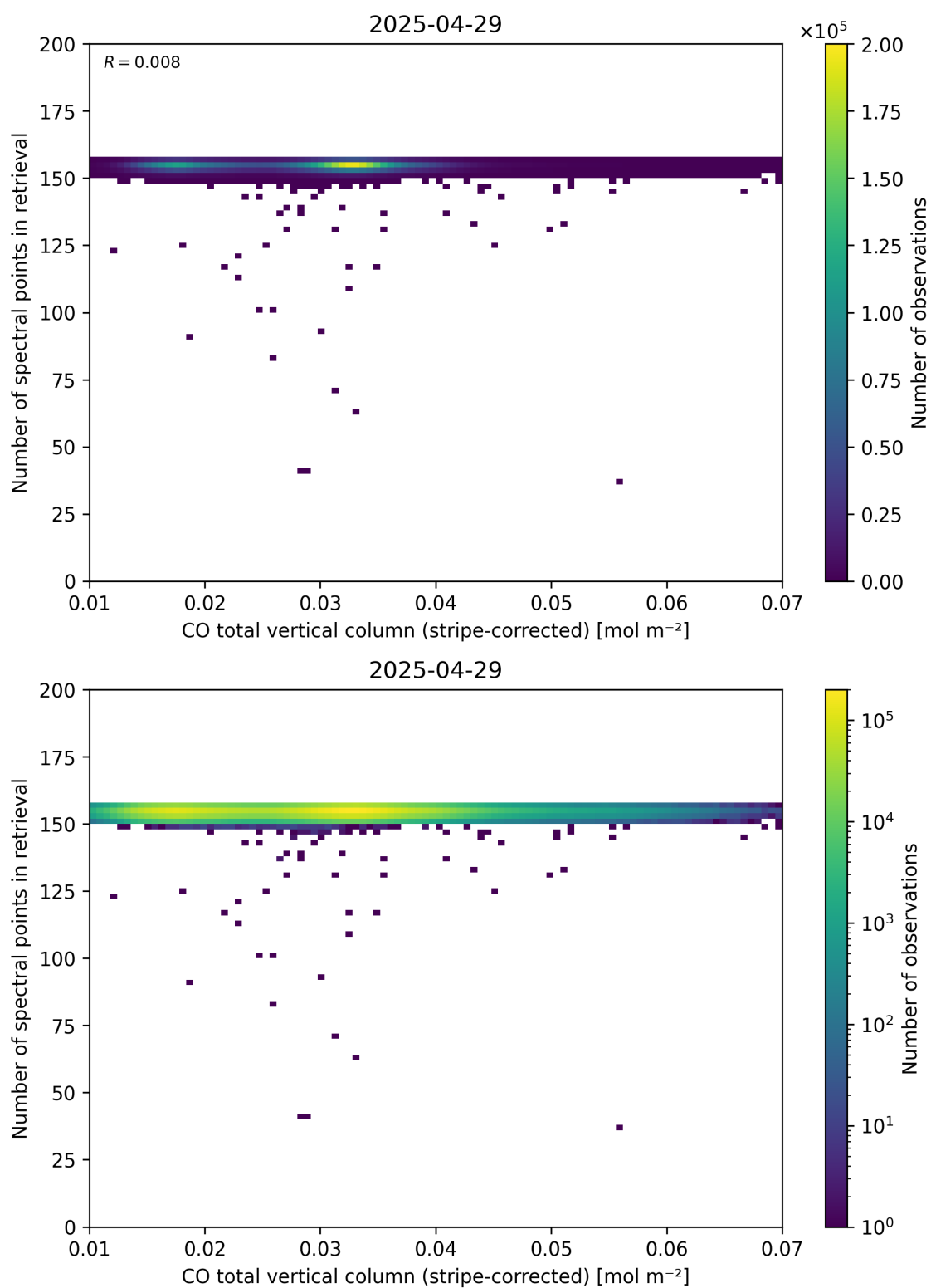
Figure 40: Scatter density plot of “CO total vertical column (stripe-corrected)” against “Number of spectral points in retrieval” for 2025-04-29 to 2025-04-30.
