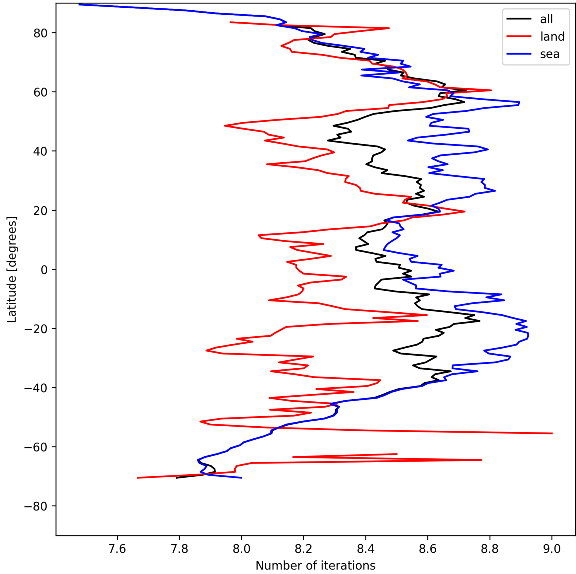
Figure 16: Zonal average of “Number of iterations” for 2025-04-29 to 2025-04-30.
