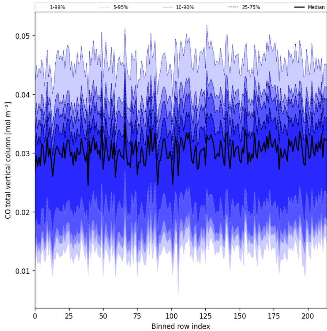
Figure 26: Along track statistics of “CO total vertical column” for 2025-04-29 to 2025-04-30
