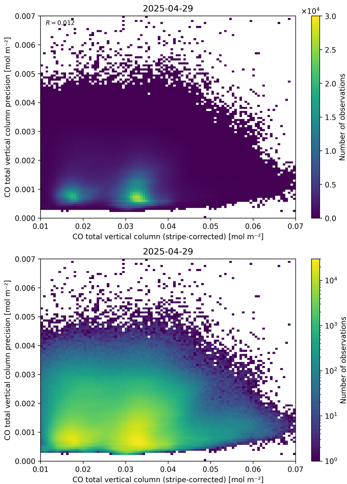
Figure 36: Scatter density plot of “CO total vertical column (stripe-corrected)” against “CO total vertical column precision” for 2025-04-29 to 2025-04-30.
