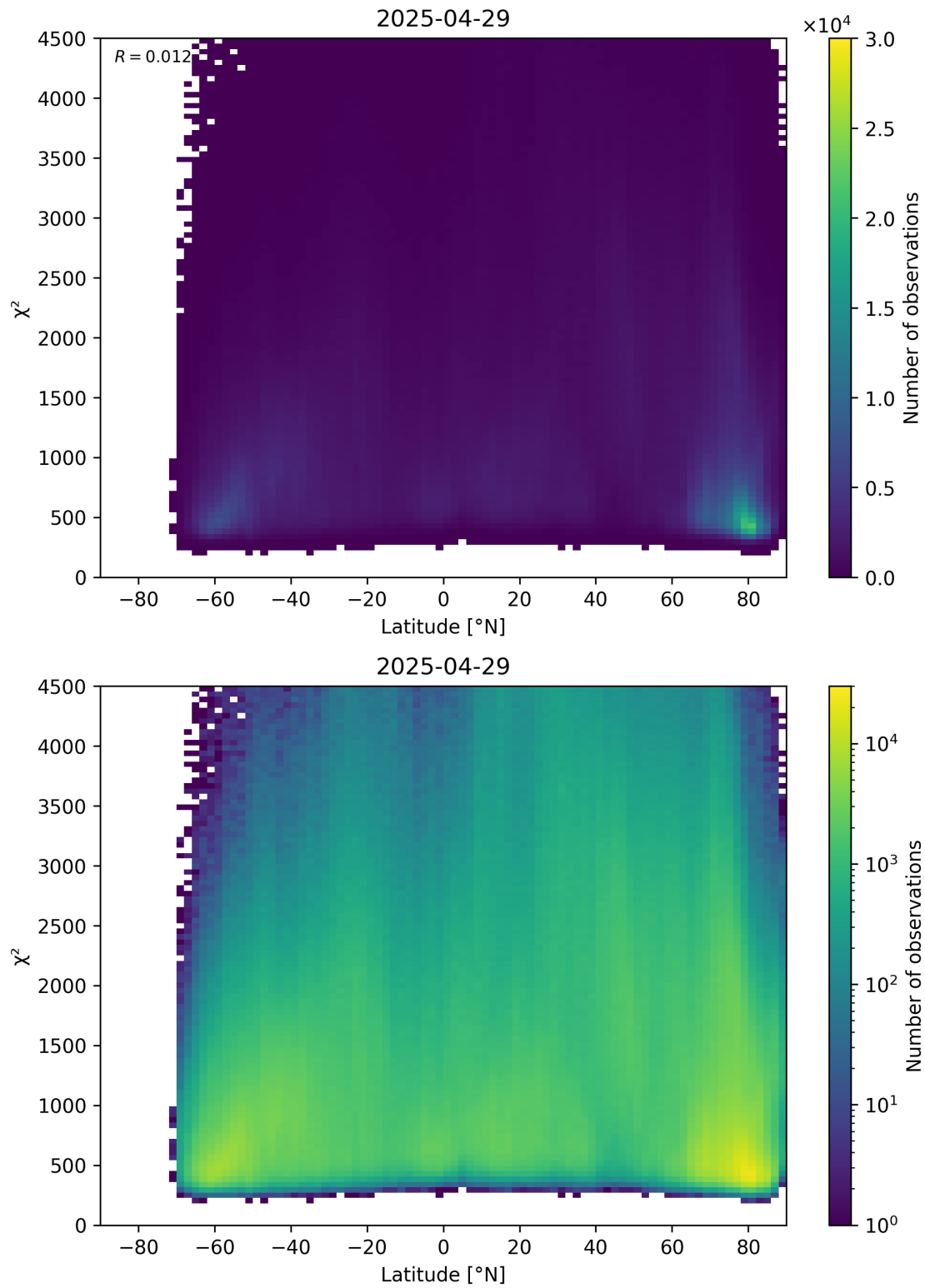
Figure 54: Scatter density plot of “Latitude” against “ \chi^2 ” for 2025-04-29 to 2025-04-30.
