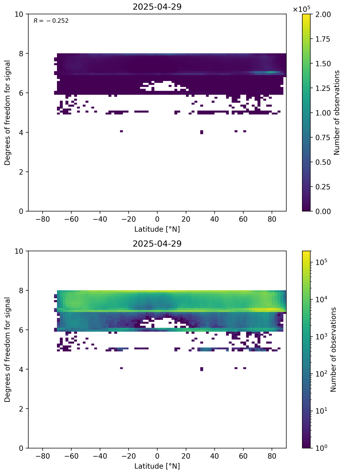
Figure 55: Scatter density plot of “Latitude” against “Degrees of freedom for signal” for 2025-04-29 to 2025-04-30.
