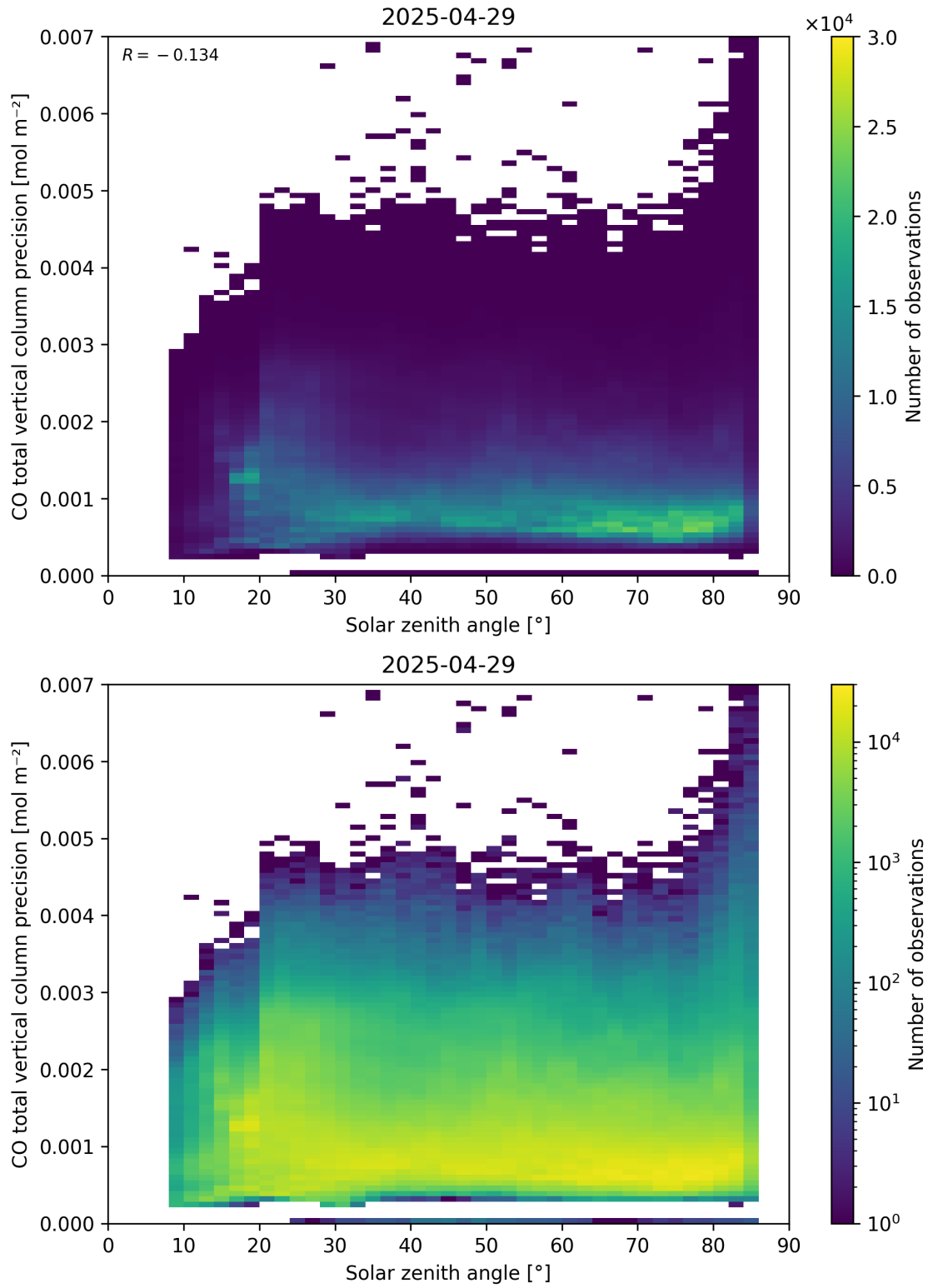
Figure 63: Scatter density plot of “Solar zenith angle” against “CO total vertical column precision” for 2025-04-29 to 2025-04-30.
