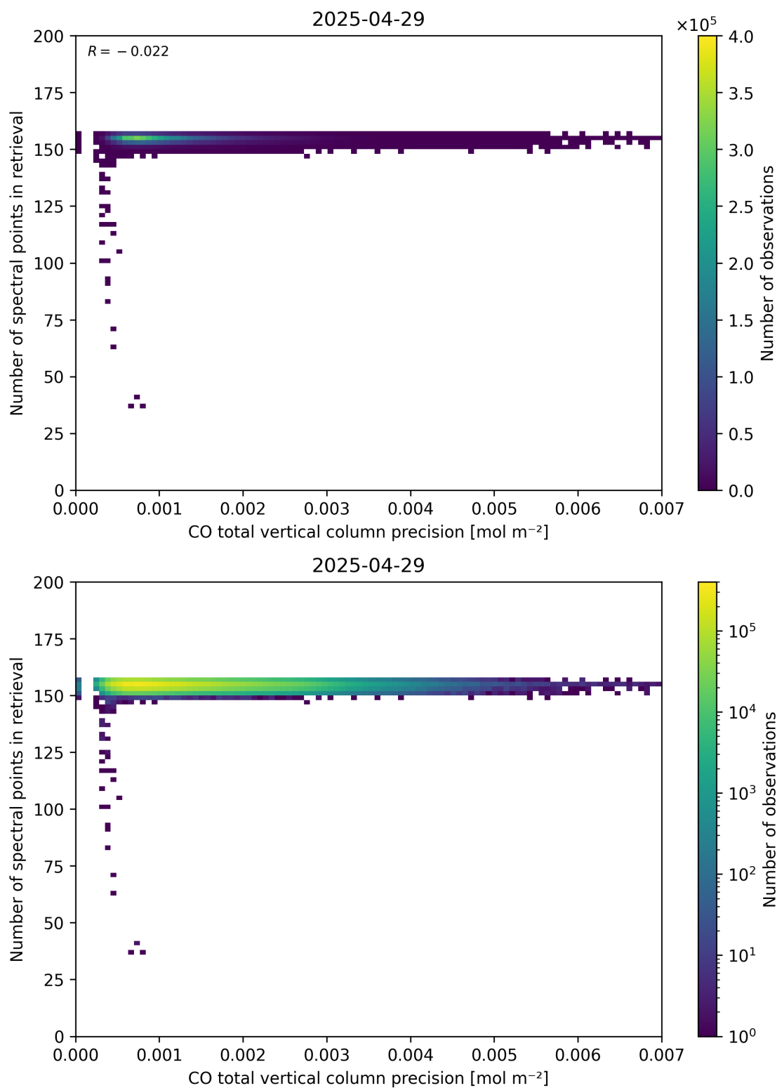
Figure 47: Scatter density plot of “CO total vertical column precision” against “Number of spectral points in retrieval” for 2025-04-29 to 2025-04-30.
