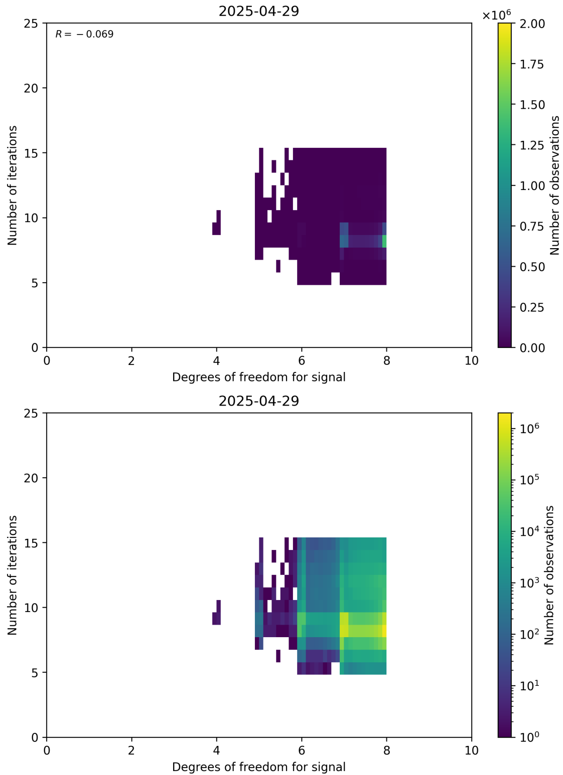
Figure 50: Scatter density plot of “Degrees of freedom for signal” against “Number of iterations” for 2025-04-29 to 2025-04-30.
