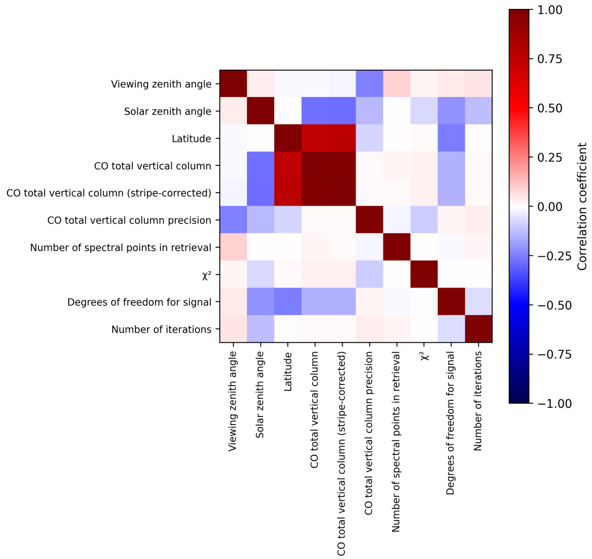
Figure 2: Map of correlation matrix for 2025-04-29 to 2025-04-30.
