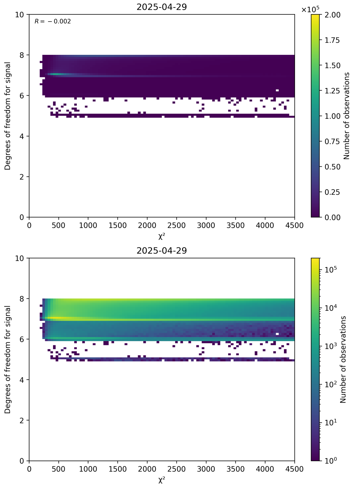
Figure 48: Scatter density plot of “ \chi^2 ” against “Degrees of freedom for signal” for 2025-04-29 to 2025-04-30.
