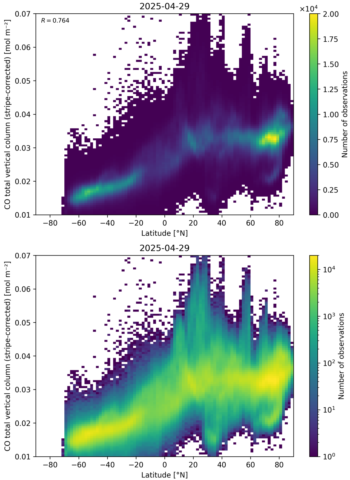
Figure 52: Scatter density plot of “Latitude” against “CO total vertical column (stripe-corrected)” for 2025-04-29 to 2025-04-30.
