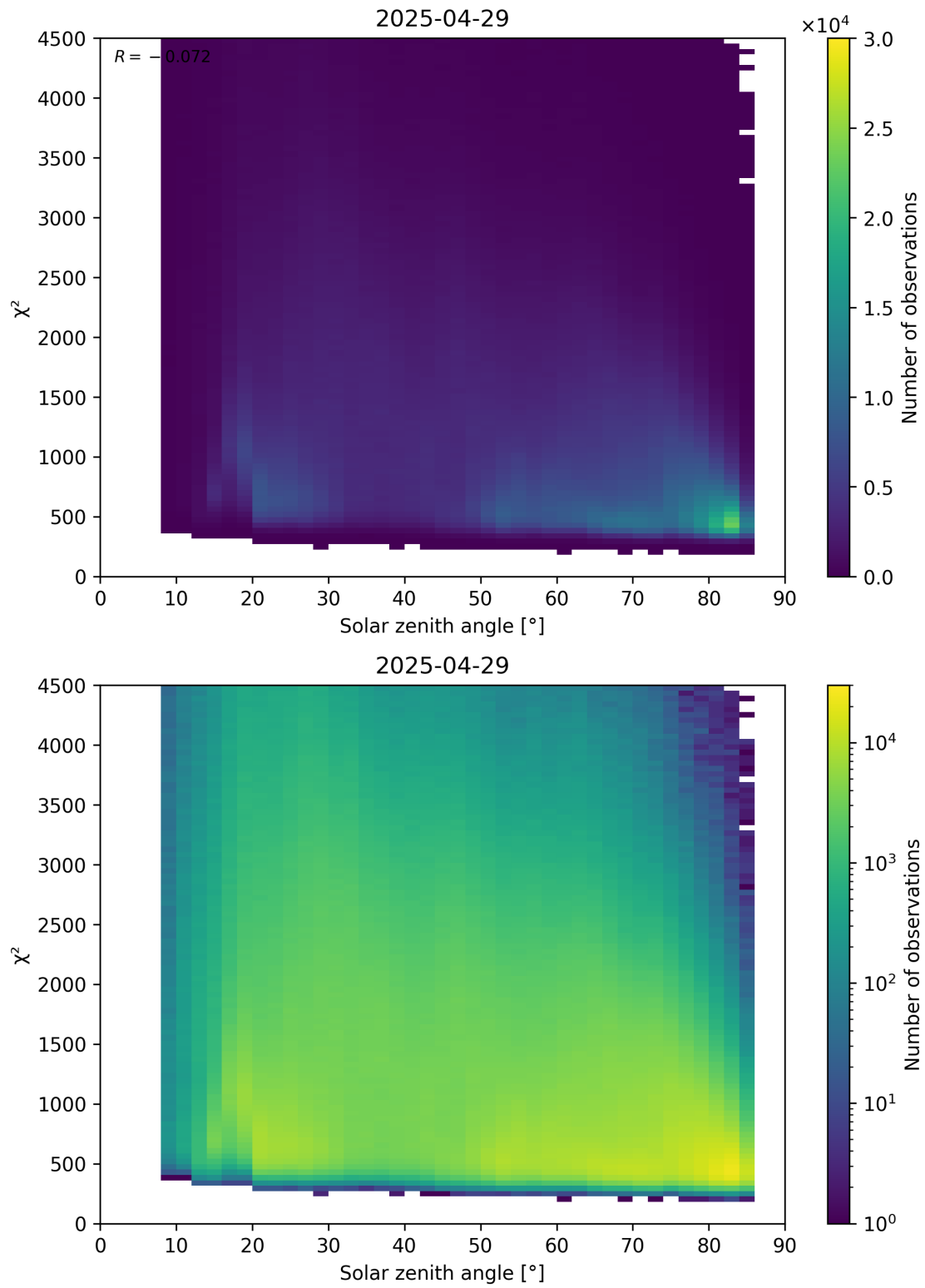
Figure 64: Scatter density plot of “Solar zenith angle” against “ \chi^2 ” for 2025-04-29 to 2025-04-30.
