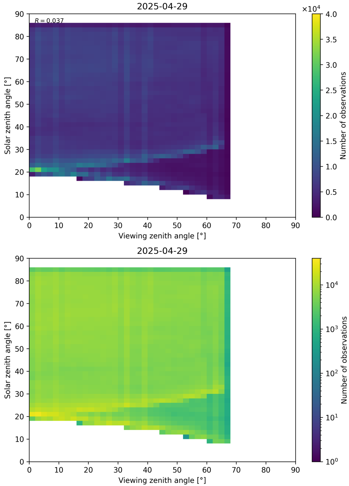
Figure 77: Scatter density plot of “Viewing zenith angle” against “Solar zenith angle” for 2025-04-29 to 2025-04-30.
