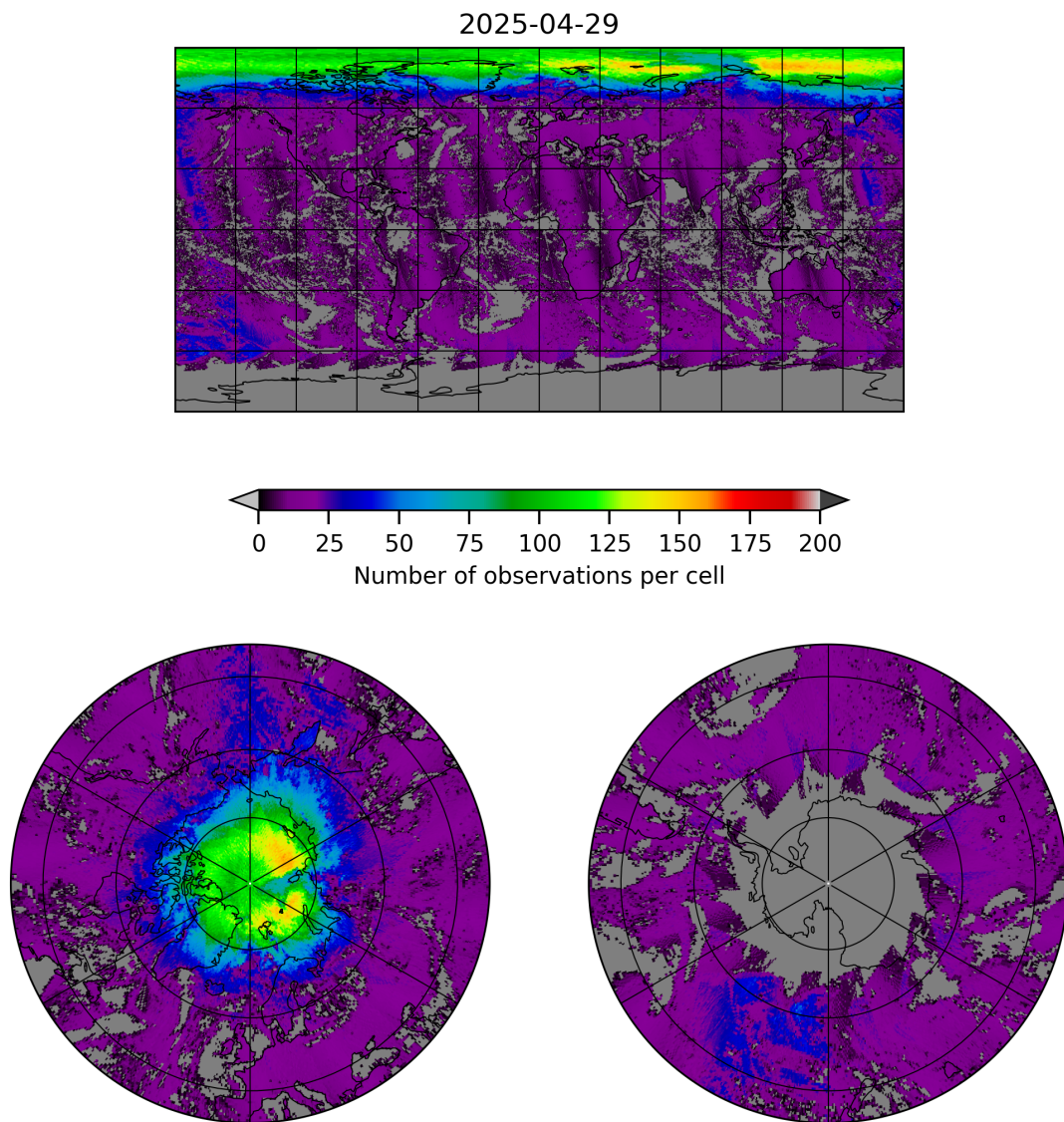
Figure 8: Map of the number of observations for 2025-04-29 to 2025-04-30
