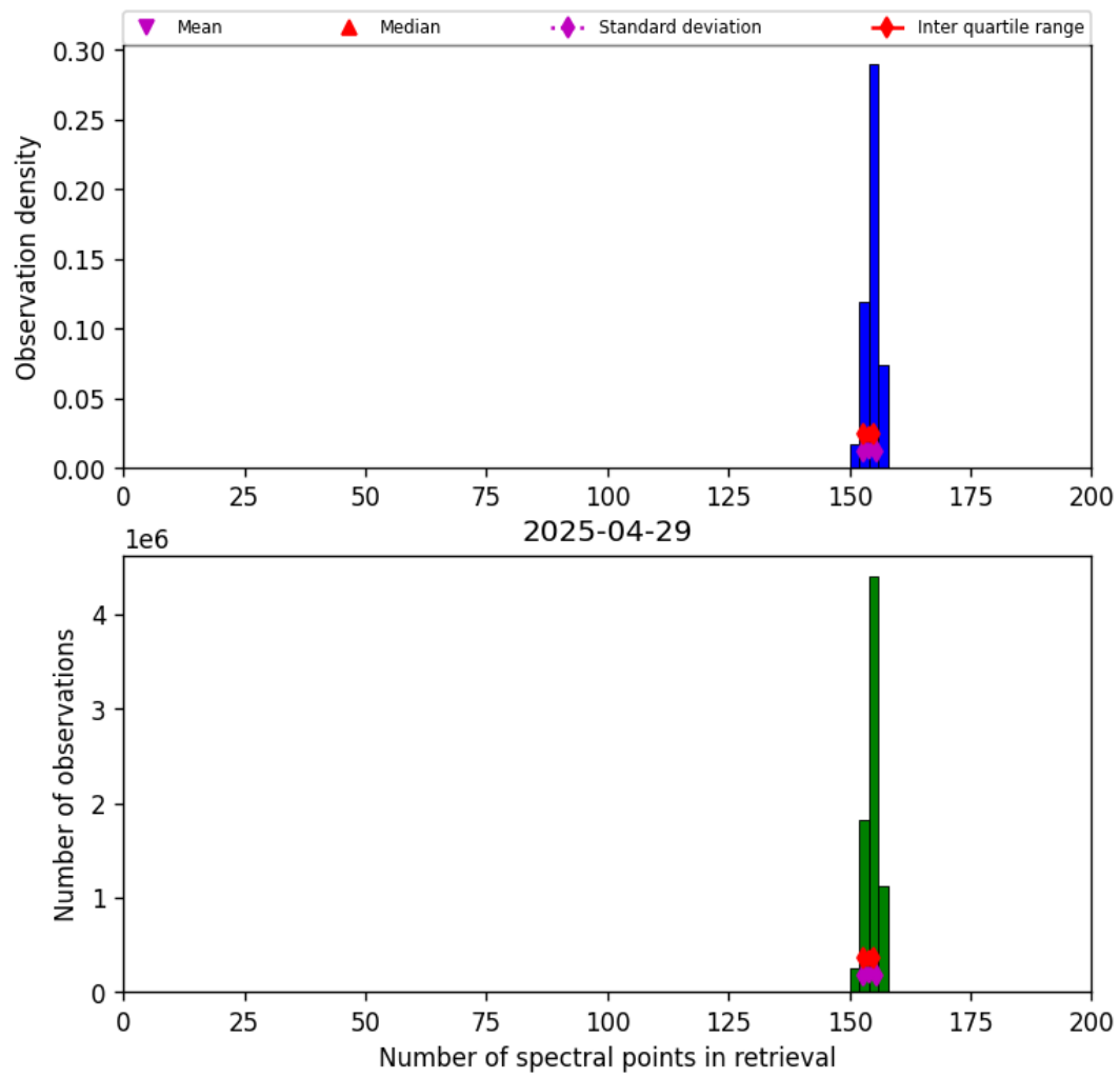
Figure 21: Histogram of “Number of spectral points in retrieval” for 2025-04-29 to 2025-04-30
