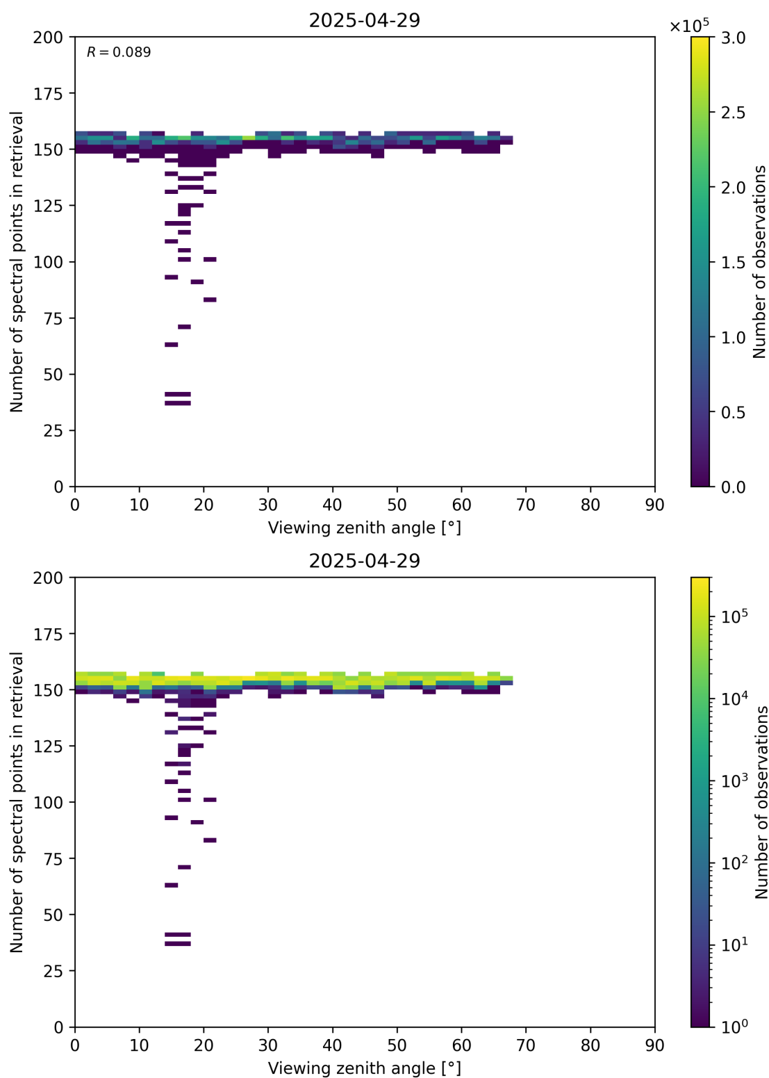
Figure 76: Scatter density plot of “Viewing zenith angle” against “Number of spectral points in retrieval” for 2025-04-29 to 2025-04-30.
