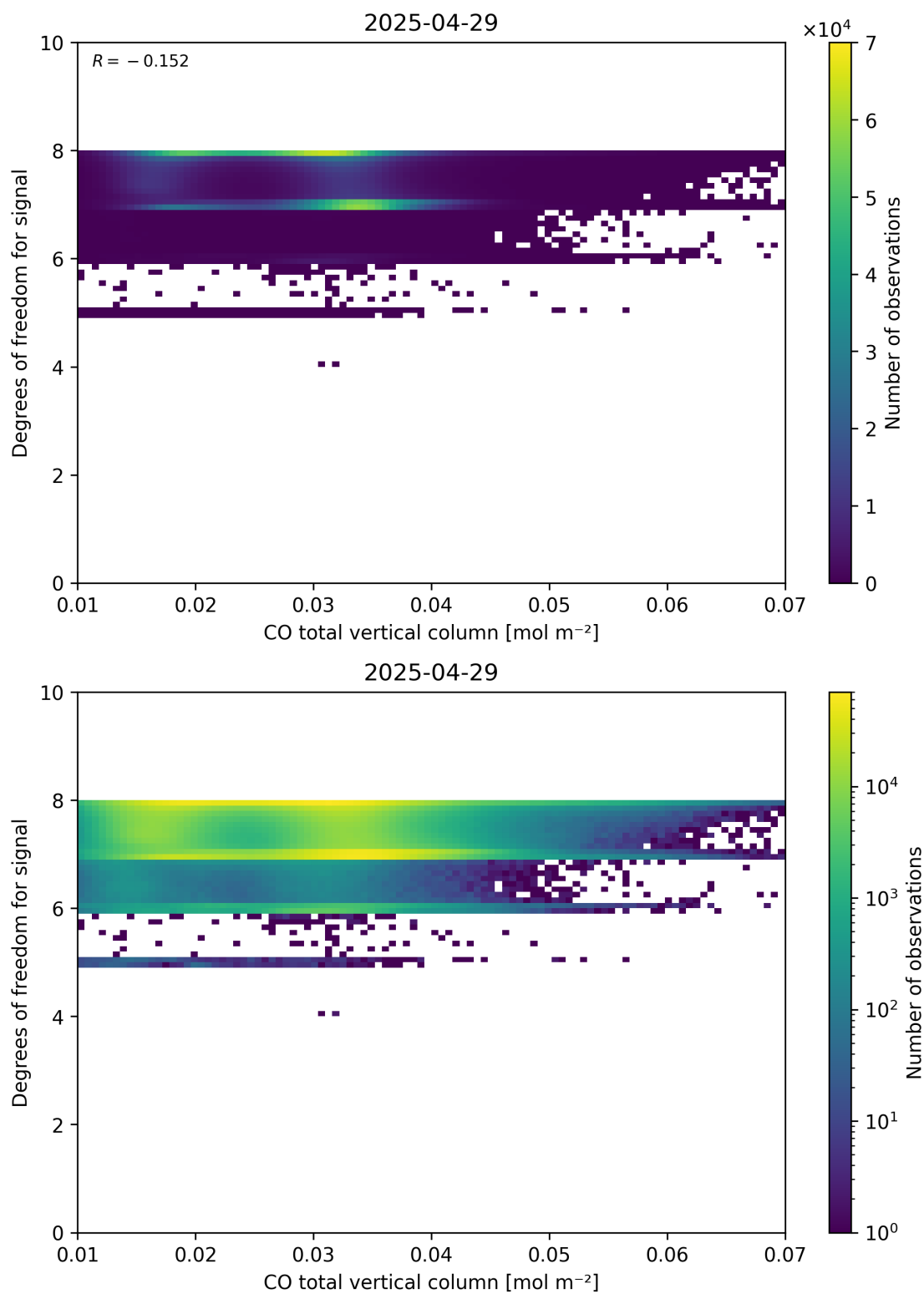
Figure 41: Scatter density plot of “CO total vertical column” against “Degrees of freedom for signal” for 2025-04-29 to 2025-04-30.
