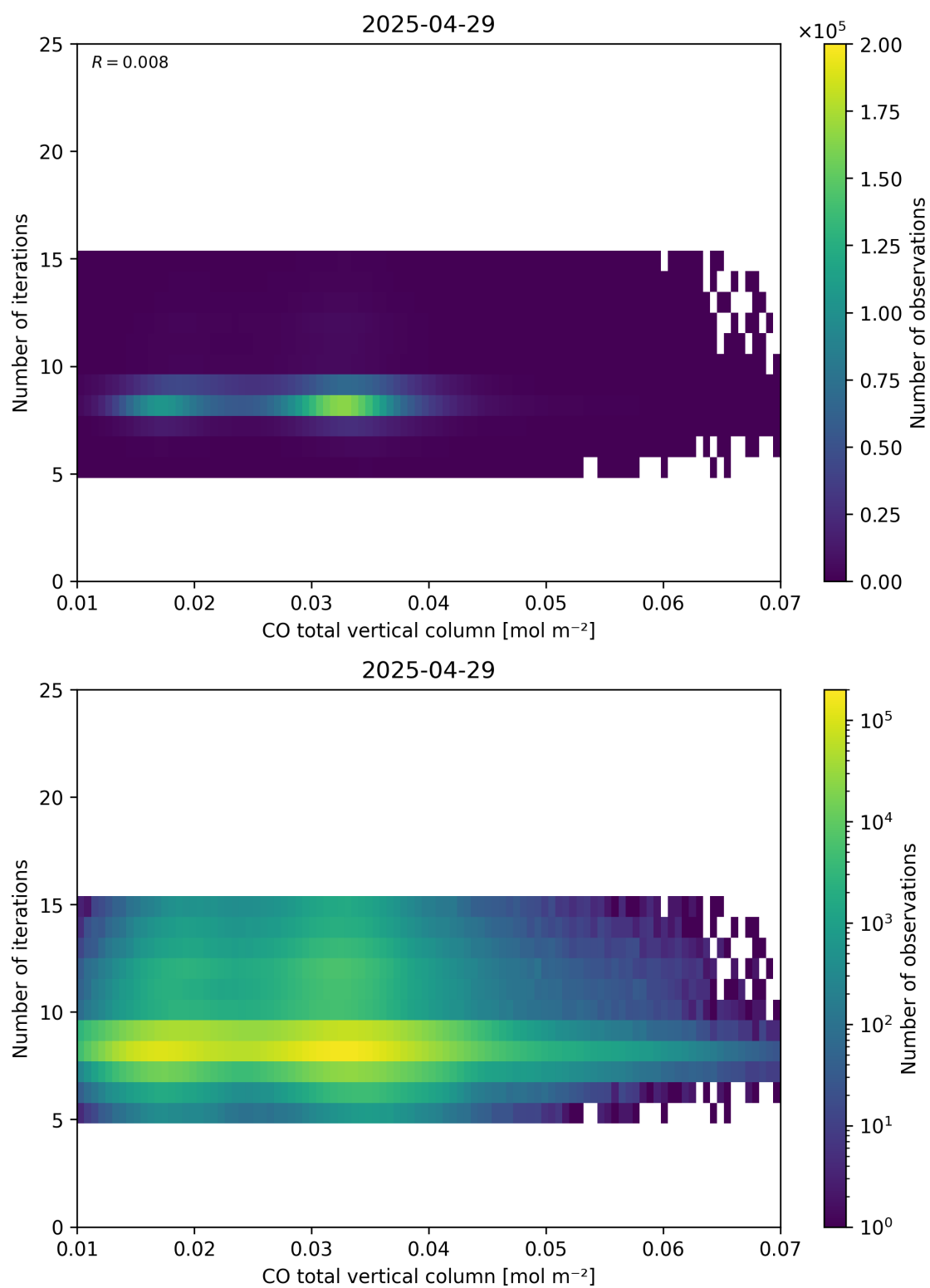
Figure 42: Scatter density plot of “CO total vertical column” against “Number of iterations” for 2025-04-29 to 2025-04-30.
