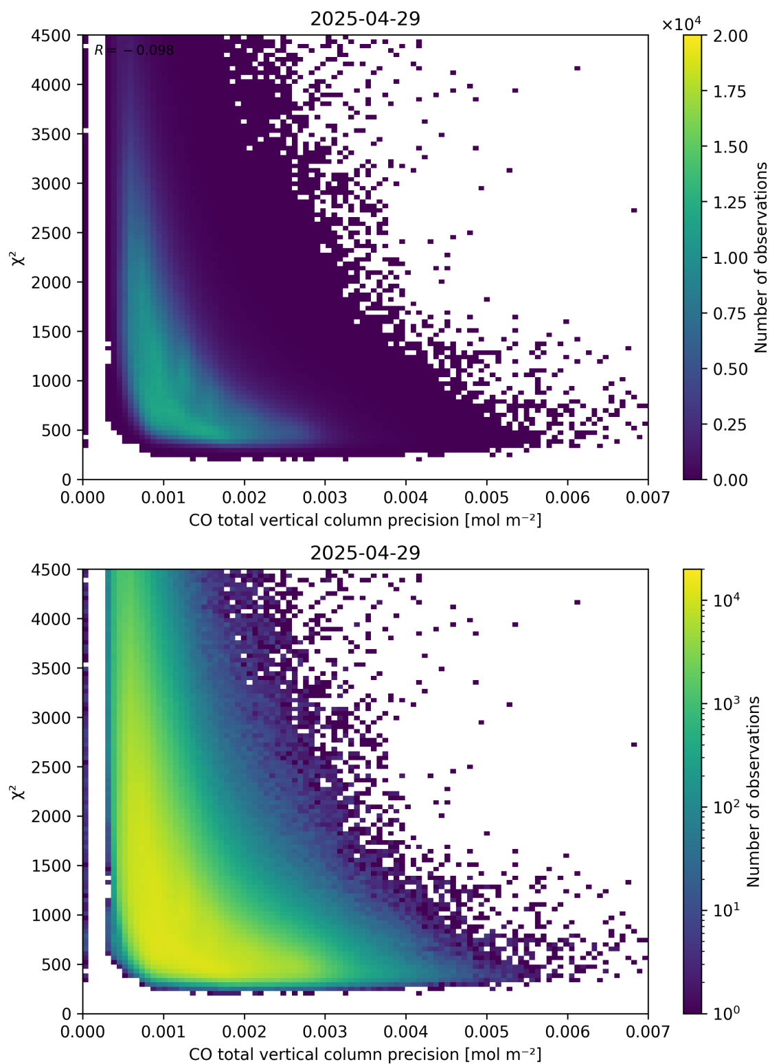
Figure 44: Scatter density plot of “CO total vertical column precision” against “ \chi^2 ” for 2025-04-29 to 2025-04-30.
