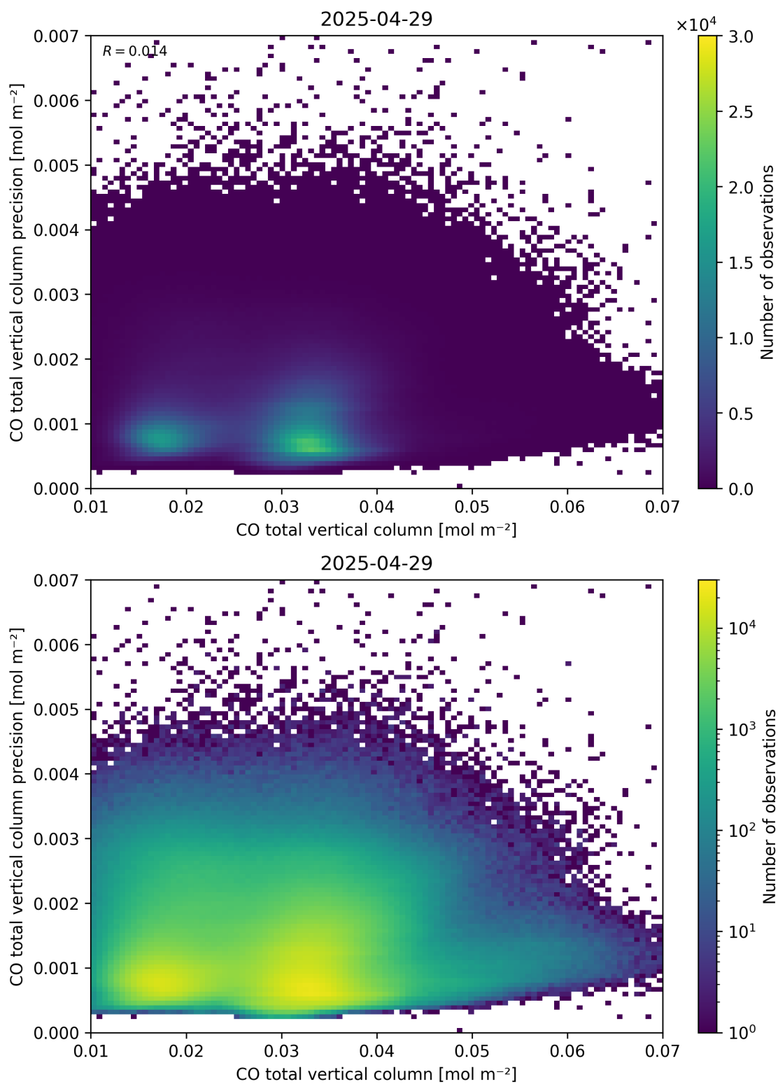
Figure 34: Scatter density plot of “CO total vertical column” against “CO total vertical column precision” for 2025-04-29 to 2025-04-30.
