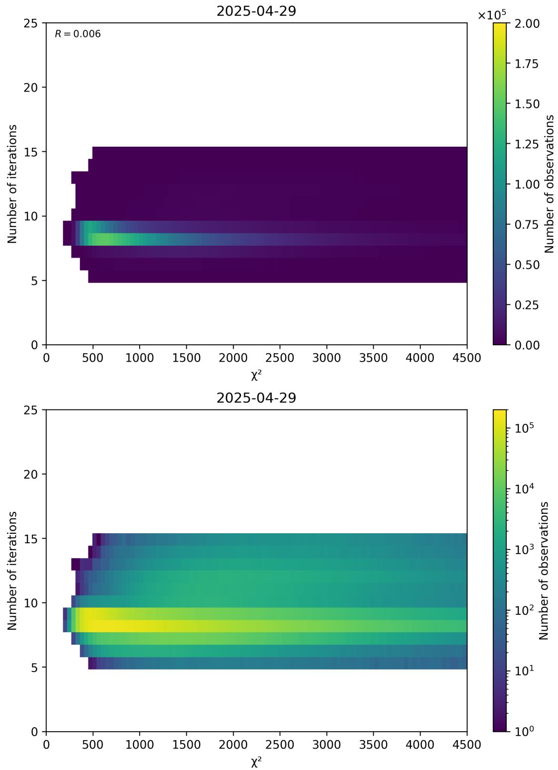
Figure 49: Scatter density plot of “ \chi^2 ” against “Number of iterations” for 2025-04-29 to 2025-04-30.
