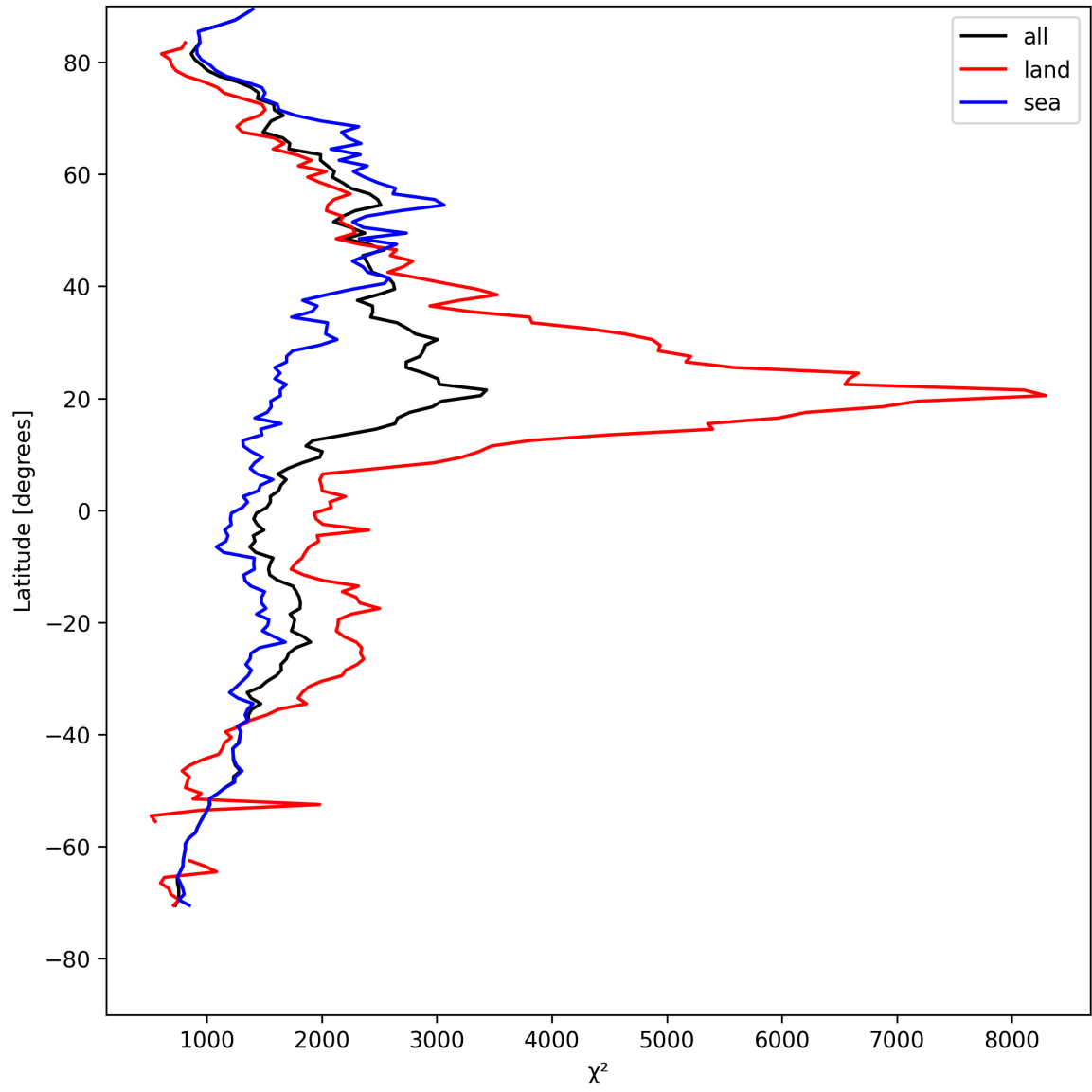
Figure 14: Zonal average of “ \chi^2 ” for 2025-04-29 to 2025-04-30.
