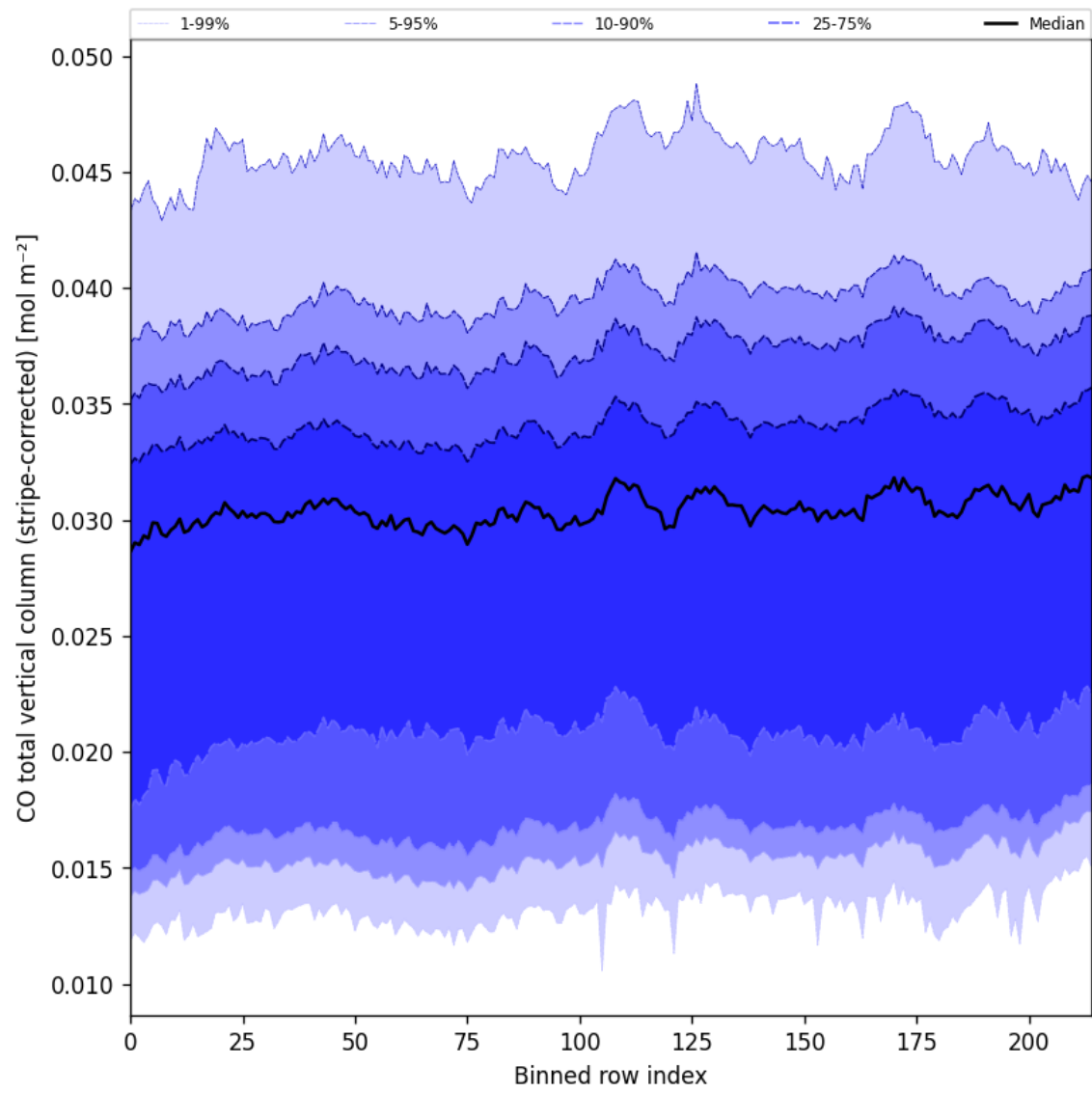
Figure 27: Along track statistics of “CO total vertical column (stripe-corrected)” for 2025-04-29 to 2025-04-30
