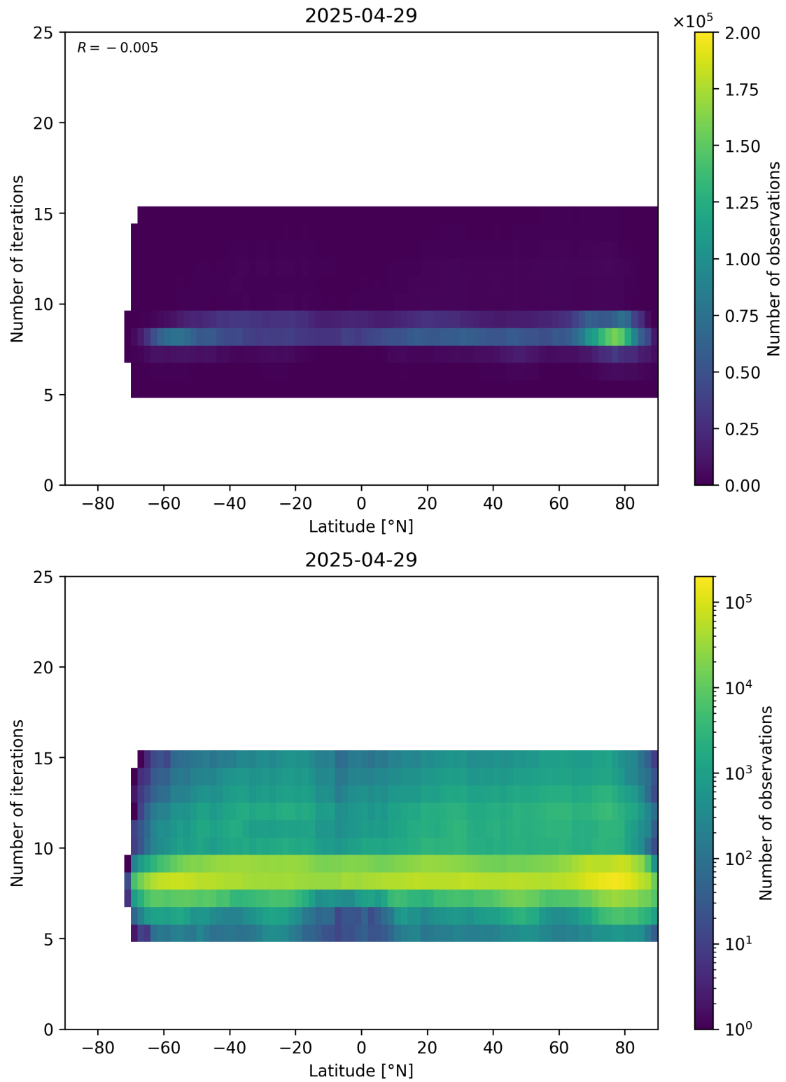
Figure 56: Scatter density plot of “Latitude” against “Number of iterations” for 2025-04-29 to 2025-04-30.
