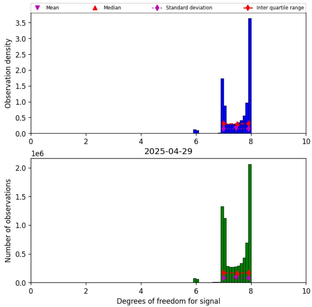
Figure 23: Histogram of “Degrees of freedom for signal” for 2025-04-29 to 2025-04-30
