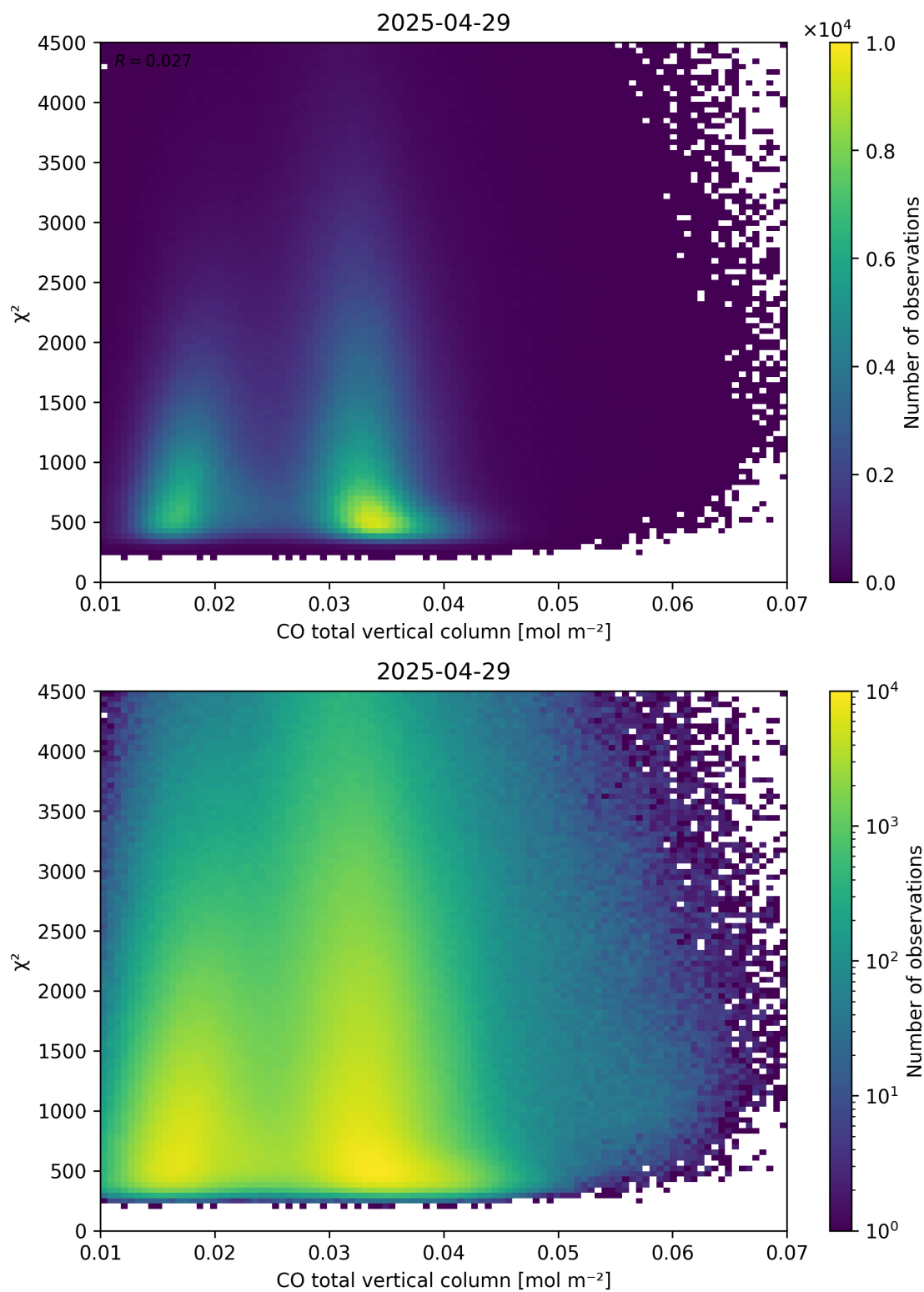
Figure 35: Scatter density plot of “CO total vertical column” against “ \chi^2 ” for 2025-04-29 to 2025-04-30.
