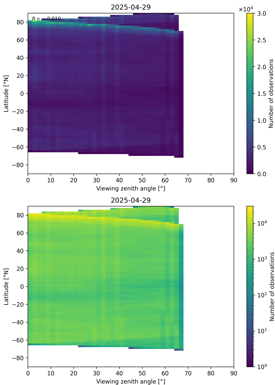
Figure 74: Scatter density plot of “Viewing zenith angle” against “Latitude” for 2025-04-29 to 2025-04-30.
