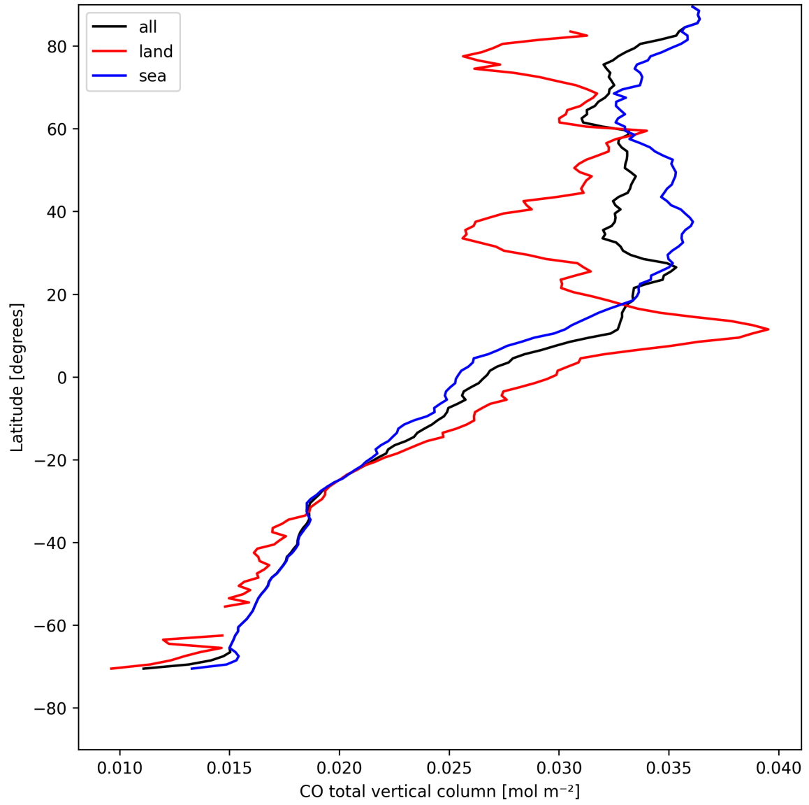
Figure 10: Zonal average of “CO total vertical column” for 2025-04-29 to 2025-04-30.
