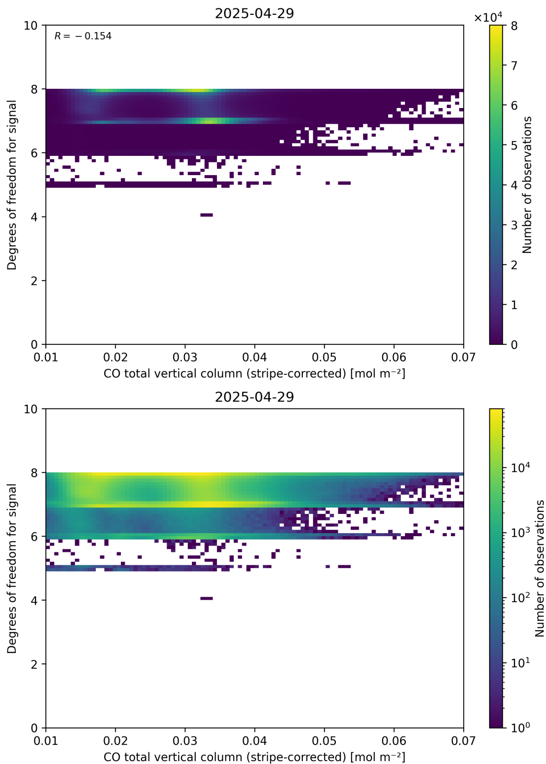
Figure 38: Scatter density plot of “CO total vertical column (stripe-corrected)” against “Degrees of freedom for signal” for 2025-04-29 to 2025-04-30.
