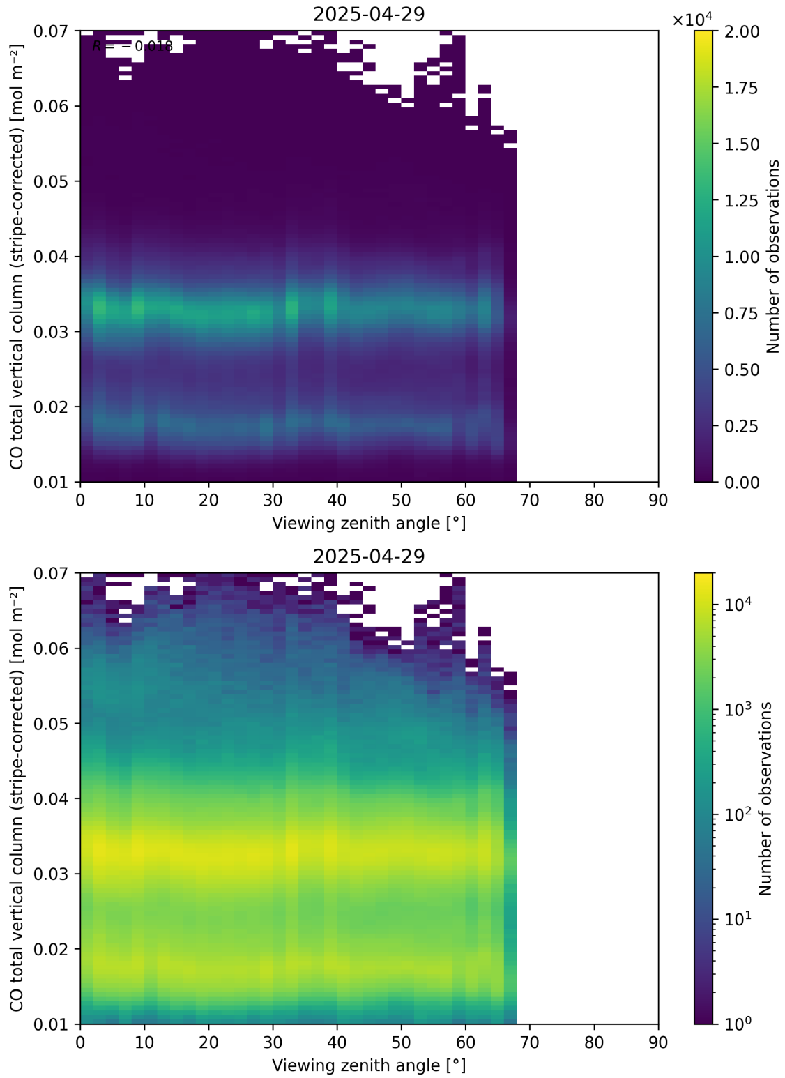
Figure 70: Scatter density plot of “Viewing zenith angle” against “CO total vertical column (stripe-corrected)” for 2025-04-29 to 2025-04-30.
