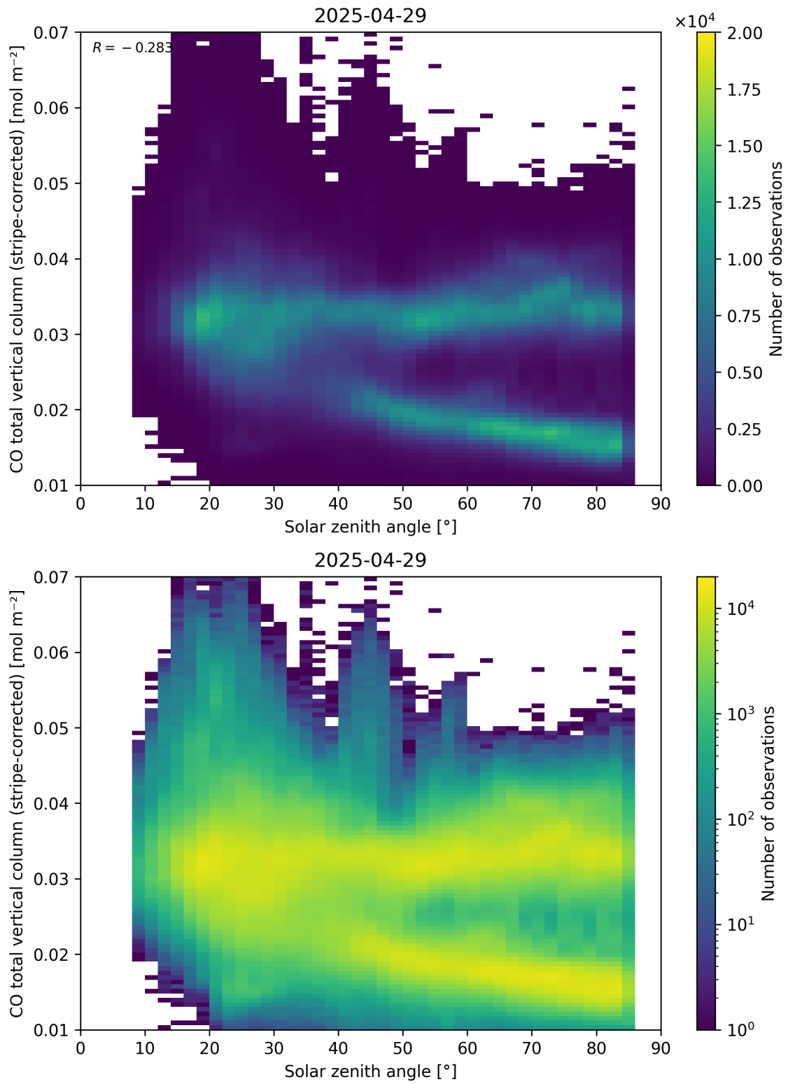
Figure 62: Scatter density plot of “Solar zenith angle” against “CO total vertical column (stripe-corrected)” for 2025-04-29 to 2025-04-30.
