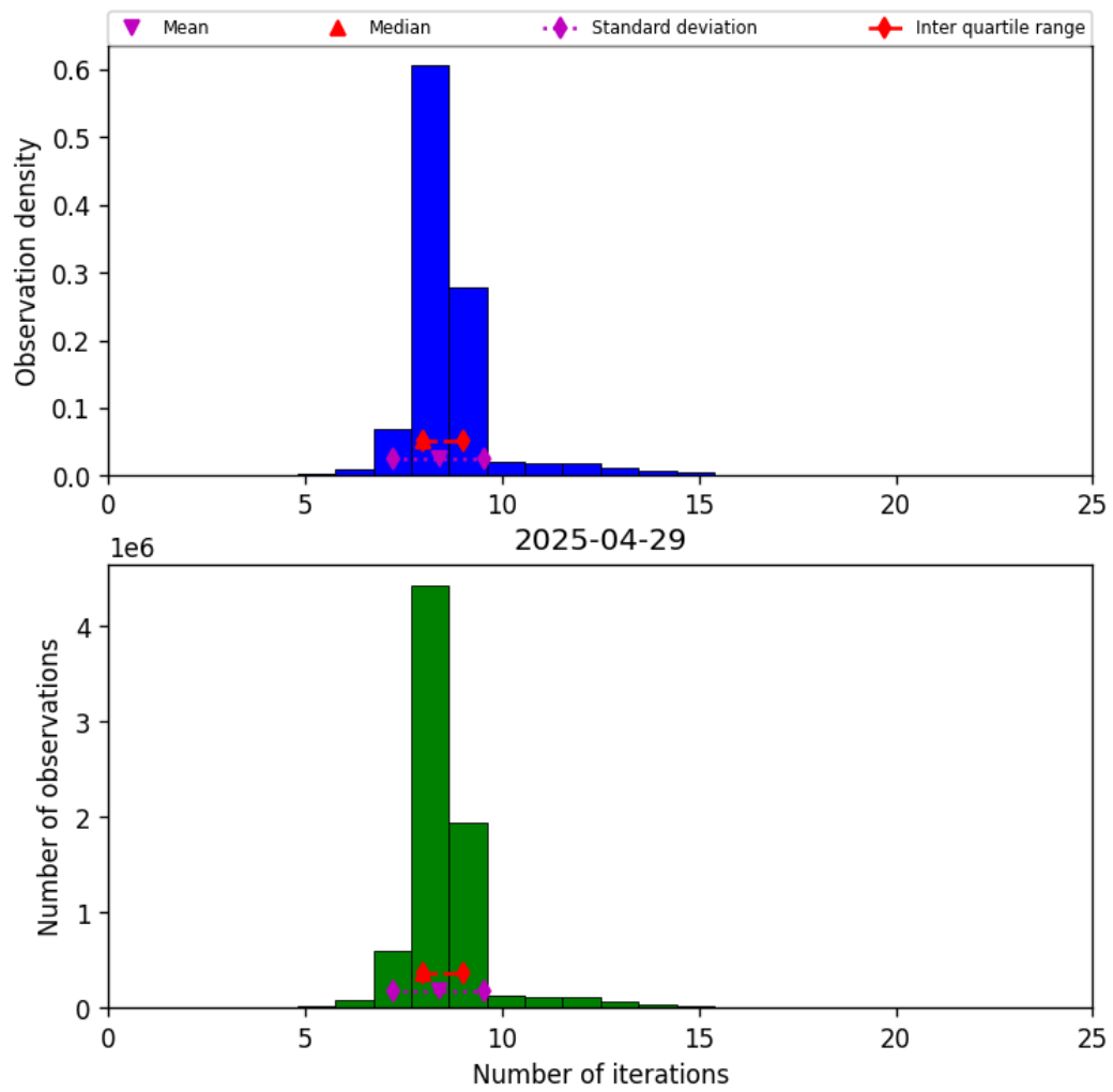
Figure 24: Histogram of “Number of iterations” for 2025-04-29 to 2025-04-30
