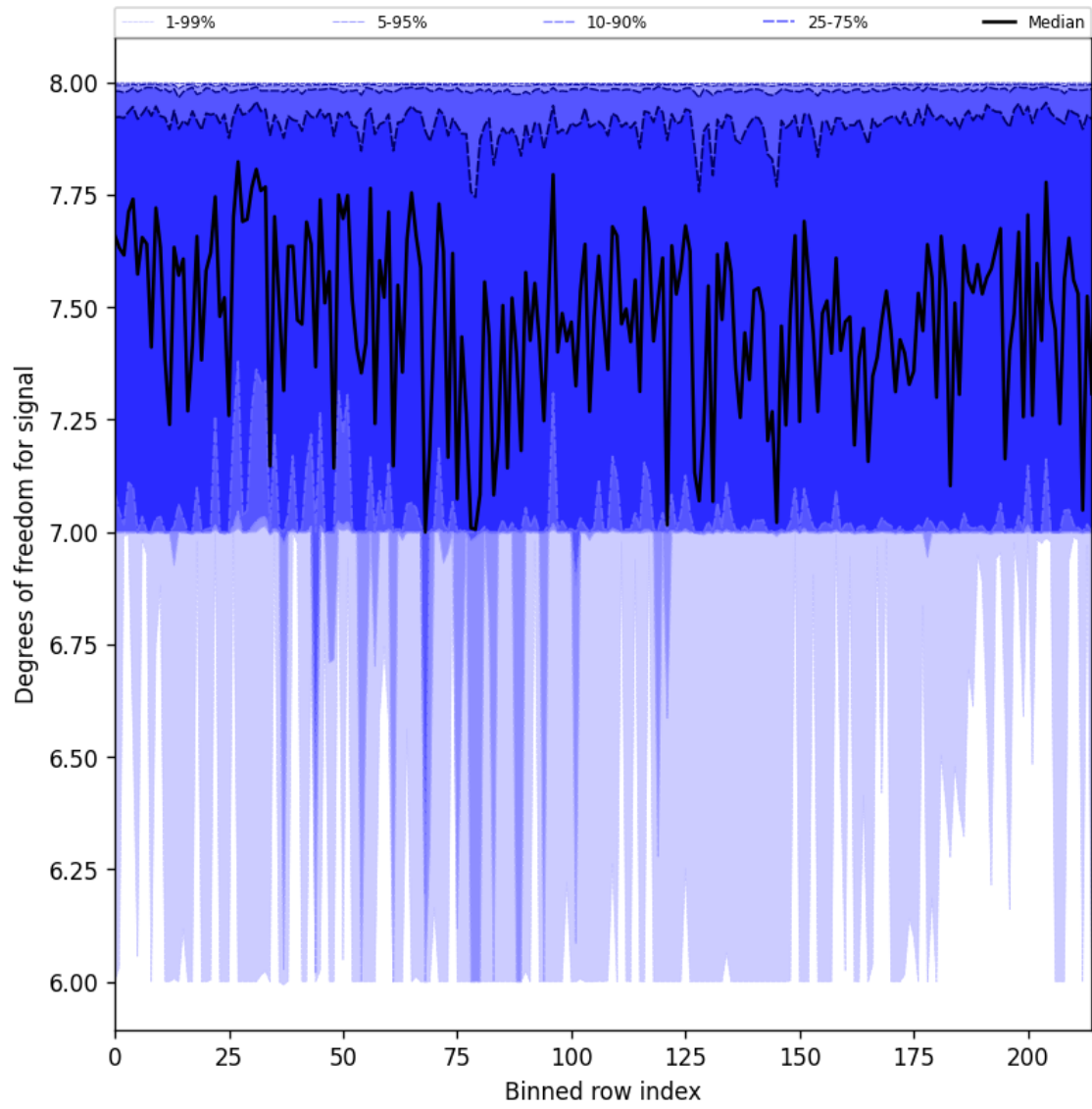
Figure 31: Along track statistics of “Degrees of freedom for signal” for 2025-04-29 to 2025-04-30
