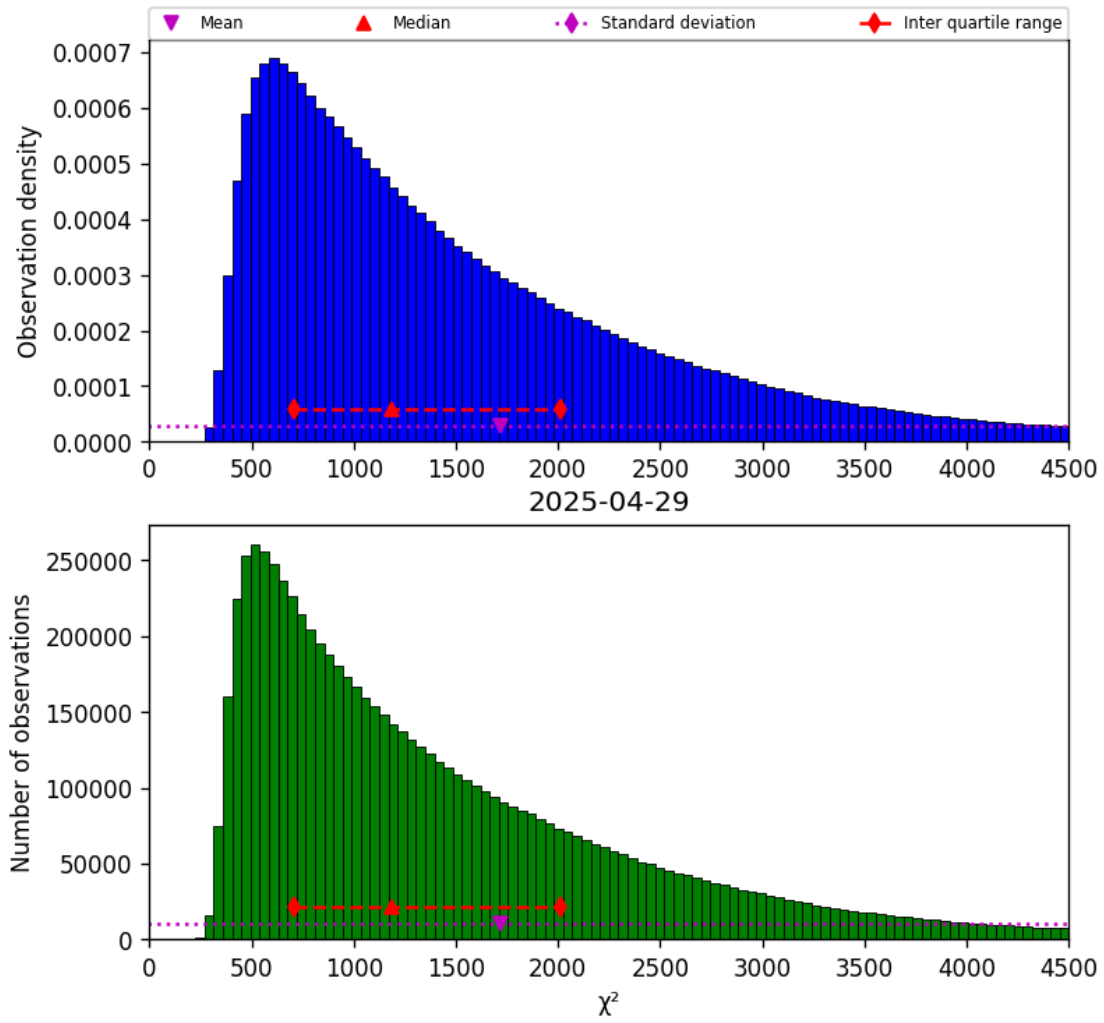
Figure 22: Histogram of “ \chi^2 ” for 2025-04-29 to 2025-04-30
