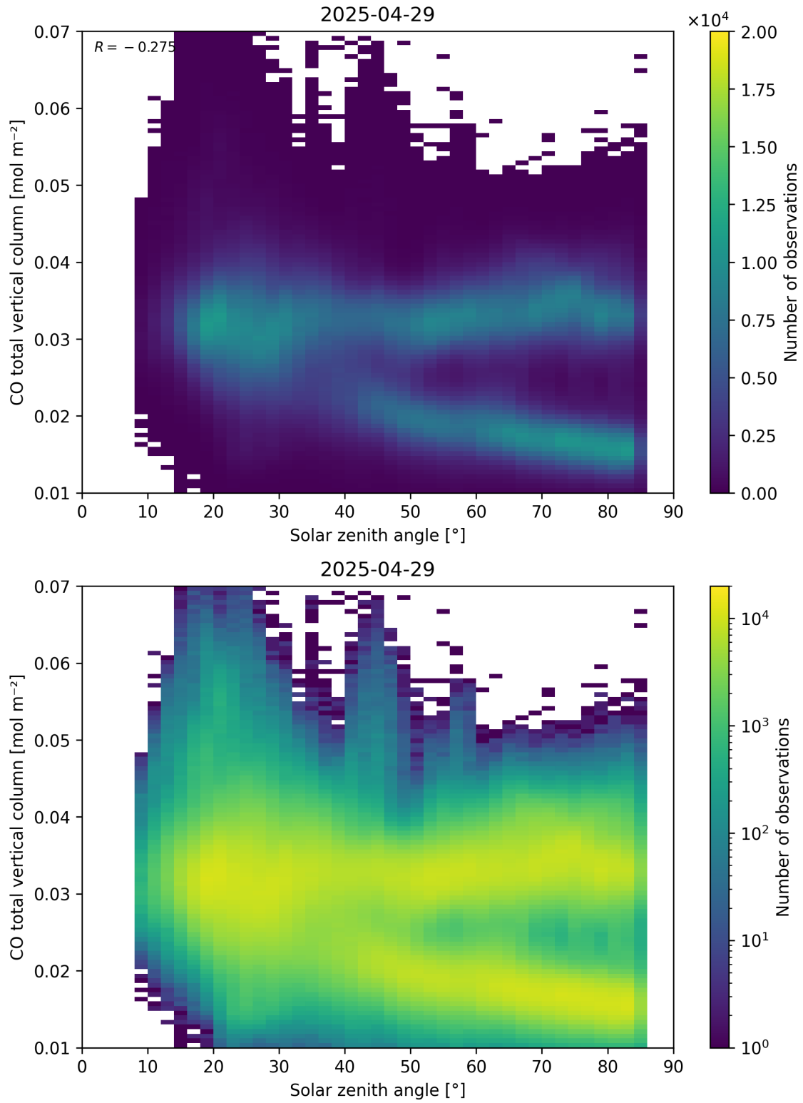
Figure 61: Scatter density plot of “Solar zenith angle” against “CO total vertical column” for 2025-04-29 to 2025-04-30.
