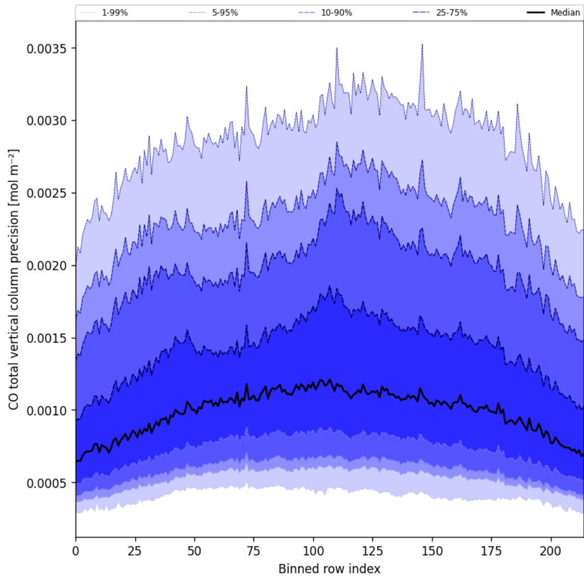
Figure 28: Along track statistics of “CO total vertical column precision” for 2025-04-29 to 2025-04-30
