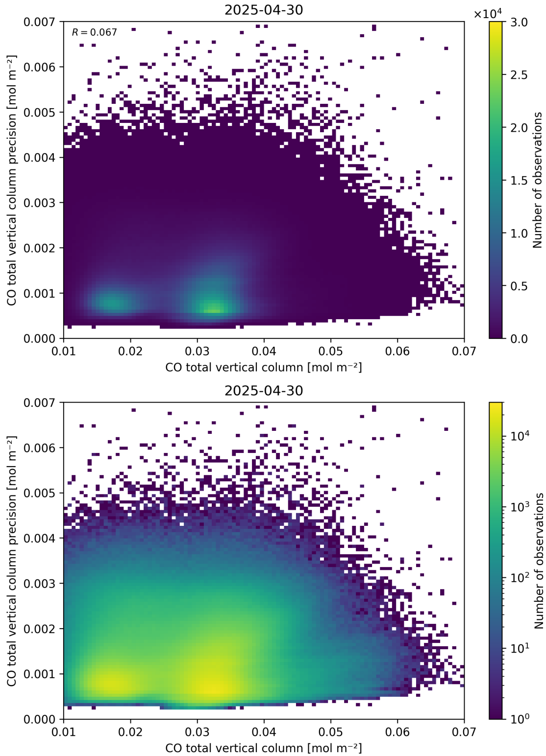
Figure 34: Scatter density plot of “CO total vertical column” against “CO total vertical column precision” for 2025-04-29 to 2025-05-01.
