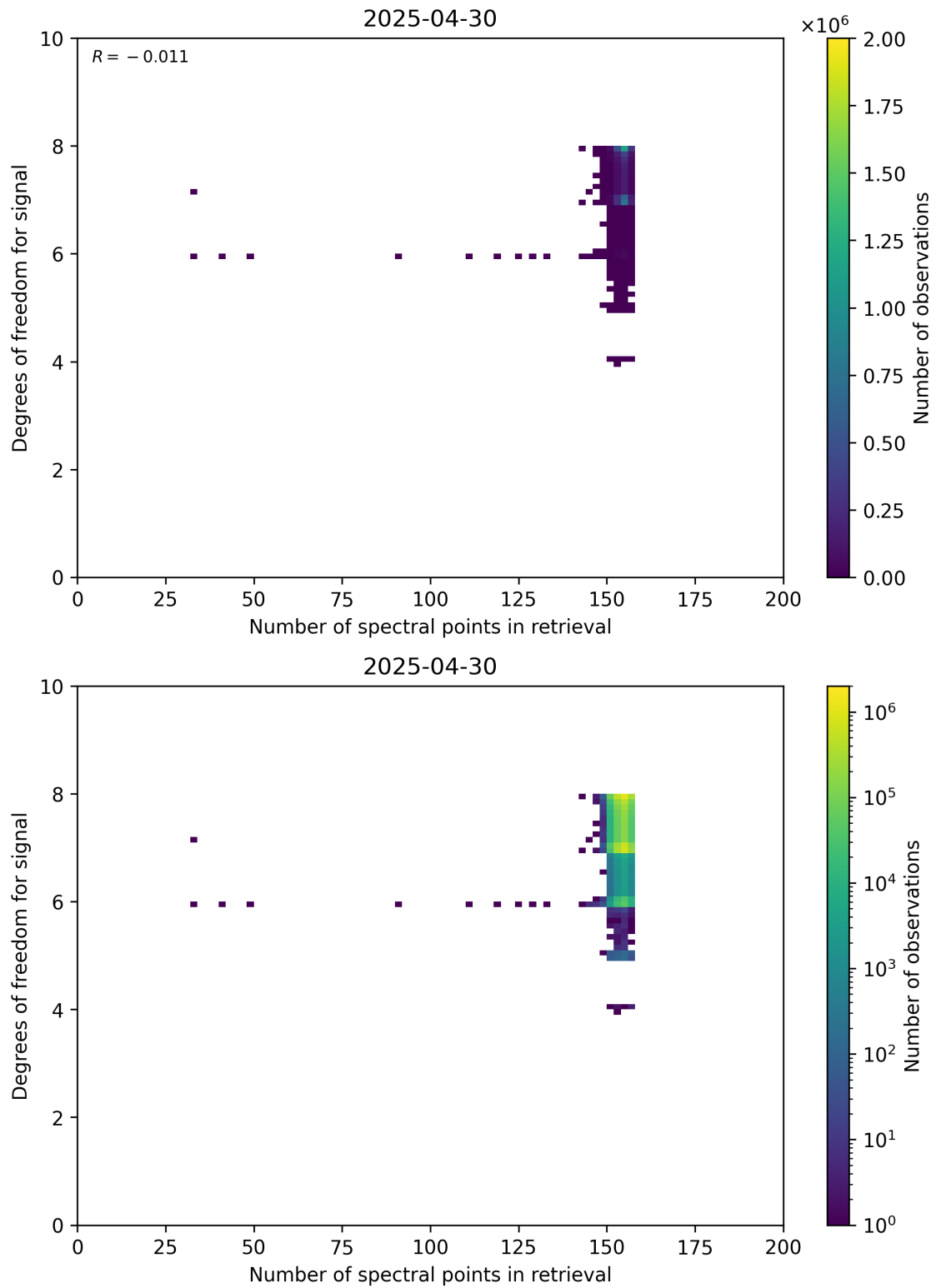
Figure 59: Scatter density plot of “Number of spectral points in retrieval” against “Degrees of freedom for signal” for 2025-04-29 to 2025-05-01.
