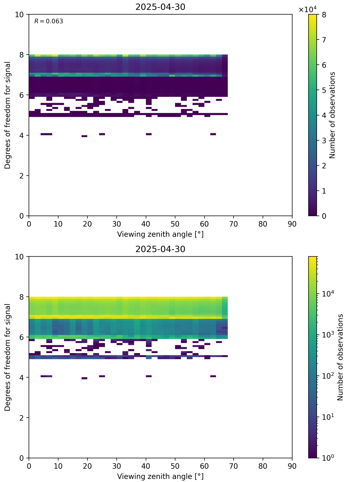
Figure 73: Scatter density plot of “Viewing zenith angle” against “Degrees of freedom for signal” for 2025-04-29 to 2025-05-01.
