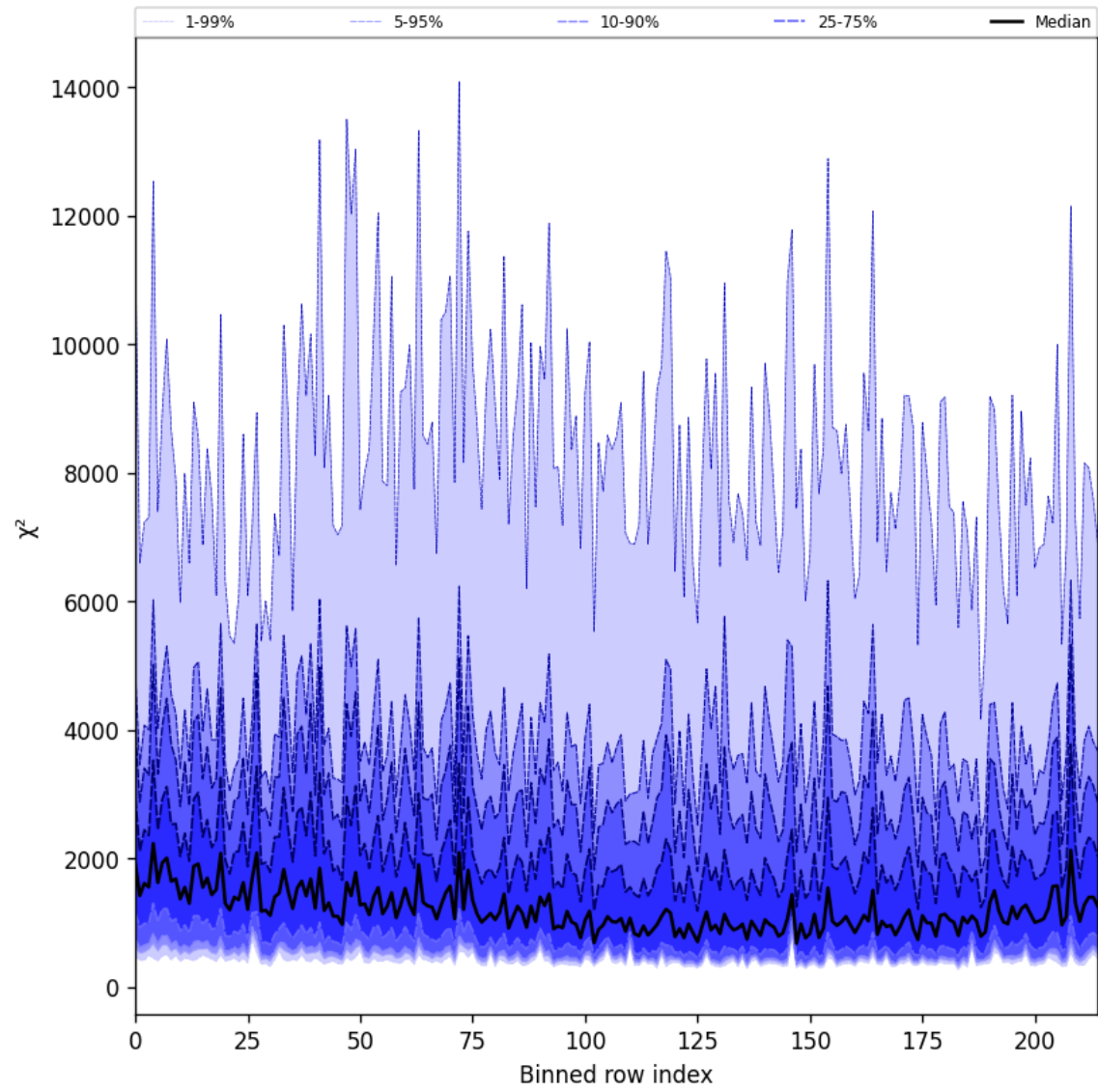
Figure 30: Along track statistics of “ \chi^2 ” for 2025-04-29 to 2025-05-01
