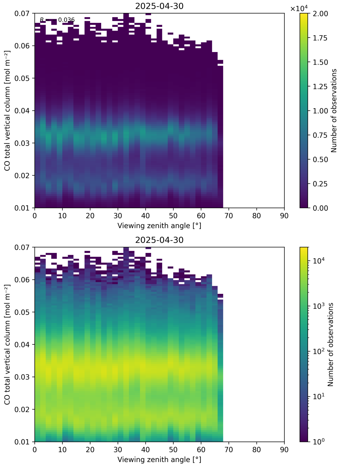
Figure 69: Scatter density plot of “Viewing zenith angle” against “CO total vertical column” for 2025-04-29 to 2025-05-01.
