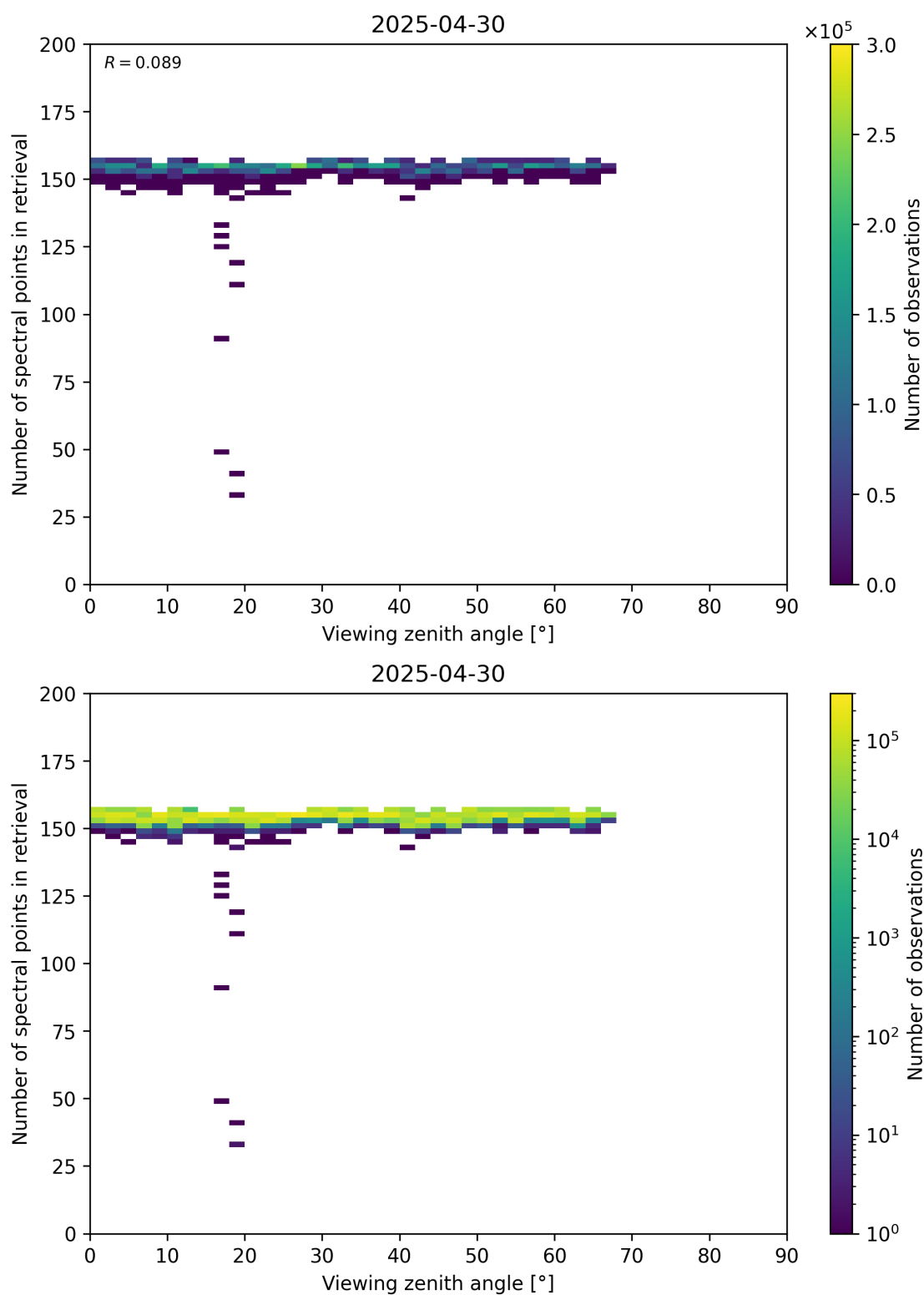
Figure 76: Scatter density plot of “Viewing zenith angle” against “Number of spectral points in retrieval” for 2025-04-29 to 2025-05-01.
