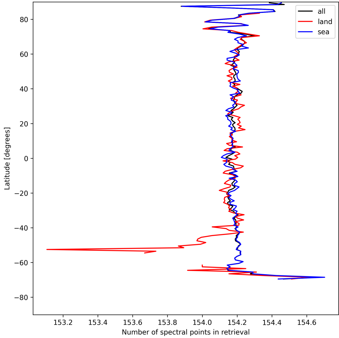
Figure 13: Zonal average of “Number of spectral points in retrieval” for 2025-04-29 to 2025-05-01.
