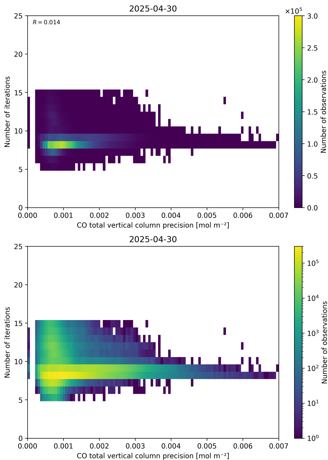
Figure 46: Scatter density plot of “CO total vertical column precision” against “Number of iterations” for 2025-04-29 to 2025-05-01.
