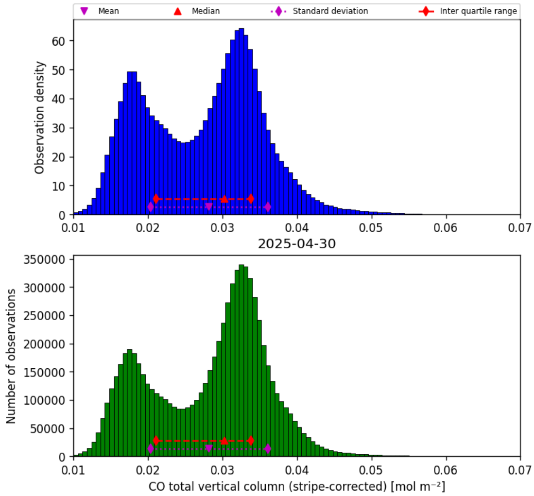
Figure 19: Histogram of “CO total vertical column (stripe-corrected)” for 2025-04-29 to 2025-05-01
