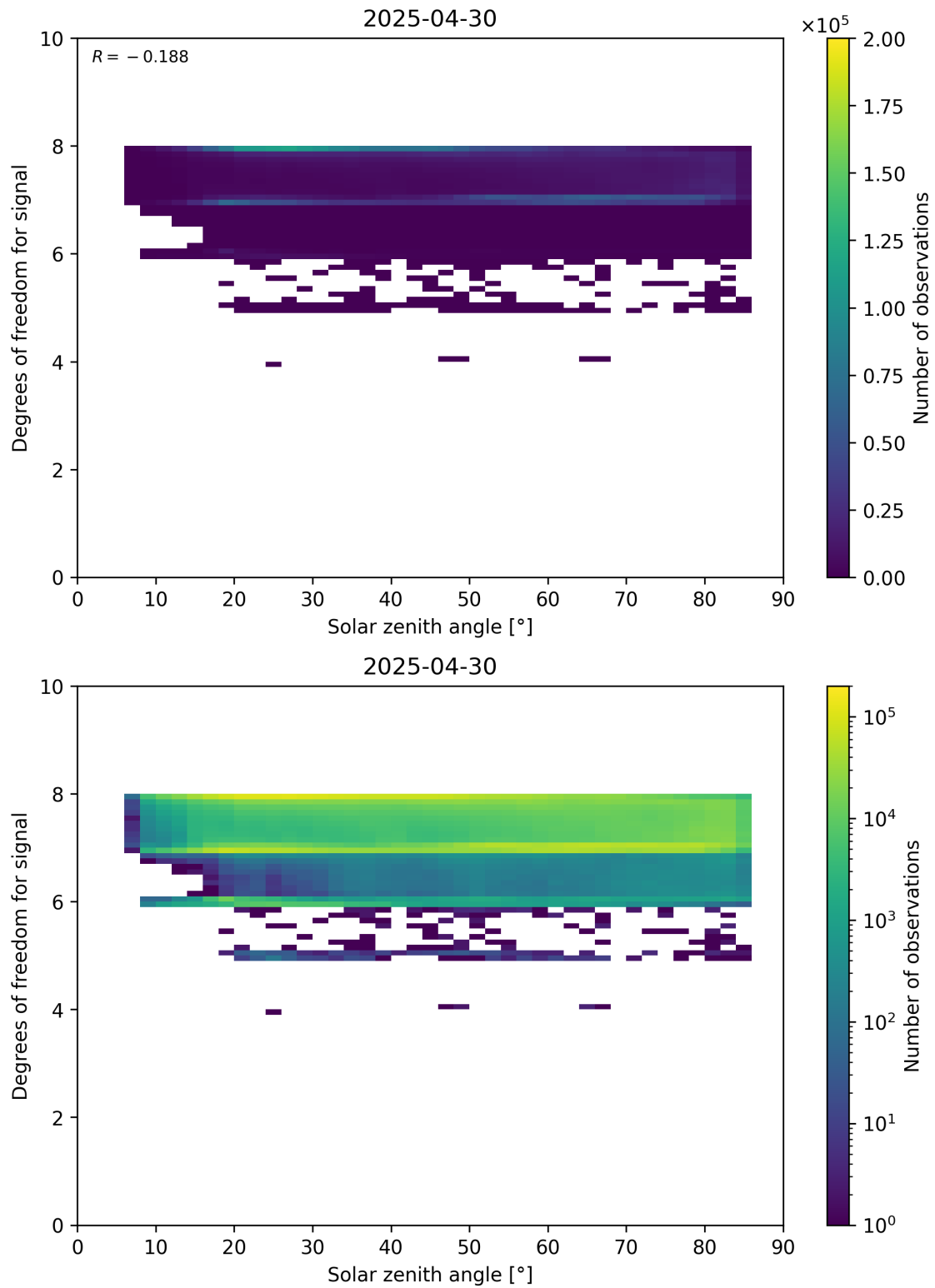
Figure 65: Scatter density plot of “Solar zenith angle” against “Degrees of freedom for signal” for 2025-04-29 to 2025-05-01.
