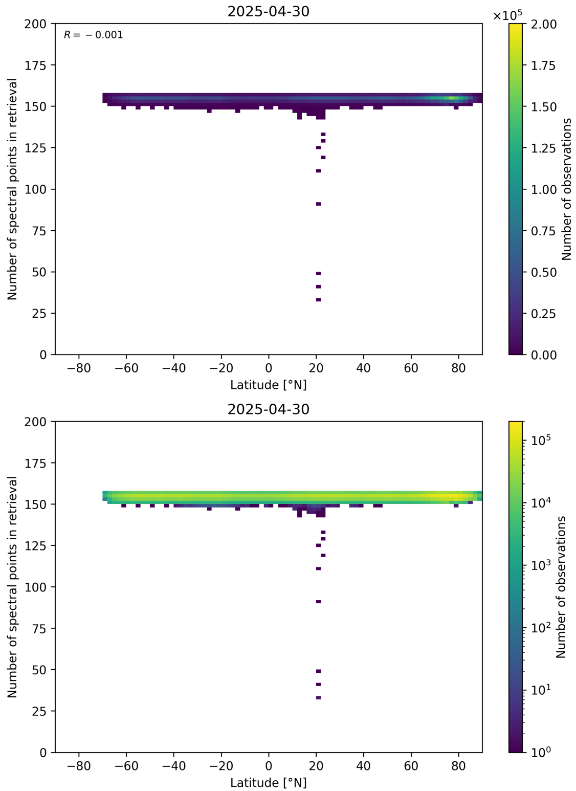
Figure 57: Scatter density plot of “Latitude” against “Number of spectral points in retrieval” for 2025-04-29 to 2025-05-01.
