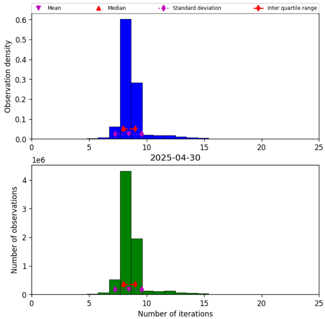
Figure 24: Histogram of “Number of iterations” for 2025-04-29 to 2025-05-01
