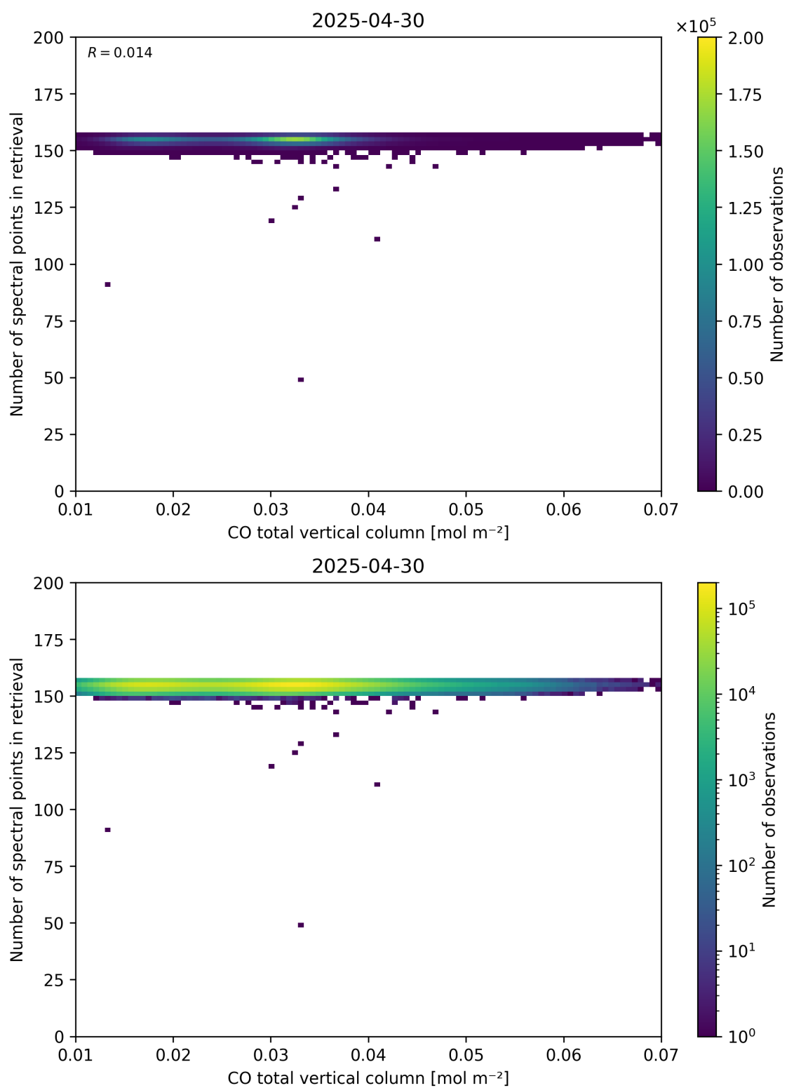
Figure 43: Scatter density plot of “CO total vertical column” against “Number of spectral points in retrieval” for 2025-04-29 to 2025-05-01.
