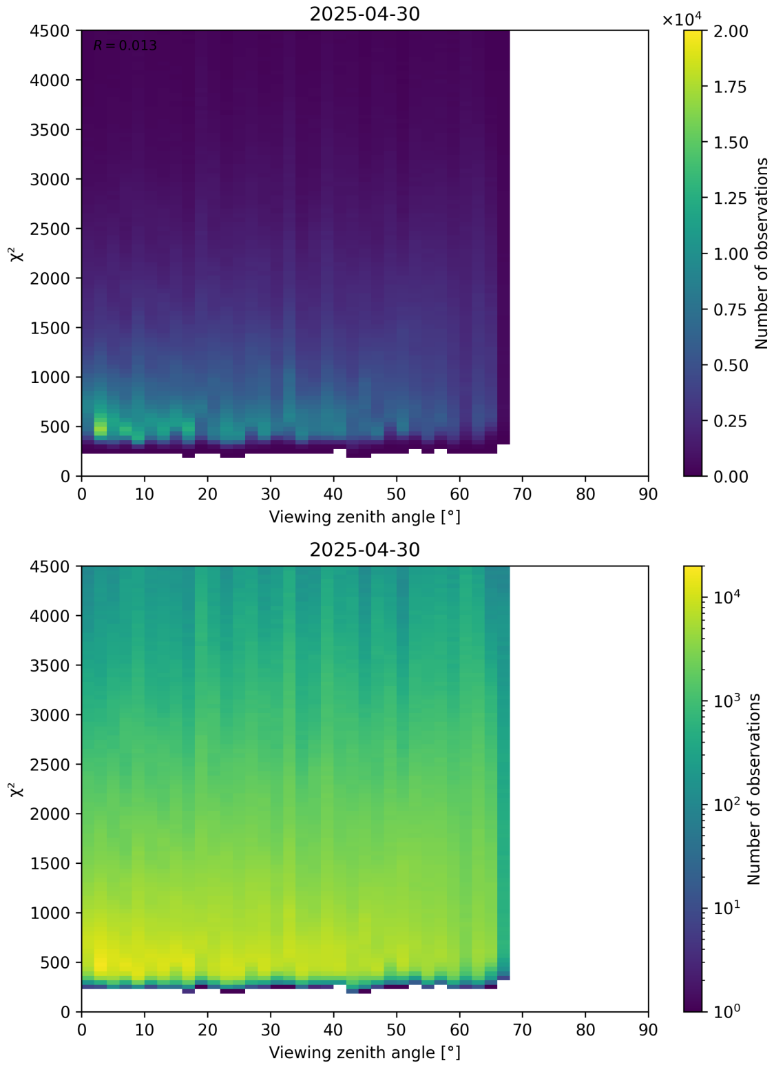
Figure 72: Scatter density plot of “Viewing zenith angle” against “ \chi^2 ” for 2025-04-29 to 2025-05-01.
