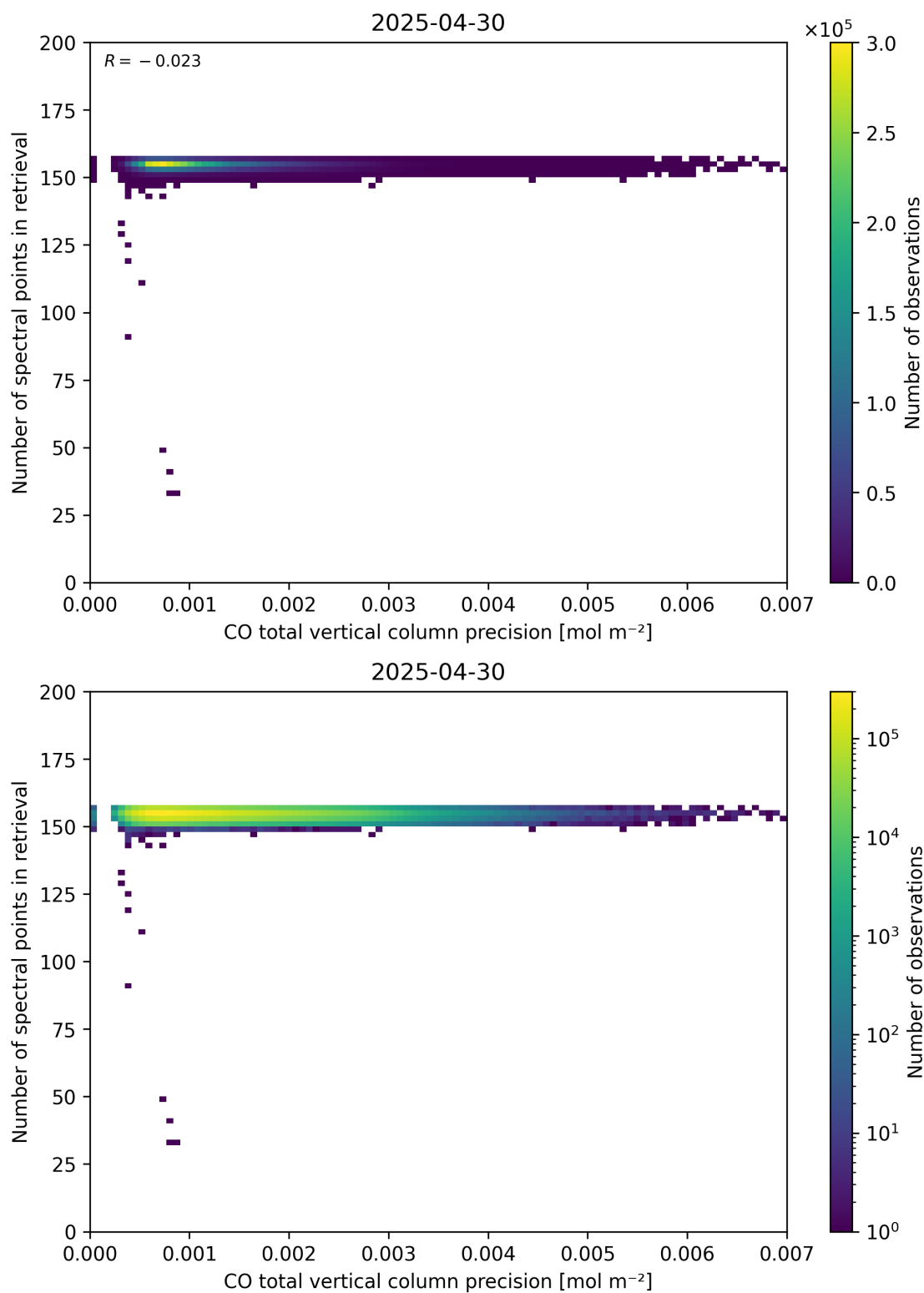
Figure 47: Scatter density plot of “CO total vertical column precision” against “Number of spectral points in retrieval” for 2025-04-29 to 2025-05-01.
