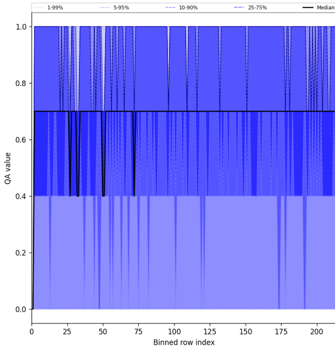
Figure 25: Along track statistics of “QA value” for 2025-04-29 to 2025-05-01
