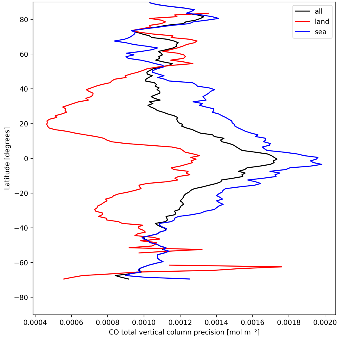
Figure 12: Zonal average of “CO total vertical column precision” for 2025-04-29 to 2025-05-01.
