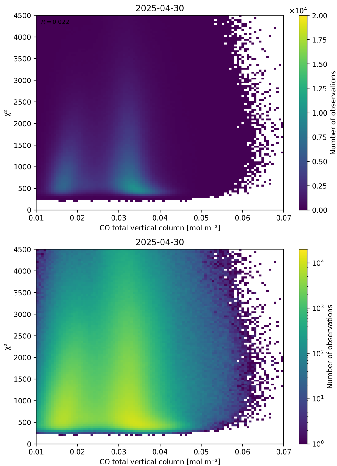
Figure 35: Scatter density plot of “CO total vertical column” against “ \chi^2 ” for 2025-04-29 to 2025-05-01.
