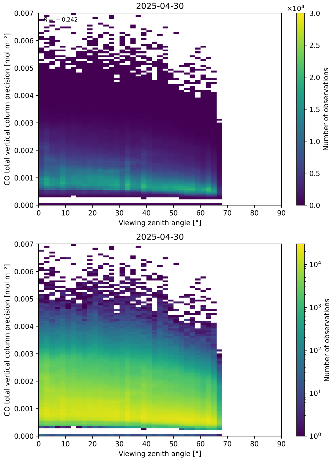
Figure 71: Scatter density plot of “Viewing zenith angle” against “CO total vertical column precision” for 2025-04-29 to 2025-05-01.
