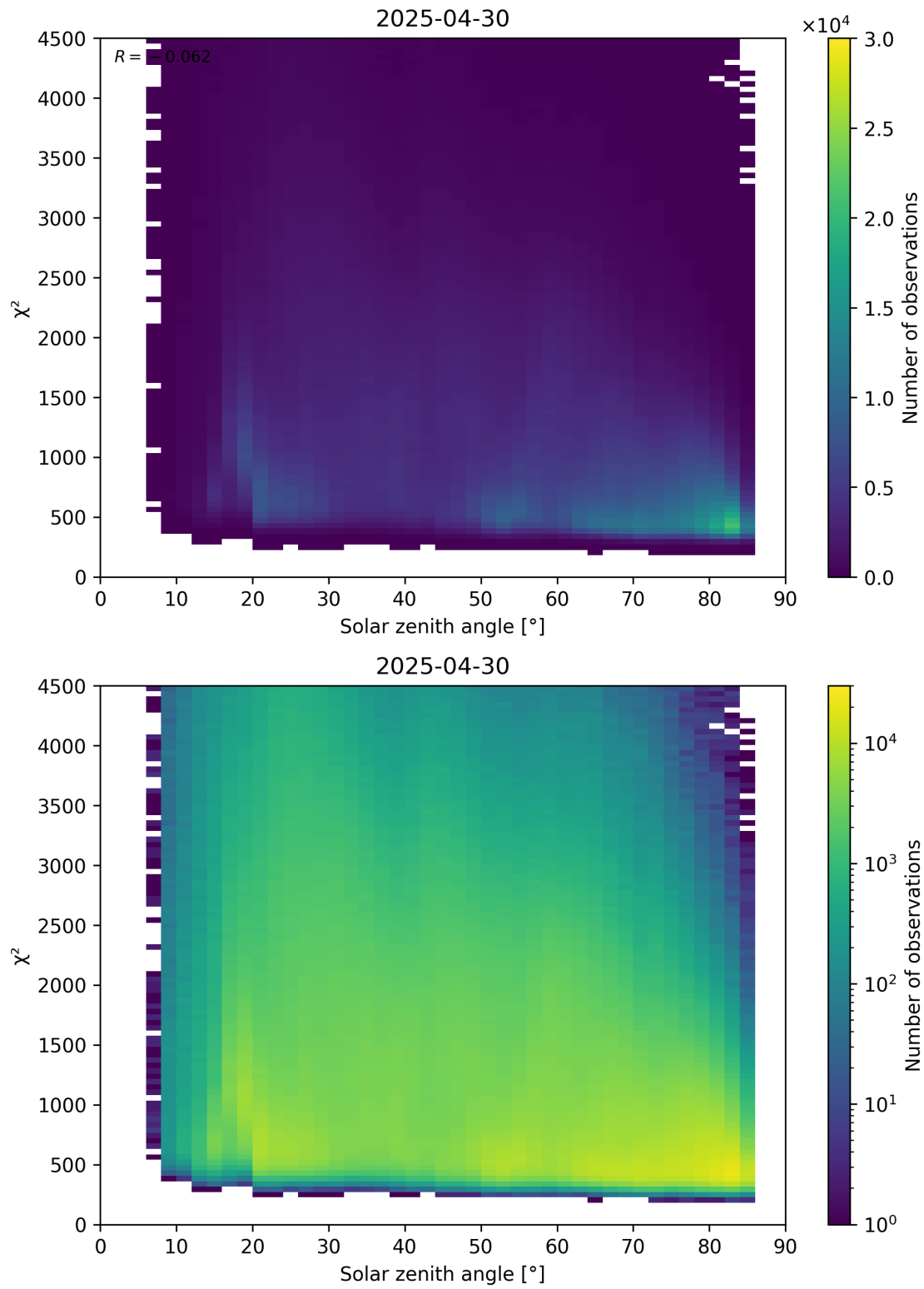
Figure 64: Scatter density plot of “Solar zenith angle” against “ \chi^2 ” for 2025-04-29 to 2025-05-01.
