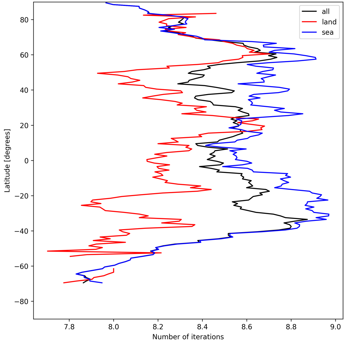
Figure 16: Zonal average of “Number of iterations” for 2025-04-29 to 2025-05-01.
