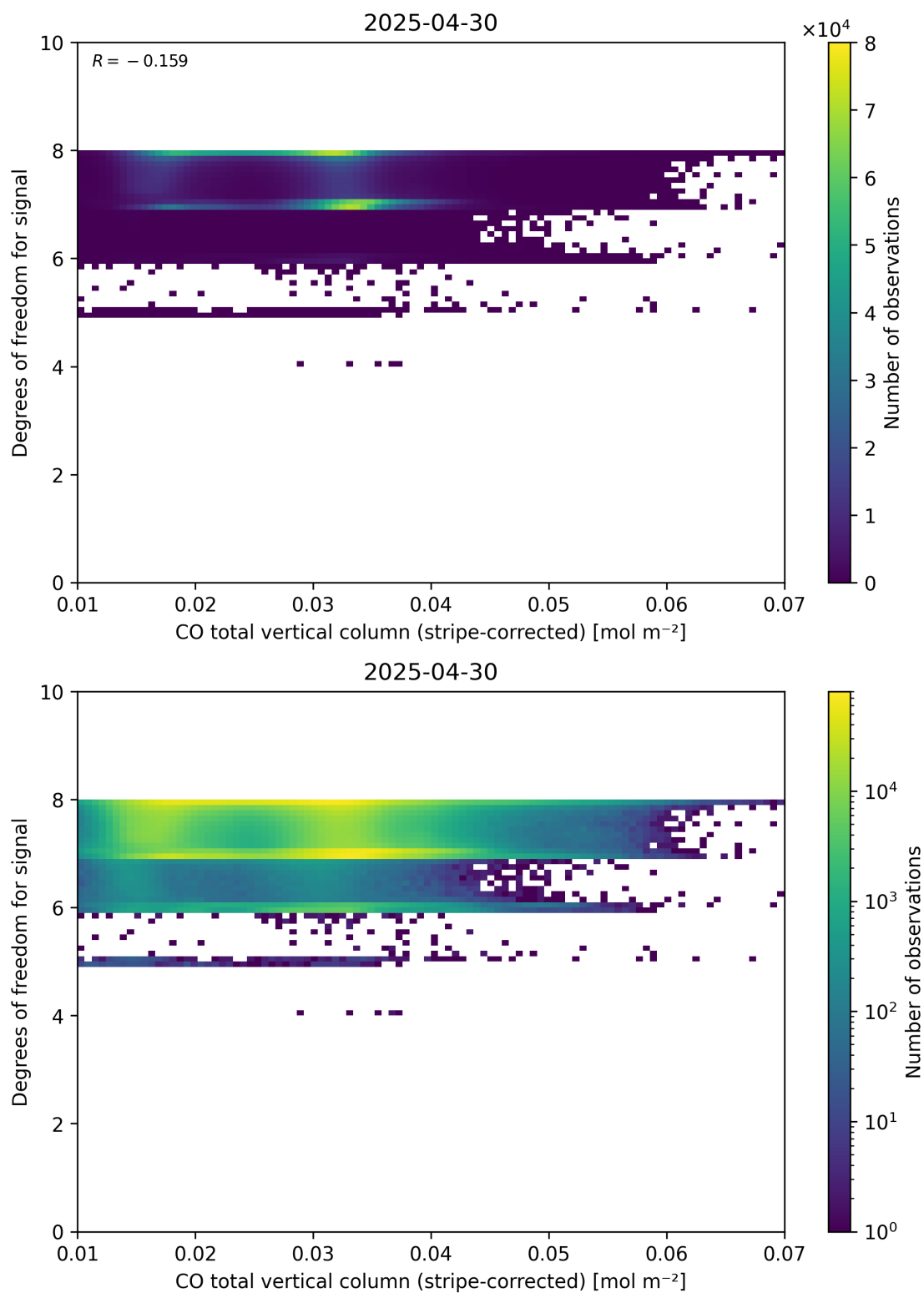
Figure 38: Scatter density plot of “CO total vertical column (stripe-corrected)” against “Degrees of freedom for signal” for 2025-04-29 to 2025-05-01.
