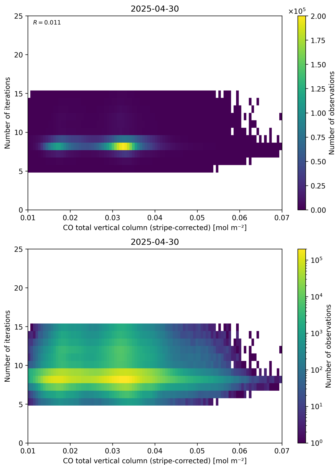
Figure 39: Scatter density plot of “CO total vertical column (stripe-corrected)” against “Number of iterations” for 2025-04-29 to 2025-05-01.
