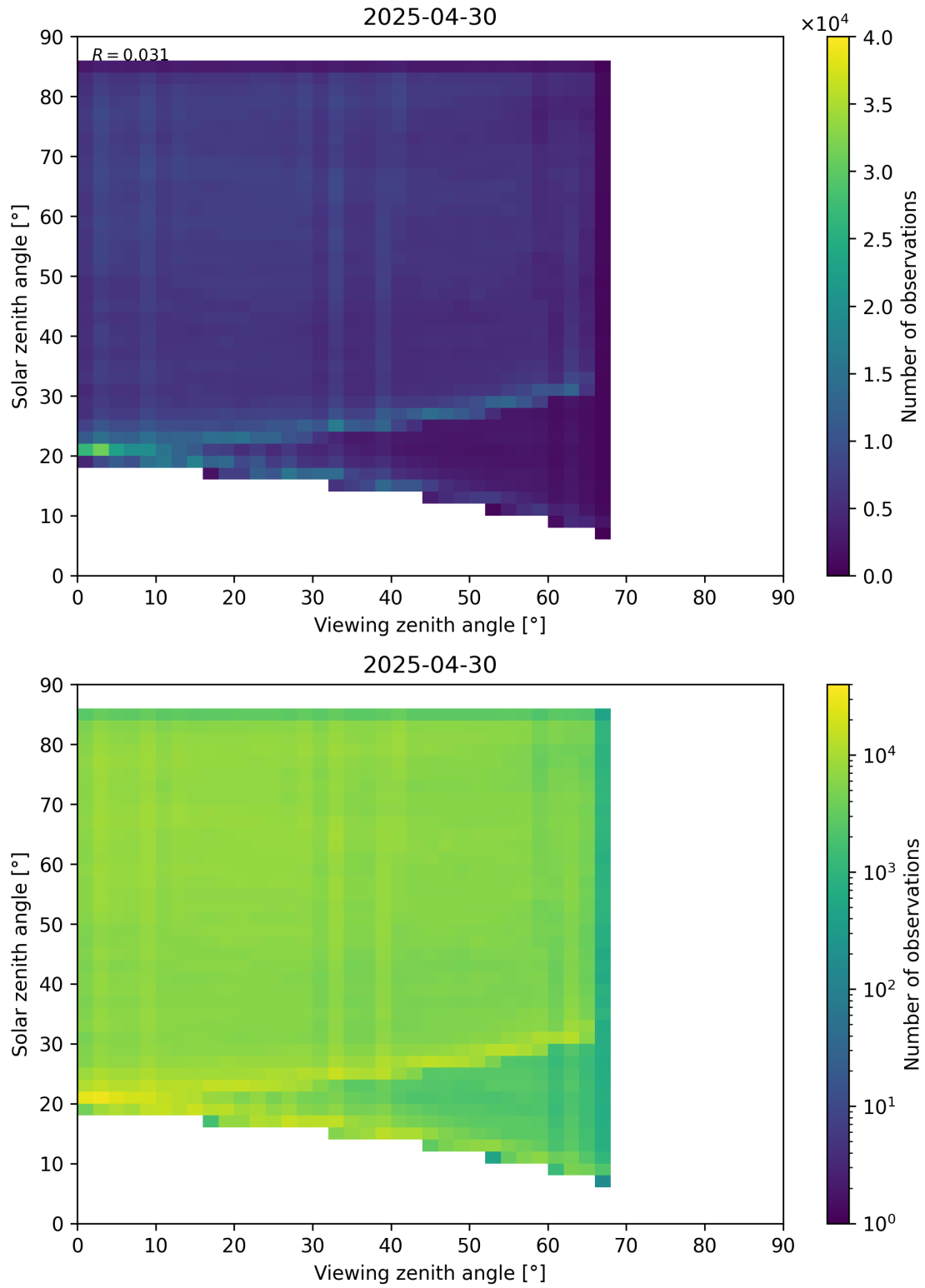
Figure 77: Scatter density plot of “Viewing zenith angle” against “Solar zenith angle” for 2025-04-29 to 2025-05-01.
