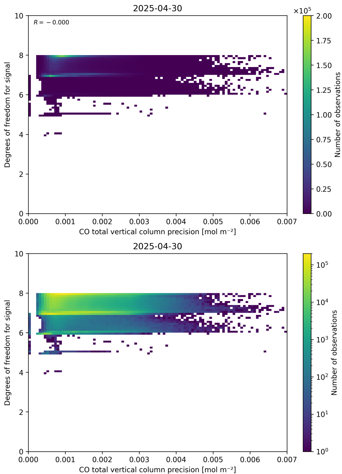
Figure 45: Scatter density plot of “CO total vertical column precision” against “Degrees of freedom for signal” for 2025-04-29 to 2025-05-01.
