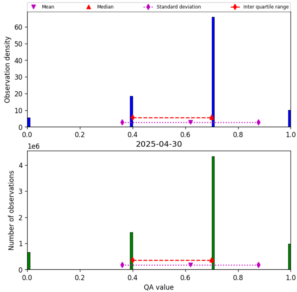
Figure 17: Histogram of “QA value” for 2025-04-29 to 2025-05-01
