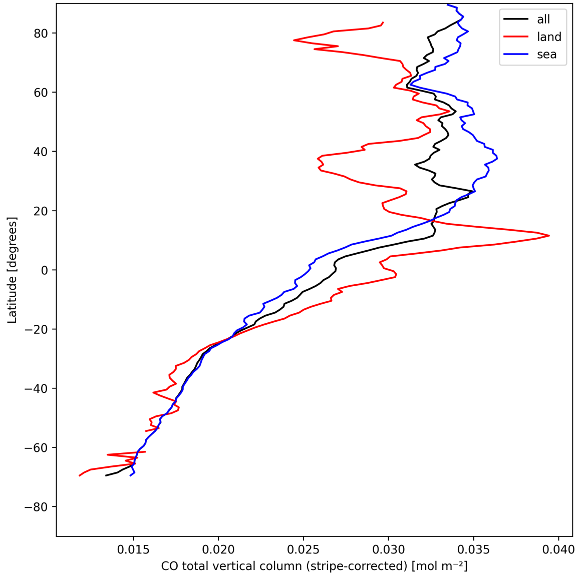
Figure 11: Zonal average of “CO total vertical column (stripe-corrected)” for 2025-04-29 to 2025-05-01.
