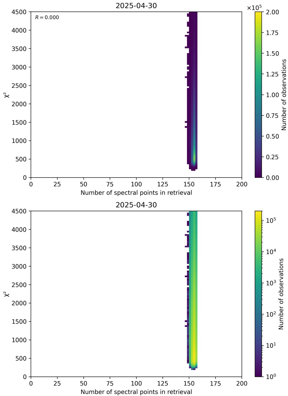
Figure 58: Scatter density plot of “Number of spectral points in retrieval” against “ \chi^2 ” for 2025-04-29 to 2025-05-01.
