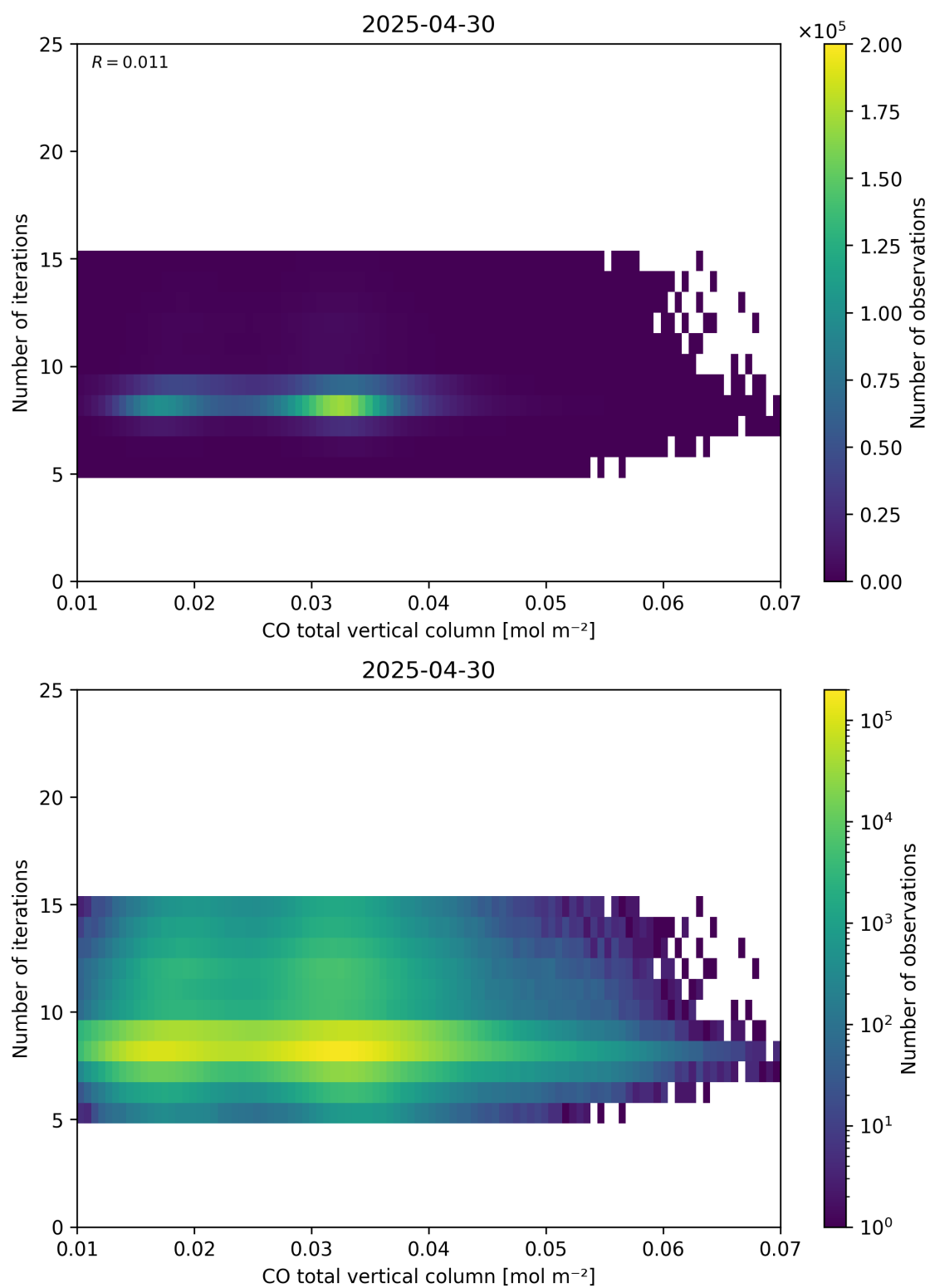
Figure 42: Scatter density plot of “CO total vertical column” against “Number of iterations” for 2025-04-29 to 2025-05-01.
