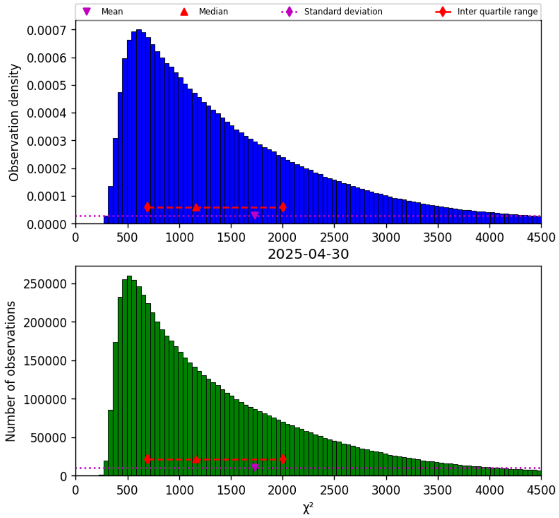
Figure 22: Histogram of “ \chi^2 ” for 2025-04-29 to 2025-05-01
