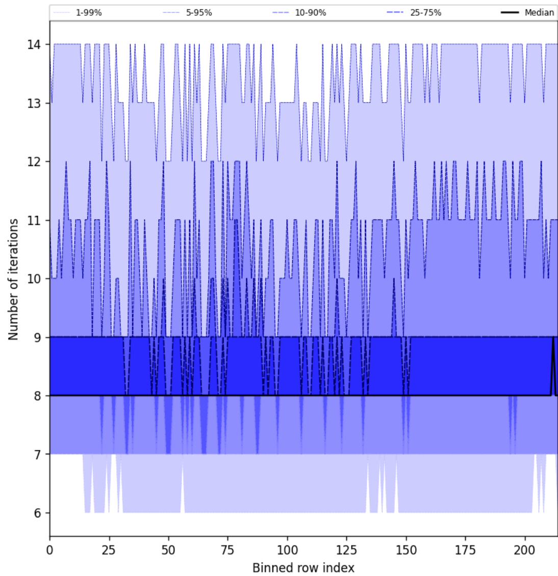
Figure 32: Along track statistics of “Number of iterations” for 2025-04-29 to 2025-05-01
