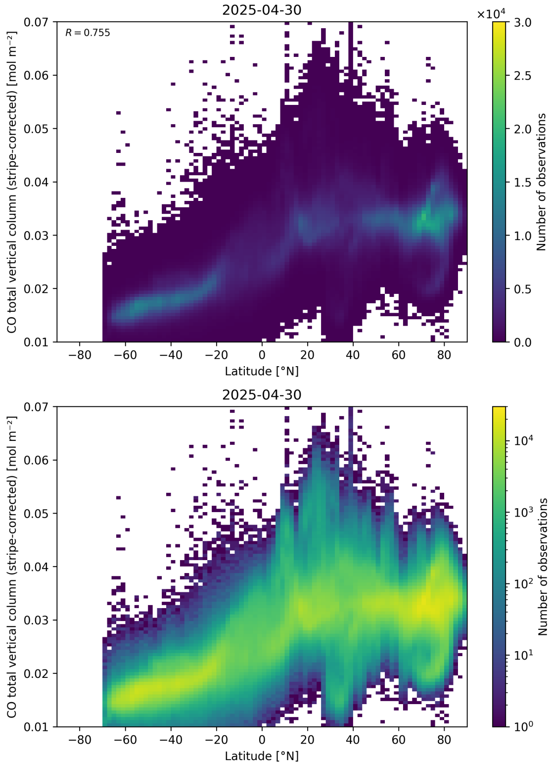
Figure 52: Scatter density plot of “Latitude” against “CO total vertical column (stripe-corrected)” for 2025-04-29 to 2025-05-01.
