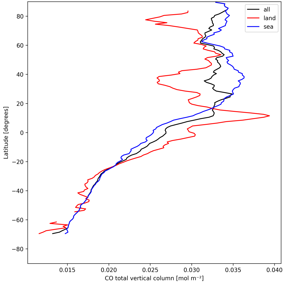
Figure 10: Zonal average of “CO total vertical column” for 2025-04-29 to 2025-05-01.
