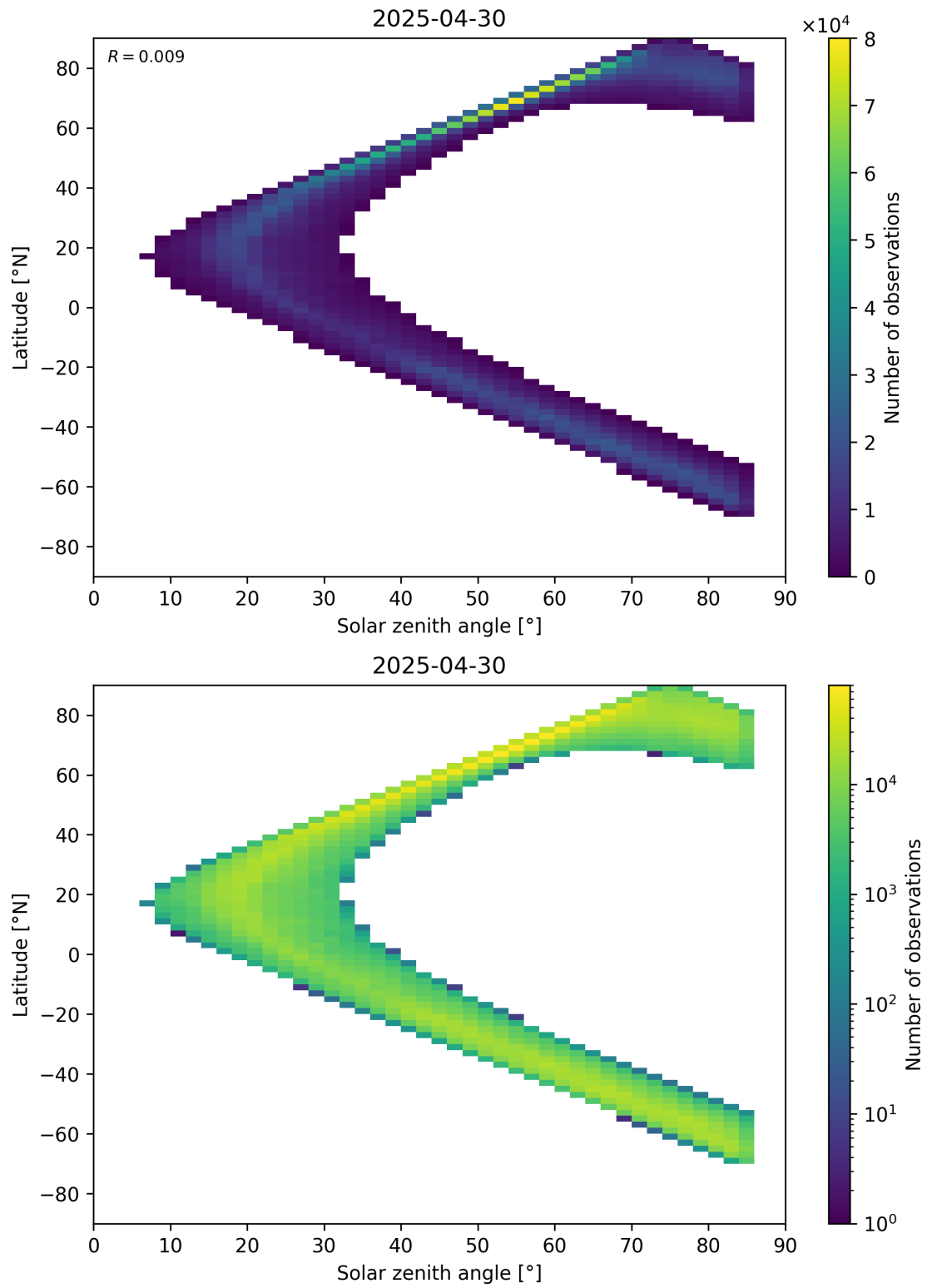
Figure 66: Scatter density plot of “Solar zenith angle” against “Latitude” for 2025-04-29 to 2025-05-01.
