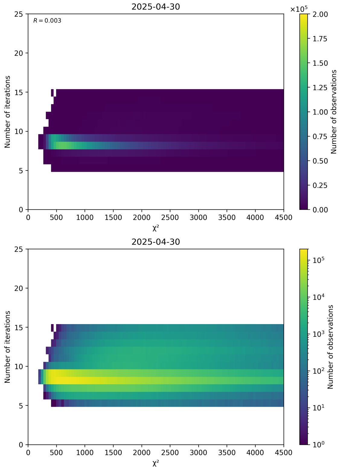
Figure 49: Scatter density plot of “ \chi^2 ” against “Number of iterations” for 2025-04-29 to 2025-05-01.
