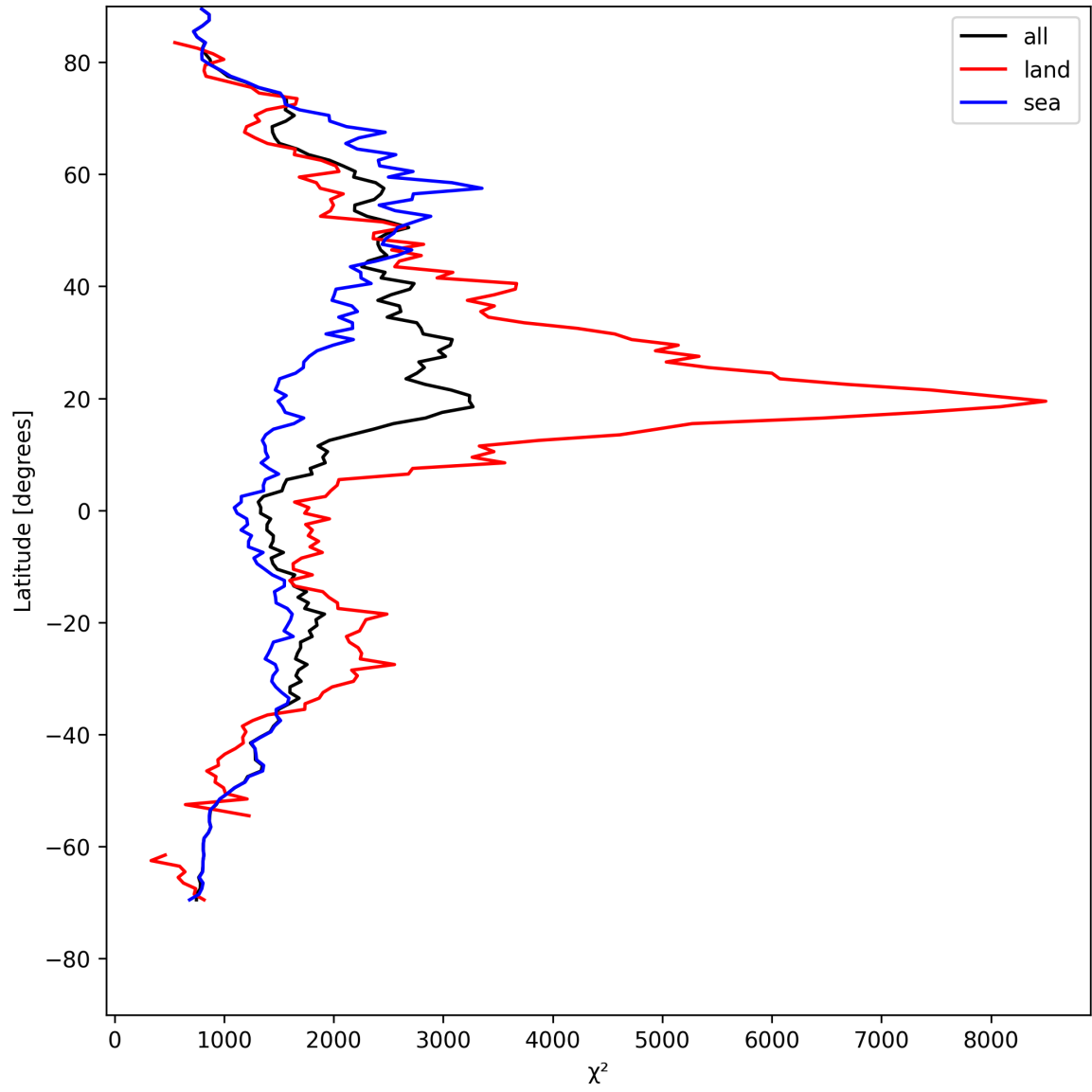
Figure 14: Zonal average of “ \chi^2 ” for 2025-04-29 to 2025-05-01.
