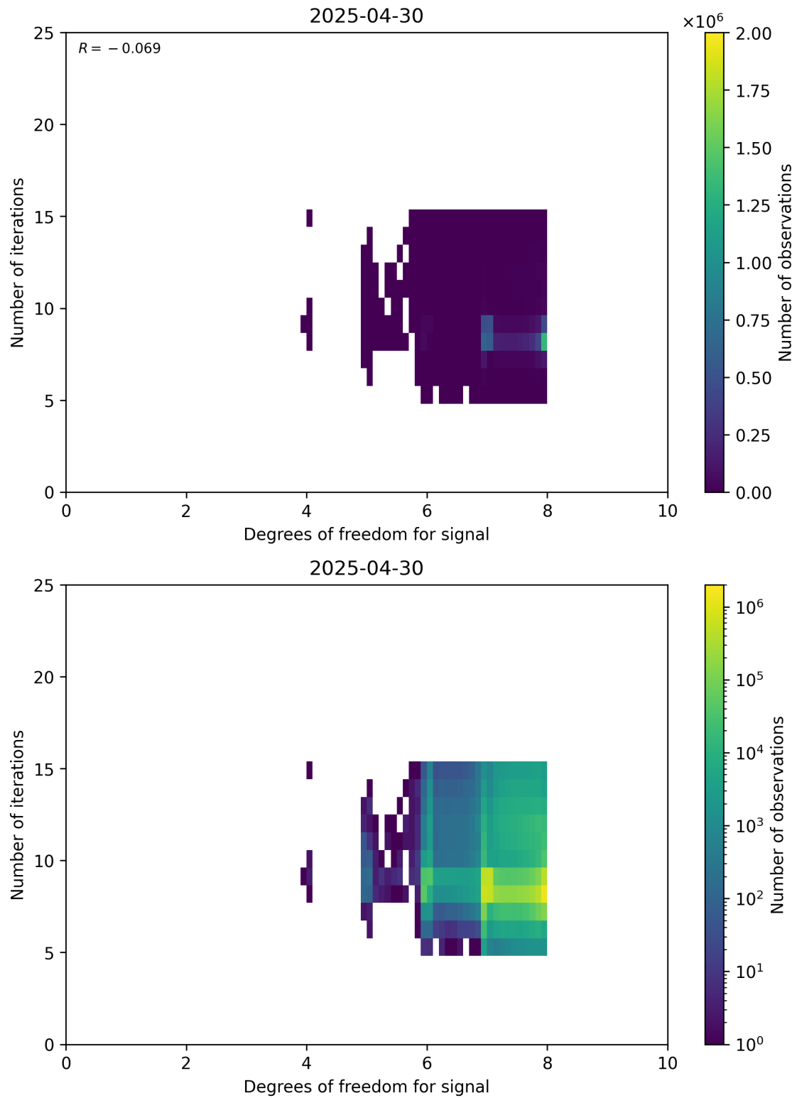
Figure 50: Scatter density plot of “Degrees of freedom for signal” against “Number of iterations” for 2025-04-29 to 2025-05-01.
