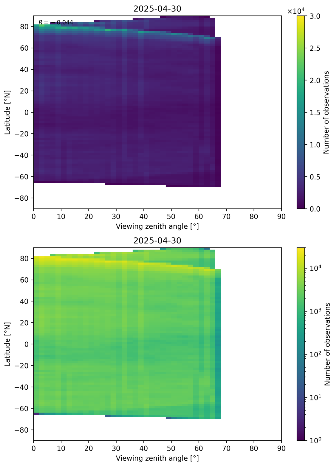
Figure 74: Scatter density plot of “Viewing zenith angle” against “Latitude” for 2025-04-29 to 2025-05-01.
