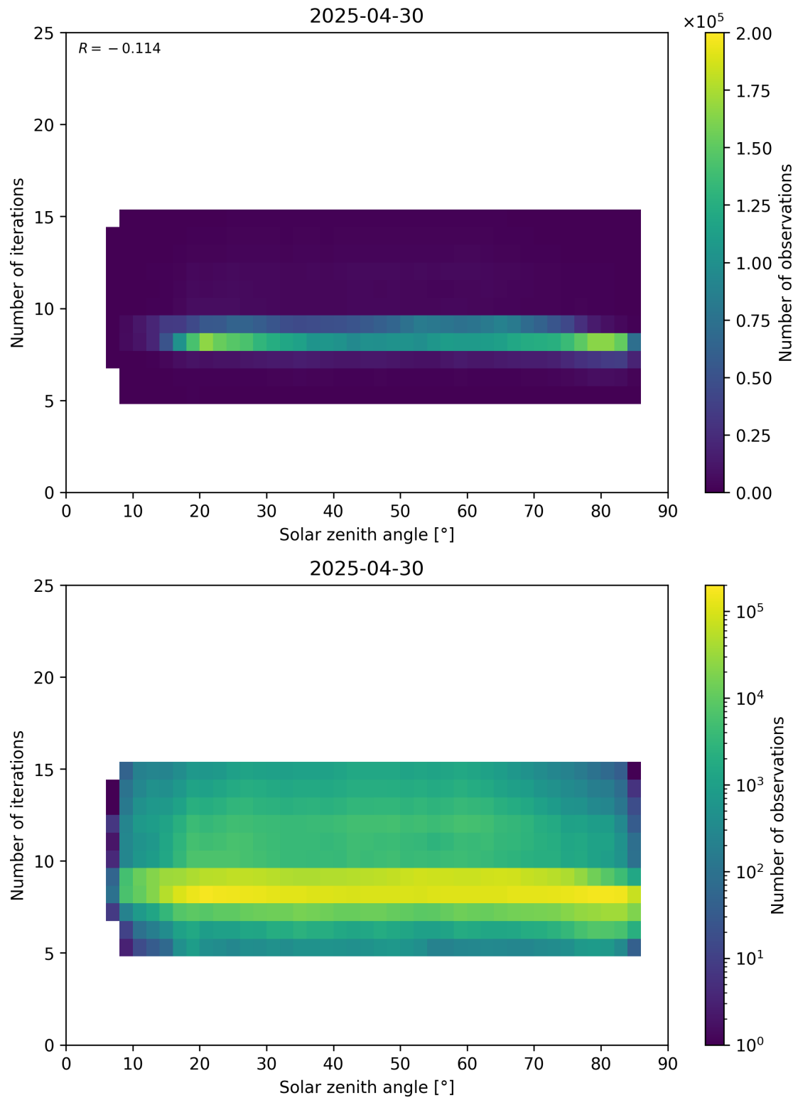
Figure 67: Scatter density plot of “Solar zenith angle” against “Number of iterations” for 2025-04-29 to 2025-05-01.
