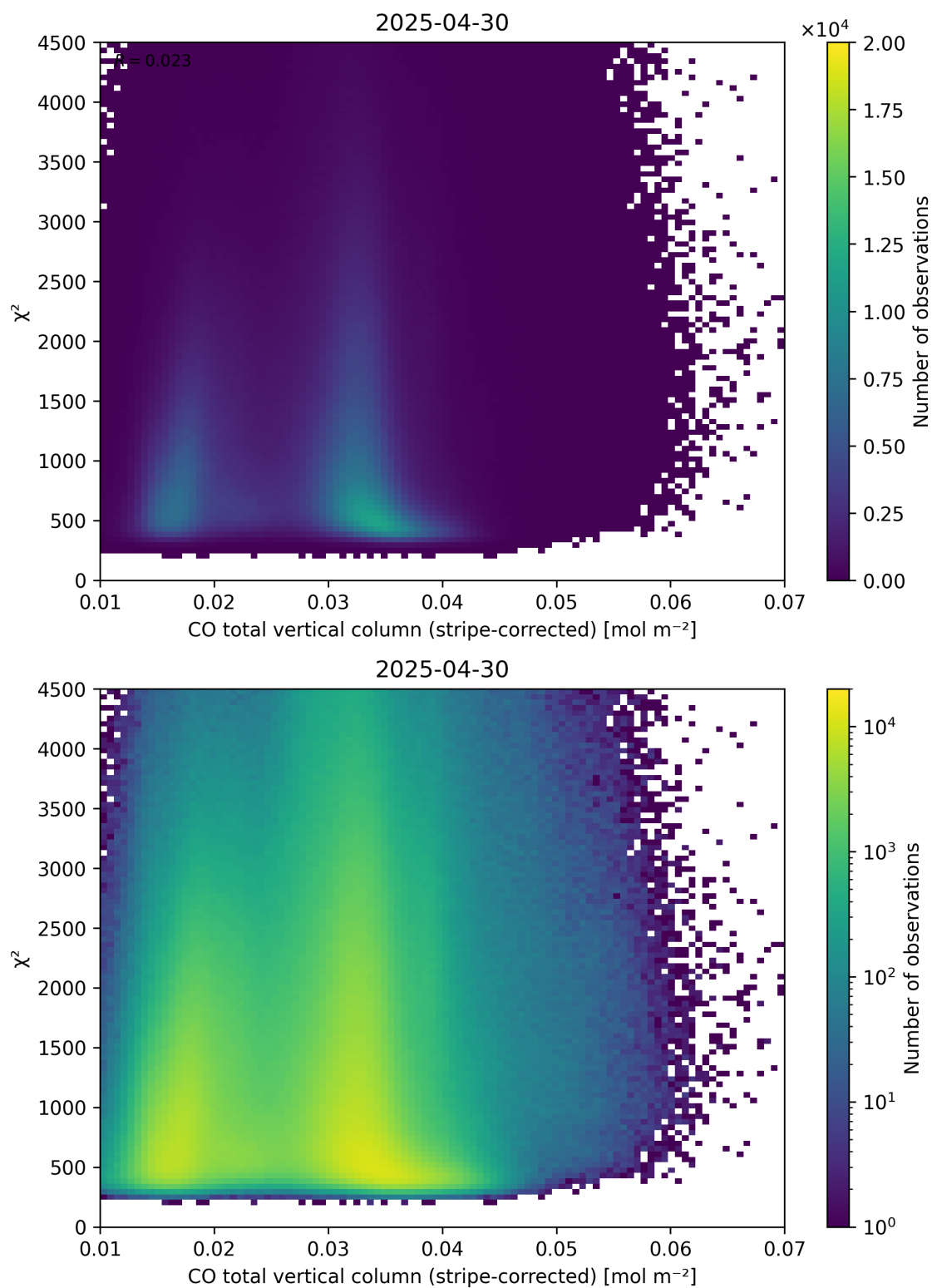
Figure 37: Scatter density plot of “CO total vertical column (stripe-corrected)” against “ \chi^2 ” for 2025-04-29 to 2025-05-01.
