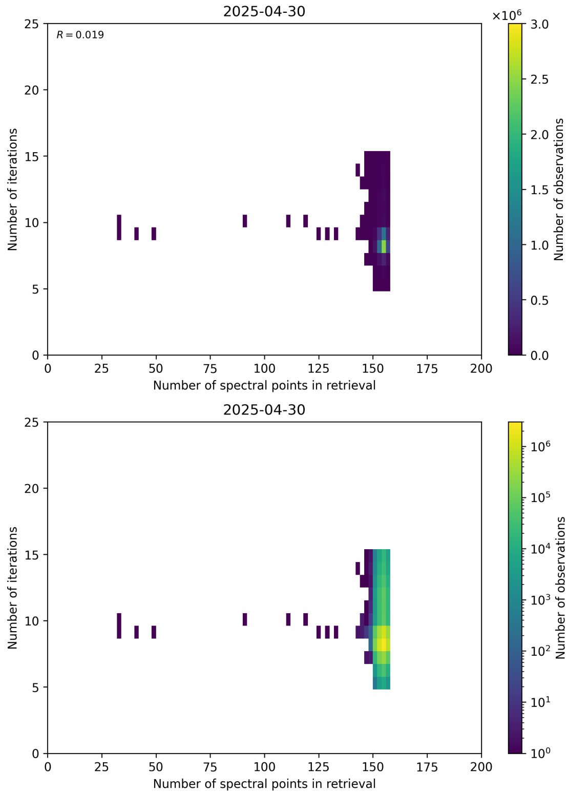
Figure 60: Scatter density plot of “Number of spectral points in retrieval” against “Number of iterations” for 2025-04-29 to 2025-05-01.
