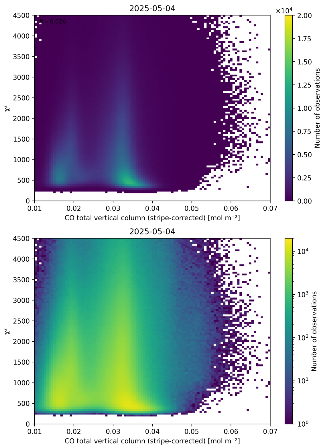
Figure 37: Scatter density plot of “CO total vertical column (stripe-corrected)” against “ \chi^2 ” for 2025-05-03 to 2025-05-05.
