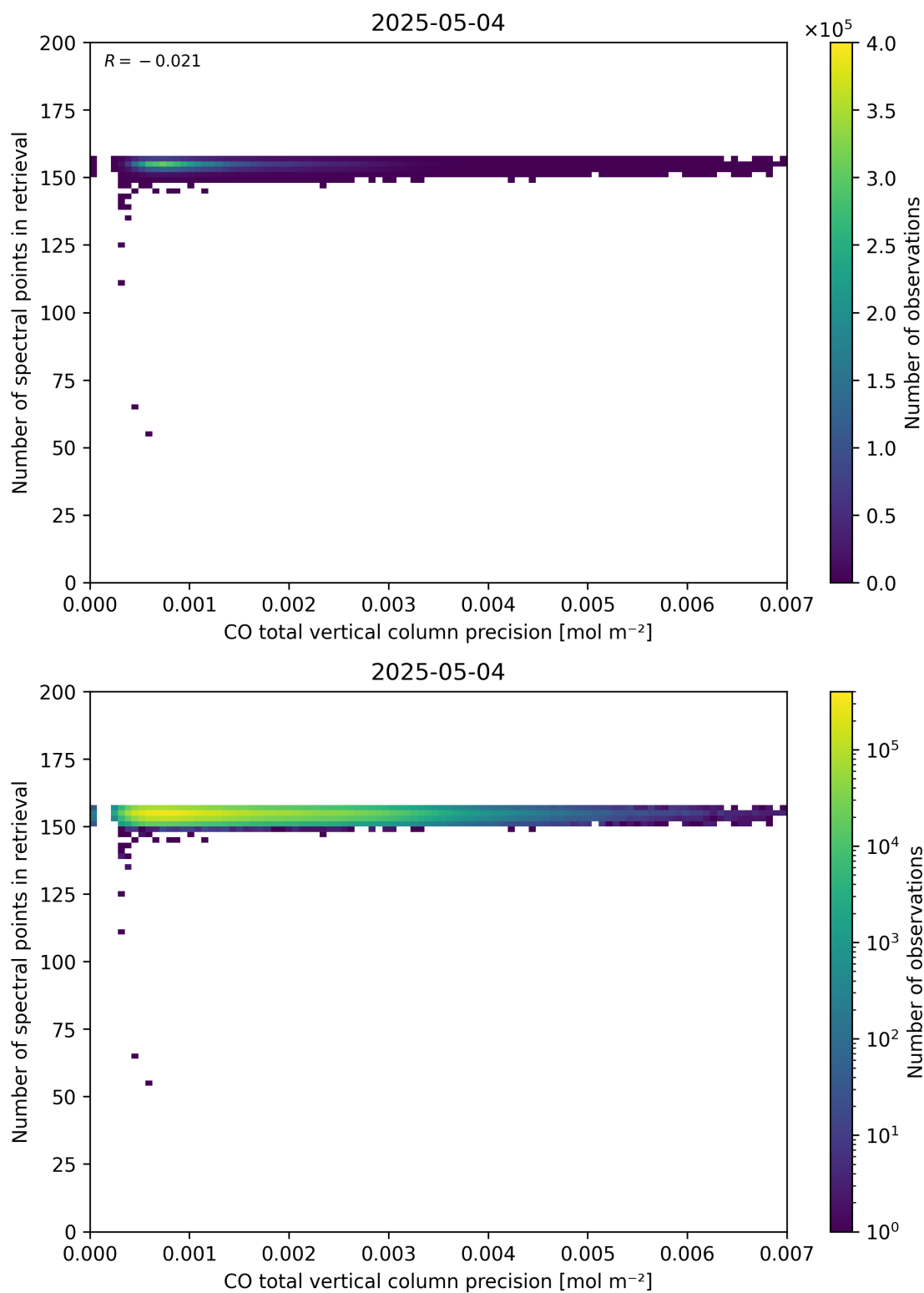
Figure 47: Scatter density plot of “CO total vertical column precision” against “Number of spectral points in retrieval” for 2025-05-03 to 2025-05-05.
