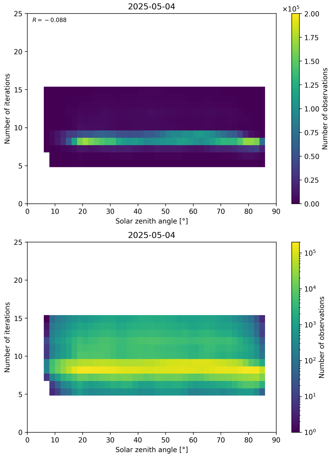
Figure 67: Scatter density plot of “Solar zenith angle” against “Number of iterations” for 2025-05-03 to 2025-05-05.
