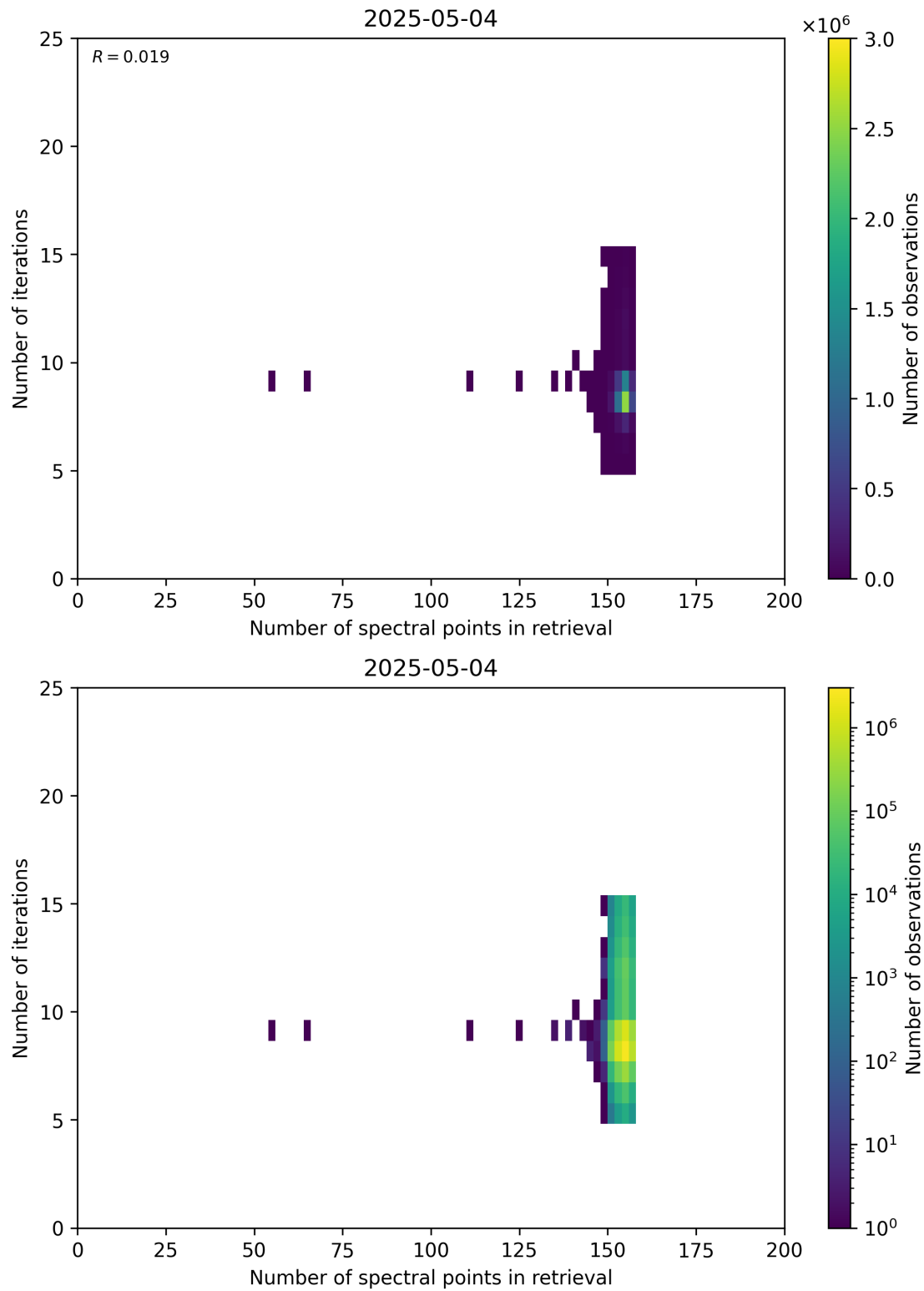
Figure 60: Scatter density plot of “Number of spectral points in retrieval” against “Number of iterations” for 2025-05-03 to 2025-05-05.
