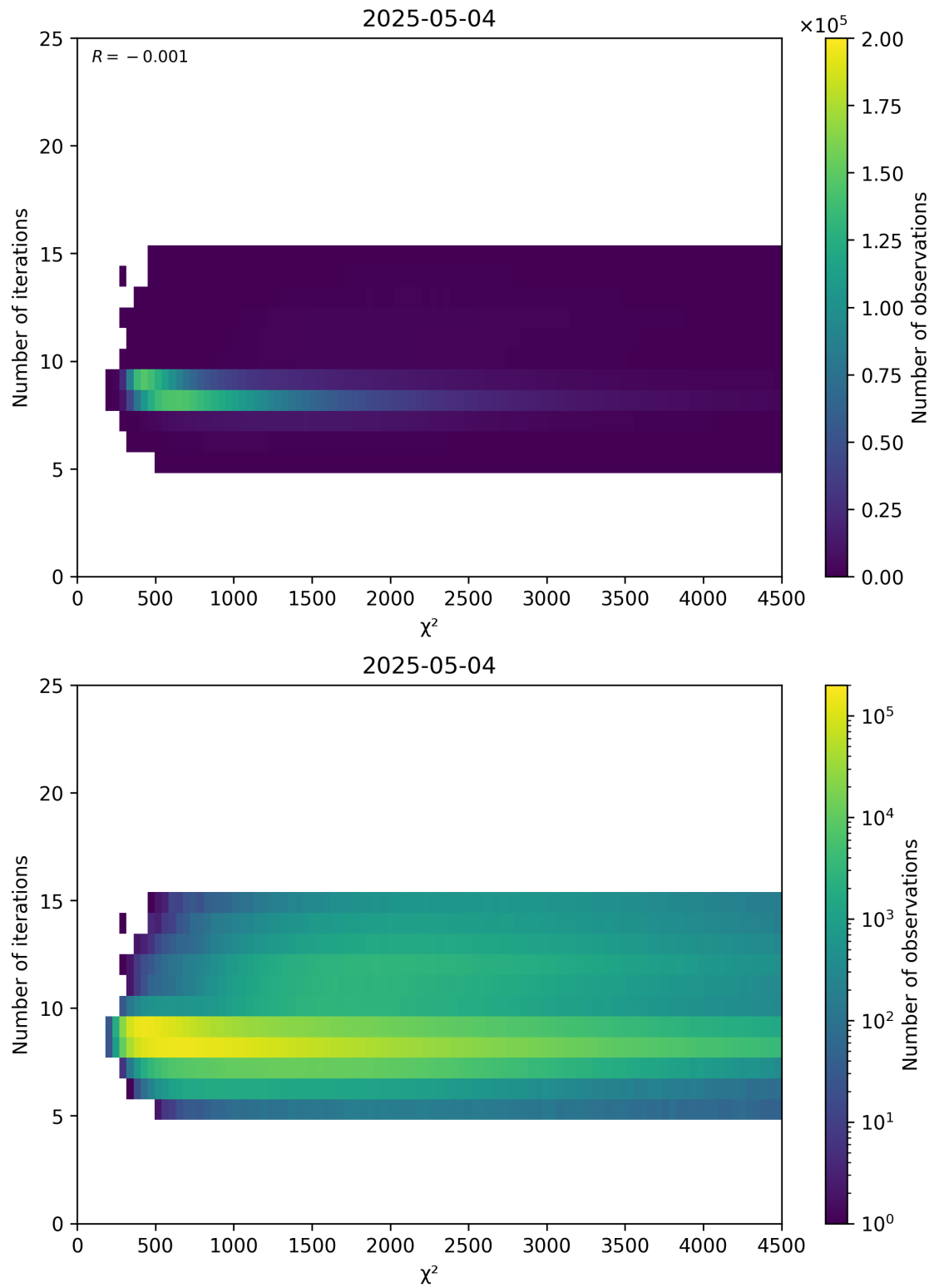
Figure 49: Scatter density plot of “ \chi^2 ” against “Number of iterations” for 2025-05-03 to 2025-05-05.
