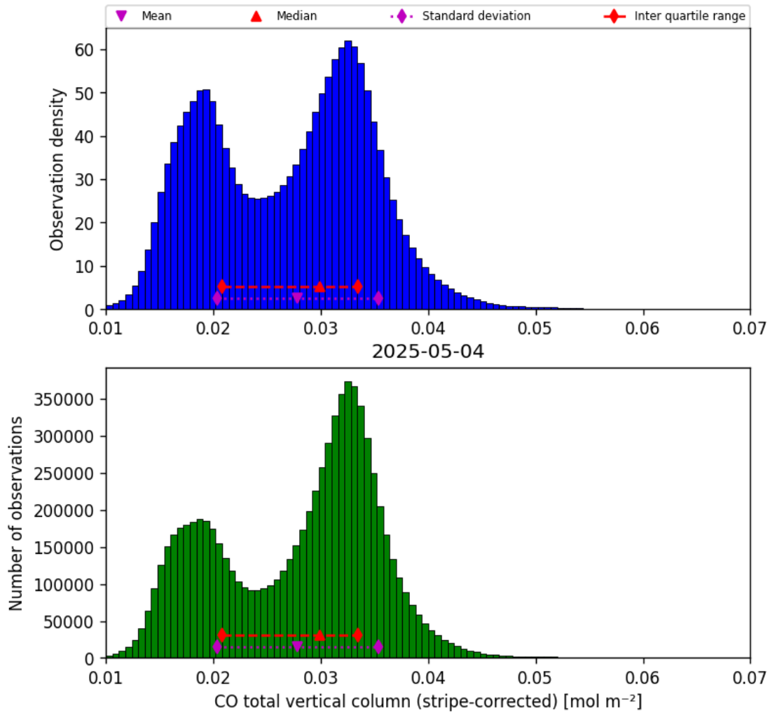
Figure 19: Histogram of “CO total vertical column (stripe-corrected)” for 2025-05-03 to 2025-05-05
