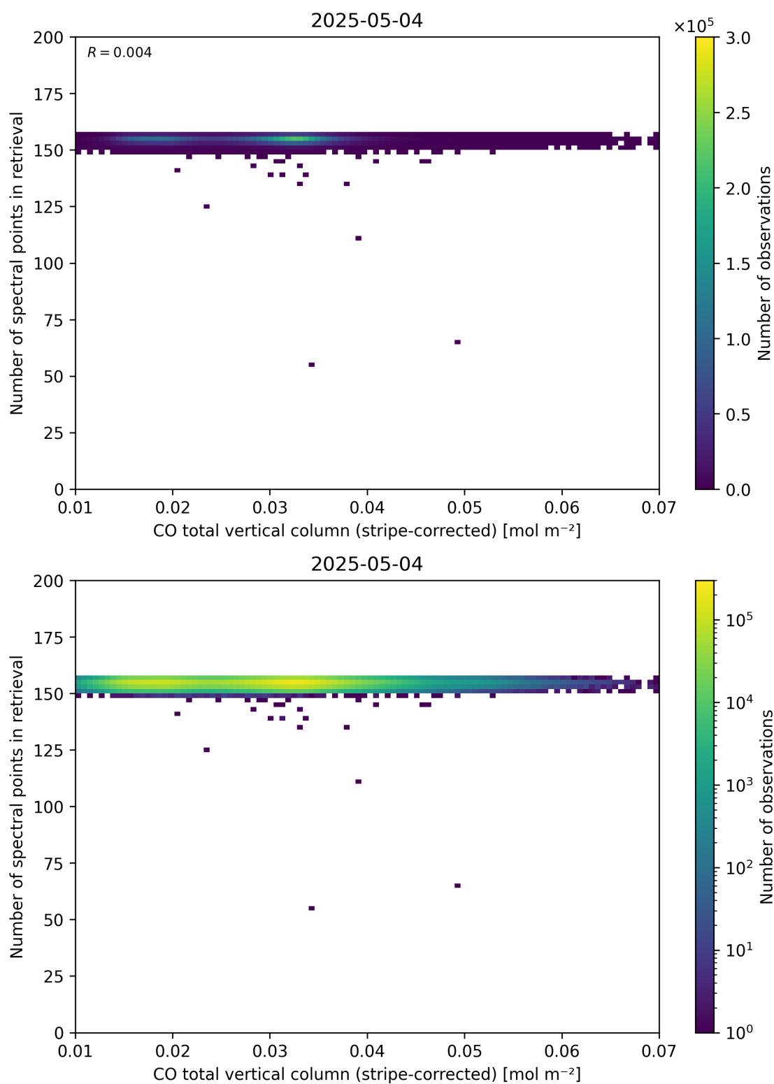
Figure 40: Scatter density plot of “CO total vertical column (stripe-corrected)” against “Number of spectral points in retrieval” for 2025-05-03 to 2025-05-05.
