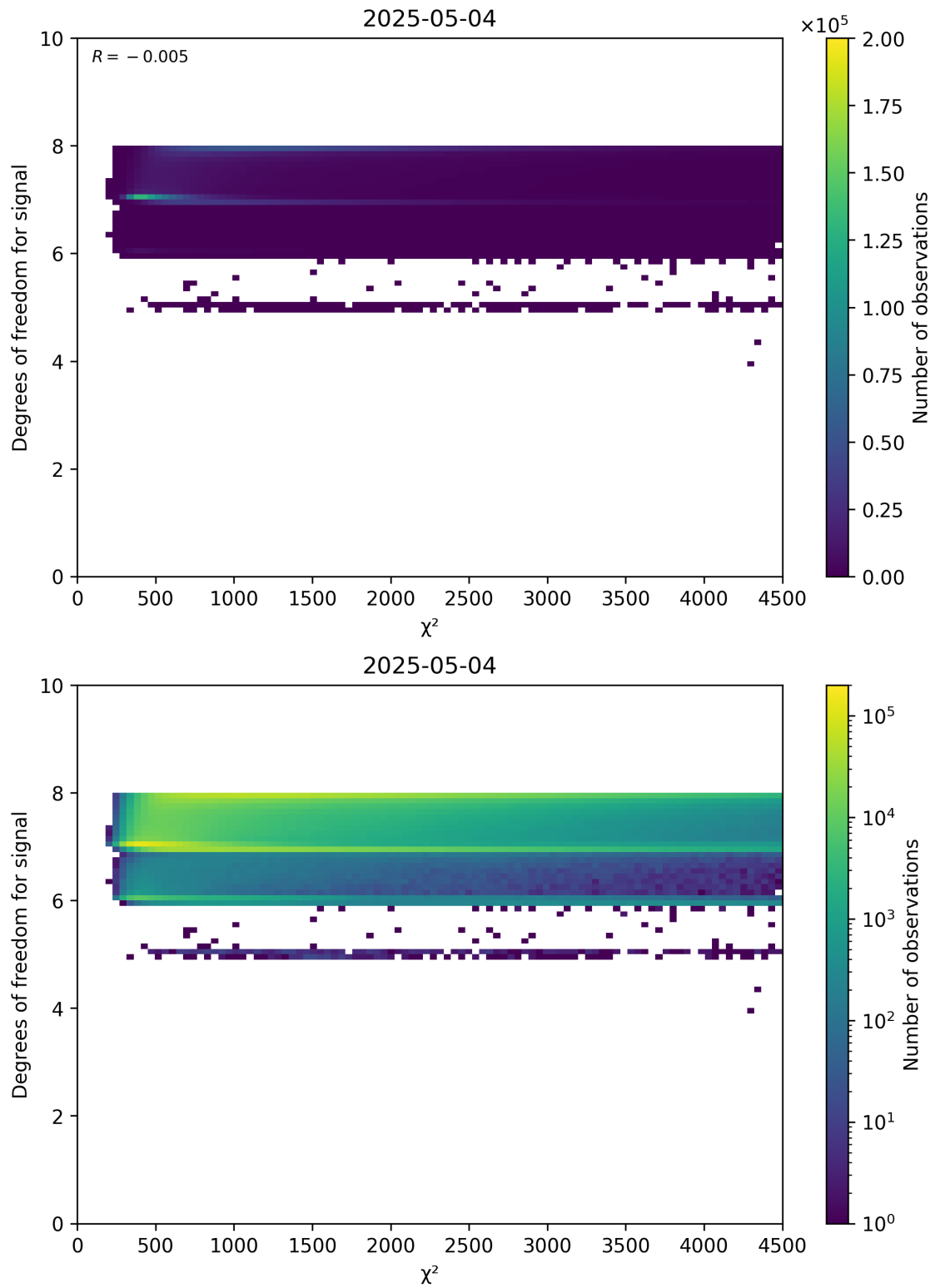
Figure 48: Scatter density plot of “ \chi^2 ” against “Degrees of freedom for signal” for 2025-05-03 to 2025-05-05.
