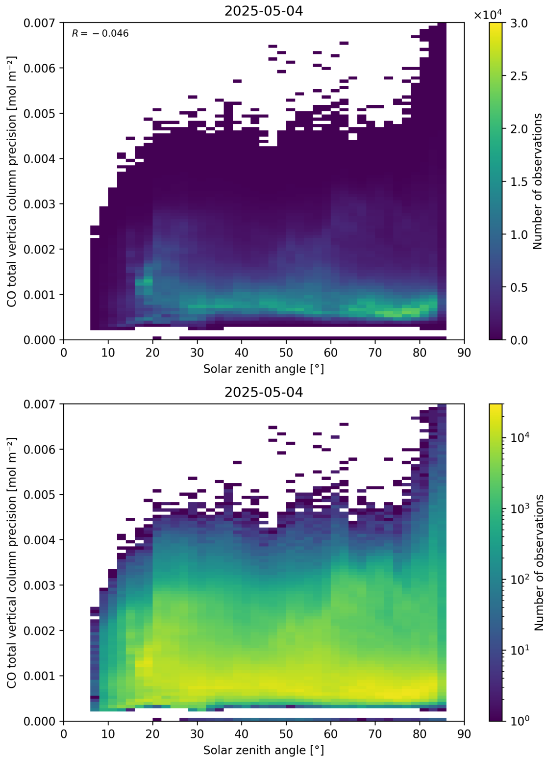
Figure 63: Scatter density plot of “Solar zenith angle” against “CO total vertical column precision” for 2025-05-03 to 2025-05-05.
