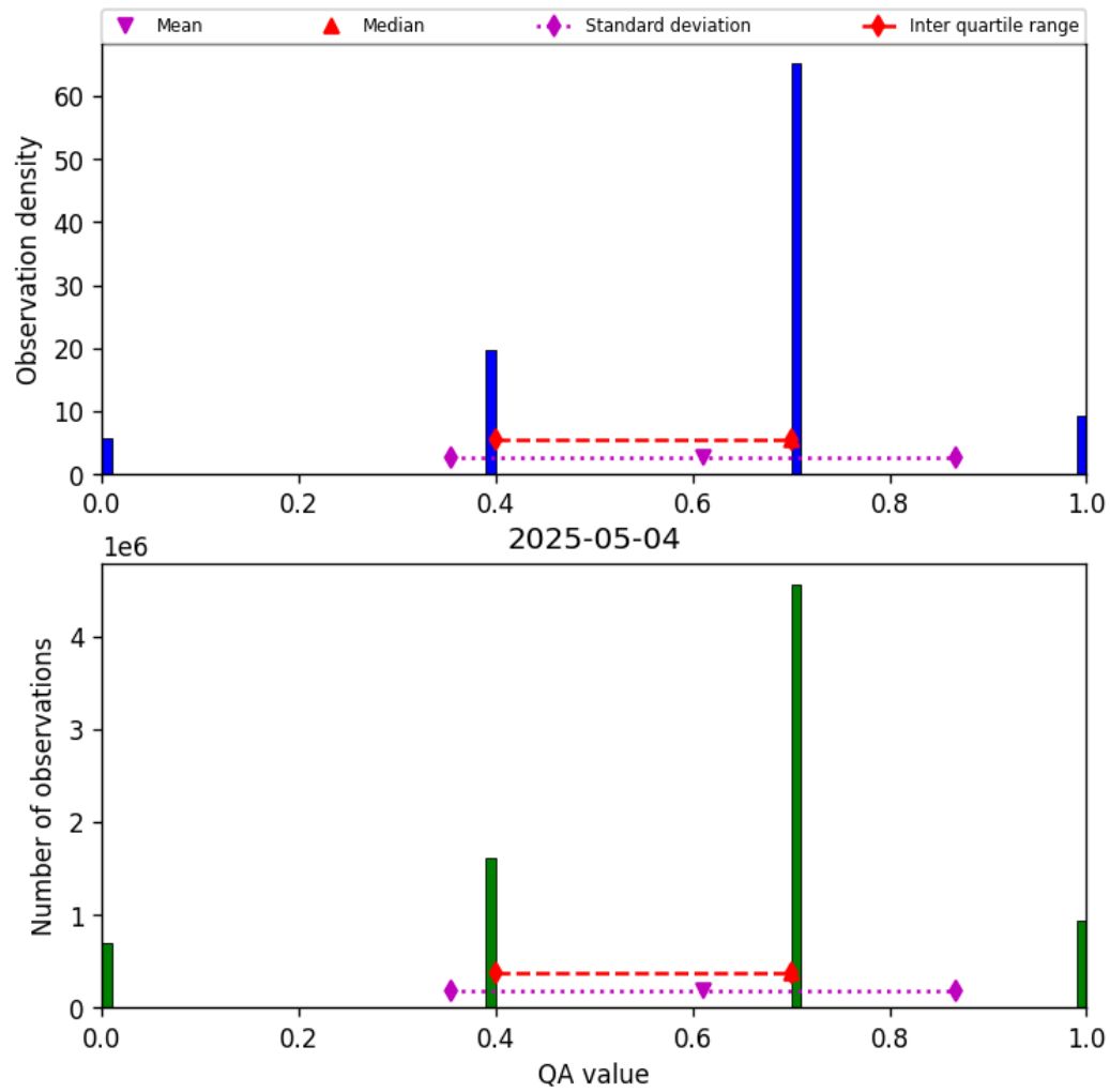
Figure 17: Histogram of “QA value” for 2025-05-03 to 2025-05-05
