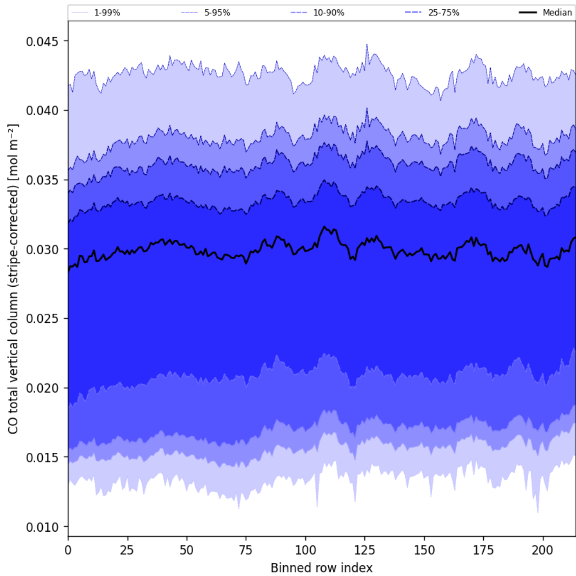
Figure 27: Along track statistics of “CO total vertical column (stripe-corrected)” for 2025-05-03 to 2025-05-05
