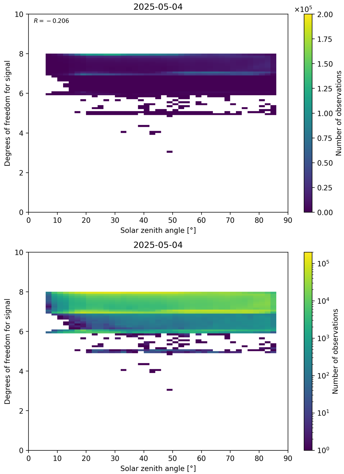
Figure 65: Scatter density plot of “Solar zenith angle” against “Degrees of freedom for signal” for 2025-05-03 to 2025-05-05.
