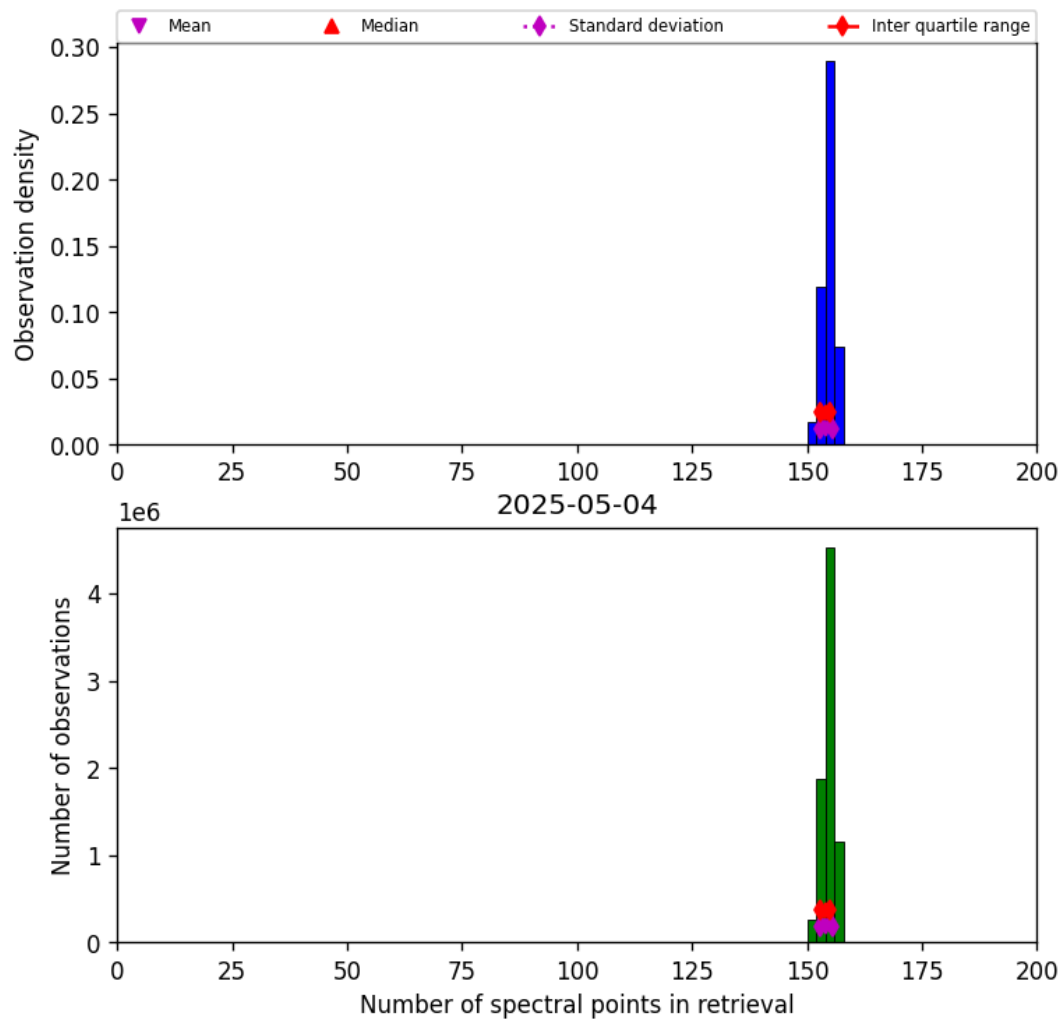
Figure 21: Histogram of “Number of spectral points in retrieval” for 2025-05-03 to 2025-05-05
