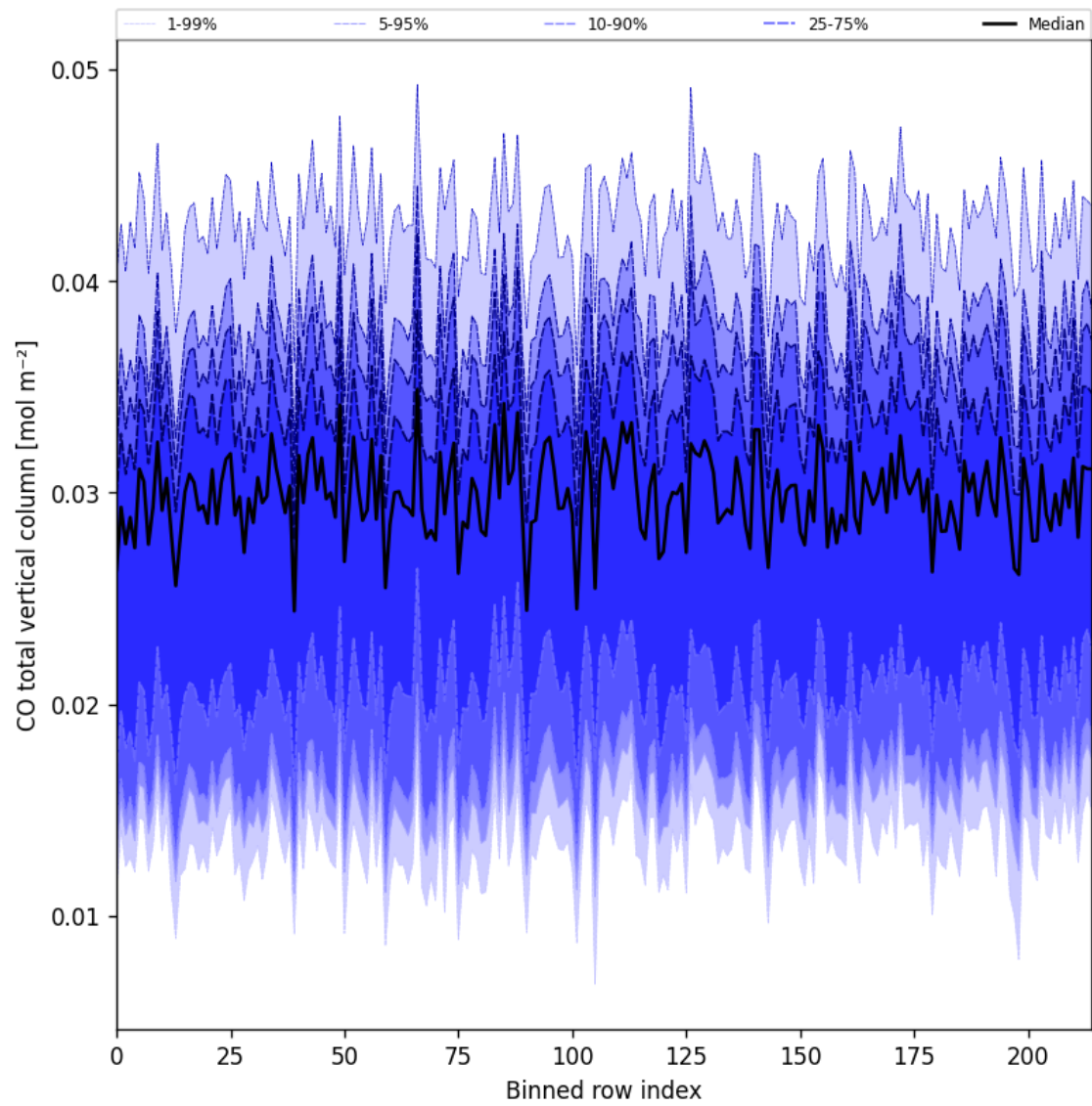
Figure 26: Along track statistics of “CO total vertical column” for 2025-05-03 to 2025-05-05
