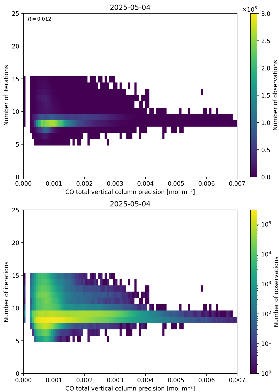
Figure 46: Scatter density plot of “CO total vertical column precision” against “Number of iterations” for 2025-05-03 to 2025-05-05.
