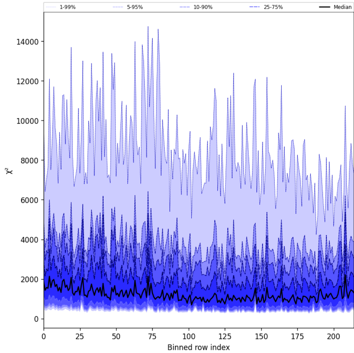
Figure 30: Along track statistics of “ \chi^2 ” for 2025-05-03 to 2025-05-05
