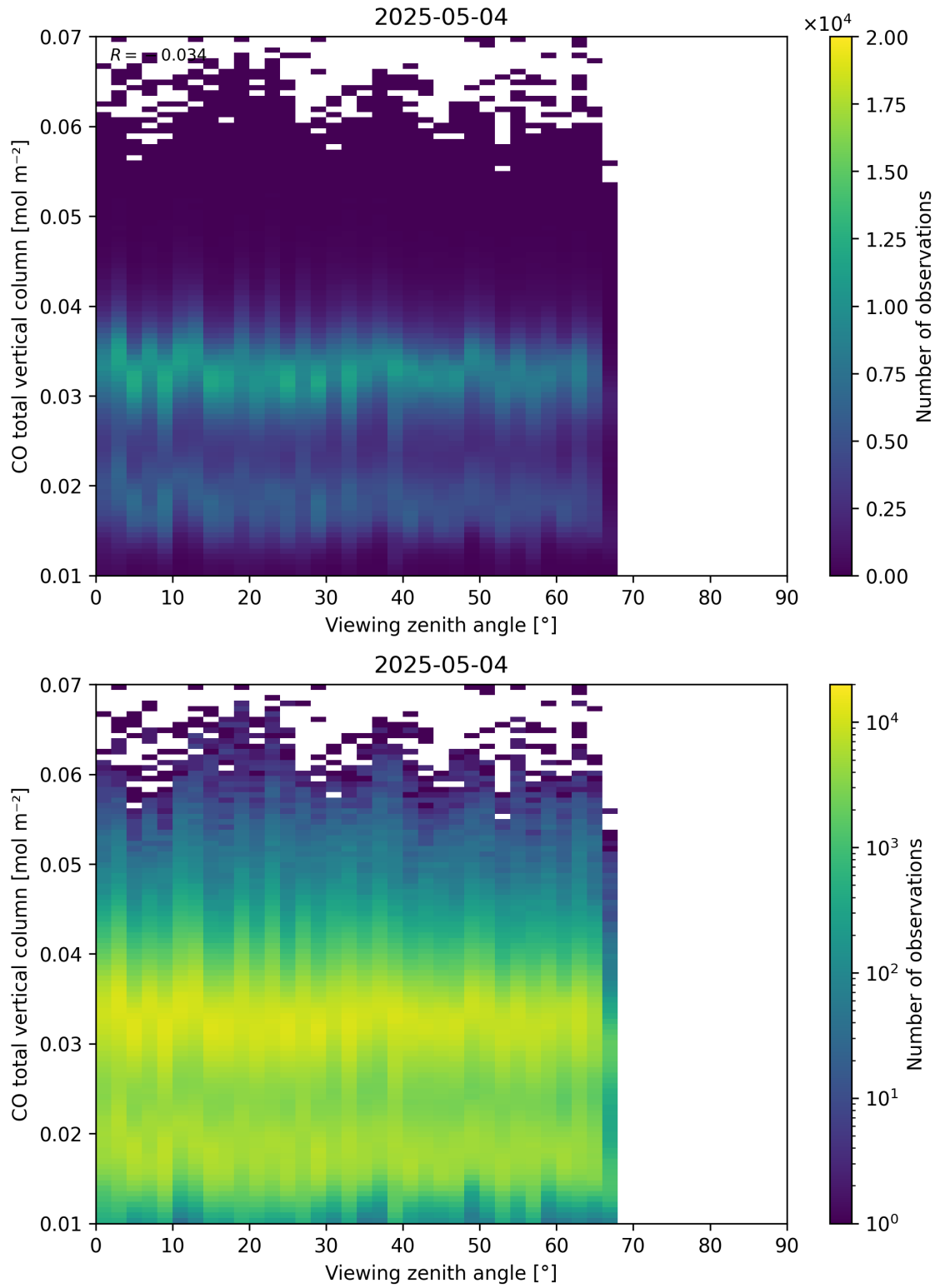
Figure 69: Scatter density plot of “Viewing zenith angle” against “CO total vertical column” for 2025-05-03 to 2025-05-05.
