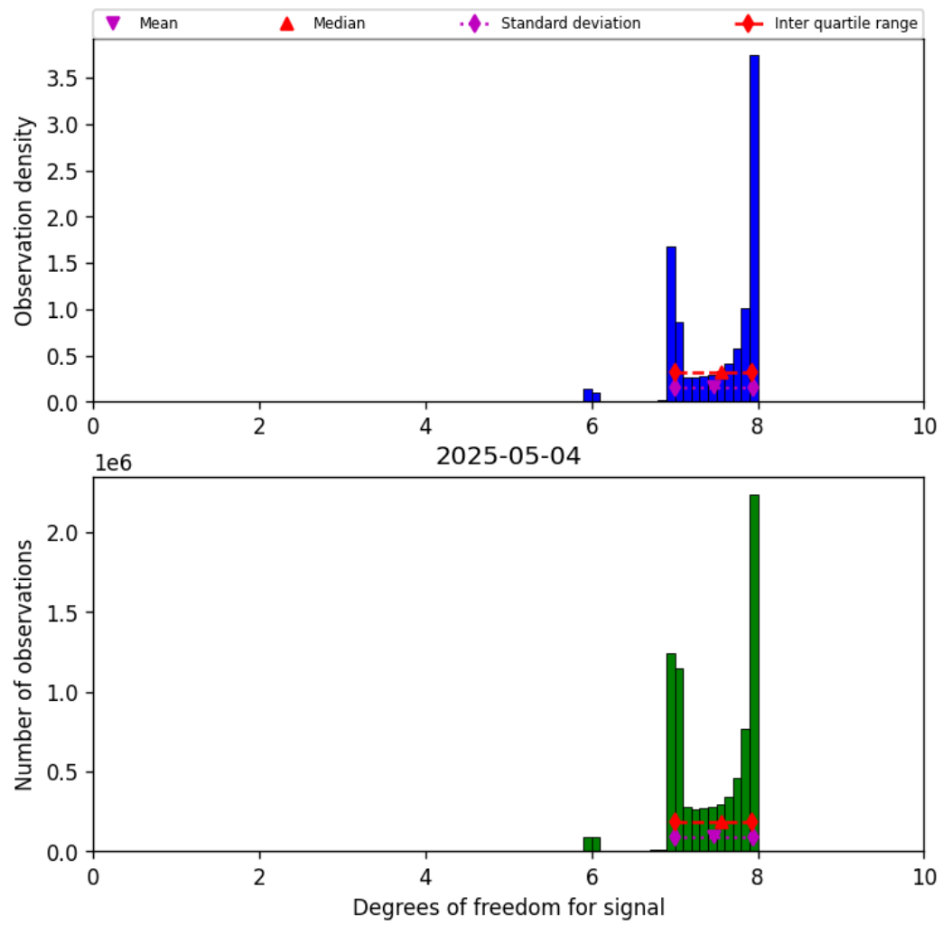
Figure 23: Histogram of “Degrees of freedom for signal” for 2025-05-03 to 2025-05-05
