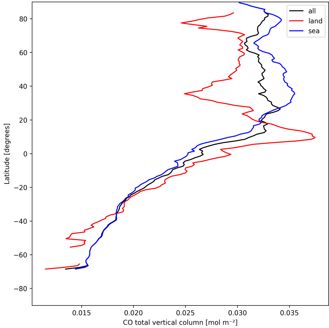
Figure 10: Zonal average of “CO total vertical column” for 2025-05-03 to 2025-05-05.
