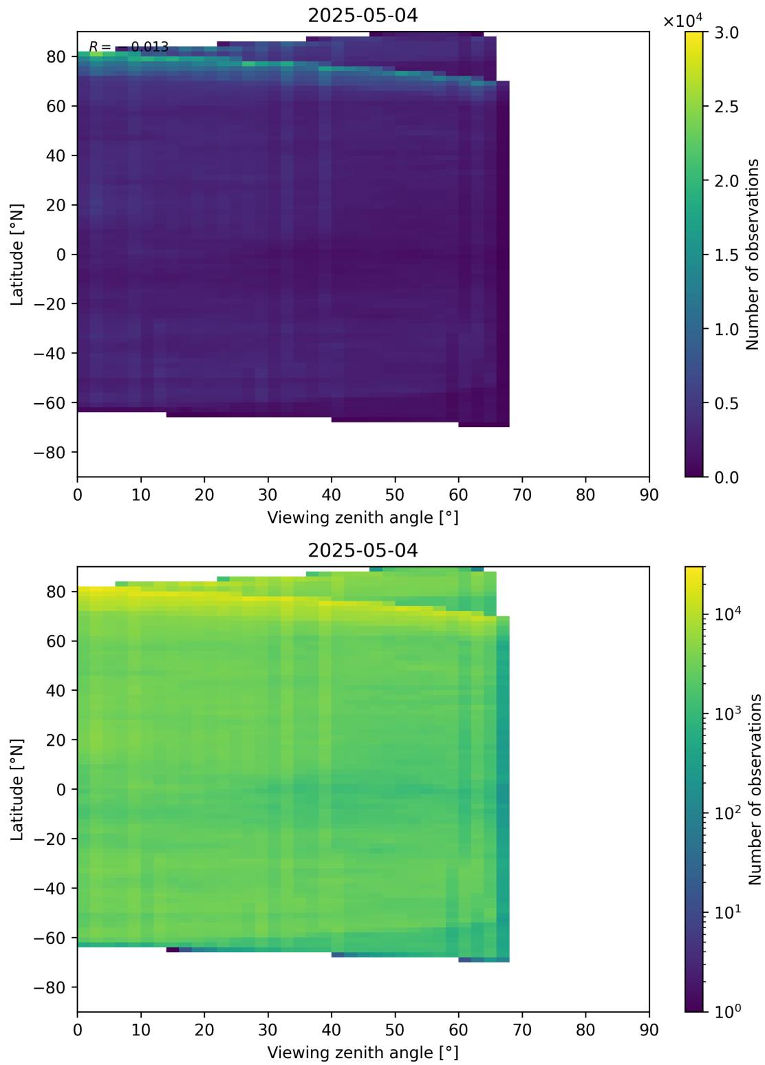
Figure 74: Scatter density plot of “Viewing zenith angle” against “Latitude” for 2025-05-03 to 2025-05-05.
