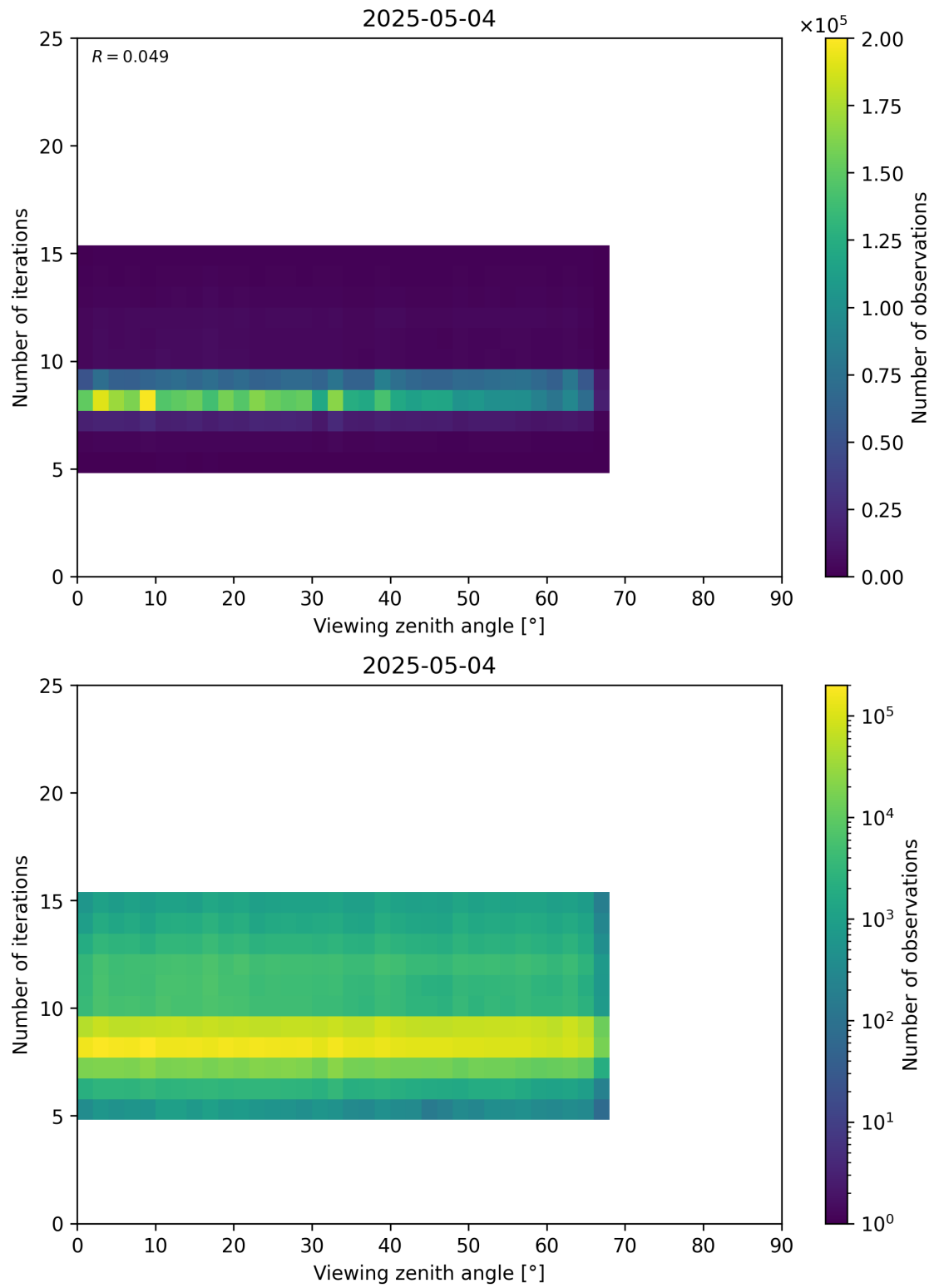
Figure 75: Scatter density plot of “Viewing zenith angle” against “Number of iterations” for 2025-05-03 to 2025-05-05.
