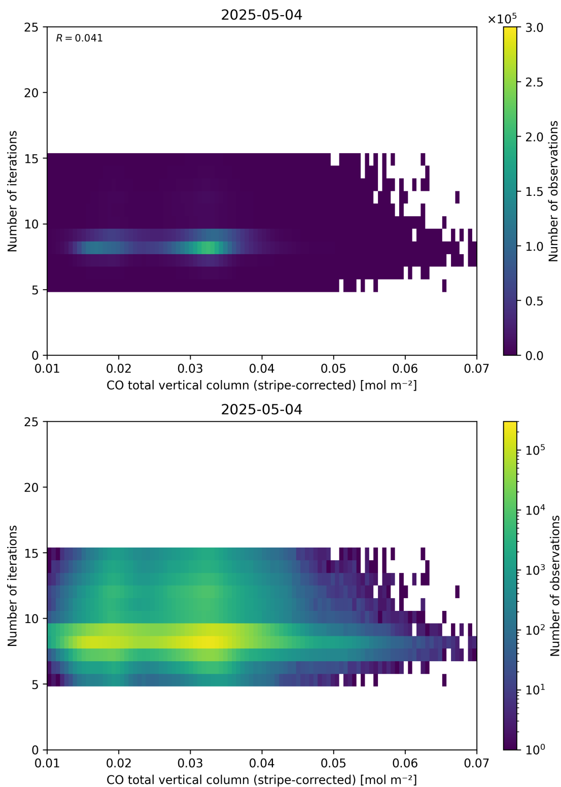
Figure 39: Scatter density plot of “CO total vertical column (stripe-corrected)” against “Number of iterations” for 2025-05-03 to 2025-05-05.
