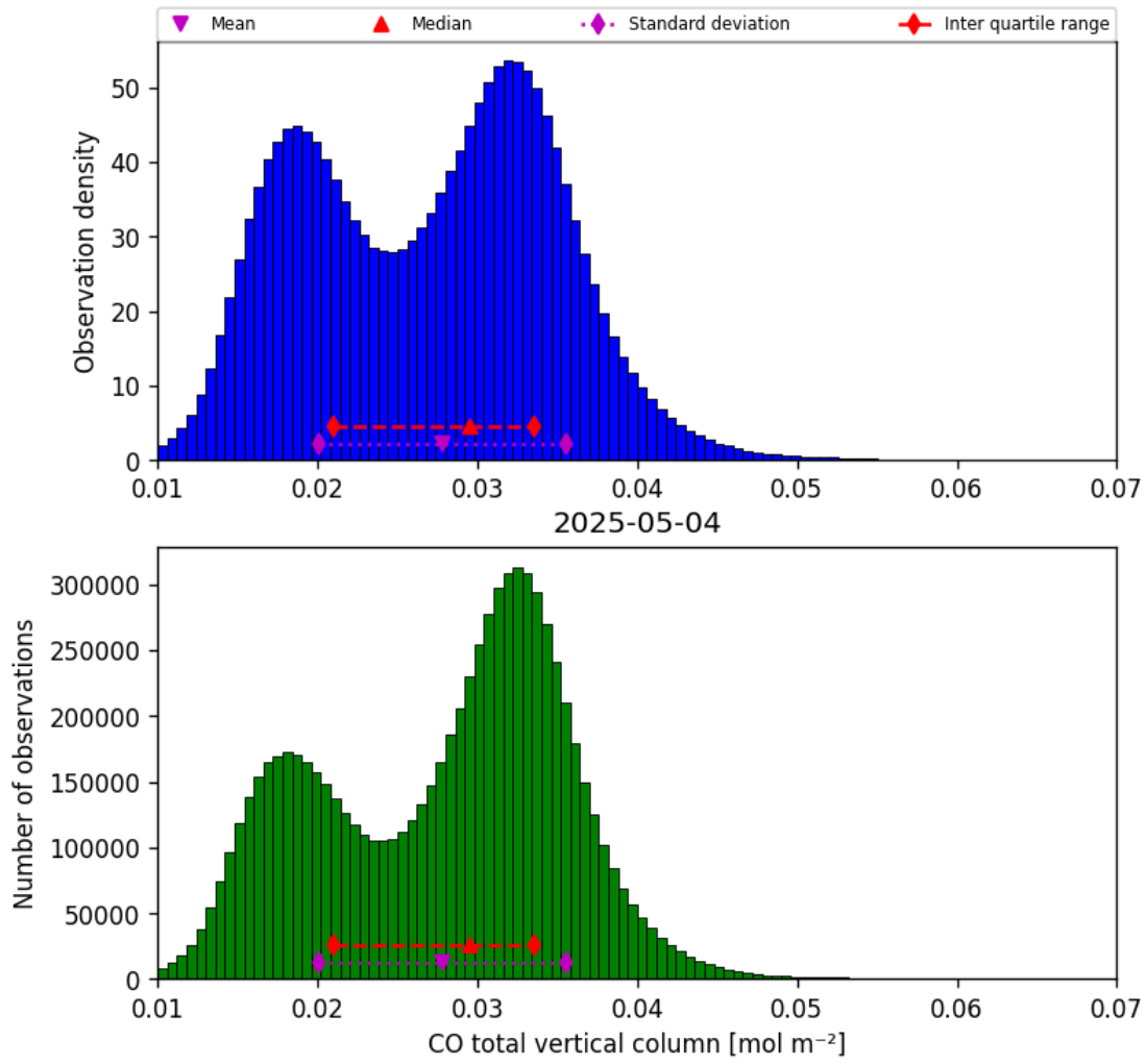
Figure 18: Histogram of “CO total vertical column” for 2025-05-03 to 2025-05-05
