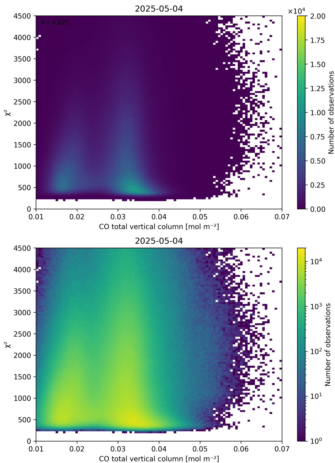
Figure 35: Scatter density plot of “CO total vertical column” against “ \chi^2 ” for 2025-05-03 to 2025-05-05.
