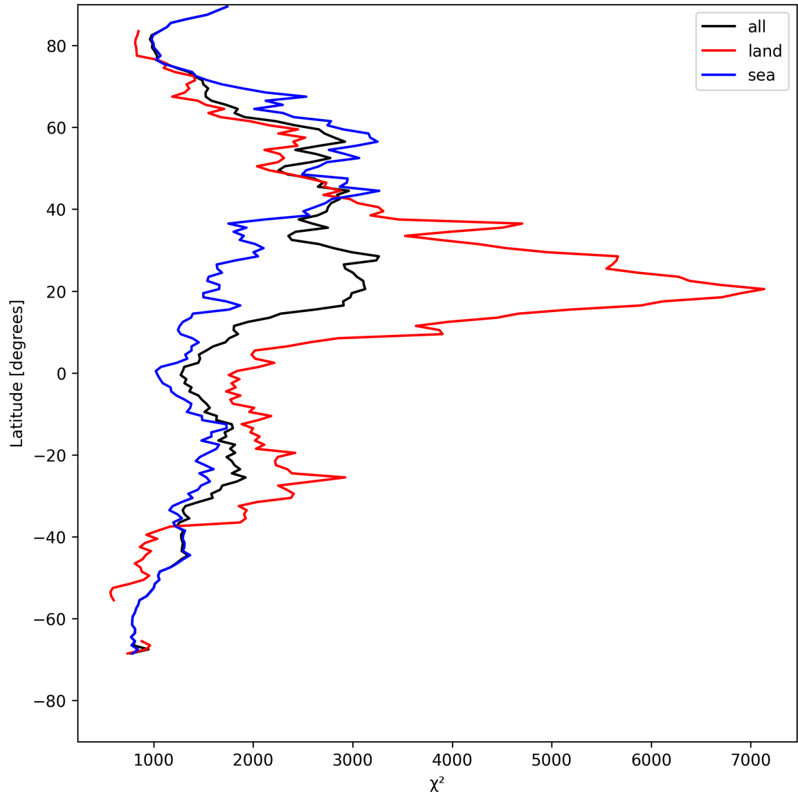
Figure 14: Zonal average of “ \chi^2 ” for 2025-05-03 to 2025-05-05.
