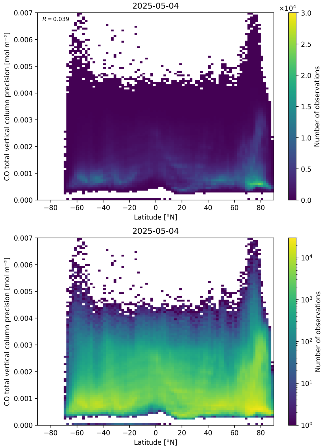
Figure 53: Scatter density plot of “Latitude” against “CO total vertical column precision” for 2025-05-03 to 2025-05-05.
