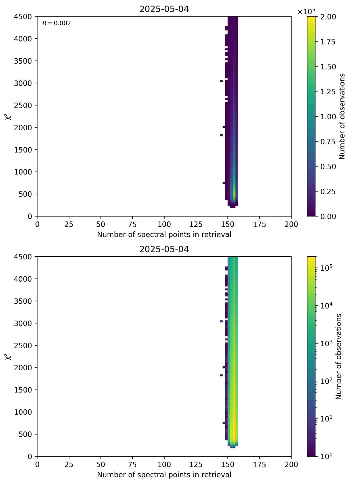
Figure 58: Scatter density plot of “Number of spectral points in retrieval” against “ \chi^2 ” for 2025-05-03 to 2025-05-05.
