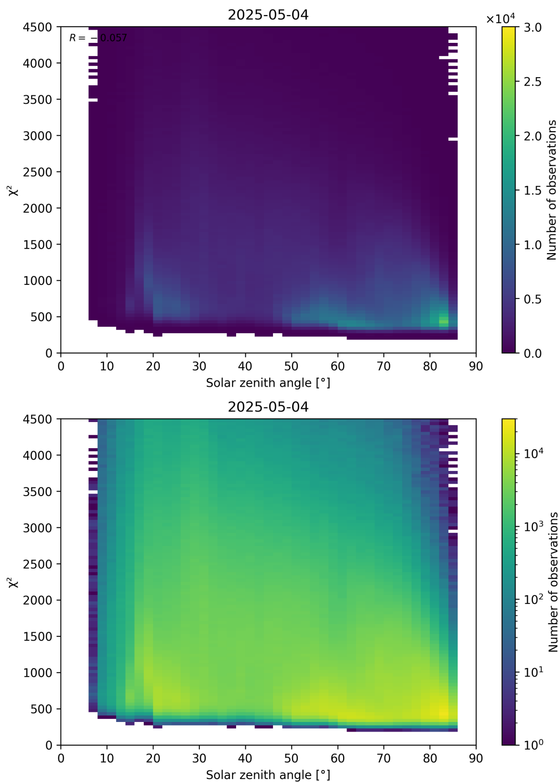
Figure 64: Scatter density plot of “Solar zenith angle” against “ \chi^2 ” for 2025-05-03 to 2025-05-05.
