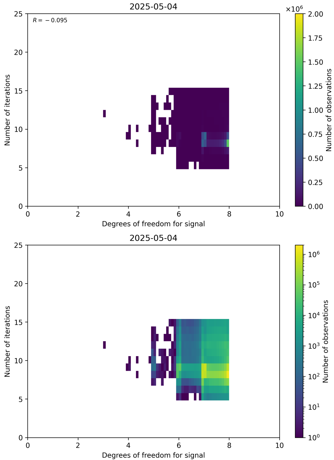
Figure 50: Scatter density plot of “Degrees of freedom for signal” against “Number of iterations” for 2025-05-03 to 2025-05-05.
