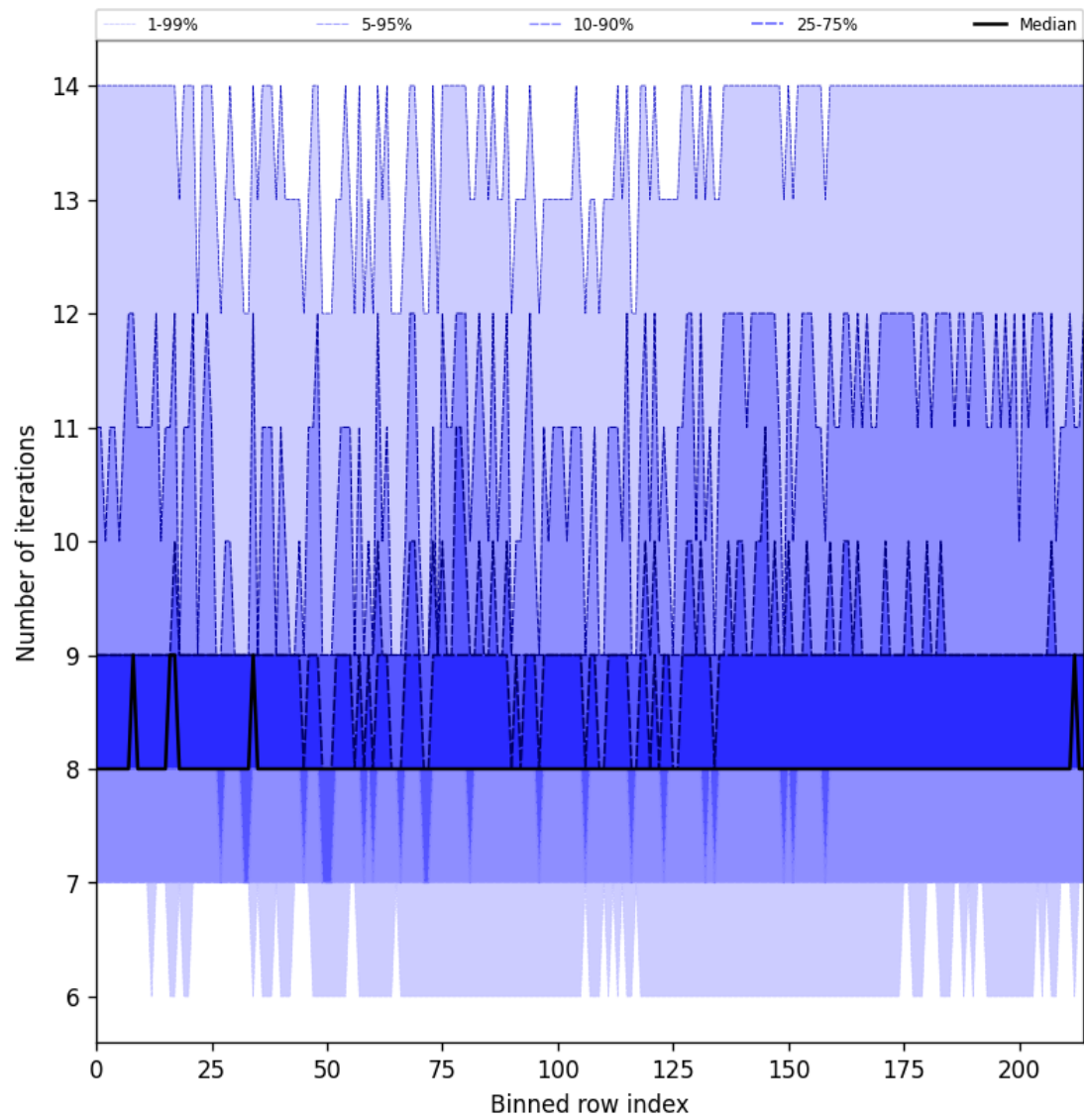
Figure 32: Along track statistics of “Number of iterations” for 2025-05-03 to 2025-05-05
