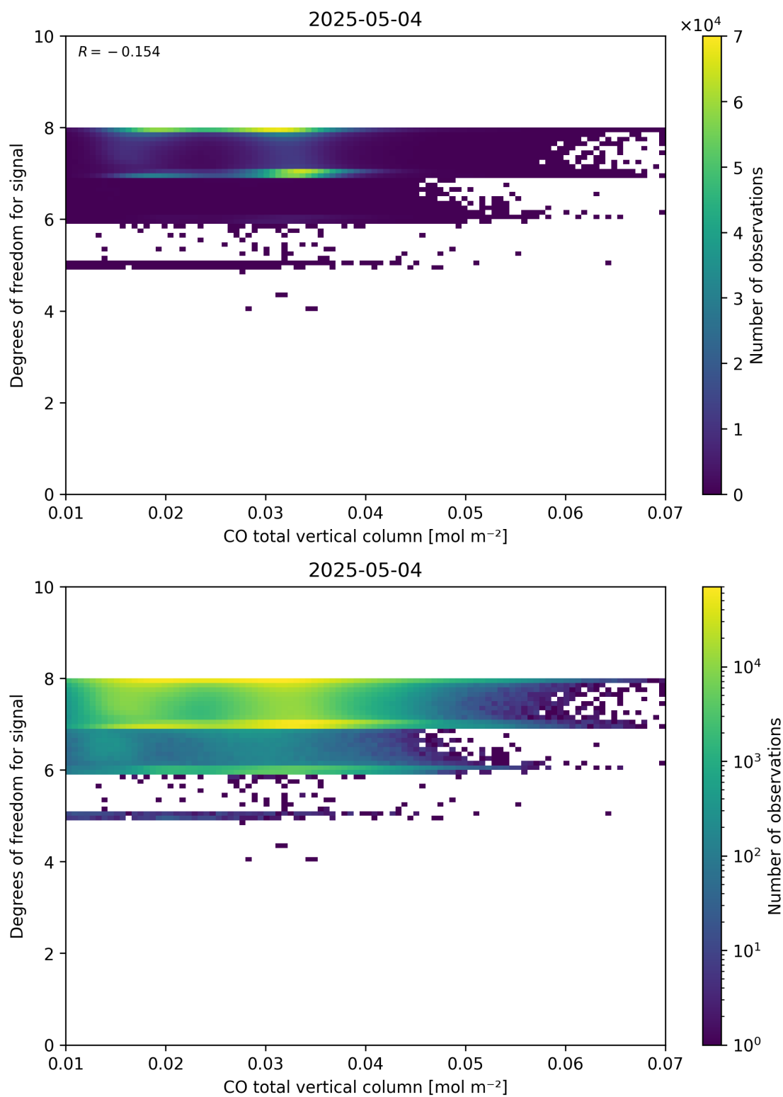
Figure 41: Scatter density plot of “CO total vertical column” against “Degrees of freedom for signal” for 2025-05-03 to 2025-05-05.
