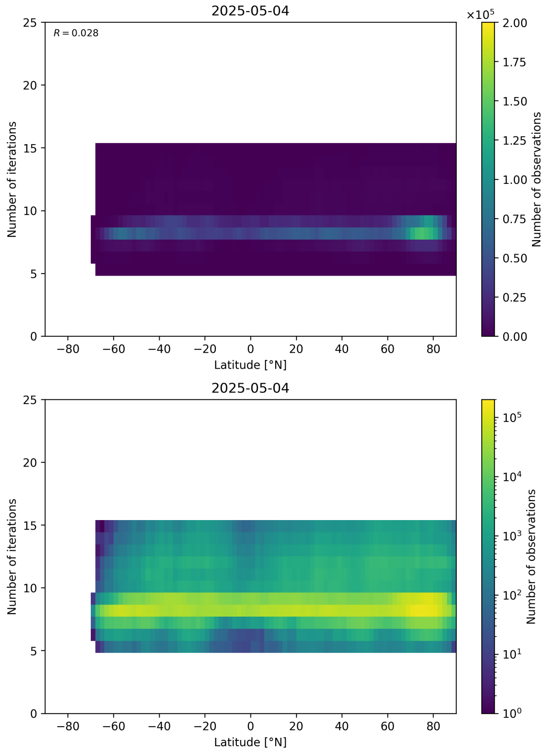
Figure 56: Scatter density plot of “Latitude” against “Number of iterations” for 2025-05-03 to 2025-05-05.
