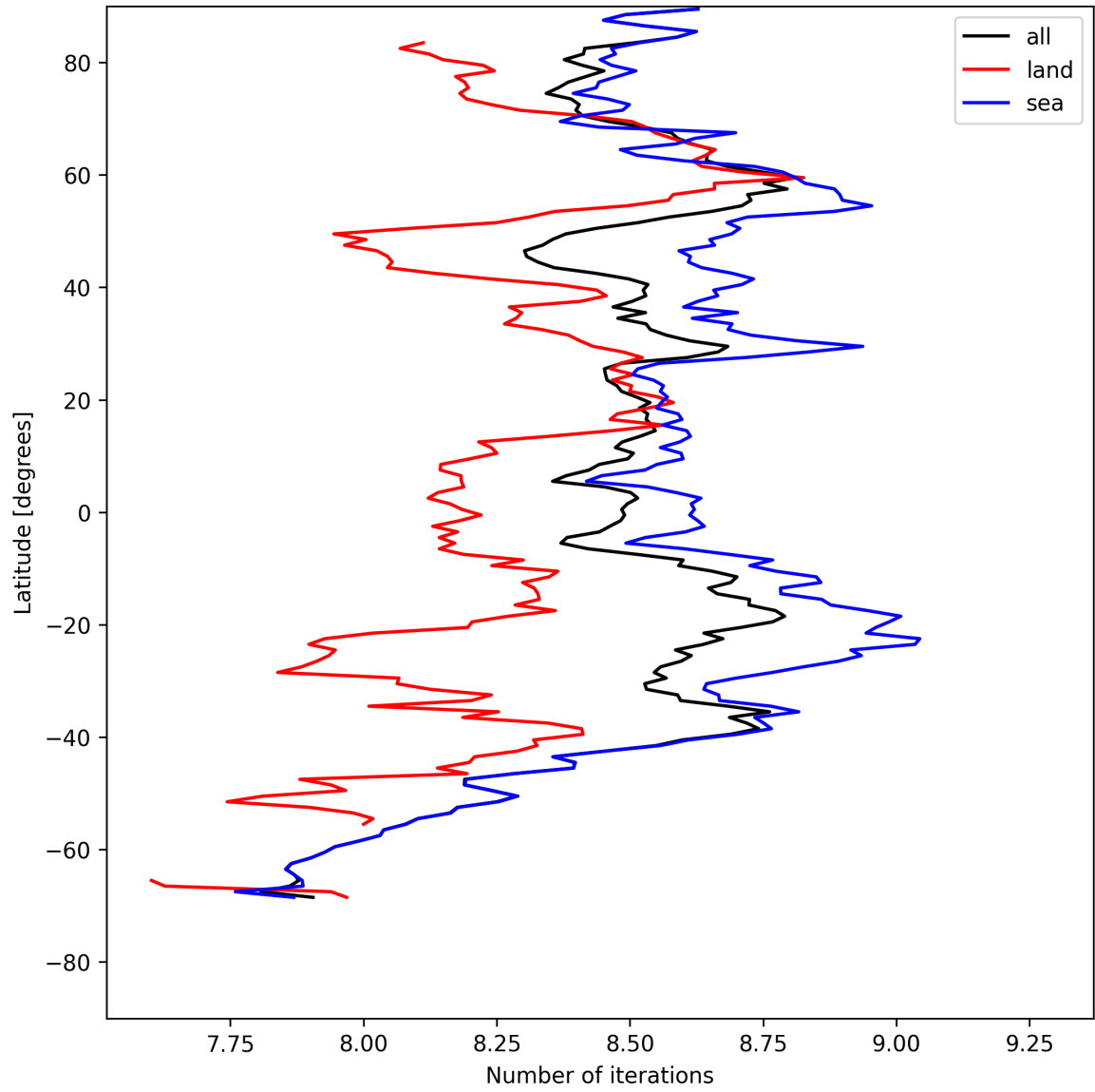
Figure 16: Zonal average of “Number of iterations” for 2025-05-03 to 2025-05-05.
