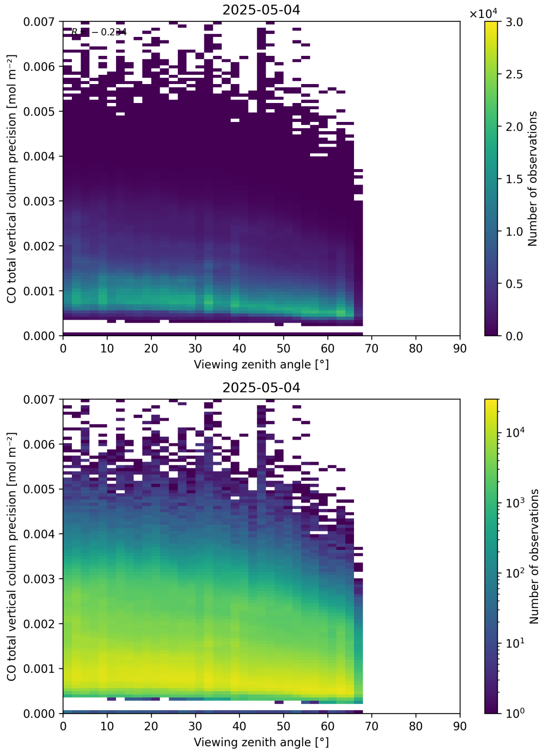
Figure 71: Scatter density plot of “Viewing zenith angle” against “CO total vertical column precision” for 2025-05-03 to 2025-05-05.
