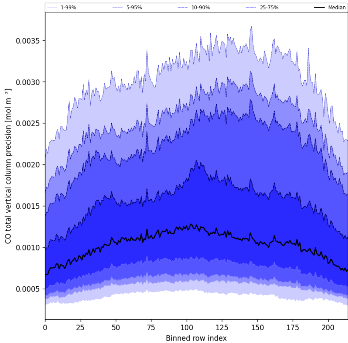
Figure 28: Along track statistics of “CO total vertical column precision” for 2025-05-03 to 2025-05-05
