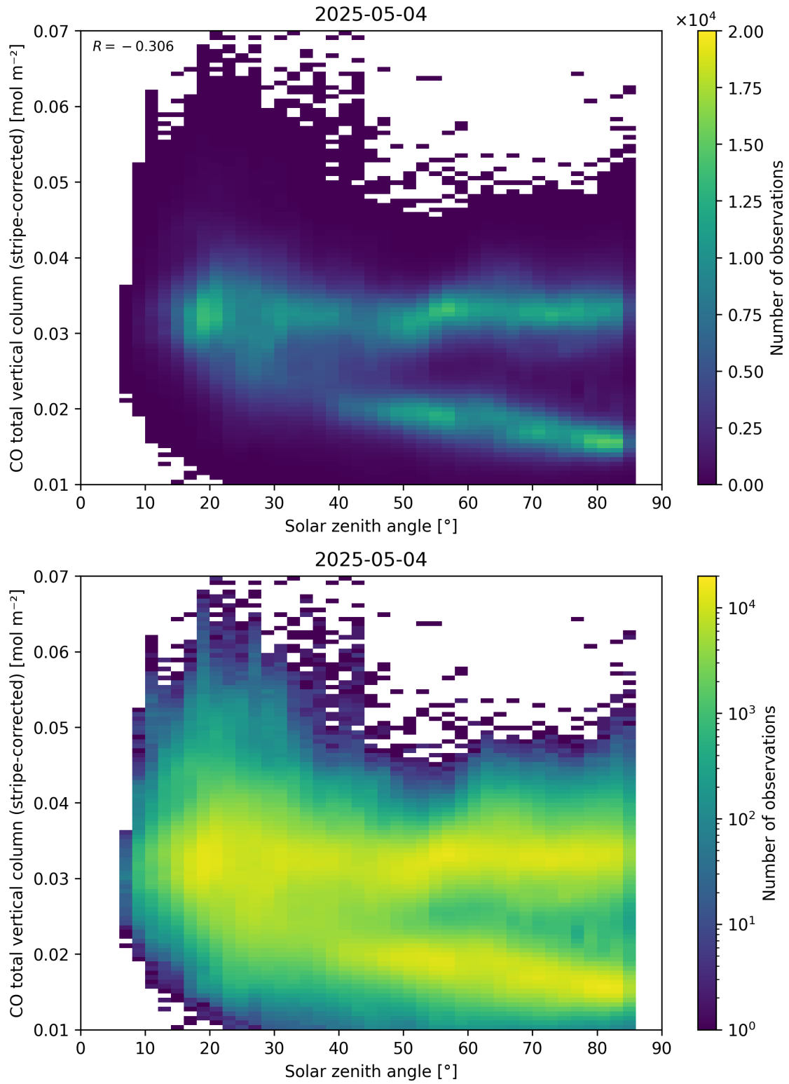
Figure 62: Scatter density plot of “Solar zenith angle” against “CO total vertical column (stripe-corrected)” for 2025-05-03 to 2025-05-05.
