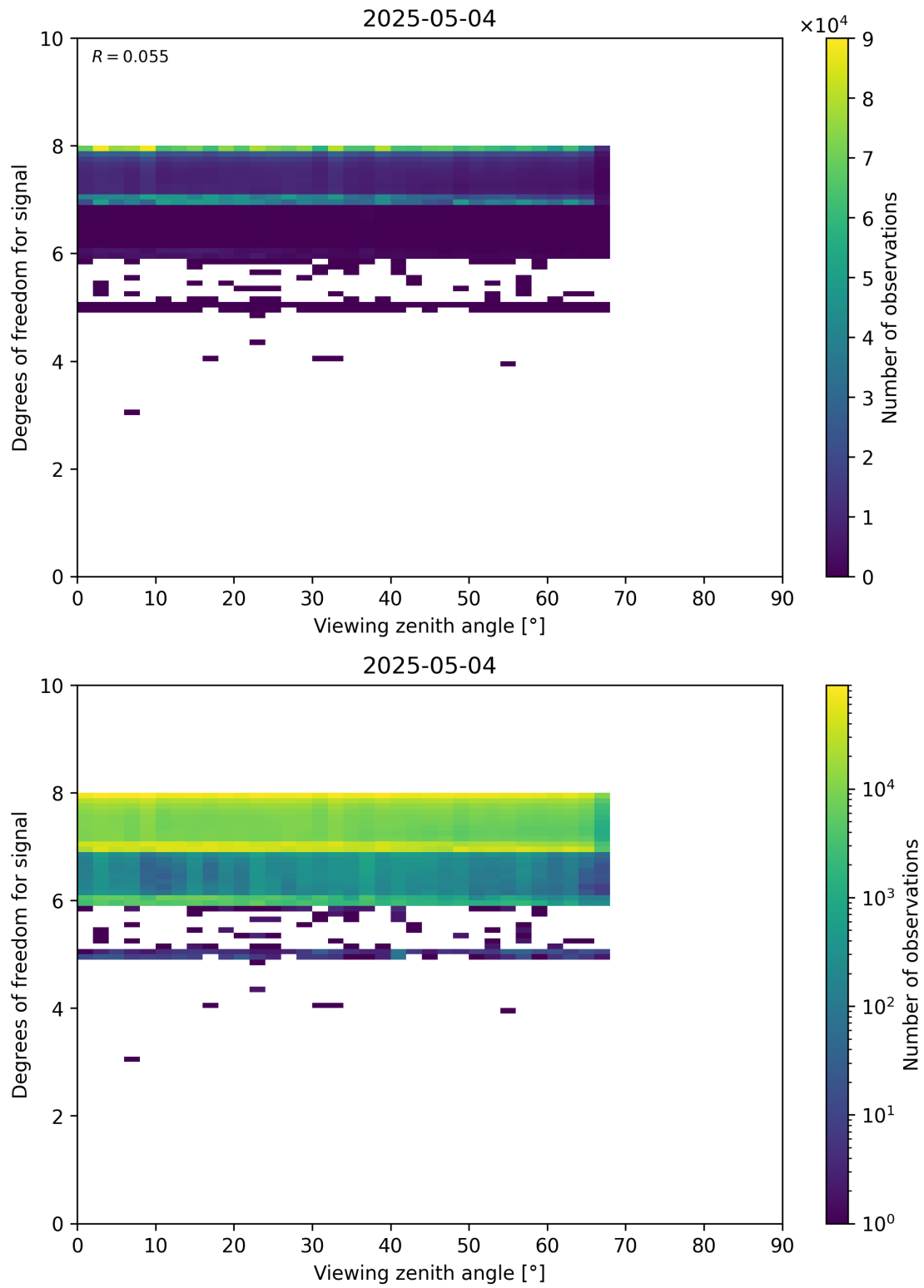
Figure 73: Scatter density plot of “Viewing zenith angle” against “Degrees of freedom for signal” for 2025-05-03 to 2025-05-05.
