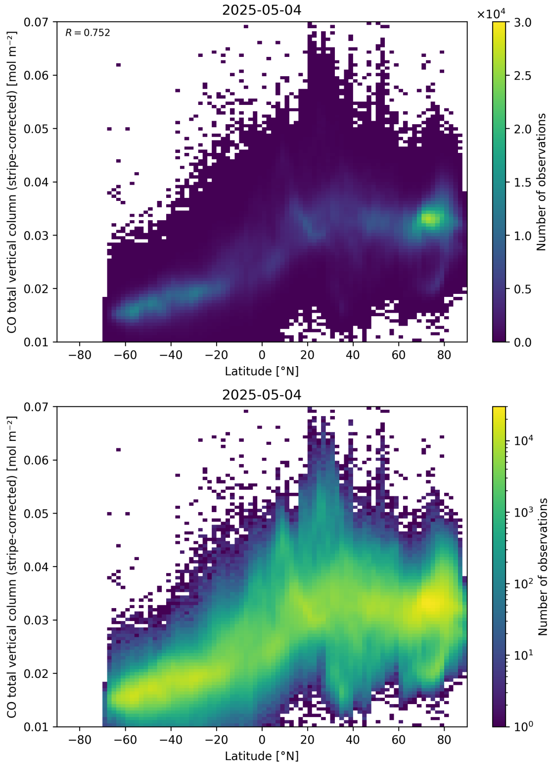
Figure 52: Scatter density plot of “Latitude” against “CO total vertical column (stripe-corrected)” for 2025-05-03 to 2025-05-05.
