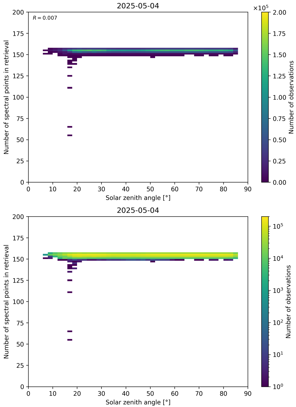
Figure 68: Scatter density plot of “Solar zenith angle” against “Number of spectral points in retrieval” for 2025-05-03 to 2025-05-05.
