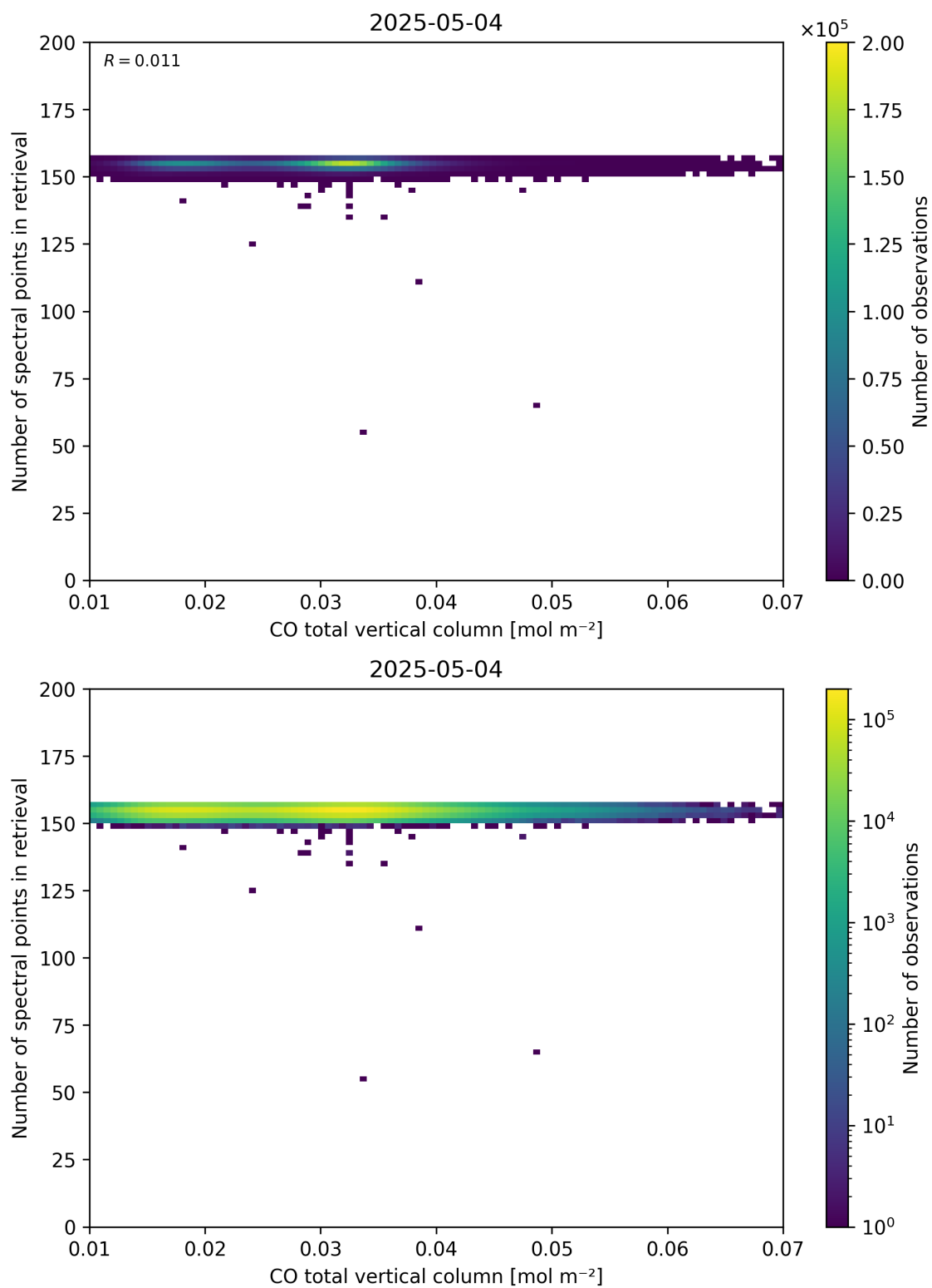
Figure 43: Scatter density plot of “CO total vertical column” against “Number of spectral points in retrieval” for 2025-05-03 to 2025-05-05.
