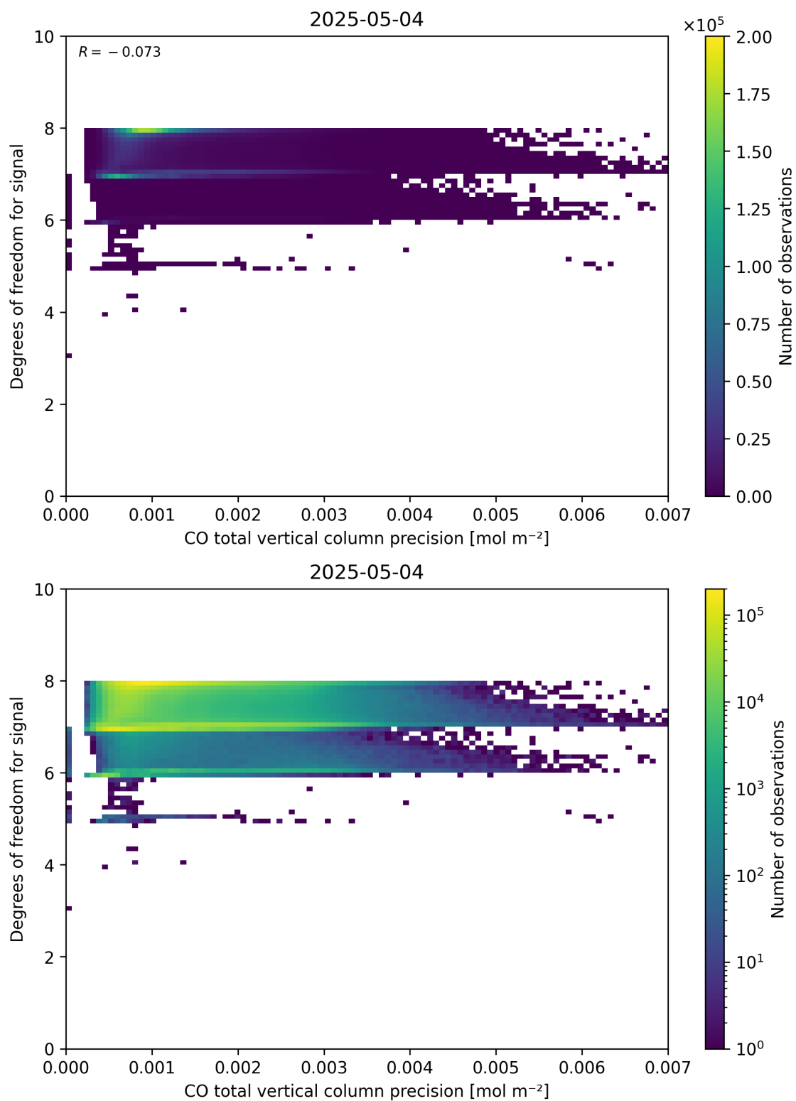
Figure 45: Scatter density plot of “CO total vertical column precision” against “Degrees of freedom for signal” for 2025-05-03 to 2025-05-05.
