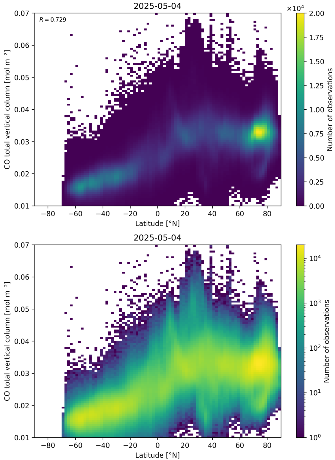
Figure 51: Scatter density plot of “Latitude” against “CO total vertical column” for 2025-05-03 to 2025-05-05.
