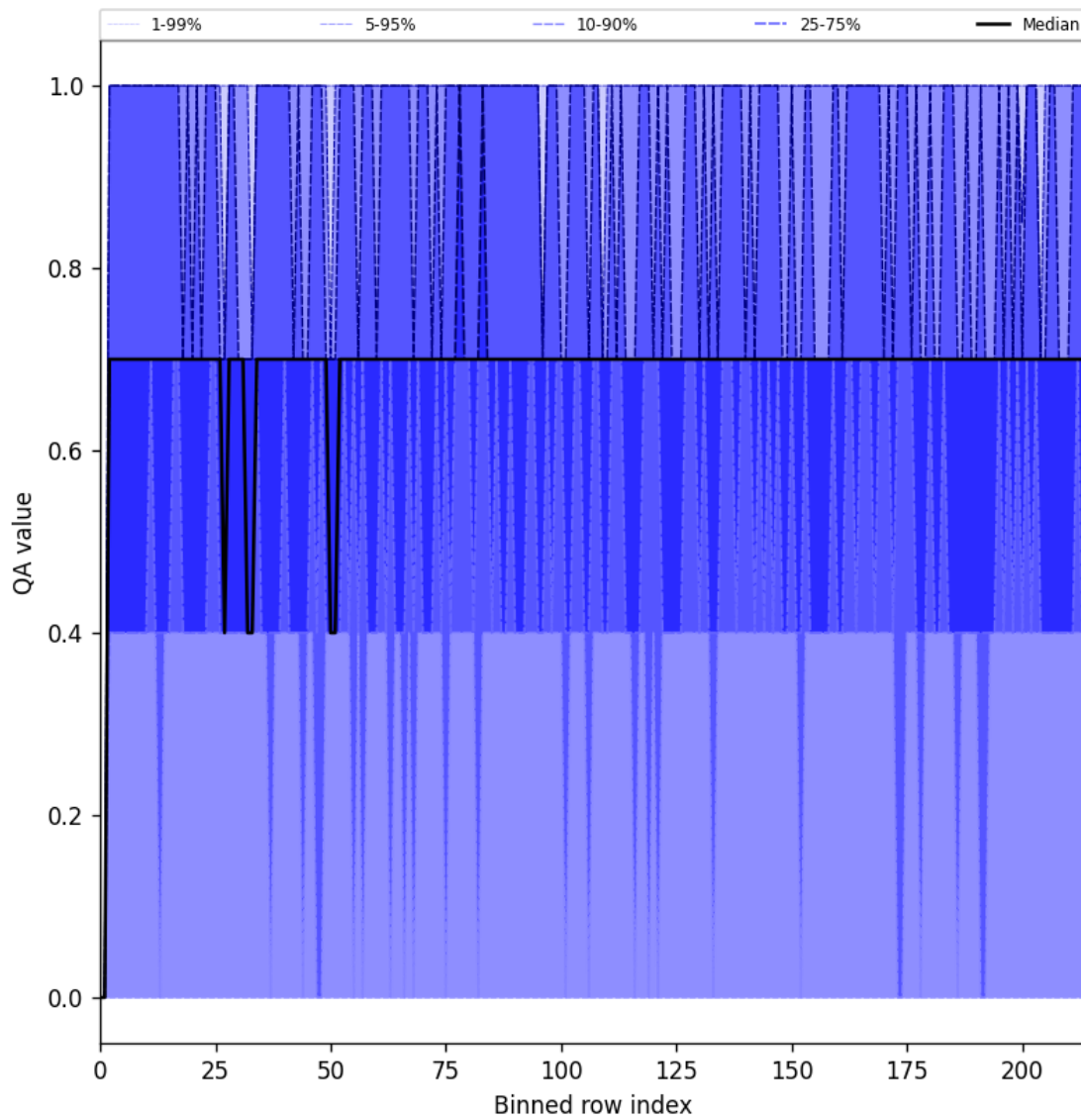
Figure 25: Along track statistics of “QA value” for 2025-05-03 to 2025-05-05
