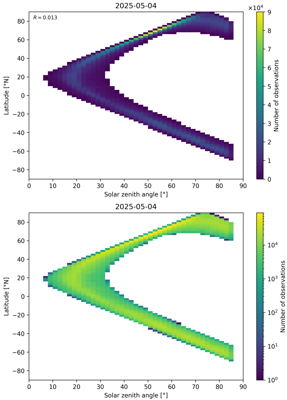
Figure 66: Scatter density plot of “Solar zenith angle” against “Latitude” for 2025-05-03 to 2025-05-05.
