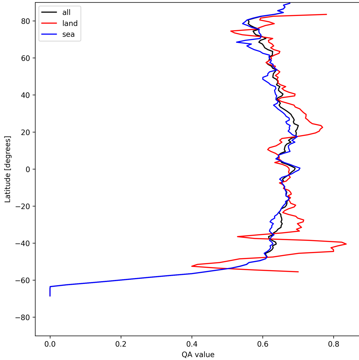
Figure 9: Zonal average of “QA value” for 2025-05-03 to 2025-05-05.
