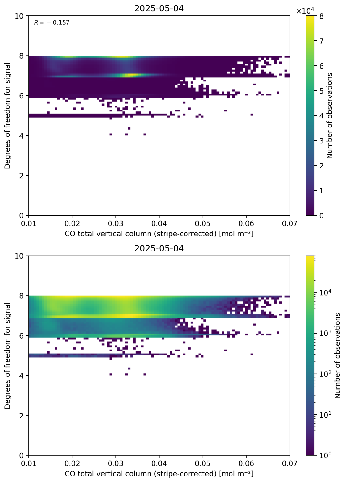
Figure 38: Scatter density plot of “CO total vertical column (stripe-corrected)” against “Degrees of freedom for signal” for 2025-05-03 to 2025-05-05.
