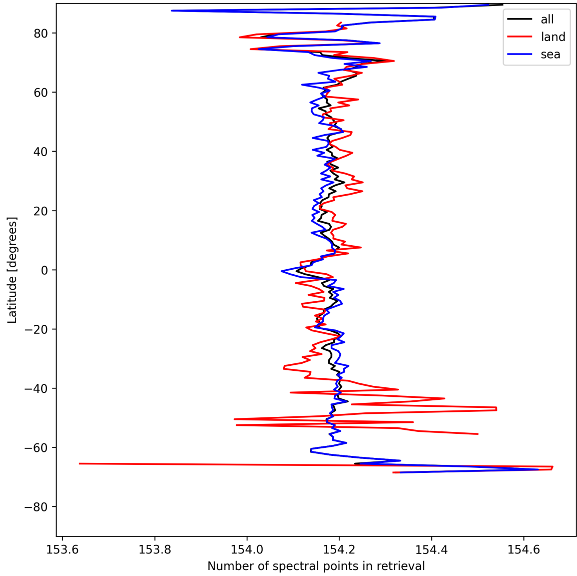
Figure 13: Zonal average of “Number of spectral points in retrieval” for 2025-05-03 to 2025-05-05.
