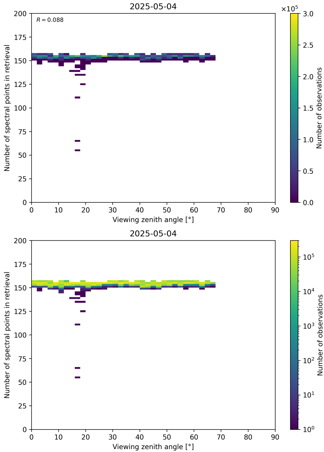
Figure 76: Scatter density plot of “Viewing zenith angle” against “Number of spectral points in retrieval” for 2025-05-03 to 2025-05-05.
