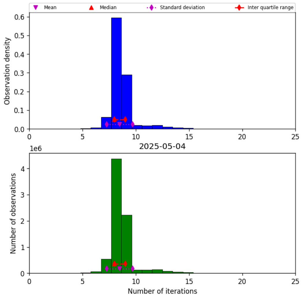
Figure 24: Histogram of “Number of iterations” for 2025-05-03 to 2025-05-05
