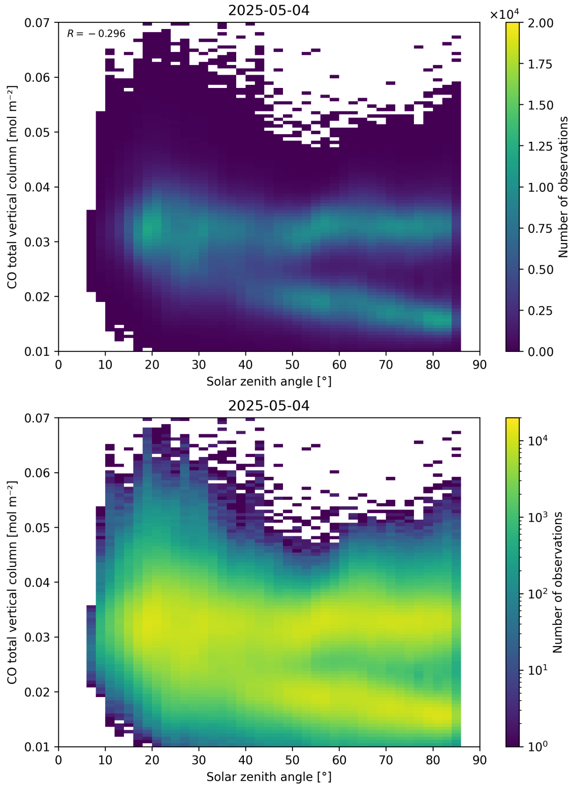
Figure 61: Scatter density plot of “Solar zenith angle” against “CO total vertical column” for 2025-05-03 to 2025-05-05.
