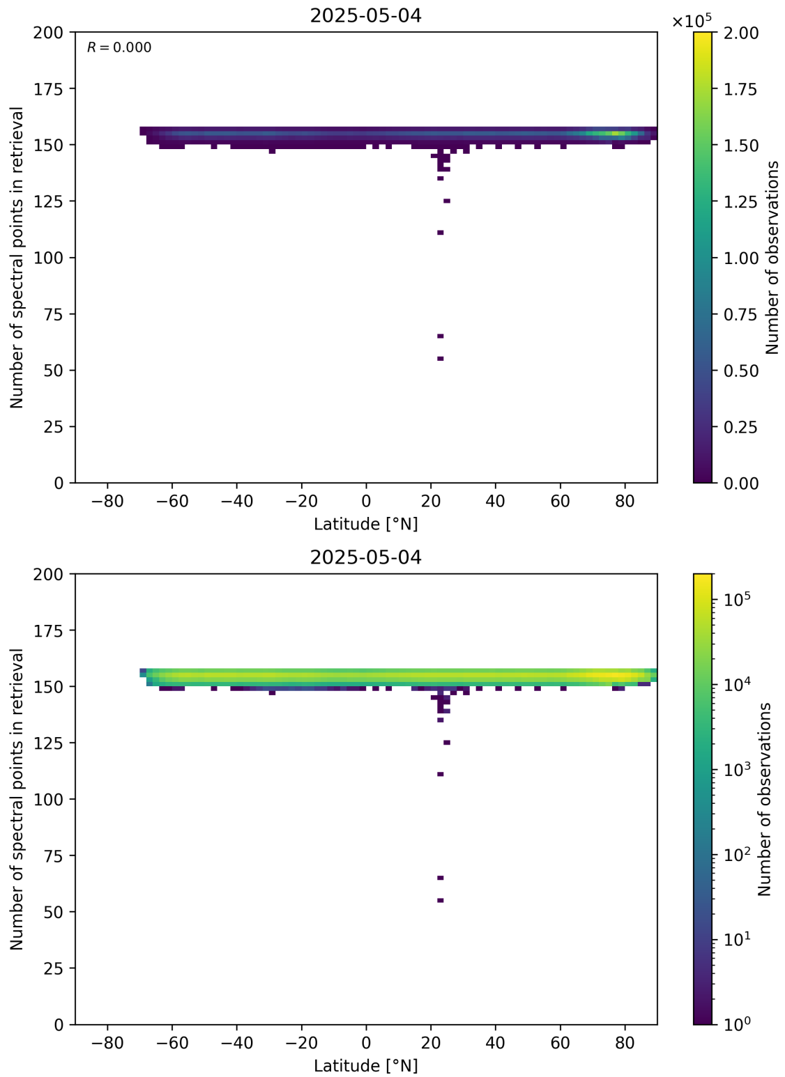
Figure 57: Scatter density plot of “Latitude” against “Number of spectral points in retrieval” for 2025-05-03 to 2025-05-05.
