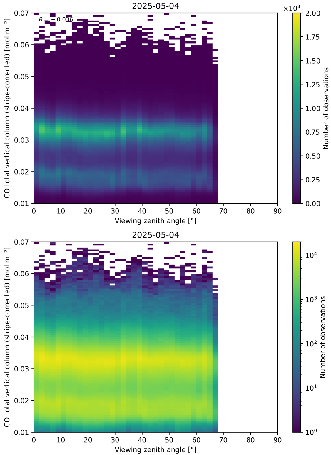
Figure 70: Scatter density plot of “Viewing zenith angle” against “CO total vertical column (stripe-corrected)” for 2025-05-03 to 2025-05-05.
