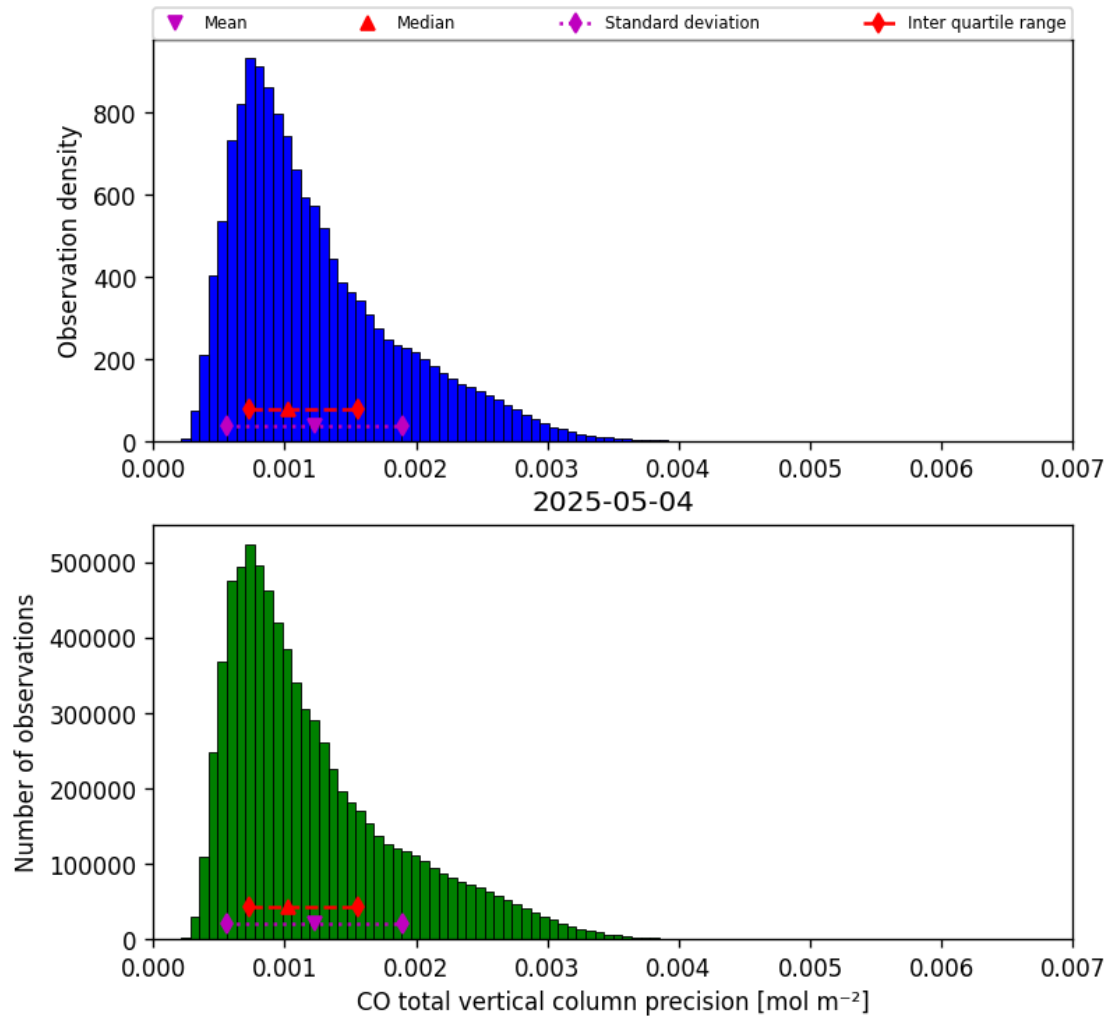
Figure 20: Histogram of “CO total vertical column precision” for 2025-05-03 to 2025-05-05
