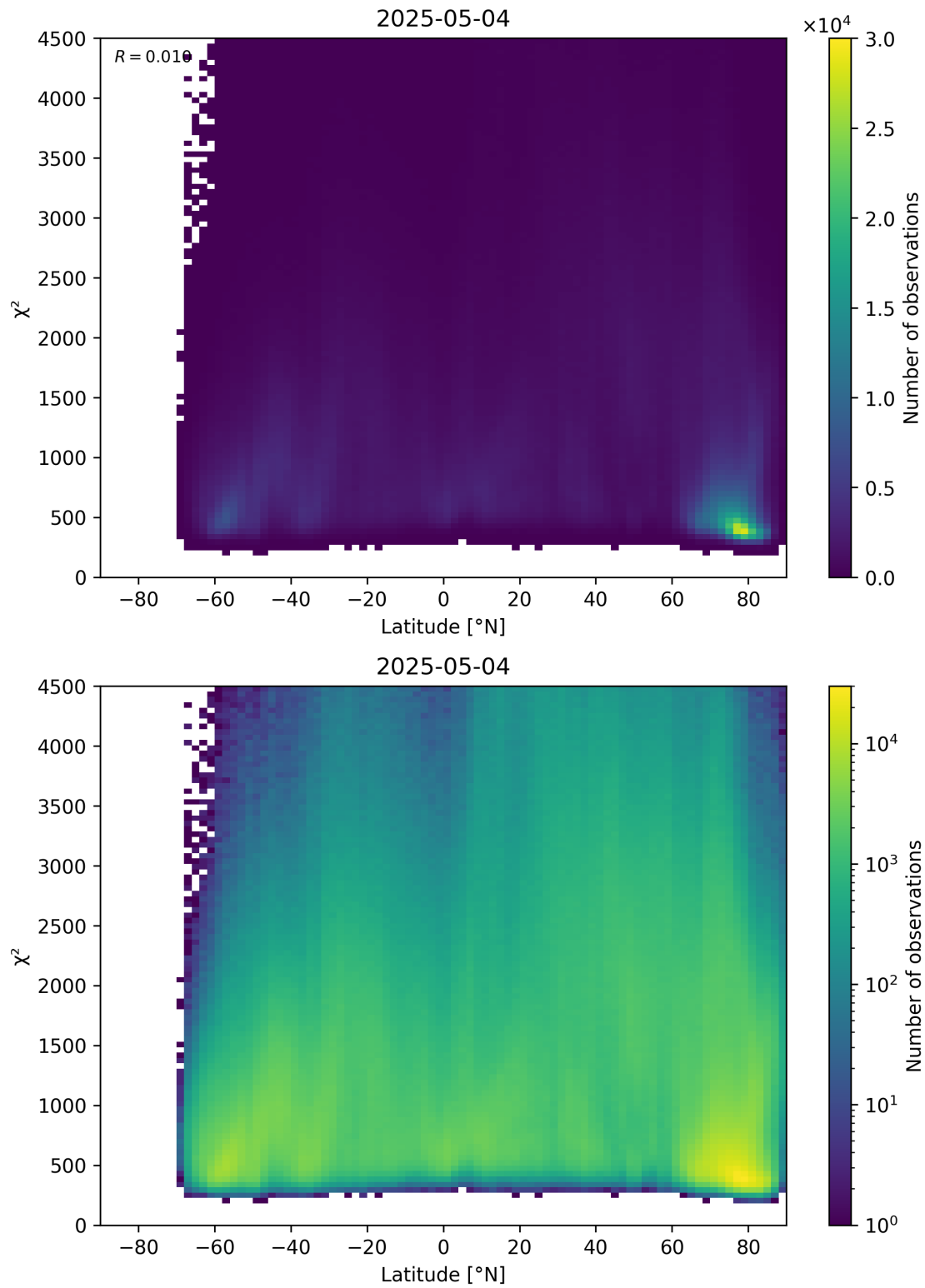
Figure 54: Scatter density plot of “Latitude” against “ \chi^2 ” for 2025-05-03 to 2025-05-05.
