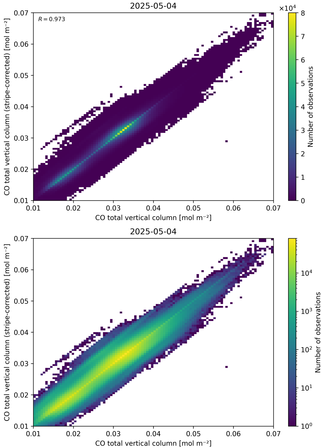
Figure 33: Scatter density plot of “CO total vertical column” against “CO total vertical column (stripe-corrected)” for 2025-05-03 to 2025-05-05.
