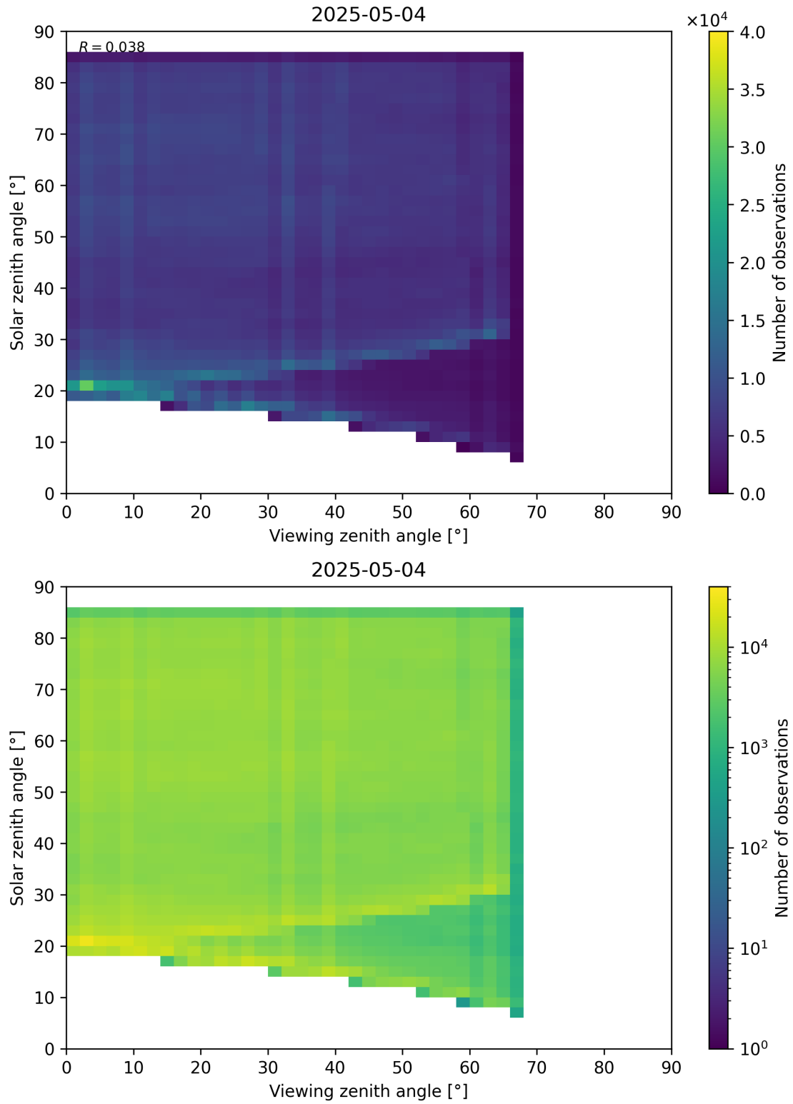
Figure 77: Scatter density plot of “Viewing zenith angle” against “Solar zenith angle” for 2025-05-03 to 2025-05-05.
