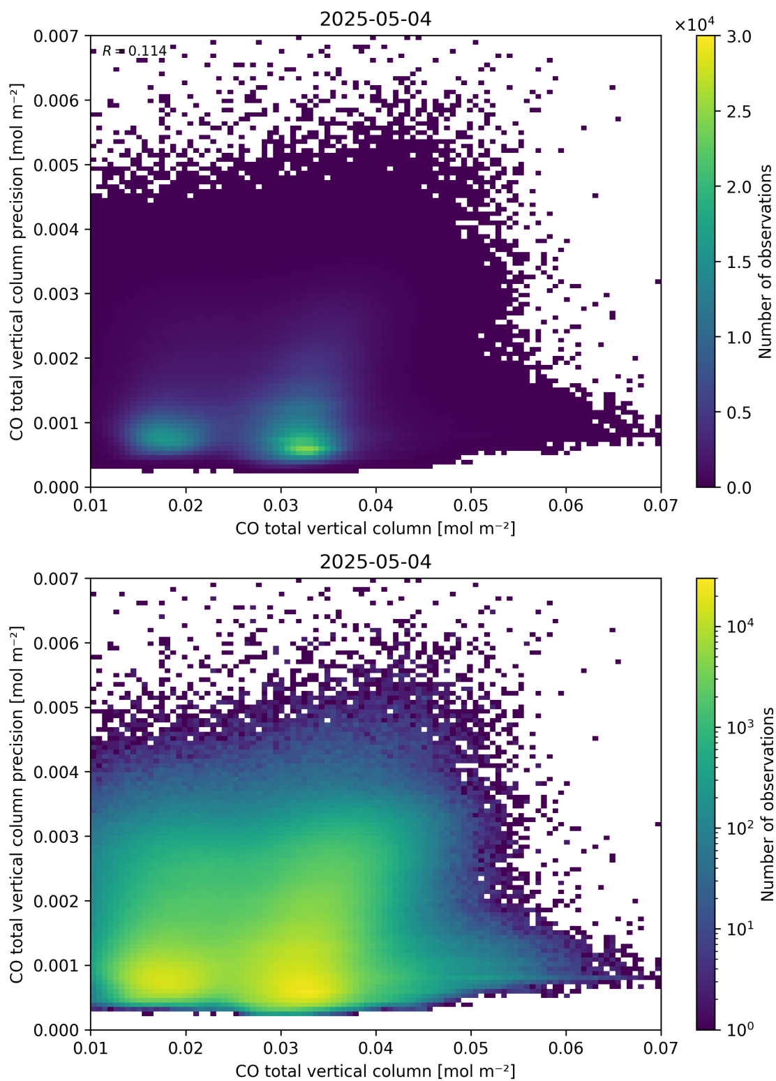
Figure 34: Scatter density plot of “CO total vertical column” against “CO total vertical column precision” for 2025-05-03 to 2025-05-05.
