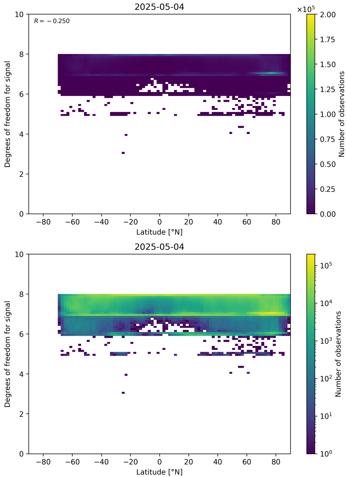
Figure 55: Scatter density plot of “Latitude” against “Degrees of freedom for signal” for 2025-05-03 to 2025-05-05.
