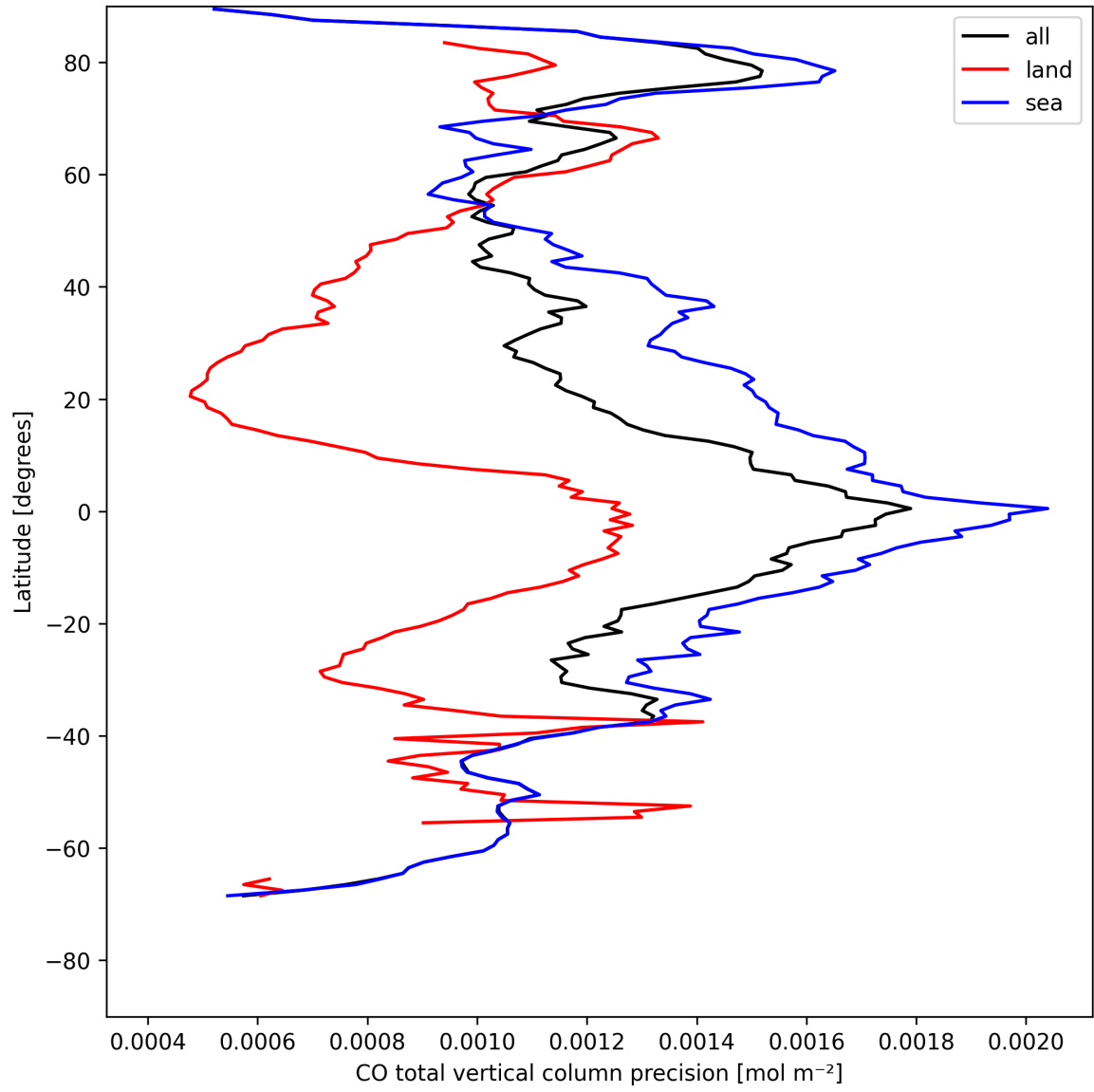
Figure 12: Zonal average of “CO total vertical column precision” for 2025-05-03 to 2025-05-05.
