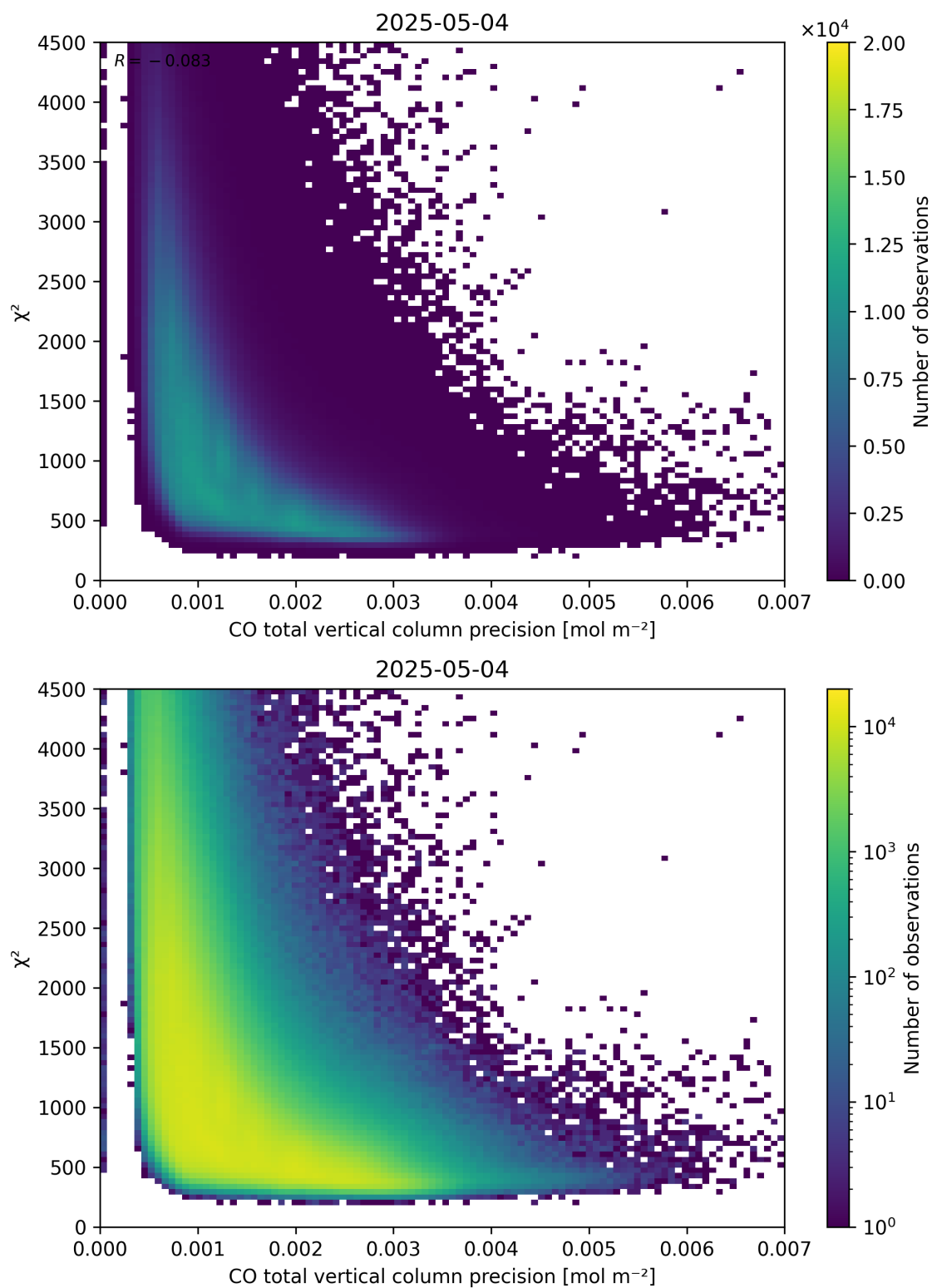
Figure 44: Scatter density plot of “CO total vertical column precision” against “ \chi^2 ” for 2025-05-03 to 2025-05-05.
