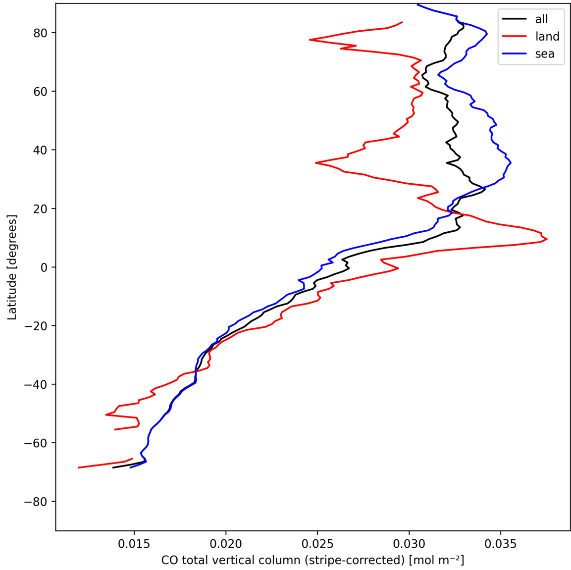
Figure 11: Zonal average of “CO total vertical column (stripe-corrected)” for 2025-05-03 to 2025-05-05.
