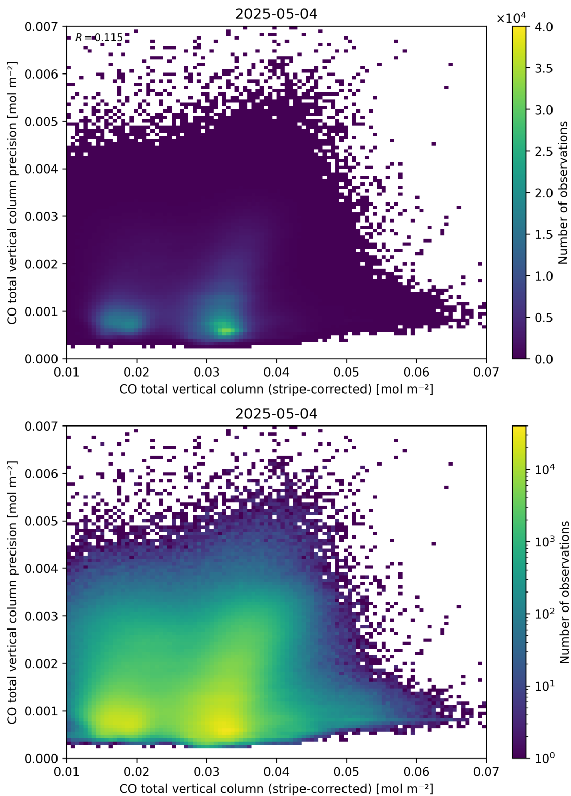
Figure 36: Scatter density plot of “CO total vertical column (stripe-corrected)” against “CO total vertical column precision” for 2025-05-03 to 2025-05-05.
