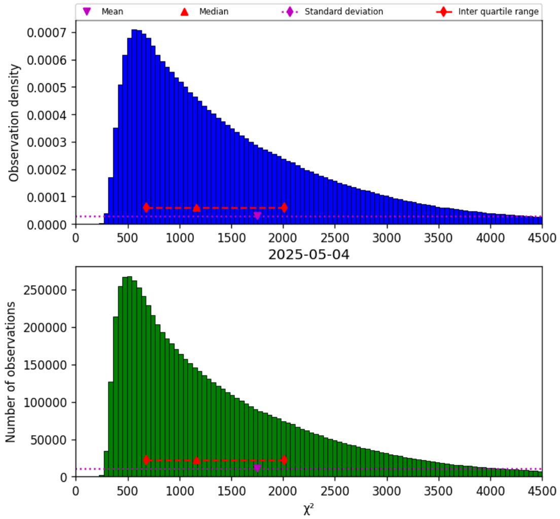
Figure 22: Histogram of “ \chi^2 ” for 2025-05-03 to 2025-05-05
