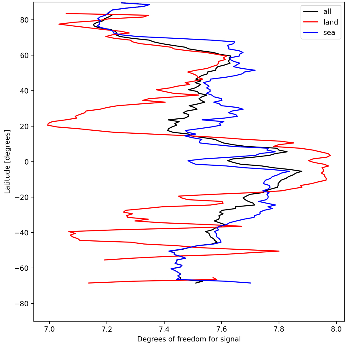
Figure 15: Zonal average of “Degrees of freedom for signal” for 2025-05-03 to 2025-05-05.
