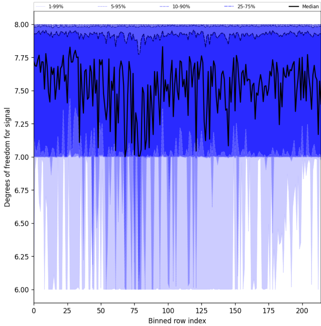
Figure 31: Along track statistics of “Degrees of freedom for signal” for 2025-05-03 to 2025-05-05
