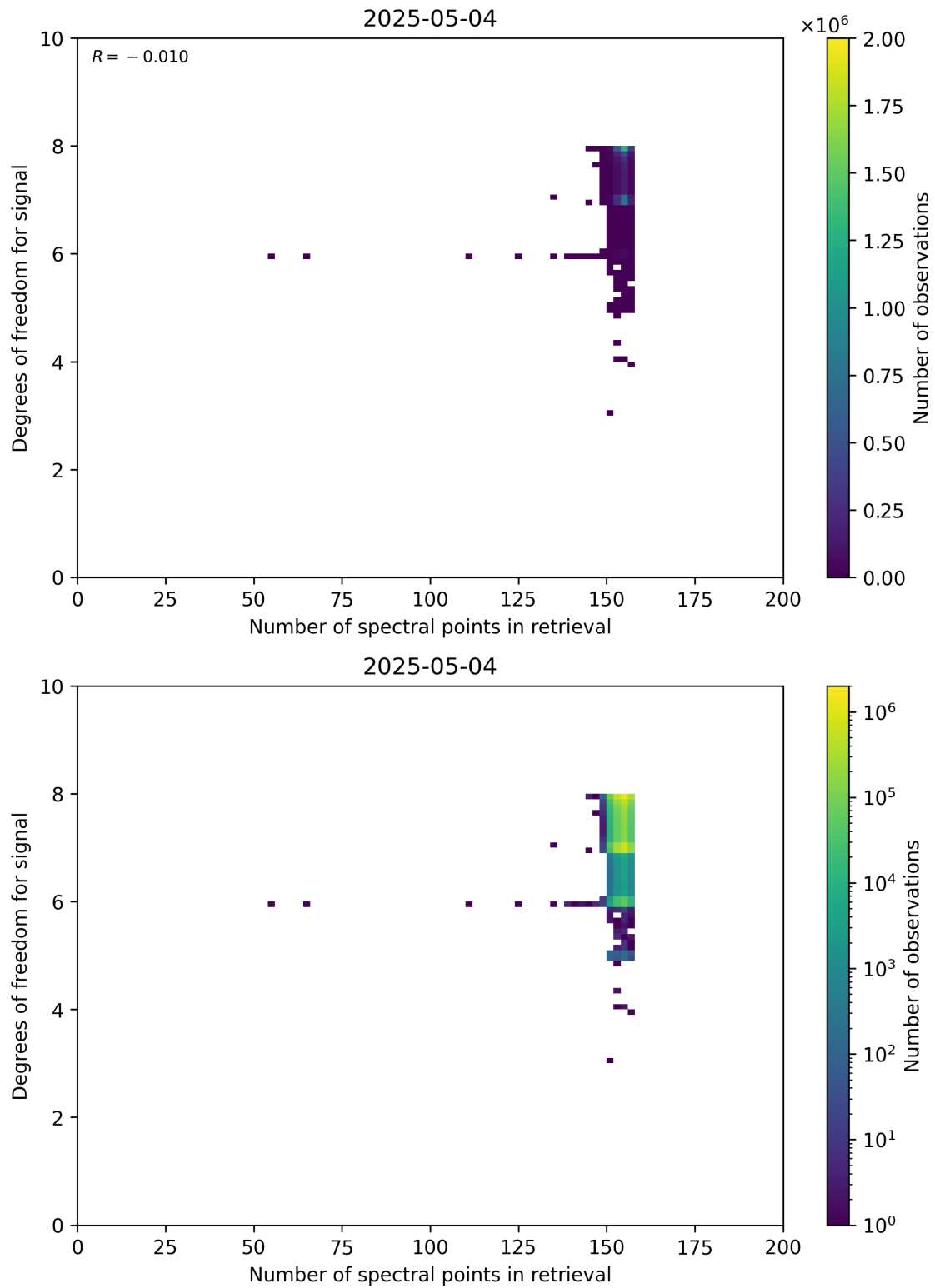
Figure 59: Scatter density plot of “Number of spectral points in retrieval” against “Degrees of freedom for signal” for 2025-05-03 to 2025-05-05.
