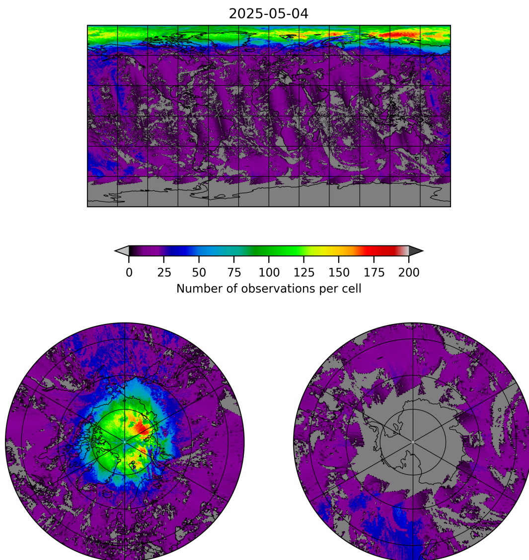
Figure 8: Map of the number of observations for 2025-05-03 to 2025-05-05
