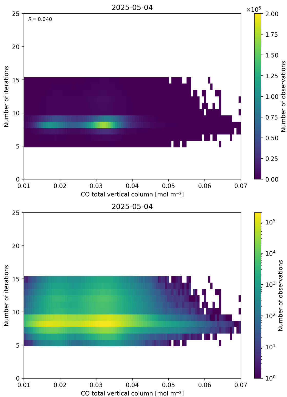
Figure 42: Scatter density plot of “CO total vertical column” against “Number of iterations” for 2025-05-03 to 2025-05-05.
