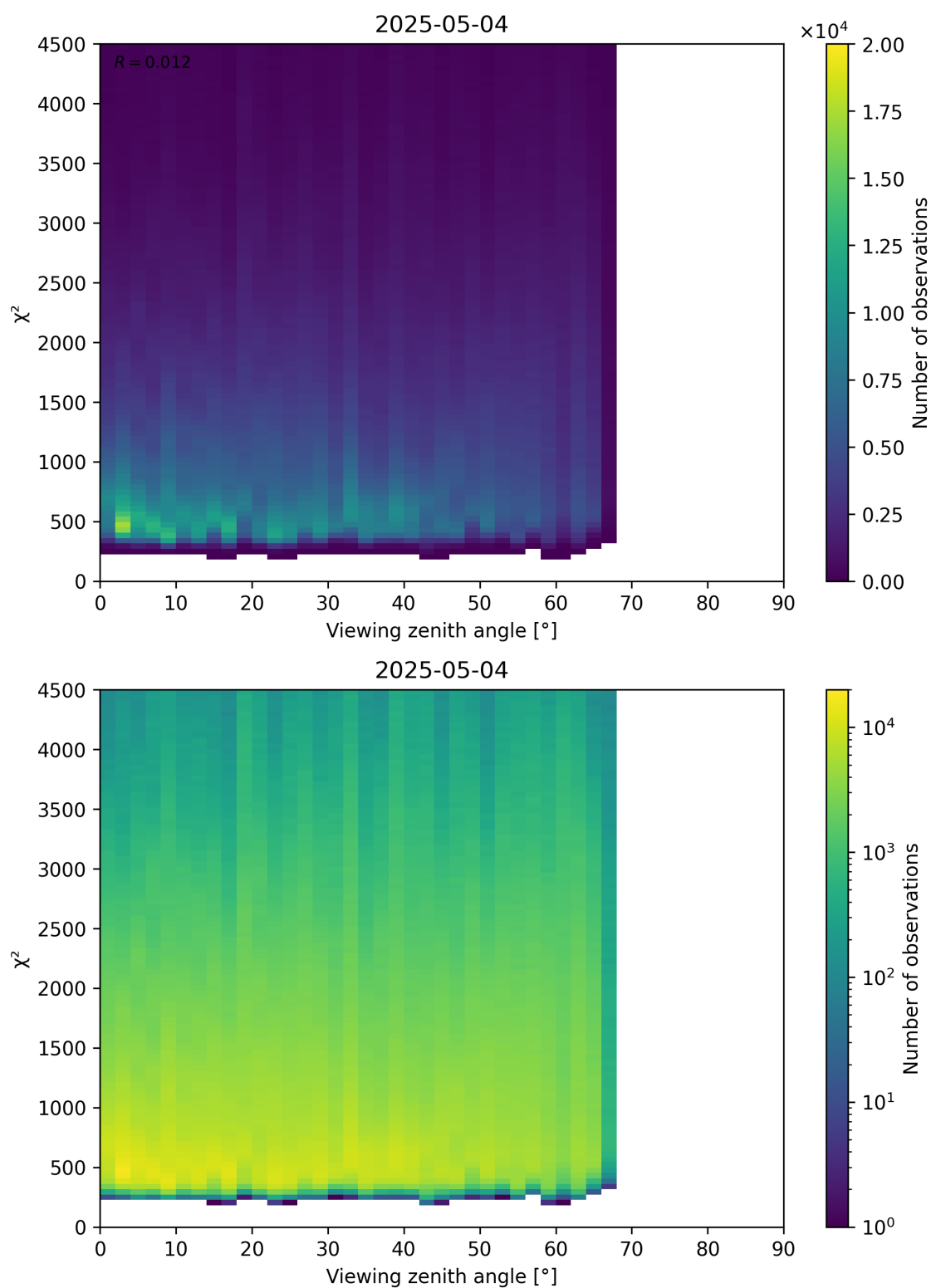
Figure 72: Scatter density plot of “Viewing zenith angle” against “ \chi^2 ” for 2025-05-03 to 2025-05-05.
