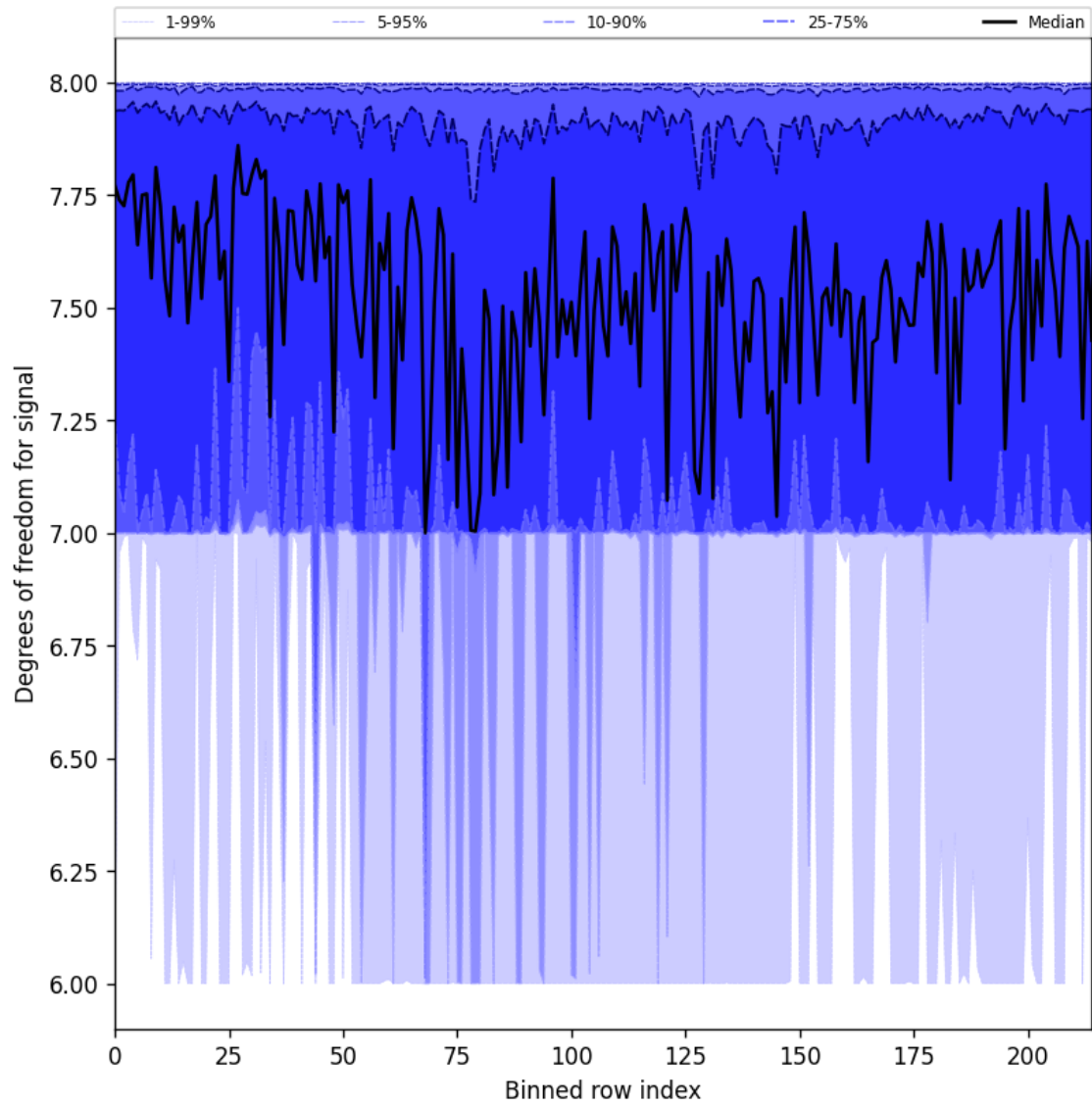
Figure 31: Along track statistics of “Degrees of freedom for signal” for 2025-05-05 to 2025-05-07
