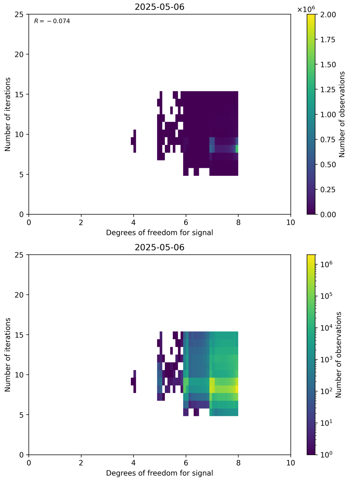
Figure 50: Scatter density plot of “Degrees of freedom for signal” against “Number of iterations” for 2025-05-05 to 2025-05-07.
