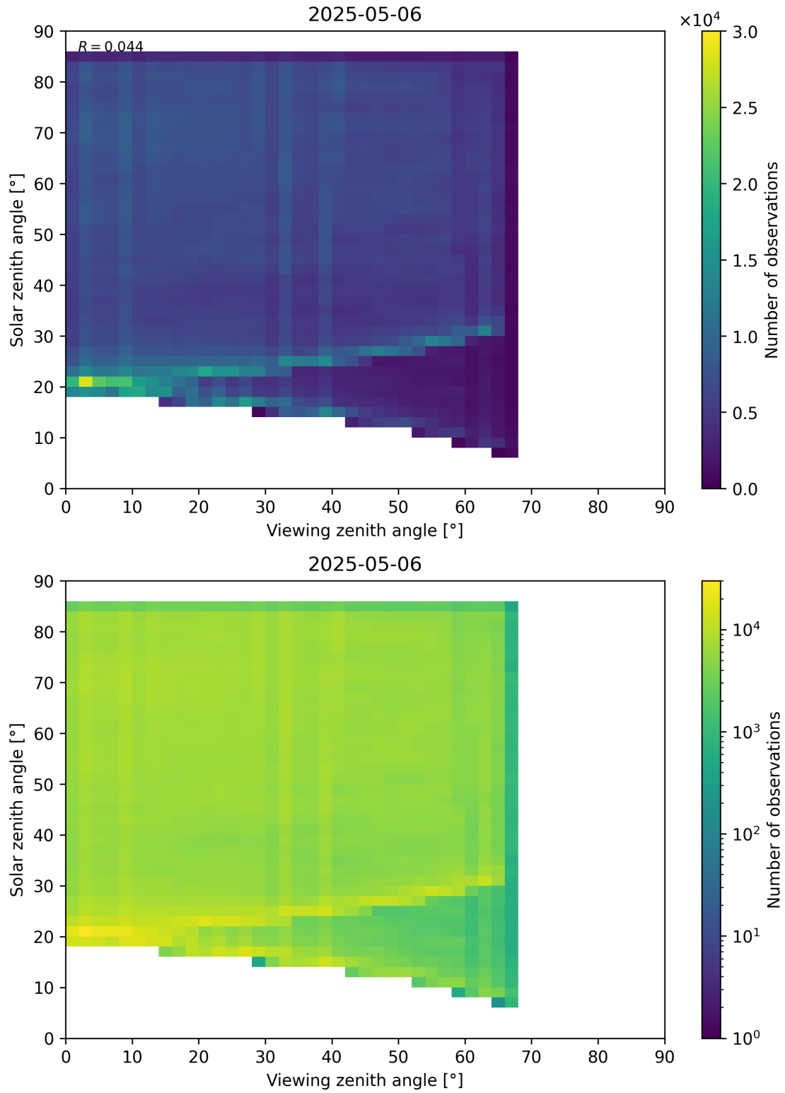
Figure 77: Scatter density plot of “Viewing zenith angle” against “Solar zenith angle” for 2025-05-05 to 2025-05-07.
