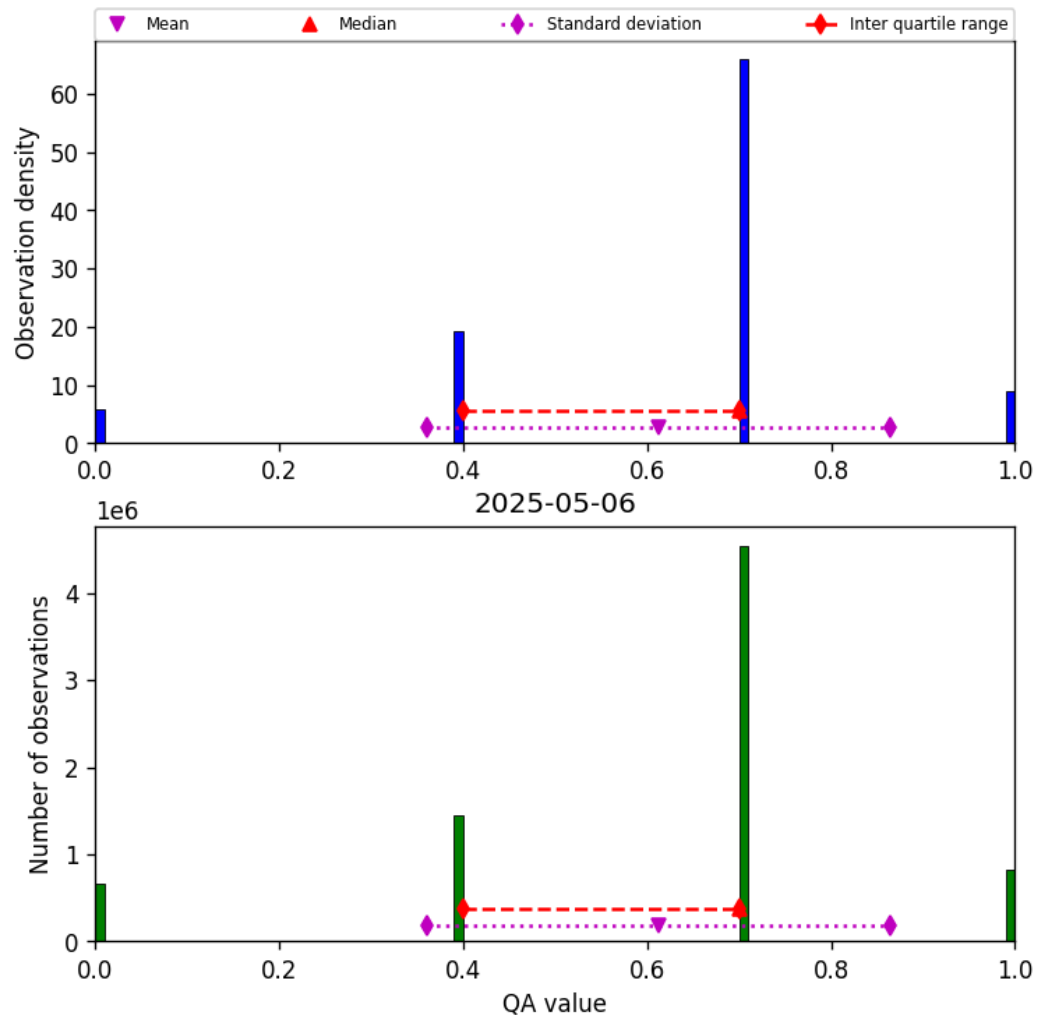
Figure 17: Histogram of “QA value” for 2025-05-05 to 2025-05-07
