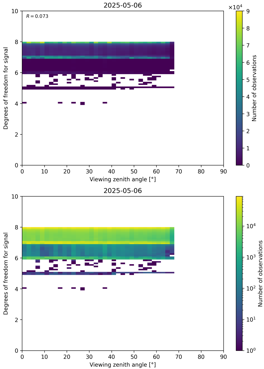
Figure 73: Scatter density plot of “Viewing zenith angle” against “Degrees of freedom for signal” for 2025-05-05 to 2025-05-07.
