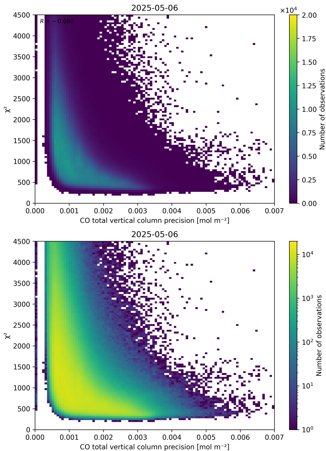
Figure 44: Scatter density plot of “CO total vertical column precision” against “ \chi^2 ” for 2025-05-05 to 2025-05-07.
