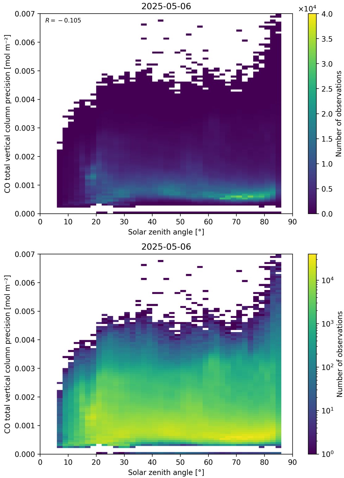
Figure 63: Scatter density plot of “Solar zenith angle” against “CO total vertical column precision” for 2025-05-05 to 2025-05-07.
