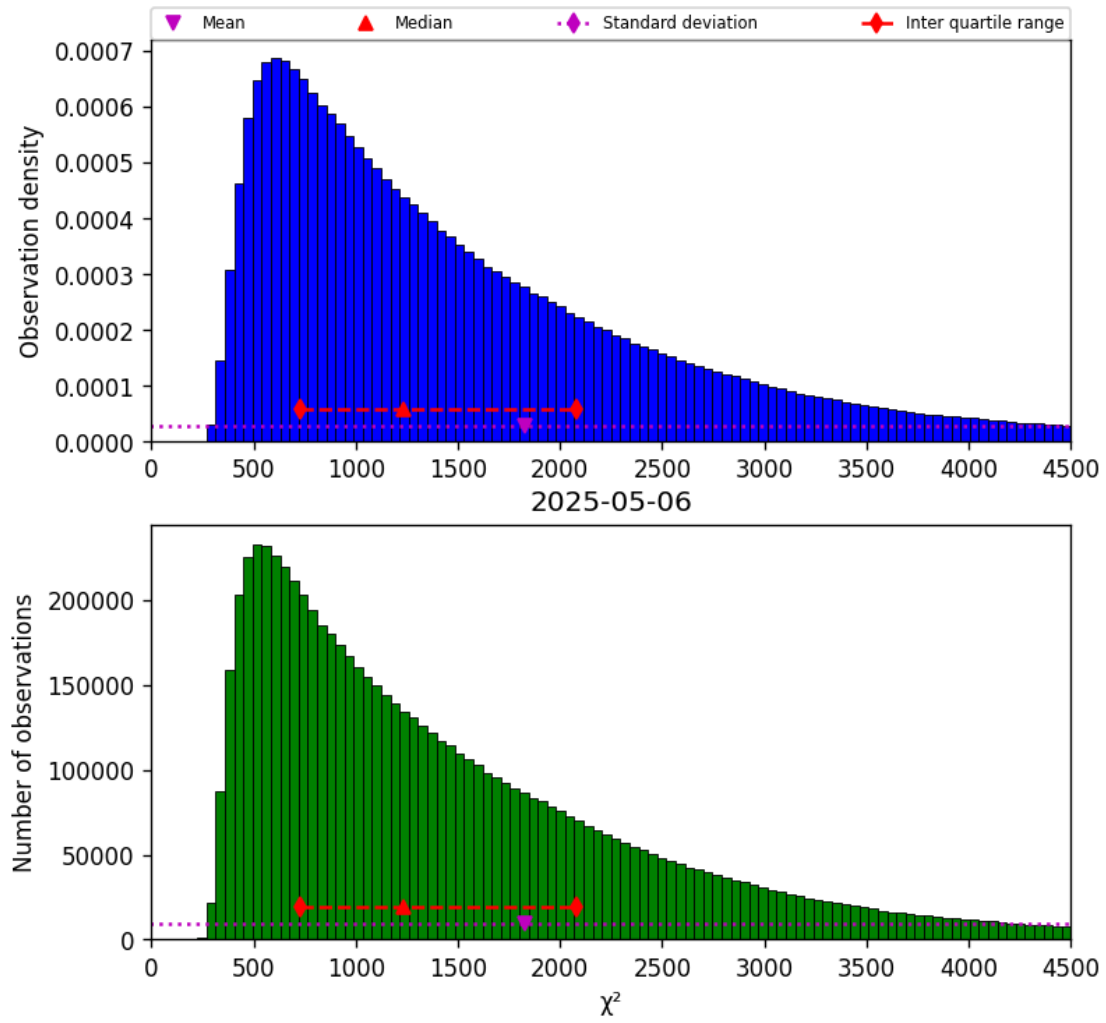
Figure 22: Histogram of " \chi^2 " for 2025-05-05 to 2025-05-07
