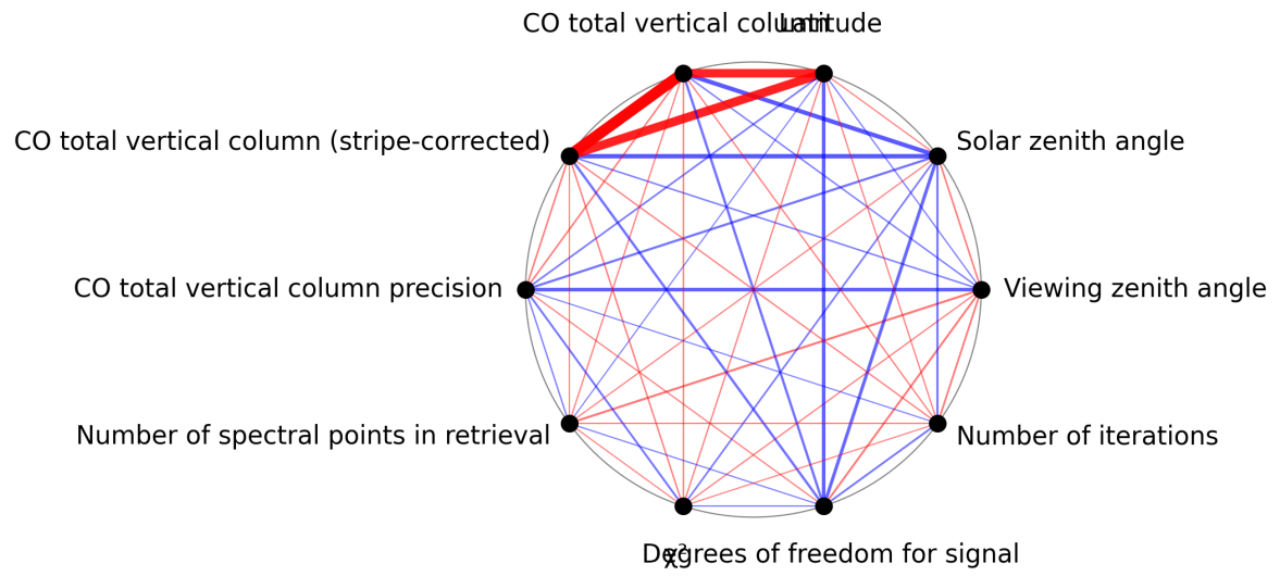
Figure 1: Map of correlation graph for 2025-05-05 to 2025-05-07.
