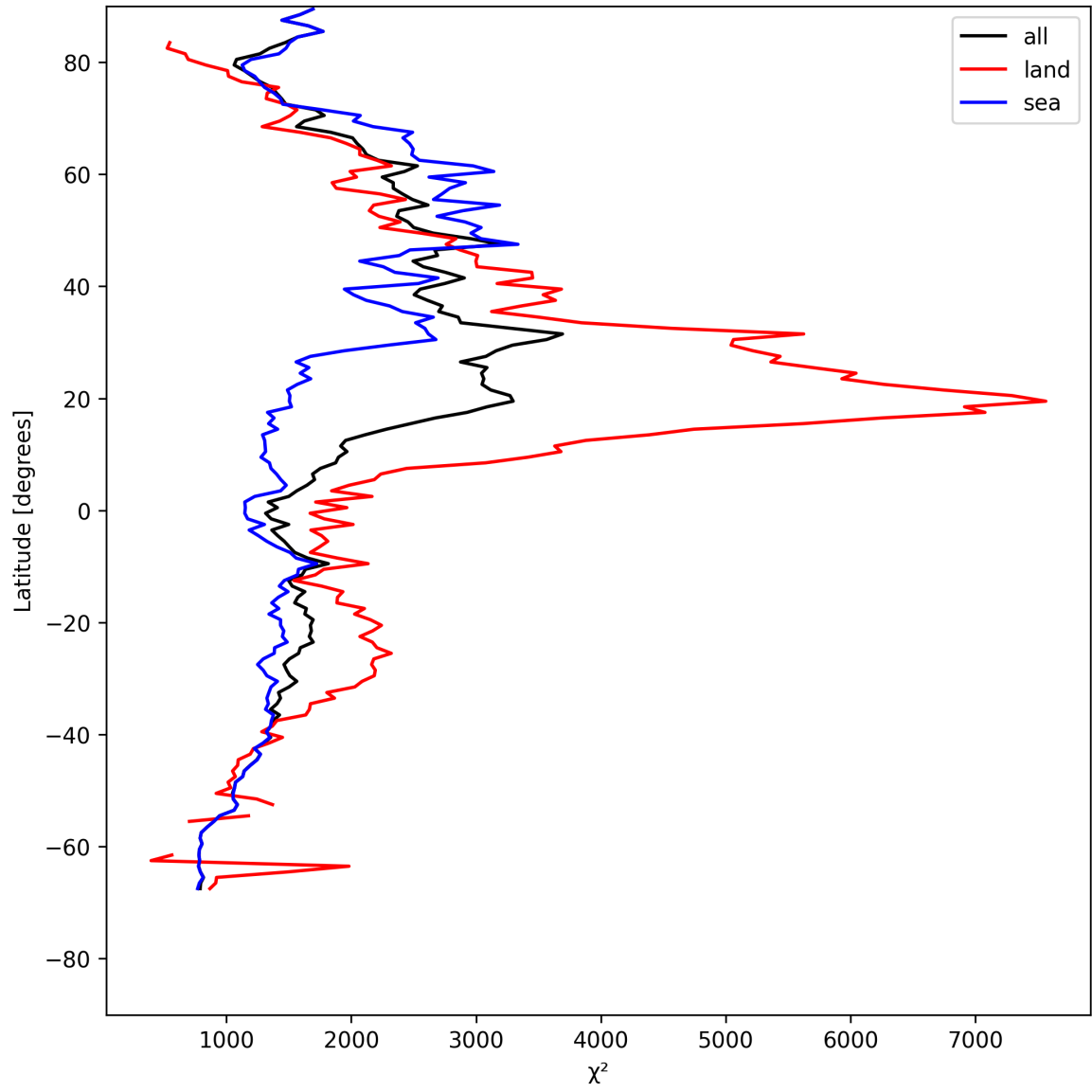
Figure 14: Zonal average of “ \chi^2 ” for 2025-05-05 to 2025-05-07.
