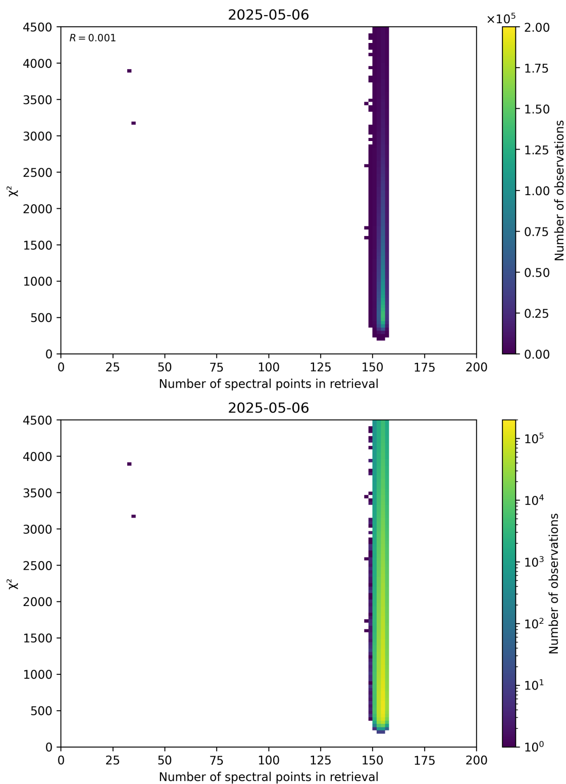
Figure 58: Scatter density plot of “Number of spectral points in retrieval” against “ \chi^2 ” for 2025-05-05 to 2025-05-07.
