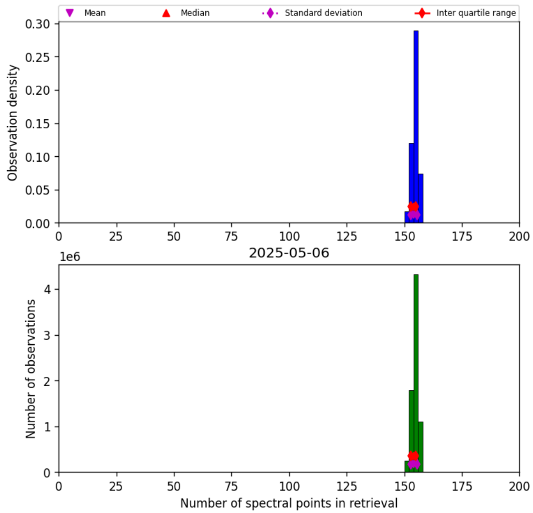
Figure 21: Histogram of “Number of spectral points in retrieval” for 2025-05-05 to 2025-05-07
