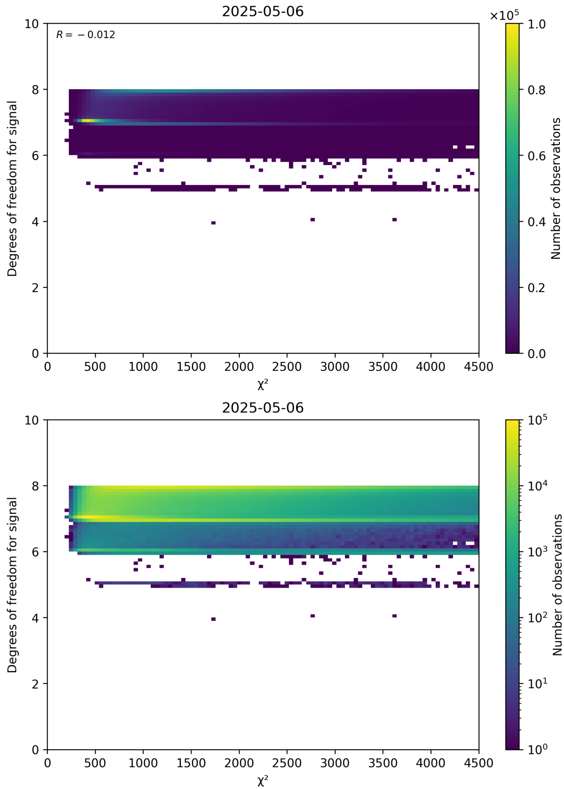
Figure 48: Scatter density plot of “ \chi^2 ” against “Degrees of freedom for signal” for 2025-05-05 to 2025-05-07.
