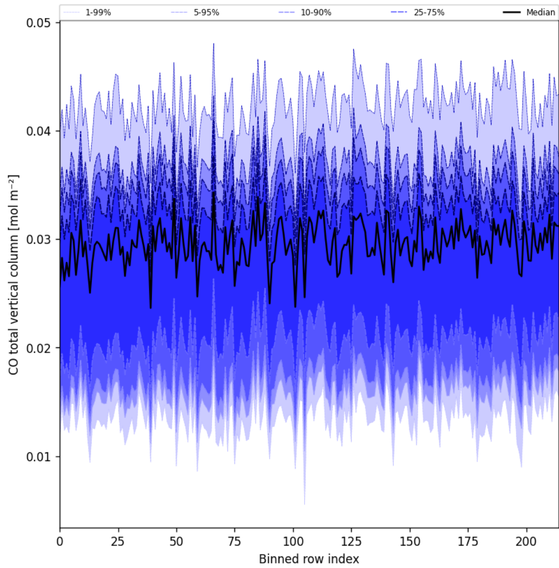
Figure 26: Along track statistics of "CO total vertical column" for 2025-05-05 to 2025-05-07
