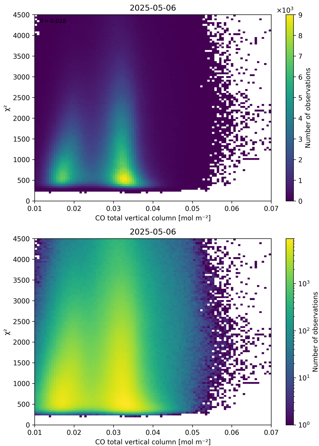
Figure 35: Scatter density plot of “CO total vertical column” against “ \chi^2 ” for 2025-05-05 to 2025-05-07.
