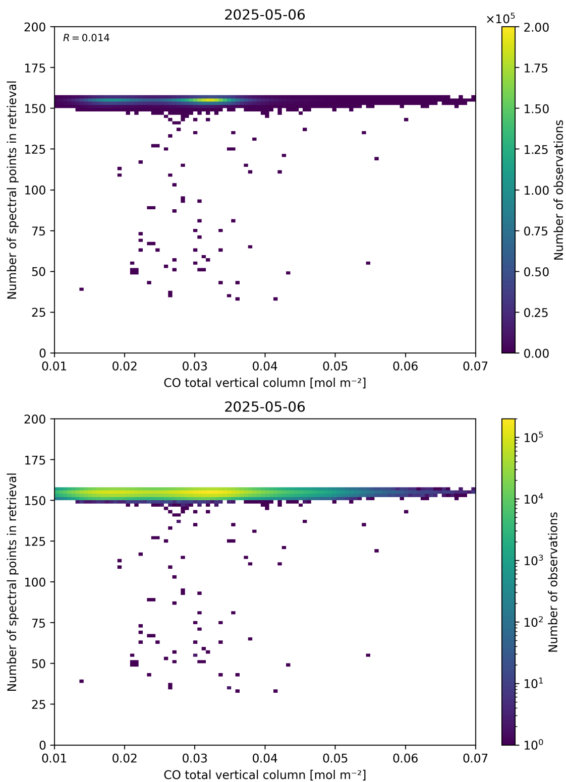
Figure 43: Scatter density plot of “CO total vertical column” against “Number of spectral points in retrieval” for 2025-05-05 to 2025-05-07.
