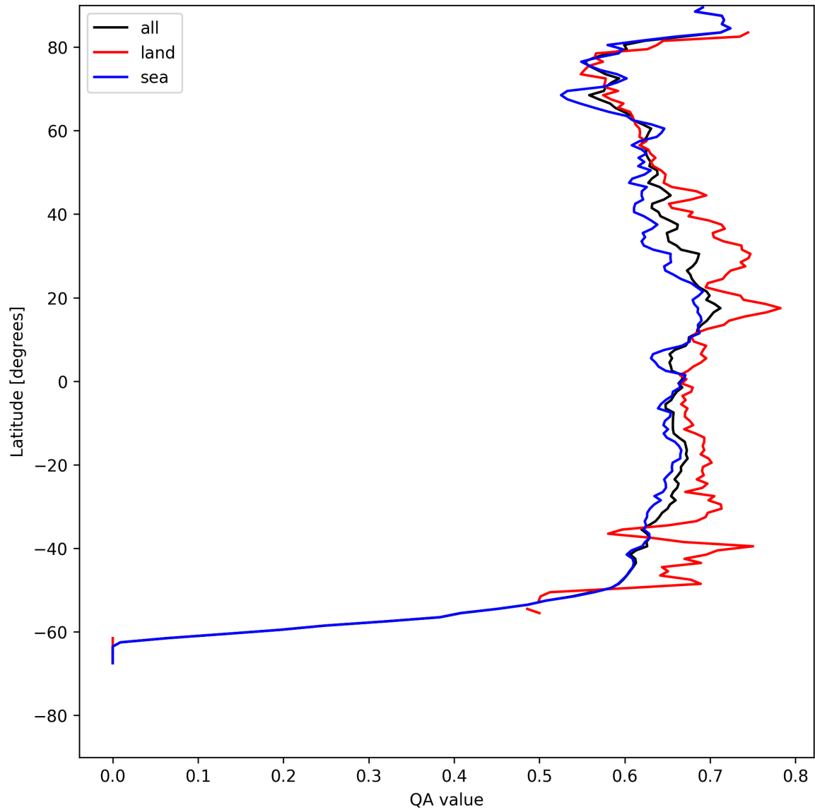
Figure 9: Zonal average of “QA value” for 2025-05-05 to 2025-05-07.
