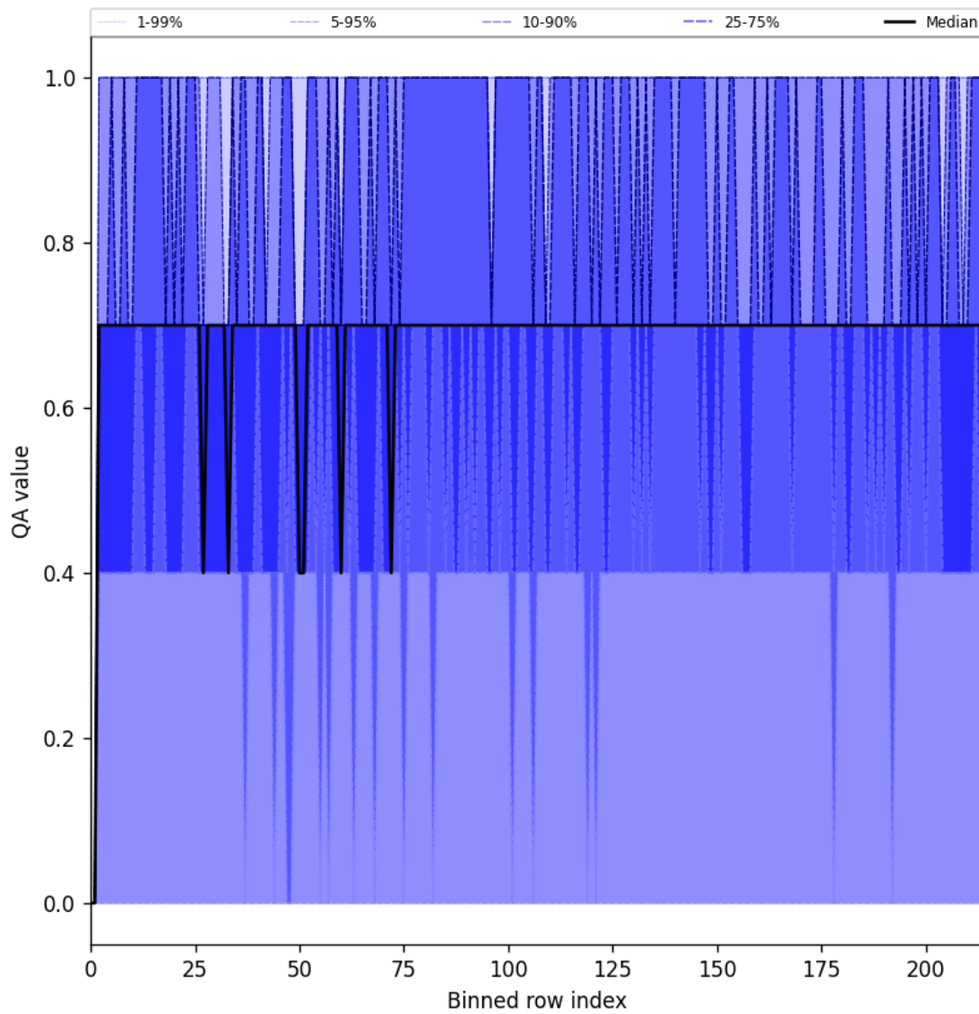
Figure 25: Along track statistics of “QA value” for 2025-05-05 to 2025-05-07
