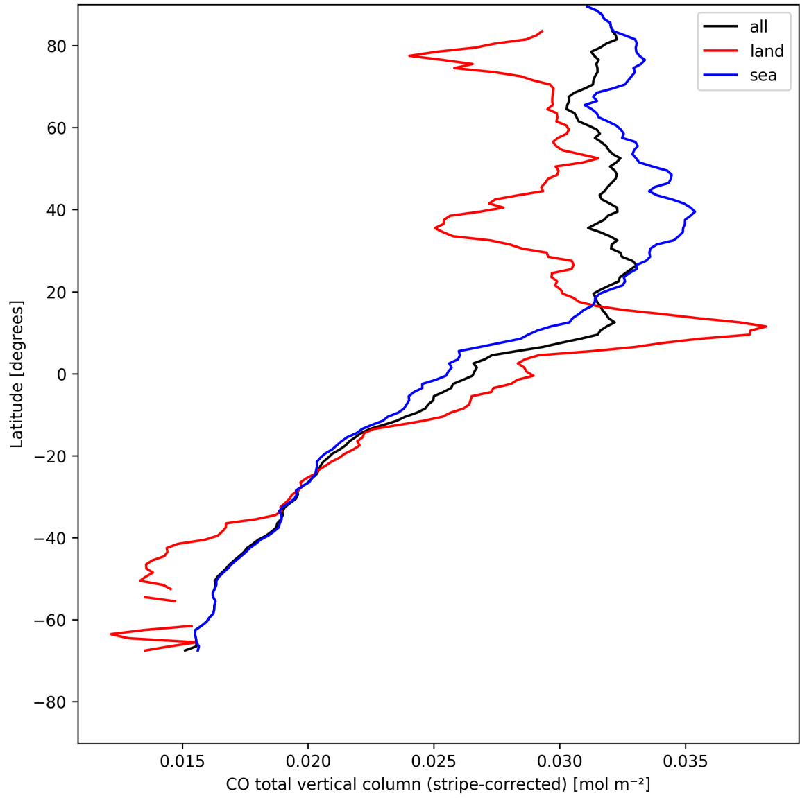
Figure 11: Zonal average of “CO total vertical column (stripe-corrected)” for 2025-05-05 to 2025-05-07.
