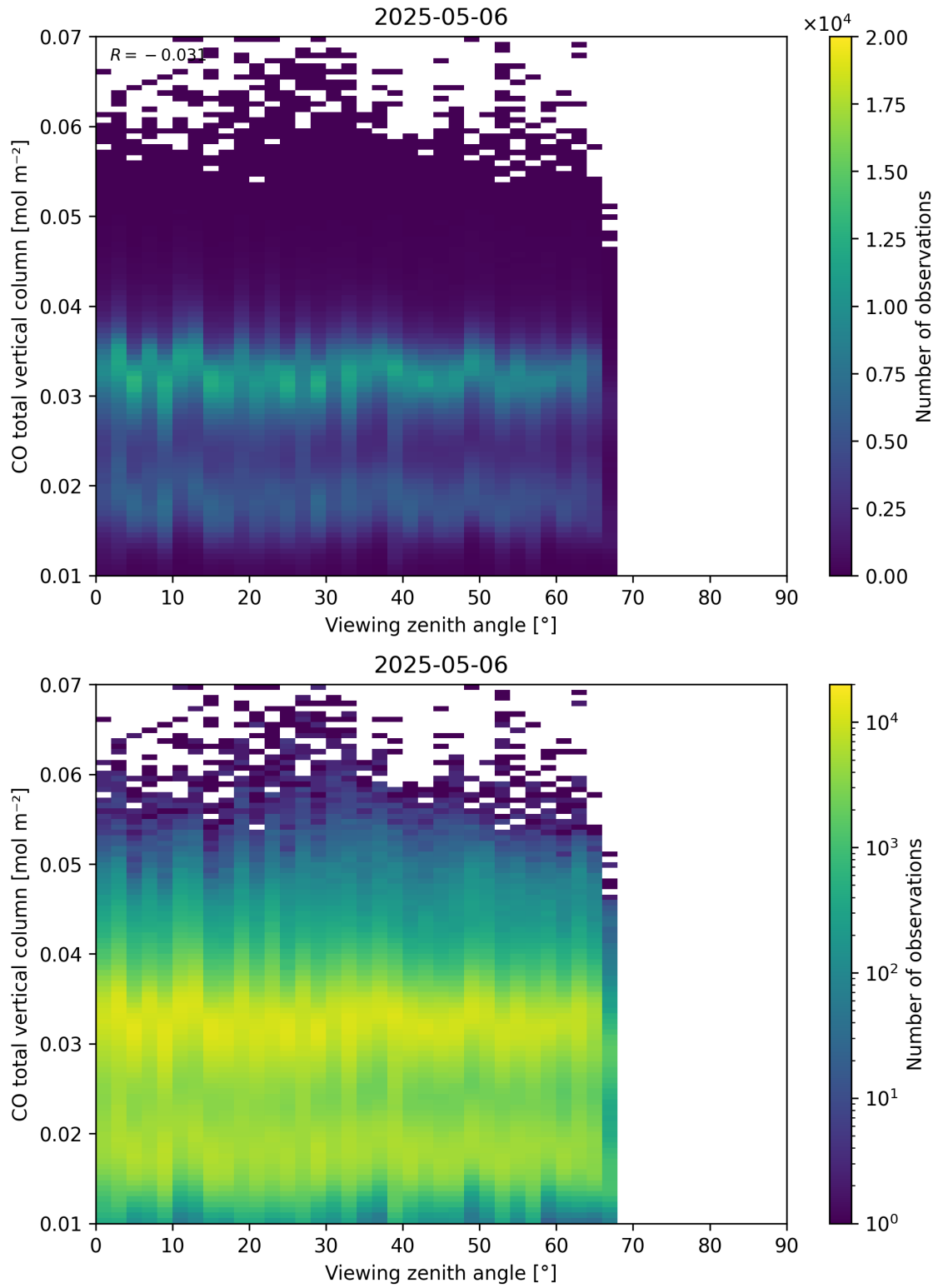
Figure 69: Scatter density plot of “Viewing zenith angle” against “CO total vertical column” for 2025-05-05 to 2025-05-07.
