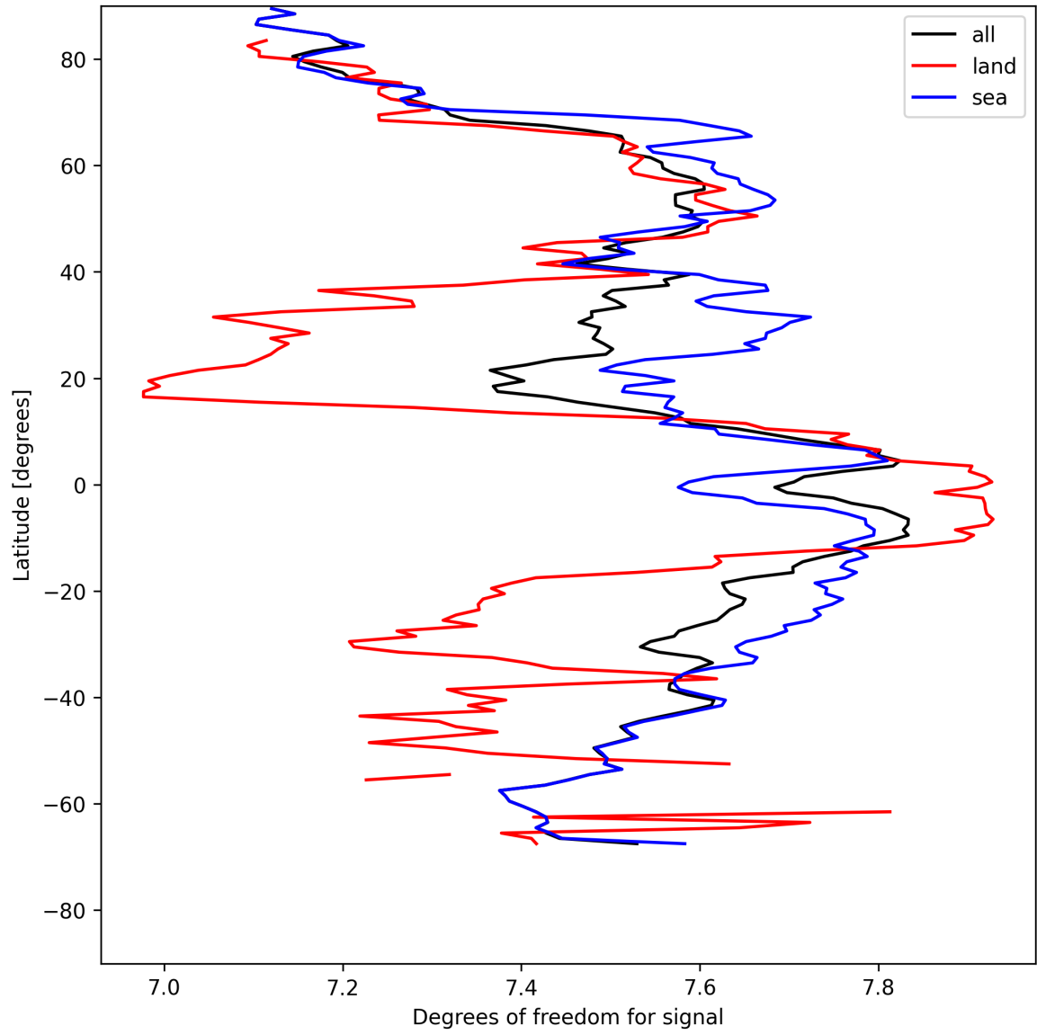
Figure 15: Zonal average of “Degrees of freedom for signal” for 2025-05-05 to 2025-05-07.
