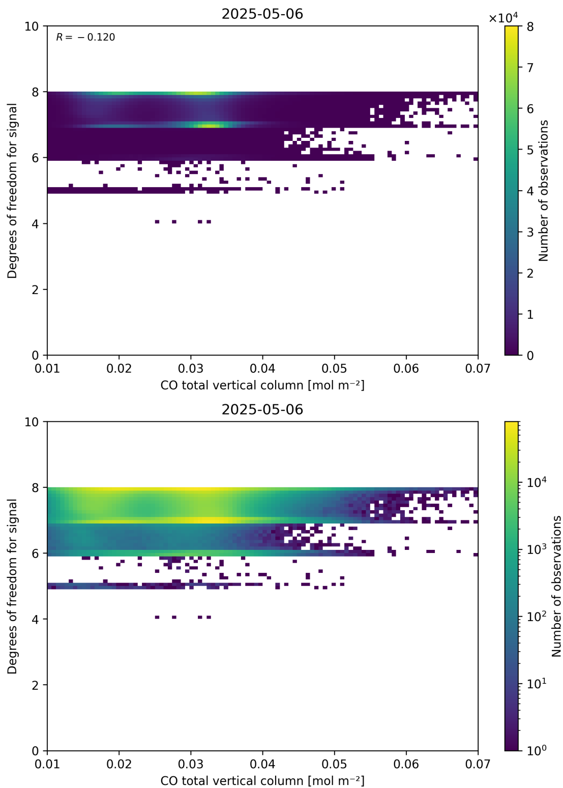
Figure 41: Scatter density plot of “CO total vertical column” against “Degrees of freedom for signal” for 2025-05-05 to 2025-05-07.
