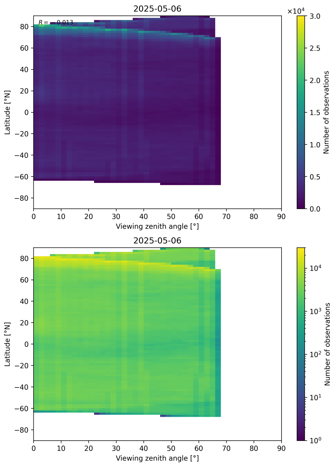
Figure 74: Scatter density plot of “Viewing zenith angle” against “Latitude” for 2025-05-05 to 2025-05-07.
