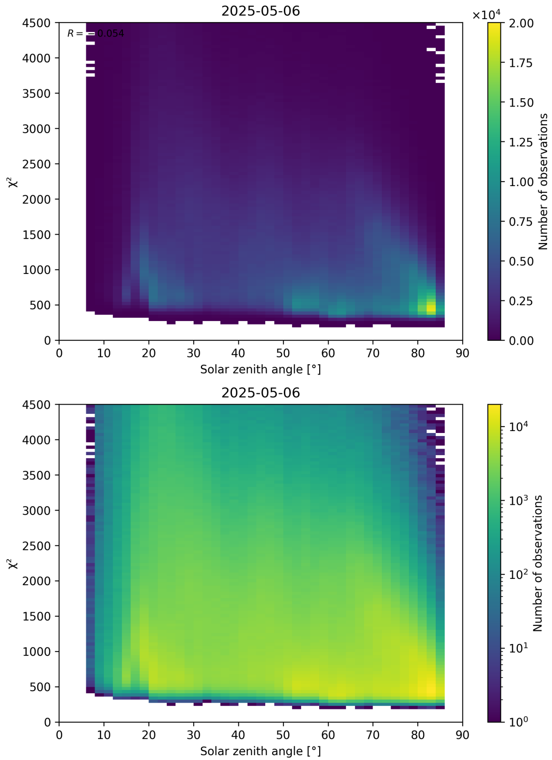
Figure 64: Scatter density plot of “Solar zenith angle” against “ \chi^2 ” for 2025-05-05 to 2025-05-07.
