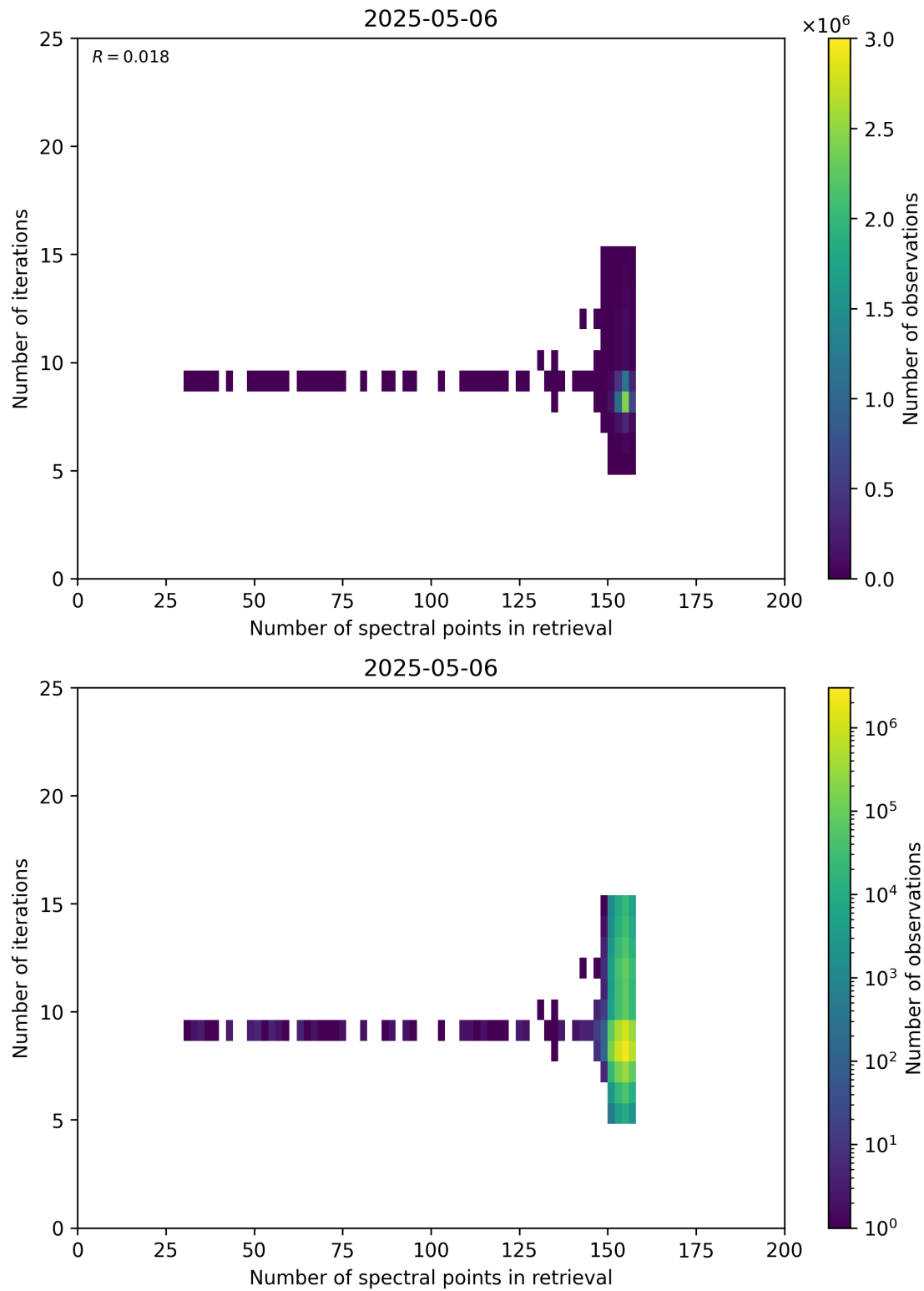
Figure 60: Scatter density plot of “Number of spectral points in retrieval” against “Number of iterations” for 2025-05-05 to 2025-05-07.
