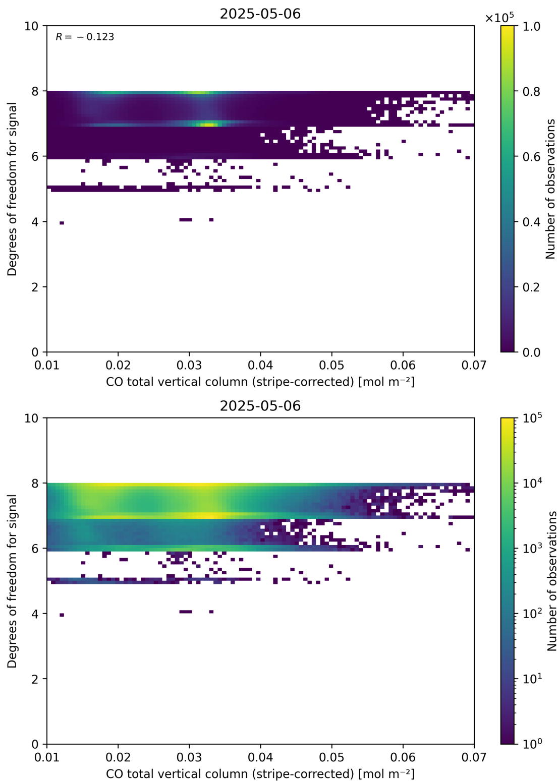
Figure 38: Scatter density plot of “CO total vertical column (stripe-corrected)” against “Degrees of freedom for signal” for 2025-05-05 to 2025-05-07.
