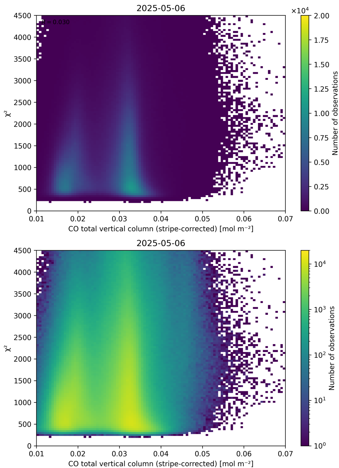
Figure 37: Scatter density plot of “CO total vertical column (stripe-corrected)” against “ \chi^2 ” for 2025-05-05 to 2025-05-07.
