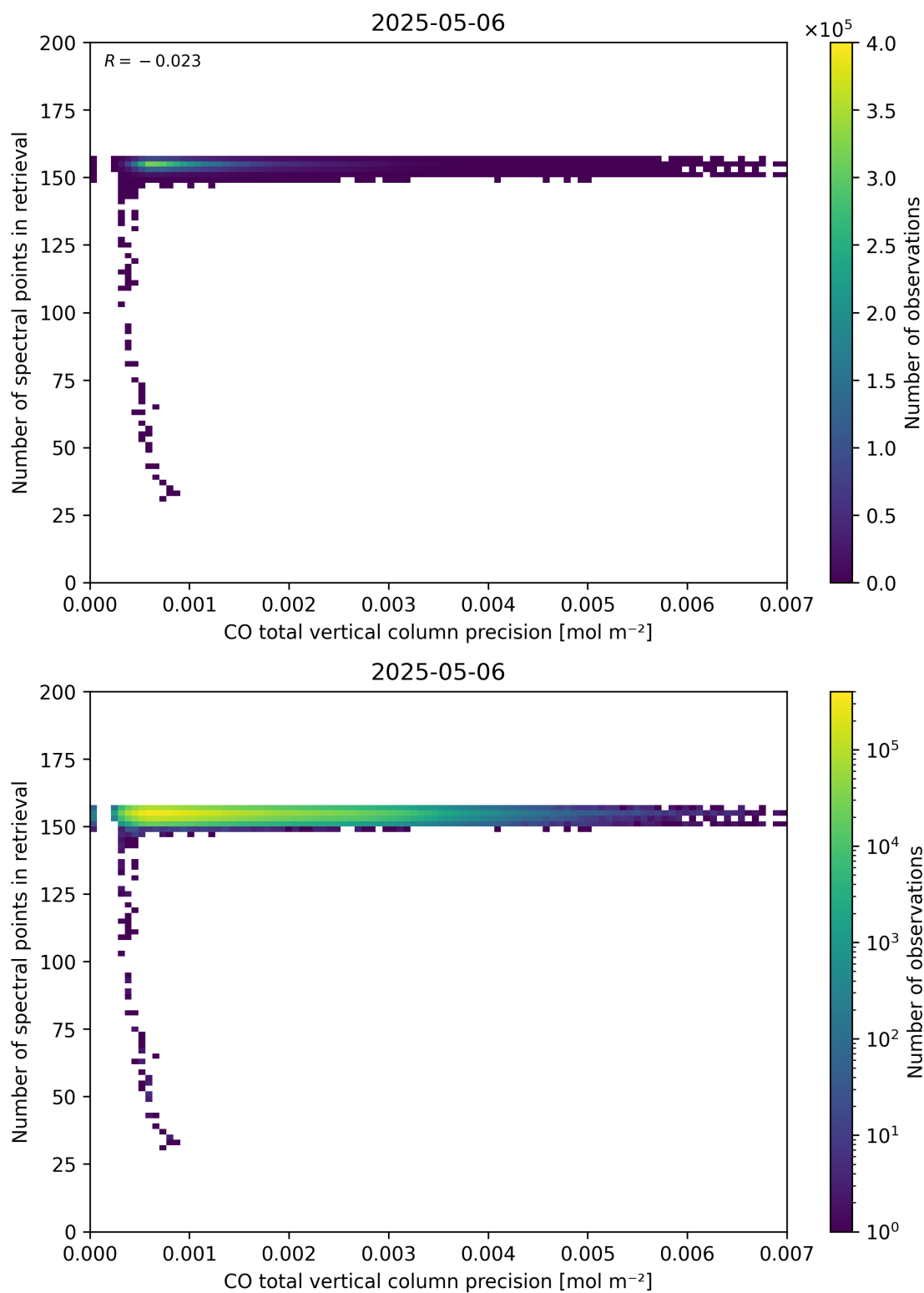
Figure 47: Scatter density plot of “CO total vertical column precision” against “Number of spectral points in retrieval” for 2025-05-05 to 2025-05-07.
