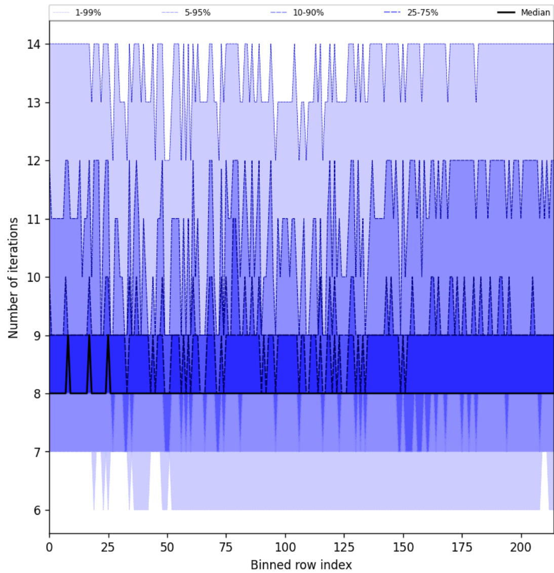
Figure 32: Along track statistics of “Number of iterations” for 2025-05-05 to 2025-05-07
