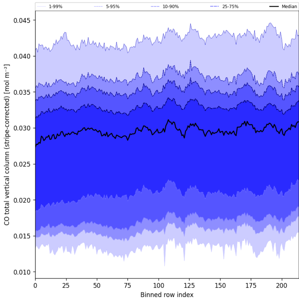
Figure 27: Along track statistics of “CO total vertical column (stripe-corrected)” for 2025-05-05 to 2025-05-07
