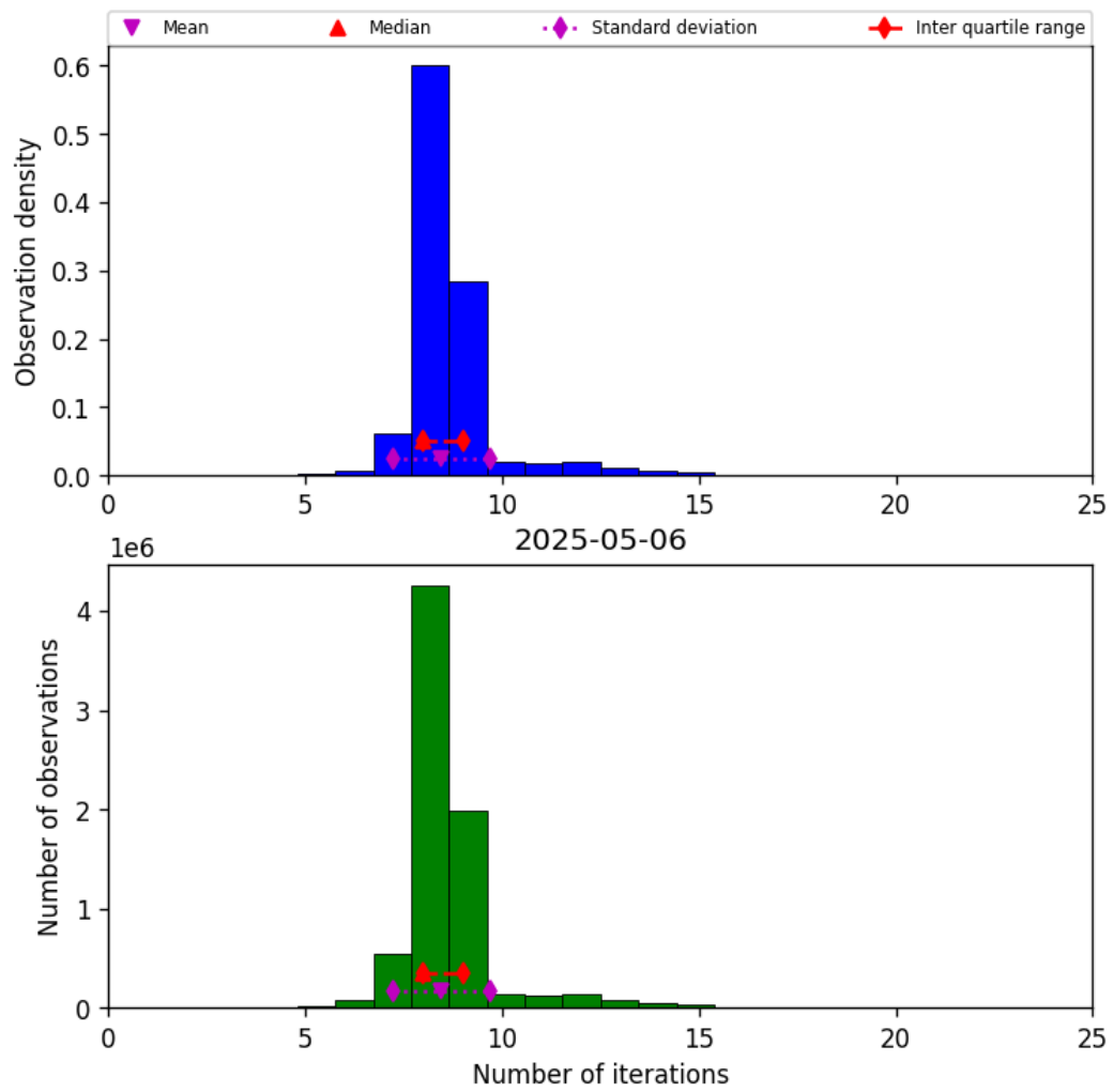
Figure 24: Histogram of "Number of iterations" for 2025-05-05 to 2025-05-07
