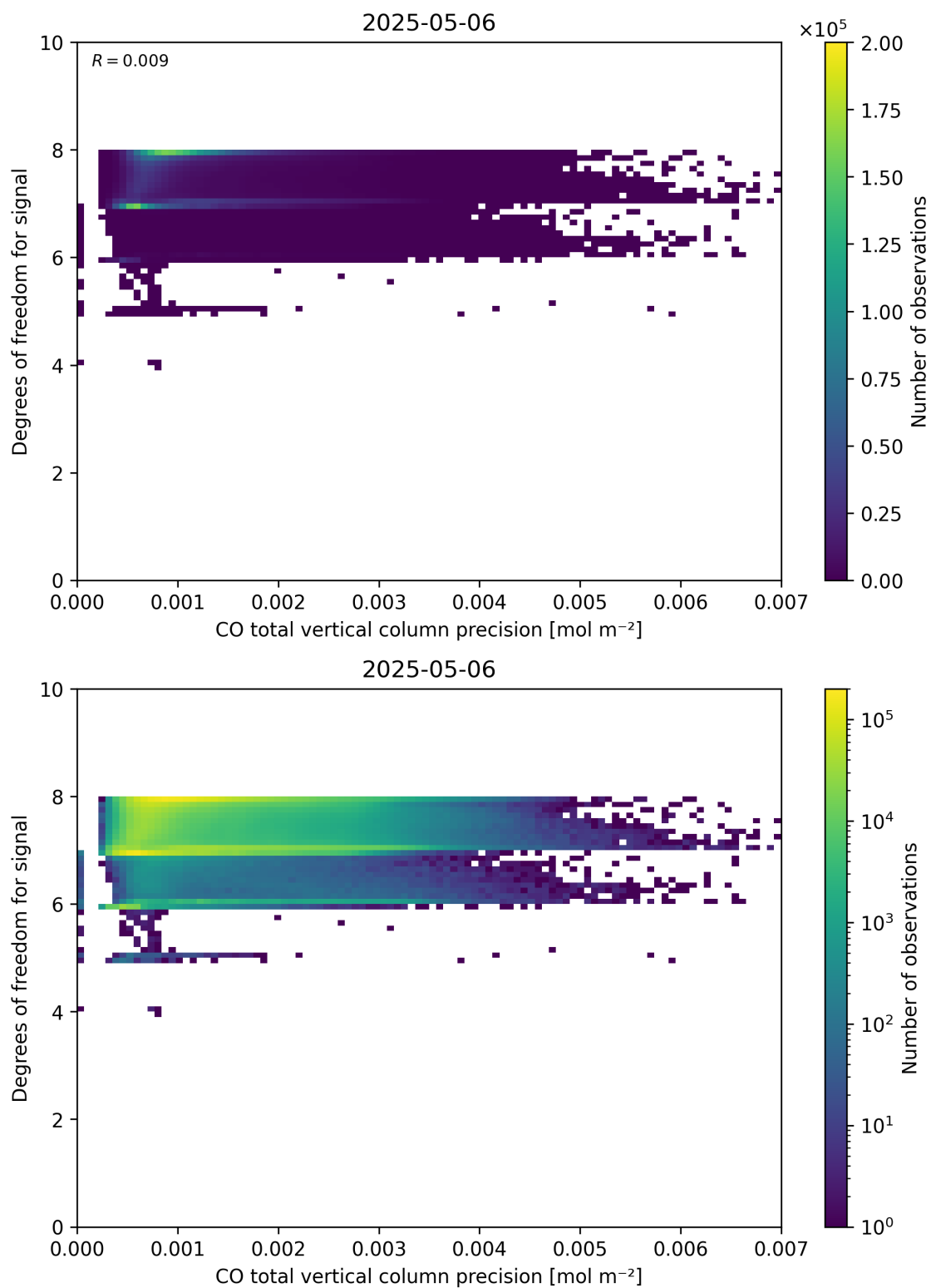
Figure 45: Scatter density plot of “CO total vertical column precision” against “Degrees of freedom for signal” for 2025-05-05 to 2025-05-07.
