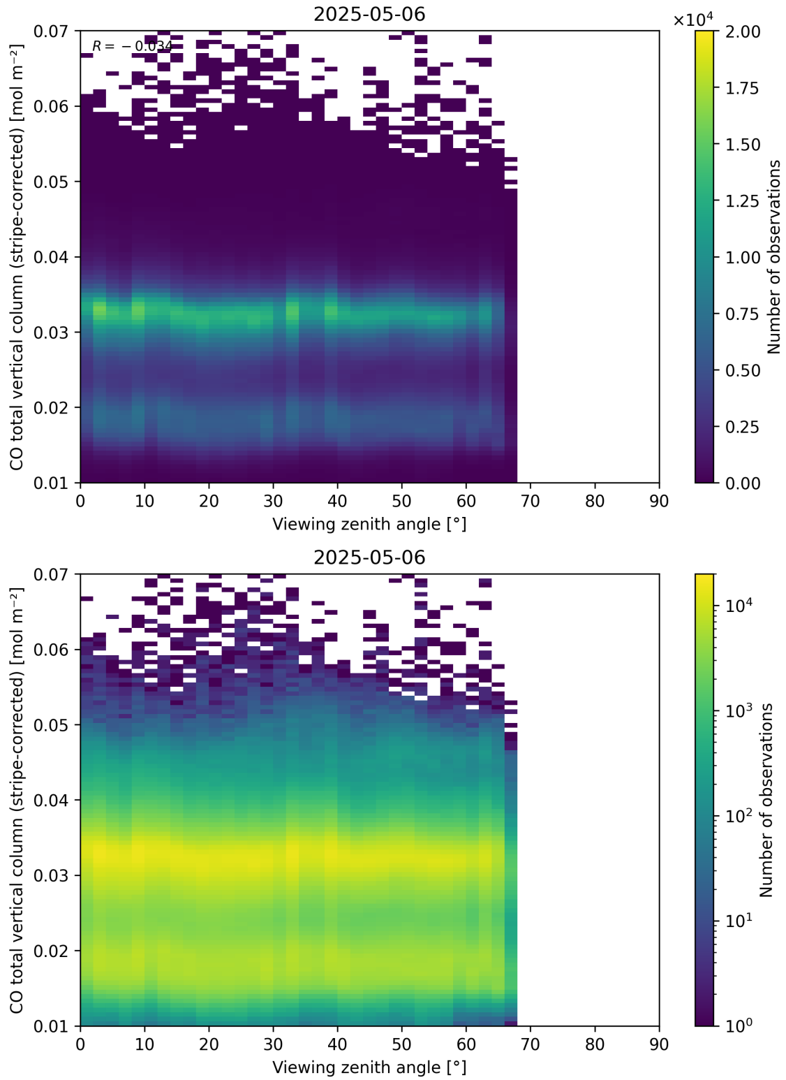
Figure 70: Scatter density plot of “Viewing zenith angle” against “CO total vertical column (stripe-corrected)” for 2025-05-05 to 2025-05-07.
