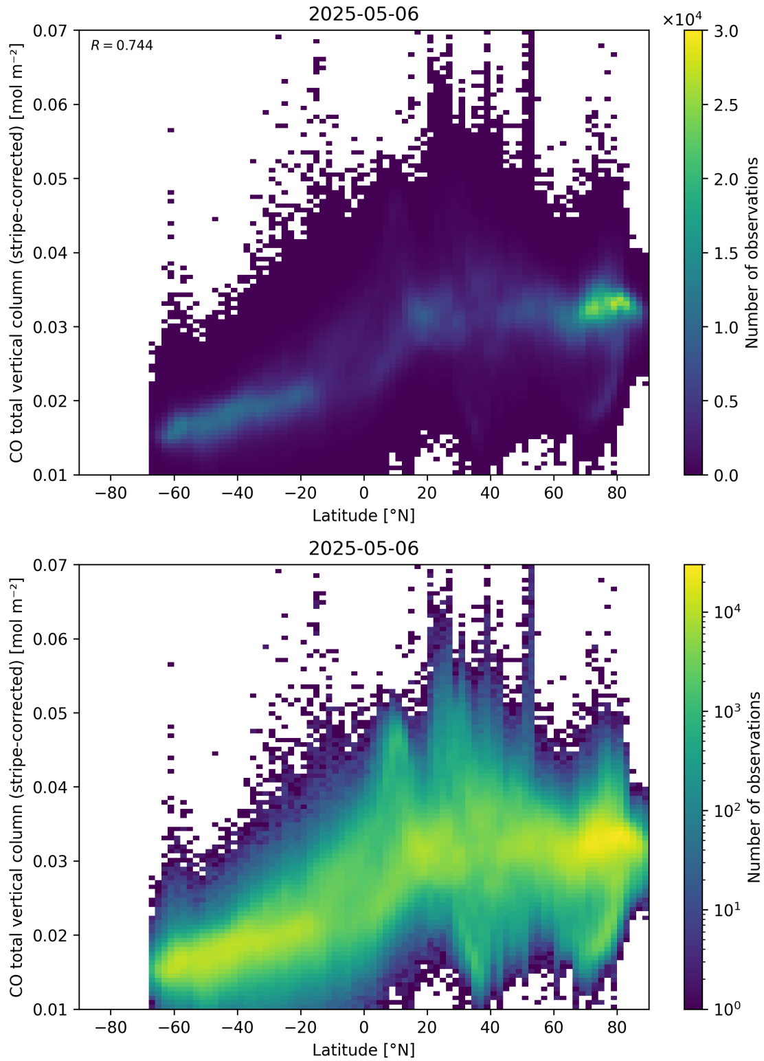
Figure 52: Scatter density plot of “Latitude” against “CO total vertical column (stripe-corrected)” for 2025-05-05 to 2025-05-07.
