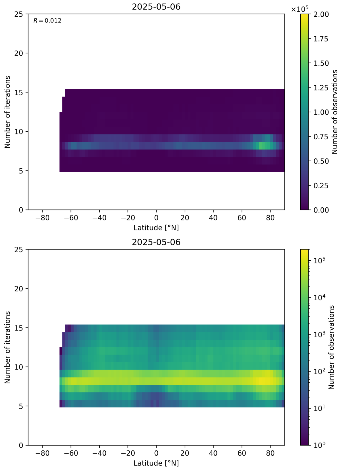
Figure 56: Scatter density plot of “Latitude” against “Number of iterations” for 2025-05-05 to 2025-05-07.
