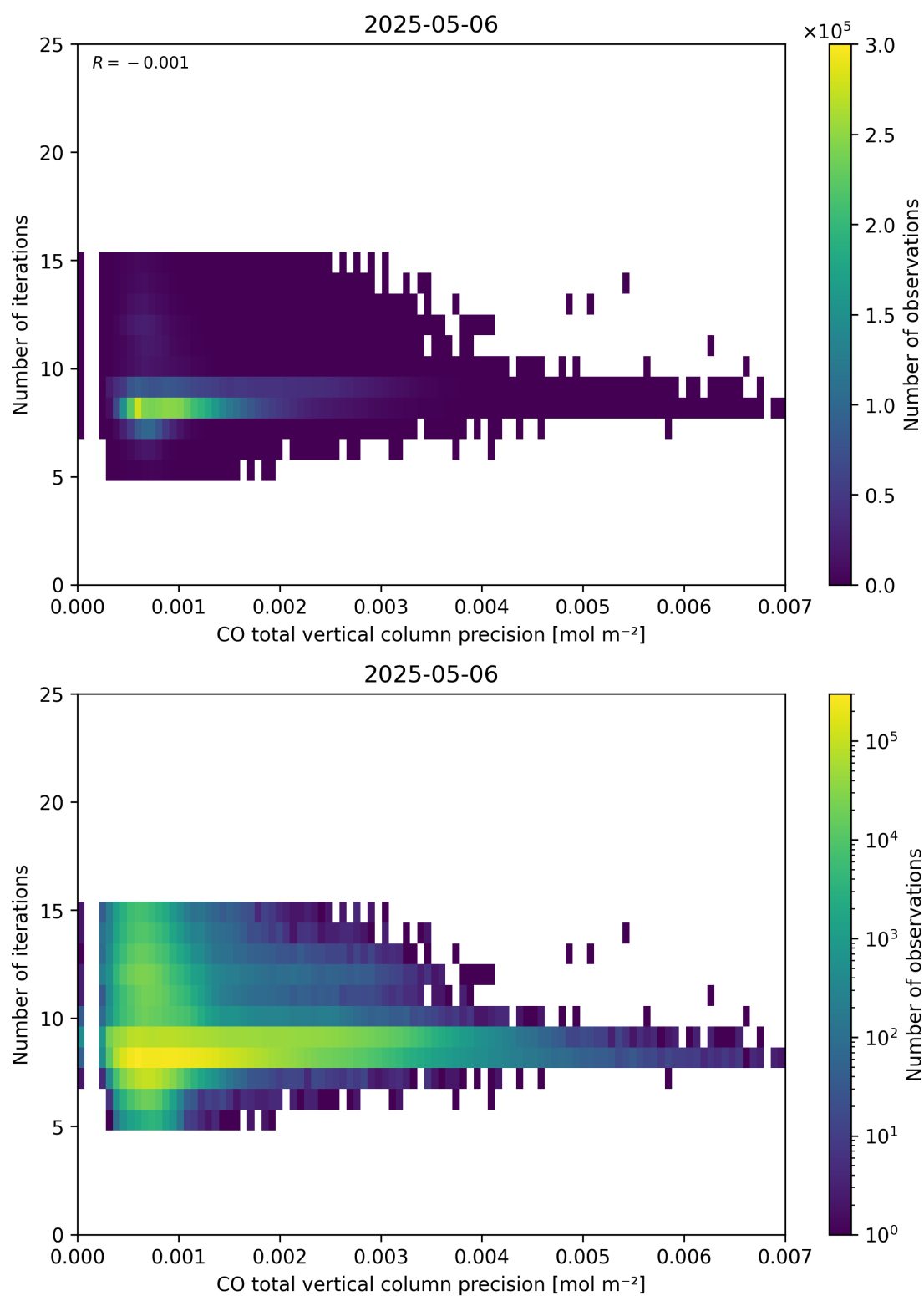
Figure 46: Scatter density plot of “CO total vertical column precision” against “Number of iterations” for 2025-05-05 to 2025-05-07.
