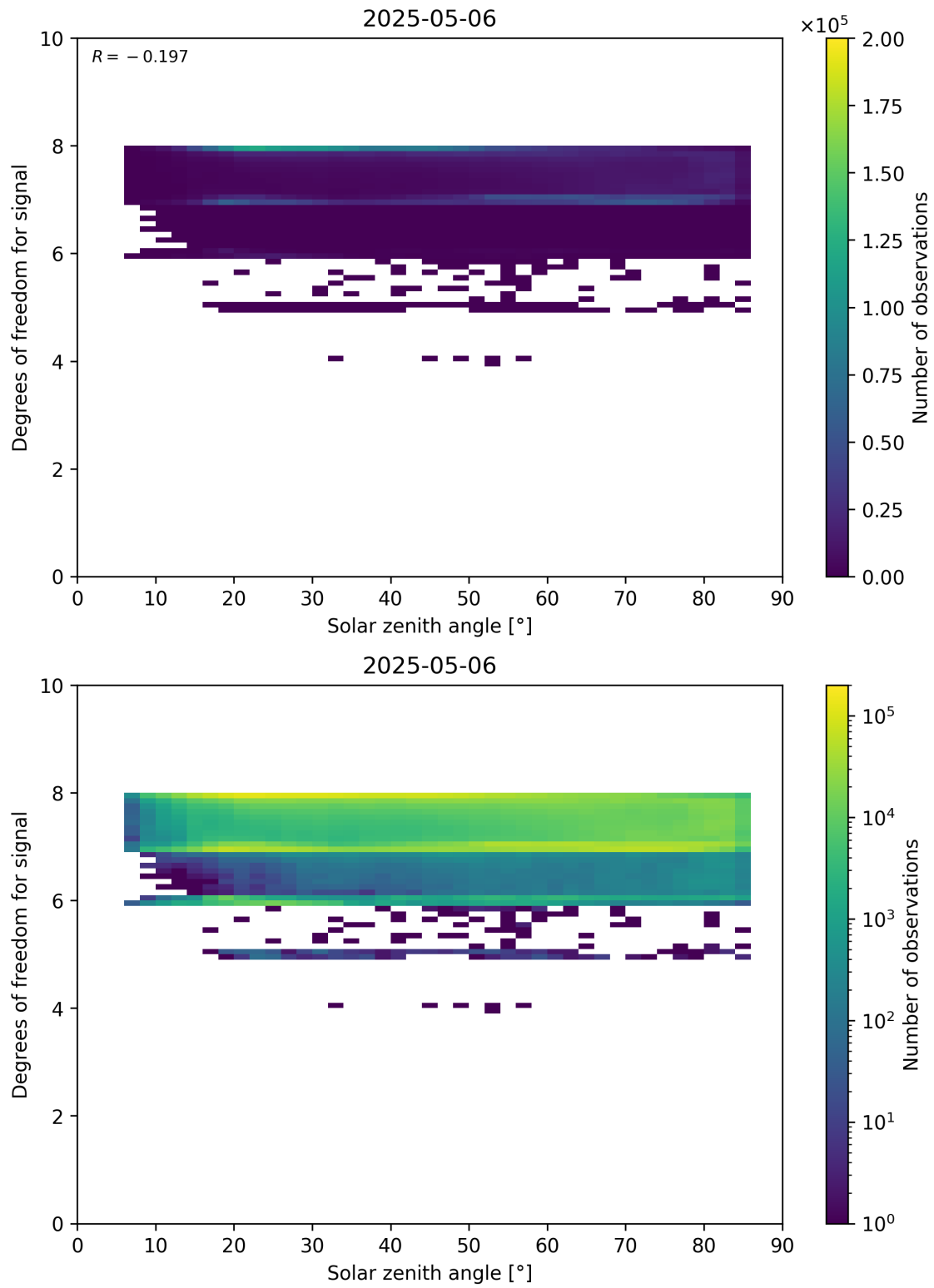
Figure 65: Scatter density plot of “Solar zenith angle” against “Degrees of freedom for signal” for 2025-05-05 to 2025-05-07.
