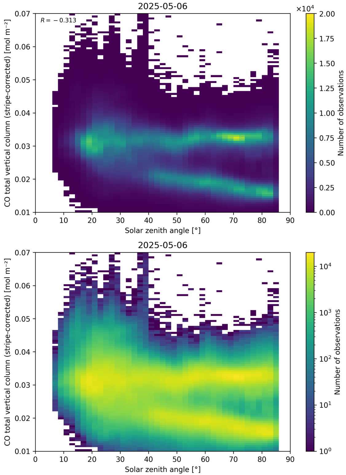
Figure 62: Scatter density plot of “Solar zenith angle” against “CO total vertical column (stripe-corrected)” for 2025-05-05 to 2025-05-07.
