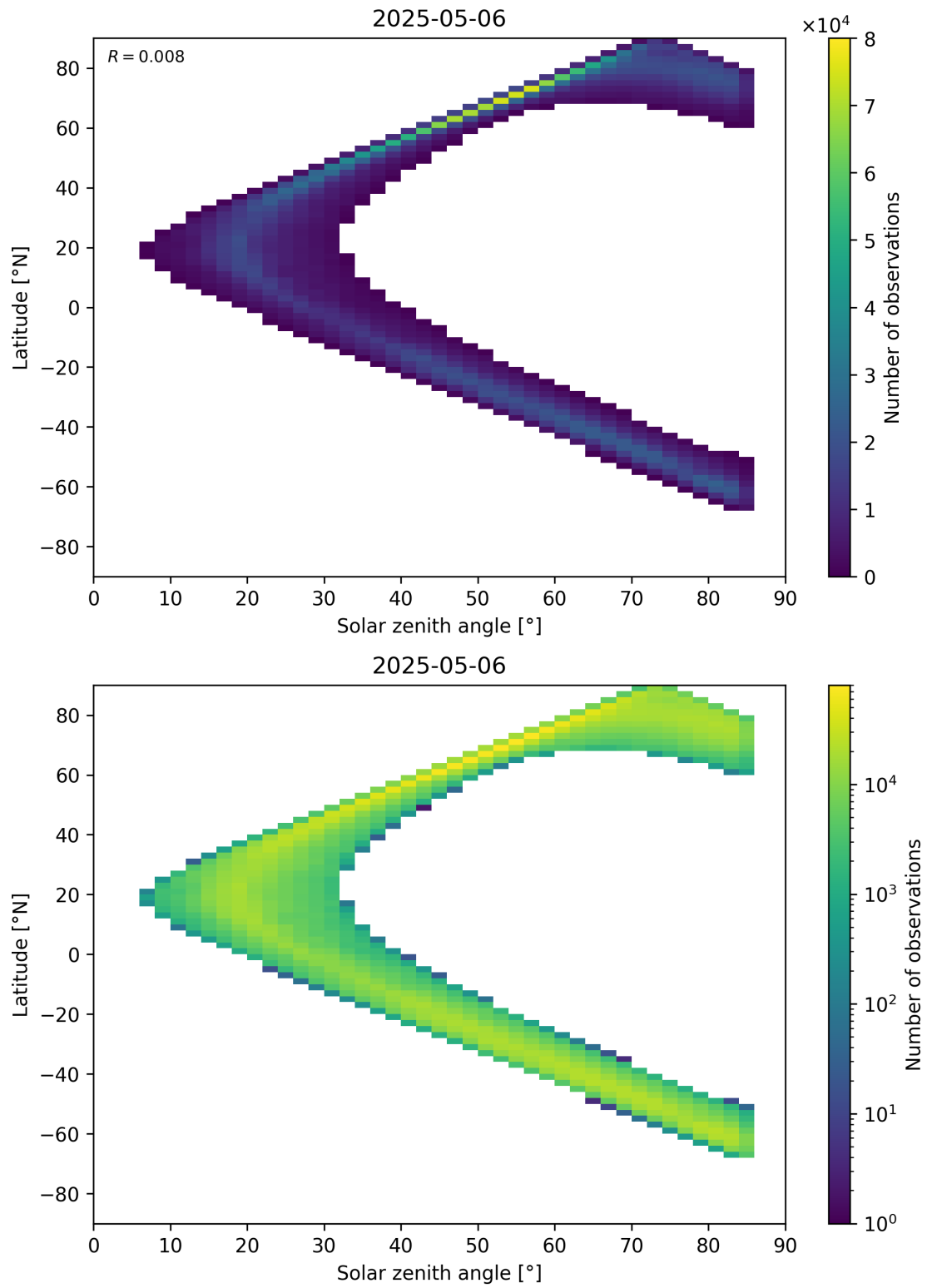
Figure 66: Scatter density plot of “Solar zenith angle” against “Latitude” for 2025-05-05 to 2025-05-07.
