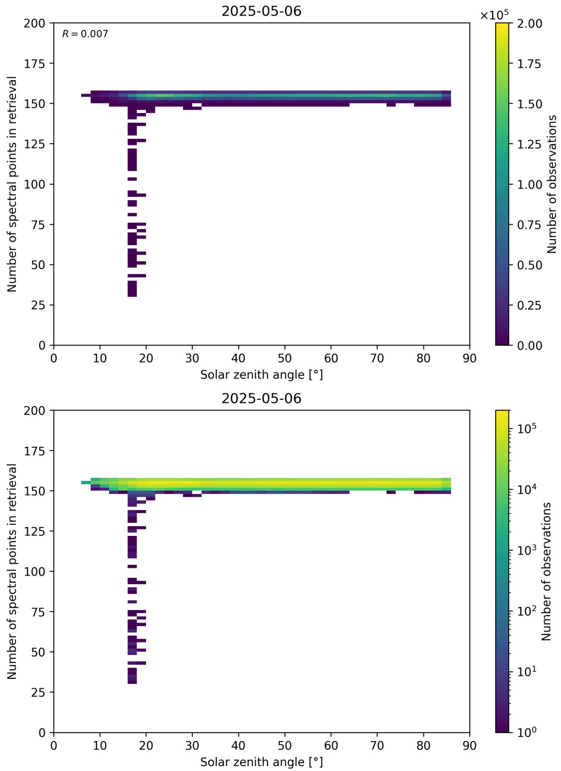
Figure 68: Scatter density plot of “Solar zenith angle” against “Number of spectral points in retrieval” for 2025-05-05 to 2025-05-07.
