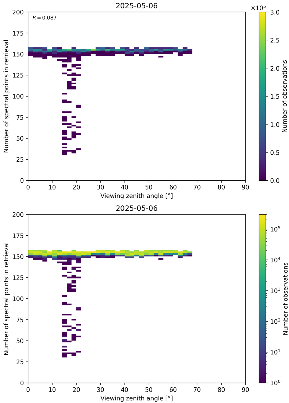
Figure 76: Scatter density plot of “Viewing zenith angle” against “Number of spectral points in retrieval” for 2025-05-05 to 2025-05-07.
