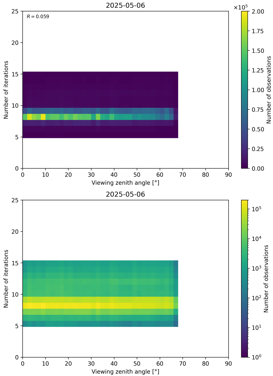
Figure 75: Scatter density plot of “Viewing zenith angle” against “Number of iterations” for 2025-05-05 to 2025-05-07.
