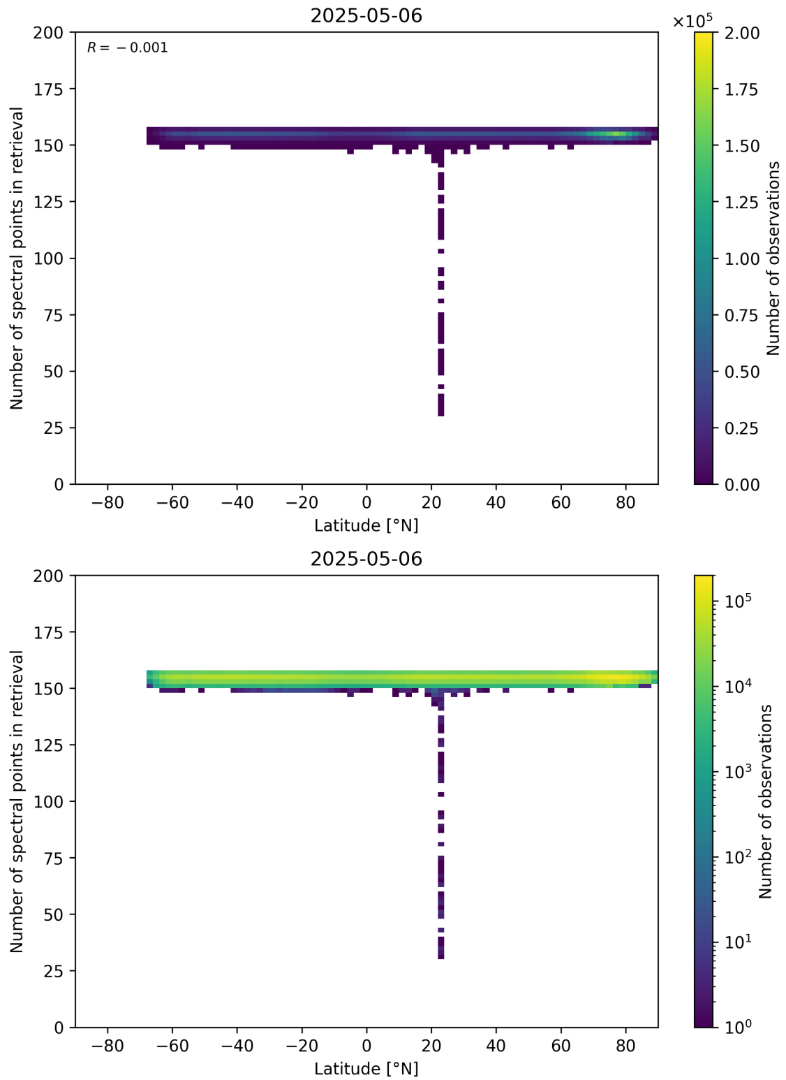
Figure 57: Scatter density plot of “Latitude” against “Number of spectral points in retrieval” for 2025-05-05 to 2025-05-07.
