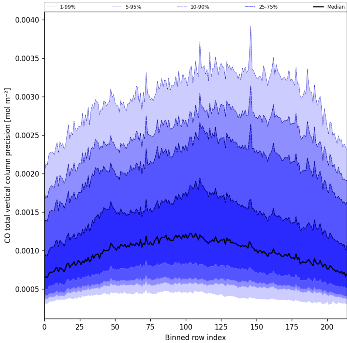
Figure 28: Along track statistics of “CO total vertical column precision” for 2025-05-05 to 2025-05-07
