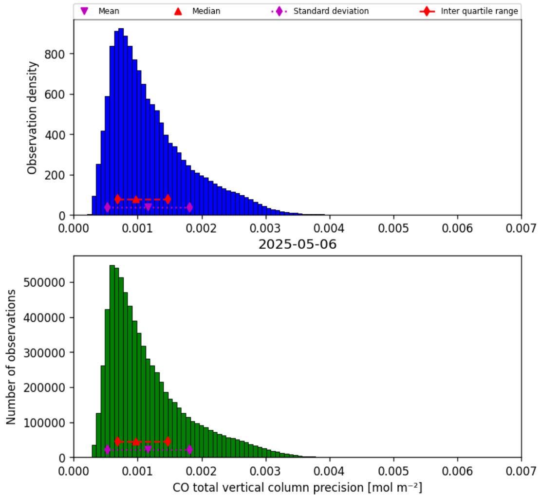
Figure 20: Histogram of “CO total vertical column precision” for 2025-05-05 to 2025-05-07
