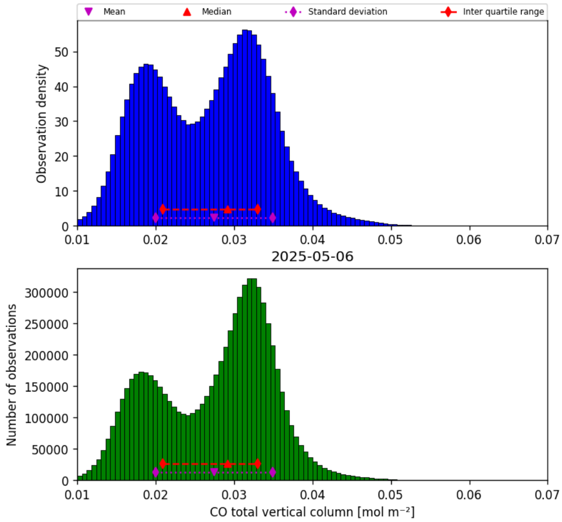
Figure 18: Histogram of “CO total vertical column” for 2025-05-05 to 2025-05-07
