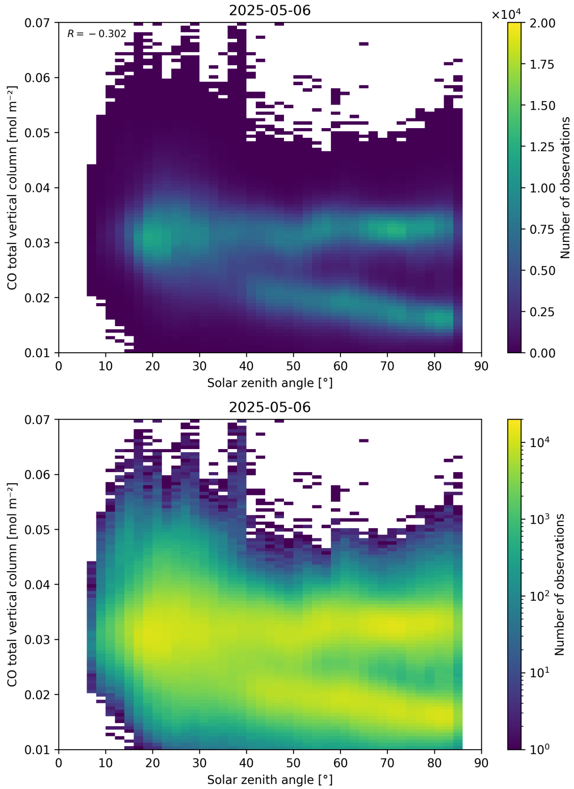
Figure 61: Scatter density plot of “Solar zenith angle” against “CO total vertical column” for 2025-05-05 to 2025-05-07.
