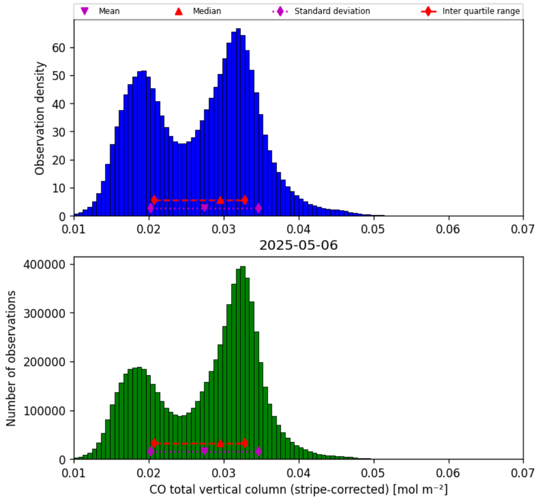
Figure 19: Histogram of “CO total vertical column (stripe-corrected)” for 2025-05-05 to 2025-05-07
