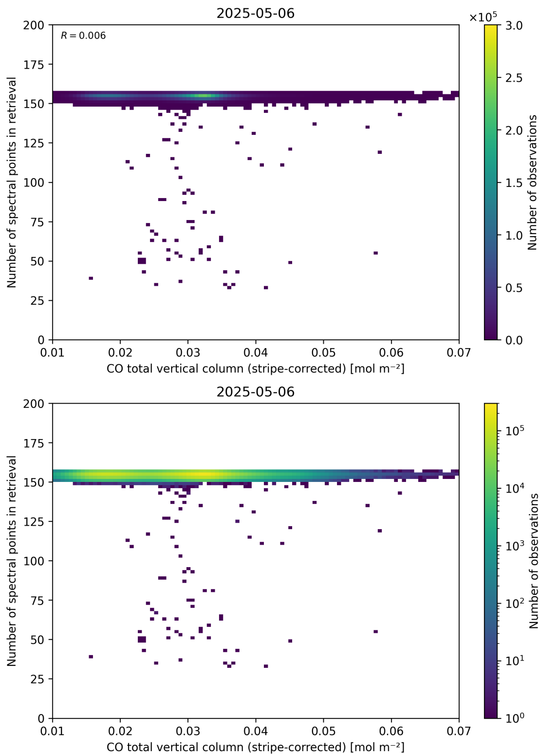
Figure 40: Scatter density plot of “CO total vertical column (stripe-corrected)” against “Number of spectral points in retrieval” for 2025-05-05 to 2025-05-07.
