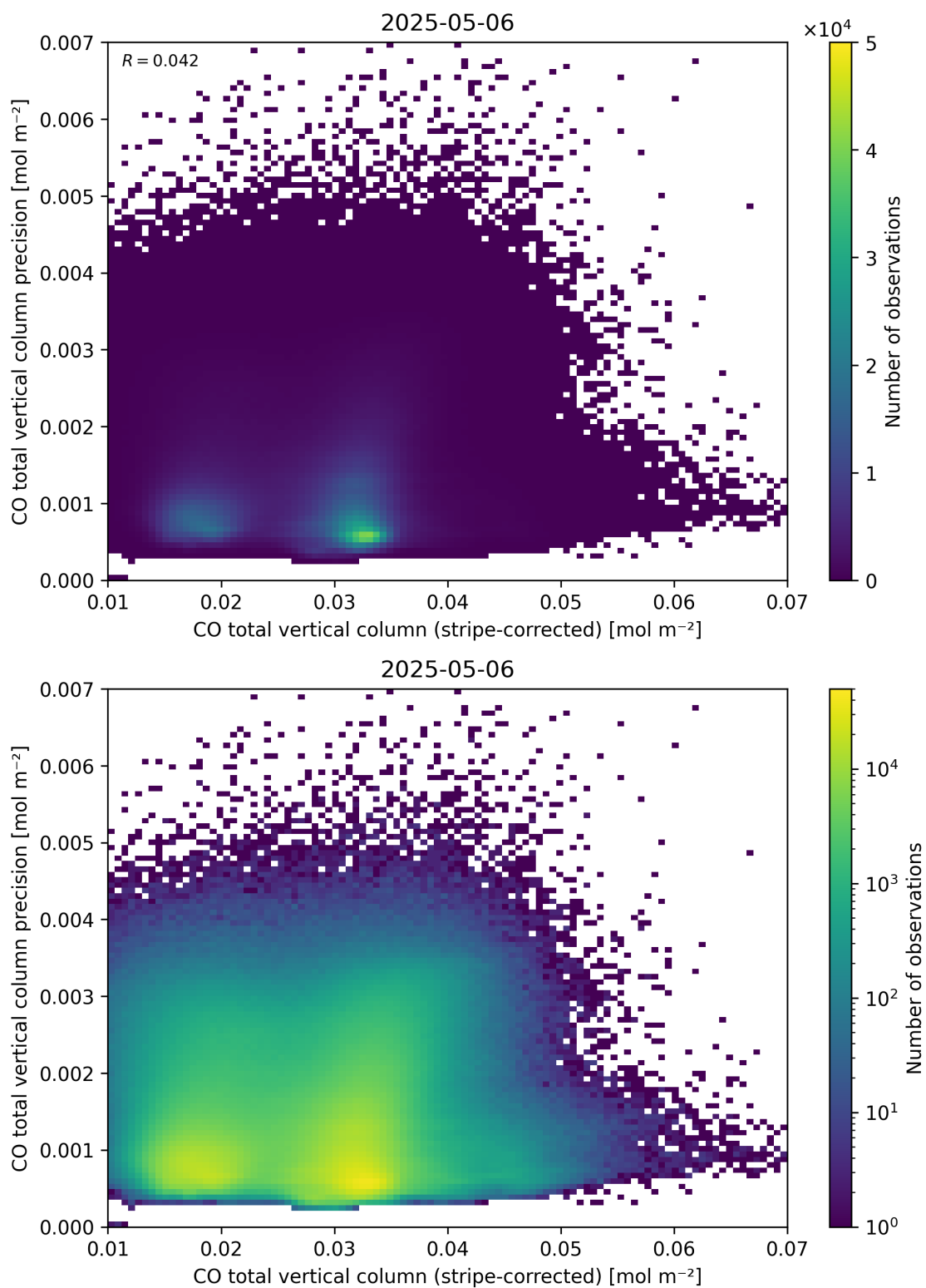
Figure 36: Scatter density plot of “CO total vertical column (stripe-corrected)” against “CO total vertical column precision” for 2025-05-05 to 2025-05-07.
