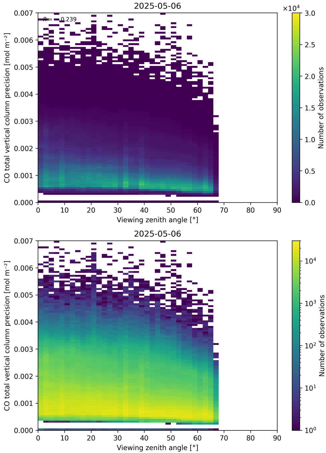
Figure 71: Scatter density plot of “Viewing zenith angle” against “CO total vertical column precision” for 2025-05-05 to 2025-05-07.
