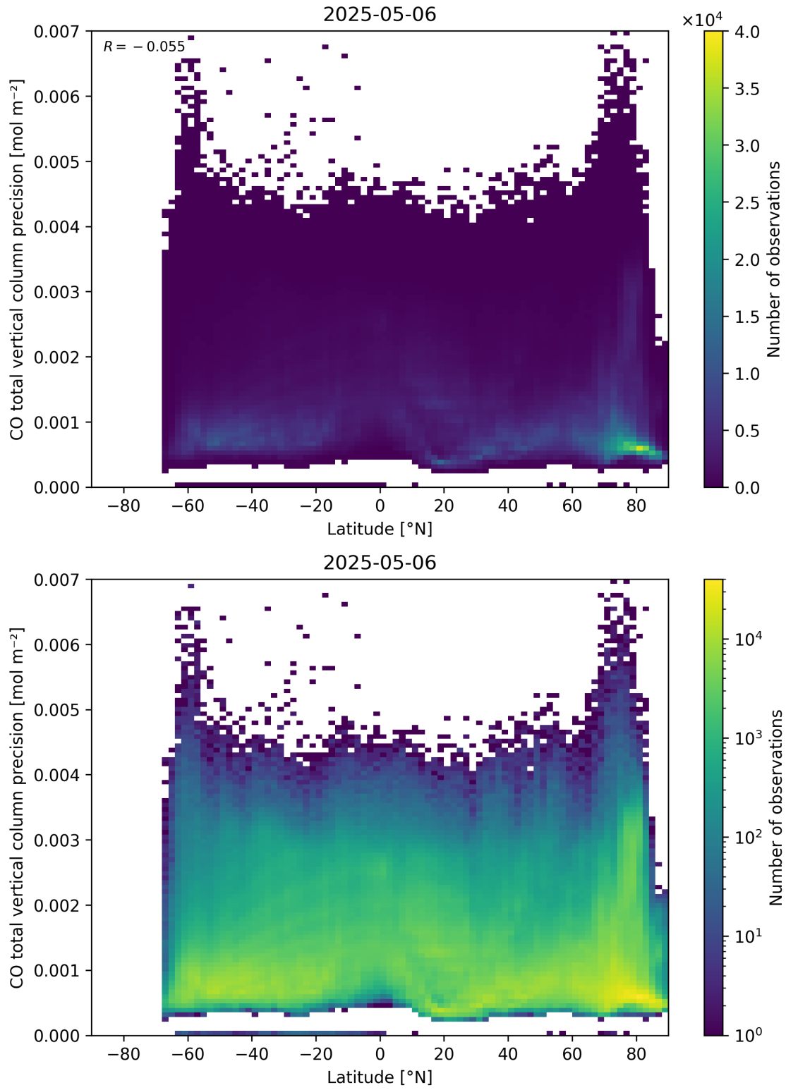
Figure 53: Scatter density plot of “Latitude” against “CO total vertical column precision” for 2025-05-05 to 2025-05-07.
