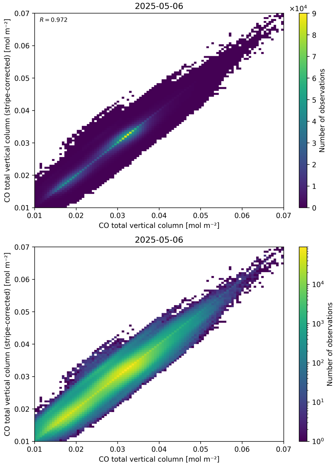
Figure 33: Scatter density plot of “CO total vertical column” against “CO total vertical column (stripe-corrected)” for 2025-05-05 to 2025-05-07.
