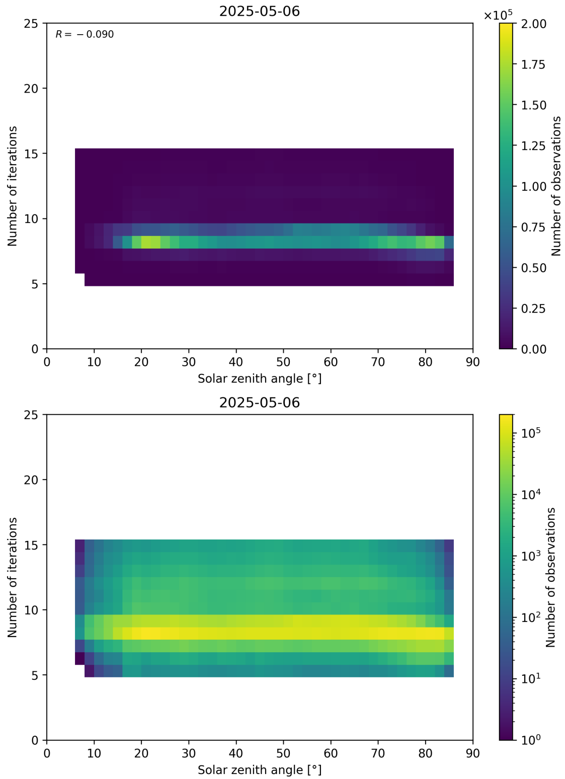
Figure 67: Scatter density plot of “Solar zenith angle” against “Number of iterations” for 2025-05-05 to 2025-05-07.
