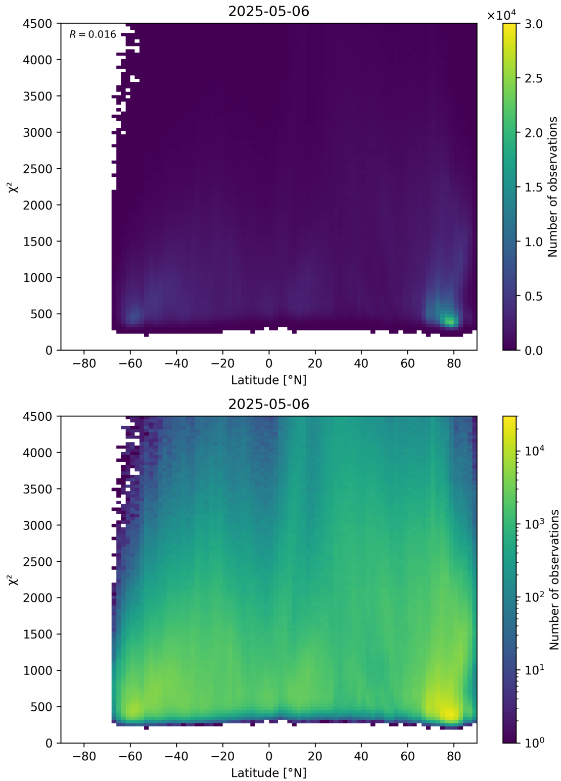
Figure 54: Scatter density plot of “Latitude” against “ \chi^2 ” for 2025-05-05 to 2025-05-07.
