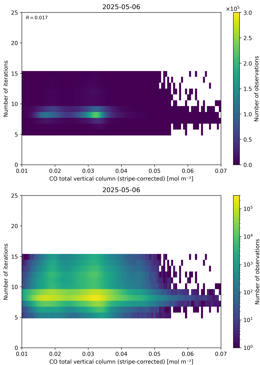
Figure 39: Scatter density plot of “CO total vertical column (stripe-corrected)” against “Number of iterations” for 2025-05-05 to 2025-05-07.
