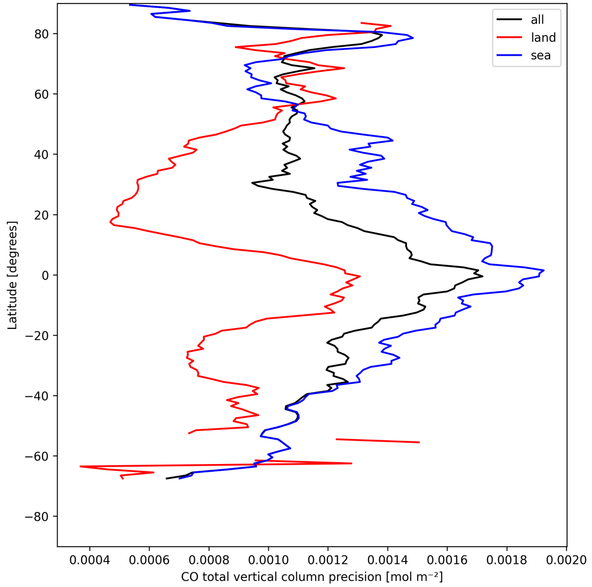
Figure 12: Zonal average of “CO total vertical column precision” for 2025-05-05 to 2025-05-07.
