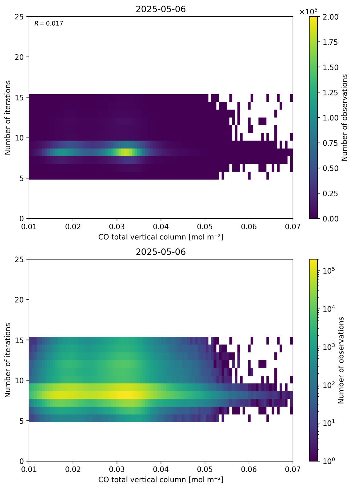
Figure 42: Scatter density plot of “CO total vertical column” against “Number of iterations” for 2025-05-05 to 2025-05-07.
