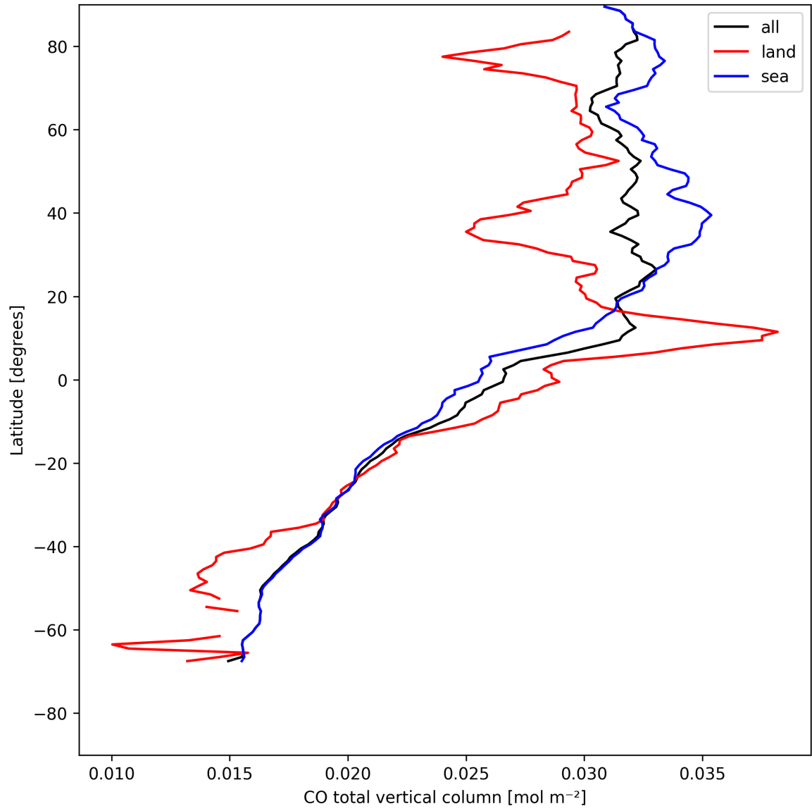
Figure 10: Zonal average of “CO total vertical column” for 2025-05-05 to 2025-05-07.
