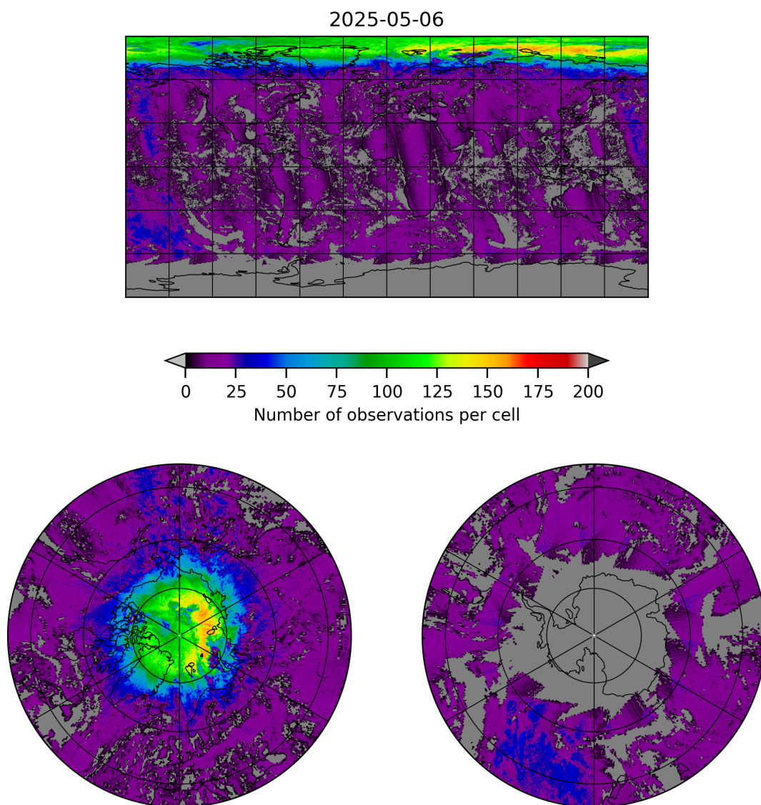
Figure 8: Map of the number of observations for 2025-05-05 to 2025-05-07
