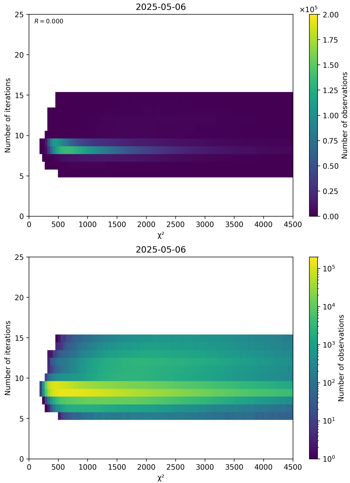
Figure 49: Scatter density plot of “ \chi^2 ” against “Number of iterations” for 2025-05-05 to 2025-05-07.
