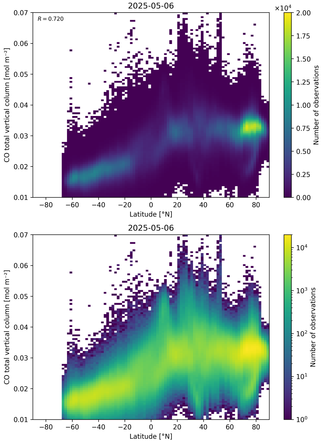
Figure 51: Scatter density plot of “Latitude” against “CO total vertical column” for 2025-05-05 to 2025-05-07.
