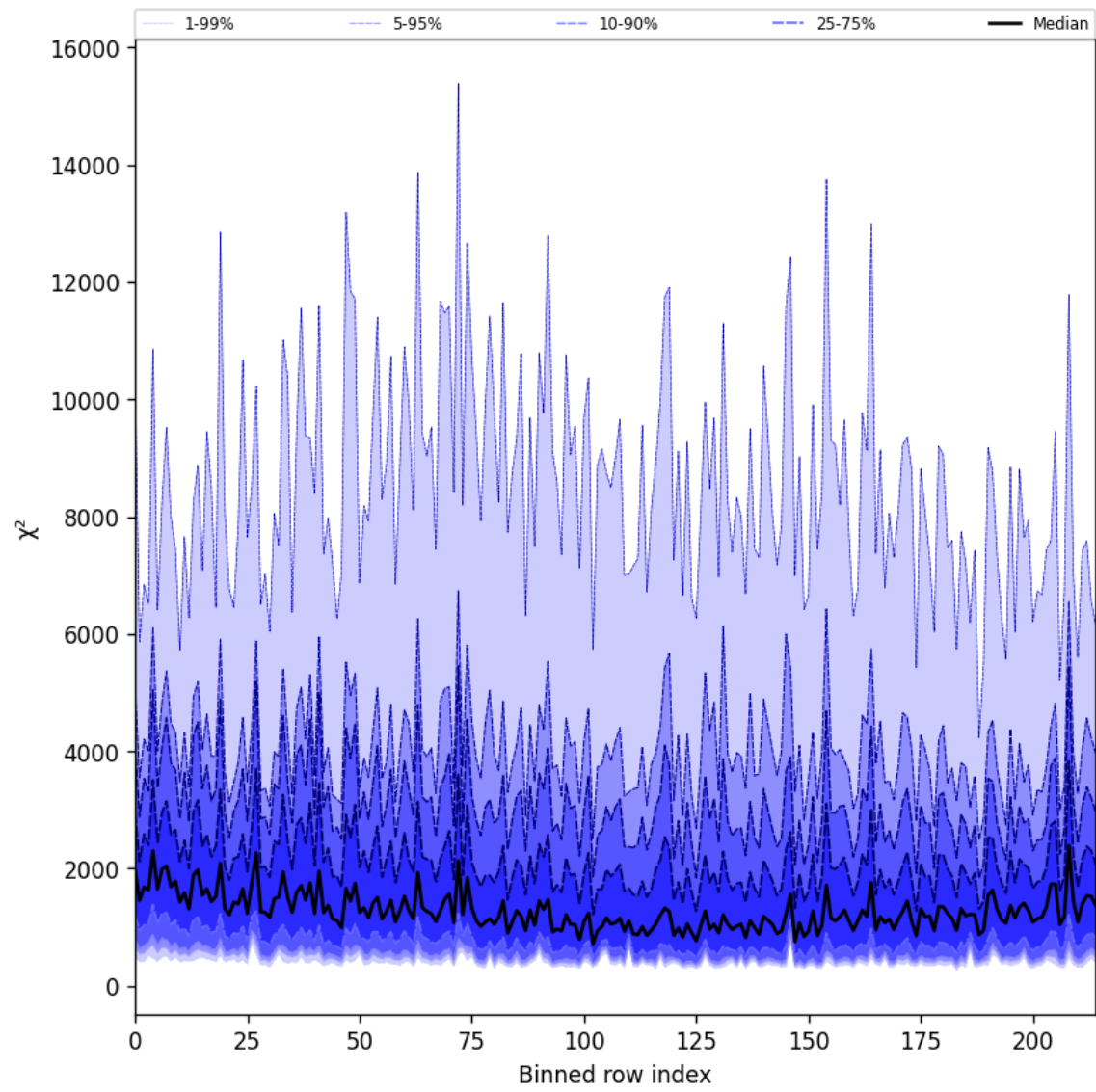
Figure 30: Along track statistics of “ \chi^2 ” for 2025-05-05 to 2025-05-07
