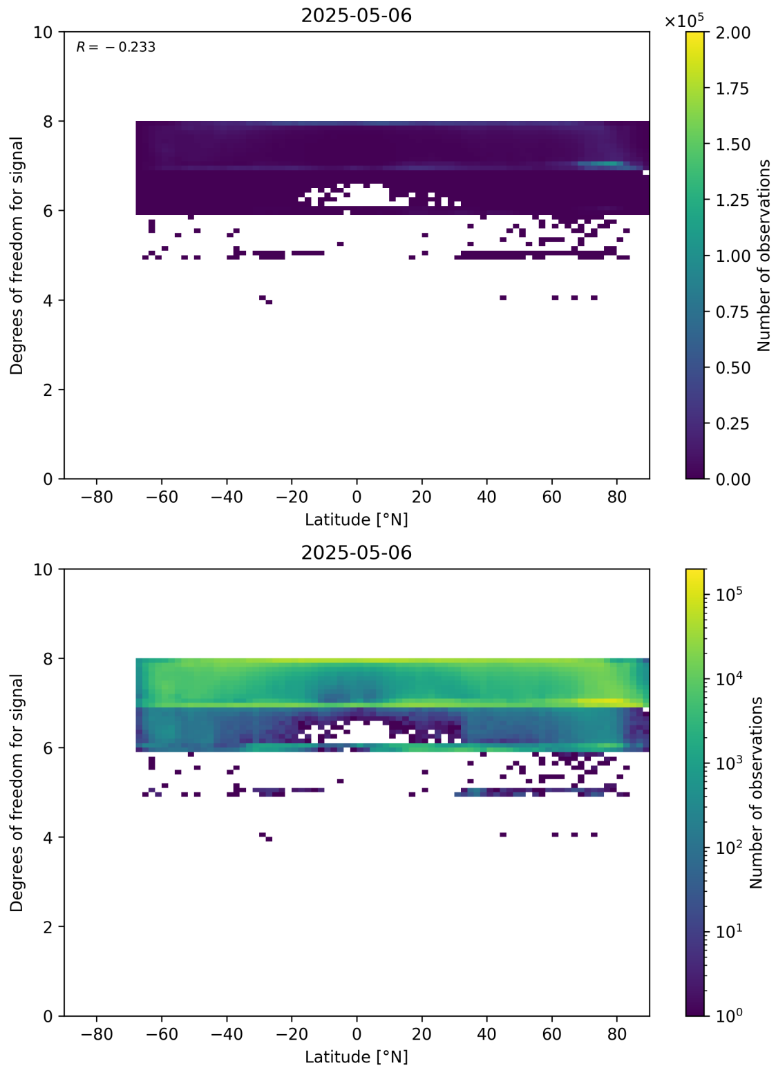
Figure 55: Scatter density plot of “Latitude” against “Degrees of freedom for signal” for 2025-05-05 to 2025-05-07.
