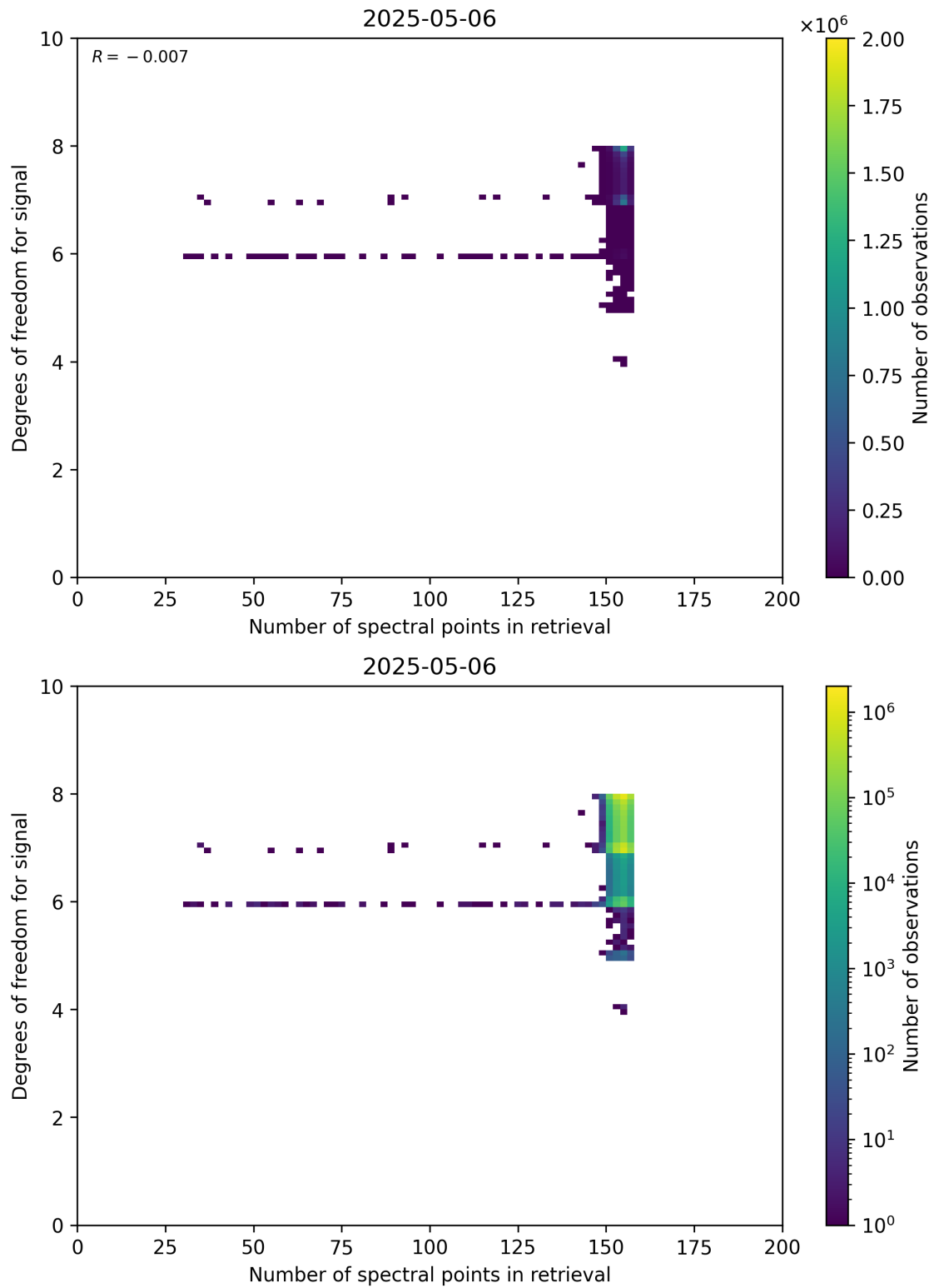
Figure 59: Scatter density plot of “Number of spectral points in retrieval” against “Degrees of freedom for signal” for 2025-05-05 to 2025-05-07.
