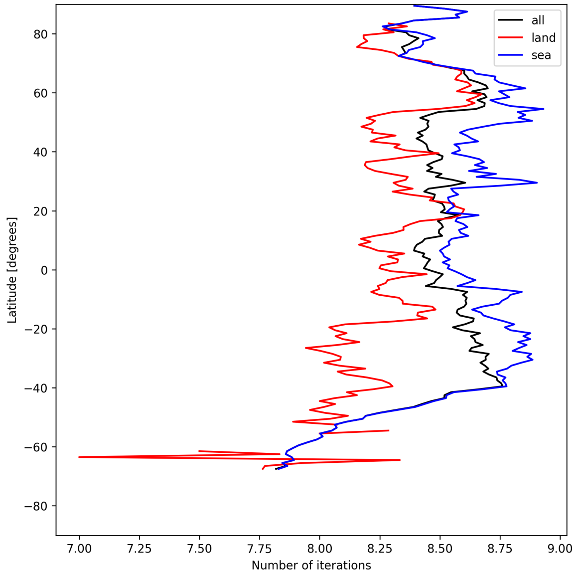
Figure 16: Zonal average of “Number of iterations” for 2025-05-05 to 2025-05-07.
