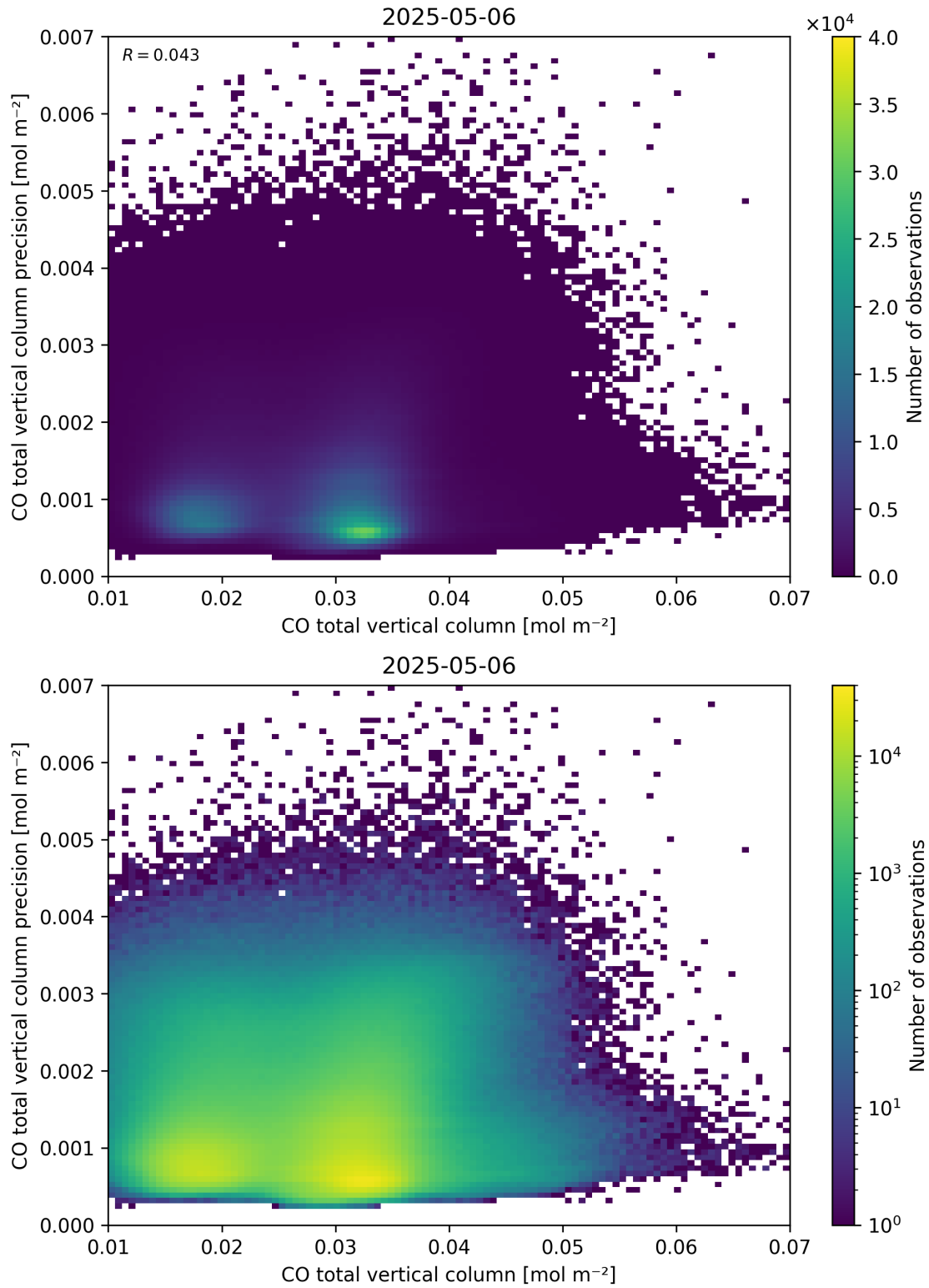
Figure 34: Scatter density plot of “CO total vertical column” against “CO total vertical column precision” for 2025-05-05 to 2025-05-07.
