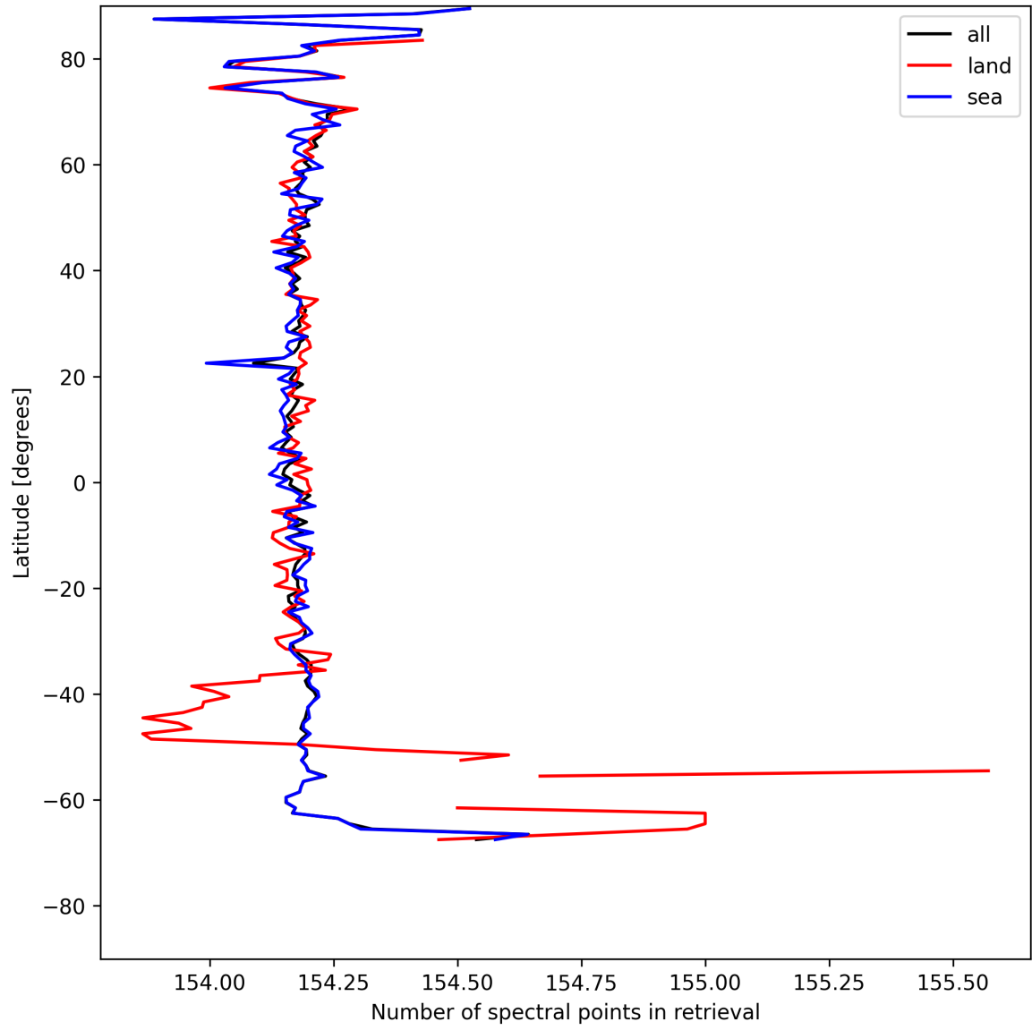
Figure 13: Zonal average of “Number of spectral points in retrieval” for 2025-05-05 to 2025-05-07.
