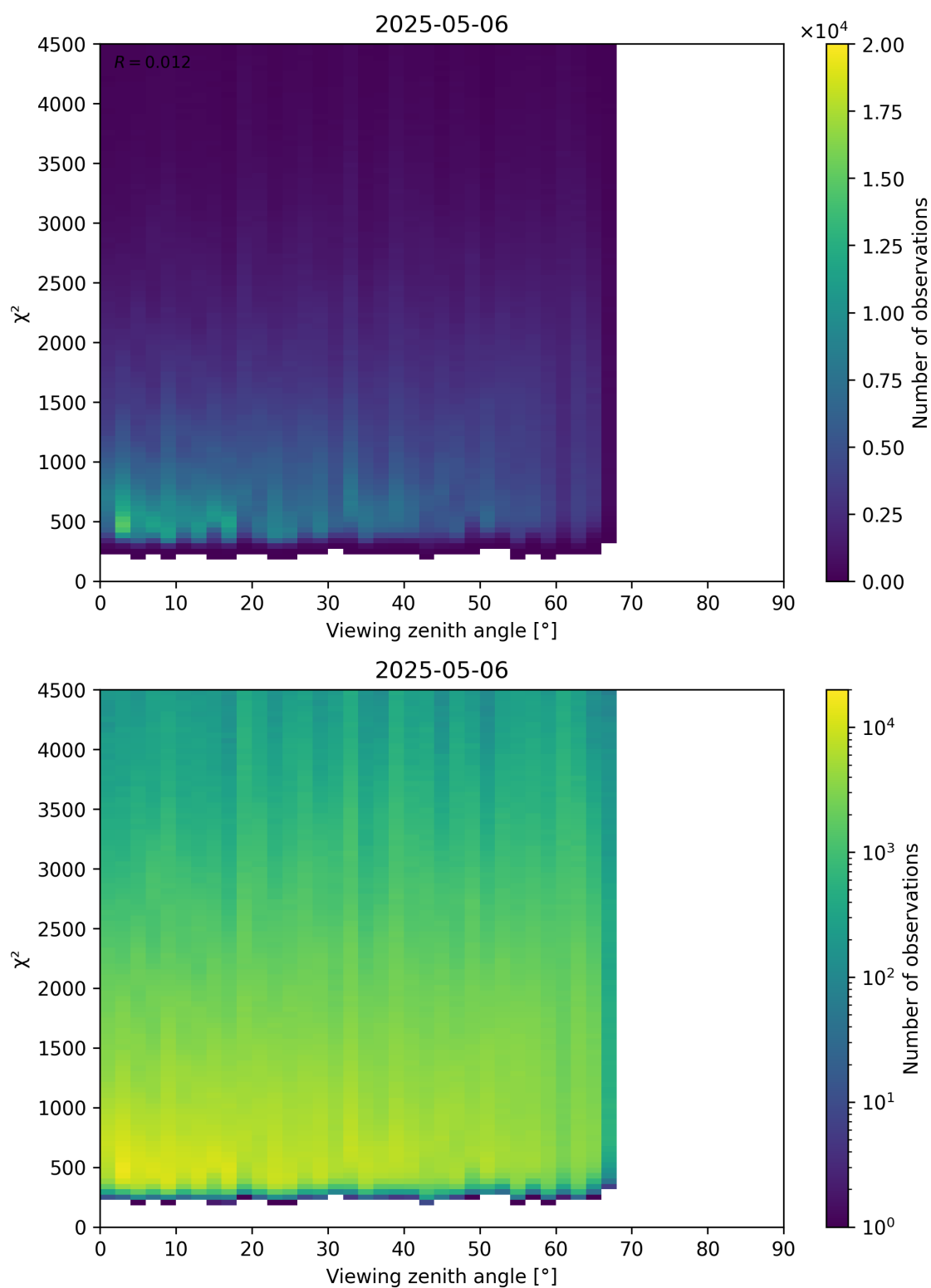
Figure 72: Scatter density plot of “Viewing zenith angle” against “ \chi^2 ” for 2025-05-05 to 2025-05-07.
