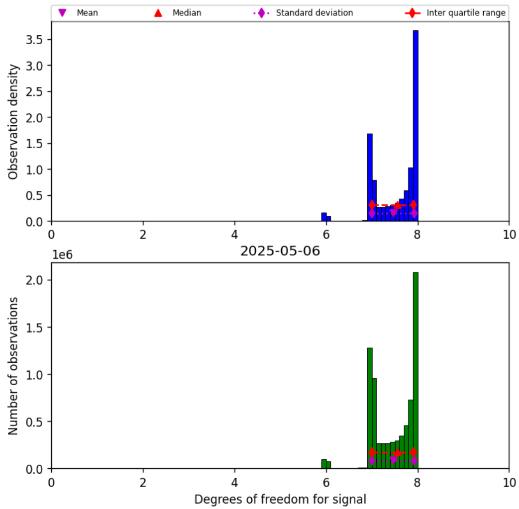
Figure 23: Histogram of “Degrees of freedom for signal” for 2025-05-05 to 2025-05-07
