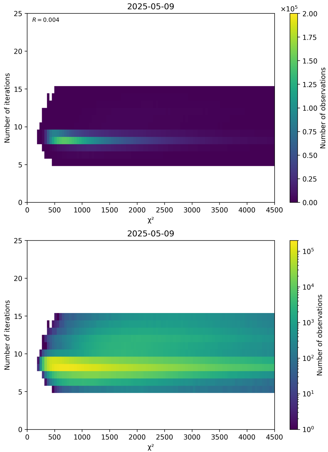
Figure 49: Scatter density plot of “ \chi^2 ” against “Number of iterations” for 2025-05-08 to 2025-05-10.
