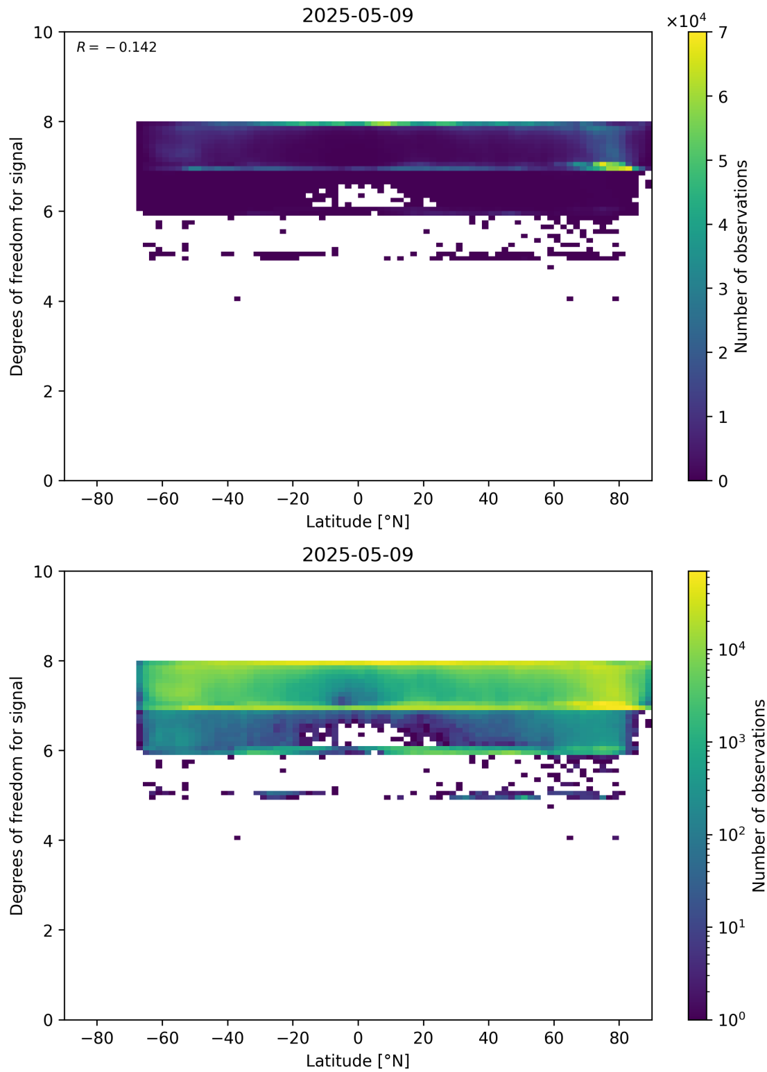
Figure 55: Scatter density plot of “Latitude” against “Degrees of freedom for signal” for 2025-05-08 to 2025-05-10.
