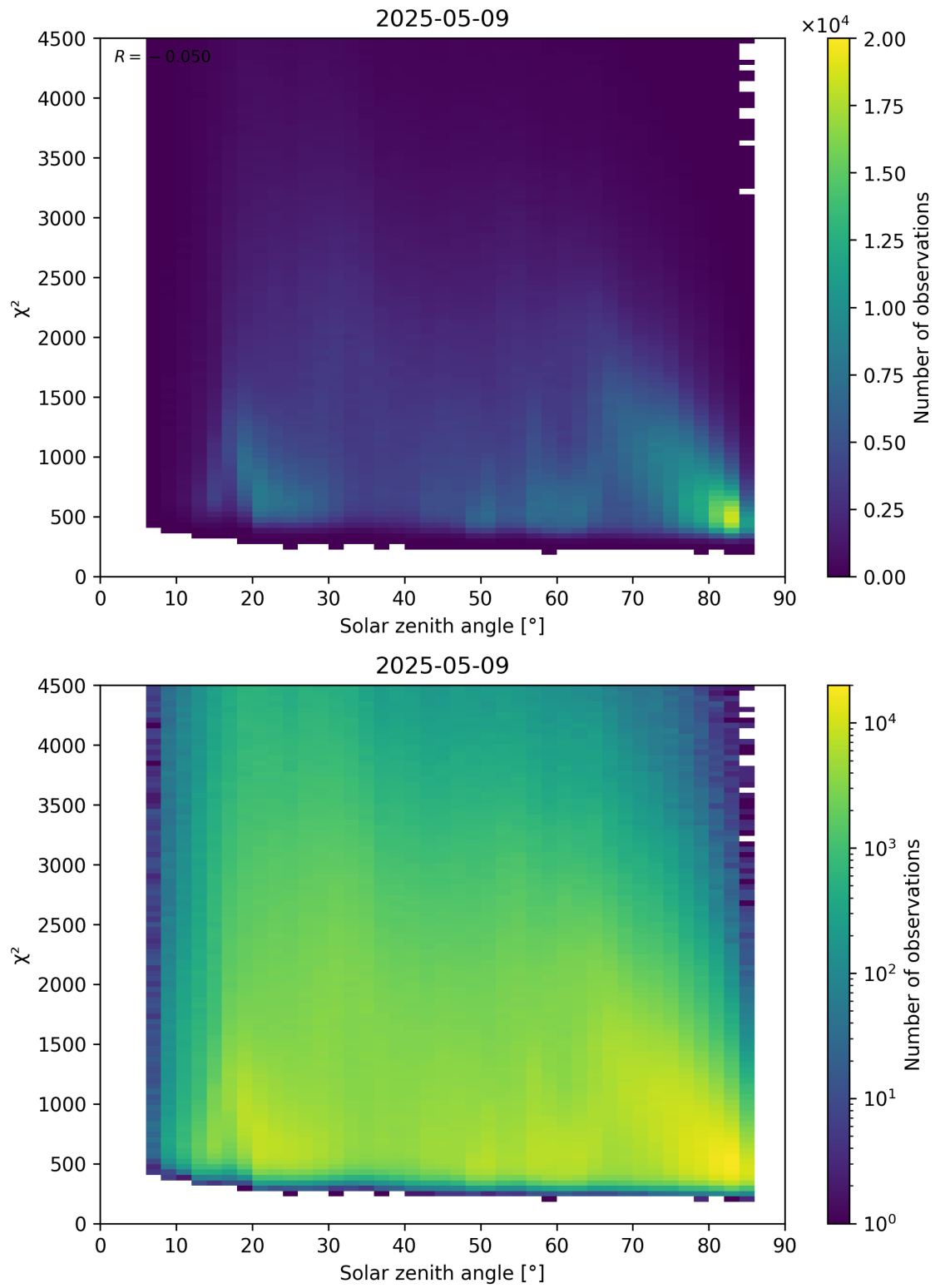
Figure 64: Scatter density plot of “Solar zenith angle” against “ \chi^2 ” for 2025-05-08 to 2025-05-10.
