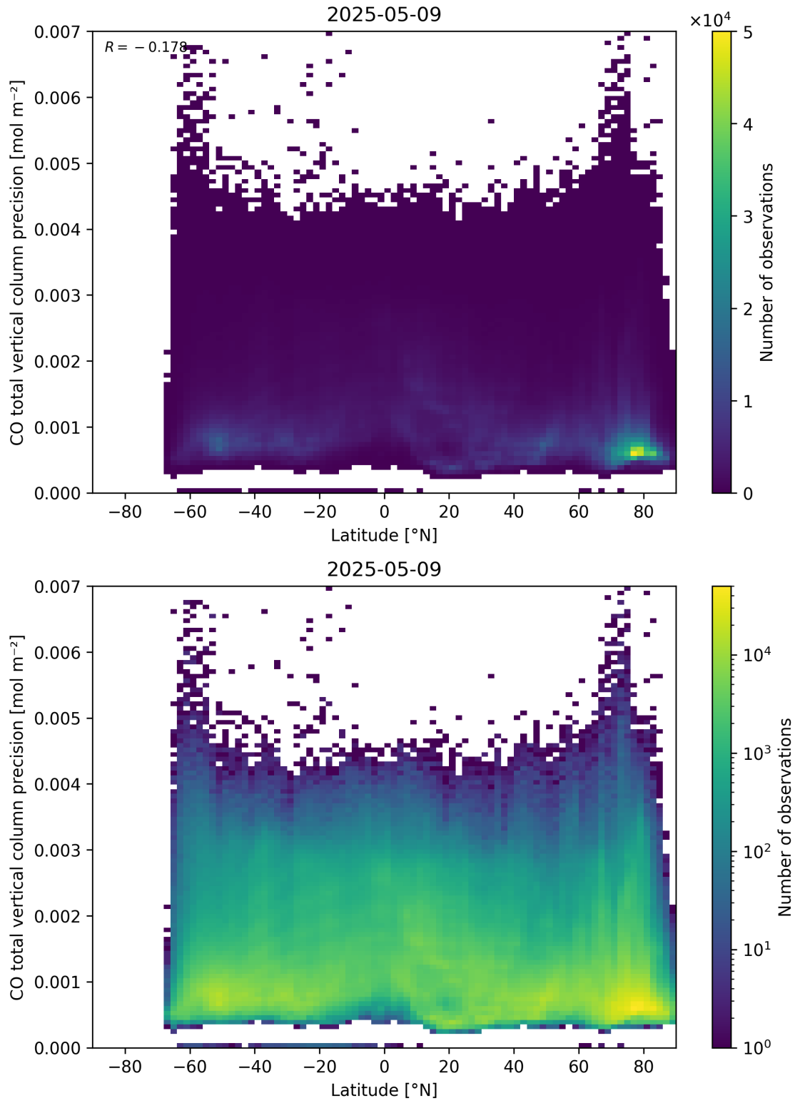
Figure 53: Scatter density plot of “Latitude” against “CO total vertical column precision” for 2025-05-08 to 2025-05-10.
