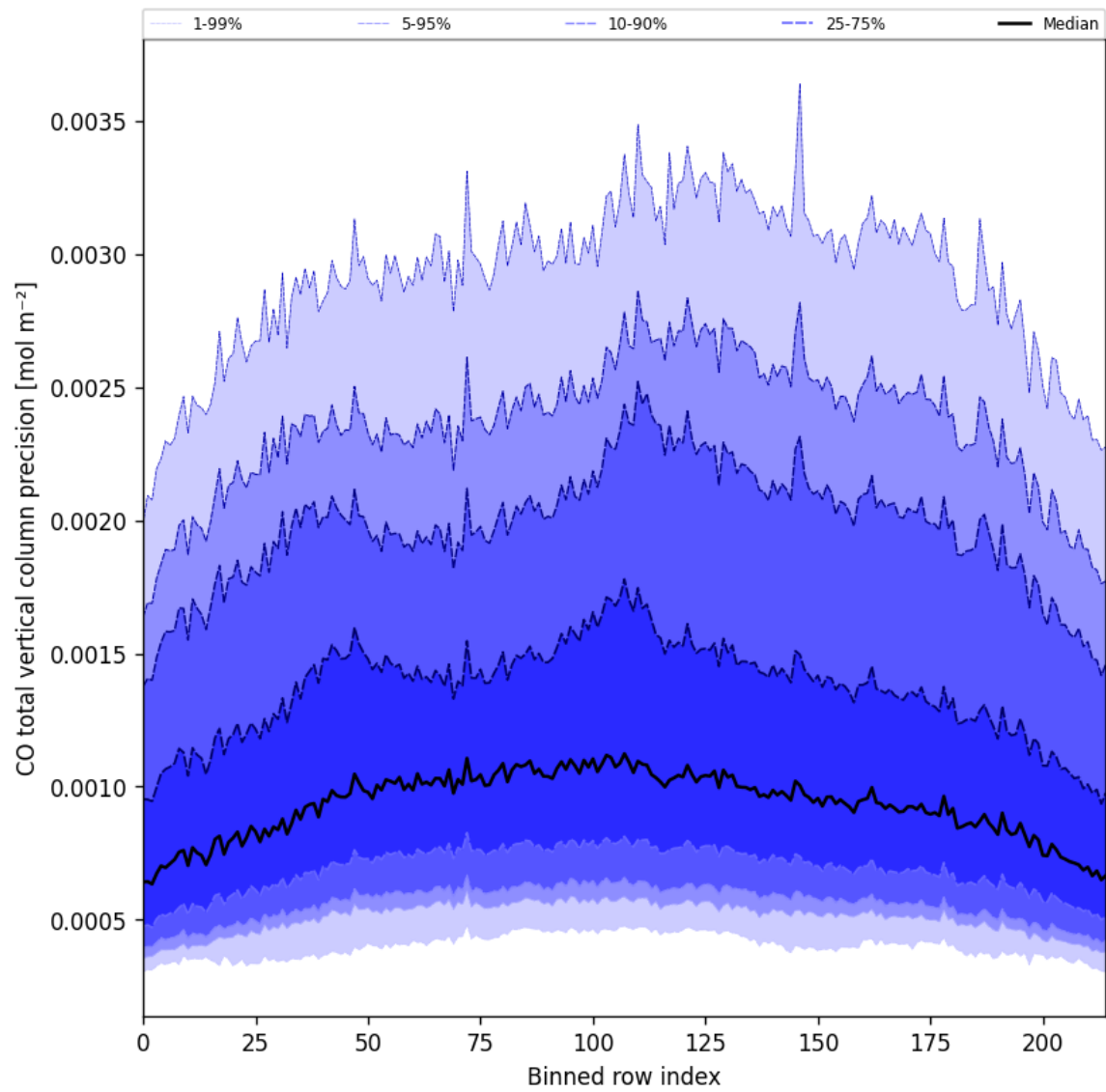
Figure 28: Along track statistics of “CO total vertical column precision” for 2025-05-08 to 2025-05-10
