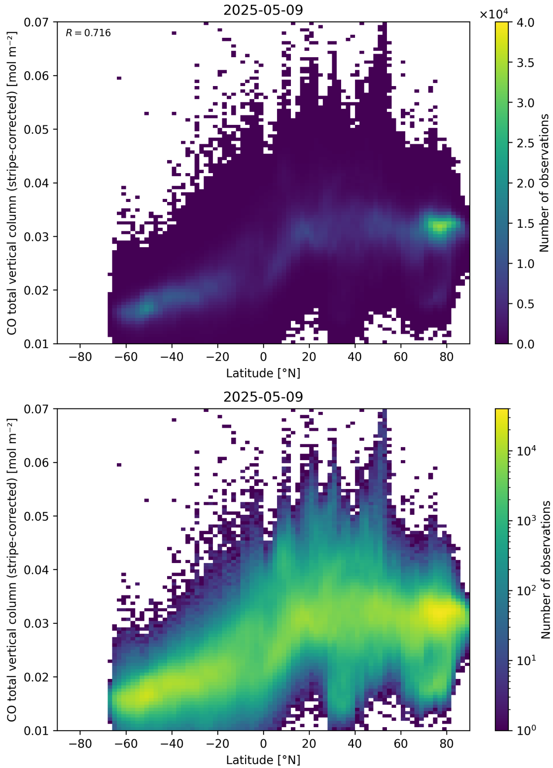
Figure 52: Scatter density plot of “Latitude” against “CO total vertical column (stripe-corrected)” for 2025-05-08 to 2025-05-10.
