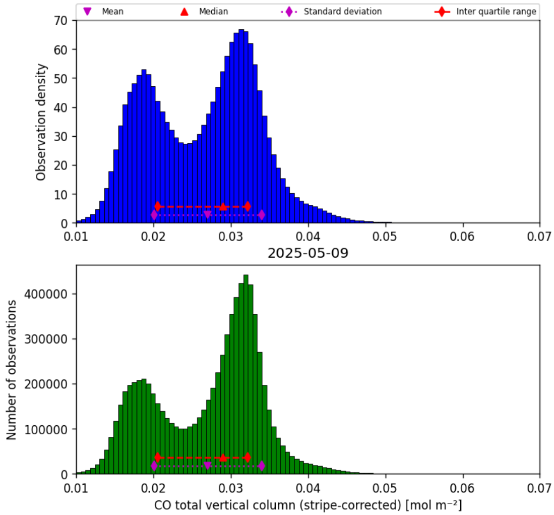
Figure 19: Histogram of “CO total vertical column (stripe-corrected)” for 2025-05-08 to 2025-05-10
