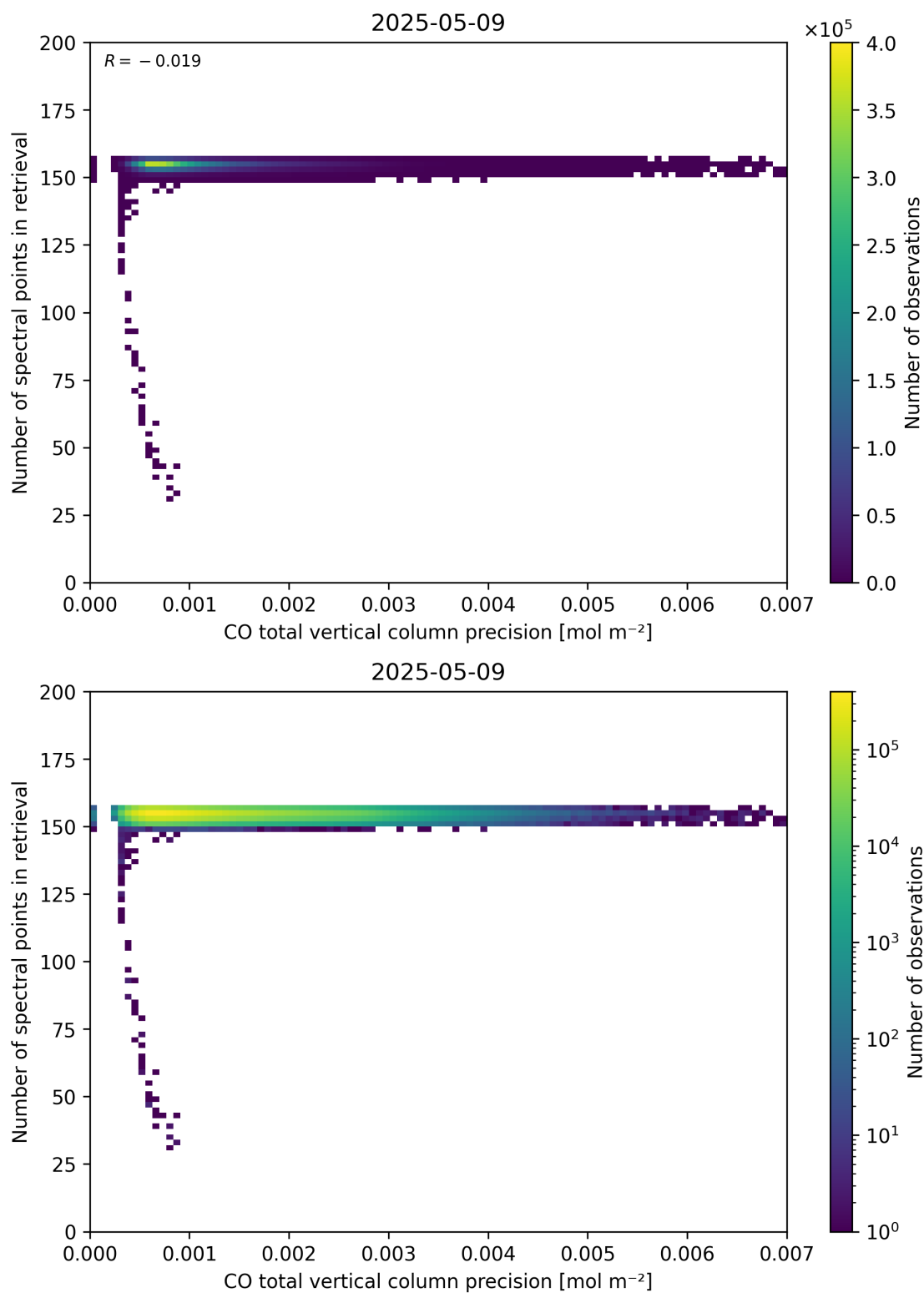
Figure 47: Scatter density plot of “CO total vertical column precision” against “Number of spectral points in retrieval” for 2025-05-08 to 2025-05-10.
