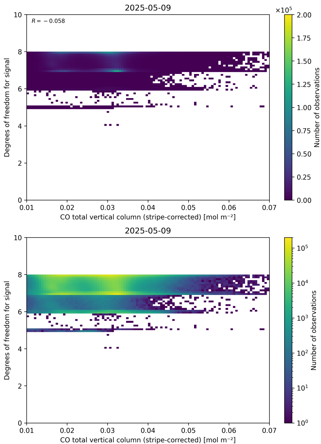
Figure 38: Scatter density plot of “CO total vertical column (stripe-corrected)” against “Degrees of freedom for signal” for 2025-05-08 to 2025-05-10.
