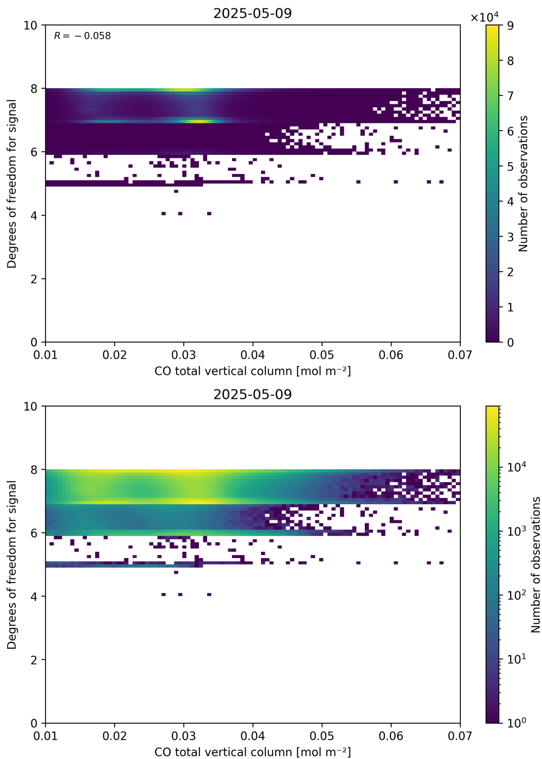
Figure 41: Scatter density plot of “CO total vertical column” against “Degrees of freedom for signal” for 2025-05-08 to 2025-05-10.
