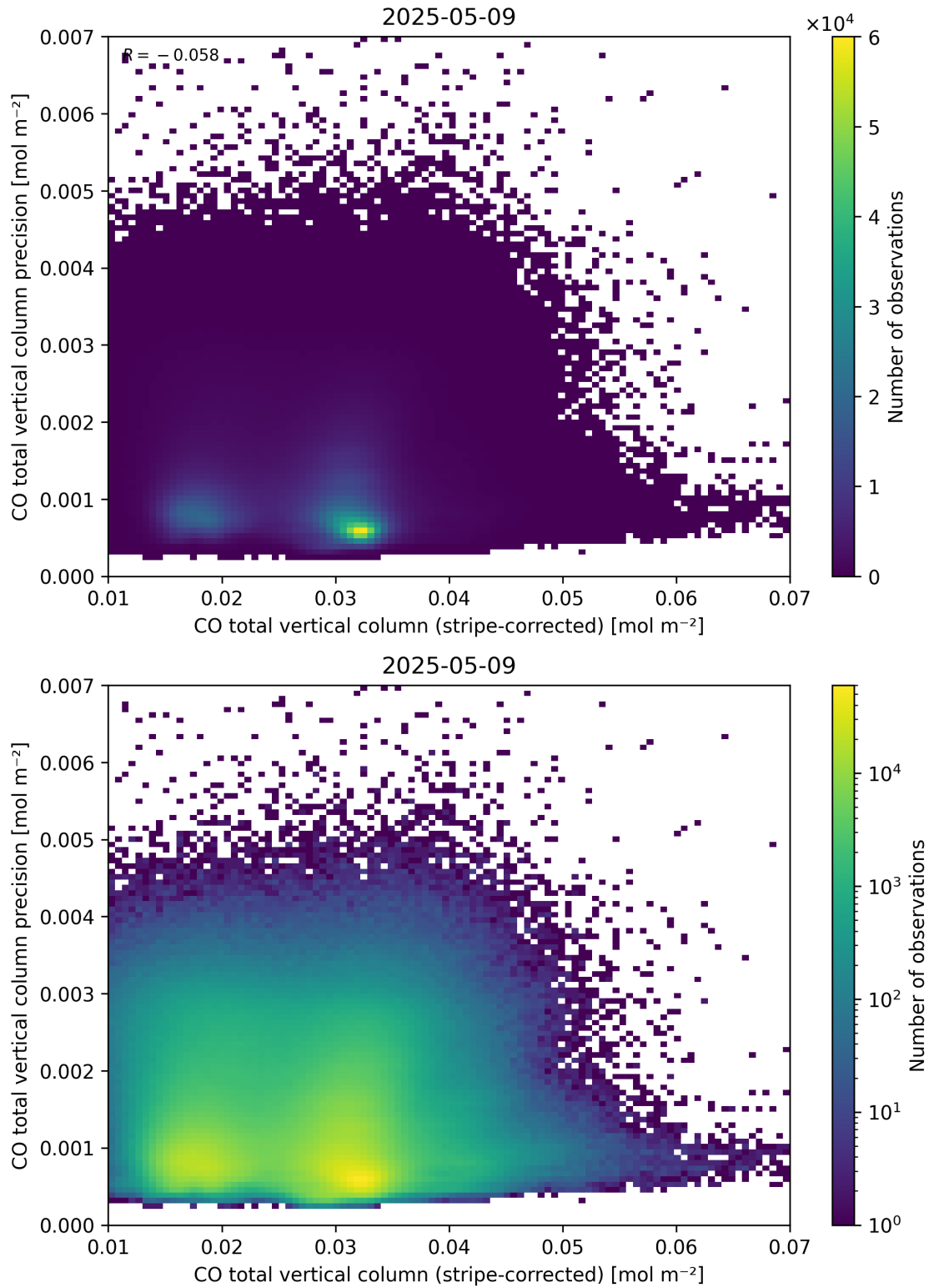
Figure 36: Scatter density plot of “CO total vertical column (stripe-corrected)” against “CO total vertical column precision” for 2025-05-08 to 2025-05-10.
