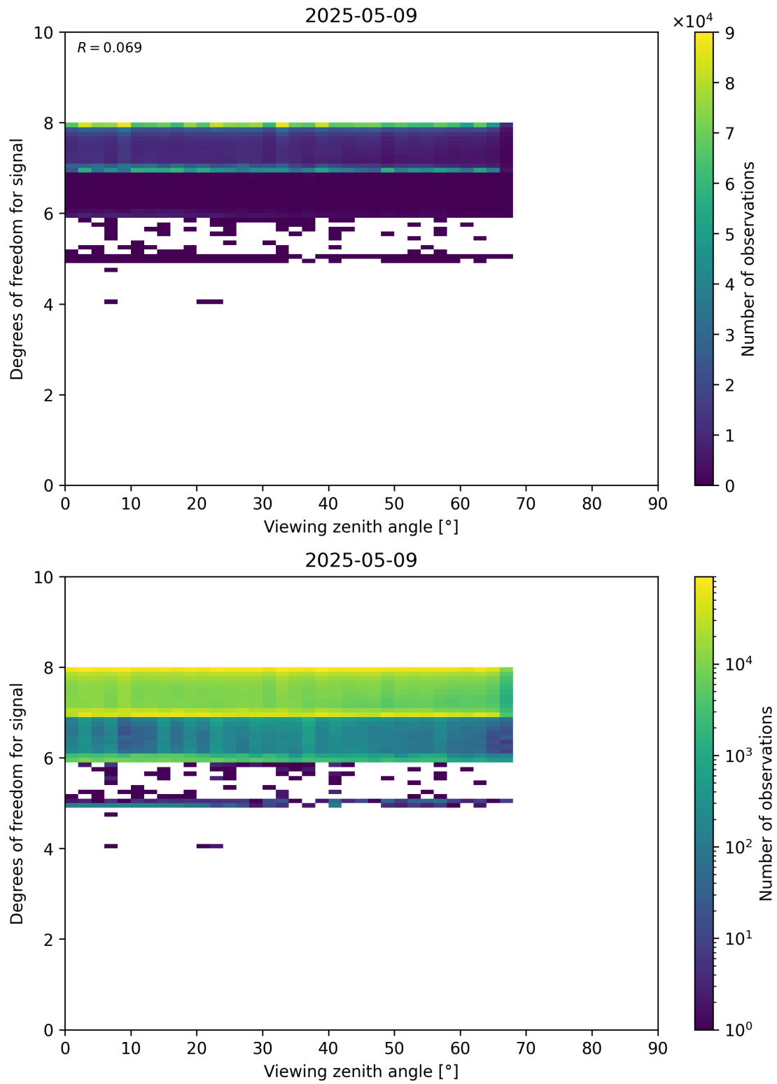
Figure 73: Scatter density plot of “Viewing zenith angle” against “Degrees of freedom for signal” for 2025-05-08 to 2025-05-10.
