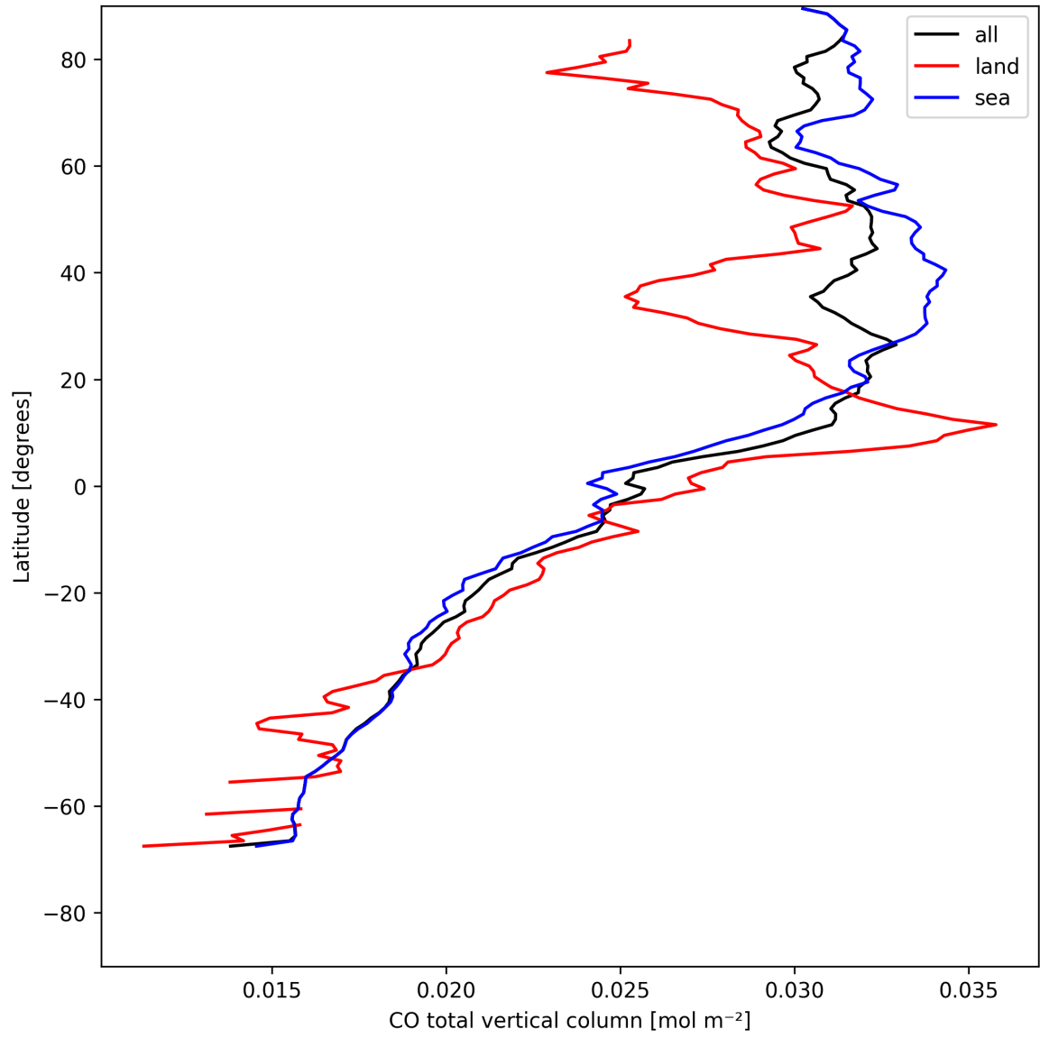
Figure 10: Zonal average of “CO total vertical column” for 2025-05-08 to 2025-05-10.
