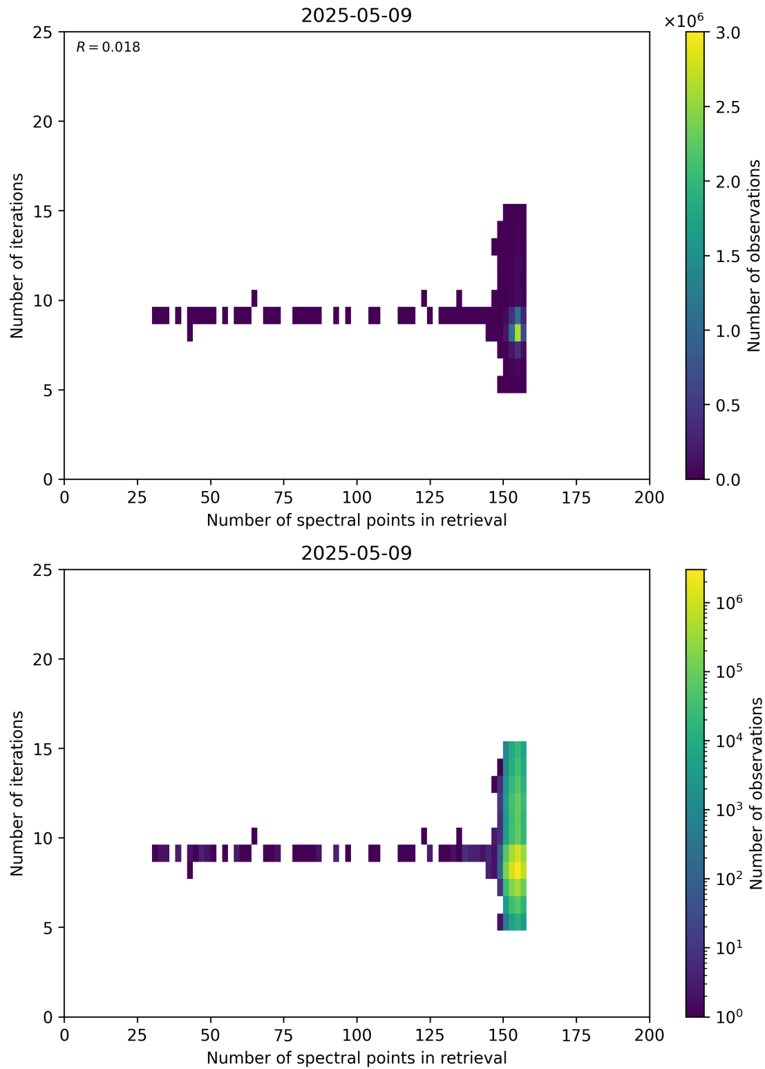
Figure 60: Scatter density plot of “Number of spectral points in retrieval” against “Number of iterations” for 2025-05-08 to 2025-05-10.
