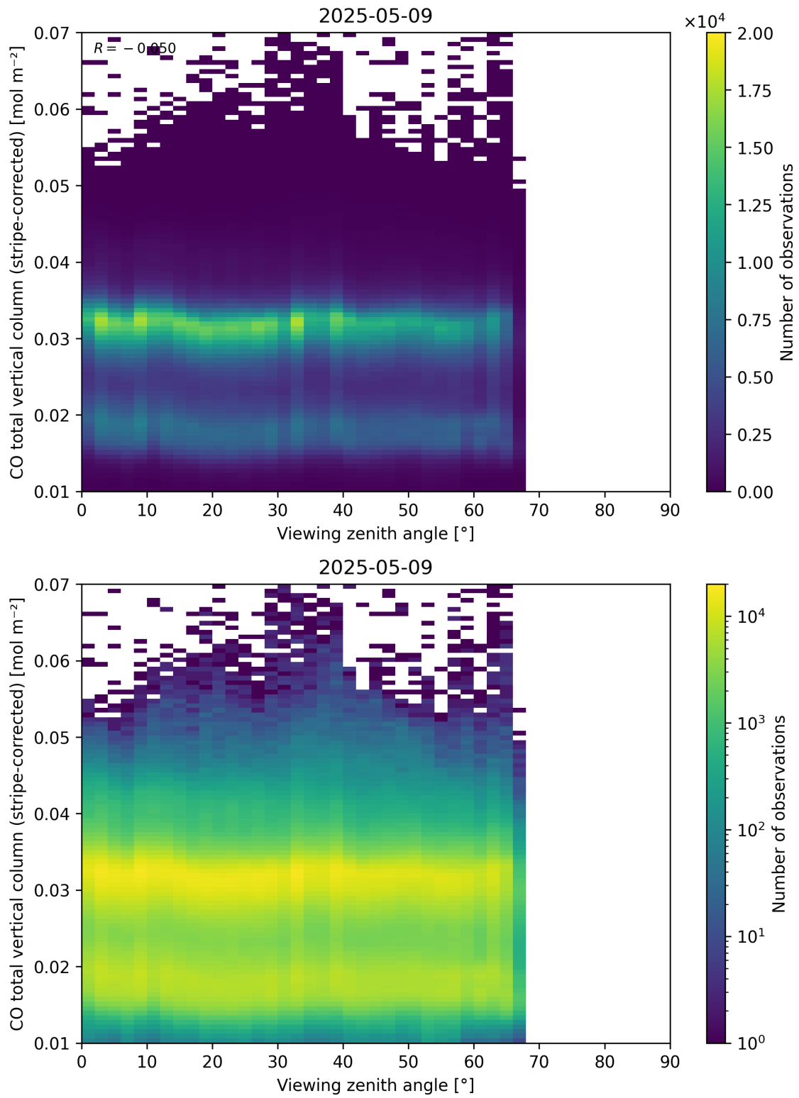
Figure 70: Scatter density plot of “Viewing zenith angle” against “CO total vertical column (stripe-corrected)” for 2025-05-08 to 2025-05-10.
