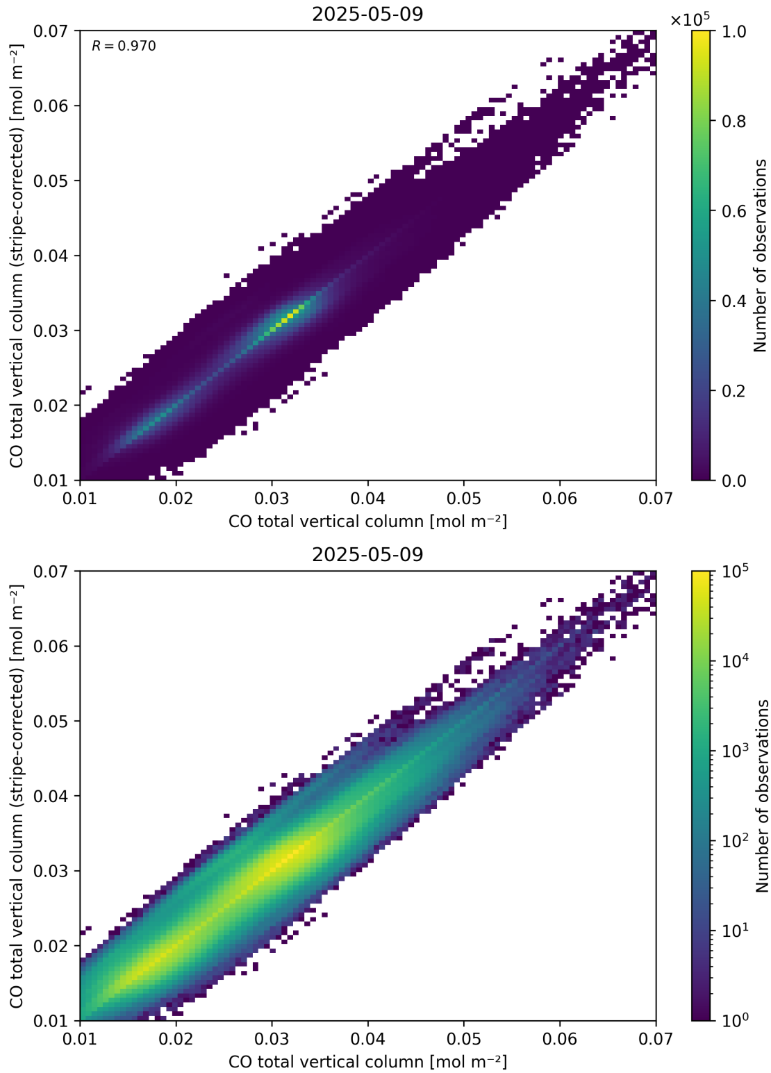
Figure 33: Scatter density plot of “CO total vertical column” against “CO total vertical column (stripe-corrected)” for 2025-05-08 to 2025-05-10.
