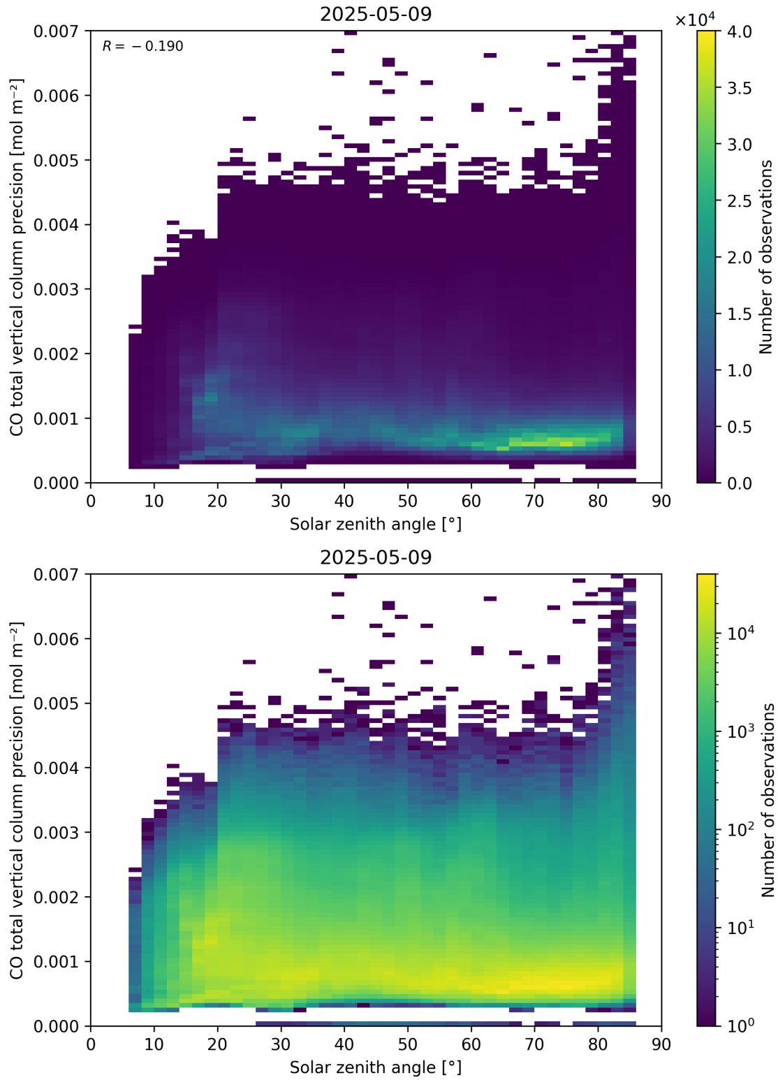
Figure 63: Scatter density plot of “Solar zenith angle” against “CO total vertical column precision” for 2025-05-08 to 2025-05-10.
