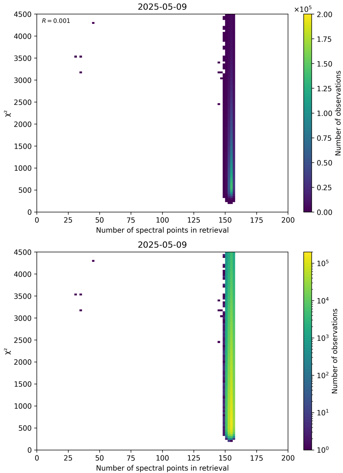
Figure 58: Scatter density plot of “Number of spectral points in retrieval” against “ \chi^2 ” for 2025-05-08 to 2025-05-10.
