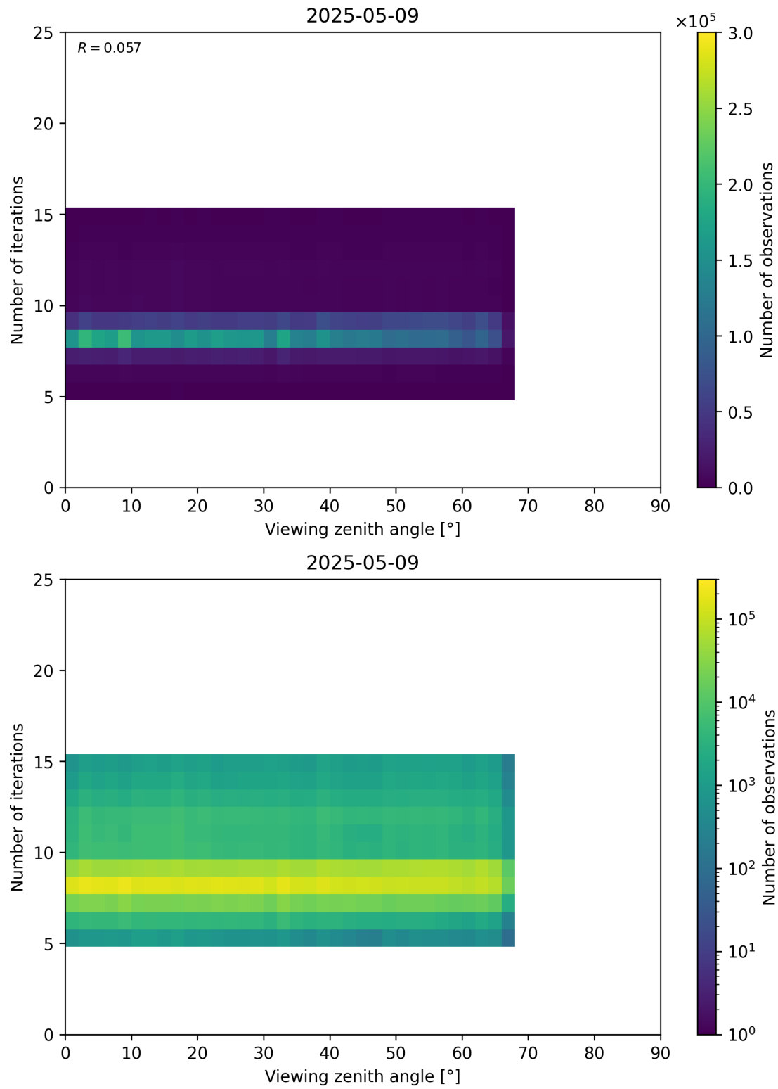
Figure 75: Scatter density plot of “Viewing zenith angle” against “Number of iterations” for 2025-05-08 to 2025-05-10.
