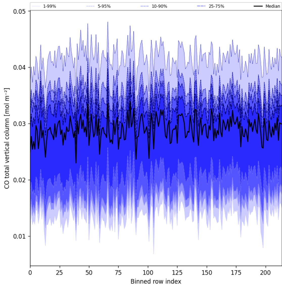
Figure 26: Along track statistics of “CO total vertical column” for 2025-05-08 to 2025-05-10
