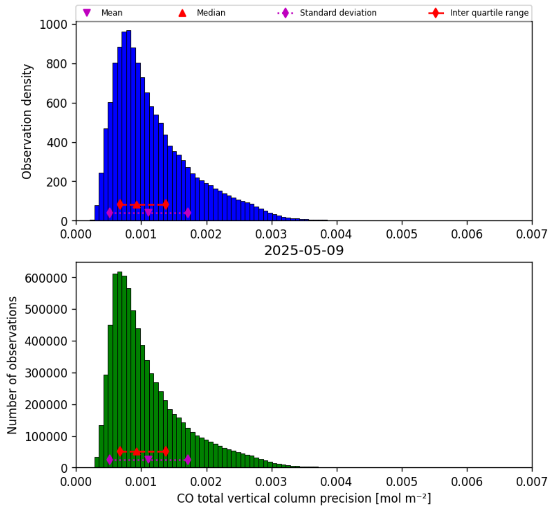
Figure 20: Histogram of “CO total vertical column precision” for 2025-05-08 to 2025-05-10
