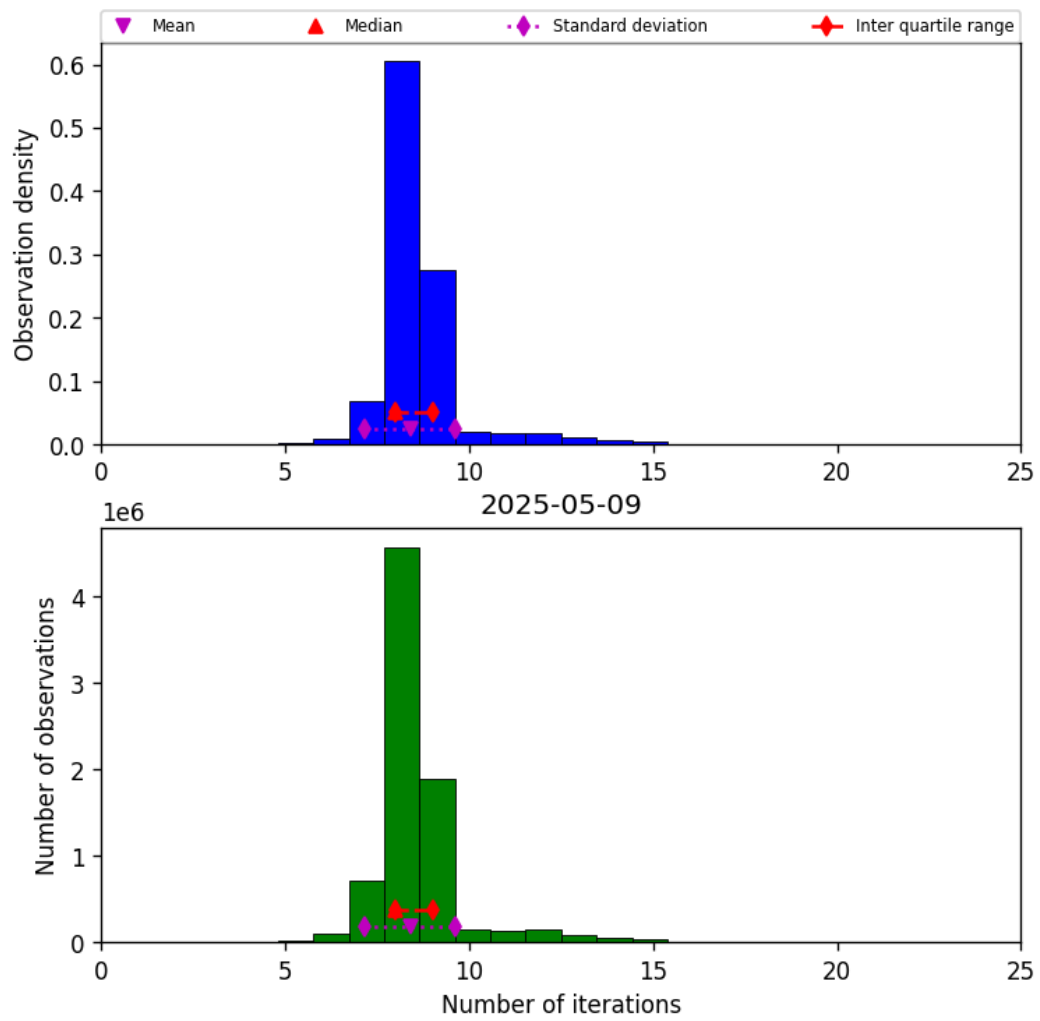
Figure 24: Histogram of “Number of iterations” for 2025-05-08 to 2025-05-10
