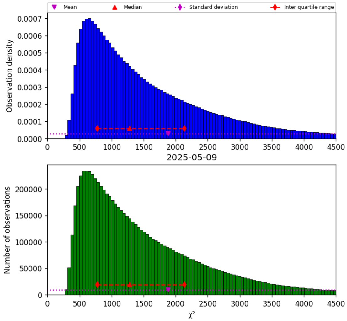
Figure 22: Histogram of “ \chi^2 ” for 2025-05-08 to 2025-05-10
