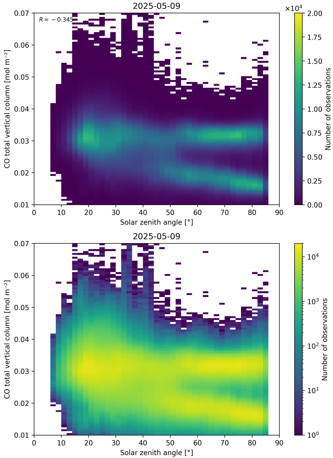
Figure 61: Scatter density plot of “Solar zenith angle” against “CO total vertical column” for 2025-05-08 to 2025-05-10.
