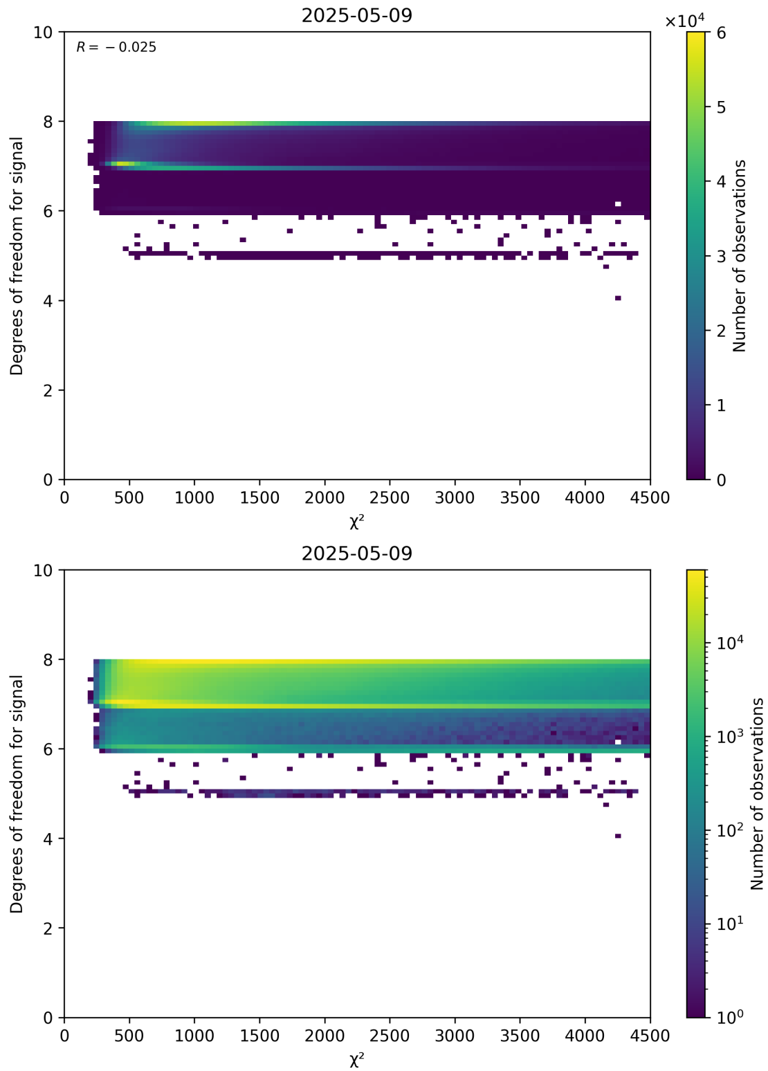
Figure 48: Scatter density plot of “ \chi^2 ” against “Degrees of freedom for signal” for 2025-05-08 to 2025-05-10.
