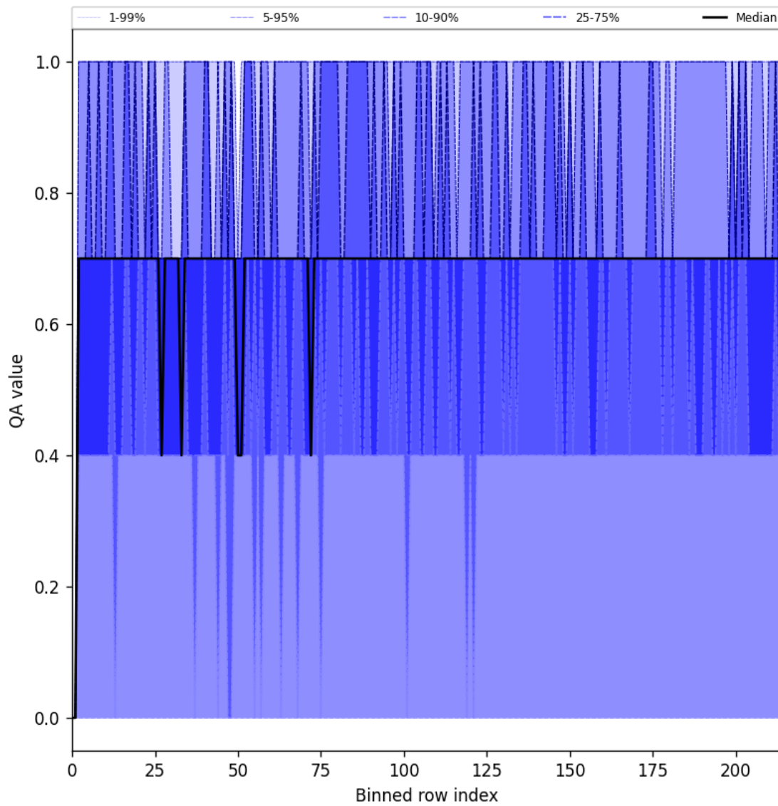
Figure 25: Along track statistics of “QA value” for 2025-05-08 to 2025-05-10
