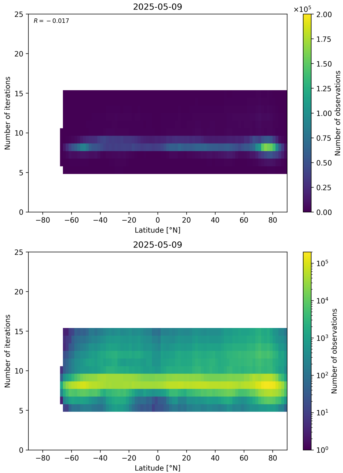
Figure 56: Scatter density plot of “Latitude” against “Number of iterations” for 2025-05-08 to 2025-05-10.
