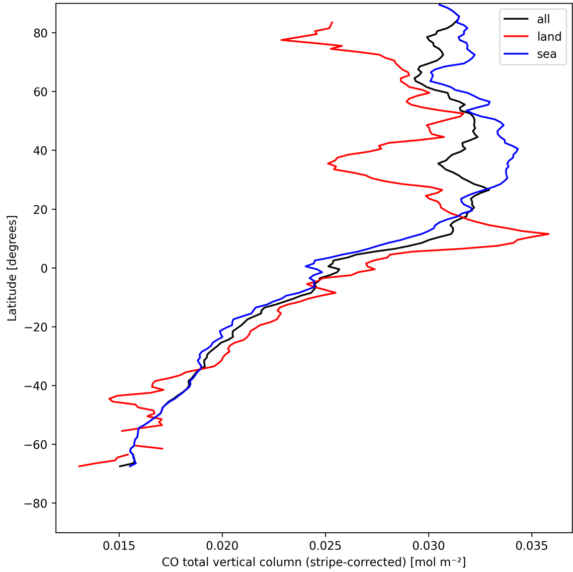
Figure 11: Zonal average of “CO total vertical column (stripe-corrected)” for 2025-05-08 to 2025-05-10.
