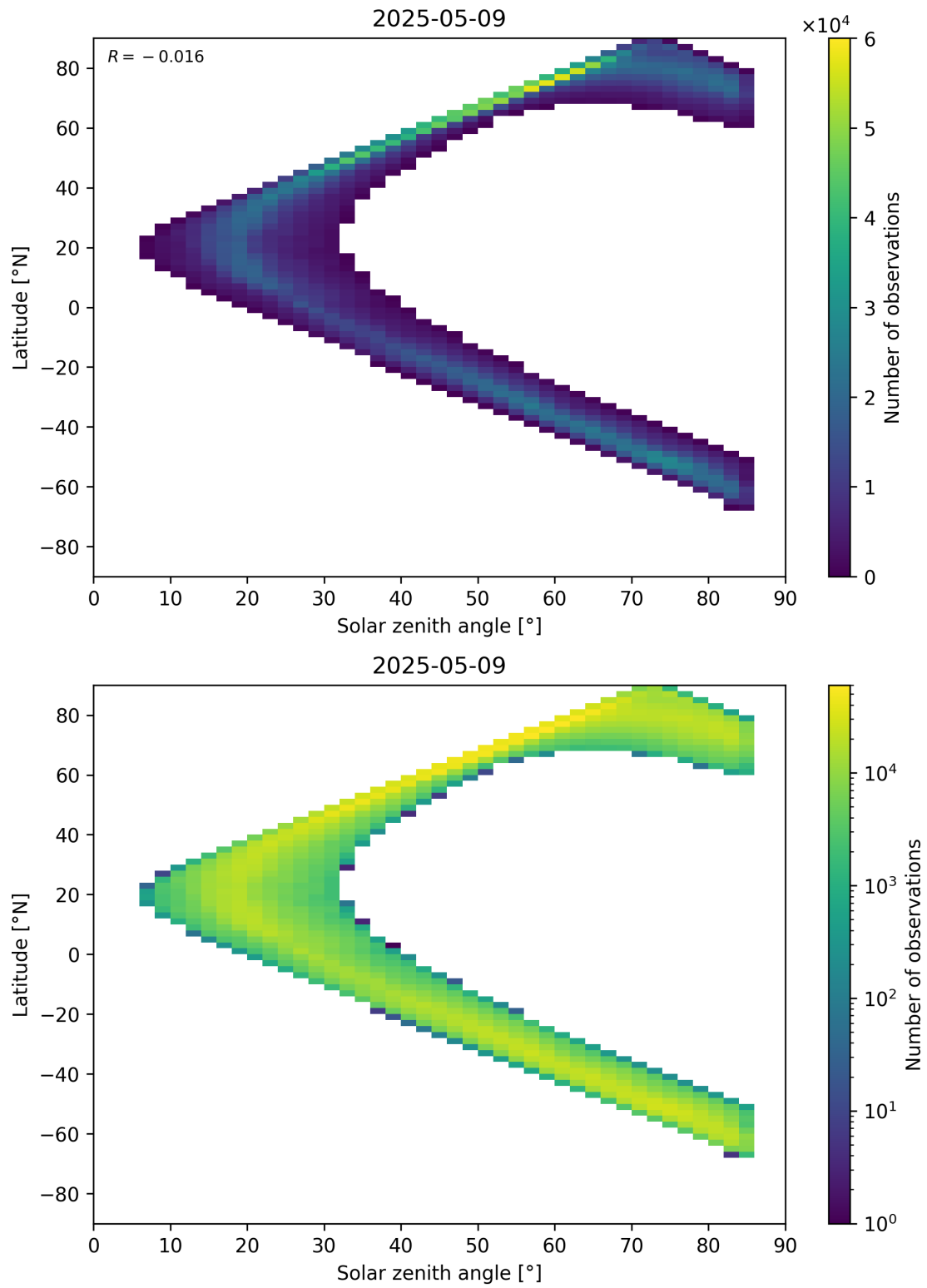
Figure 66: Scatter density plot of “Solar zenith angle” against “Latitude” for 2025-05-08 to 2025-05-10.
