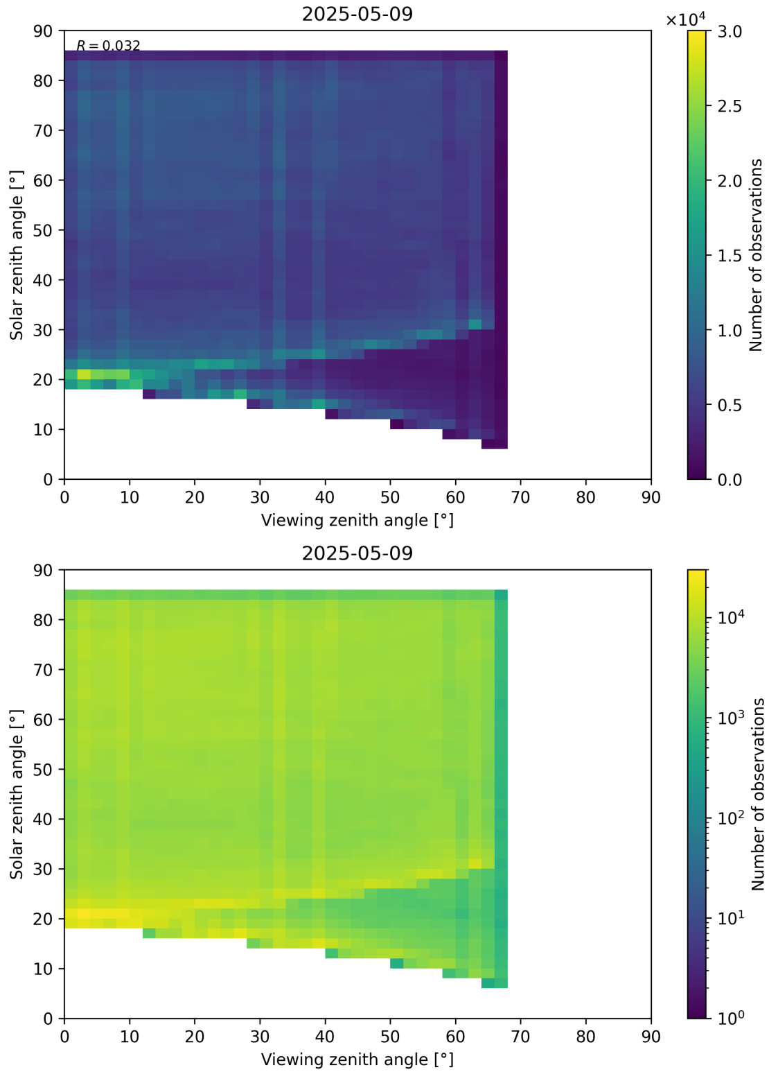
Figure 77: Scatter density plot of “Viewing zenith angle” against “Solar zenith angle” for 2025-05-08 to 2025-05-10.
