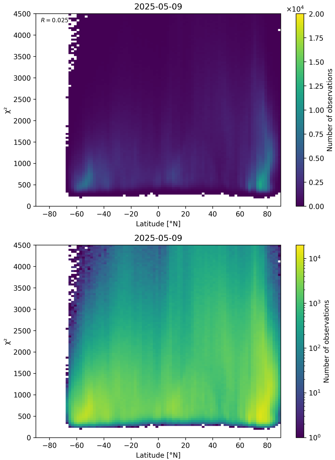
Figure 54: Scatter density plot of “Latitude” against “ \chi^2 ” for 2025-05-08 to 2025-05-10.
