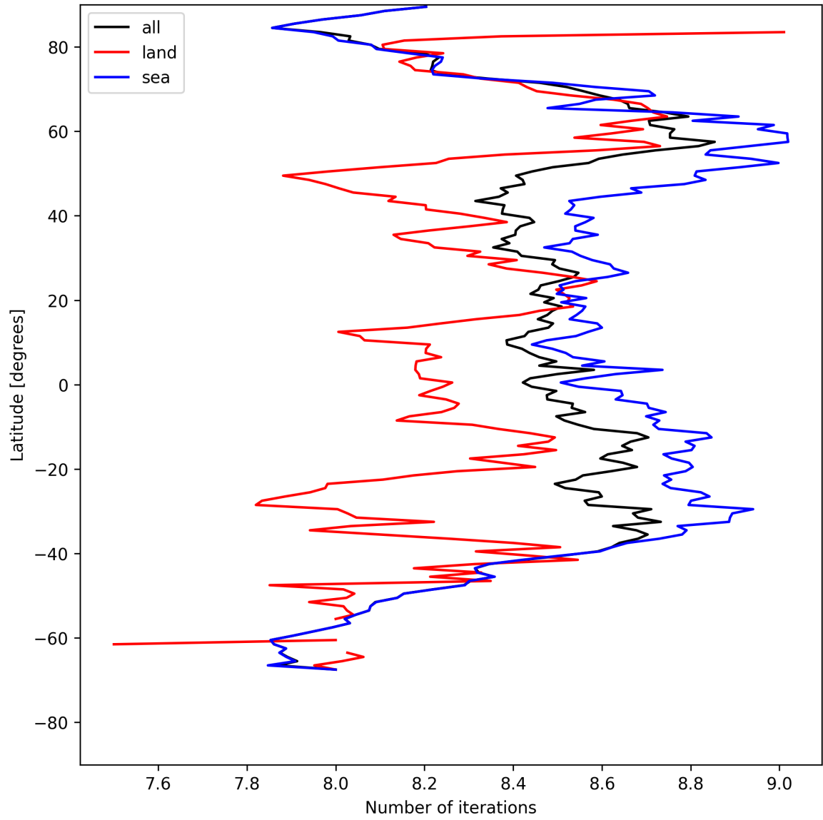
Figure 16: Zonal average of “Number of iterations” for 2025-05-08 to 2025-05-10.
