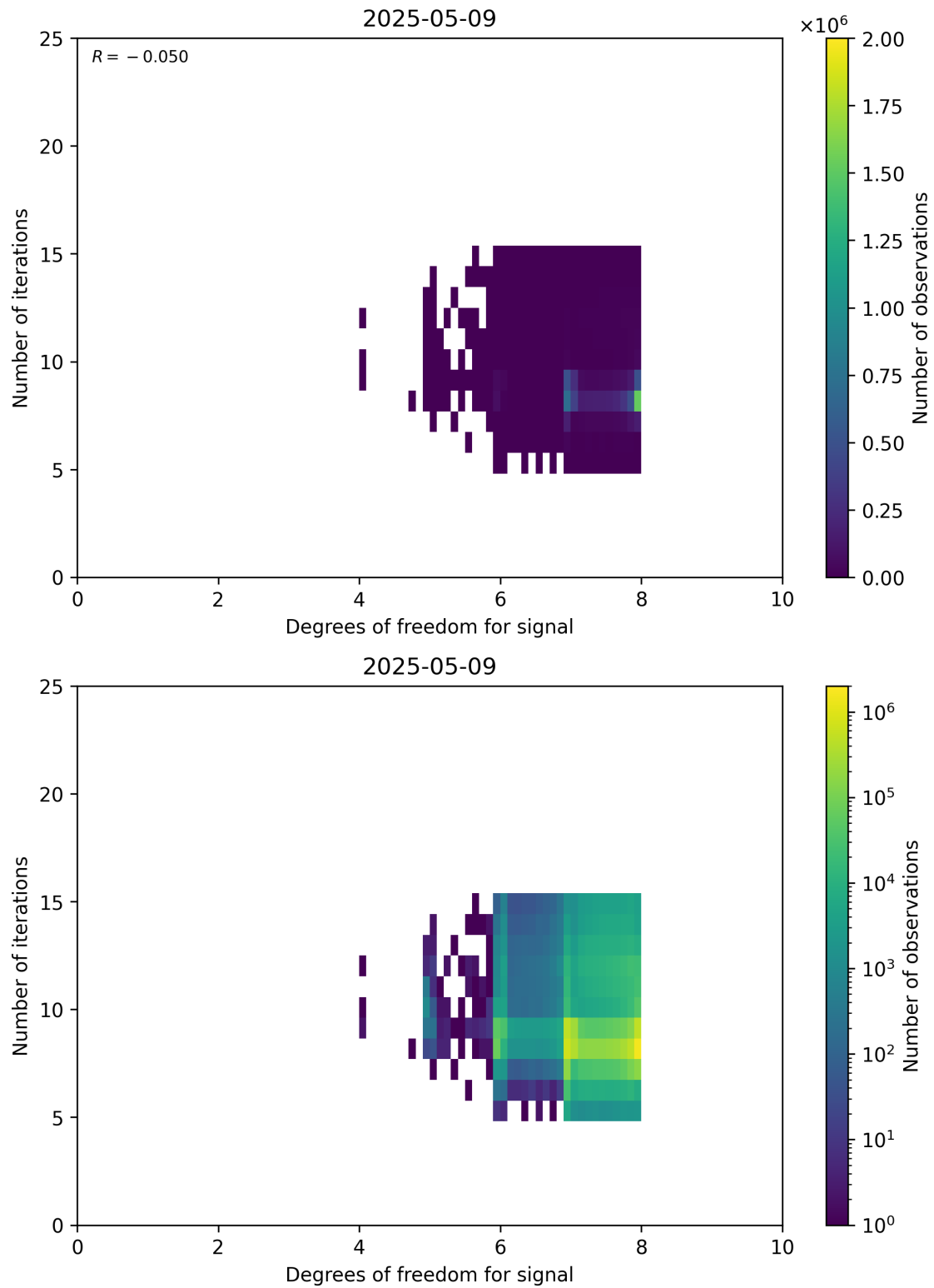
Figure 50: Scatter density plot of “Degrees of freedom for signal” against “Number of iterations” for 2025-05-08 to 2025-05-10.
