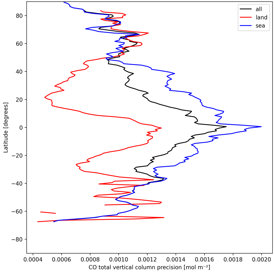
Figure 12: Zonal average of “CO total vertical column precision” for 2025-05-08 to 2025-05-10.
