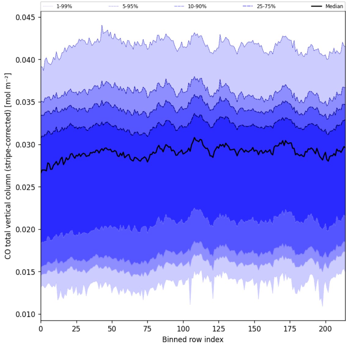
Figure 27: Along track statistics of “CO total vertical column (stripe-corrected)” for 2025-05-08 to 2025-05-10
