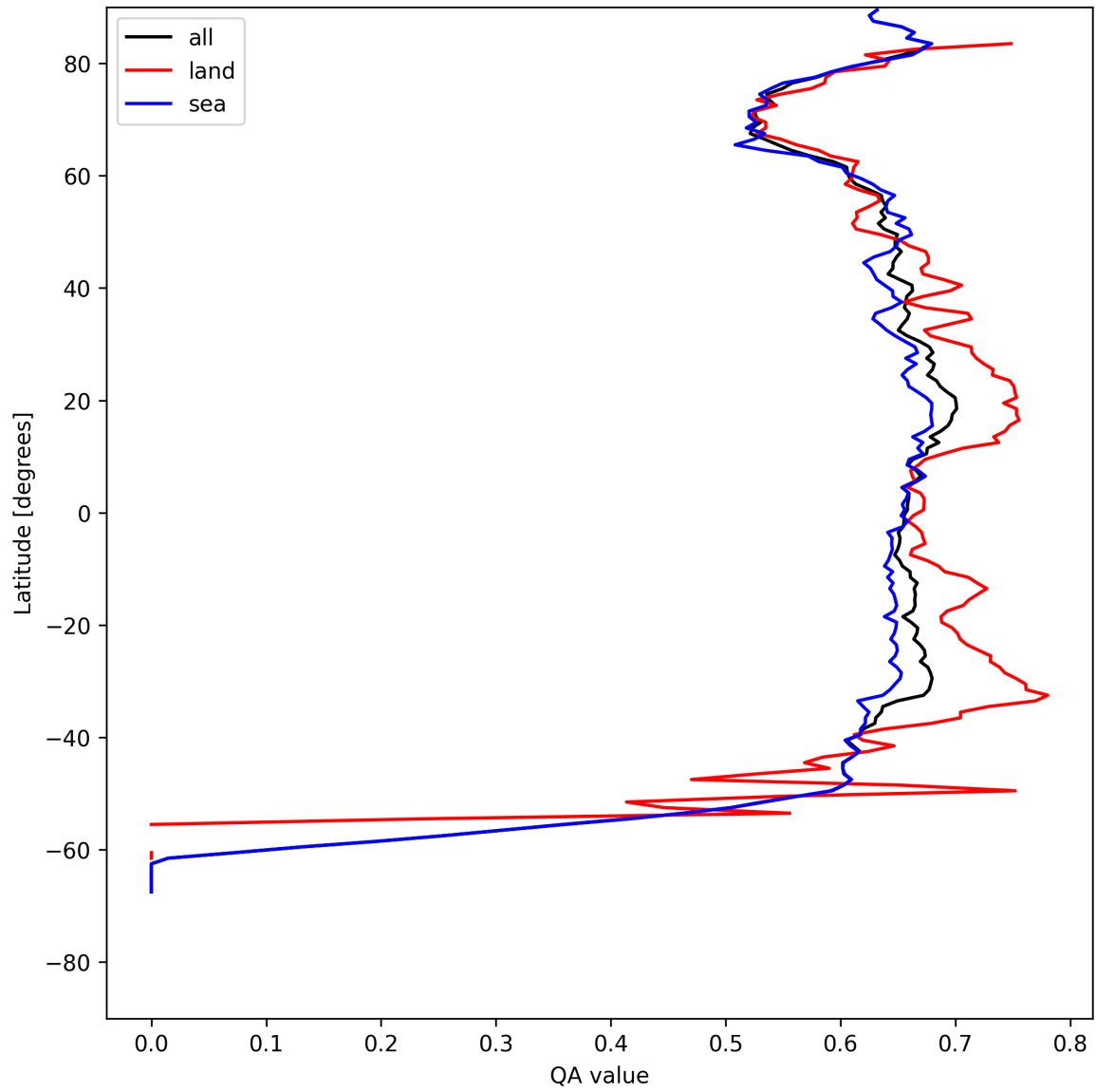
Figure 9: Zonal average of “QA value” for 2025-05-08 to 2025-05-10.
