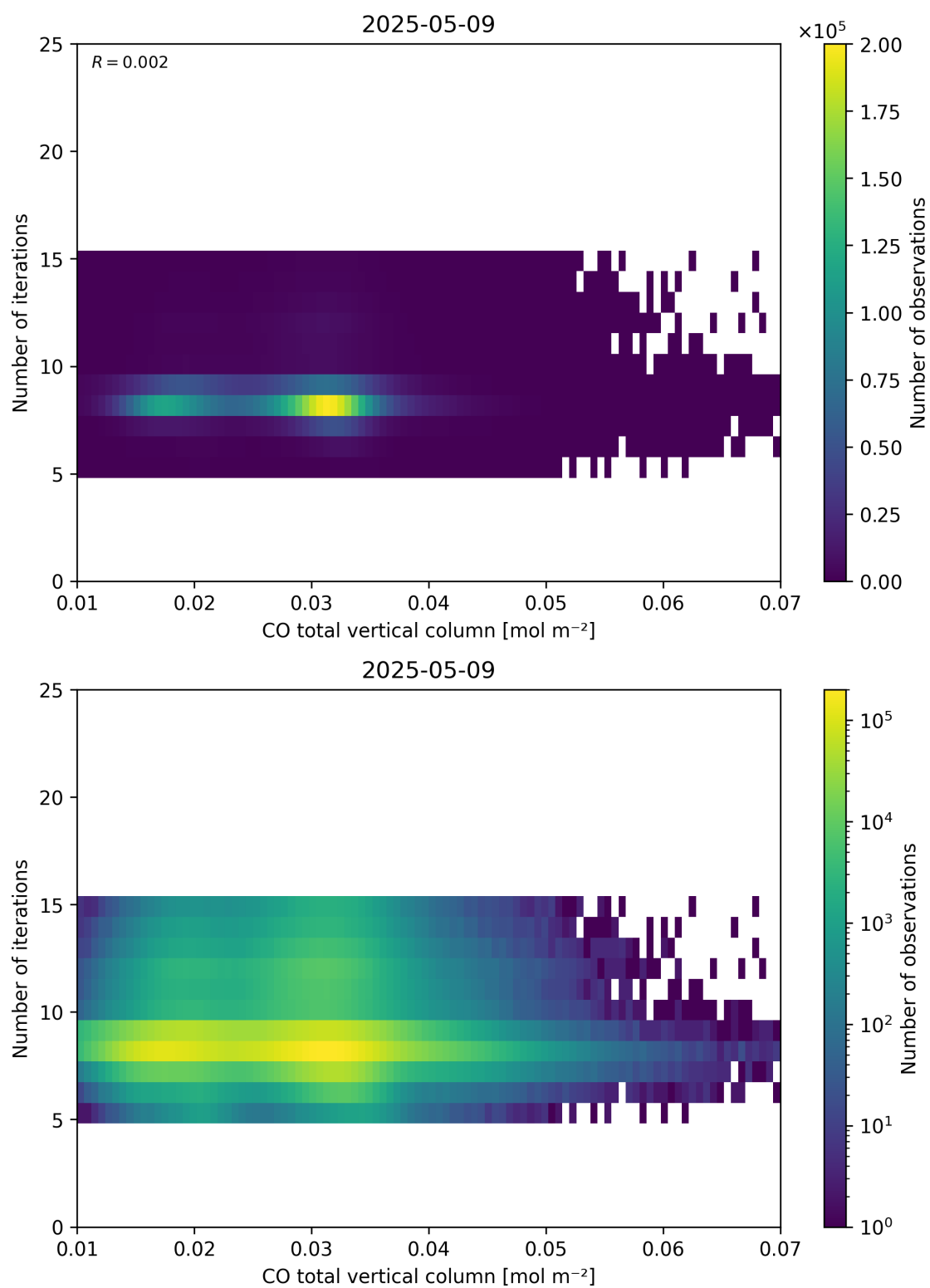
Figure 42: Scatter density plot of “CO total vertical column” against “Number of iterations” for 2025-05-08 to 2025-05-10.
