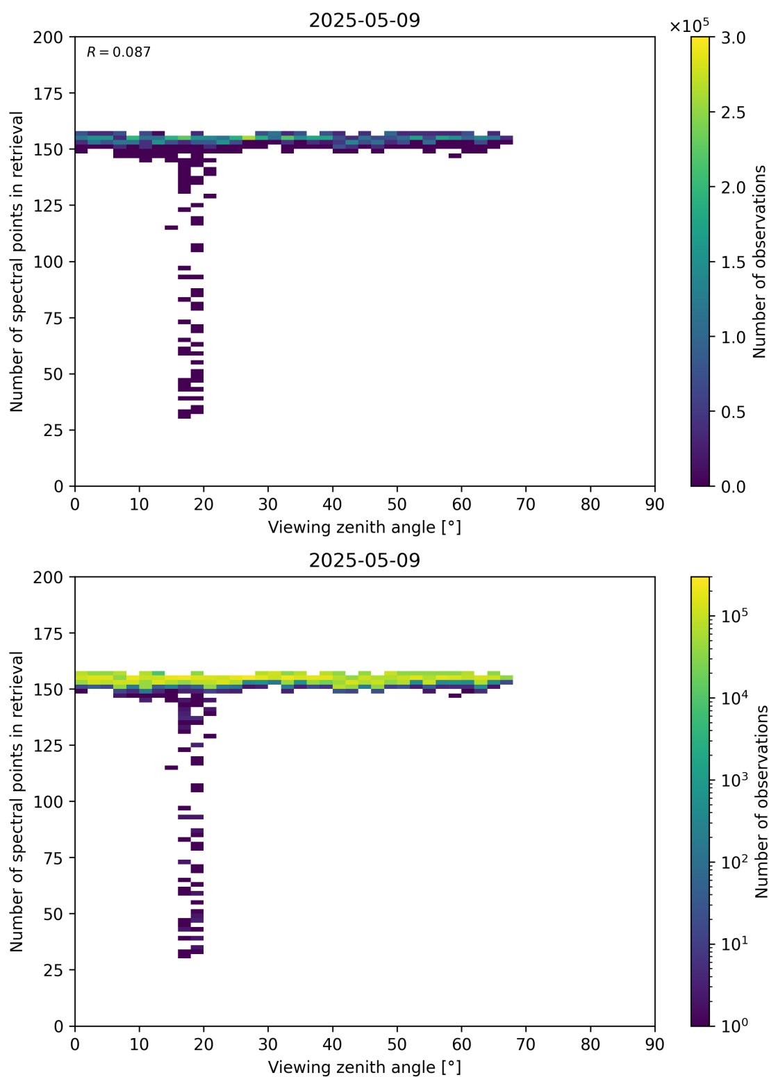
Figure 76: Scatter density plot of “Viewing zenith angle” against “Number of spectral points in retrieval” for 2025-05-08 to 2025-05-10.
