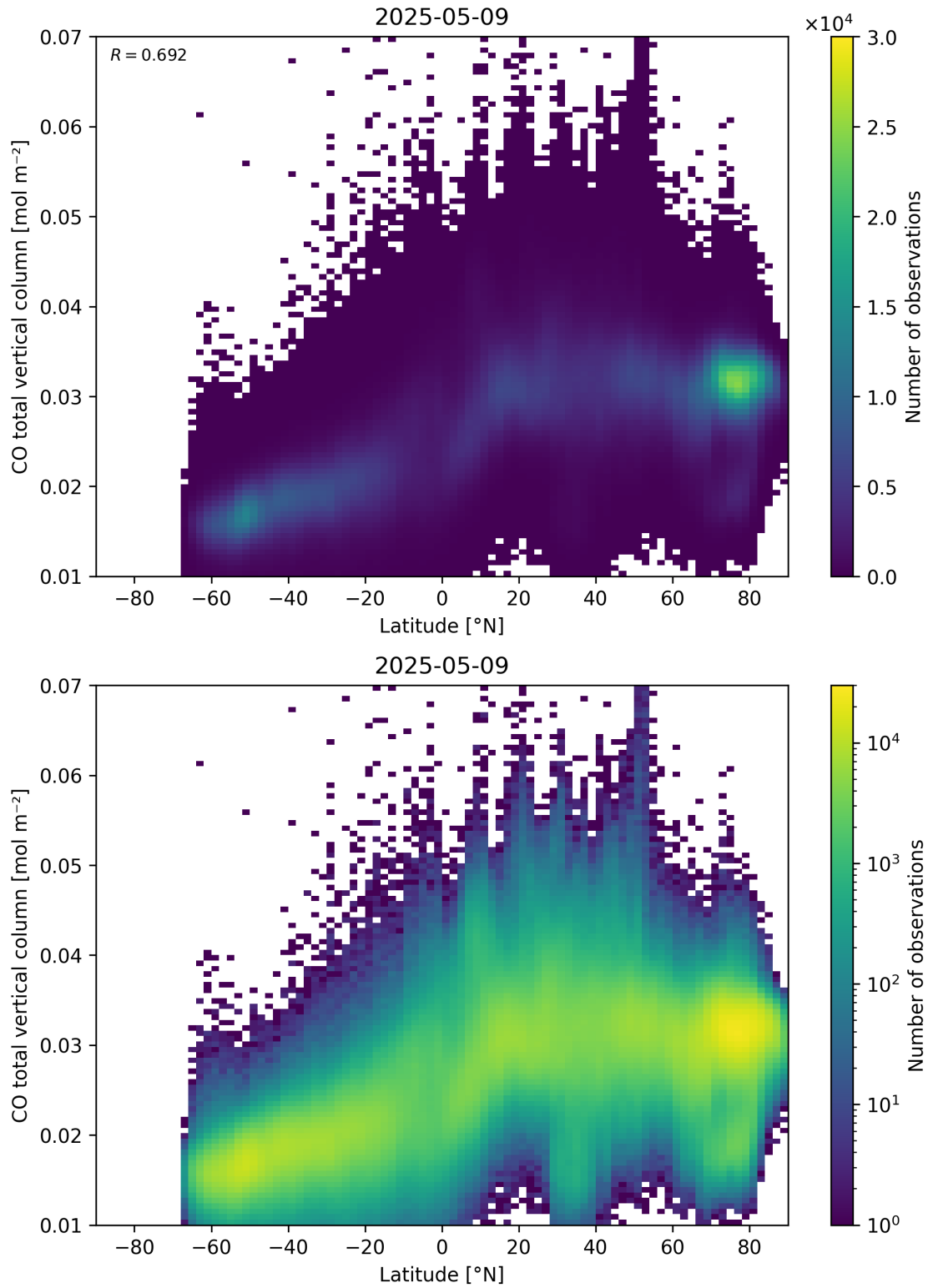
Figure 51: Scatter density plot of “Latitude” against “CO total vertical column” for 2025-05-08 to 2025-05-10.
