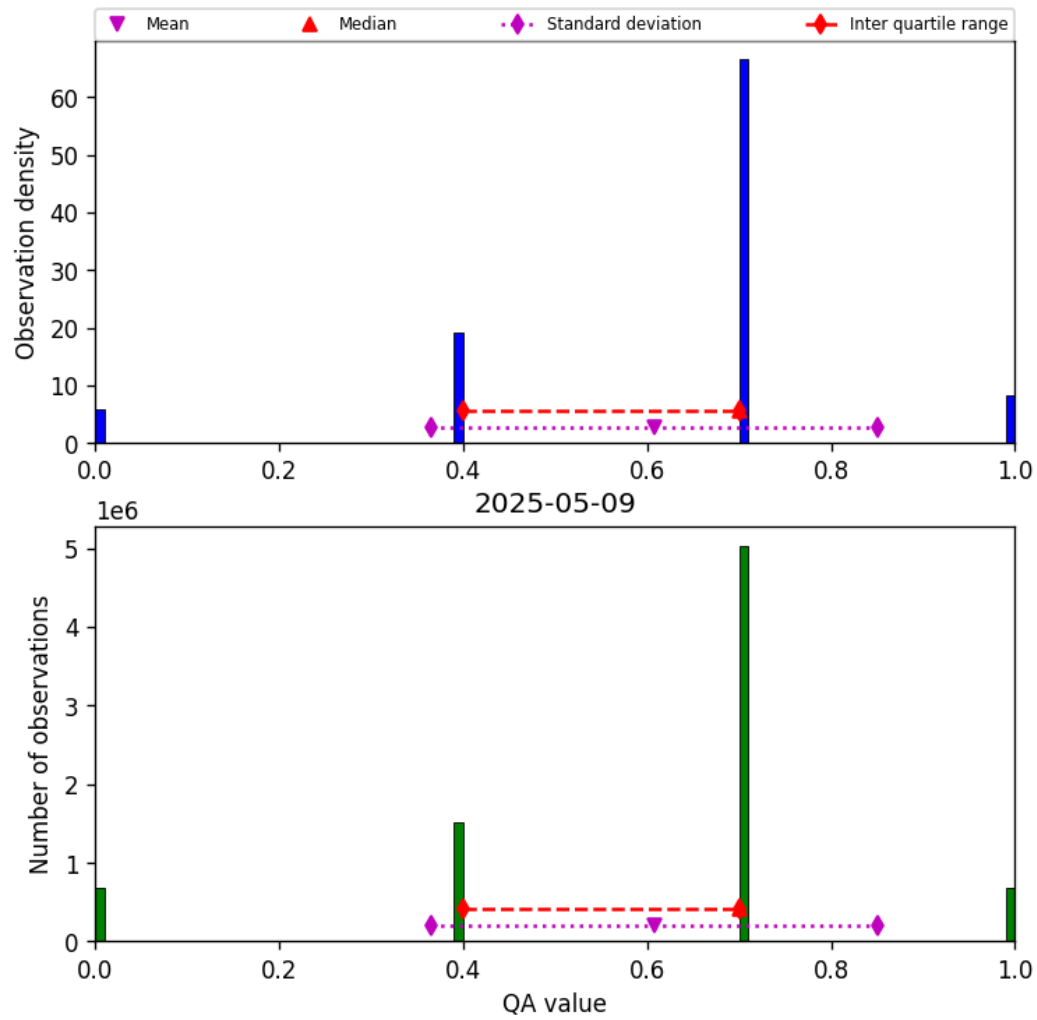
Figure 17: Histogram of “QA value” for 2025-05-08 to 2025-05-10
