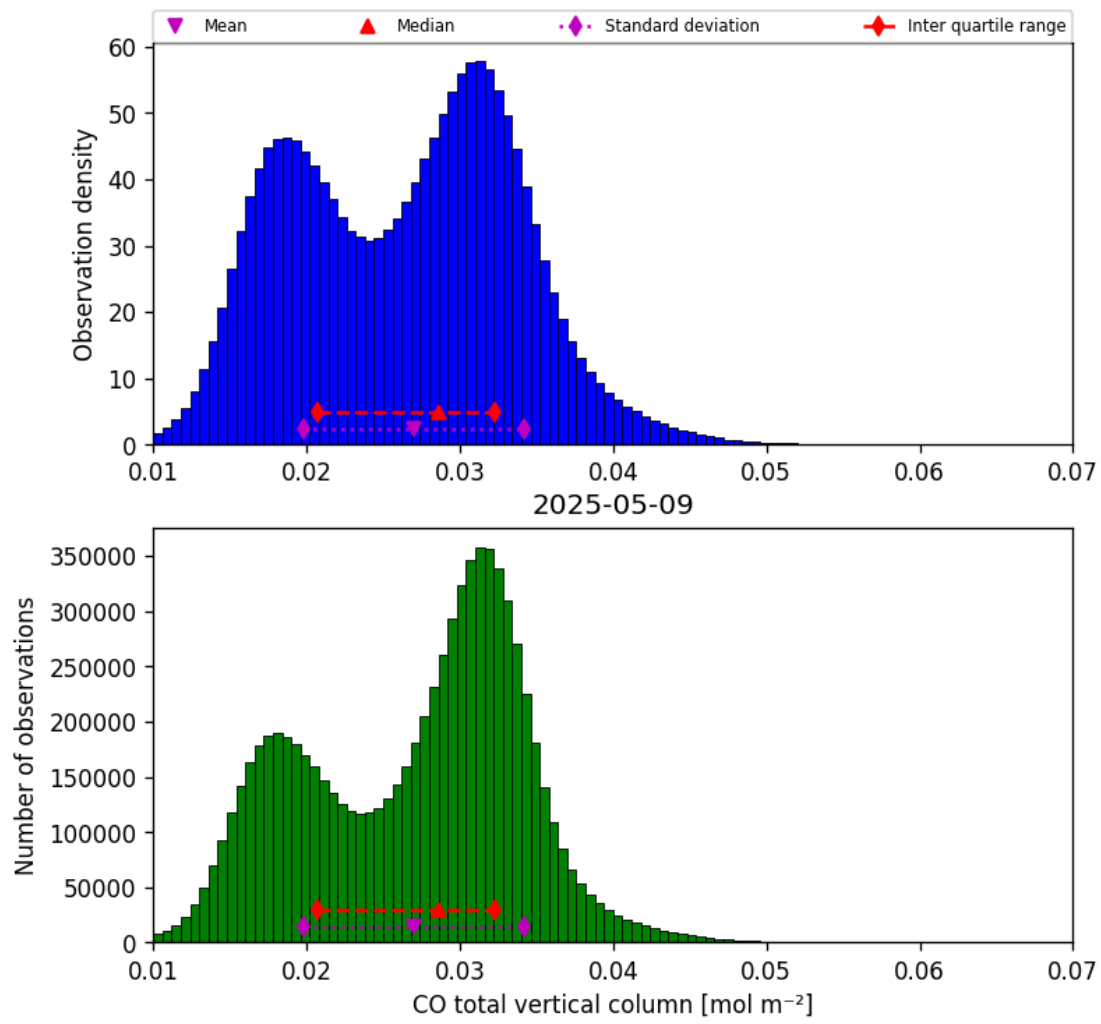
Figure 18: Histogram of “CO total vertical column” for 2025-05-08 to 2025-05-10
