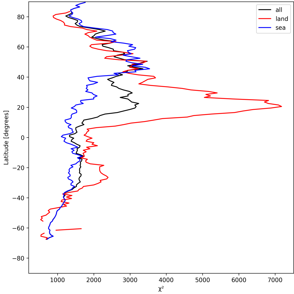
Figure 14: Zonal average of “ \chi^2 ” for 2025-05-08 to 2025-05-10.
