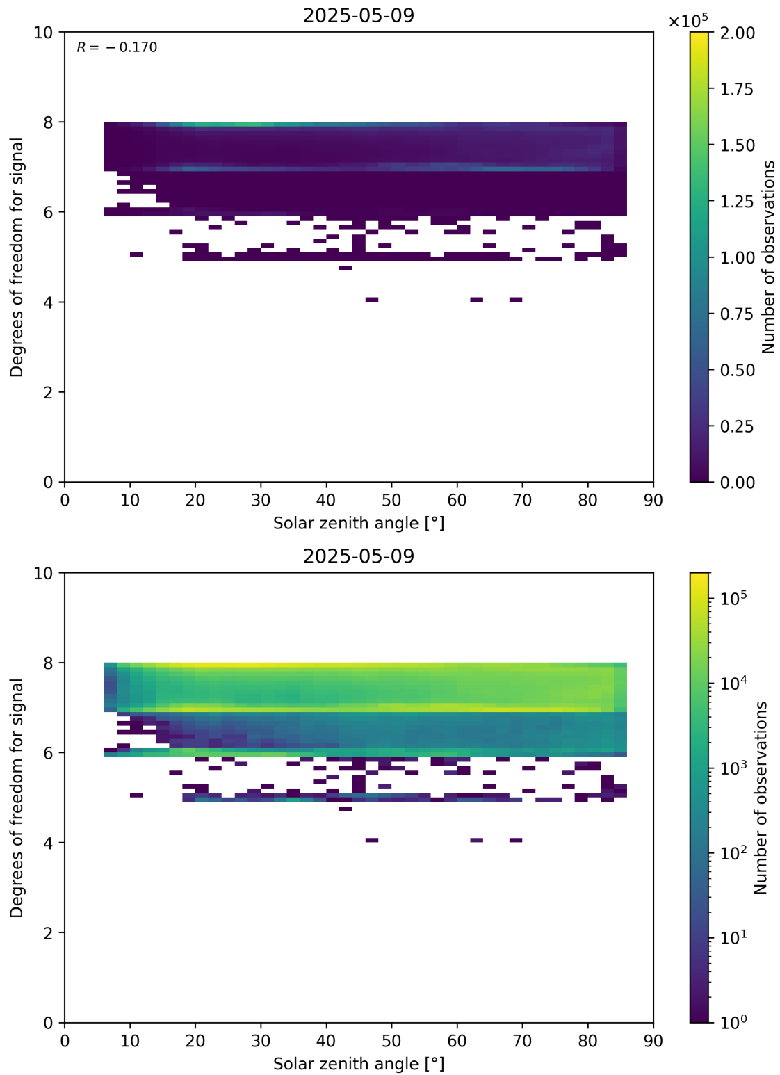
Figure 65: Scatter density plot of “Solar zenith angle” against “Degrees of freedom for signal” for 2025-05-08 to 2025-05-10.
