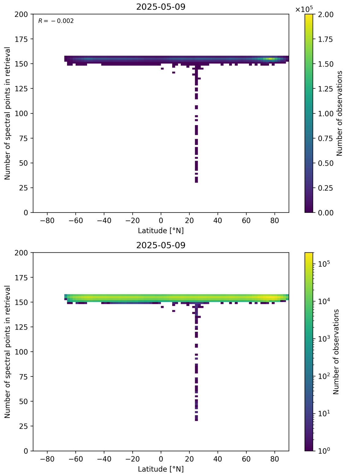
Figure 57: Scatter density plot of “Latitude” against “Number of spectral points in retrieval” for 2025-05-08 to 2025-05-10.
