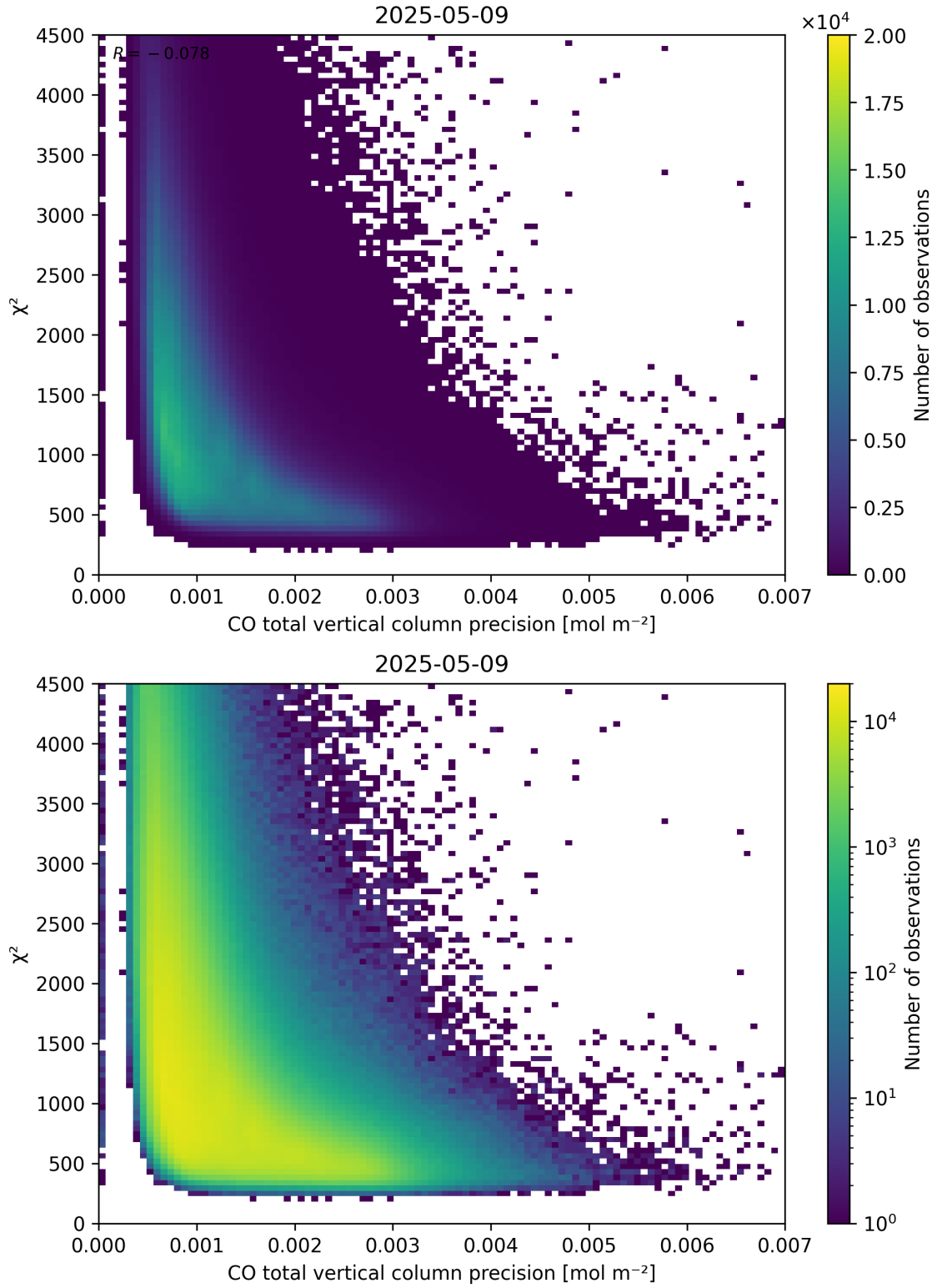
Figure 44: Scatter density plot of “CO total vertical column precision” against “ \chi^2 ” for 2025-05-08 to 2025-05-10.
