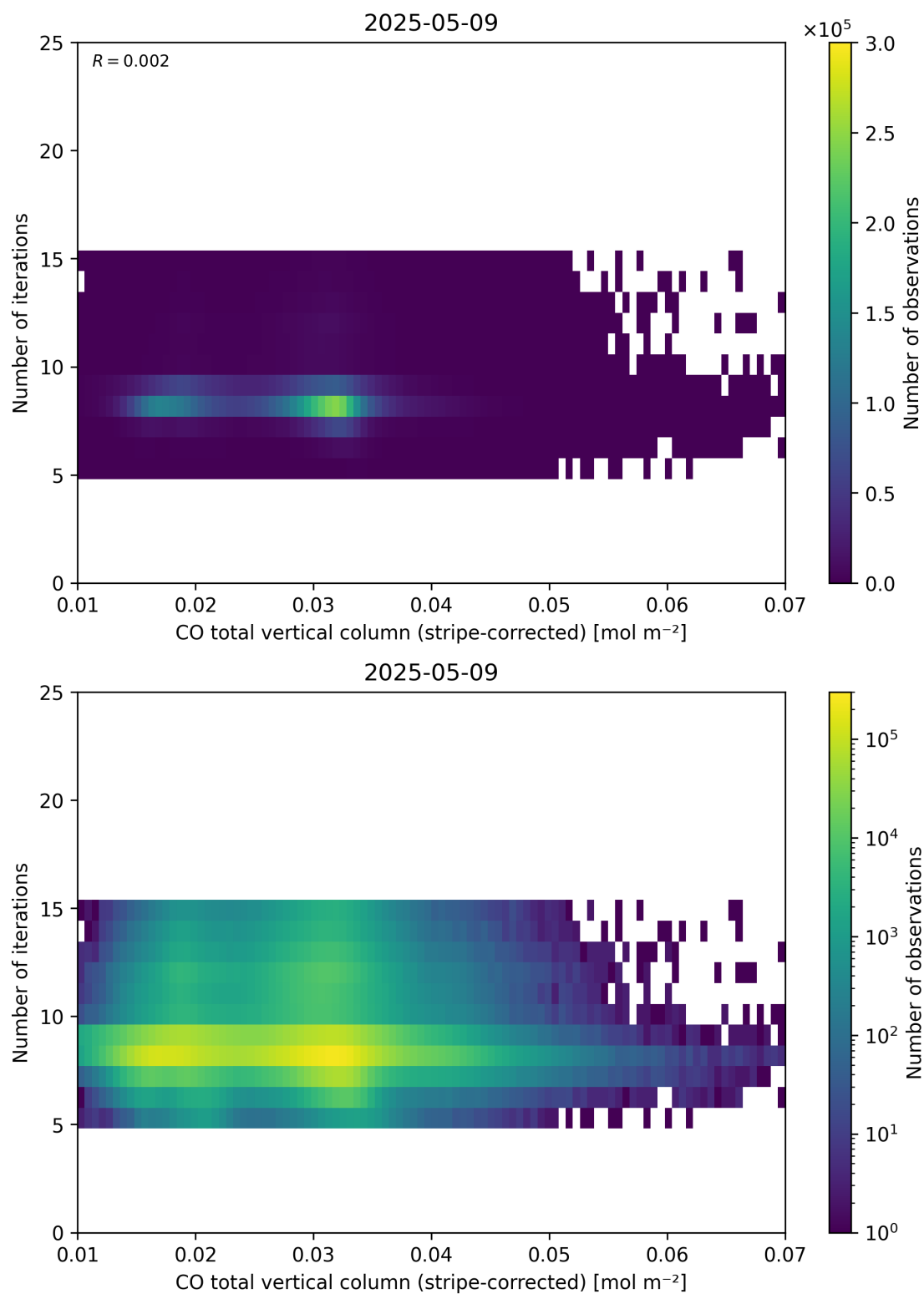
Figure 39: Scatter density plot of “CO total vertical column (stripe-corrected)” against “Number of iterations” for 2025-05-08 to 2025-05-10.
