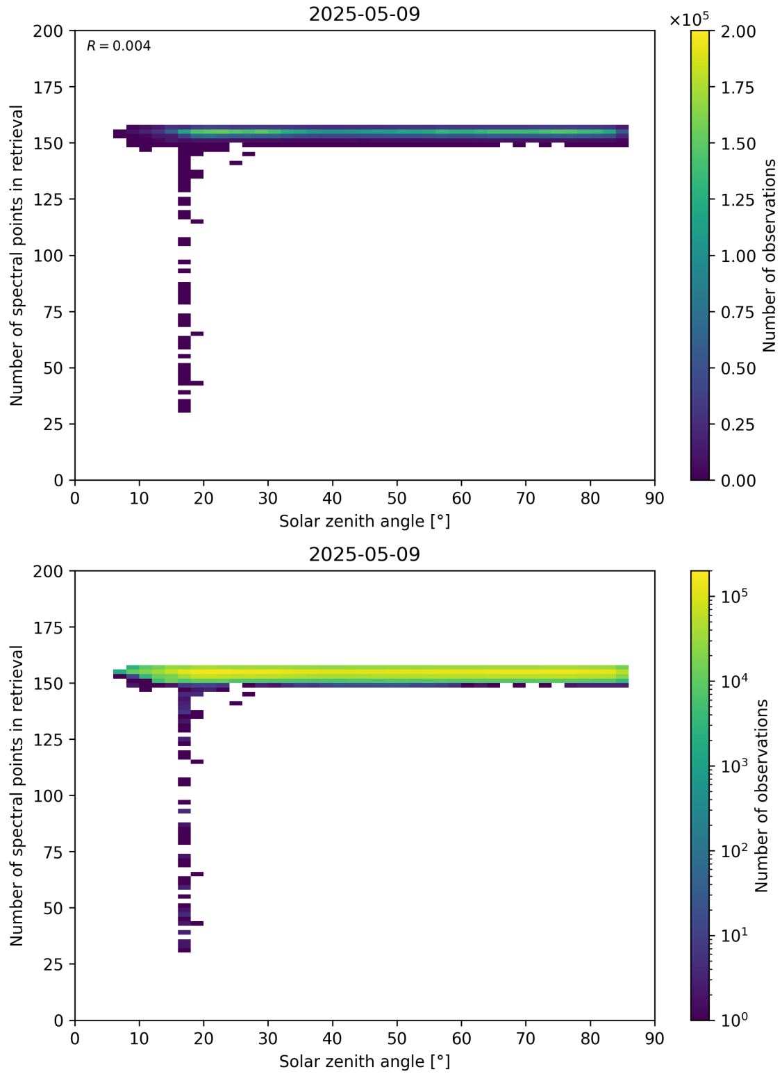
Figure 68: Scatter density plot of “Solar zenith angle” against “Number of spectral points in retrieval” for 2025-05-08 to 2025-05-10.
