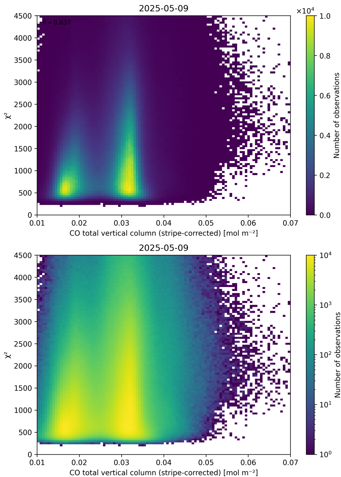
Figure 37: Scatter density plot of “CO total vertical column (stripe-corrected)” against “ \chi^2 ” for 2025-05-08 to 2025-05-10.
