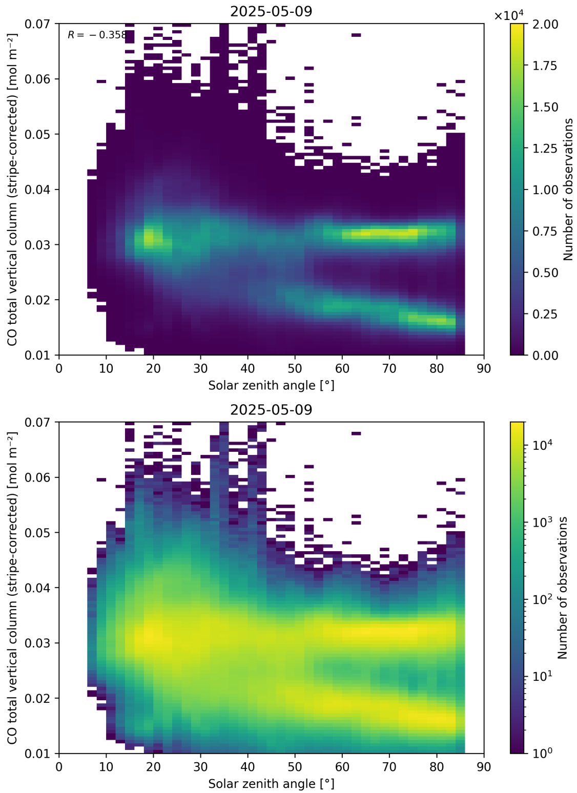
Figure 62: Scatter density plot of “Solar zenith angle” against “CO total vertical column (stripe-corrected)” for 2025-05-08 to 2025-05-10.
