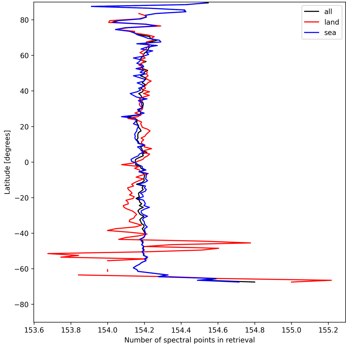
Figure 13: Zonal average of “Number of spectral points in retrieval” for 2025-05-08 to 2025-05-10.
