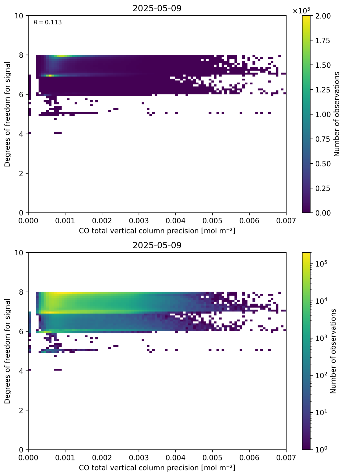
Figure 45: Scatter density plot of “CO total vertical column precision” against “Degrees of freedom for signal” for 2025-05-08 to 2025-05-10.
