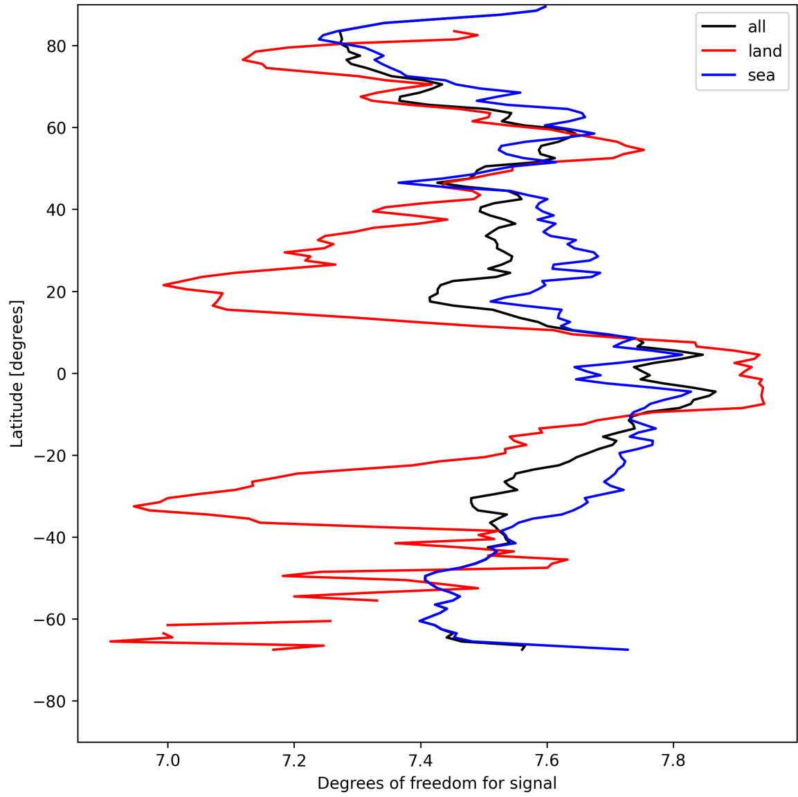
Figure 15: Zonal average of “Degrees of freedom for signal” for 2025-05-08 to 2025-05-10.
