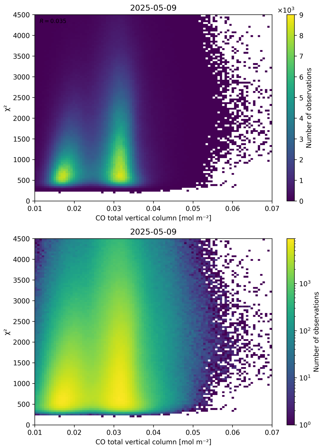
Figure 35: Scatter density plot of “CO total vertical column” against “ \chi^2 ” for 2025-05-08 to 2025-05-10.
