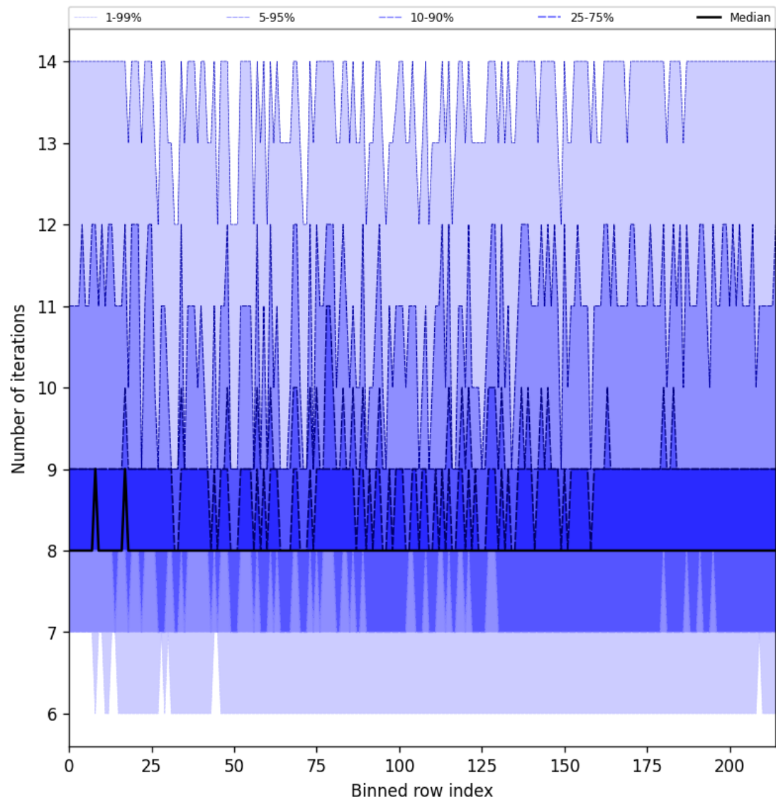
Figure 32: Along track statistics of “Number of iterations” for 2025-05-08 to 2025-05-10
