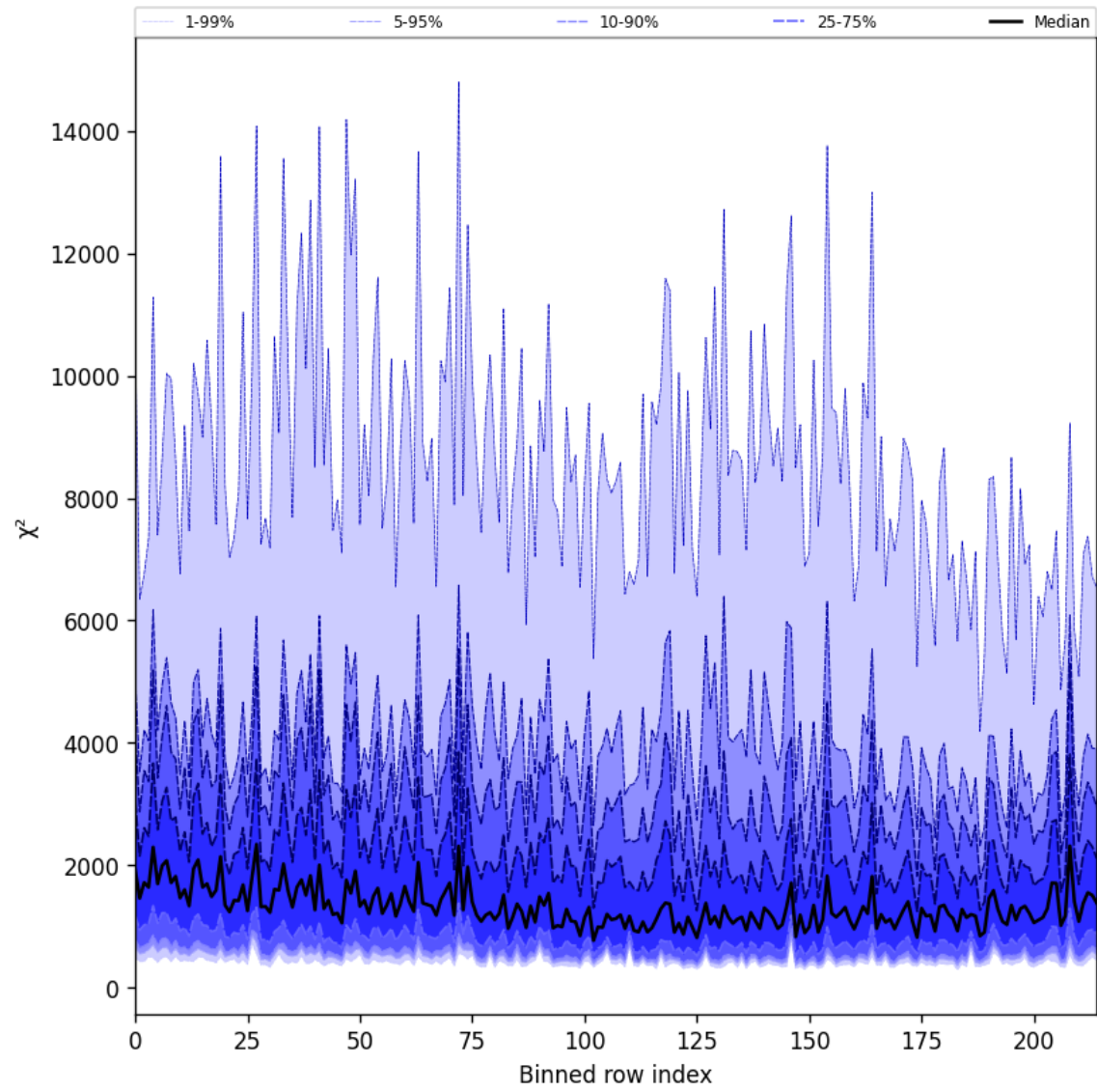
Figure 30: Along track statistics of “ \chi^2 ” for 2025-05-08 to 2025-05-10
