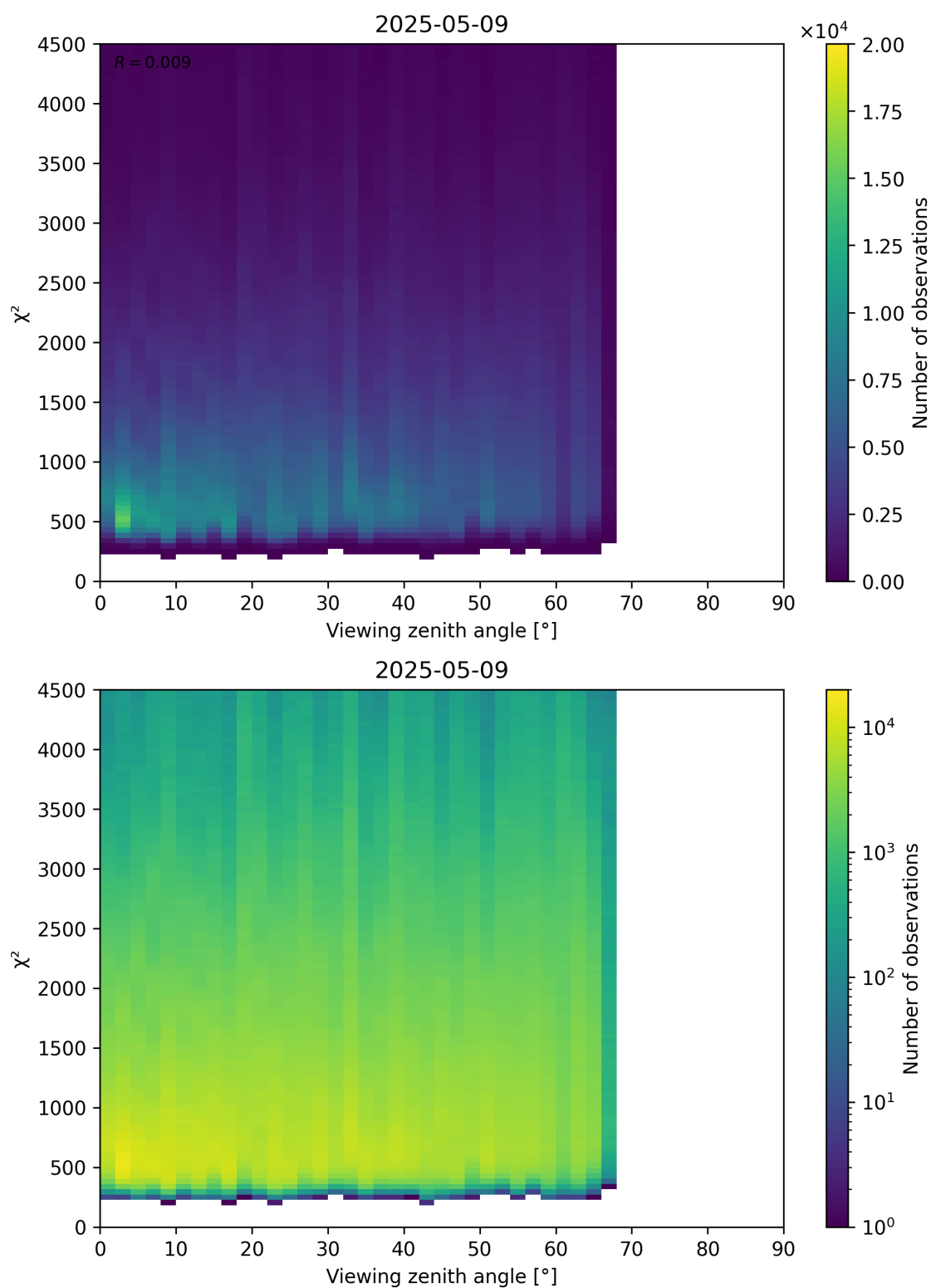
Figure 72: Scatter density plot of “Viewing zenith angle” against “ \chi^2 ” for 2025-05-08 to 2025-05-10.
