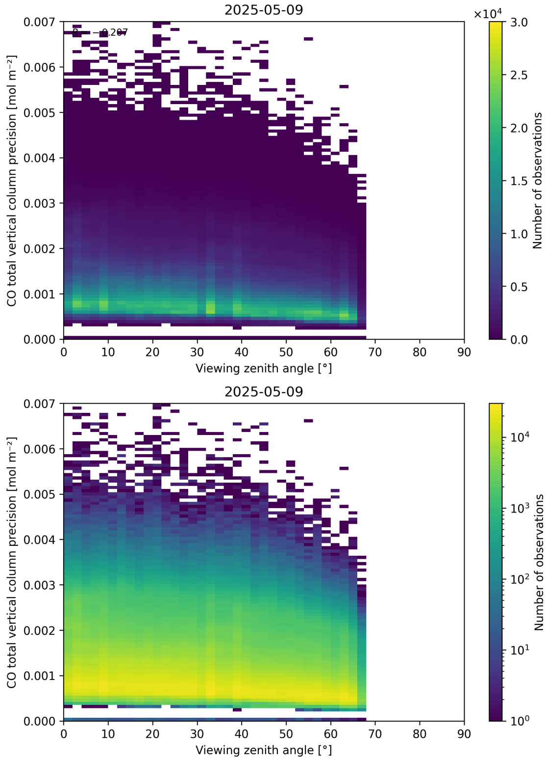
Figure 71: Scatter density plot of “Viewing zenith angle” against “CO total vertical column precision” for 2025-05-08 to 2025-05-10.
