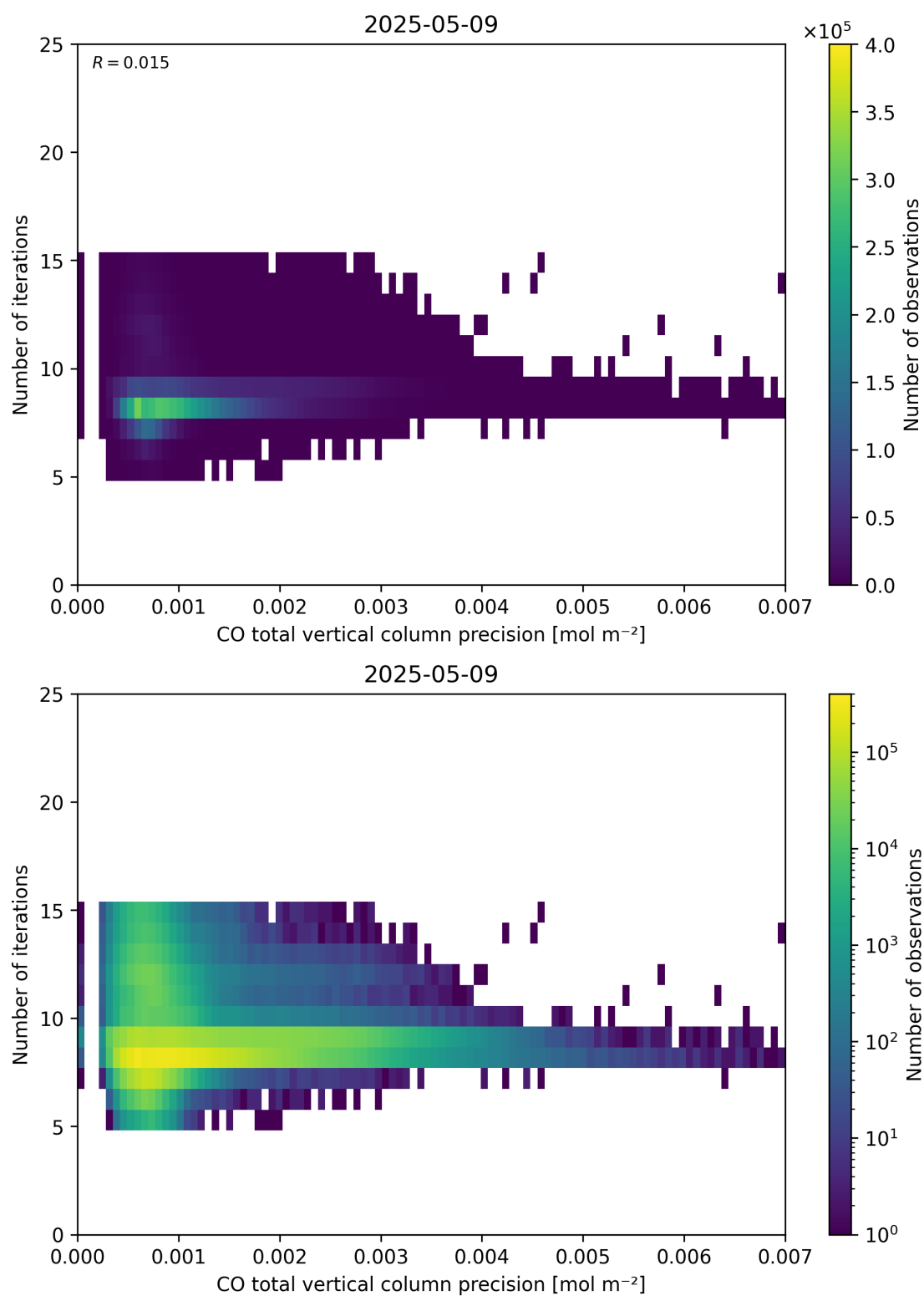
Figure 46: Scatter density plot of “CO total vertical column precision” against “Number of iterations” for 2025-05-08 to 2025-05-10.
