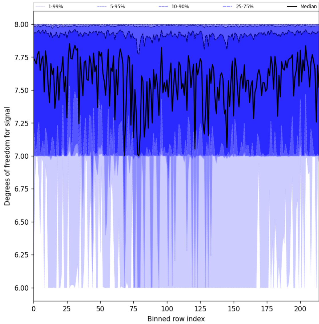
Figure 31: Along track statistics of “Degrees of freedom for signal” for 2025-05-08 to 2025-05-10
