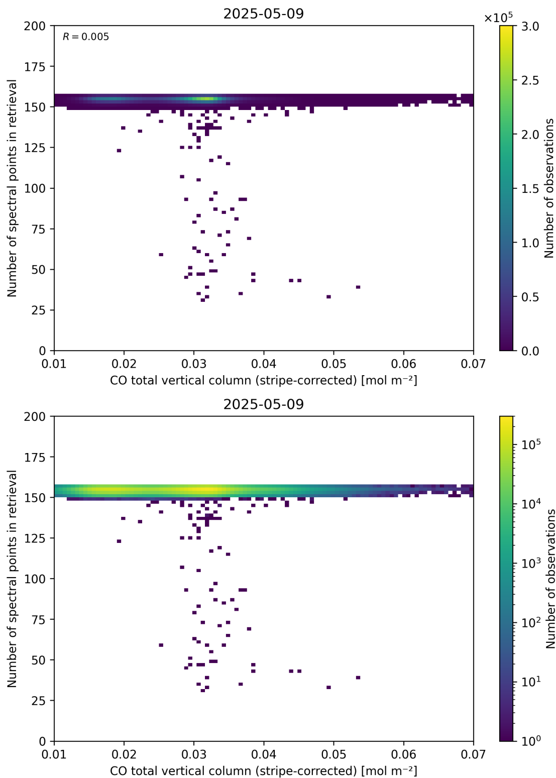
Figure 40: Scatter density plot of “CO total vertical column (stripe-corrected)” against “Number of spectral points in retrieval” for 2025-05-08 to 2025-05-10.
