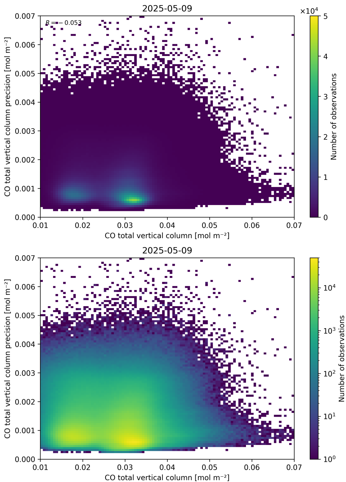
Figure 34: Scatter density plot of “CO total vertical column” against “CO total vertical column precision” for 2025-05-08 to 2025-05-10.
