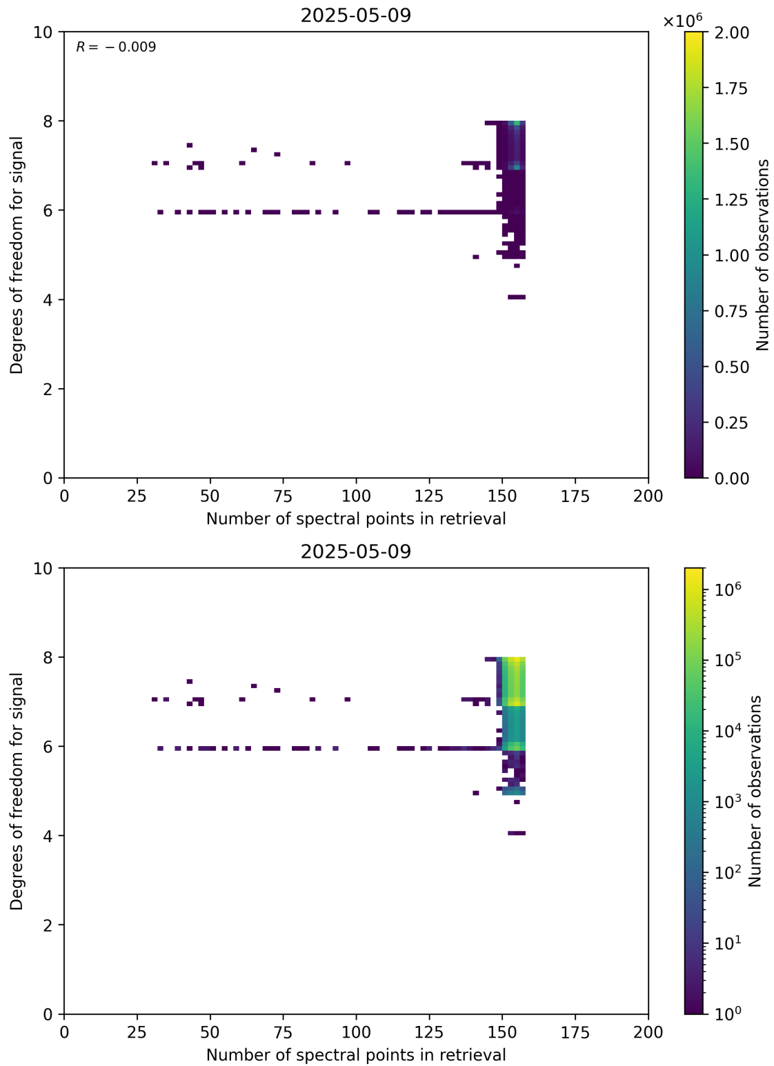
Figure 59: Scatter density plot of “Number of spectral points in retrieval” against “Degrees of freedom for signal” for 2025-05-08 to 2025-05-10.
