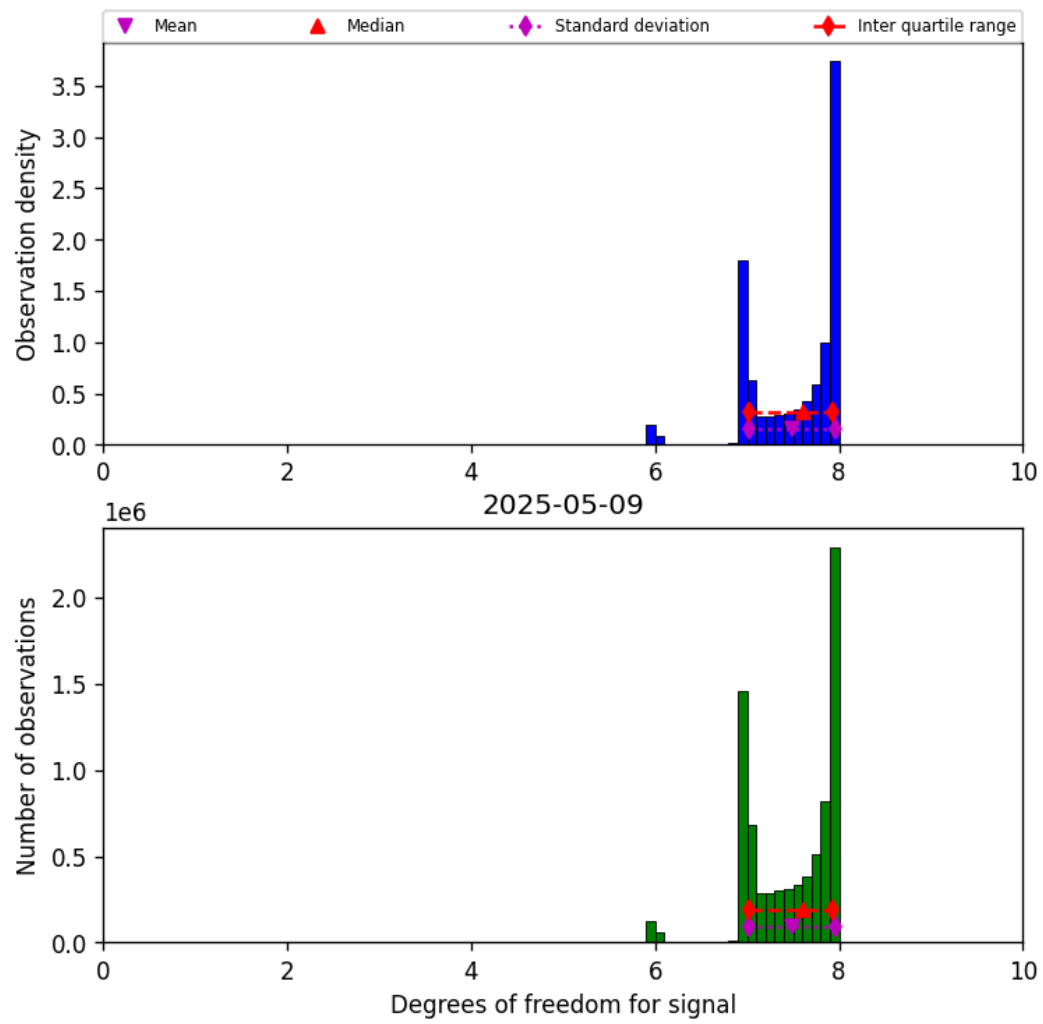
Figure 23: Histogram of “Degrees of freedom for signal” for 2025-05-08 to 2025-05-10
