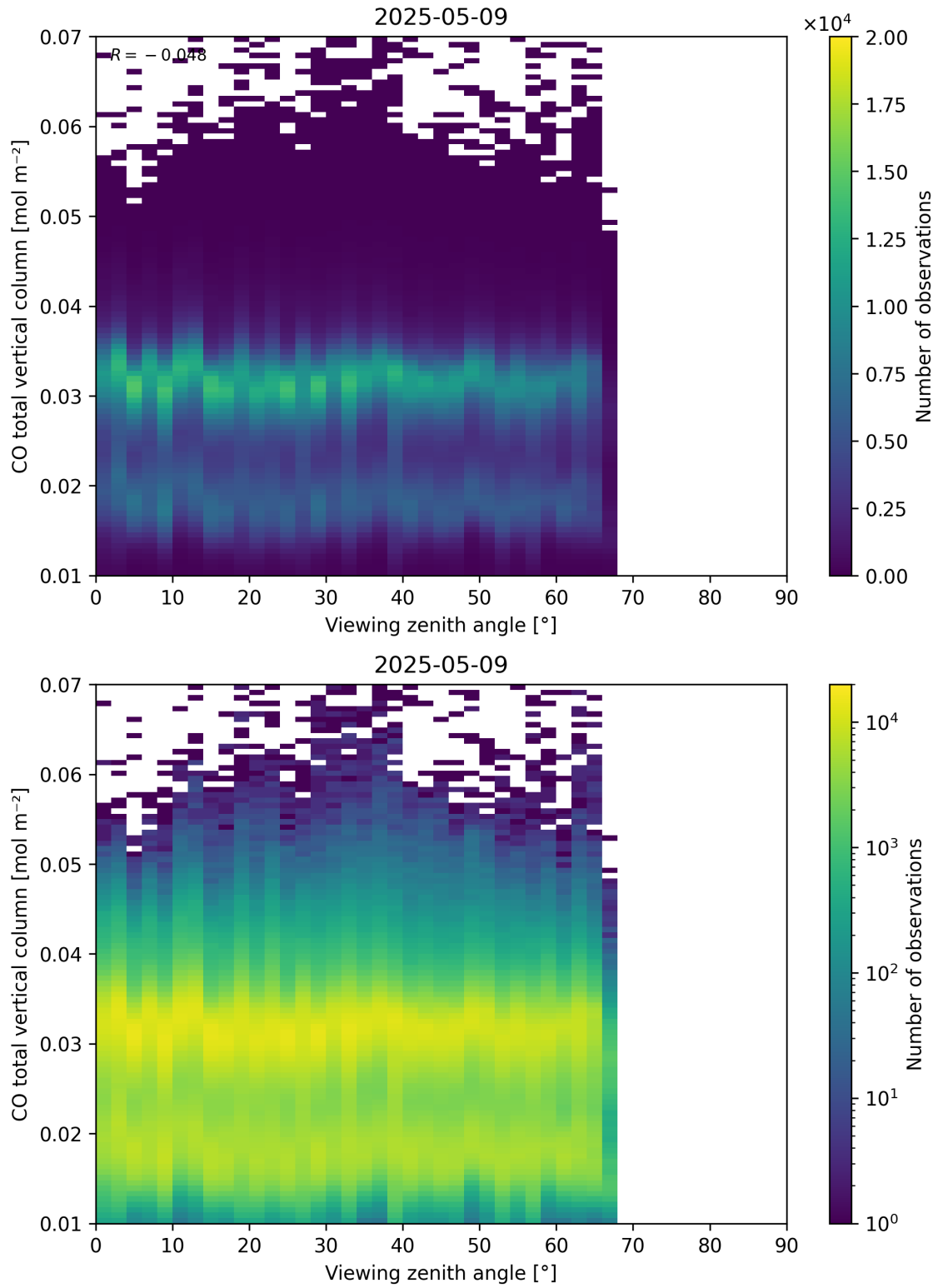
Figure 69: Scatter density plot of “Viewing zenith angle” against “CO total vertical column” for 2025-05-08 to 2025-05-10.
