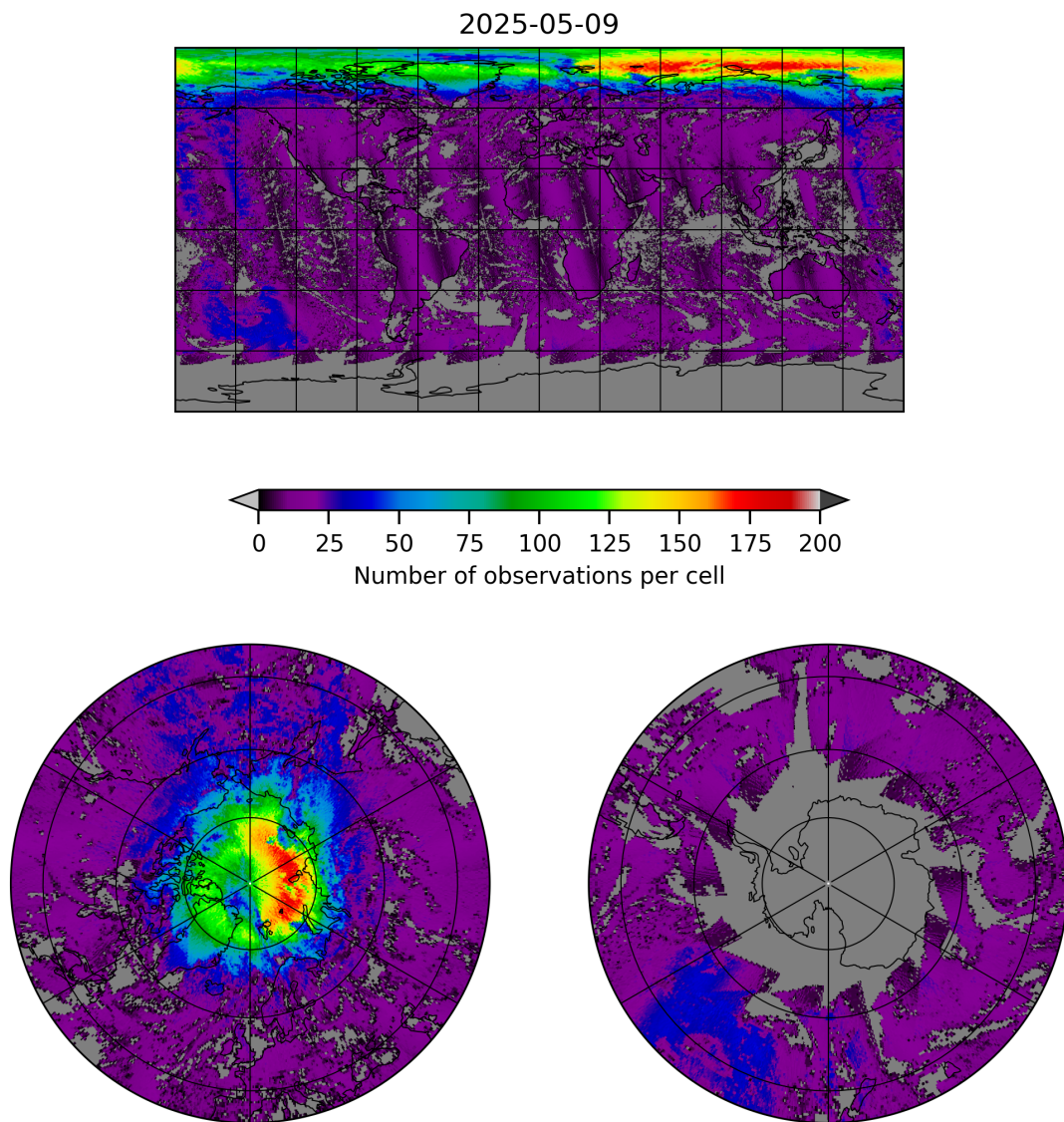
Figure 8: Map of the number of observations for 2025-05-08 to 2025-05-10
