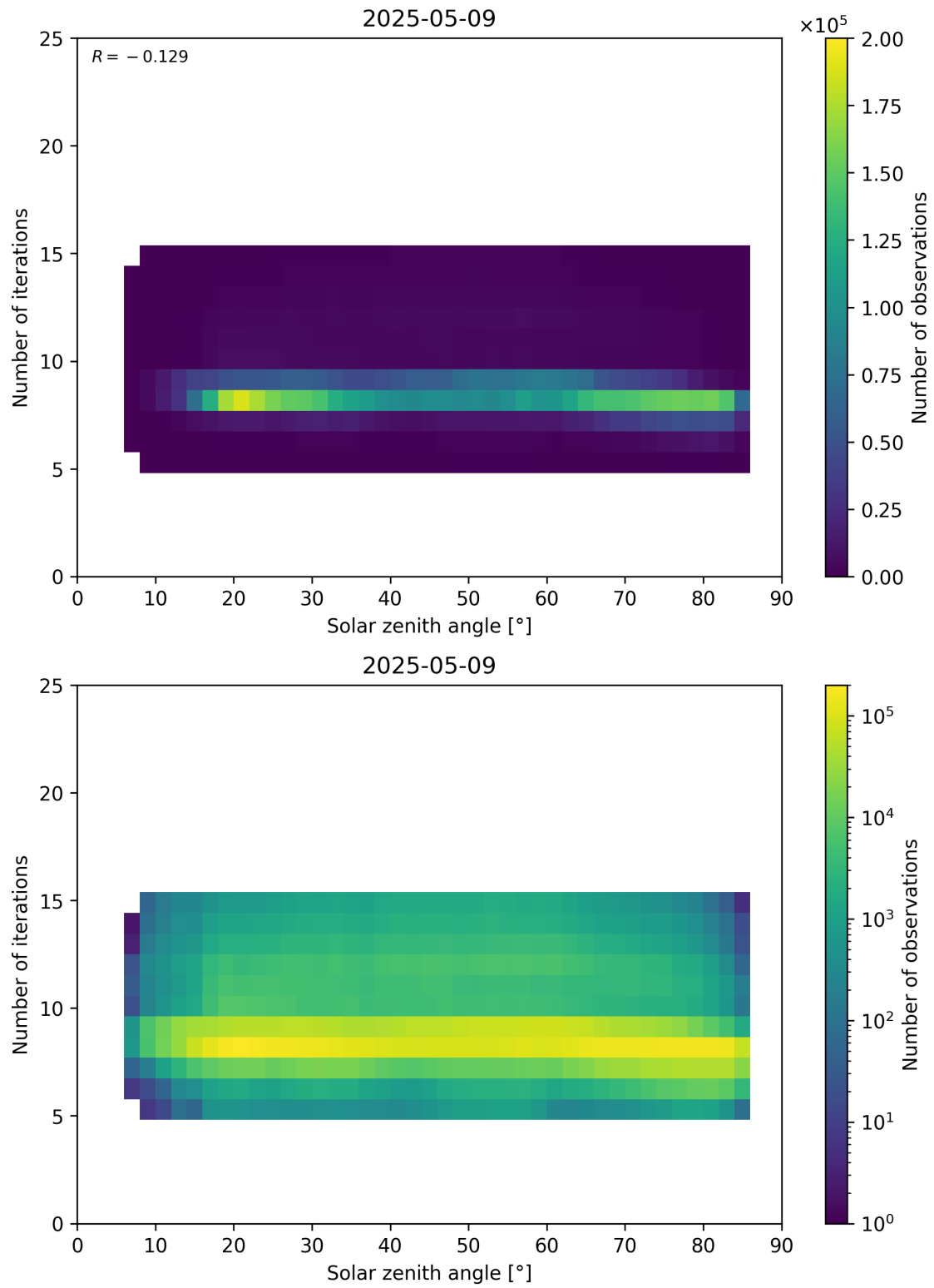
Figure 67: Scatter density plot of “Solar zenith angle” against “Number of iterations” for 2025-05-08 to 2025-05-10.
