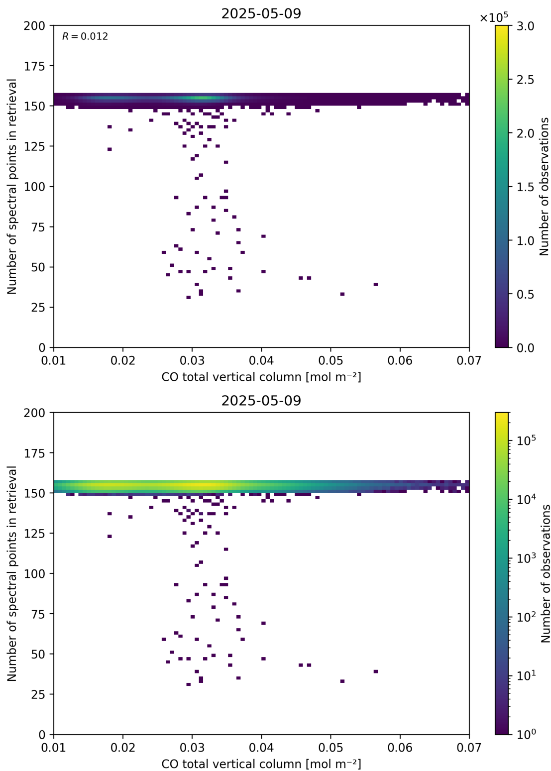
Figure 43: Scatter density plot of “CO total vertical column” against “Number of spectral points in retrieval” for 2025-05-08 to 2025-05-10.
