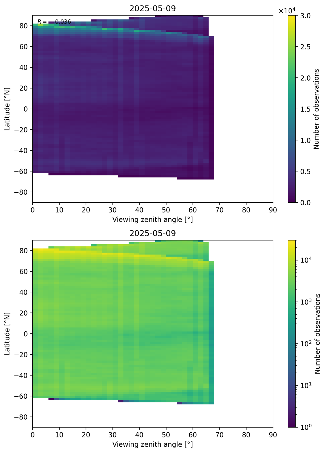
Figure 74: Scatter density plot of “Viewing zenith angle” against “Latitude” for 2025-05-08 to 2025-05-10.
