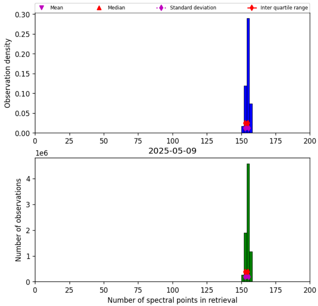
Figure 21: Histogram of “Number of spectral points in retrieval” for 2025-05-08 to 2025-05-10
