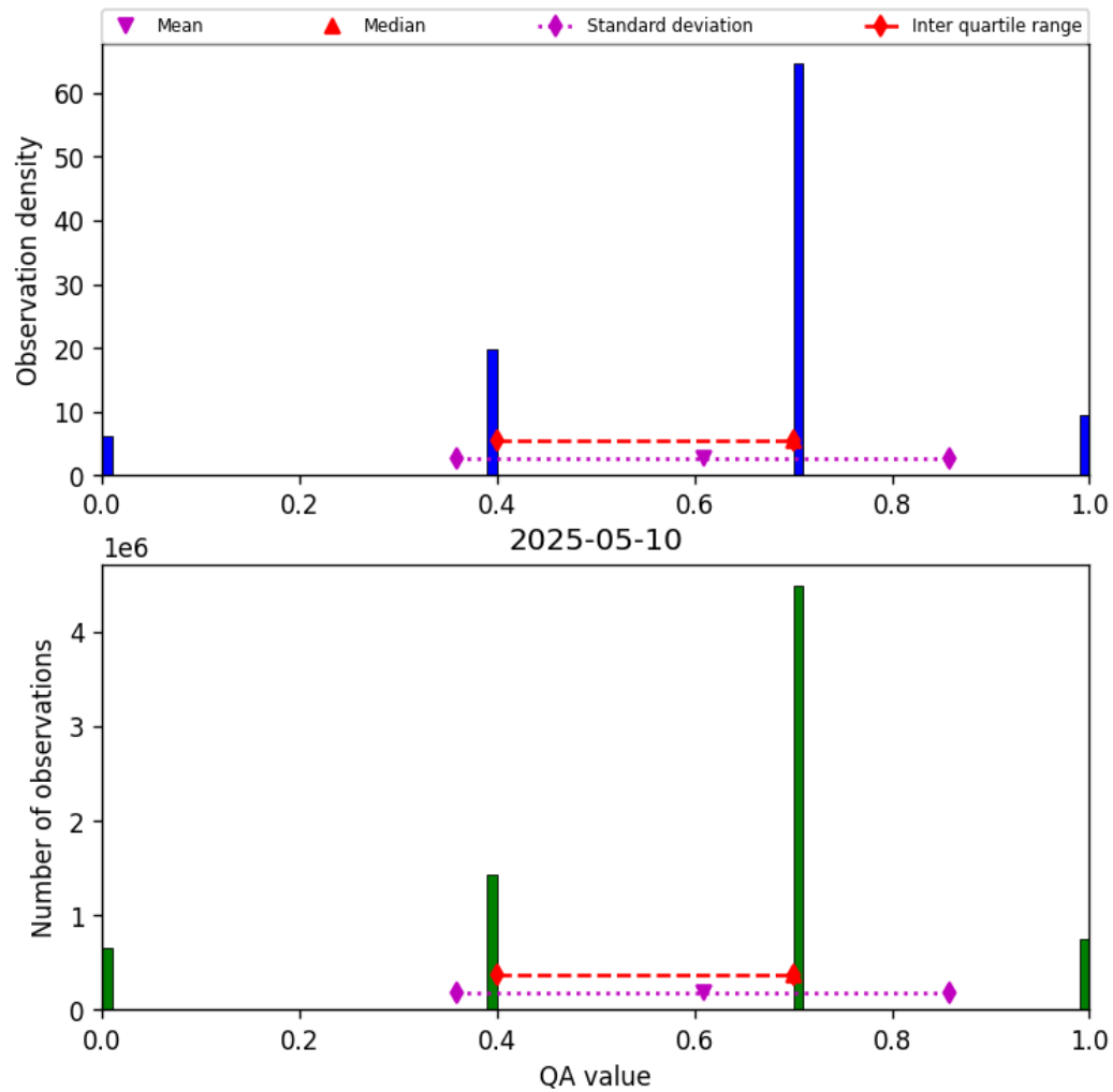
Figure 17: Histogram of “QA value” for 2025-05-10 to 2025-05-11
