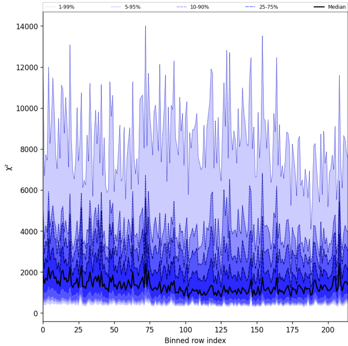
Figure 30: Along track statistics of “ \chi^2 ” for 2025-05-10 to 2025-05-11
