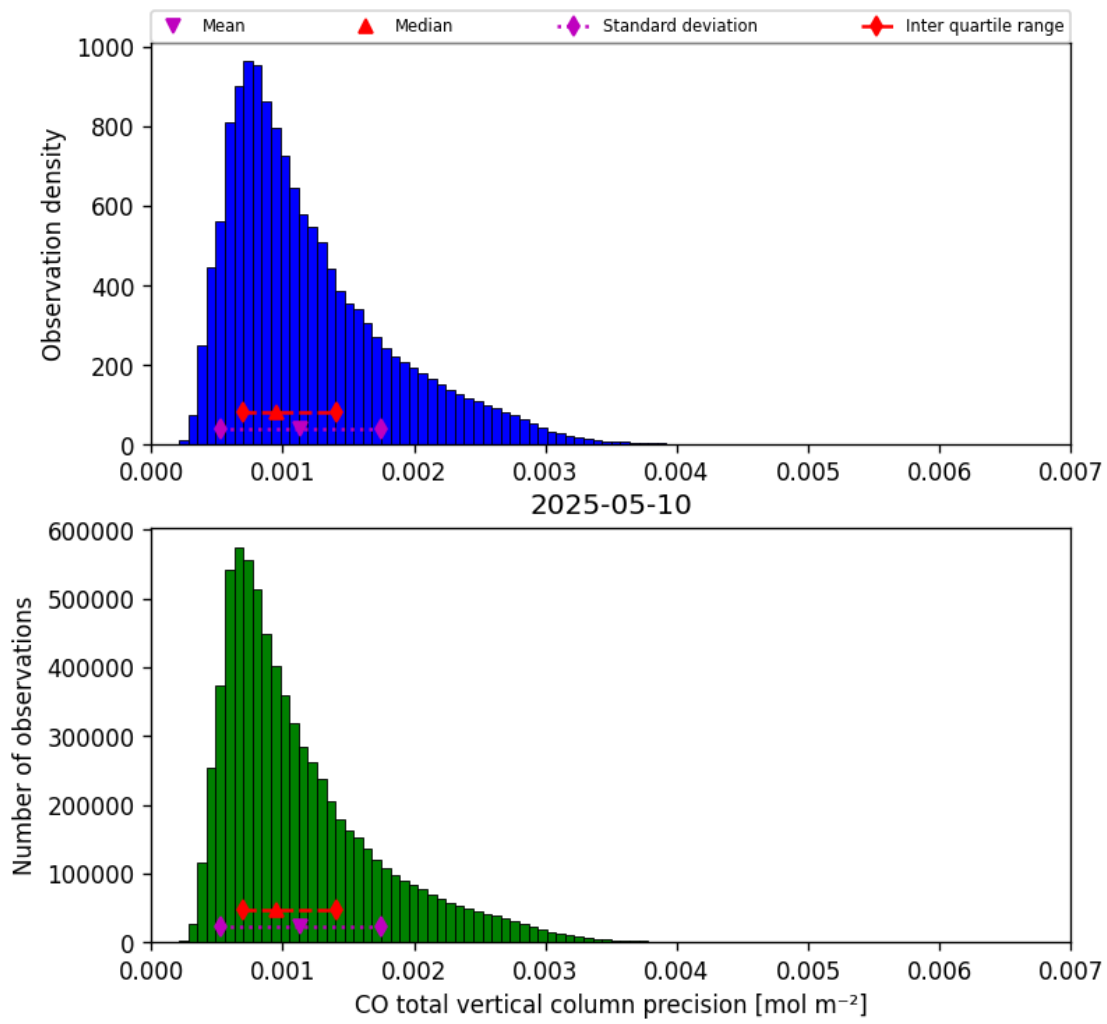
Figure 20: Histogram of “CO total vertical column precision” for 2025-05-10 to 2025-05-11
