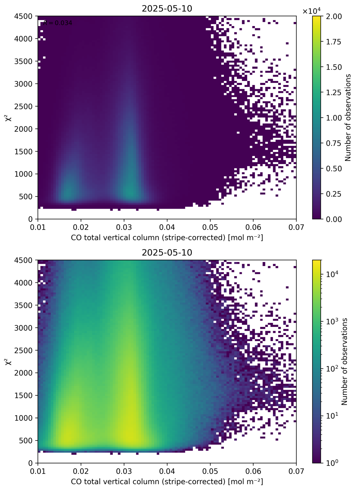
Figure 37: Scatter density plot of “CO total vertical column (stripe-corrected)” against “ \chi^2 ” for 2025-05-10 to 2025-05-11.
