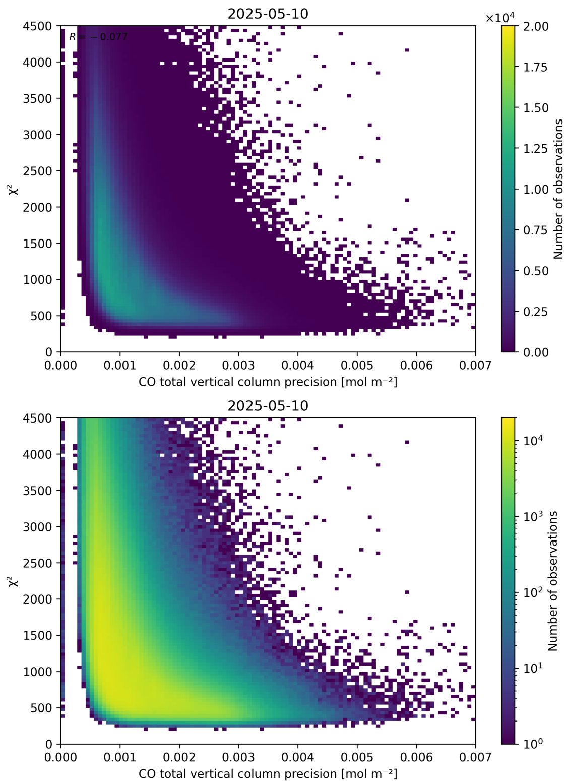
Figure 44: Scatter density plot of “CO total vertical column precision” against “ \chi^2 ” for 2025-05-10 to 2025-05-11.
