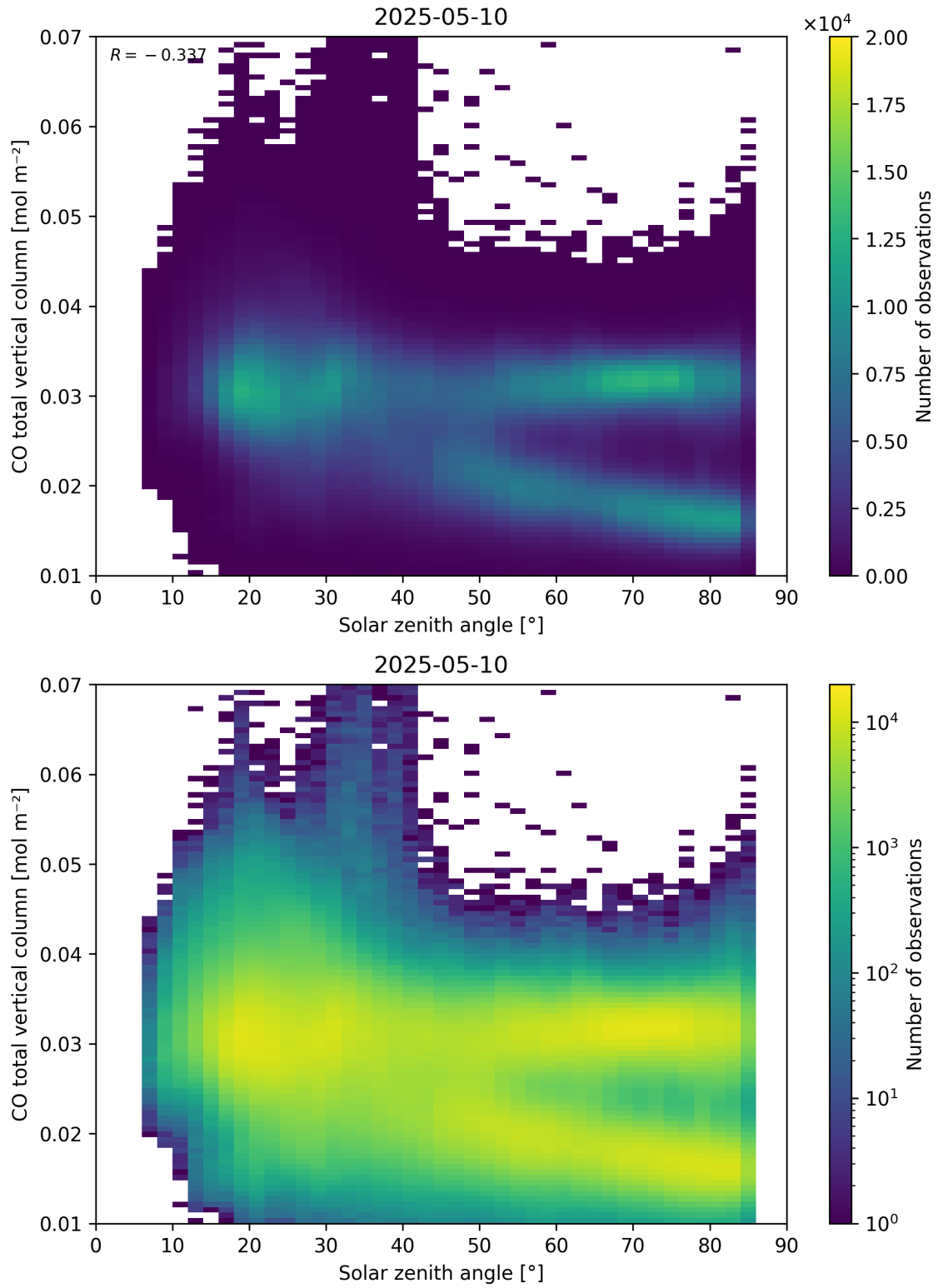
Figure 61: Scatter density plot of “Solar zenith angle” against “CO total vertical column” for 2025-05-10 to 2025-05-11.
