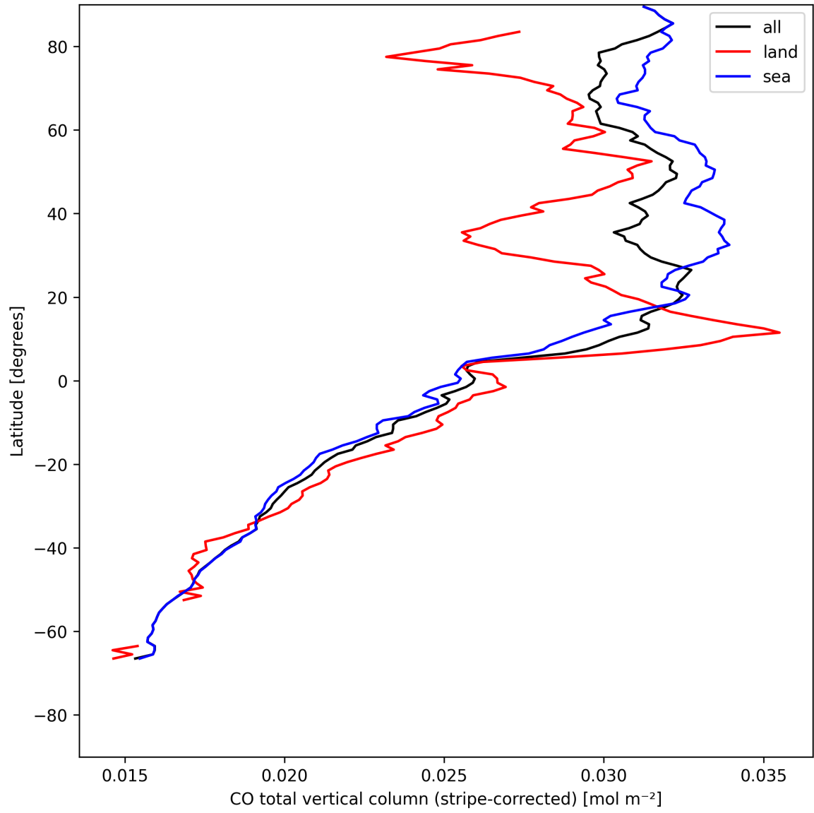
Figure 11: Zonal average of “CO total vertical column (stripe-corrected)” for 2025-05-10 to 2025-05-11.
