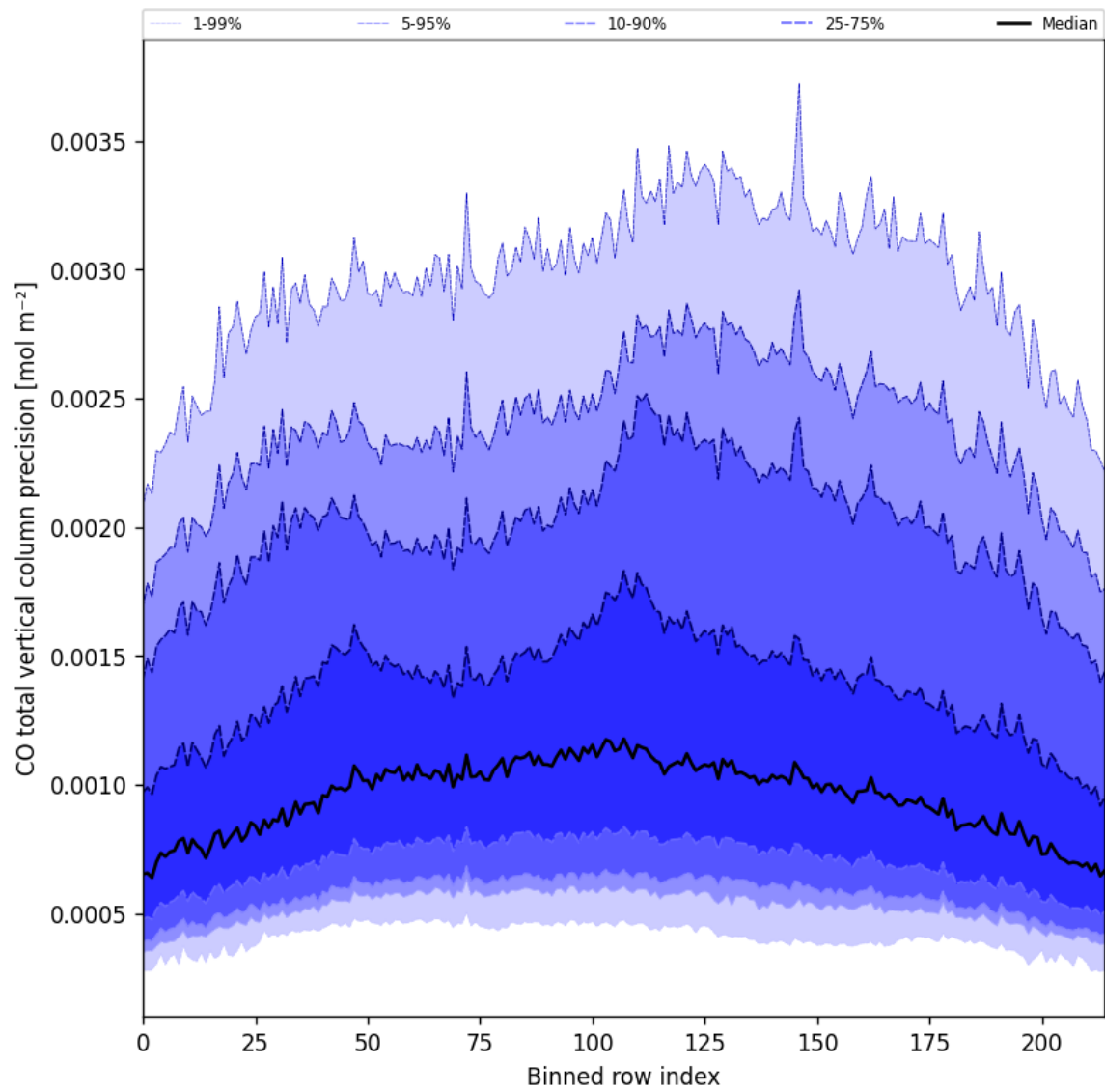
Figure 28: Along track statistics of “CO total vertical column precision” for 2025-05-10 to 2025-05-11
