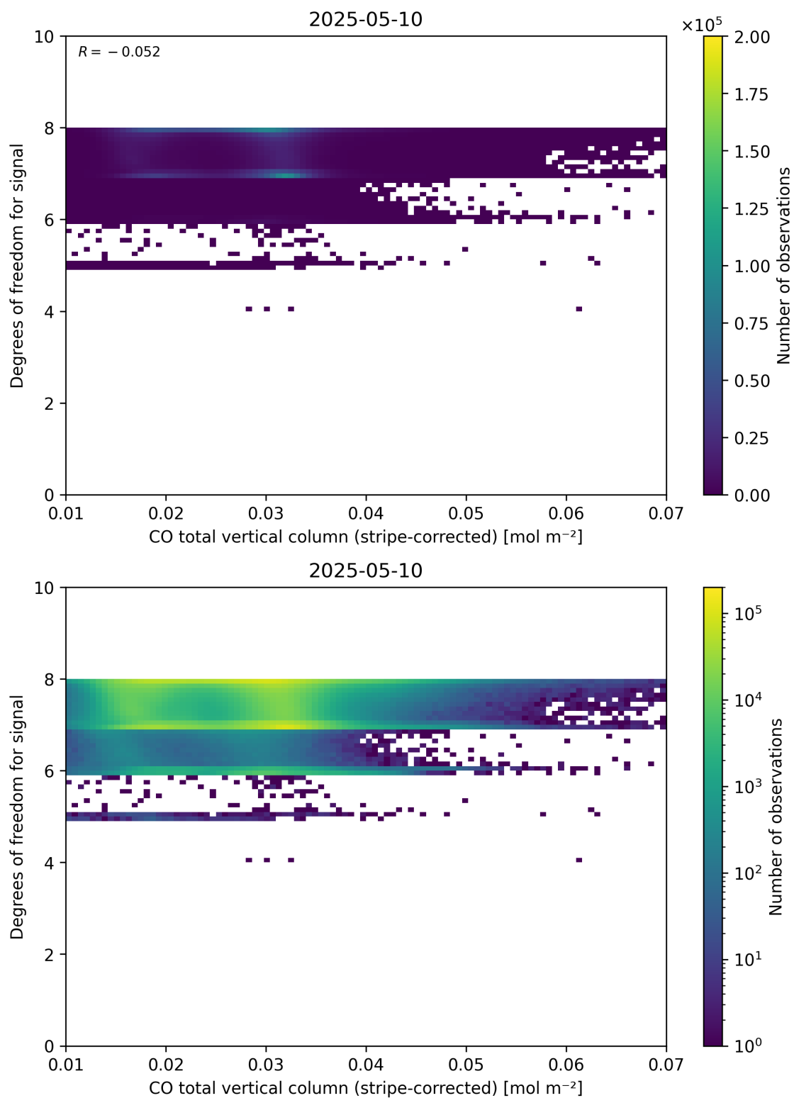
Figure 38: Scatter density plot of “CO total vertical column (stripe-corrected)” against “Degrees of freedom for signal” for 2025-05-10 to 2025-05-11.
