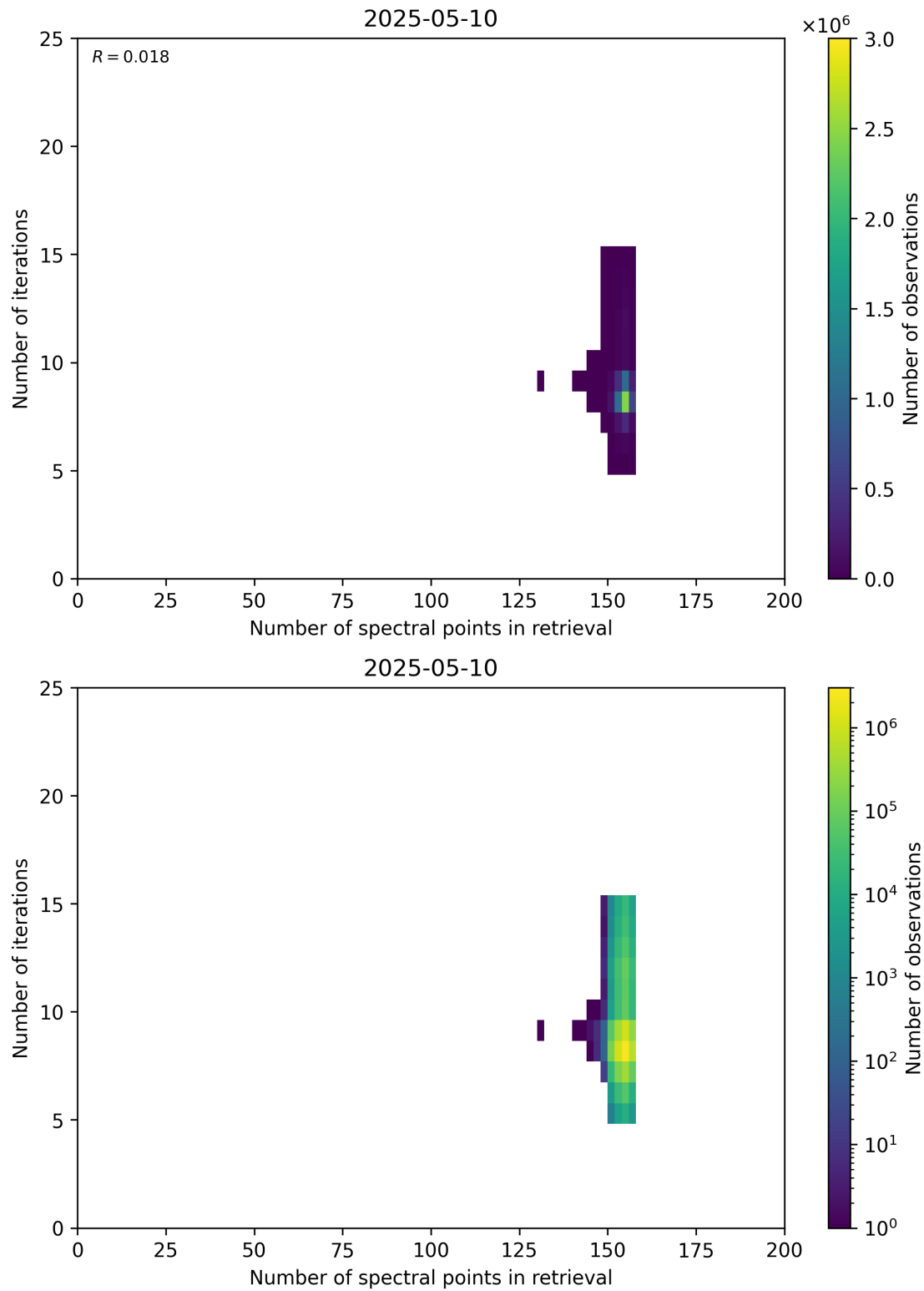
Figure 60: Scatter density plot of “Number of spectral points in retrieval” against “Number of iterations” for 2025-05-10 to 2025-05-11.
