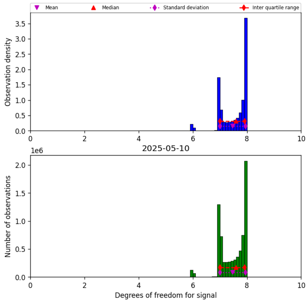
Figure 23: Histogram of “Degrees of freedom for signal” for 2025-05-10 to 2025-05-11
