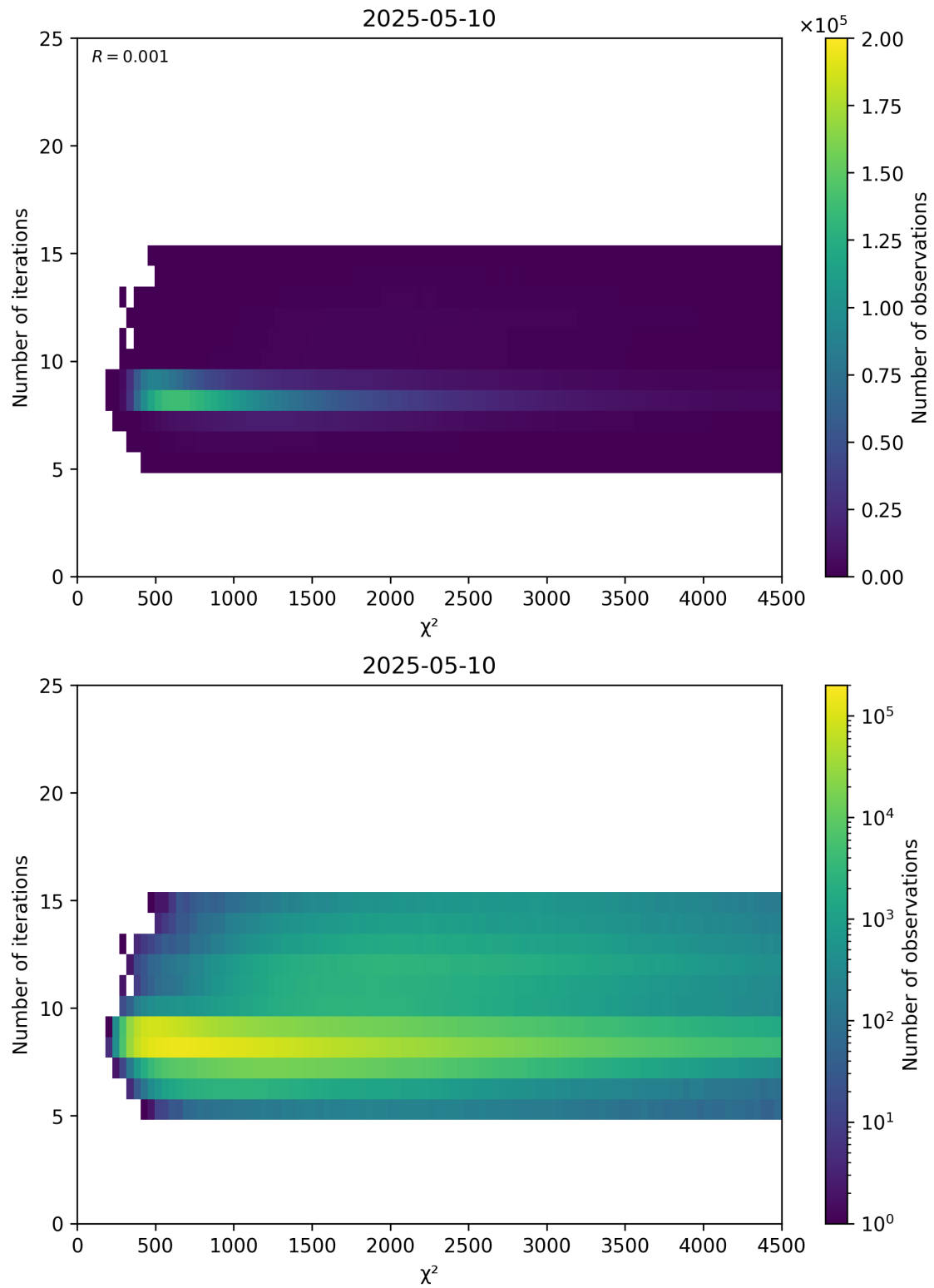
Figure 49: Scatter density plot of “ \chi^2 ” against “Number of iterations” for 2025-05-10 to 2025-05-11.
