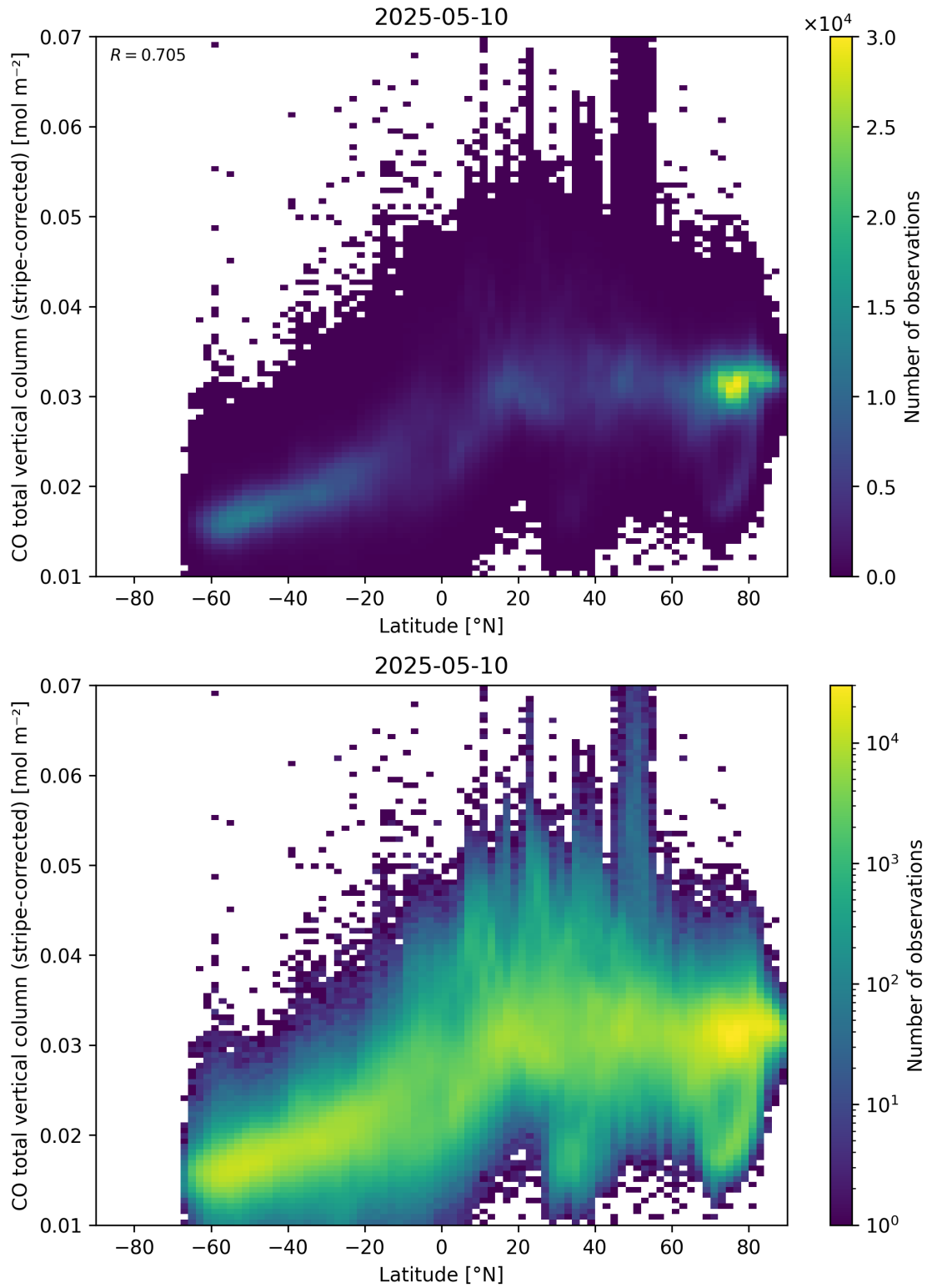
Figure 52: Scatter density plot of “Latitude” against “CO total vertical column (stripe-corrected)” for 2025-05-10 to 2025-05-11.
