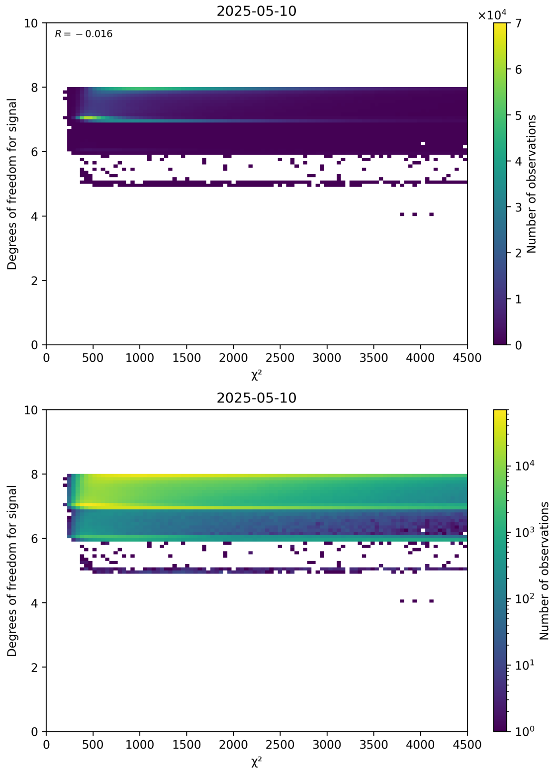
Figure 48: Scatter density plot of “ \chi^2 ” against “Degrees of freedom for signal” for 2025-05-10 to 2025-05-11.
