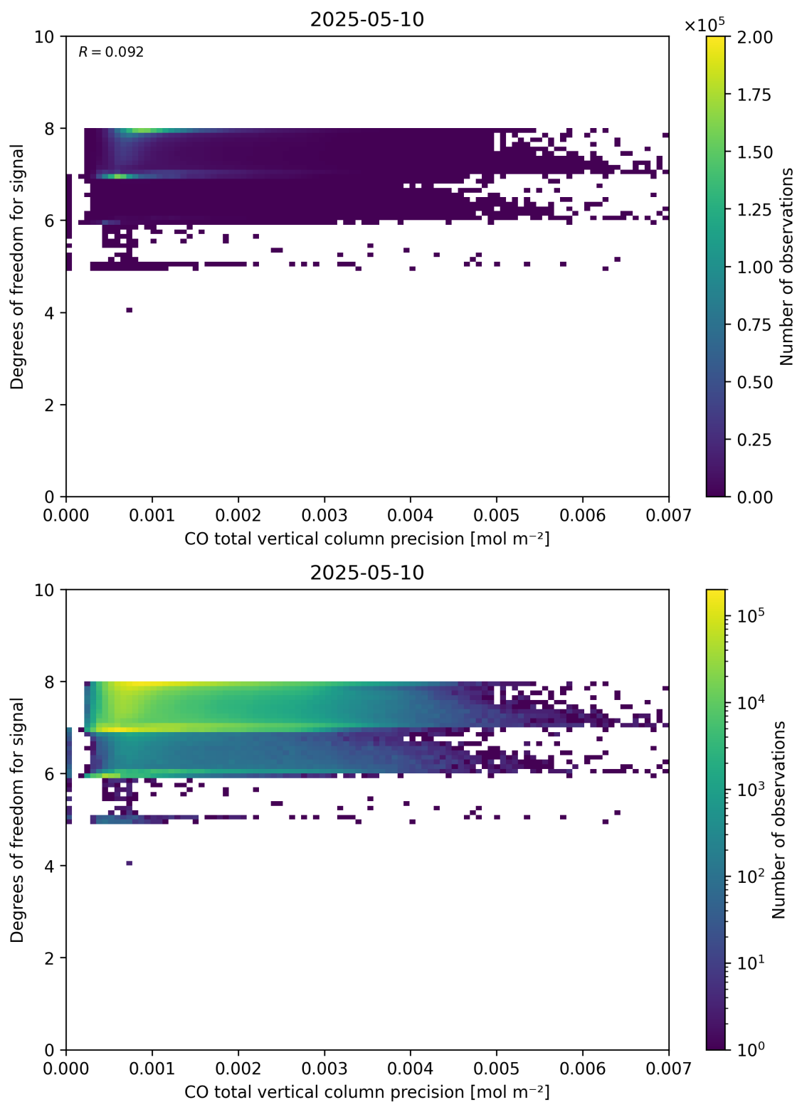
Figure 45: Scatter density plot of “CO total vertical column precision” against “Degrees of freedom for signal” for 2025-05-10 to 2025-05-11.
