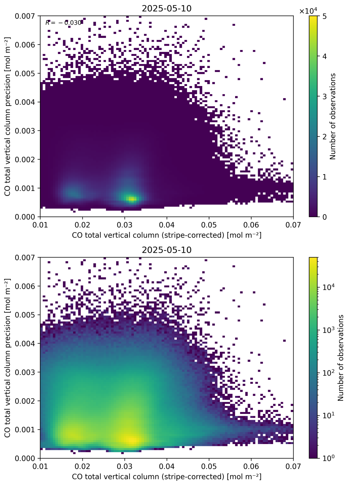
Figure 36: Scatter density plot of “CO total vertical column (stripe-corrected)” against “CO total vertical column precision” for 2025-05-10 to 2025-05-11.
