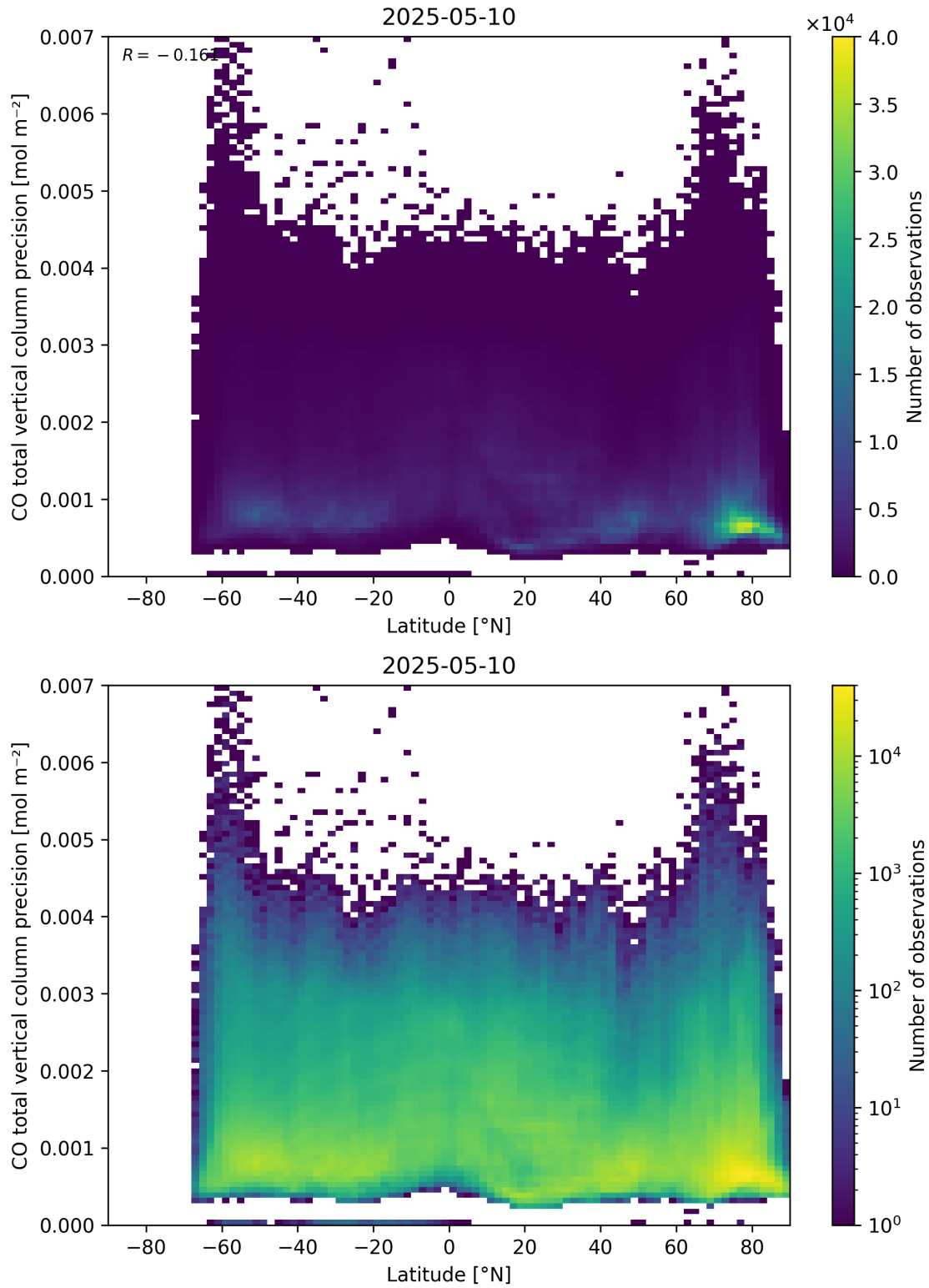
Figure 53: Scatter density plot of “Latitude” against “CO total vertical column precision” for 2025-05-10 to 2025-05-11.
