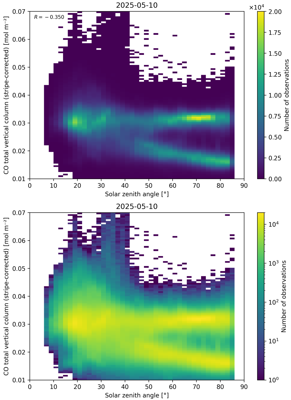
Figure 62: Scatter density plot of “Solar zenith angle” against “CO total vertical column (stripe-corrected)” for 2025-05-10 to 2025-05-11.
