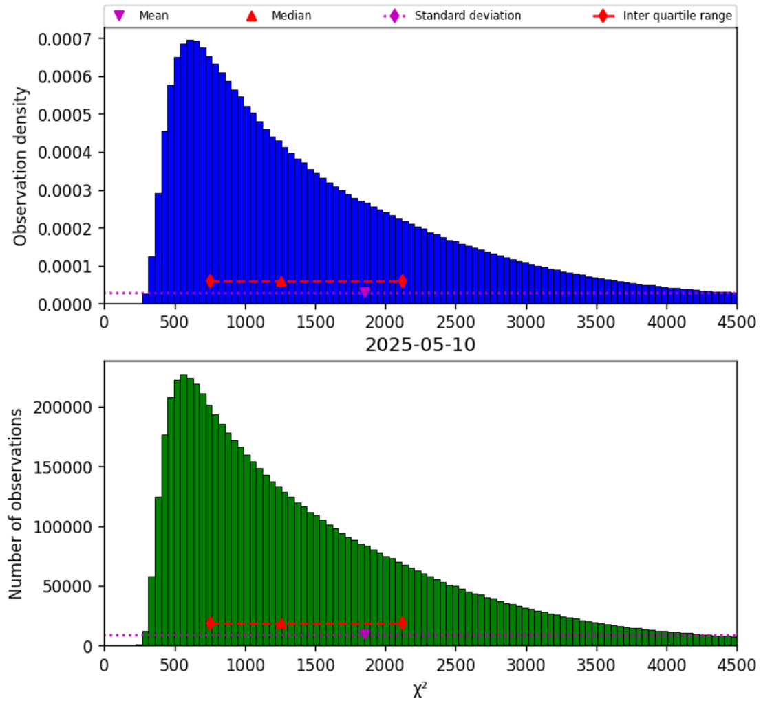
Figure 22: Histogram of “ \chi^2 ” for 2025-05-10 to 2025-05-11
