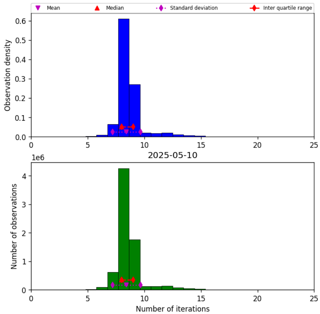
Figure 24: Histogram of “Number of iterations” for 2025-05-10 to 2025-05-11
