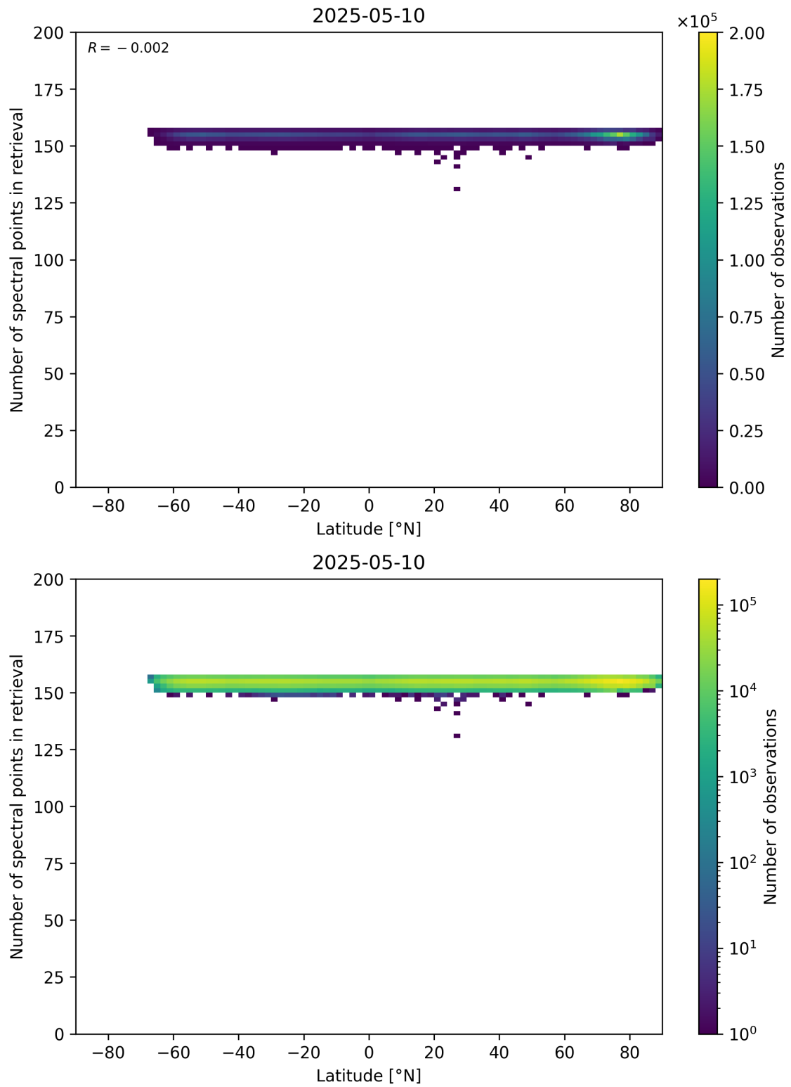
Figure 57: Scatter density plot of “Latitude” against “Number of spectral points in retrieval” for 2025-05-10 to 2025-05-11.
