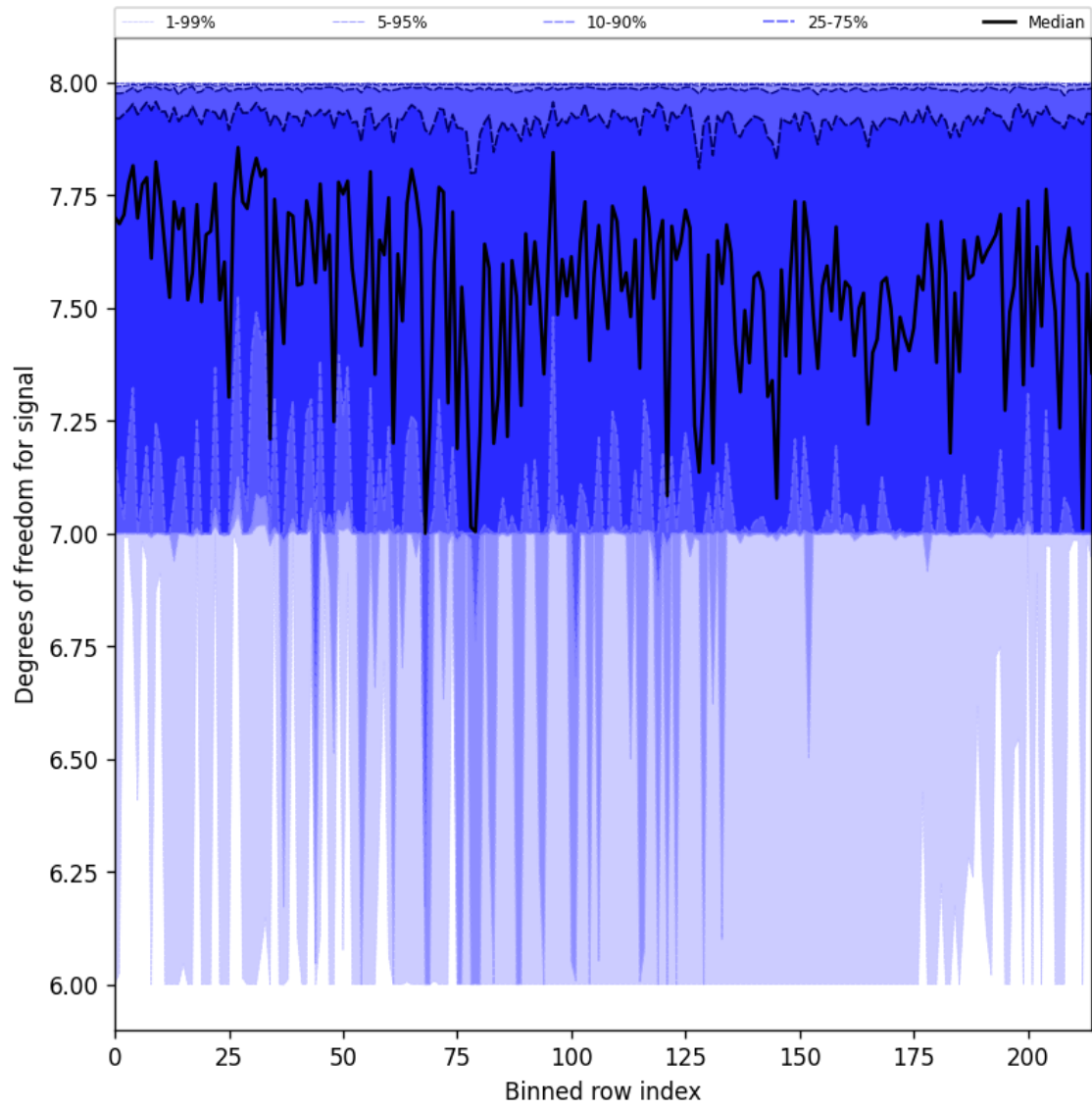
Figure 31: Along track statistics of “Degrees of freedom for signal” for 2025-05-10 to 2025-05-11
