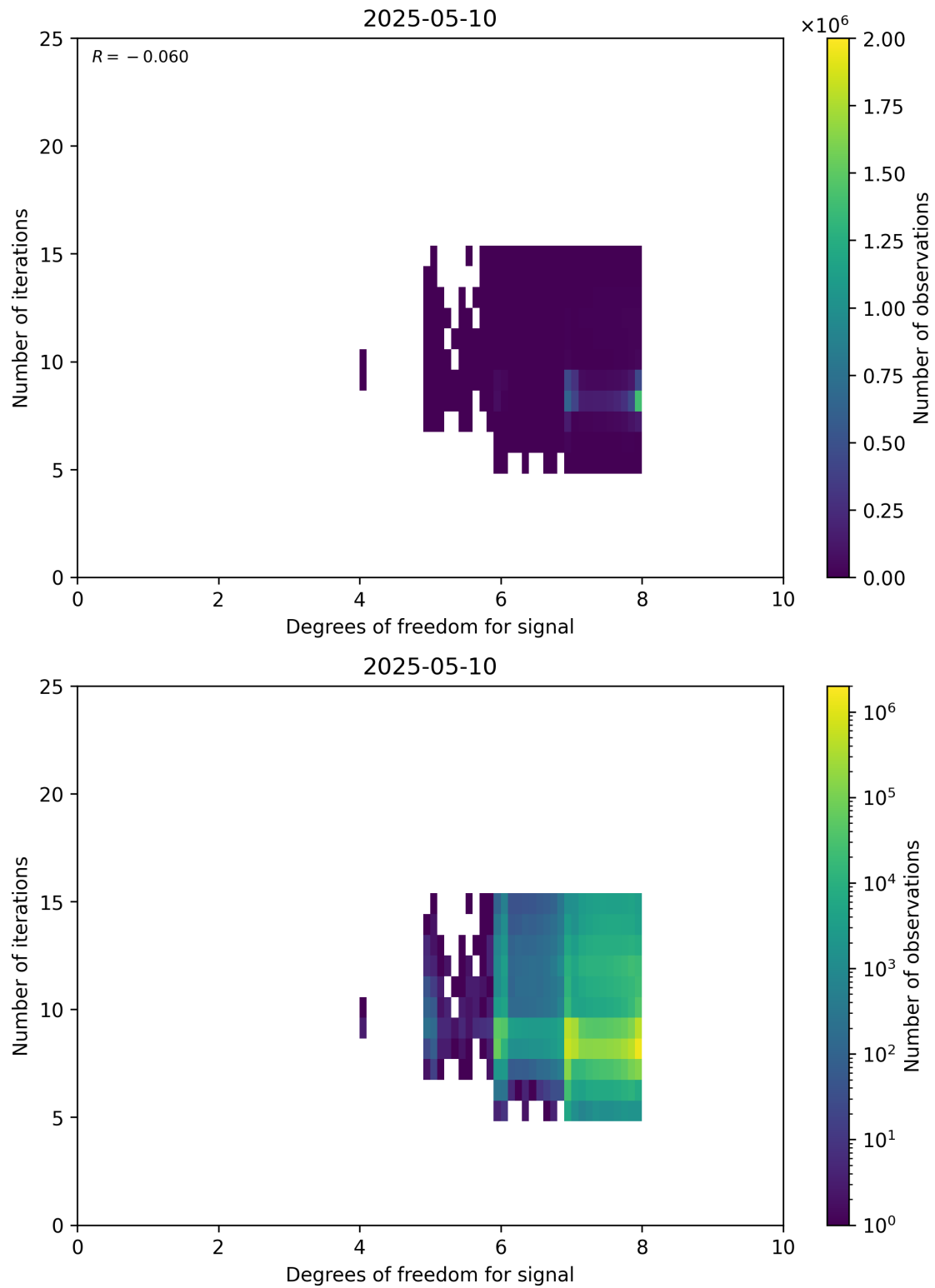
Figure 50: Scatter density plot of “Degrees of freedom for signal” against “Number of iterations” for 2025-05-10 to 2025-05-11.
