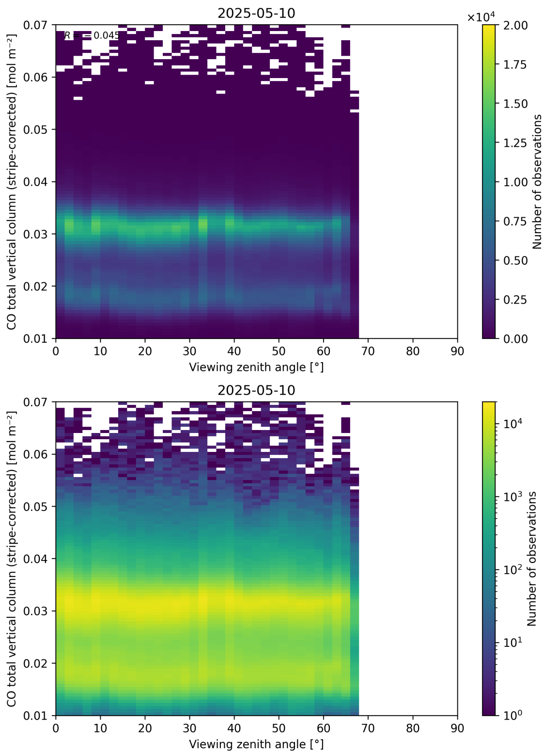
Figure 70: Scatter density plot of “Viewing zenith angle” against “CO total vertical column (stripe-corrected)” for 2025-05-10 to 2025-05-11.
