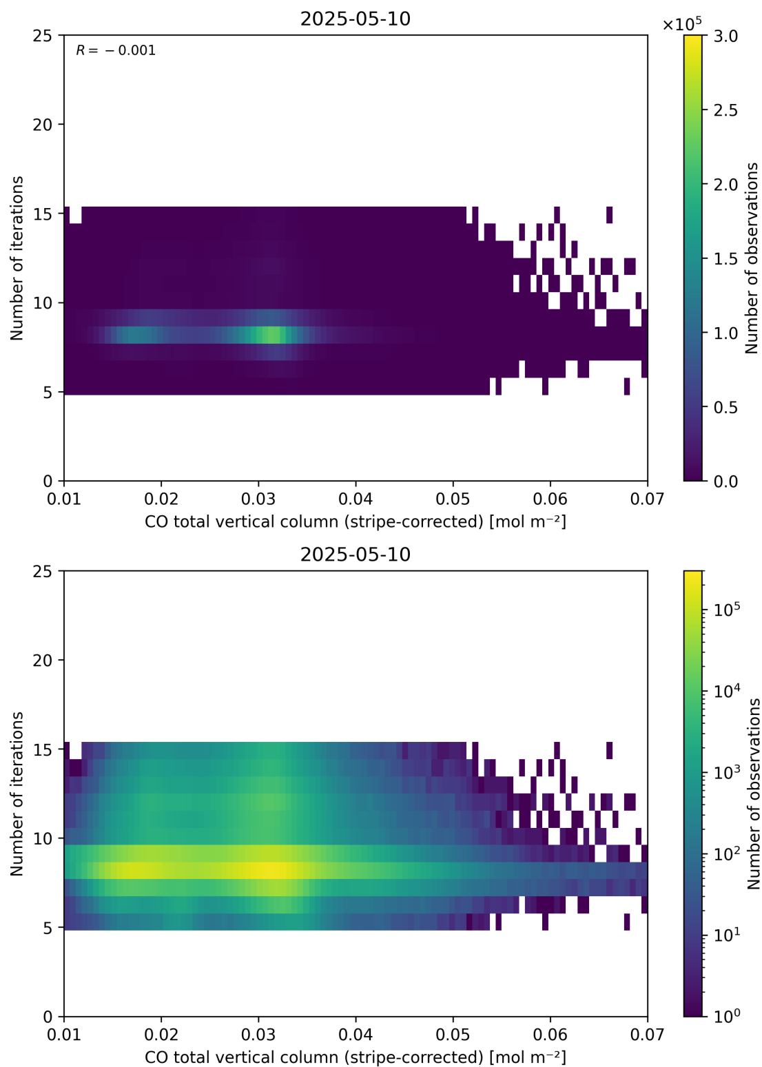
Figure 39: Scatter density plot of “CO total vertical column (stripe-corrected)” against “Number of iterations” for 2025-05-10 to 2025-05-11.
