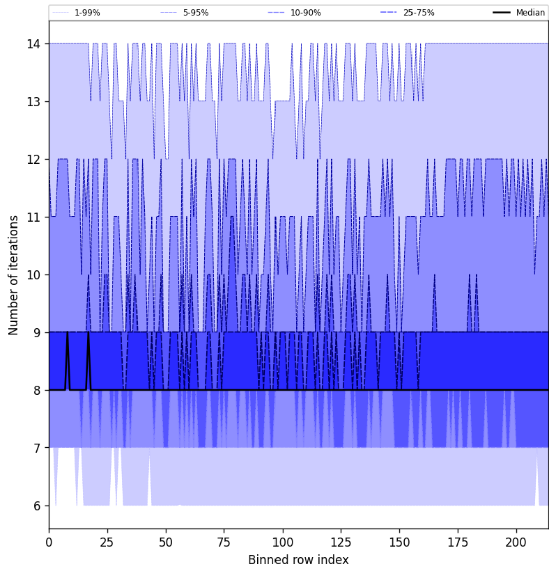
Figure 32: Along track statistics of “Number of iterations” for 2025-05-10 to 2025-05-11
