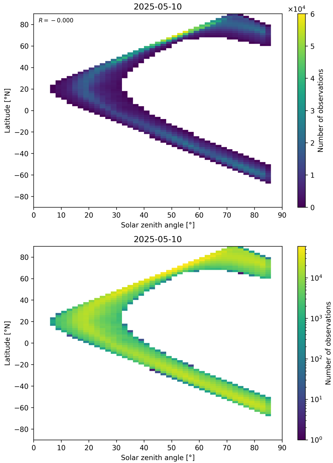
Figure 66: Scatter density plot of “Solar zenith angle” against “Latitude” for 2025-05-10 to 2025-05-11.
