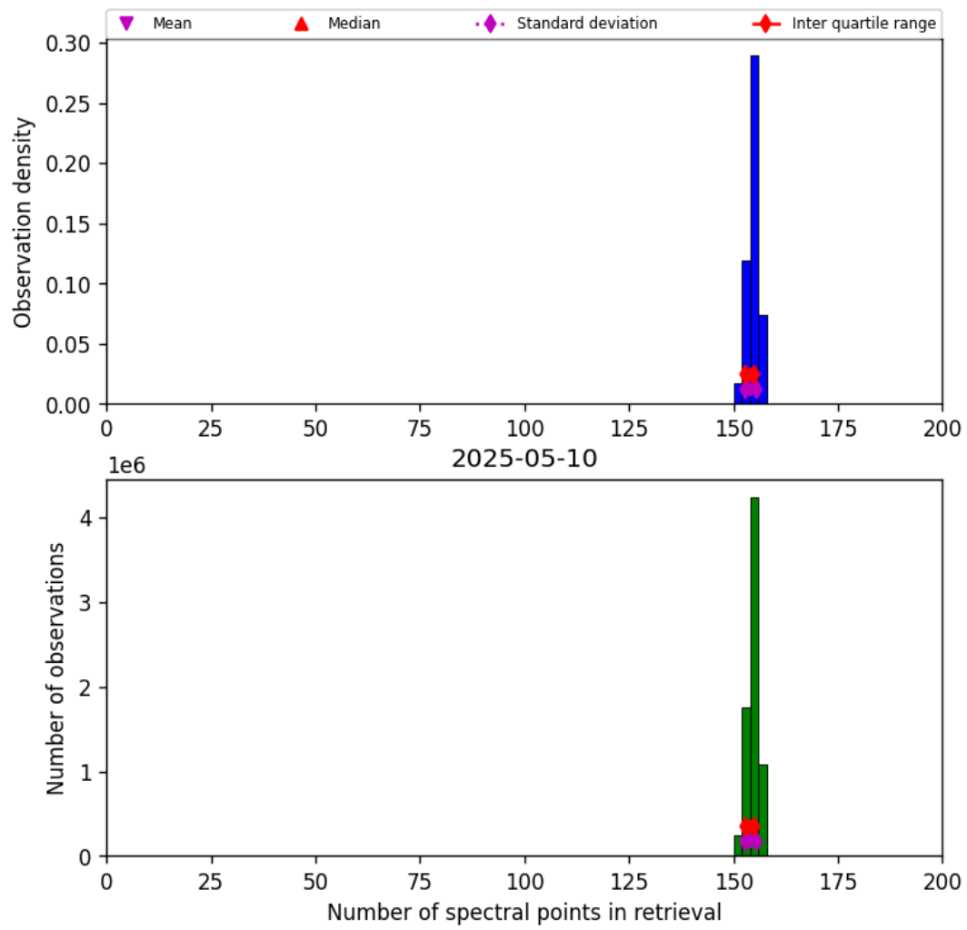
Figure 21: Histogram of “Number of spectral points in retrieval” for 2025-05-10 to 2025-05-11
