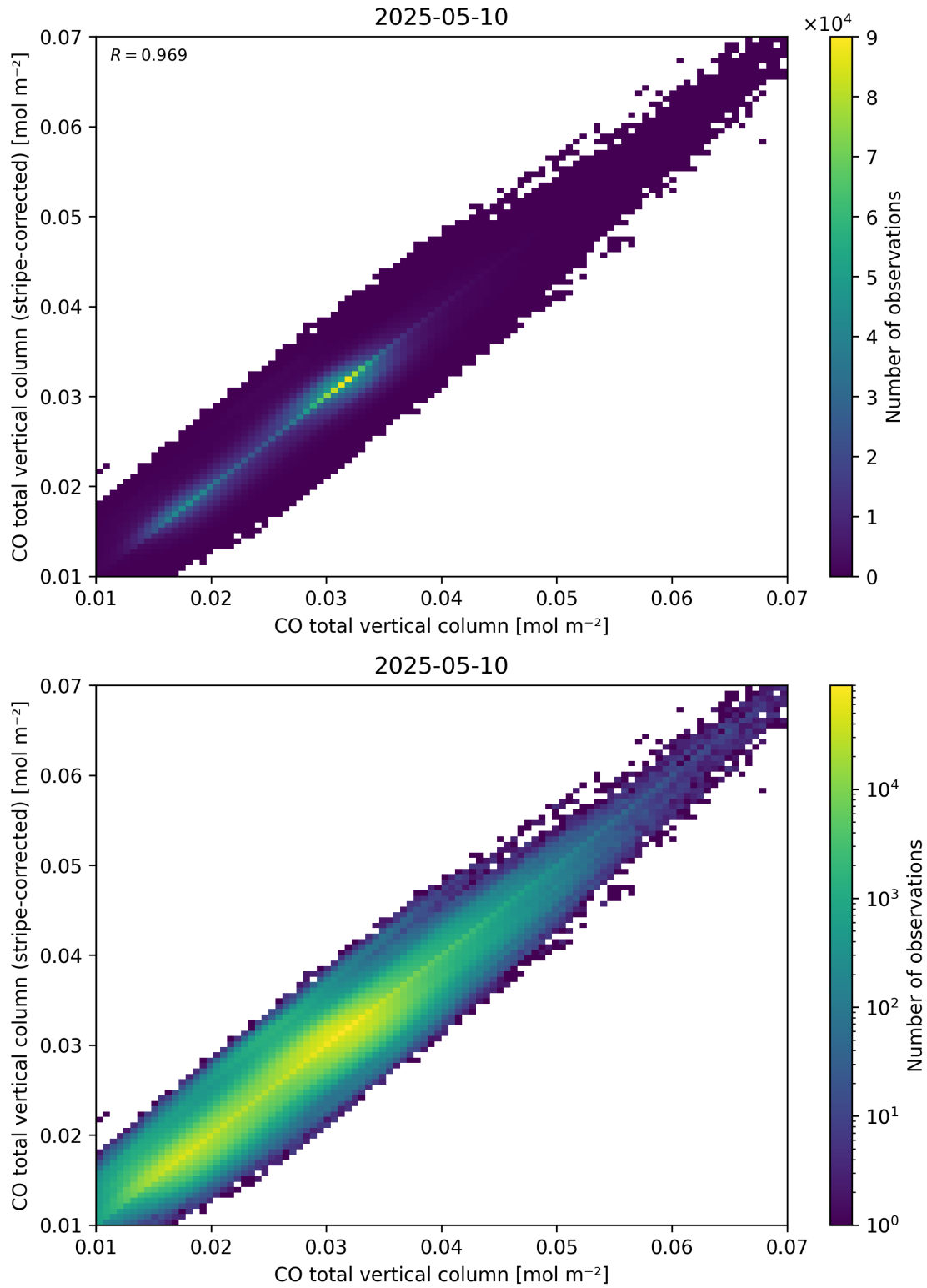
Figure 33: Scatter density plot of “CO total vertical column” against “CO total vertical column (stripe-corrected)” for 2025-05-10 to 2025-05-11.
