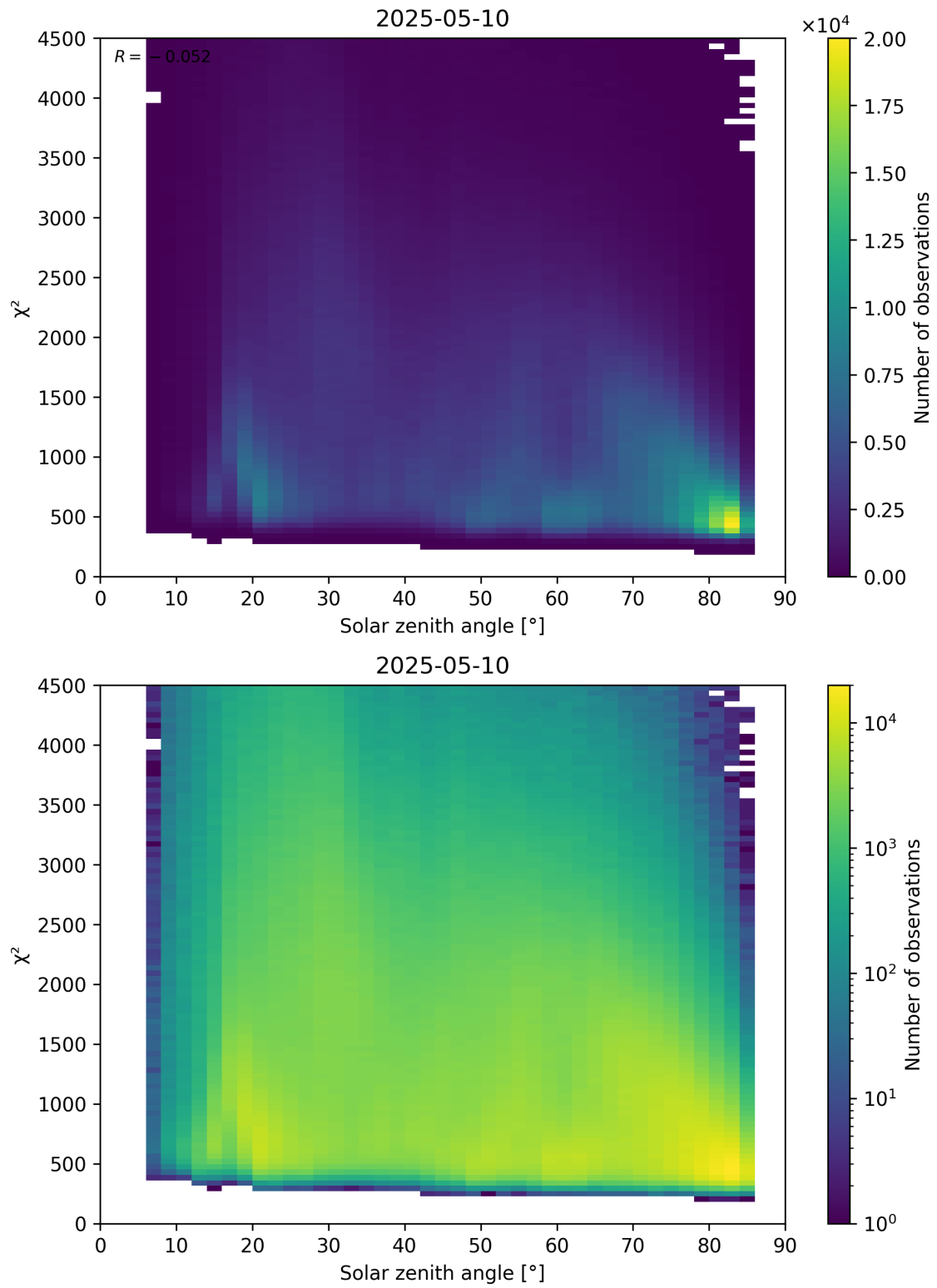
Figure 64: Scatter density plot of “Solar zenith angle” against “ \chi^2 ” for 2025-05-10 to 2025-05-11.
