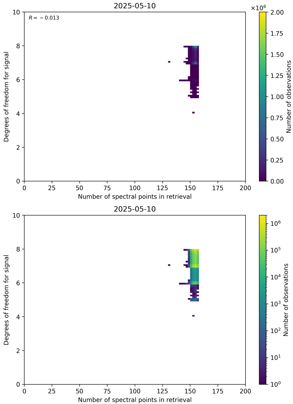
Figure 59: Scatter density plot of “Number of spectral points in retrieval” against “Degrees of freedom for signal” for 2025-05-10 to 2025-05-11.
