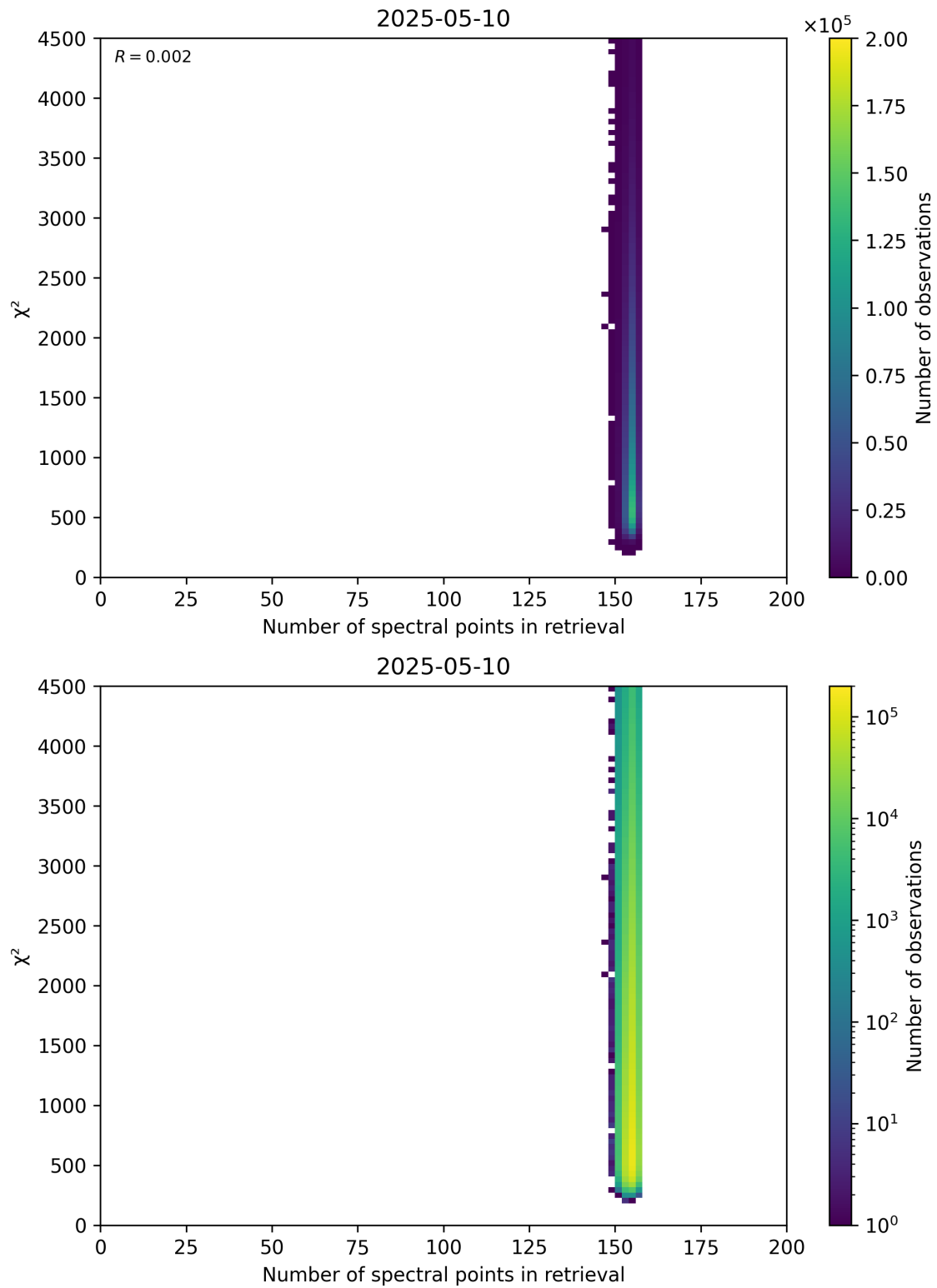
Figure 58: Scatter density plot of “Number of spectral points in retrieval” against “ \chi^2 ” for 2025-05-10 to 2025-05-11.
