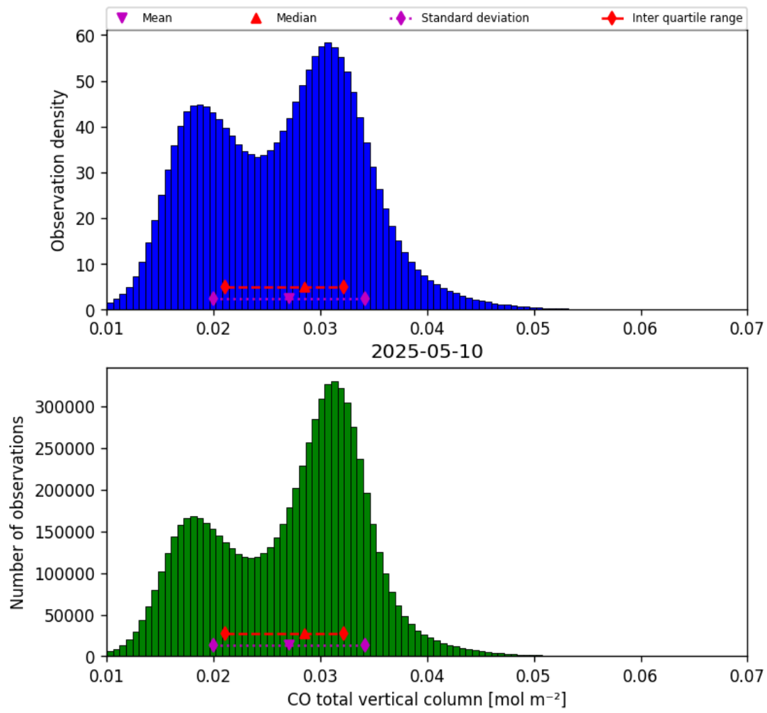
Figure 18: Histogram of “CO total vertical column” for 2025-05-10 to 2025-05-11
