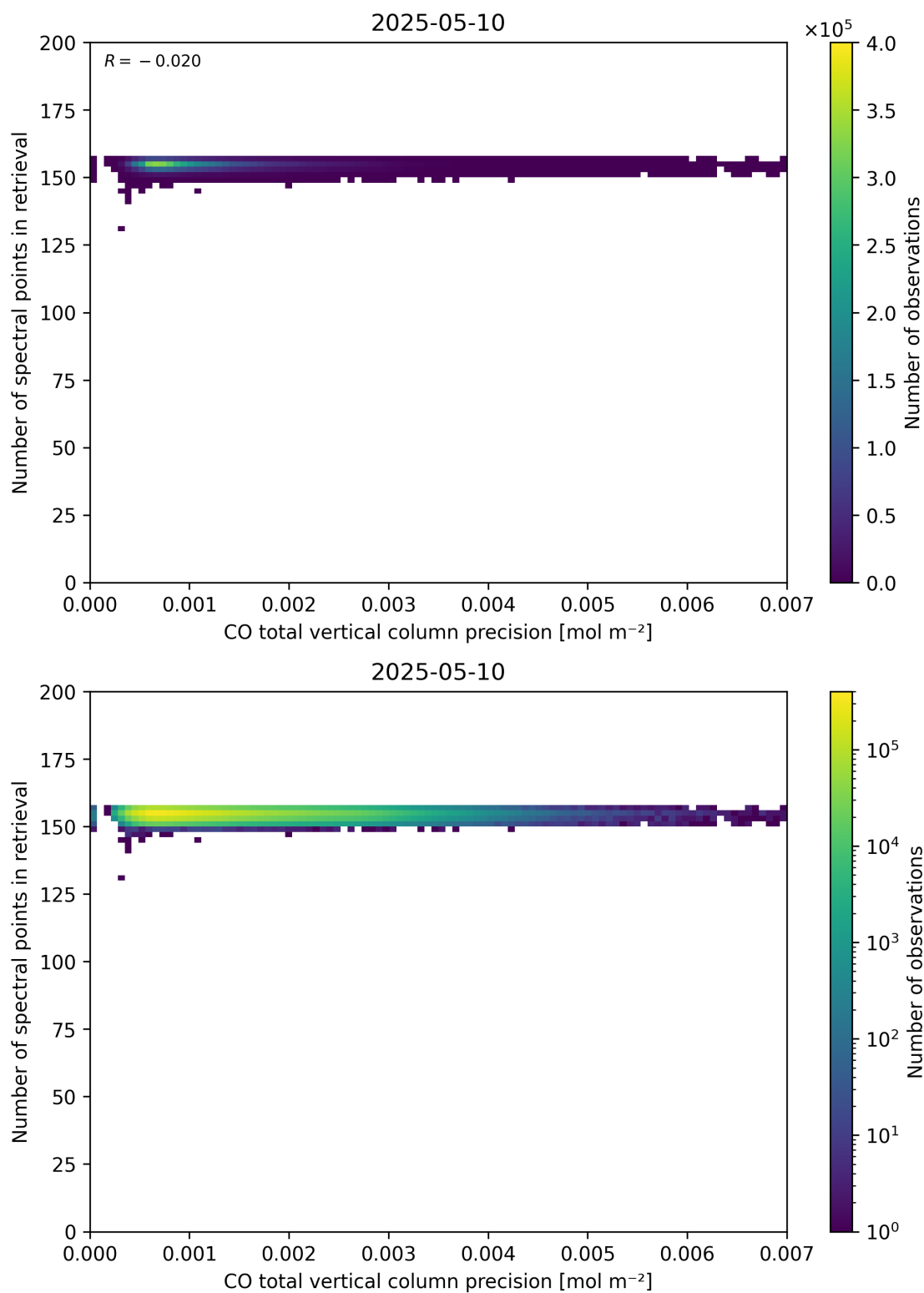
Figure 47: Scatter density plot of “CO total vertical column precision” against “Number of spectral points in retrieval” for 2025-05-10 to 2025-05-11.
