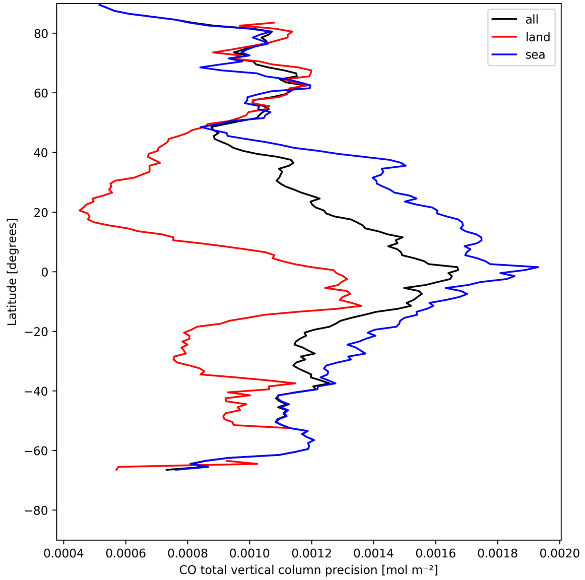
Figure 12: Zonal average of “CO total vertical column precision” for 2025-05-10 to 2025-05-11.
