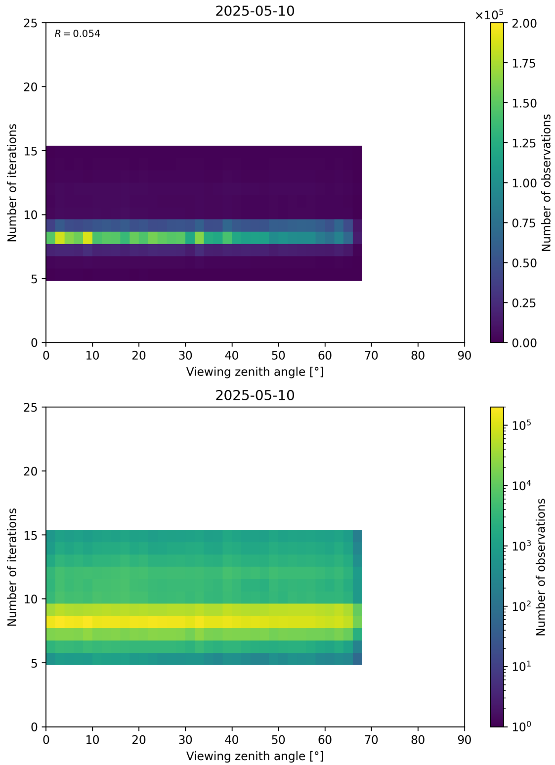
Figure 75: Scatter density plot of “Viewing zenith angle” against “Number of iterations” for 2025-05-10 to 2025-05-11.
