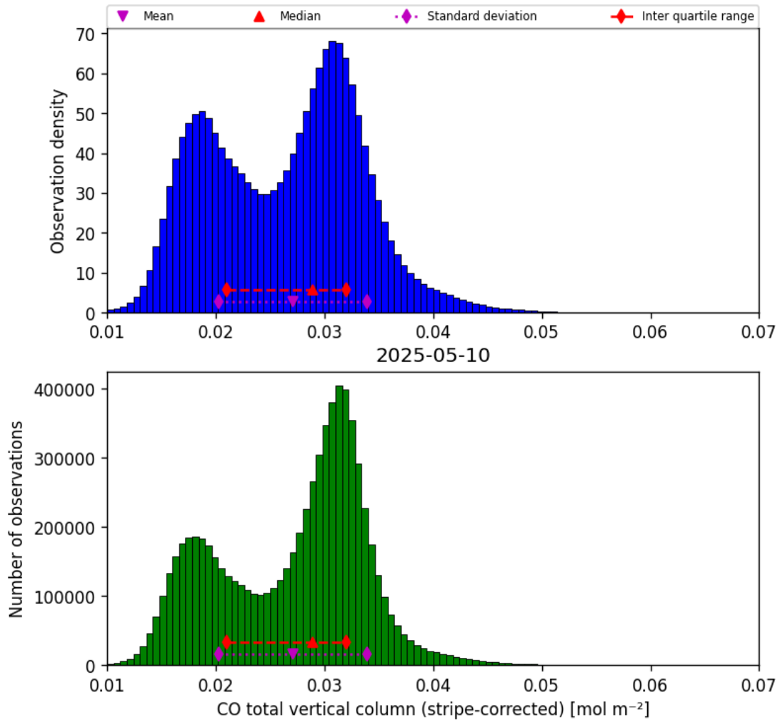
Figure 19: Histogram of “CO total vertical column (stripe-corrected)” for 2025-05-10 to 2025-05-11
