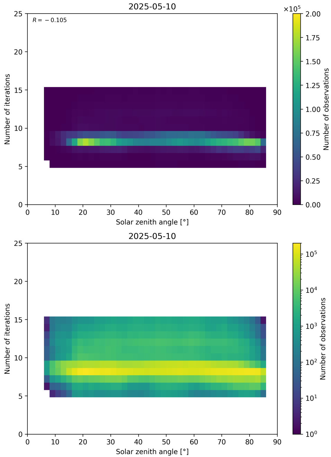
Figure 67: Scatter density plot of “Solar zenith angle” against “Number of iterations” for 2025-05-10 to 2025-05-11.
