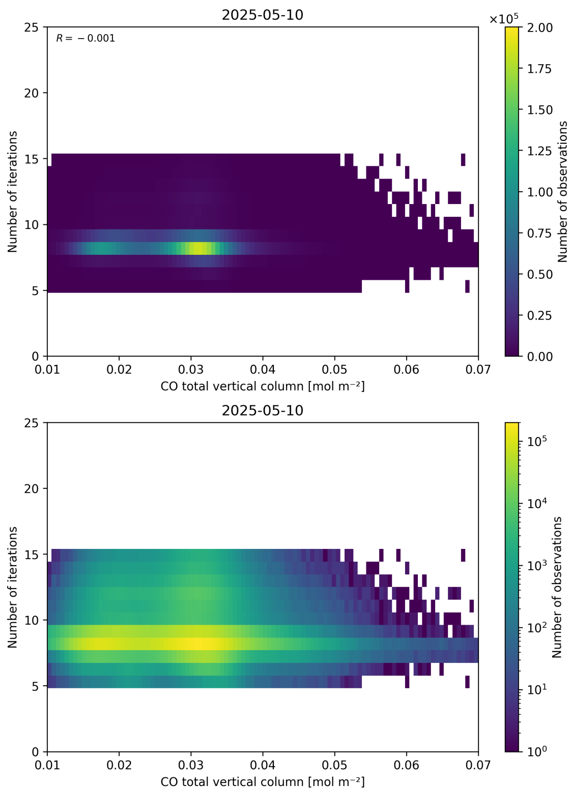
Figure 42: Scatter density plot of “CO total vertical column” against “Number of iterations” for 2025-05-10 to 2025-05-11.
