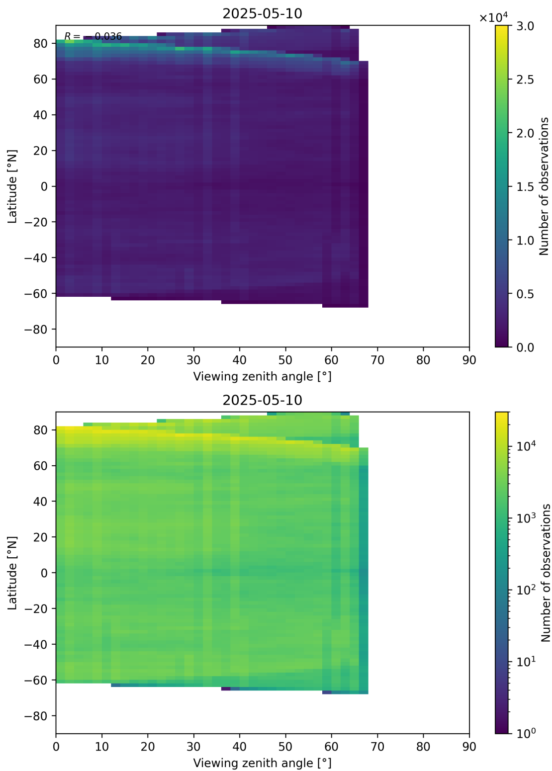
Figure 74: Scatter density plot of “Viewing zenith angle” against “Latitude” for 2025-05-10 to 2025-05-11.
