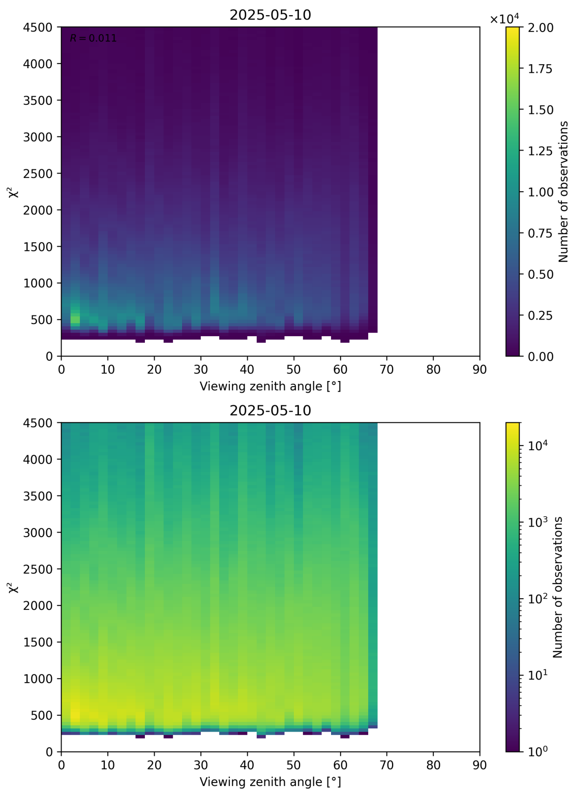
Figure 72: Scatter density plot of “Viewing zenith angle” against “ \chi^2 ” for 2025-05-10 to 2025-05-11.
