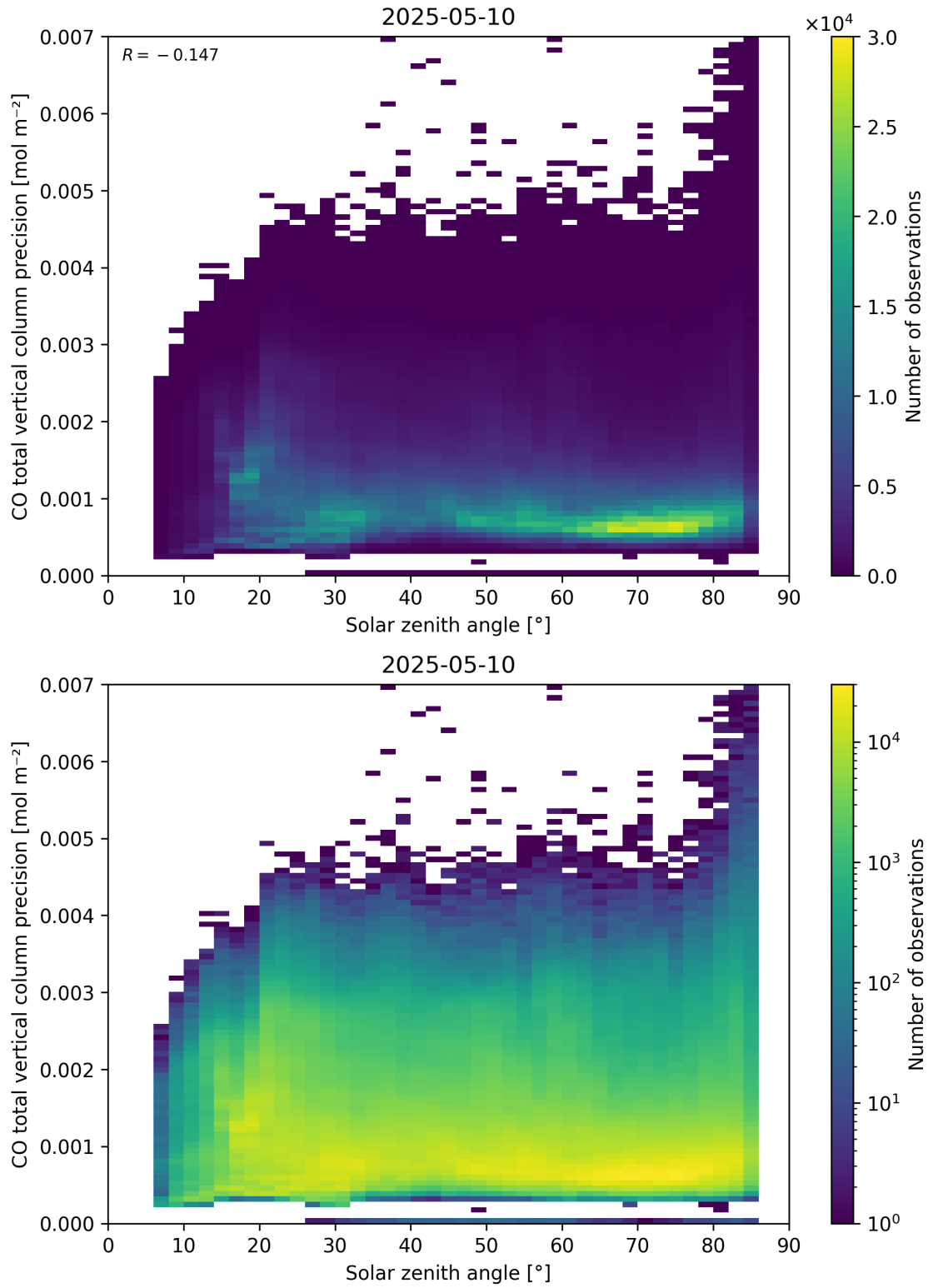
Figure 63: Scatter density plot of “Solar zenith angle” against “CO total vertical column precision” for 2025-05-10 to 2025-05-11.
