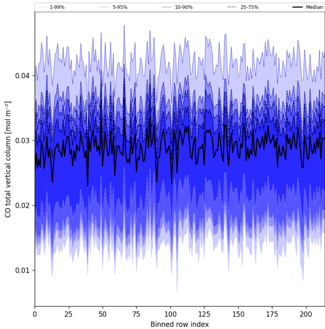
Figure 26: Along track statistics of "CO total vertical column" for 2025-05-10 to 2025-05-11
