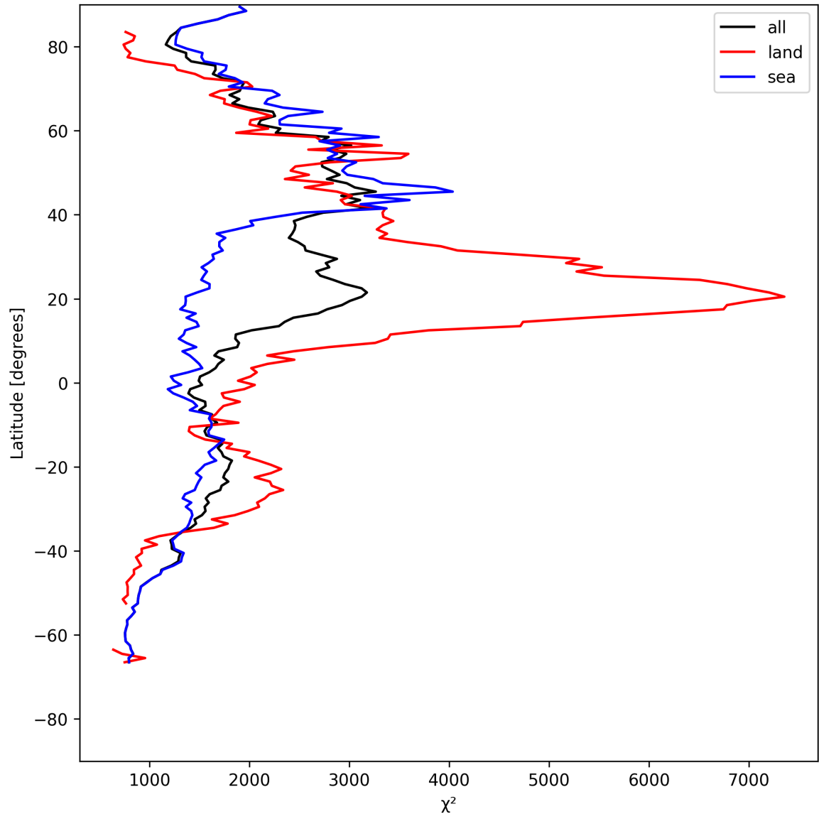
Figure 14: Zonal average of “ \chi^2 ” for 2025-05-10 to 2025-05-11.
