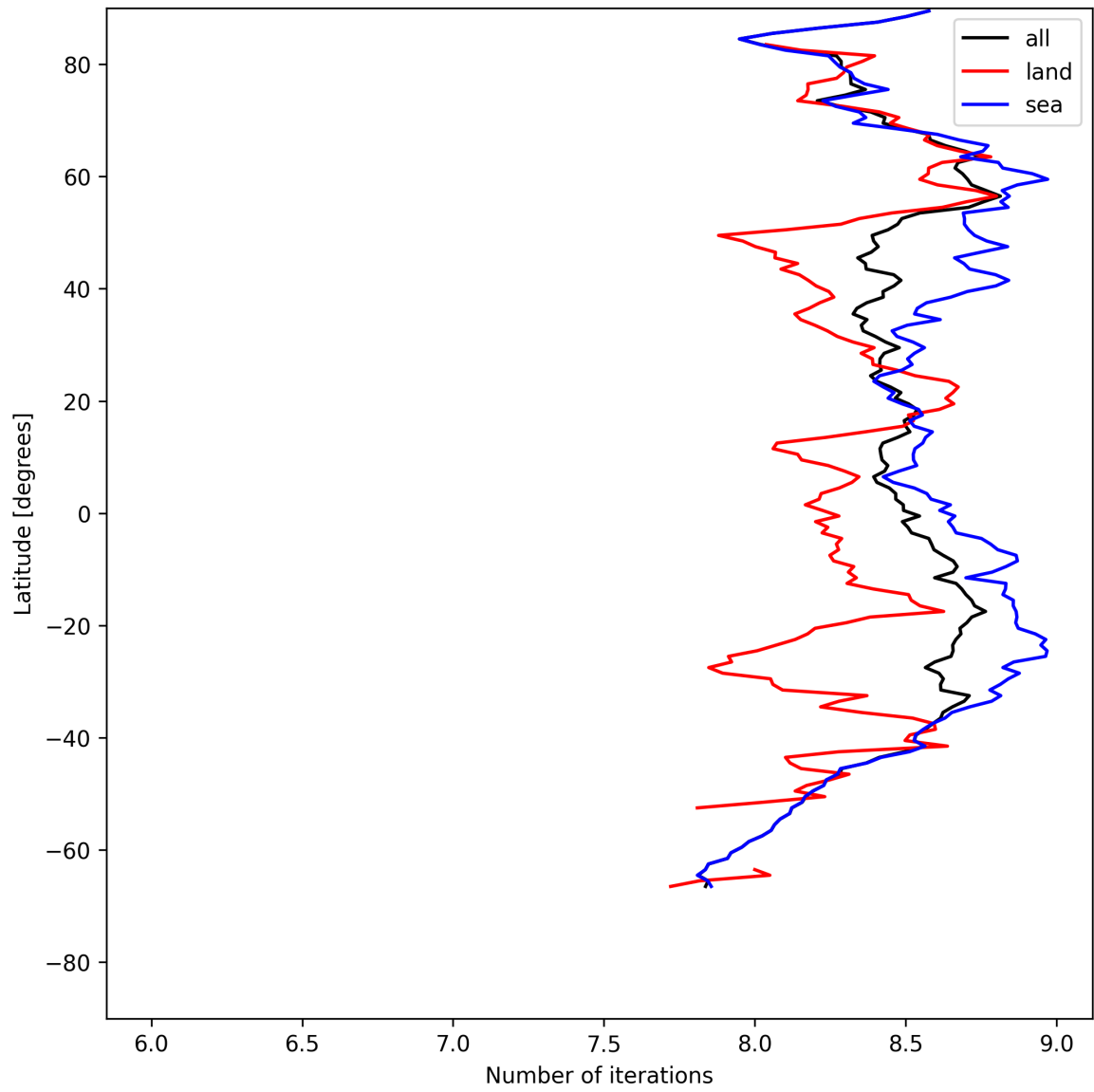
Figure 16: Zonal average of “Number of iterations” for 2025-05-10 to 2025-05-11.
