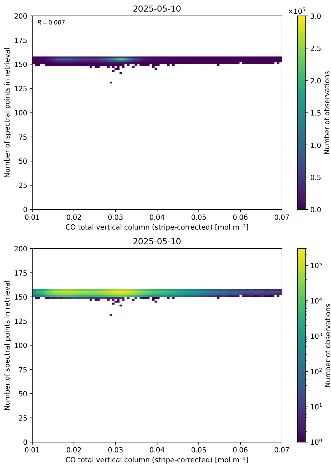
Figure 40: Scatter density plot of “CO total vertical column (stripe-corrected)” against “Number of spectral points in retrieval” for 2025-05-10 to 2025-05-11.
