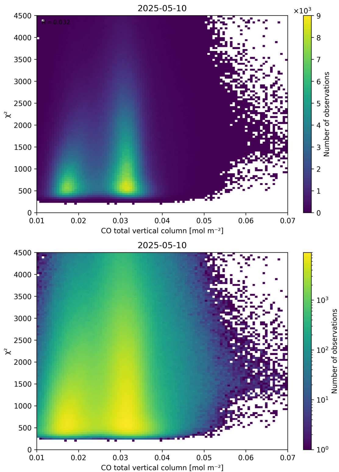
Figure 35: Scatter density plot of “CO total vertical column” against “ \chi^2 ” for 2025-05-10 to 2025-05-11.
