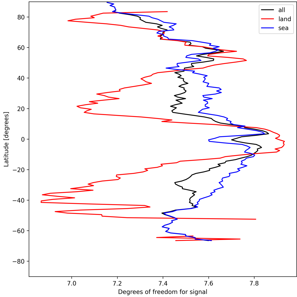
Figure 15: Zonal average of “Degrees of freedom for signal” for 2025-05-10 to 2025-05-11.
