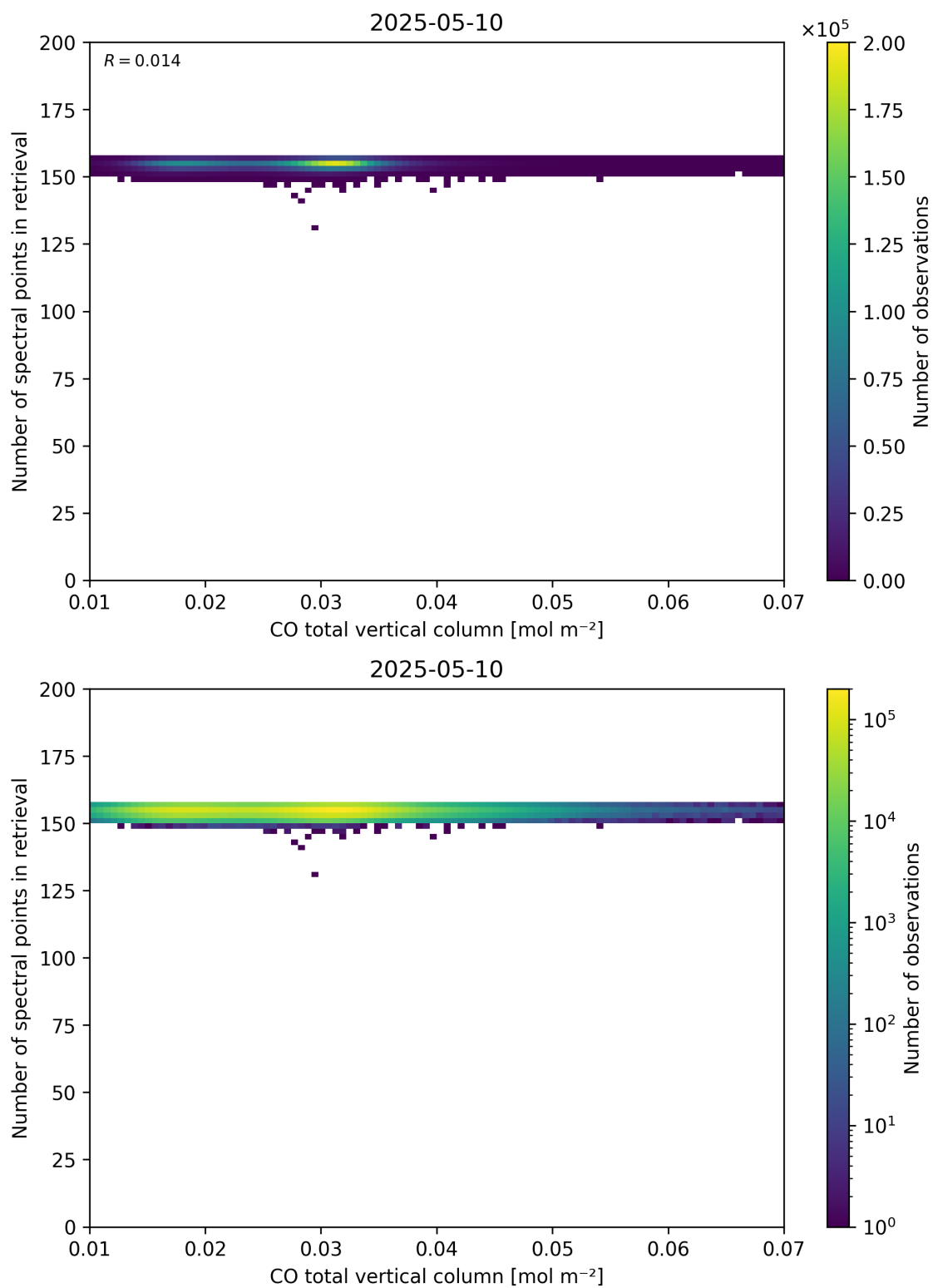
Figure 43: Scatter density plot of “CO total vertical column” against “Number of spectral points in retrieval” for 2025-05-10 to 2025-05-11.
