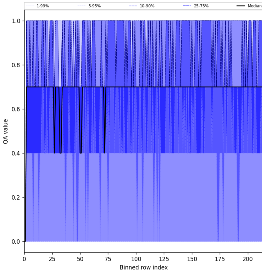
Figure 25: Along track statistics of “QA value” for 2025-05-10 to 2025-05-11
