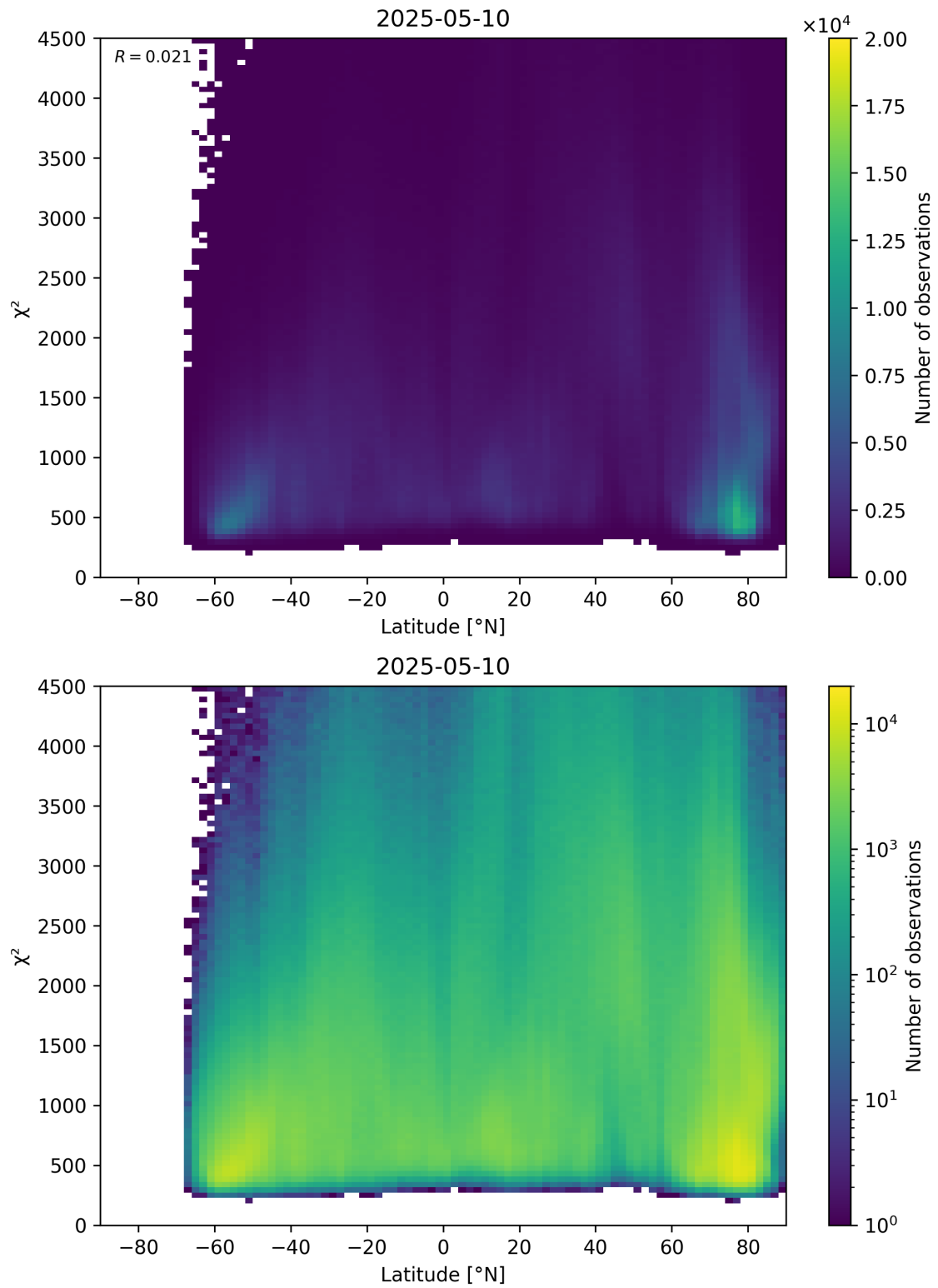
Figure 54: Scatter density plot of “Latitude” against “ \chi^2 ” for 2025-05-10 to 2025-05-11.
