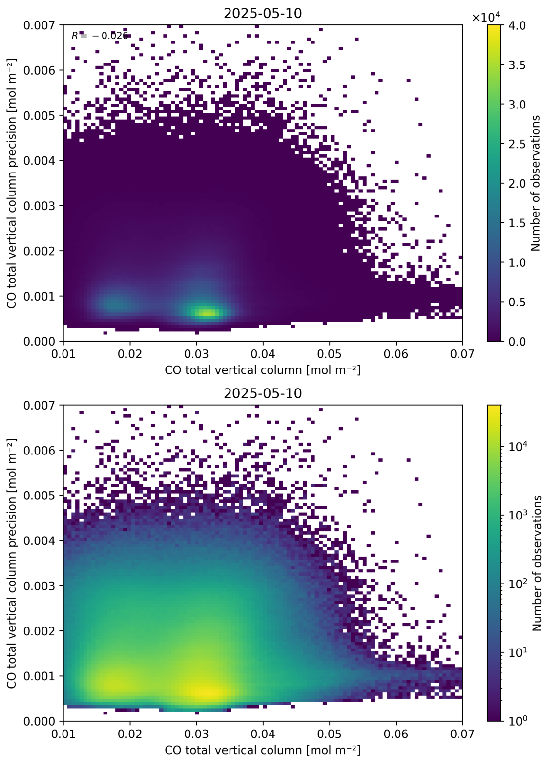
Figure 34: Scatter density plot of “CO total vertical column” against “CO total vertical column precision” for 2025-05-10 to 2025-05-11.
