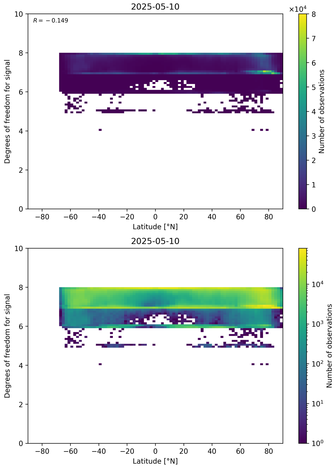
Figure 55: Scatter density plot of “Latitude” against “Degrees of freedom for signal” for 2025-05-10 to 2025-05-11.
