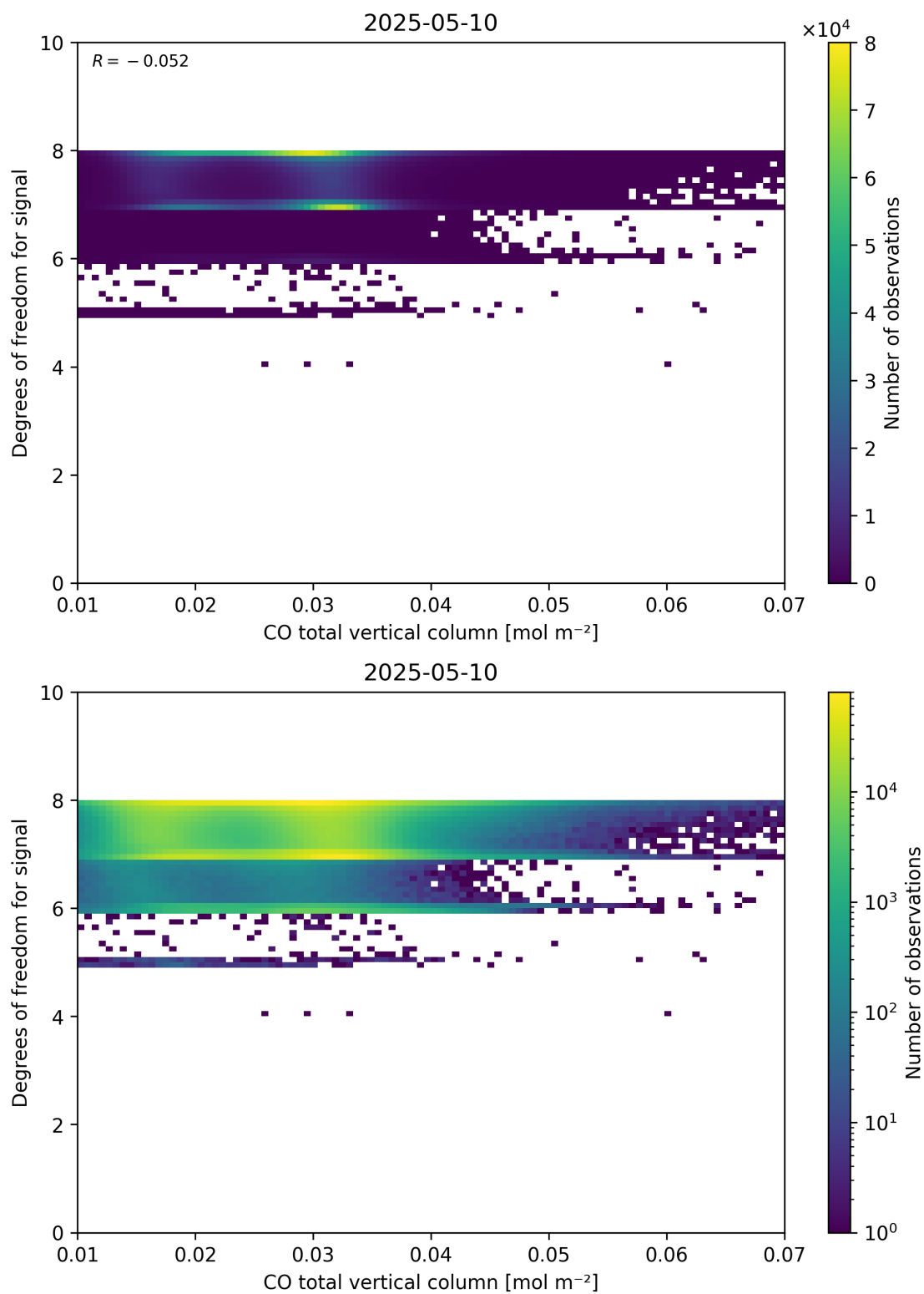
Figure 41: Scatter density plot of “CO total vertical column” against “Degrees of freedom for signal” for 2025-05-10 to 2025-05-11.
