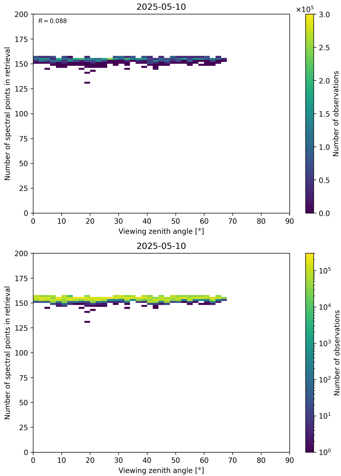
Figure 76: Scatter density plot of “Viewing zenith angle” against “Number of spectral points in retrieval” for 2025-05-10 to 2025-05-11.
