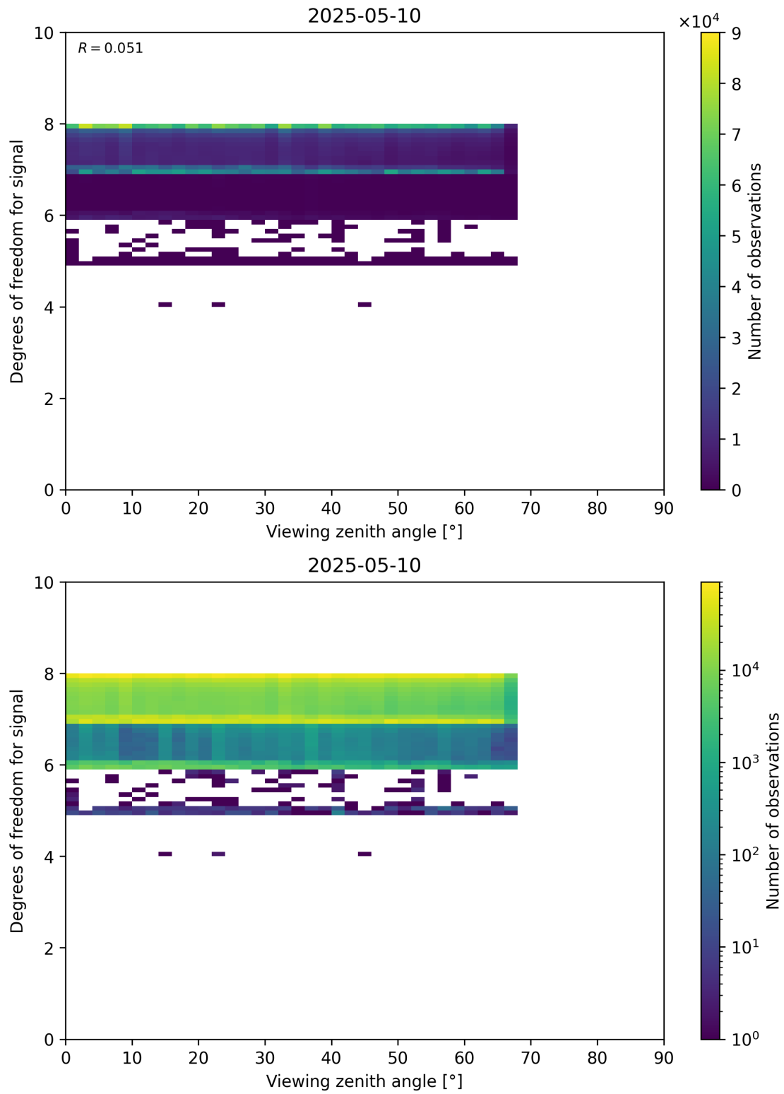
Figure 73: Scatter density plot of “Viewing zenith angle” against “Degrees of freedom for signal” for 2025-05-10 to 2025-05-11.
