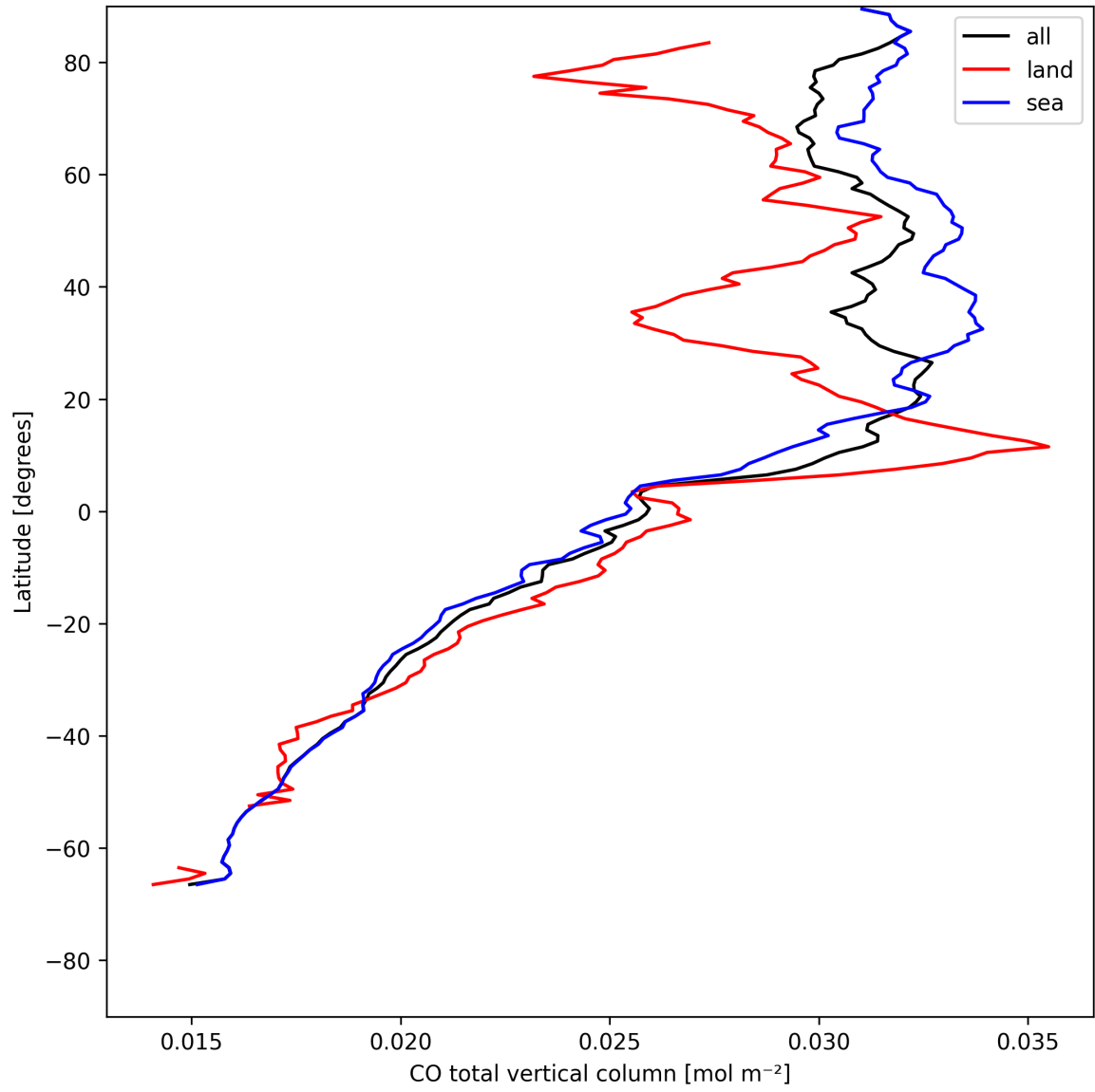
Figure 10: Zonal average of “CO total vertical column” for 2025-05-10 to 2025-05-11.
