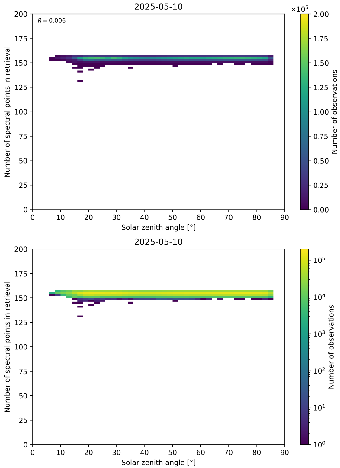
Figure 68: Scatter density plot of “Solar zenith angle” against “Number of spectral points in retrieval” for 2025-05-10 to 2025-05-11.
