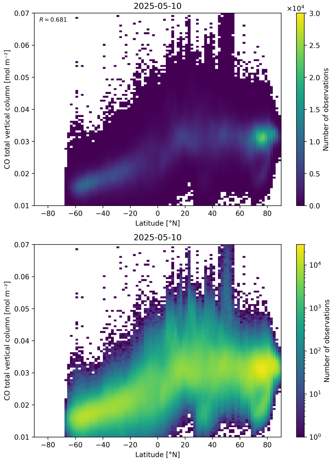
Figure 51: Scatter density plot of “Latitude” against “CO total vertical column” for 2025-05-10 to 2025-05-11.
