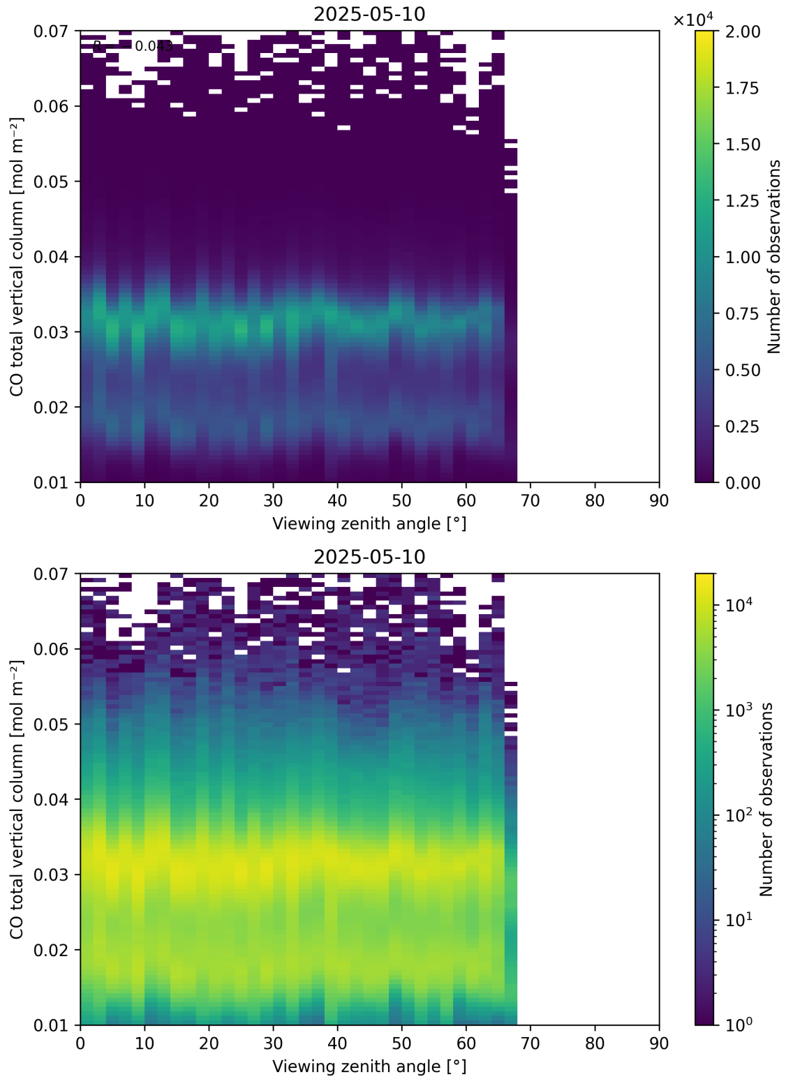
Figure 69: Scatter density plot of “Viewing zenith angle” against “CO total vertical column” for 2025-05-10 to 2025-05-11.
