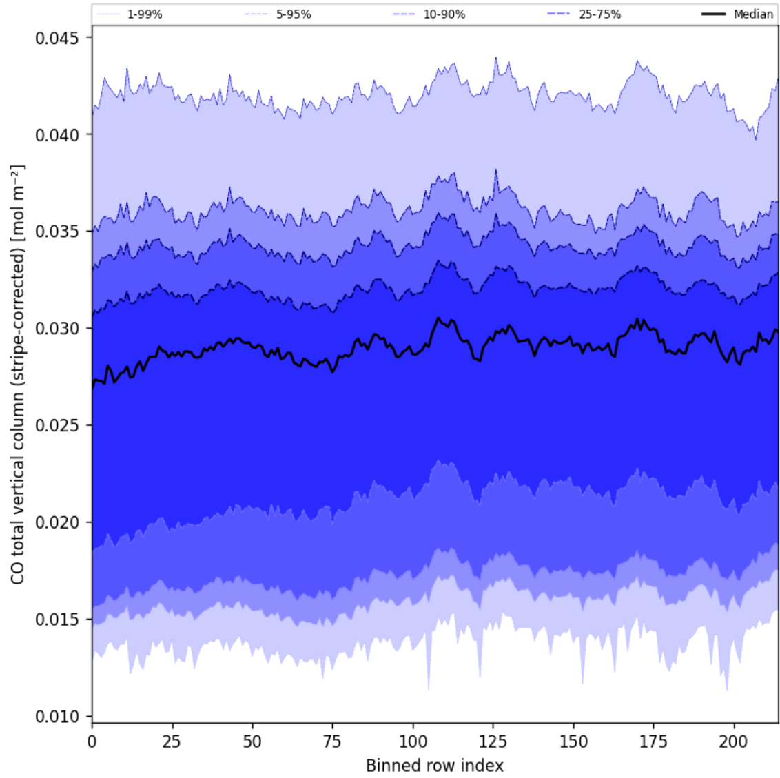
Figure 27: Along track statistics of “CO total vertical column (stripe-corrected)” for 2025-05-10 to 2025-05-11
