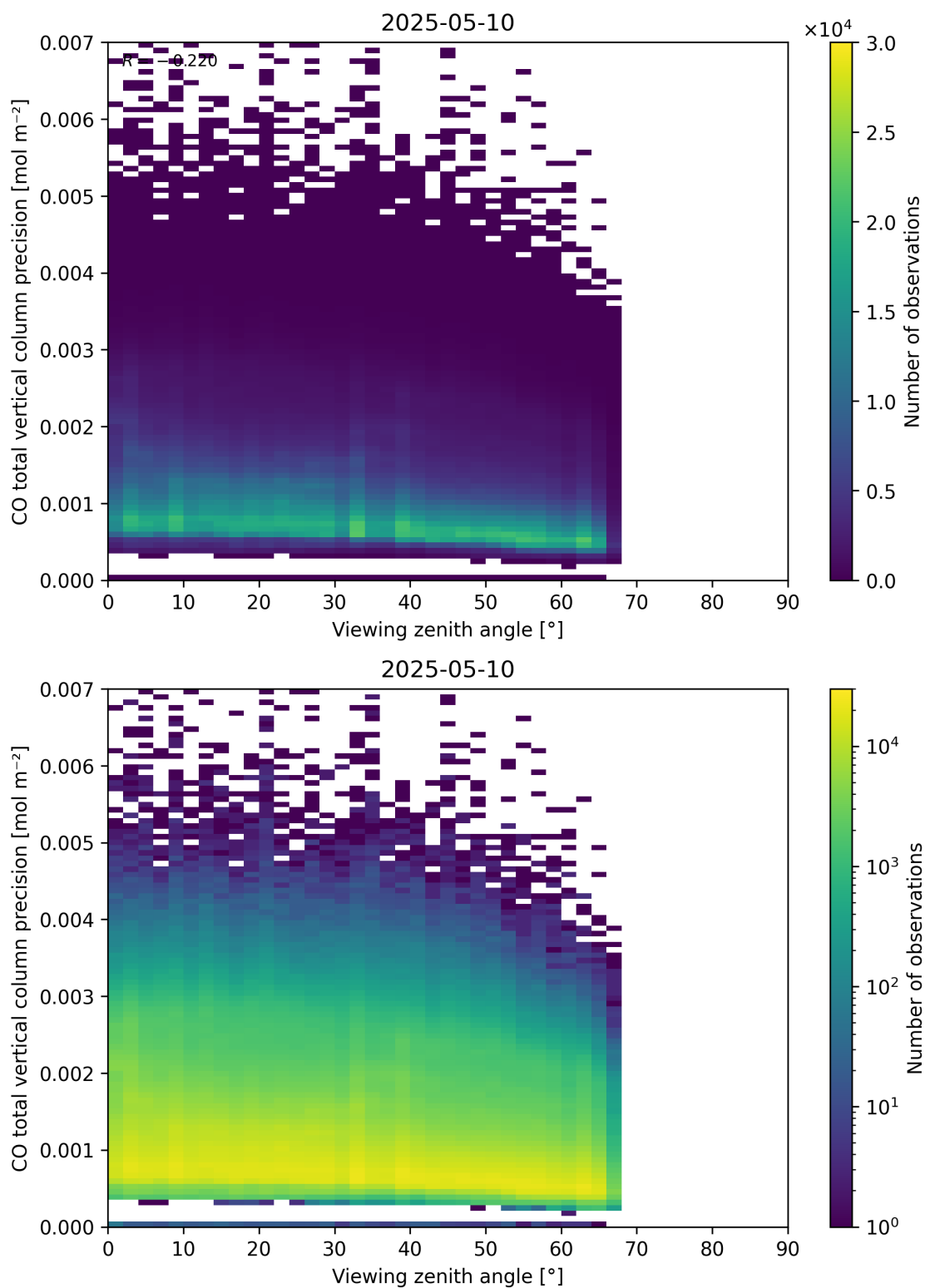
Figure 71: Scatter density plot of “Viewing zenith angle” against “CO total vertical column precision” for 2025-05-10 to 2025-05-11.
