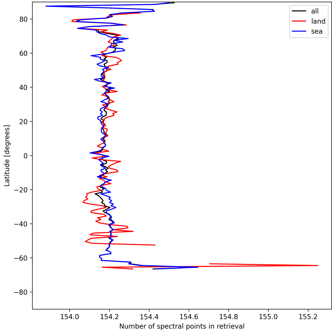
Figure 13: Zonal average of “Number of spectral points in retrieval” for 2025-05-10 to 2025-05-11.
