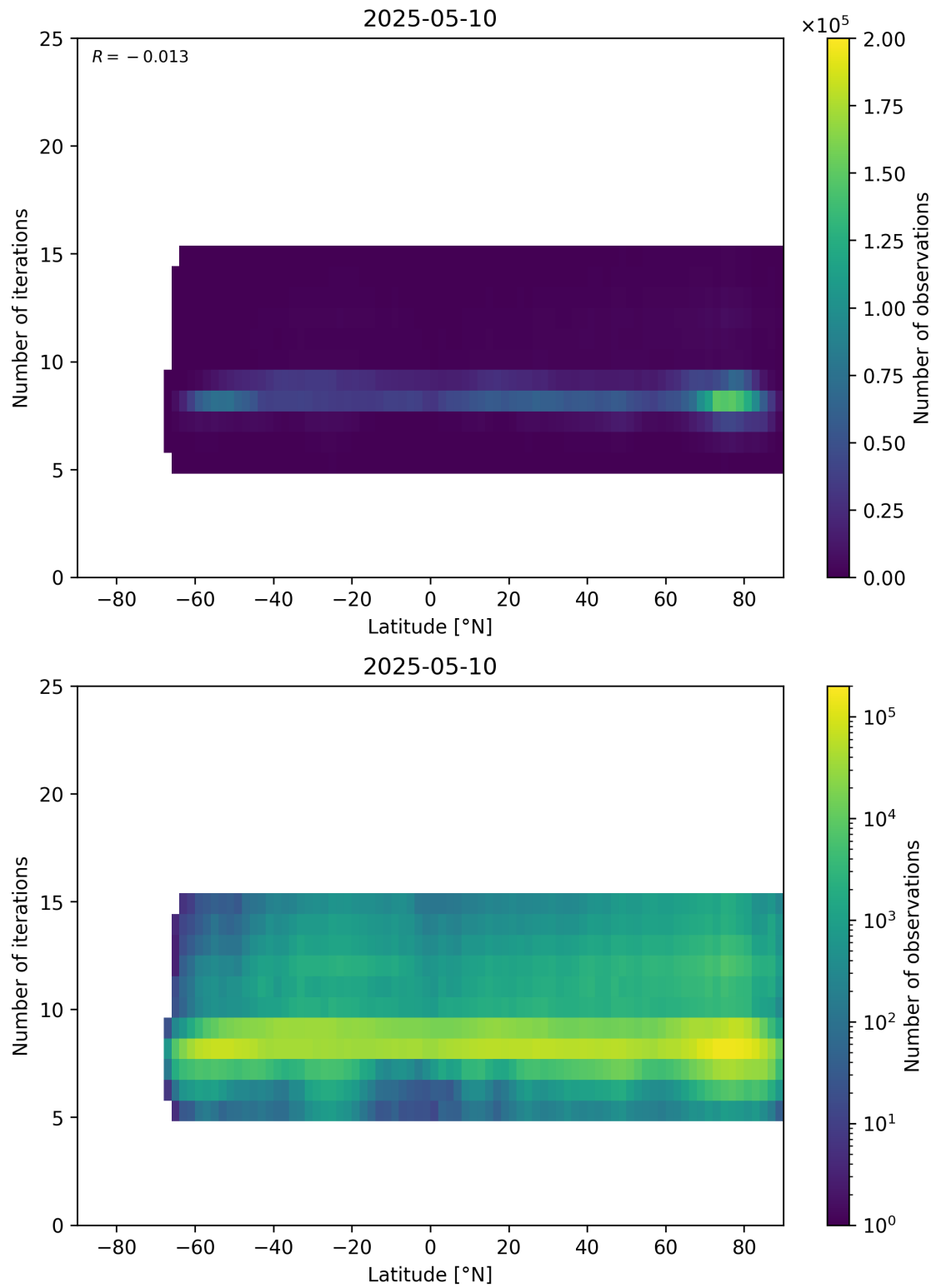
Figure 56: Scatter density plot of “Latitude” against “Number of iterations” for 2025-05-10 to 2025-05-11.
