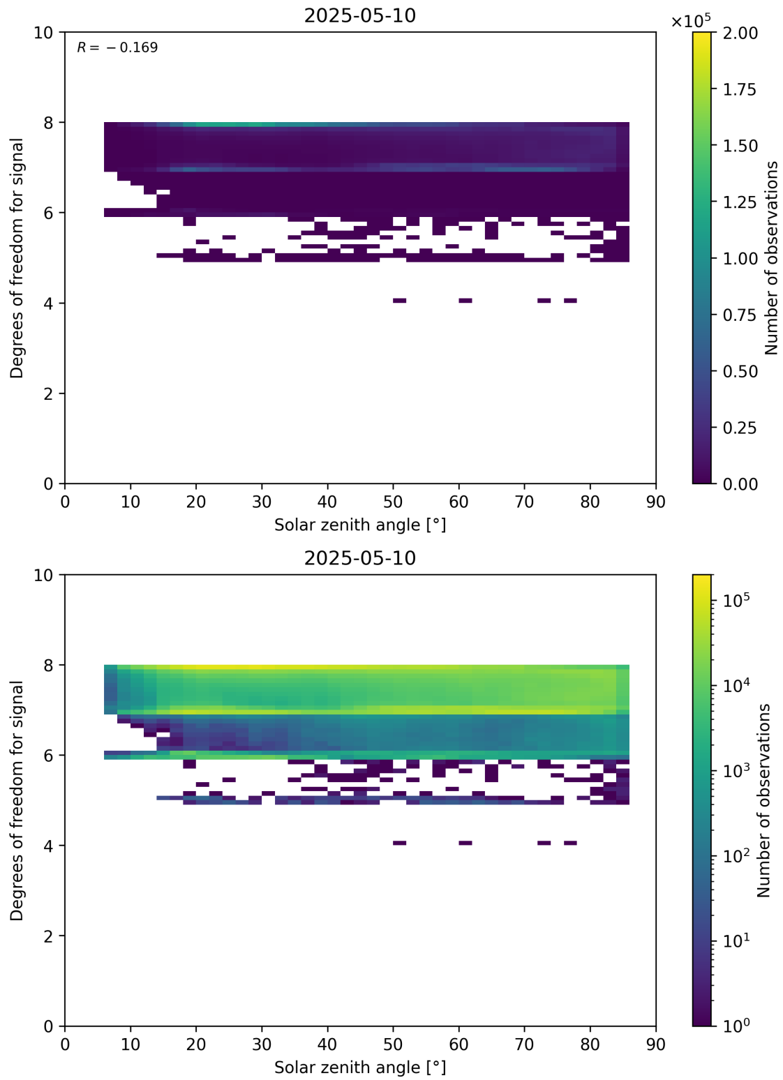
Figure 65: Scatter density plot of “Solar zenith angle” against “Degrees of freedom for signal” for 2025-05-10 to 2025-05-11.
