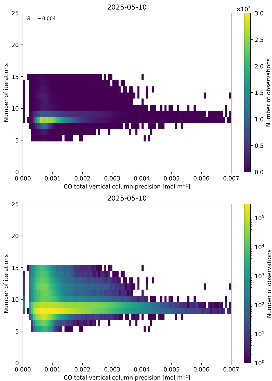
Figure 46: Scatter density plot of “CO total vertical column precision” against “Number of iterations” for 2025-05-10 to 2025-05-11.
