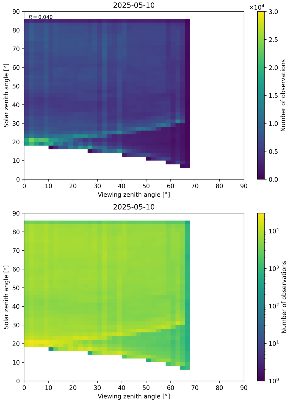
Figure 77: Scatter density plot of “Viewing zenith angle” against “Solar zenith angle” for 2025-05-10 to 2025-05-11.
