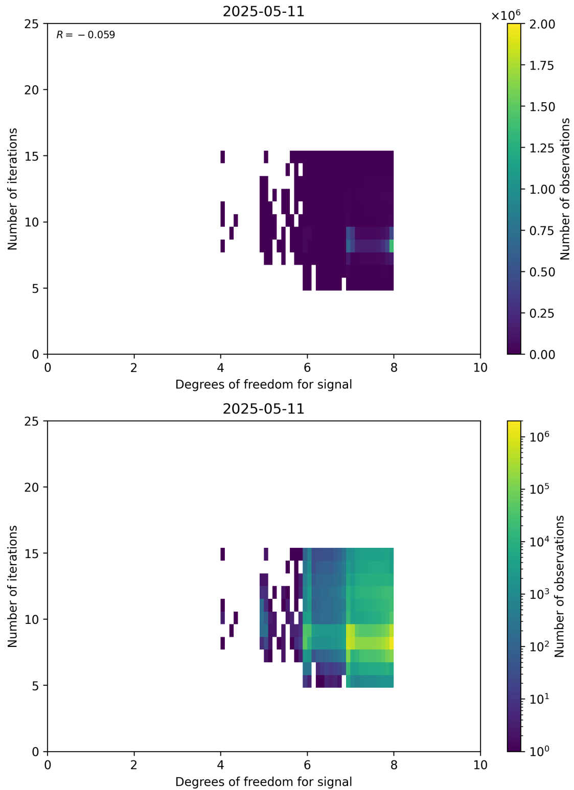
Figure 50: Scatter density plot of “Degrees of freedom for signal” against “Number of iterations” for 2025-05-10 to 2025-05-12.
