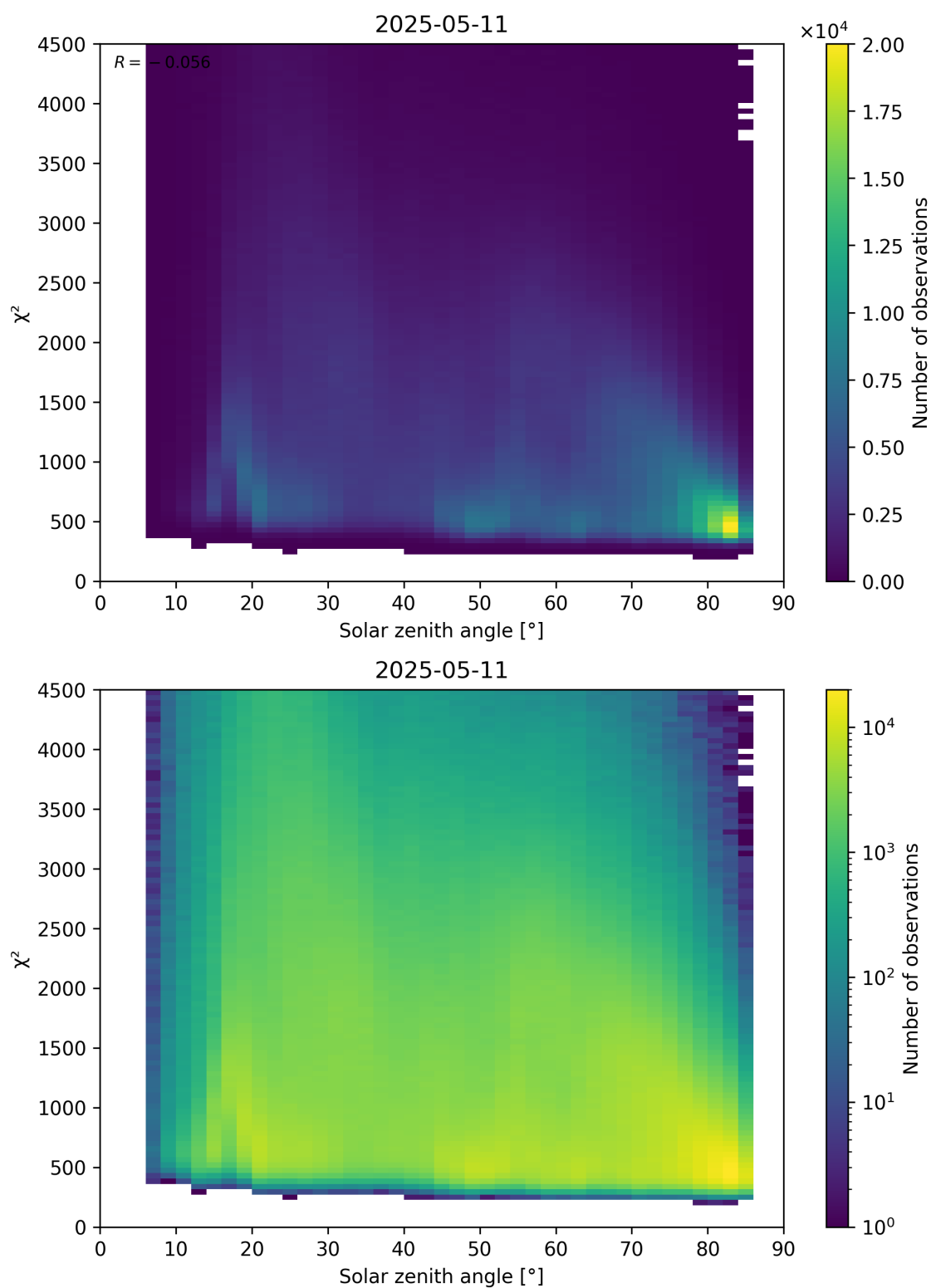
Figure 64: Scatter density plot of “Solar zenith angle” against “ \chi^2 ” for 2025-05-10 to 2025-05-12.
