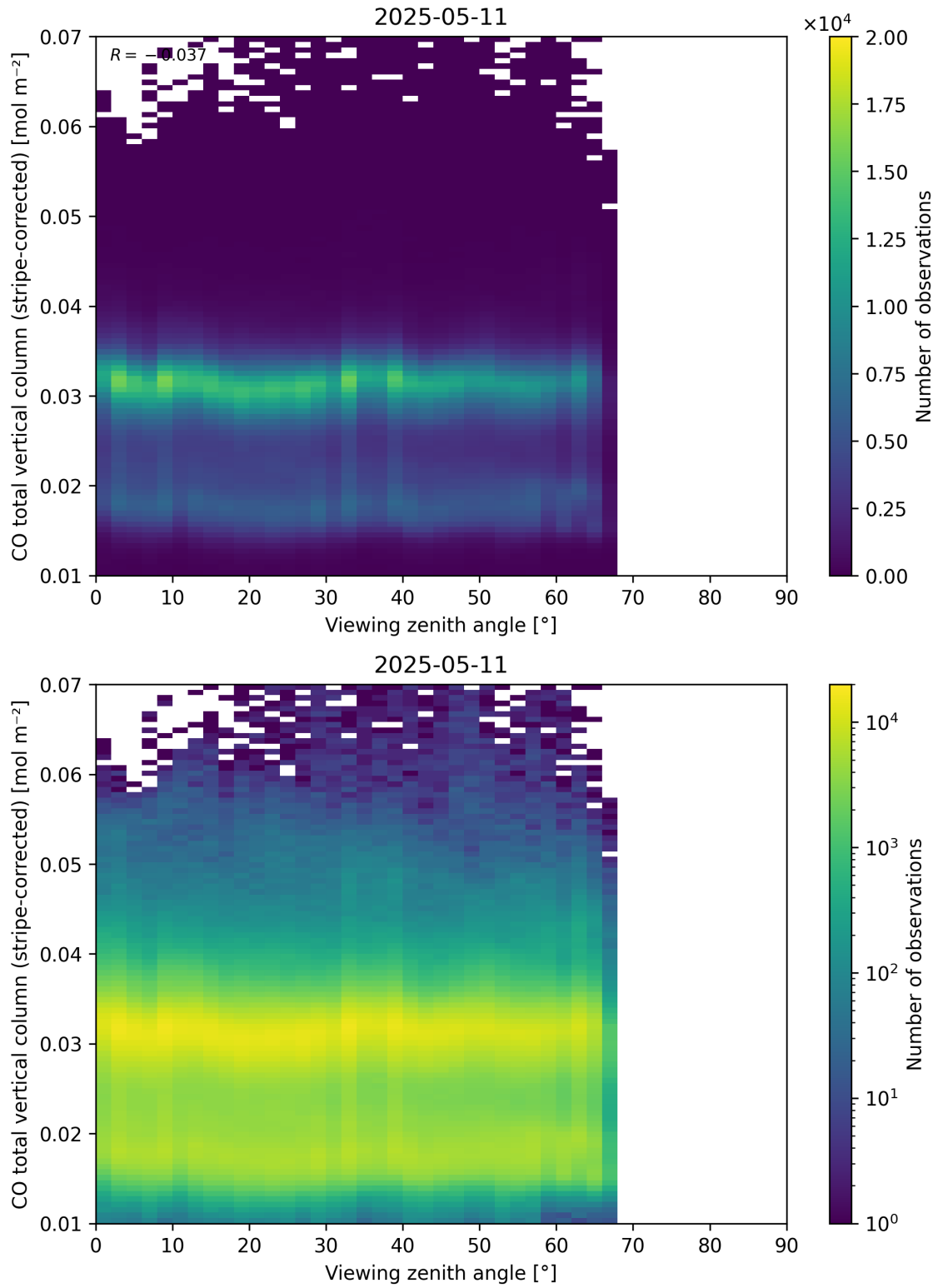
Figure 70: Scatter density plot of “Viewing zenith angle” against “CO total vertical column (stripe-corrected)” for 2025-05-10 to 2025-05-12.
