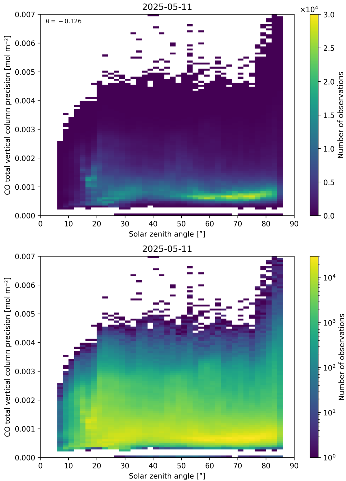
Figure 63: Scatter density plot of “Solar zenith angle” against “CO total vertical column precision” for 2025-05-10 to 2025-05-12.
