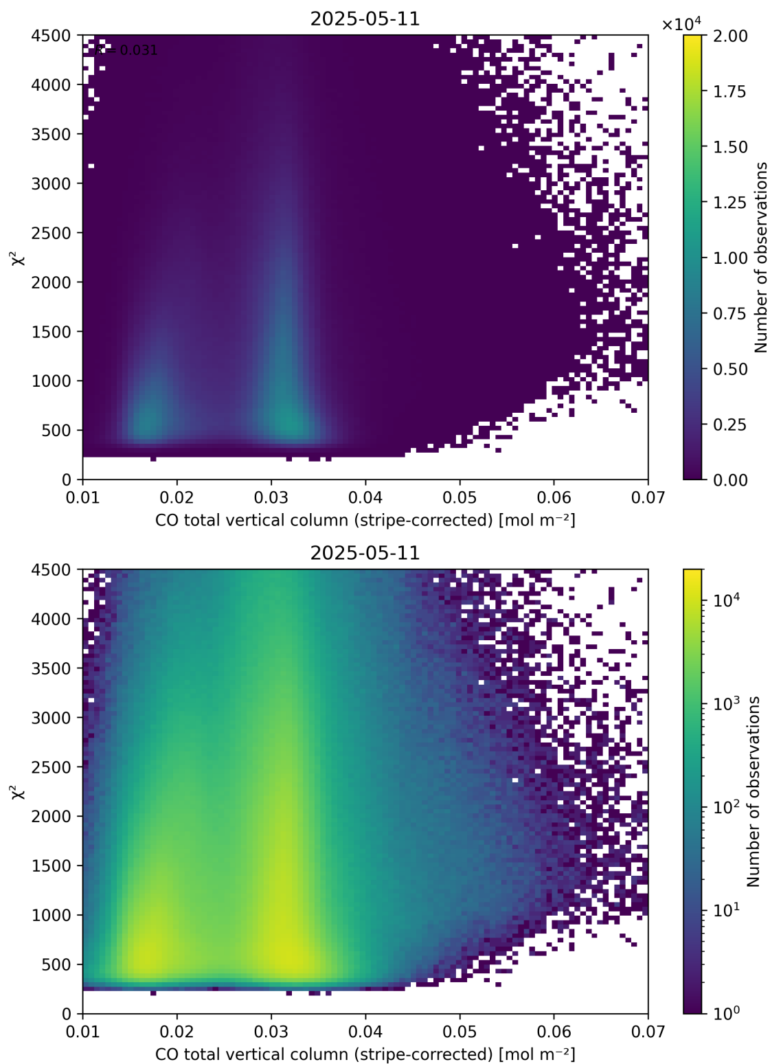
Figure 37: Scatter density plot of “CO total vertical column (stripe-corrected)” against “ \chi^2 ” for 2025-05-10 to 2025-05-12.
