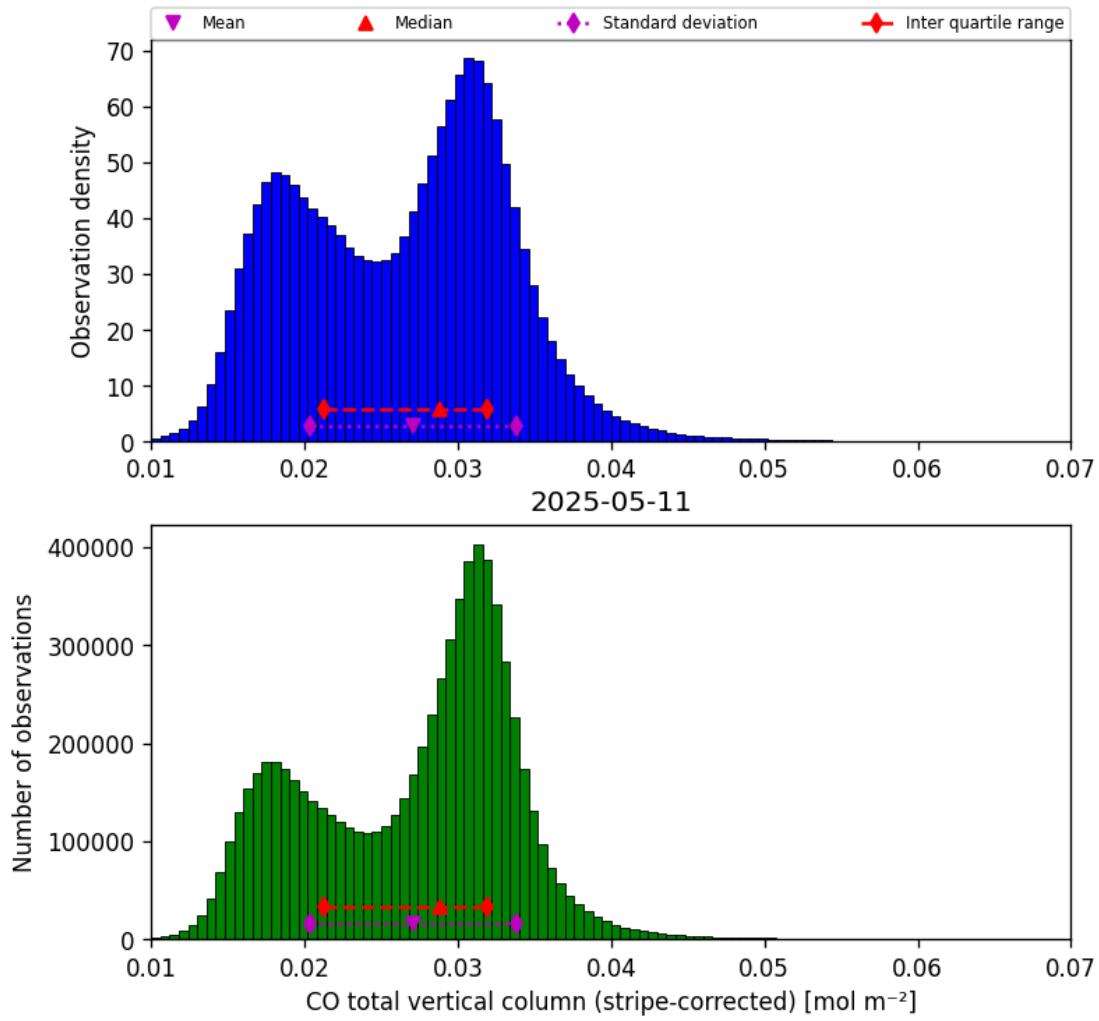
Figure 19: Histogram of “CO total vertical column (stripe-corrected)” for 2025-05-10 to 2025-05-12
