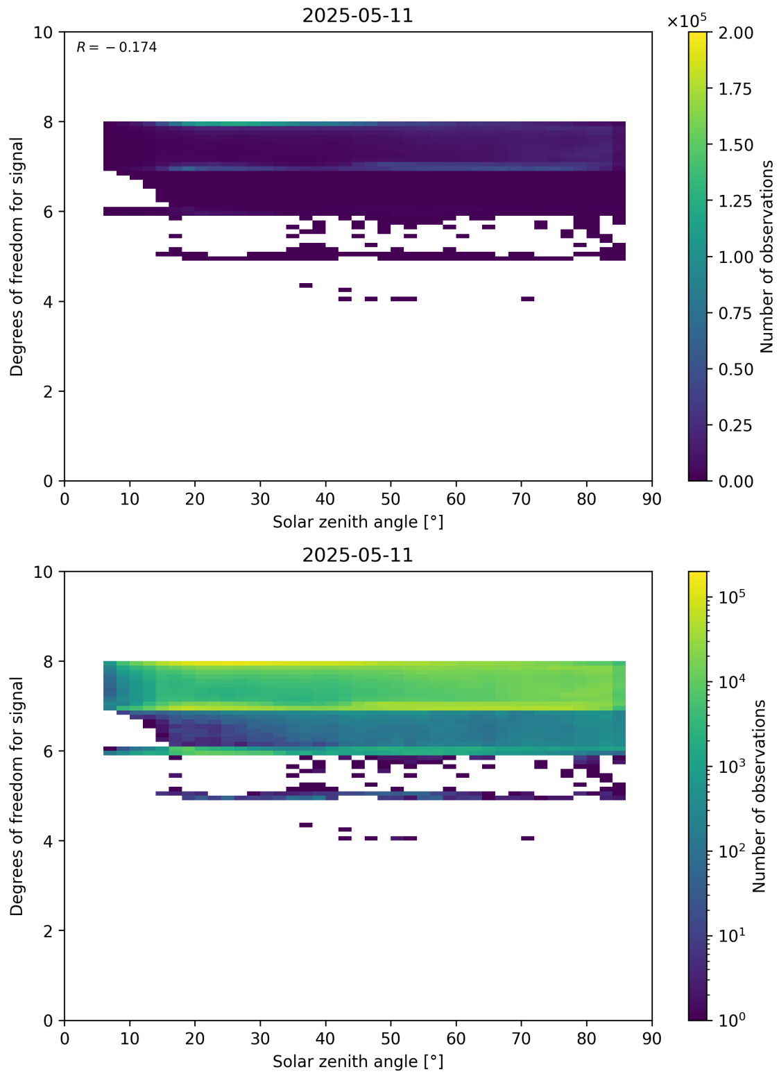
Figure 65: Scatter density plot of “Solar zenith angle” against “Degrees of freedom for signal” for 2025-05-10 to 2025-05-12.
