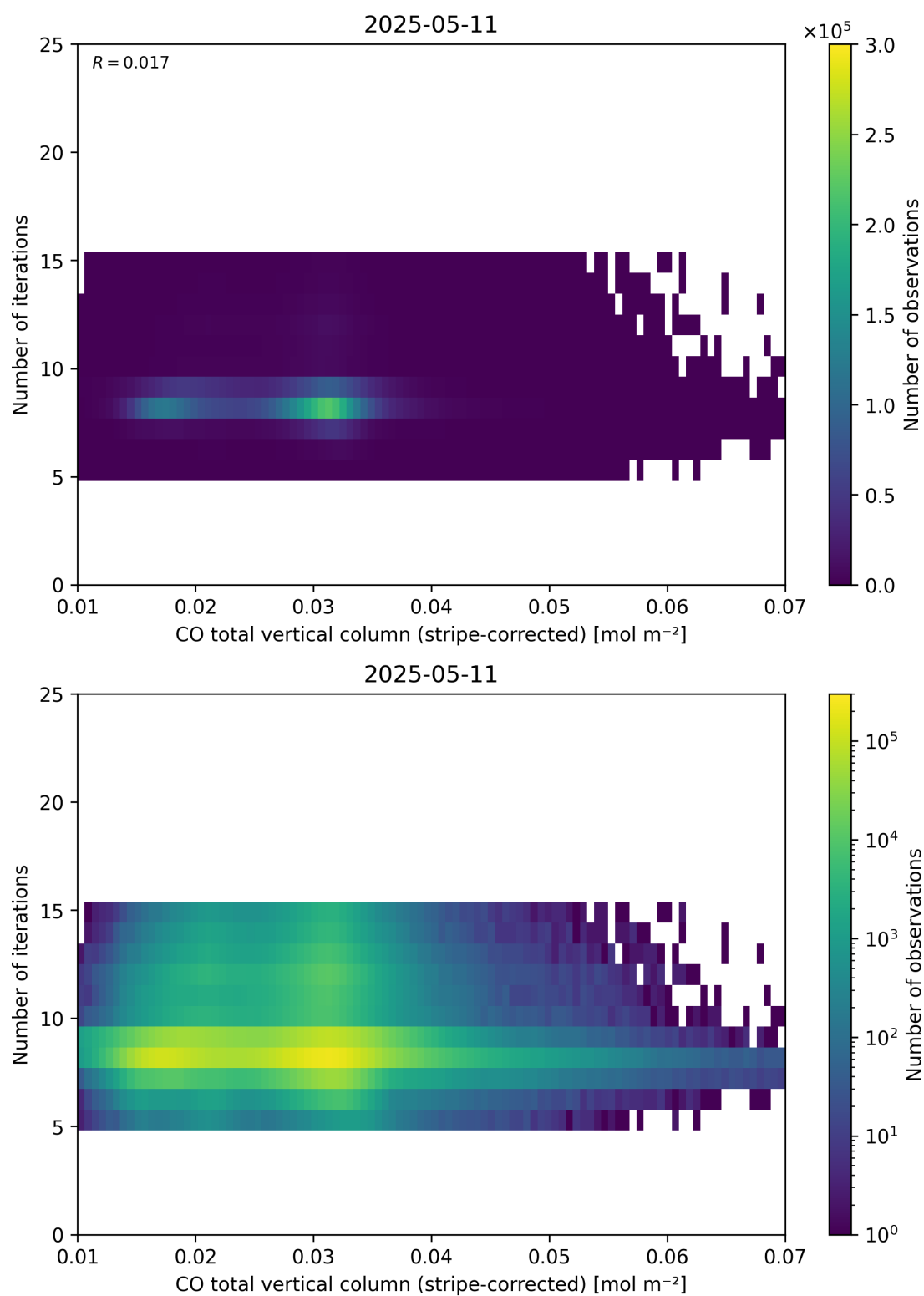
Figure 39: Scatter density plot of “CO total vertical column (stripe-corrected)” against “Number of iterations” for 2025-05-10 to 2025-05-12.
