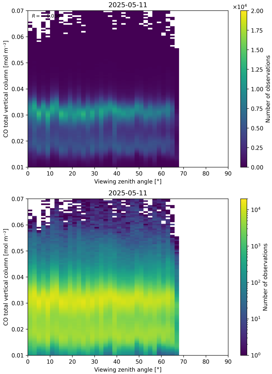
Figure 69: Scatter density plot of “Viewing zenith angle” against “CO total vertical column” for 2025-05-10 to 2025-05-12.
