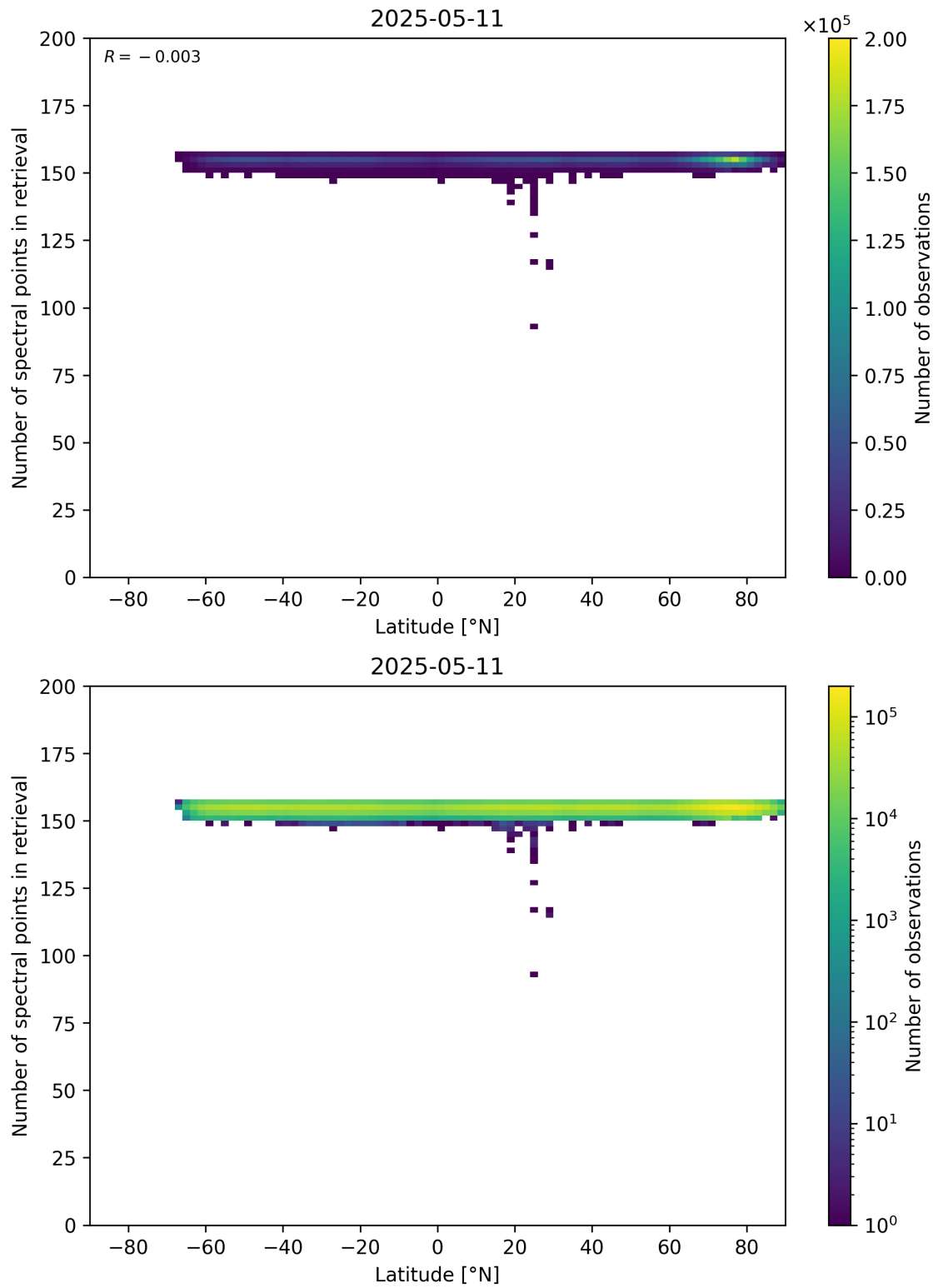
Figure 57: Scatter density plot of “Latitude” against “Number of spectral points in retrieval” for 2025-05-10 to 2025-05-12.
