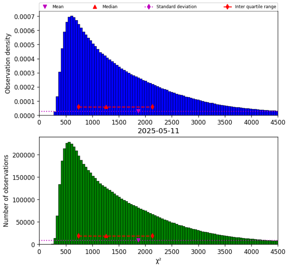
Figure 22: Histogram of “ \chi^2 ” for 2025-05-10 to 2025-05-12
