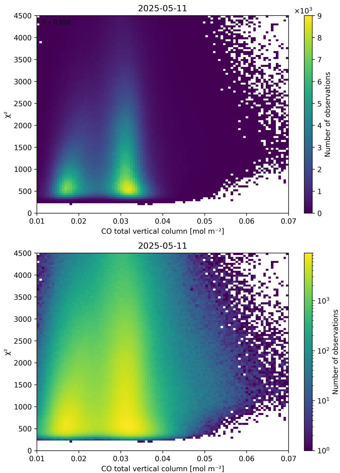
Figure 35: Scatter density plot of “CO total vertical column” against “ \chi^2 ” for 2025-05-10 to 2025-05-12.
