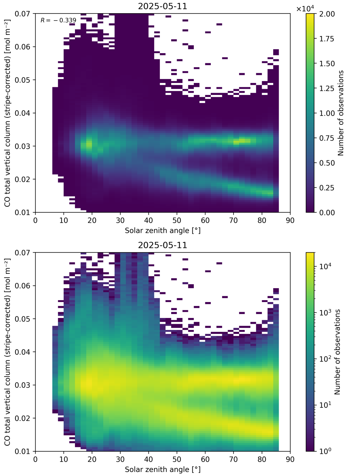
Figure 62: Scatter density plot of “Solar zenith angle” against “CO total vertical column (stripe-corrected)” for 2025-05-10 to 2025-05-12.
