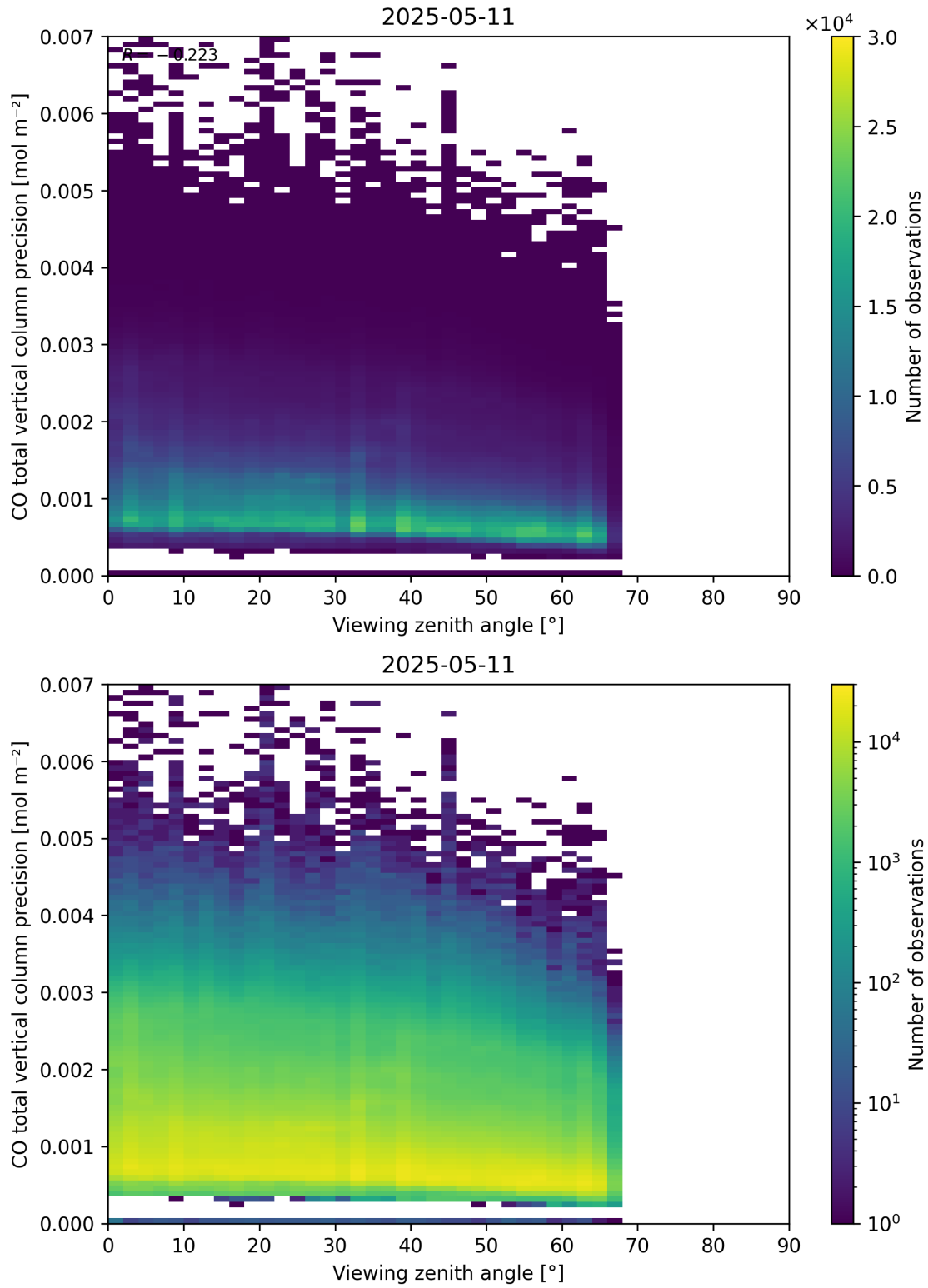
Figure 71: Scatter density plot of “Viewing zenith angle” against “CO total vertical column precision” for 2025-05-10 to 2025-05-12.
