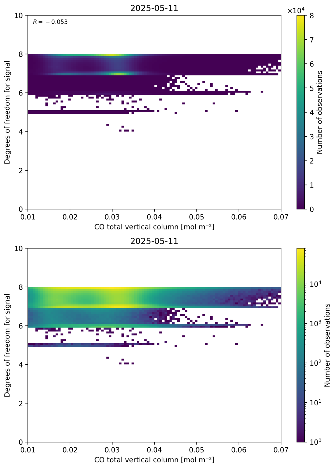
Figure 41: Scatter density plot of “CO total vertical column” against “Degrees of freedom for signal” for 2025-05-10 to 2025-05-12.
