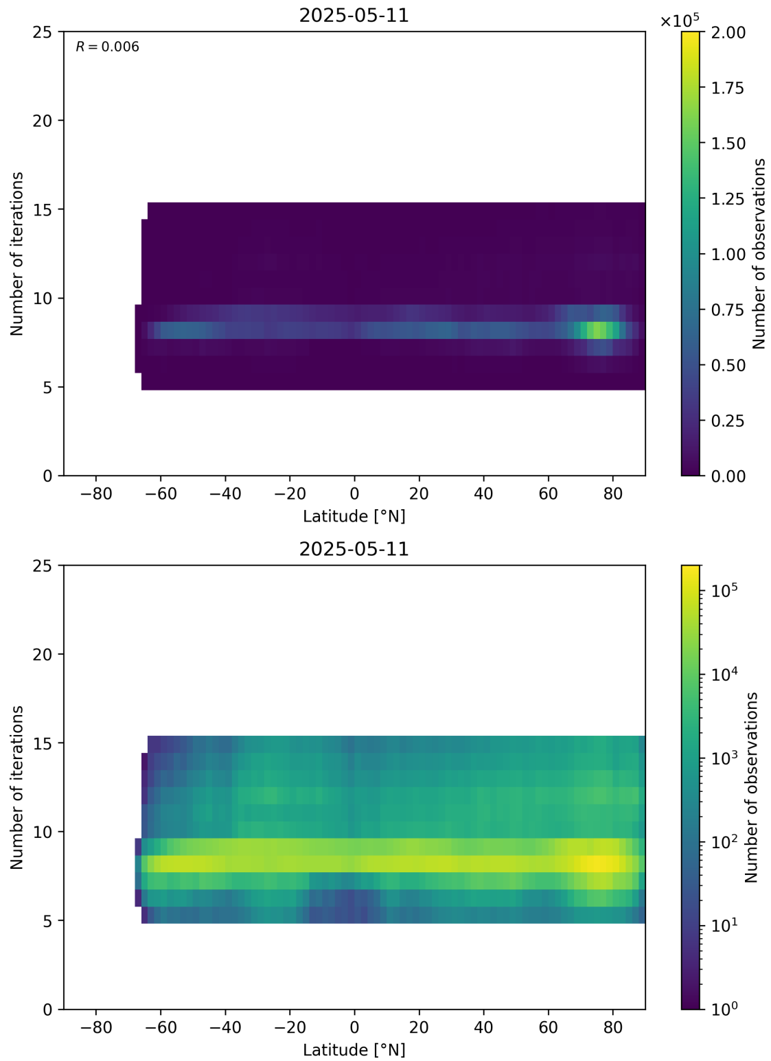
Figure 56: Scatter density plot of “Latitude” against “Number of iterations” for 2025-05-10 to 2025-05-12.
