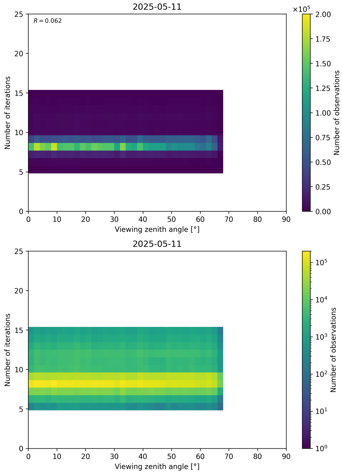
Figure 75: Scatter density plot of “Viewing zenith angle” against “Number of iterations” for 2025-05-10 to 2025-05-12.
