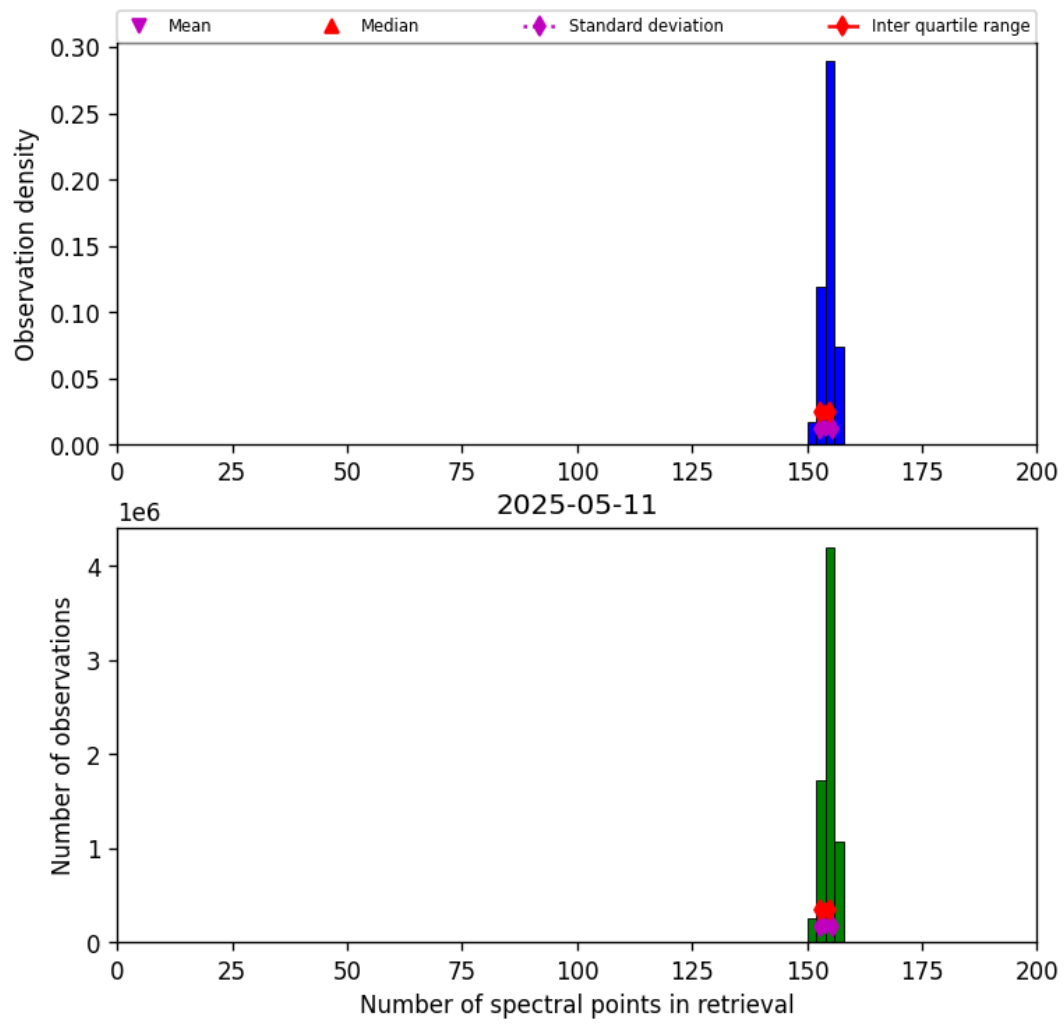
Figure 21: Histogram of “Number of spectral points in retrieval” for 2025-05-10 to 2025-05-12
