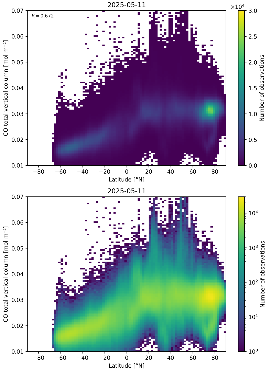
Figure 51: Scatter density plot of “Latitude” against “CO total vertical column” for 2025-05-10 to 2025-05-12.
