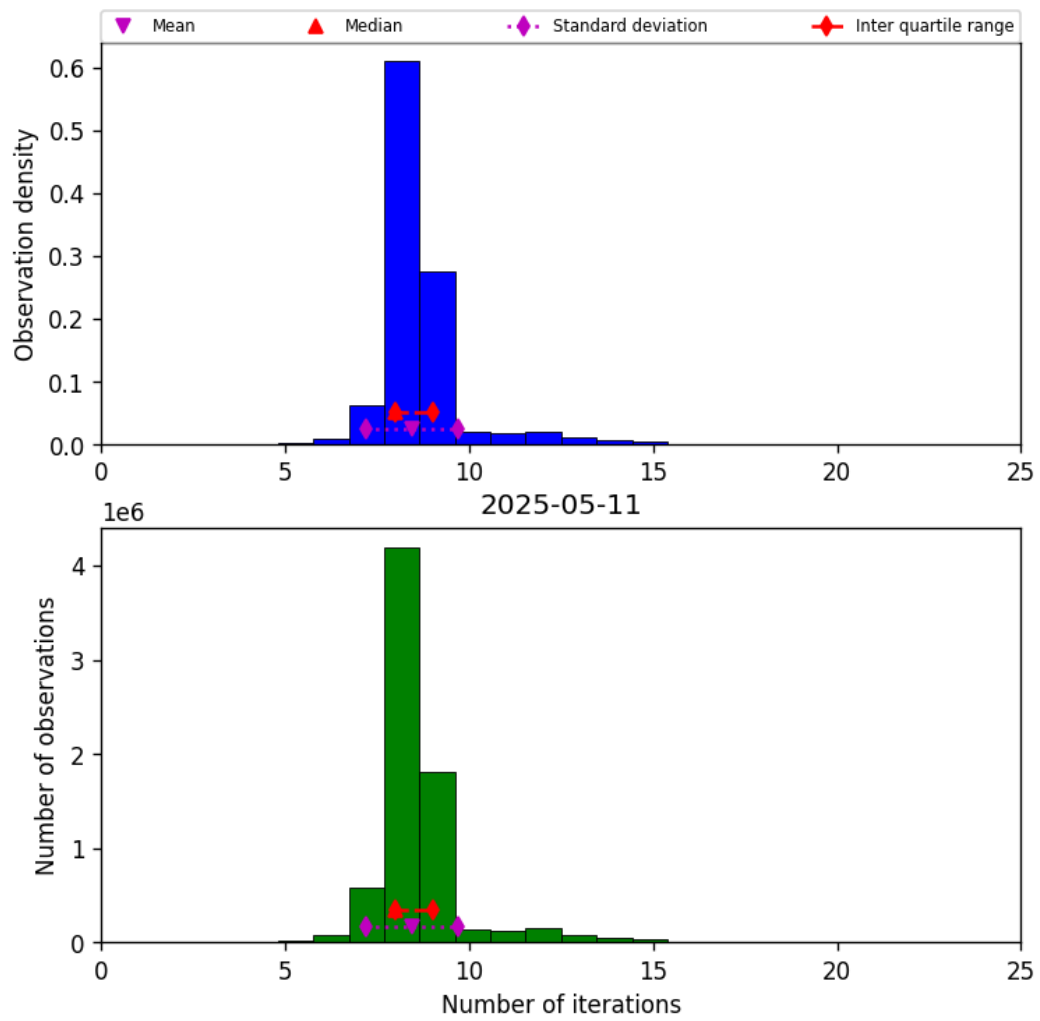
Figure 24: Histogram of “Number of iterations” for 2025-05-10 to 2025-05-12
