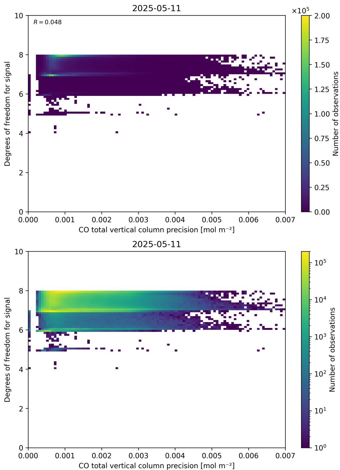
Figure 45: Scatter density plot of “CO total vertical column precision” against “Degrees of freedom for signal” for 2025-05-10 to 2025-05-12.
