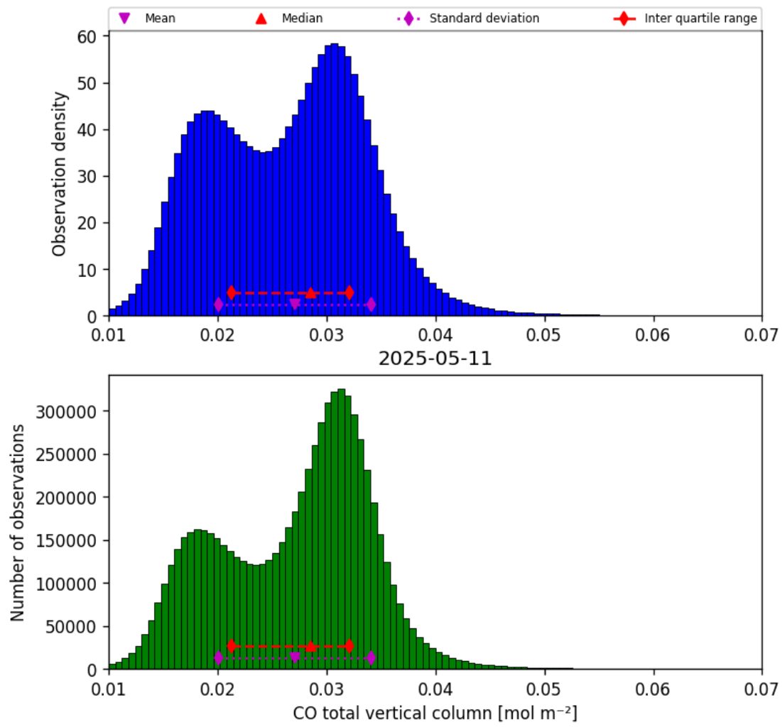
Figure 18: Histogram of “CO total vertical column” for 2025-05-10 to 2025-05-12
