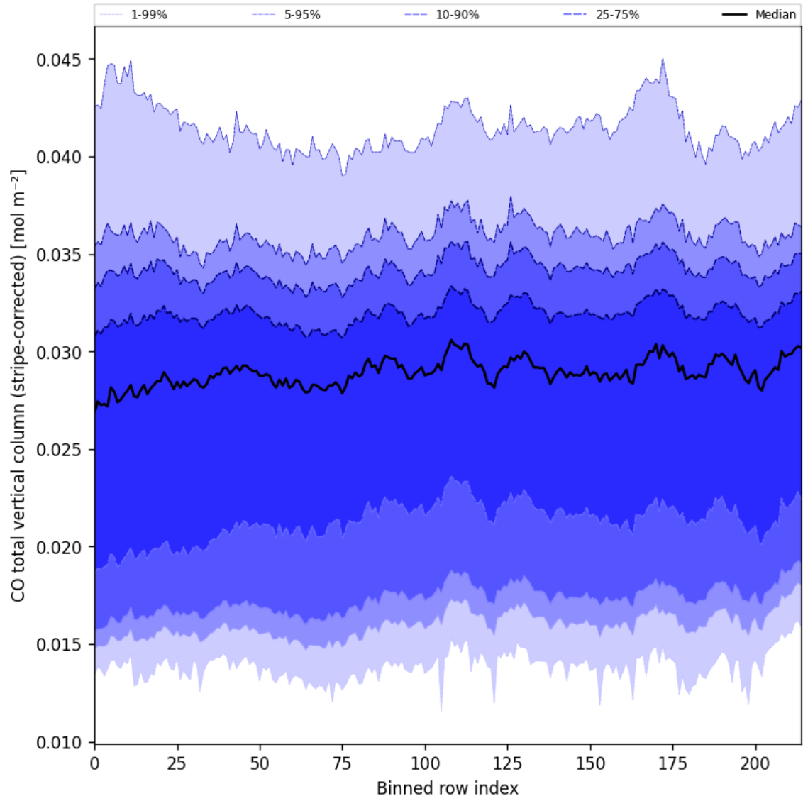
Figure 27: Along track statistics of “CO total vertical column (stripe-corrected)” for 2025-05-10 to 2025-05-12
