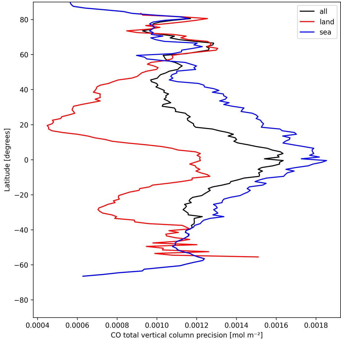
Figure 12: Zonal average of “CO total vertical column precision” for 2025-05-10 to 2025-05-12.
