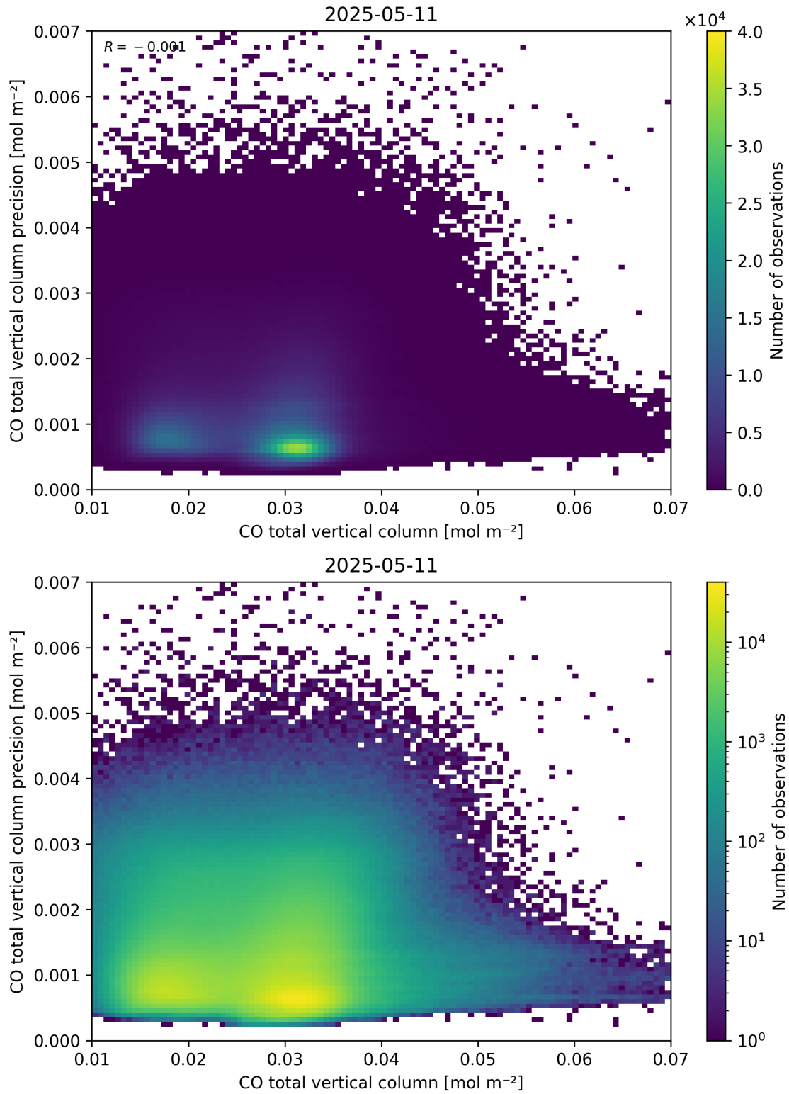
Figure 34: Scatter density plot of “CO total vertical column” against “CO total vertical column precision” for 2025-05-10 to 2025-05-12.
