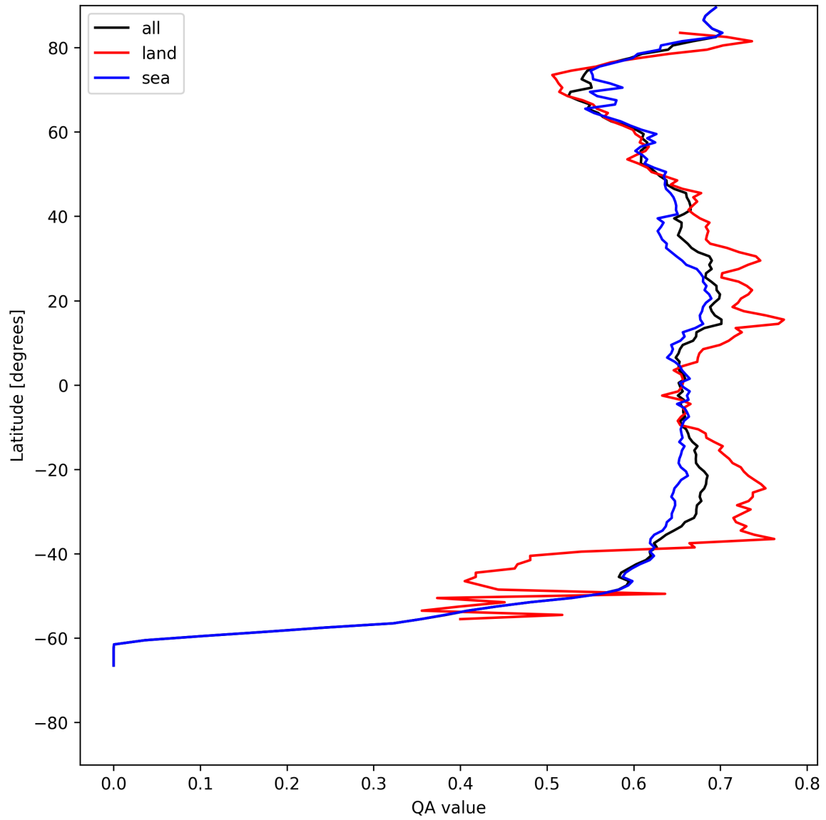
Figure 9: Zonal average of “QA value” for 2025-05-10 to 2025-05-12.
