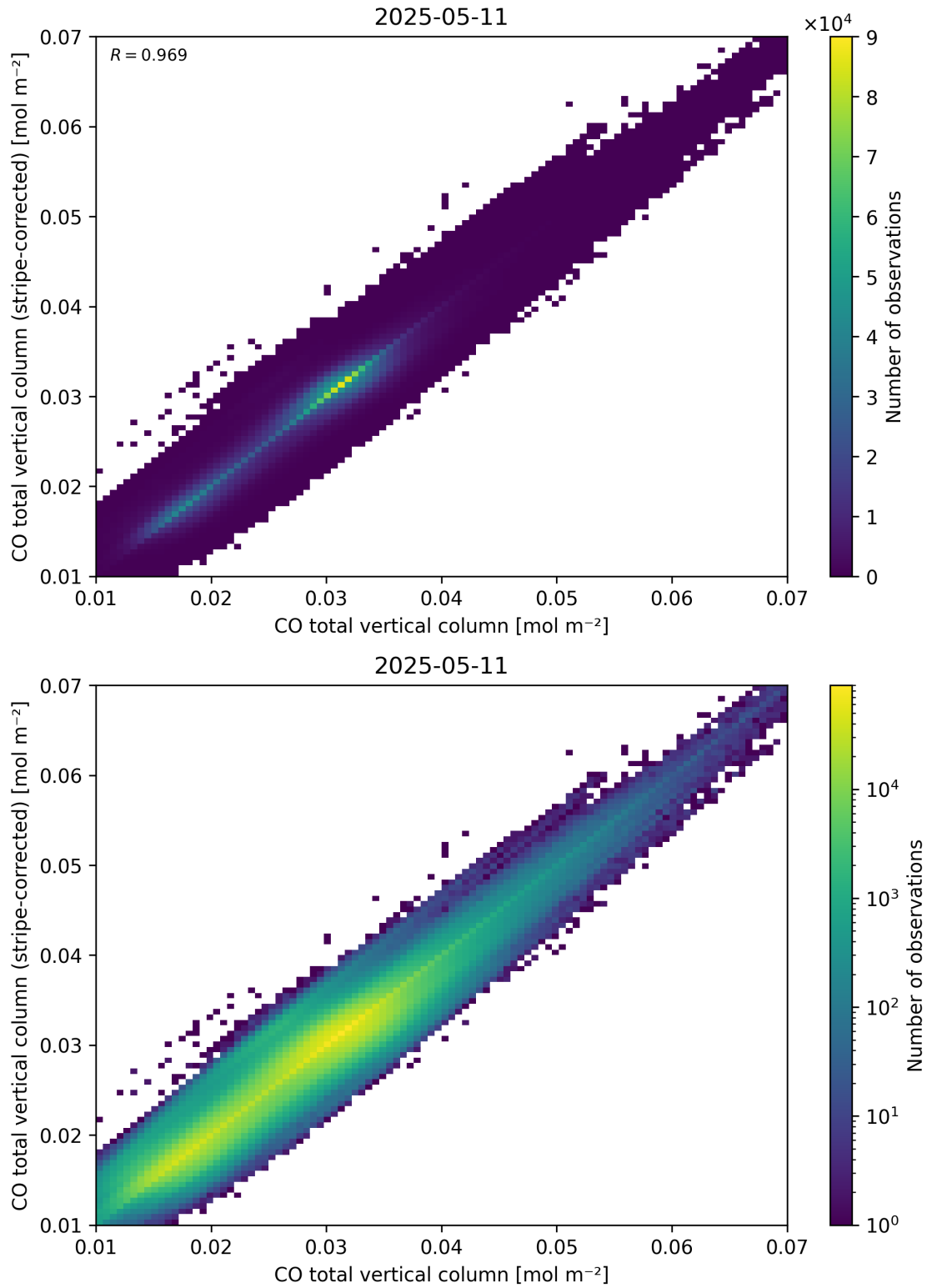
Figure 33: Scatter density plot of “CO total vertical column” against “CO total vertical column (stripe-corrected)” for 2025-05-10 to 2025-05-12.
