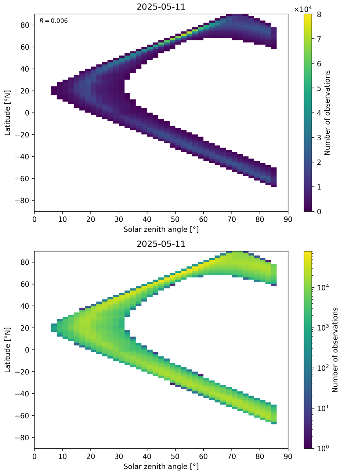
Figure 66: Scatter density plot of “Solar zenith angle” against “Latitude” for 2025-05-10 to 2025-05-12.
