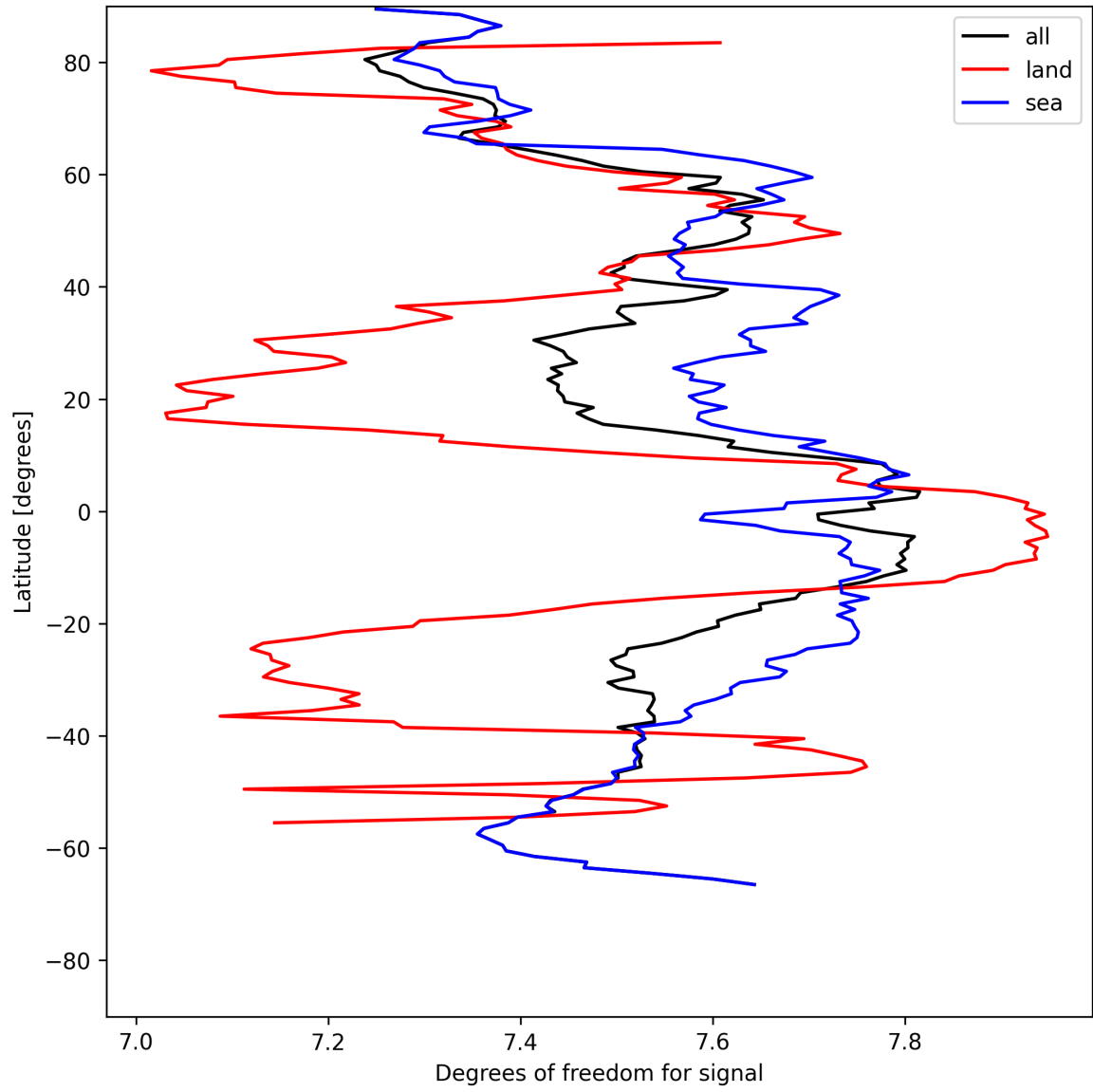
Figure 15: Zonal average of “Degrees of freedom for signal” for 2025-05-10 to 2025-05-12.
