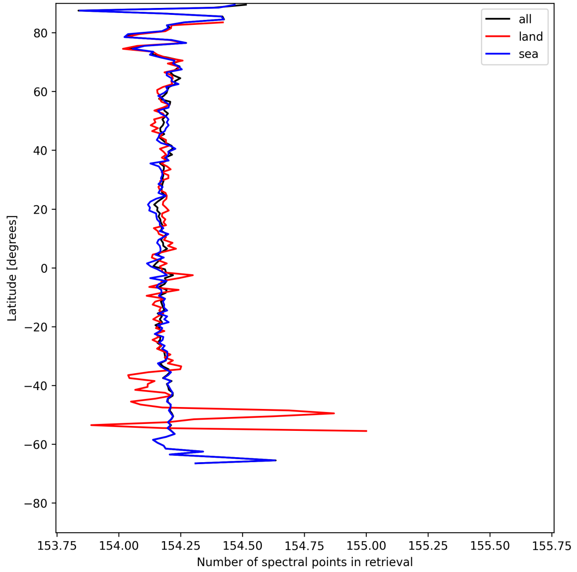
Figure 13: Zonal average of “Number of spectral points in retrieval” for 2025-05-10 to 2025-05-12.
