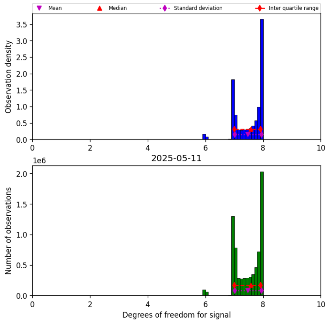
Figure 23: Histogram of “Degrees of freedom for signal” for 2025-05-10 to 2025-05-12
