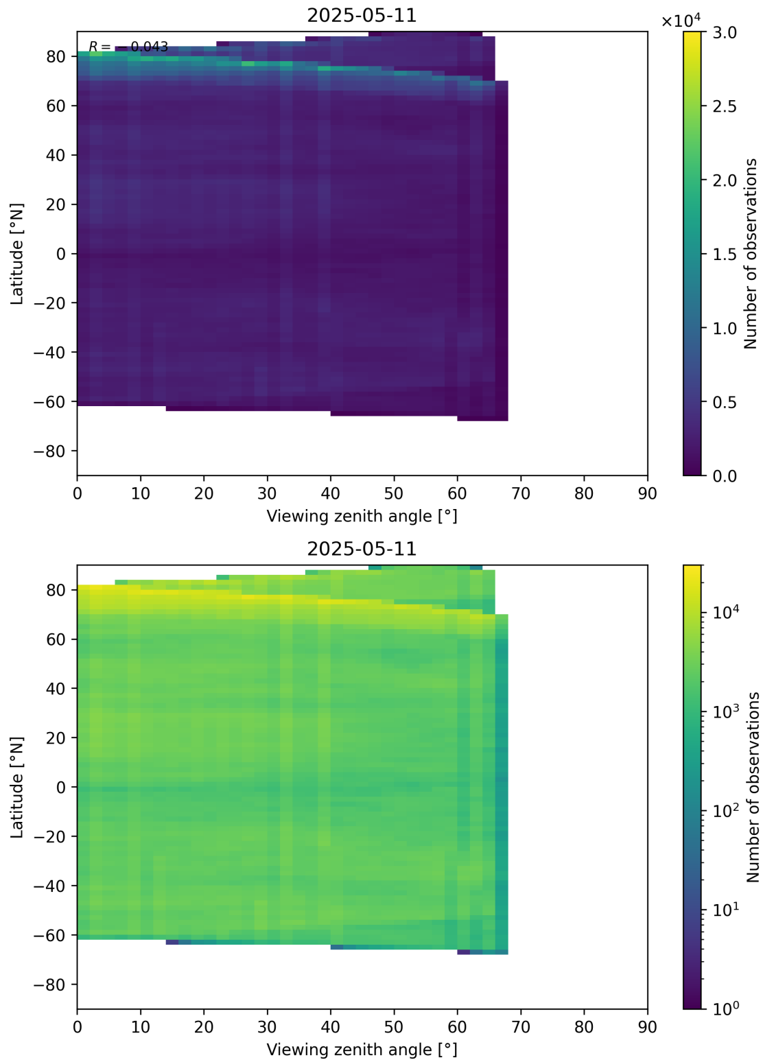
Figure 74: Scatter density plot of “Viewing zenith angle” against “Latitude” for 2025-05-10 to 2025-05-12.
