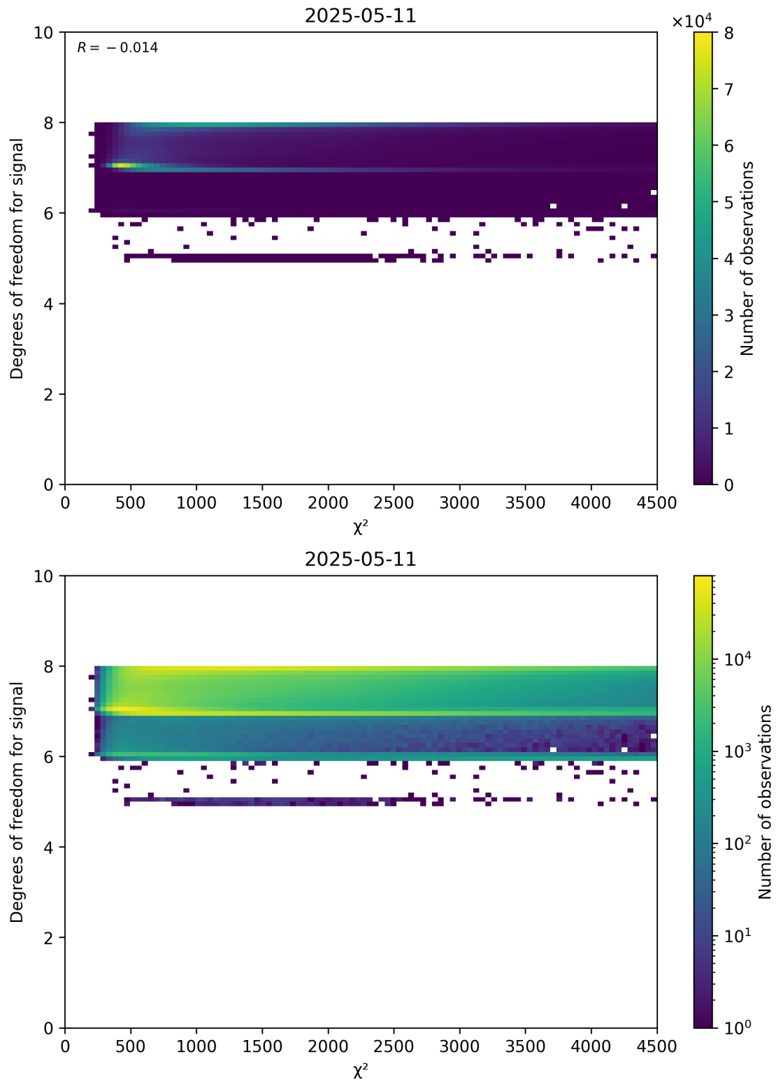
Figure 48: Scatter density plot of “ \chi^2 ” against “Degrees of freedom for signal” for 2025-05-10 to 2025-05-12.
