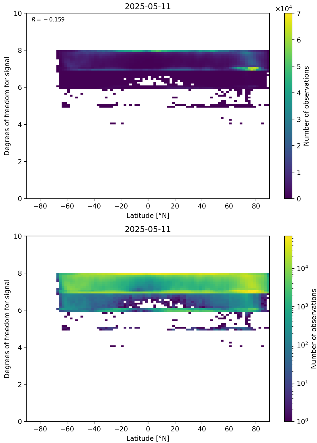
Figure 55: Scatter density plot of “Latitude” against “Degrees of freedom for signal” for 2025-05-10 to 2025-05-12.
