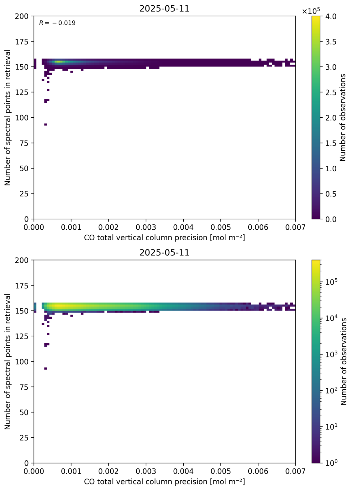
Figure 47: Scatter density plot of “CO total vertical column precision” against “Number of spectral points in retrieval” for 2025-05-10 to 2025-05-12.
