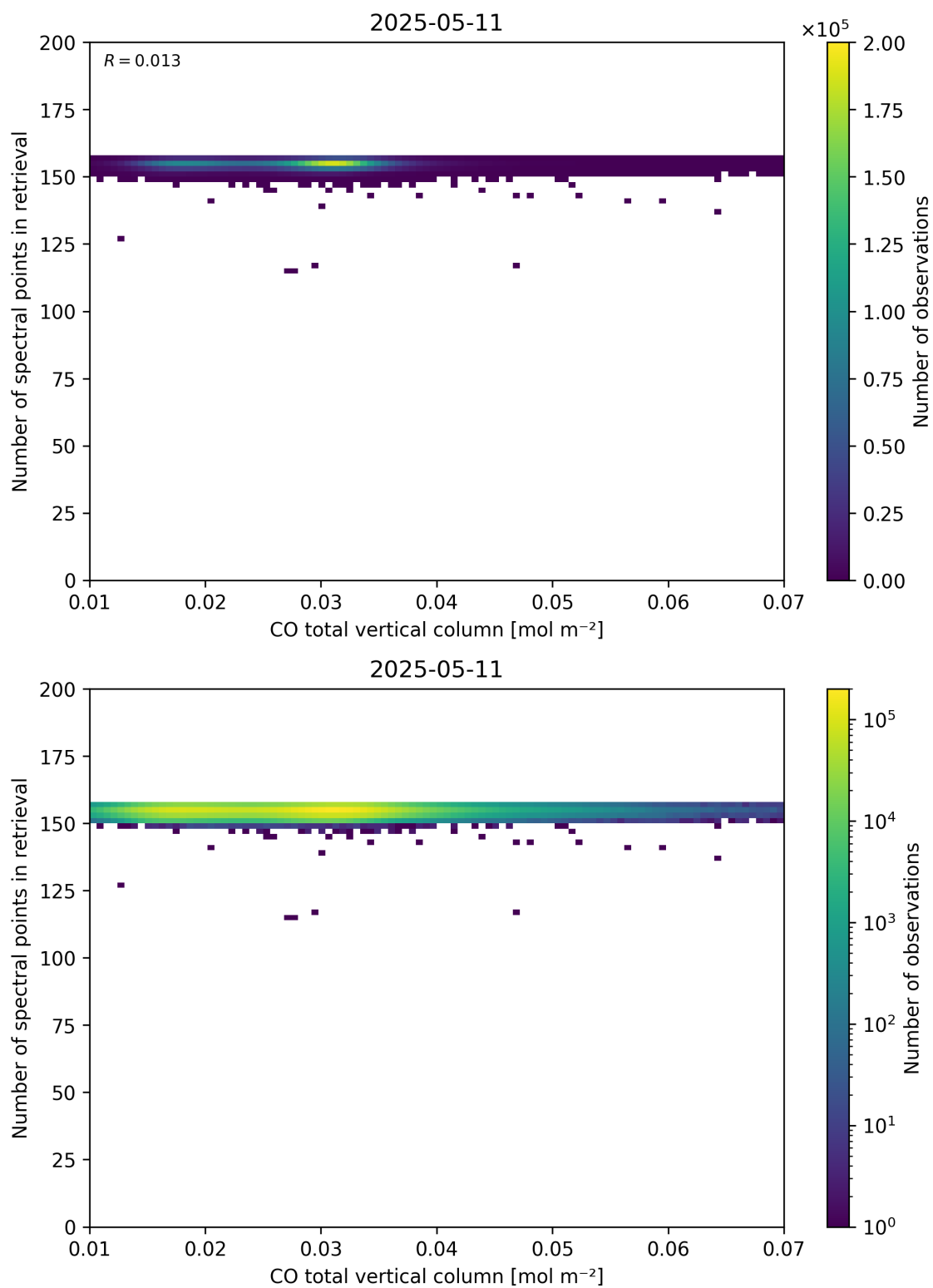
Figure 43: Scatter density plot of “CO total vertical column” against “Number of spectral points in retrieval” for 2025-05-10 to 2025-05-12.
