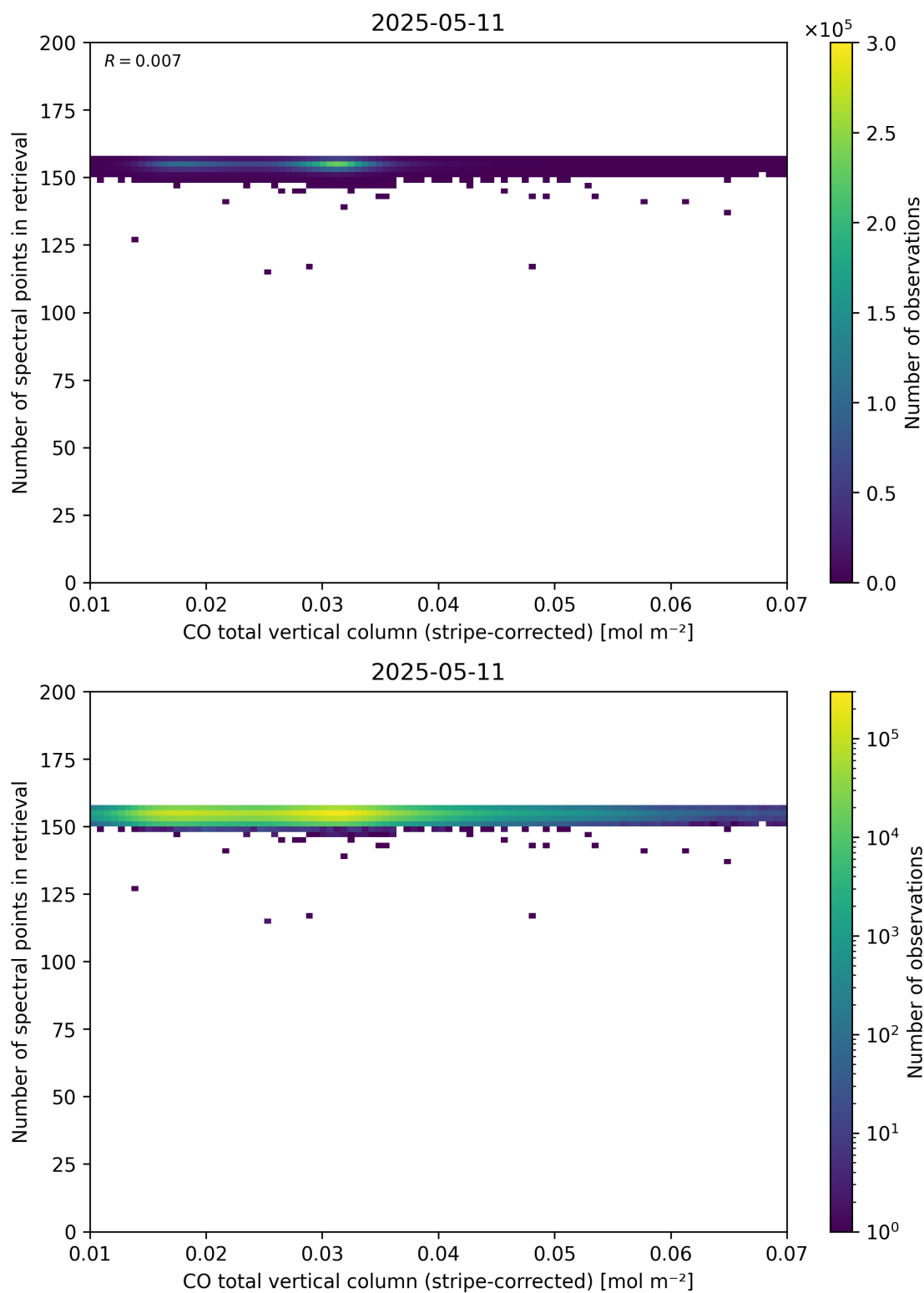
Figure 40: Scatter density plot of “CO total vertical column (stripe-corrected)” against “Number of spectral points in retrieval” for 2025-05-10 to 2025-05-12.
