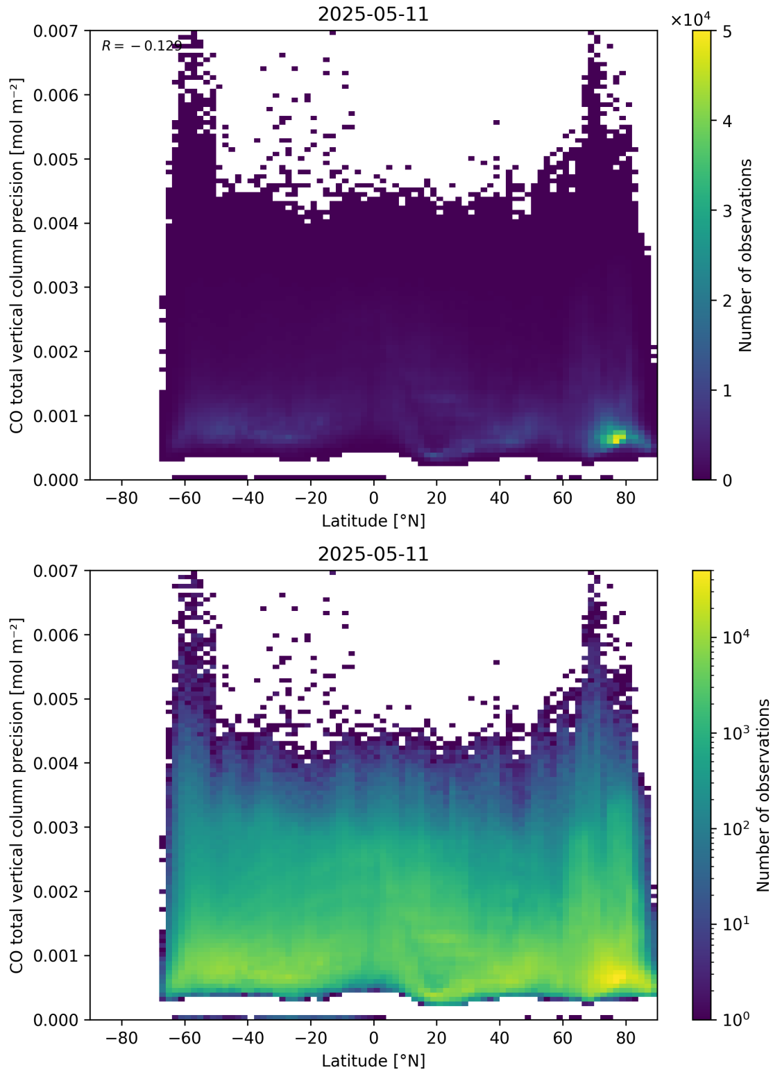
Figure 53: Scatter density plot of “Latitude” against “CO total vertical column precision” for 2025-05-10 to 2025-05-12.
