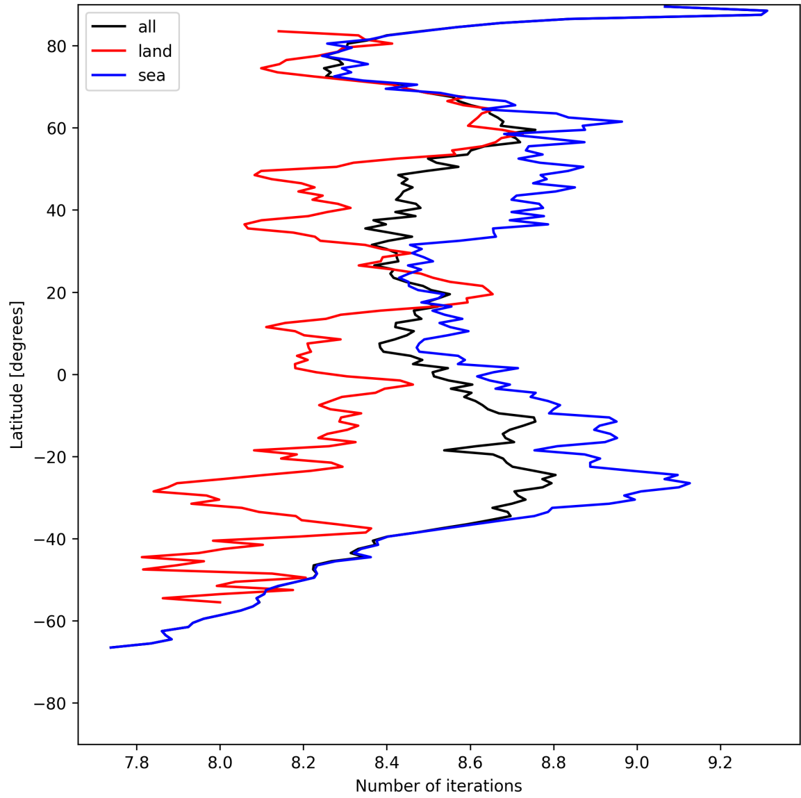
Figure 16: Zonal average of “Number of iterations” for 2025-05-10 to 2025-05-12.
