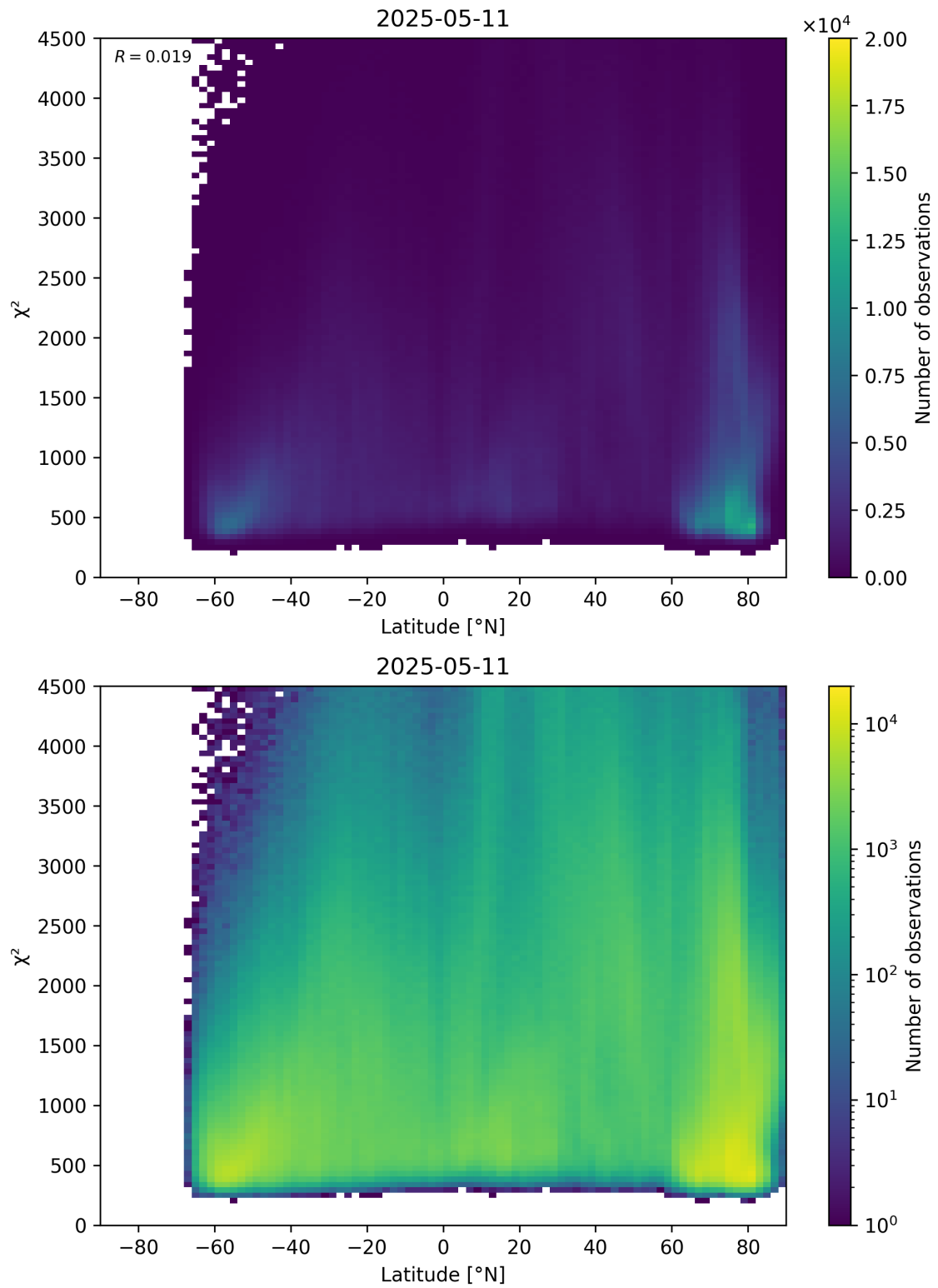
Figure 54: Scatter density plot of “Latitude” against “ \chi^2 ” for 2025-05-10 to 2025-05-12.
