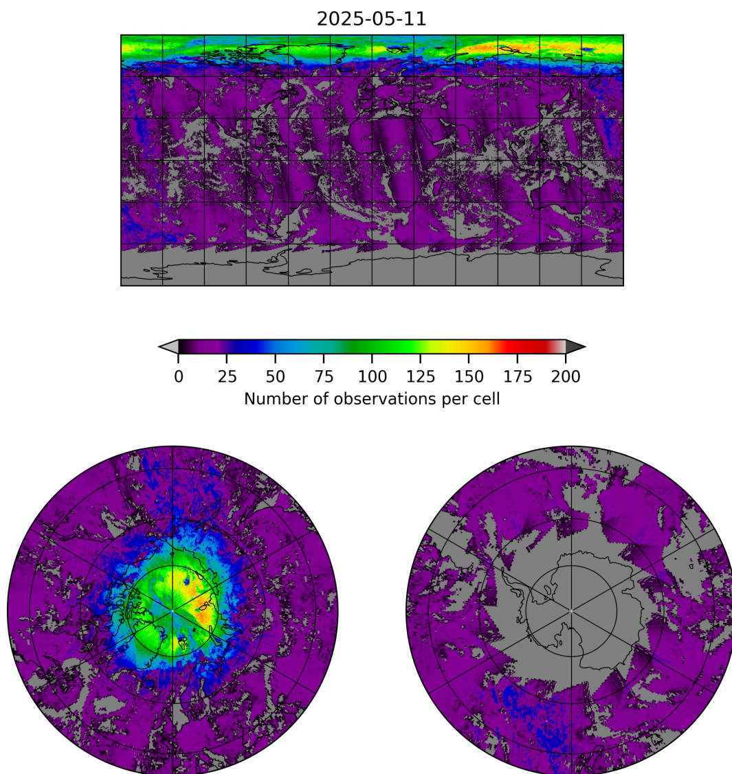
Figure 8: Map of the number of observations for 2025-05-10 to 2025-05-12
