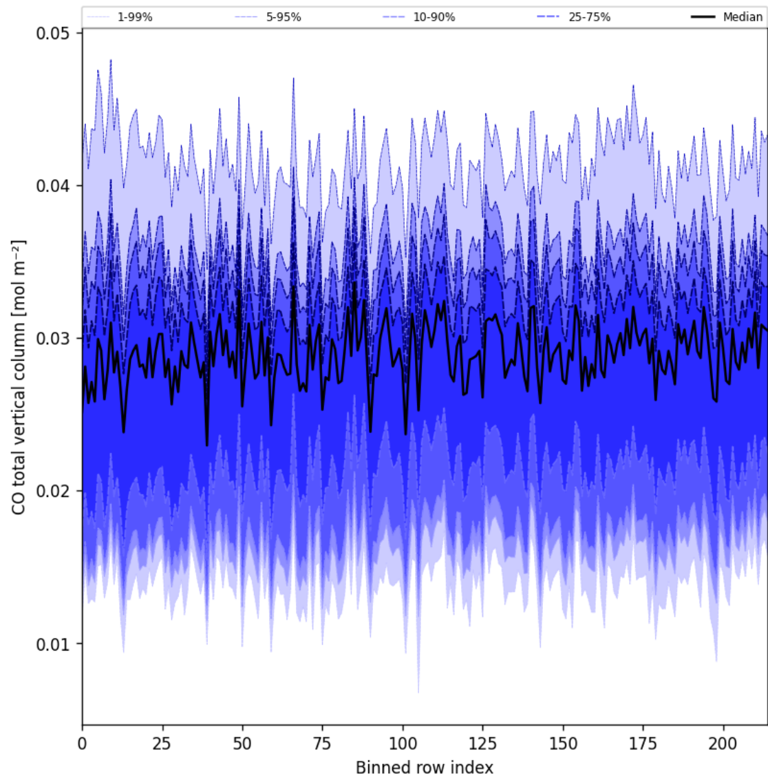
Figure 26: Along track statistics of "CO total vertical column" for 2025-05-10 to 2025-05-12
