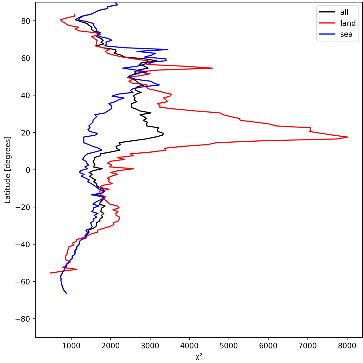
Figure 14: Zonal average of “ \chi^2 ” for 2025-05-10 to 2025-05-12.
