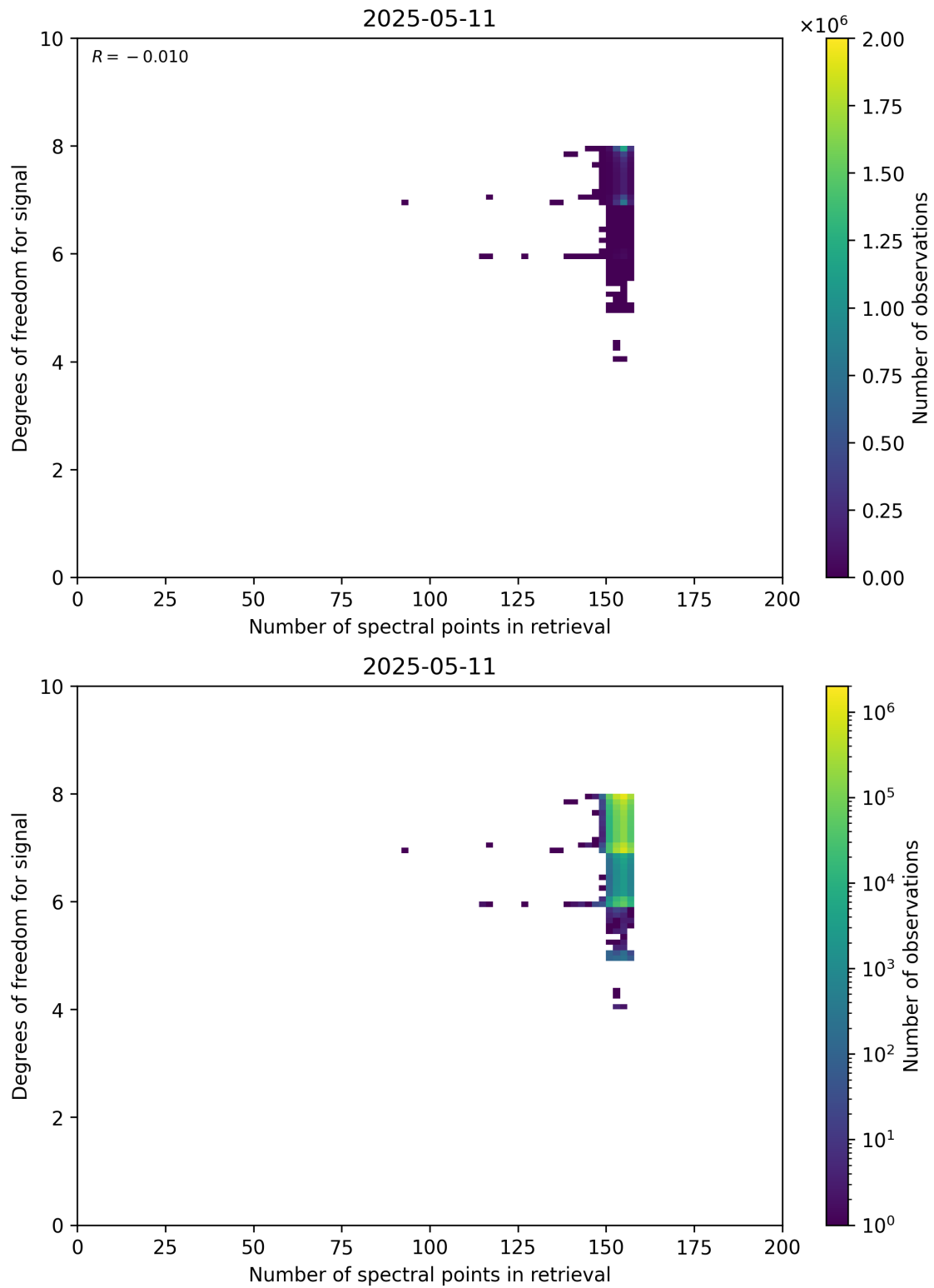
Figure 59: Scatter density plot of “Number of spectral points in retrieval” against “Degrees of freedom for signal” for 2025-05-10 to 2025-05-12.
