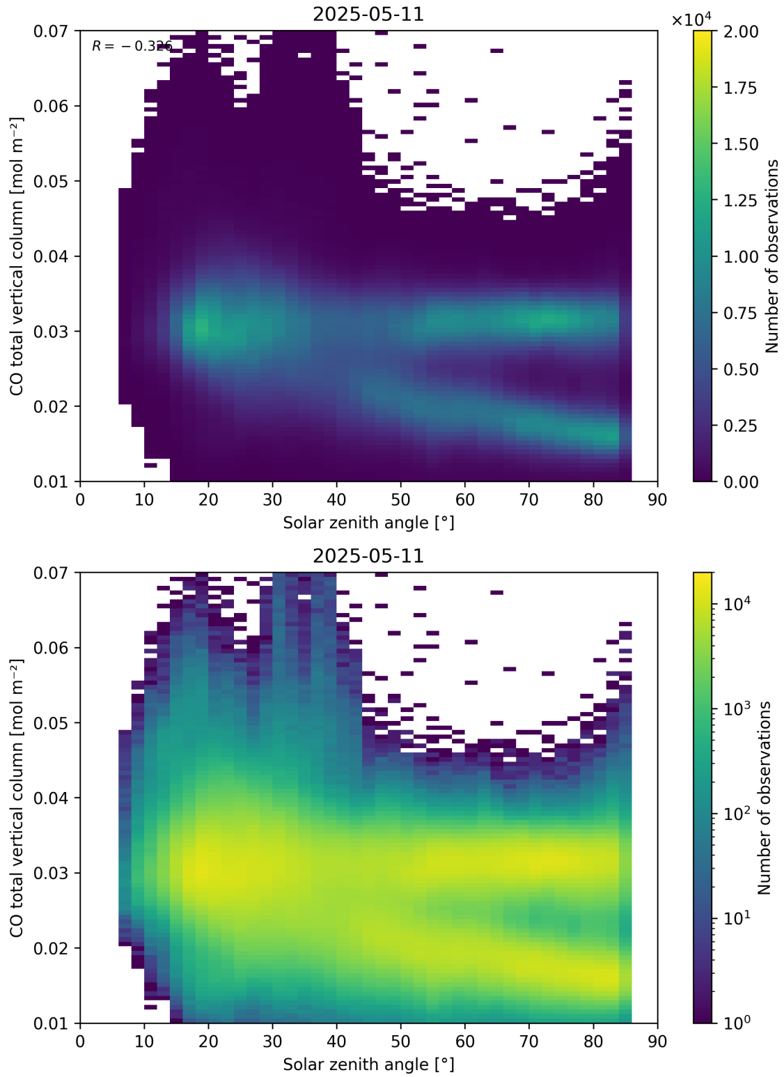
Figure 61: Scatter density plot of “Solar zenith angle” against “CO total vertical column” for 2025-05-10 to 2025-05-12.
