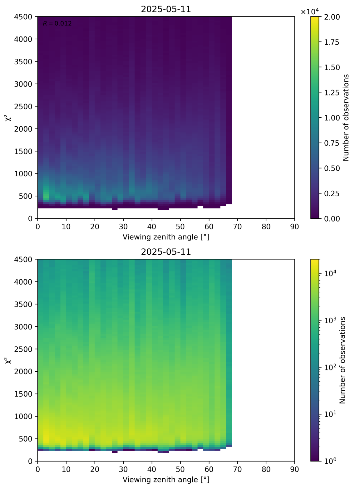
Figure 72: Scatter density plot of “Viewing zenith angle” against “ \chi^2 ” for 2025-05-10 to 2025-05-12.
