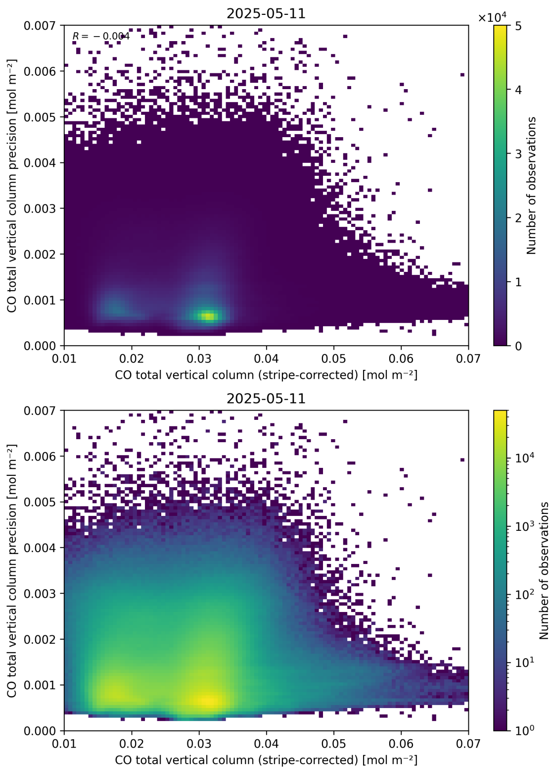
Figure 36: Scatter density plot of “CO total vertical column (stripe-corrected)” against “CO total vertical column precision” for 2025-05-10 to 2025-05-12.
