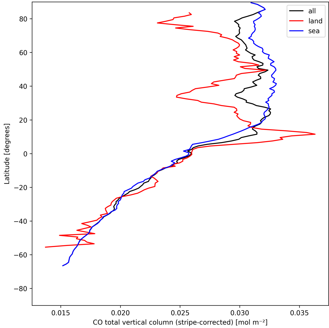
Figure 11: Zonal average of “CO total vertical column (stripe-corrected)” for 2025-05-10 to 2025-05-12.
