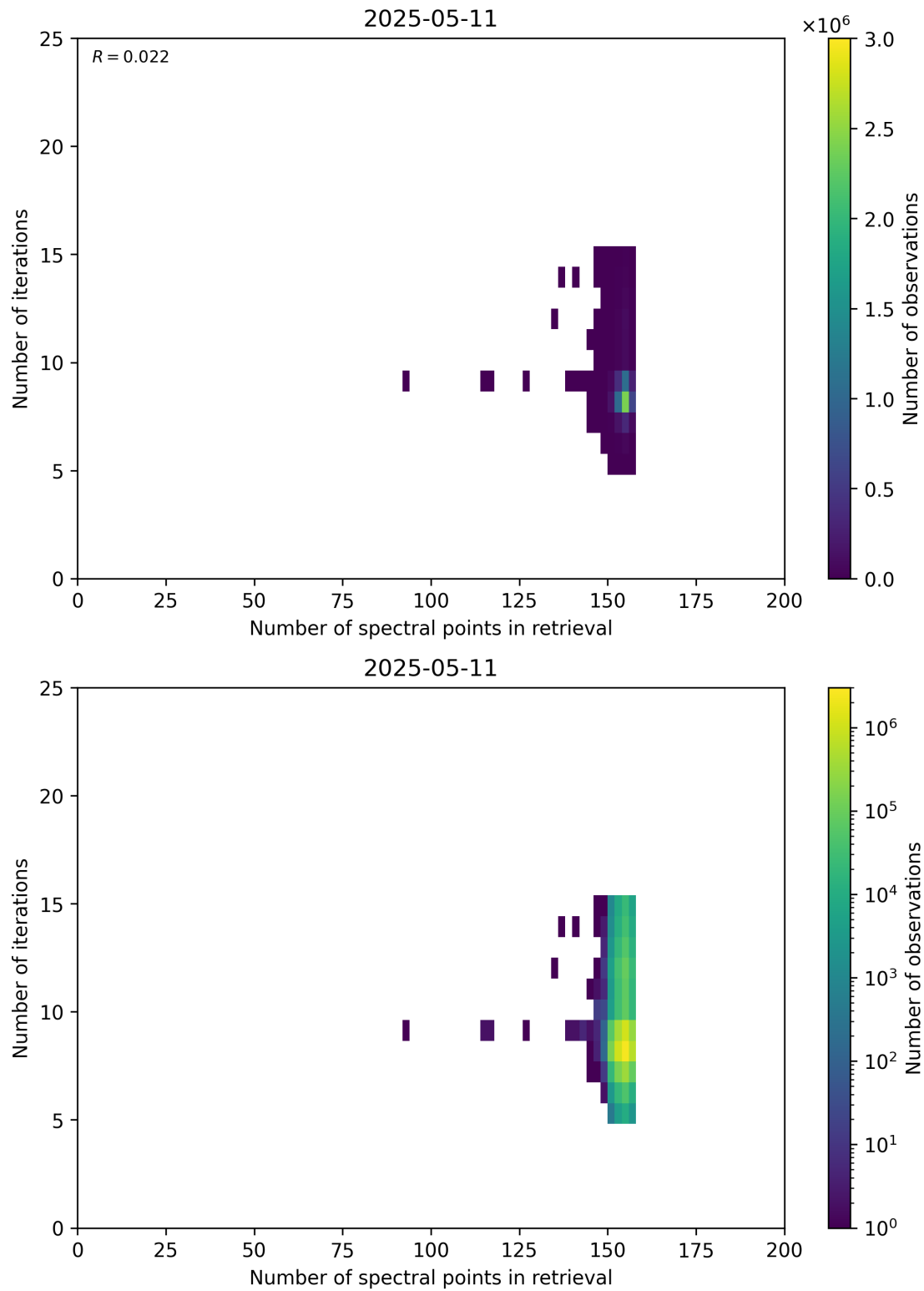
Figure 60: Scatter density plot of “Number of spectral points in retrieval” against “Number of iterations” for 2025-05-10 to 2025-05-12.
