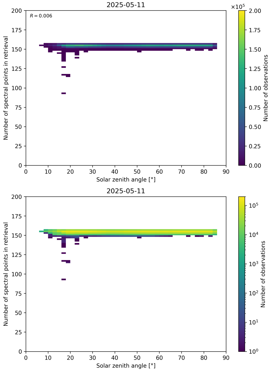
Figure 68: Scatter density plot of “Solar zenith angle” against “Number of spectral points in retrieval” for 2025-05-10 to 2025-05-12.
