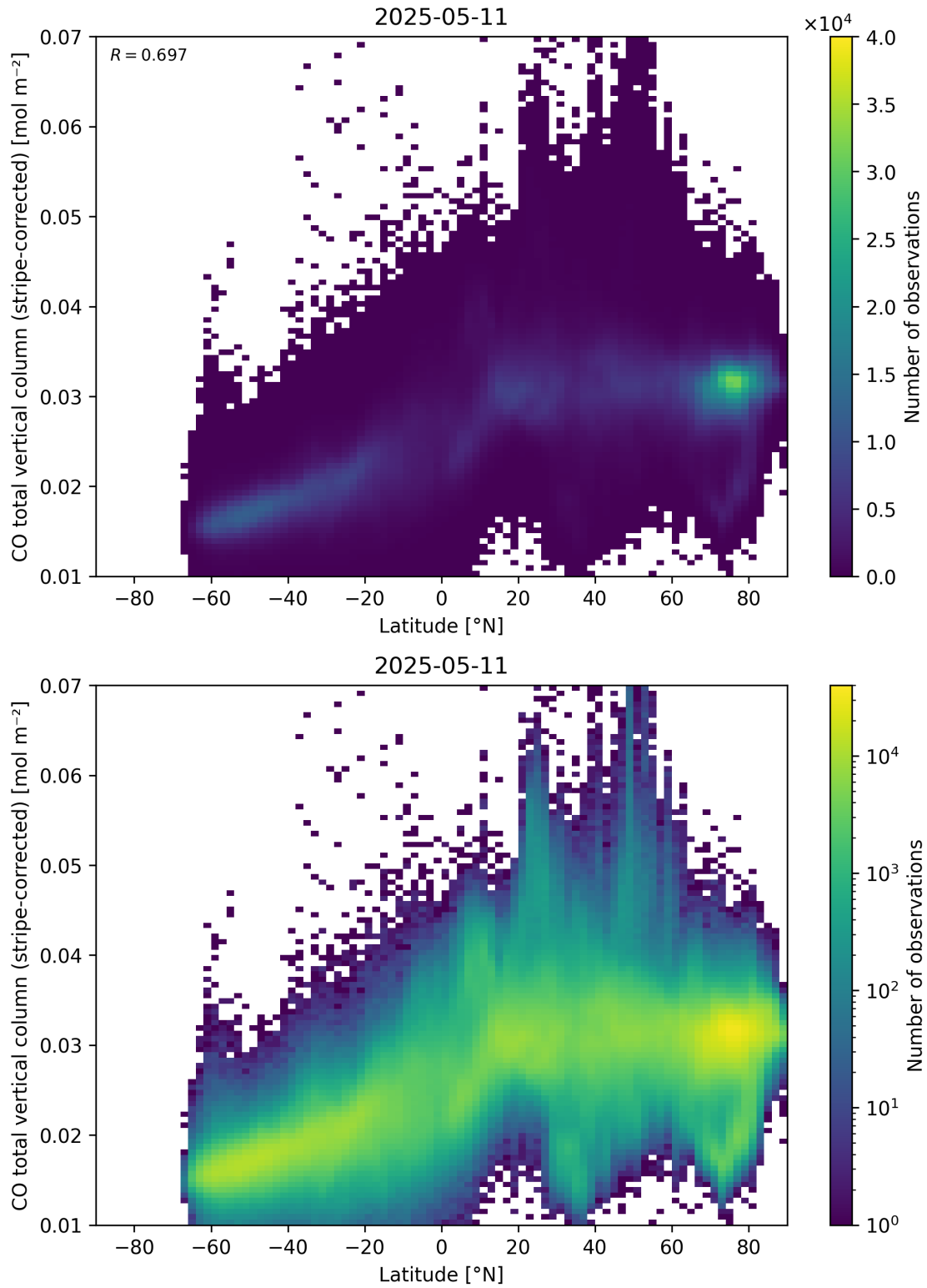
Figure 52: Scatter density plot of “Latitude” against “CO total vertical column (stripe-corrected)” for 2025-05-10 to 2025-05-12.
