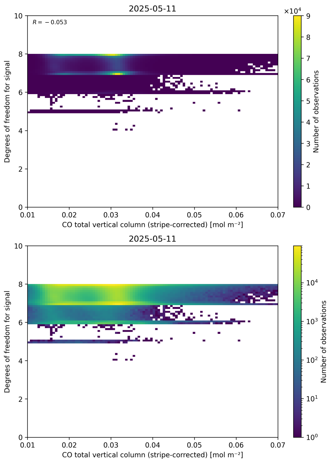
Figure 38: Scatter density plot of “CO total vertical column (stripe-corrected)” against “Degrees of freedom for signal” for 2025-05-10 to 2025-05-12.
