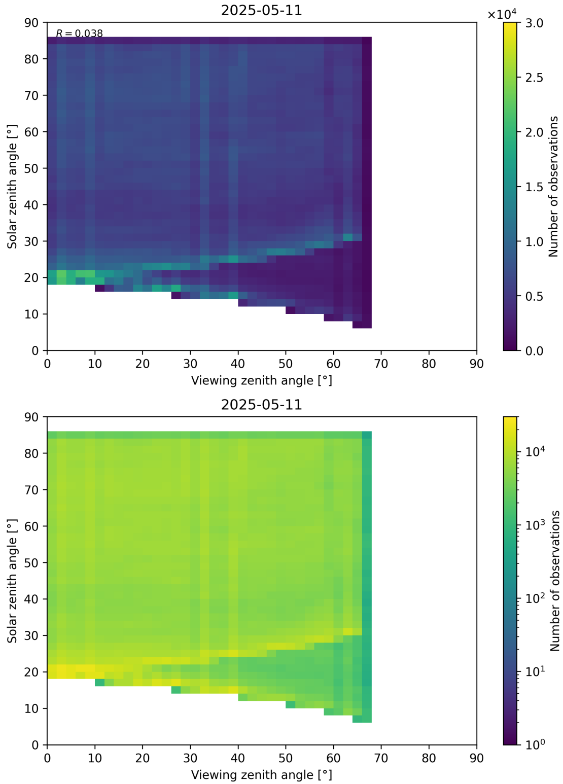
Figure 77: Scatter density plot of “Viewing zenith angle” against “Solar zenith angle” for 2025-05-10 to 2025-05-12.
