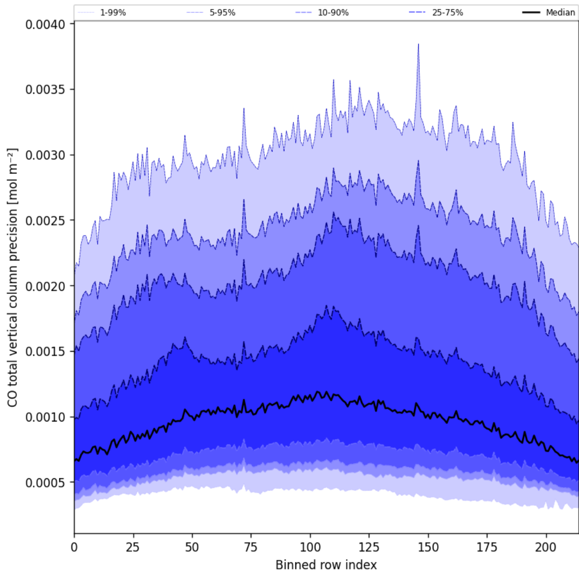
Figure 28: Along track statistics of “CO total vertical column precision” for 2025-05-10 to 2025-05-12
