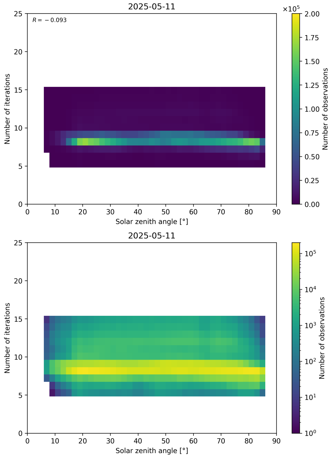
Figure 67: Scatter density plot of “Solar zenith angle” against “Number of iterations” for 2025-05-10 to 2025-05-12.
