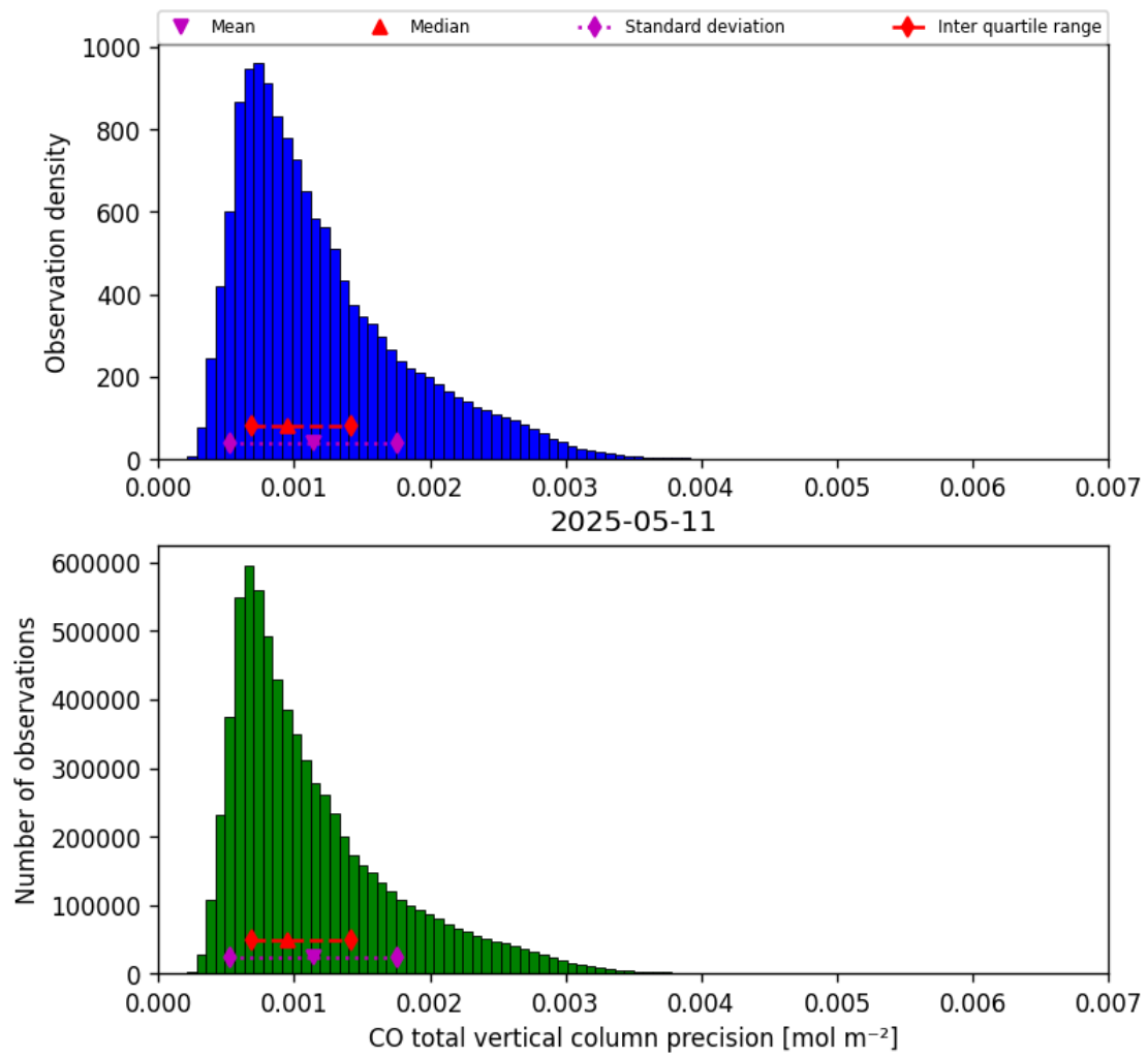
Figure 20: Histogram of “CO total vertical column precision” for 2025-05-10 to 2025-05-12
