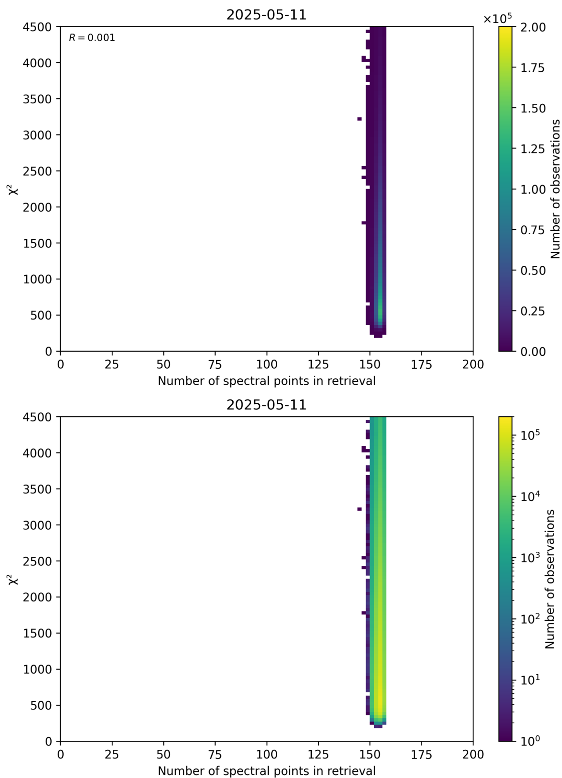
Figure 58: Scatter density plot of “Number of spectral points in retrieval” against “ \chi^2 ” for 2025-05-10 to 2025-05-12.
