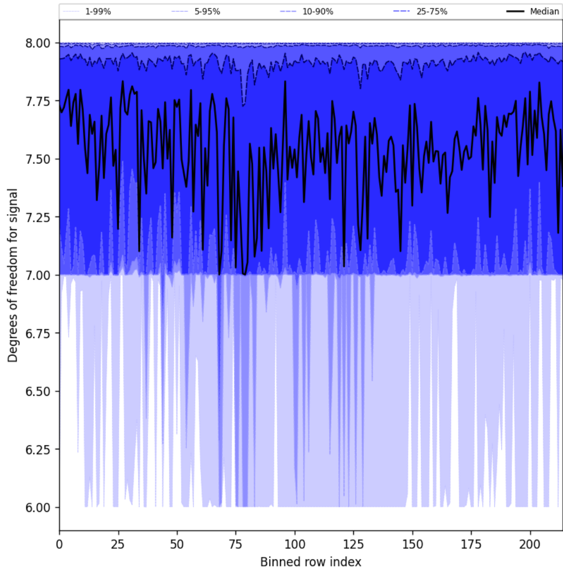
Figure 31: Along track statistics of “Degrees of freedom for signal” for 2025-05-10 to 2025-05-12
