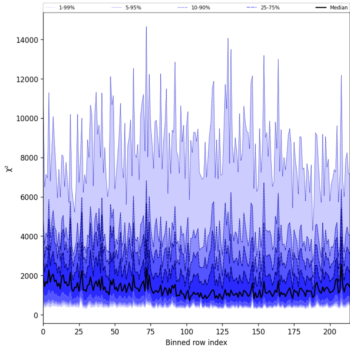
Figure 30: Along track statistics of “ \chi^2 ” for 2025-05-10 to 2025-05-12
