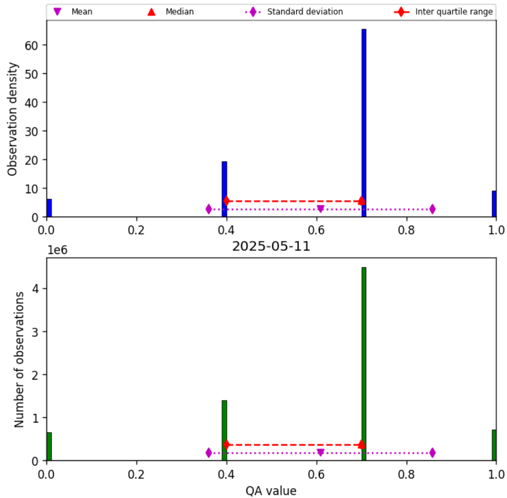
Figure 17: Histogram of “QA value” for 2025-05-10 to 2025-05-12
