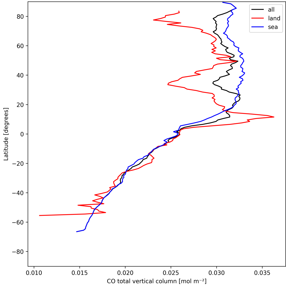
Figure 10: Zonal average of “CO total vertical column” for 2025-05-10 to 2025-05-12.
