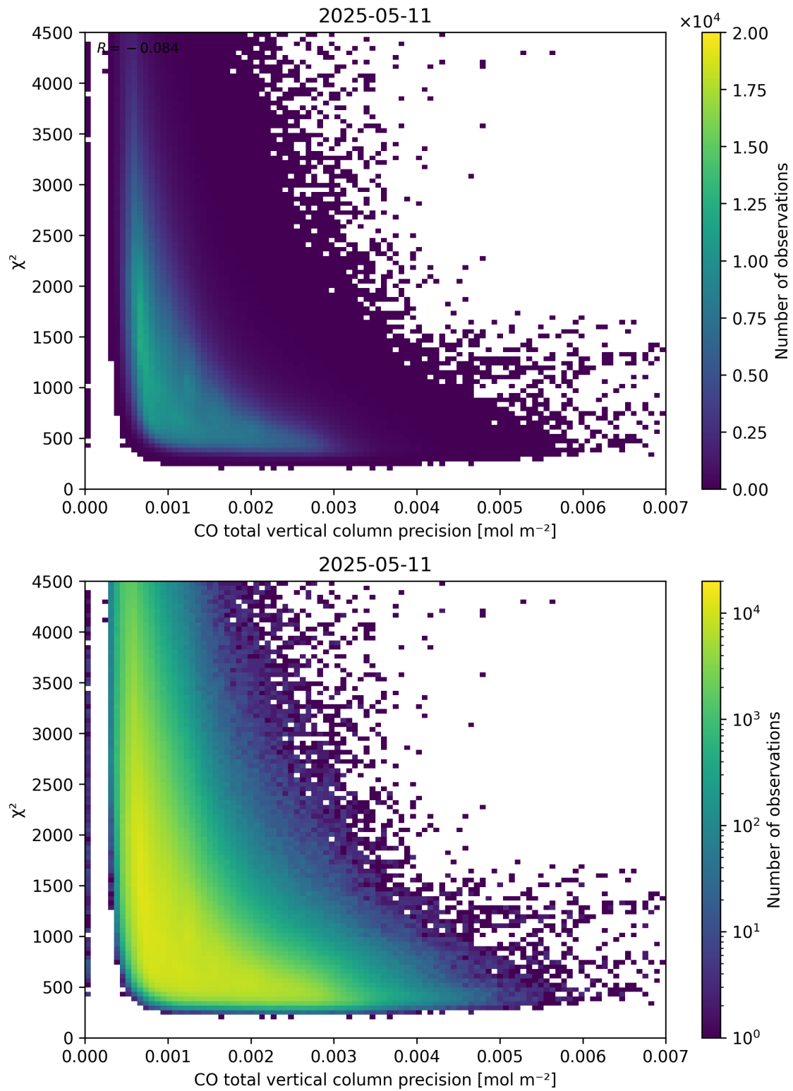
Figure 44: Scatter density plot of “CO total vertical column precision” against “ \chi^2 ” for 2025-05-10 to 2025-05-12.
