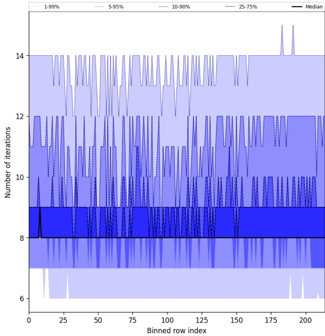
Figure 32: Along track statistics of “Number of iterations” for 2025-05-10 to 2025-05-12
