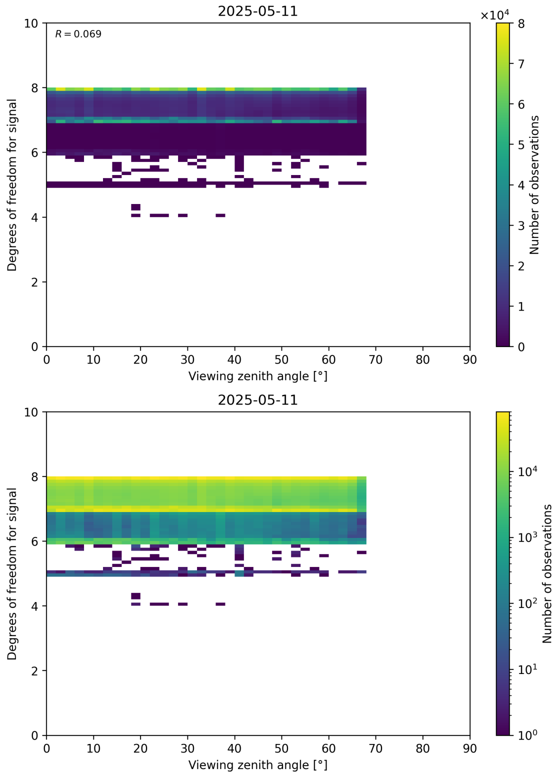
Figure 73: Scatter density plot of “Viewing zenith angle” against “Degrees of freedom for signal” for 2025-05-10 to 2025-05-12.
