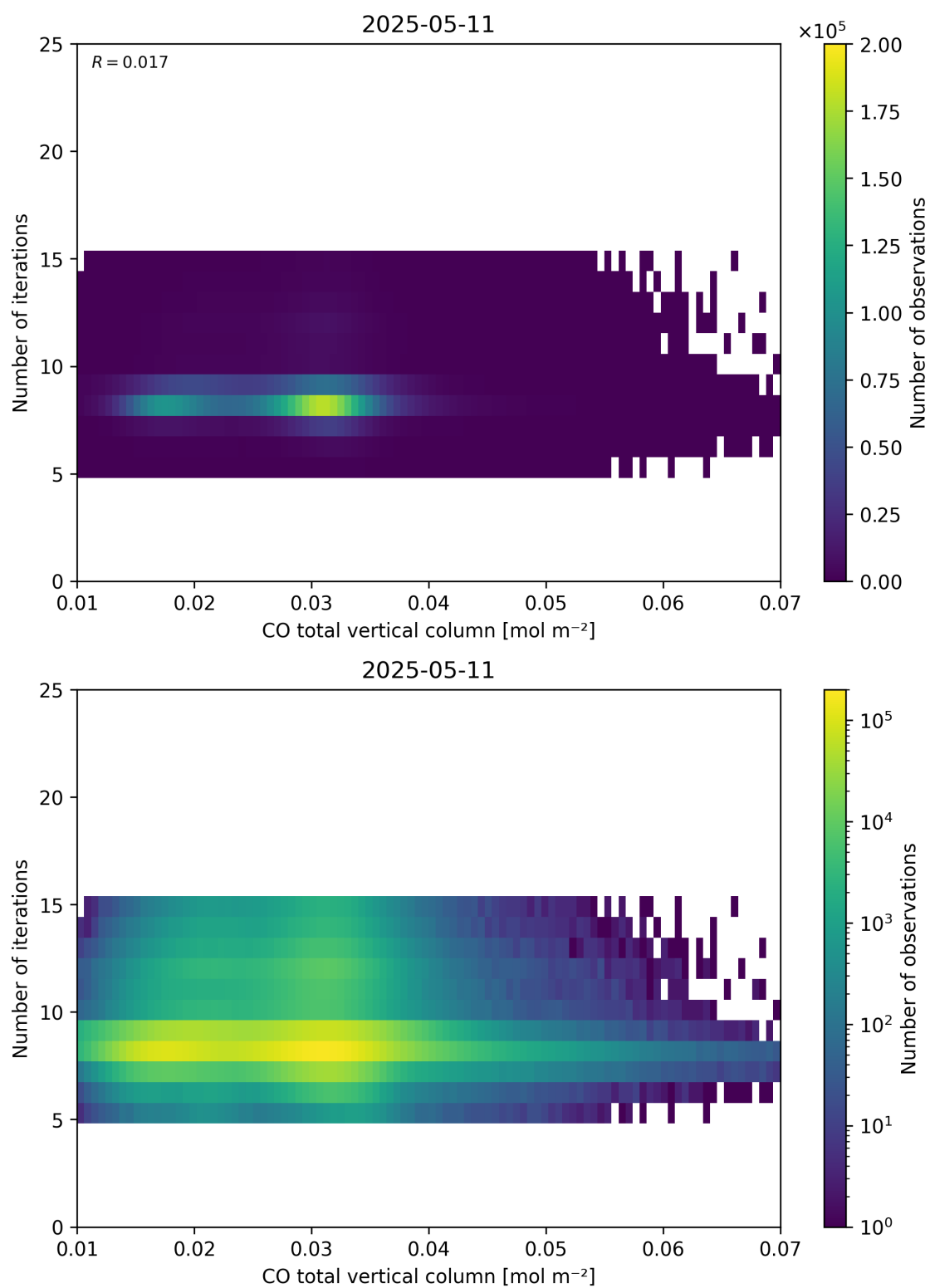
Figure 42: Scatter density plot of “CO total vertical column” against “Number of iterations” for 2025-05-10 to 2025-05-12.
