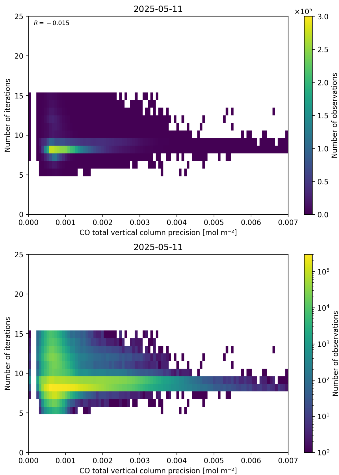
Figure 46: Scatter density plot of “CO total vertical column precision” against “Number of iterations” for 2025-05-10 to 2025-05-12.
