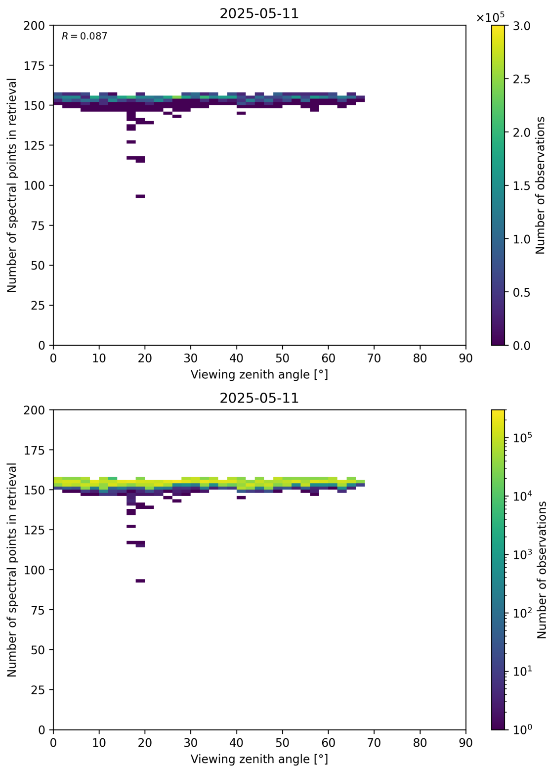
Figure 76: Scatter density plot of “Viewing zenith angle” against “Number of spectral points in retrieval” for 2025-05-10 to 2025-05-12.
