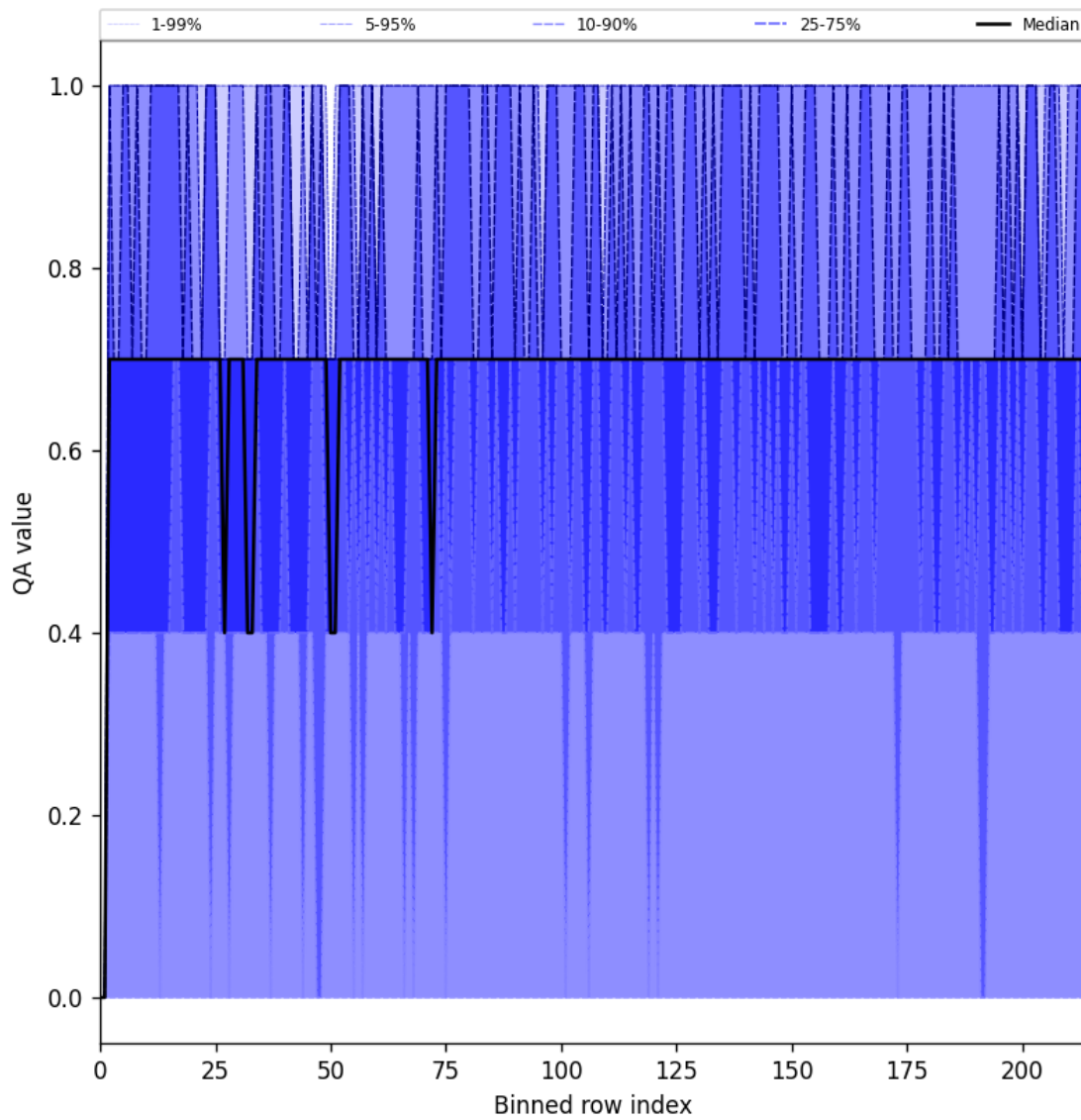
Figure 25: Along track statistics of “QA value” for 2025-05-10 to 2025-05-12
