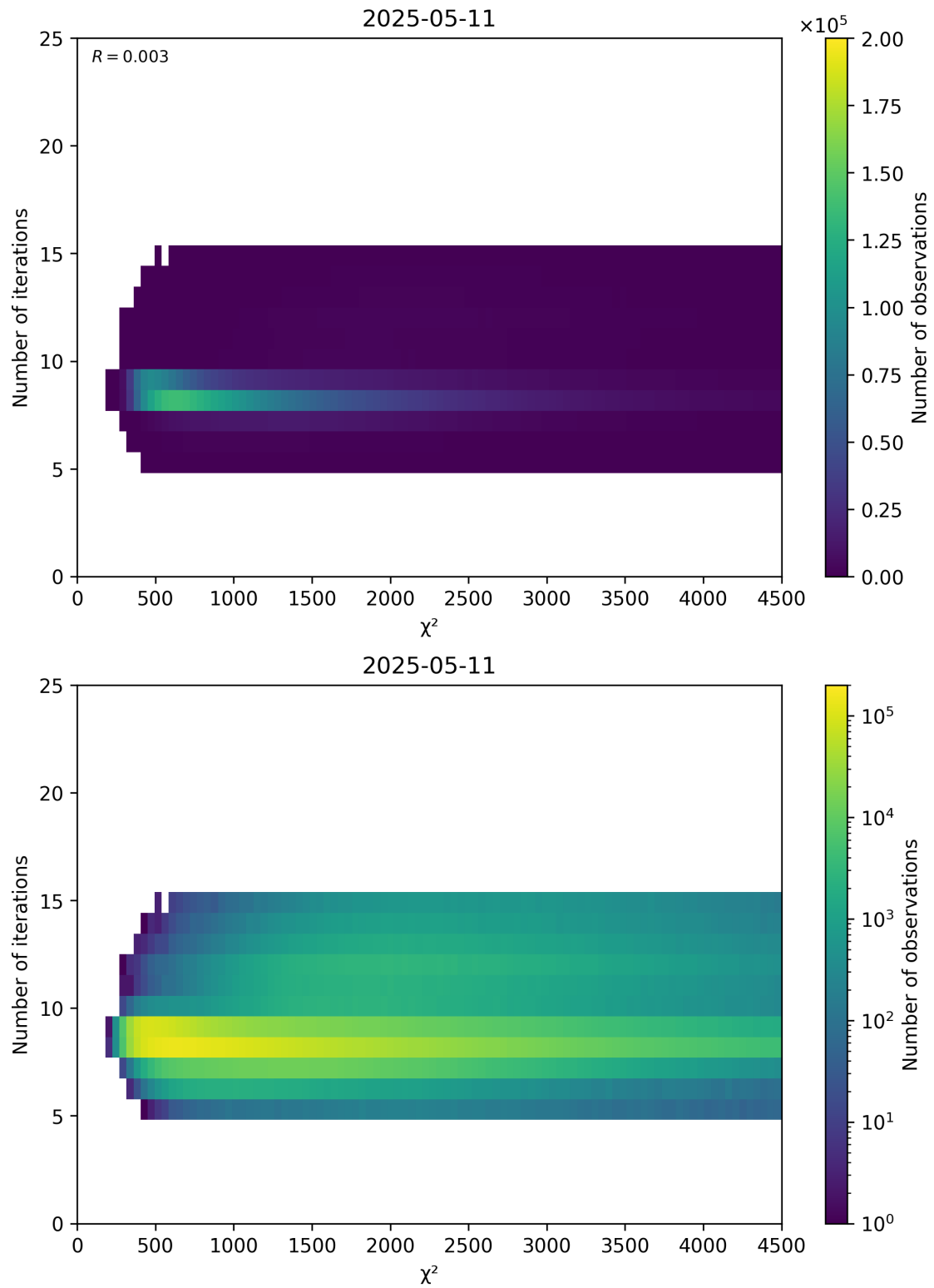
Figure 49: Scatter density plot of “ \chi^2 ” against “Number of iterations” for 2025-05-10 to 2025-05-12.
