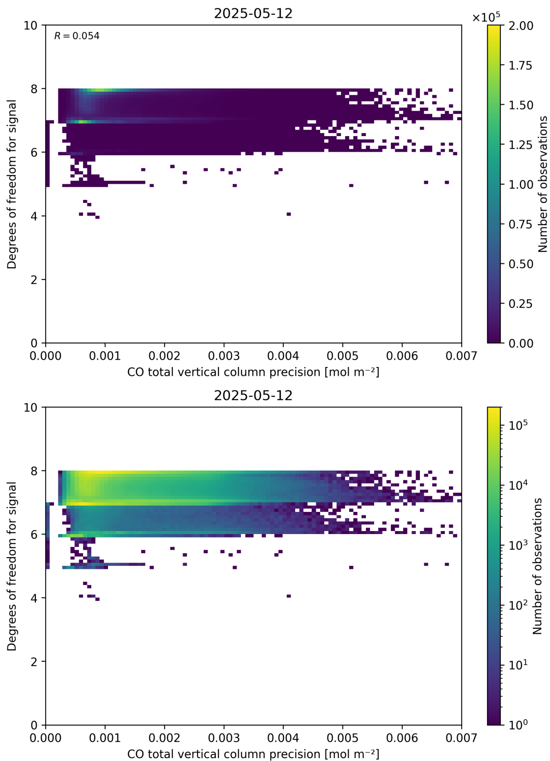
Figure 45: Scatter density plot of “CO total vertical column precision” against “Degrees of freedom for signal” for 2025-05-11 to 2025-05-13.
