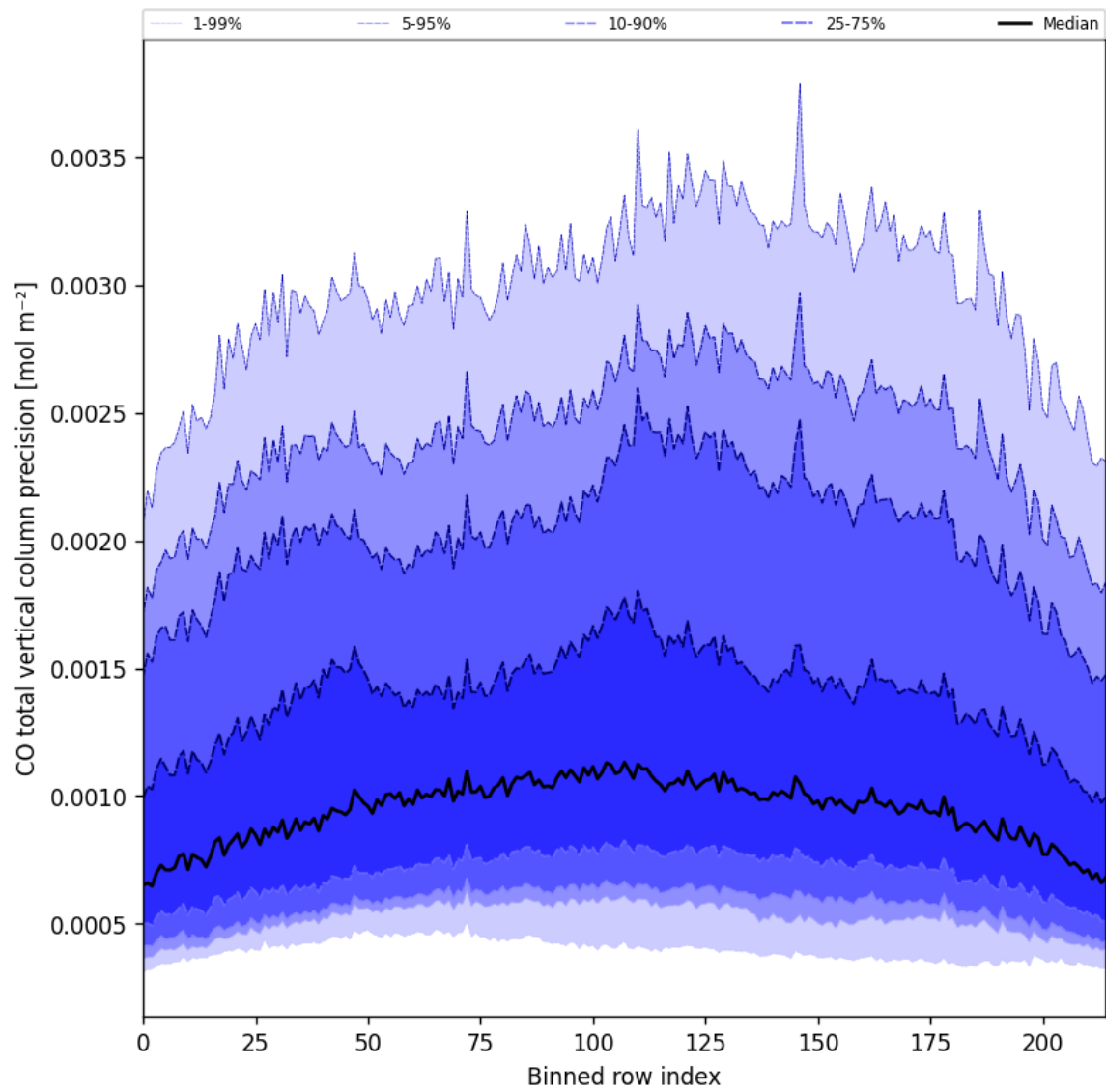
Figure 28: Along track statistics of “CO total vertical column precision” for 2025-05-11 to 2025-05-13
