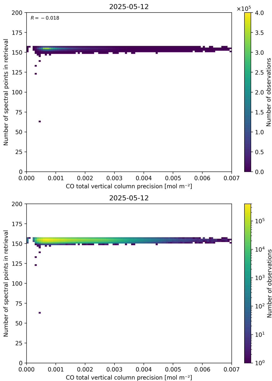
Figure 47: Scatter density plot of “CO total vertical column precision” against “Number of spectral points in retrieval” for 2025-05-11 to 2025-05-13.
