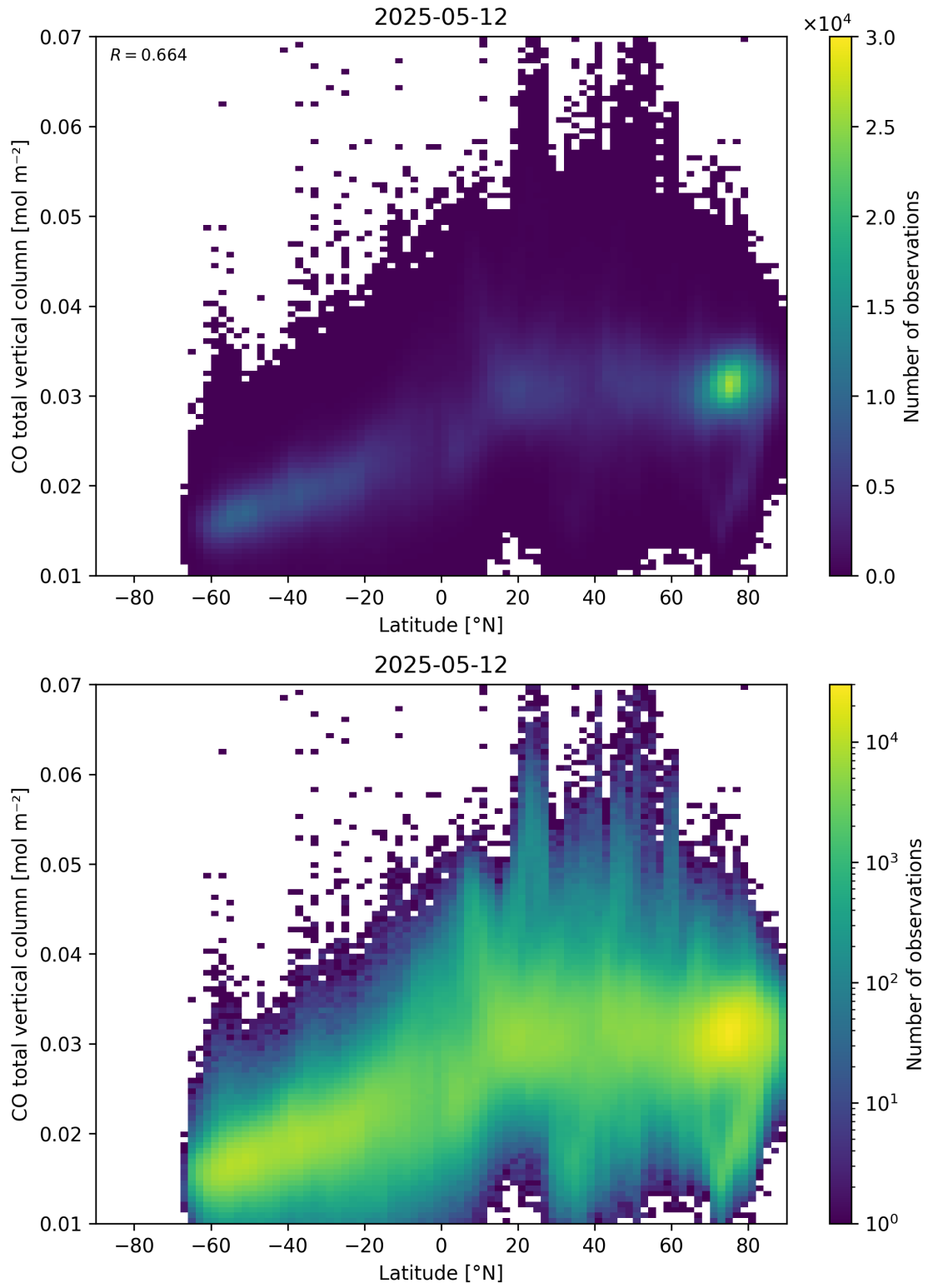
Figure 51: Scatter density plot of “Latitude” against “CO total vertical column” for 2025-05-11 to 2025-05-13.
