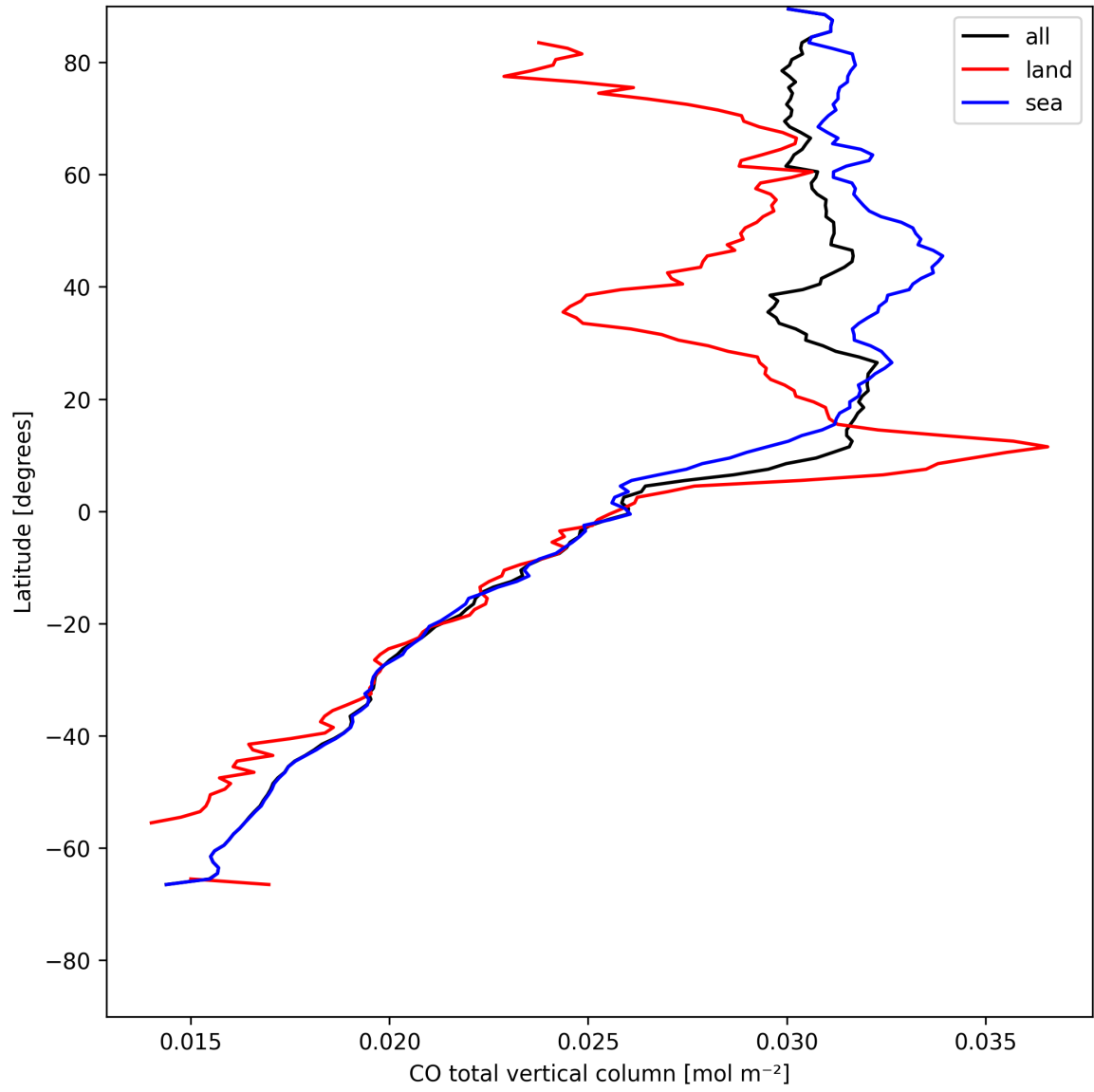
Figure 10: Zonal average of “CO total vertical column” for 2025-05-11 to 2025-05-13.
