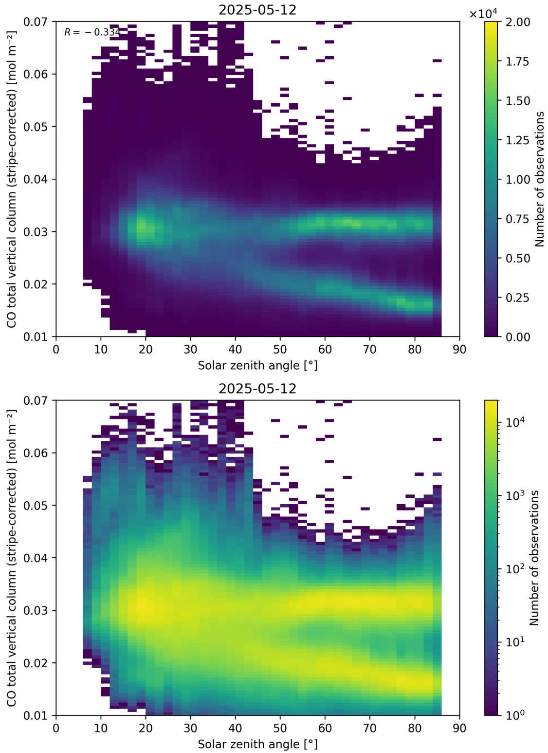
Figure 62: Scatter density plot of “Solar zenith angle” against “CO total vertical column (stripe-corrected)” for 2025-05-11 to 2025-05-13.
