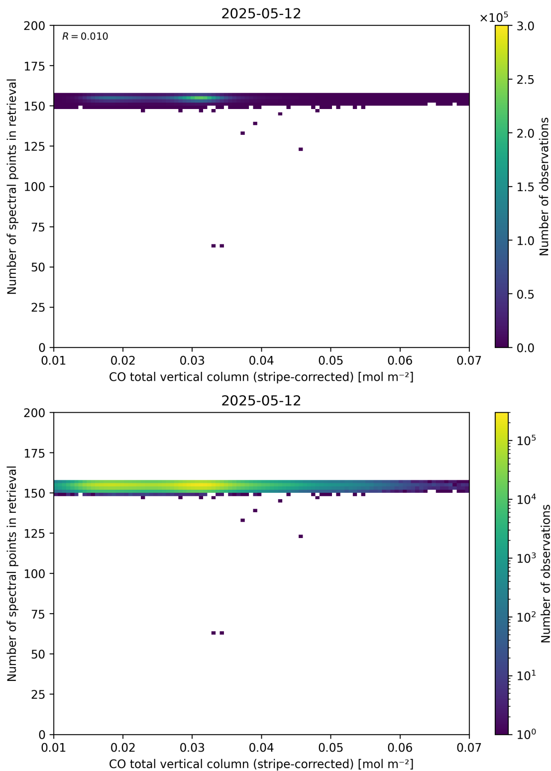
Figure 40: Scatter density plot of “CO total vertical column (stripe-corrected)” against “Number of spectral points in retrieval” for 2025-05-11 to 2025-05-13.
