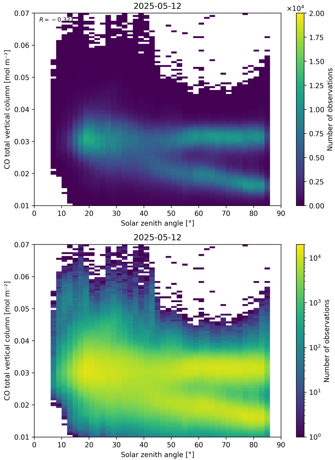
Figure 61: Scatter density plot of “Solar zenith angle” against “CO total vertical column” for 2025-05-11 to 2025-05-13.
