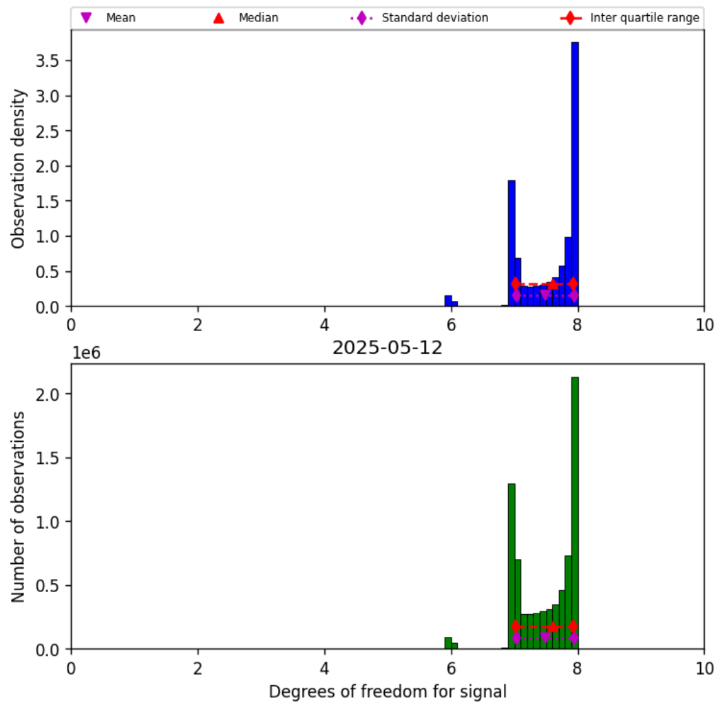
Figure 23: Histogram of “Degrees of freedom for signal” for 2025-05-11 to 2025-05-13
