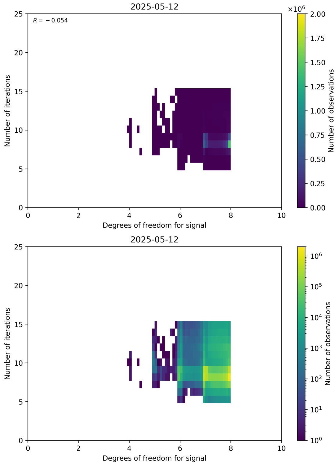
Figure 50: Scatter density plot of “Degrees of freedom for signal” against “Number of iterations” for 2025-05-11 to 2025-05-13.
