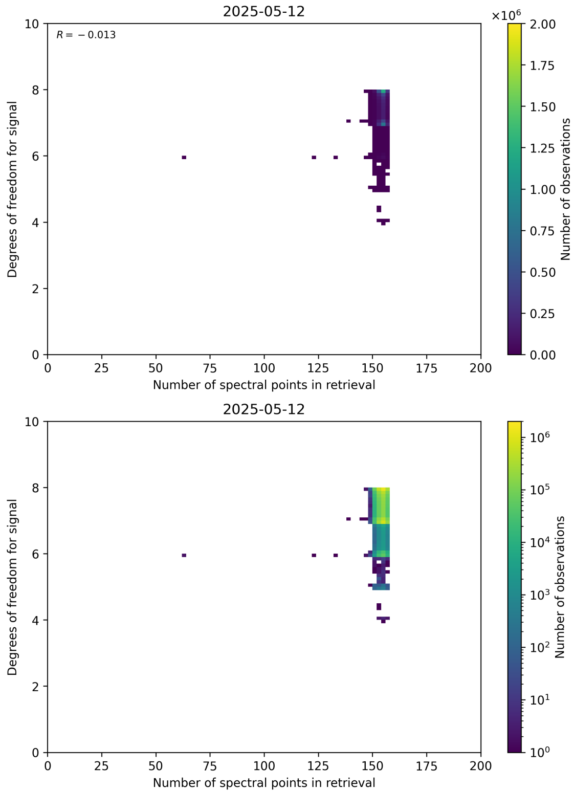
Figure 59: Scatter density plot of “Number of spectral points in retrieval” against “Degrees of freedom for signal” for 2025-05-11 to 2025-05-13.
