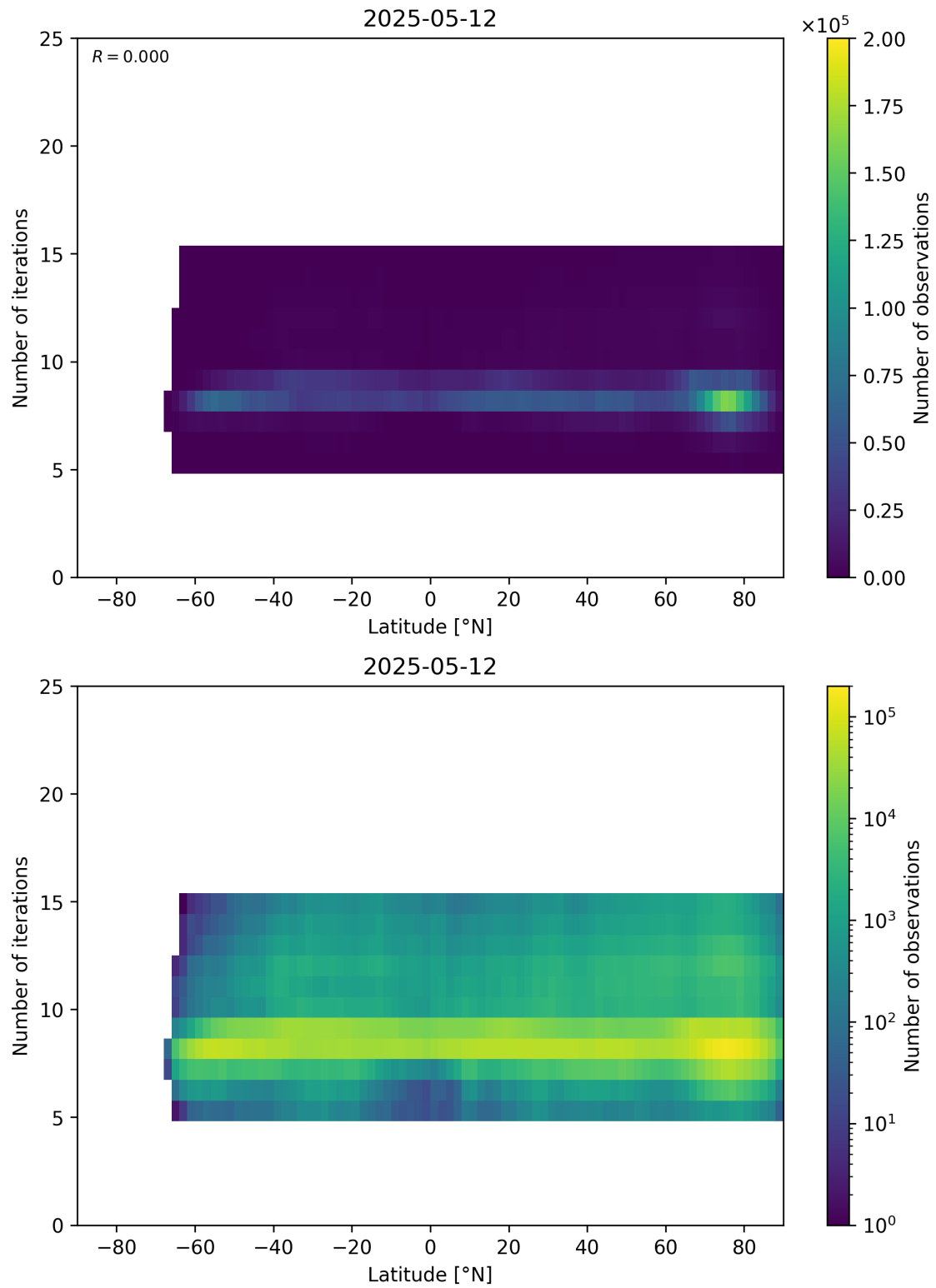
Figure 56: Scatter density plot of “Latitude” against “Number of iterations” for 2025-05-11 to 2025-05-13.
