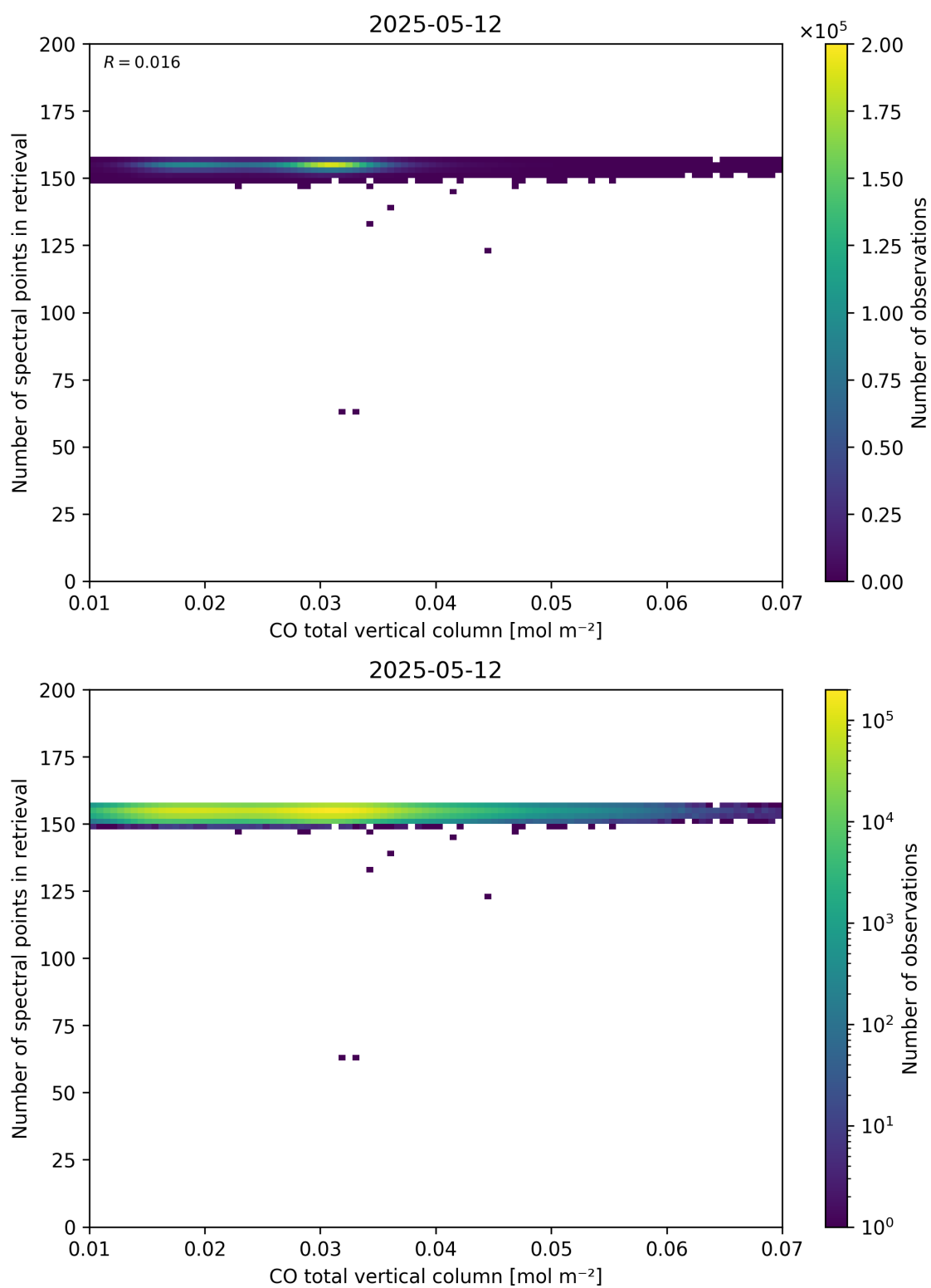
Figure 43: Scatter density plot of “CO total vertical column” against “Number of spectral points in retrieval” for 2025-05-11 to 2025-05-13.
