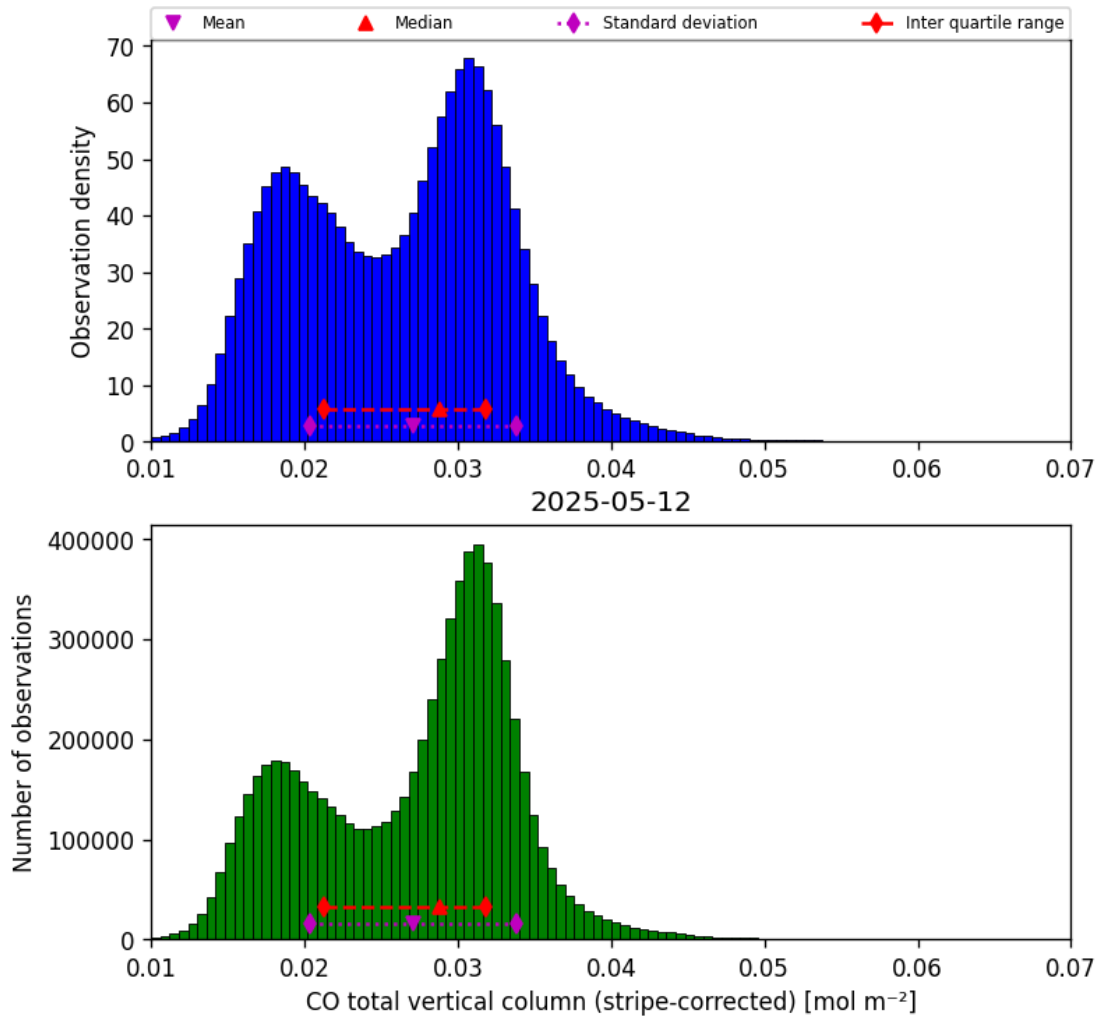
Figure 19: Histogram of “CO total vertical column (stripe-corrected)” for 2025-05-11 to 2025-05-13
