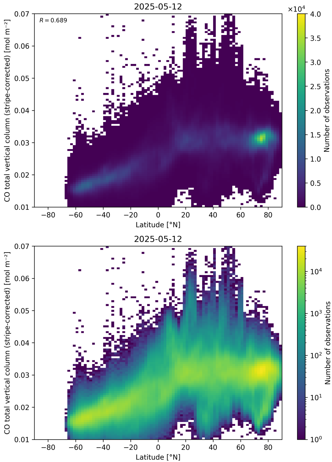
Figure 52: Scatter density plot of “Latitude” against “CO total vertical column (stripe-corrected)” for 2025-05-11 to 2025-05-13.
