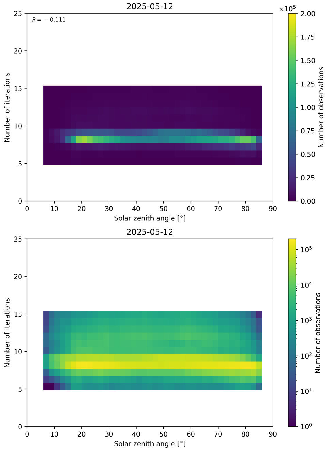
Figure 67: Scatter density plot of “Solar zenith angle” against “Number of iterations” for 2025-05-11 to 2025-05-13.
