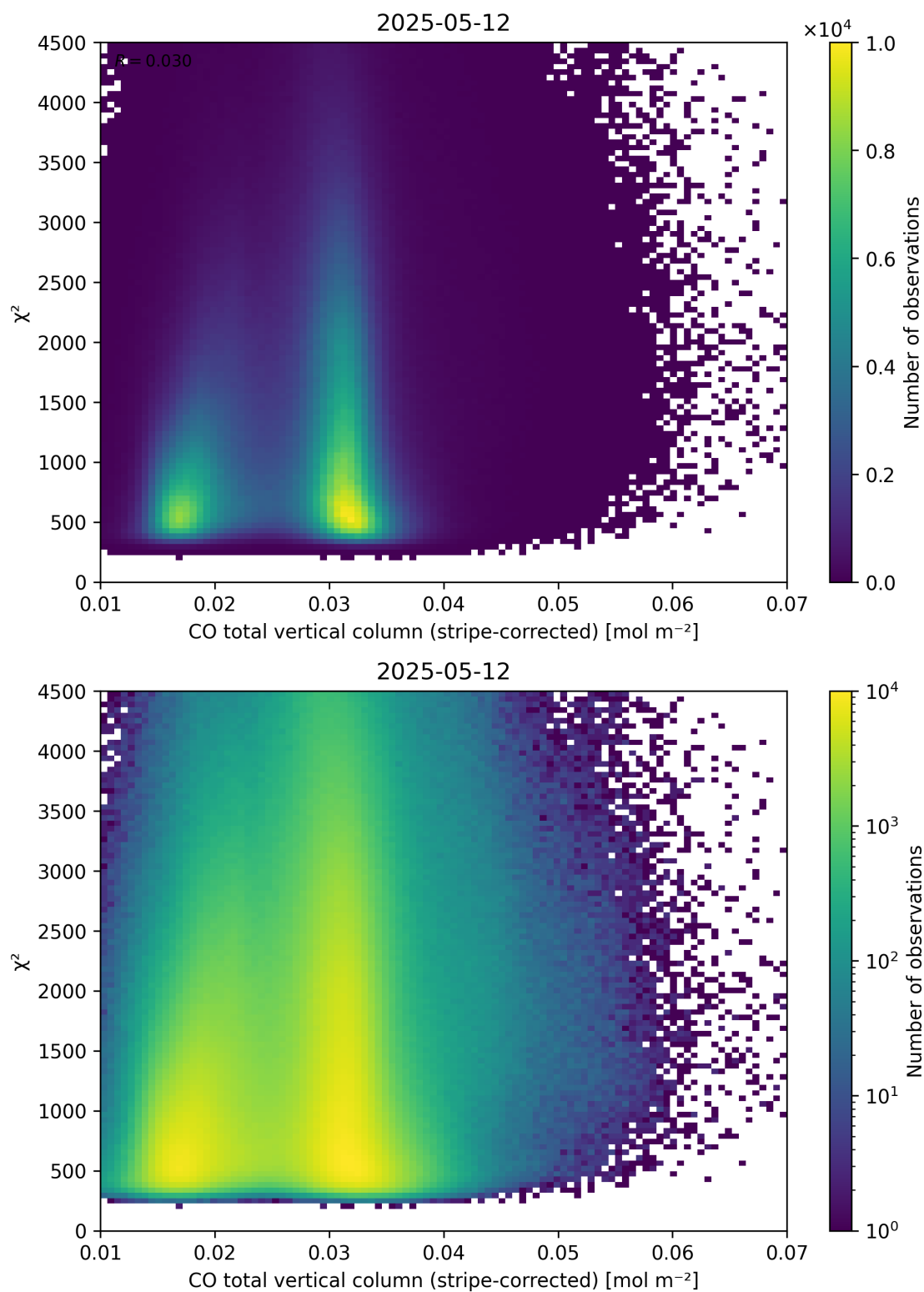
Figure 37: Scatter density plot of “CO total vertical column (stripe-corrected)” against “ \chi^2 ” for 2025-05-11 to 2025-05-13.
