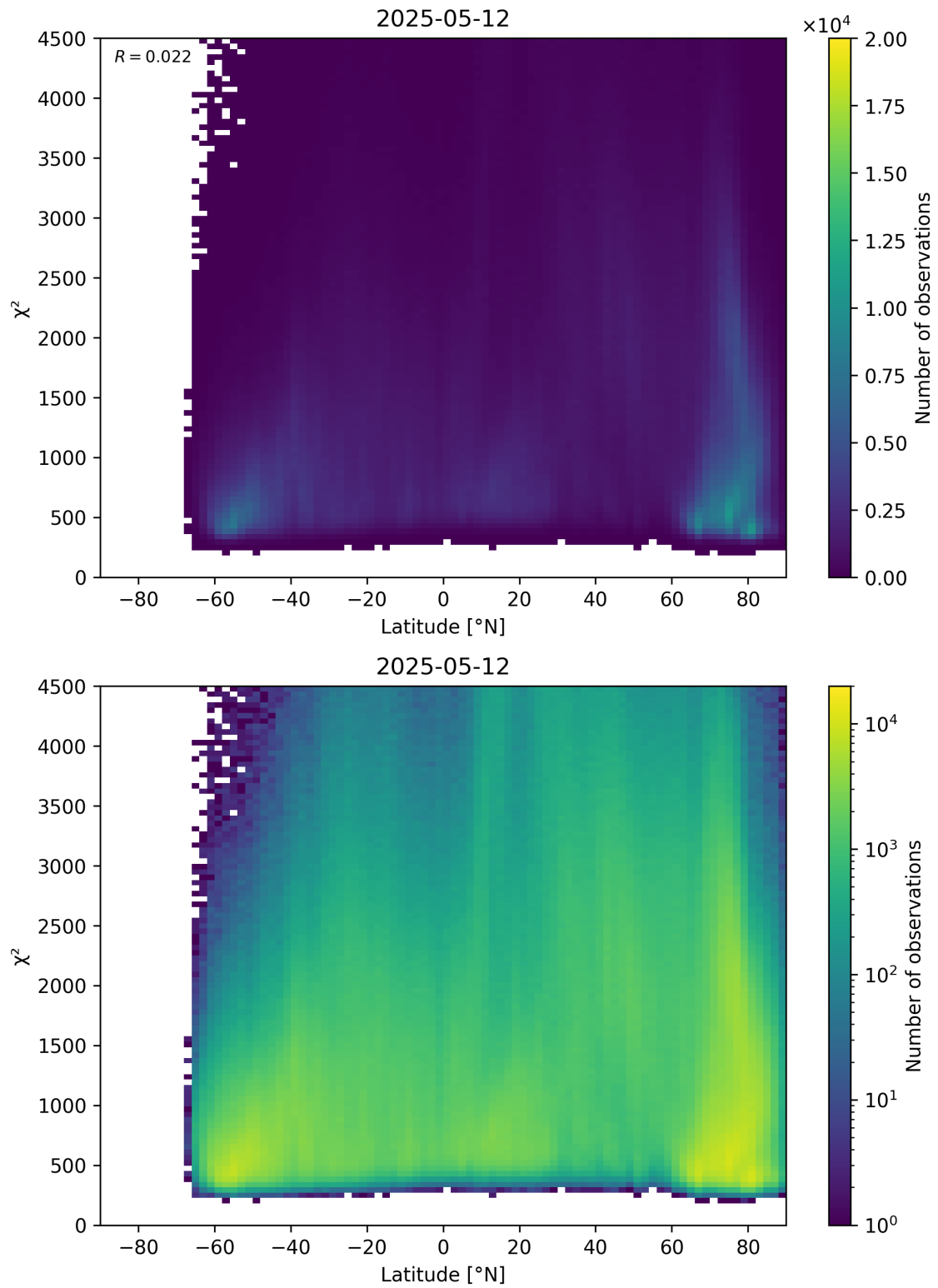
Figure 54: Scatter density plot of “Latitude” against “ \chi^2 ” for 2025-05-11 to 2025-05-13.
