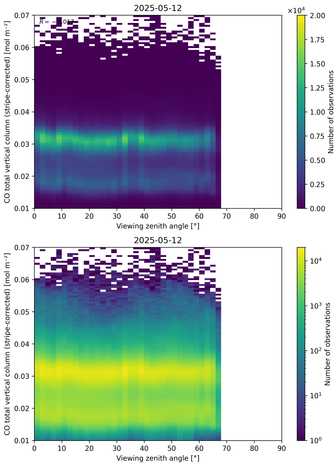
Figure 70: Scatter density plot of “Viewing zenith angle” against “CO total vertical column (stripe-corrected)” for 2025-05-11 to 2025-05-13.
