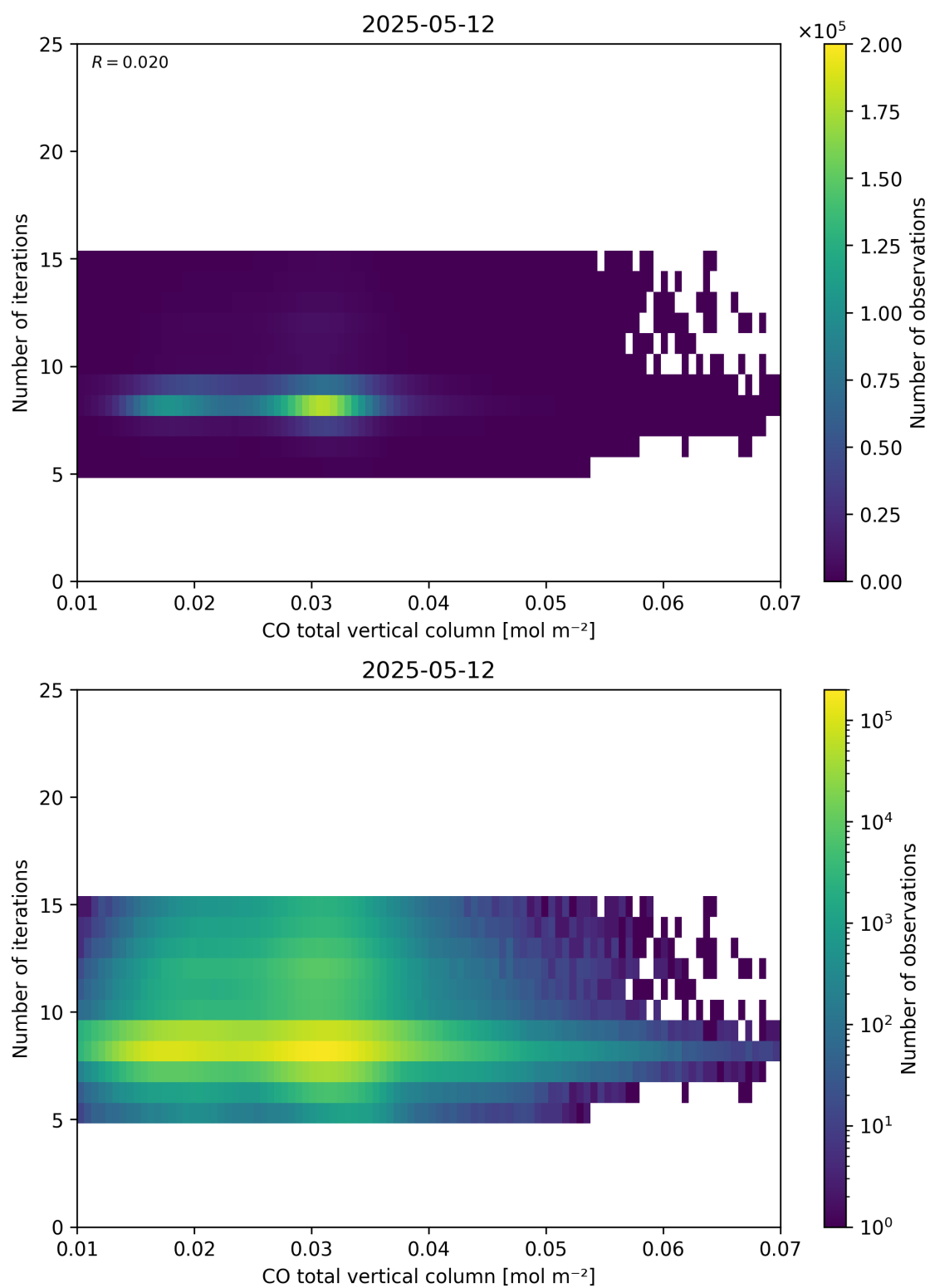
Figure 42: Scatter density plot of “CO total vertical column” against “Number of iterations” for 2025-05-11 to 2025-05-13.
