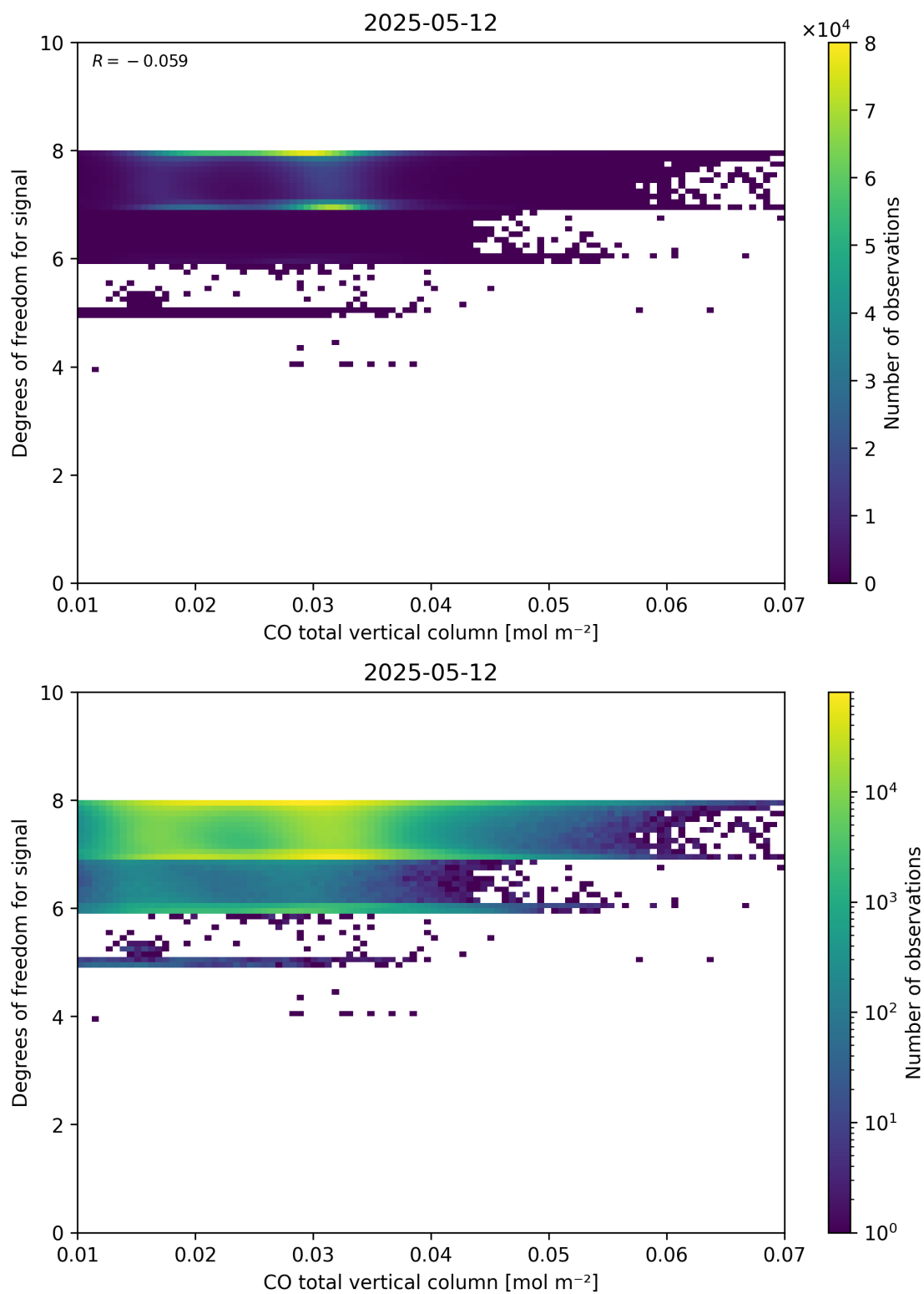
Figure 41: Scatter density plot of “CO total vertical column” against “Degrees of freedom for signal” for 2025-05-11 to 2025-05-13.
