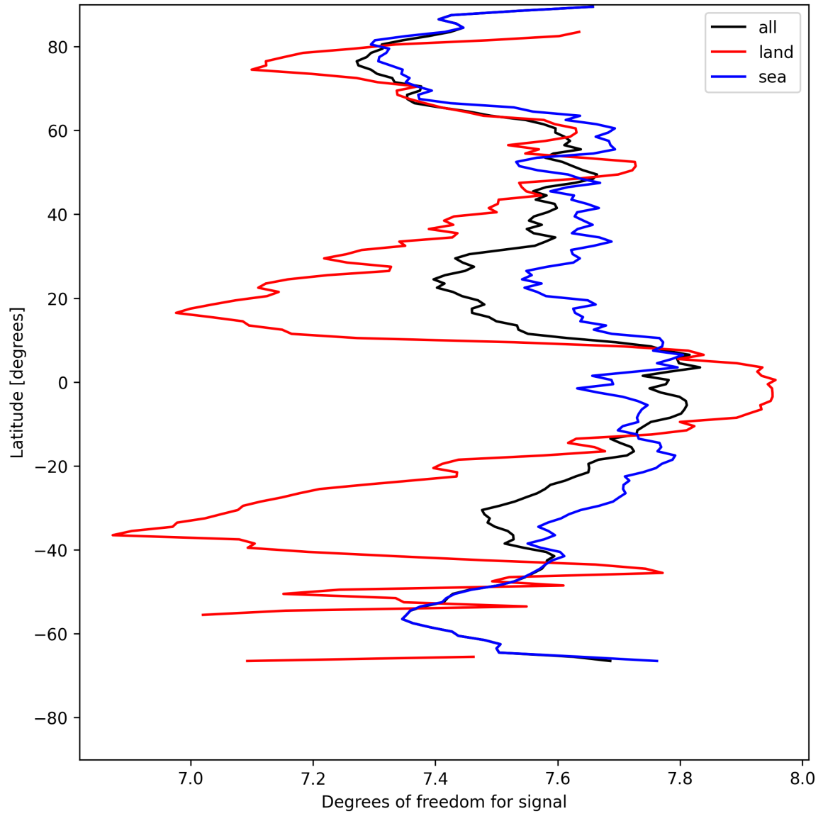
Figure 15: Zonal average of “Degrees of freedom for signal” for 2025-05-11 to 2025-05-13.
