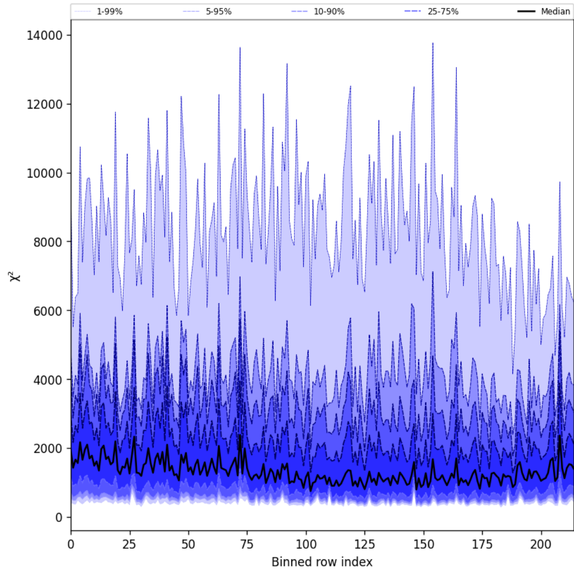
Figure 30: Along track statistics of “ \chi^2 ” for 2025-05-11 to 2025-05-13
