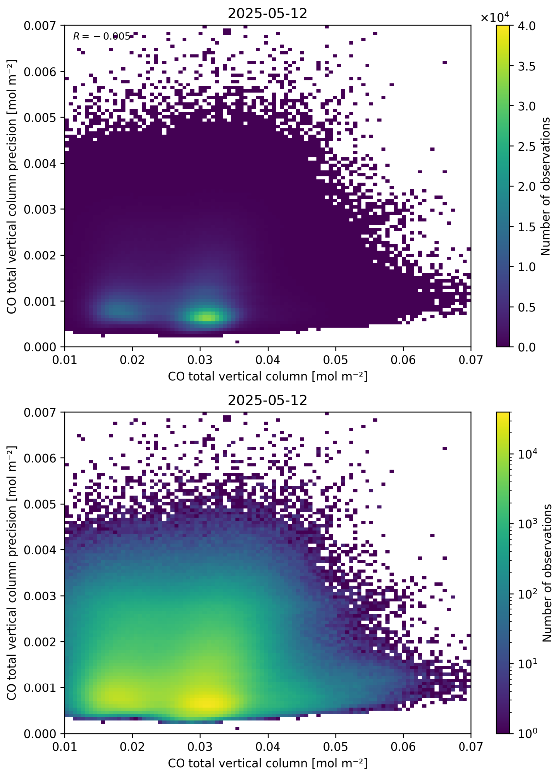
Figure 34: Scatter density plot of “CO total vertical column” against “CO total vertical column precision” for 2025-05-11 to 2025-05-13.
