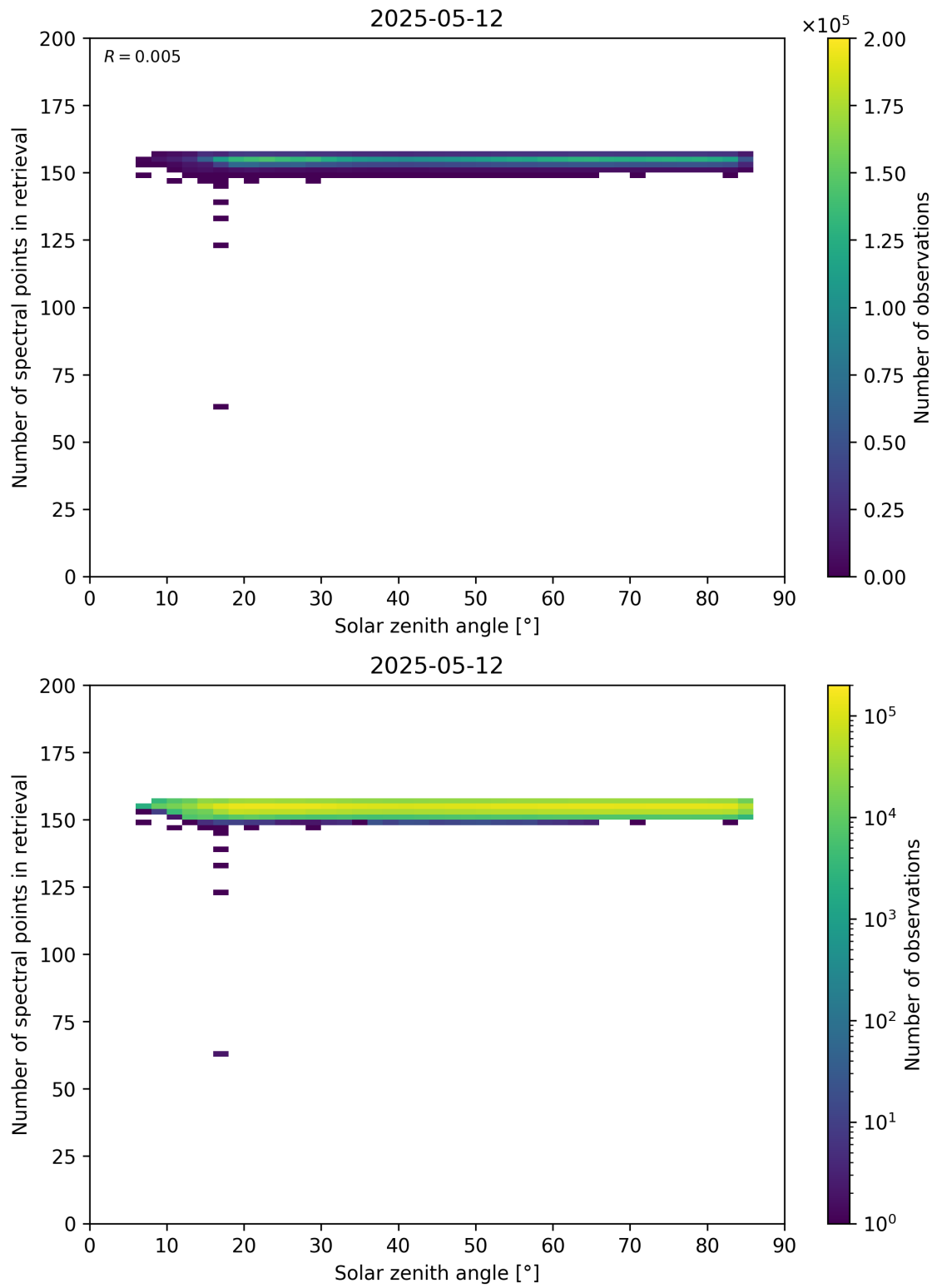
Figure 68: Scatter density plot of “Solar zenith angle” against “Number of spectral points in retrieval” for 2025-05-11 to 2025-05-13.
