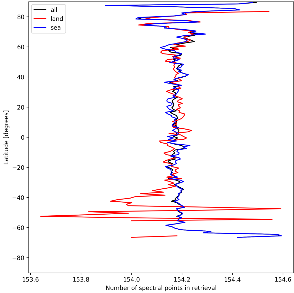
Figure 13: Zonal average of “Number of spectral points in retrieval” for 2025-05-11 to 2025-05-13.
