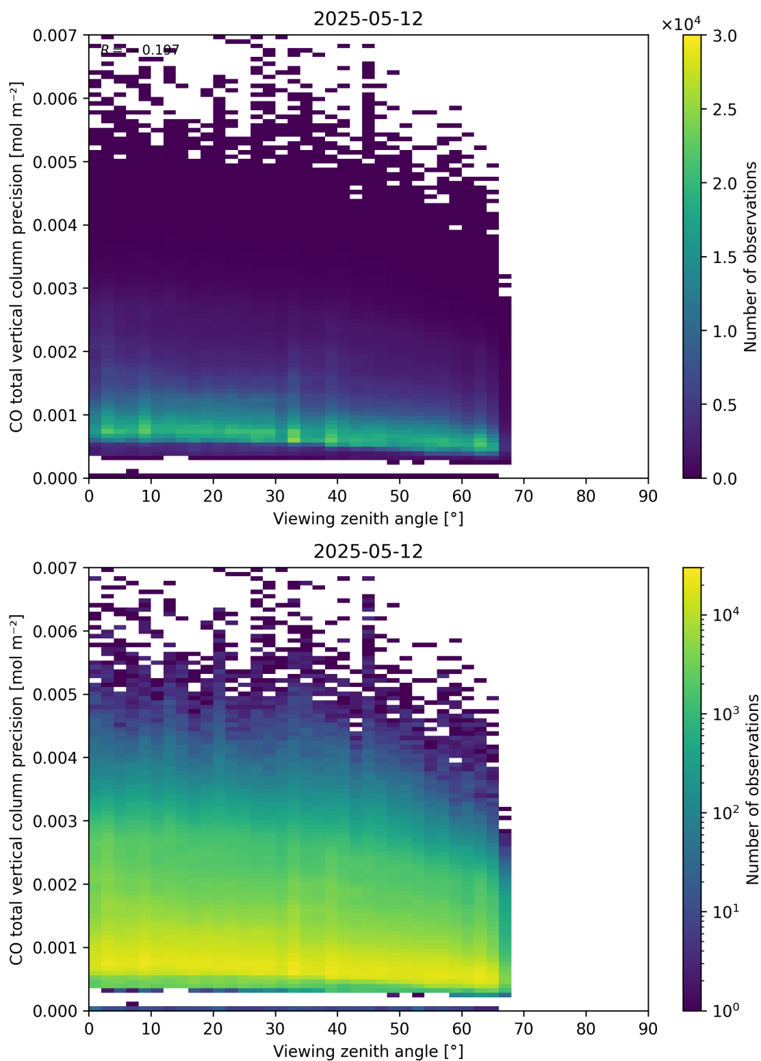
Figure 71: Scatter density plot of “Viewing zenith angle” against “CO total vertical column precision” for 2025-05-11 to 2025-05-13.
