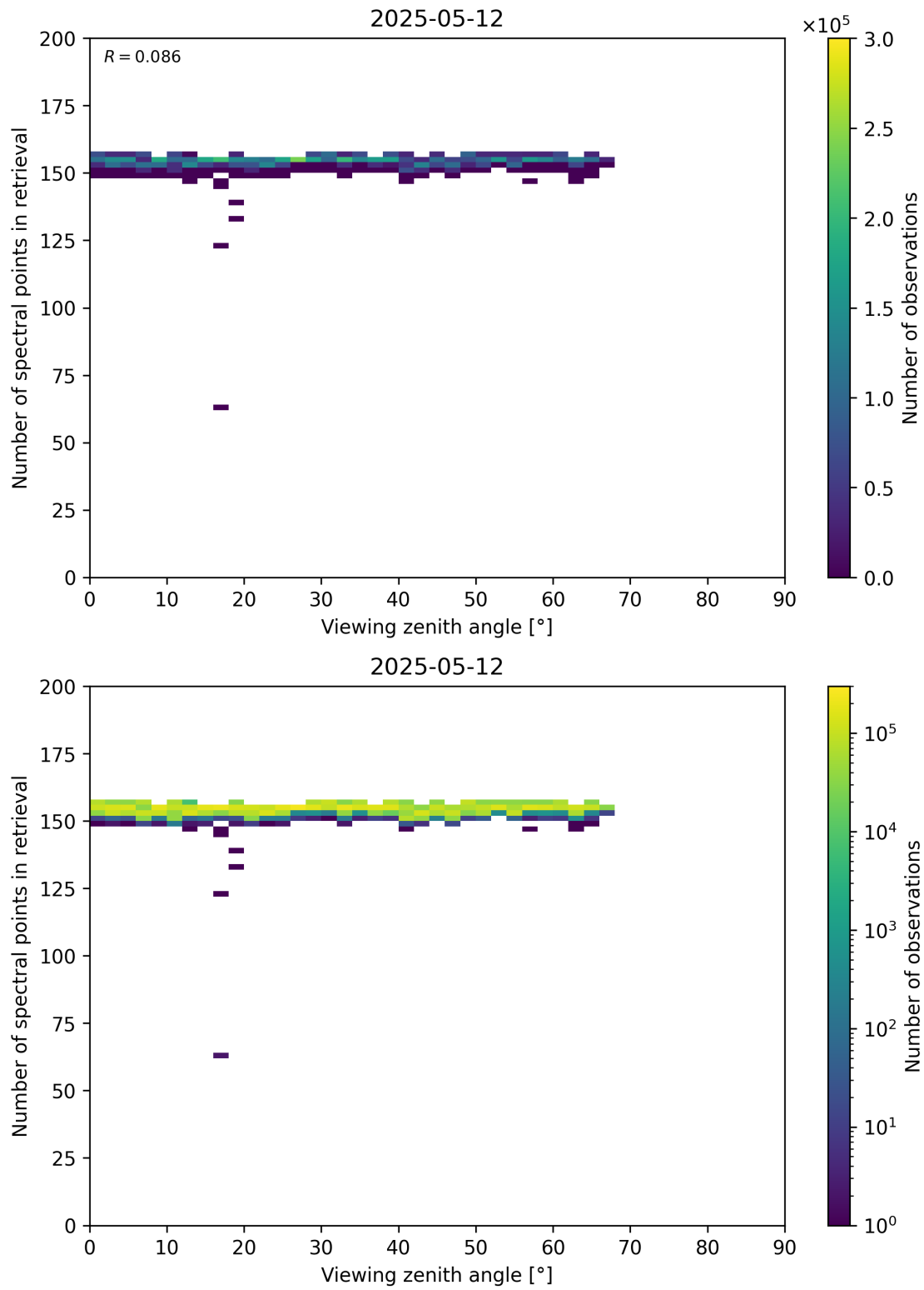
Figure 76: Scatter density plot of “Viewing zenith angle” against “Number of spectral points in retrieval” for 2025-05-11 to 2025-05-13.
