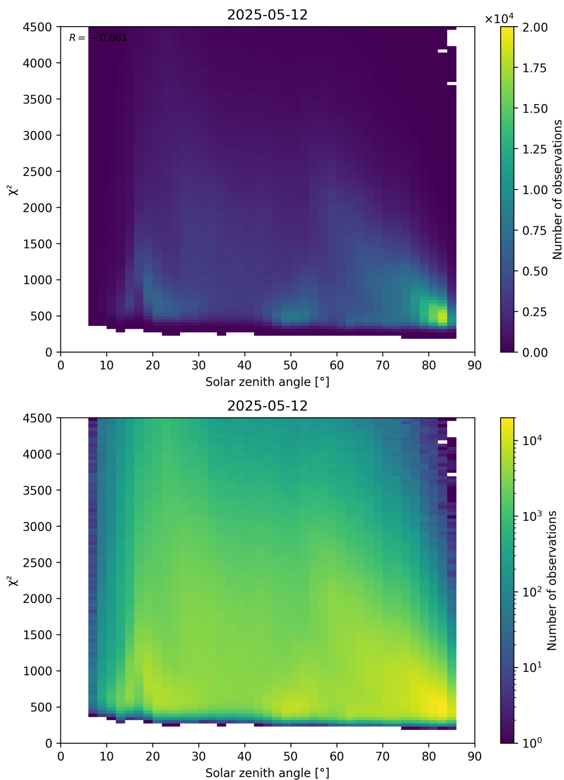
Figure 64: Scatter density plot of “Solar zenith angle” against “ \chi^2 ” for 2025-05-11 to 2025-05-13.
