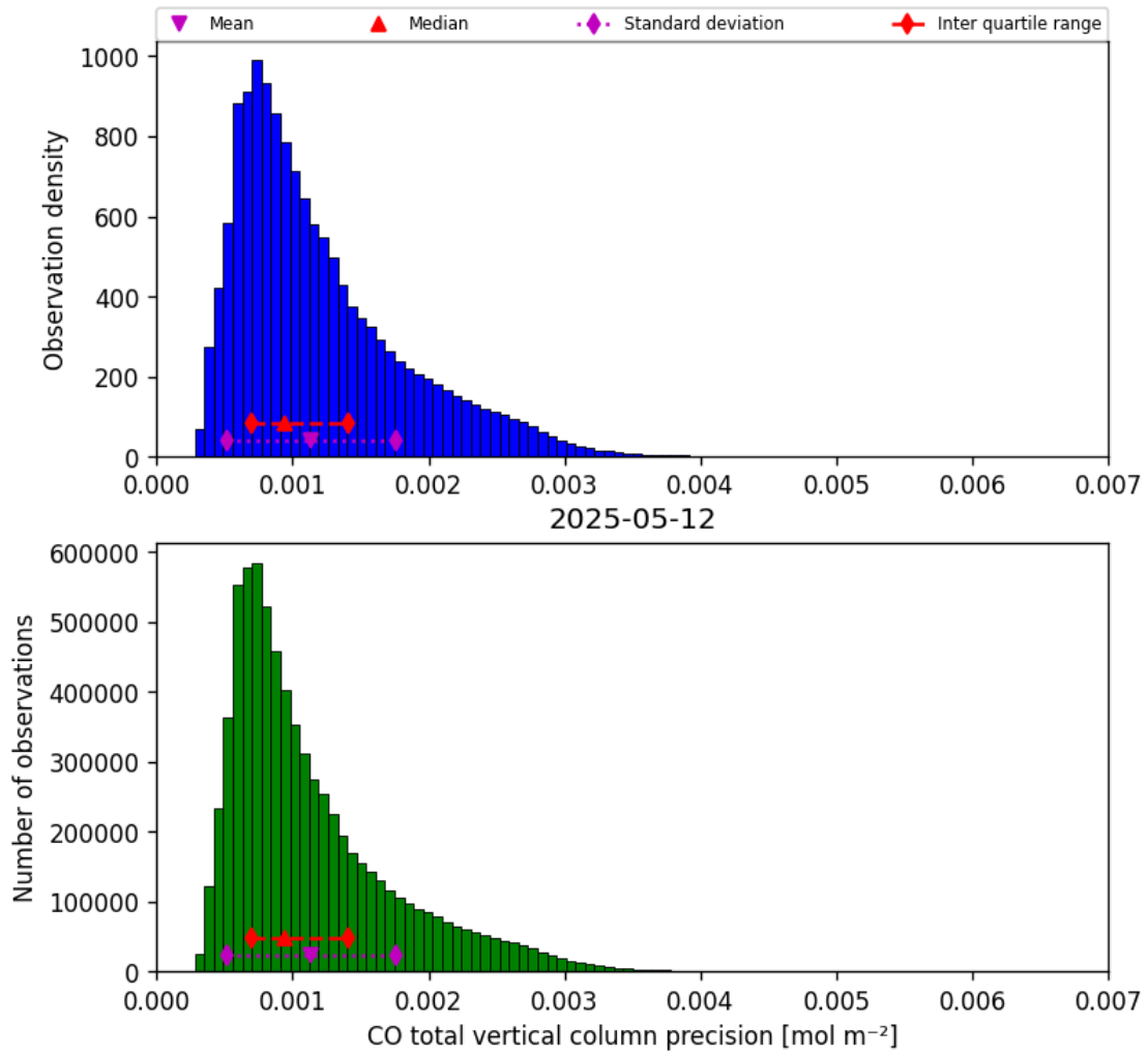
Figure 20: Histogram of “CO total vertical column precision” for 2025-05-11 to 2025-05-13
