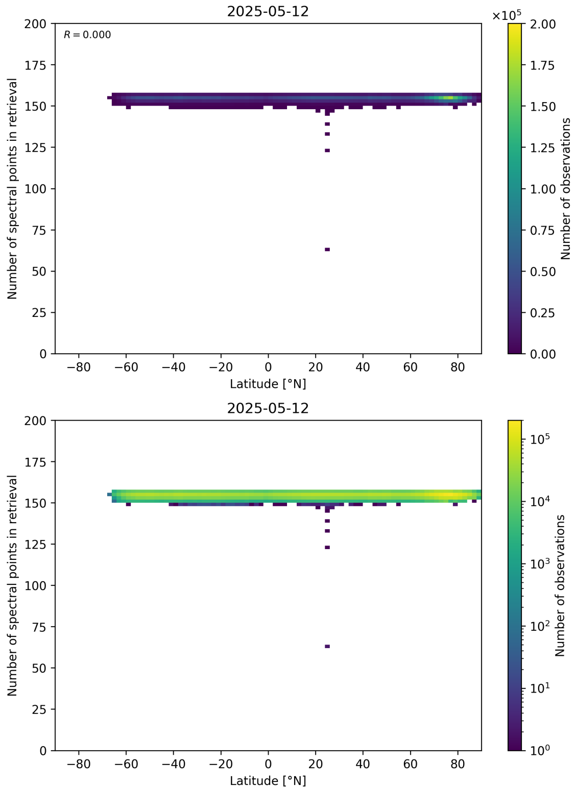
Figure 57: Scatter density plot of “Latitude” against “Number of spectral points in retrieval” for 2025-05-11 to 2025-05-13.
