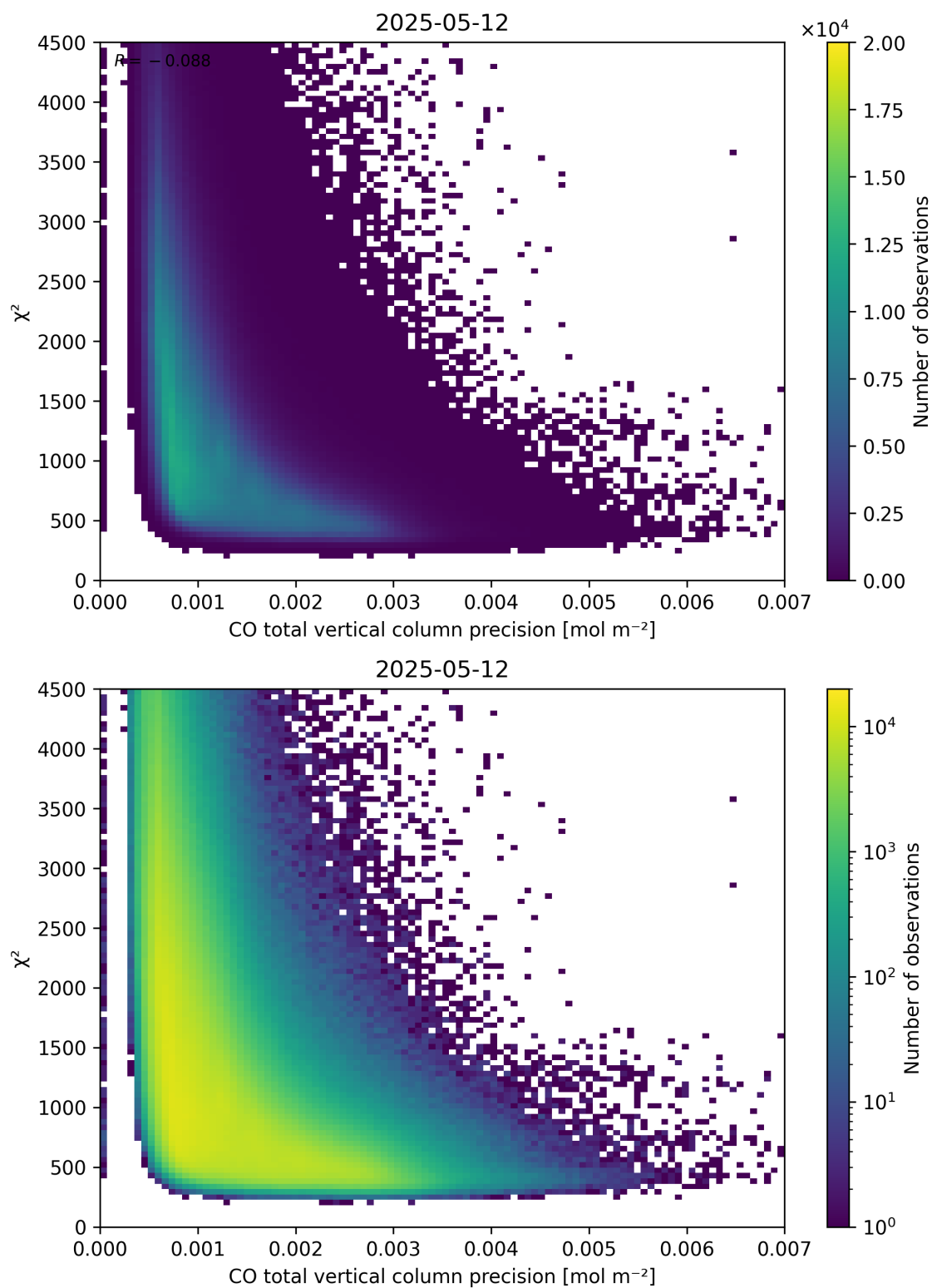
Figure 44: Scatter density plot of “CO total vertical column precision” against “ \chi^2 ” for 2025-05-11 to 2025-05-13.
