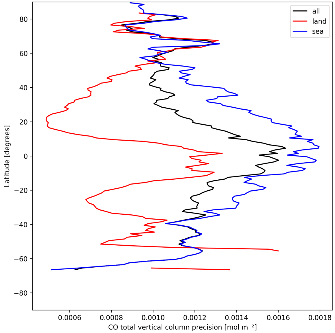
Figure 12: Zonal average of “CO total vertical column precision” for 2025-05-11 to 2025-05-13.
