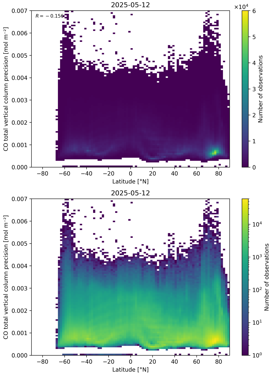
Figure 53: Scatter density plot of “Latitude” against “CO total vertical column precision” for 2025-05-11 to 2025-05-13.
