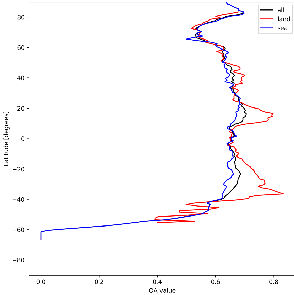
Figure 9: Zonal average of “QA value” for 2025-05-11 to 2025-05-13.
