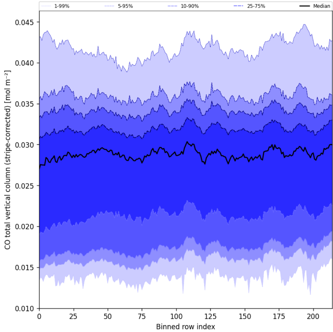
Figure 27: Along track statistics of “CO total vertical column (stripe-corrected)” for 2025-05-11 to 2025-05-13
