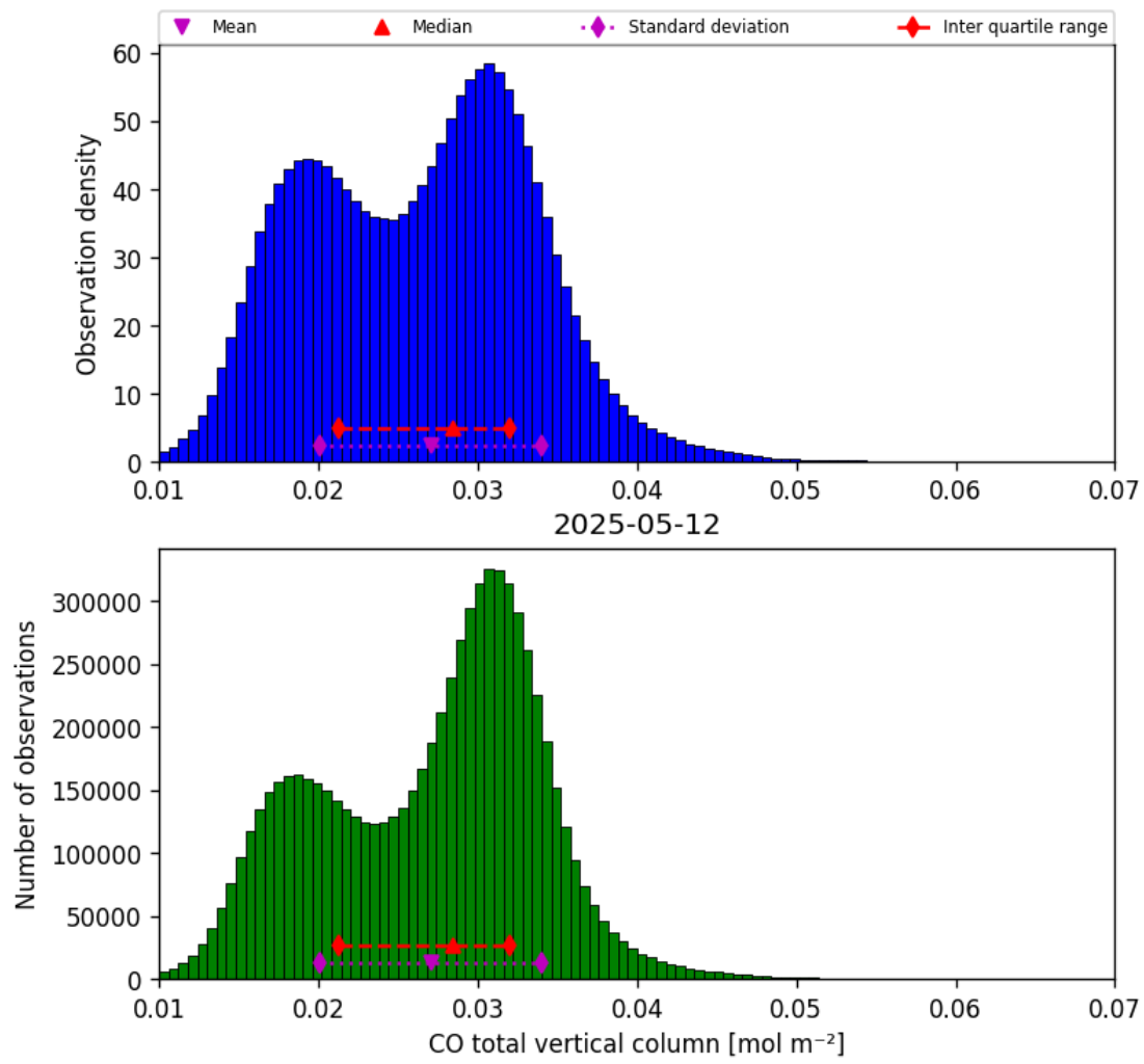
Figure 18: Histogram of “CO total vertical column” for 2025-05-11 to 2025-05-13
