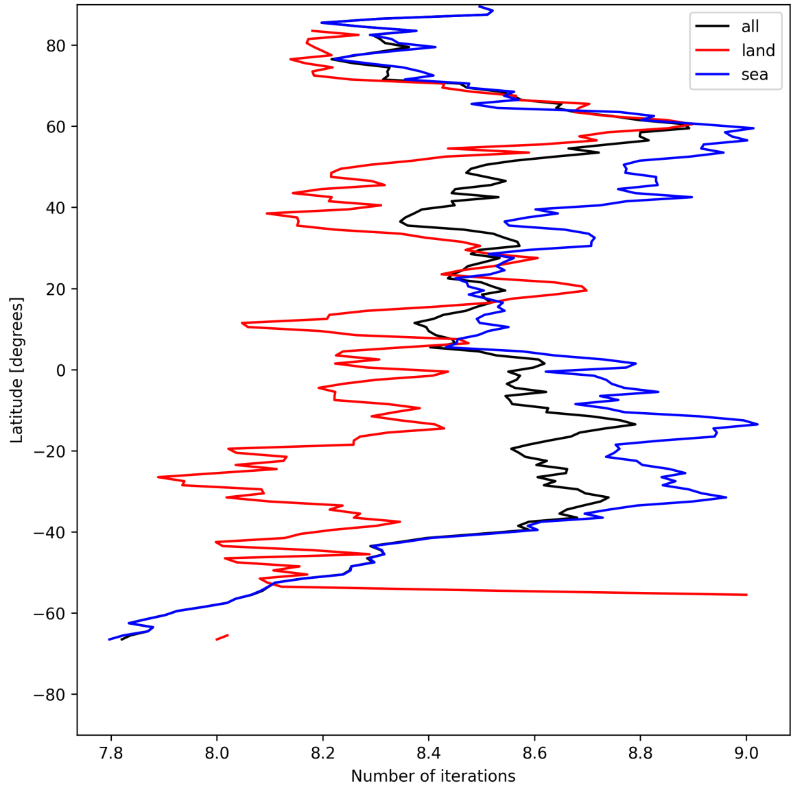
Figure 16: Zonal average of “Number of iterations” for 2025-05-11 to 2025-05-13.
