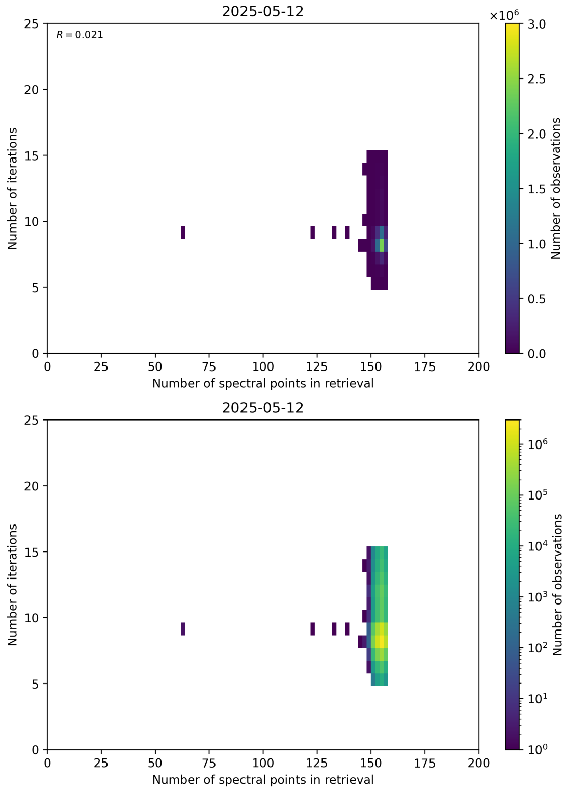
Figure 60: Scatter density plot of “Number of spectral points in retrieval” against “Number of iterations” for 2025-05-11 to 2025-05-13.
