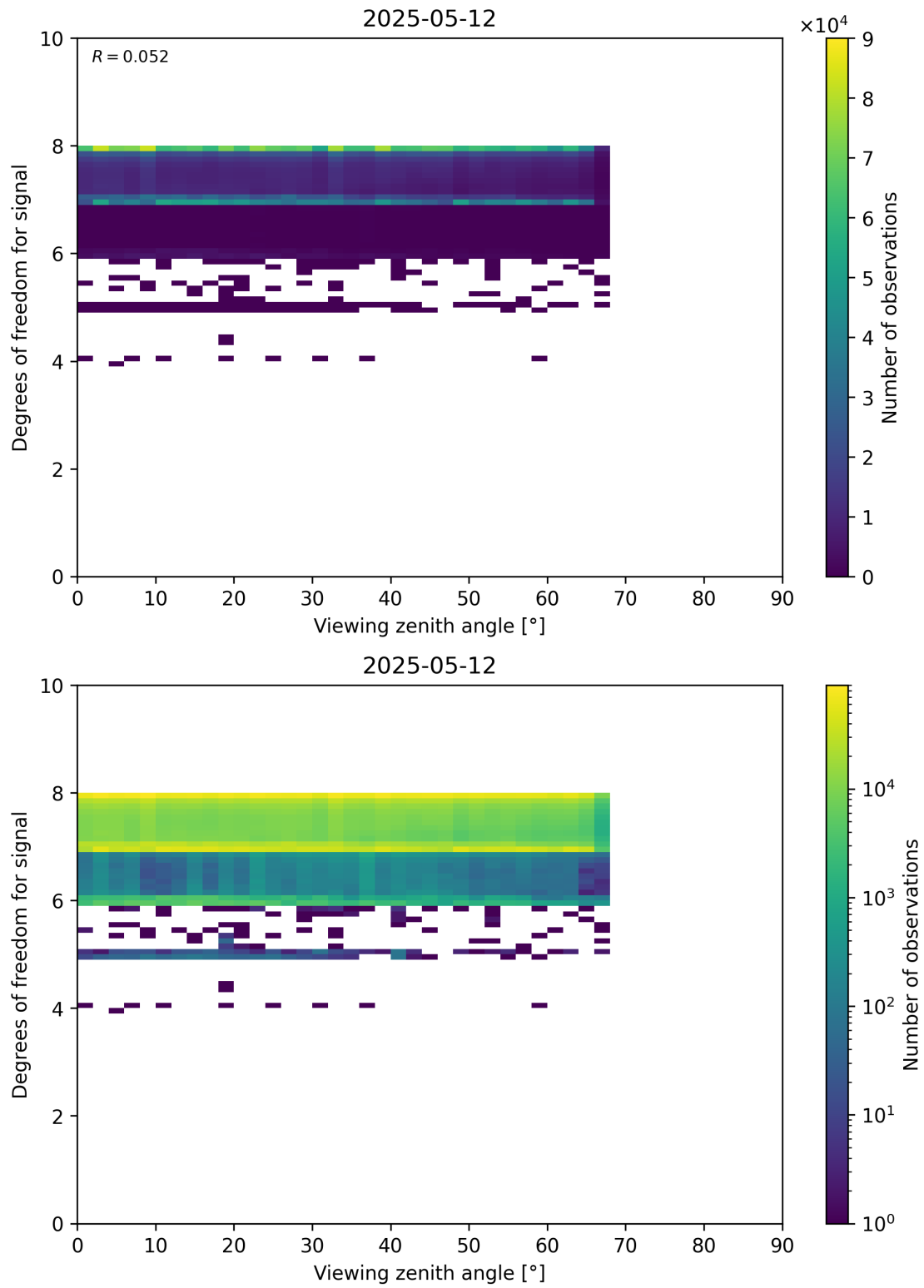
Figure 73: Scatter density plot of “Viewing zenith angle” against “Degrees of freedom for signal” for 2025-05-11 to 2025-05-13.
