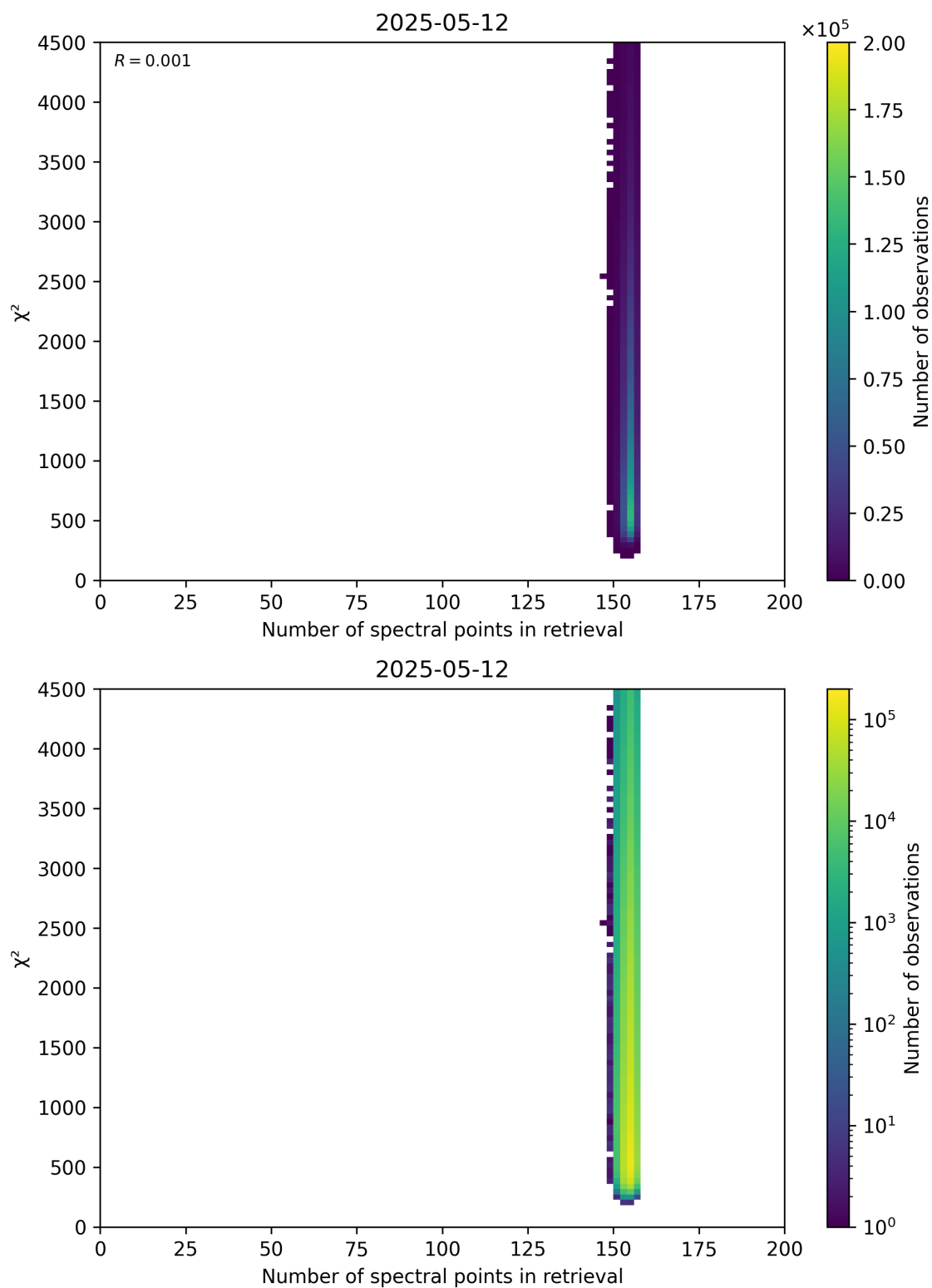
Figure 58: Scatter density plot of “Number of spectral points in retrieval” against “ \chi^2 ” for 2025-05-11 to 2025-05-13.
