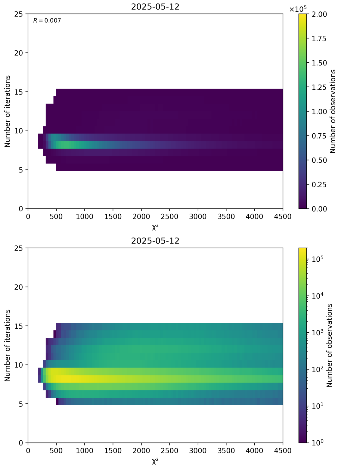
Figure 49: Scatter density plot of “ \chi^2 ” against “Number of iterations” for 2025-05-11 to 2025-05-13.
