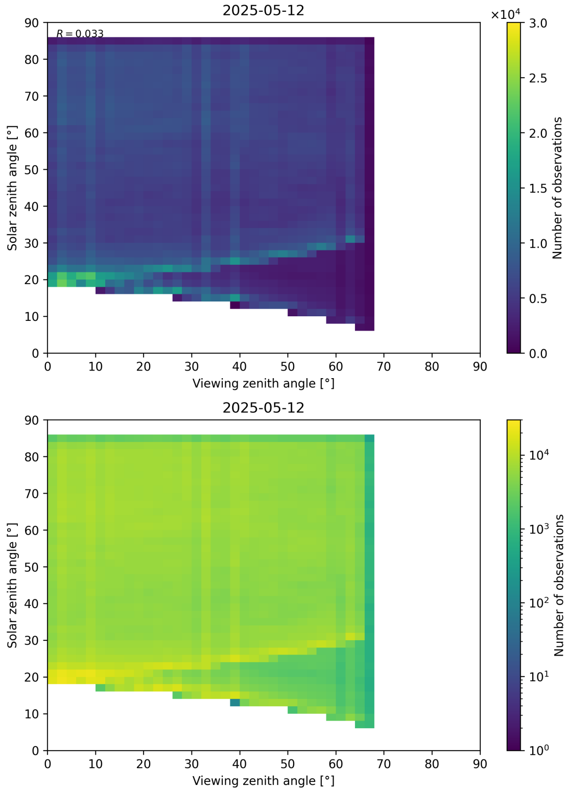
Figure 77: Scatter density plot of “Viewing zenith angle” against “Solar zenith angle” for 2025-05-11 to 2025-05-13.
