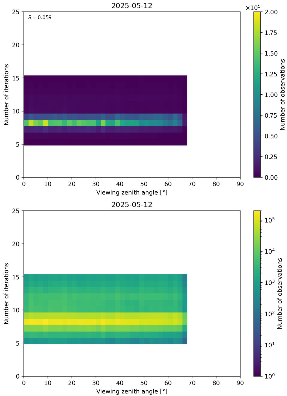
Figure 75: Scatter density plot of “Viewing zenith angle” against “Number of iterations” for 2025-05-11 to 2025-05-13.
