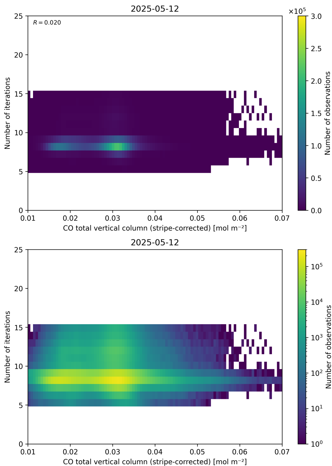
Figure 39: Scatter density plot of “CO total vertical column (stripe-corrected)” against “Number of iterations” for 2025-05-11 to 2025-05-13.
