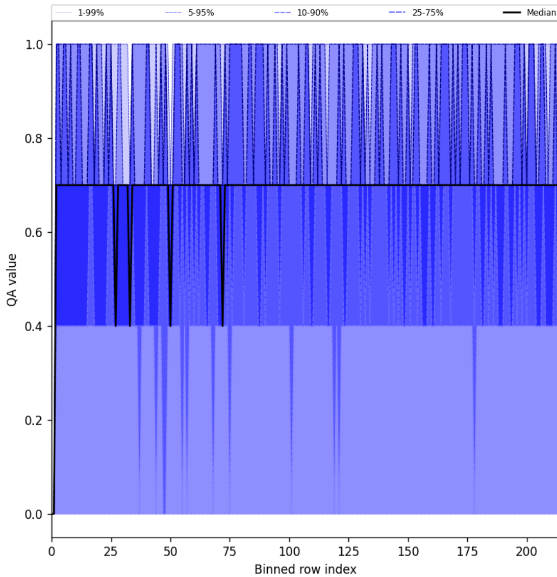
Figure 25: Along track statistics of “QA value” for 2025-05-11 to 2025-05-13
