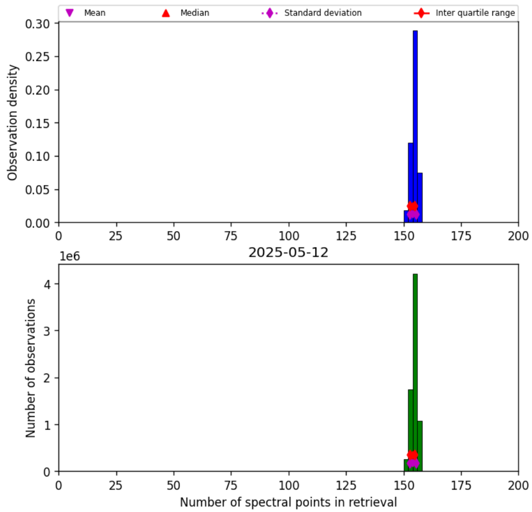
Figure 21: Histogram of “Number of spectral points in retrieval” for 2025-05-11 to 2025-05-13
