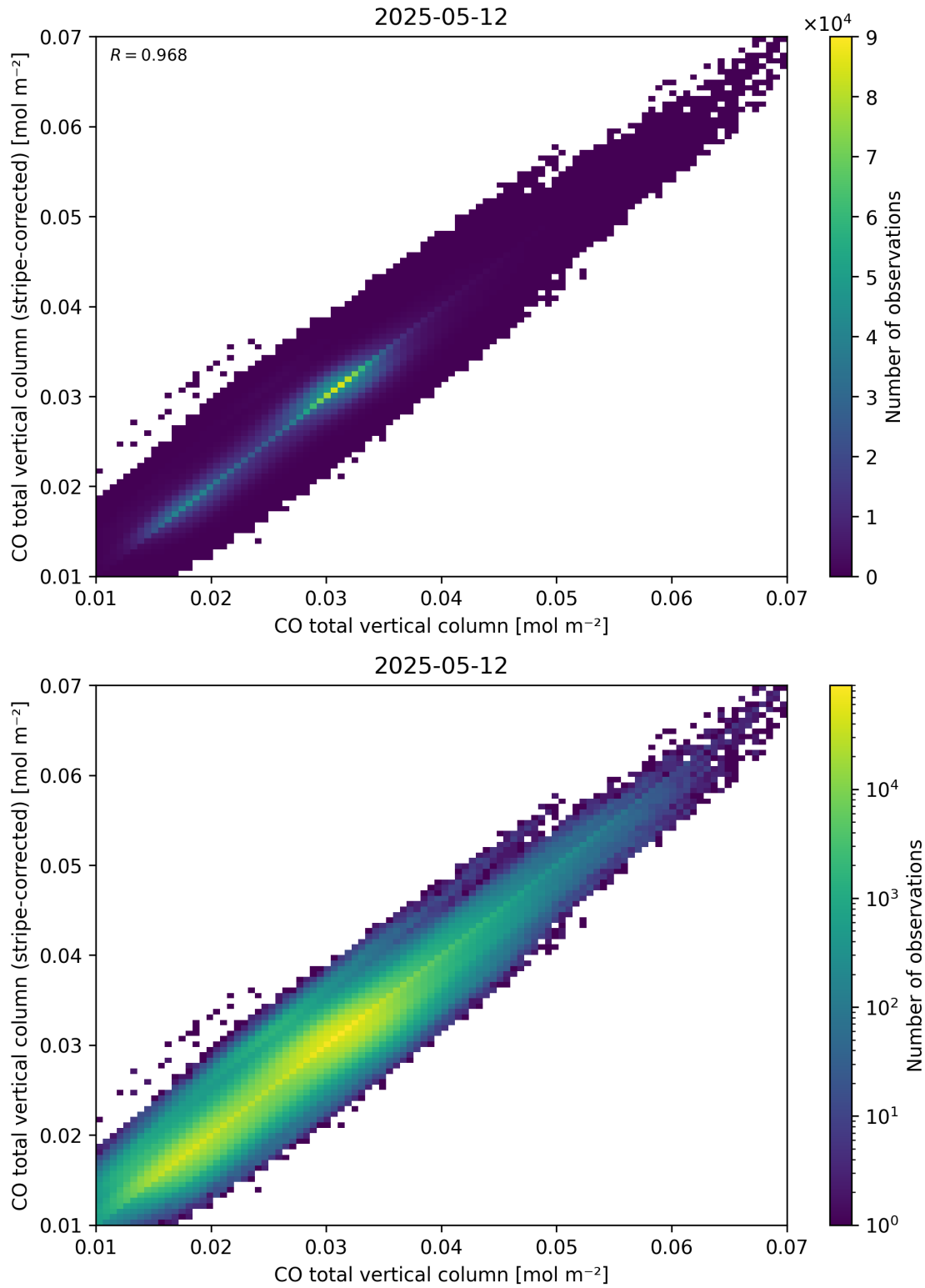
Figure 33: Scatter density plot of “CO total vertical column” against “CO total vertical column (stripe-corrected)” for 2025-05-11 to 2025-05-13.
