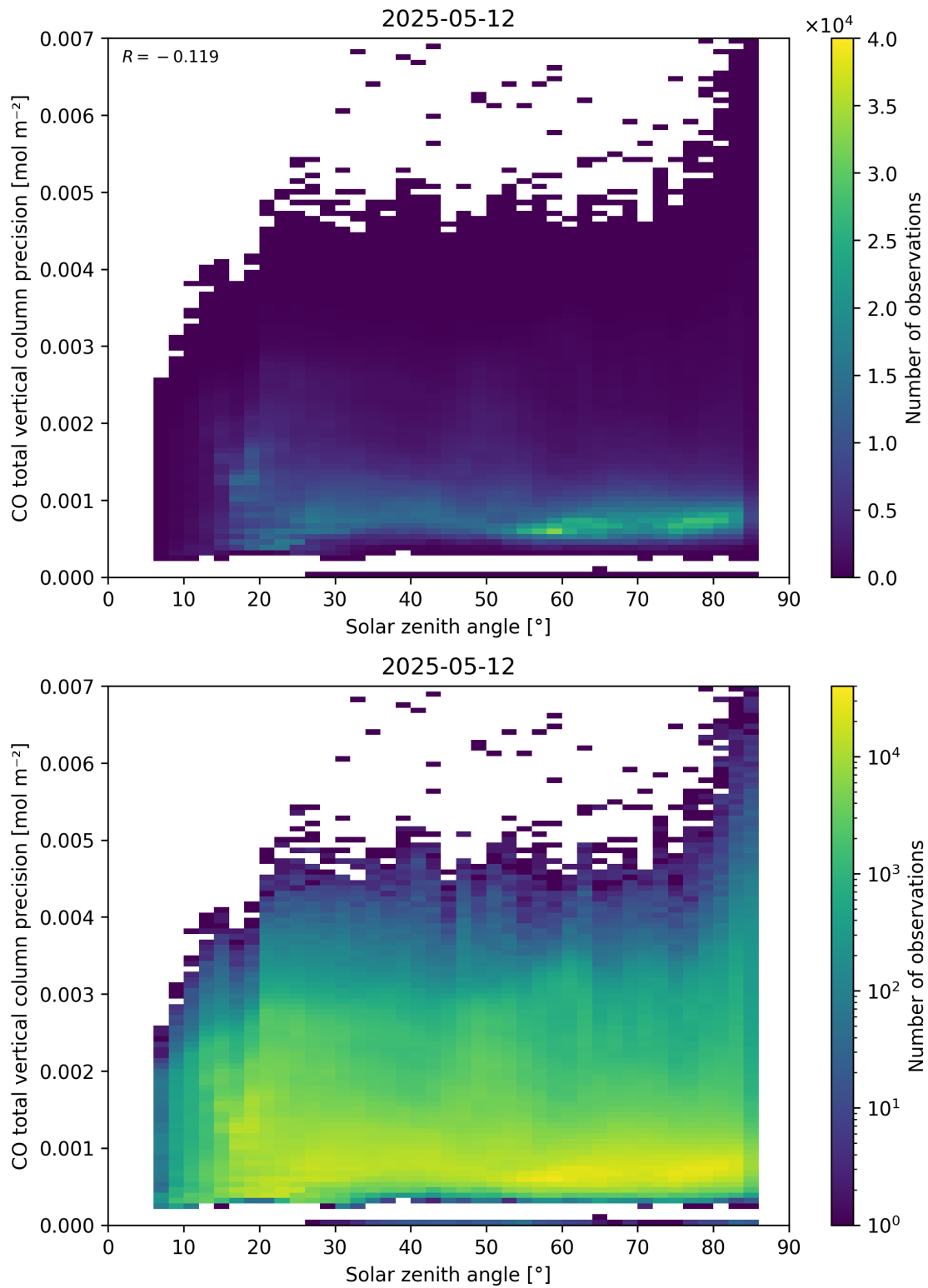
Figure 63: Scatter density plot of “Solar zenith angle” against “CO total vertical column precision” for 2025-05-11 to 2025-05-13.
