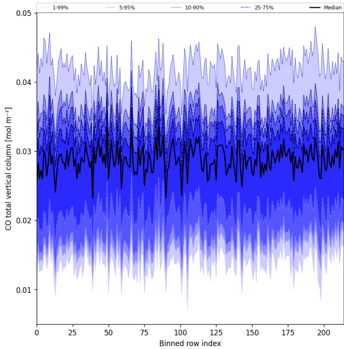
Figure 26: Along track statistics of “CO total vertical column” for 2025-05-11 to 2025-05-13
