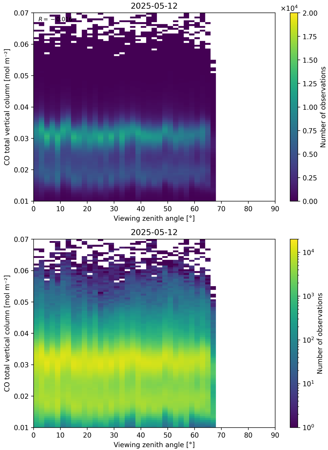
Figure 69: Scatter density plot of “Viewing zenith angle” against “CO total vertical column” for 2025-05-11 to 2025-05-13.
