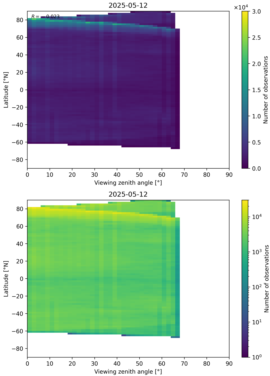
Figure 74: Scatter density plot of “Viewing zenith angle” against “Latitude” for 2025-05-11 to 2025-05-13.
