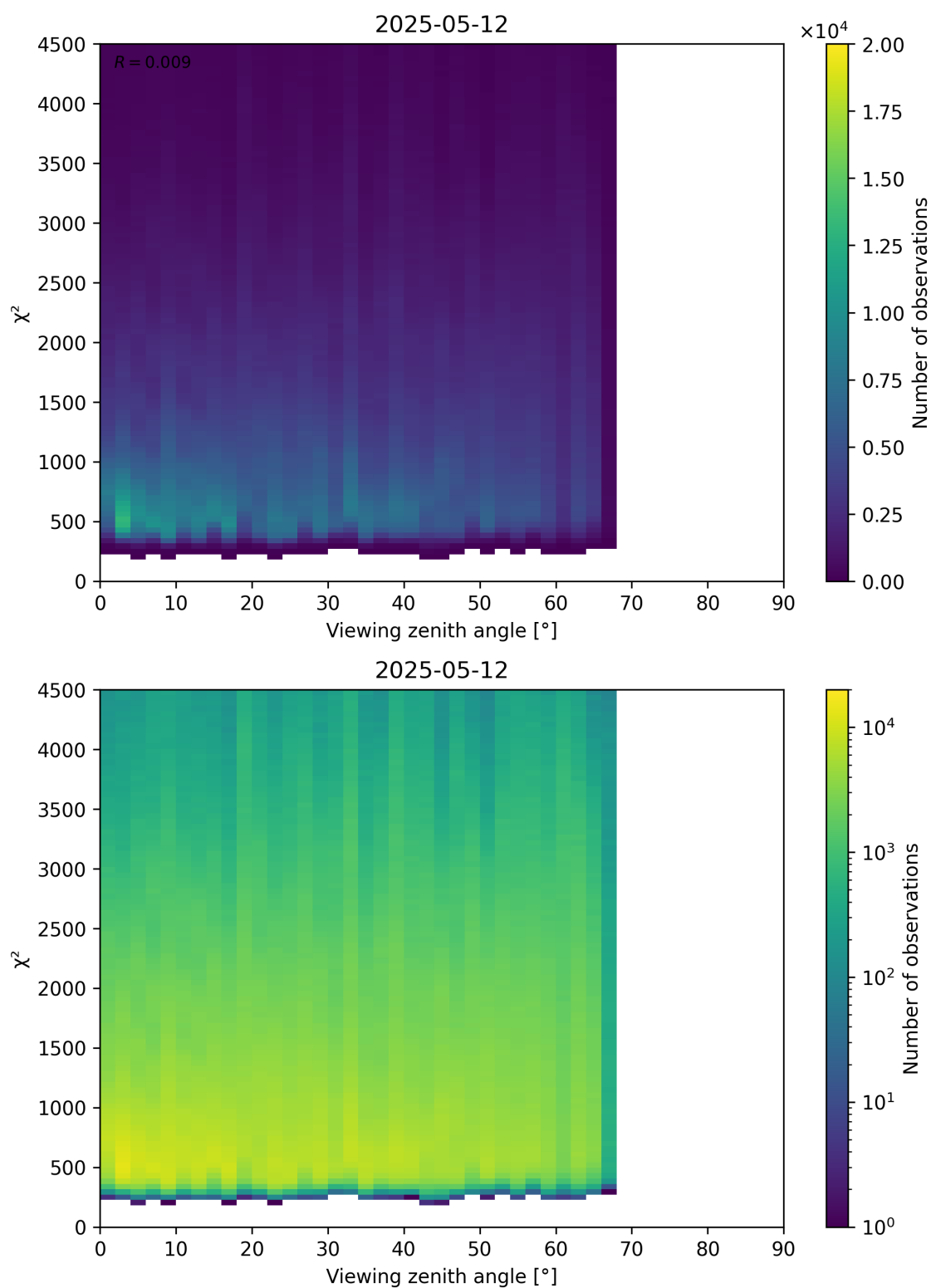
Figure 72: Scatter density plot of “Viewing zenith angle” against “ \chi^2 ” for 2025-05-11 to 2025-05-13.
