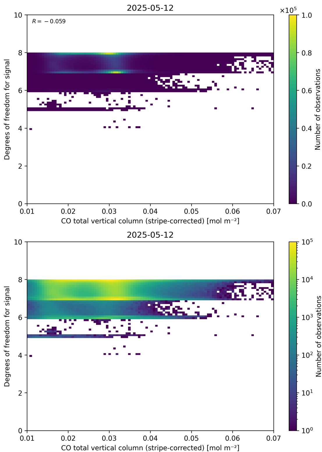
Figure 38: Scatter density plot of “CO total vertical column (stripe-corrected)” against “Degrees of freedom for signal” for 2025-05-11 to 2025-05-13.
