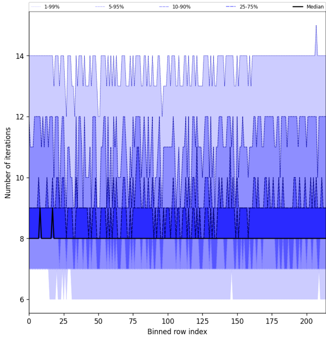
Figure 32: Along track statistics of “Number of iterations” for 2025-05-11 to 2025-05-13
