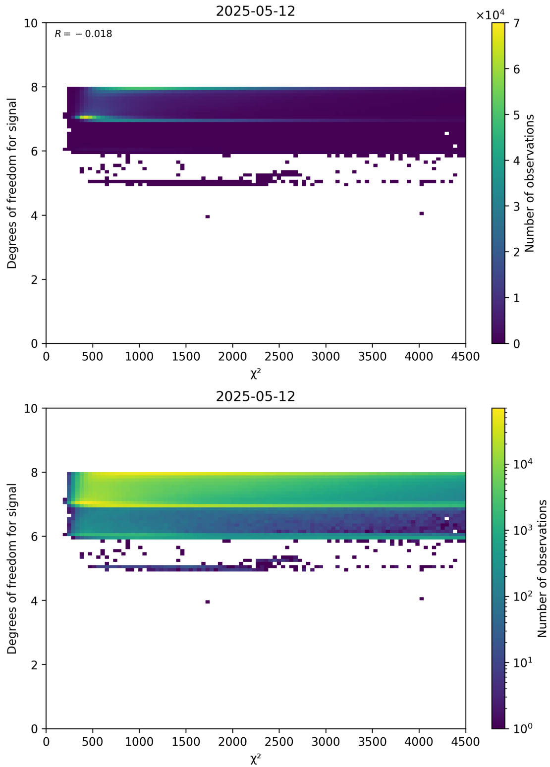
Figure 48: Scatter density plot of “ \chi^2 ” against “Degrees of freedom for signal” for 2025-05-11 to 2025-05-13.
