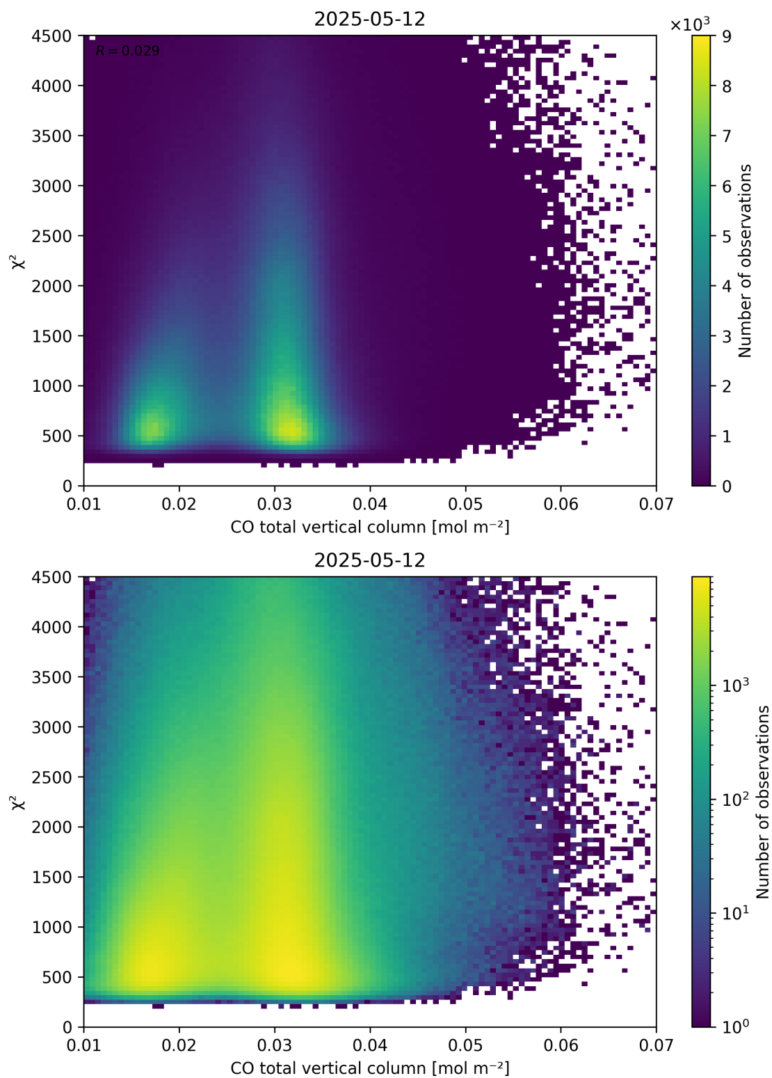
Figure 35: Scatter density plot of “CO total vertical column” against “ \chi^2 ” for 2025-05-11 to 2025-05-13.
