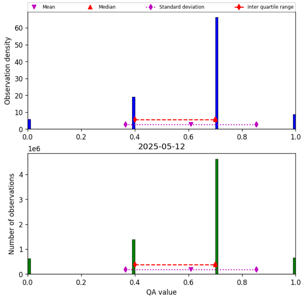
Figure 17: Histogram of “QA value” for 2025-05-11 to 2025-05-13
