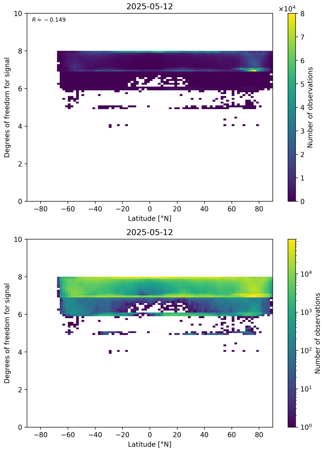
Figure 55: Scatter density plot of “Latitude” against “Degrees of freedom for signal” for 2025-05-11 to 2025-05-13.
