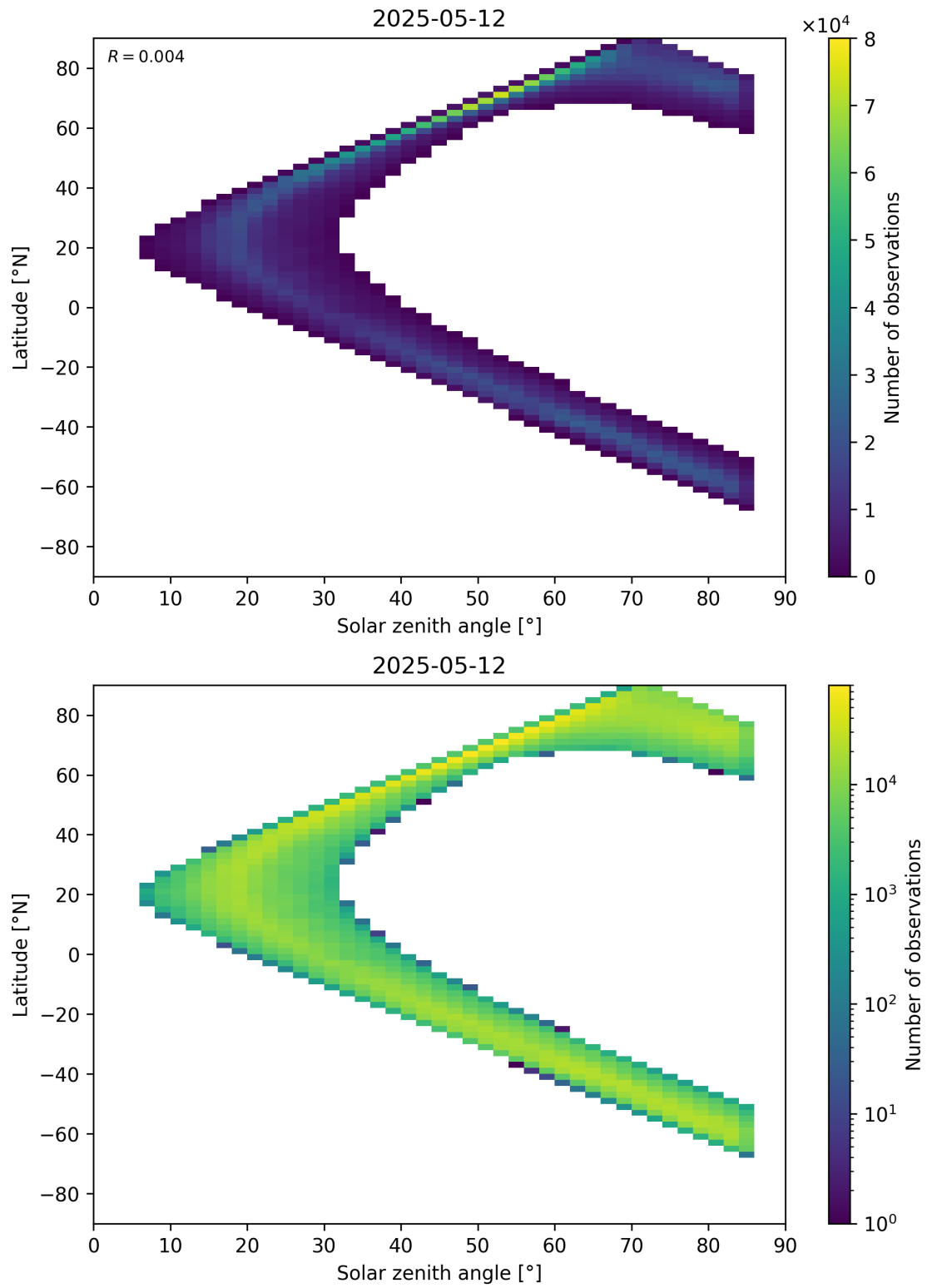
Figure 66: Scatter density plot of “Solar zenith angle” against “Latitude” for 2025-05-11 to 2025-05-13.
