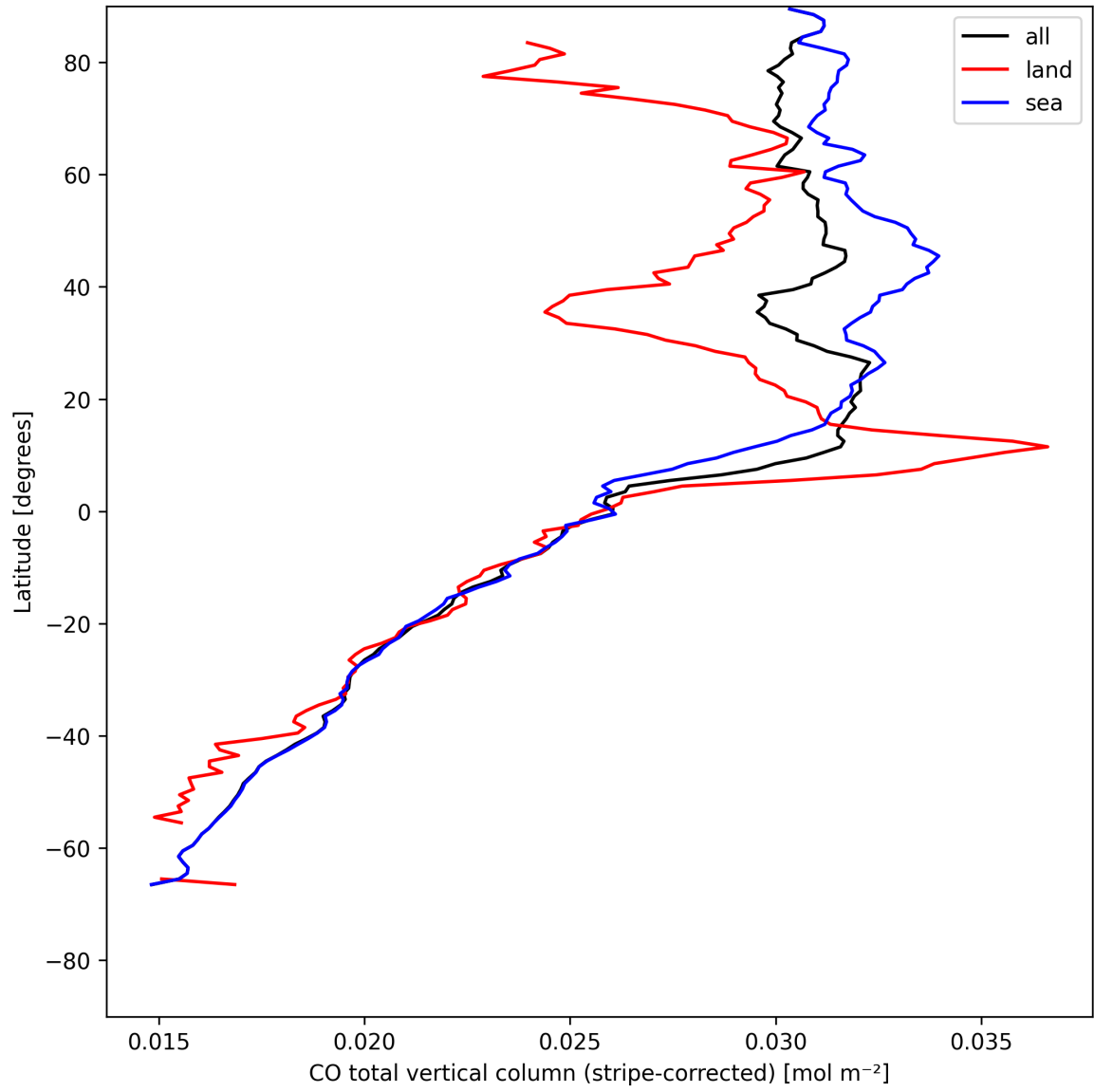
Figure 11: Zonal average of “CO total vertical column (stripe-corrected)” for 2025-05-11 to 2025-05-13.
