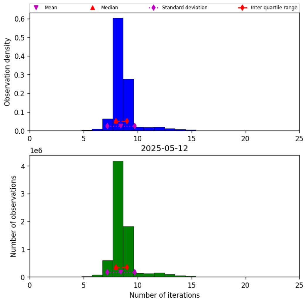
Figure 24: Histogram of “Number of iterations” for 2025-05-11 to 2025-05-13
