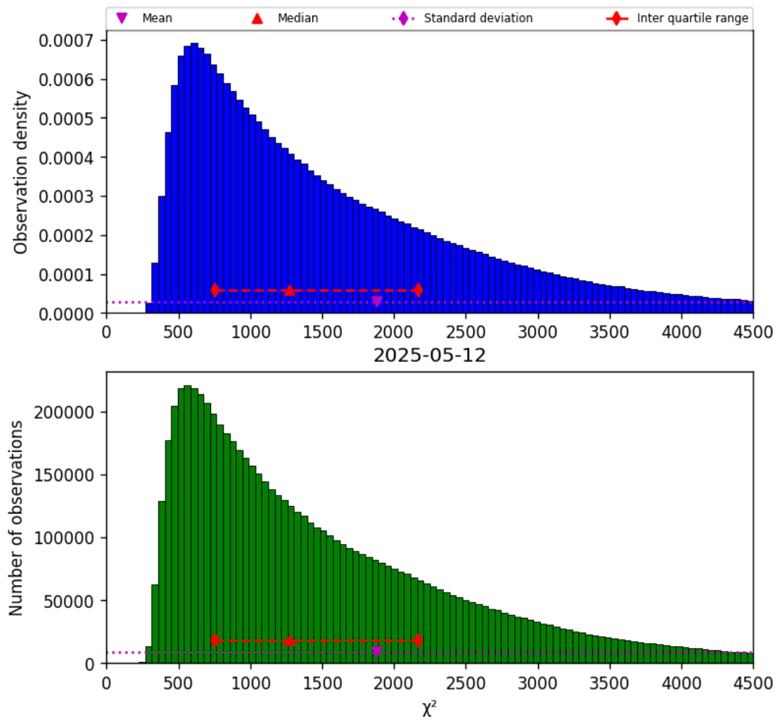
Figure 22: Histogram of “ \chi^2 ” for 2025-05-11 to 2025-05-13
