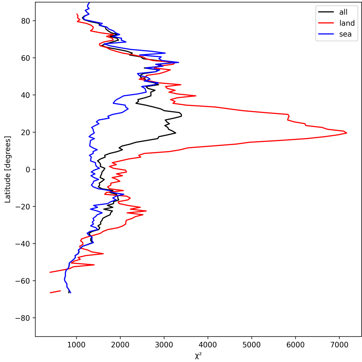
Figure 14: Zonal average of “ \chi^2 ” for 2025-05-11 to 2025-05-13.
