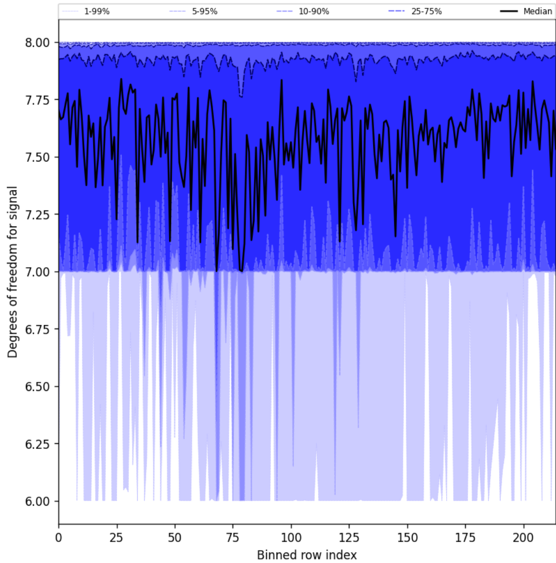
Figure 31: Along track statistics of “Degrees of freedom for signal” for 2025-05-11 to 2025-05-13
