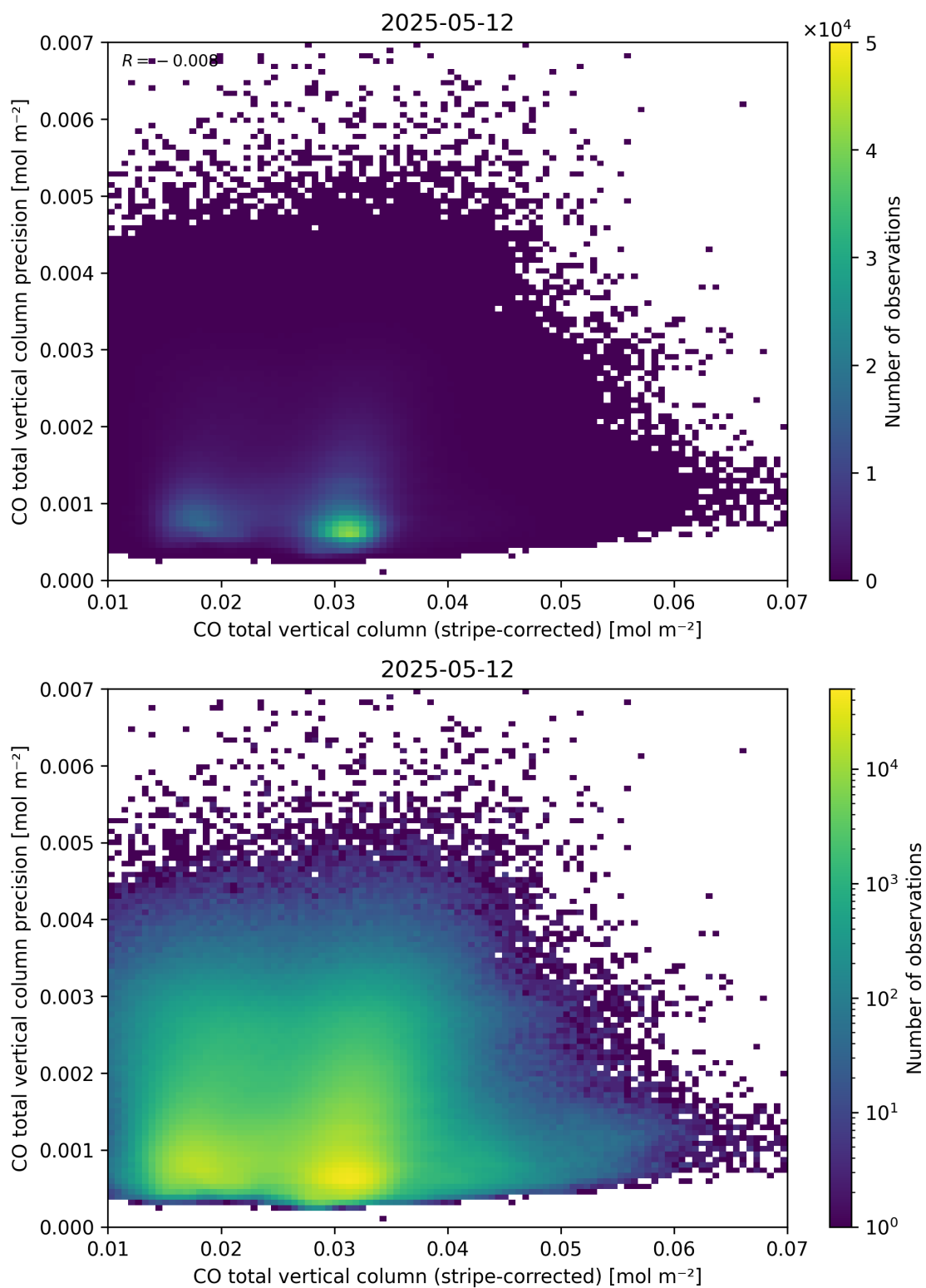
Figure 36: Scatter density plot of “CO total vertical column (stripe-corrected)” against “CO total vertical column precision” for 2025-05-11 to 2025-05-13.
