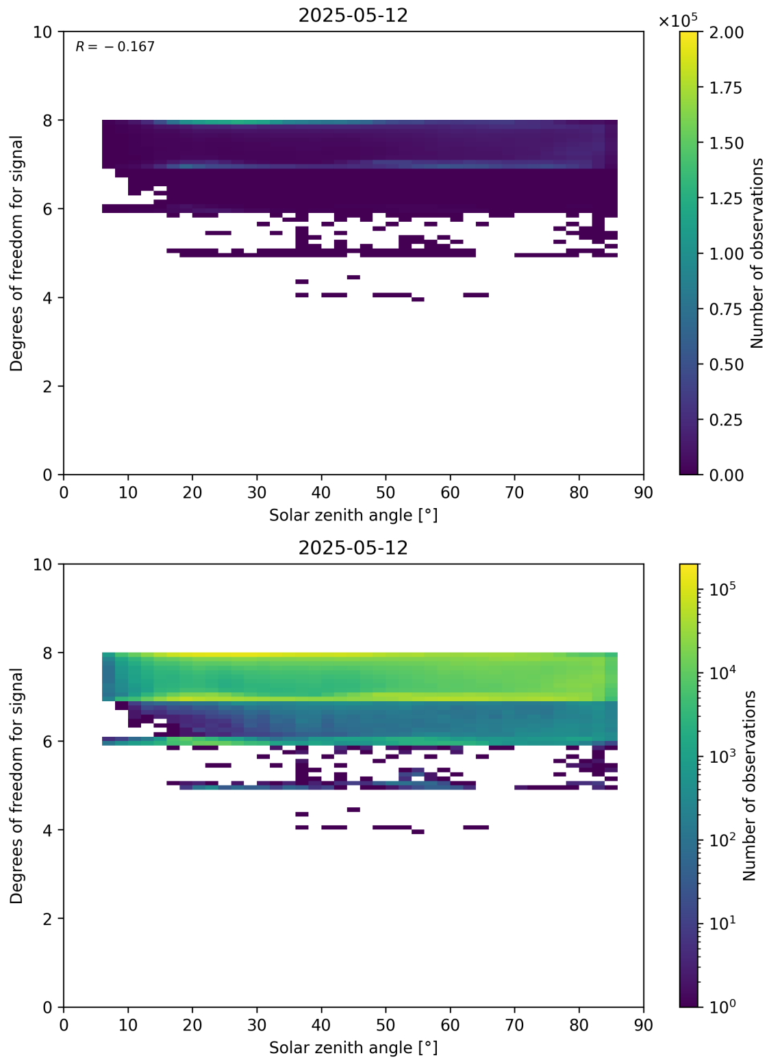
Figure 65: Scatter density plot of “Solar zenith angle” against “Degrees of freedom for signal” for 2025-05-11 to 2025-05-13.
