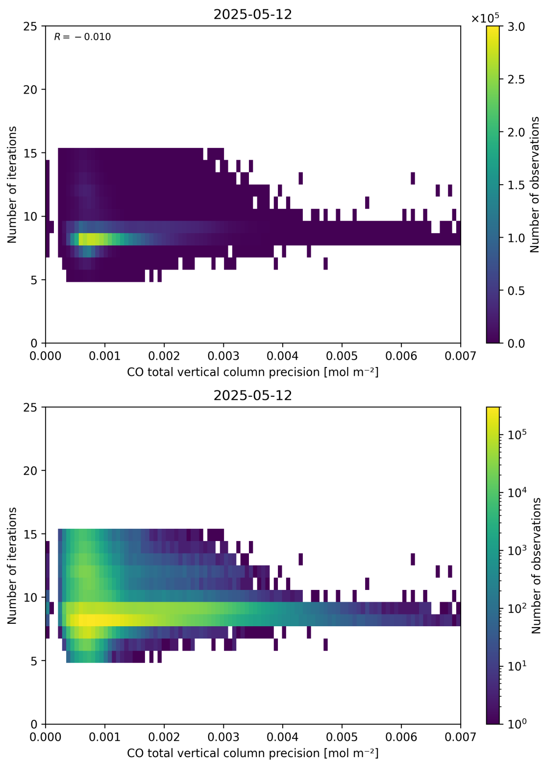
Figure 46: Scatter density plot of “CO total vertical column precision” against “Number of iterations” for 2025-05-11 to 2025-05-13.
