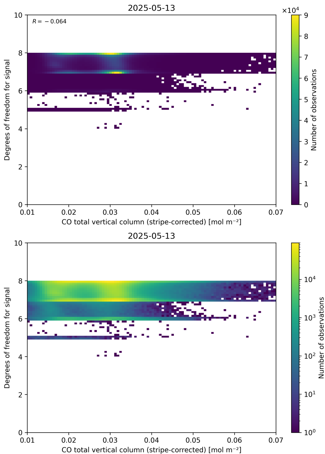
Figure 38: Scatter density plot of “CO total vertical column (stripe-corrected)” against “Degrees of freedom for signal” for 2025-05-12 to 2025-05-14.
