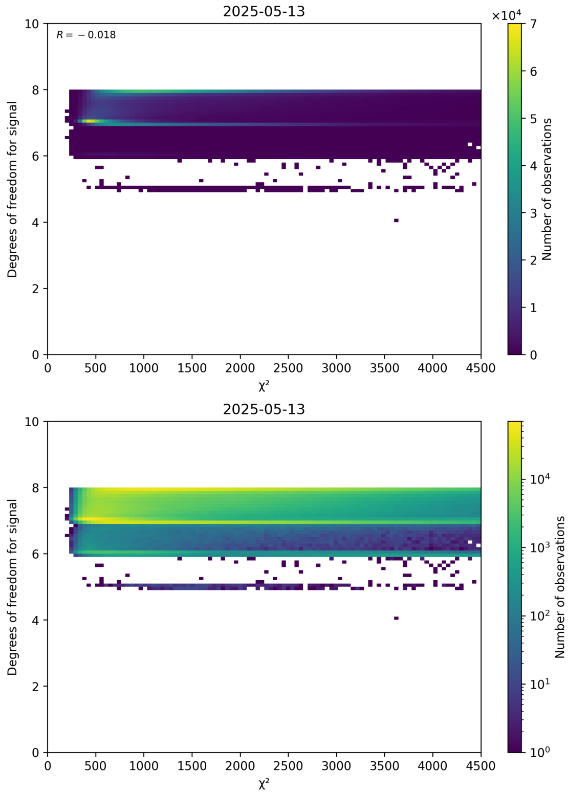
Figure 48: Scatter density plot of “ \chi^2 ” against “Degrees of freedom for signal” for 2025-05-12 to 2025-05-14.
