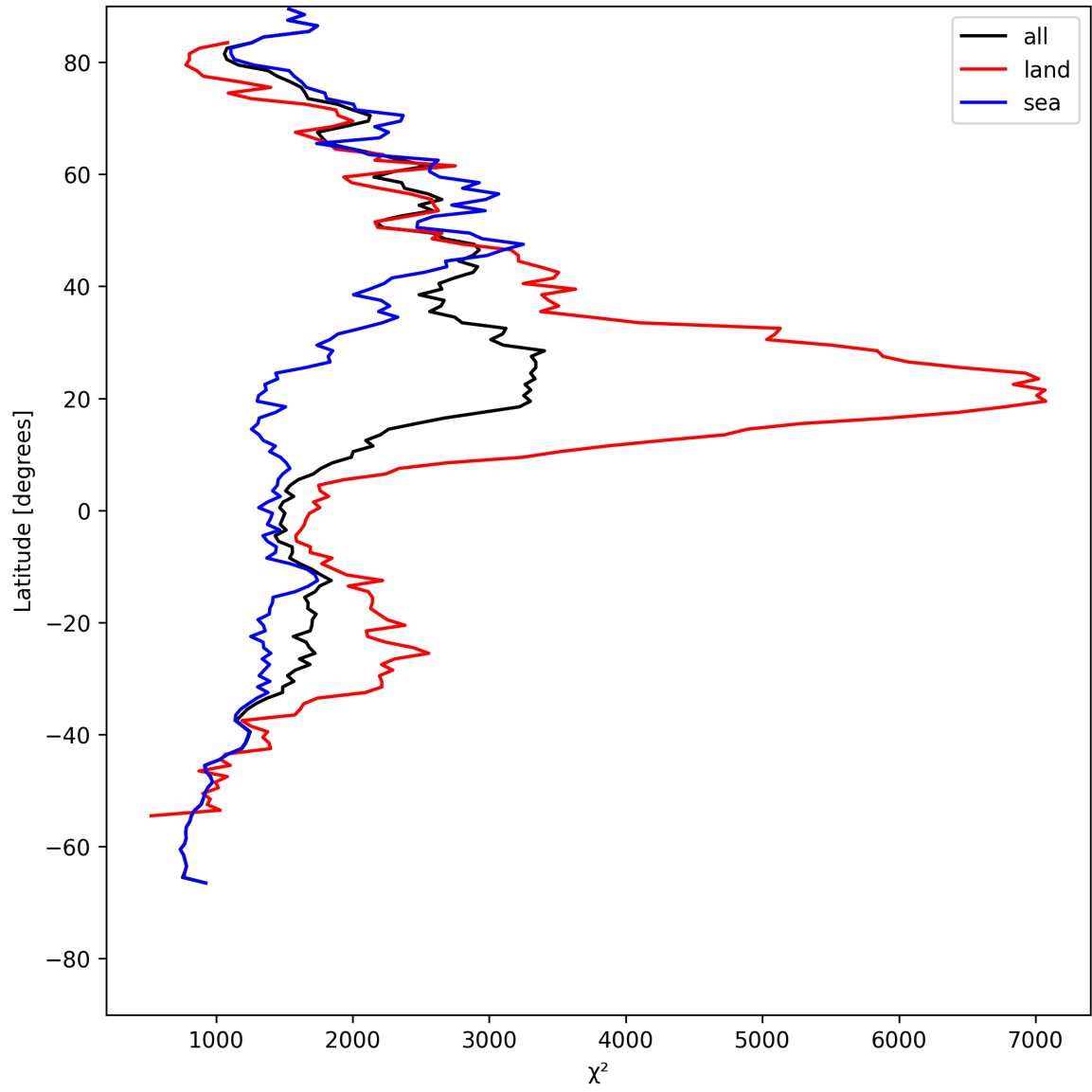
Figure 14: Zonal average of “ \chi^2 ” for 2025-05-12 to 2025-05-14.
