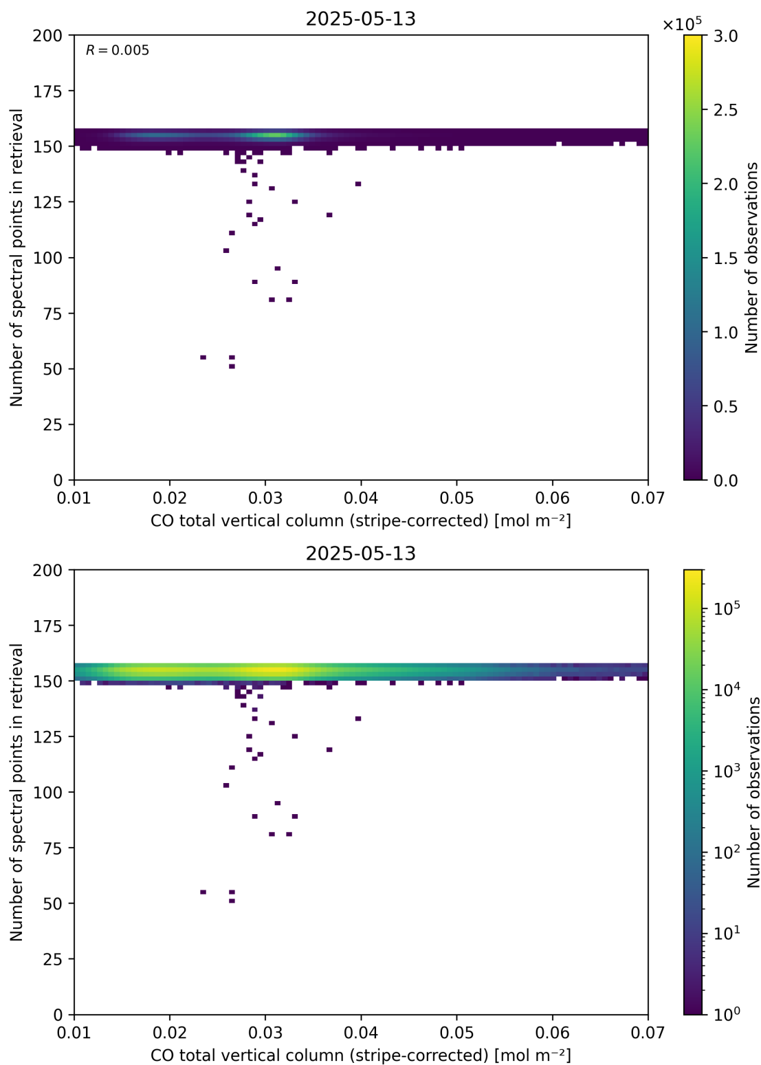
Figure 40: Scatter density plot of “CO total vertical column (stripe-corrected)” against “Number of spectral points in retrieval” for 2025-05-12 to 2025-05-14.
