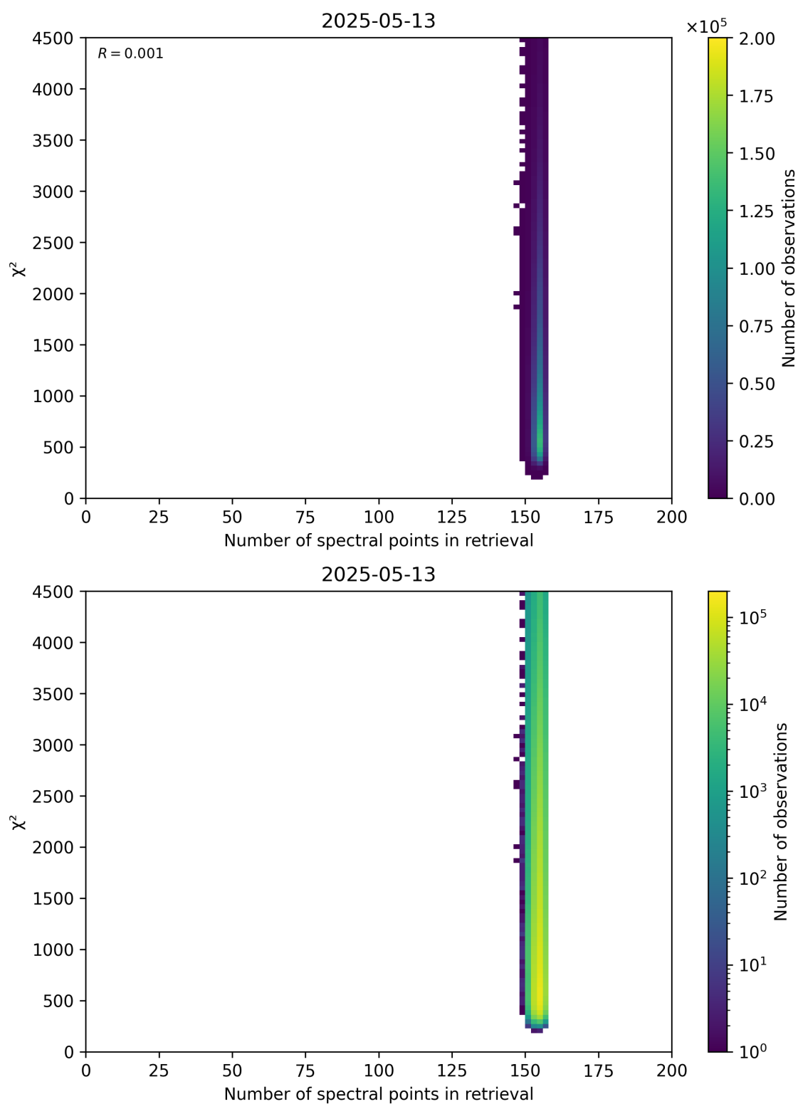
Figure 58: Scatter density plot of “Number of spectral points in retrieval” against “ \chi^2 ” for 2025-05-12 to 2025-05-14.
