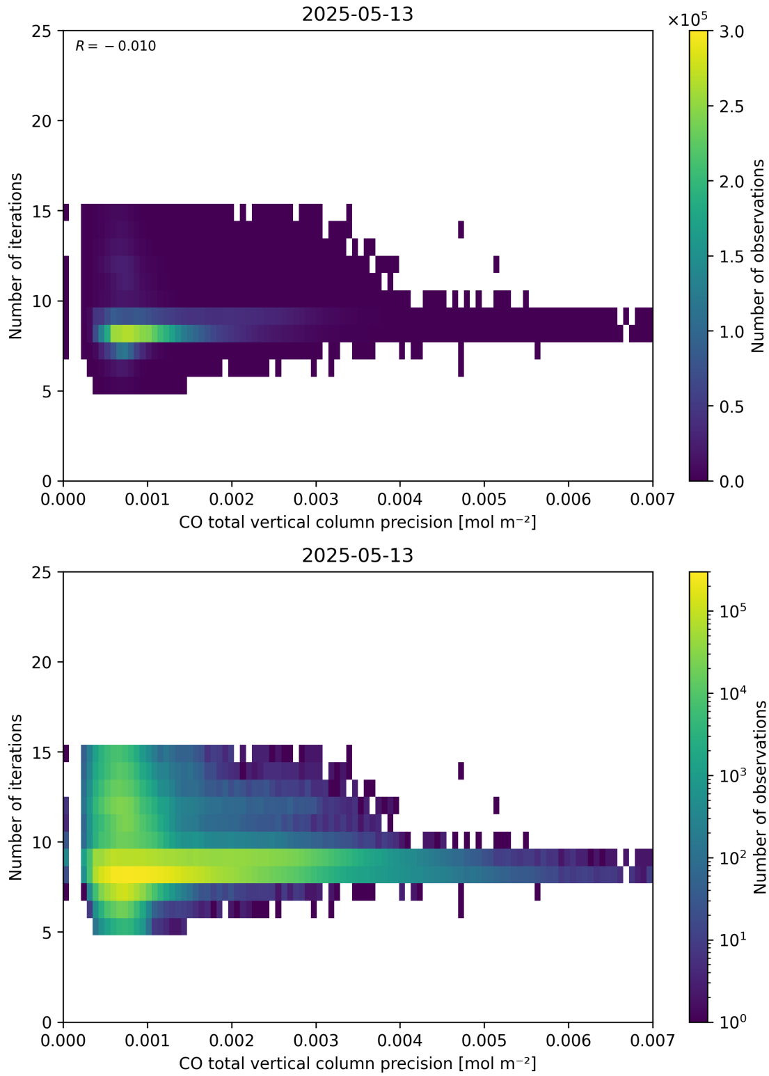
Figure 46: Scatter density plot of “CO total vertical column precision” against “Number of iterations” for 2025-05-12 to 2025-05-14.
