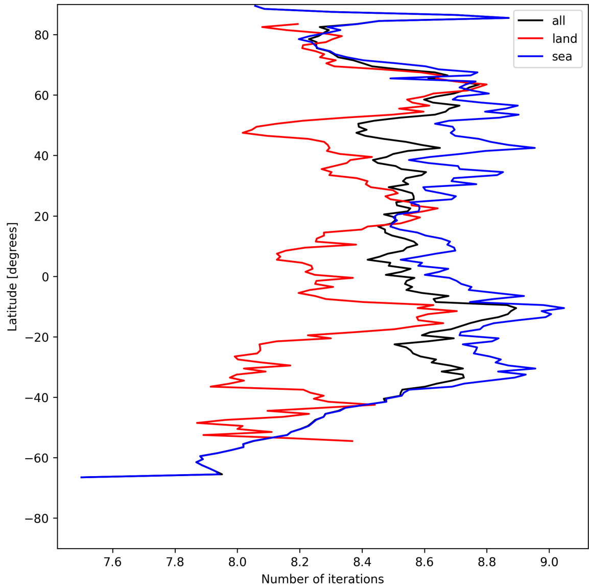
Figure 16: Zonal average of “Number of iterations” for 2025-05-12 to 2025-05-14.
