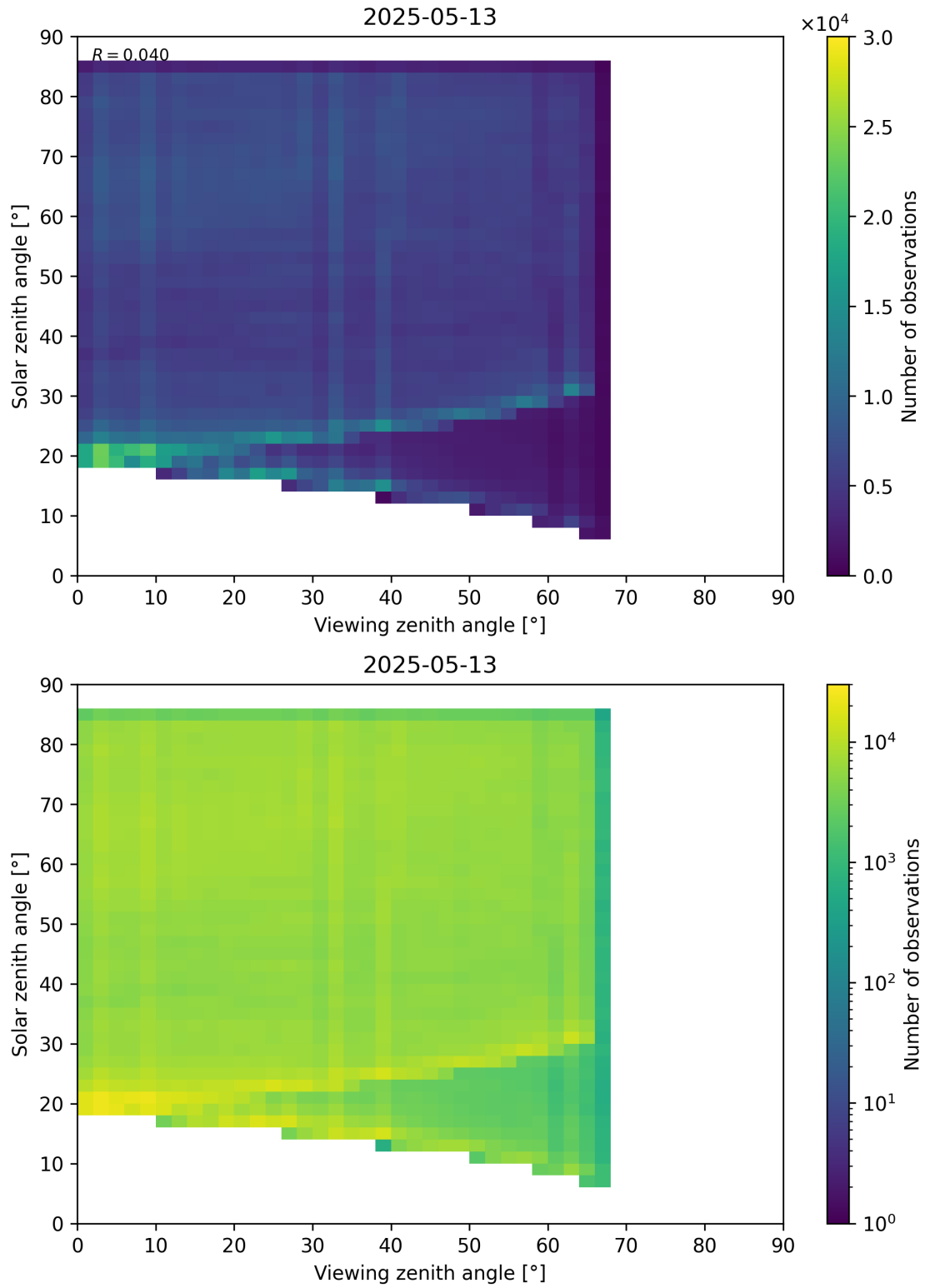
Figure 77: Scatter density plot of “Viewing zenith angle” against “Solar zenith angle” for 2025-05-12 to 2025-05-14.
