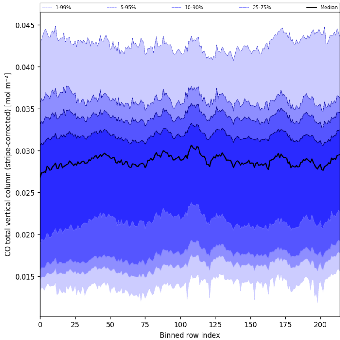
Figure 27: Along track statistics of “CO total vertical column (stripe-corrected)” for 2025-05-12 to 2025-05-14
