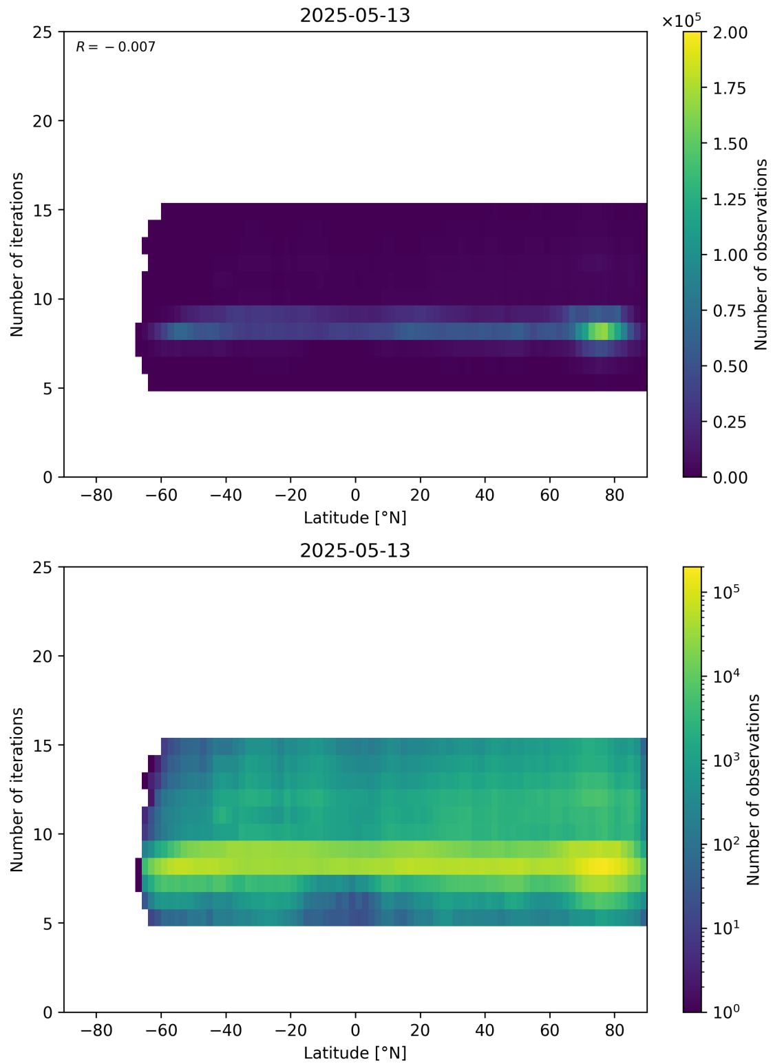
Figure 56: Scatter density plot of “Latitude” against “Number of iterations” for 2025-05-12 to 2025-05-14.
