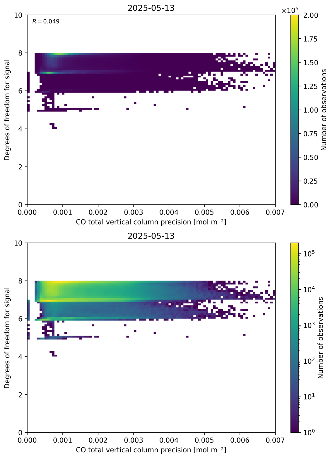
Figure 45: Scatter density plot of “CO total vertical column precision” against “Degrees of freedom for signal” for 2025-05-12 to 2025-05-14.
