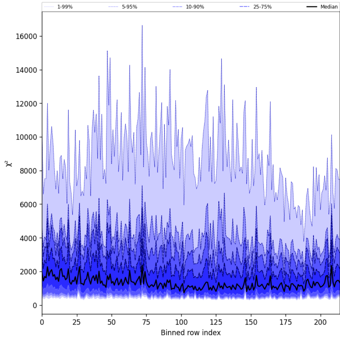
Figure 30: Along track statistics of “ \chi^2 ” for 2025-05-12 to 2025-05-14
