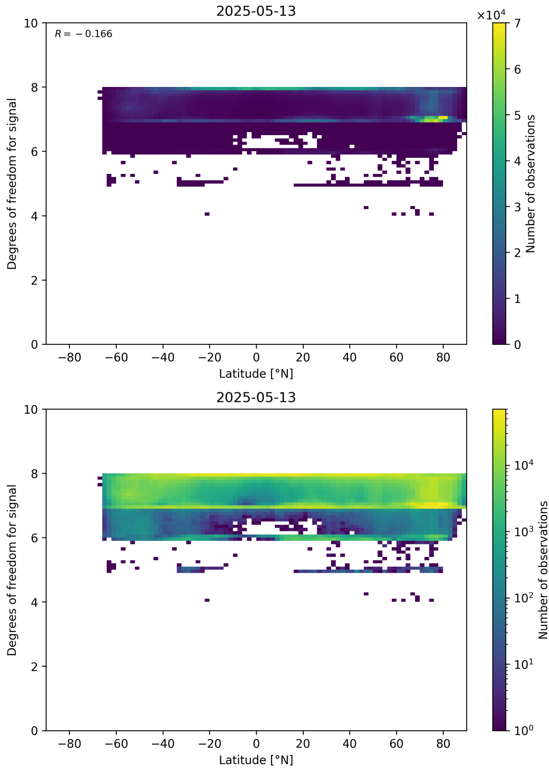
Figure 55: Scatter density plot of “Latitude” against “Degrees of freedom for signal” for 2025-05-12 to 2025-05-14.
