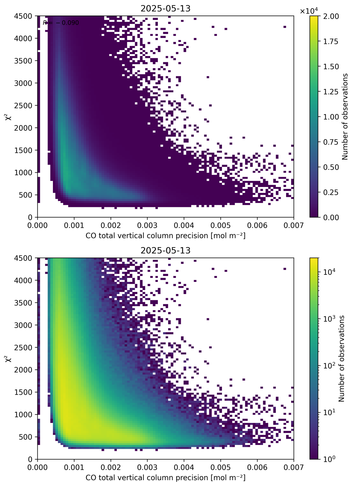
Figure 44: Scatter density plot of “CO total vertical column precision” against “ \chi^2 ” for 2025-05-12 to 2025-05-14.
