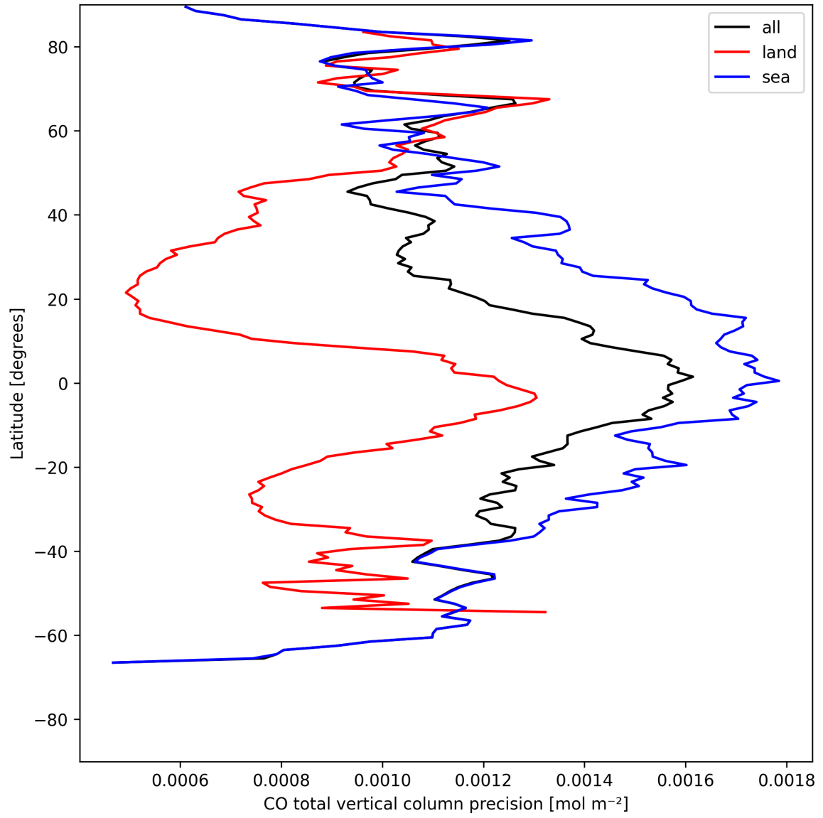
Figure 12: Zonal average of “CO total vertical column precision” for 2025-05-12 to 2025-05-14.
