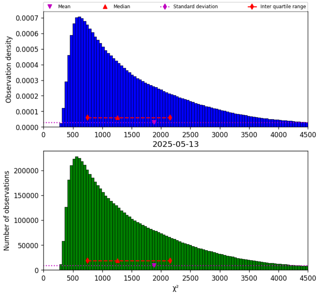
Figure 22: Histogram of “ \chi^2 ” for 2025-05-12 to 2025-05-14
