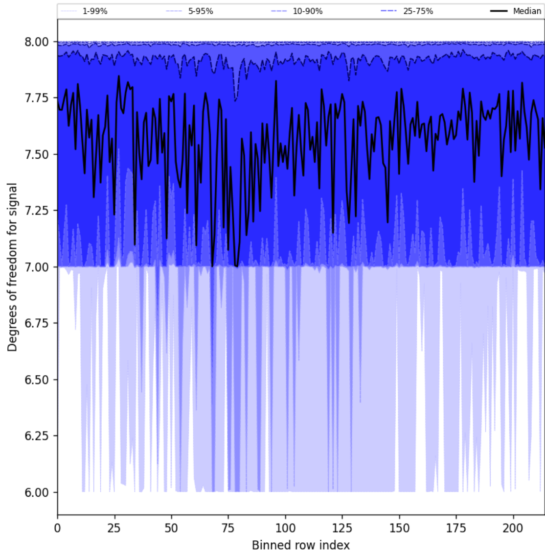
Figure 31: Along track statistics of “Degrees of freedom for signal” for 2025-05-12 to 2025-05-14
