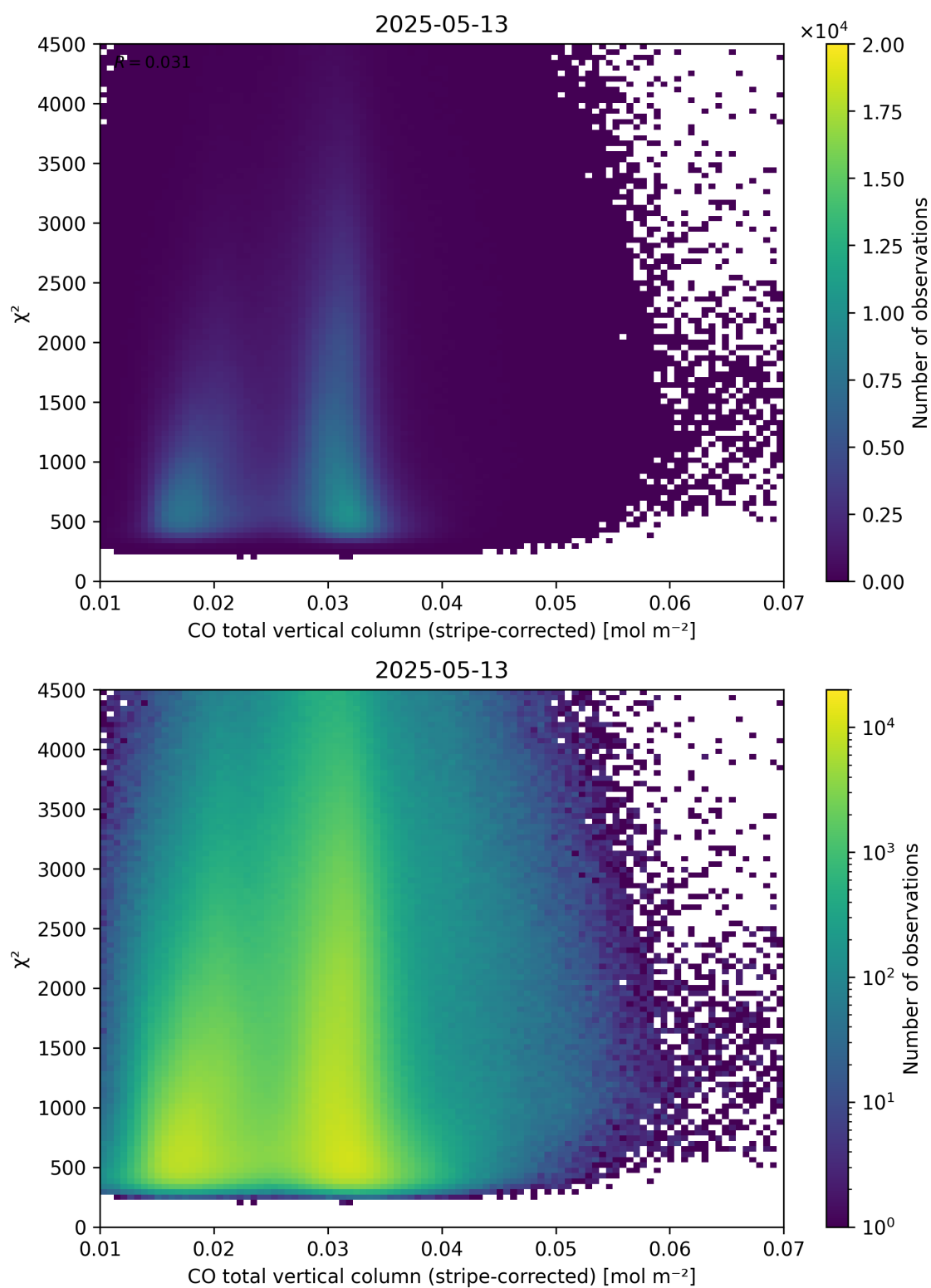
Figure 37: Scatter density plot of “CO total vertical column (stripe-corrected)” against “ \chi^2 ” for 2025-05-12 to 2025-05-14.
