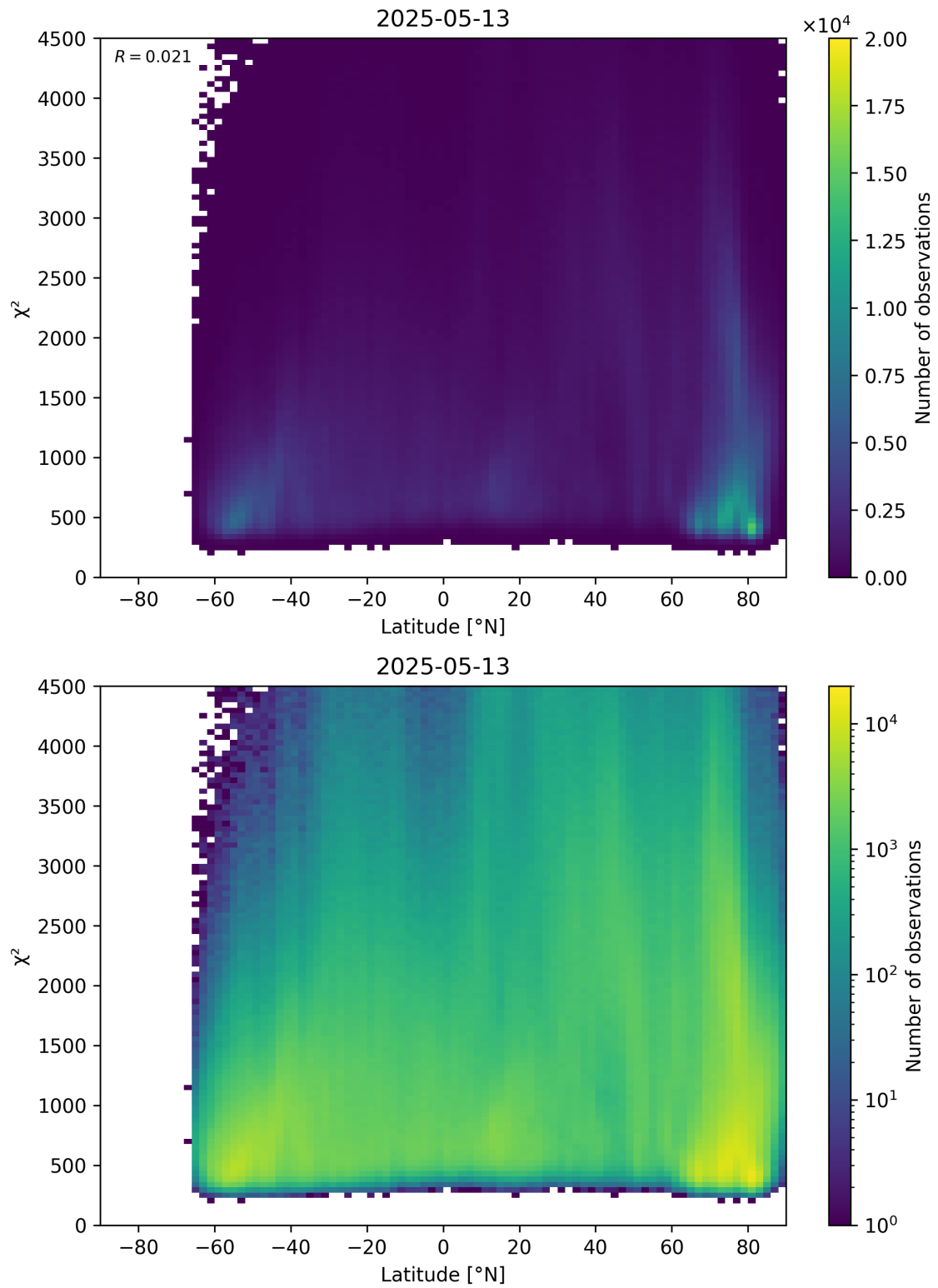
Figure 54: Scatter density plot of “Latitude” against “ \chi^2 ” for 2025-05-12 to 2025-05-14.
