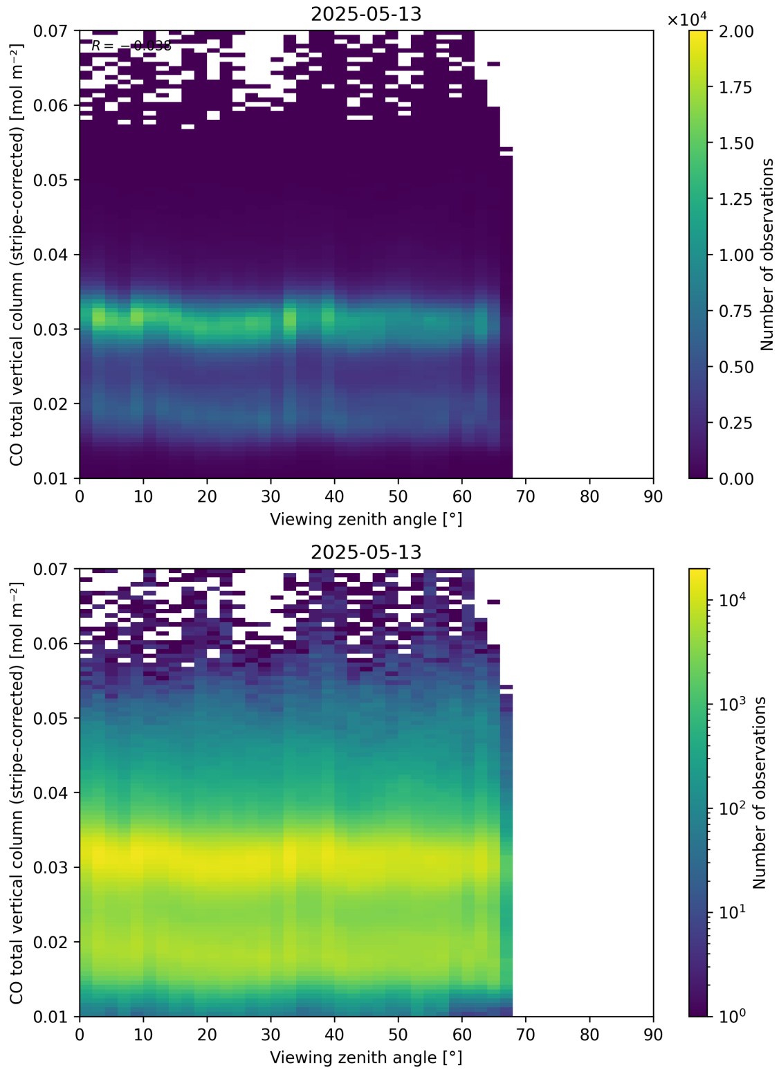
Figure 70: Scatter density plot of “Viewing zenith angle” against “CO total vertical column (stripe-corrected)” for 2025-05-12 to 2025-05-14.
