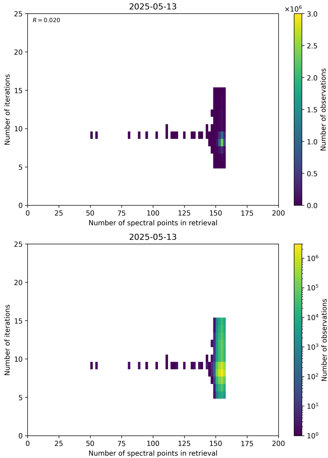
Figure 60: Scatter density plot of “Number of spectral points in retrieval” against “Number of iterations” for 2025-05-12 to 2025-05-14.
