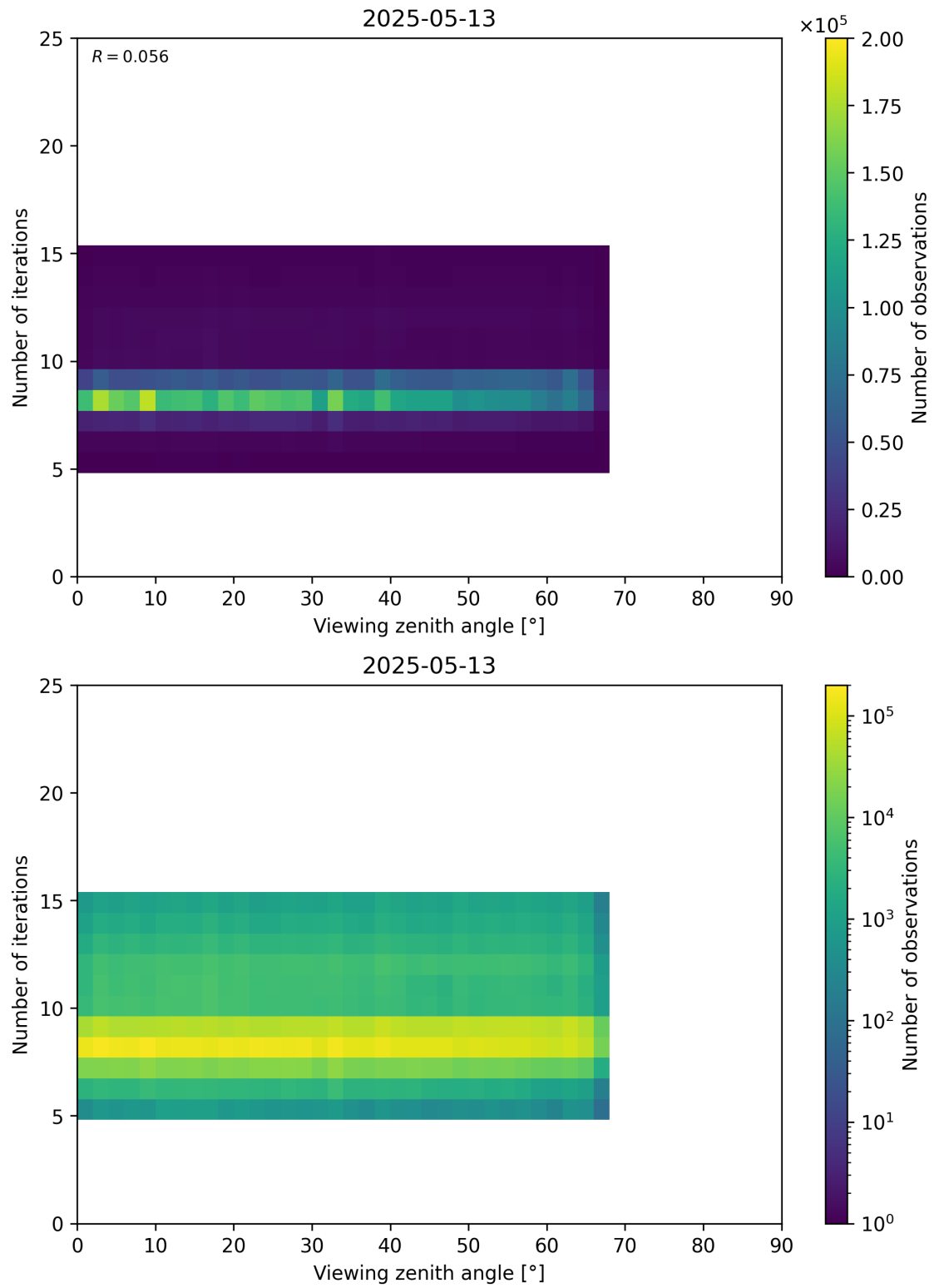
Figure 75: Scatter density plot of “Viewing zenith angle” against “Number of iterations” for 2025-05-12 to 2025-05-14.
