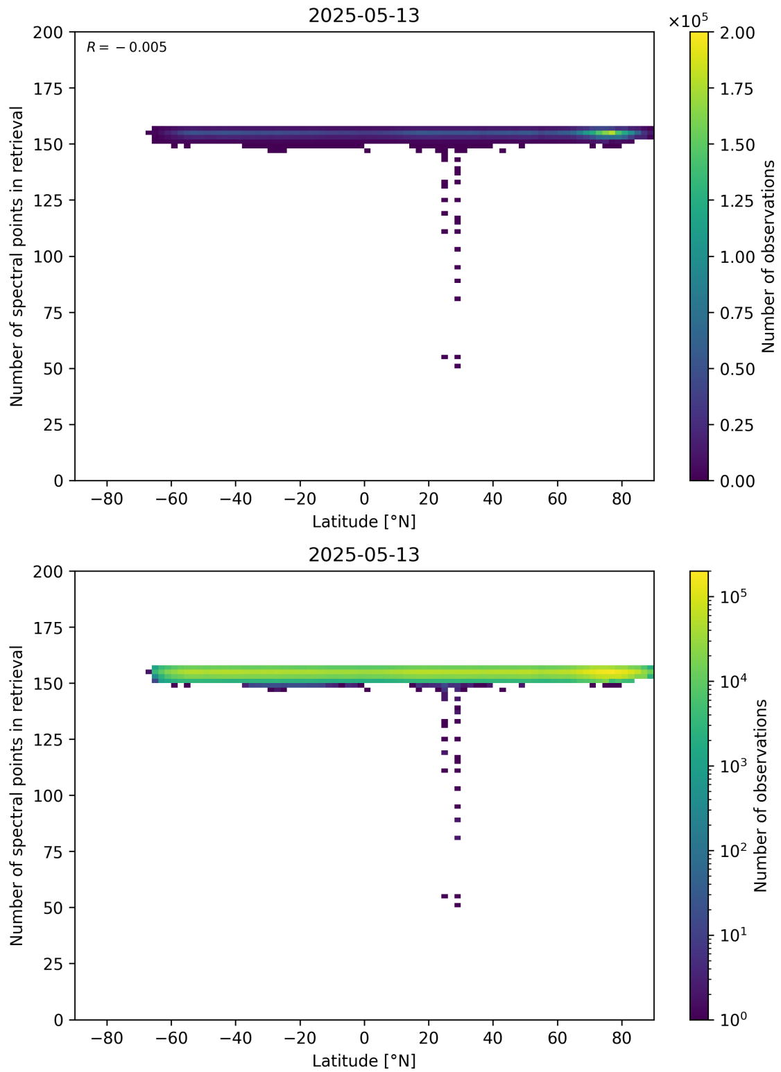
Figure 57: Scatter density plot of “Latitude” against “Number of spectral points in retrieval” for 2025-05-12 to 2025-05-14.
