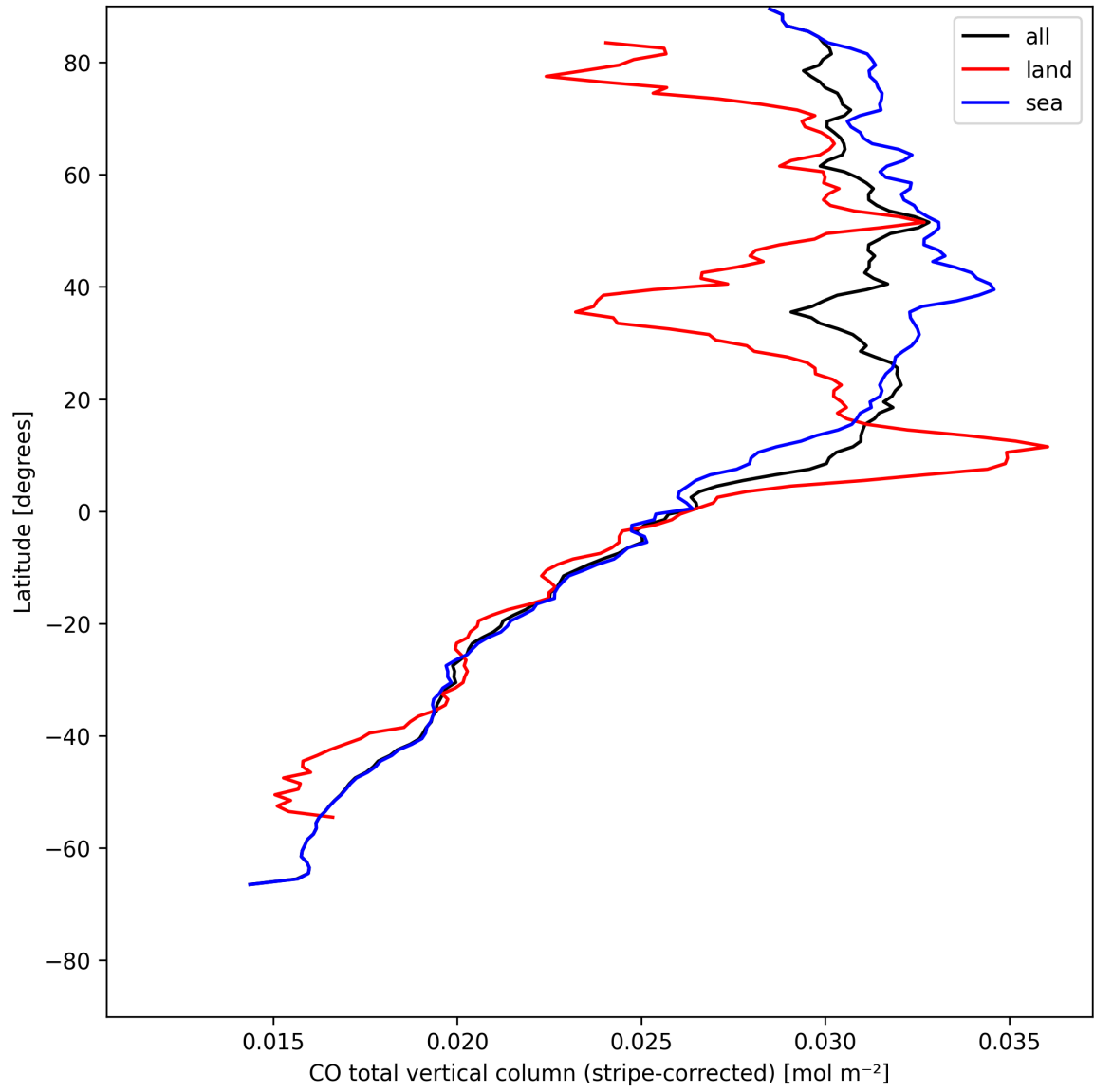
Figure 11: Zonal average of “CO total vertical column (stripe-corrected)” for 2025-05-12 to 2025-05-14.
