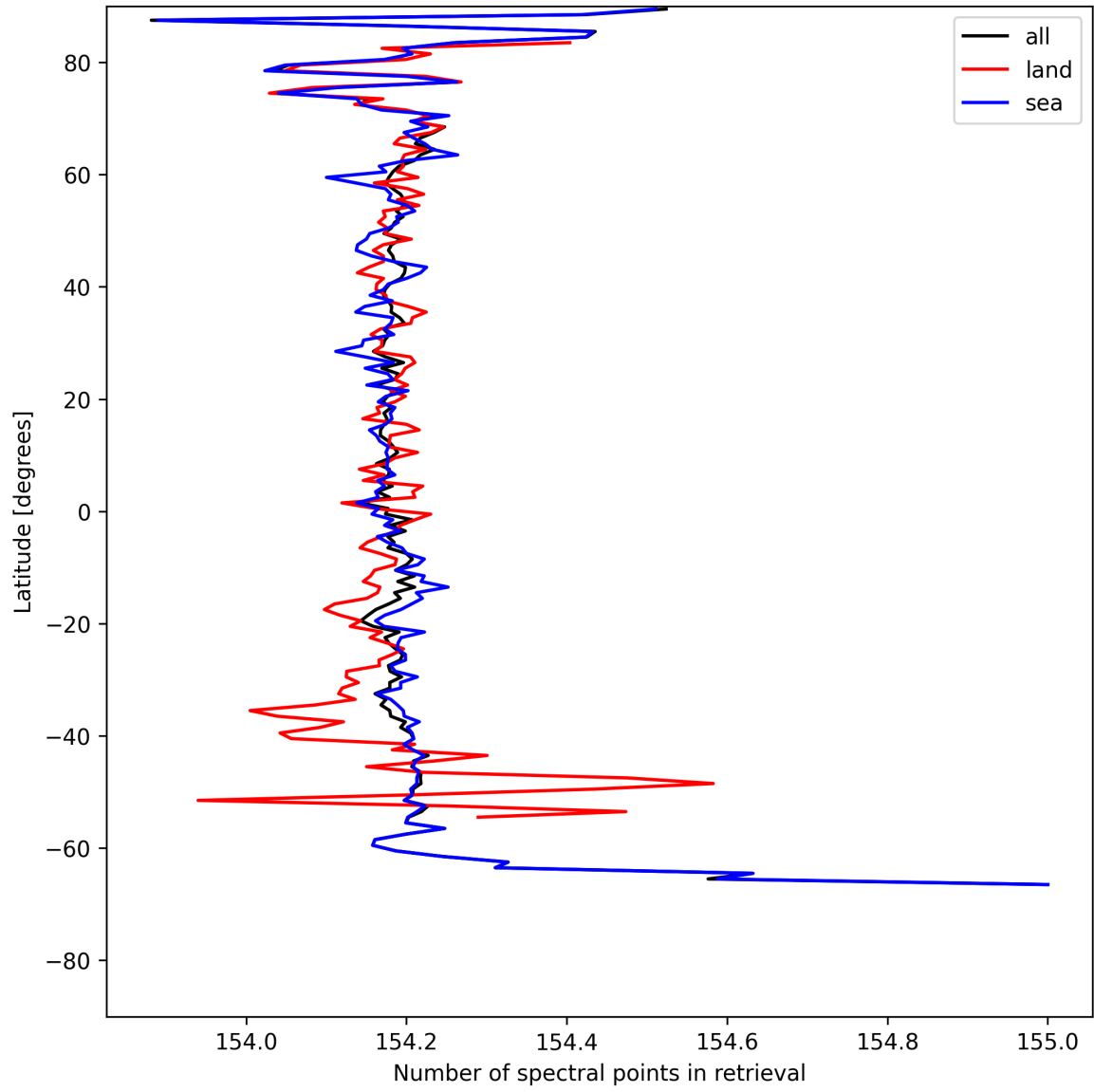
Figure 13: Zonal average of “Number of spectral points in retrieval” for 2025-05-12 to 2025-05-14.
