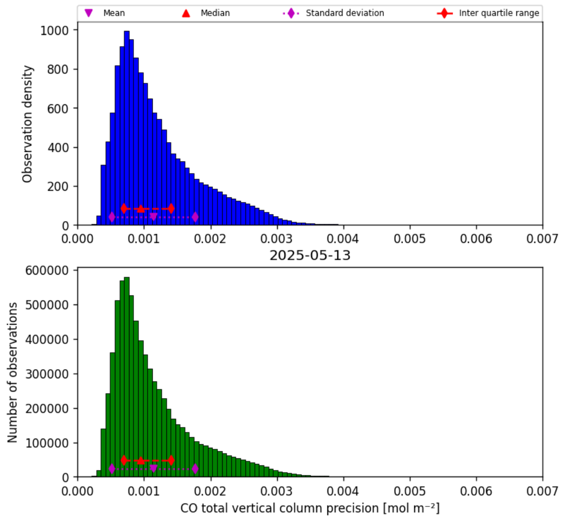
Figure 20: Histogram of “CO total vertical column precision” for 2025-05-12 to 2025-05-14
