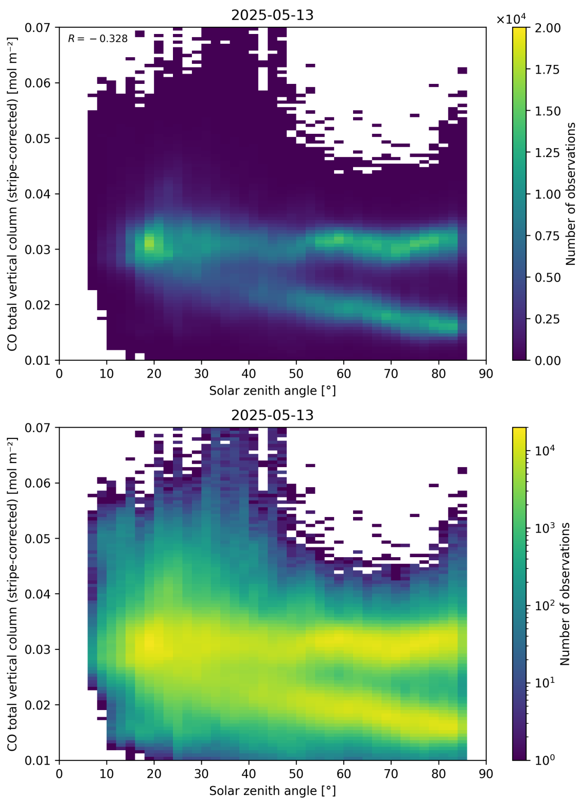
Figure 62: Scatter density plot of “Solar zenith angle” against “CO total vertical column (stripe-corrected)” for 2025-05-12 to 2025-05-14.
