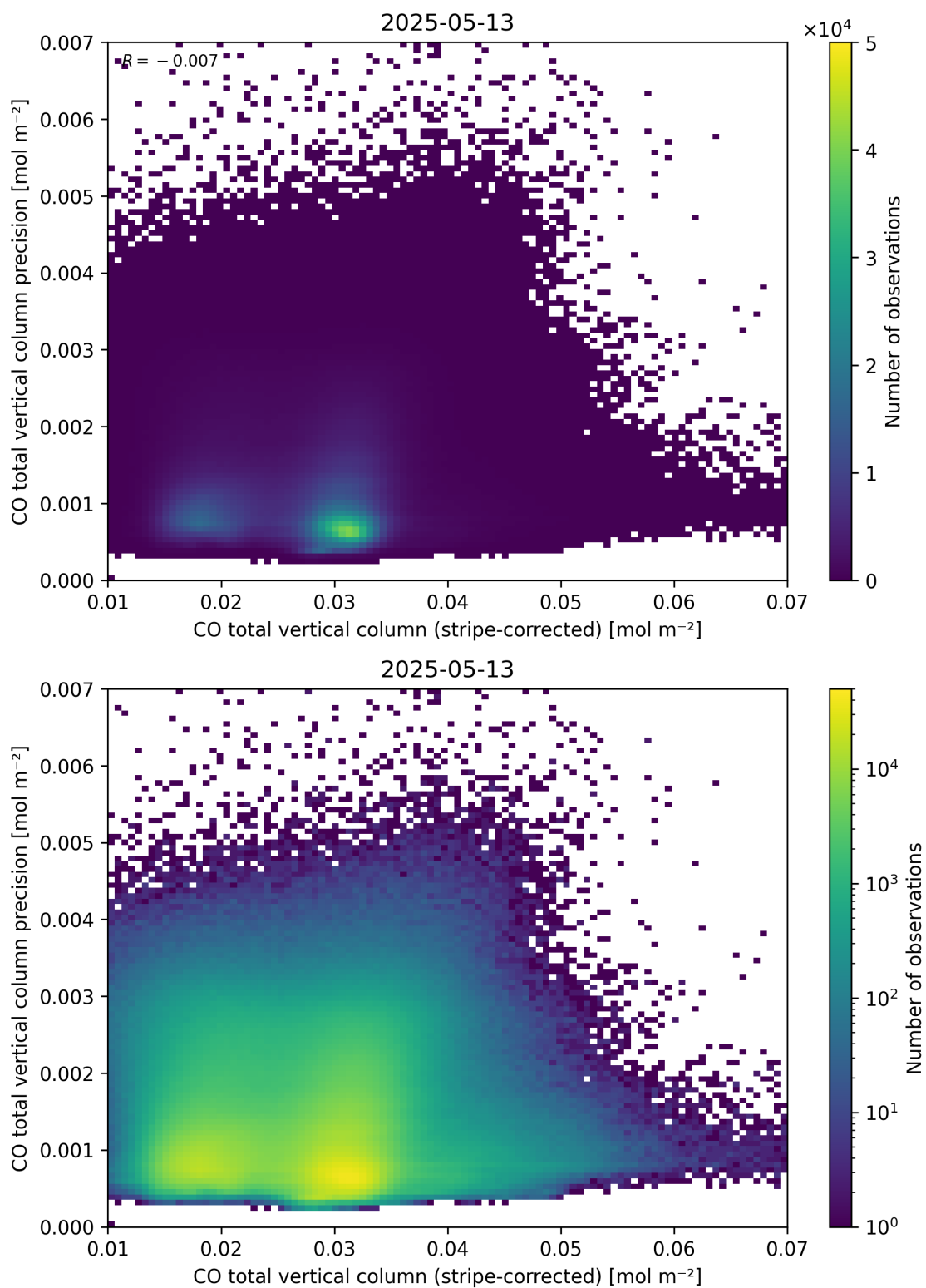
Figure 36: Scatter density plot of “CO total vertical column (stripe-corrected)” against “CO total vertical column precision” for 2025-05-12 to 2025-05-14.
