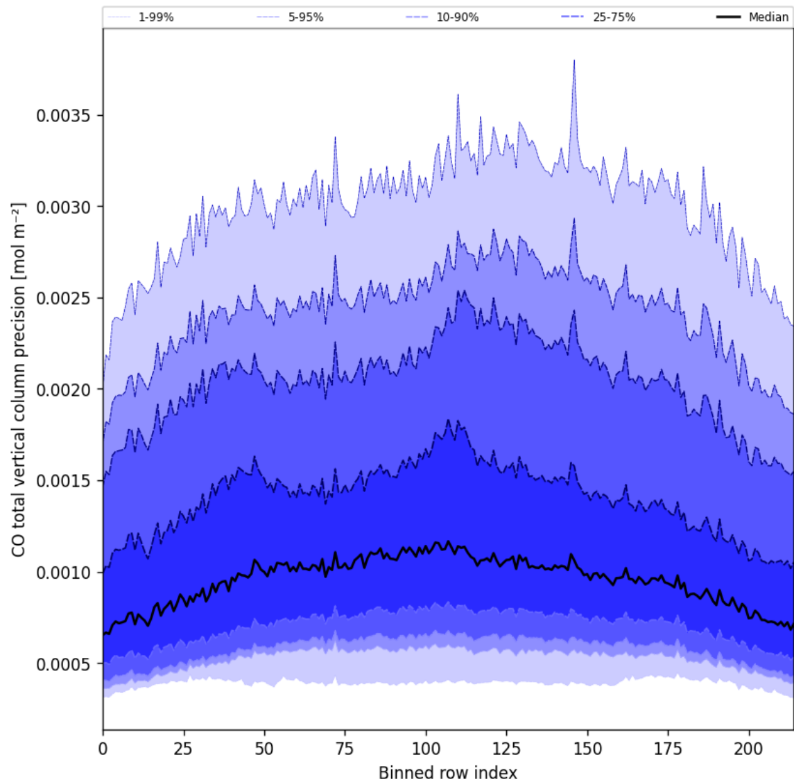
Figure 28: Along track statistics of “CO total vertical column precision” for 2025-05-12 to 2025-05-14
