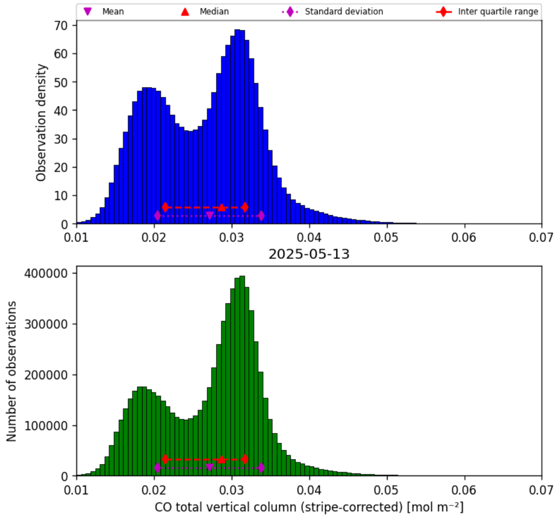
Figure 19: Histogram of “CO total vertical column (stripe-corrected)” for 2025-05-12 to 2025-05-14
