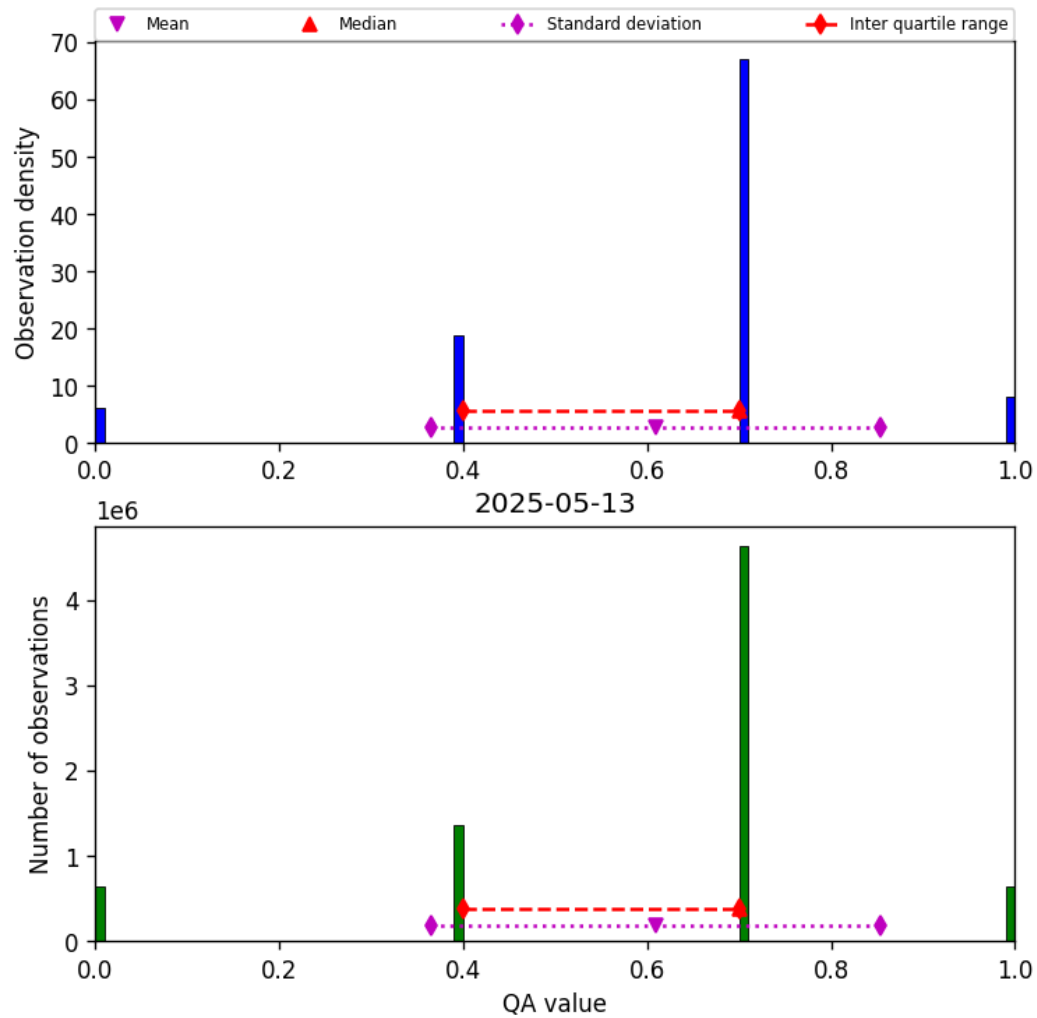
Figure 17: Histogram of “QA value” for 2025-05-12 to 2025-05-14
