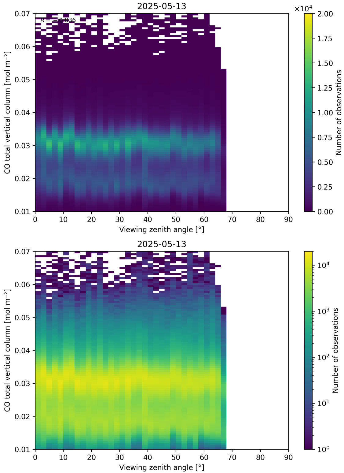
Figure 69: Scatter density plot of “Viewing zenith angle” against “CO total vertical column” for 2025-05-12 to 2025-05-14.
