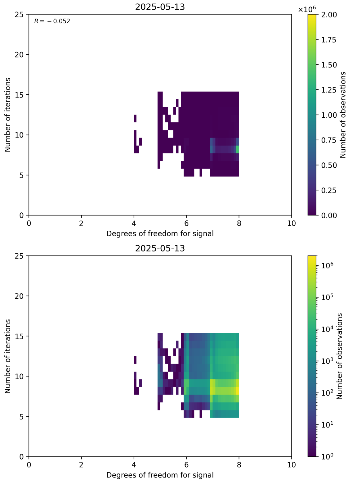
Figure 50: Scatter density plot of “Degrees of freedom for signal” against “Number of iterations” for 2025-05-12 to 2025-05-14.
