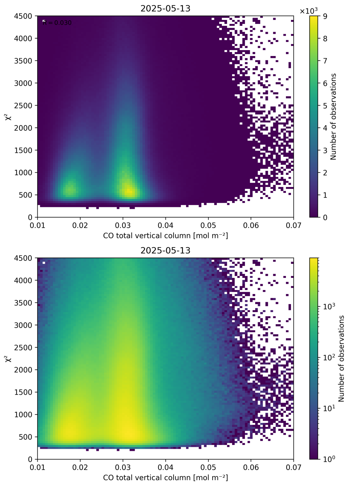
Figure 35: Scatter density plot of “CO total vertical column” against “ \chi^2 ” for 2025-05-12 to 2025-05-14.
