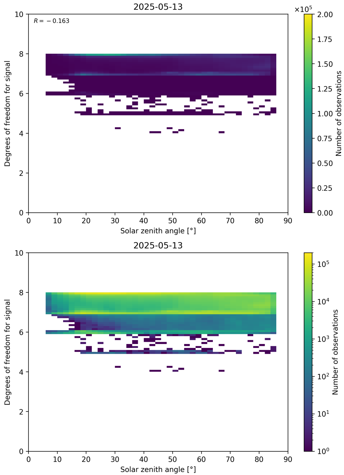
Figure 65: Scatter density plot of “Solar zenith angle” against “Degrees of freedom for signal” for 2025-05-12 to 2025-05-14.
