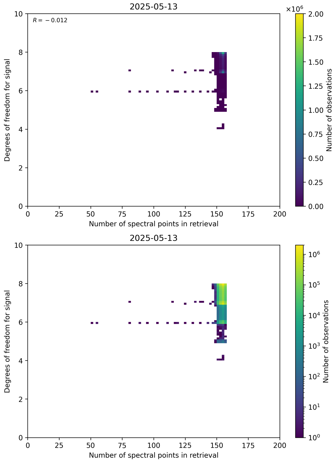
Figure 59: Scatter density plot of “Number of spectral points in retrieval” against “Degrees of freedom for signal” for 2025-05-12 to 2025-05-14.
