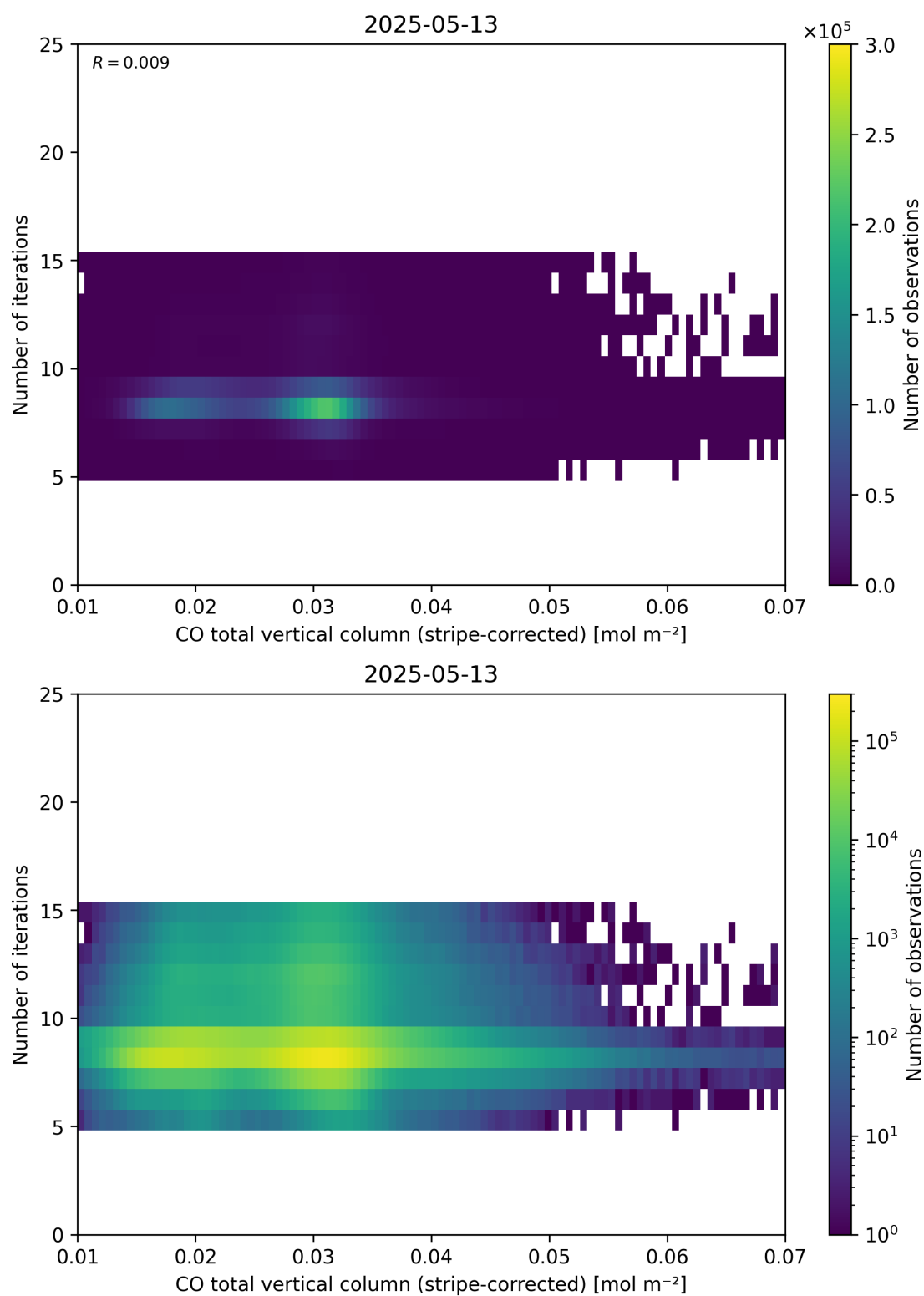
Figure 39: Scatter density plot of “CO total vertical column (stripe-corrected)” against “Number of iterations” for 2025-05-12 to 2025-05-14.
