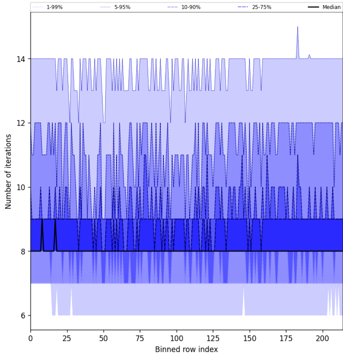
Figure 32: Along track statistics of “Number of iterations” for 2025-05-12 to 2025-05-14
