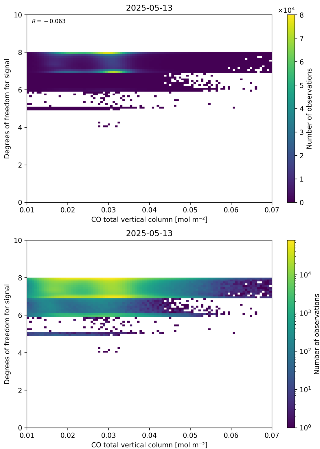
Figure 41: Scatter density plot of “CO total vertical column” against “Degrees of freedom for signal” for 2025-05-12 to 2025-05-14.
