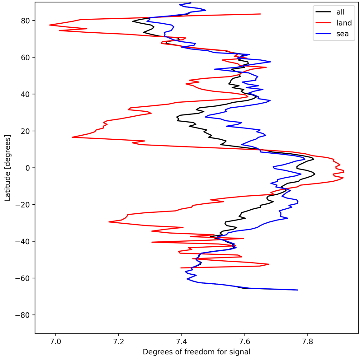
Figure 15: Zonal average of “Degrees of freedom for signal” for 2025-05-12 to 2025-05-14.
