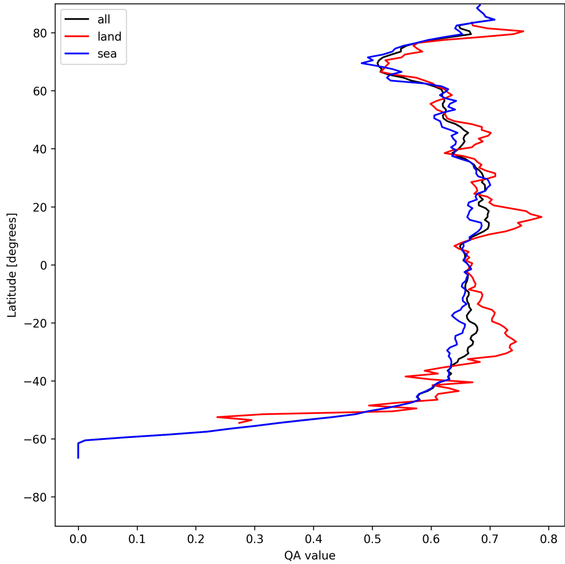
Figure 9: Zonal average of “QA value” for 2025-05-12 to 2025-05-14.
