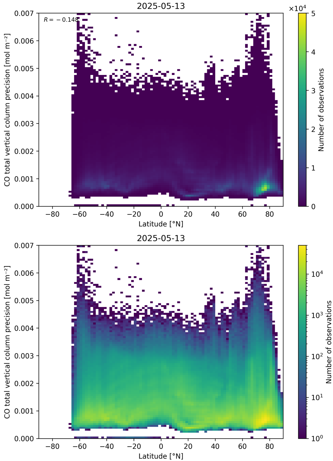
Figure 53: Scatter density plot of “Latitude” against “CO total vertical column precision” for 2025-05-12 to 2025-05-14.
