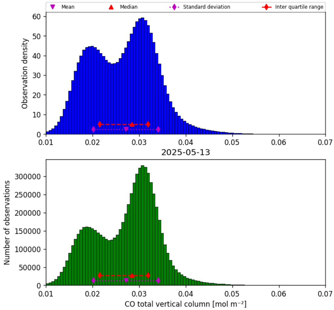
Figure 18: Histogram of “CO total vertical column” for 2025-05-12 to 2025-05-14
