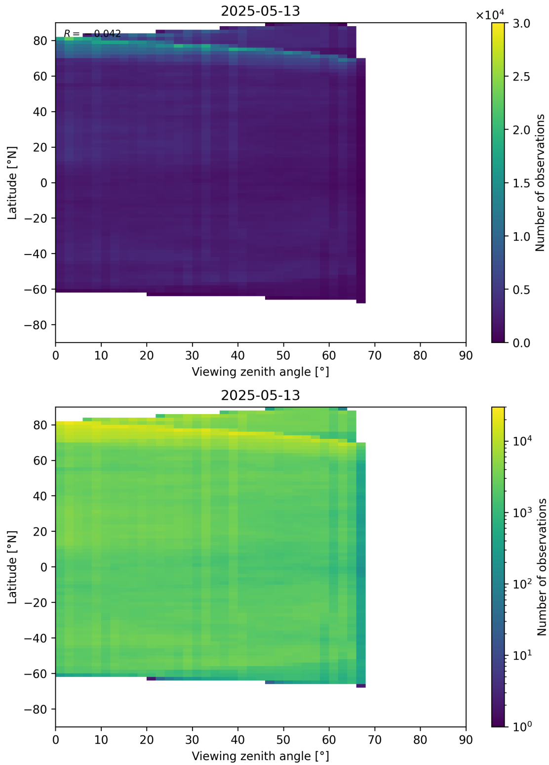
Figure 74: Scatter density plot of “Viewing zenith angle” against “Latitude” for 2025-05-12 to 2025-05-14.
