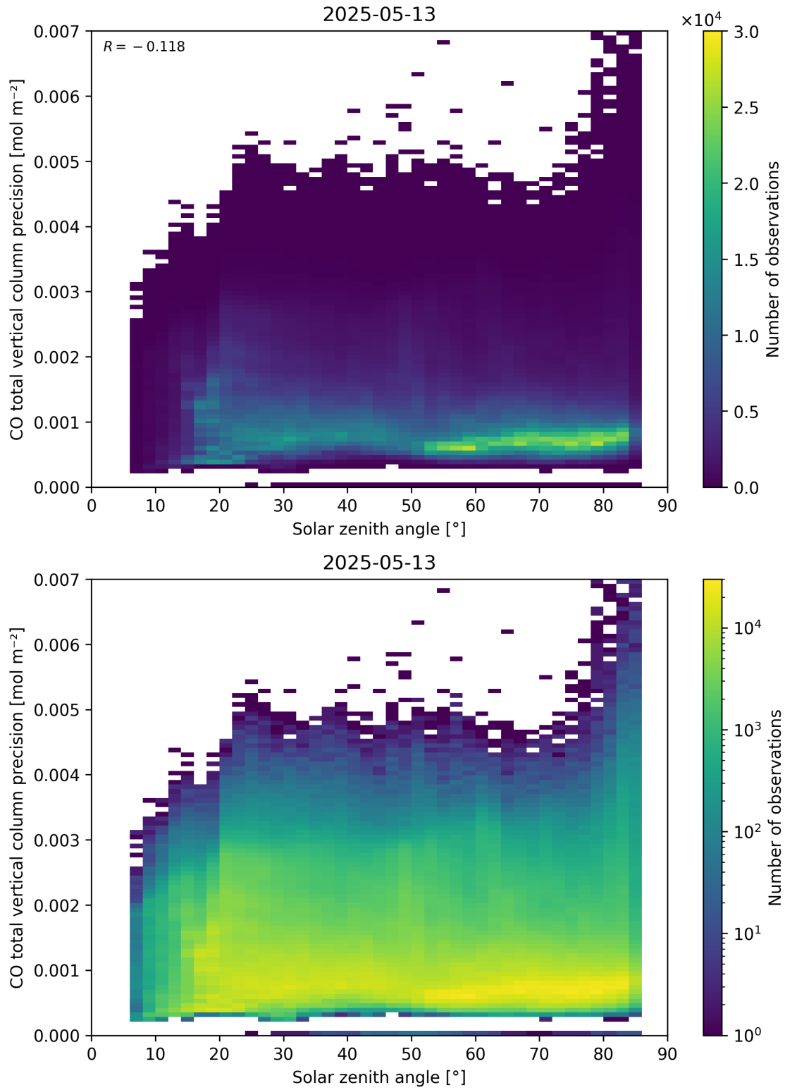
Figure 63: Scatter density plot of “Solar zenith angle” against “CO total vertical column precision” for 2025-05-12 to 2025-05-14.
