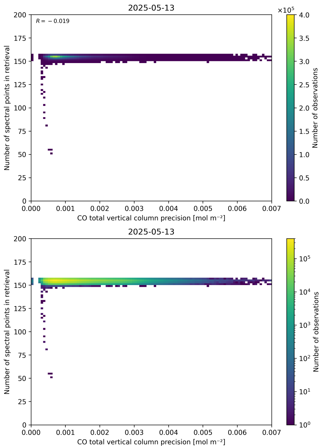
Figure 47: Scatter density plot of “CO total vertical column precision” against “Number of spectral points in retrieval” for 2025-05-12 to 2025-05-14.
