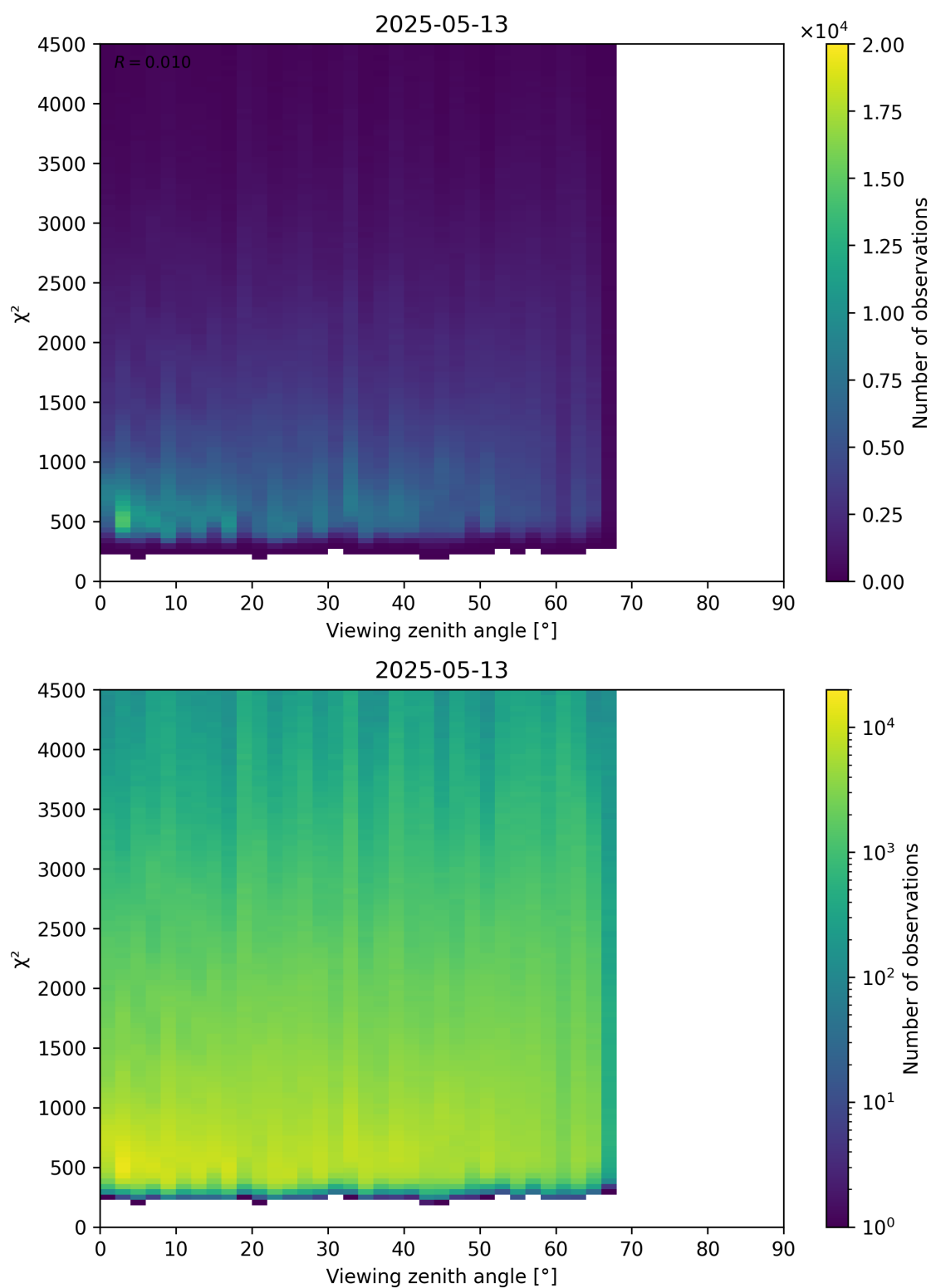
Figure 72: Scatter density plot of “Viewing zenith angle” against “ \chi^2 ” for 2025-05-12 to 2025-05-14.
