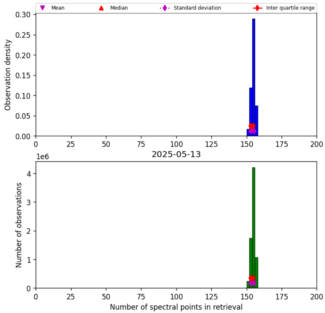
Figure 21: Histogram of “Number of spectral points in retrieval” for 2025-05-12 to 2025-05-14
