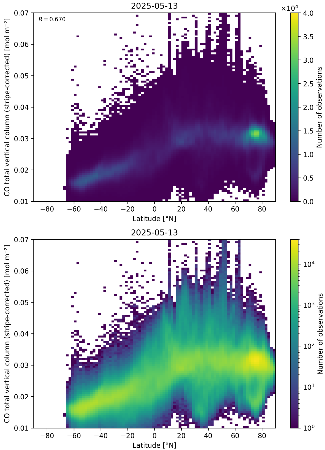
Figure 52: Scatter density plot of “Latitude” against “CO total vertical column (stripe-corrected)” for 2025-05-12 to 2025-05-14.
