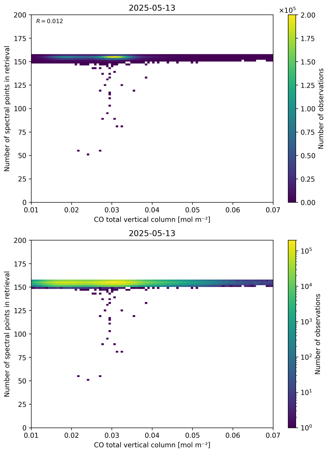
Figure 43: Scatter density plot of “CO total vertical column” against “Number of spectral points in retrieval” for 2025-05-12 to 2025-05-14.
