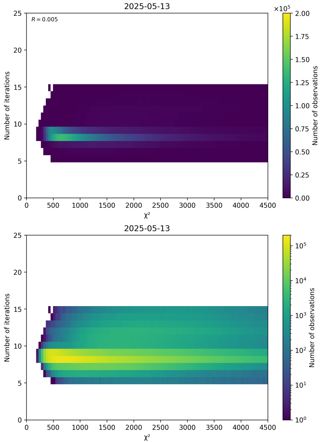
Figure 49: Scatter density plot of “ \chi^2 ” against “Number of iterations” for 2025-05-12 to 2025-05-14.
