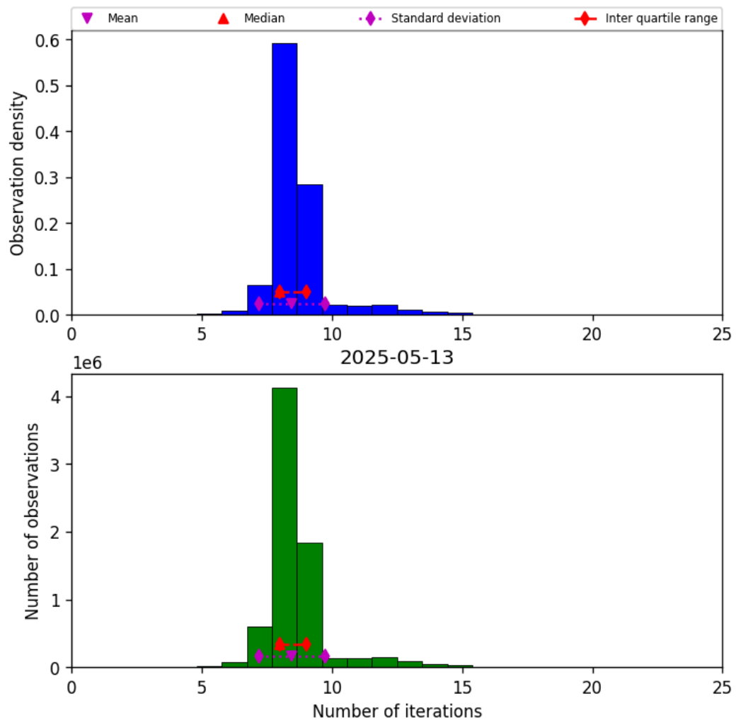
Figure 24: Histogram of “Number of iterations” for 2025-05-12 to 2025-05-14
