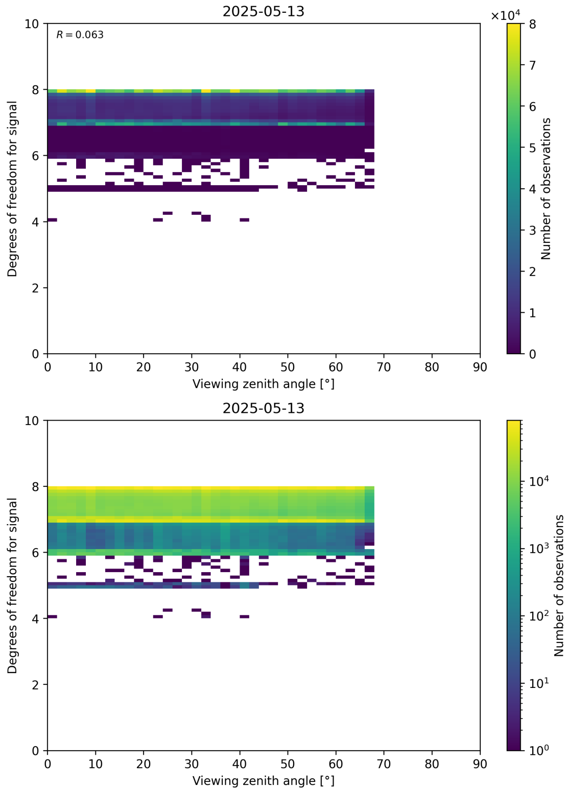
Figure 73: Scatter density plot of “Viewing zenith angle” against “Degrees of freedom for signal” for 2025-05-12 to 2025-05-14.
