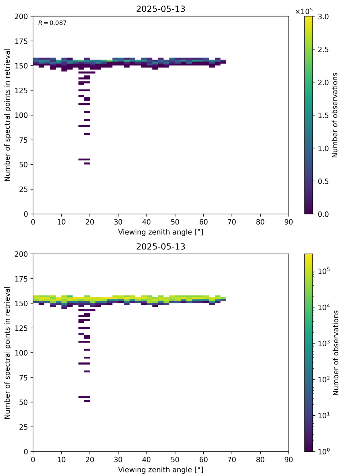
Figure 76: Scatter density plot of “Viewing zenith angle” against “Number of spectral points in retrieval” for 2025-05-12 to 2025-05-14.
