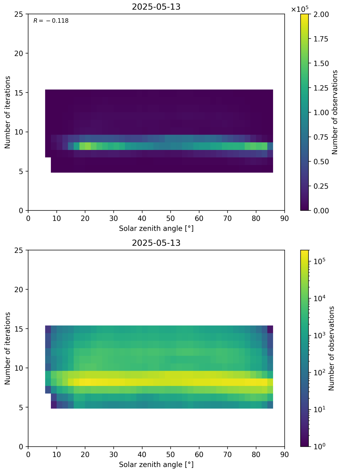
Figure 67: Scatter density plot of “Solar zenith angle” against “Number of iterations” for 2025-05-12 to 2025-05-14.
