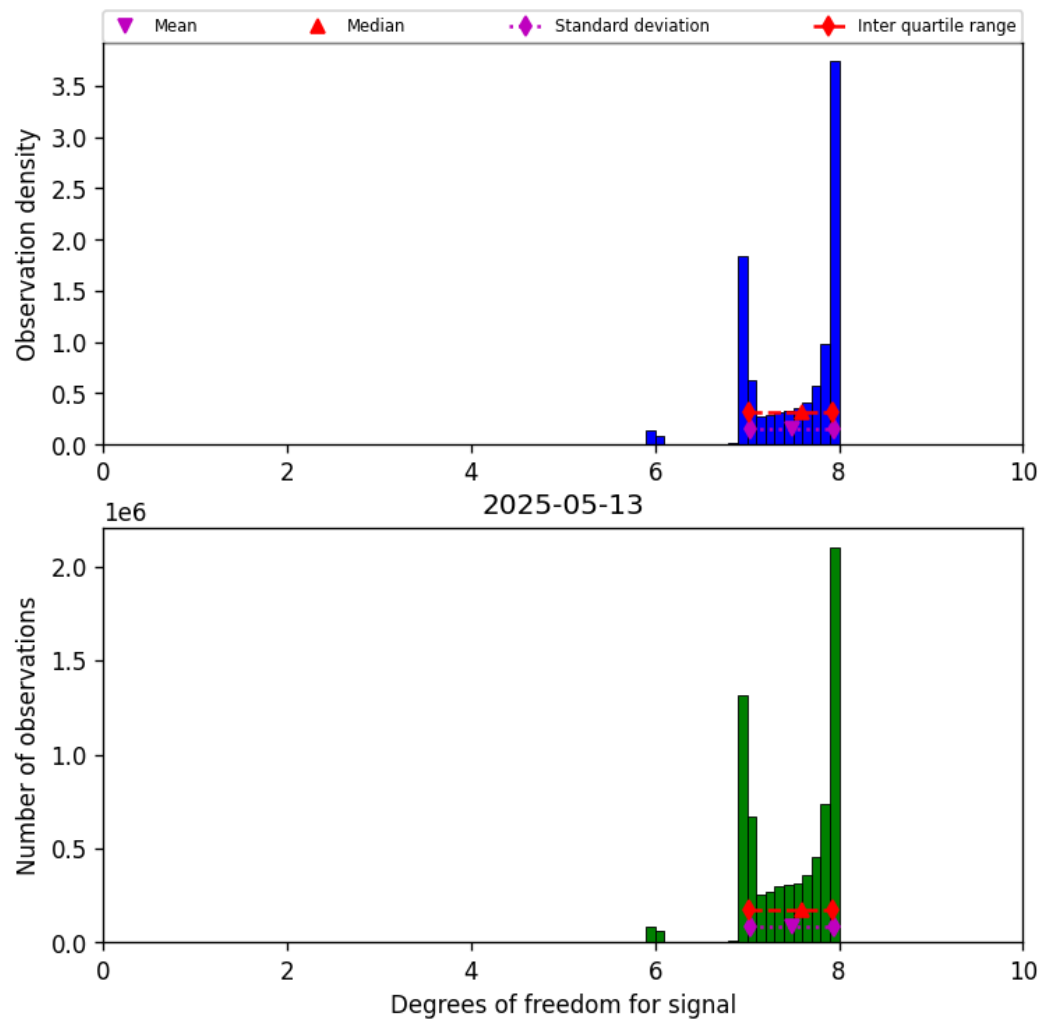
Figure 23: Histogram of “Degrees of freedom for signal” for 2025-05-12 to 2025-05-14
