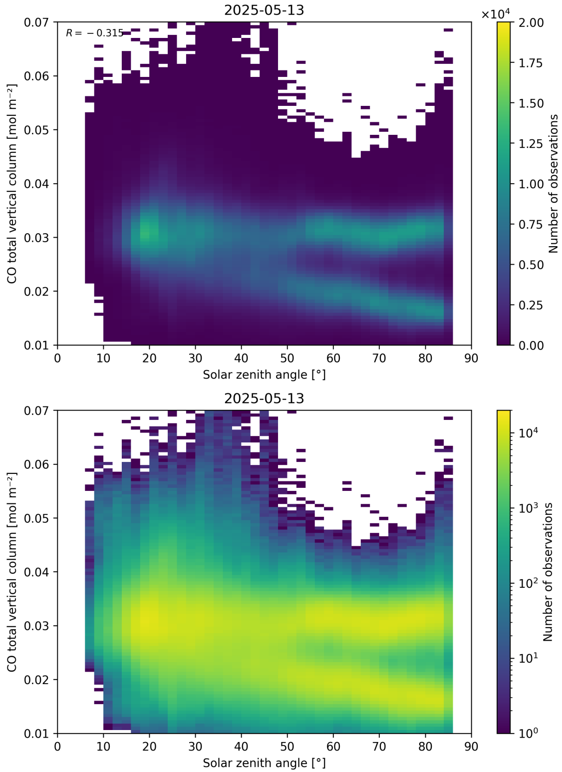
Figure 61: Scatter density plot of “Solar zenith angle” against “CO total vertical column” for 2025-05-12 to 2025-05-14.
