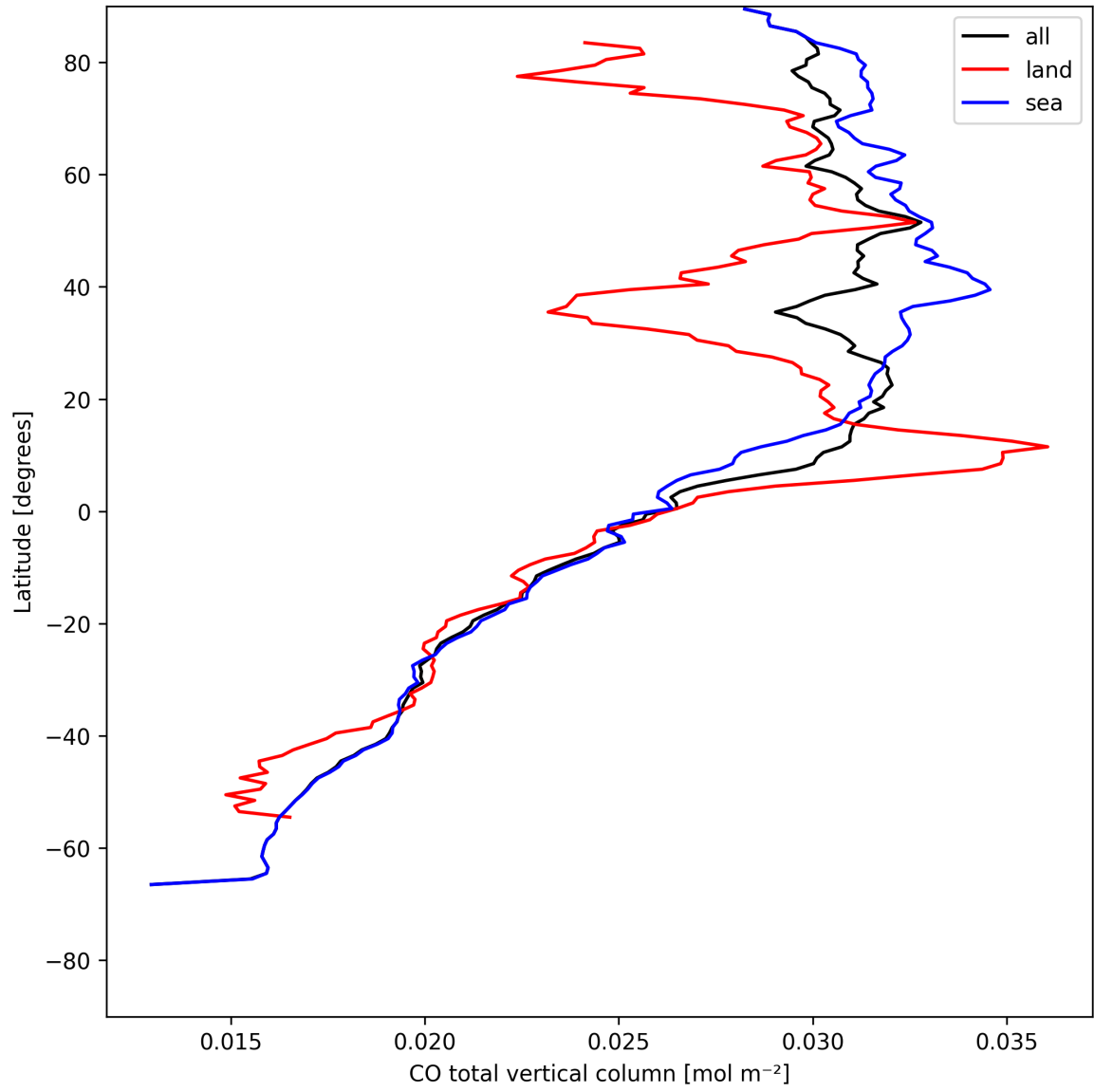
Figure 10: Zonal average of “CO total vertical column” for 2025-05-12 to 2025-05-14.
