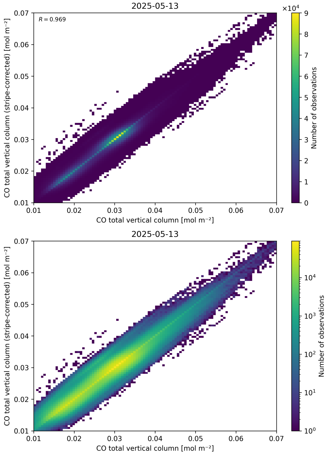
Figure 33: Scatter density plot of “CO total vertical column” against “CO total vertical column (stripe-corrected)” for 2025-05-12 to 2025-05-14.
