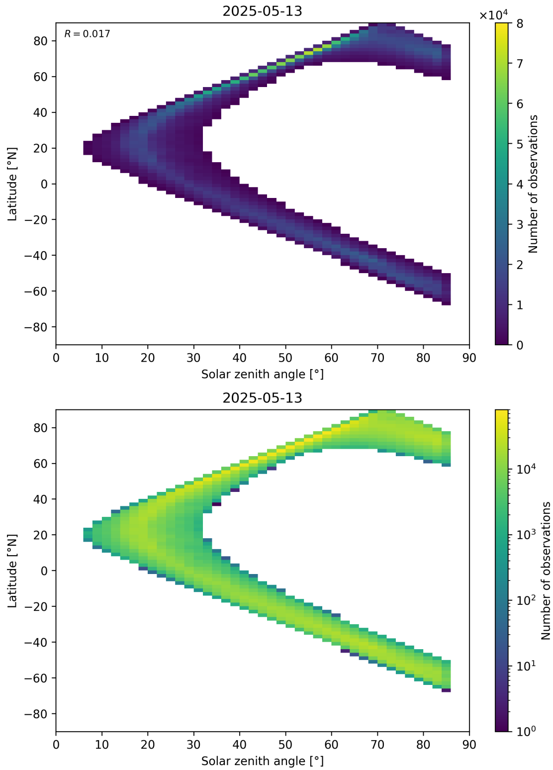
Figure 66: Scatter density plot of “Solar zenith angle” against “Latitude” for 2025-05-12 to 2025-05-14.
