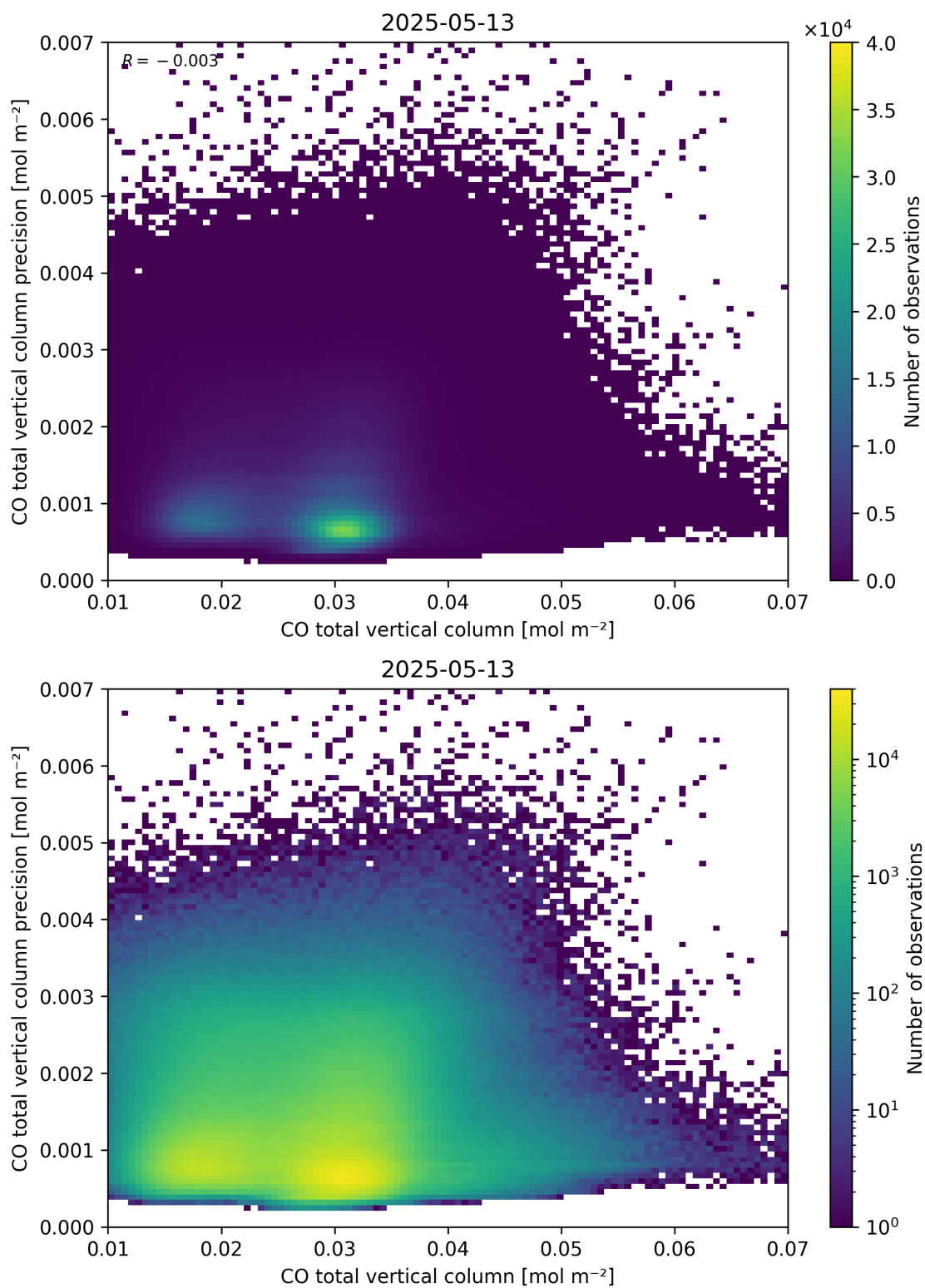
Figure 34: Scatter density plot of “CO total vertical column” against “CO total vertical column precision” for 2025-05-12 to 2025-05-14.
