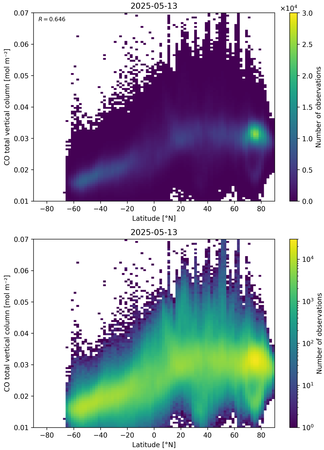
Figure 51: Scatter density plot of “Latitude” against “CO total vertical column” for 2025-05-12 to 2025-05-14.
