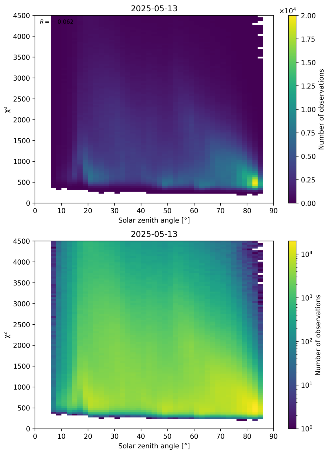
Figure 64: Scatter density plot of “Solar zenith angle” against “ \chi^2 ” for 2025-05-12 to 2025-05-14.
