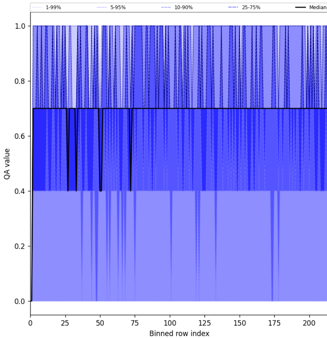
Figure 25: Along track statistics of “QA value” for 2025-05-12 to 2025-05-14
