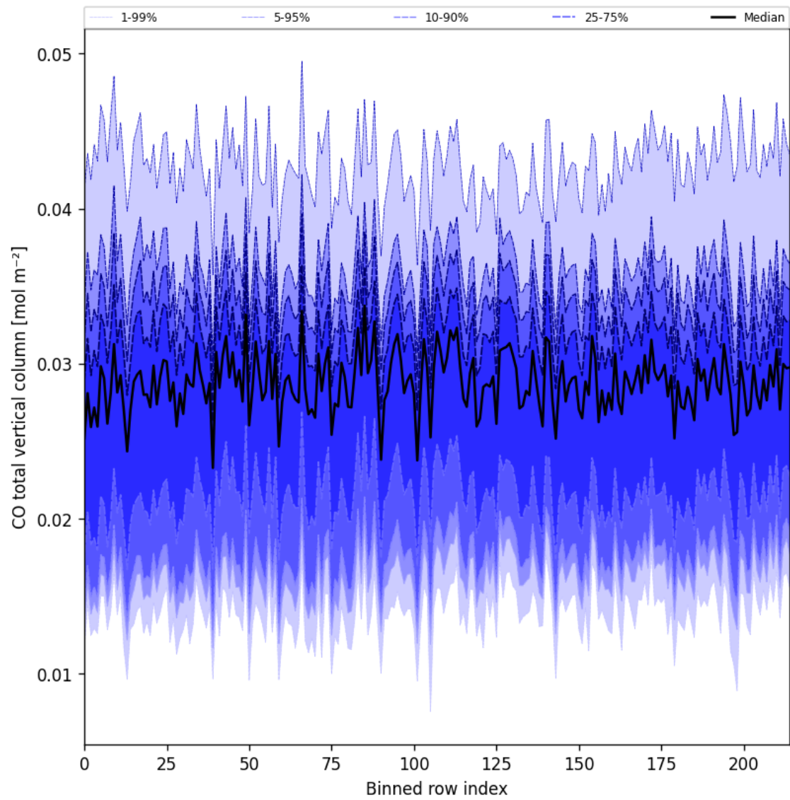
Figure 26: Along track statistics of “CO total vertical column” for 2025-05-12 to 2025-05-14
