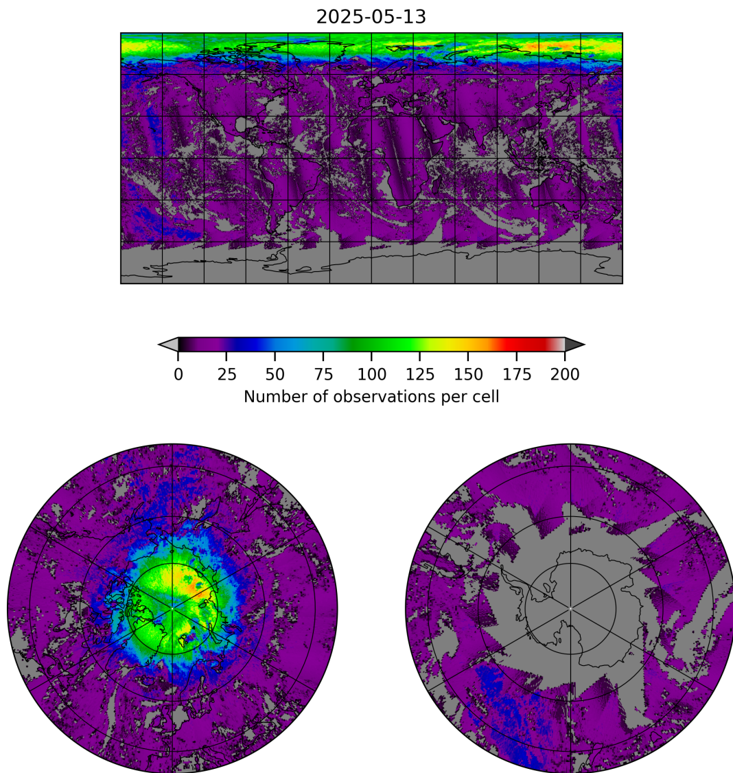
Figure 8: Map of the number of observations for 2025-05-12 to 2025-05-14
