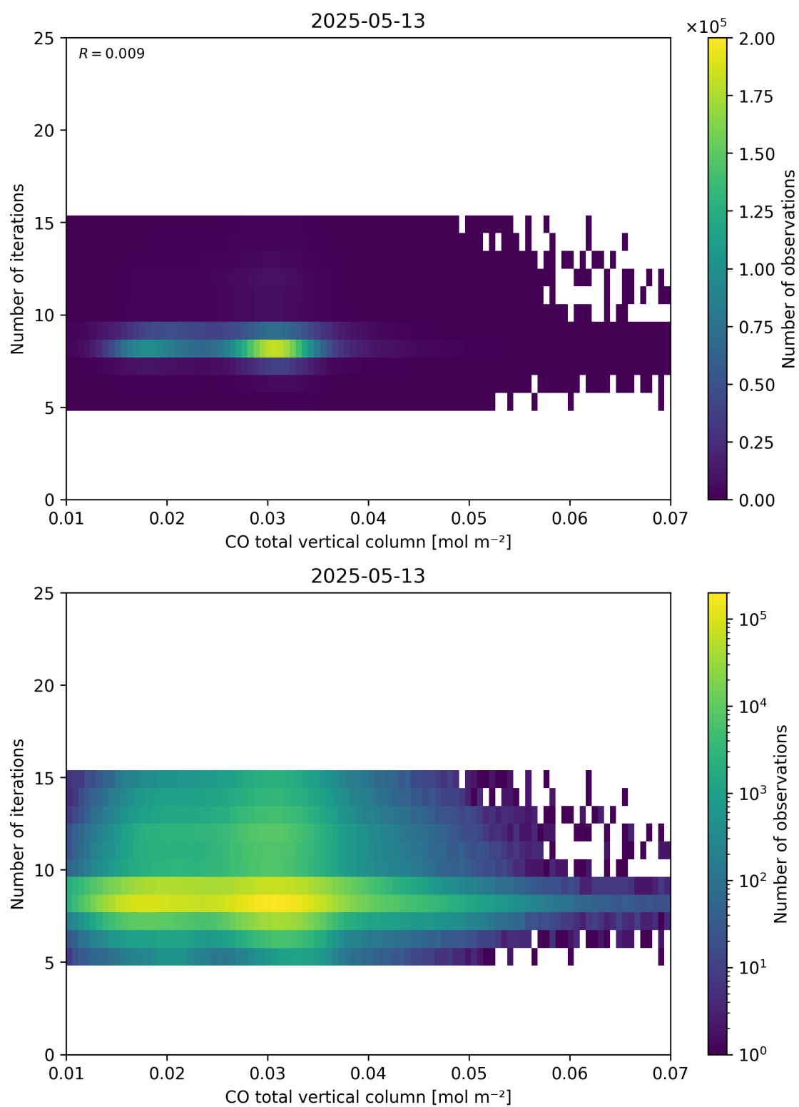
Figure 42: Scatter density plot of “CO total vertical column” against “Number of iterations” for 2025-05-12 to 2025-05-14.
