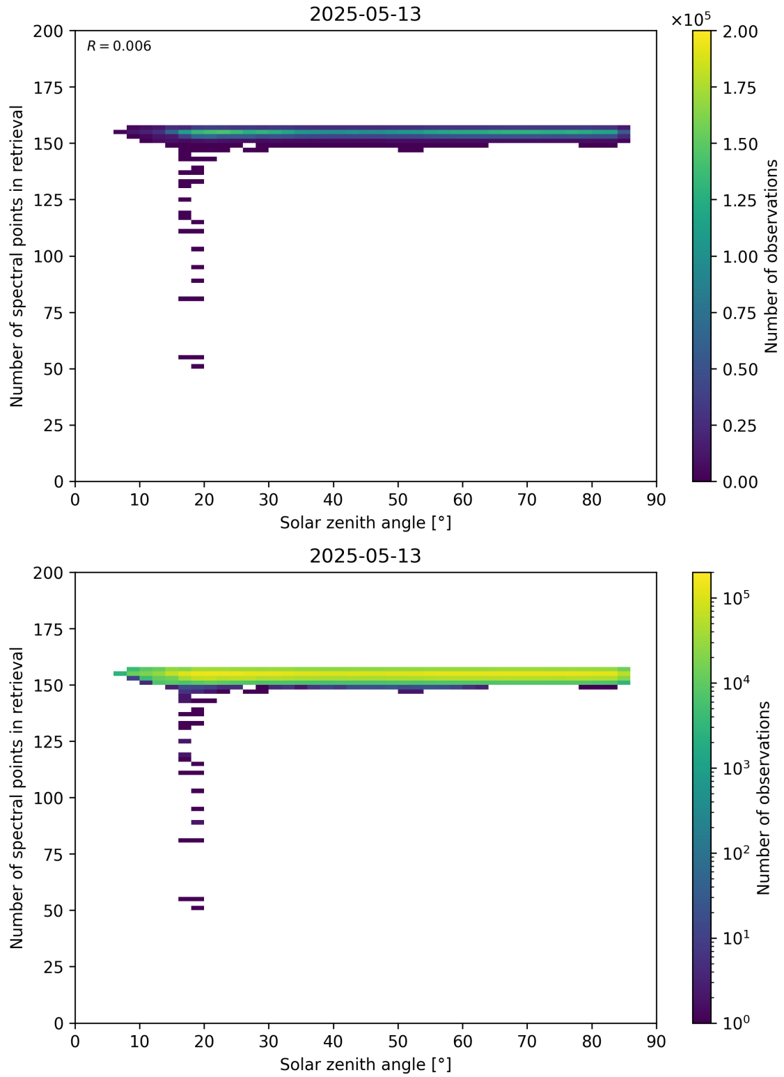
Figure 68: Scatter density plot of “Solar zenith angle” against “Number of spectral points in retrieval” for 2025-05-12 to 2025-05-14.
