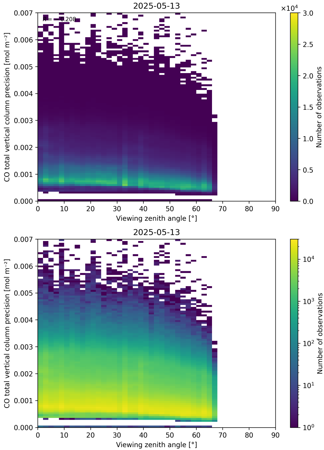
Figure 71: Scatter density plot of “Viewing zenith angle” against “CO total vertical column precision” for 2025-05-12 to 2025-05-14.
