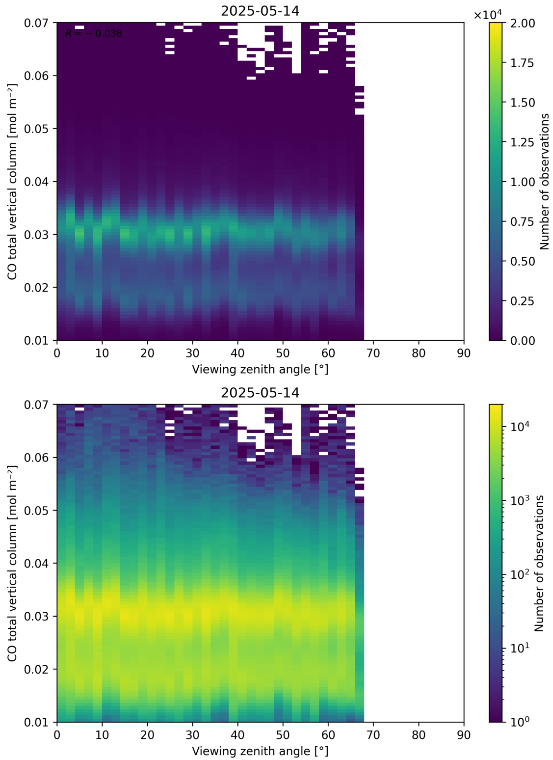
Figure 69: Scatter density plot of “Viewing zenith angle” against “CO total vertical column” for 2025-05-13 to 2025-05-15.
