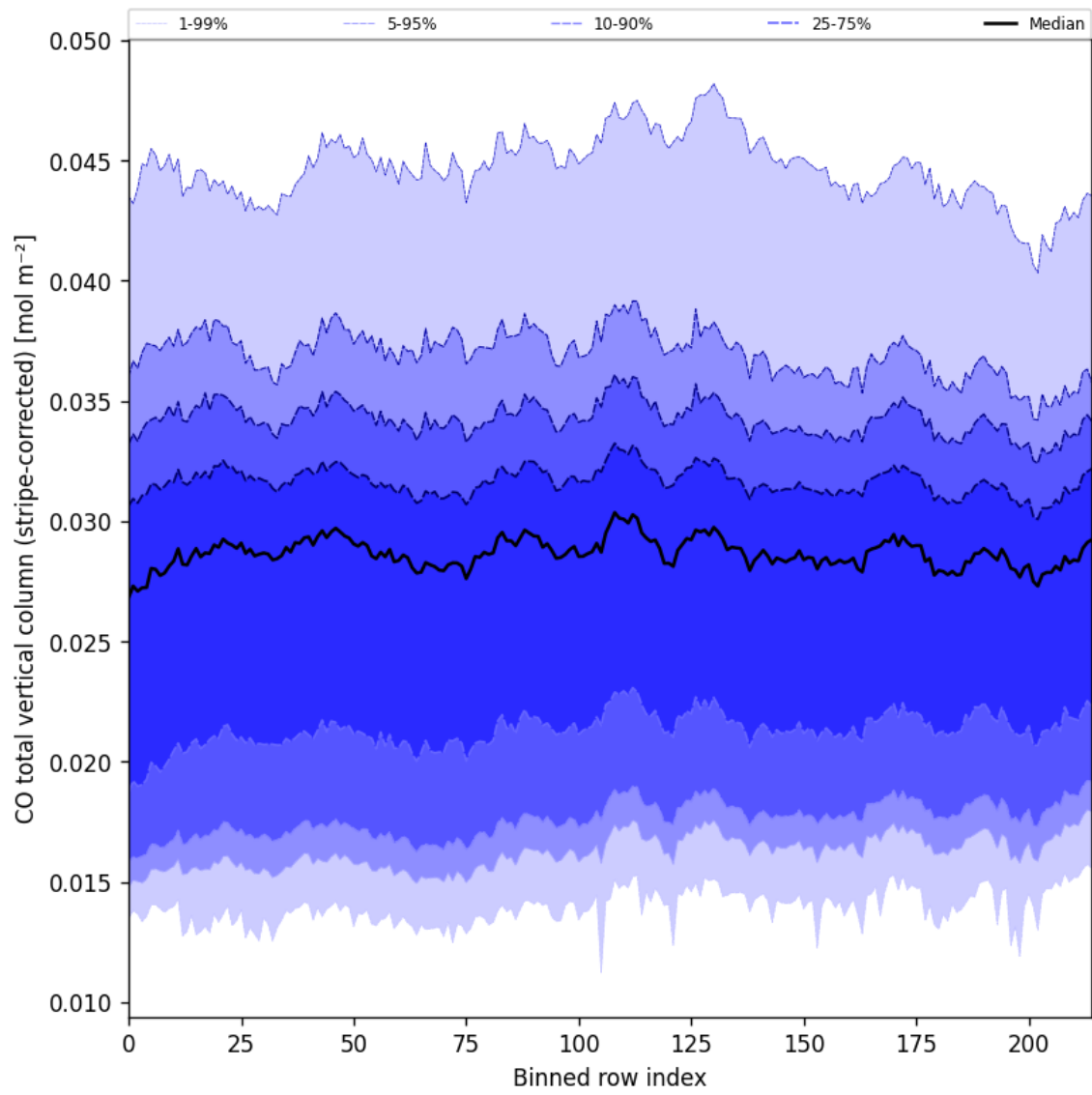
Figure 27: Along track statistics of “CO total vertical column (stripe-corrected)” for 2025-05-13 to 2025-05-15
