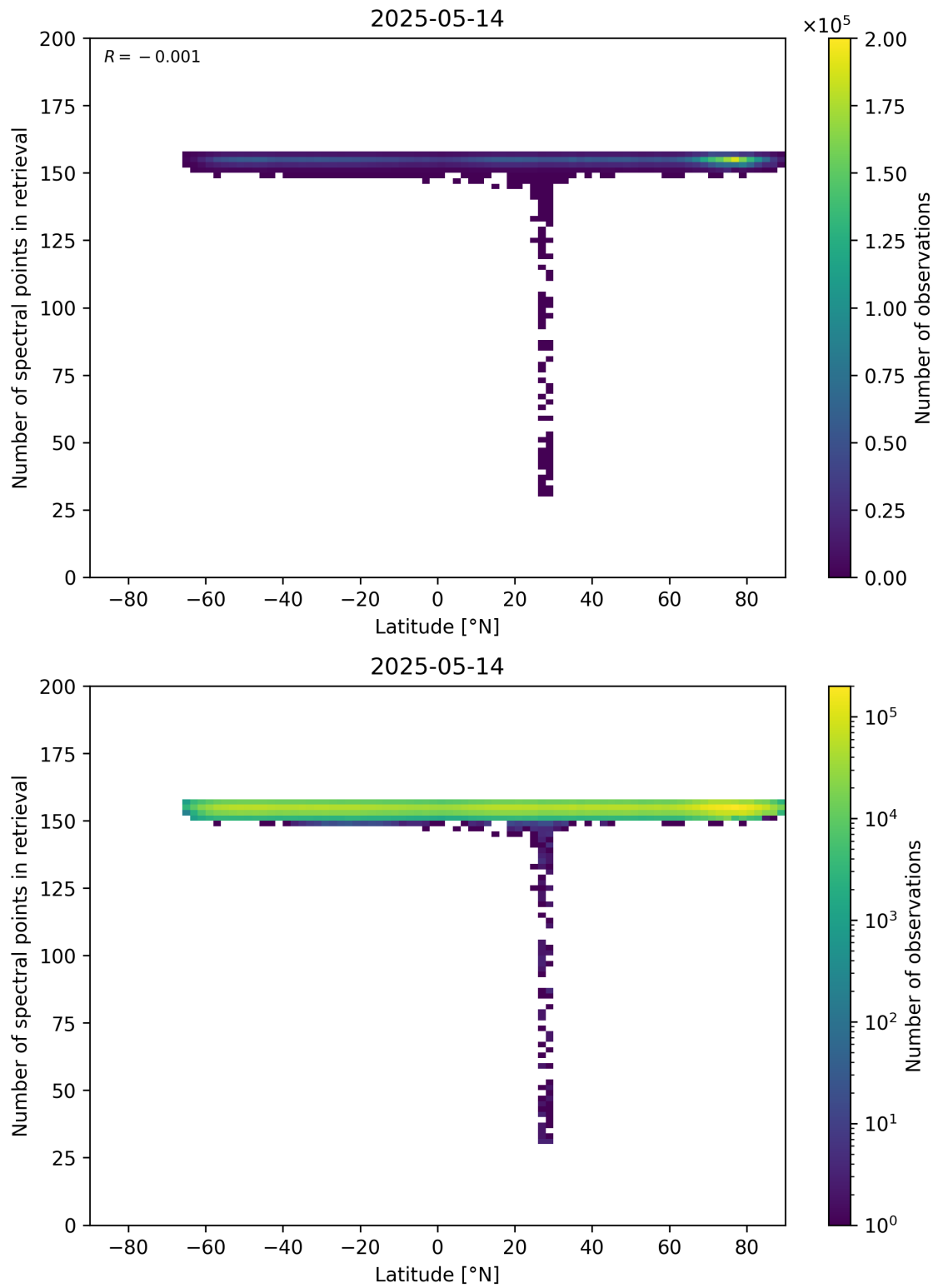
Figure 57: Scatter density plot of “Latitude” against “Number of spectral points in retrieval” for 2025-05-13 to 2025-05-15.
