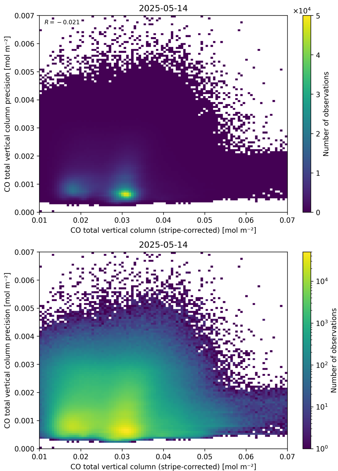
Figure 36: Scatter density plot of “CO total vertical column (stripe-corrected)” against “CO total vertical column precision” for 2025-05-13 to 2025-05-15.
