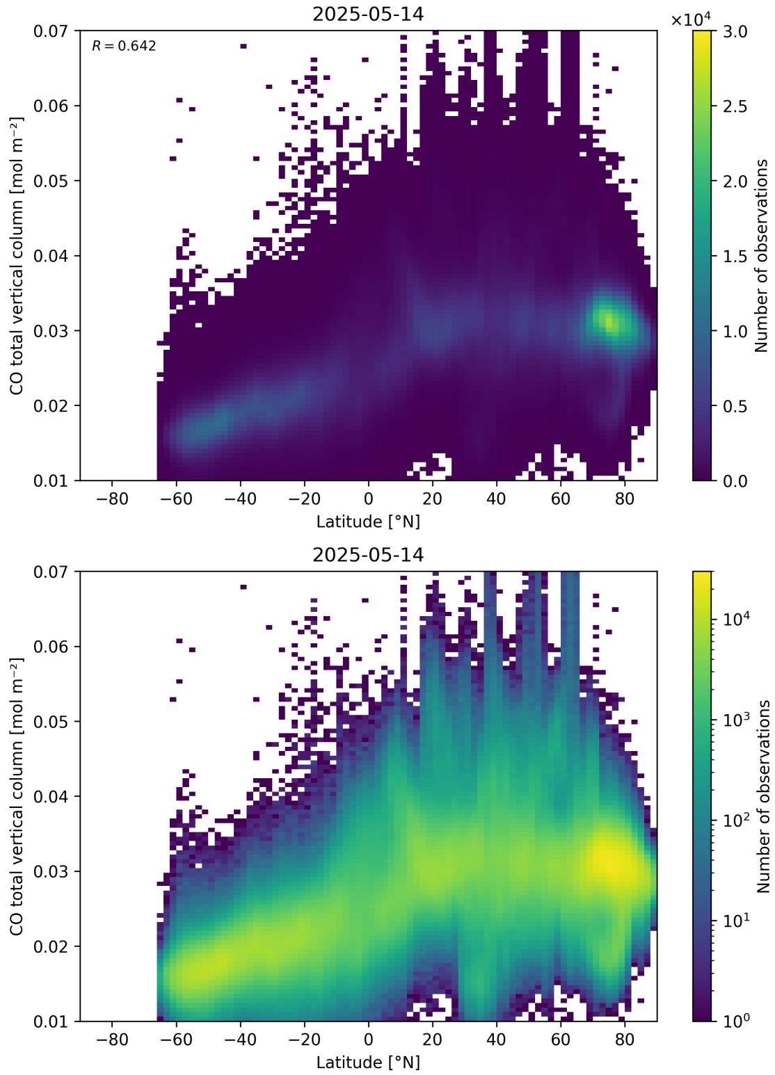
Figure 51: Scatter density plot of “Latitude” against “CO total vertical column” for 2025-05-13 to 2025-05-15.
