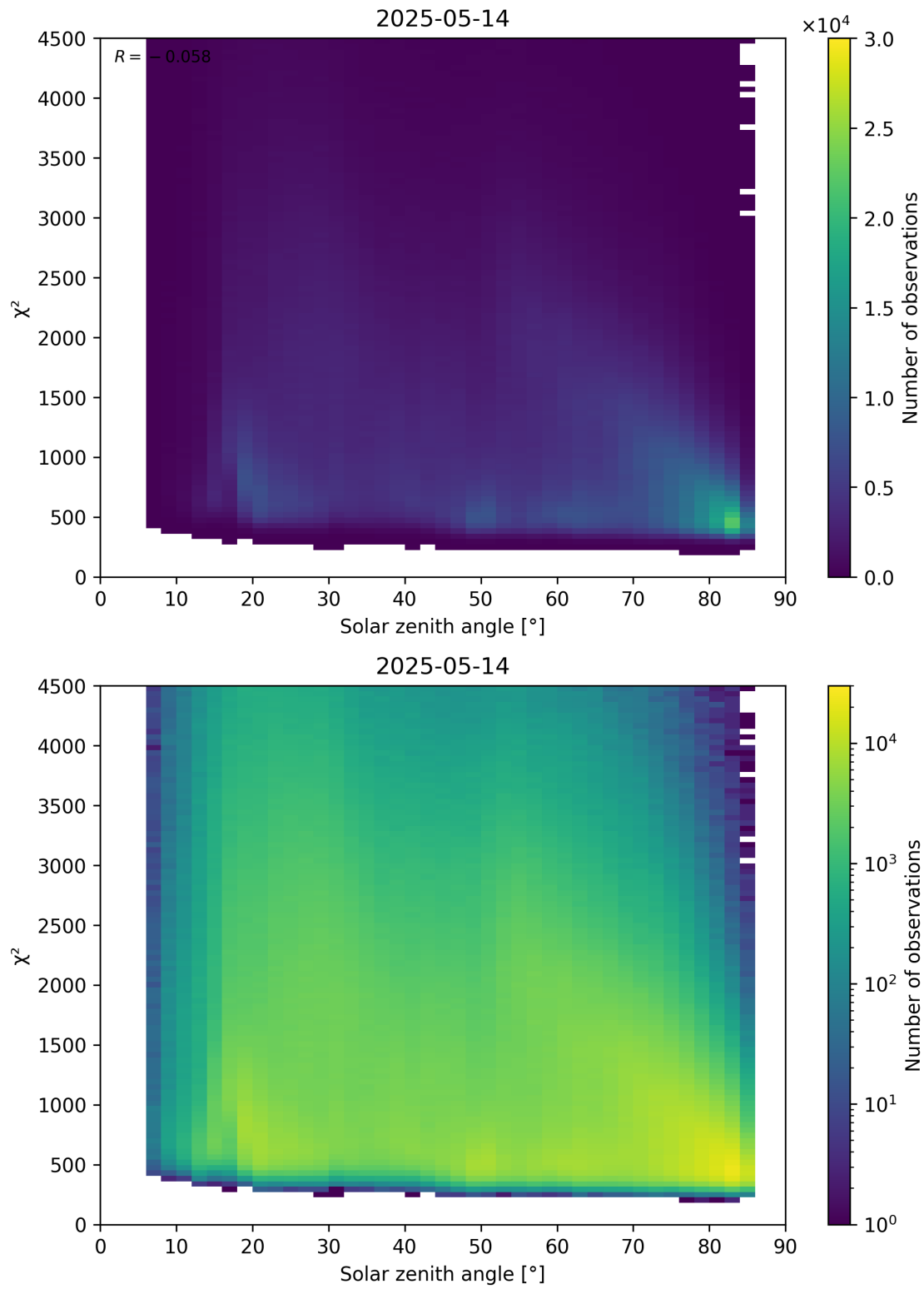
Figure 64: Scatter density plot of “Solar zenith angle” against “ \chi^2 ” for 2025-05-13 to 2025-05-15.
