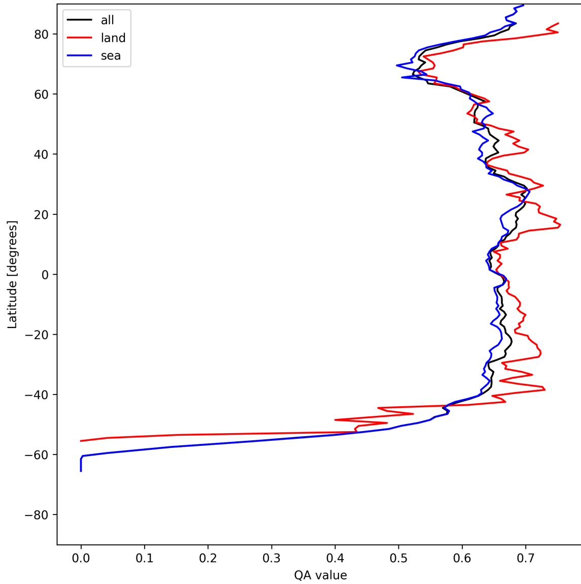
Figure 9: Zonal average of “QA value” for 2025-05-13 to 2025-05-15.
