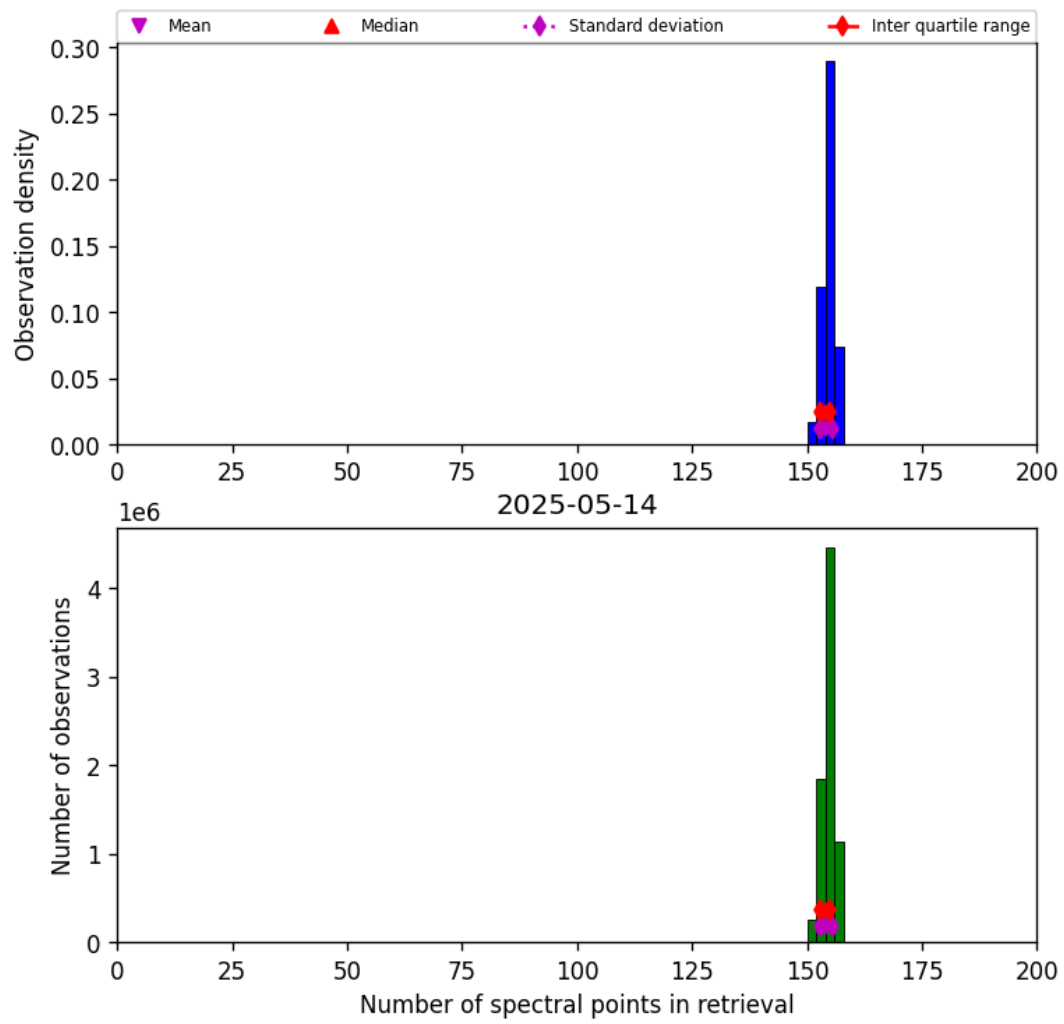
Figure 21: Histogram of “Number of spectral points in retrieval” for 2025-05-13 to 2025-05-15
