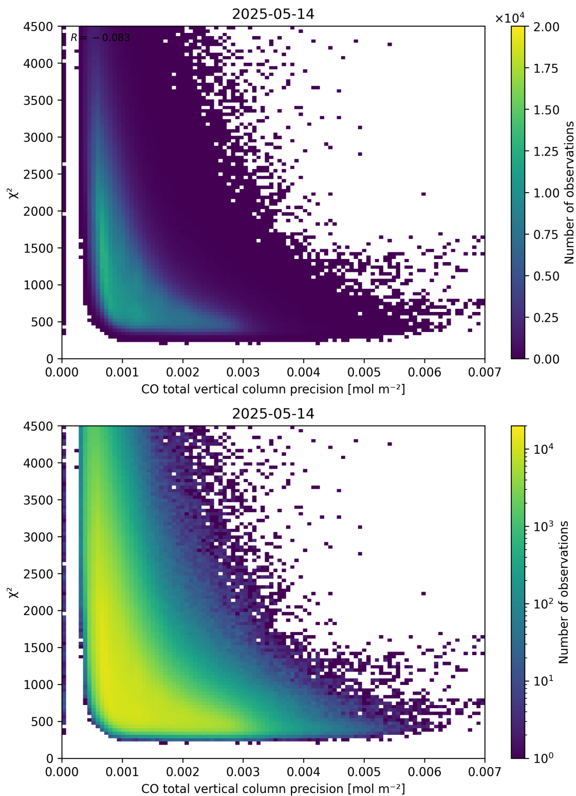
Figure 44: Scatter density plot of “CO total vertical column precision” against “ \chi^2 ” for 2025-05-13 to 2025-05-15.
