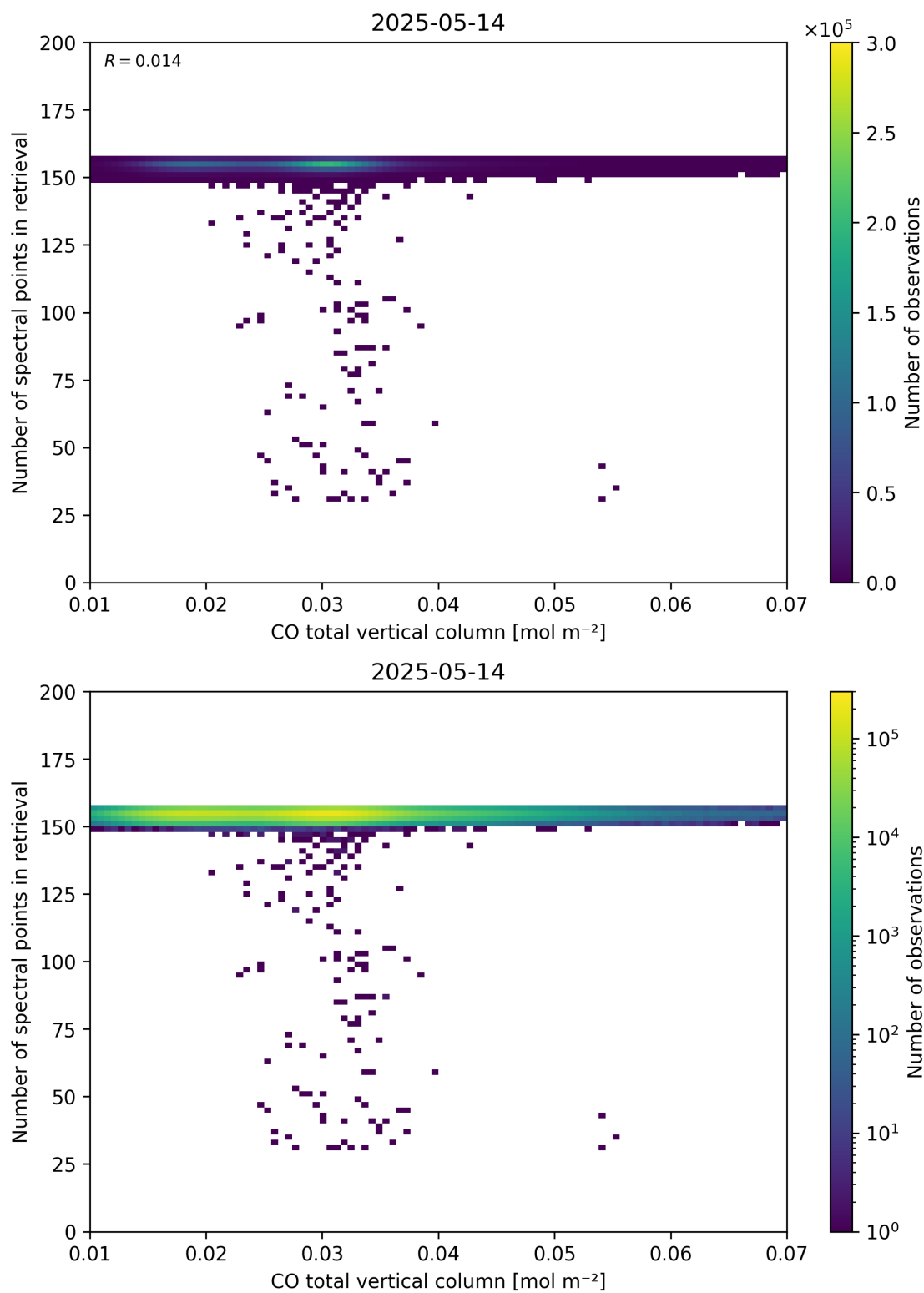
Figure 43: Scatter density plot of “CO total vertical column” against “Number of spectral points in retrieval” for 2025-05-13 to 2025-05-15.
