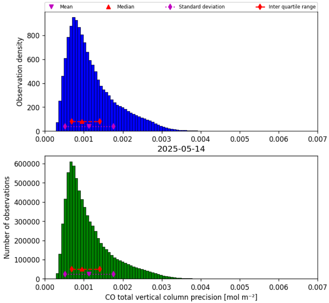
Figure 20: Histogram of “CO total vertical column precision” for 2025-05-13 to 2025-05-15
