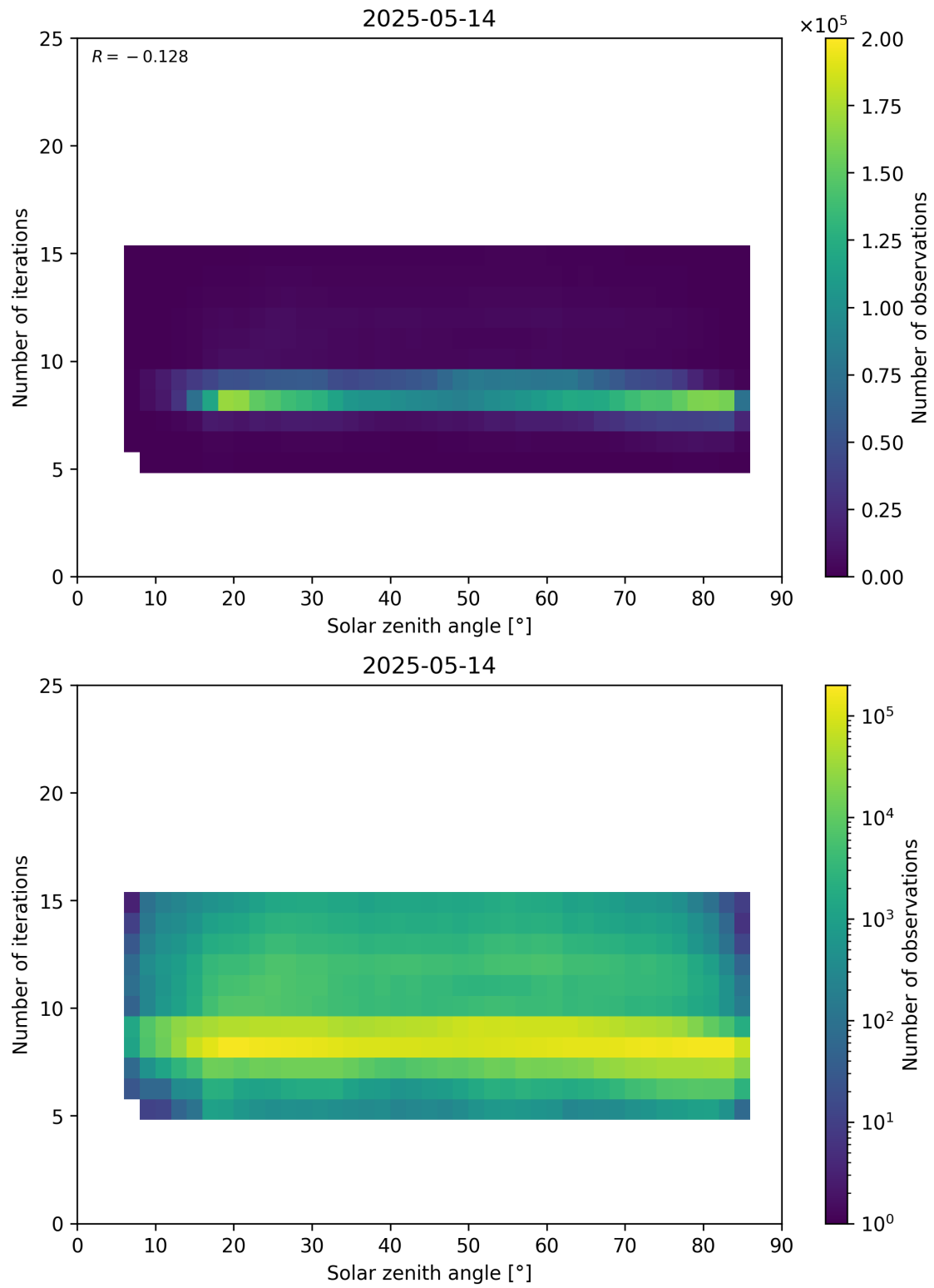
Figure 67: Scatter density plot of “Solar zenith angle” against “Number of iterations” for 2025-05-13 to 2025-05-15.
