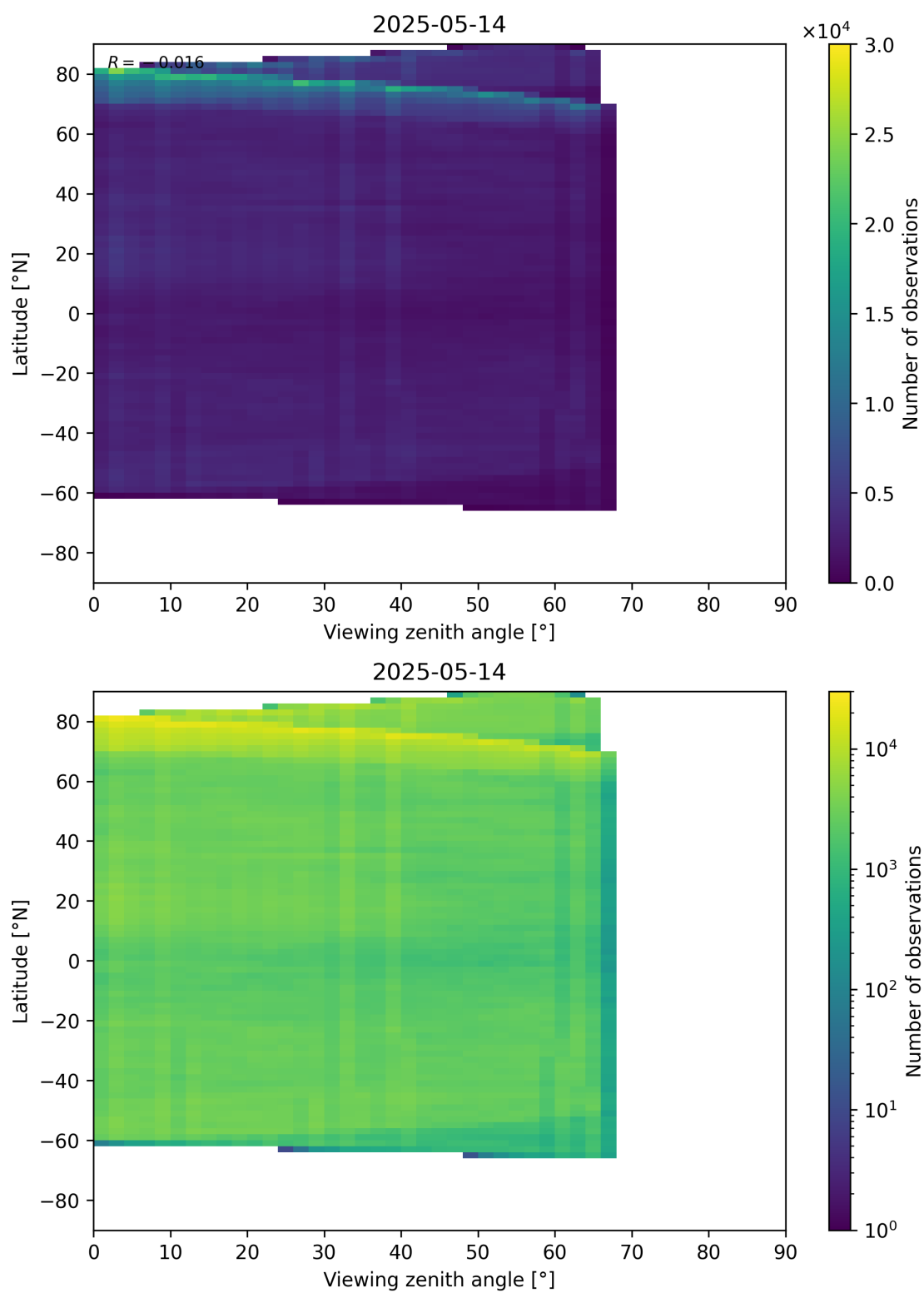
Figure 74: Scatter density plot of “Viewing zenith angle” against “Latitude” for 2025-05-13 to 2025-05-15.
