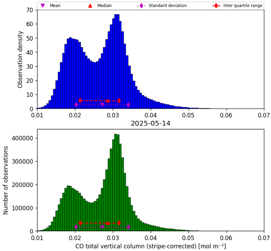
Figure 19: Histogram of “CO total vertical column (stripe-corrected)” for 2025-05-13 to 2025-05-15
