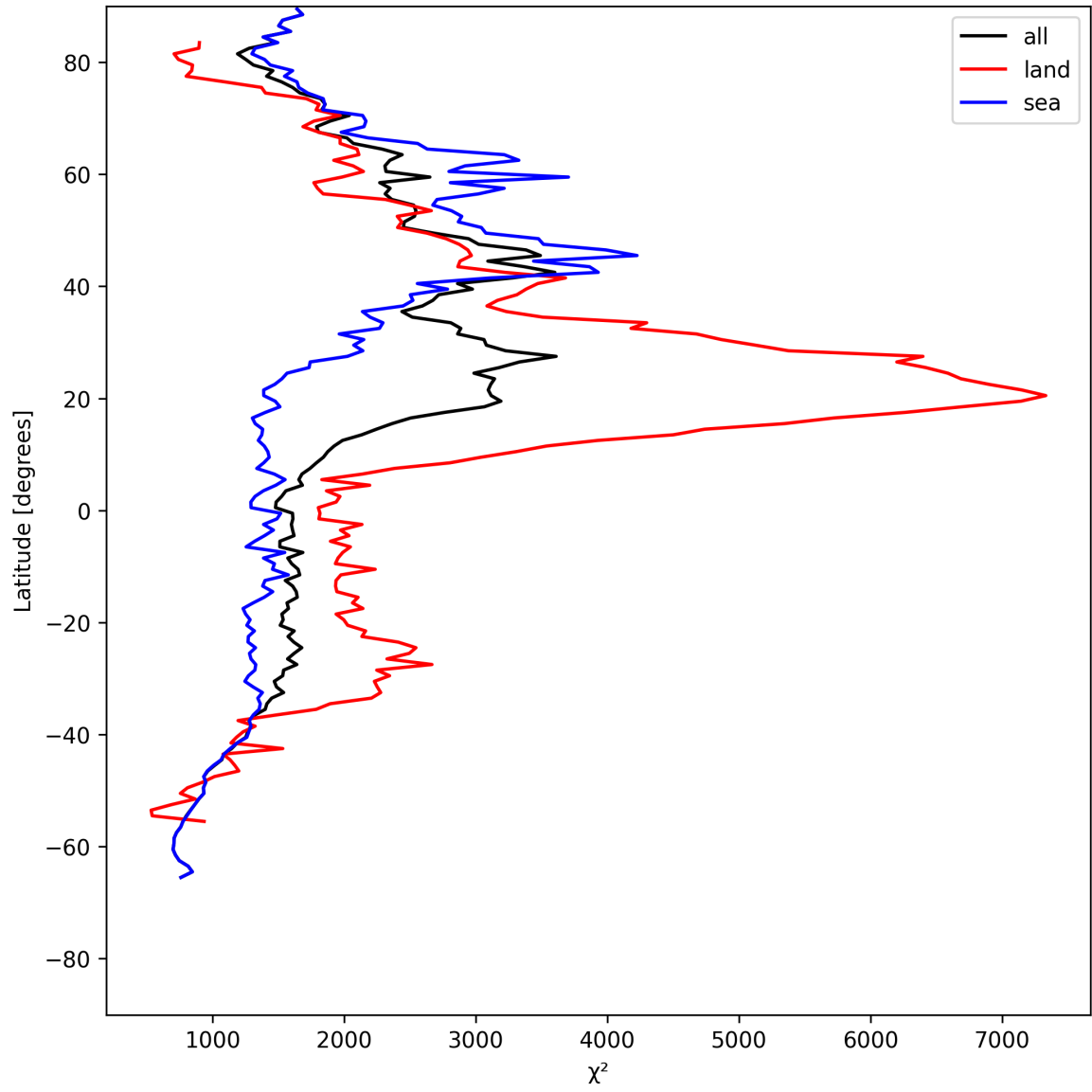
Figure 14: Zonal average of “ \chi^2 ” for 2025-05-13 to 2025-05-15.
