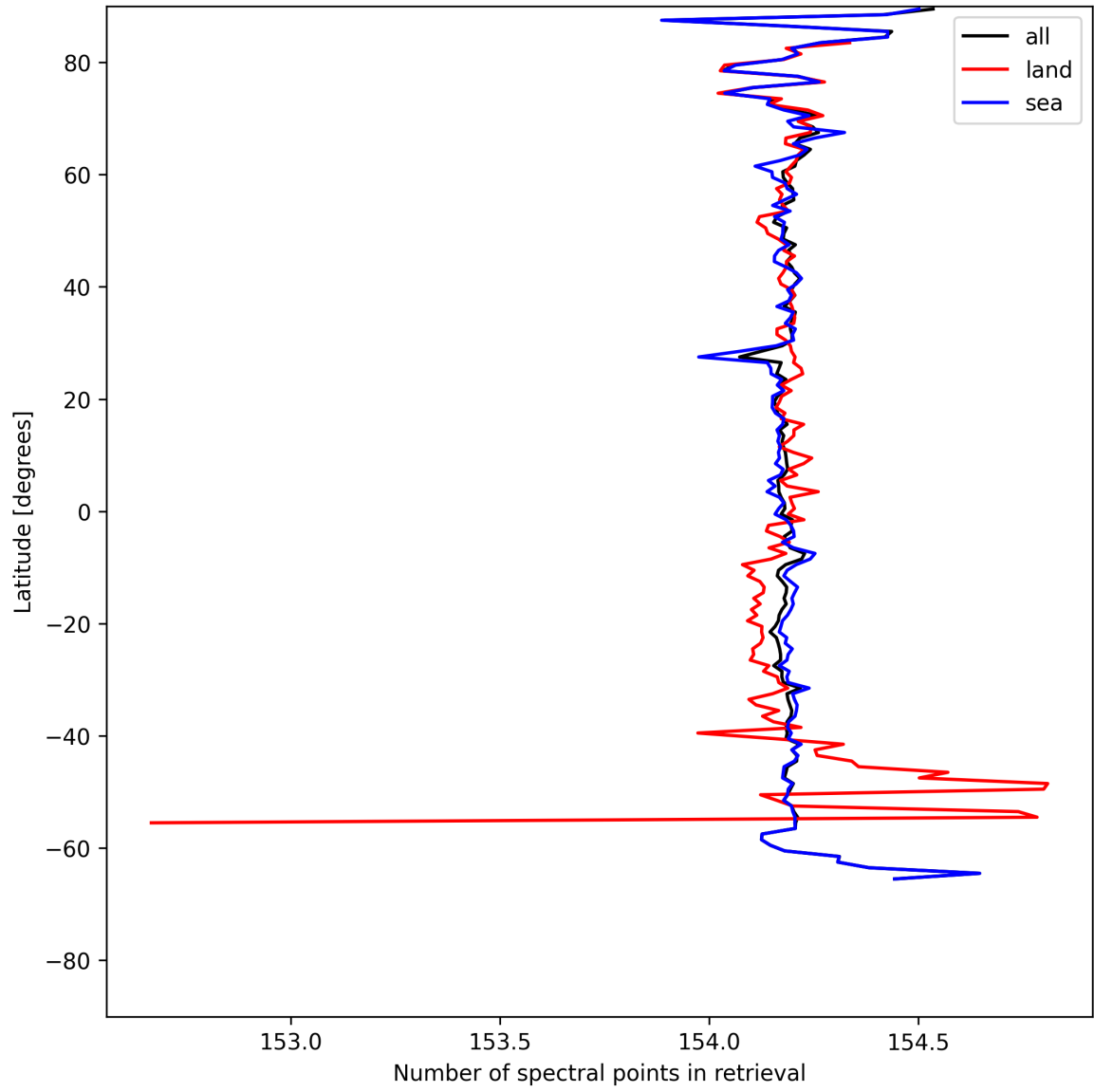
Figure 13: Zonal average of “Number of spectral points in retrieval” for 2025-05-13 to 2025-05-15.
