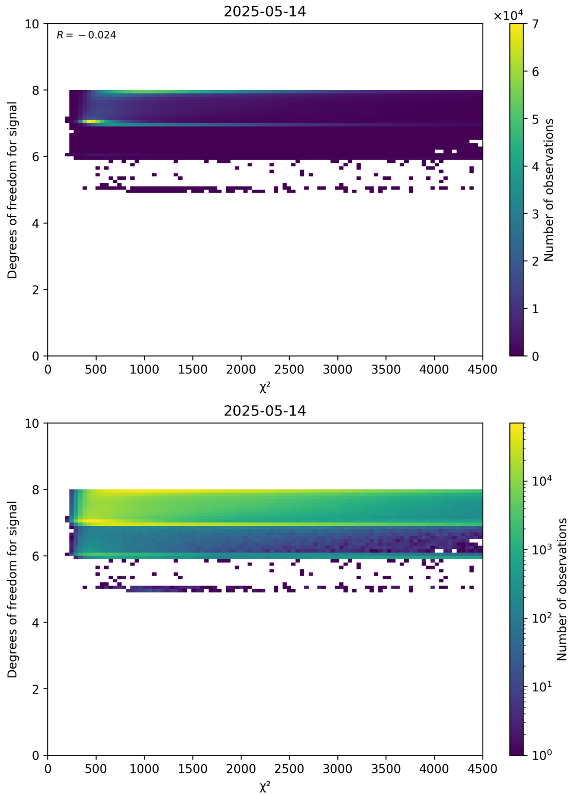
Figure 48: Scatter density plot of “ \chi^2 ” against “Degrees of freedom for signal” for 2025-05-13 to 2025-05-15.
