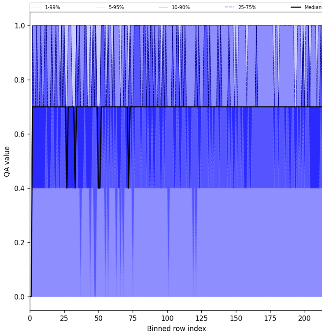
Figure 25: Along track statistics of “QA value” for 2025-05-13 to 2025-05-15
