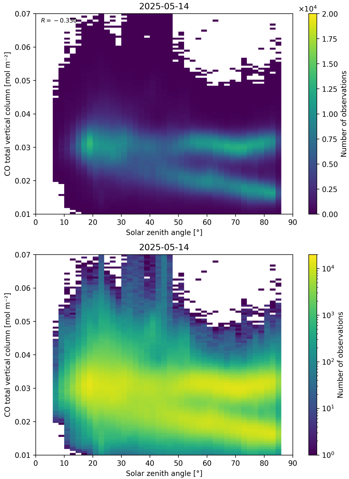
Figure 61: Scatter density plot of “Solar zenith angle” against “CO total vertical column” for 2025-05-13 to 2025-05-15.
