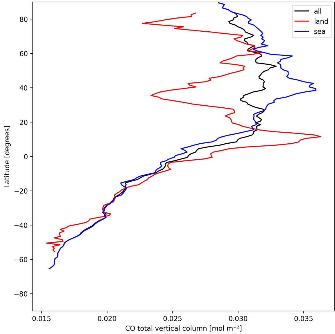
Figure 10: Zonal average of “CO total vertical column” for 2025-05-13 to 2025-05-15.
