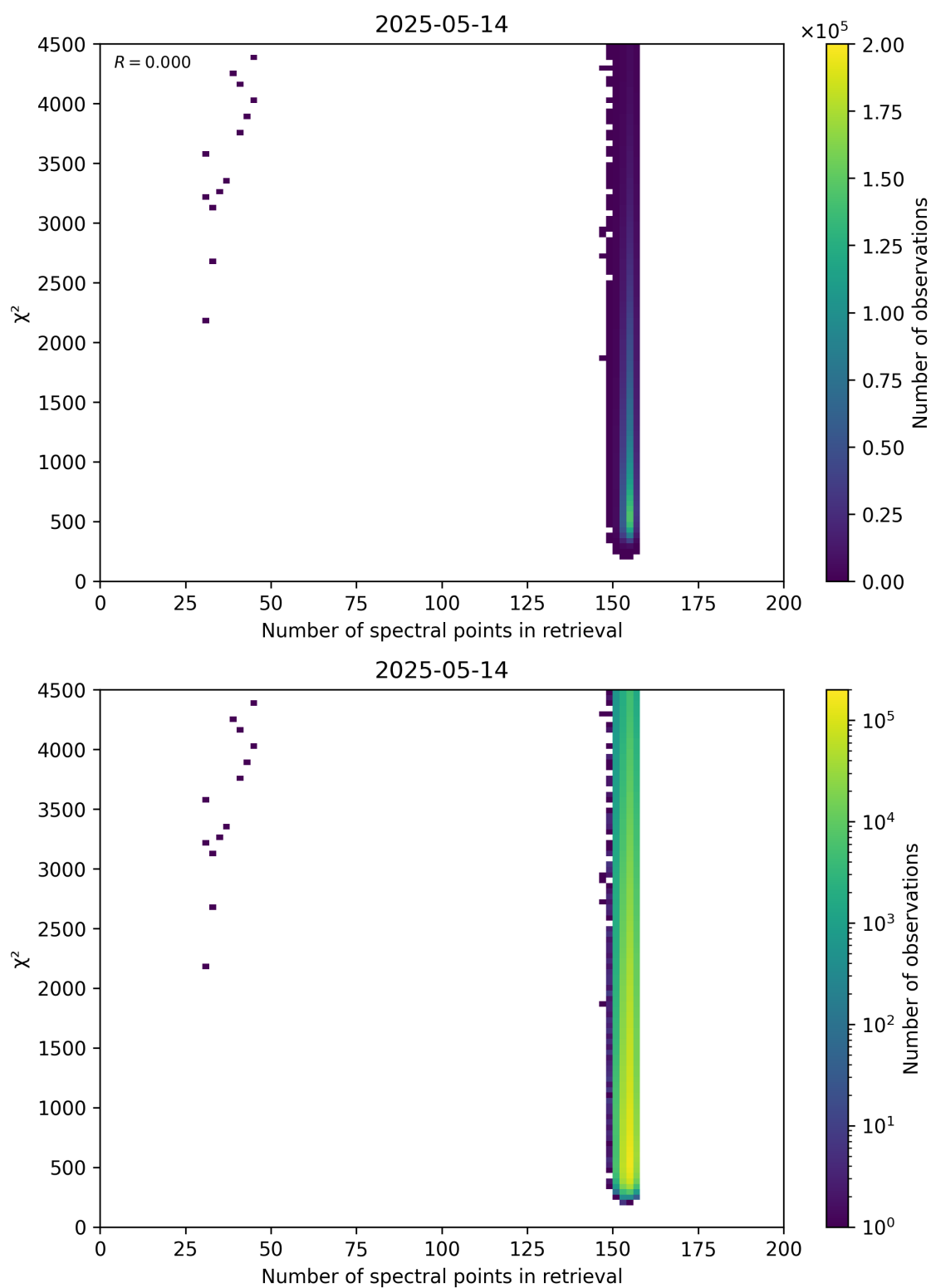
Figure 58: Scatter density plot of “Number of spectral points in retrieval” against “ \chi^2 ” for 2025-05-13 to 2025-05-15.
