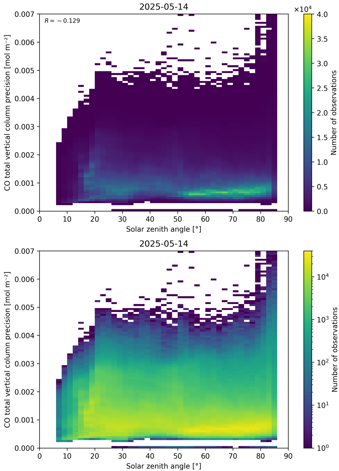
Figure 63: Scatter density plot of “Solar zenith angle” against “CO total vertical column precision” for 2025-05-13 to 2025-05-15.
