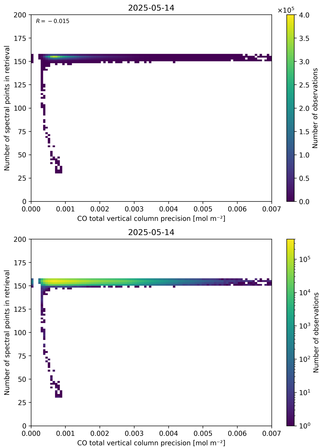
Figure 47: Scatter density plot of “CO total vertical column precision” against “Number of spectral points in retrieval” for 2025-05-13 to 2025-05-15.
