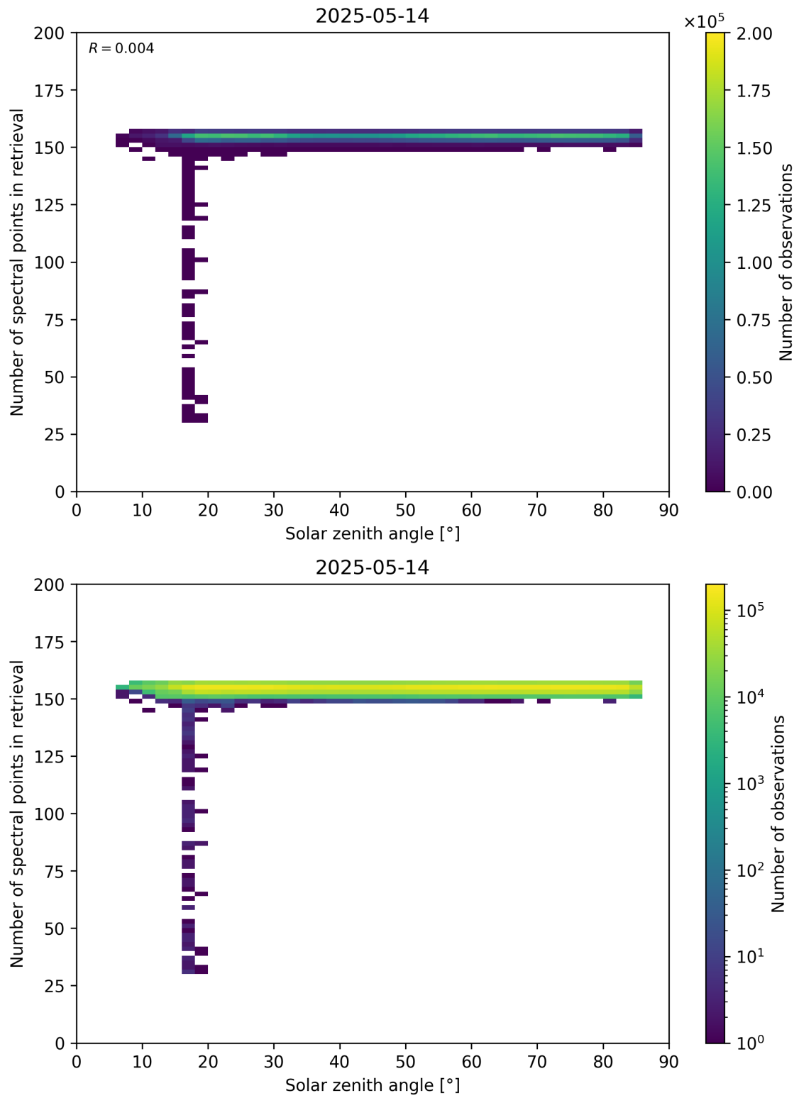
Figure 68: Scatter density plot of “Solar zenith angle” against “Number of spectral points in retrieval” for 2025-05-13 to 2025-05-15.
