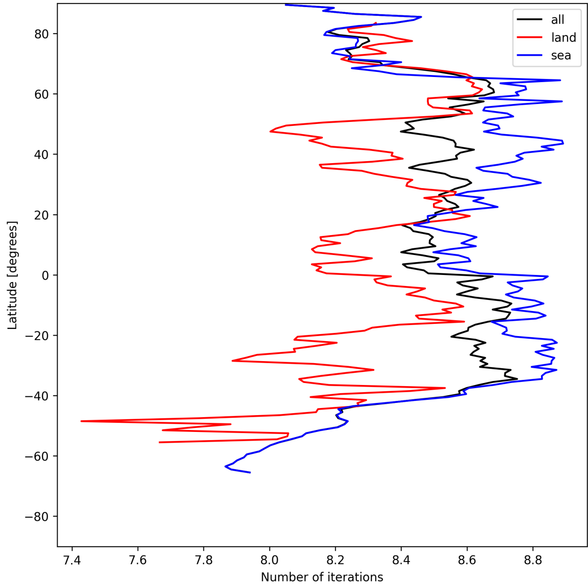
Figure 16: Zonal average of “Number of iterations” for 2025-05-13 to 2025-05-15.
