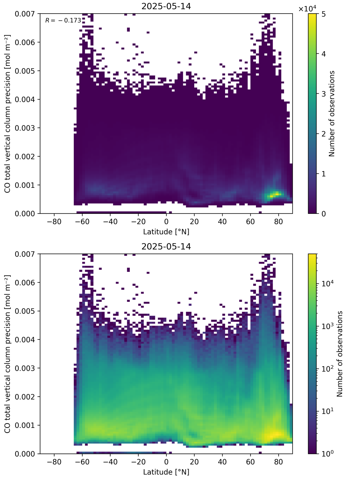
Figure 53: Scatter density plot of “Latitude” against “CO total vertical column precision” for 2025-05-13 to 2025-05-15.
