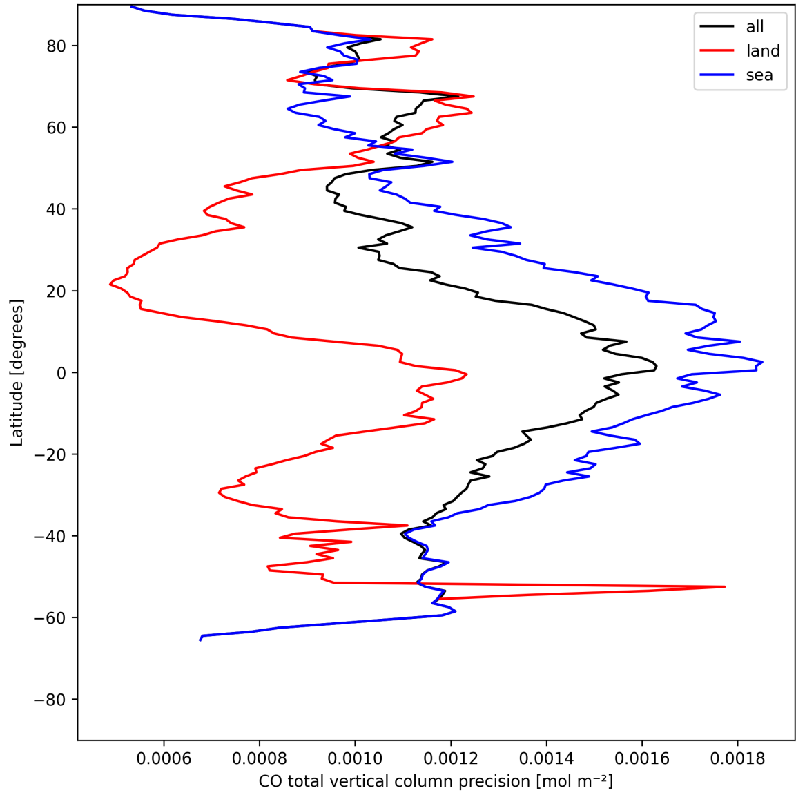
Figure 12: Zonal average of “CO total vertical column precision” for 2025-05-13 to 2025-05-15.
