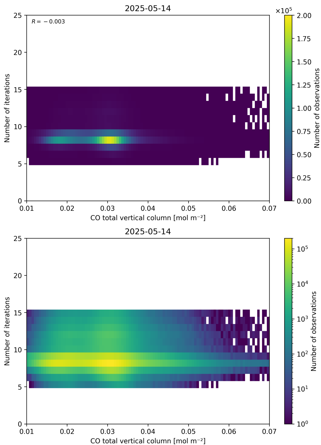
Figure 42: Scatter density plot of “CO total vertical column” against “Number of iterations” for 2025-05-13 to 2025-05-15.
