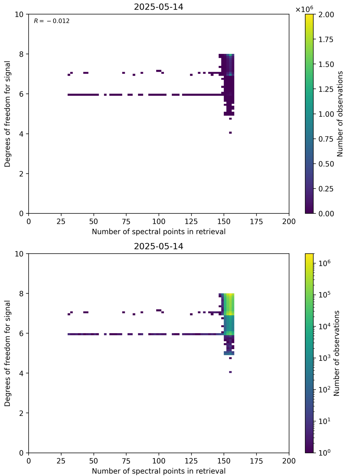
Figure 59: Scatter density plot of “Number of spectral points in retrieval” against “Degrees of freedom for signal” for 2025-05-13 to 2025-05-15.
