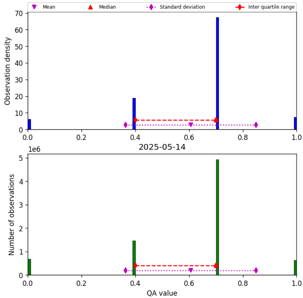
Figure 17: Histogram of "QA value" for 2025-05-13 to 2025-05-15
