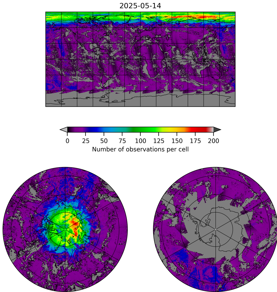
Figure 8: Map of the number of observations for 2025-05-13 to 2025-05-15
