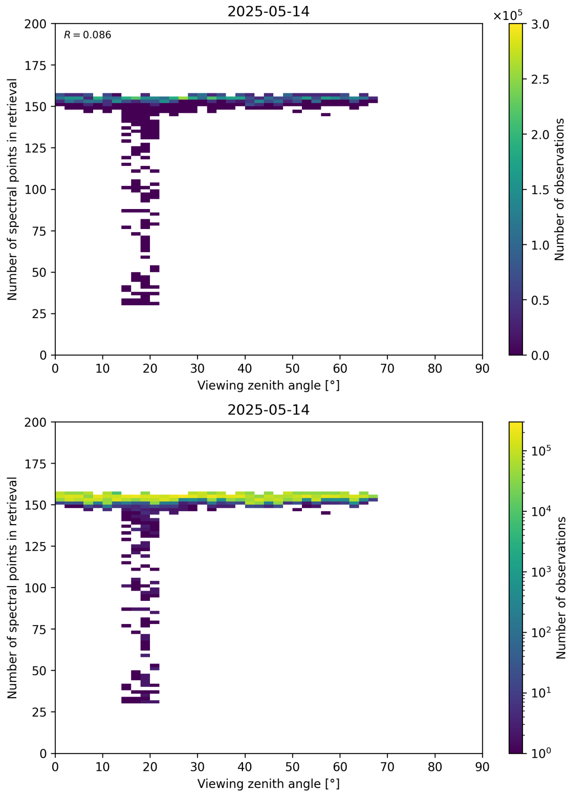
Figure 76: Scatter density plot of “Viewing zenith angle” against “Number of spectral points in retrieval” for 2025-05-13 to 2025-05-15.
