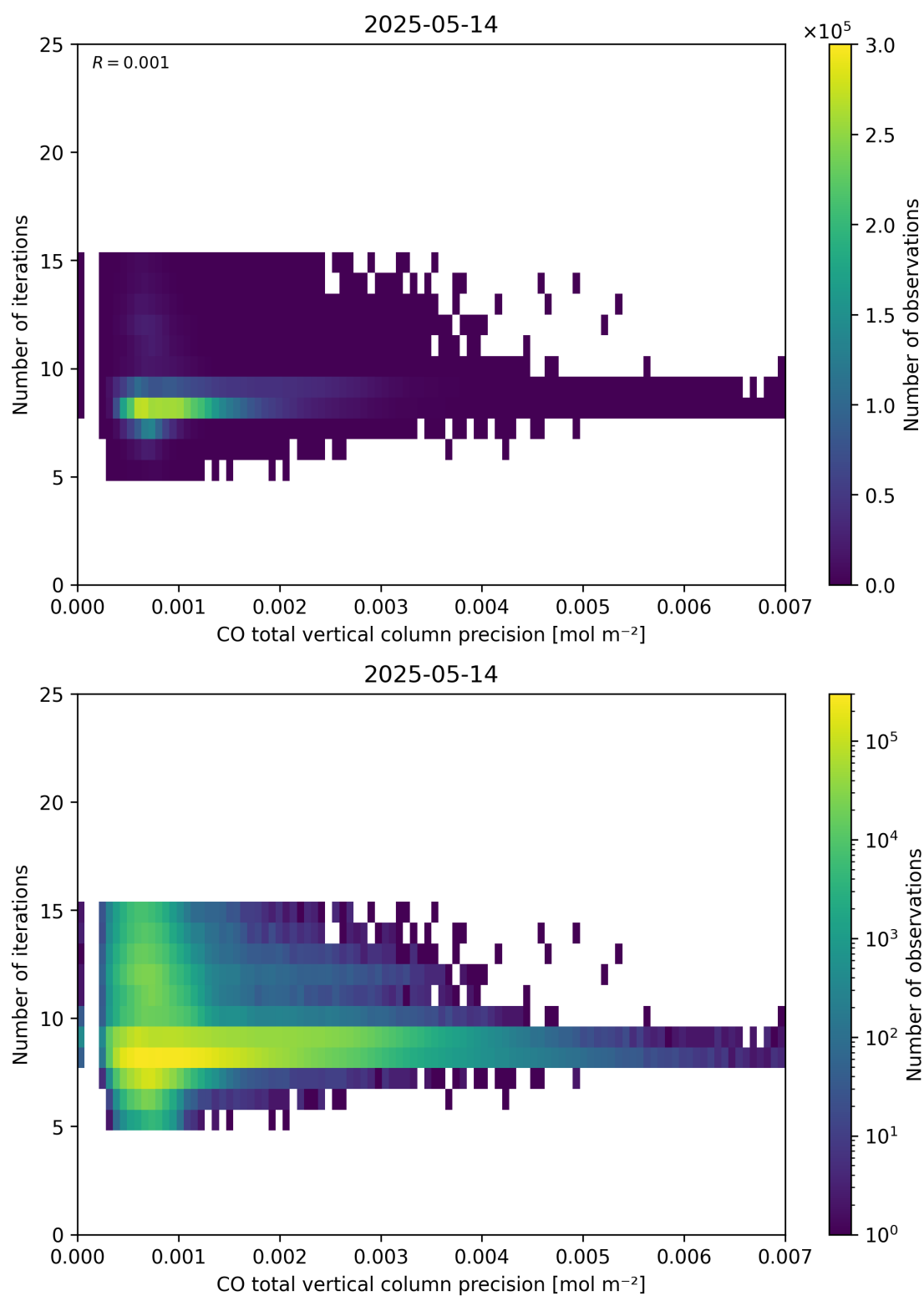
Figure 46: Scatter density plot of “CO total vertical column precision” against “Number of iterations” for 2025-05-13 to 2025-05-15.
