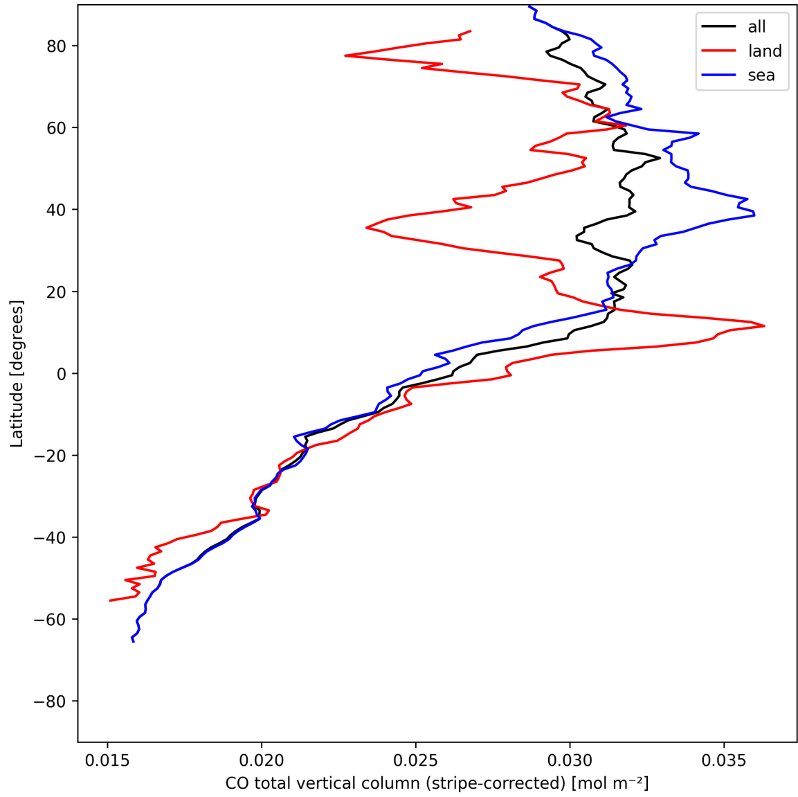
Figure 11: Zonal average of “CO total vertical column (stripe-corrected)” for 2025-05-13 to 2025-05-15.
