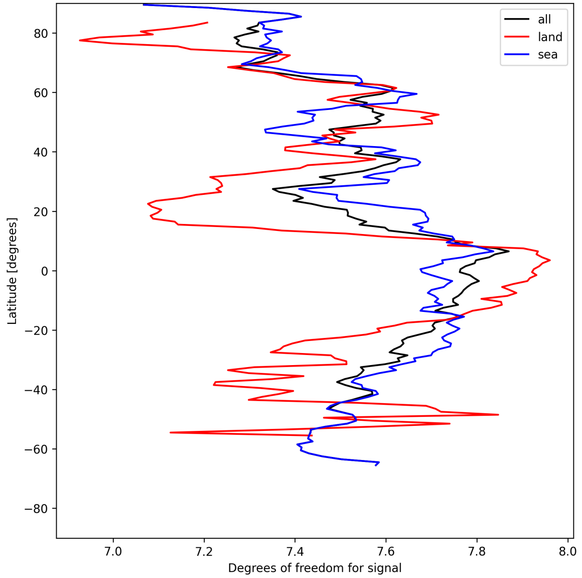
Figure 15: Zonal average of “Degrees of freedom for signal” for 2025-05-13 to 2025-05-15.
