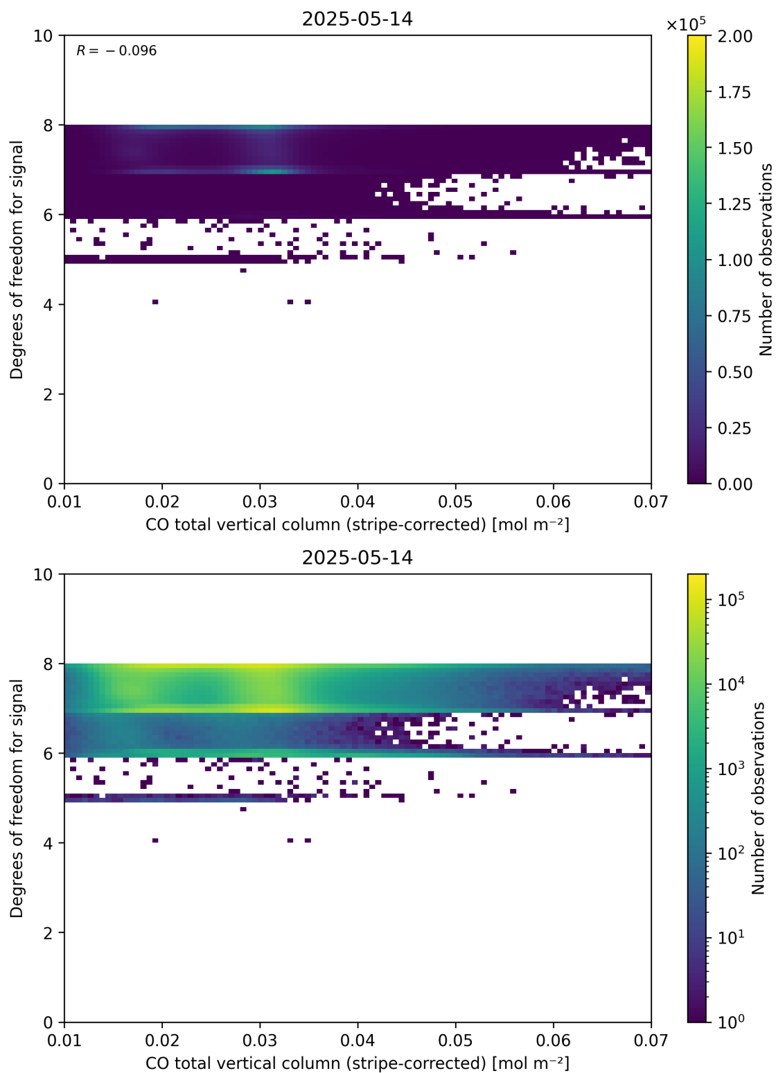
Figure 38: Scatter density plot of “CO total vertical column (stripe-corrected)” against “Degrees of freedom for signal” for 2025-05-13 to 2025-05-15.
