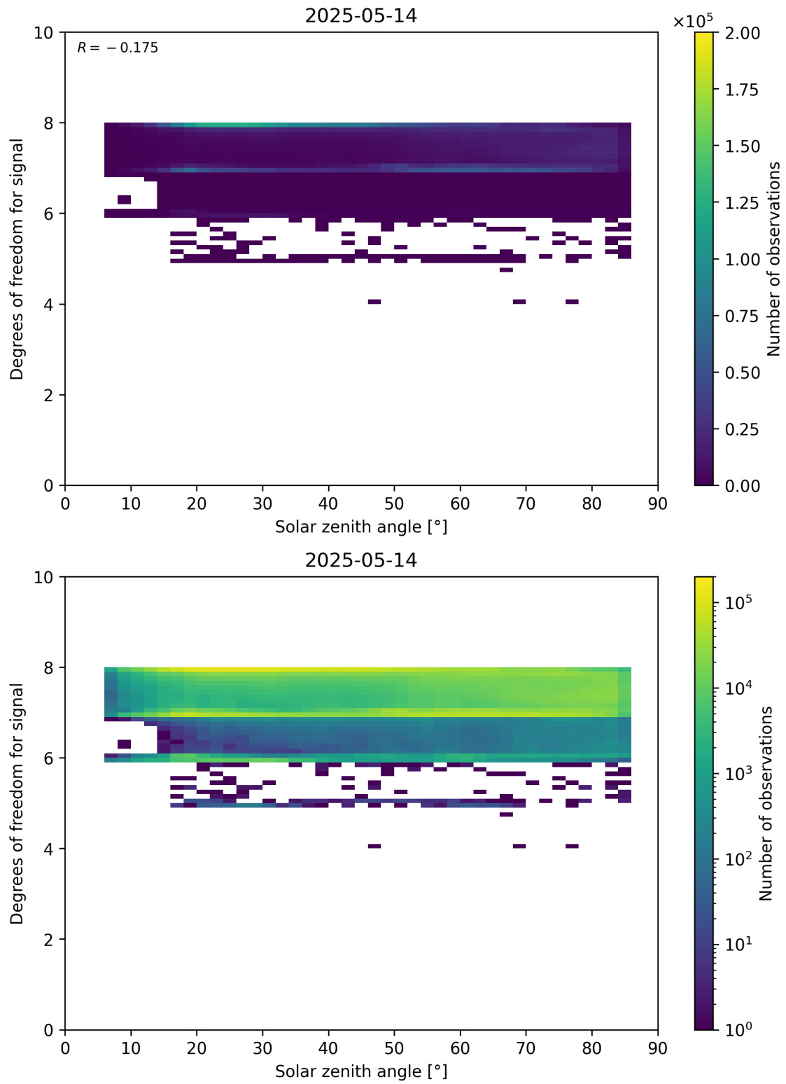
Figure 65: Scatter density plot of “Solar zenith angle” against “Degrees of freedom for signal” for 2025-05-13 to 2025-05-15.
