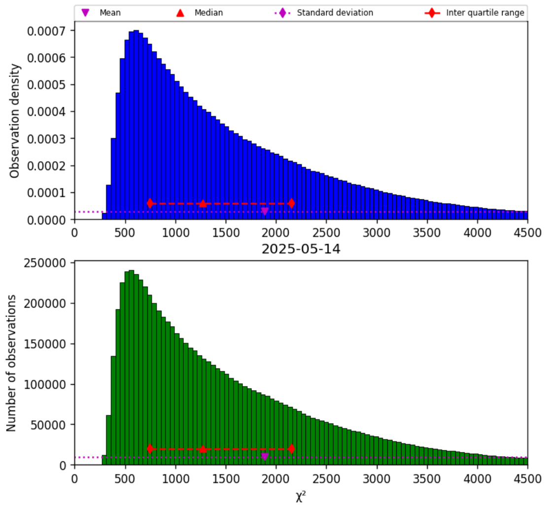
Figure 22: Histogram of “ \chi^2 ” for 2025-05-13 to 2025-05-15
