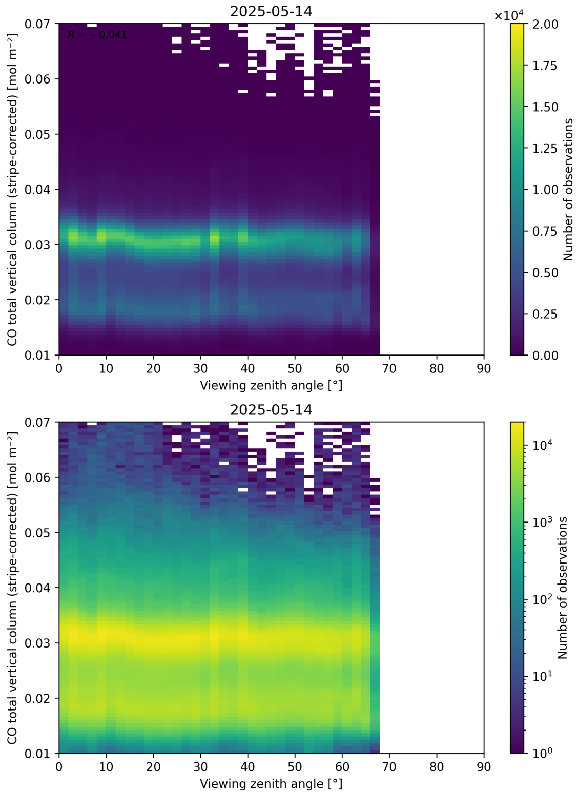
Figure 70: Scatter density plot of “Viewing zenith angle” against “CO total vertical column (stripe-corrected)” for 2025-05-13 to 2025-05-15.
