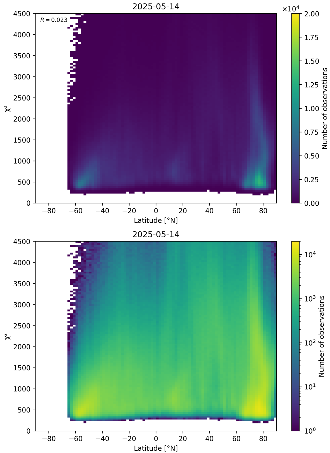
Figure 54: Scatter density plot of “Latitude” against “ \chi^2 ” for 2025-05-13 to 2025-05-15.
