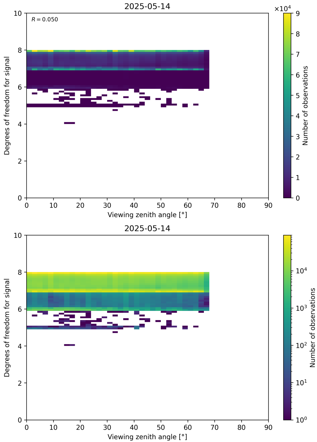
Figure 73: Scatter density plot of “Viewing zenith angle” against “Degrees of freedom for signal” for 2025-05-13 to 2025-05-15.
