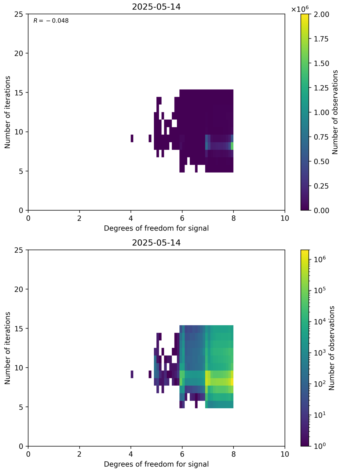
Figure 50: Scatter density plot of “Degrees of freedom for signal” against “Number of iterations” for 2025-05-13 to 2025-05-15.
