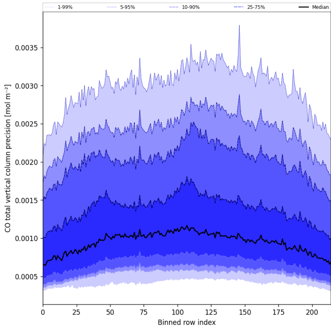
Figure 28: Along track statistics of “CO total vertical column precision” for 2025-05-13 to 2025-05-15
