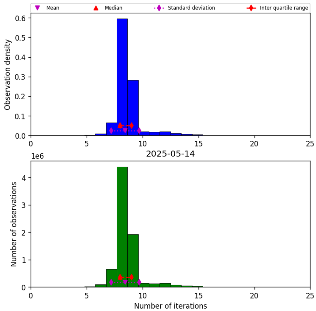
Figure 24: Histogram of “Number of iterations” for 2025-05-13 to 2025-05-15
