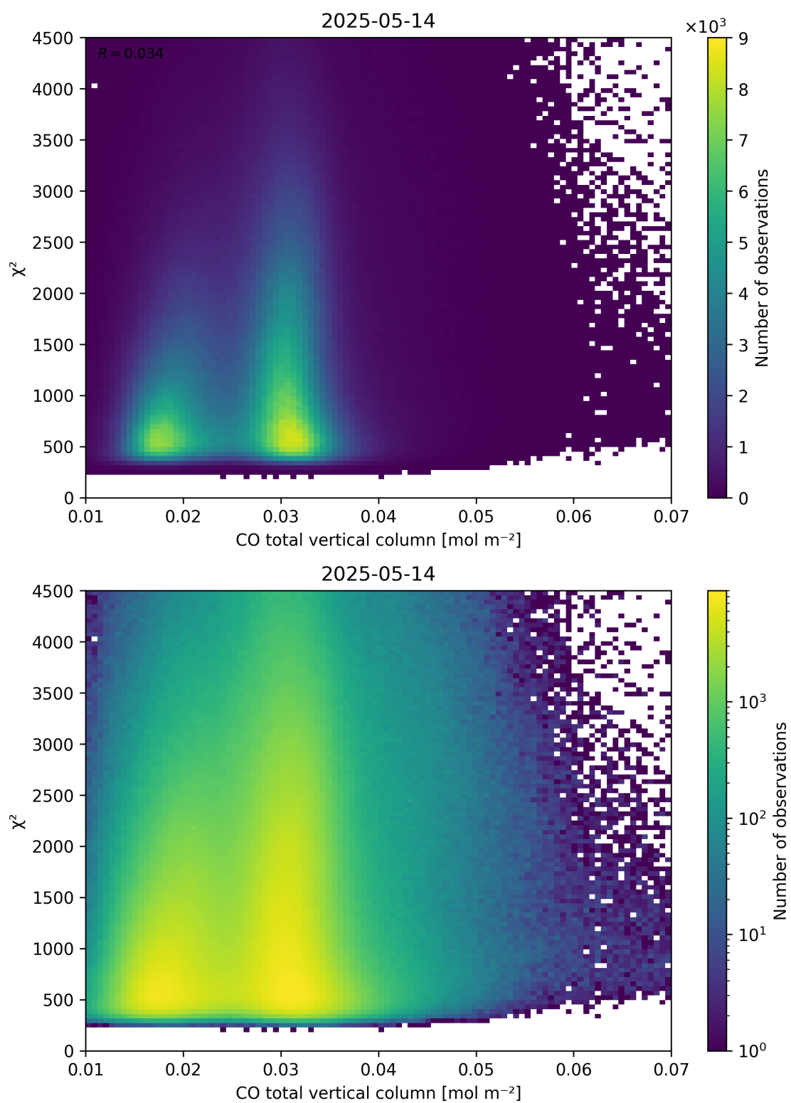
Figure 35: Scatter density plot of “CO total vertical column” against “ \chi^2 ” for 2025-05-13 to 2025-05-15.
