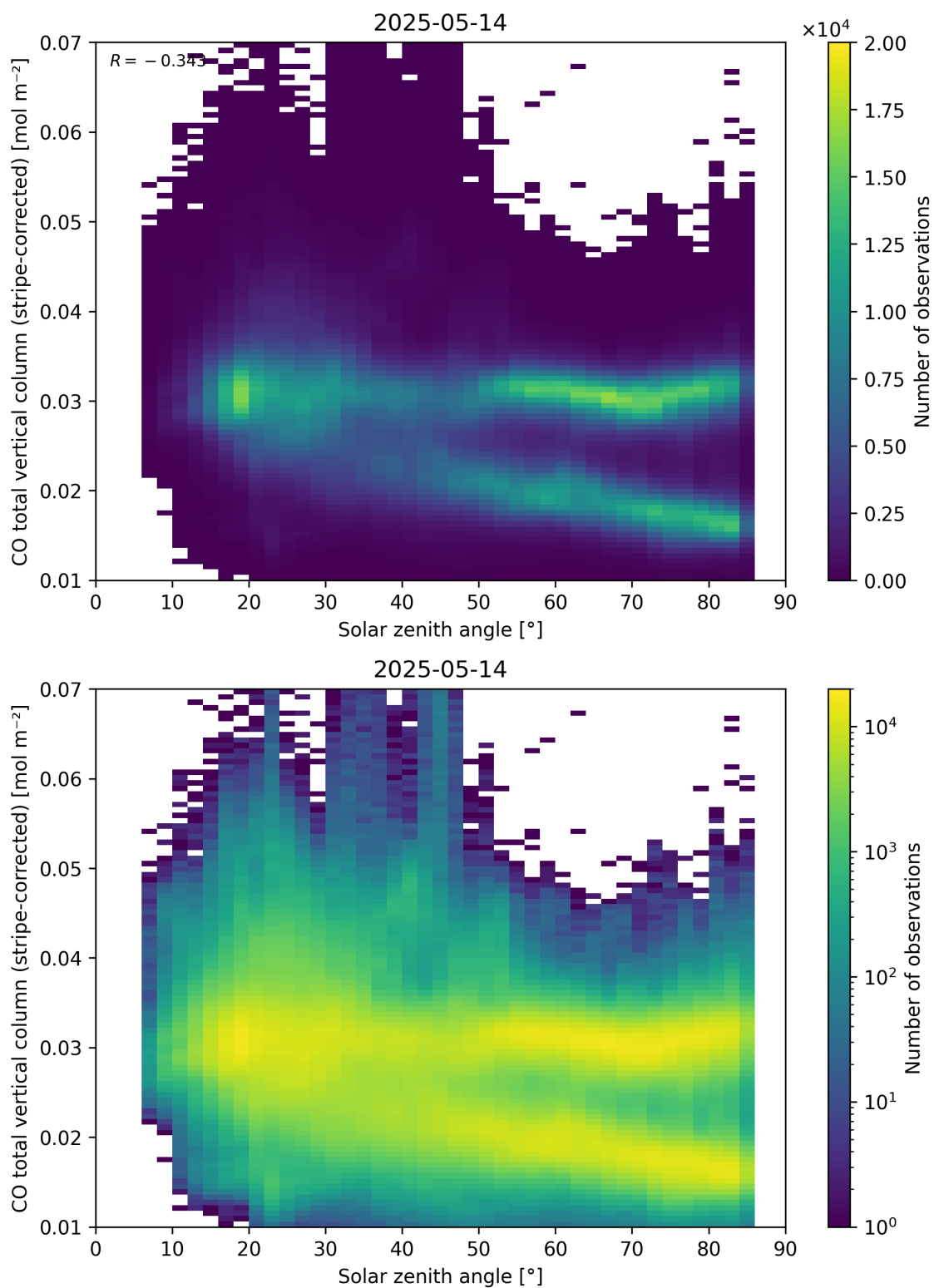
Figure 62: Scatter density plot of “Solar zenith angle” against “CO total vertical column (stripe-corrected)” for 2025-05-13 to 2025-05-15.
