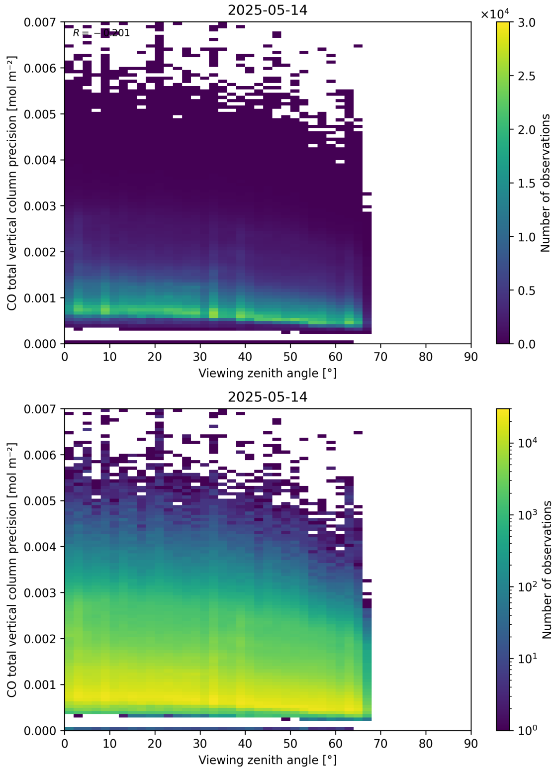
Figure 71: Scatter density plot of “Viewing zenith angle” against “CO total vertical column precision” for 2025-05-13 to 2025-05-15.
