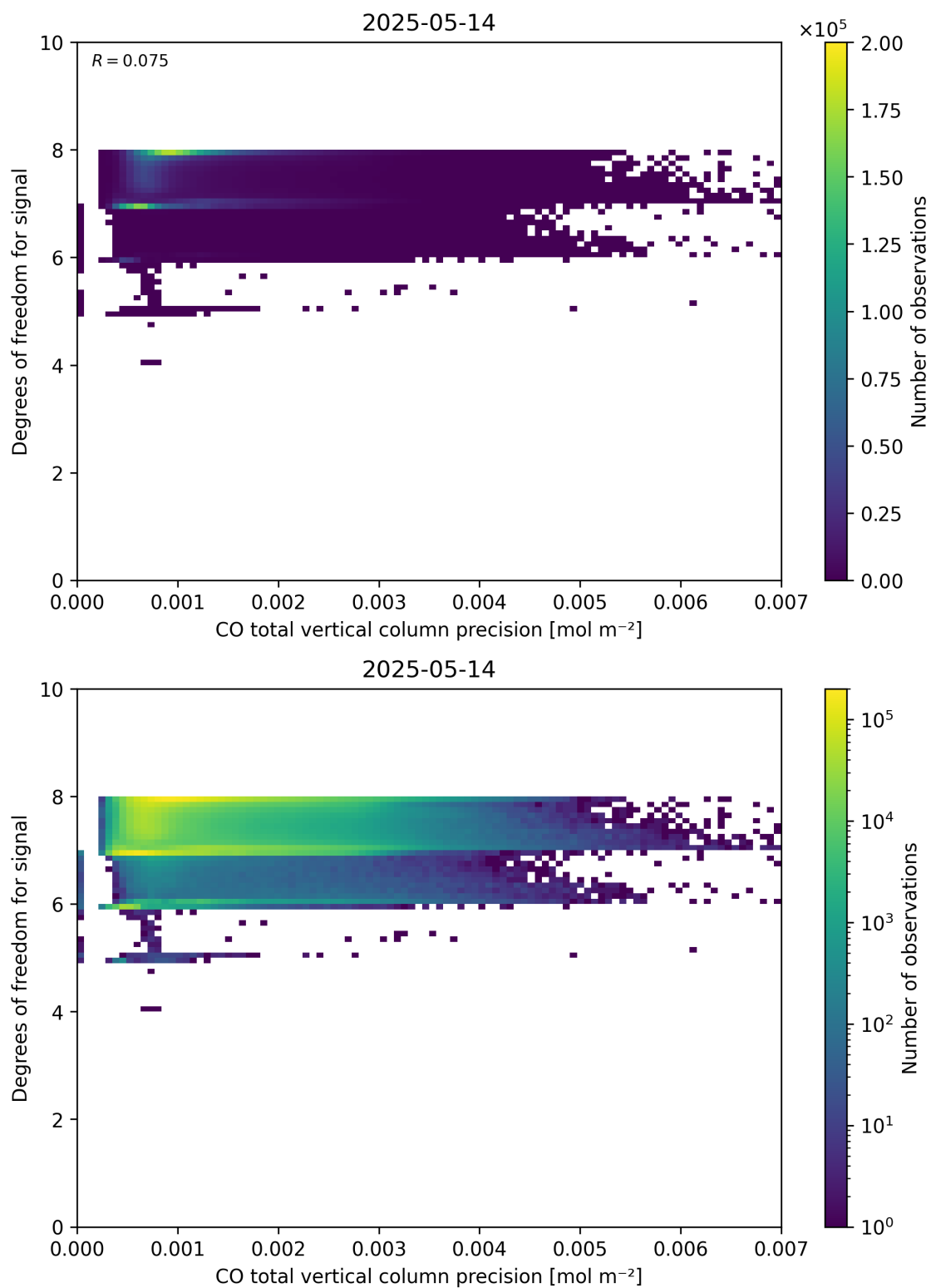
Figure 45: Scatter density plot of “CO total vertical column precision” against “Degrees of freedom for signal” for 2025-05-13 to 2025-05-15.
