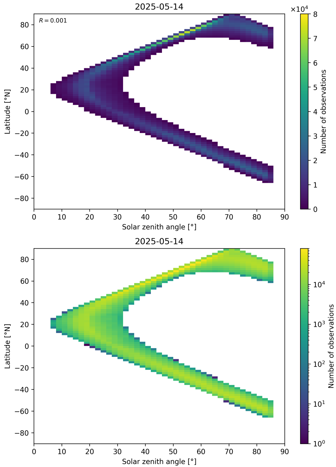
Figure 66: Scatter density plot of “Solar zenith angle” against “Latitude” for 2025-05-13 to 2025-05-15.
