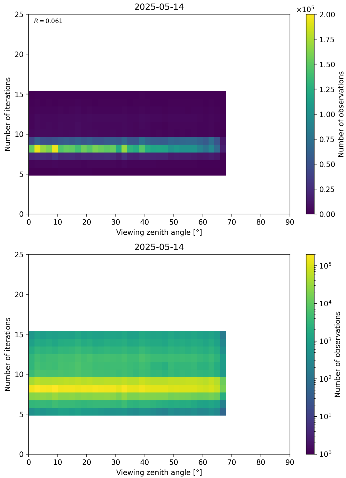
Figure 75: Scatter density plot of “Viewing zenith angle” against “Number of iterations” for 2025-05-13 to 2025-05-15.
