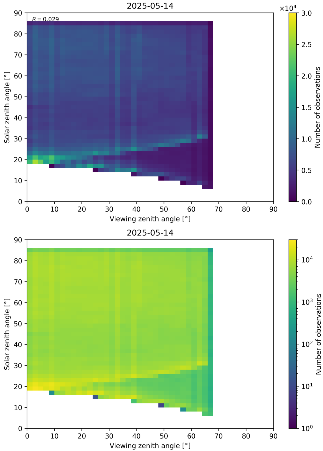
Figure 77: Scatter density plot of “Viewing zenith angle” against “Solar zenith angle” for 2025-05-13 to 2025-05-15.
