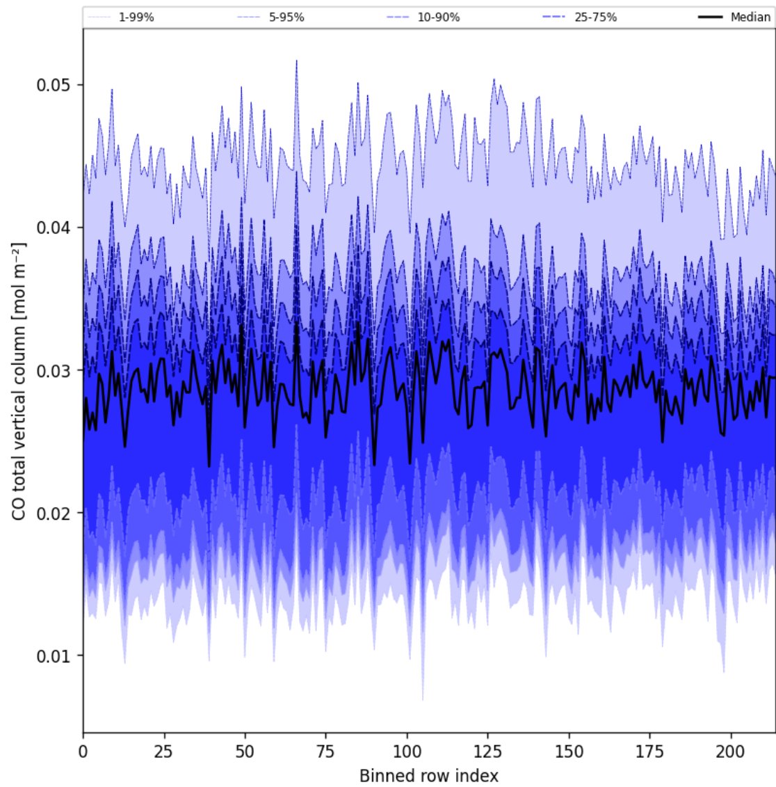
Figure 26: Along track statistics of “CO total vertical column” for 2025-05-13 to 2025-05-15
