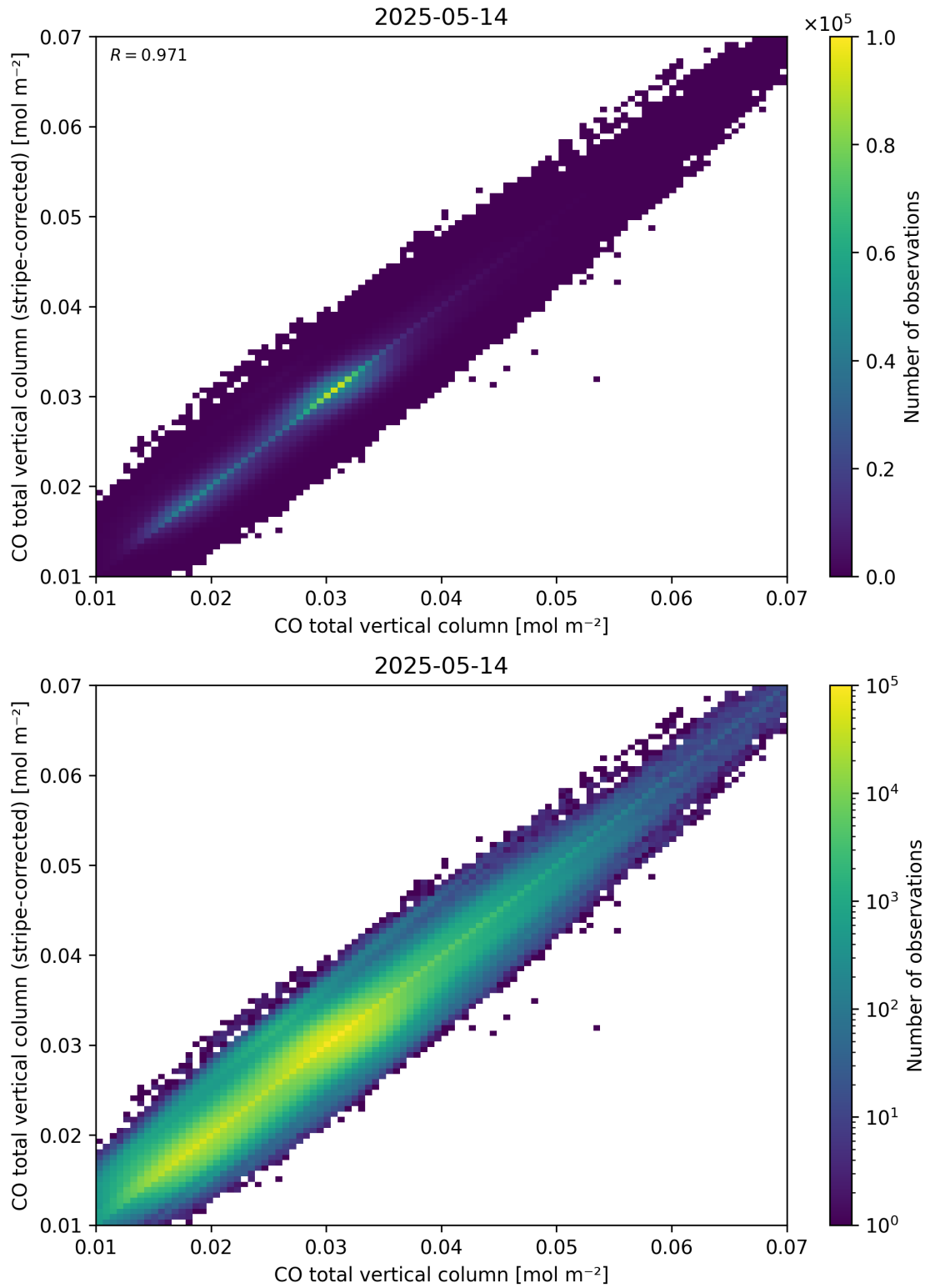
Figure 33: Scatter density plot of “CO total vertical column” against “CO total vertical column (stripe-corrected)” for 2025-05-13 to 2025-05-15.
