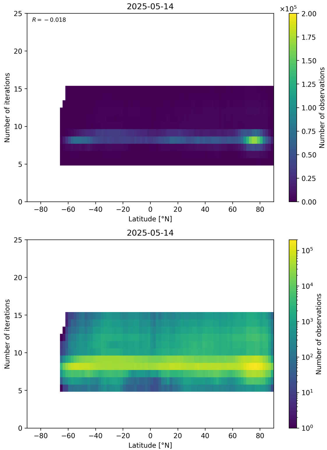
Figure 56: Scatter density plot of “Latitude” against “Number of iterations” for 2025-05-13 to 2025-05-15.
