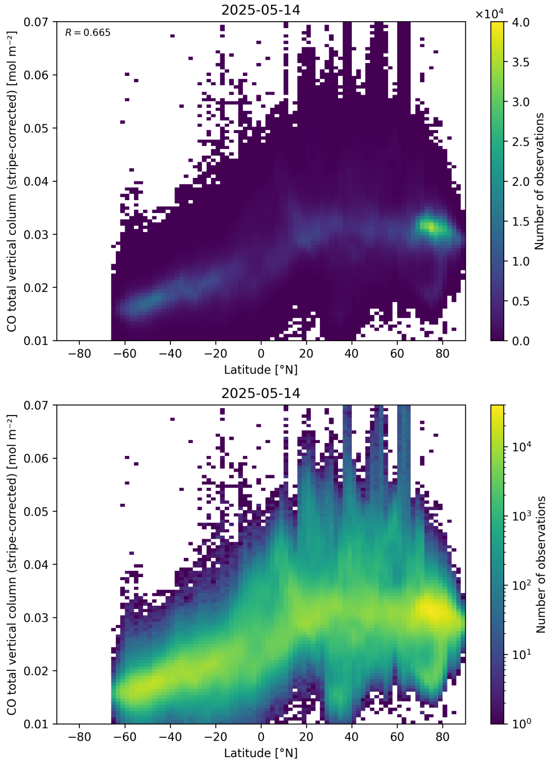
Figure 52: Scatter density plot of “Latitude” against “CO total vertical column (stripe-corrected)” for 2025-05-13 to 2025-05-15.
