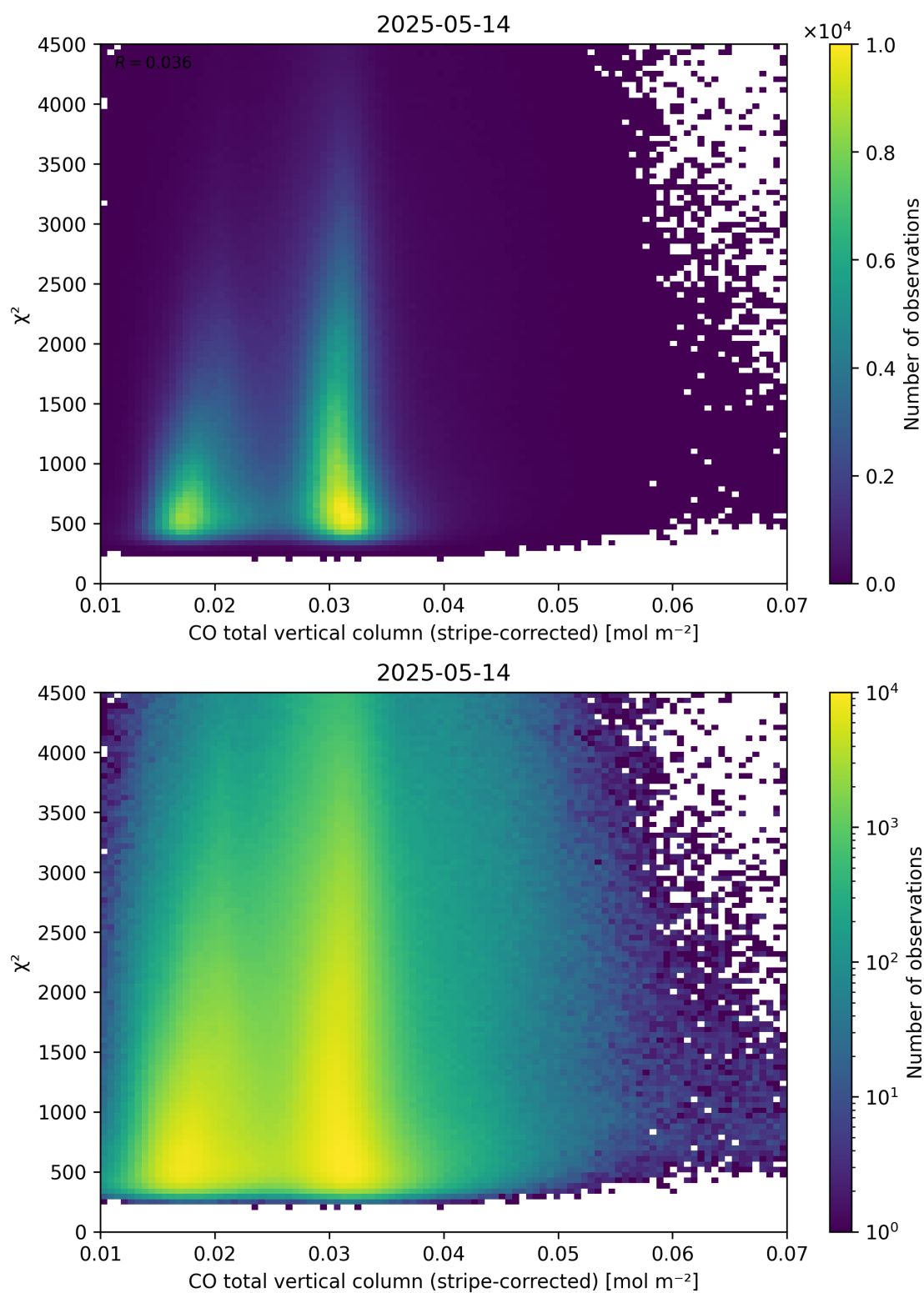
Figure 37: Scatter density plot of “CO total vertical column (stripe-corrected)” against “ \chi^2 ” for 2025-05-13 to 2025-05-15.
