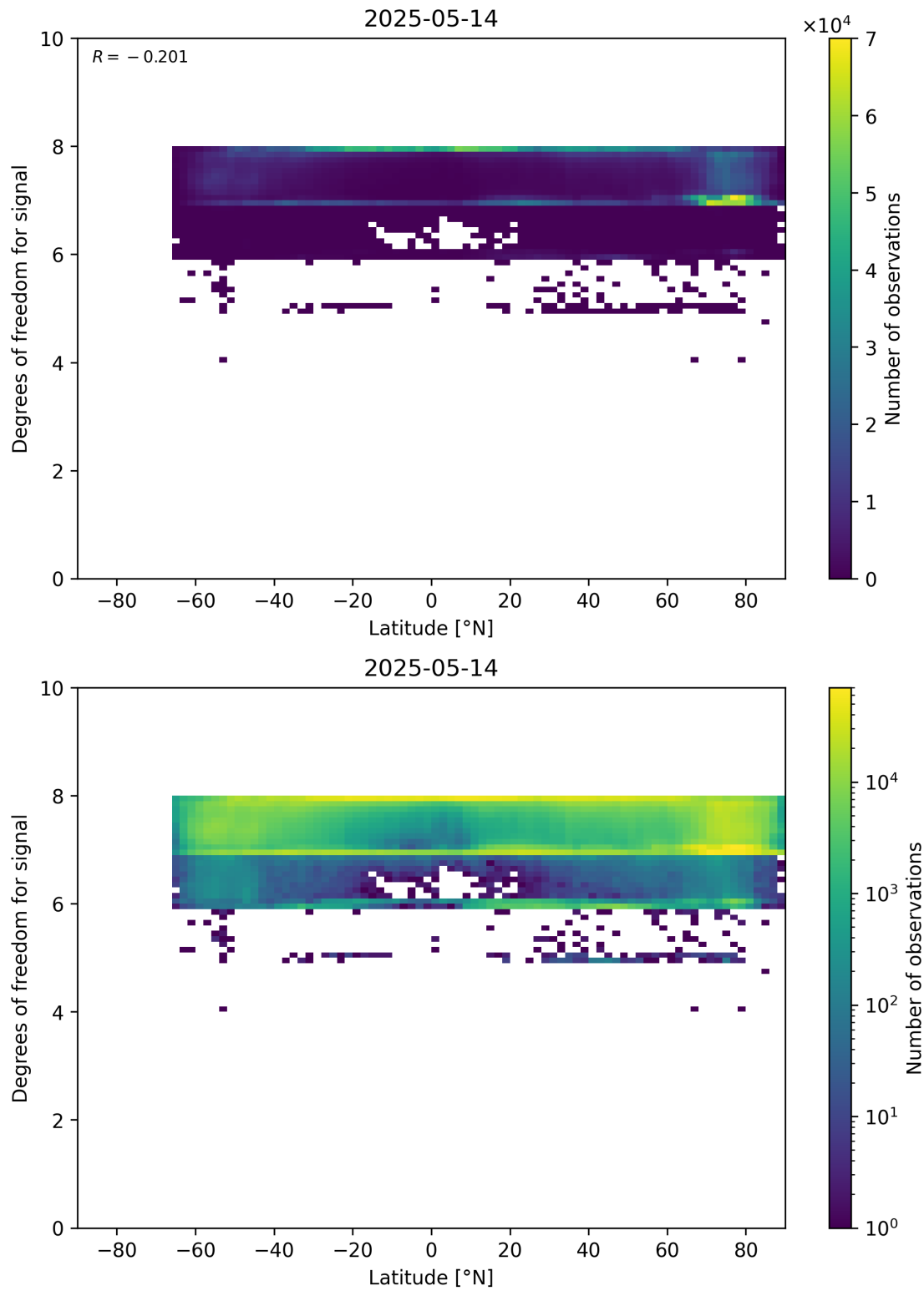
Figure 55: Scatter density plot of “Latitude” against “Degrees of freedom for signal” for 2025-05-13 to 2025-05-15.
