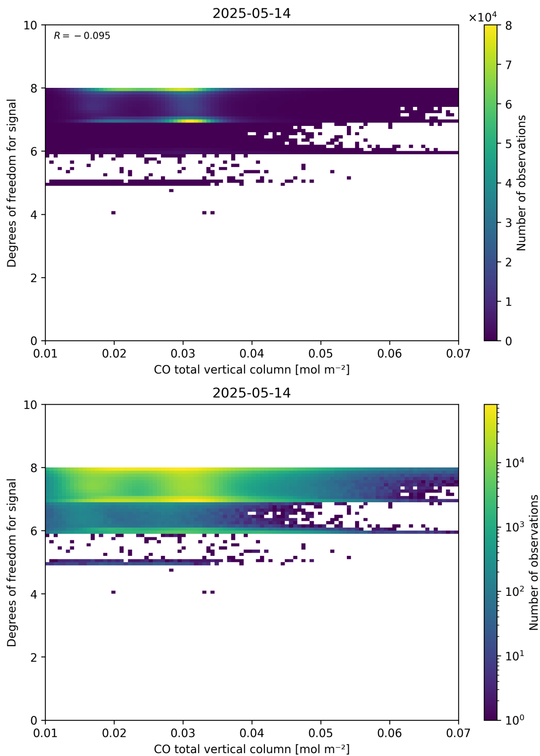
Figure 41: Scatter density plot of “CO total vertical column” against “Degrees of freedom for signal” for 2025-05-13 to 2025-05-15.
