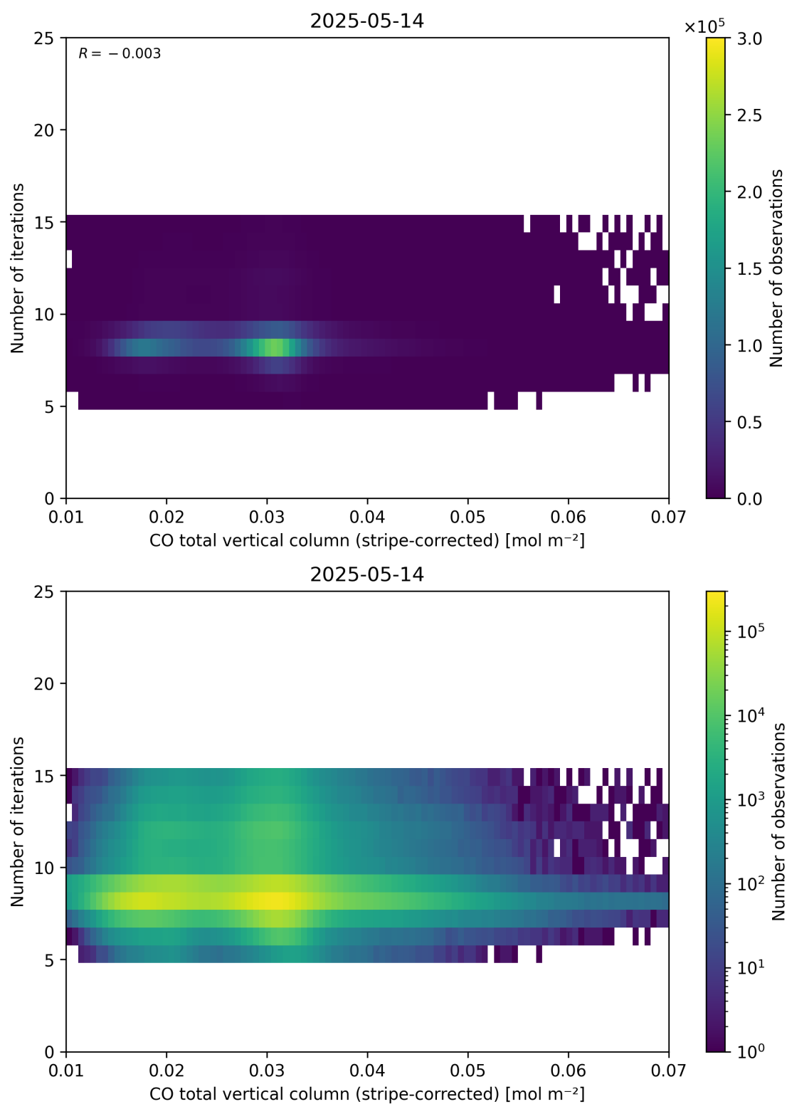
Figure 39: Scatter density plot of “CO total vertical column (stripe-corrected)” against “Number of iterations” for 2025-05-13 to 2025-05-15.
