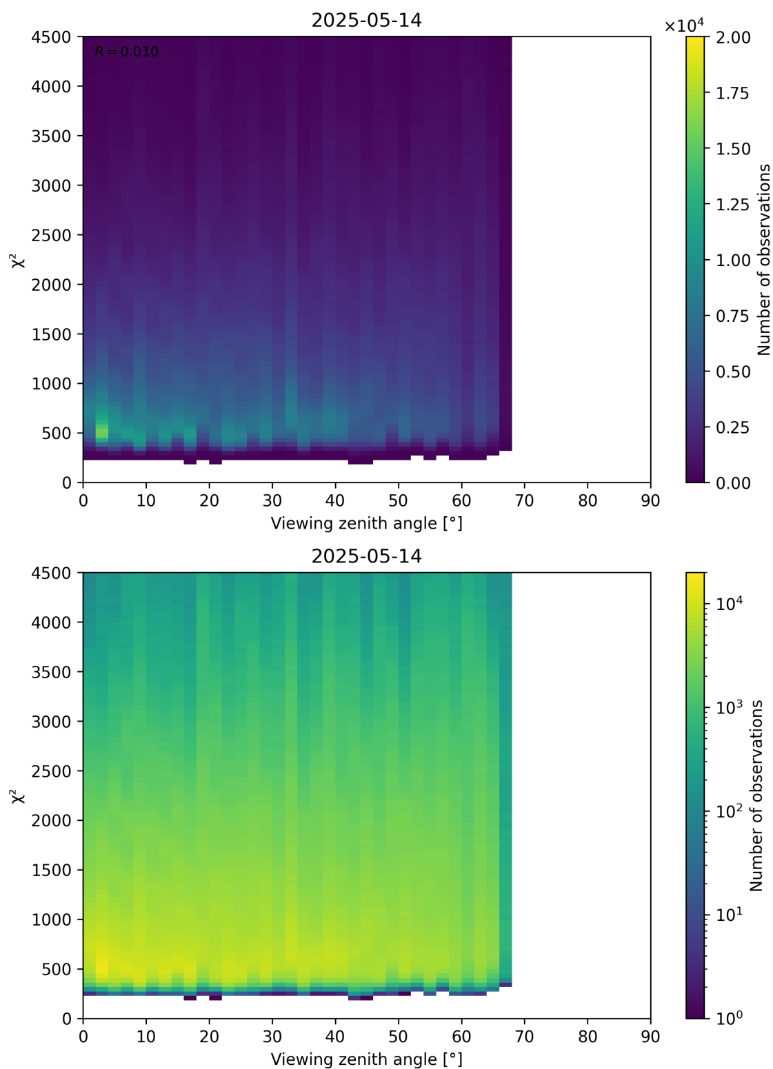
Figure 72: Scatter density plot of “Viewing zenith angle” against “ \chi^2 ” for 2025-05-13 to 2025-05-15.
