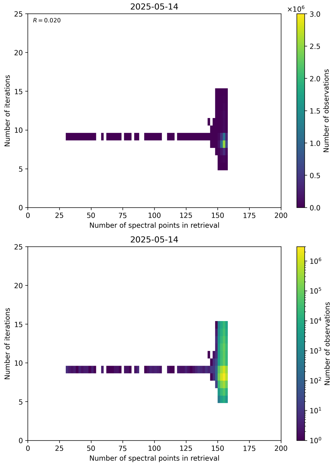
Figure 60: Scatter density plot of “Number of spectral points in retrieval” against “Number of iterations” for 2025-05-13 to 2025-05-15.
