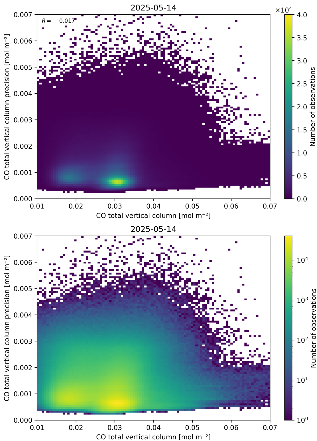
Figure 34: Scatter density plot of “CO total vertical column” against “CO total vertical column precision” for 2025-05-13 to 2025-05-15.
