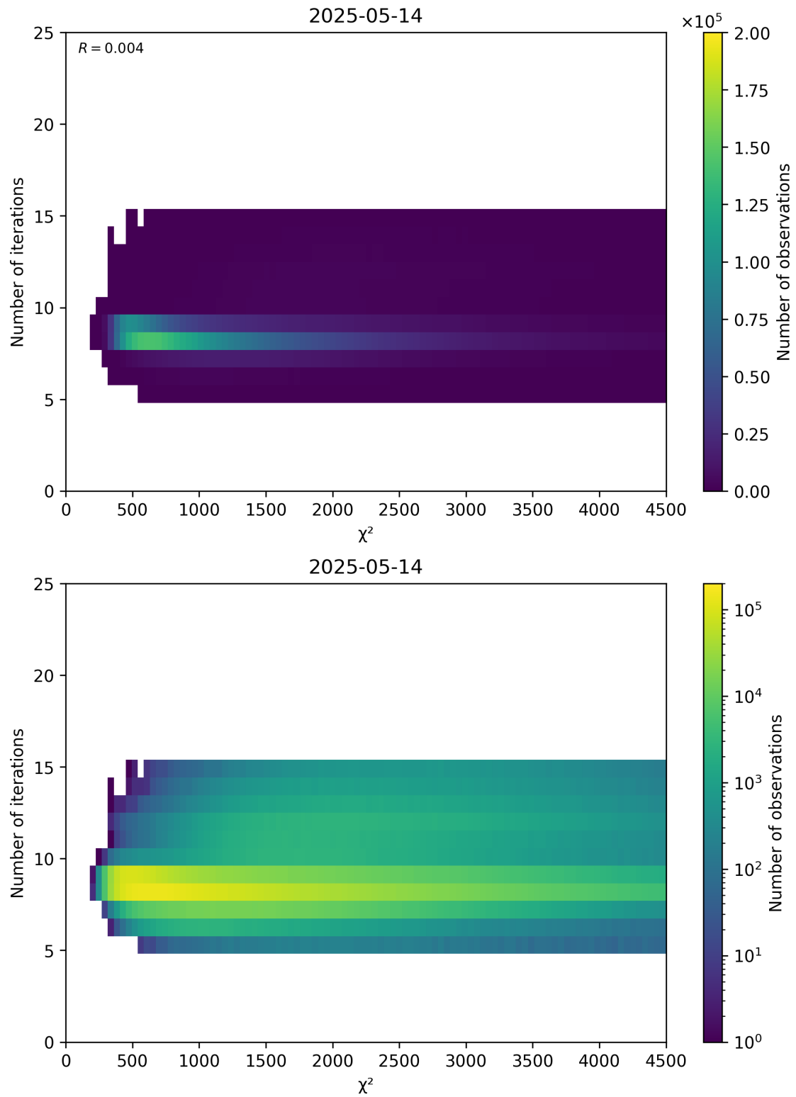
Figure 49: Scatter density plot of “ \chi^2 ” against “Number of iterations” for 2025-05-13 to 2025-05-15.
