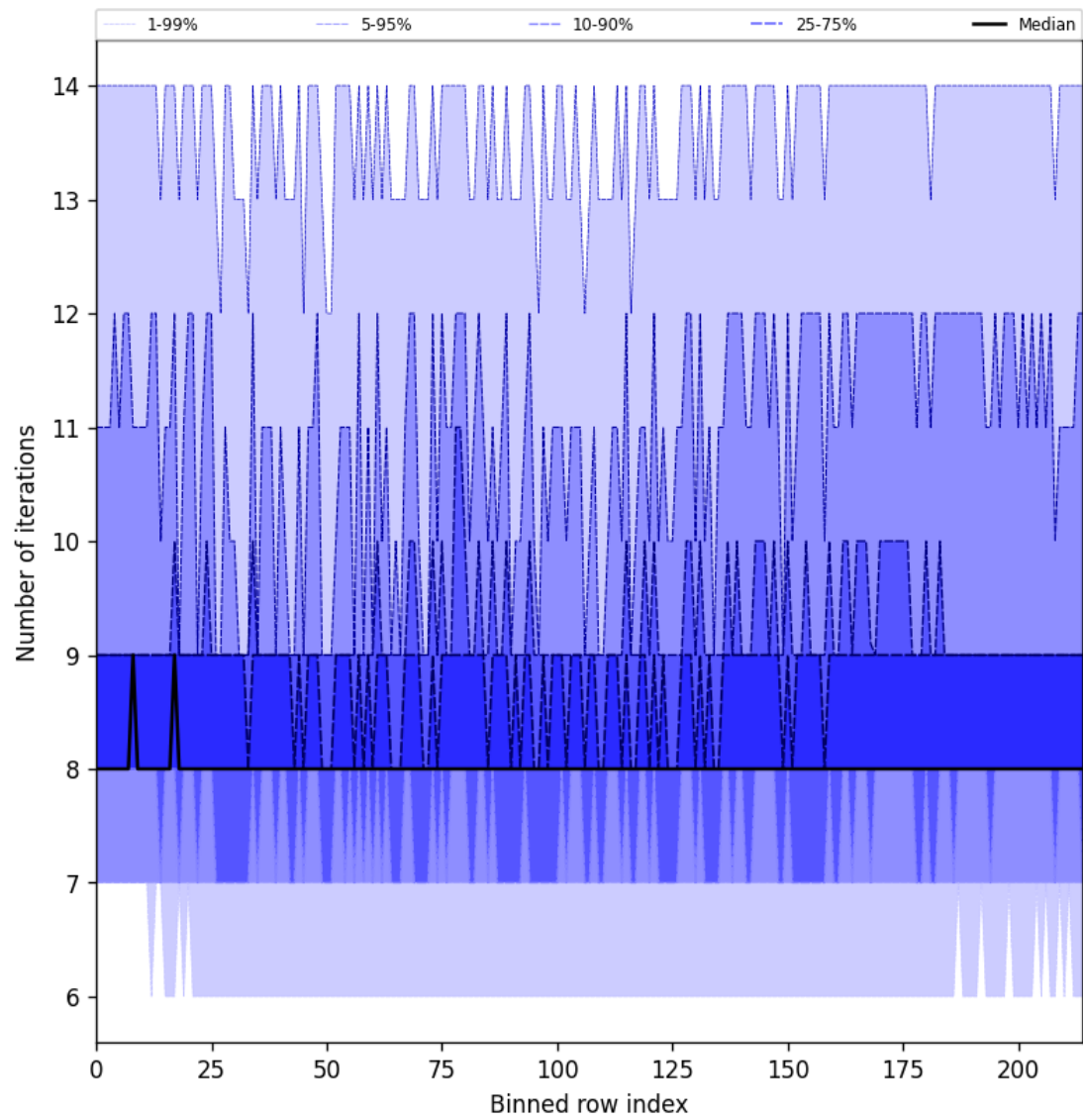
Figure 32: Along track statistics of “Number of iterations” for 2025-05-13 to 2025-05-15
