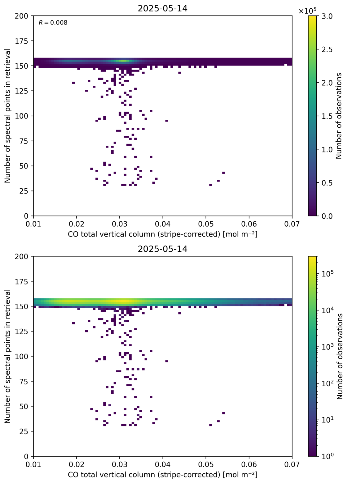
Figure 40: Scatter density plot of “CO total vertical column (stripe-corrected)” against “Number of spectral points in retrieval” for 2025-05-13 to 2025-05-15.
