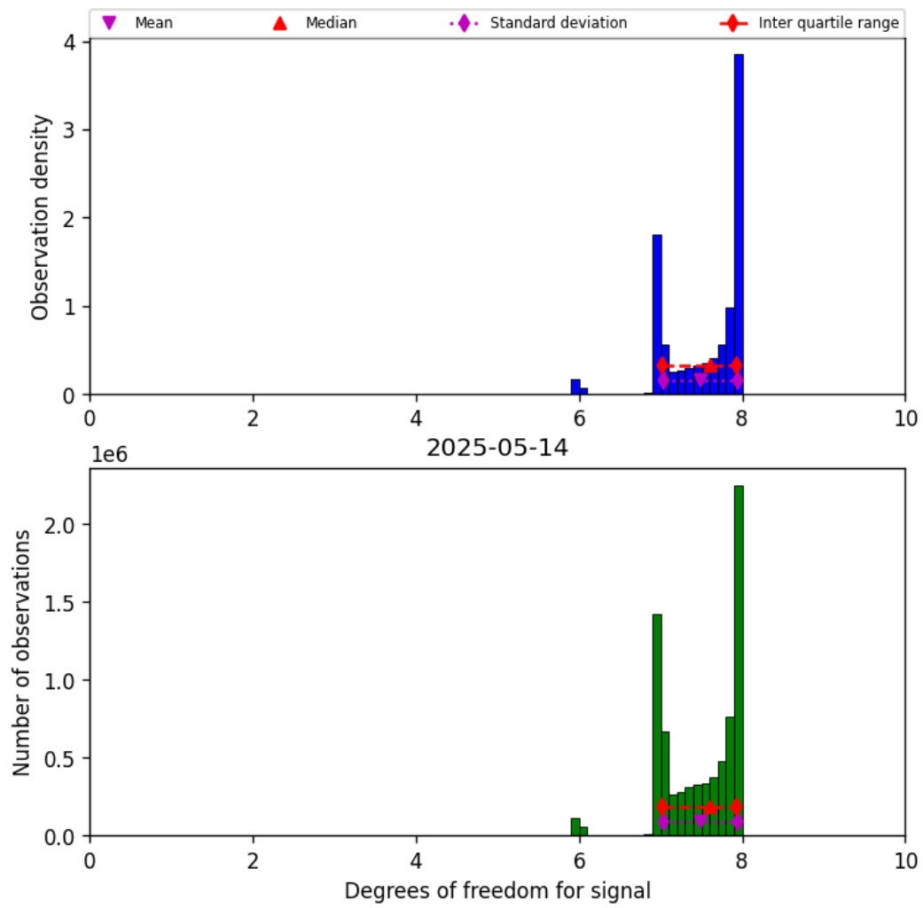
Figure 23: Histogram of “Degrees of freedom for signal” for 2025-05-13 to 2025-05-15
