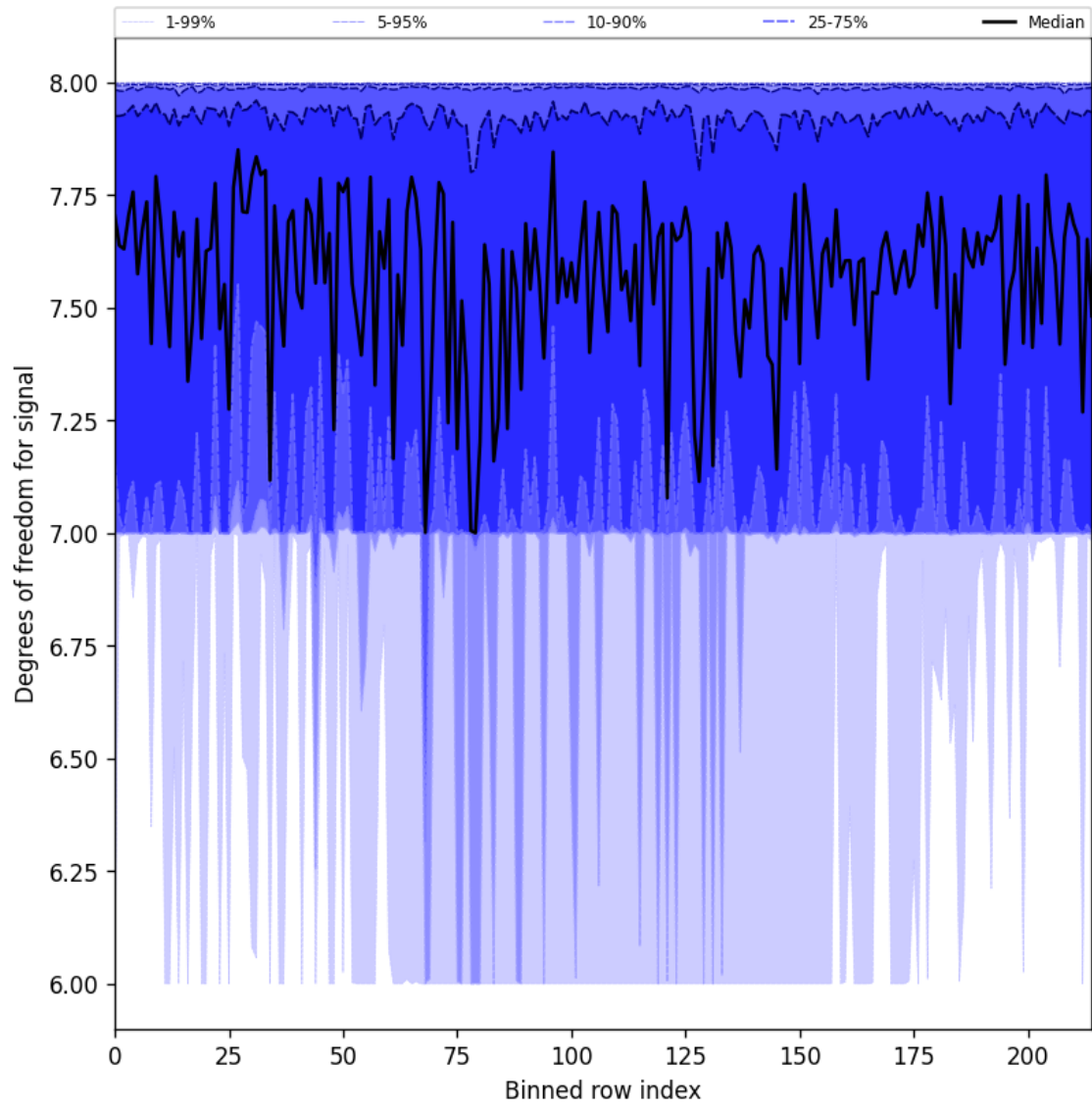
Figure 31: Along track statistics of “Degrees of freedom for signal” for 2025-05-13 to 2025-05-15
