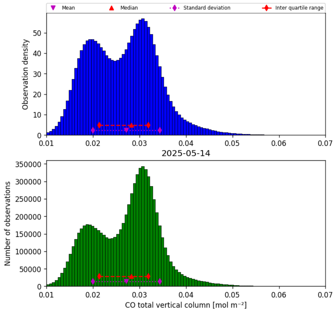
Figure 18: Histogram of “CO total vertical column” for 2025-05-13 to 2025-05-15
