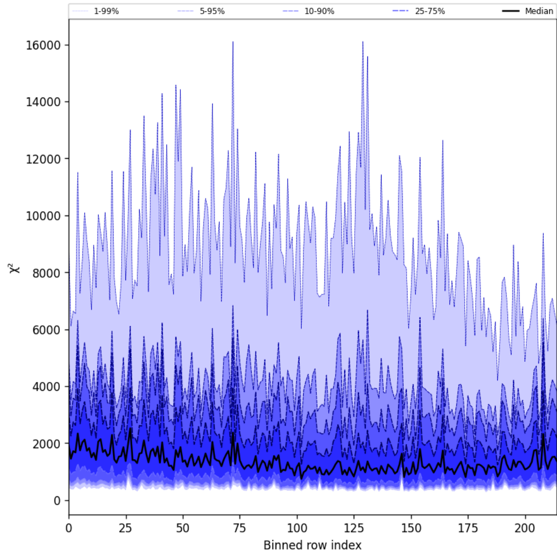
Figure 30: Along track statistics of “ \chi^2 ” for 2025-05-13 to 2025-05-15
