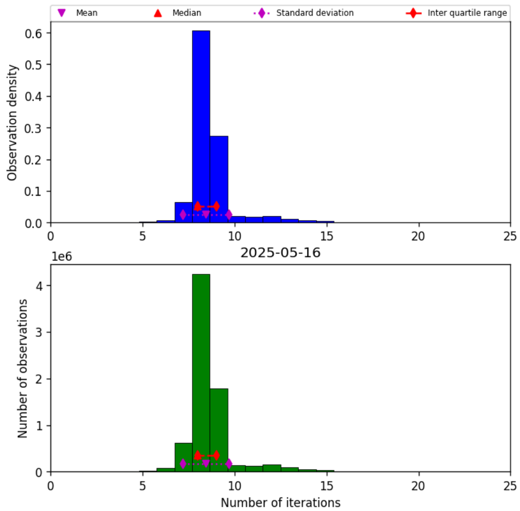
Figure 24: Histogram of “Number of iterations” for 2025-05-15 to 2025-05-17
