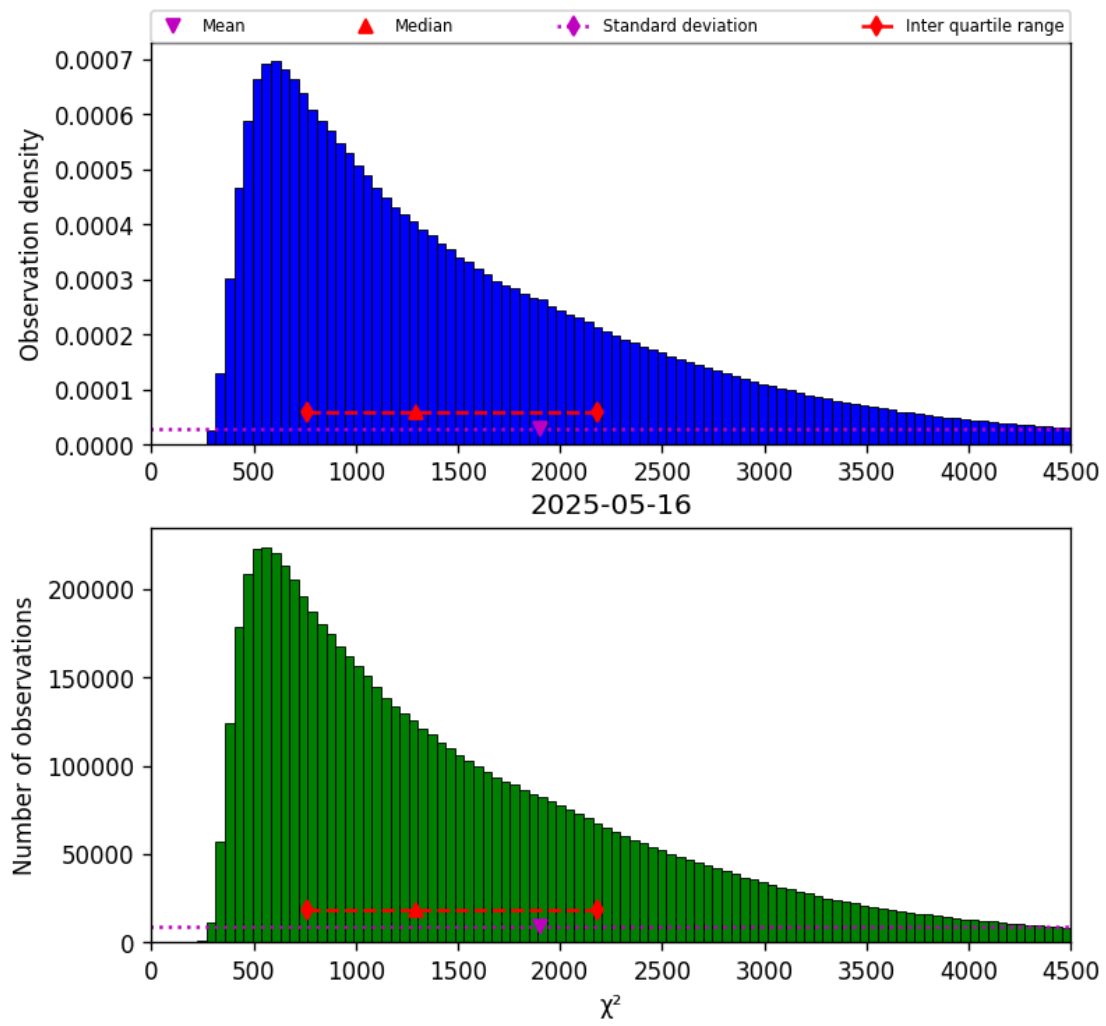
Figure 22: Histogram of “ \chi^2 ” for 2025-05-15 to 2025-05-17
