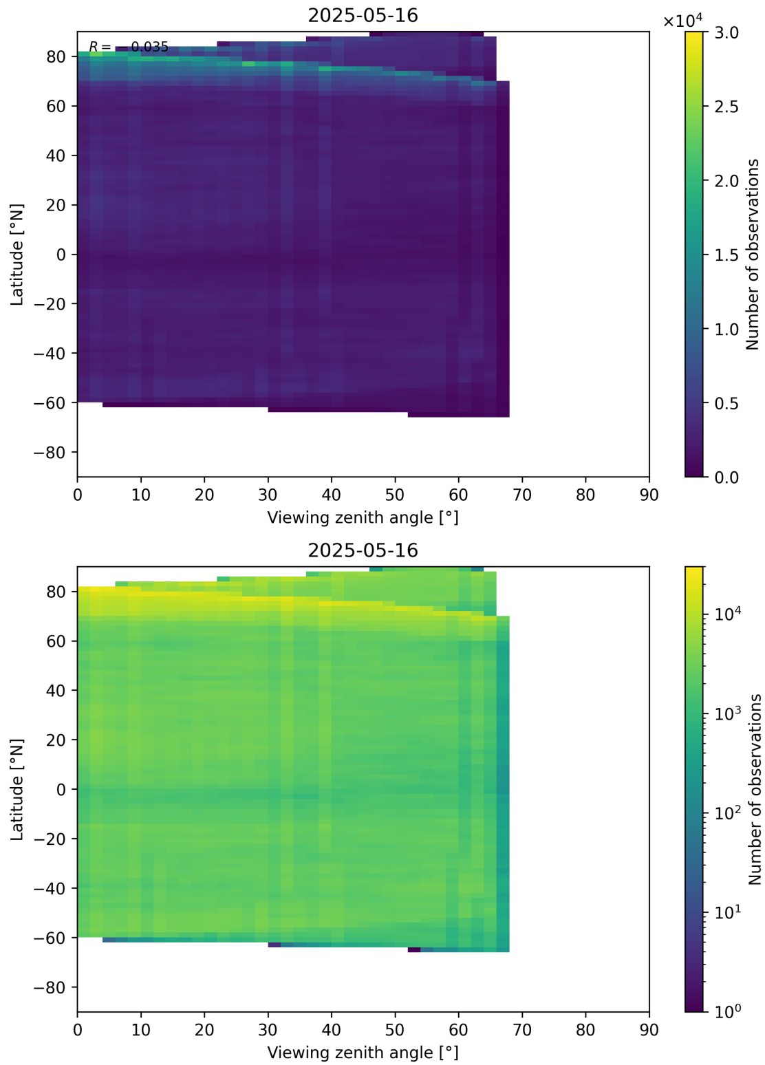
Figure 74: Scatter density plot of “Viewing zenith angle” against “Latitude” for 2025-05-15 to 2025-05-17.
