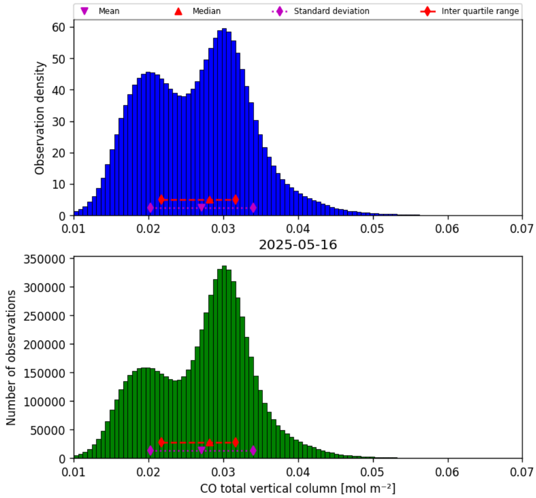
Figure 18: Histogram of “CO total vertical column” for 2025-05-15 to 2025-05-17
