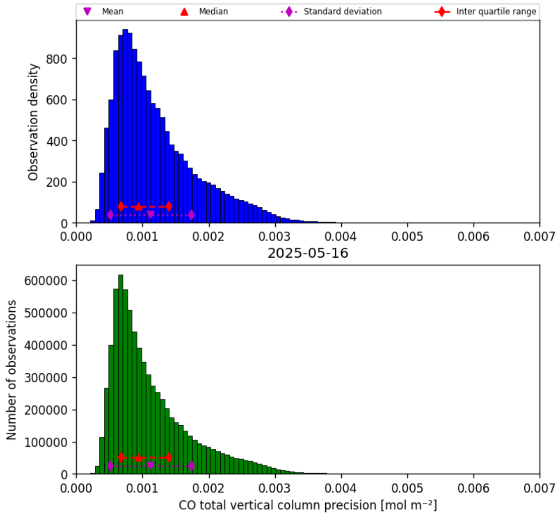
Figure 20: Histogram of “CO total vertical column precision” for 2025-05-15 to 2025-05-17
