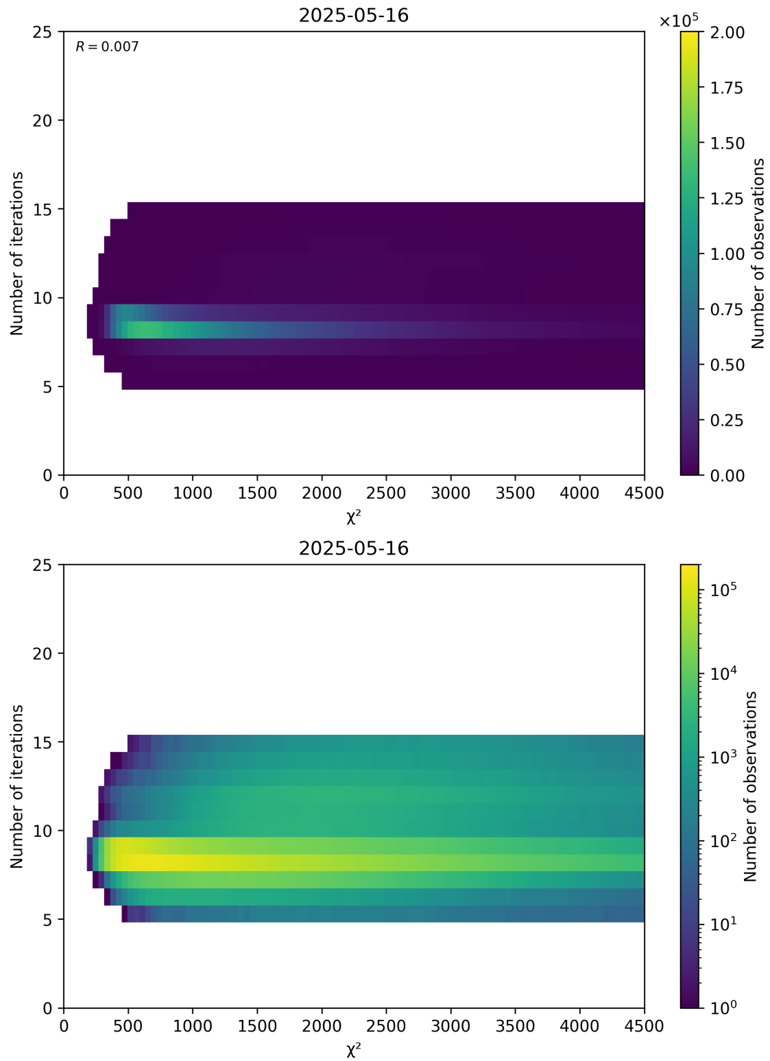
Figure 49: Scatter density plot of “ \chi^2 ” against “Number of iterations” for 2025-05-15 to 2025-05-17.
