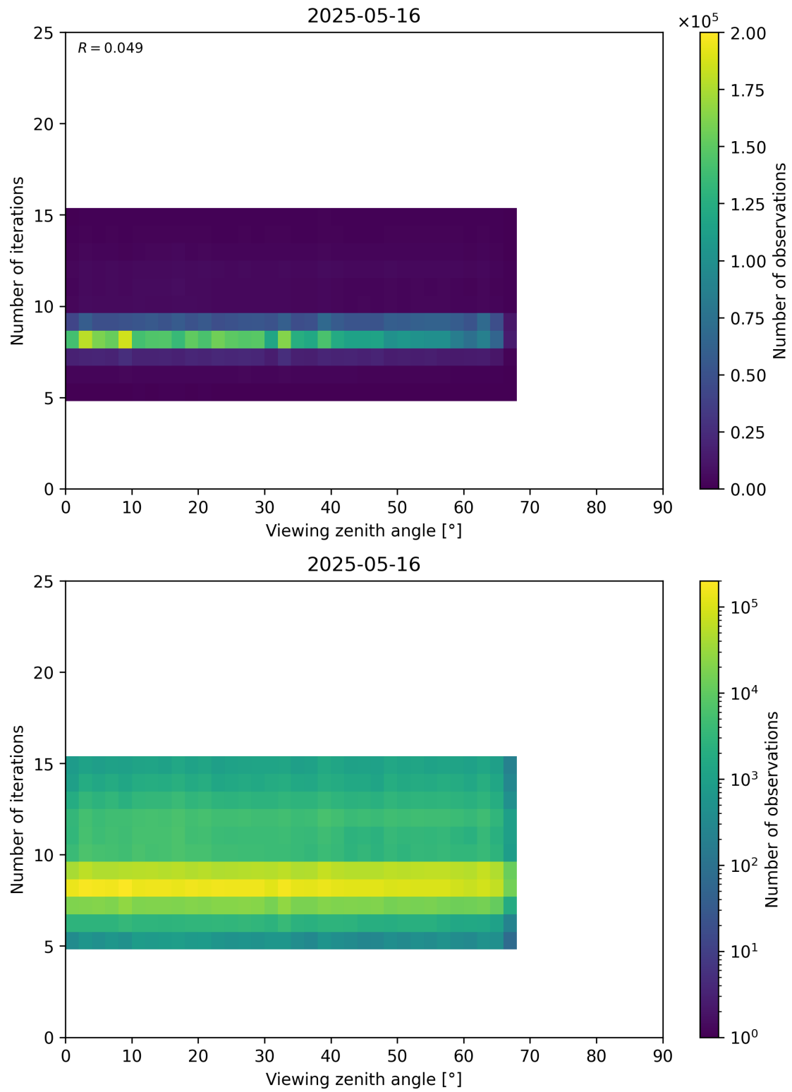
Figure 75: Scatter density plot of “Viewing zenith angle” against “Number of iterations” for 2025-05-15 to 2025-05-17.
