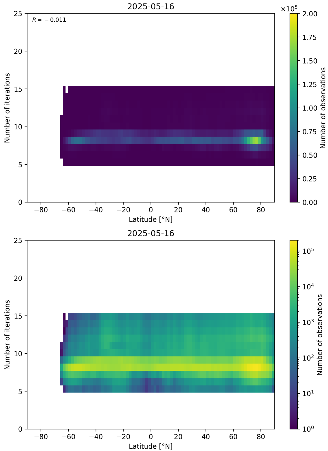
Figure 56: Scatter density plot of “Latitude” against “Number of iterations” for 2025-05-15 to 2025-05-17.
