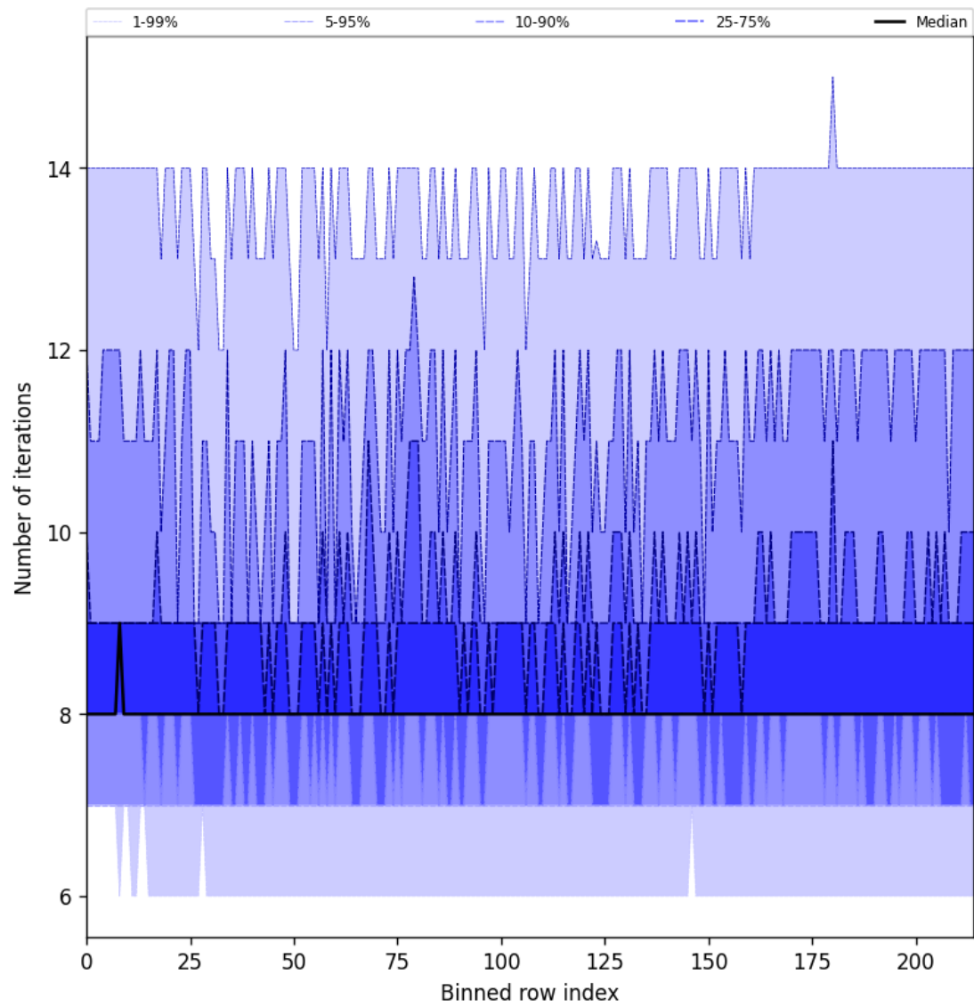
Figure 32: Along track statistics of “Number of iterations” for 2025-05-15 to 2025-05-17
