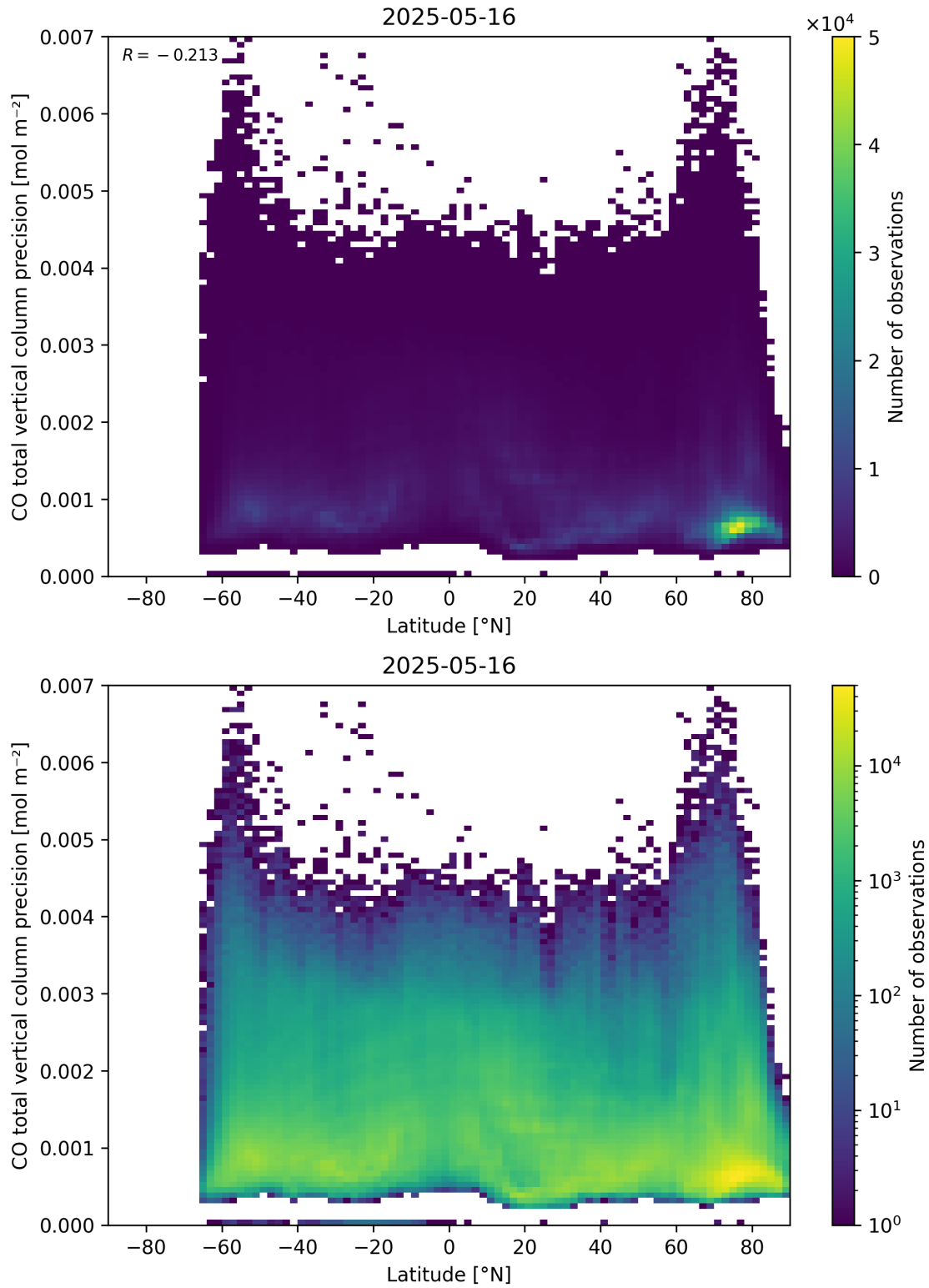
Figure 53: Scatter density plot of “Latitude” against “CO total vertical column precision” for 2025-05-15 to 2025-05-17.
