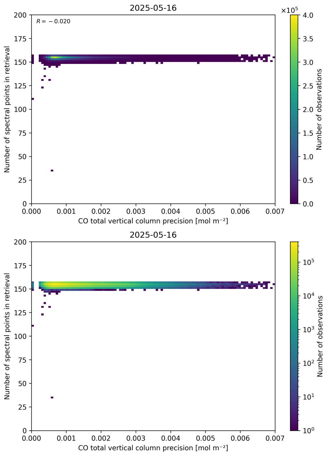
Figure 47: Scatter density plot of “CO total vertical column precision” against “Number of spectral points in retrieval” for 2025-05-15 to 2025-05-17.
