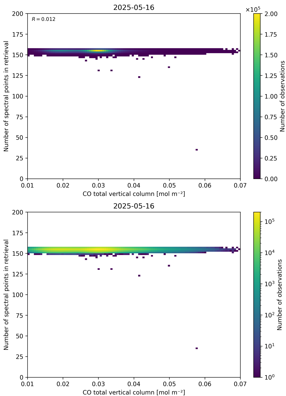
Figure 43: Scatter density plot of “CO total vertical column” against “Number of spectral points in retrieval” for 2025-05-15 to 2025-05-17.
