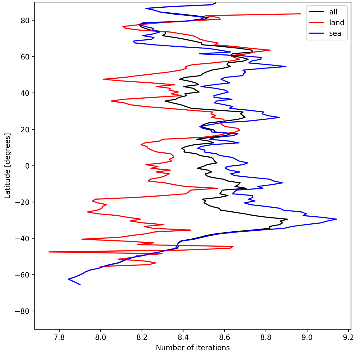
Figure 16: Zonal average of “Number of iterations” for 2025-05-15 to 2025-05-17.
