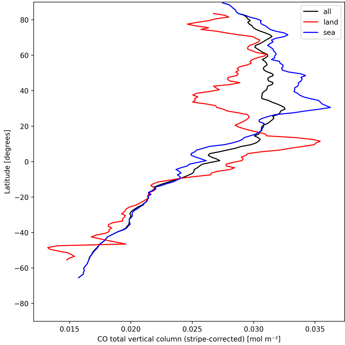
Figure 11: Zonal average of “CO total vertical column (stripe-corrected)” for 2025-05-15 to 2025-05-17.
