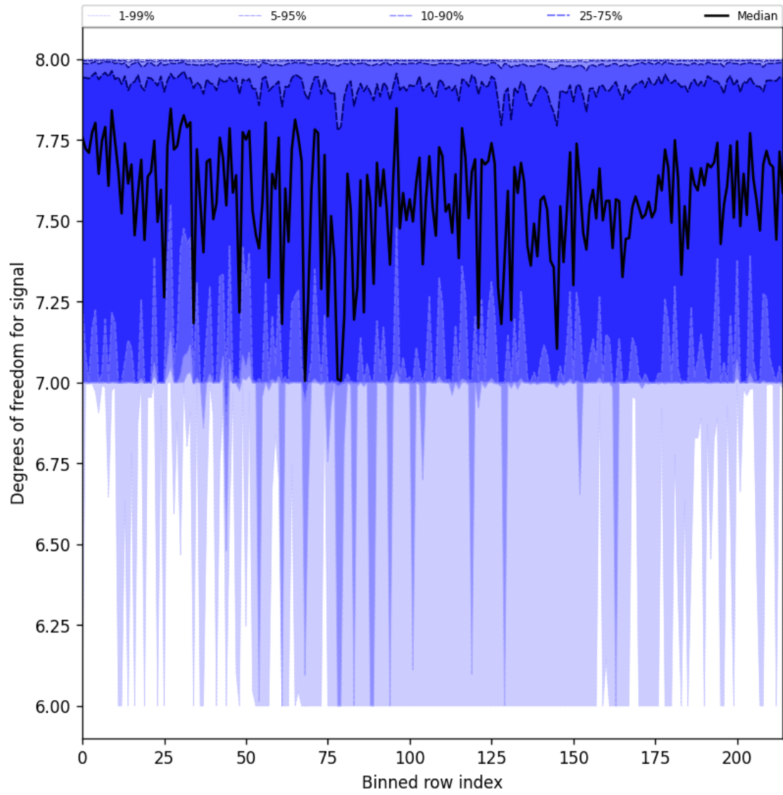
Figure 31: Along track statistics of “Degrees of freedom for signal” for 2025-05-15 to 2025-05-17
