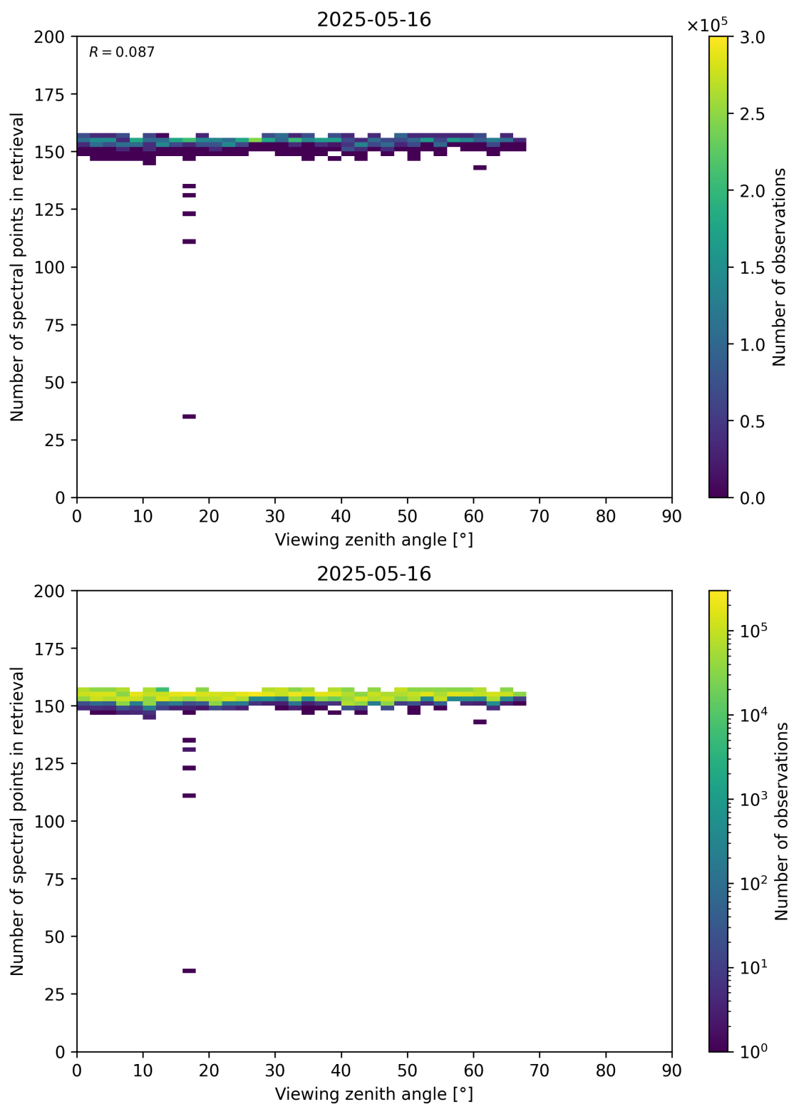
Figure 76: Scatter density plot of “Viewing zenith angle” against “Number of spectral points in retrieval” for 2025-05-15 to 2025-05-17.
