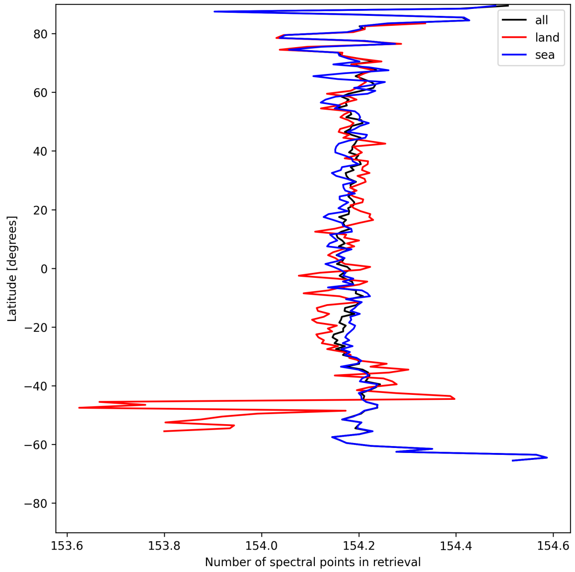
Figure 13: Zonal average of “Number of spectral points in retrieval” for 2025-05-15 to 2025-05-17.
