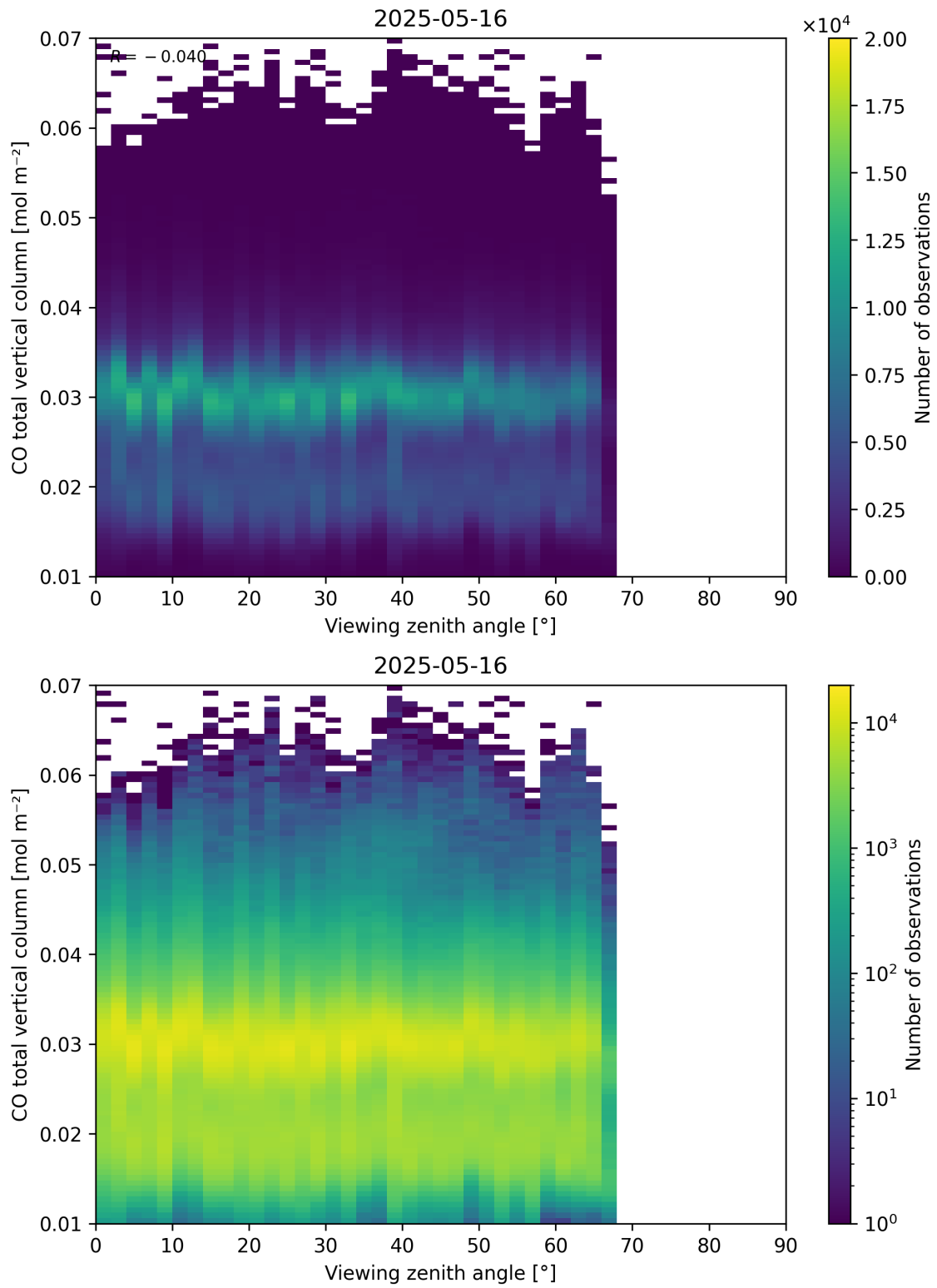
Figure 69: Scatter density plot of “Viewing zenith angle” against “CO total vertical column” for 2025-05-15 to 2025-05-17.
