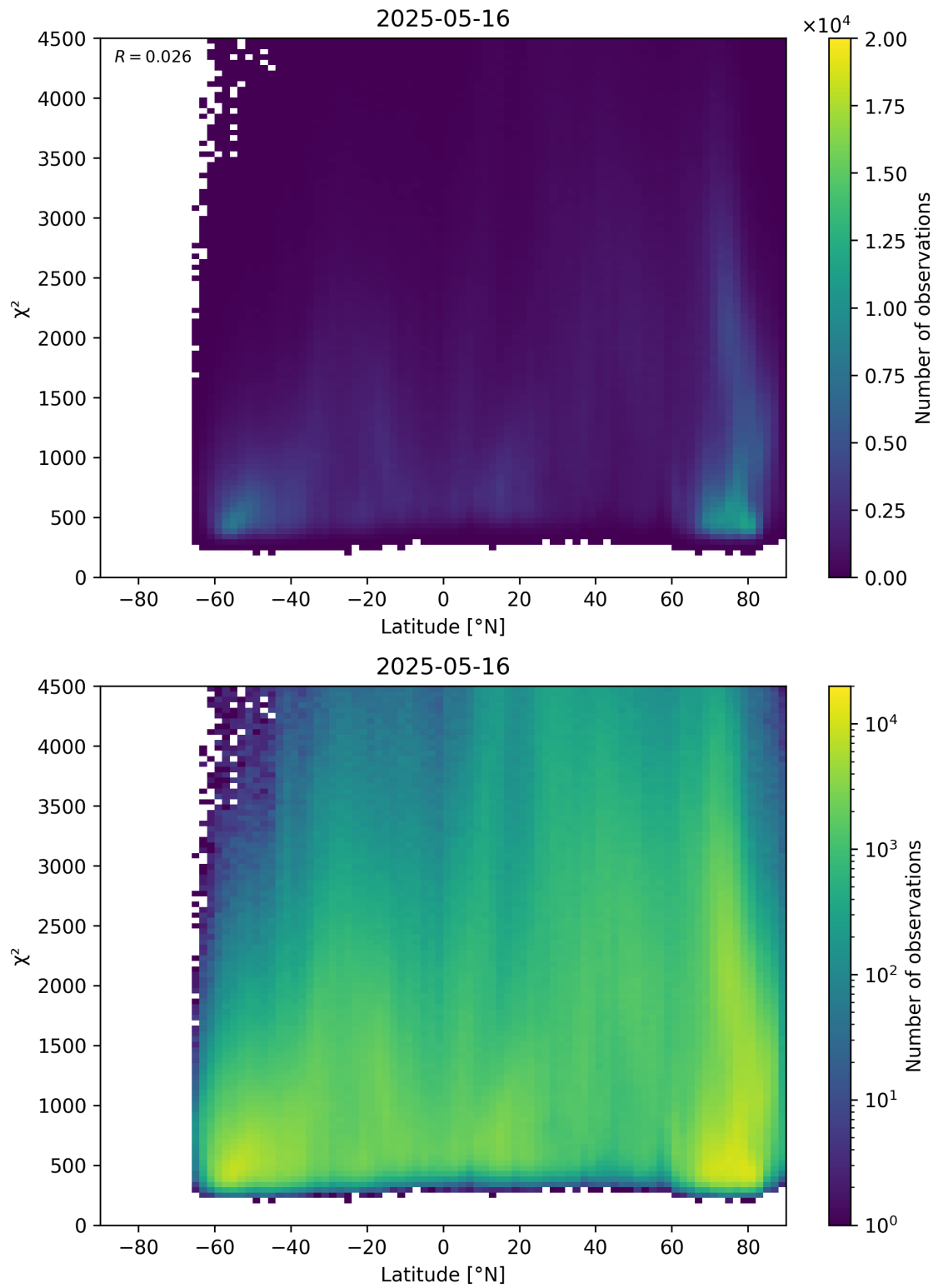
Figure 54: Scatter density plot of “Latitude” against “ \chi^2 ” for 2025-05-15 to 2025-05-17.
