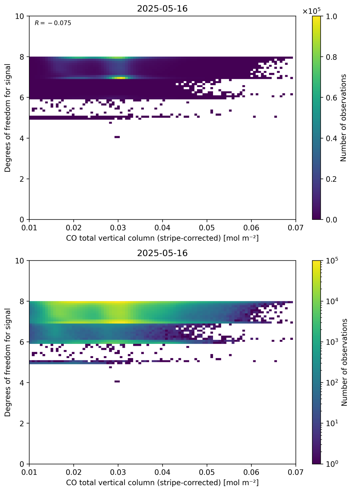
Figure 38: Scatter density plot of “CO total vertical column (stripe-corrected)” against “Degrees of freedom for signal” for 2025-05-15 to 2025-05-17.
