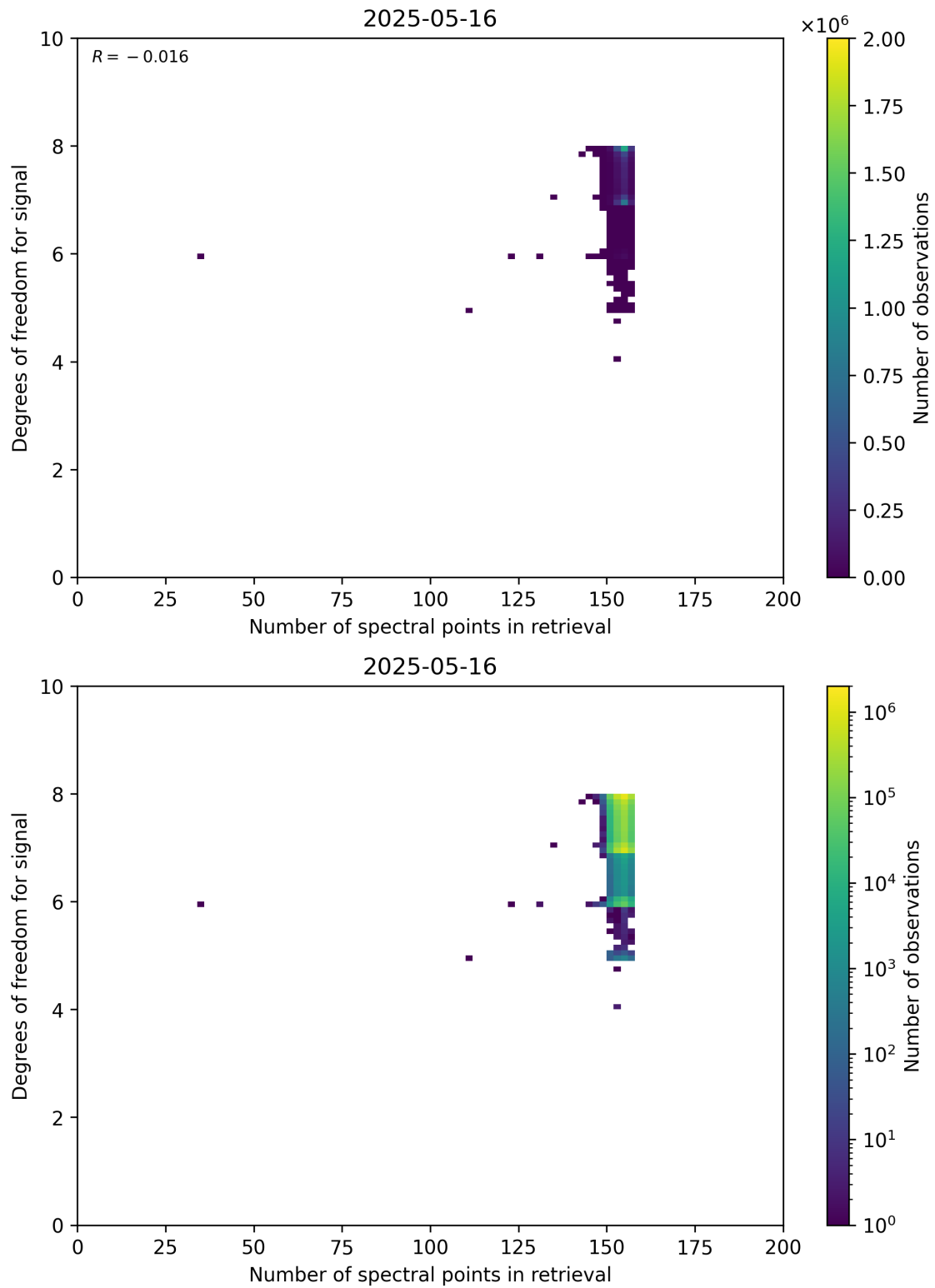
Figure 59: Scatter density plot of “Number of spectral points in retrieval” against “Degrees of freedom for signal” for 2025-05-15 to 2025-05-17.
