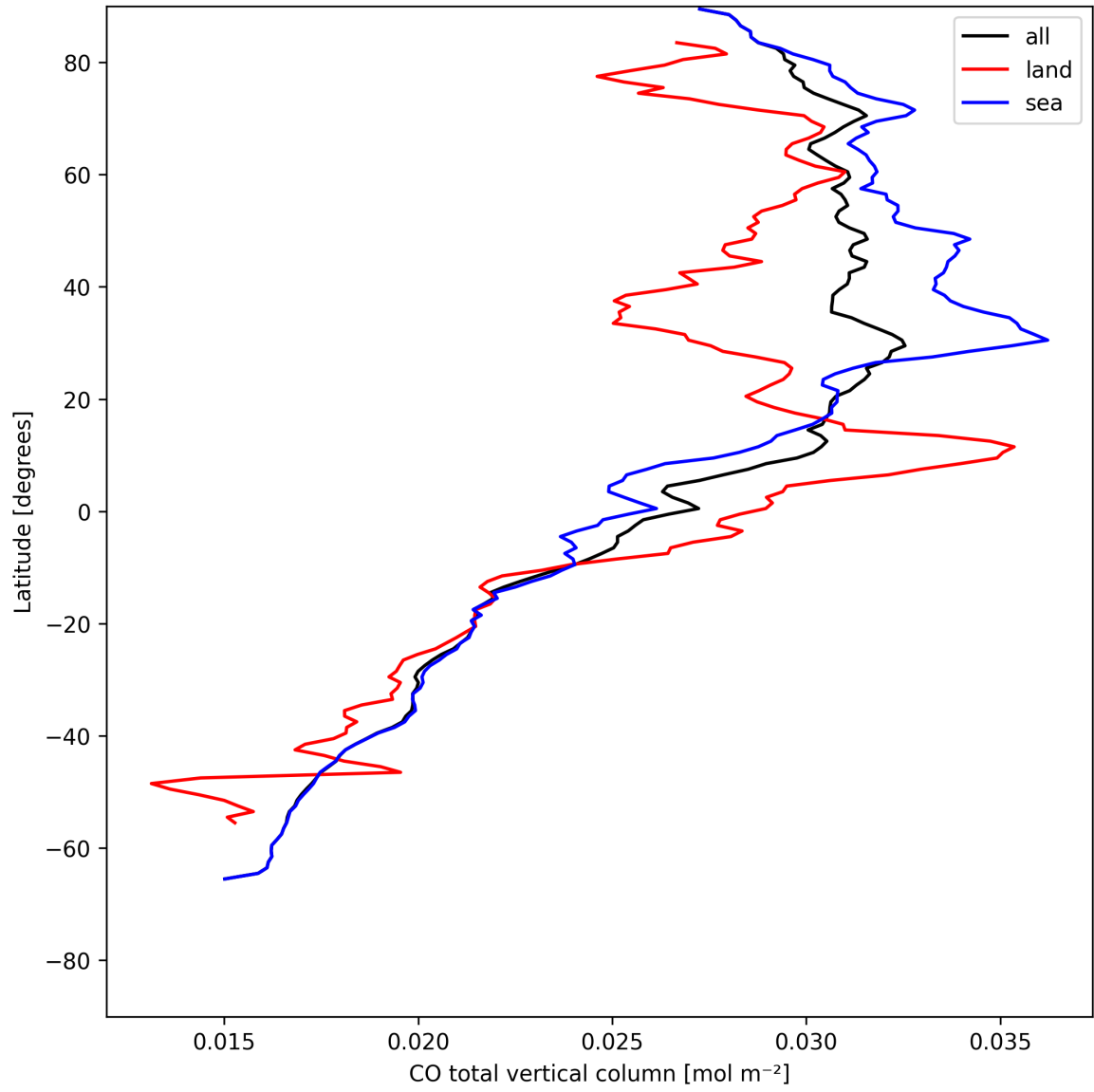
Figure 10: Zonal average of “CO total vertical column” for 2025-05-15 to 2025-05-17.
