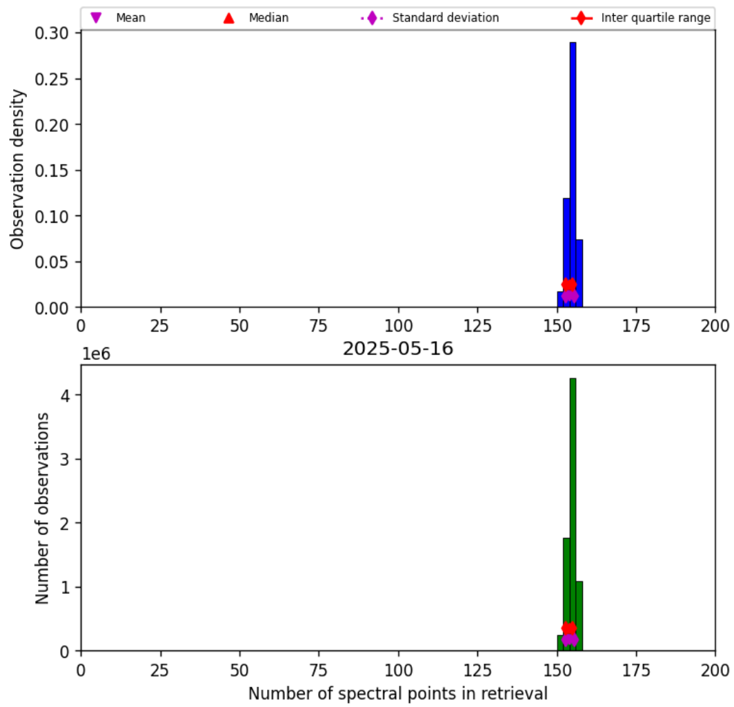
Figure 21: Histogram of “Number of spectral points in retrieval” for 2025-05-15 to 2025-05-17
