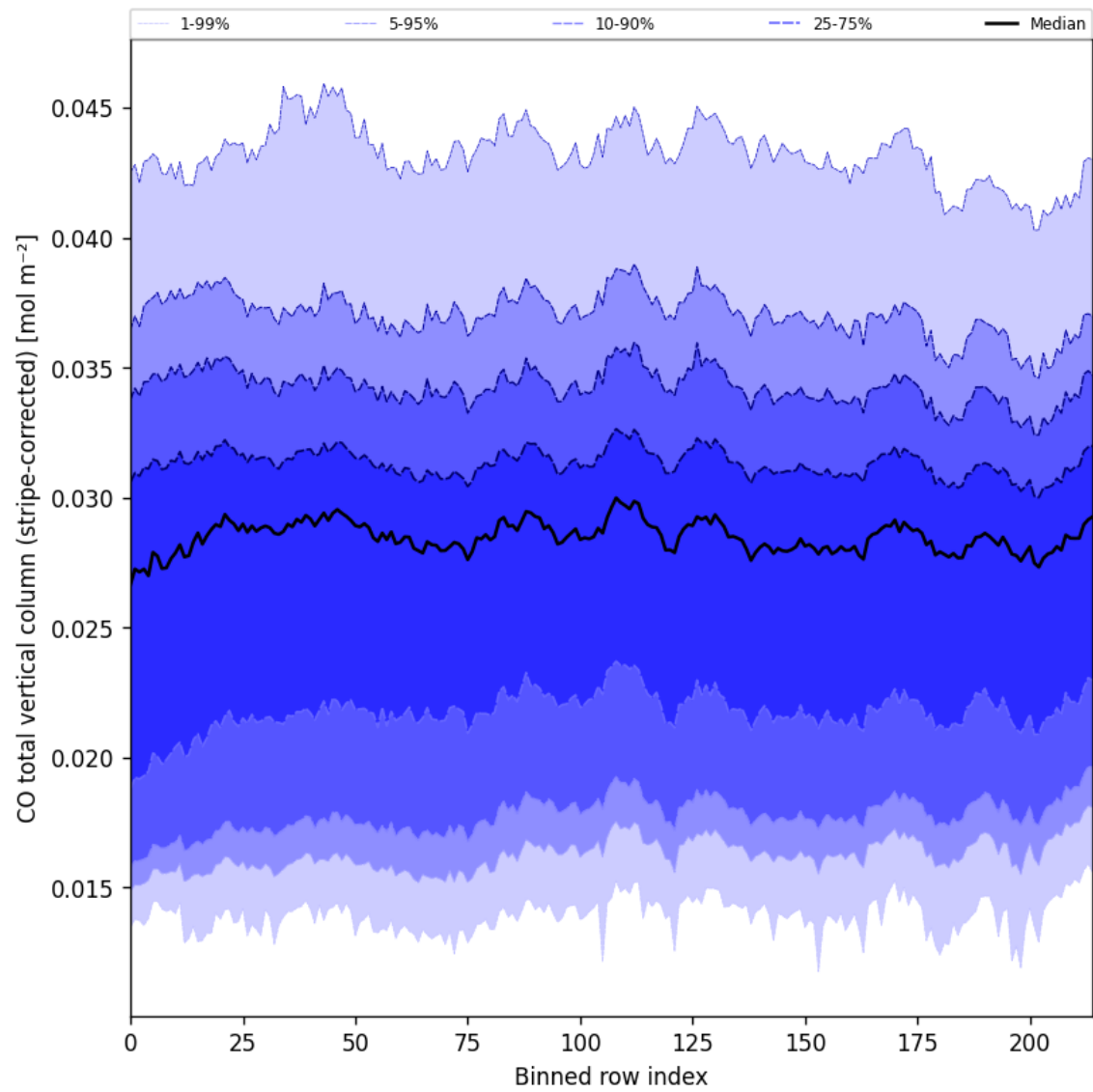
Figure 27: Along track statistics of “CO total vertical column (stripe-corrected)” for 2025-05-15 to 2025-05-17
