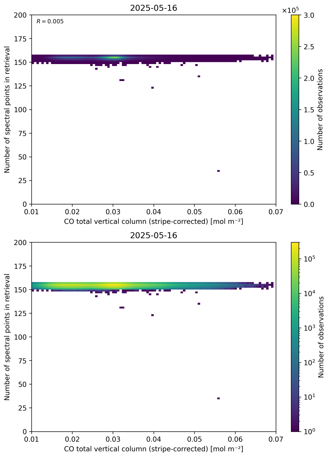
Figure 40: Scatter density plot of “CO total vertical column (stripe-corrected)” against “Number of spectral points in retrieval” for 2025-05-15 to 2025-05-17.
