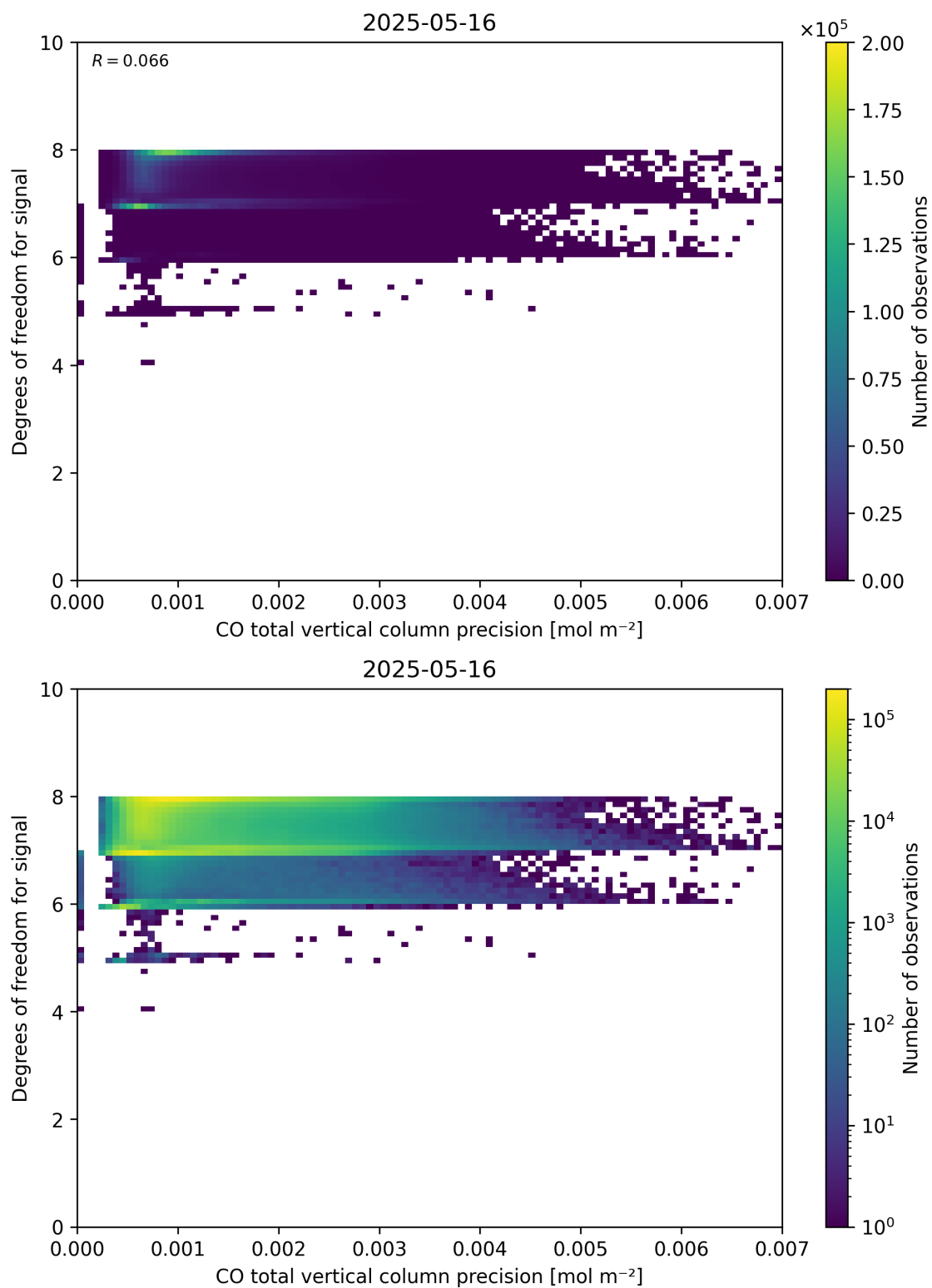
Figure 45: Scatter density plot of “CO total vertical column precision” against “Degrees of freedom for signal” for 2025-05-15 to 2025-05-17.
