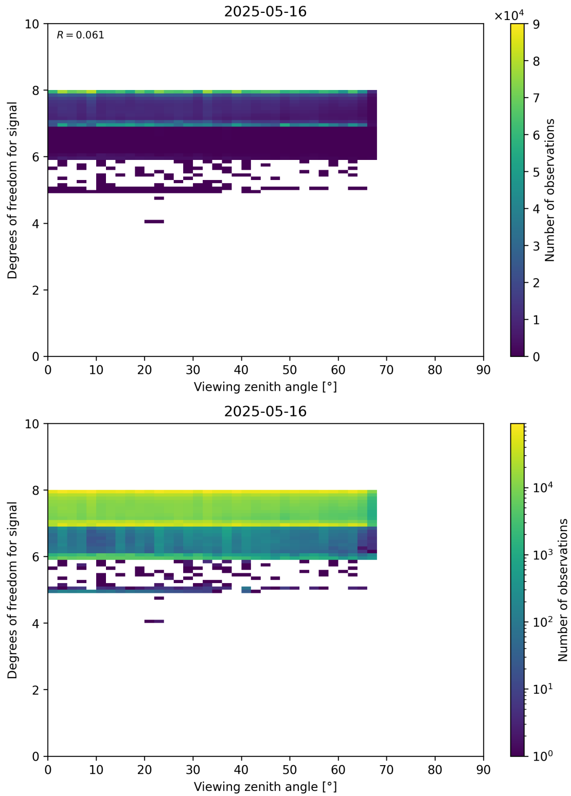
Figure 73: Scatter density plot of “Viewing zenith angle” against “Degrees of freedom for signal” for 2025-05-15 to 2025-05-17.
