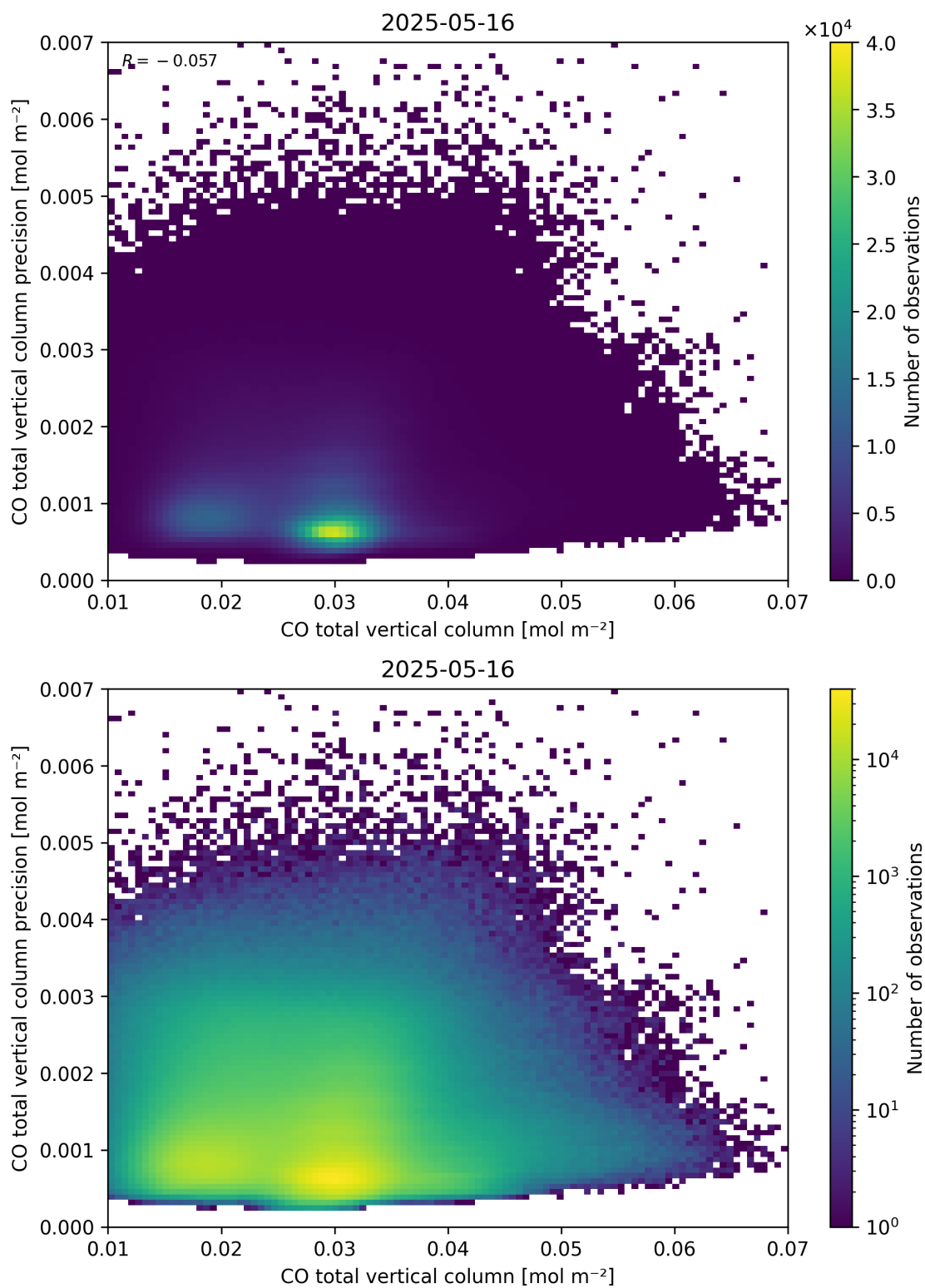
Figure 34: Scatter density plot of “CO total vertical column” against “CO total vertical column precision” for 2025-05-15 to 2025-05-17.
