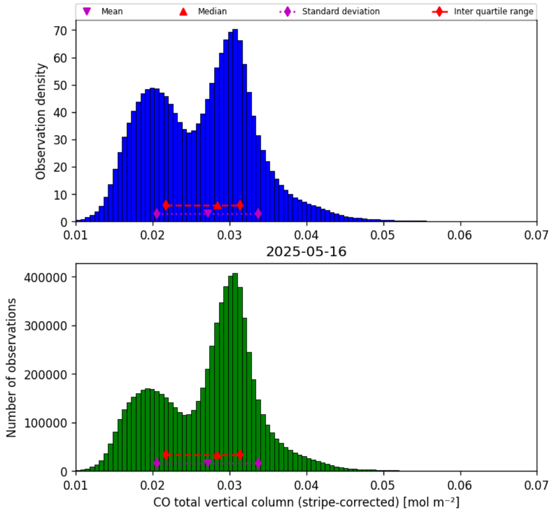
Figure 19: Histogram of “CO total vertical column (stripe-corrected)” for 2025-05-15 to 2025-05-17
