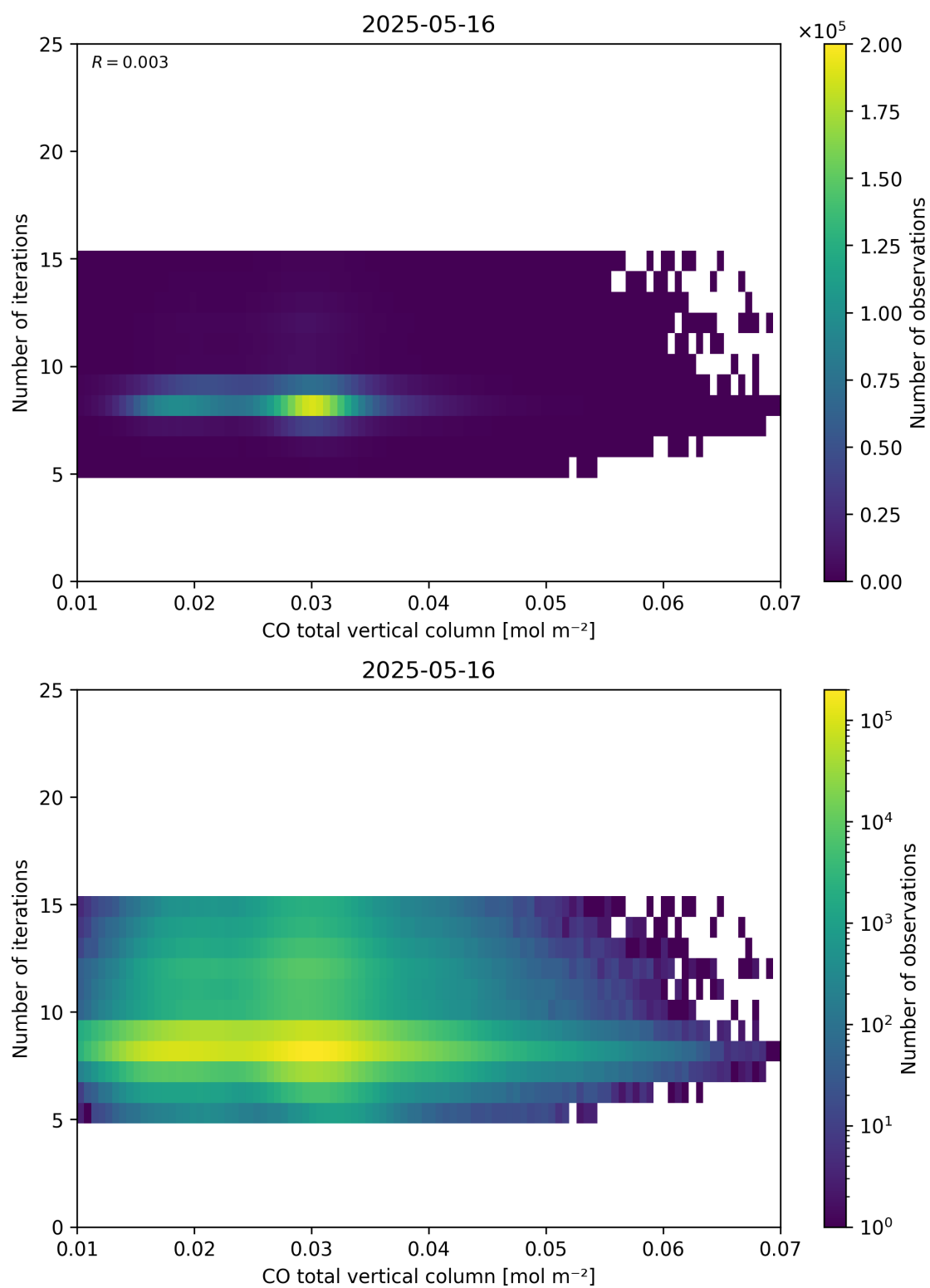
Figure 42: Scatter density plot of “CO total vertical column” against “Number of iterations” for 2025-05-15 to 2025-05-17.
