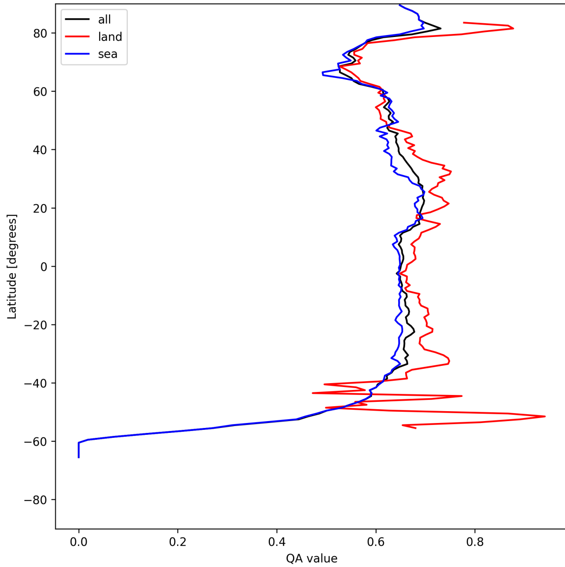
Figure 9: Zonal average of “QA value” for 2025-05-15 to 2025-05-17.
