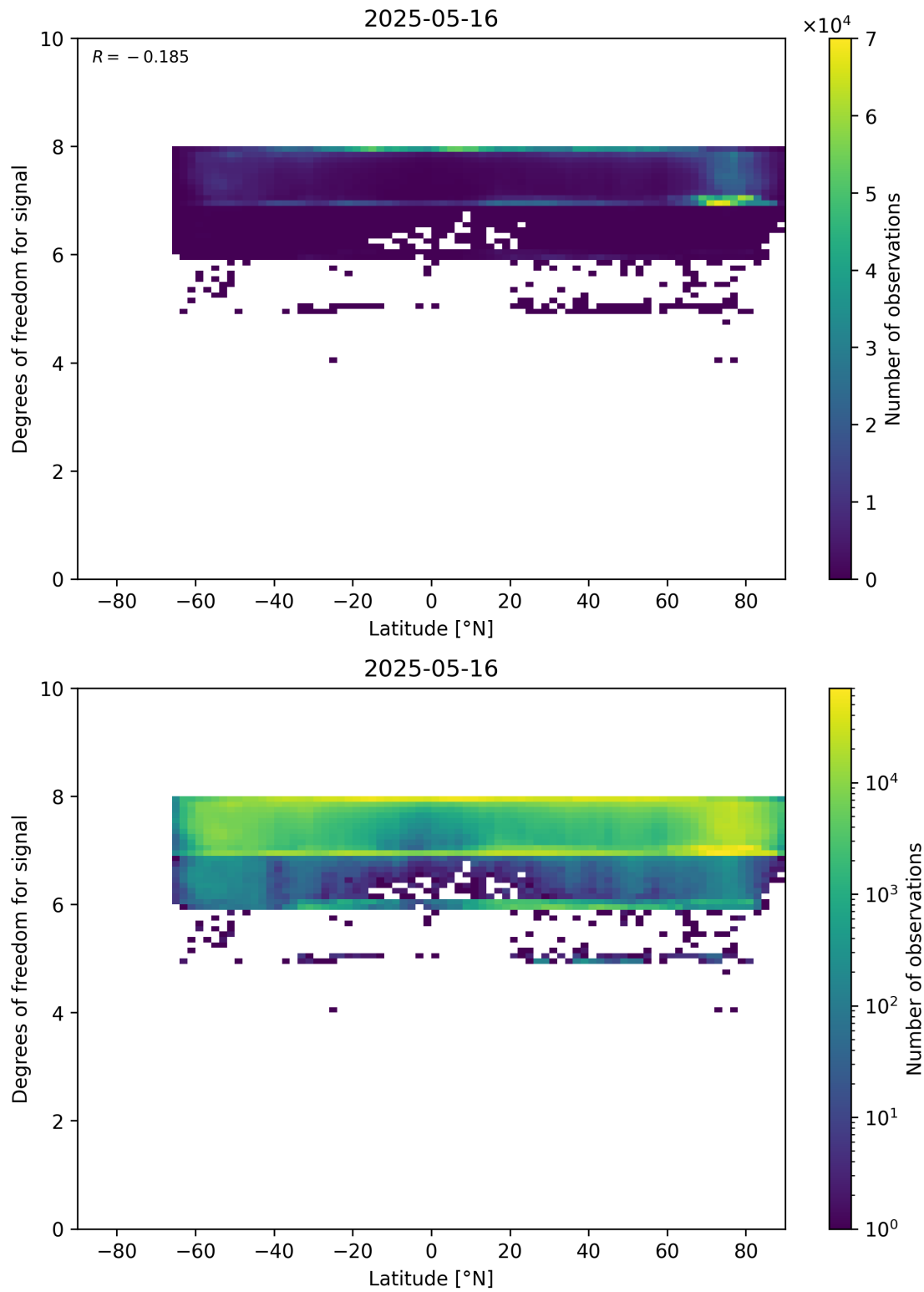
Figure 55: Scatter density plot of “Latitude” against “Degrees of freedom for signal” for 2025-05-15 to 2025-05-17.
