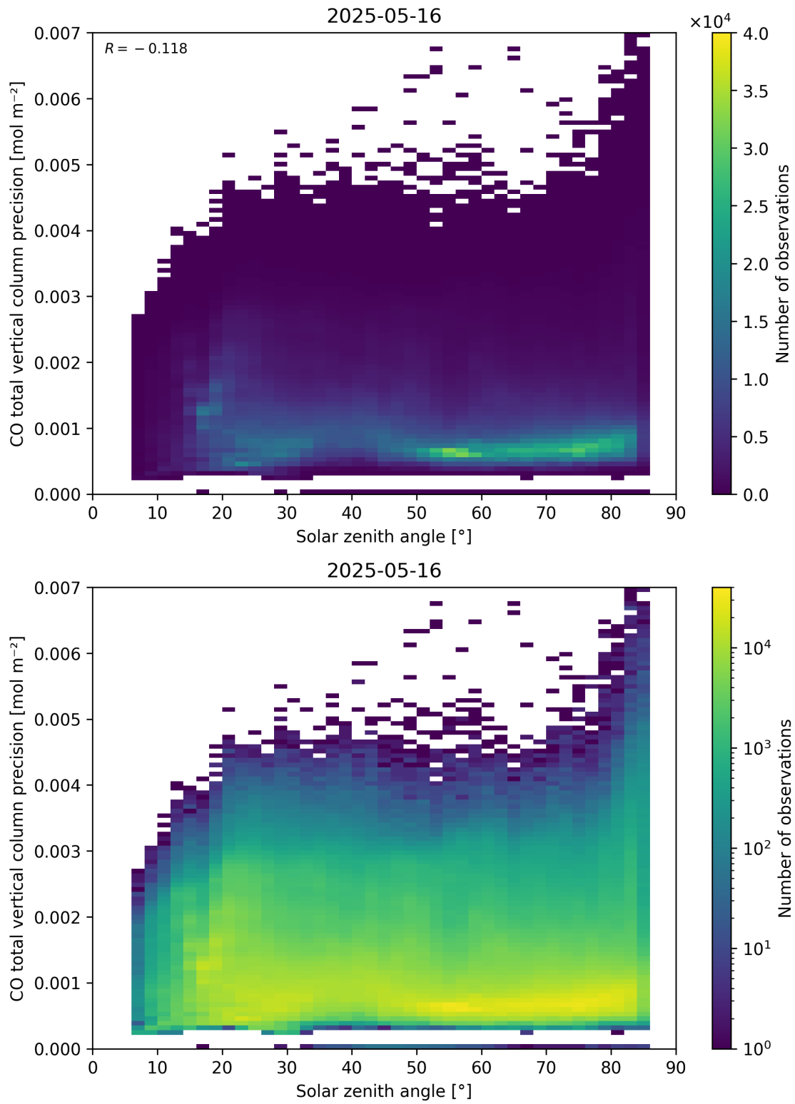
Figure 63: Scatter density plot of “Solar zenith angle” against “CO total vertical column precision” for 2025-05-15 to 2025-05-17.
