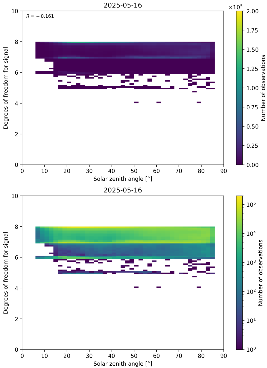
Figure 65: Scatter density plot of “Solar zenith angle” against “Degrees of freedom for signal” for 2025-05-15 to 2025-05-17.
