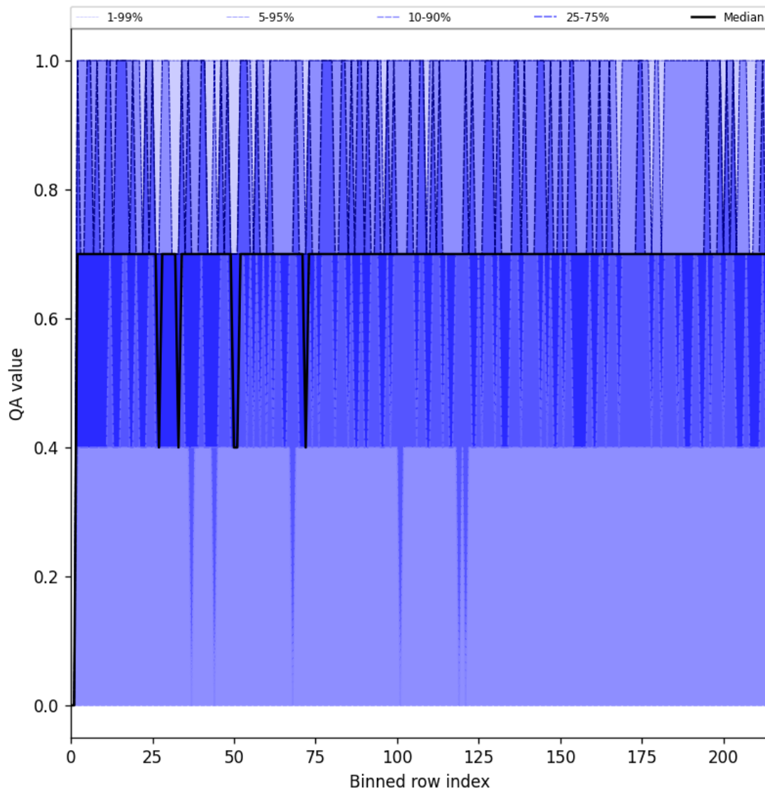
Figure 25: Along track statistics of “QA value” for 2025-05-15 to 2025-05-17
