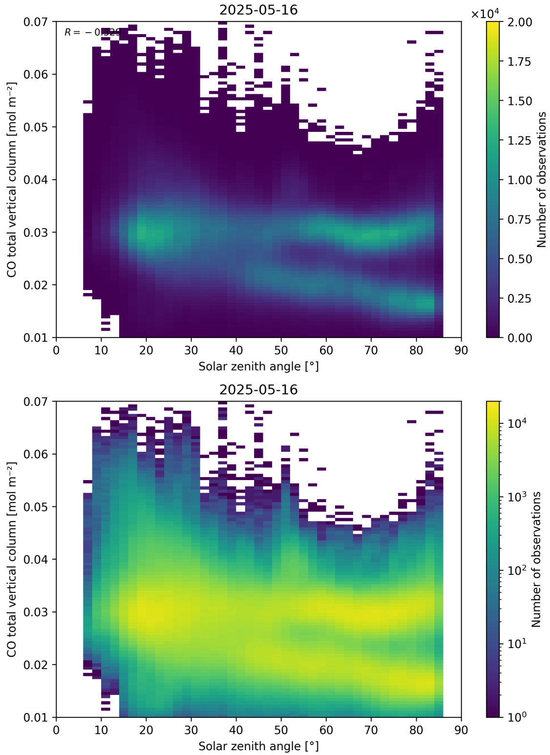
Figure 61: Scatter density plot of “Solar zenith angle” against “CO total vertical column” for 2025-05-15 to 2025-05-17.
