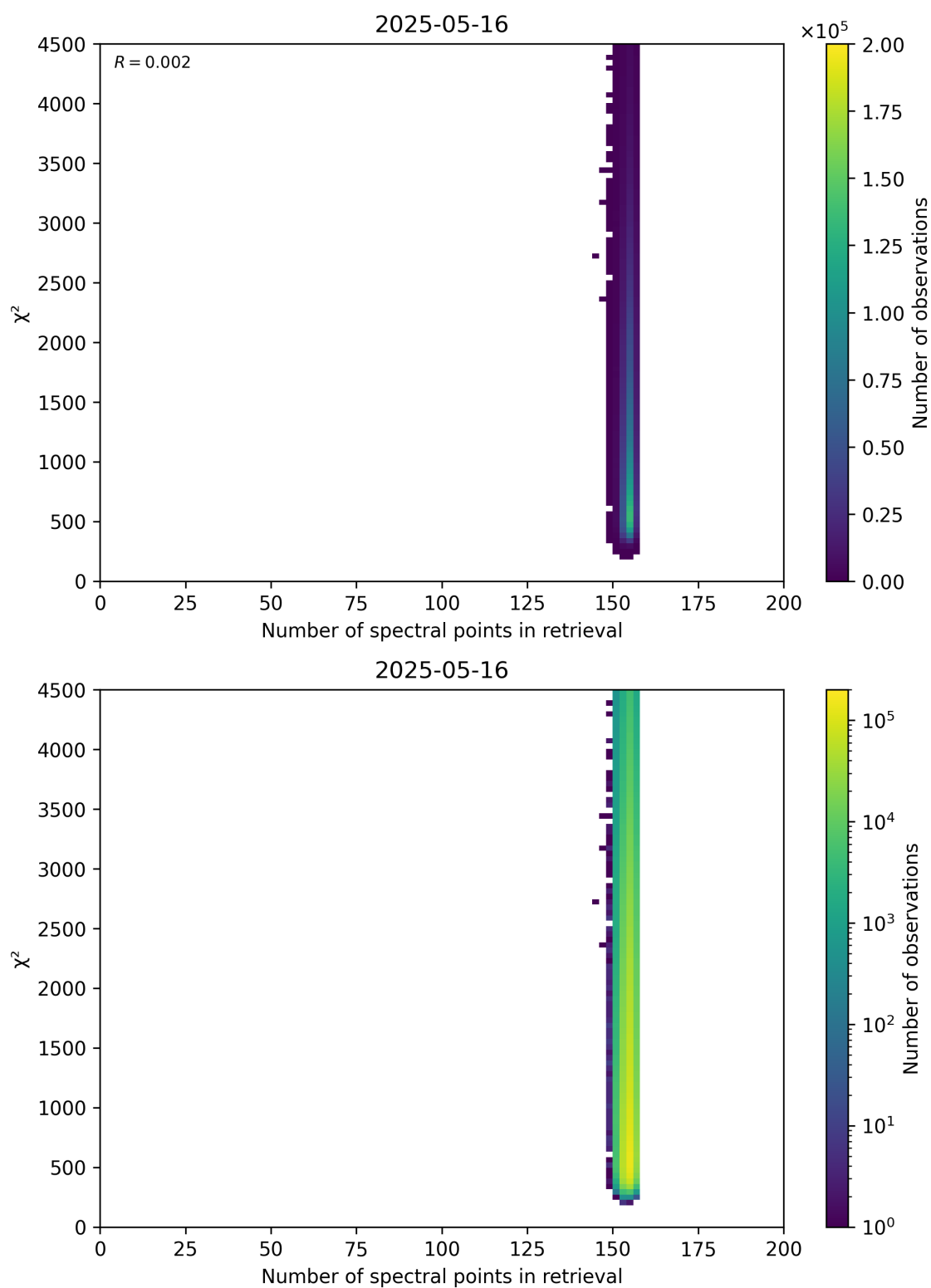
Figure 58: Scatter density plot of “Number of spectral points in retrieval” against “ \chi^2 ” for 2025-05-15 to 2025-05-17.
