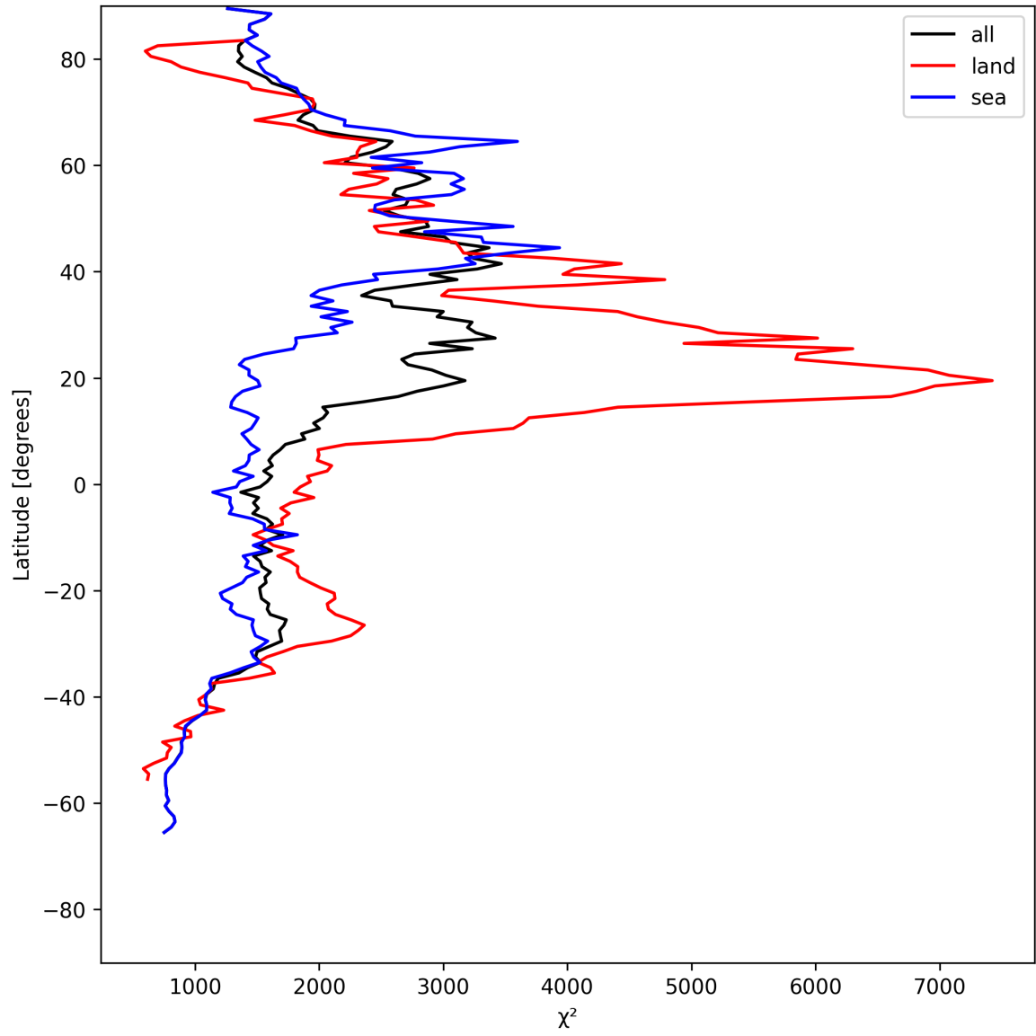
Figure 14: Zonal average of “ \chi^2 ” for 2025-05-15 to 2025-05-17.
