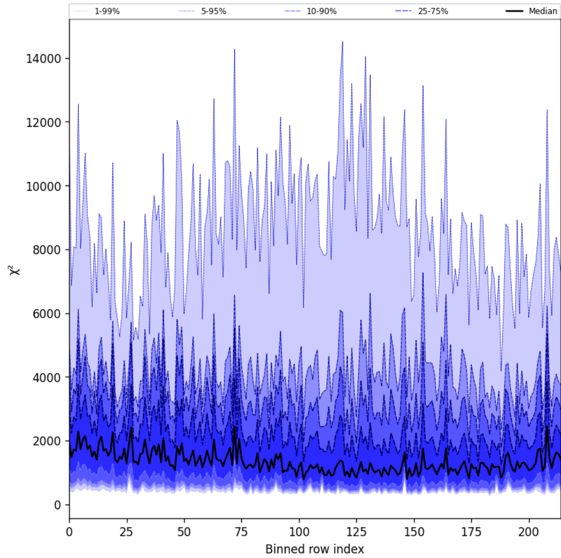
Figure 30: Along track statistics of “ \chi^2 ” for 2025-05-15 to 2025-05-17
