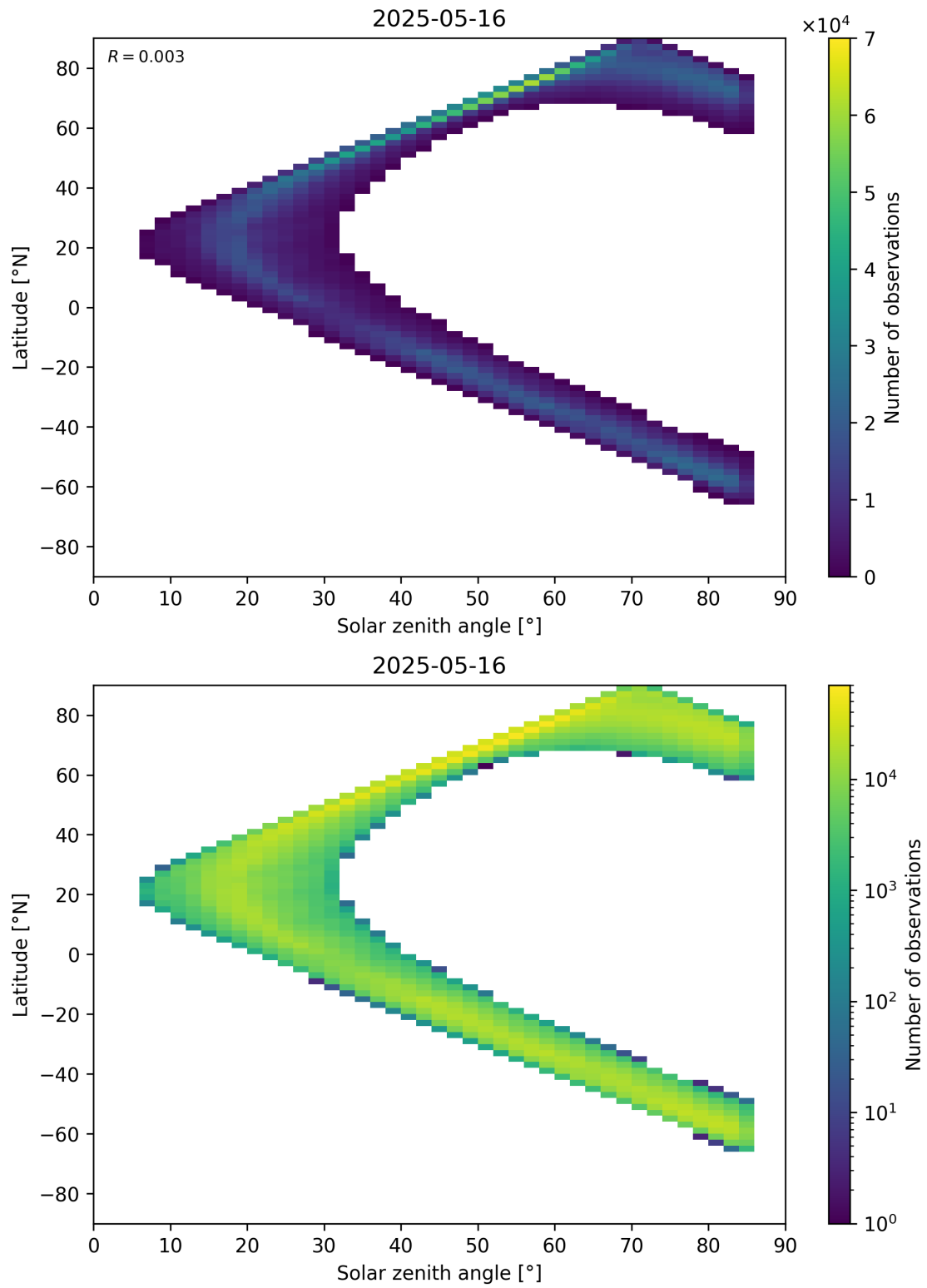
Figure 66: Scatter density plot of “Solar zenith angle” against “Latitude” for 2025-05-15 to 2025-05-17.
