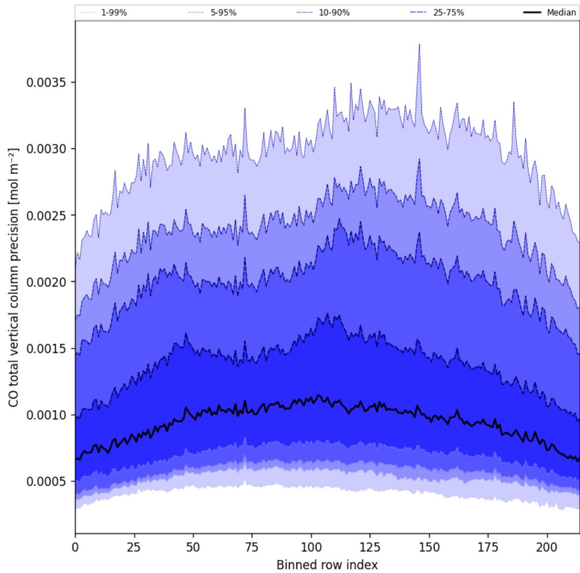
Figure 28: Along track statistics of “CO total vertical column precision” for 2025-05-15 to 2025-05-17
