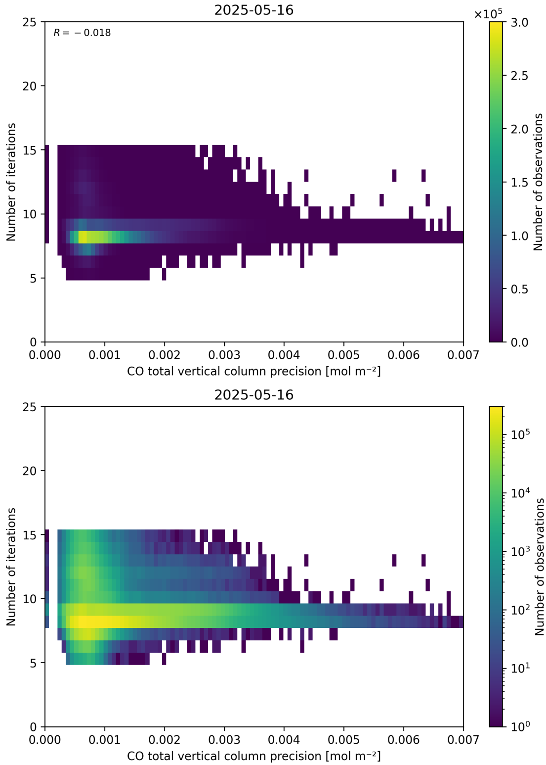
Figure 46: Scatter density plot of “CO total vertical column precision” against “Number of iterations” for 2025-05-15 to 2025-05-17.
