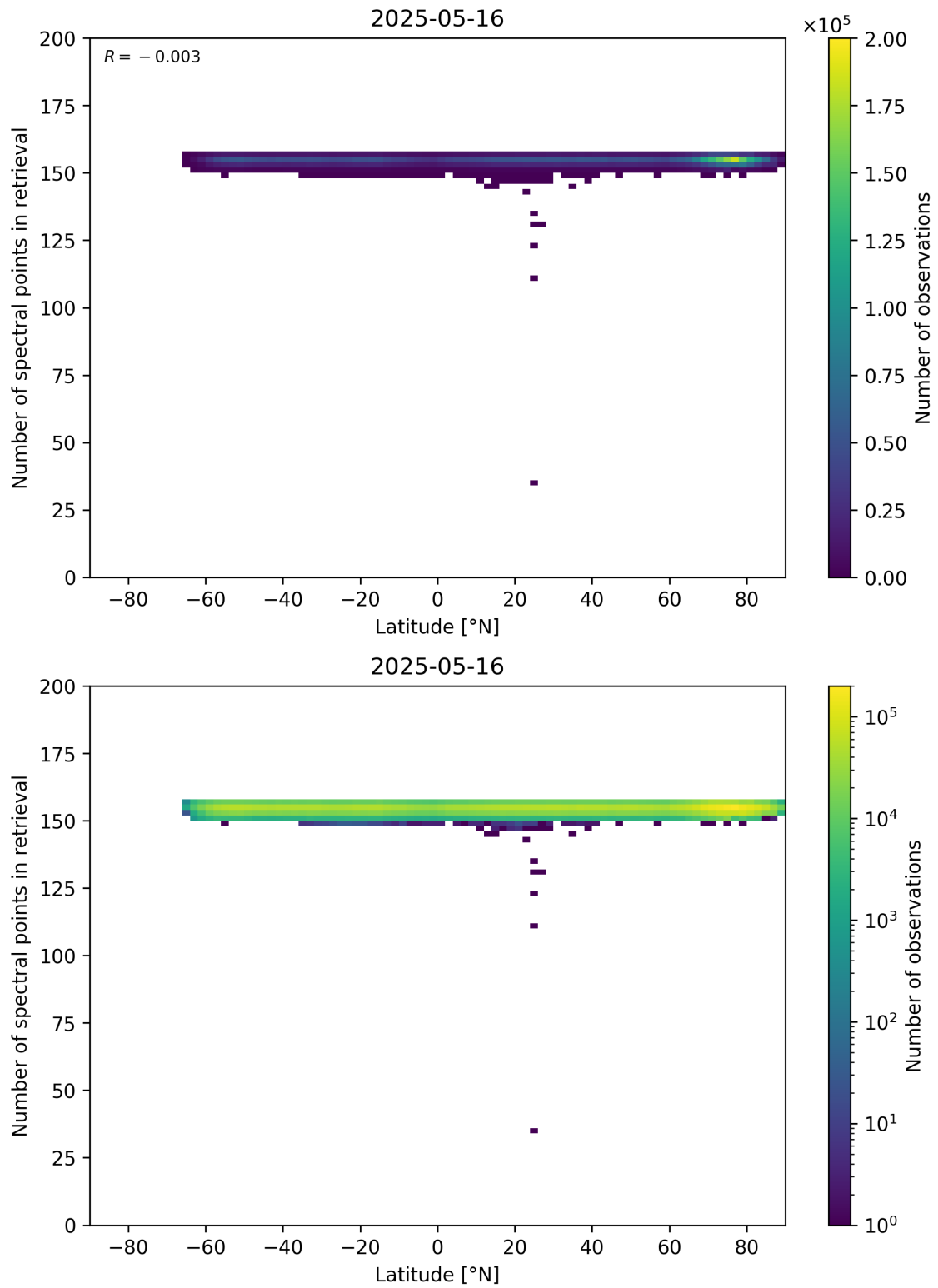
Figure 57: Scatter density plot of “Latitude” against “Number of spectral points in retrieval” for 2025-05-15 to 2025-05-17.
