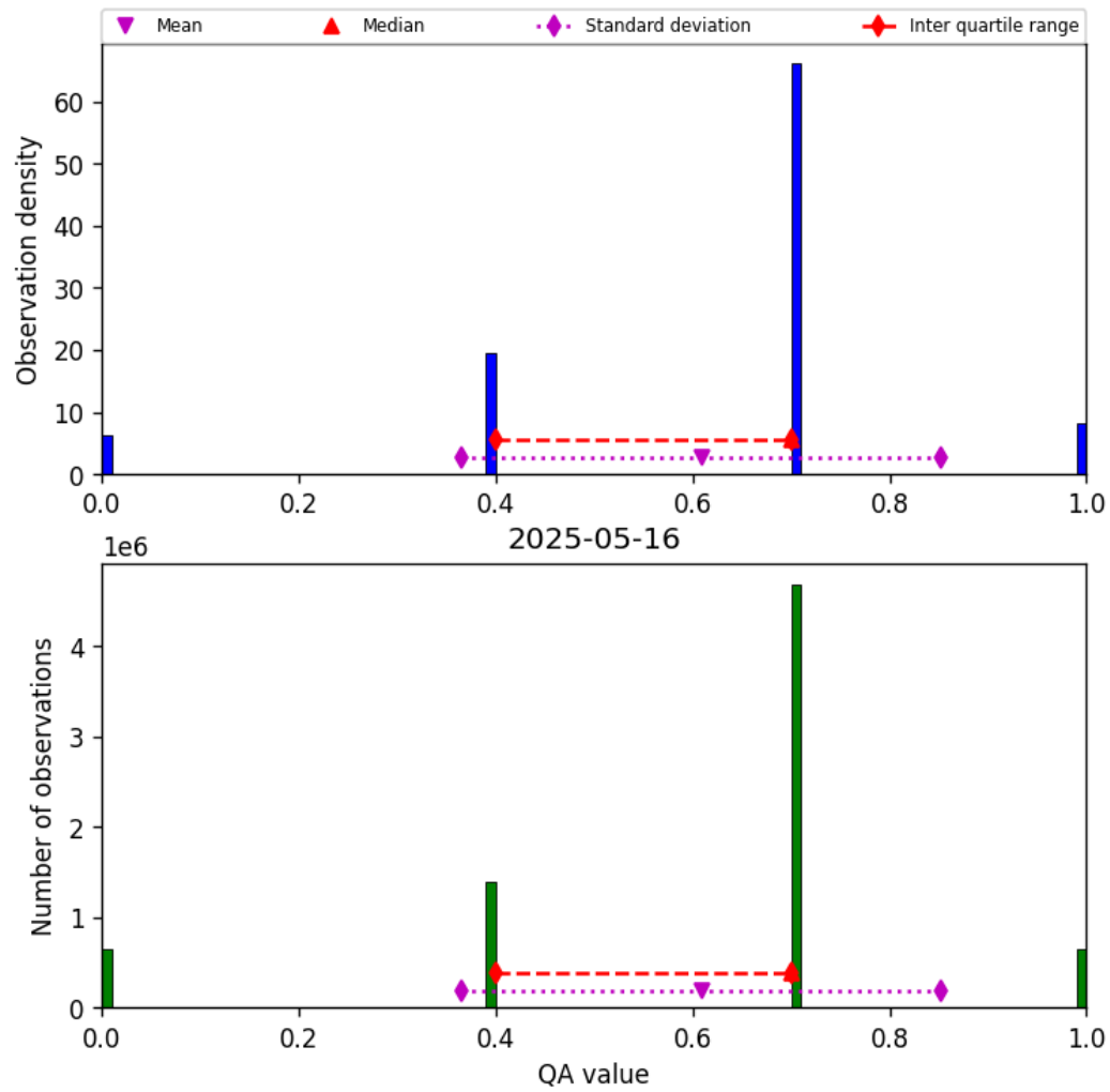
Figure 17: Histogram of “QA value” for 2025-05-15 to 2025-05-17
