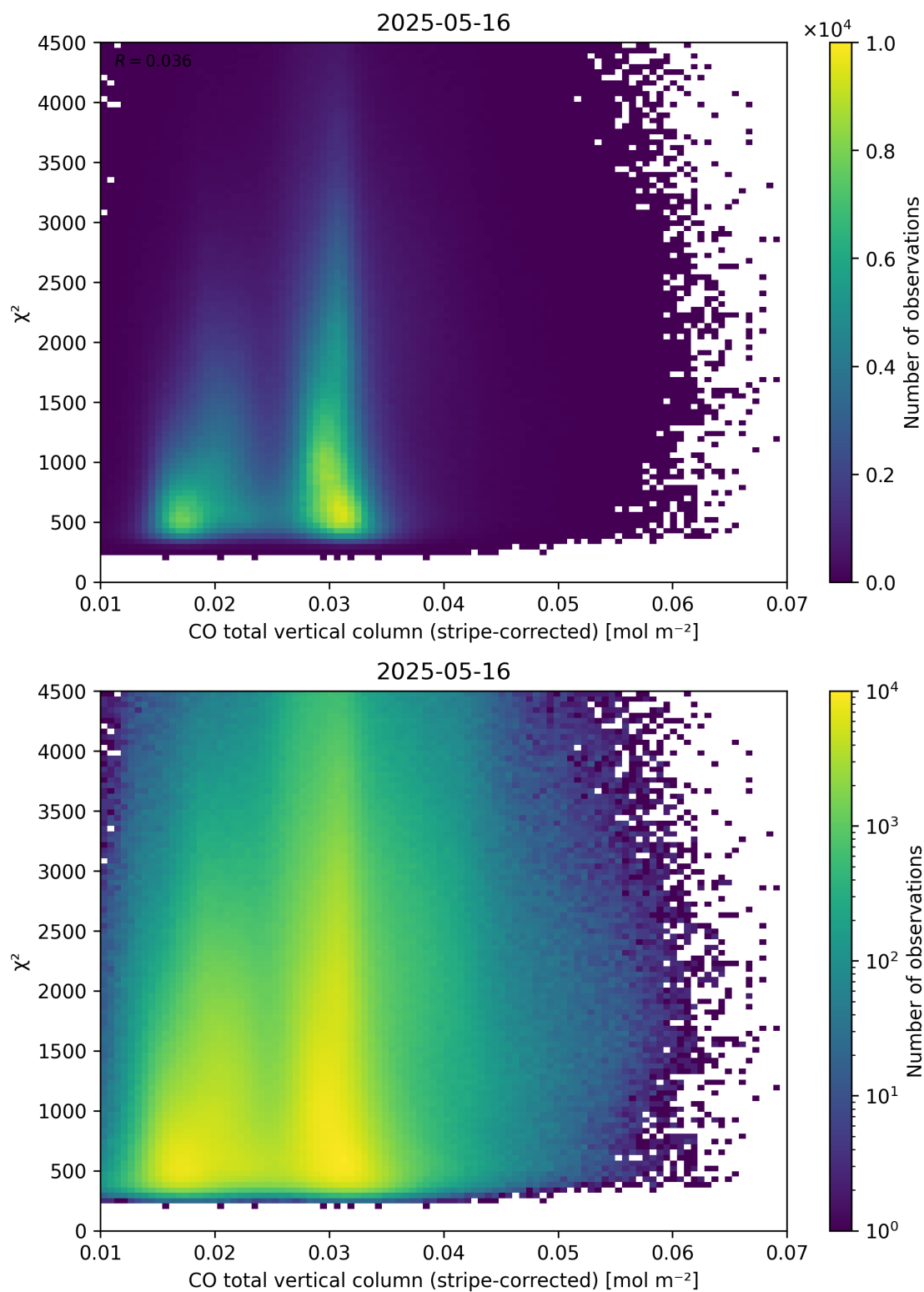
Figure 37: Scatter density plot of “CO total vertical column (stripe-corrected)” against “ \chi^2 ” for 2025-05-15 to 2025-05-17.
