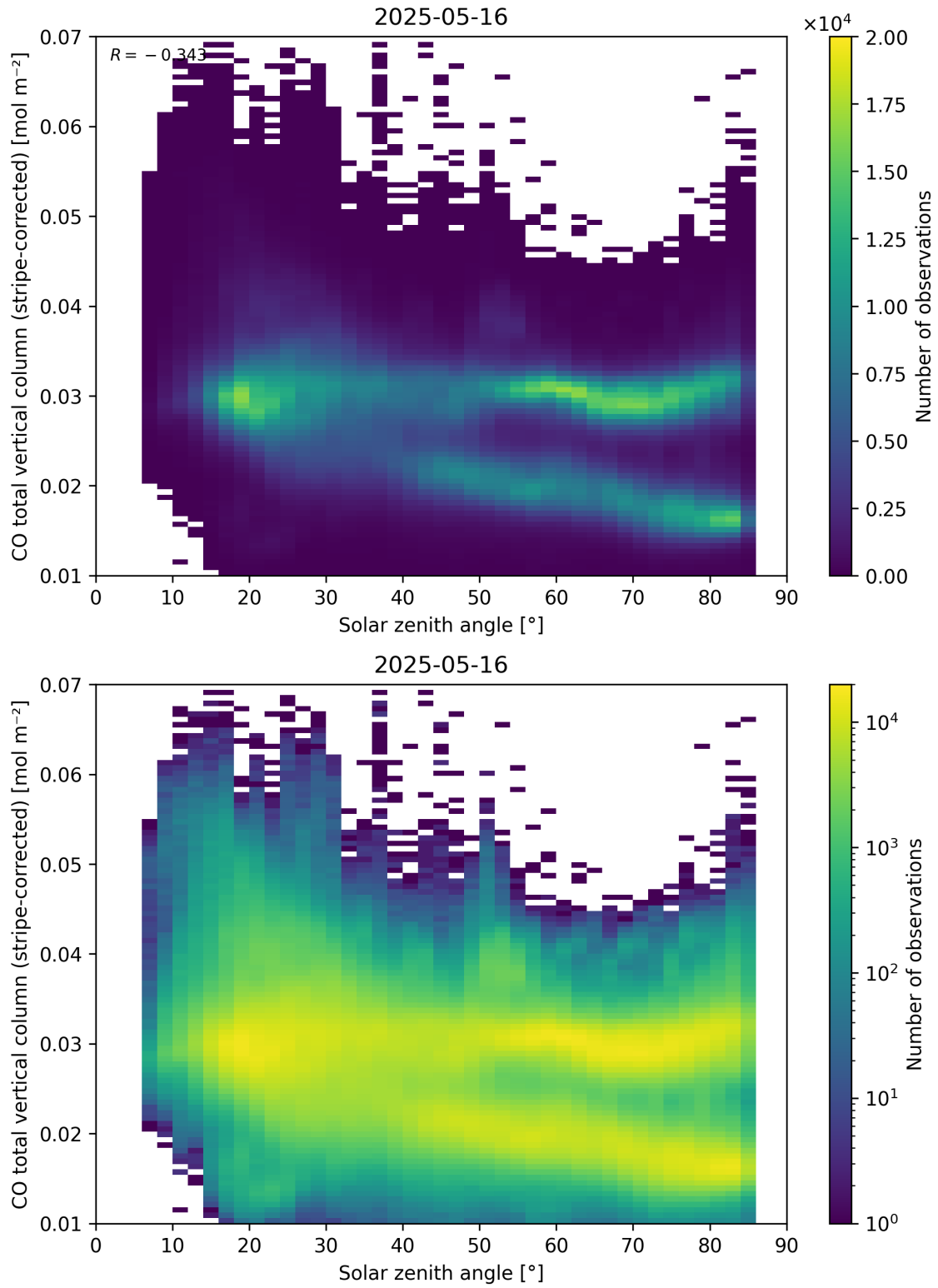
Figure 62: Scatter density plot of “Solar zenith angle” against “CO total vertical column (stripe-corrected)” for 2025-05-15 to 2025-05-17.
