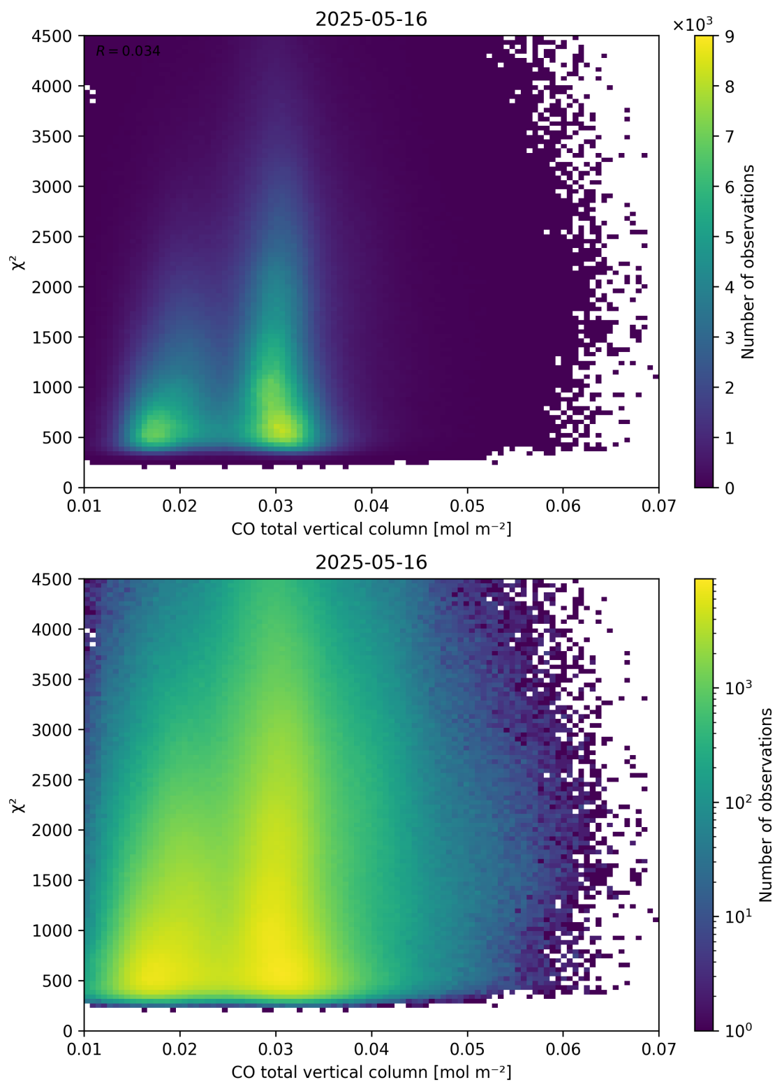
Figure 35: Scatter density plot of “CO total vertical column” against “ \chi^2 ” for 2025-05-15 to 2025-05-17.
