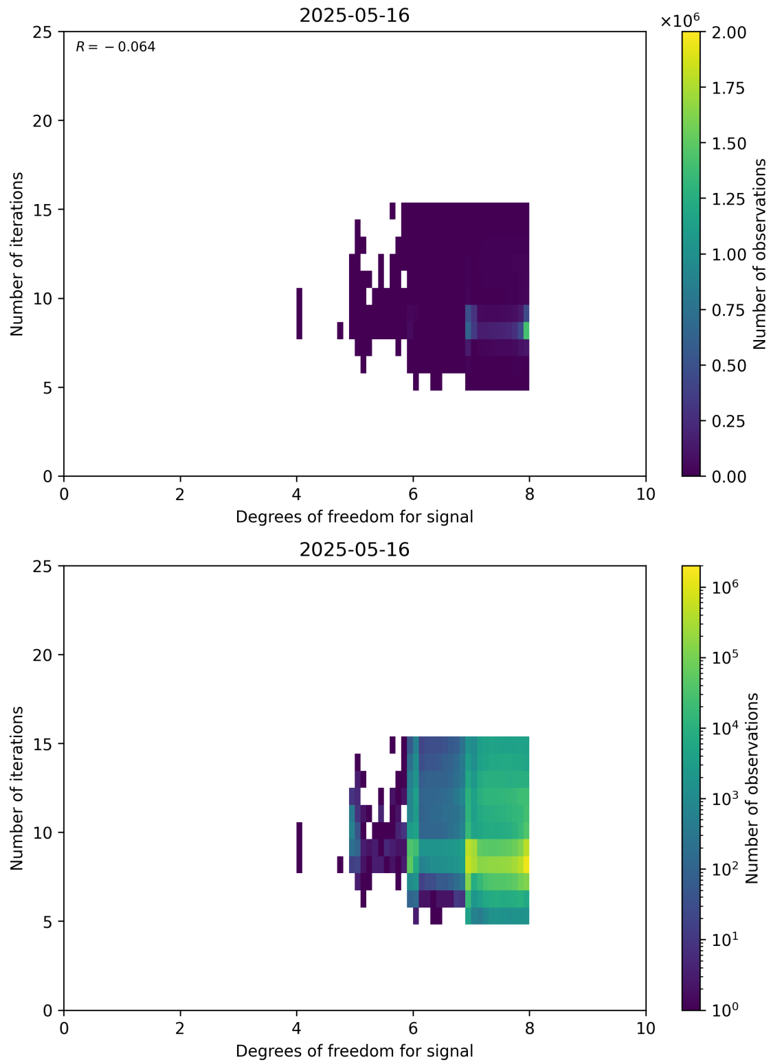
Figure 50: Scatter density plot of “Degrees of freedom for signal” against “Number of iterations” for 2025-05-15 to 2025-05-17.
