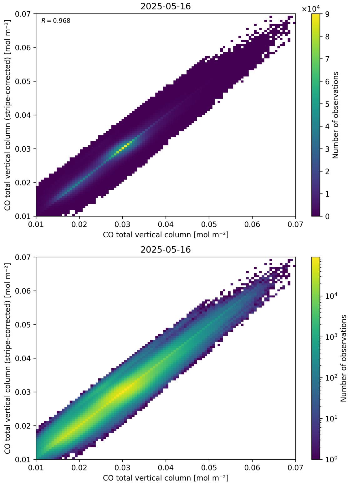
Figure 33: Scatter density plot of “CO total vertical column” against “CO total vertical column (stripe-corrected)” for 2025-05-15 to 2025-05-17.
