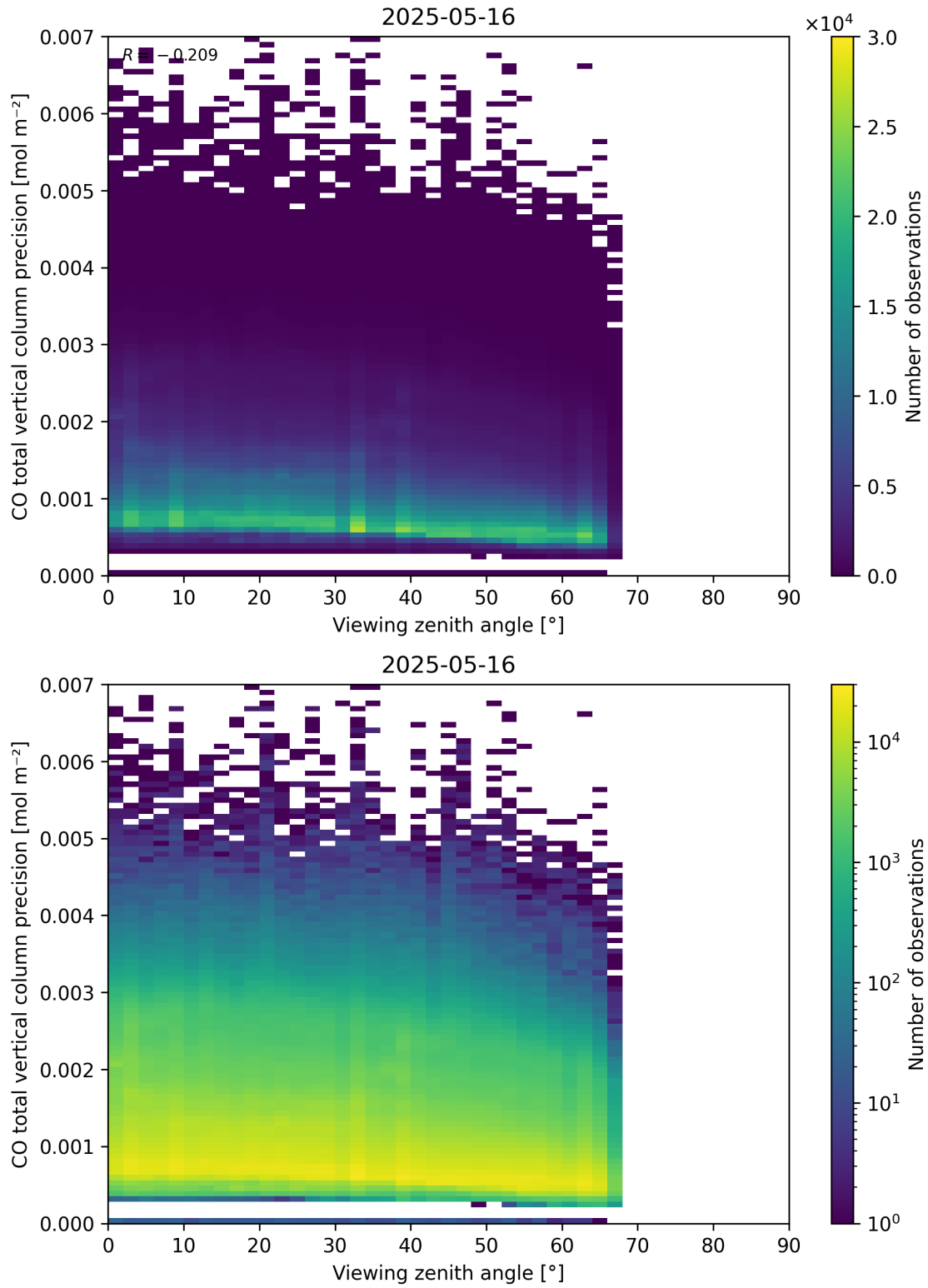
Figure 71: Scatter density plot of “Viewing zenith angle” against “CO total vertical column precision” for 2025-05-15 to 2025-05-17.
