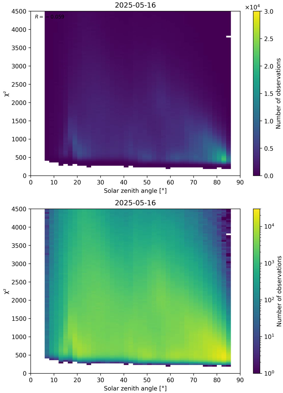
Figure 64: Scatter density plot of “Solar zenith angle” against “ \chi^2 ” for 2025-05-15 to 2025-05-17.
