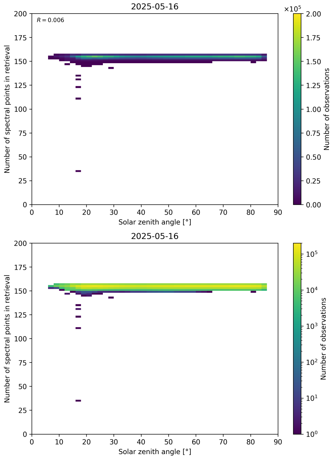
Figure 68: Scatter density plot of “Solar zenith angle” against “Number of spectral points in retrieval” for 2025-05-15 to 2025-05-17.
