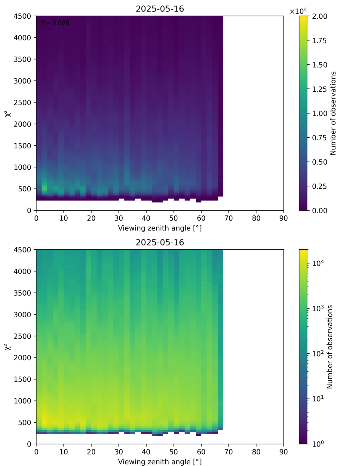
Figure 72: Scatter density plot of “Viewing zenith angle” against “ \chi^2 ” for 2025-05-15 to 2025-05-17.
