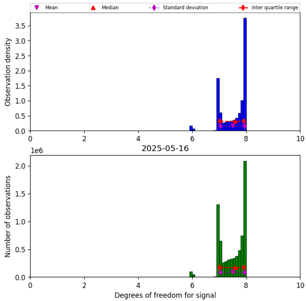
Figure 23: Histogram of “Degrees of freedom for signal” for 2025-05-15 to 2025-05-17
