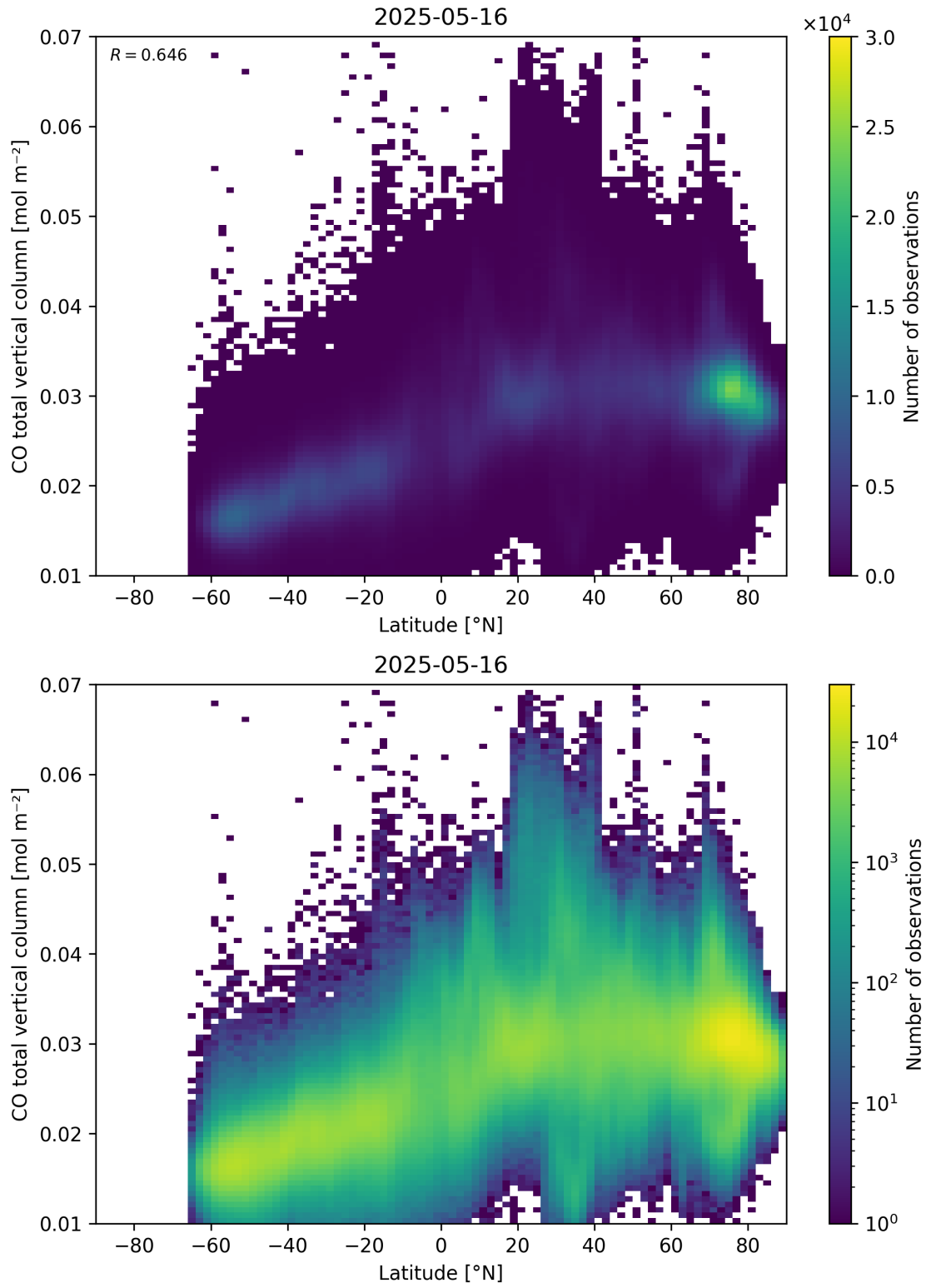
Figure 51: Scatter density plot of “Latitude” against “CO total vertical column” for 2025-05-15 to 2025-05-17.
