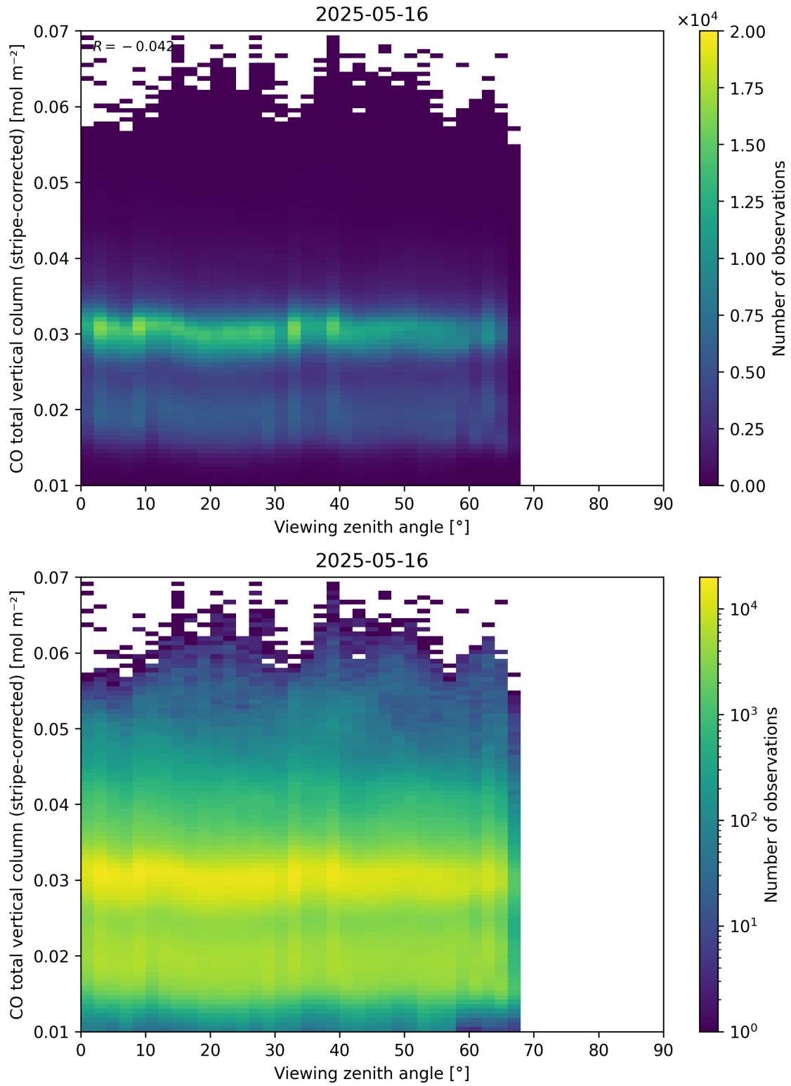
Figure 70: Scatter density plot of “Viewing zenith angle” against “CO total vertical column (stripe-corrected)” for 2025-05-15 to 2025-05-17.
