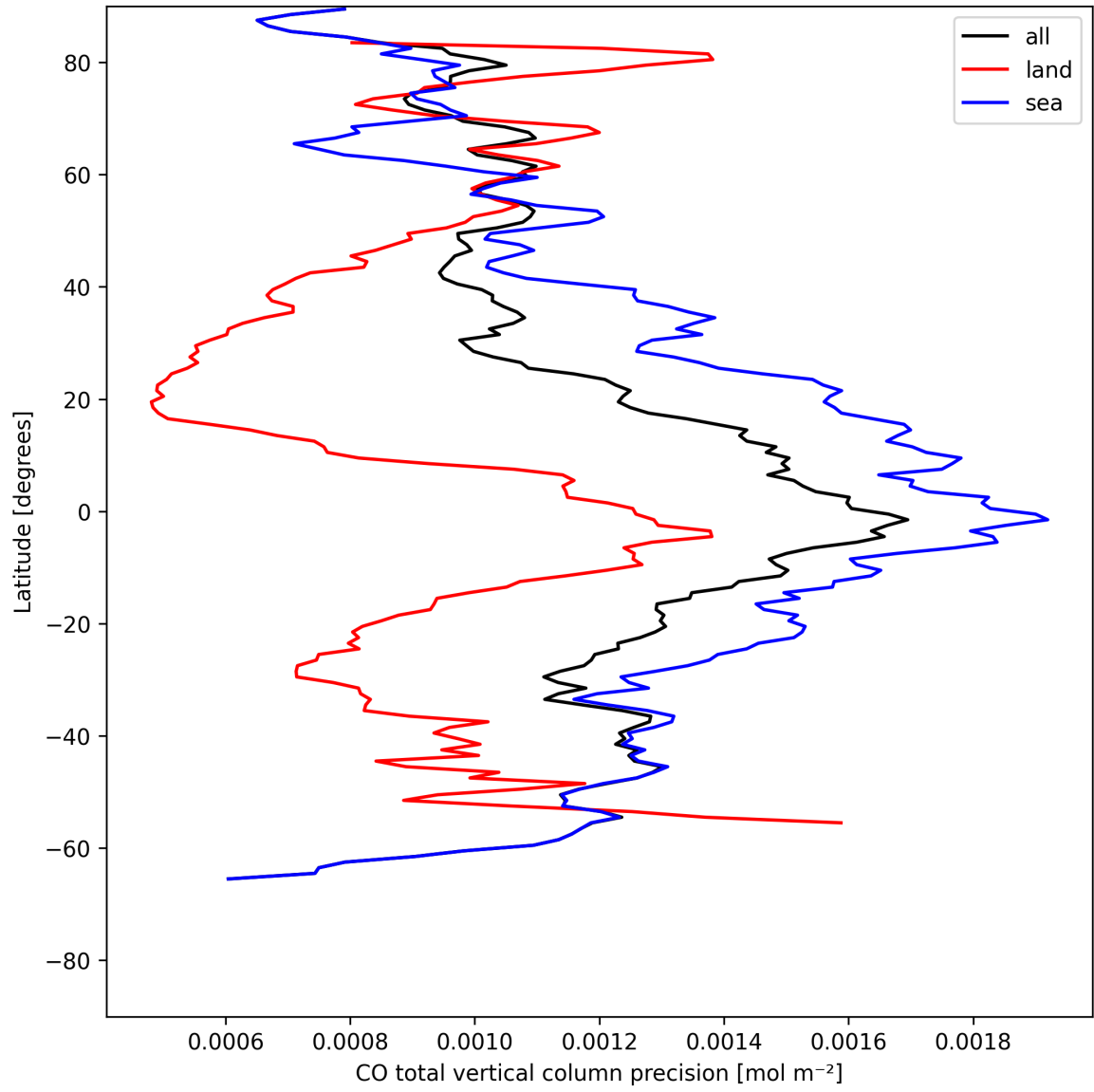
Figure 12: Zonal average of “CO total vertical column precision” for 2025-05-15 to 2025-05-17.
