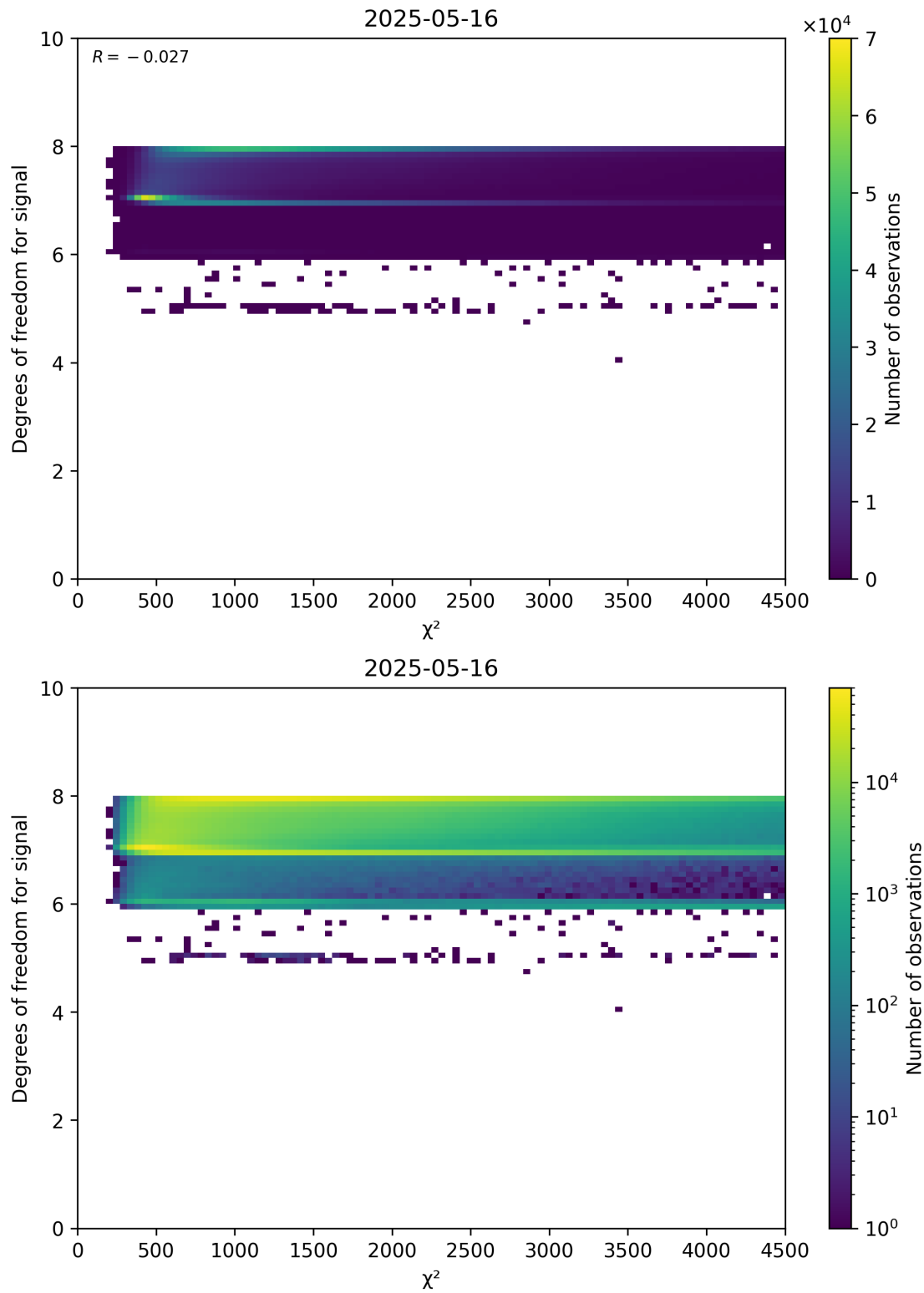
Figure 48: Scatter density plot of “ \chi^2 ” against “Degrees of freedom for signal” for 2025-05-15 to 2025-05-17.
