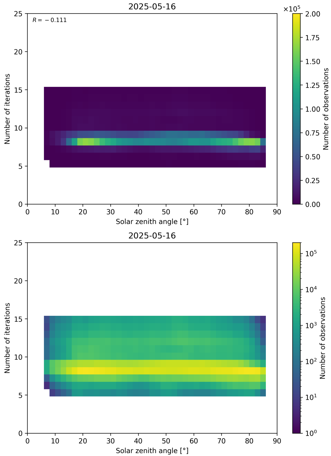
Figure 67: Scatter density plot of “Solar zenith angle” against “Number of iterations” for 2025-05-15 to 2025-05-17.
