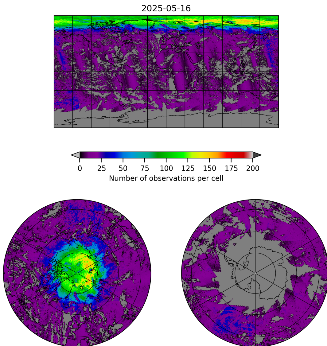
Figure 8: Map of the number of observations for 2025-05-15 to 2025-05-17
