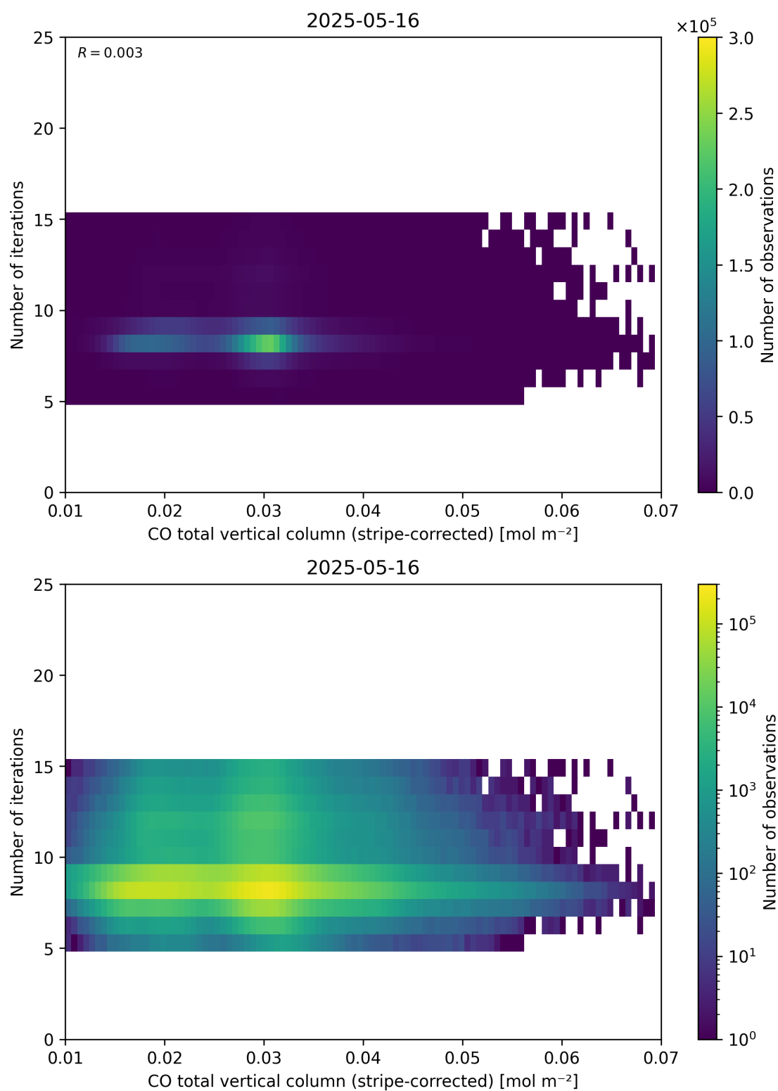
Figure 39: Scatter density plot of “CO total vertical column (stripe-corrected)” against “Number of iterations” for 2025-05-15 to 2025-05-17.
