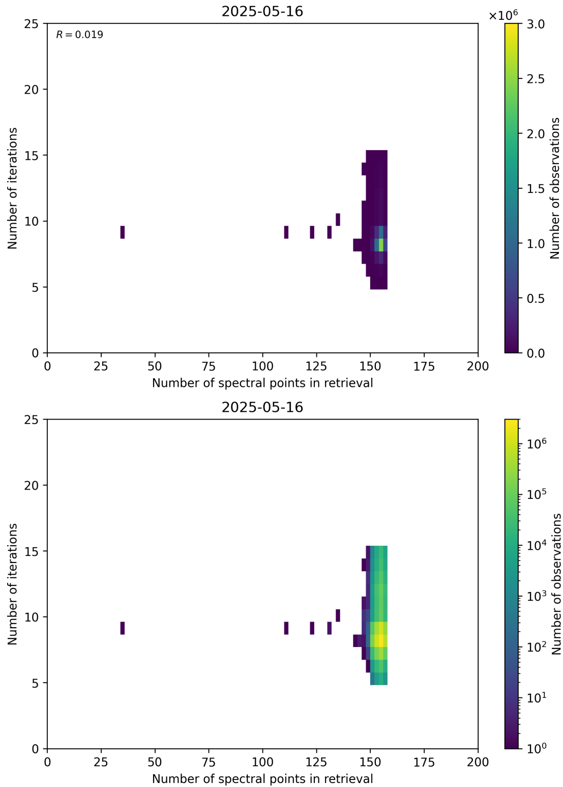
Figure 60: Scatter density plot of “Number of spectral points in retrieval” against “Number of iterations” for 2025-05-15 to 2025-05-17.
