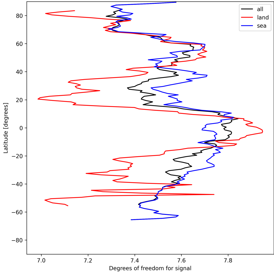
Figure 15: Zonal average of “Degrees of freedom for signal” for 2025-05-15 to 2025-05-17.
