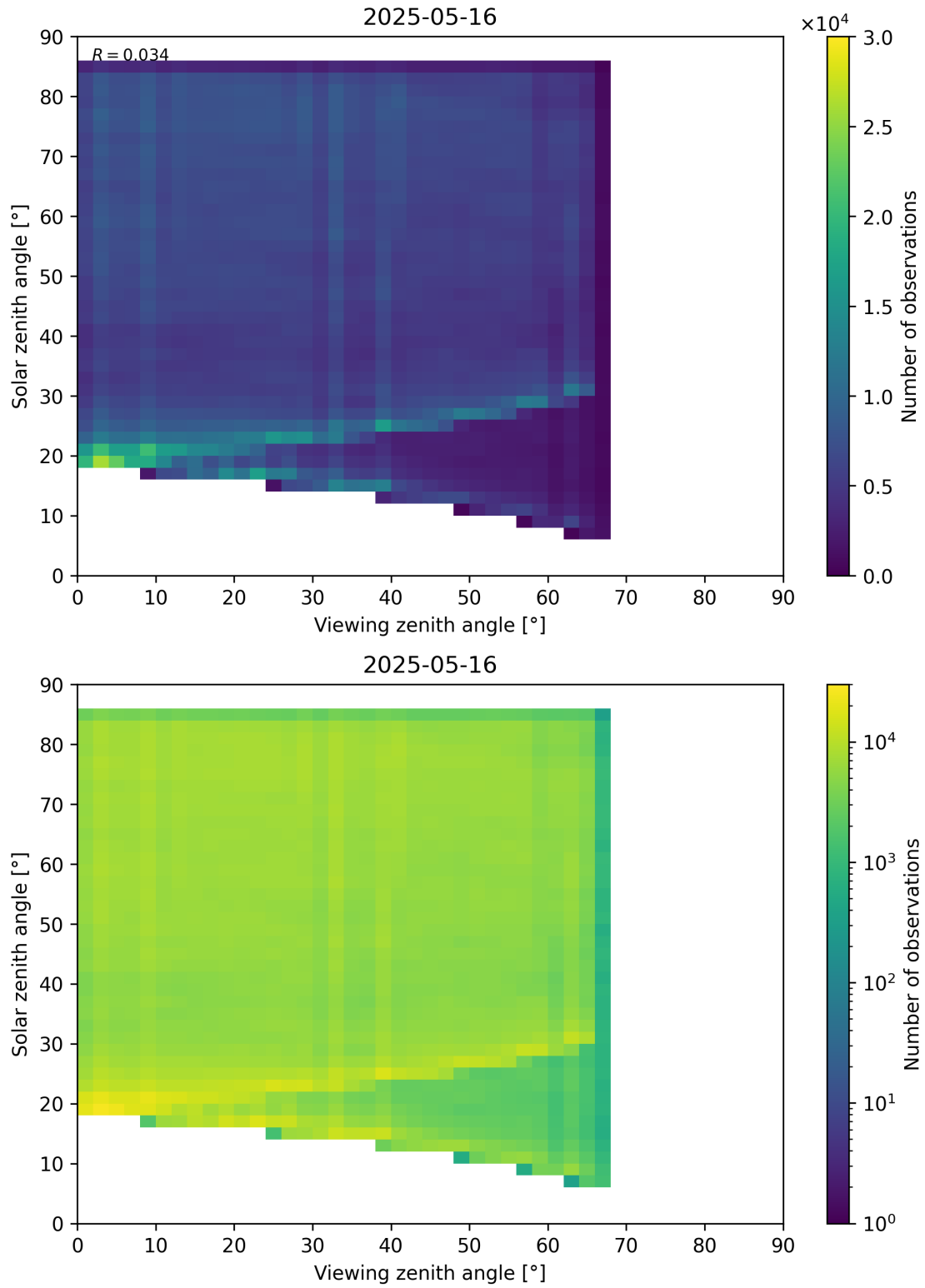
Figure 77: Scatter density plot of “Viewing zenith angle” against “Solar zenith angle” for 2025-05-15 to 2025-05-17.
