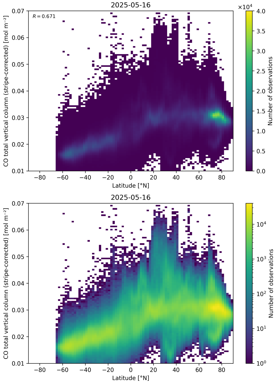
Figure 52: Scatter density plot of “Latitude” against “CO total vertical column (stripe-corrected)” for 2025-05-15 to 2025-05-17.
