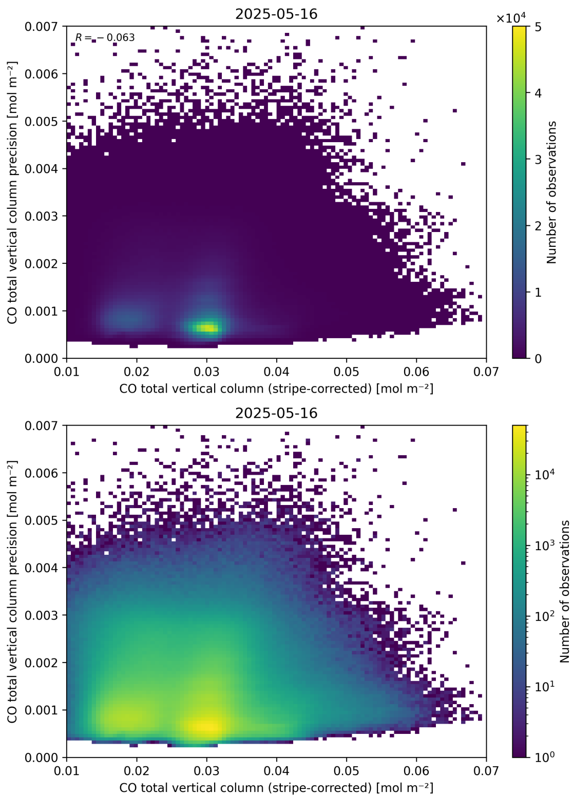
Figure 36: Scatter density plot of “CO total vertical column (stripe-corrected)” against “CO total vertical column precision” for 2025-05-15 to 2025-05-17.
