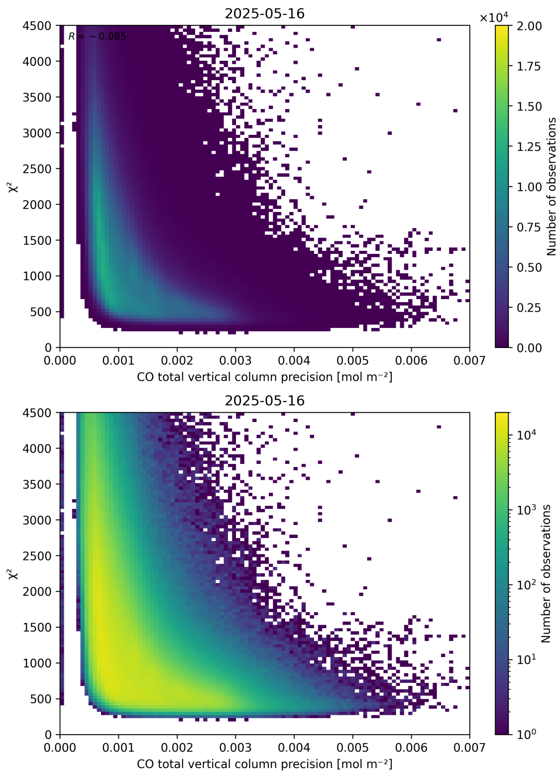
Figure 44: Scatter density plot of “CO total vertical column precision” against “ \chi^2 ” for 2025-05-15 to 2025-05-17.
