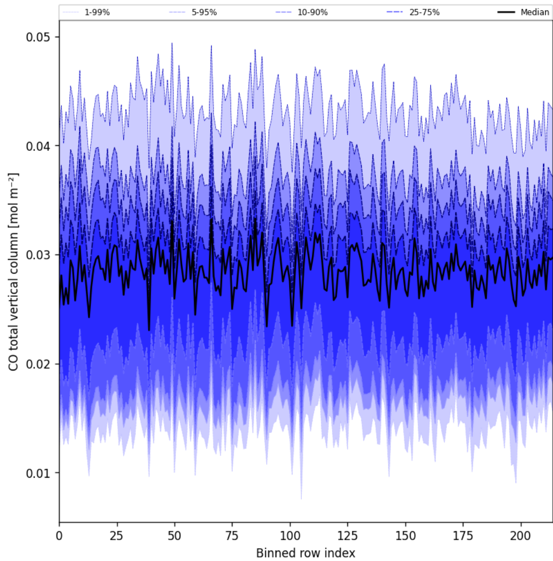
Figure 26: Along track statistics of “CO total vertical column” for 2025-05-15 to 2025-05-17
