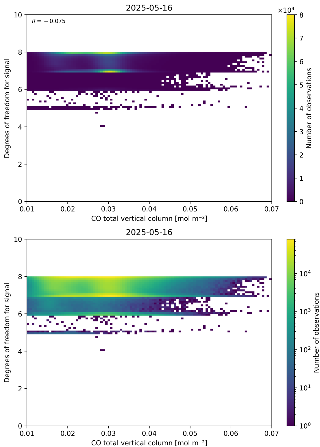
Figure 41: Scatter density plot of “CO total vertical column” against “Degrees of freedom for signal” for 2025-05-15 to 2025-05-17.
