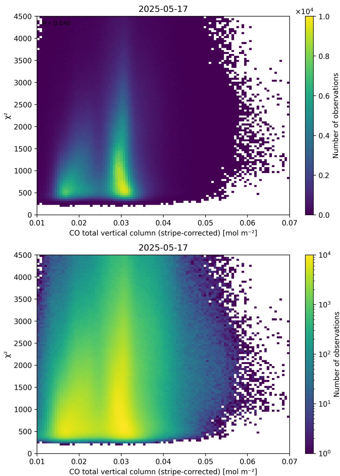
Figure 37: Scatter density plot of “CO total vertical column (stripe-corrected)” against “ \chi^2 ” for 2025-05-16 to 2025-05-18.
