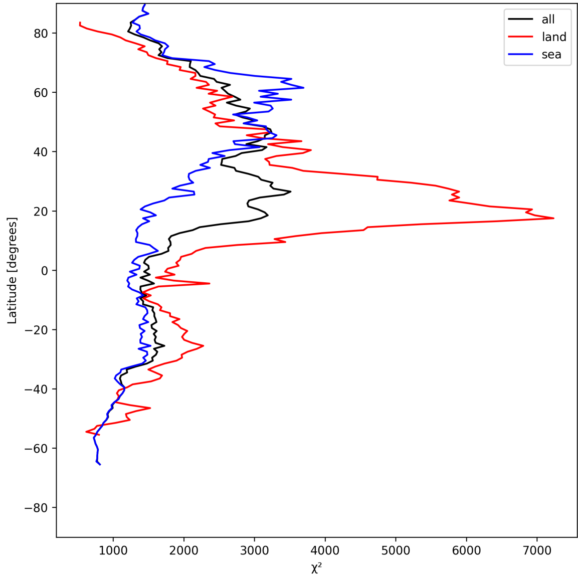
Figure 14: Zonal average of “ \chi^2 ” for 2025-05-16 to 2025-05-18.
