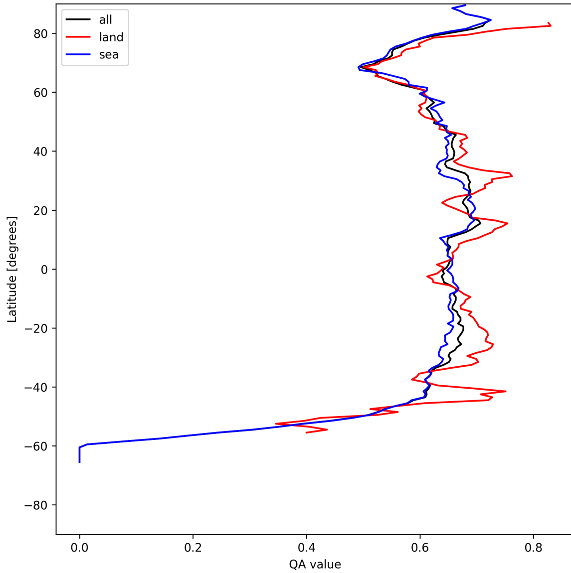
Figure 9: Zonal average of “QA value” for 2025-05-16 to 2025-05-18.
