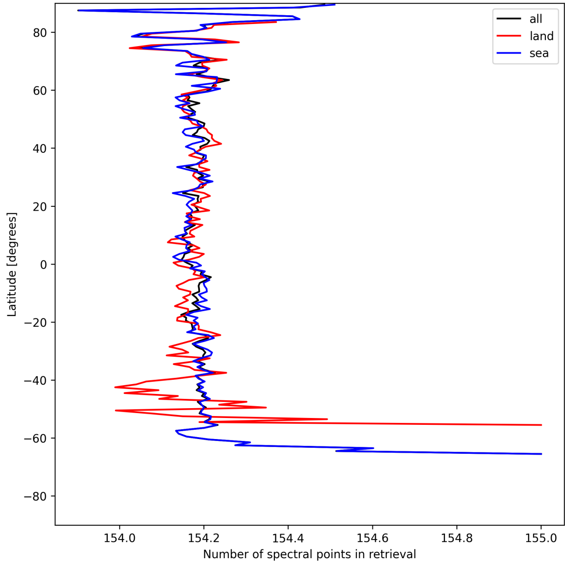
Figure 13: Zonal average of “Number of spectral points in retrieval” for 2025-05-16 to 2025-05-18.
