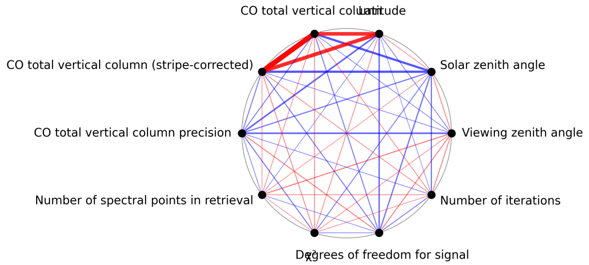
Figure 1: Map of correlation graph for 2025-05-16 to 2025-05-18.
