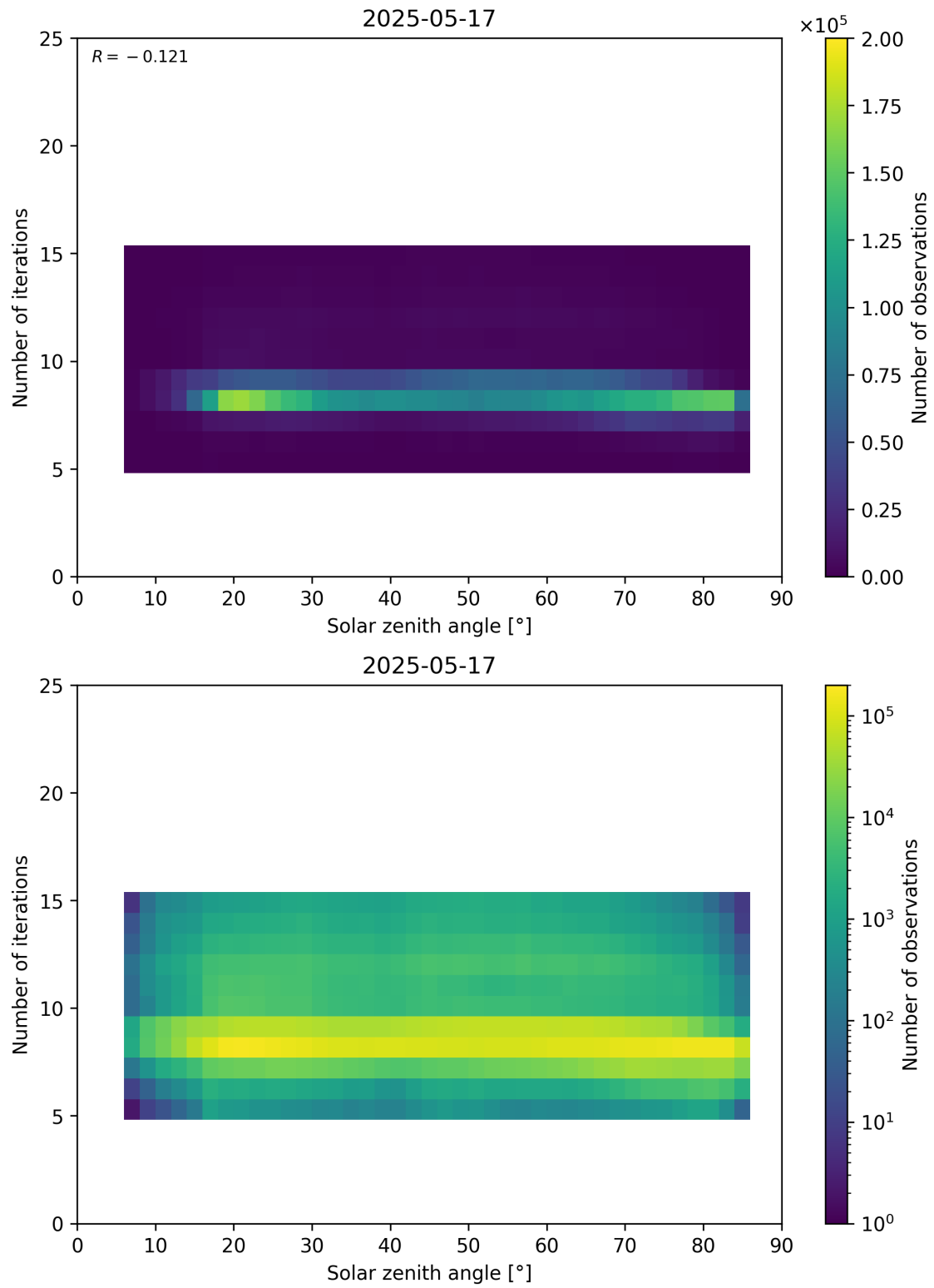
Figure 67: Scatter density plot of “Solar zenith angle” against “Number of iterations” for 2025-05-16 to 2025-05-18.
