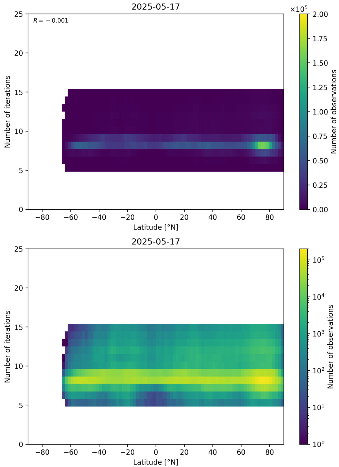
Figure 56: Scatter density plot of “Latitude” against “Number of iterations” for 2025-05-16 to 2025-05-18.
