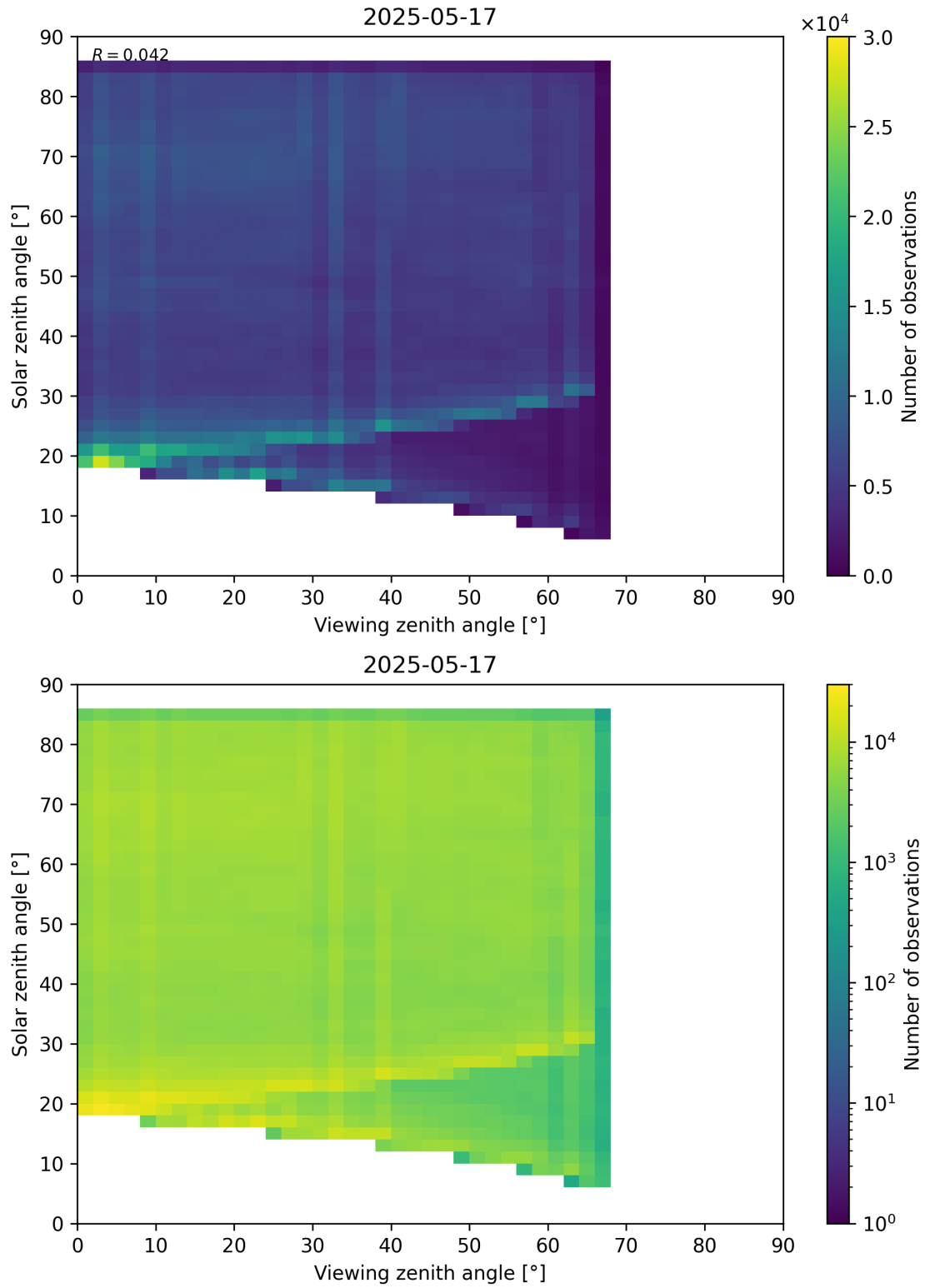
Figure 77: Scatter density plot of “Viewing zenith angle” against “Solar zenith angle” for 2025-05-16 to 2025-05-18.
