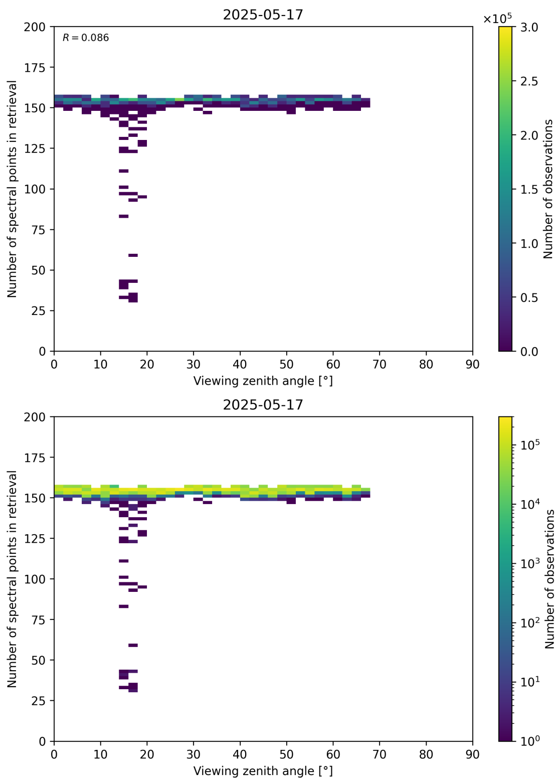
Figure 76: Scatter density plot of “Viewing zenith angle” against “Number of spectral points in retrieval” for 2025-05-16 to 2025-05-18.
