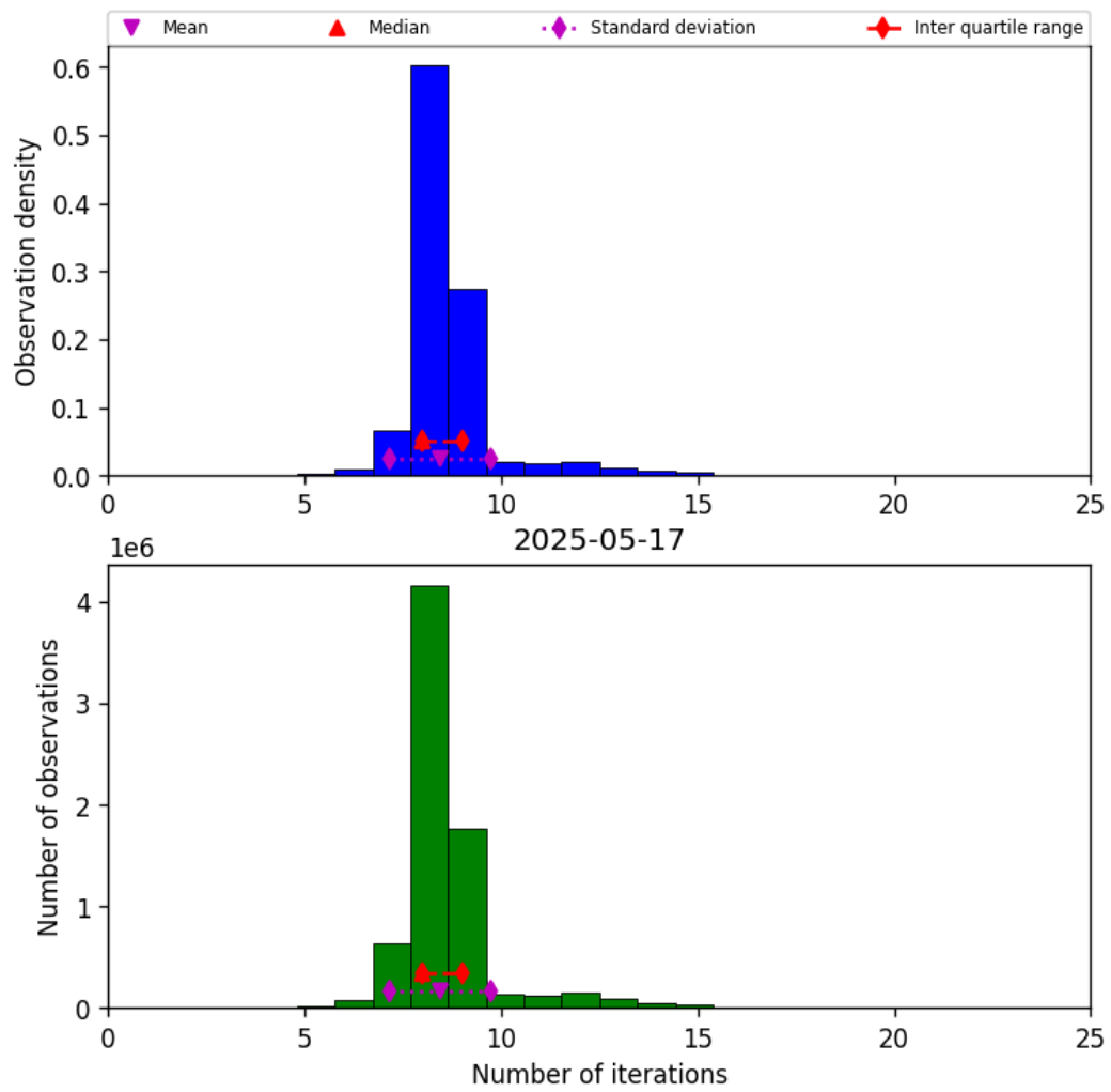
Figure 24: Histogram of “Number of iterations” for 2025-05-16 to 2025-05-18
