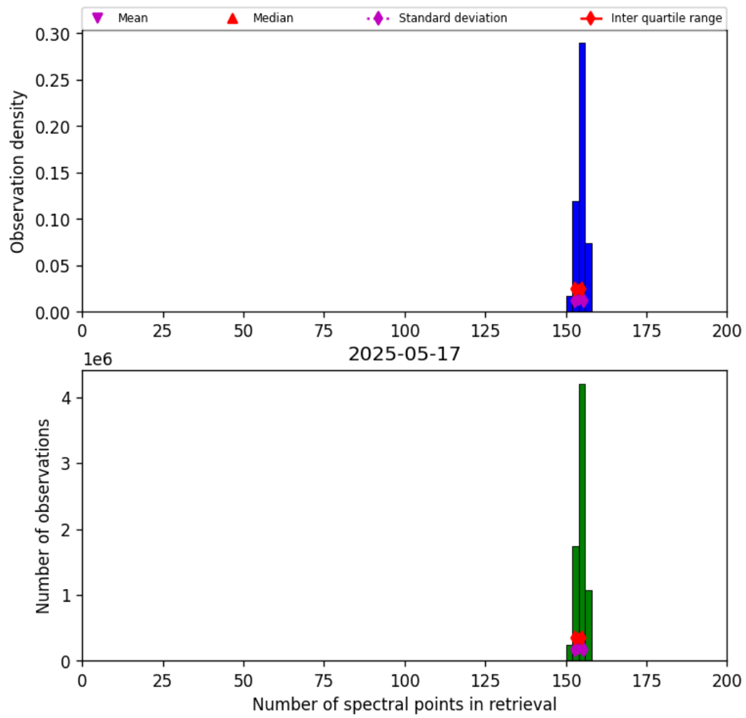
Figure 21: Histogram of “Number of spectral points in retrieval” for 2025-05-16 to 2025-05-18
