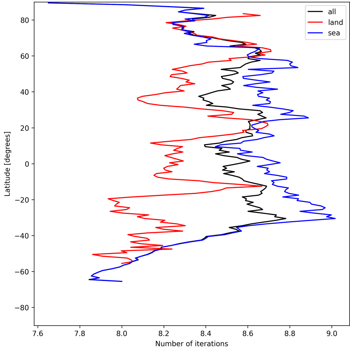
Figure 16: Zonal average of “Number of iterations” for 2025-05-16 to 2025-05-18.
