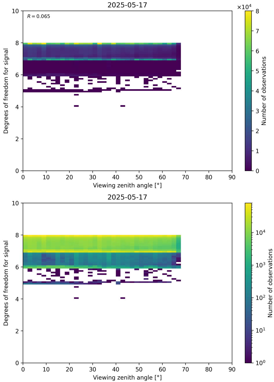
Figure 73: Scatter density plot of “Viewing zenith angle” against “Degrees of freedom for signal” for 2025-05-16 to 2025-05-18.
