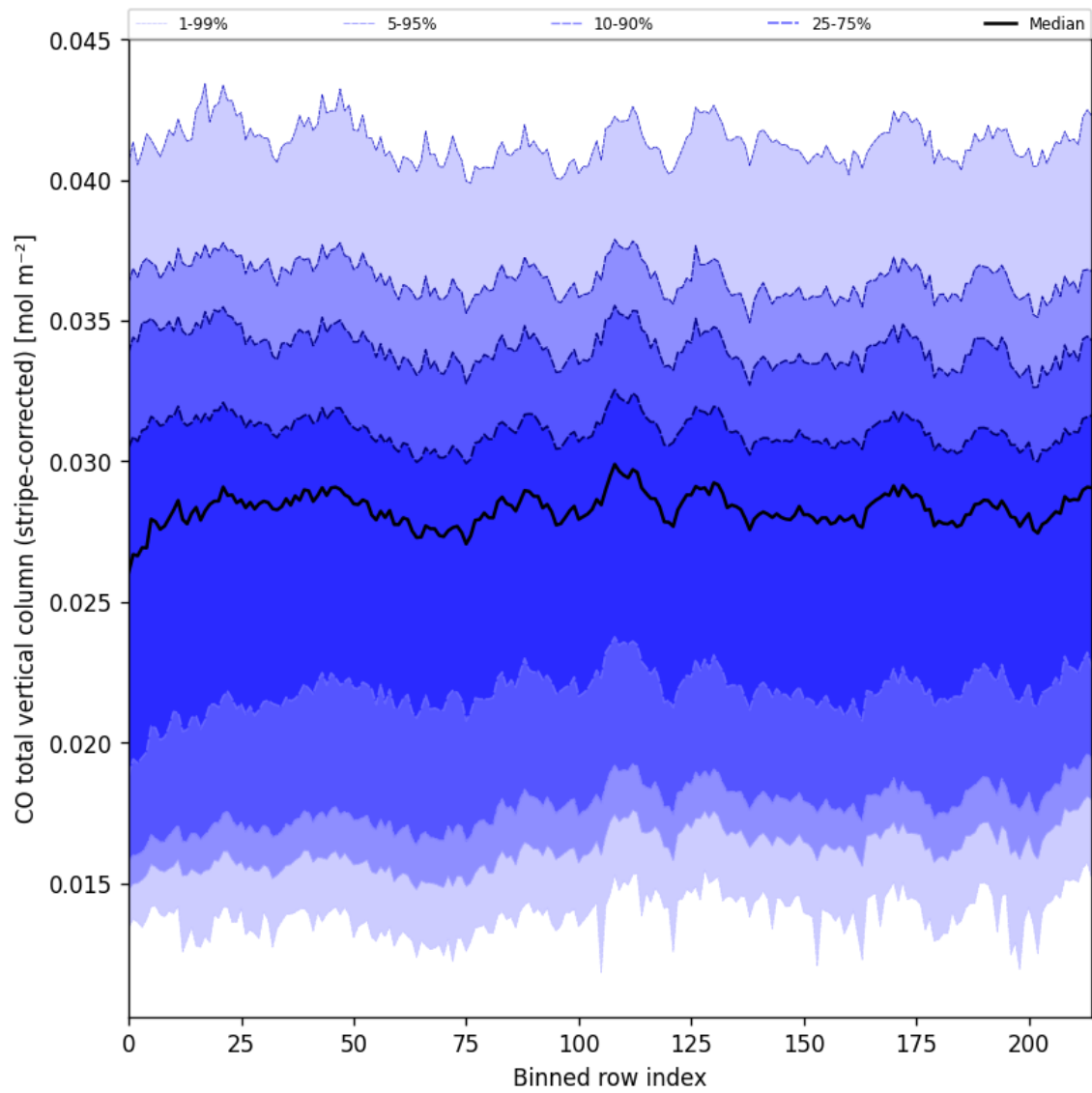
Figure 27: Along track statistics of “CO total vertical column (stripe-corrected)” for 2025-05-16 to 2025-05-18
