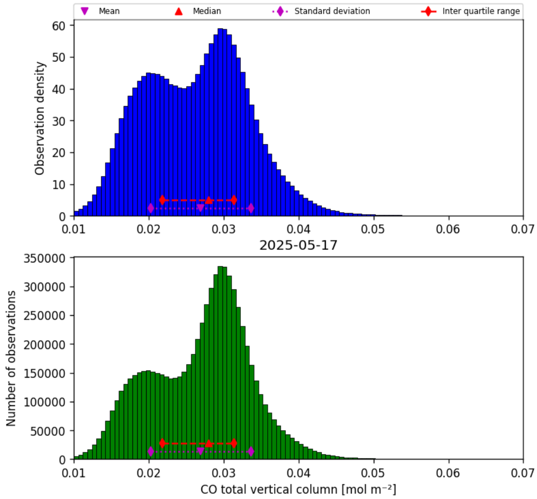
Figure 18: Histogram of “CO total vertical column” for 2025-05-16 to 2025-05-18
