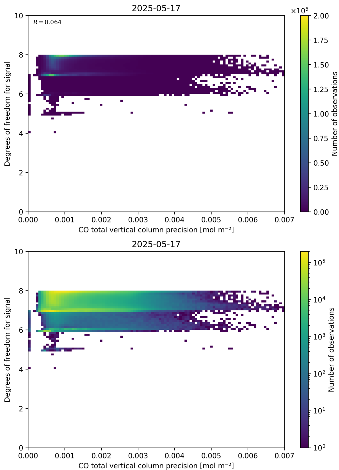
Figure 45: Scatter density plot of “CO total vertical column precision” against “Degrees of freedom for signal” for 2025-05-16 to 2025-05-18.
