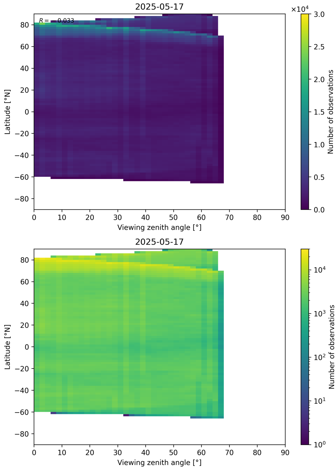
Figure 74: Scatter density plot of “Viewing zenith angle” against “Latitude” for 2025-05-16 to 2025-05-18.
