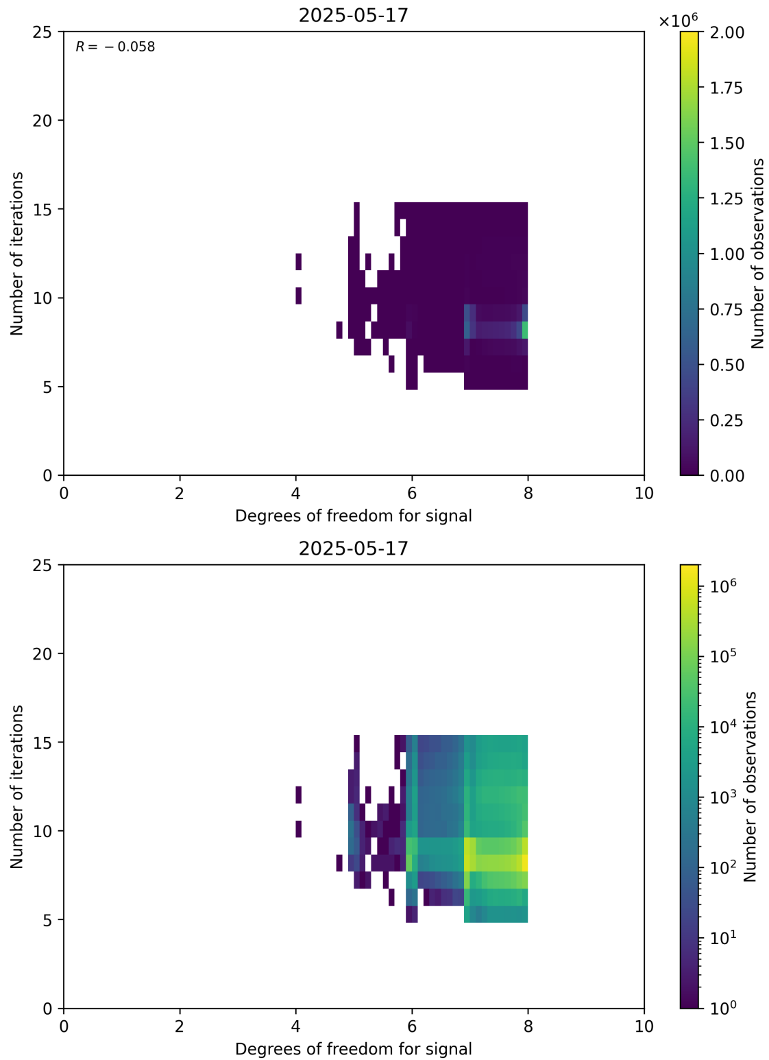
Figure 50: Scatter density plot of “Degrees of freedom for signal” against “Number of iterations” for 2025-05-16 to 2025-05-18.
