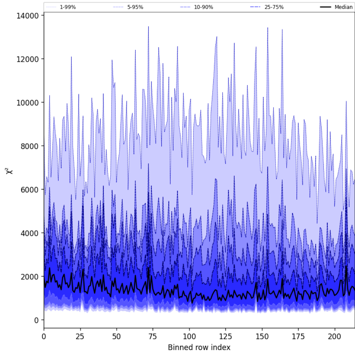
Figure 30: Along track statistics of “ \chi^2 ” for 2025-05-16 to 2025-05-18
