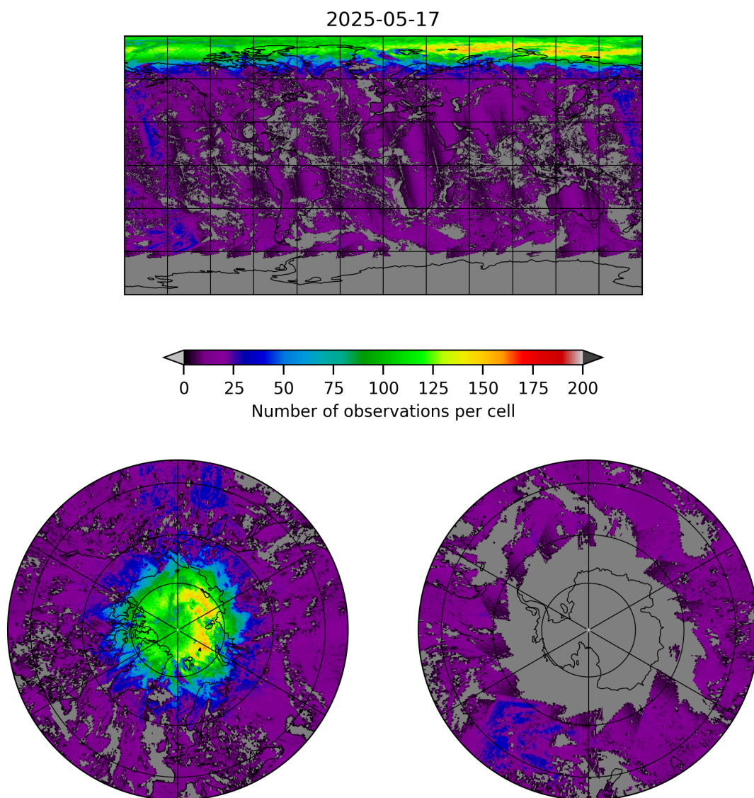
Figure 8: Map of the number of observations for 2025-05-16 to 2025-05-18
