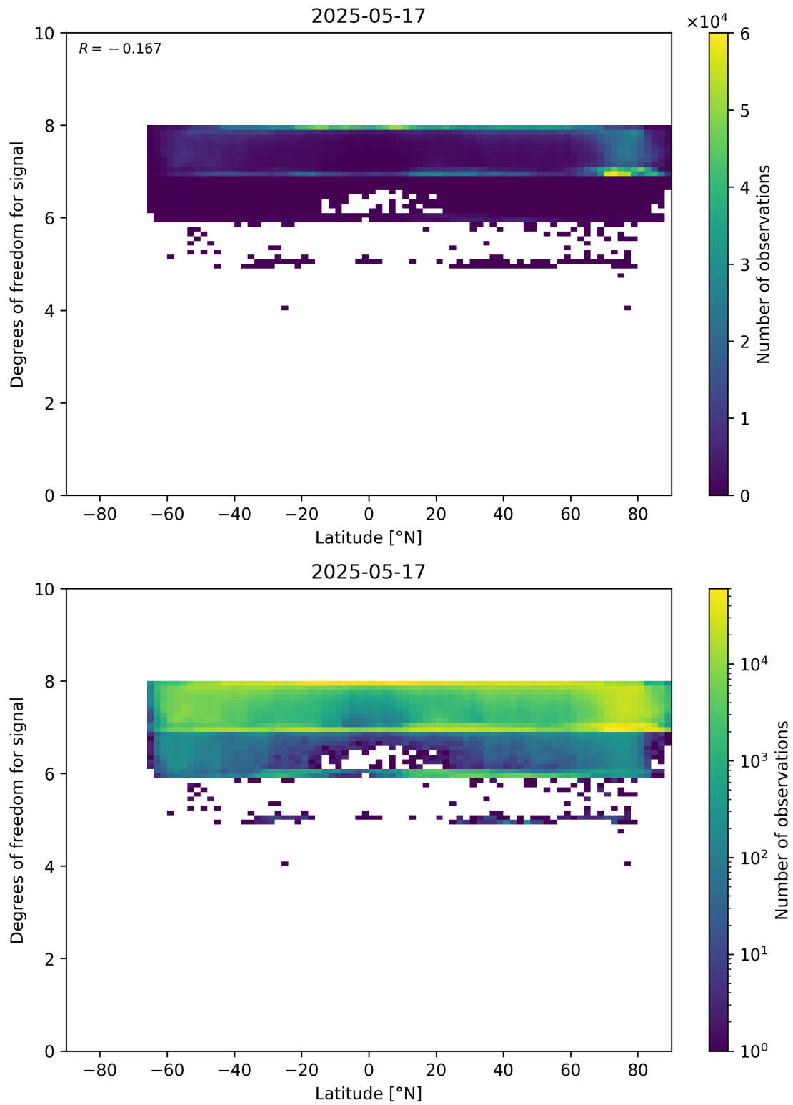
Figure 55: Scatter density plot of “Latitude” against “Degrees of freedom for signal” for 2025-05-16 to 2025-05-18.
