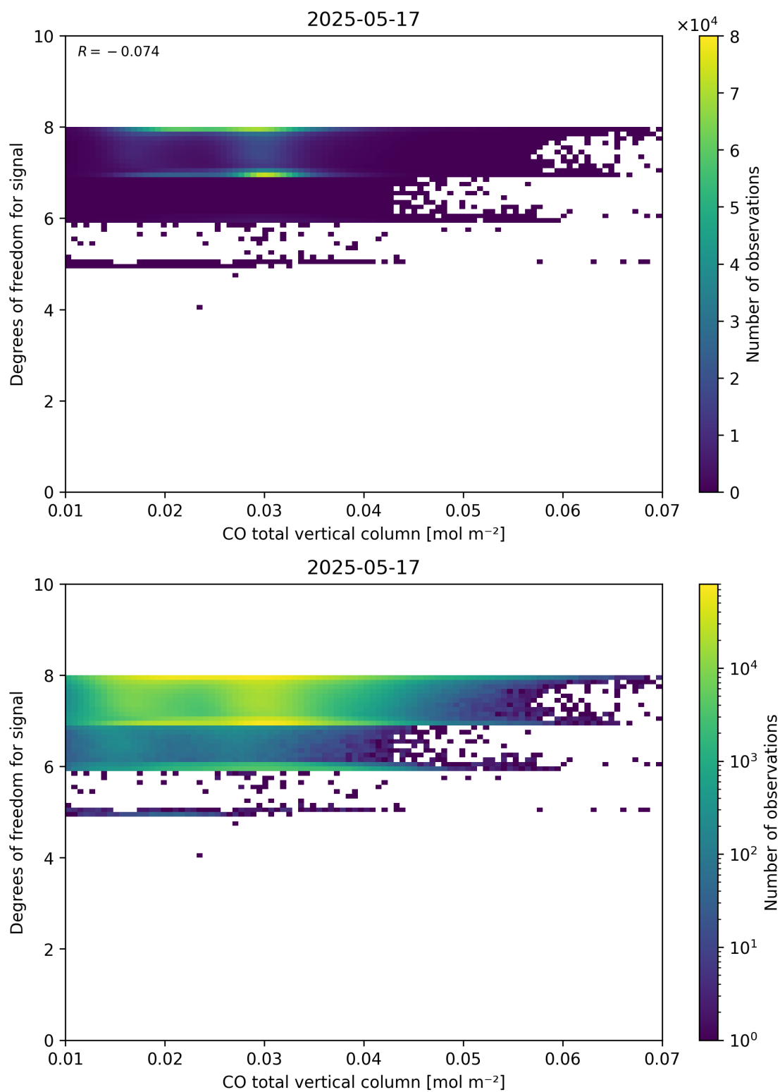
Figure 41: Scatter density plot of “CO total vertical column” against “Degrees of freedom for signal” for 2025-05-16 to 2025-05-18.
