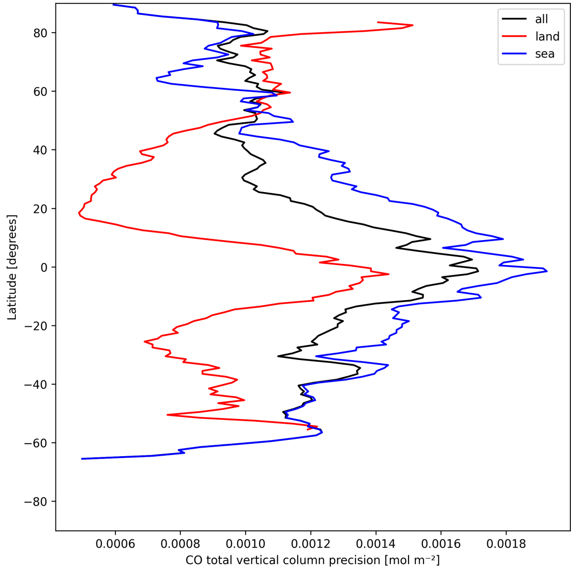
Figure 12: Zonal average of “CO total vertical column precision” for 2025-05-16 to 2025-05-18.
