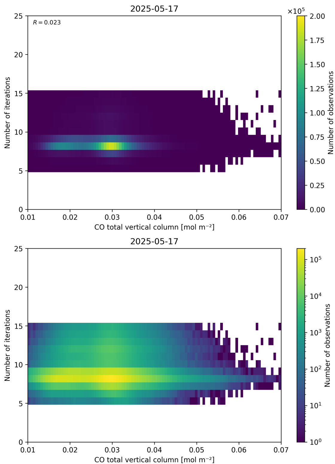
Figure 42: Scatter density plot of “CO total vertical column” against “Number of iterations” for 2025-05-16 to 2025-05-18.
