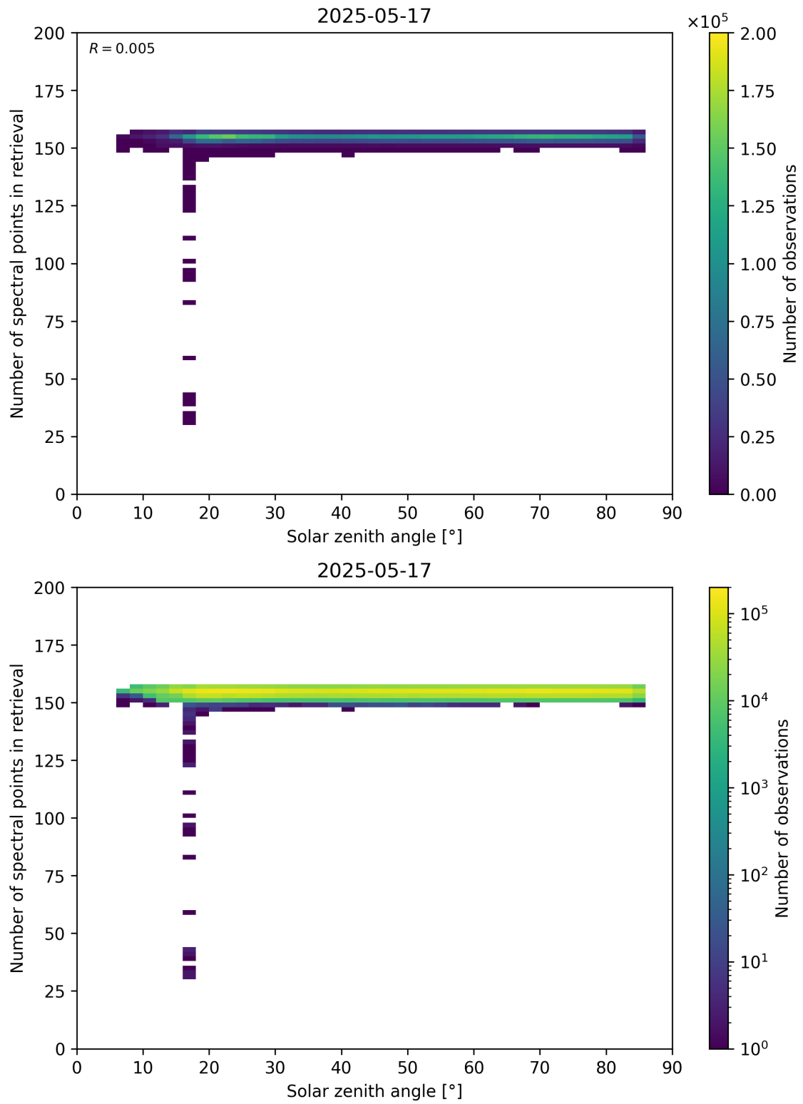
Figure 68: Scatter density plot of “Solar zenith angle” against “Number of spectral points in retrieval” for 2025-05-16 to 2025-05-18.
