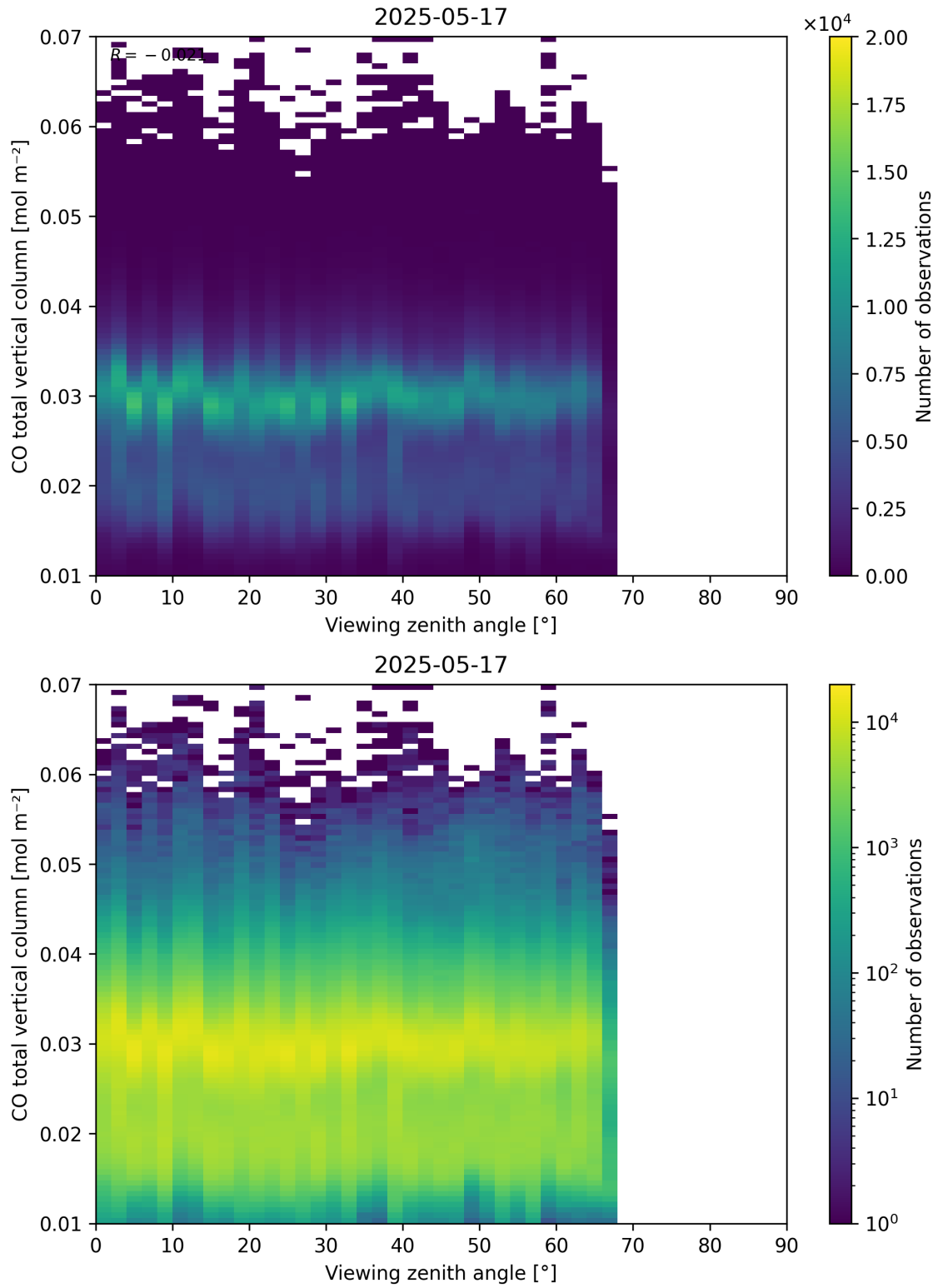
Figure 69: Scatter density plot of “Viewing zenith angle” against “CO total vertical column” for 2025-05-16 to 2025-05-18.
