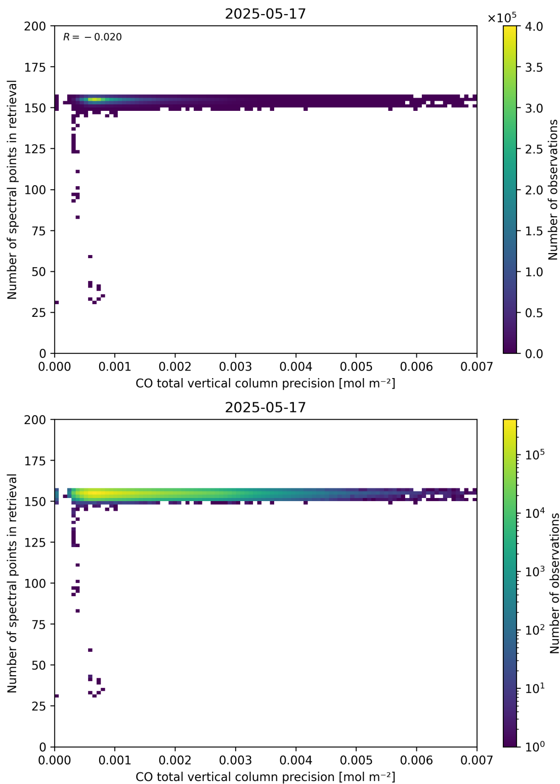
Figure 47: Scatter density plot of “CO total vertical column precision” against “Number of spectral points in retrieval” for 2025-05-16 to 2025-05-18.
