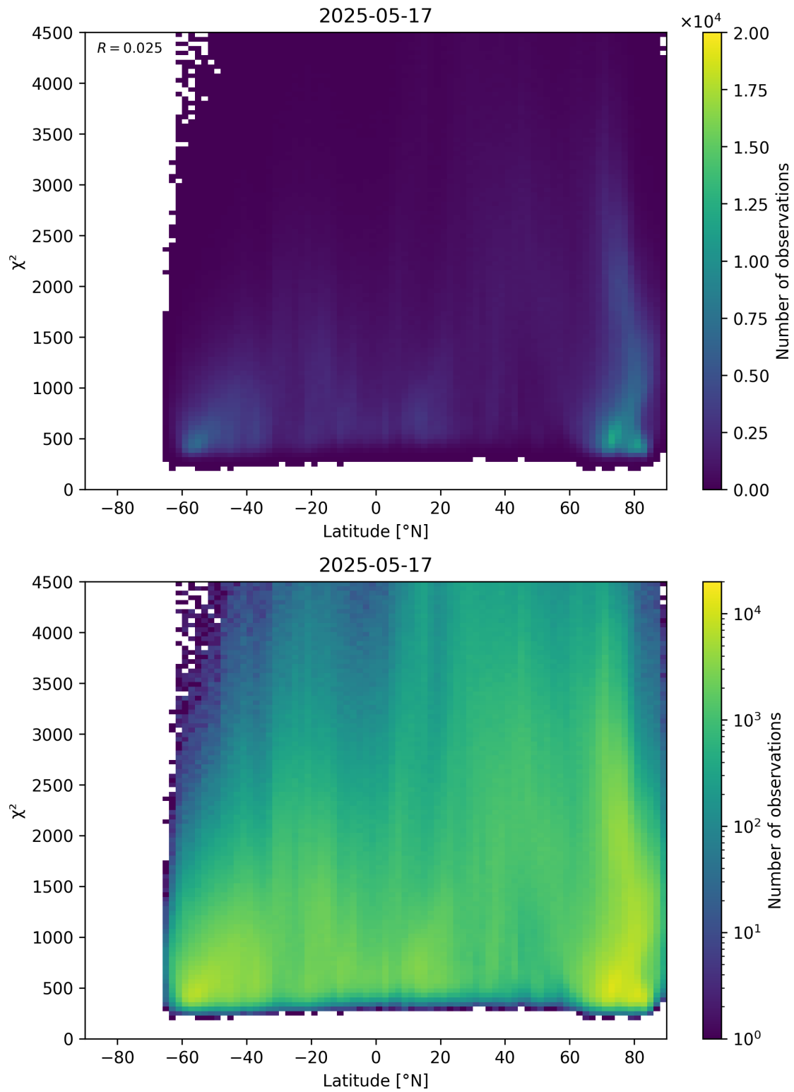
Figure 54: Scatter density plot of “Latitude” against “ \chi^2 ” for 2025-05-16 to 2025-05-18.
