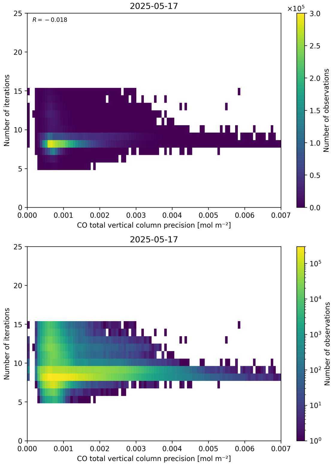
Figure 46: Scatter density plot of “CO total vertical column precision” against “Number of iterations” for 2025-05-16 to 2025-05-18.
