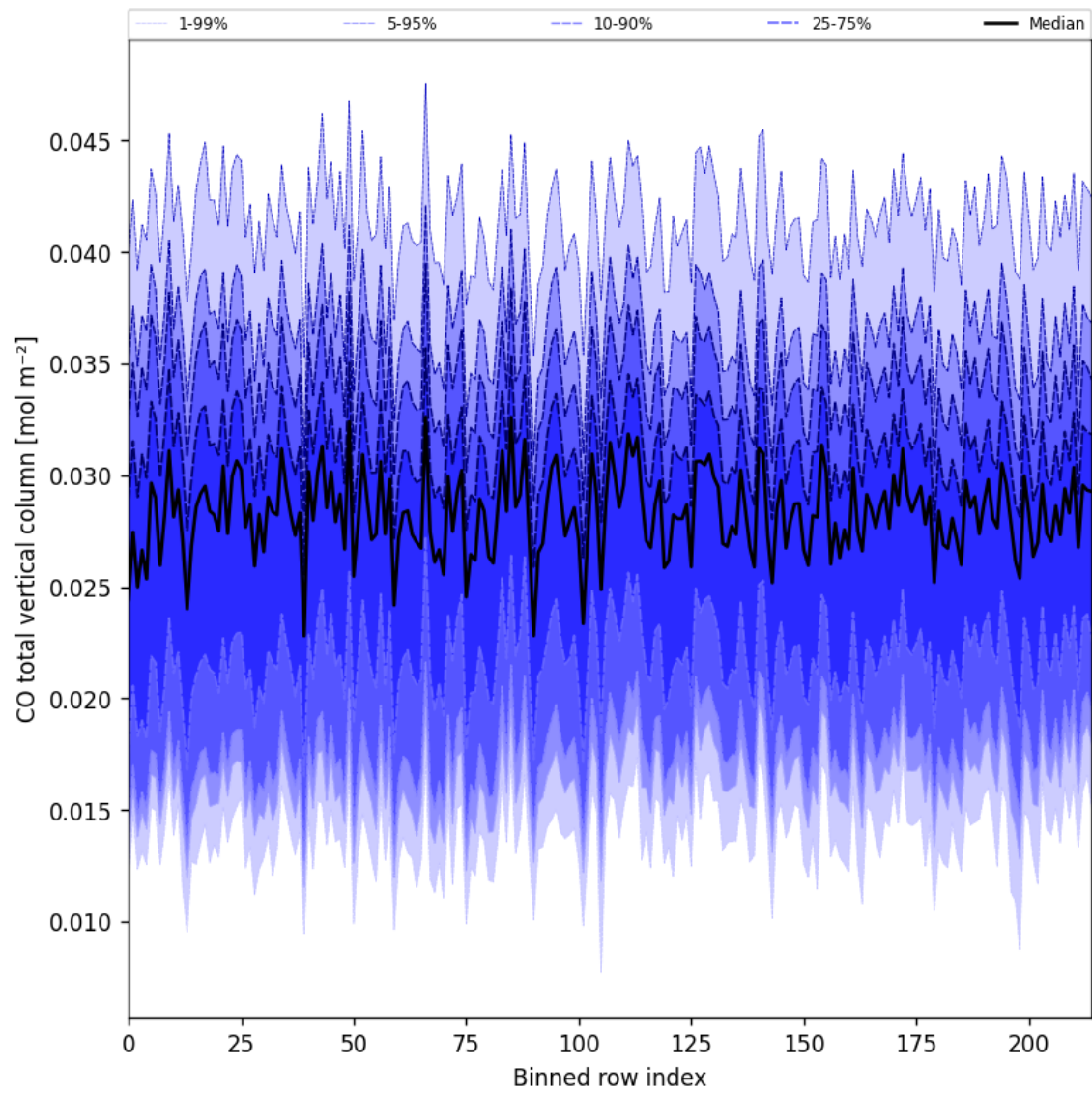
Figure 26: Along track statistics of “CO total vertical column” for 2025-05-16 to 2025-05-18
