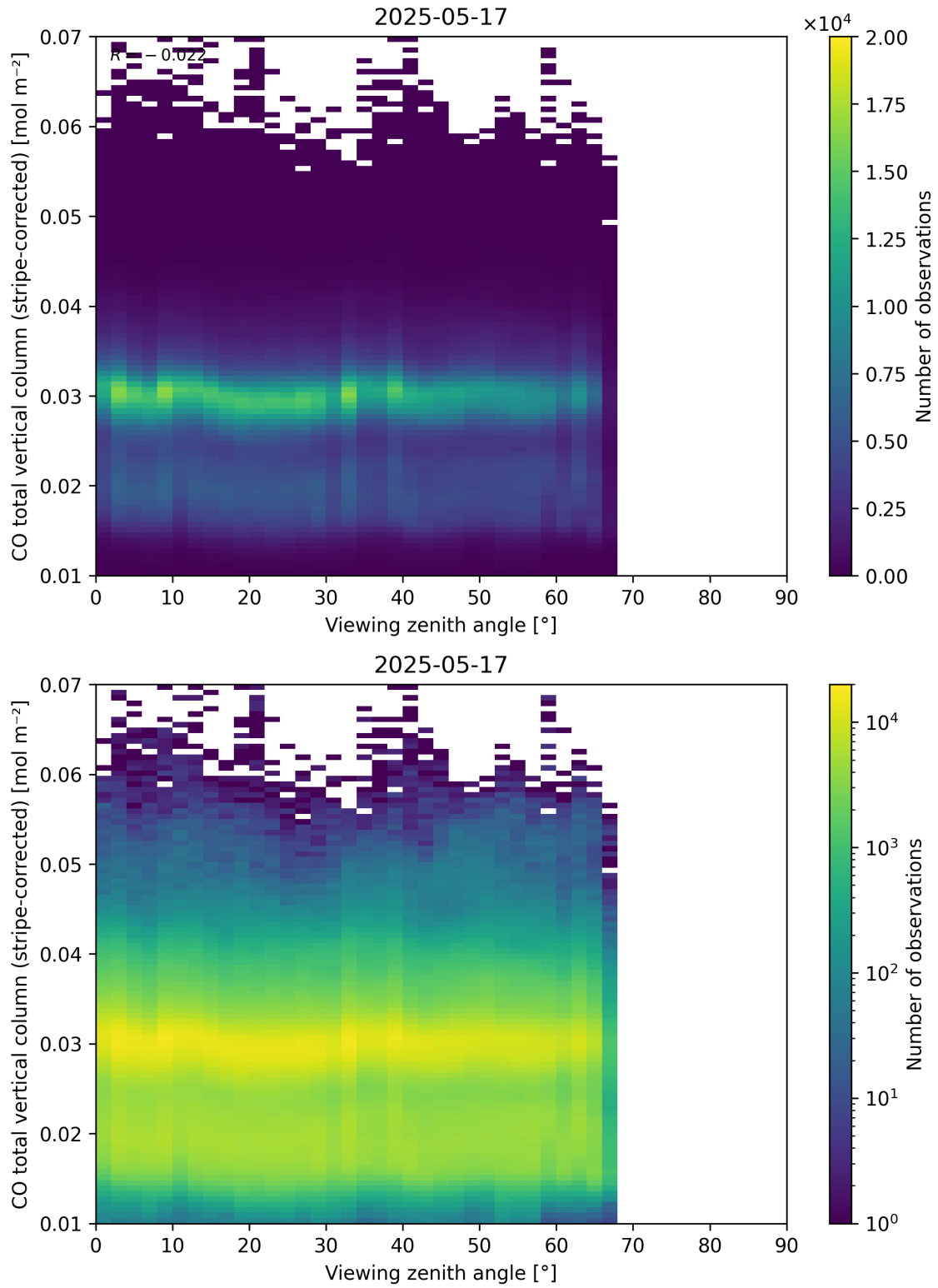
Figure 70: Scatter density plot of “Viewing zenith angle” against “CO total vertical column (stripe-corrected)” for 2025-05-16 to 2025-05-18.
