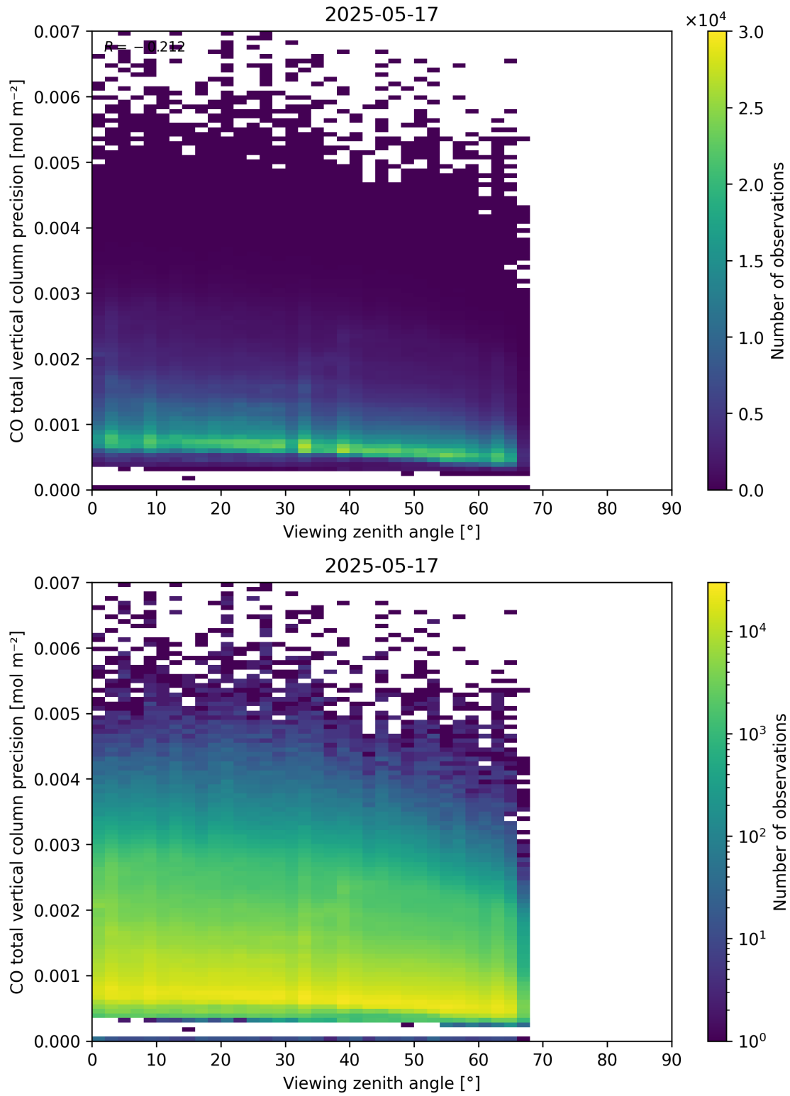
Figure 71: Scatter density plot of “Viewing zenith angle” against “CO total vertical column precision” for 2025-05-16 to 2025-05-18.
