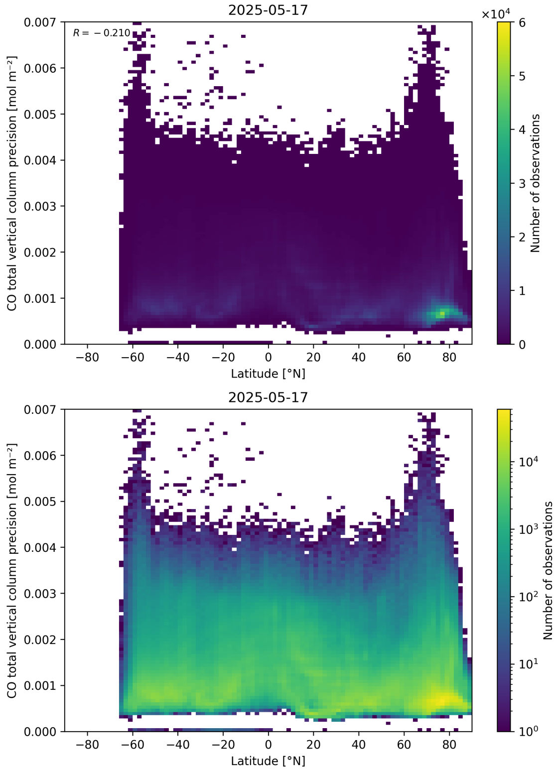
Figure 53: Scatter density plot of “Latitude” against “CO total vertical column precision” for 2025-05-16 to 2025-05-18.
