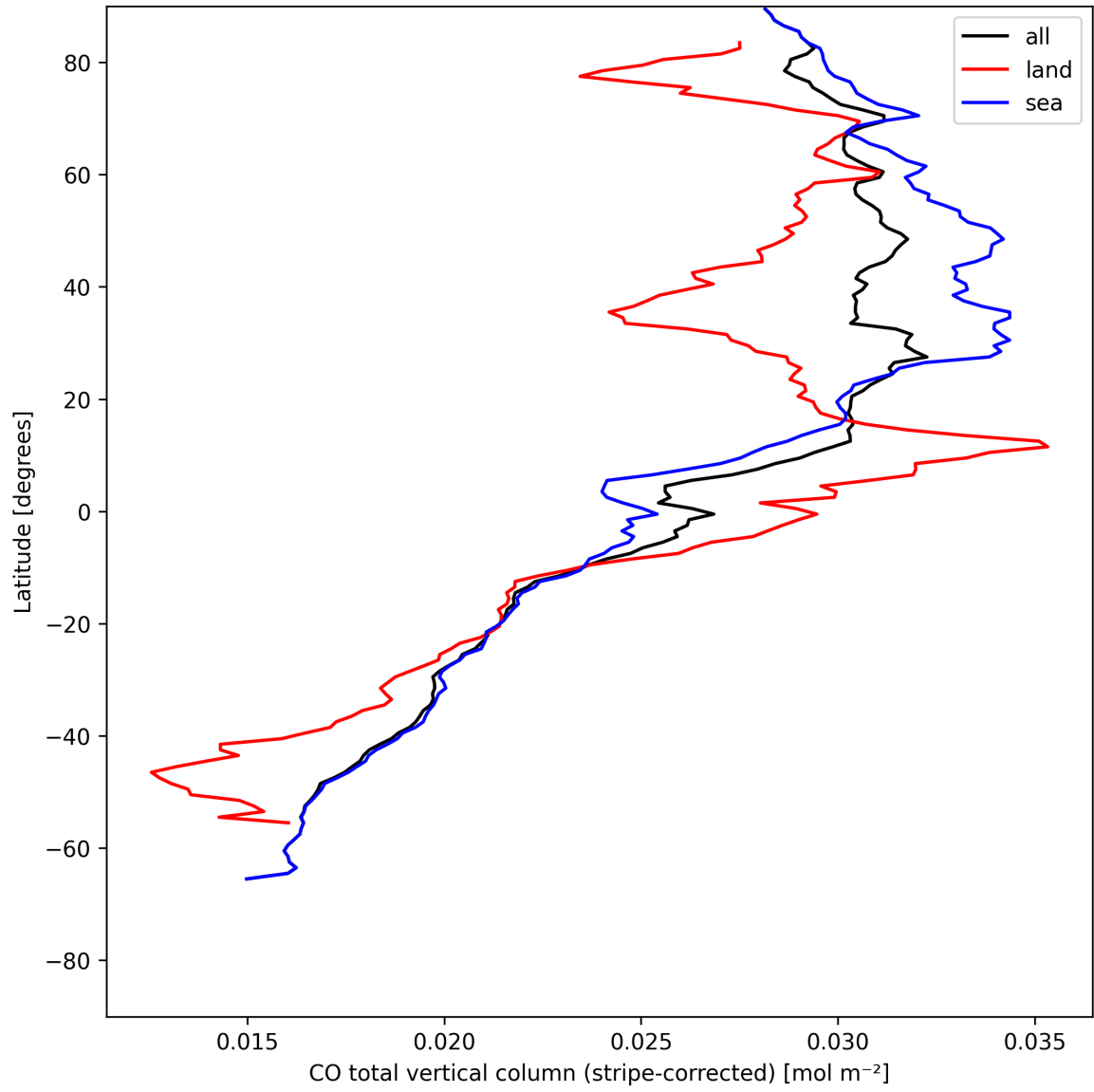
Figure 11: Zonal average of “CO total vertical column (stripe-corrected)” for 2025-05-16 to 2025-05-18.
