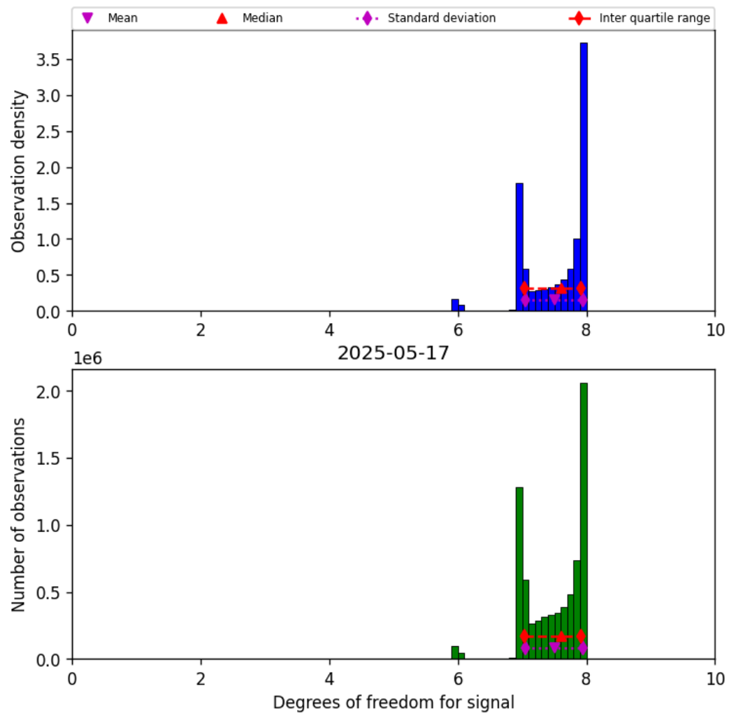
Figure 23: Histogram of “Degrees of freedom for signal” for 2025-05-16 to 2025-05-18
