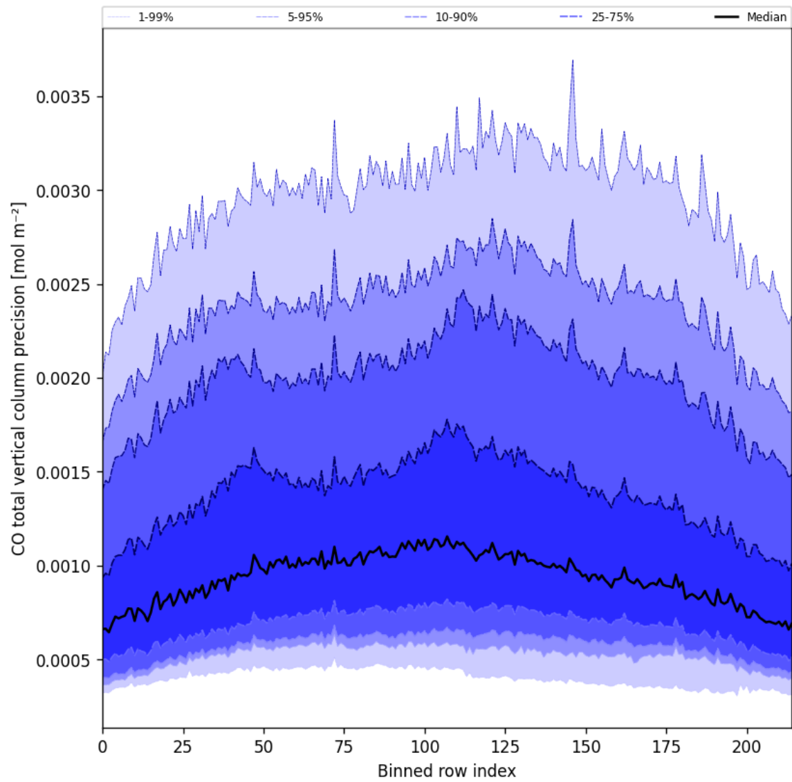
Figure 28: Along track statistics of “CO total vertical column precision” for 2025-05-16 to 2025-05-18
