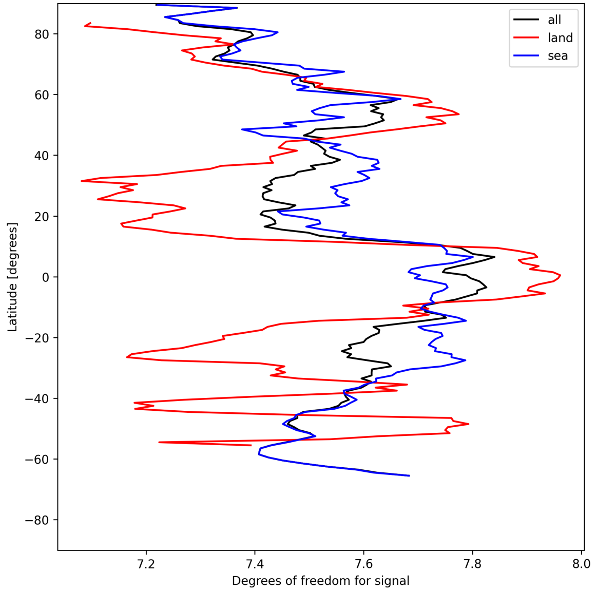
Figure 15: Zonal average of “Degrees of freedom for signal” for 2025-05-16 to 2025-05-18.
