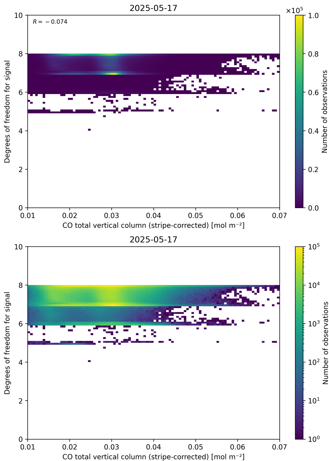
Figure 38: Scatter density plot of “CO total vertical column (stripe-corrected)” against “Degrees of freedom for signal” for 2025-05-16 to 2025-05-18.
