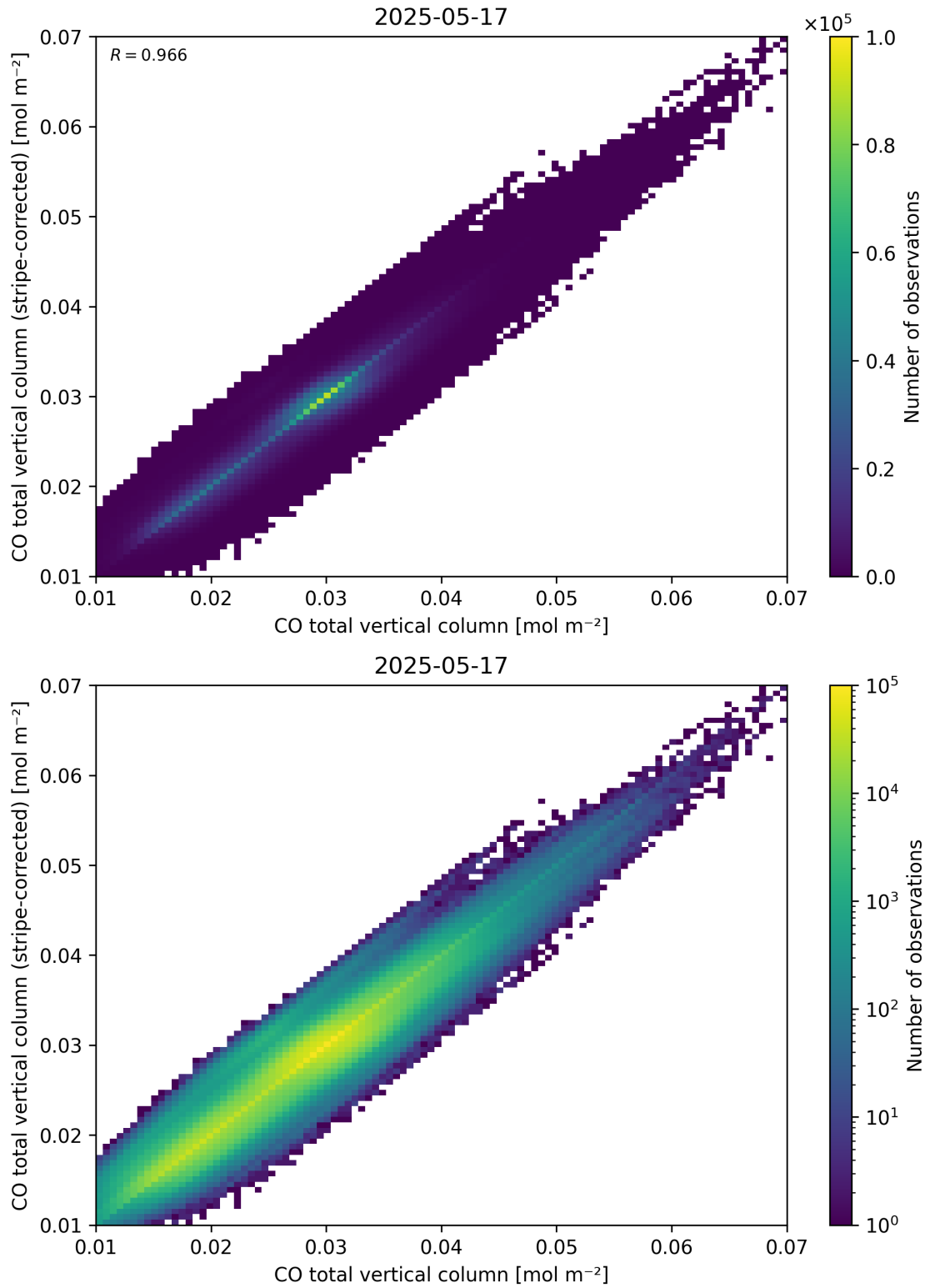
Figure 33: Scatter density plot of “CO total vertical column” against “CO total vertical column (stripe-corrected)” for 2025-05-16 to 2025-05-18.
