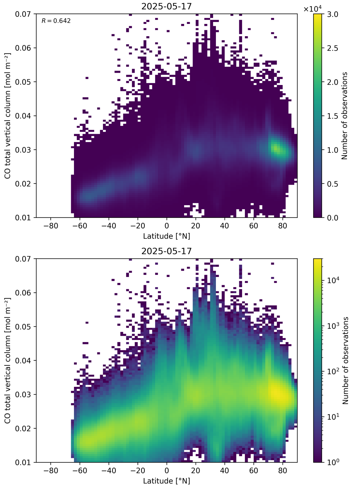
Figure 51: Scatter density plot of “Latitude” against “CO total vertical column” for 2025-05-16 to 2025-05-18.
