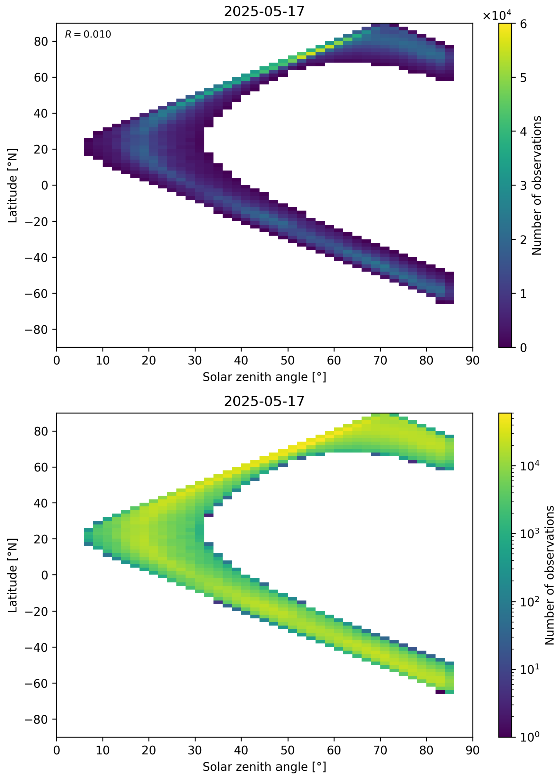
Figure 66: Scatter density plot of “Solar zenith angle” against “Latitude” for 2025-05-16 to 2025-05-18.
