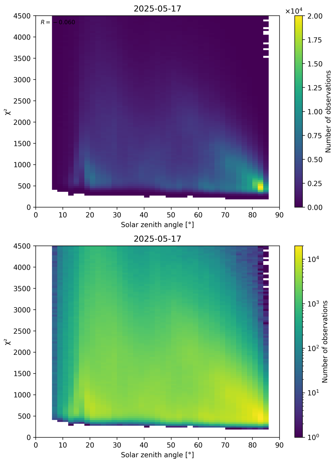
Figure 64: Scatter density plot of “Solar zenith angle” against “ \chi^2 ” for 2025-05-16 to 2025-05-18.
