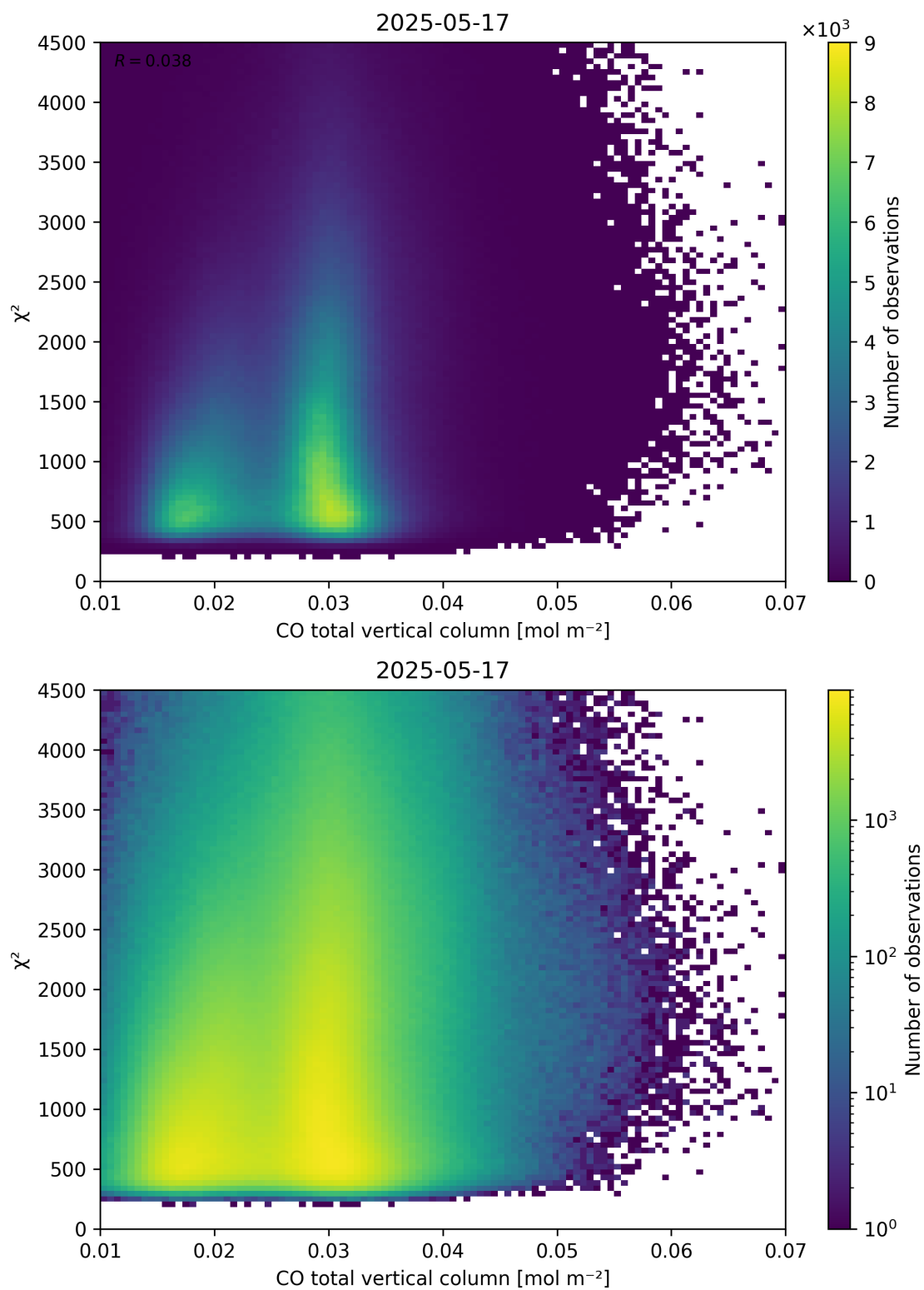
Figure 35: Scatter density plot of “CO total vertical column” against “ \chi^2 ” for 2025-05-16 to 2025-05-18.
