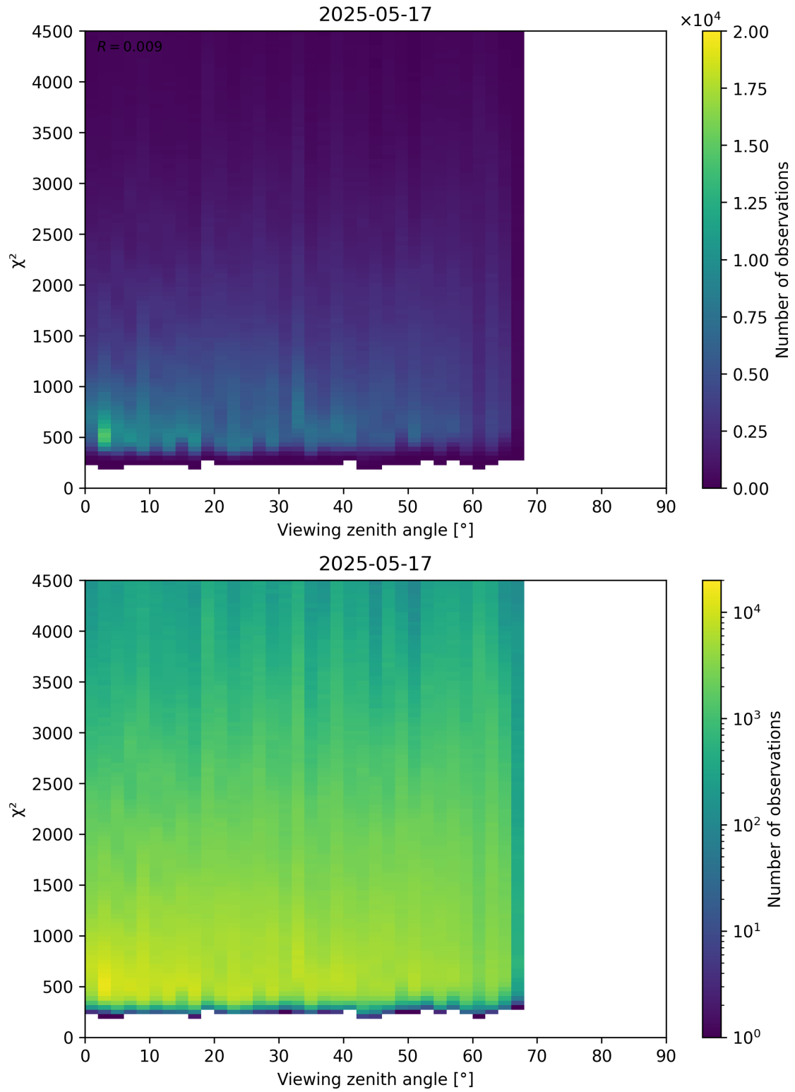
Figure 72: Scatter density plot of “Viewing zenith angle” against “ \chi^2 ” for 2025-05-16 to 2025-05-18.
