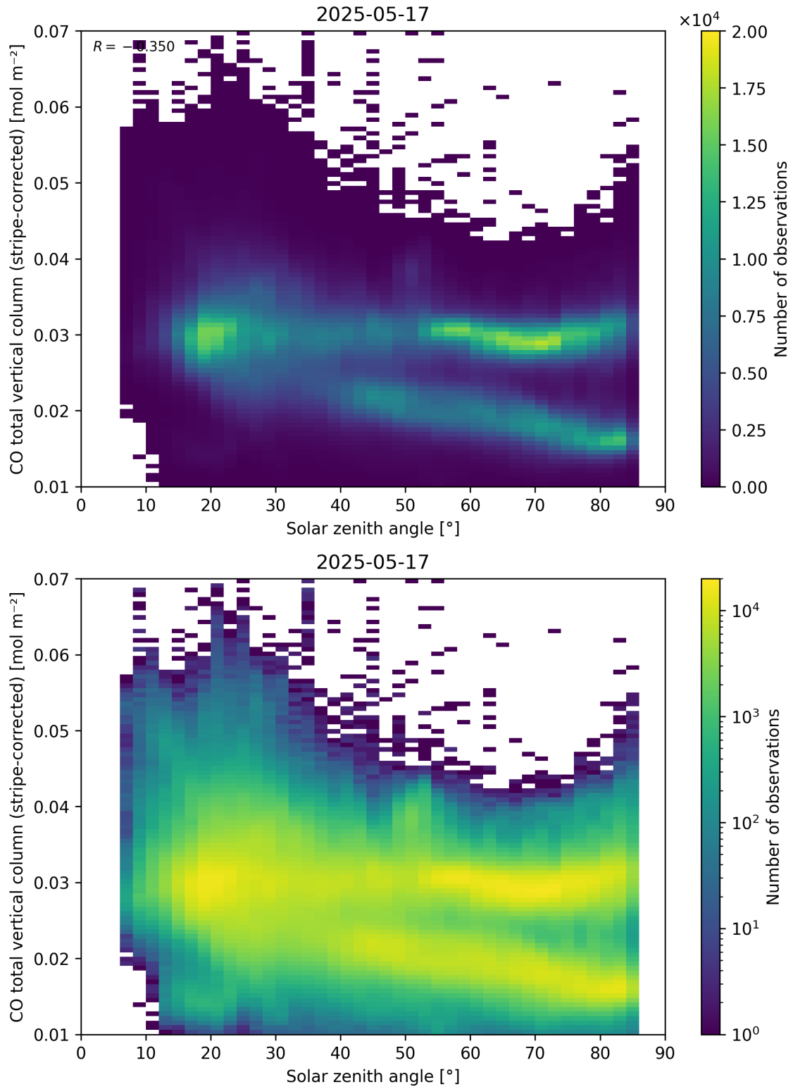
Figure 62: Scatter density plot of “Solar zenith angle” against “CO total vertical column (stripe-corrected)” for 2025-05-16 to 2025-05-18.
