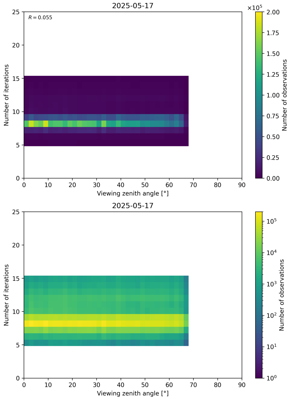
Figure 75: Scatter density plot of “Viewing zenith angle” against “Number of iterations” for 2025-05-16 to 2025-05-18.
