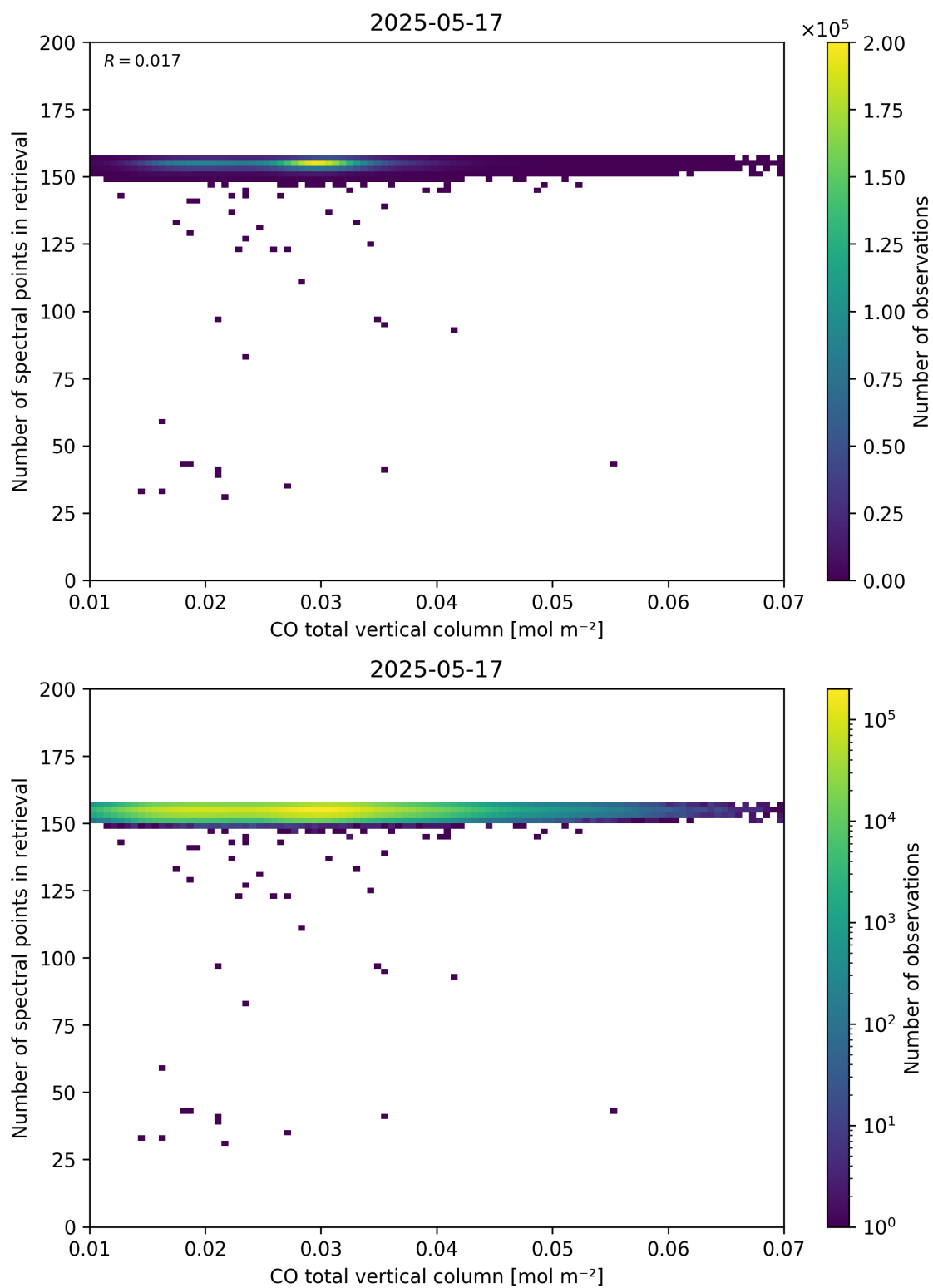
Figure 43: Scatter density plot of “CO total vertical column” against “Number of spectral points in retrieval” for 2025-05-16 to 2025-05-18.
