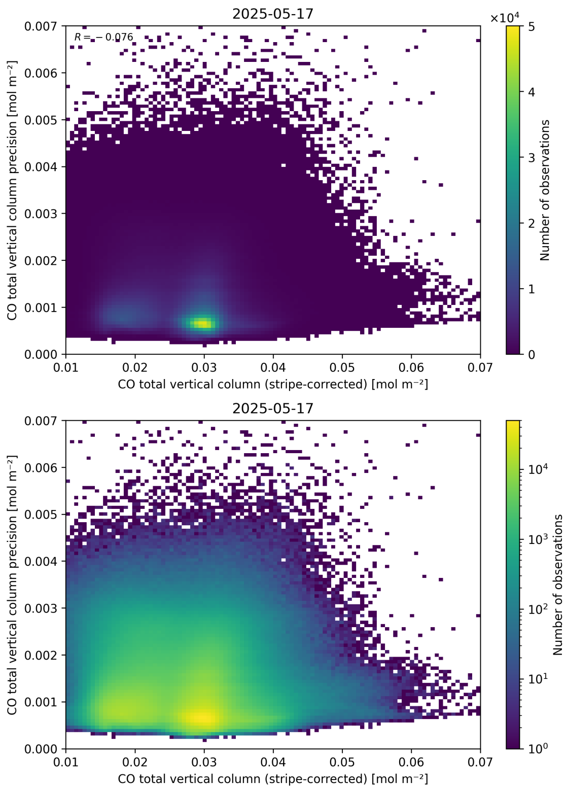
Figure 36: Scatter density plot of “CO total vertical column (stripe-corrected)” against “CO total vertical column precision” for 2025-05-16 to 2025-05-18.
