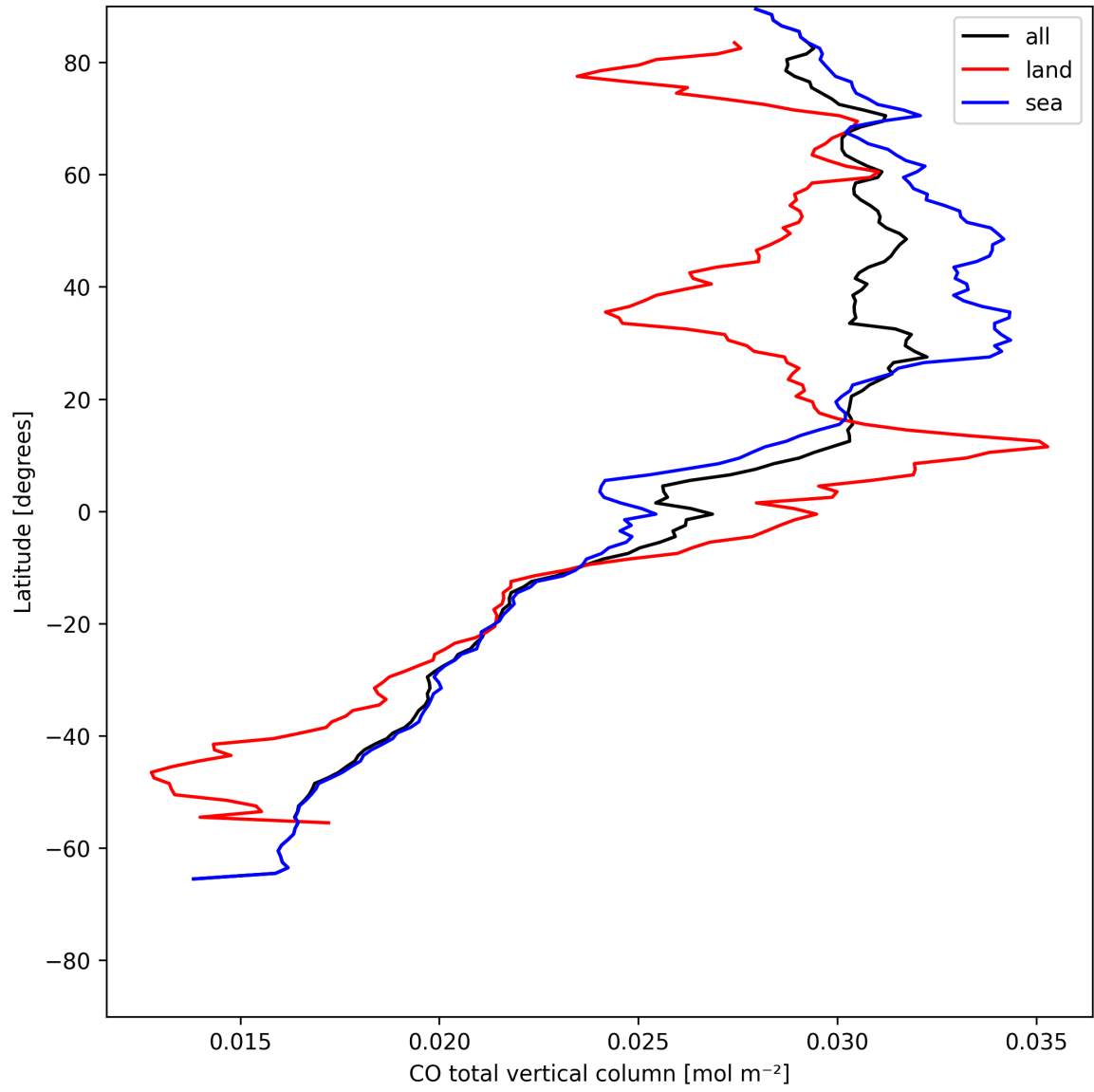
Figure 10: Zonal average of “CO total vertical column” for 2025-05-16 to 2025-05-18.
