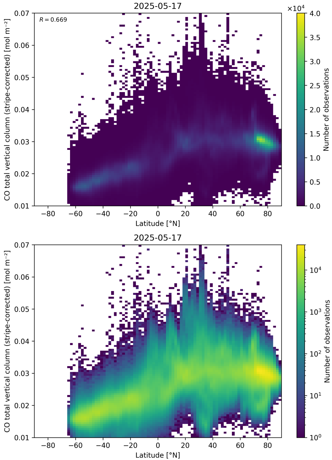
Figure 52: Scatter density plot of “Latitude” against “CO total vertical column (stripe-corrected)” for 2025-05-16 to 2025-05-18.
