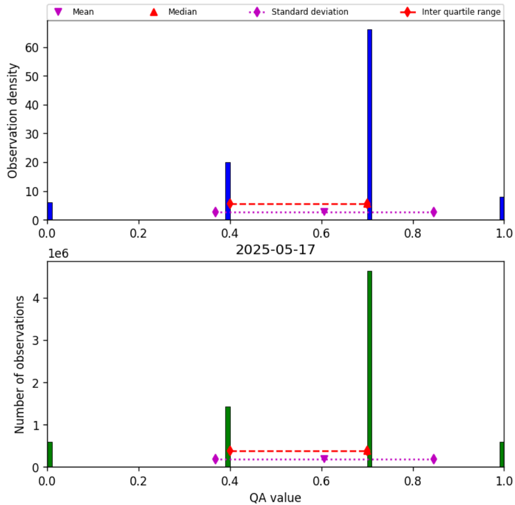
Figure 17: Histogram of “QA value” for 2025-05-16 to 2025-05-18
