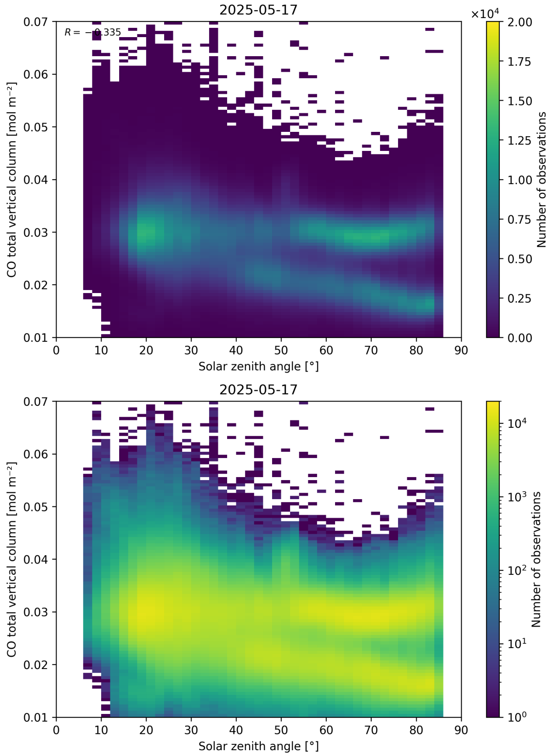
Figure 61: Scatter density plot of “Solar zenith angle” against “CO total vertical column” for 2025-05-16 to 2025-05-18.
