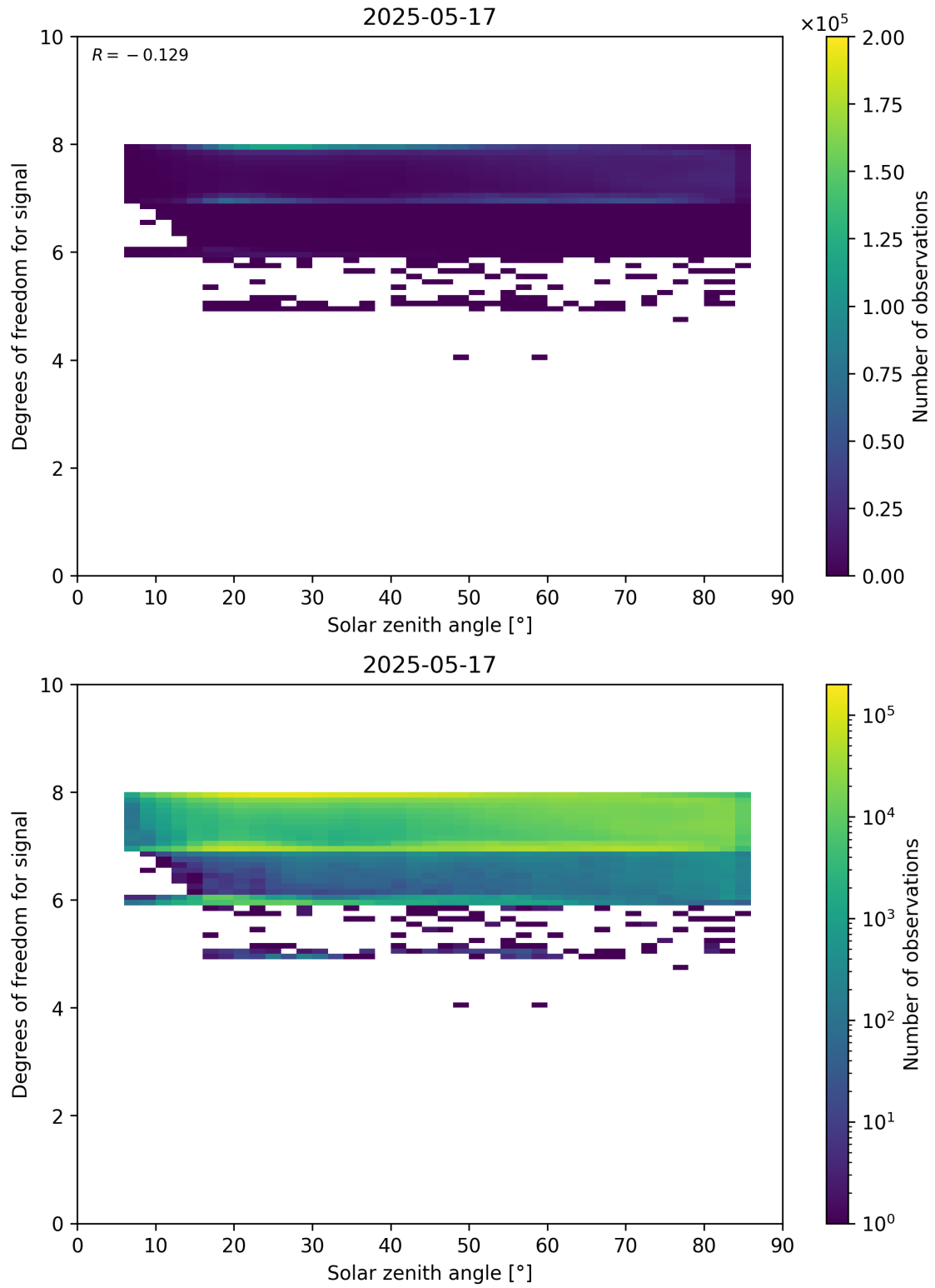
Figure 65: Scatter density plot of “Solar zenith angle” against “Degrees of freedom for signal” for 2025-05-16 to 2025-05-18.
