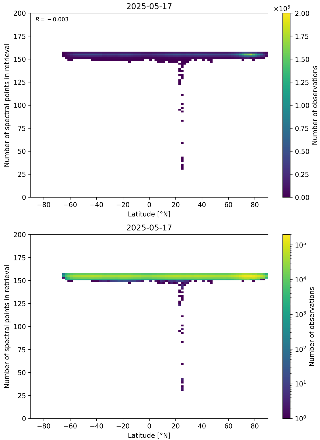
Figure 57: Scatter density plot of “Latitude” against “Number of spectral points in retrieval” for 2025-05-16 to 2025-05-18.
