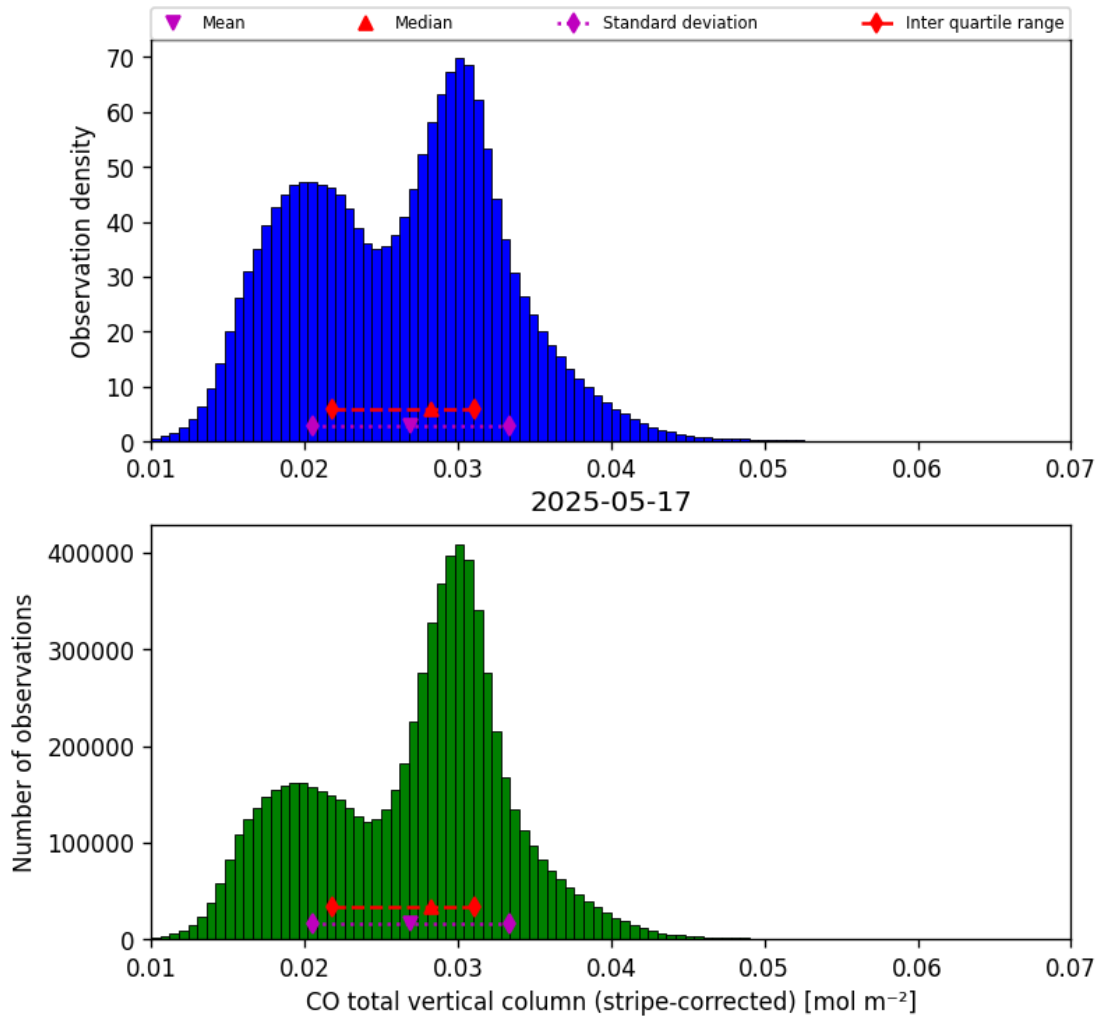
Figure 19: Histogram of “CO total vertical column (stripe-corrected)” for 2025-05-16 to 2025-05-18
