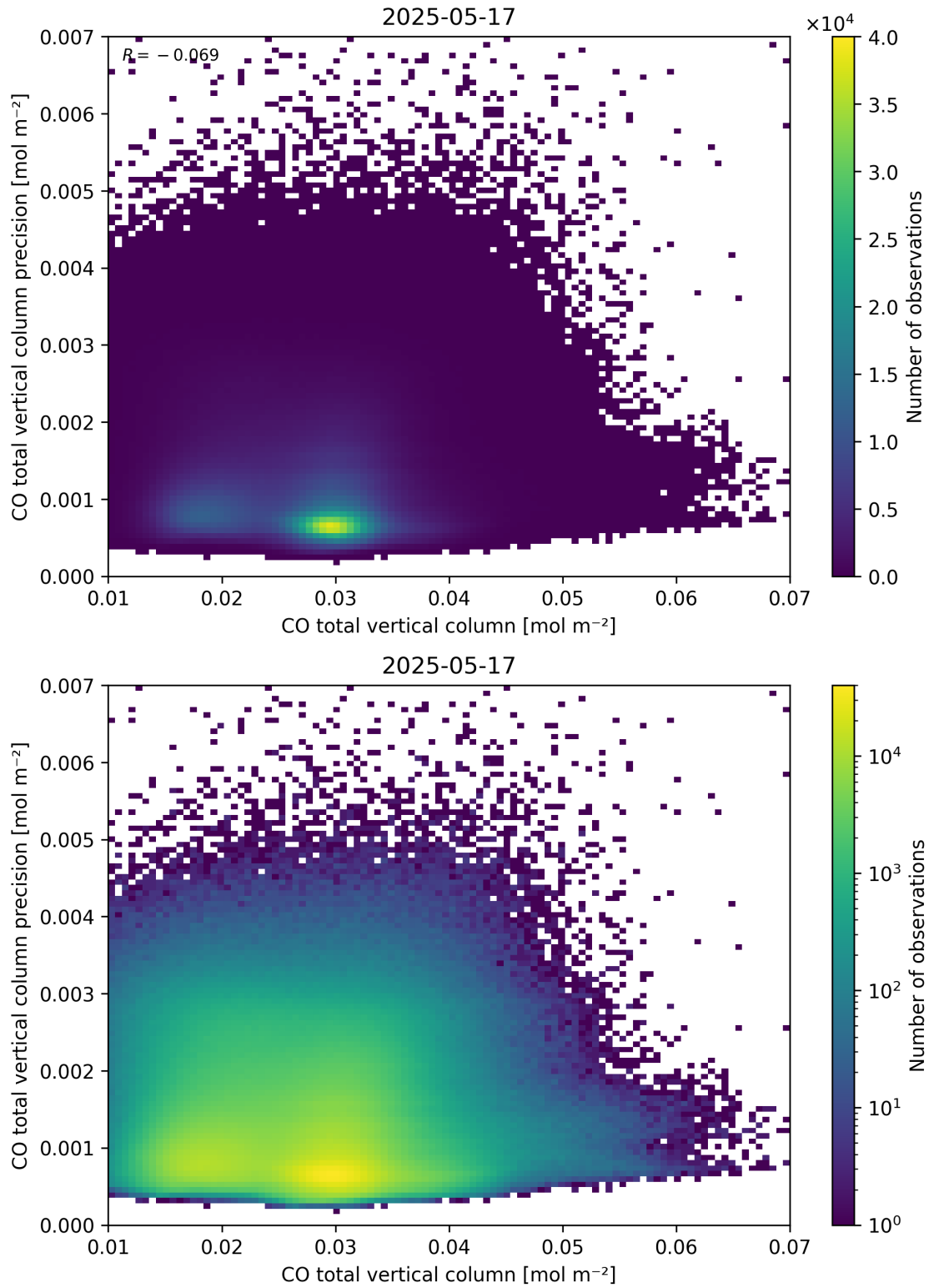
Figure 34: Scatter density plot of “CO total vertical column” against “CO total vertical column precision” for 2025-05-16 to 2025-05-18.
