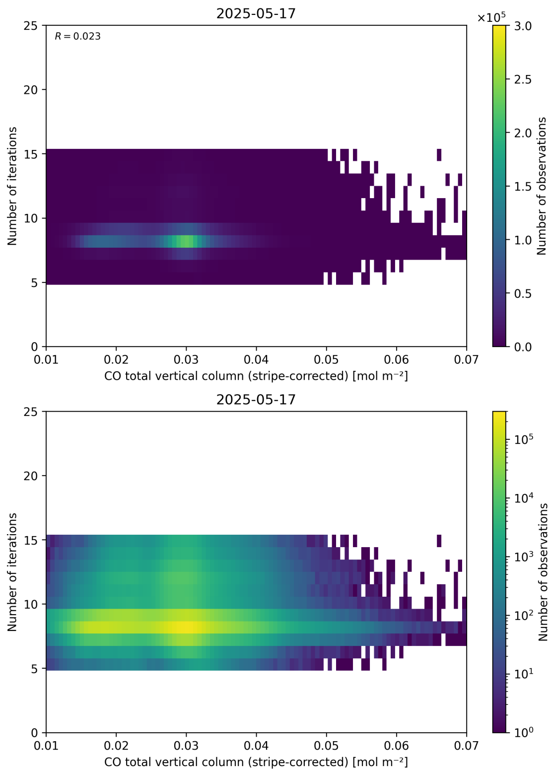
Figure 39: Scatter density plot of “CO total vertical column (stripe-corrected)” against “Number of iterations” for 2025-05-16 to 2025-05-18.
