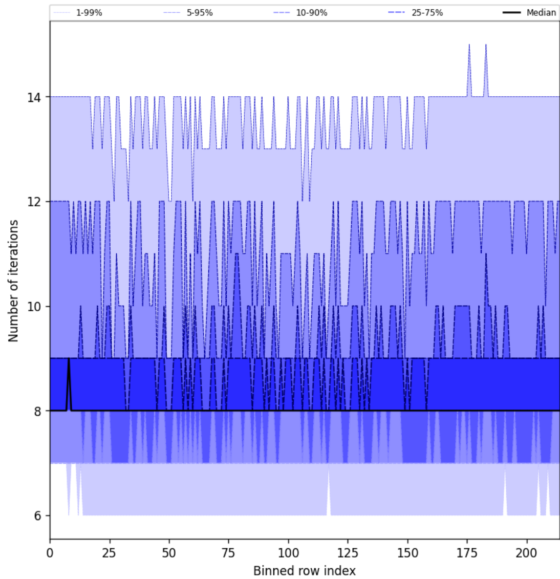
Figure 32: Along track statistics of “Number of iterations” for 2025-05-16 to 2025-05-18
