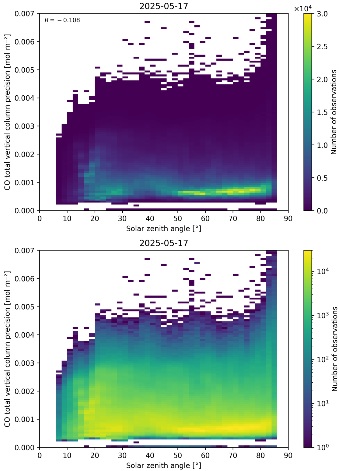
Figure 63: Scatter density plot of “Solar zenith angle” against “CO total vertical column precision” for 2025-05-16 to 2025-05-18.
