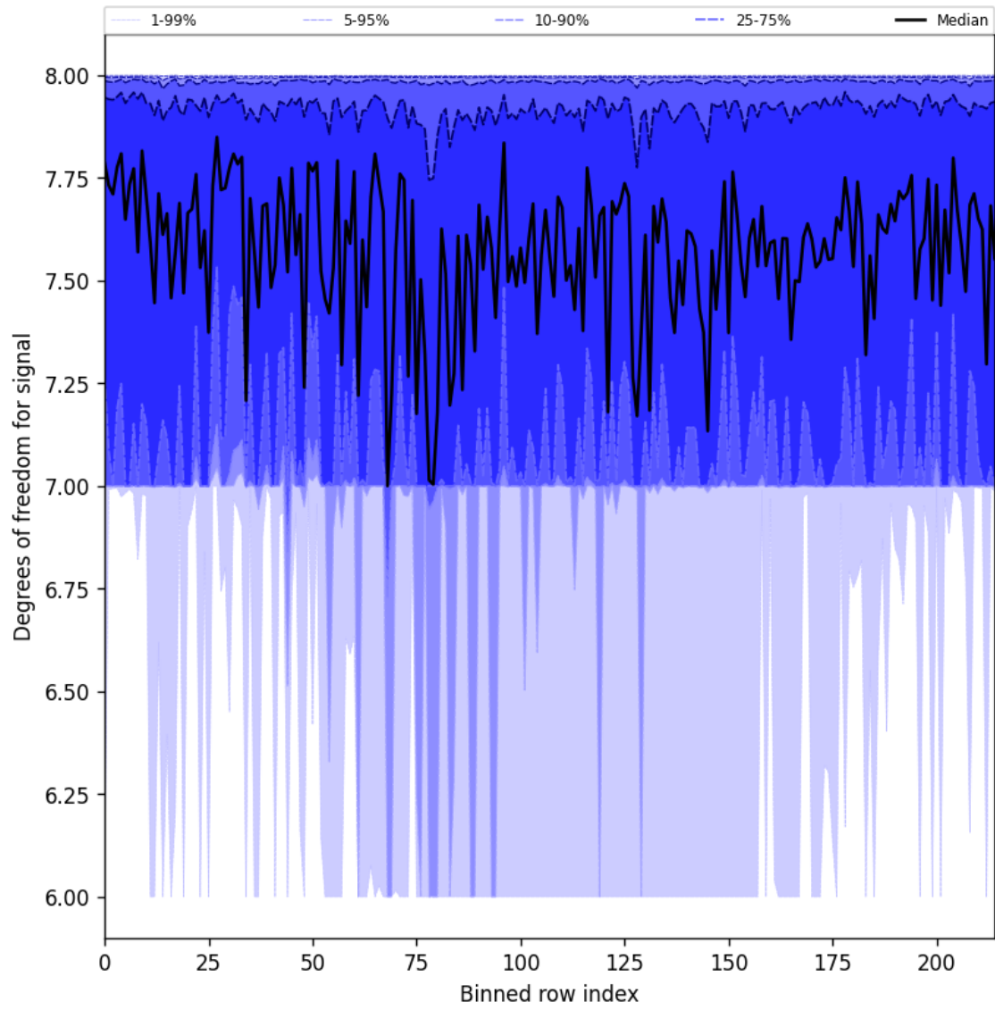
Figure 31: Along track statistics of “Degrees of freedom for signal” for 2025-05-16 to 2025-05-18
