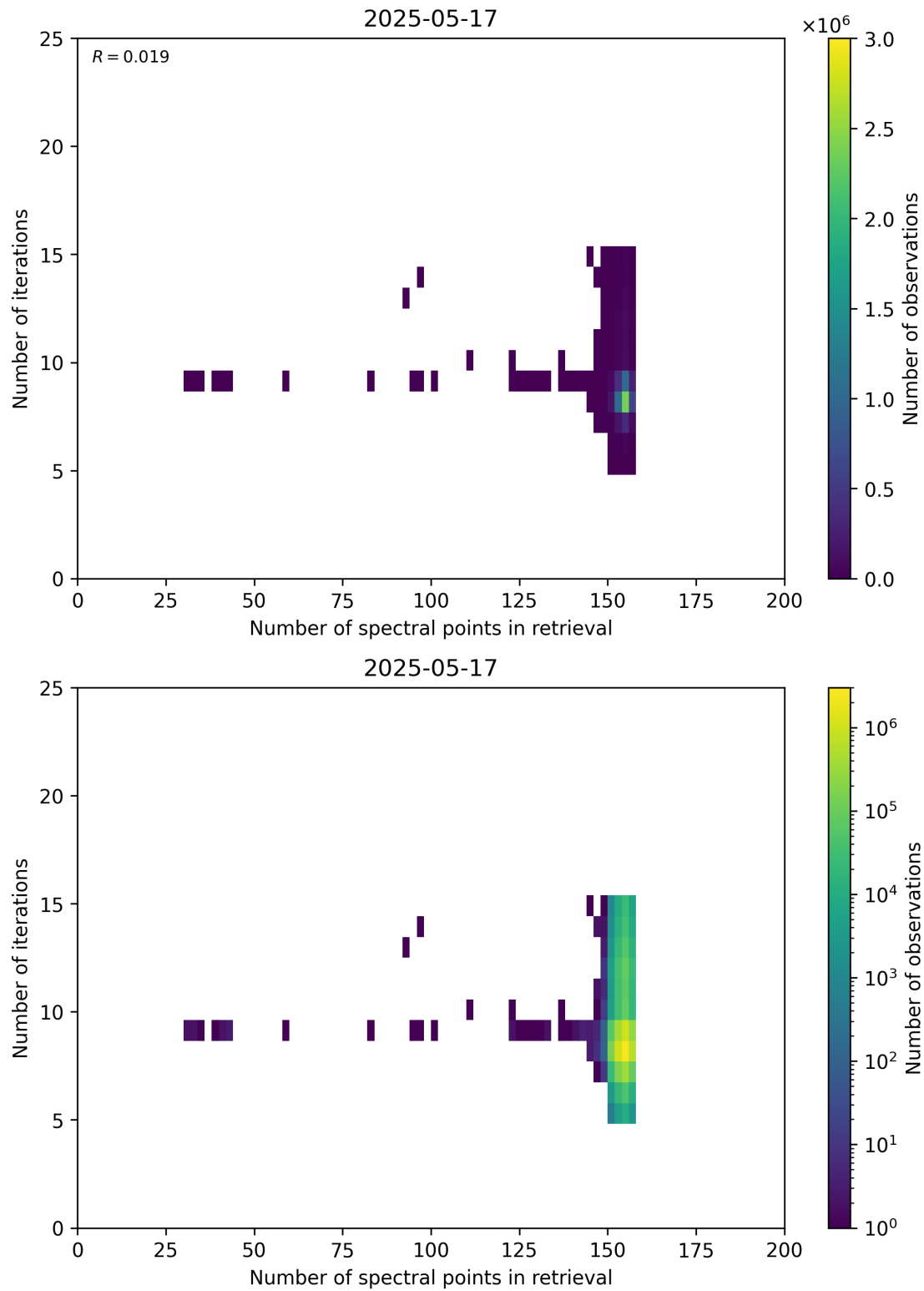
Figure 60: Scatter density plot of “Number of spectral points in retrieval” against “Number of iterations” for 2025-05-16 to 2025-05-18.
