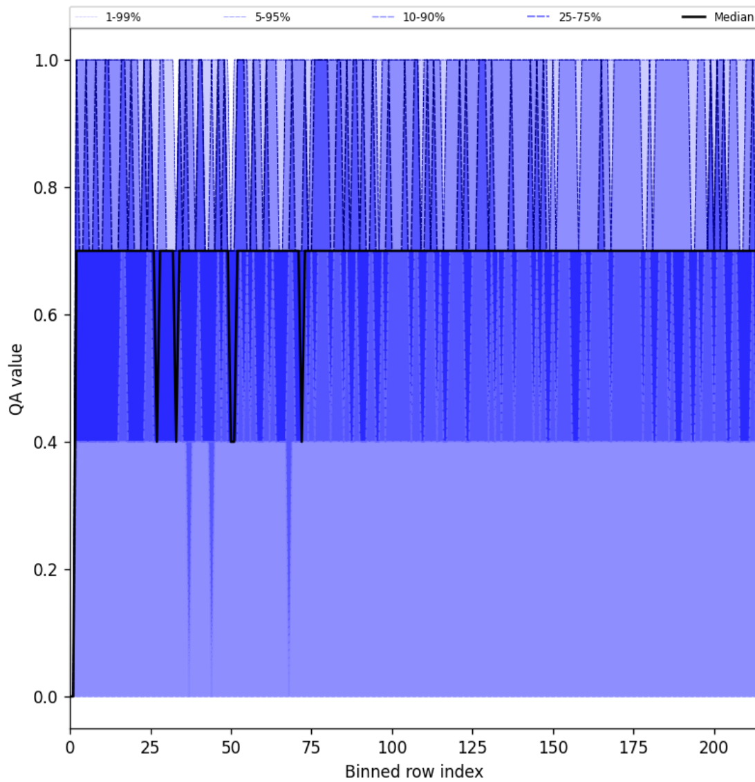
Figure 25: Along track statistics of “QA value” for 2025-05-16 to 2025-05-18
