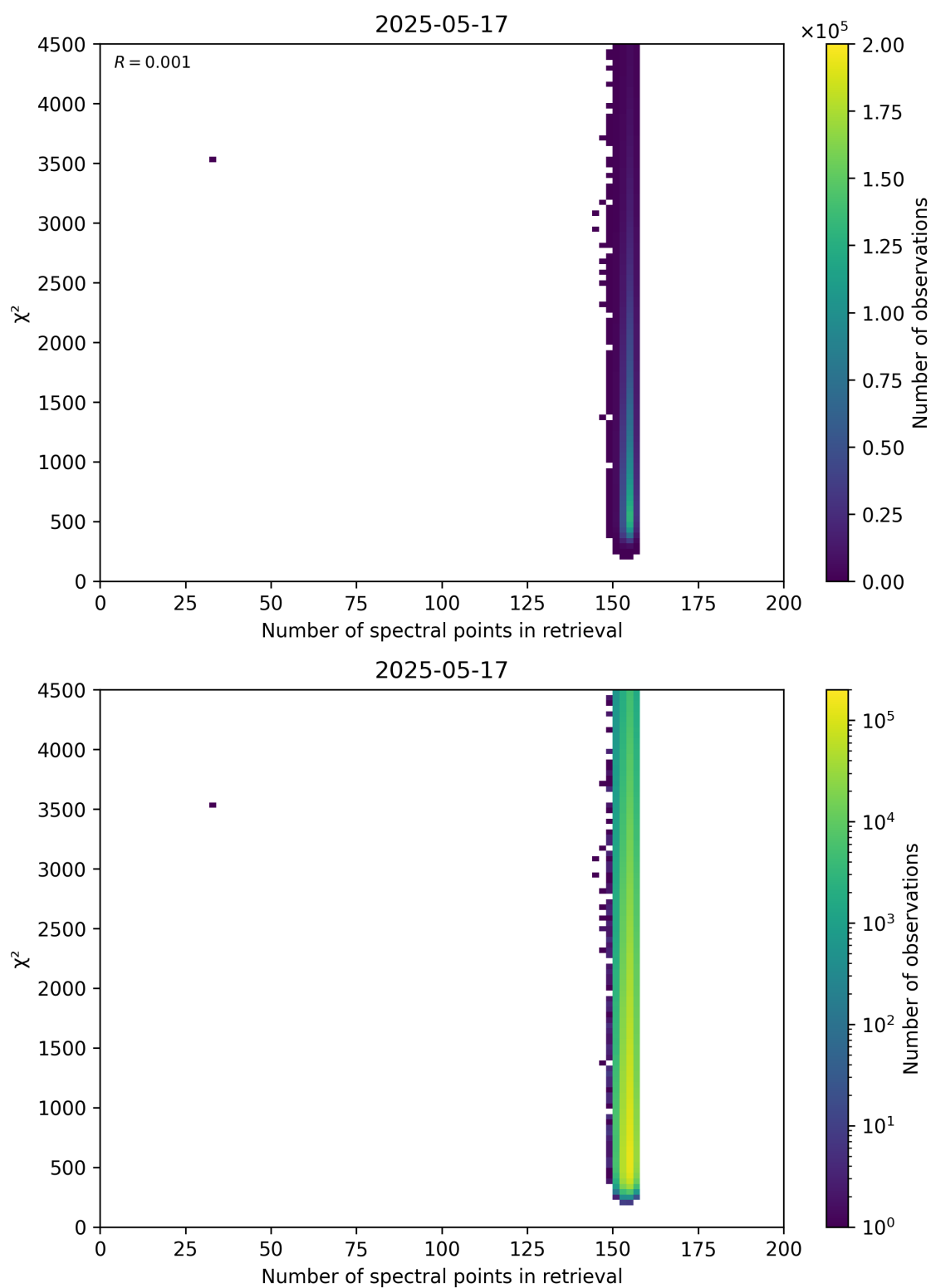
Figure 58: Scatter density plot of “Number of spectral points in retrieval” against “ \chi^2 ” for 2025-05-16 to 2025-05-18.
