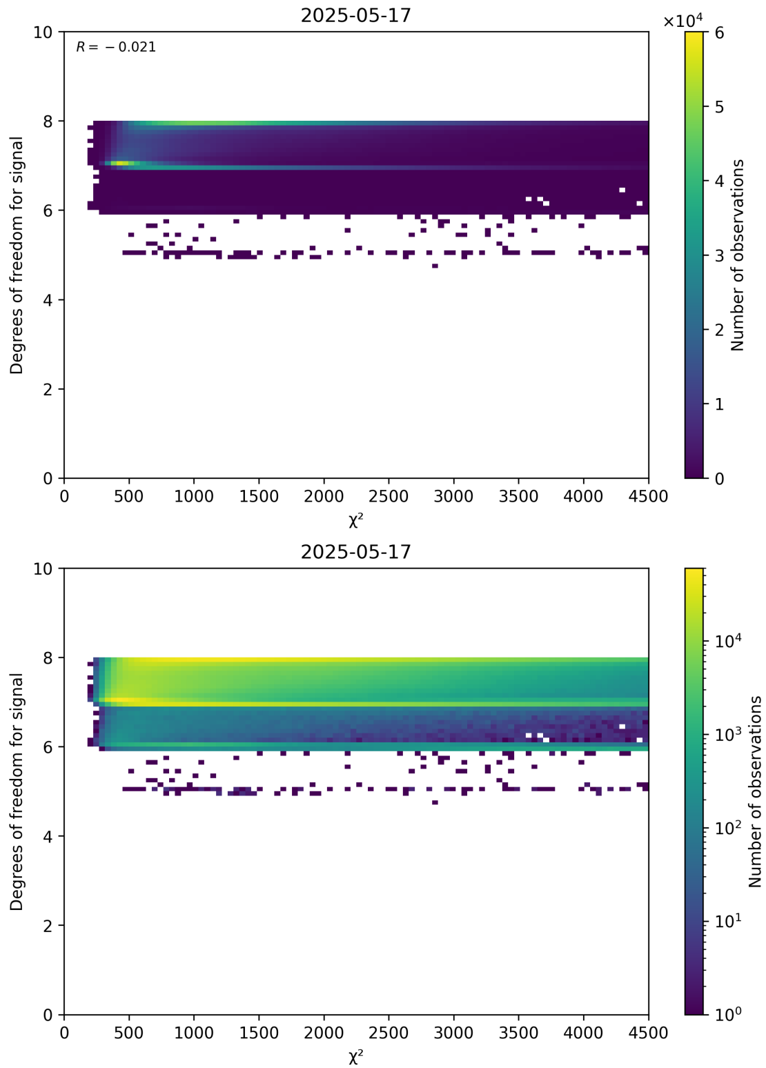
Figure 48: Scatter density plot of “ \chi^2 ” against “Degrees of freedom for signal” for 2025-05-16 to 2025-05-18.
