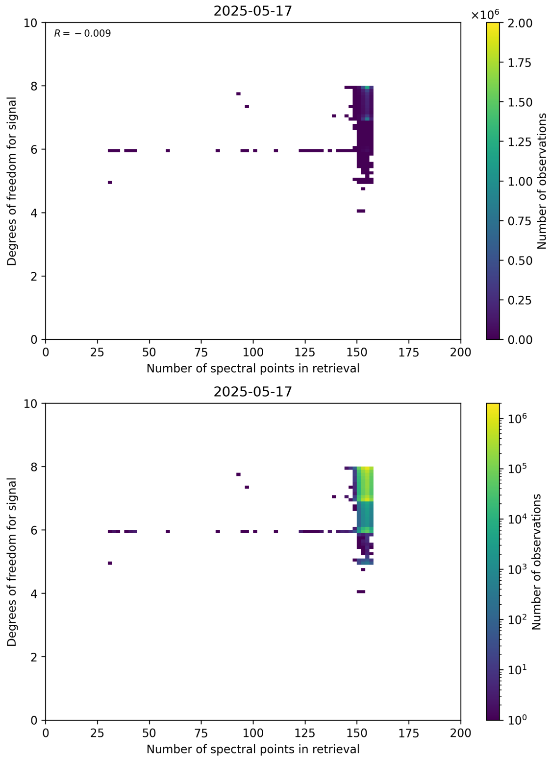
Figure 59: Scatter density plot of “Number of spectral points in retrieval” against “Degrees of freedom for signal” for 2025-05-16 to 2025-05-18.
