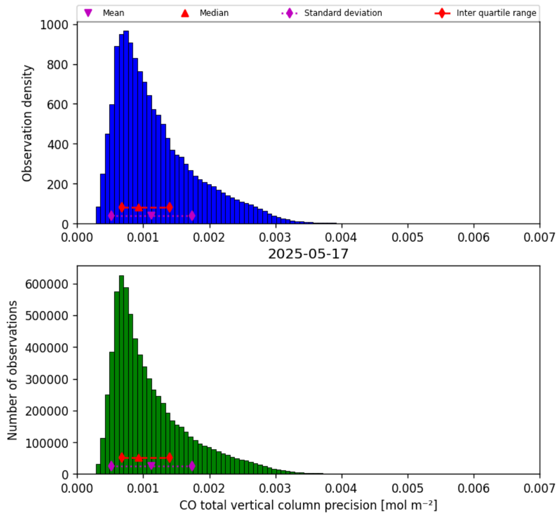
Figure 20: Histogram of “CO total vertical column precision” for 2025-05-16 to 2025-05-18
