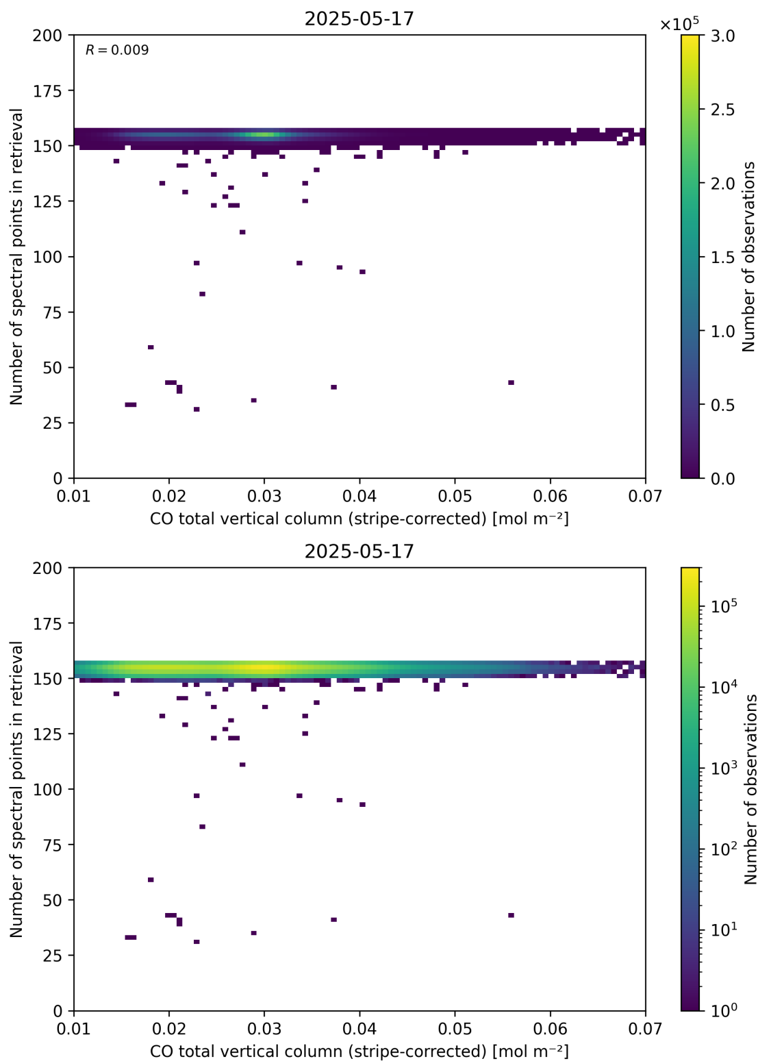
Figure 40: Scatter density plot of “CO total vertical column (stripe-corrected)” against “Number of spectral points in retrieval” for 2025-05-16 to 2025-05-18.
