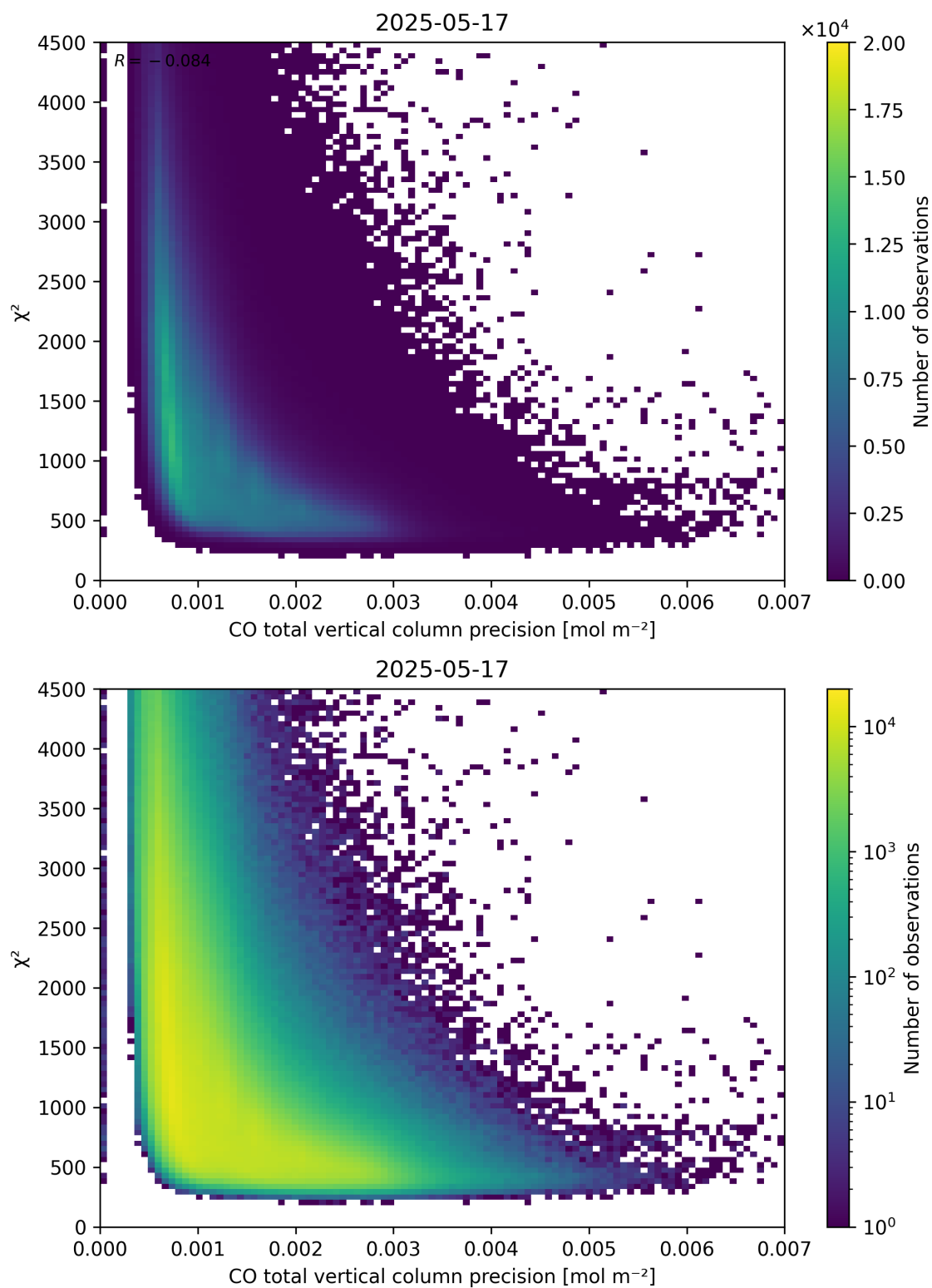
Figure 44: Scatter density plot of “CO total vertical column precision” against “ \chi^2 ” for 2025-05-16 to 2025-05-18.
