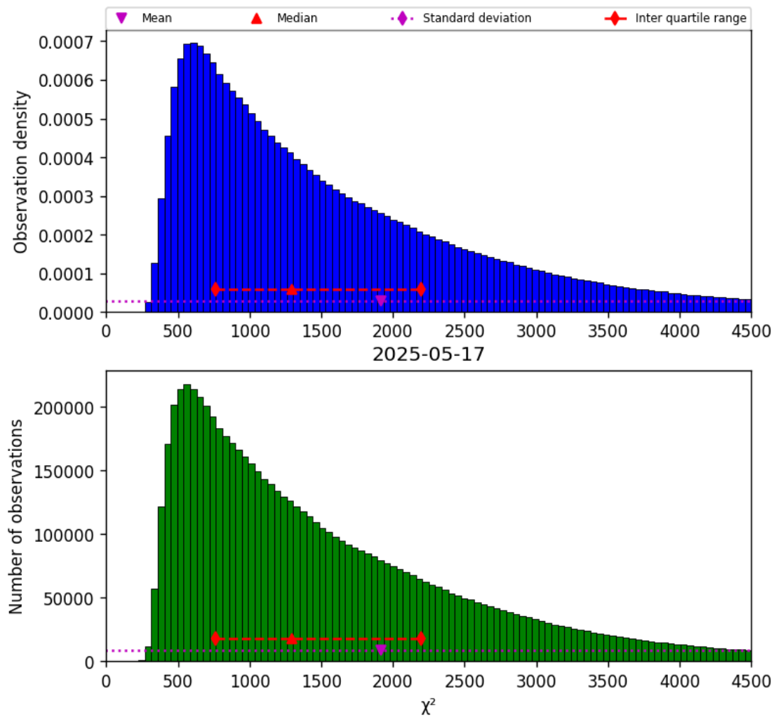
Figure 22: Histogram of “ \chi^2 ” for 2025-05-16 to 2025-05-18
