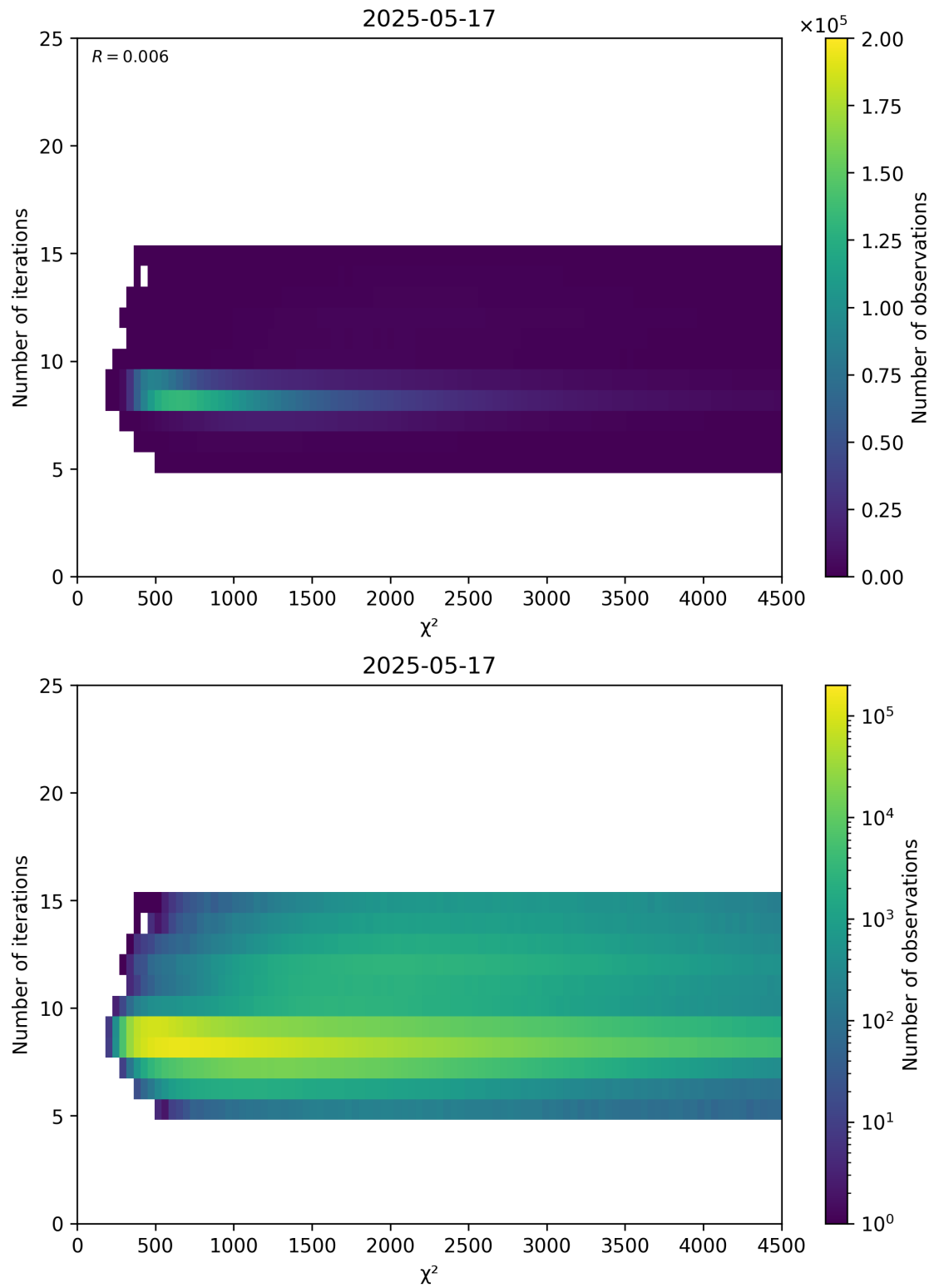
Figure 49: Scatter density plot of " \chi^2 " against "Number of iterations" for 2025-05-16 to 2025-05-18.
